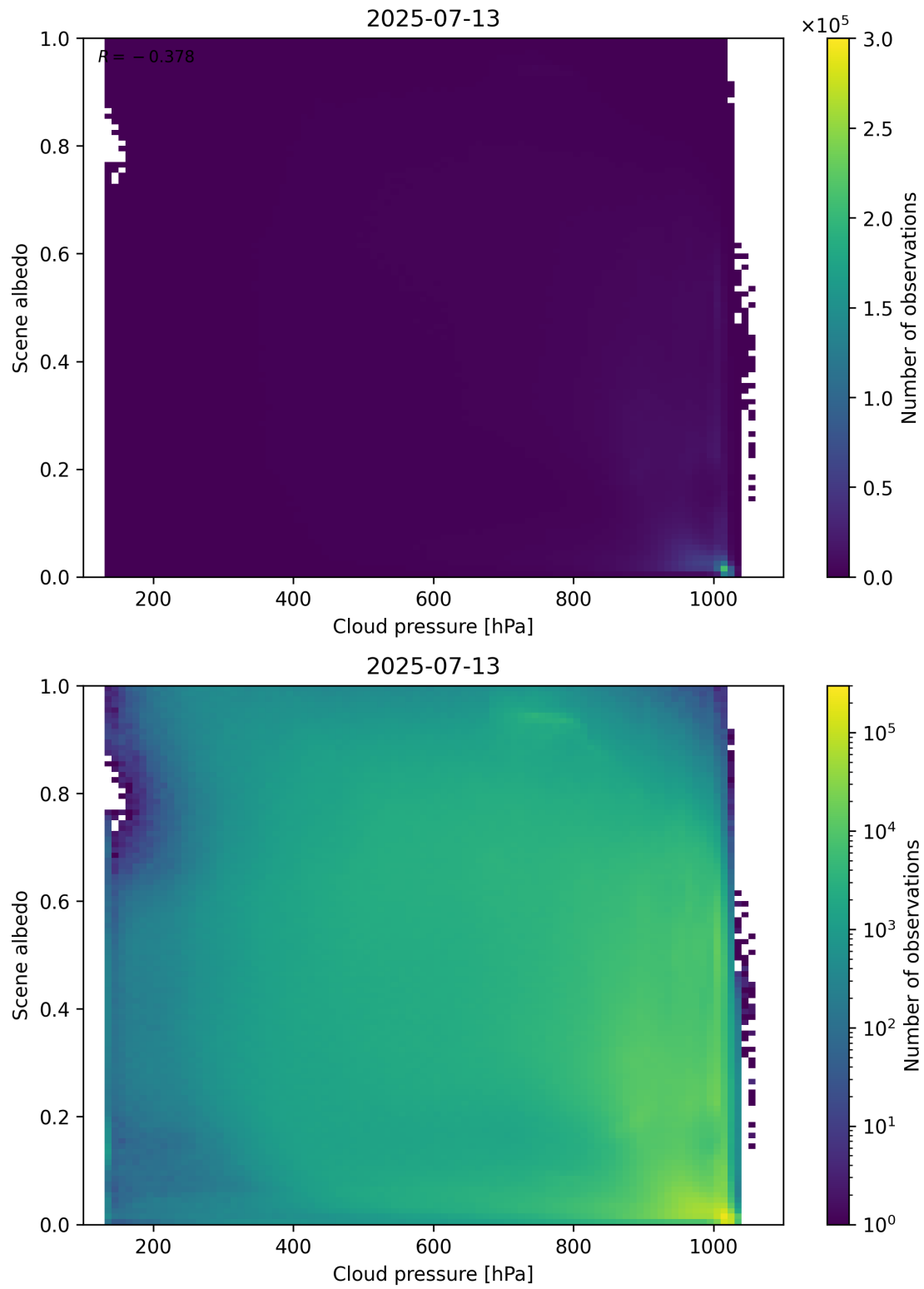
Figure 83: Scatter density plot of “Cloud pressure” against “Scene albedo” for 2025-07-13 to 2025-07-14.
