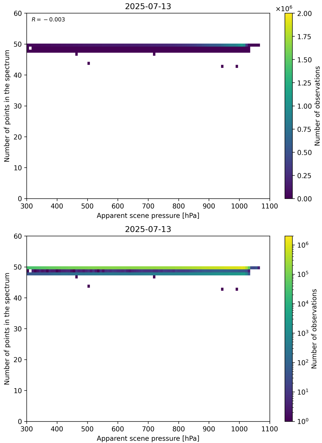
Figure 66: Scatter density plot of “Apparent scene pressure” against “Number of points in the spectrum” for 2025-07-13 to 2025-07-14.
