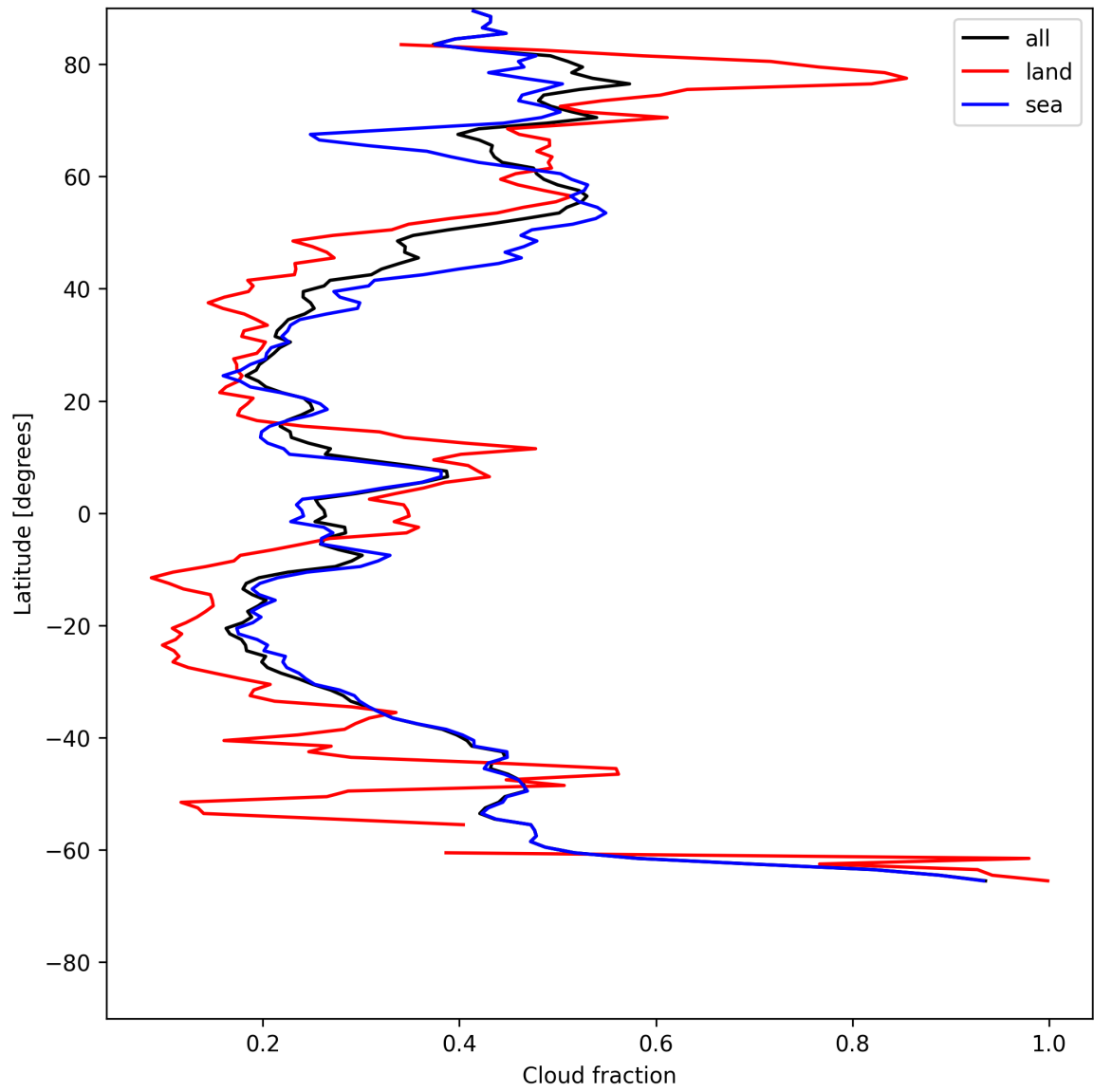
Figure 15: Zonal average of “Cloud fraction” for 2025-07-13 to 2025-07-14.
