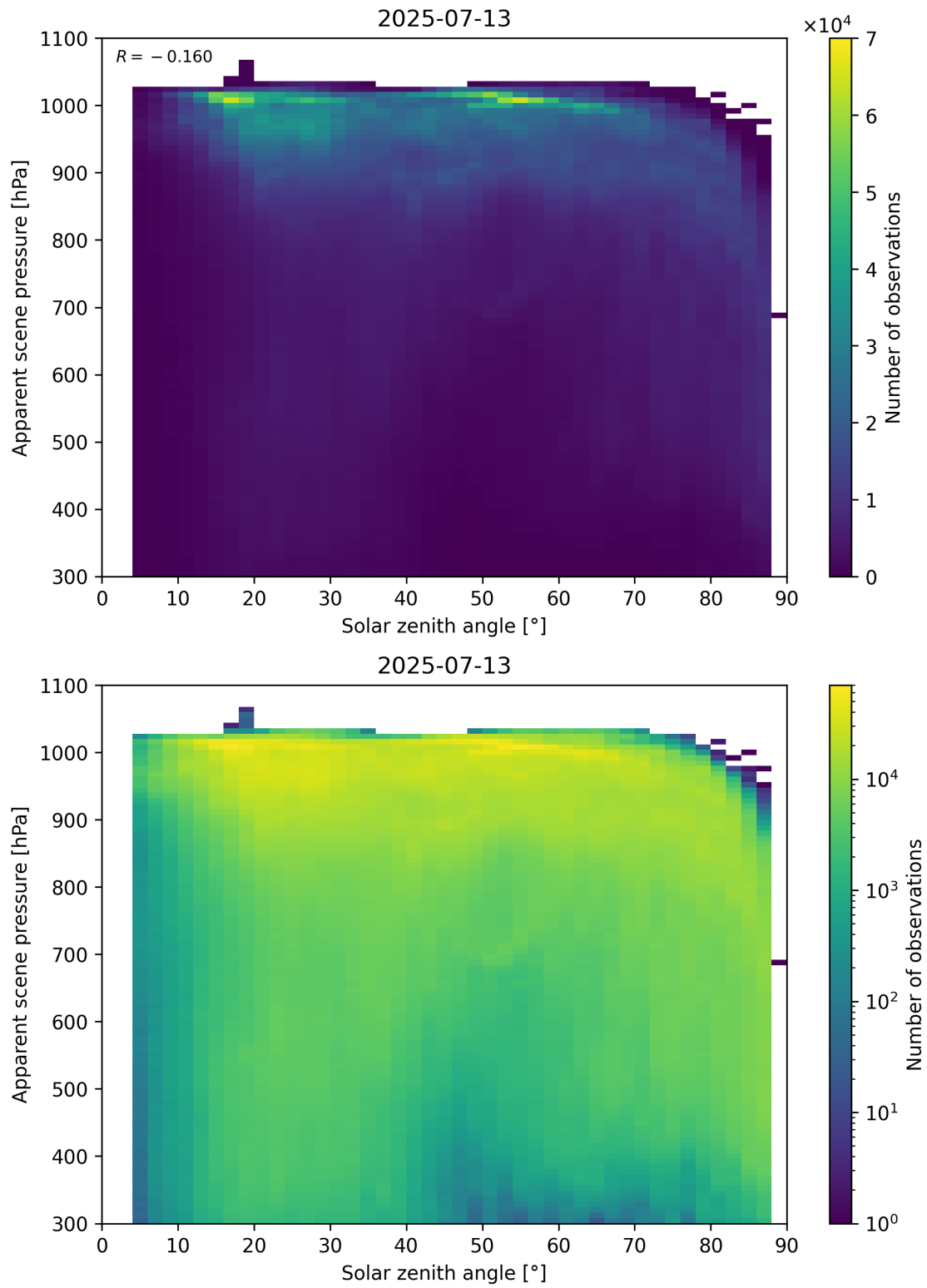
Figure 108: Scatter density plot of “Solar zenith angle” against “Apparent scene pressure” for 2025-07-13 to 2025-07-14.
