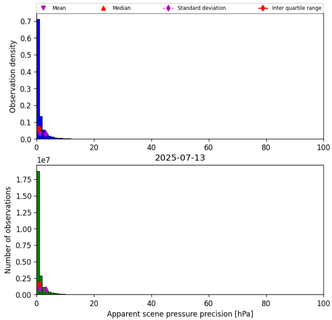
Figure 37: Histogram of “Apparent scene pressure precision” for 2025-07-13 to 2025-07-14
