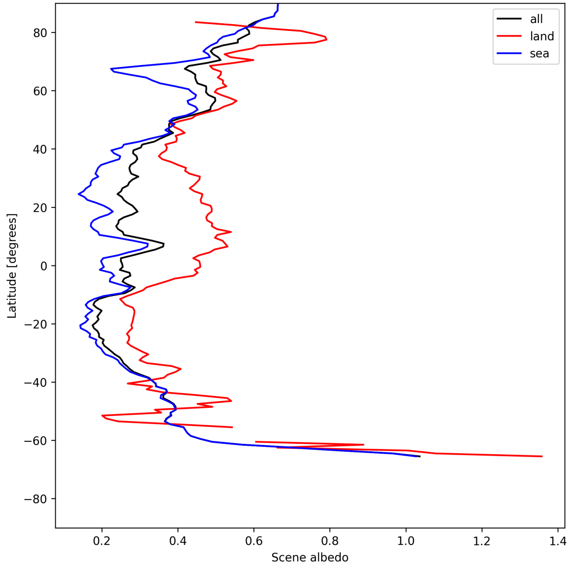
Figure 17: Zonal average of “Scene albedo” for 2025-07-13 to 2025-07-14.
