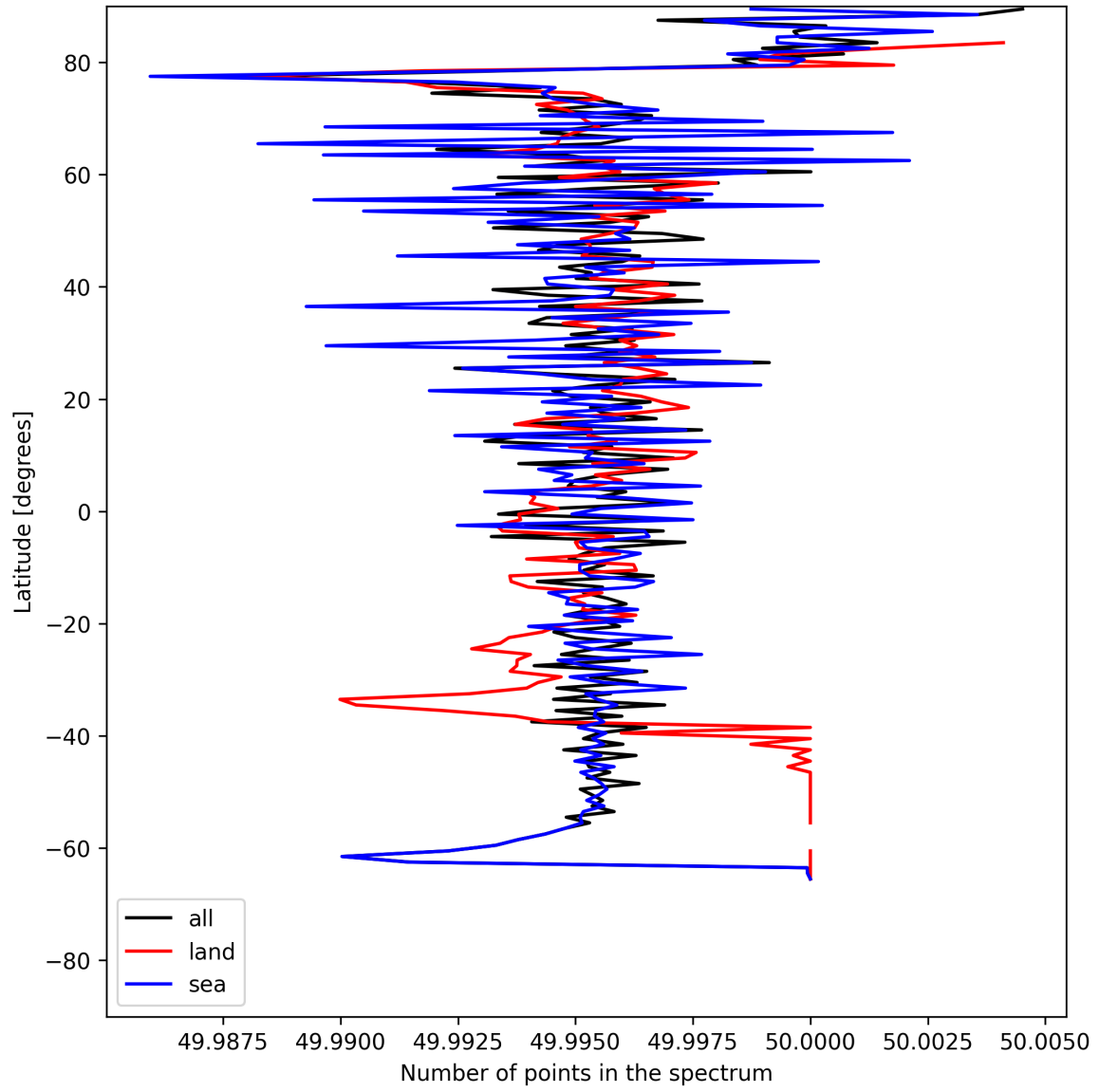
Figure 27: Zonal average of “Number of points in the spectrum” for 2025-07-13 to 2025-07-14.
