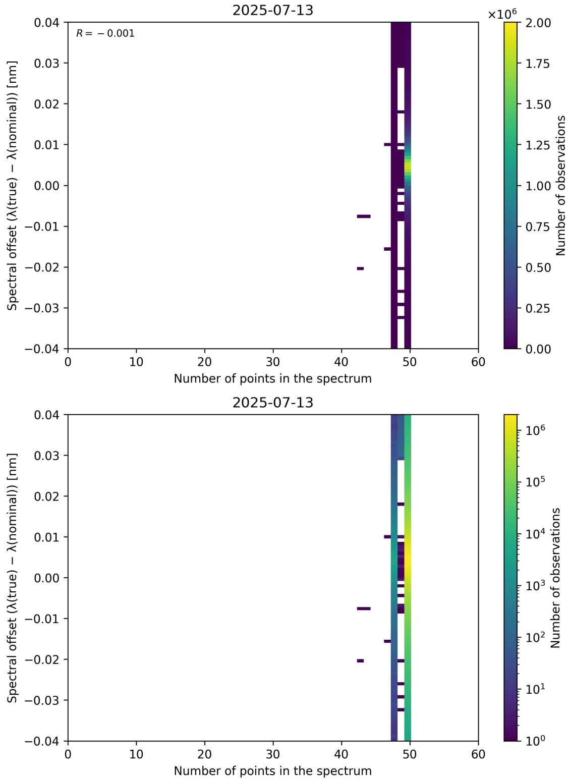
Figure 101: Scatter density plot of “Number of points in the spectrum” against “Spectral offset ( \lambda_{\text{true}} - \lambda_{\text{nominal}} )” for 2025-07-13 to 2025-07-14.
