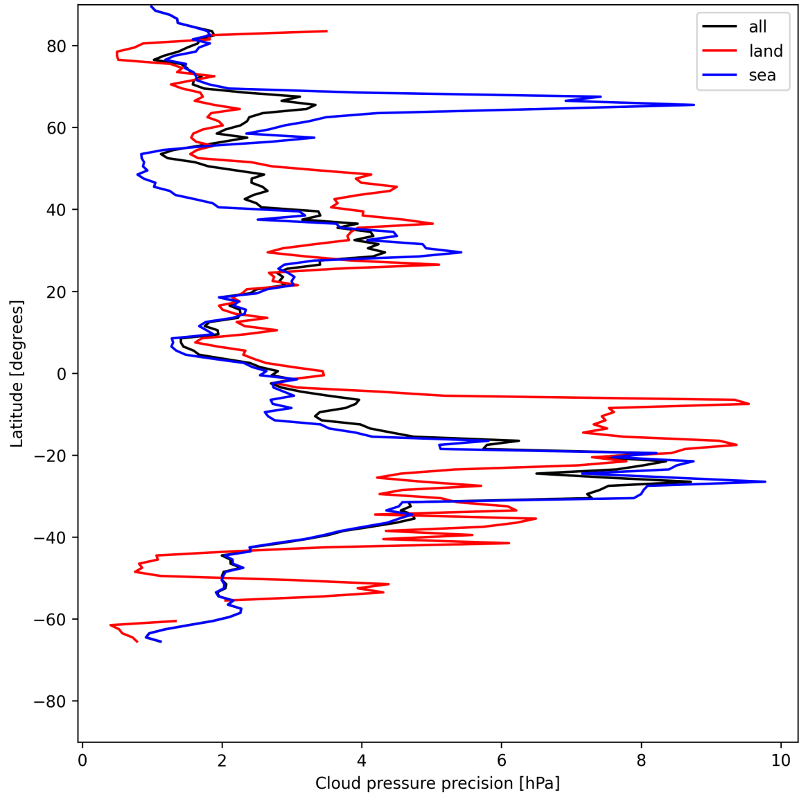
Figure 14: Zonal average of "Cloud pressure precision" for 2025-07-13 to 2025-07-14.
