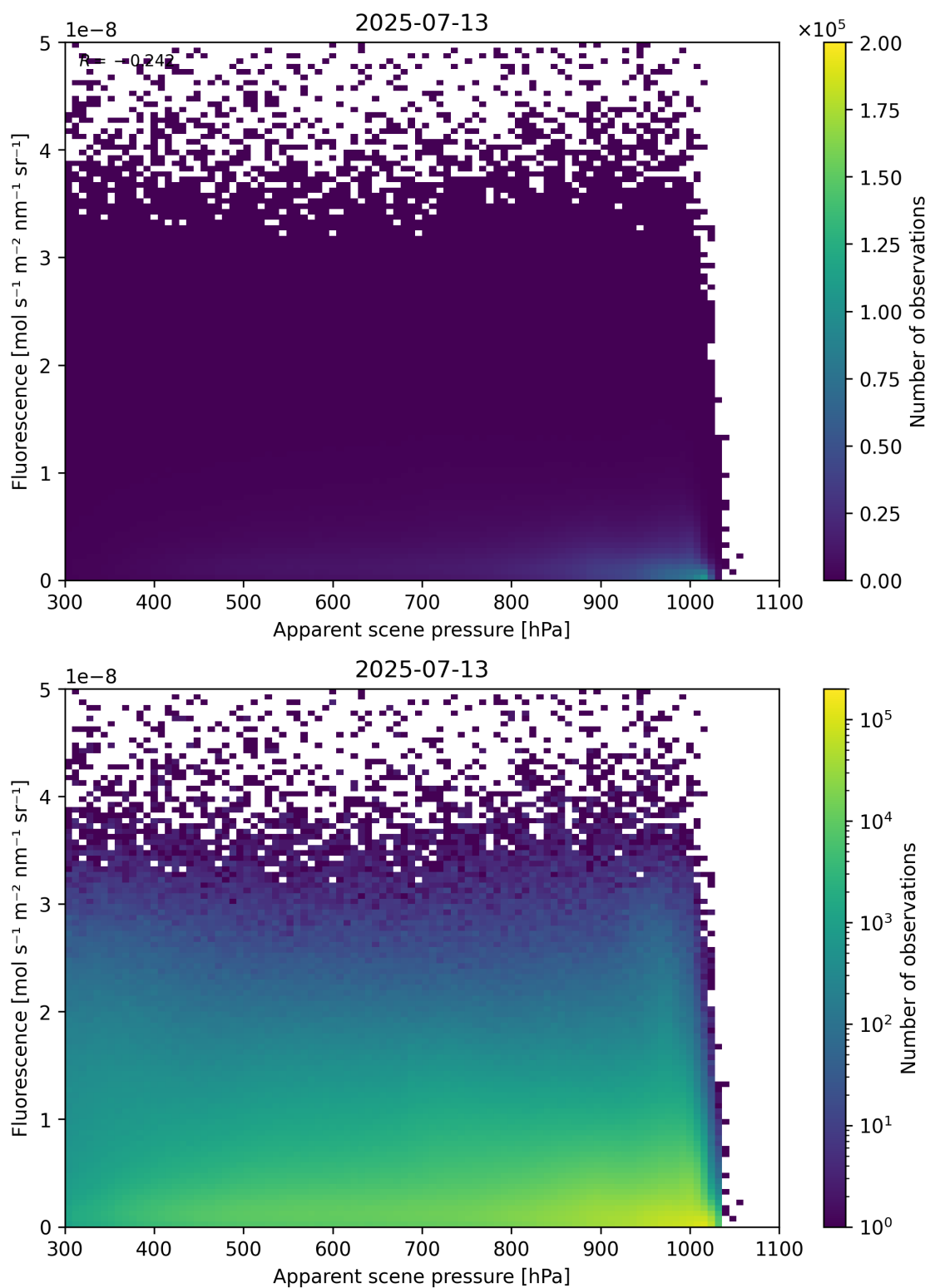
Figure 64: Scatter density plot of “Apparent scene pressure” against “Fluorescence” for 2025-07-13 to 2025-07-14.
