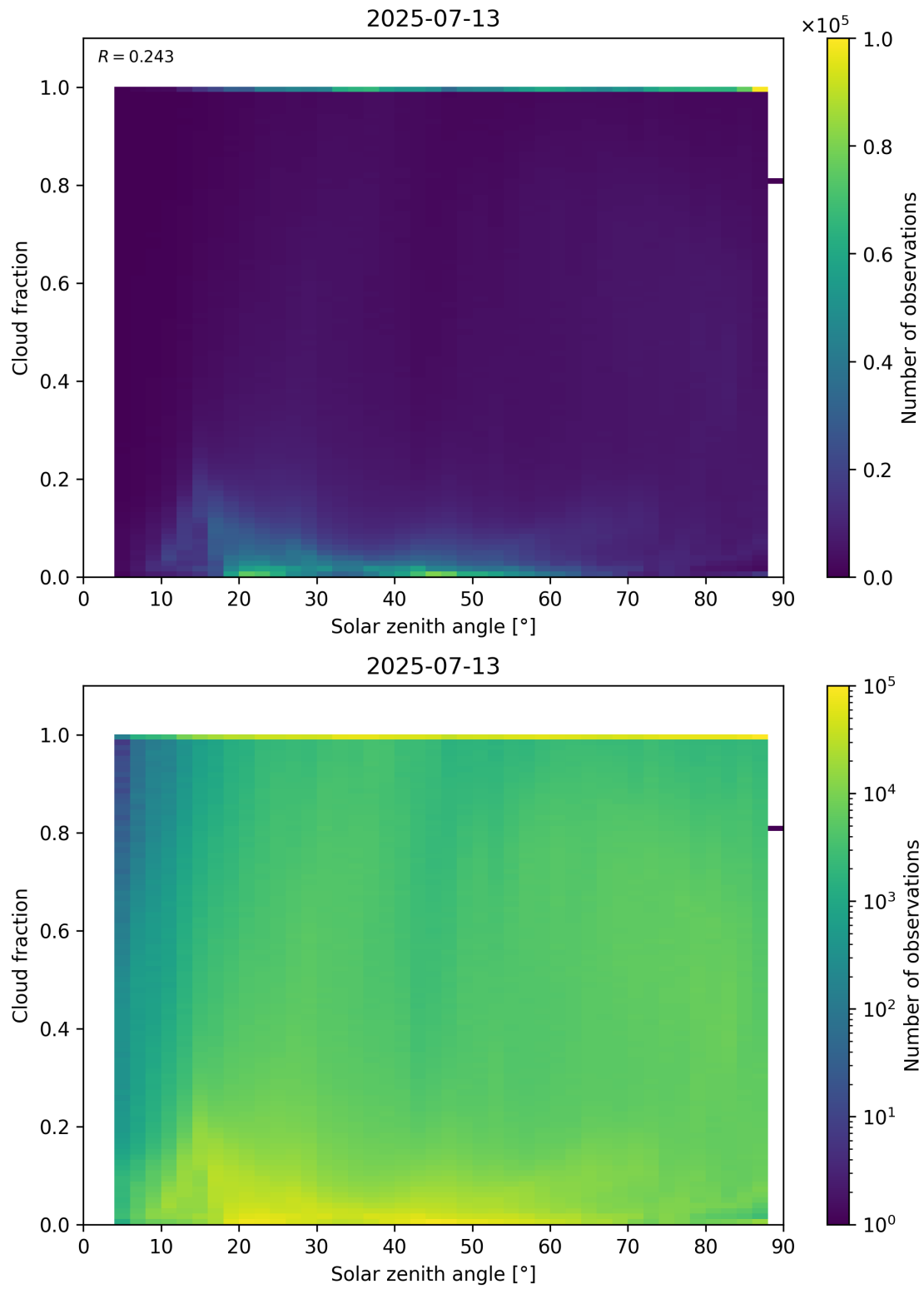
Figure 110: Scatter density plot of “Solar zenith angle” against “Cloud fraction” for 2025-07-13 to 2025-07-14.
