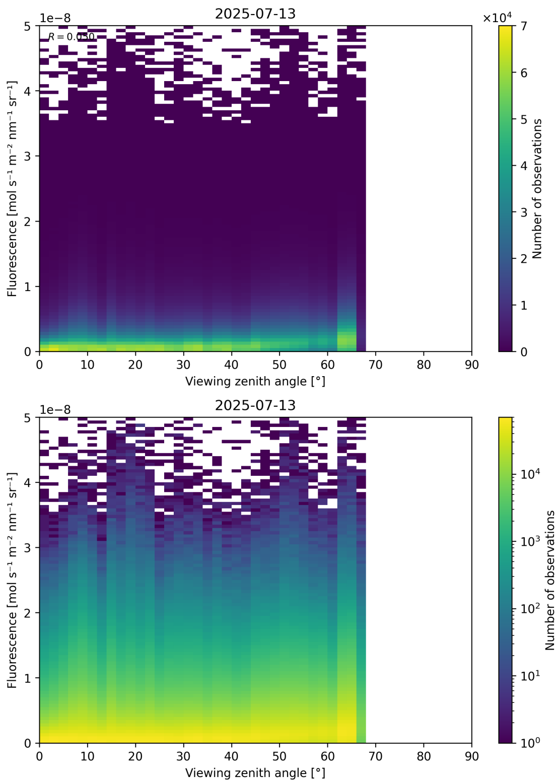
Figure 122: Scatter density plot of “Viewing zenith angle” against “Fluorescence” for 2025-07-13 to 2025-07-14.
