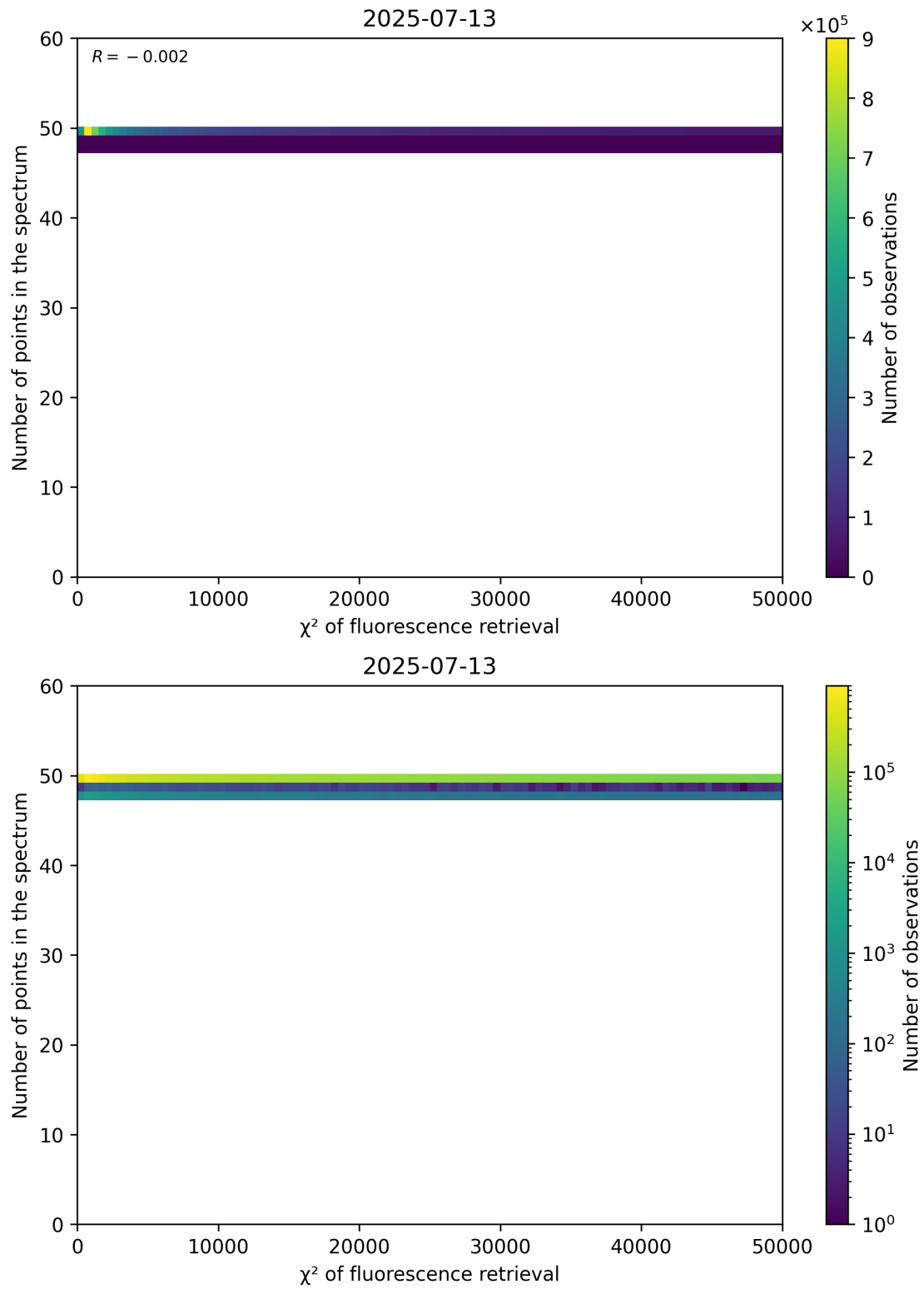
Figure 68: Scatter density plot of “ \chi^2 of fluorescence retrieval” against “Number of points in the spectrum” for 2025-07-13 to 2025-07-14.
