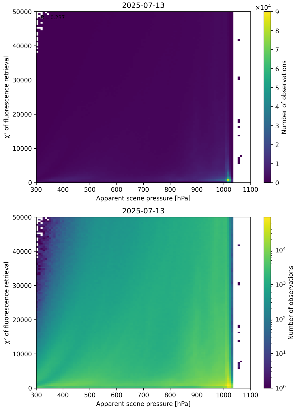
Figure 63: Scatter density plot of “Apparent scene pressure” against “ \chi^2 of fluorescence retrieval” for 2025-07-13 to 2025-07-14.
