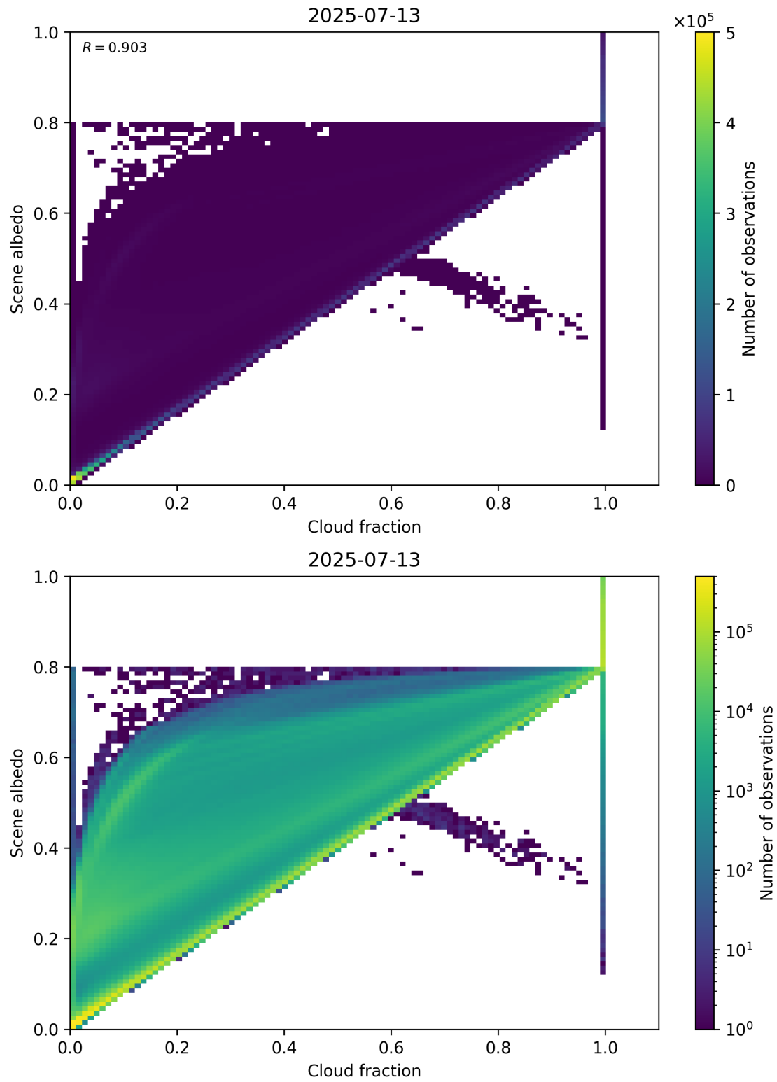
Figure 75: Scatter density plot of “Cloud fraction” against “Scene albedo” for 2025-07-13 to 2025-07-14.
