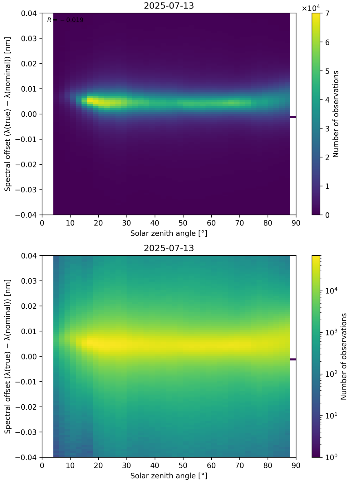
Figure 117: Scatter density plot of “Solar zenith angle” against “Spectral offset ( \lambda_{\text{true}} - \lambda_{\text{nominal}} )” for 2025-07-13 to 2025-07-14.
