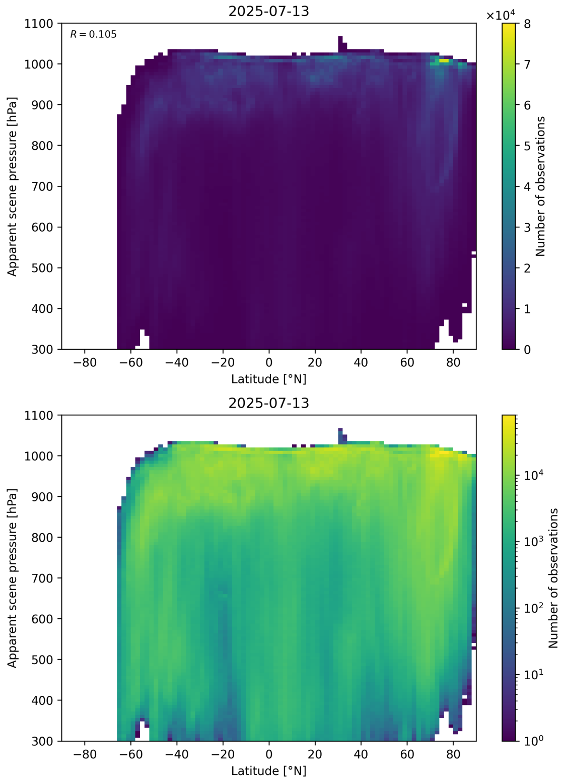
Figure 88: Scatter density plot of “Latitude” against “Apparent scene pressure” for 2025-07-13 to 2025-07-14.
