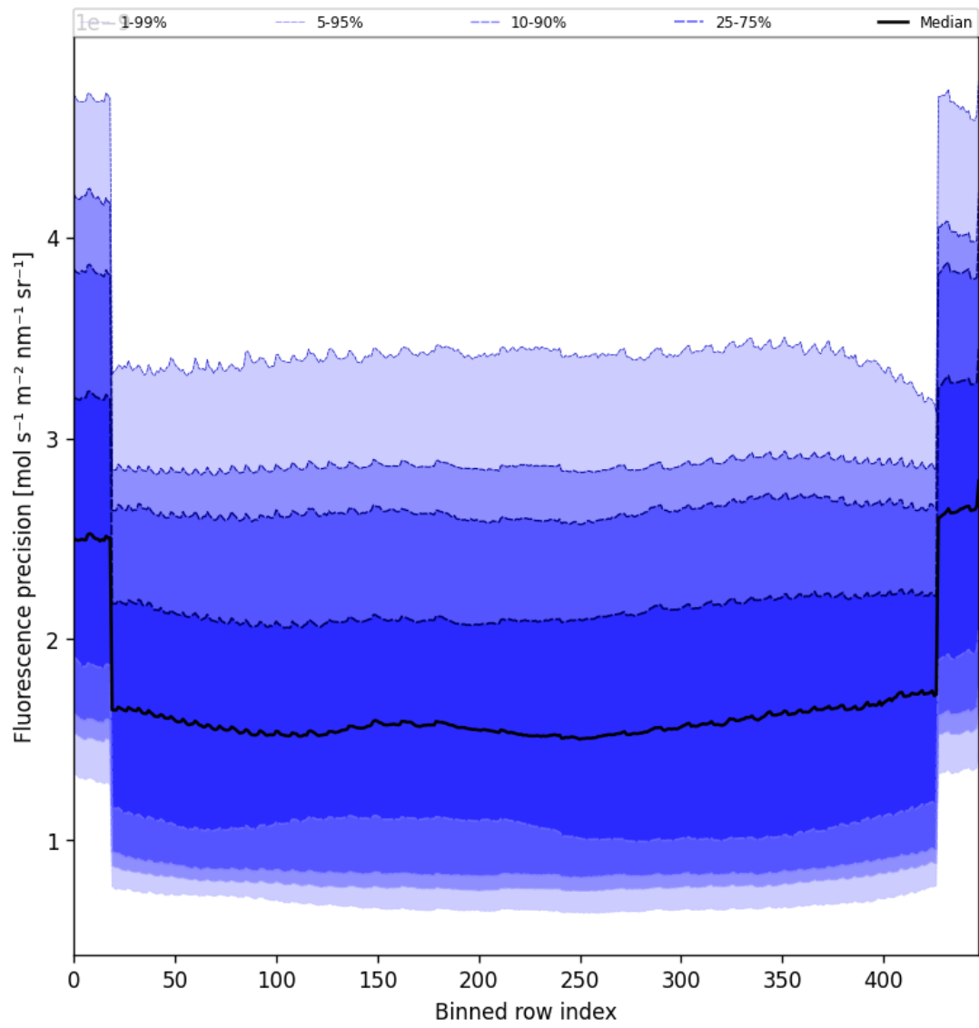
Figure 58: Along track statistics of “Fluorescence precision” for 2025-07-13 to 2025-07-14
