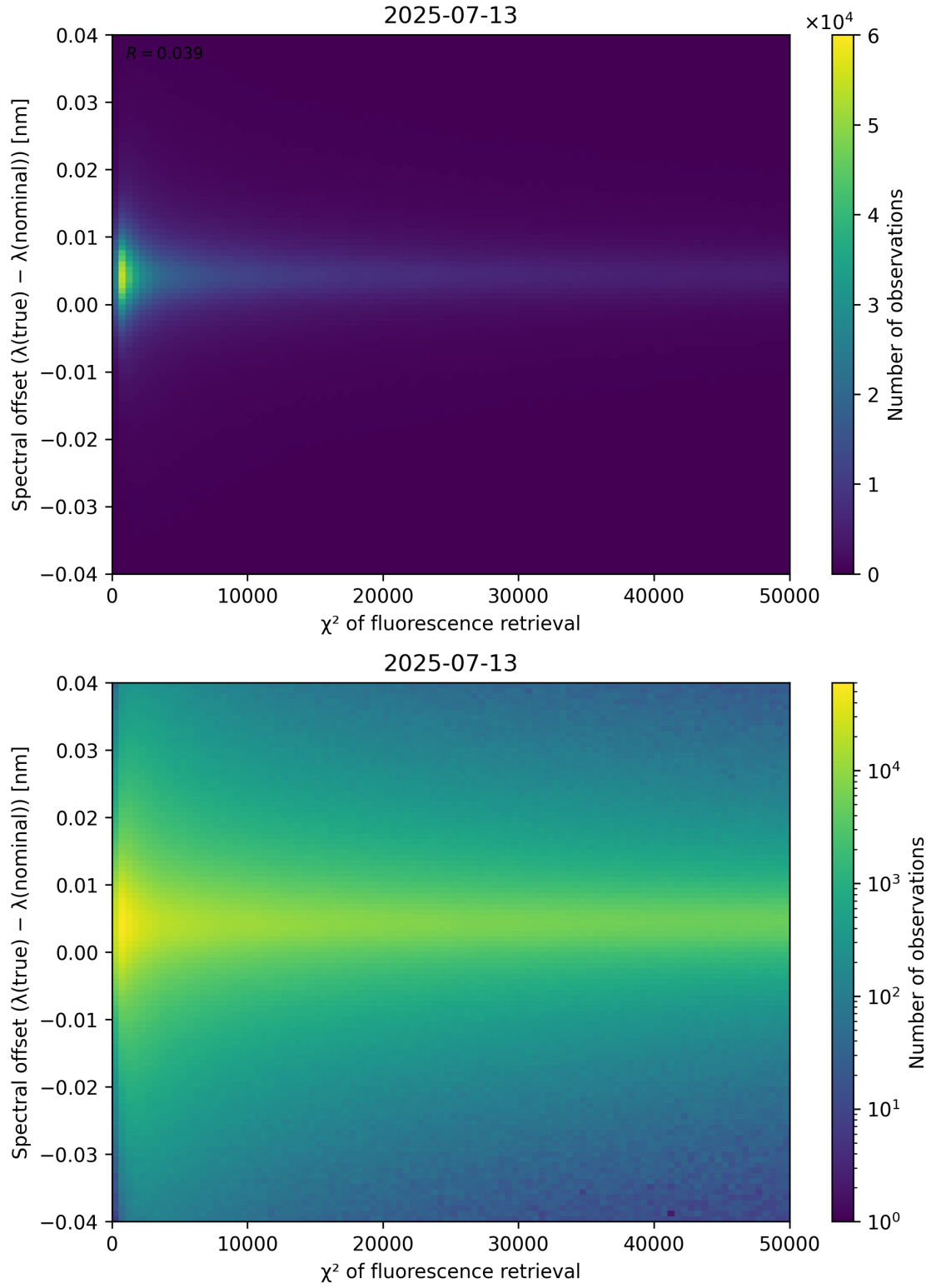
Figure 69: Scatter density plot of “ \chi^2 of fluorescence retrieval” against “Spectral offset ( \lambda_{\text{true}} - \lambda_{\text{nominal}} )” for 2025-07-13 to 2025-07-14.
