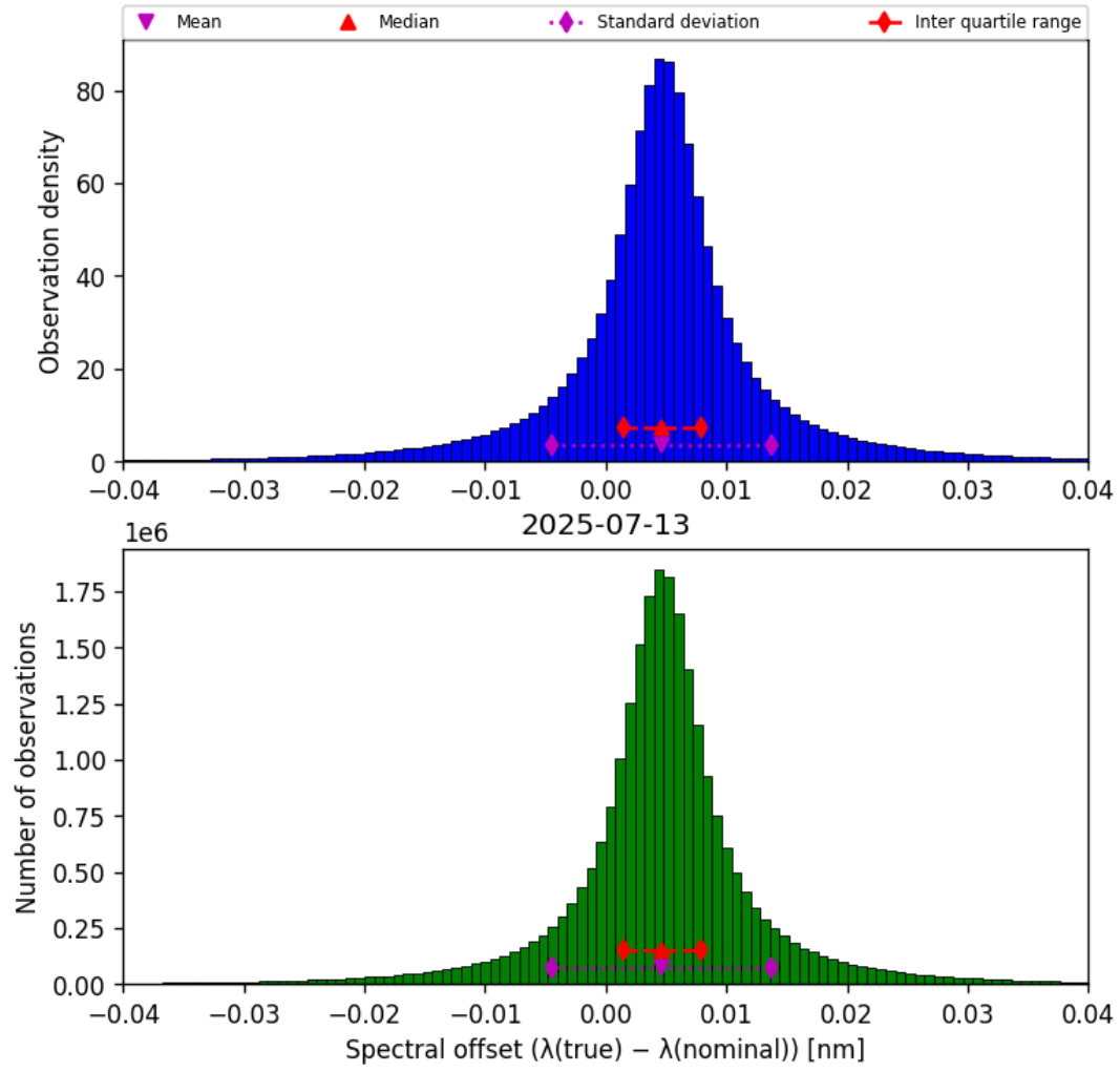
Figure 45: Histogram of “Spectral offset ( \lambda_{\text{true}} - \lambda_{\text{nominal}} )” for 2025-07-13 to 2025-07-14
