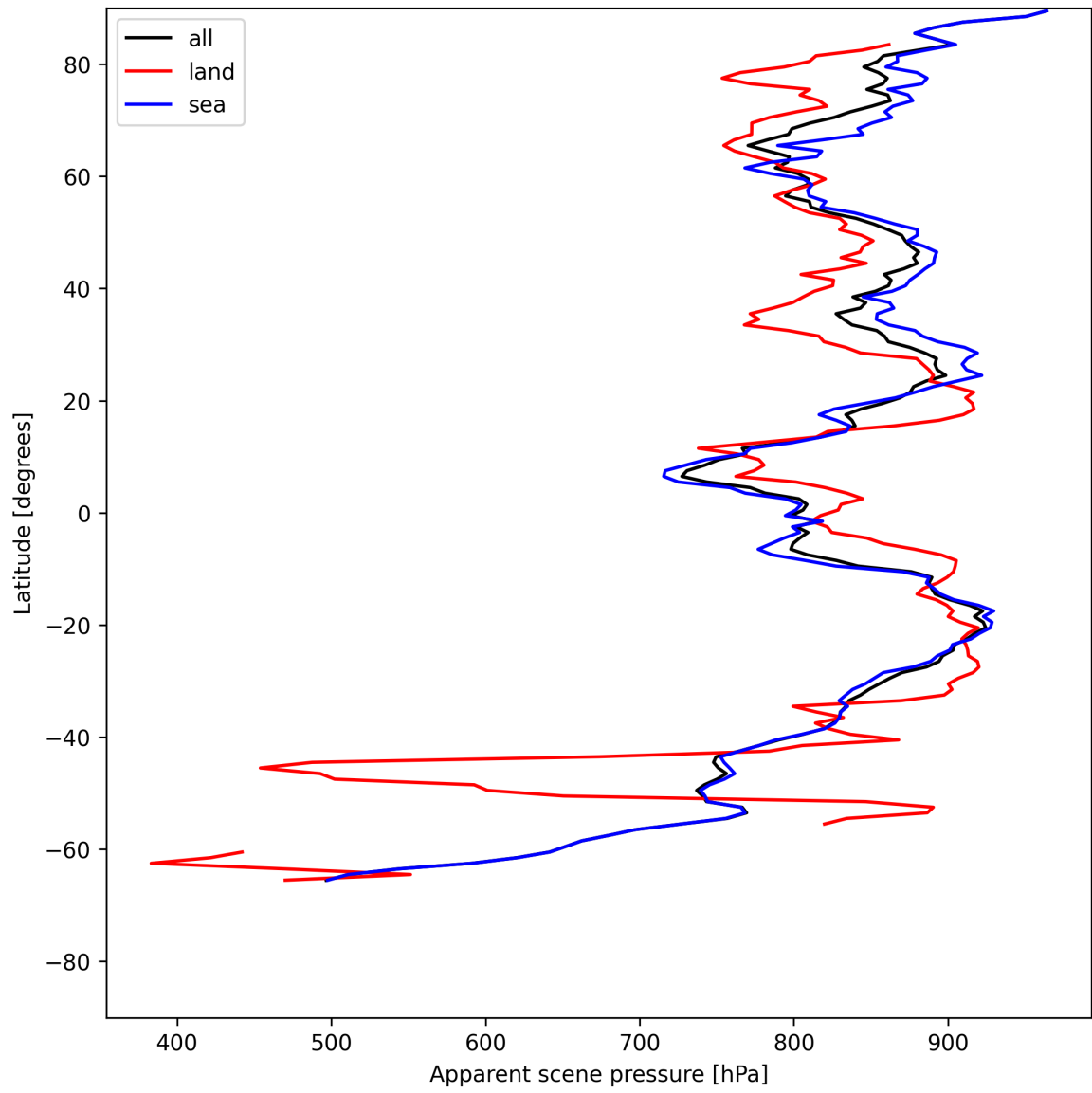
Figure 19: Zonal average of “Apparent scene pressure” for 2025-07-13 to 2025-07-14.
