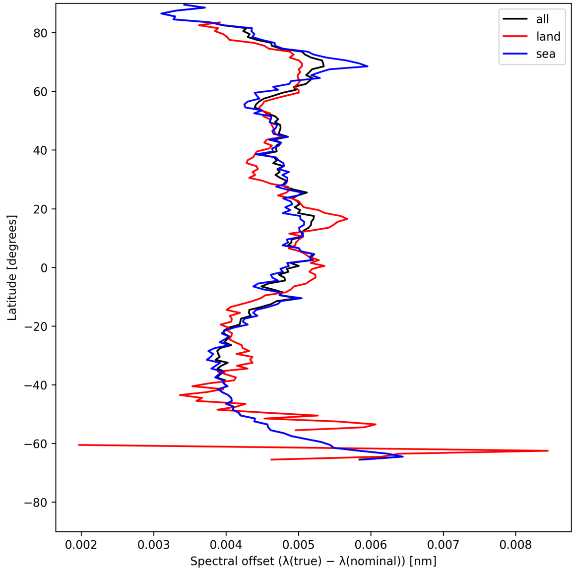
Figure 28: Zonal average of “Spectral offset ( \lambda_{\text{true}} - \lambda_{\text{nominal}} )” for 2025-07-13 to 2025-07-14.
