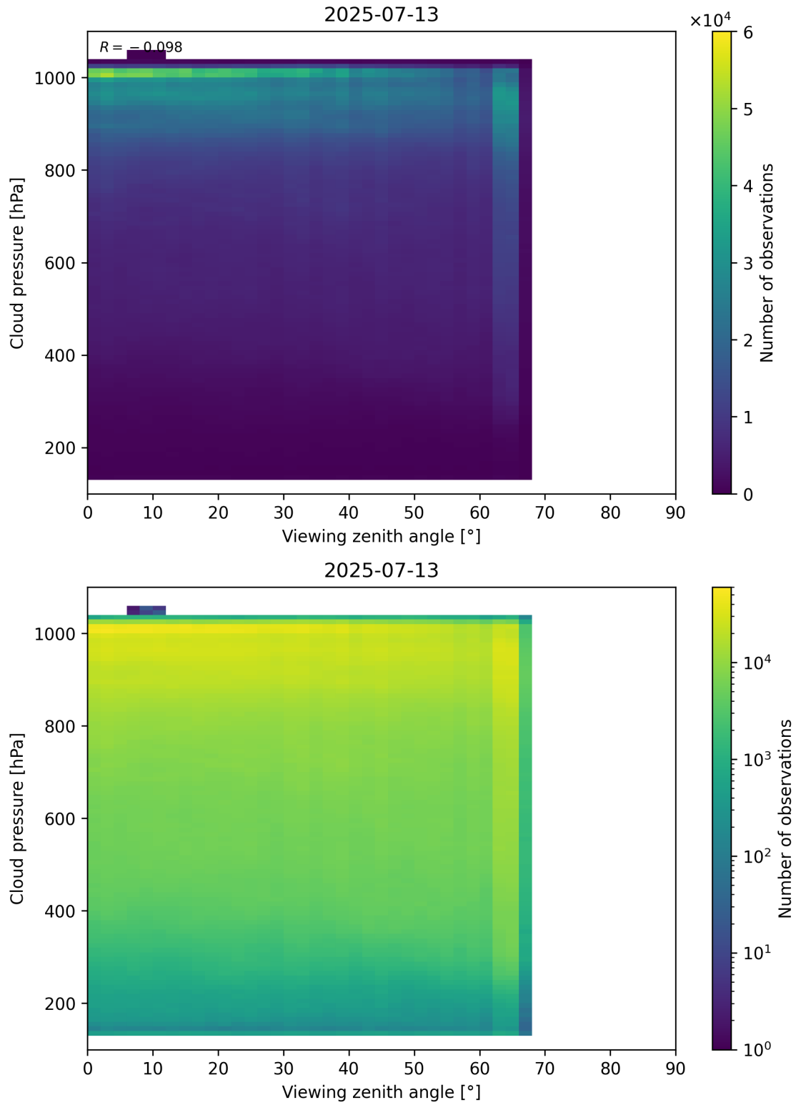
Figure 121: Scatter density plot of “Viewing zenith angle” against “Cloud pressure” for 2025-07-13 to 2025-07-14.
