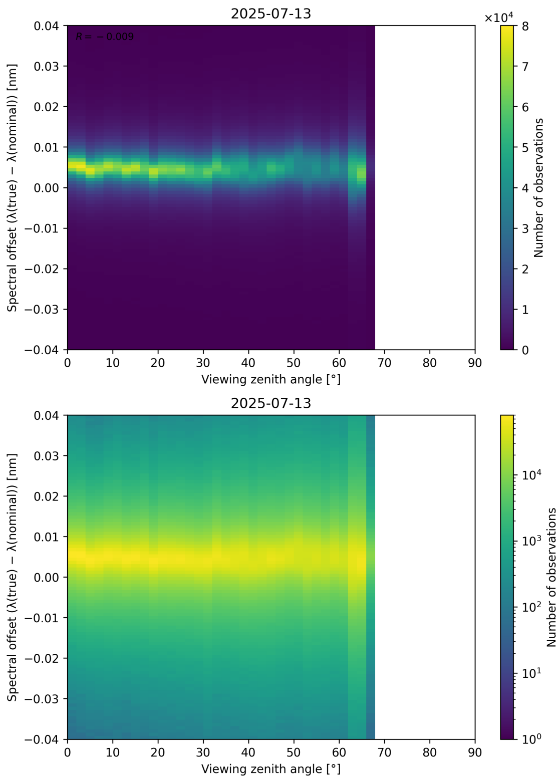
Figure 128: Scatter density plot of “Viewing zenith angle” against “Spectral offset ( \lambda_{\text{true}} - \lambda_{\text{nominal}} )” for 2025-07-13 to 2025-07-14.
