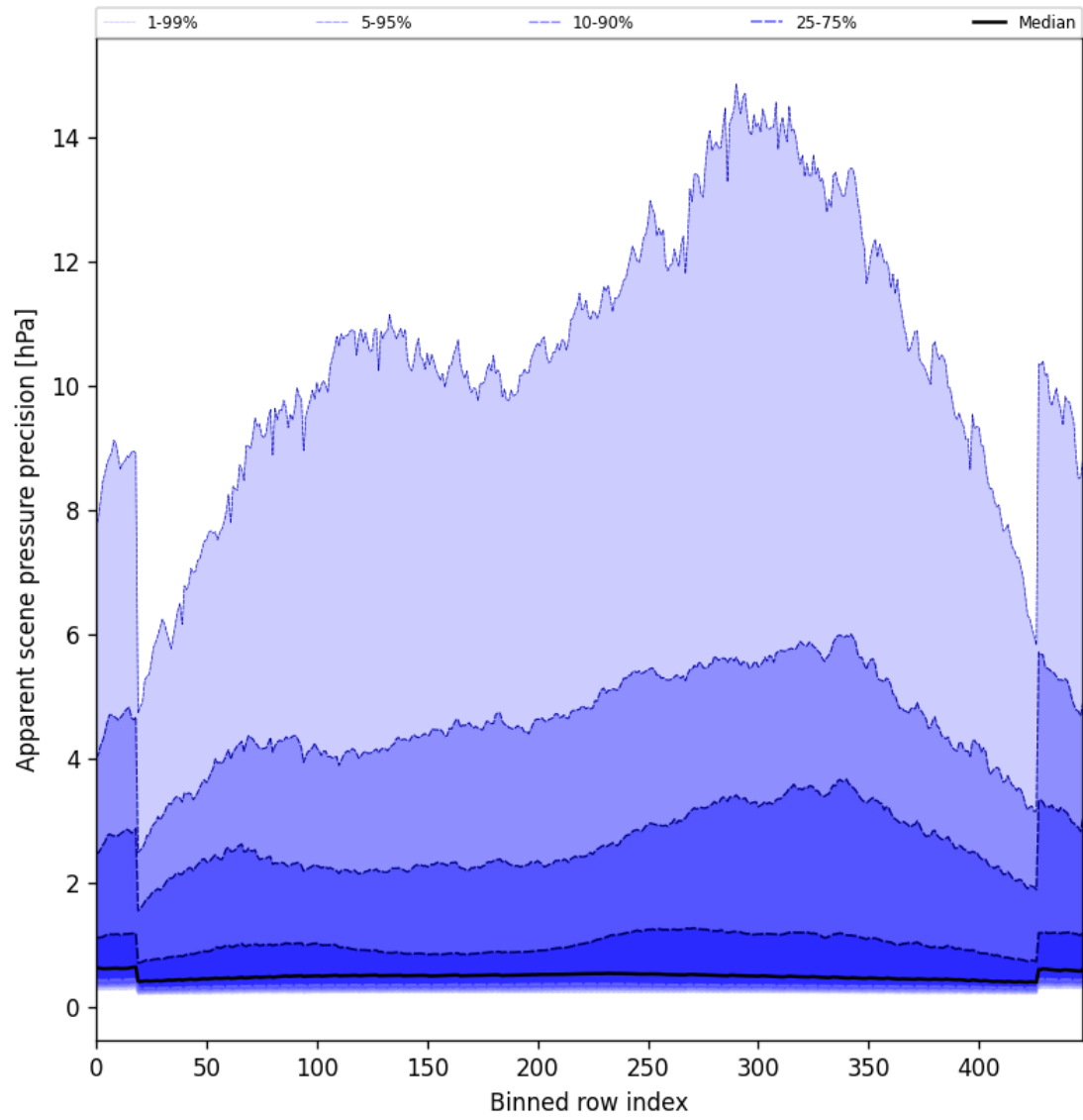
Figure 54: Along track statistics of “Apparent scene pressure precision” for 2025-07-13 to 2025-07-14
