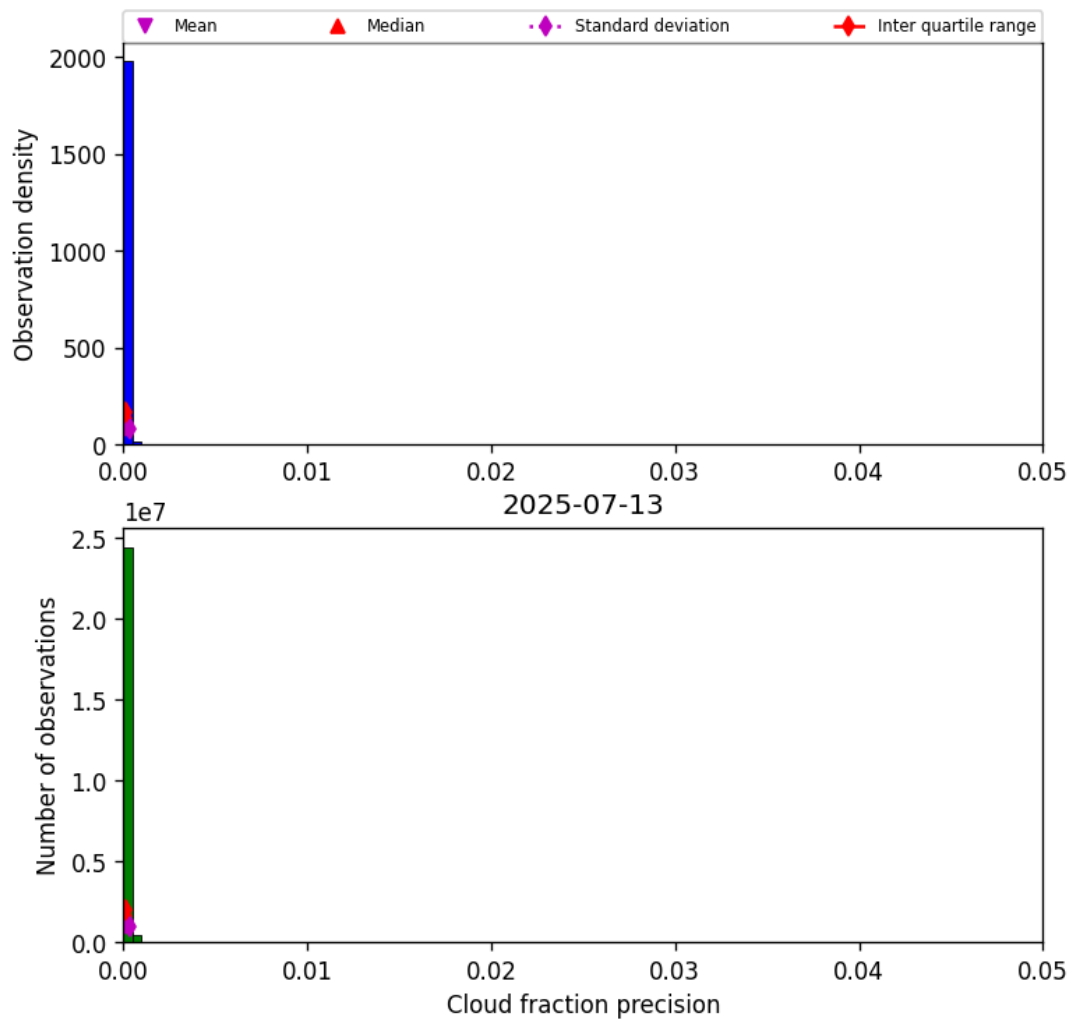
Figure 33: Histogram of “Cloud fraction precision” for 2025-07-13 to 2025-07-14
