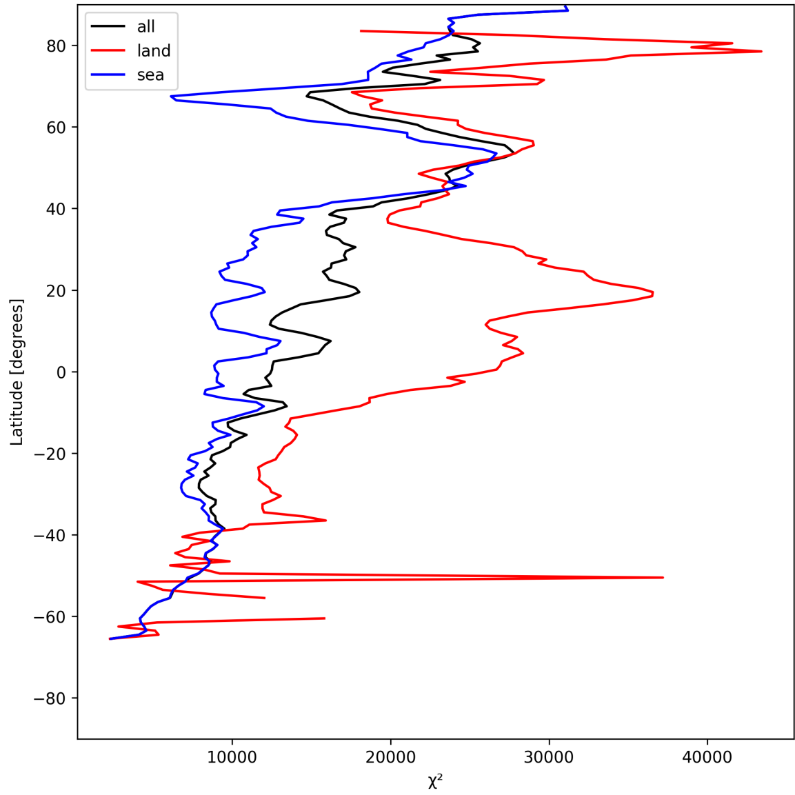
Figure 21: Zonal average of “ \chi^2 ” for 2025-07-13 to 2025-07-14.
