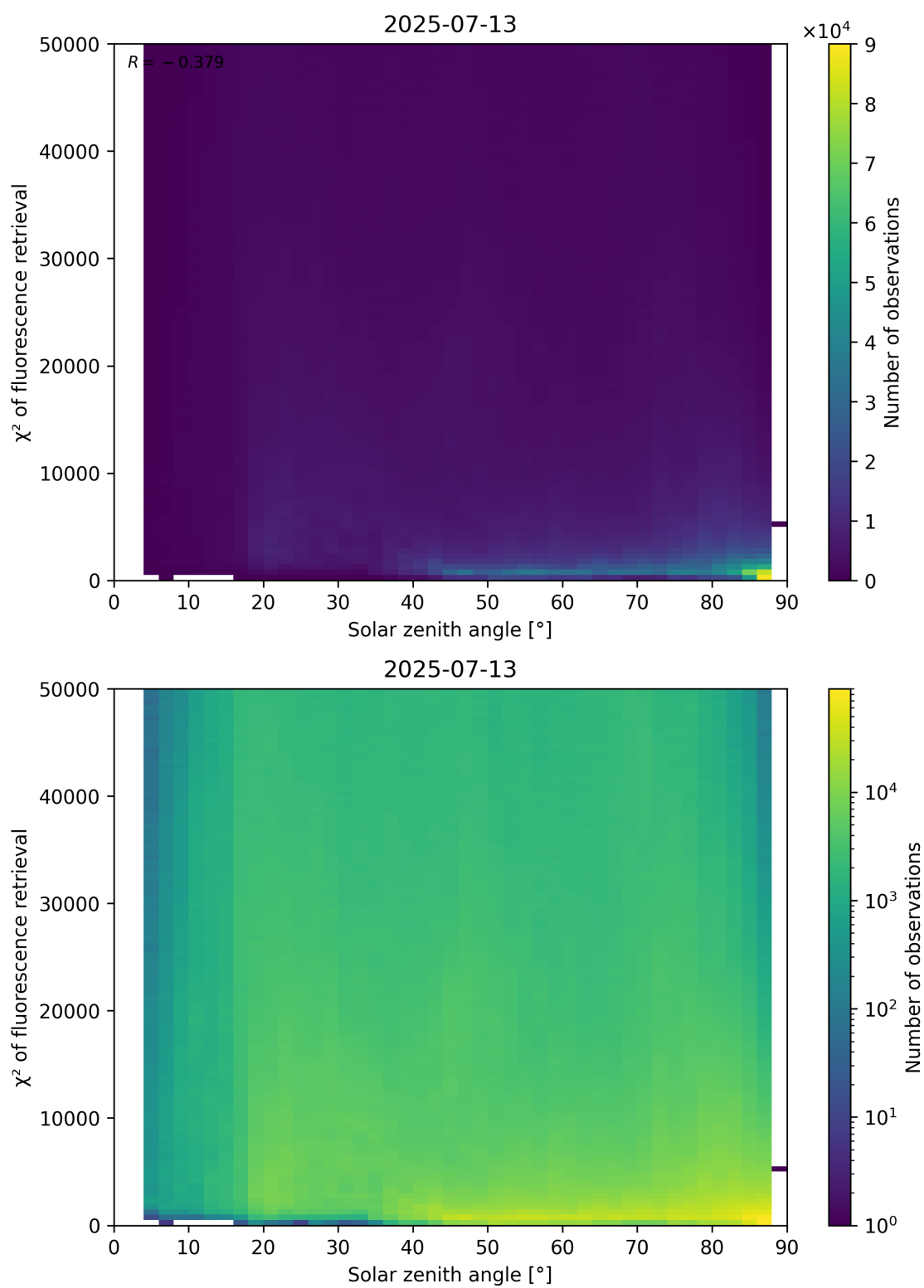
Figure 109: Scatter density plot of “Solar zenith angle” against “ \chi^2 of fluorescence retrieval” for 2025-07-13 to 2025-07-14.
