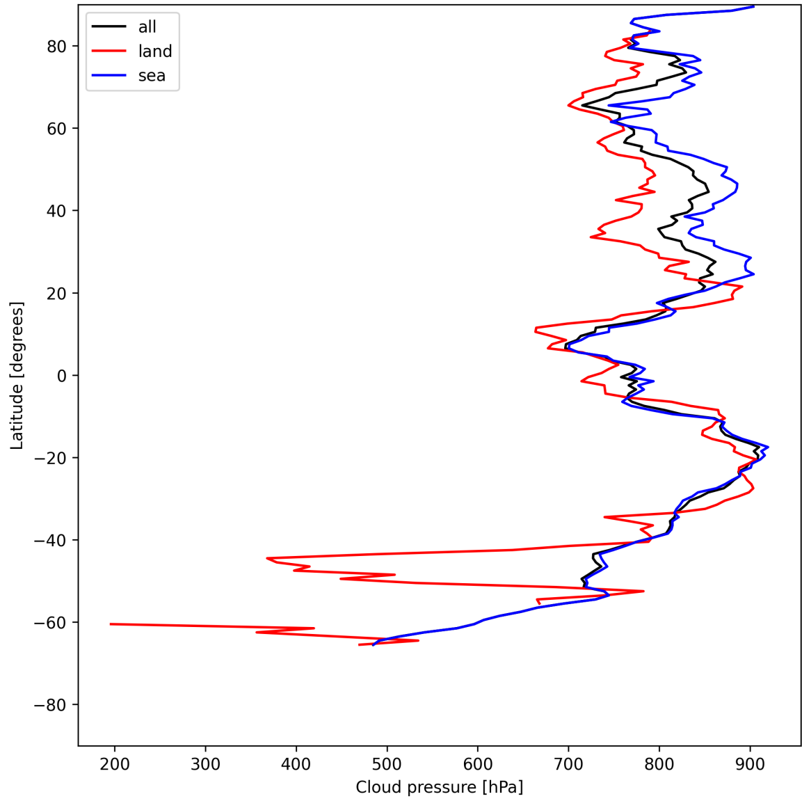
Figure 13: Zonal average of “Cloud pressure” for 2025-07-13 to 2025-07-14.
