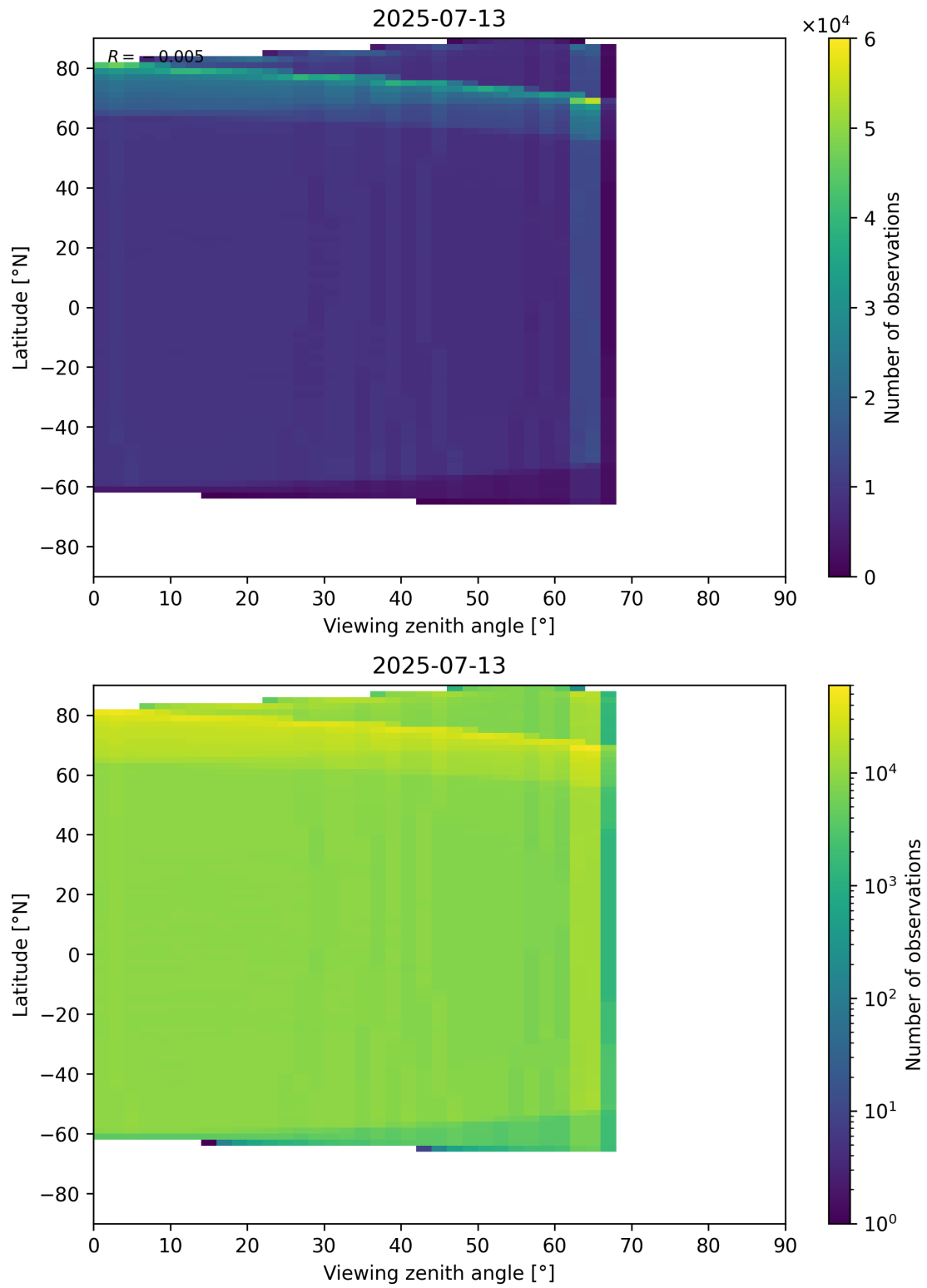
Figure 123: Scatter density plot of “Viewing zenith angle” against “Latitude” for 2025-07-13 to 2025-07-14.
