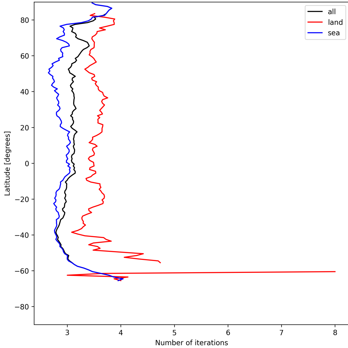
Figure 22: Zonal average of “Number of iterations” for 2025-07-13 to 2025-07-14.
