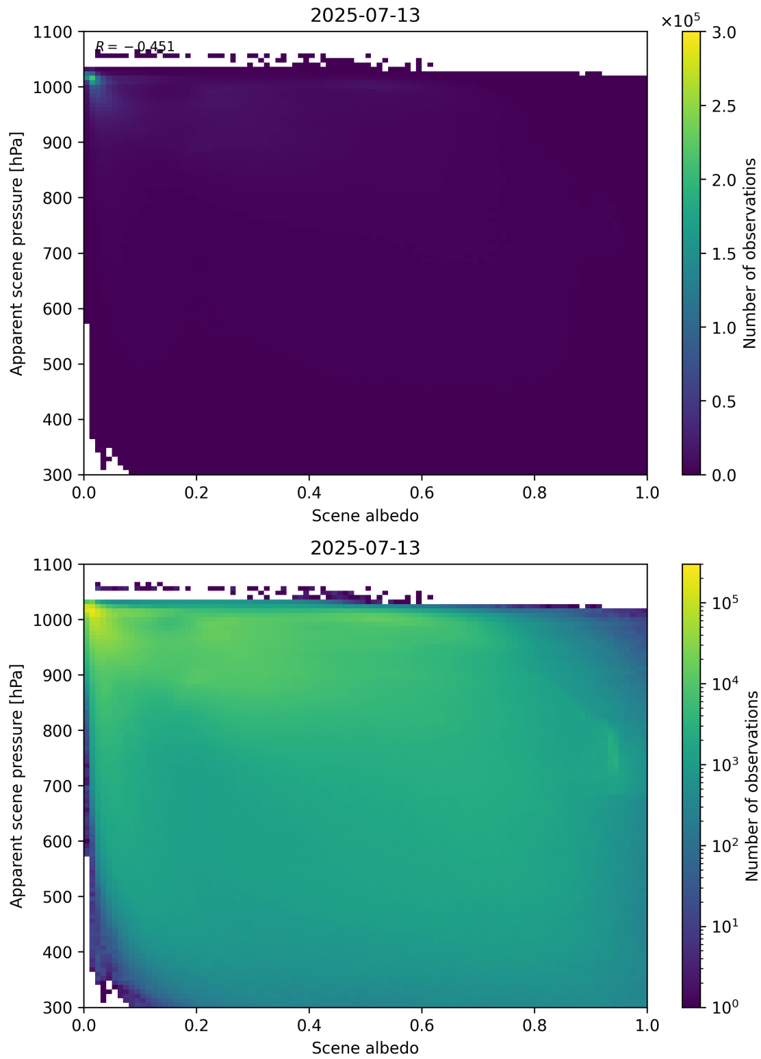
Figure 102: Scatter density plot of “Scene albedo” against “Apparent scene pressure” for 2025-07-13 to 2025-07-14.
