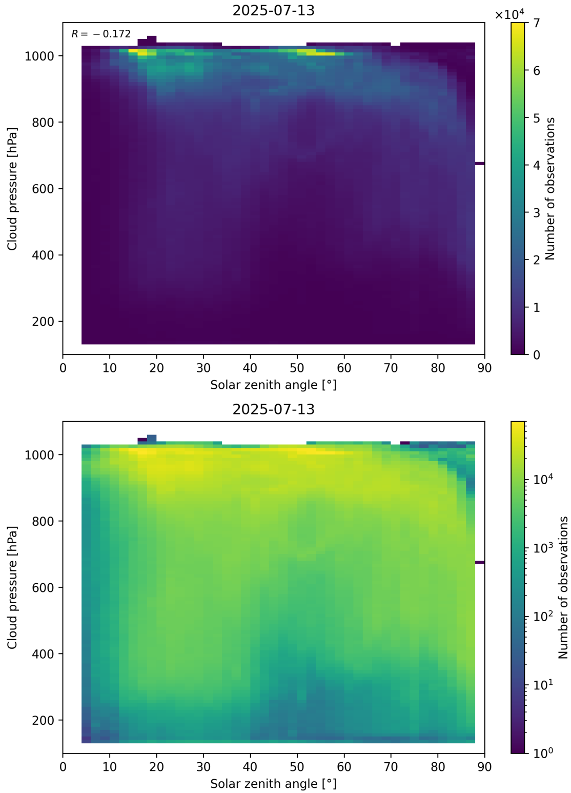
Figure 111: Scatter density plot of “Solar zenith angle” against “Cloud pressure” for 2025-07-13 to 2025-07-14.
