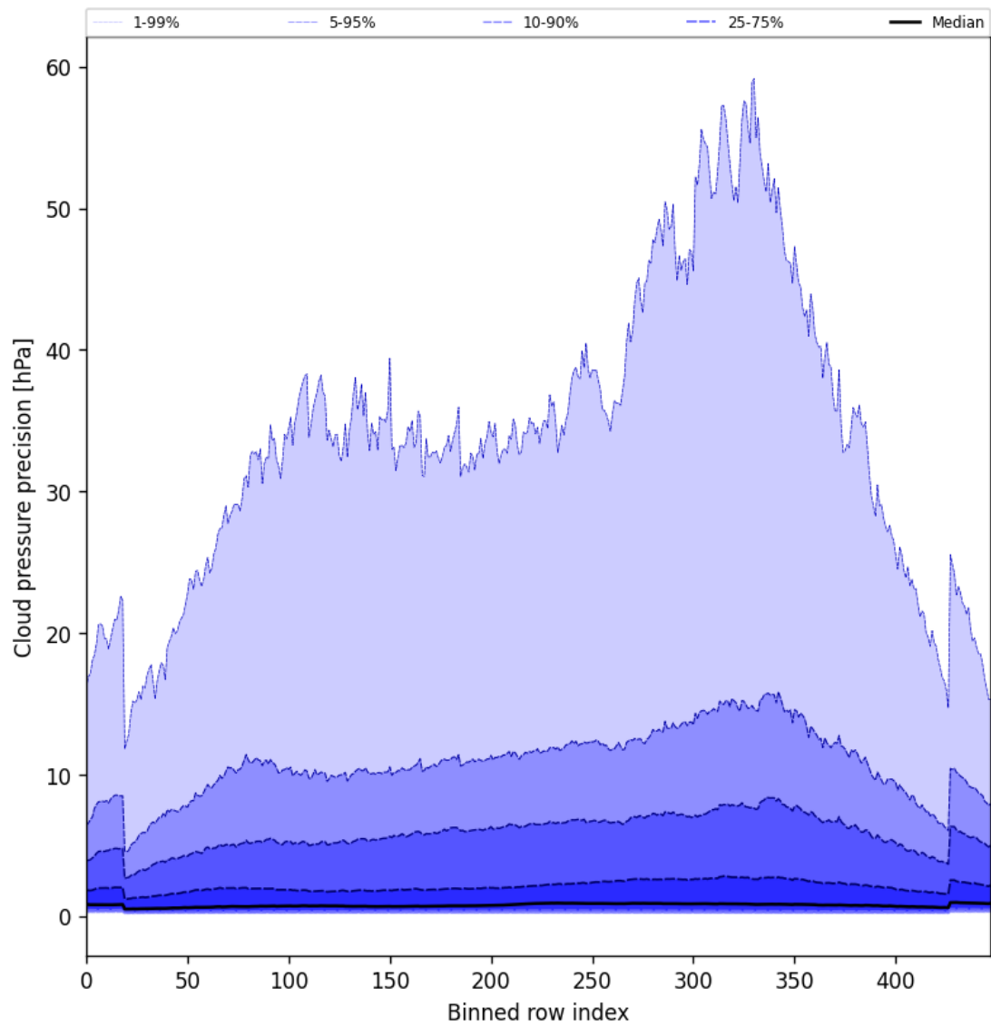
Figure 48: Along track statistics of “Cloud pressure precision” for 2025-07-13 to 2025-07-14
