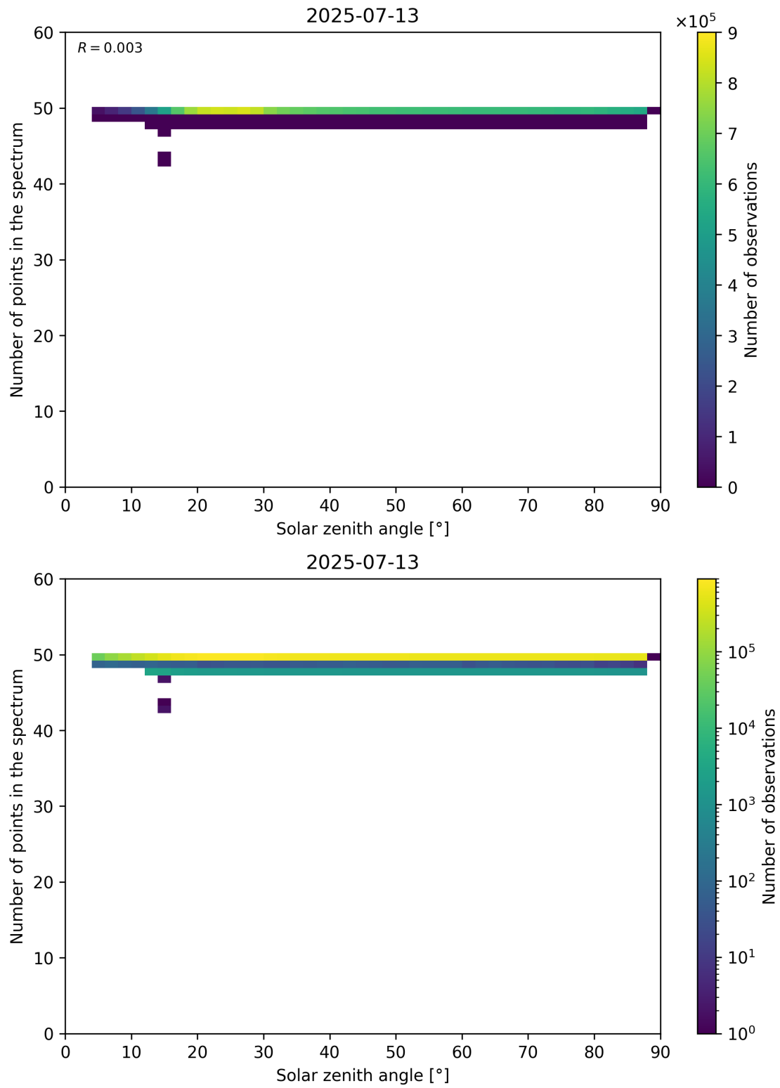
Figure 115: Scatter density plot of “Solar zenith angle” against “Number of points in the spectrum” for 2025-07-13 to 2025-07-14.
