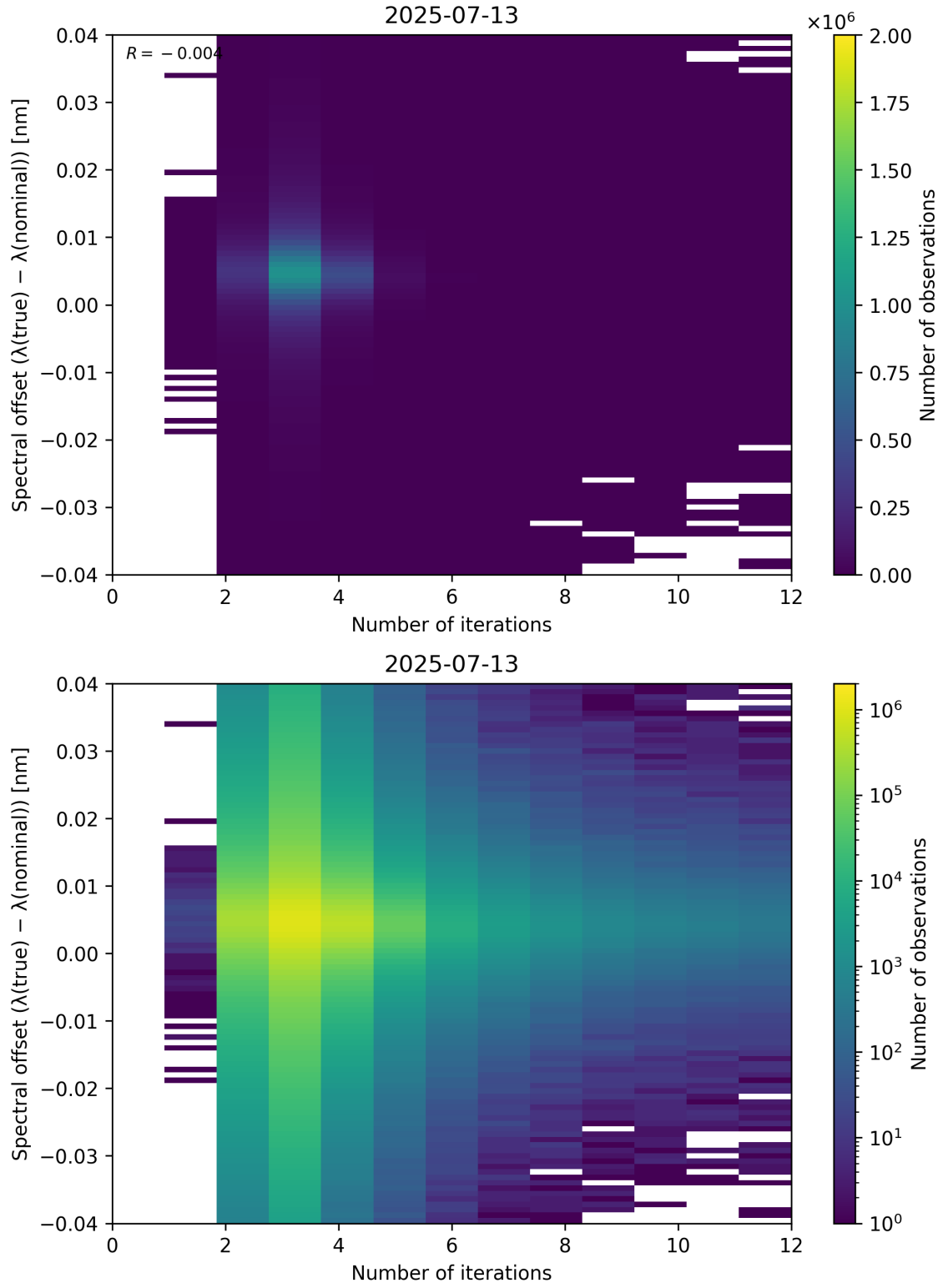
Figure 100: Scatter density plot of “Number of iterations” against “Spectral offset ( \lambda_{\text{true}} - \lambda_{\text{nominal}} )” for 2025-07-13 to 2025-07-14.
