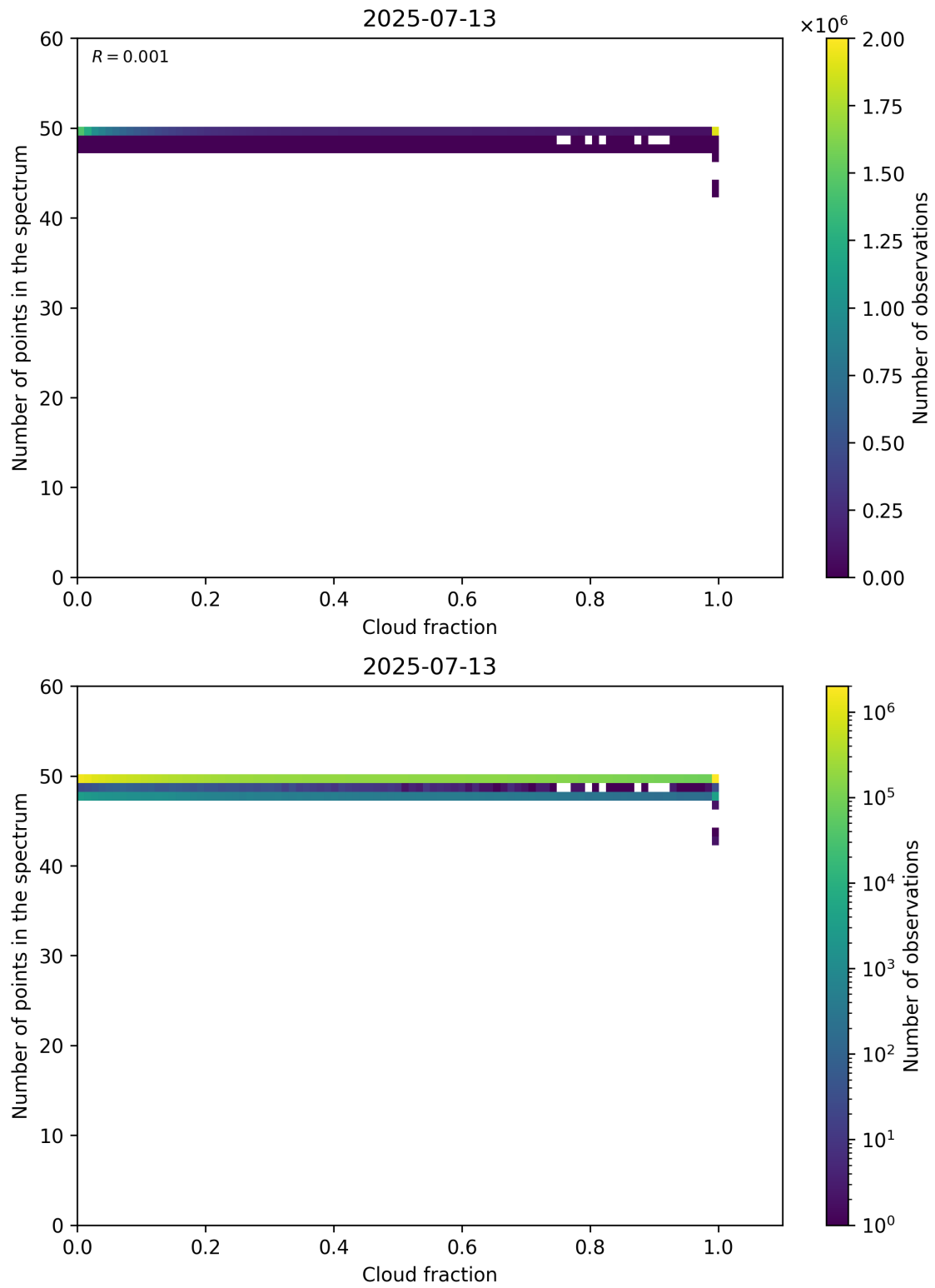
Figure 74: Scatter density plot of “Cloud fraction” against “Number of points in the spectrum” for 2025-07-13 to 2025-07-14.
