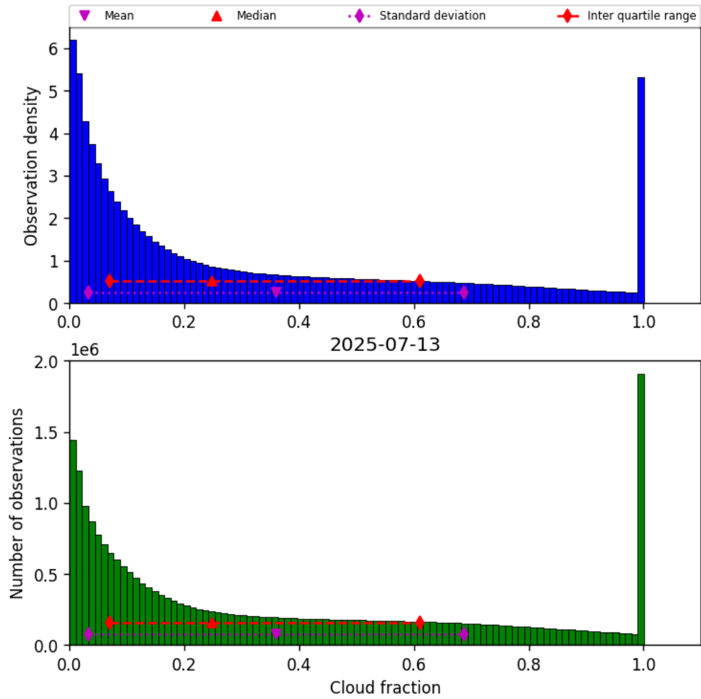
Figure 32: Histogram of “Cloud fraction” for 2025-07-13 to 2025-07-14
