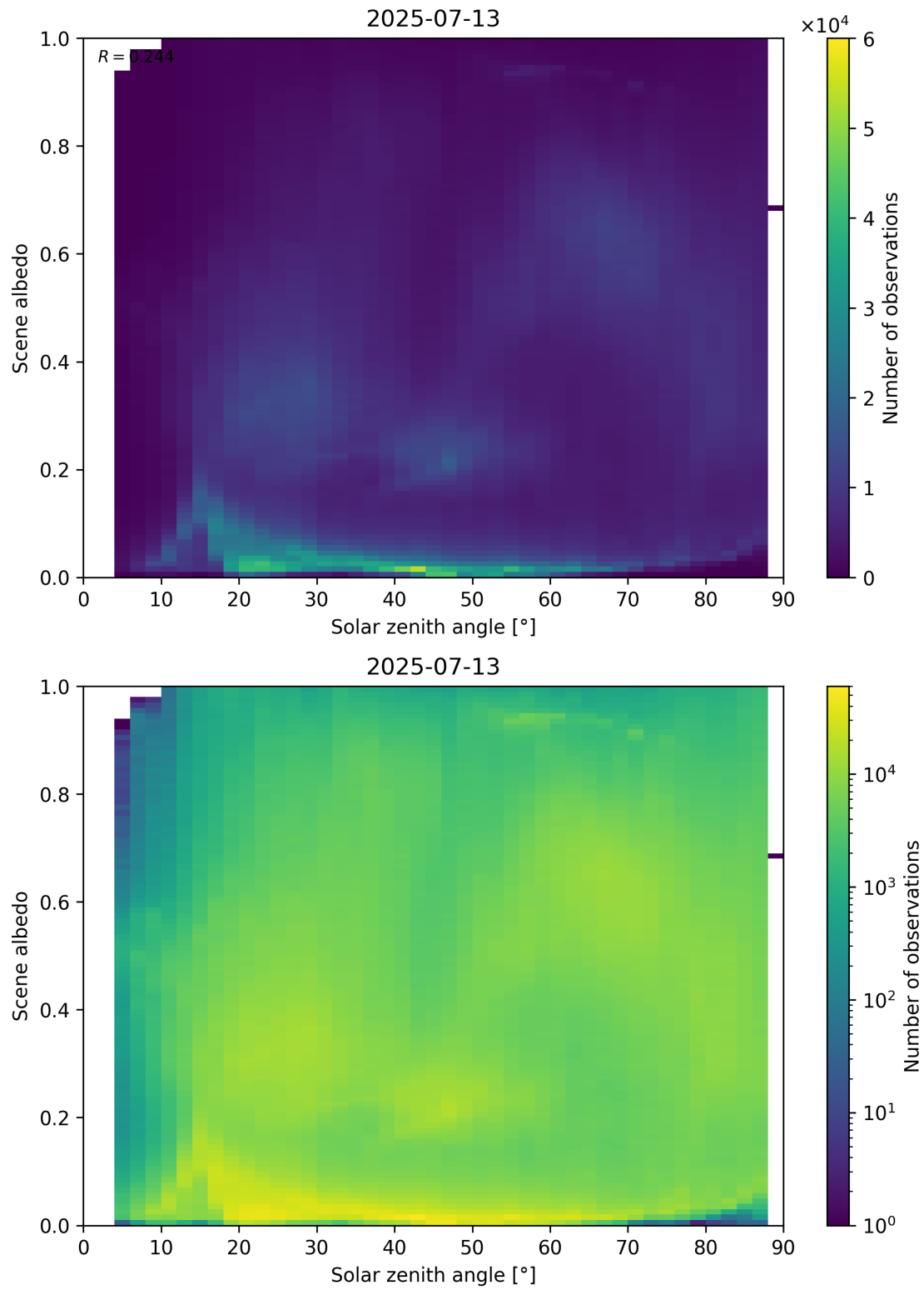
Figure 116: Scatter density plot of “Solar zenith angle” against “Scene albedo” for 2025-07-13 to 2025-07-14.
