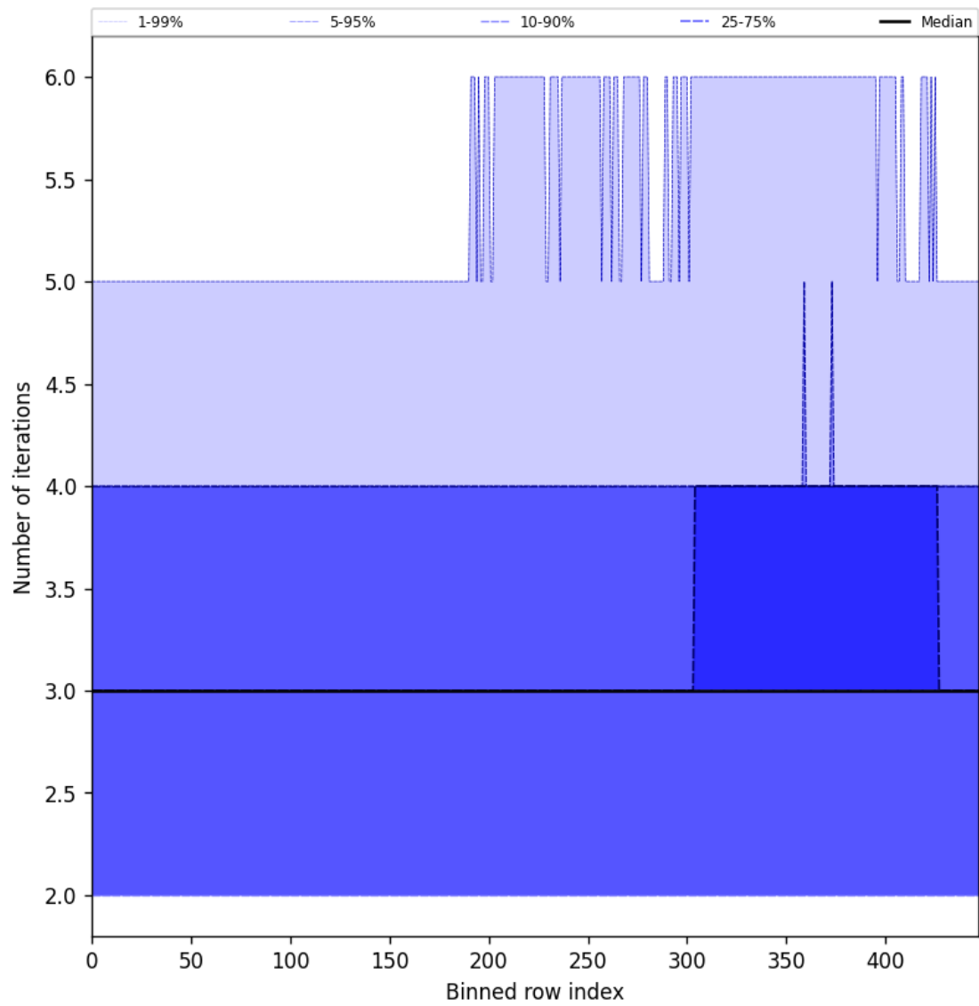
Figure 56: Along track statistics of “Number of iterations” for 2025-07-13 to 2025-07-14
