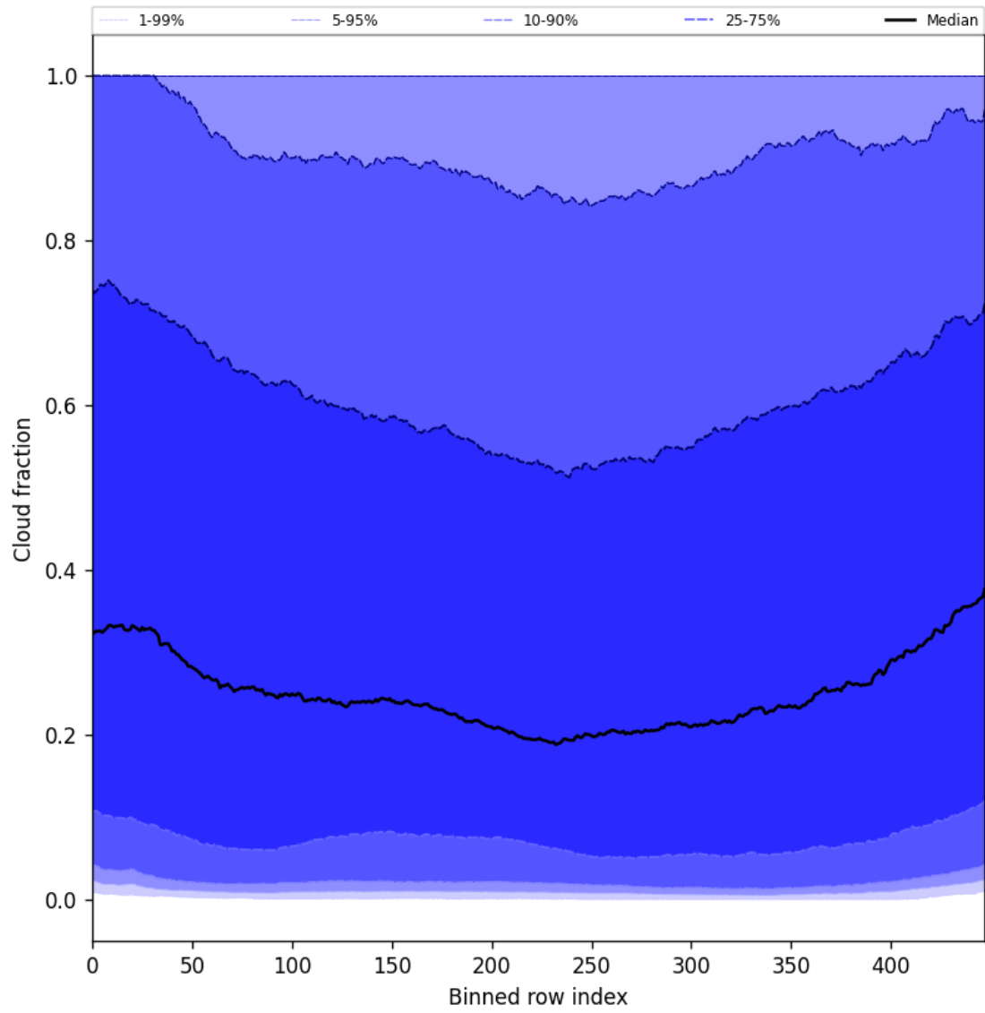
Figure 49: Along track statistics of “Cloud fraction” for 2025-07-13 to 2025-07-14
