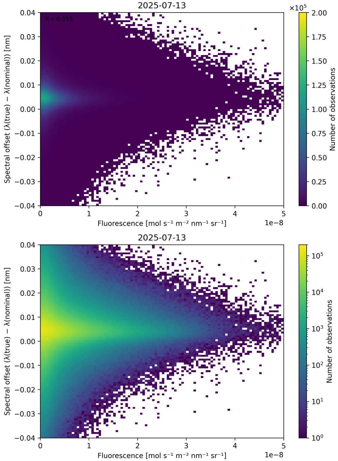
Figure 87: Scatter density plot of “Fluorescence” against “Spectral offset ( \lambda_{\text{true}} - \lambda_{\text{nominal}} )” for 2025-07-13 to 2025-07-14.
