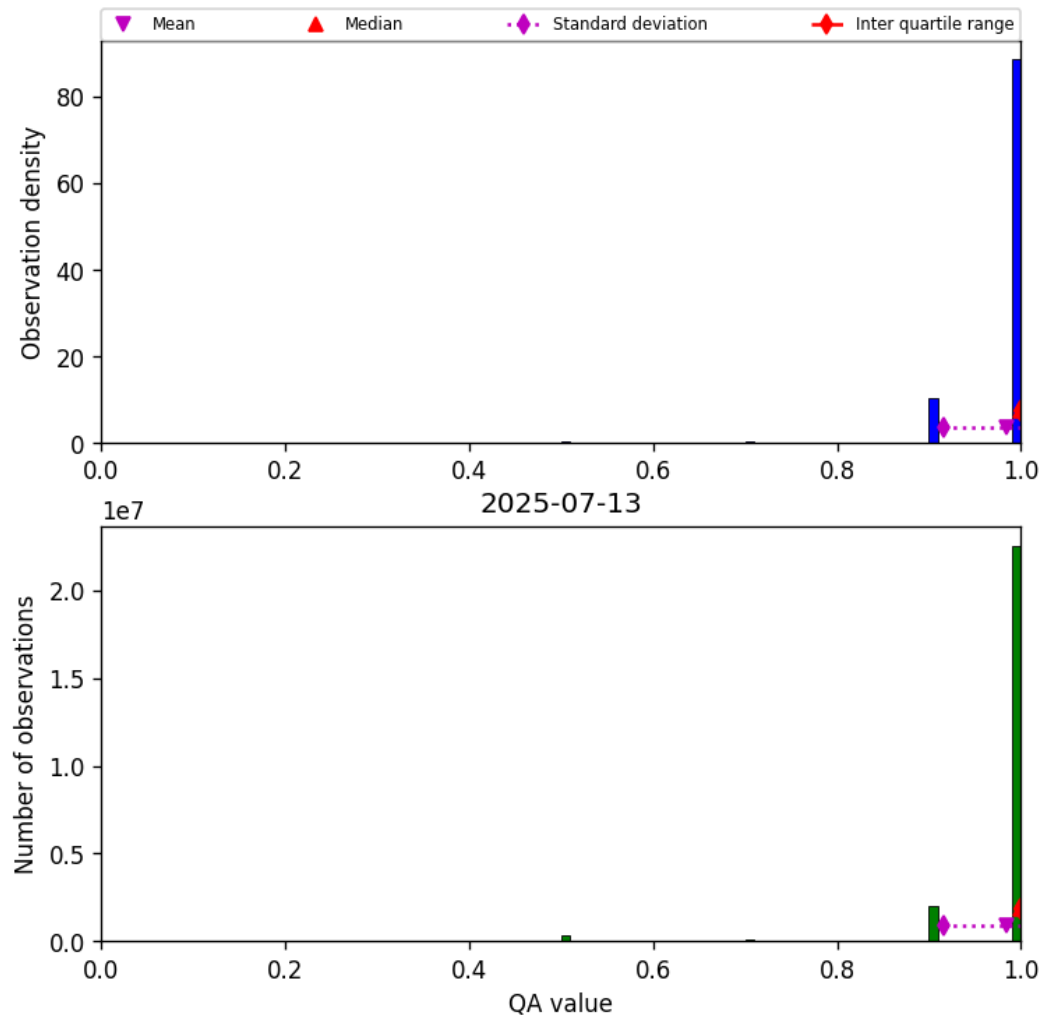
Figure 29: Histogram of “QA value” for 2025-07-13 to 2025-07-14
