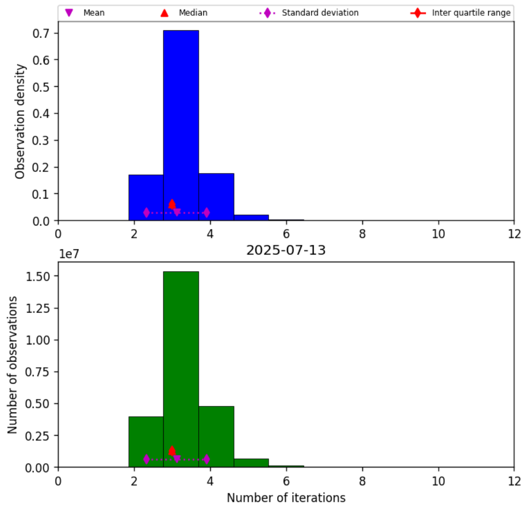
Figure 39: Histogram of “Number of iterations” for 2025-07-13 to 2025-07-14
