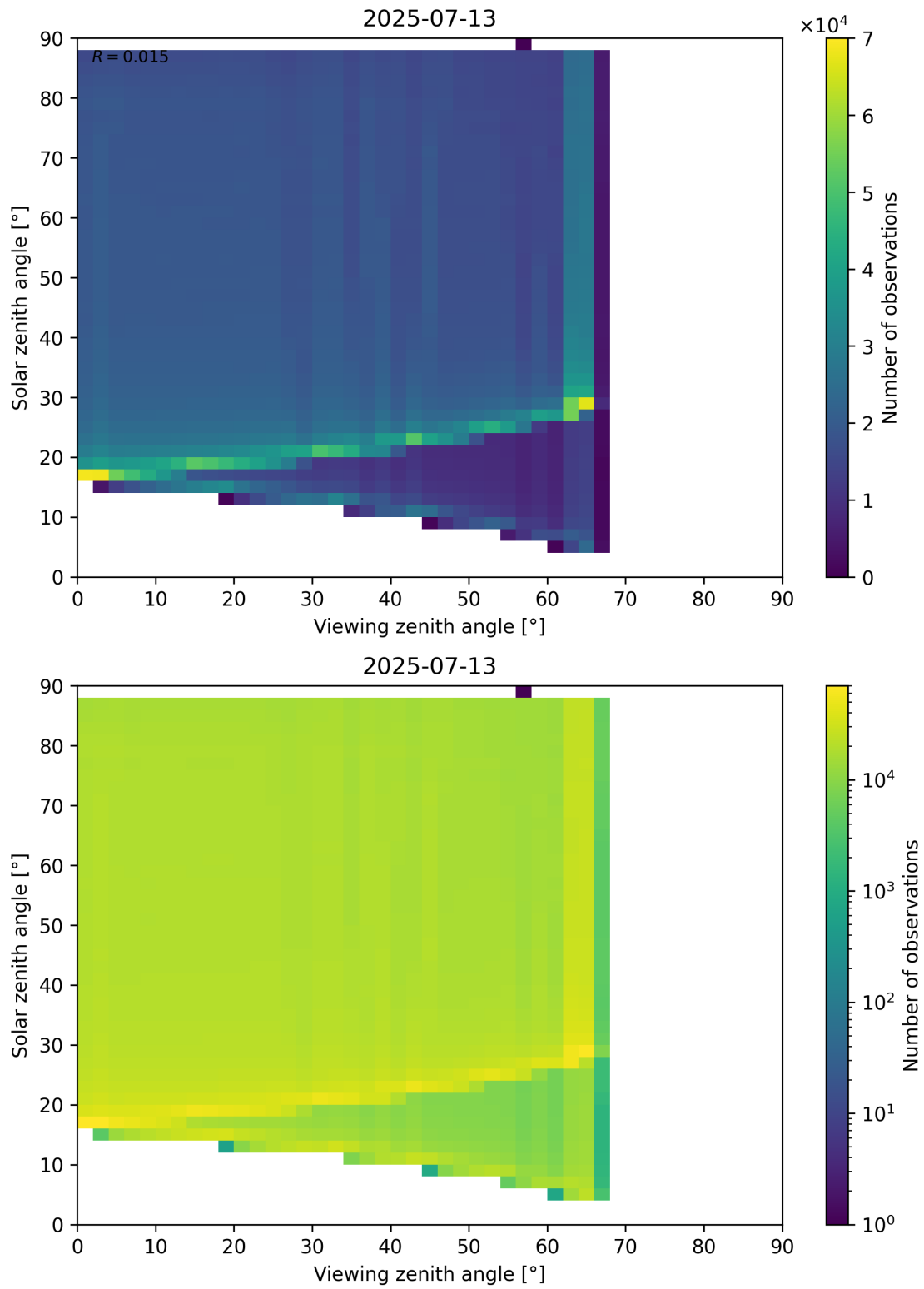
Figure 127: Scatter density plot of “Viewing zenith angle” against “Solar zenith angle” for 2025-07-13 to 2025-07-14.
