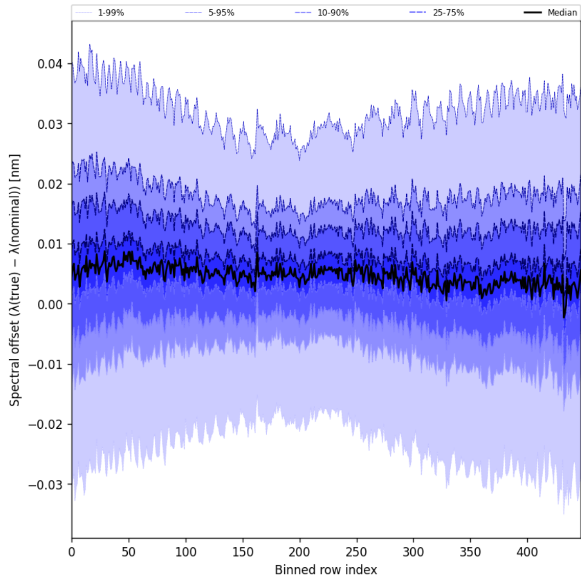
Figure 62: Along track statistics of “Spectral offset ( \lambda_{\text{true}} - \lambda_{\text{nominal}} )” for 2025-07-13 to 2025-07-14
