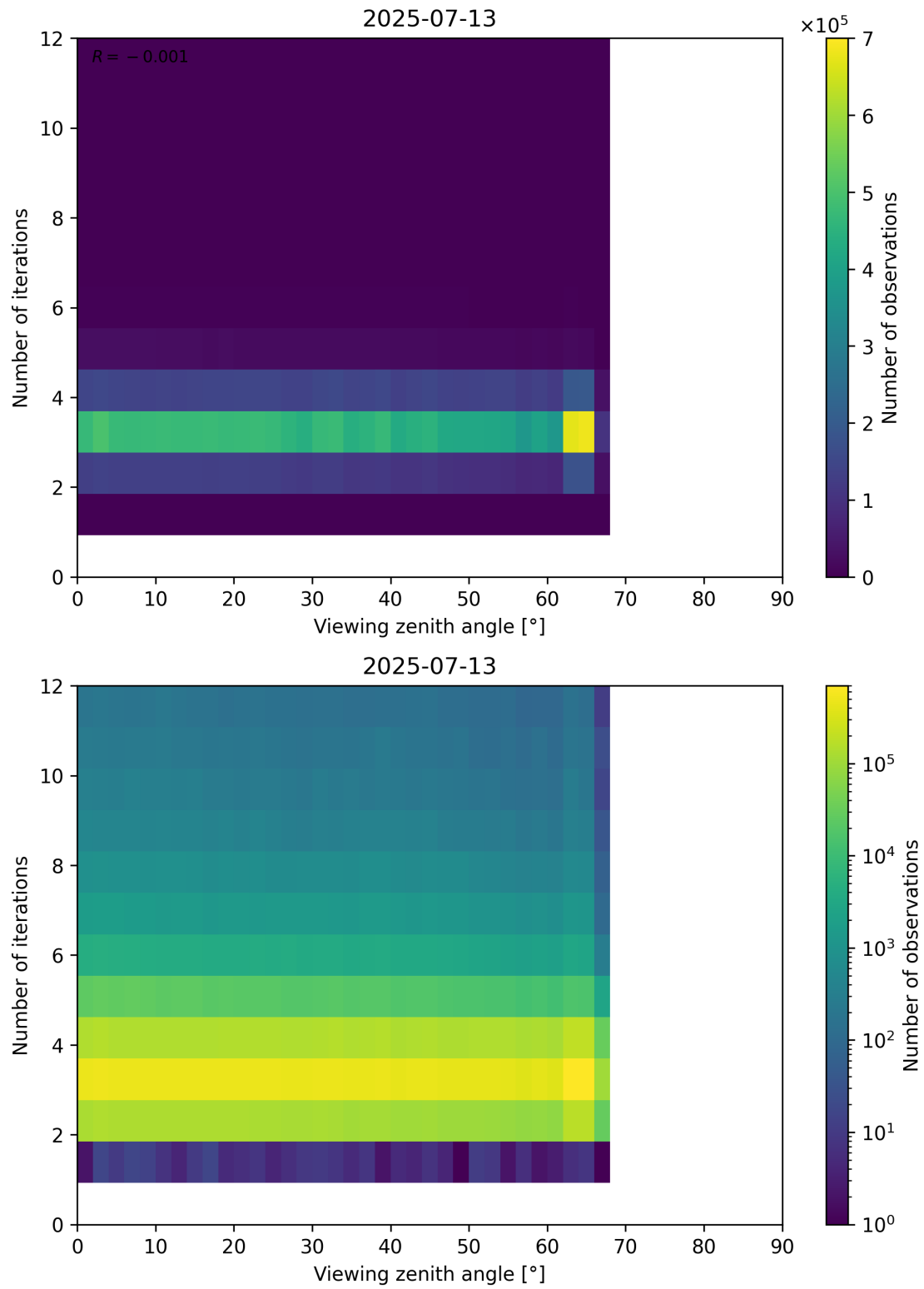
Figure 124: Scatter density plot of “Viewing zenith angle” against “Number of iterations” for 2025-07-13 to 2025-07-14.
