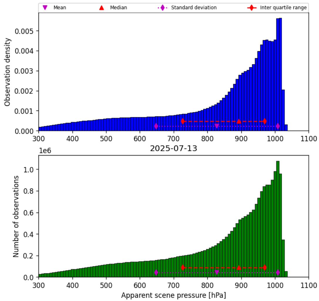
Figure 36: Histogram of “Apparent scene pressure” for 2025-07-13 to 2025-07-14
