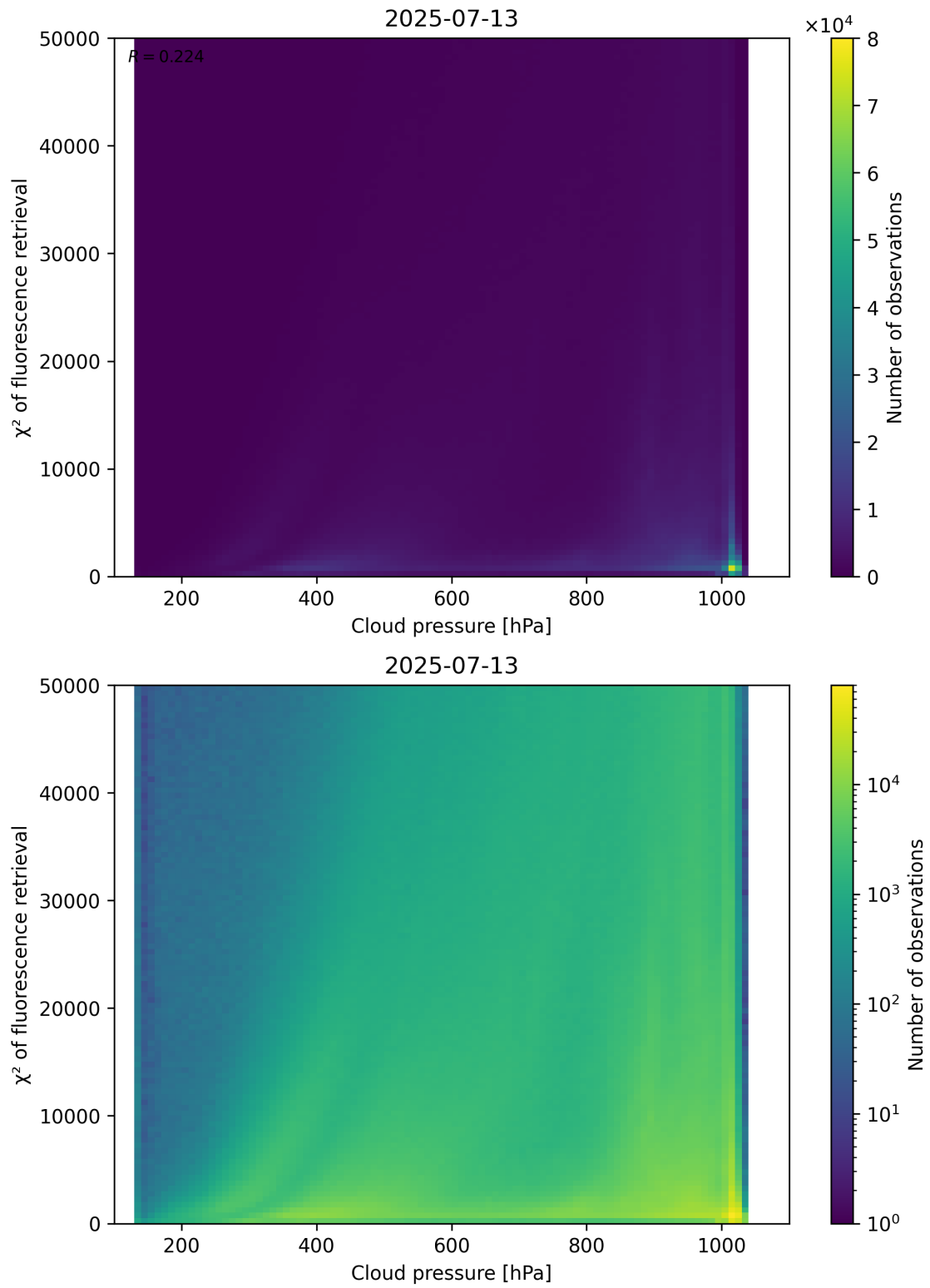
Figure 78: Scatter density plot of “Cloud pressure” against “ \chi^2 of fluorescence retrieval” for 2025-07-13 to 2025-07-14.
