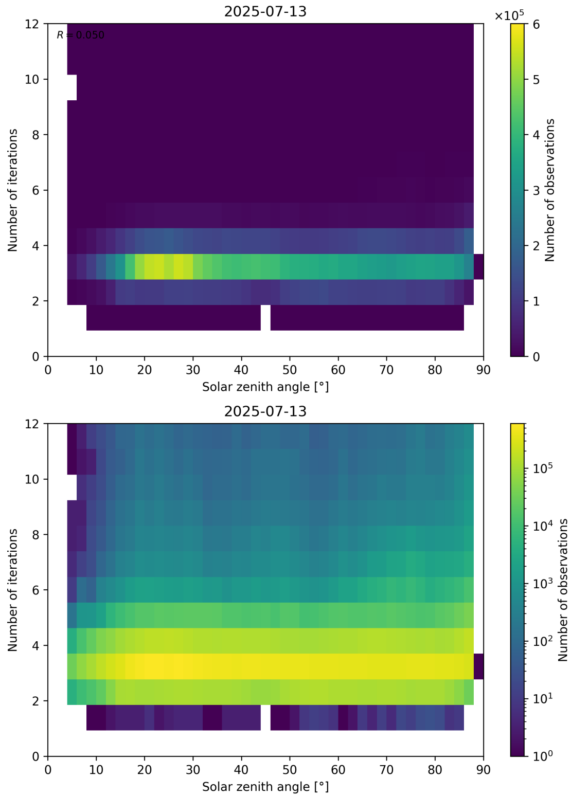
Figure 114: Scatter density plot of “Solar zenith angle” against “Number of iterations” for 2025-07-13 to 2025-07-14.
