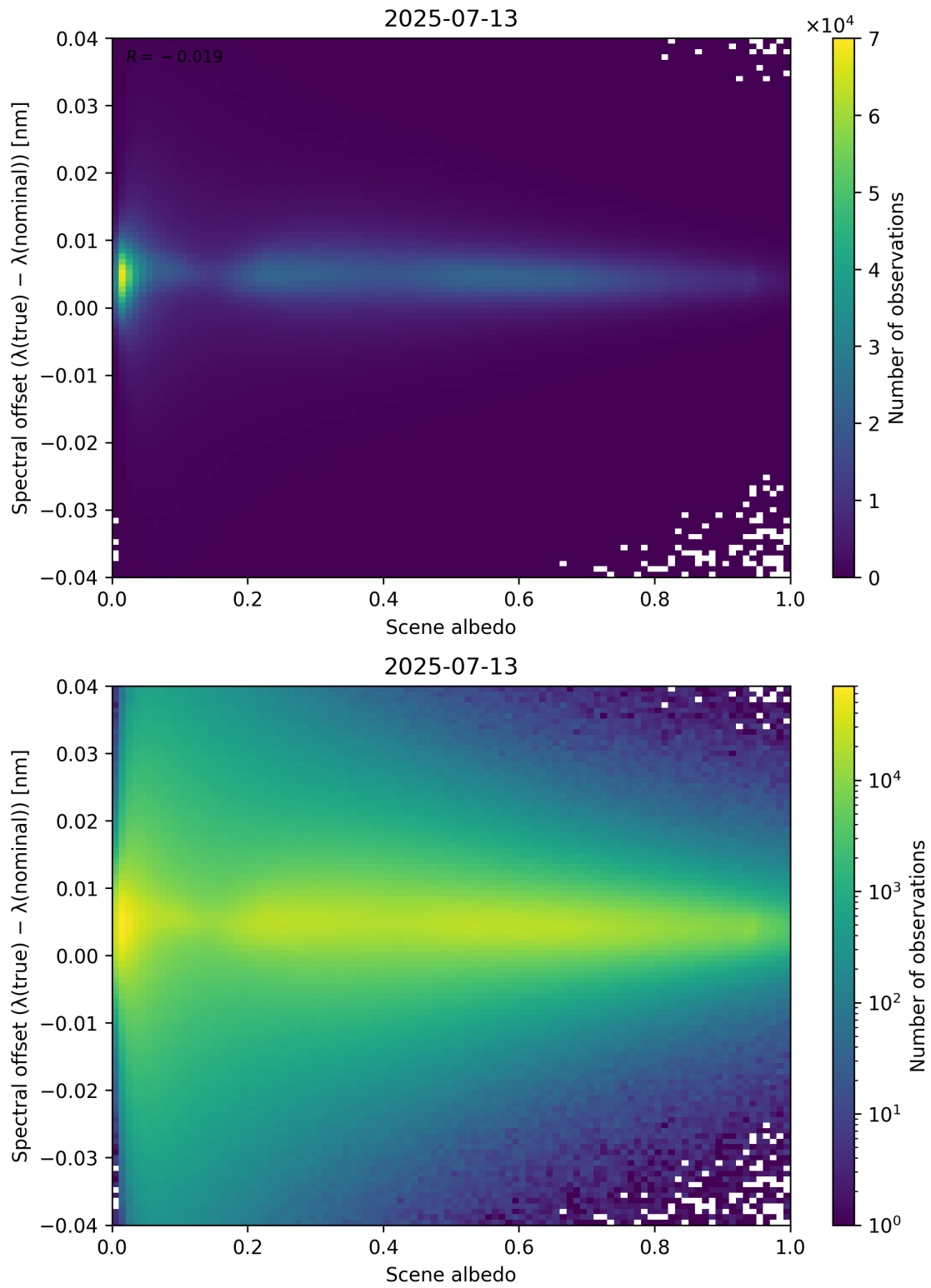
Figure 107: Scatter density plot of “Scene albedo” against “Spectral offset ( \lambda_{\text{true}} - \lambda_{\text{nominal}} )” for 2025-07-13 to 2025-07-14.
