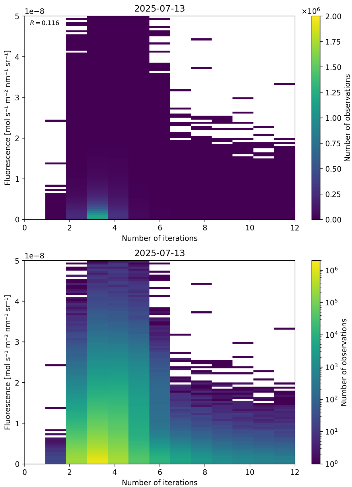
Figure 98: Scatter density plot of “Number of iterations” against “Fluorescence” for 2025-07-13 to 2025-07-14.
