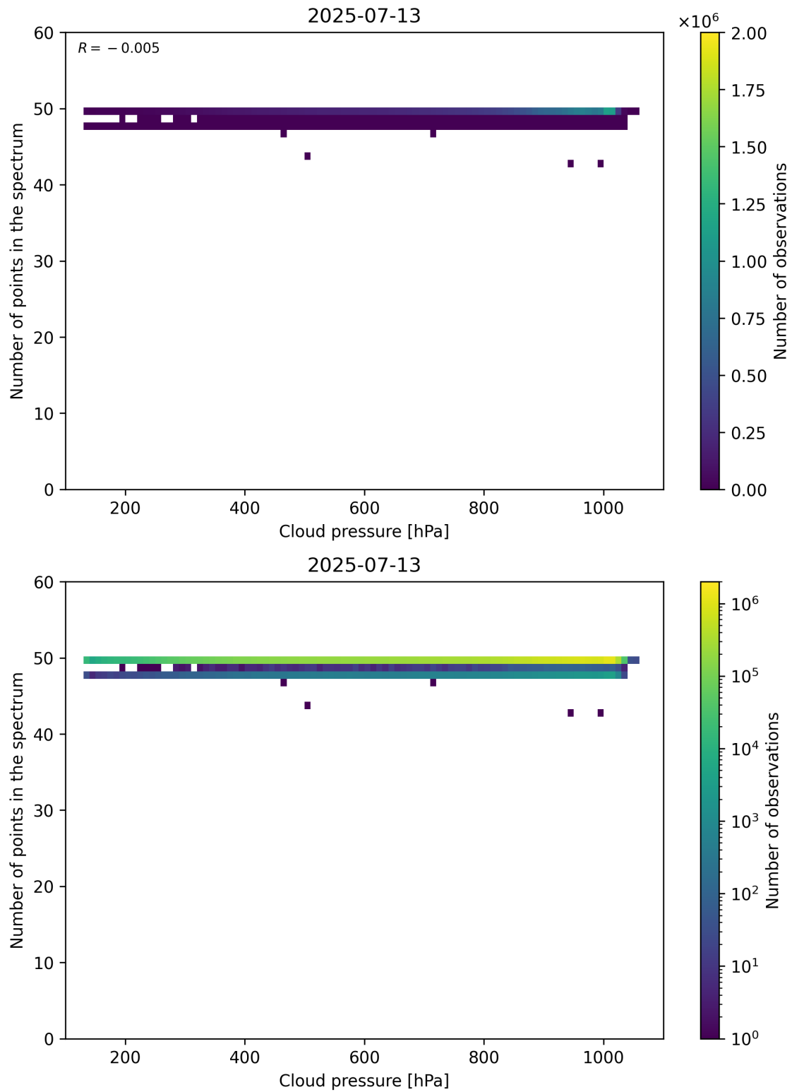
Figure 82: Scatter density plot of “Cloud pressure” against “Number of points in the spectrum” for 2025-07-13 to 2025-07-14.
