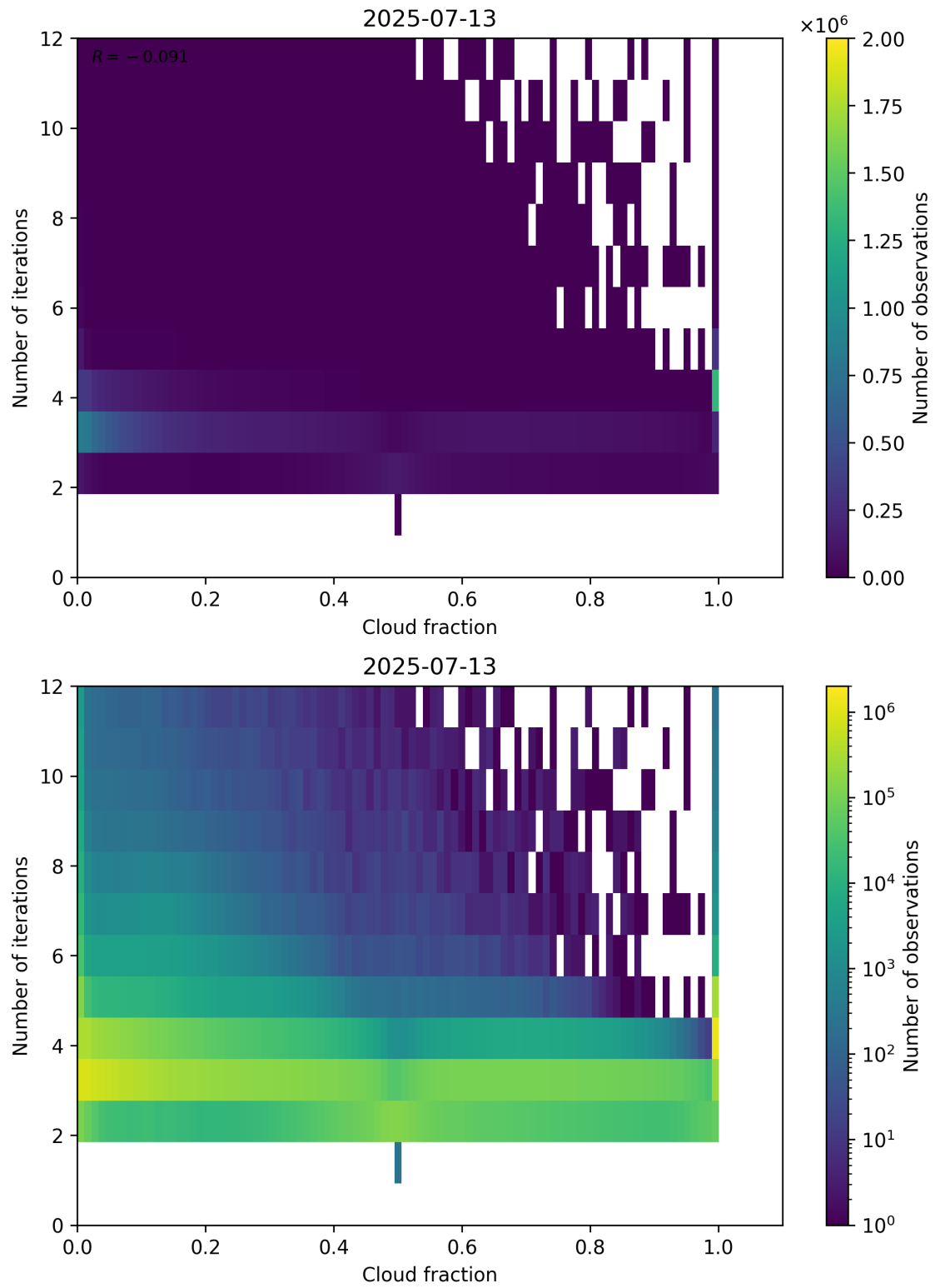
Figure 73: Scatter density plot of “Cloud fraction” against “Number of iterations” for 2025-07-13 to 2025-07-14.
