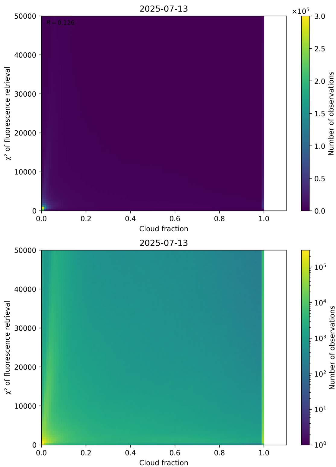
Figure 71: Scatter density plot of “Cloud fraction” against “ \chi^2 of fluorescence retrieval” for 2025-07-13 to 2025-07-14.
