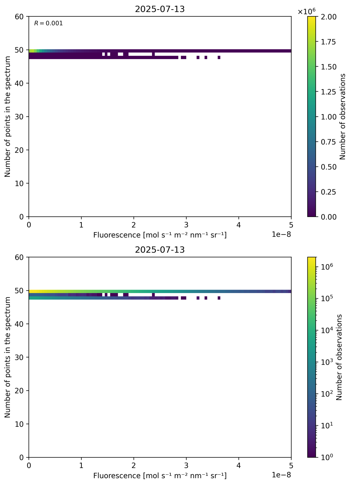
Figure 86: Scatter density plot of “Fluorescence” against “Number of points in the spectrum” for 2025-07-13 to 2025-07-14.
