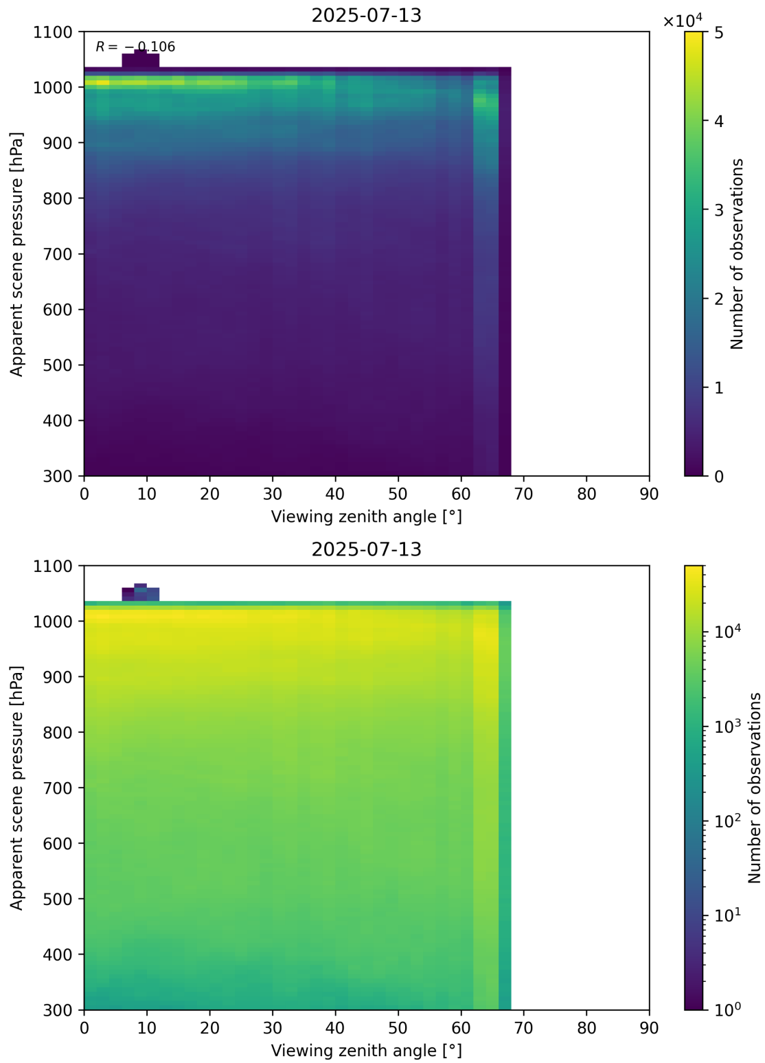
Figure 118: Scatter density plot of “Viewing zenith angle” against “Apparent scene pressure” for 2025-07-13 to 2025-07-14.
