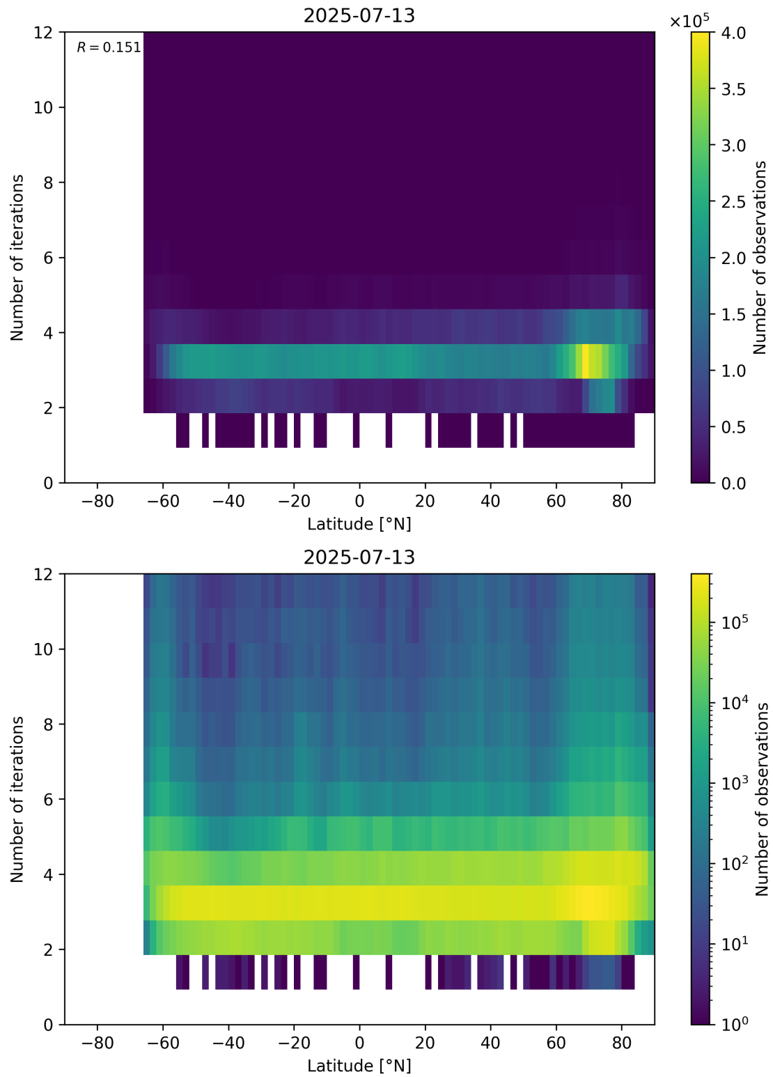
Figure 93: Scatter density plot of “Latitude” against “Number of iterations” for 2025-07-13 to 2025-07-14.
