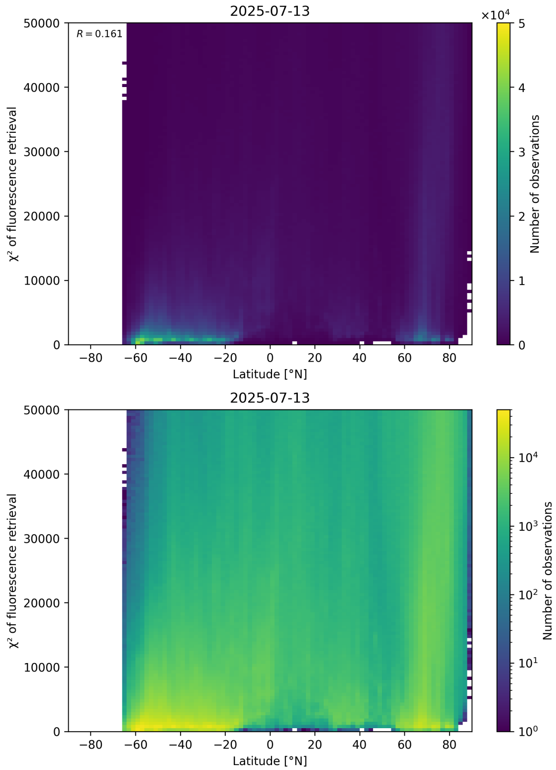
Figure 89: Scatter density plot of “Latitude” against “ \chi^2 of fluorescence retrieval” for 2025-07-13 to 2025-07-14.
