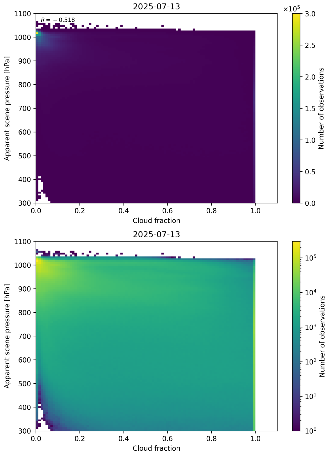
Figure 70: Scatter density plot of “Cloud fraction” against “Apparent scene pressure” for 2025-07-13 to 2025-07-14.
