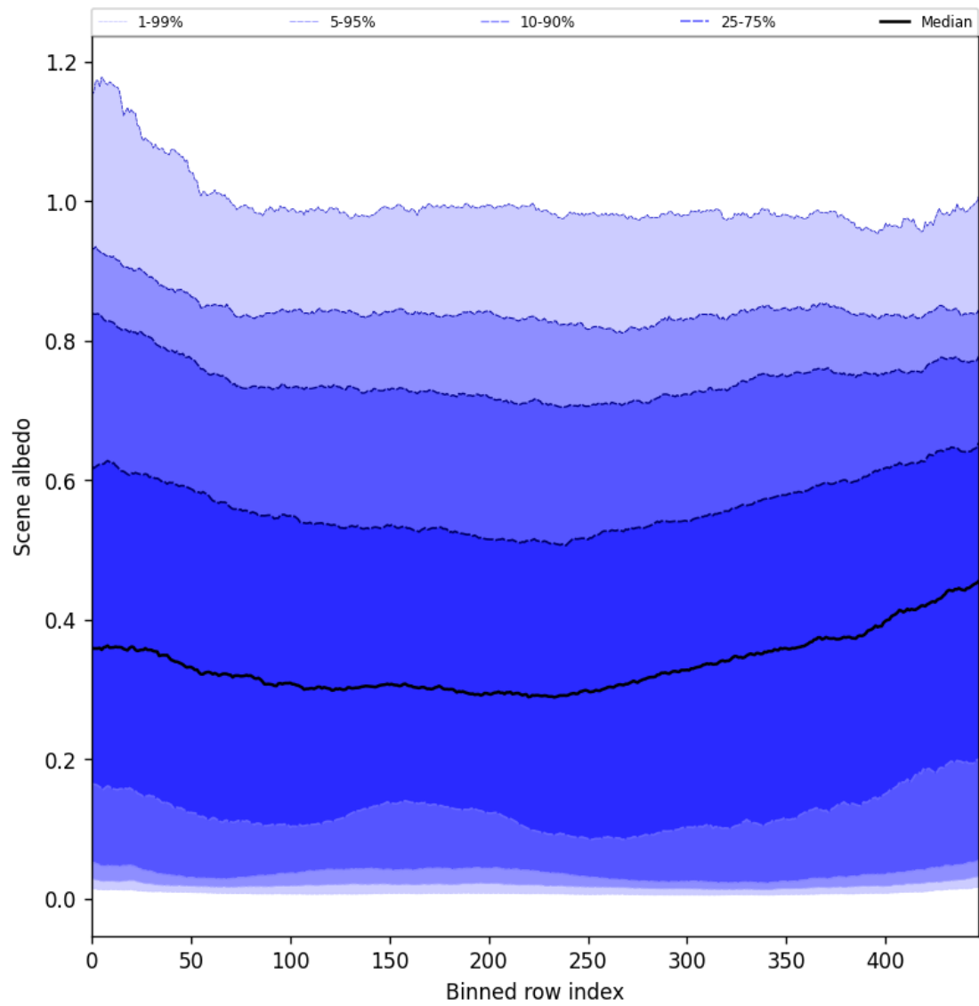
Figure 51: Along track statistics of “Scene albedo” for 2025-07-13 to 2025-07-14
