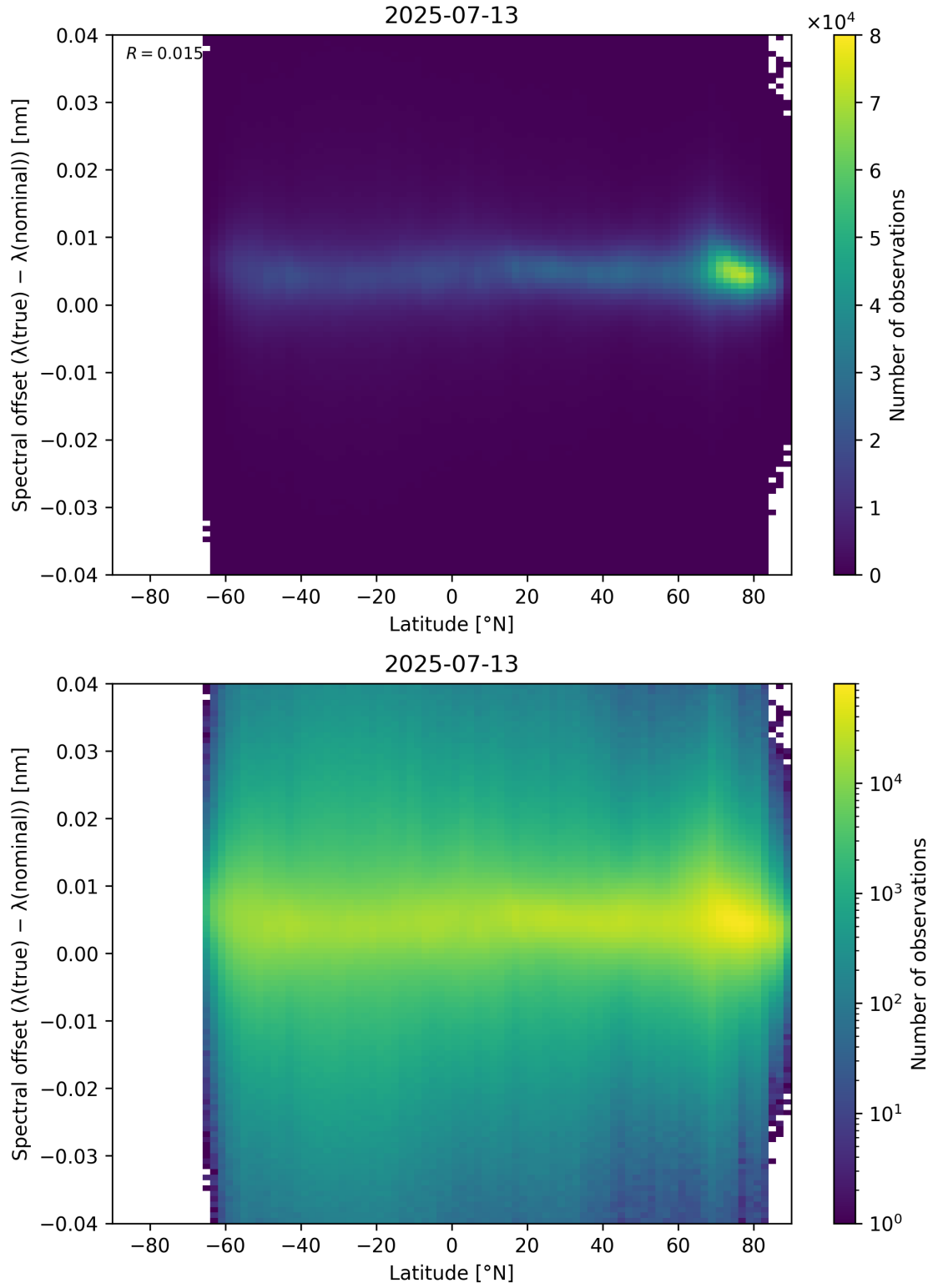
Figure 96: Scatter density plot of “Latitude” against “Spectral offset ( \lambda_{\text{true}} - \lambda_{\text{nominal}} )” for 2025-07-13 to 2025-07-14.
