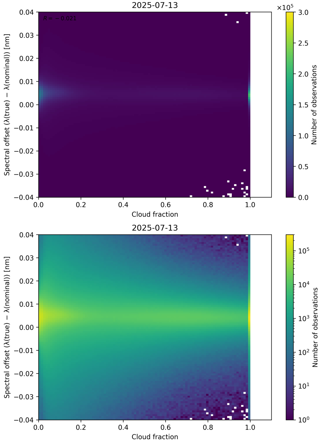
Figure 76: Scatter density plot of “Cloud fraction” against “Spectral offset ( \lambda_{\text{true}} - \lambda_{\text{nominal}} )” for 2025-07-13 to 2025-07-14.
