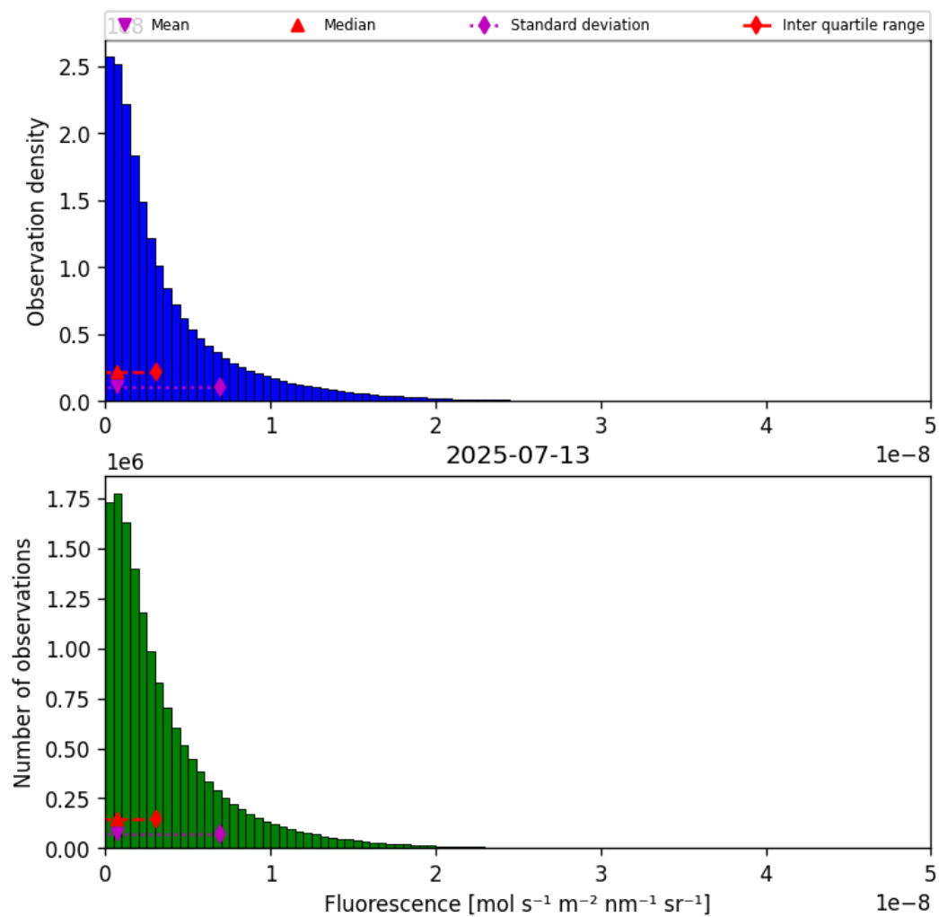
Figure 40: Histogram of “Fluorescence” for 2025-07-13 to 2025-07-14
