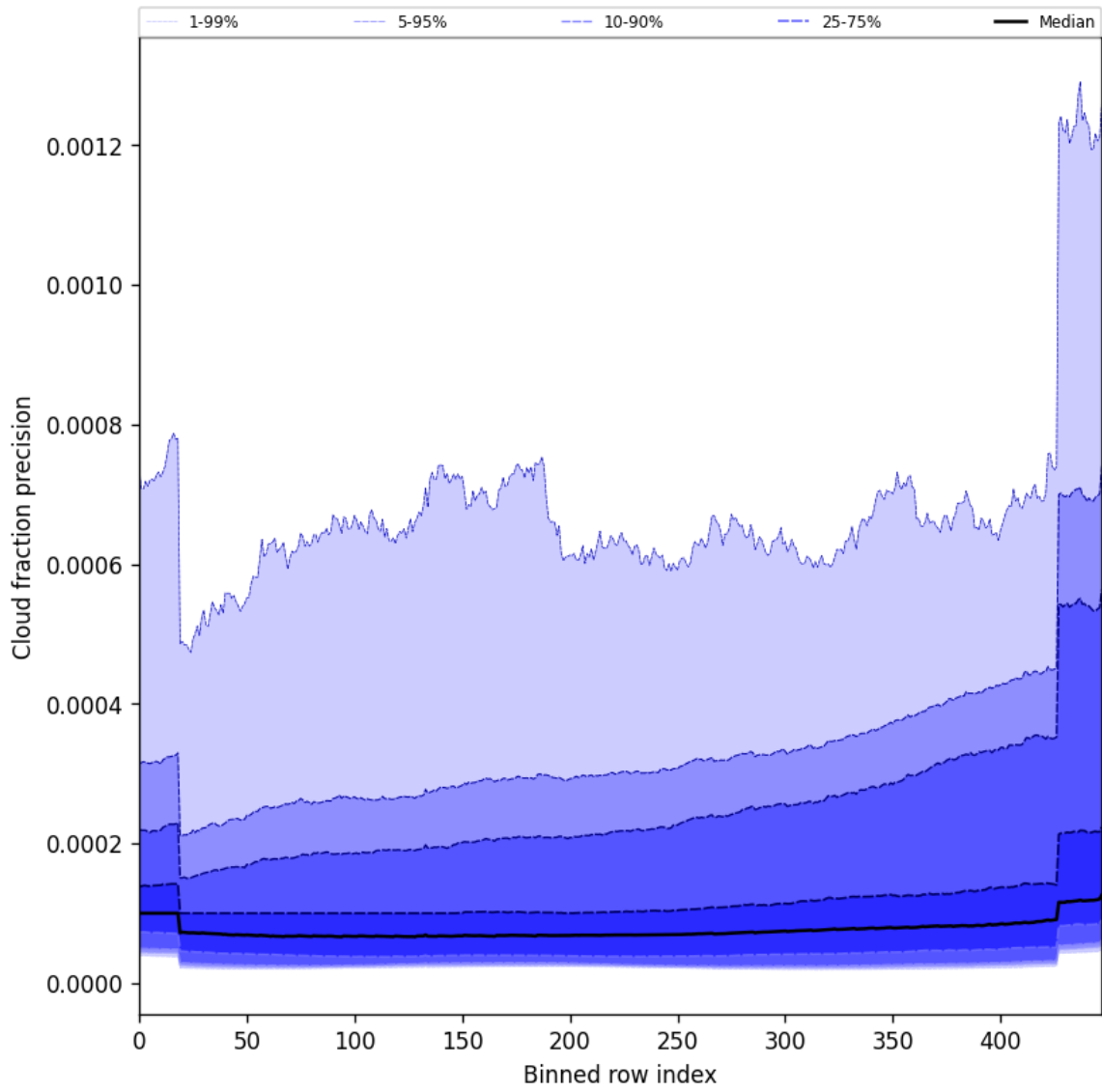
Figure 50: Along track statistics of “Cloud fraction precision” for 2025-07-13 to 2025-07-14
