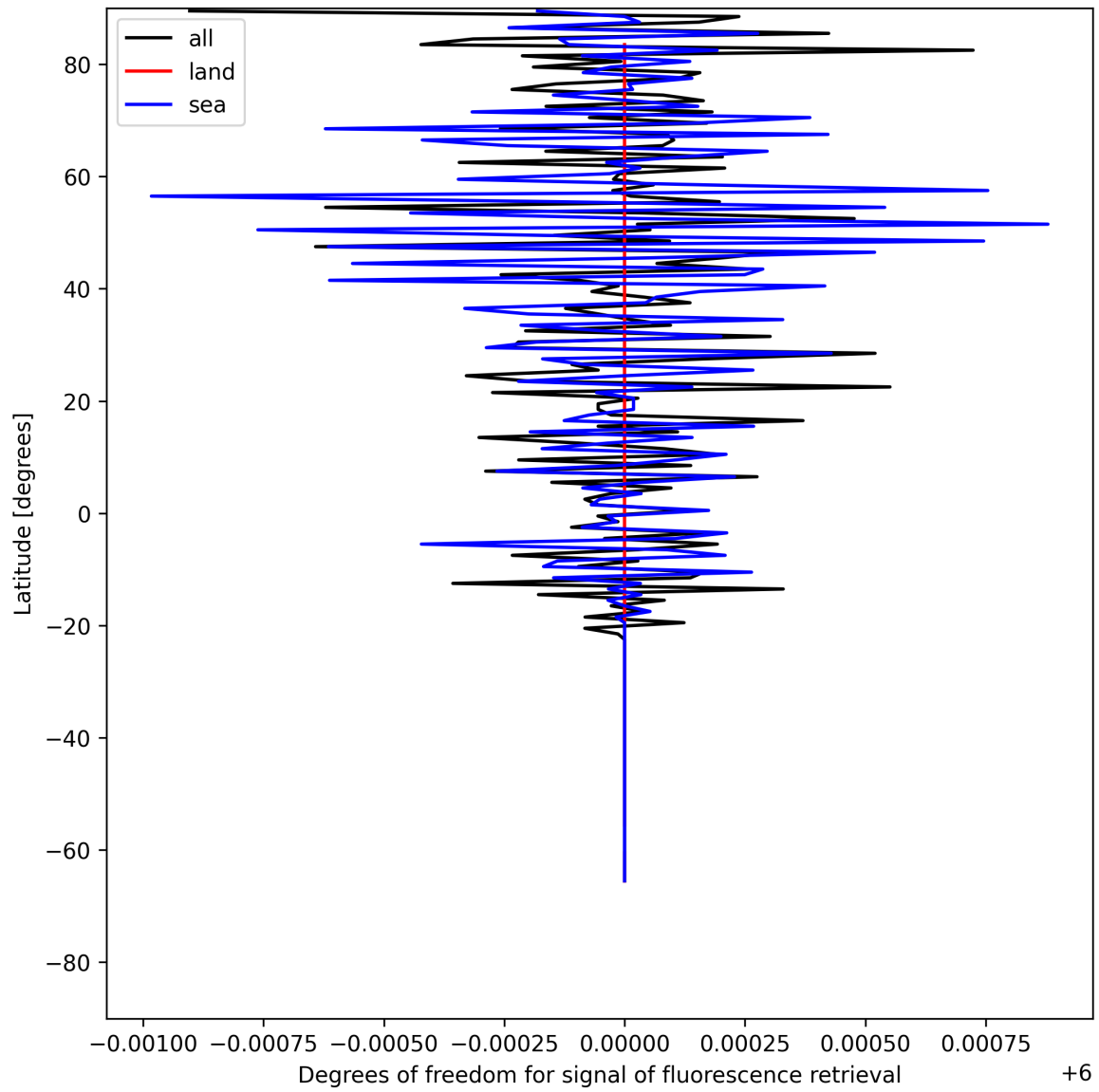
Figure 26: Zonal average of “Degrees of freedom for signal of fluorescence retrieval” for 2025-07-13 to 2025-07-14.
