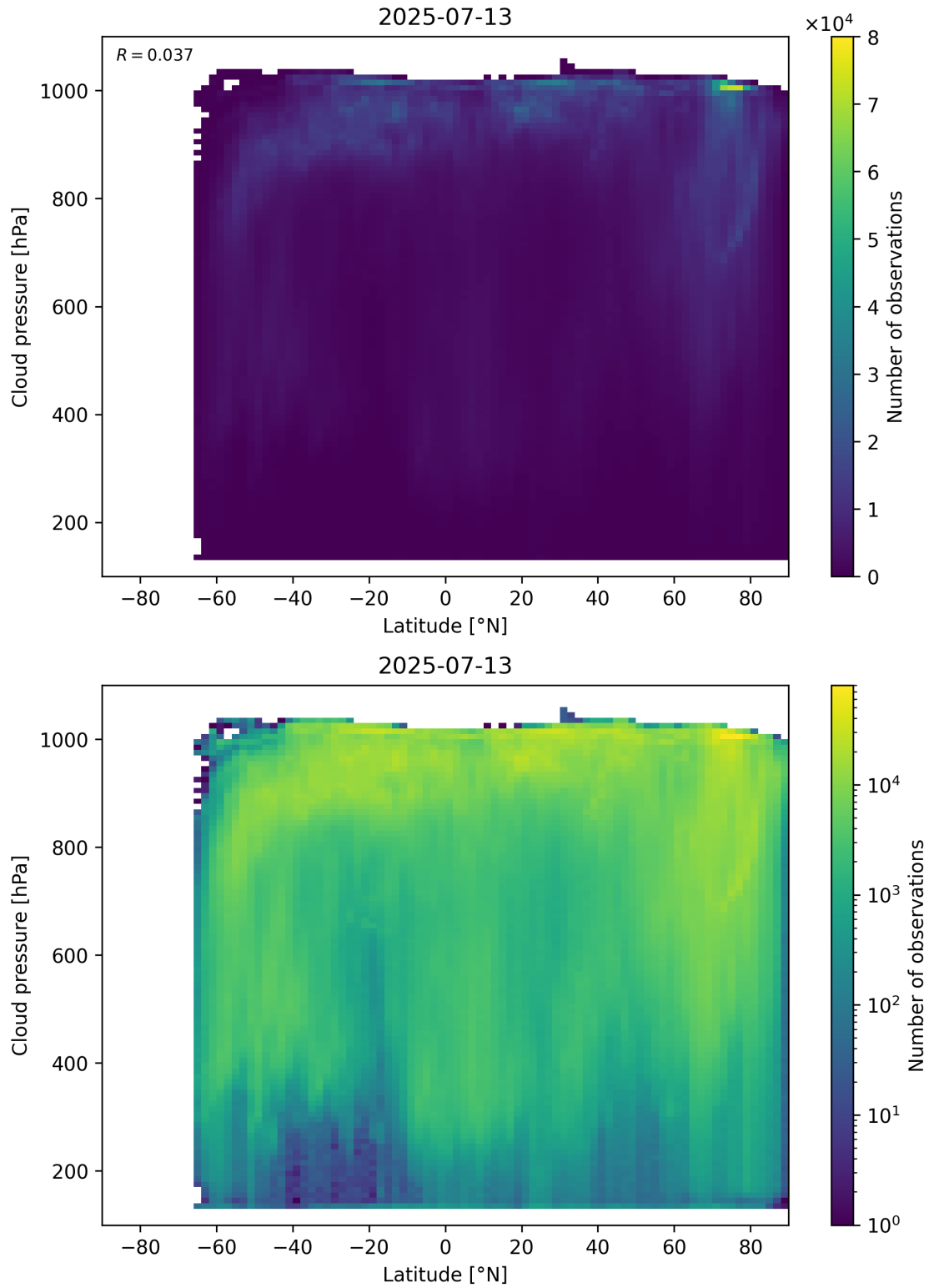
Figure 91: Scatter density plot of “Latitude” against “Cloud pressure” for 2025-07-13 to 2025-07-14.
