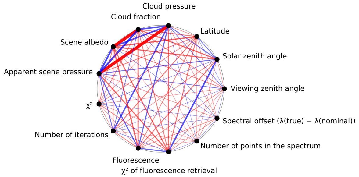
Figure 1: Map of correlation graph for 2025-07-13 to 2025-07-14.
