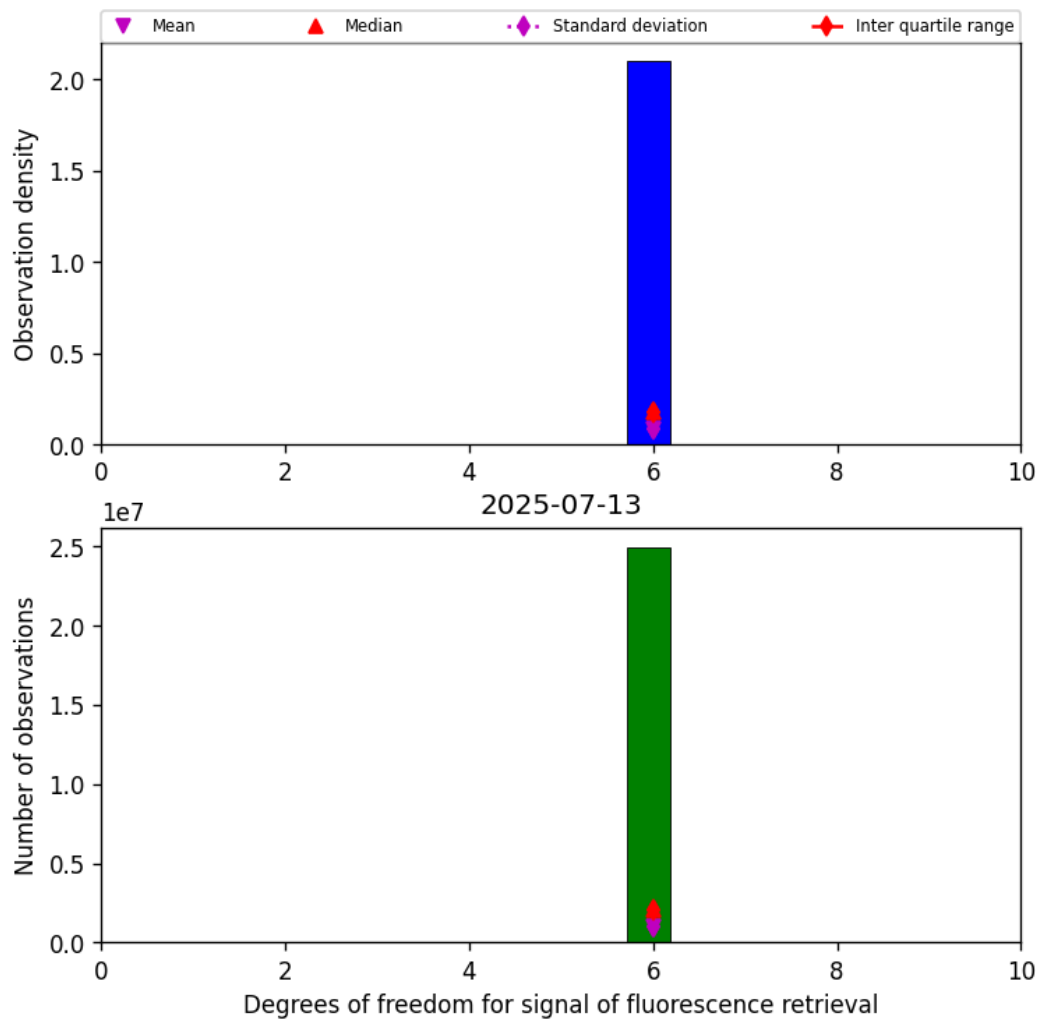
Figure 43: Histogram of “Degrees of freedom for signal of fluorescence retrieval” for 2025-07-13 to 2025-07-14
