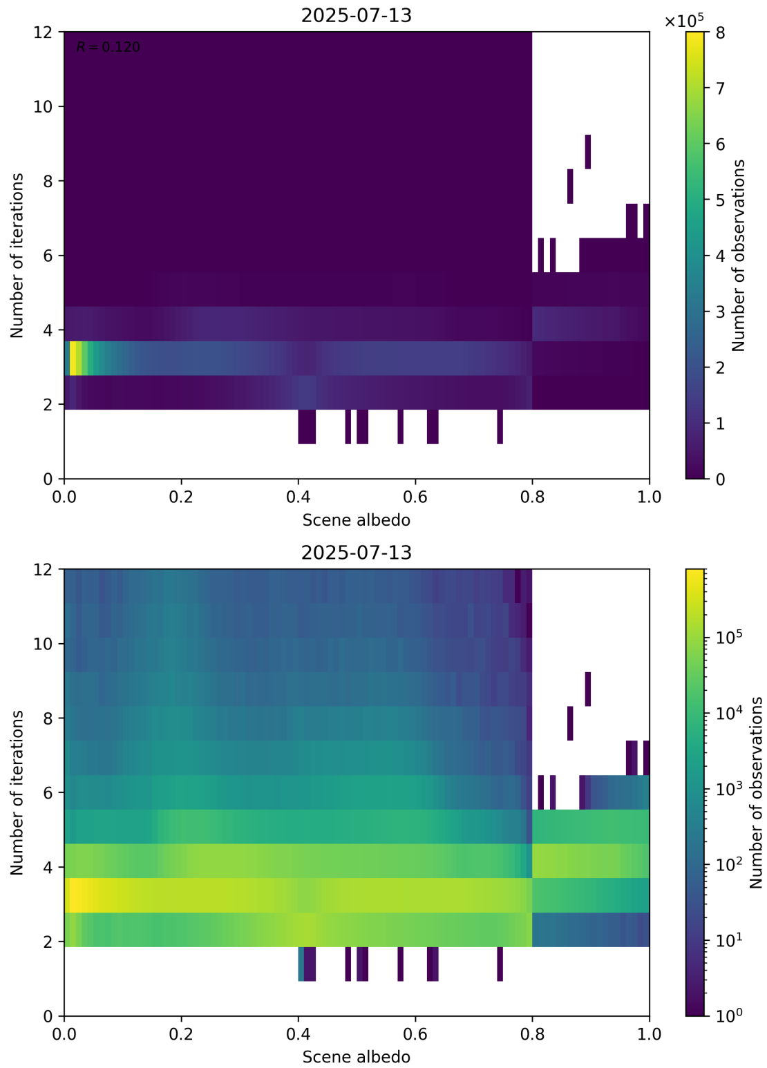
Figure 105: Scatter density plot of “Scene albedo” against “Number of iterations” for 2025-07-13 to 2025-07-14.
