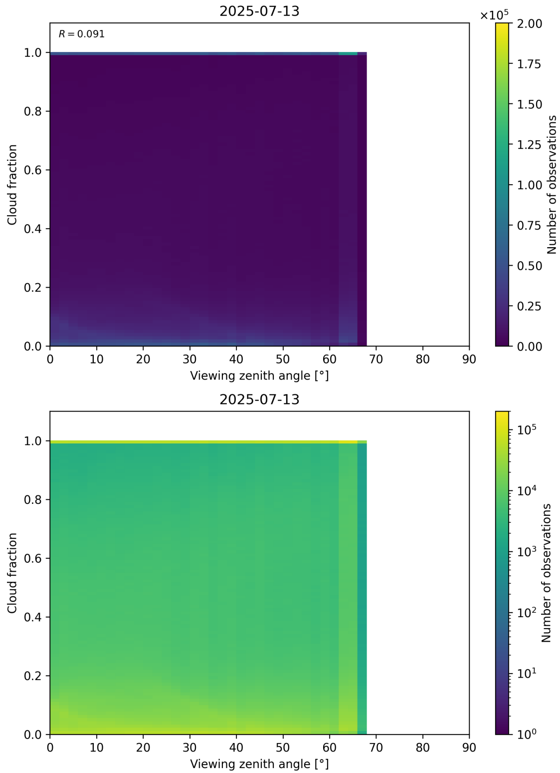
Figure 120: Scatter density plot of “Viewing zenith angle” against “Cloud fraction” for 2025-07-13 to 2025-07-14.
