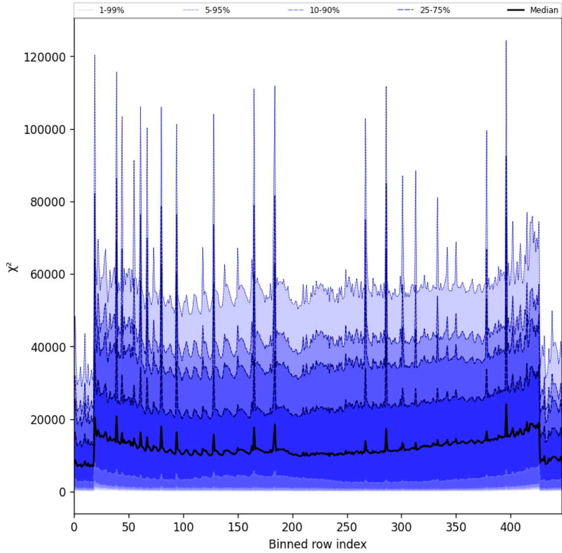
Figure 55: Along track statistics of “ \chi^2 ” for 2025-07-13 to 2025-07-14
