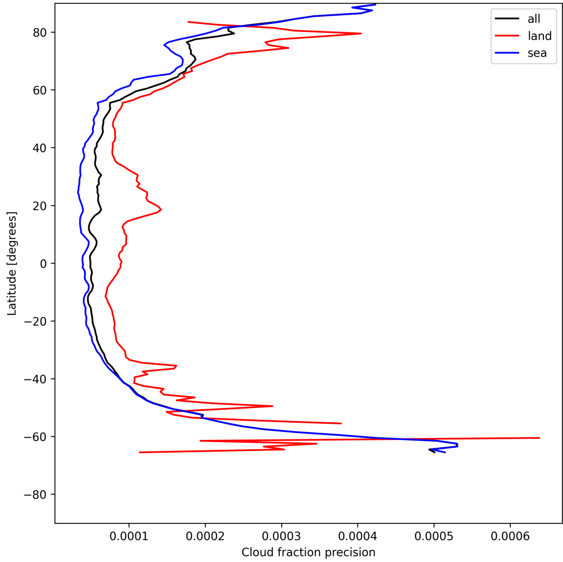
Figure 16: Zonal average of “Cloud fraction precision” for 2025-07-13 to 2025-07-14.
