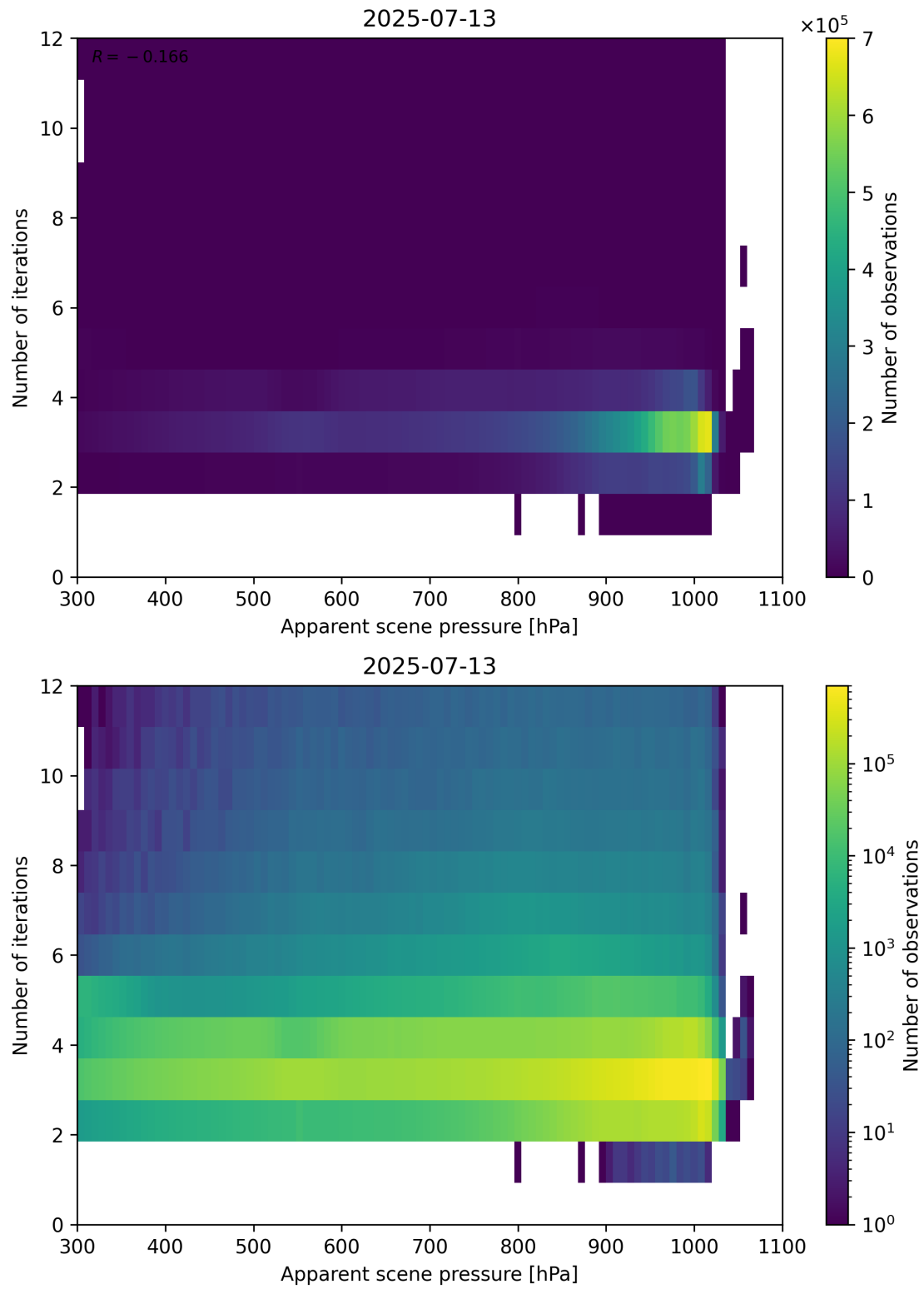
Figure 65: Scatter density plot of “Apparent scene pressure” against “Number of iterations” for 2025-07-13 to 2025-07-14.
