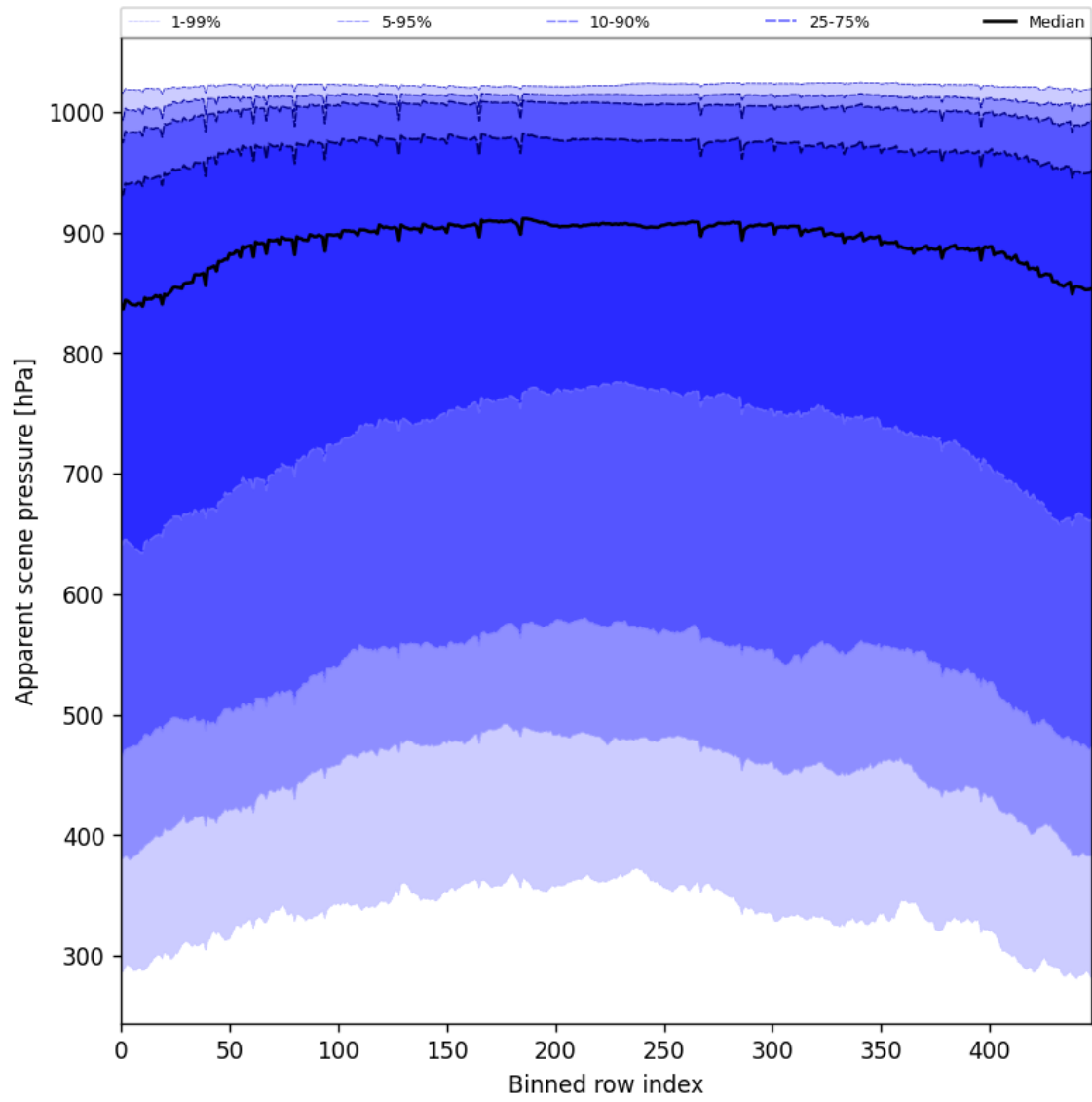
Figure 53: Along track statistics of “Apparent scene pressure” for 2025-07-13 to 2025-07-14
