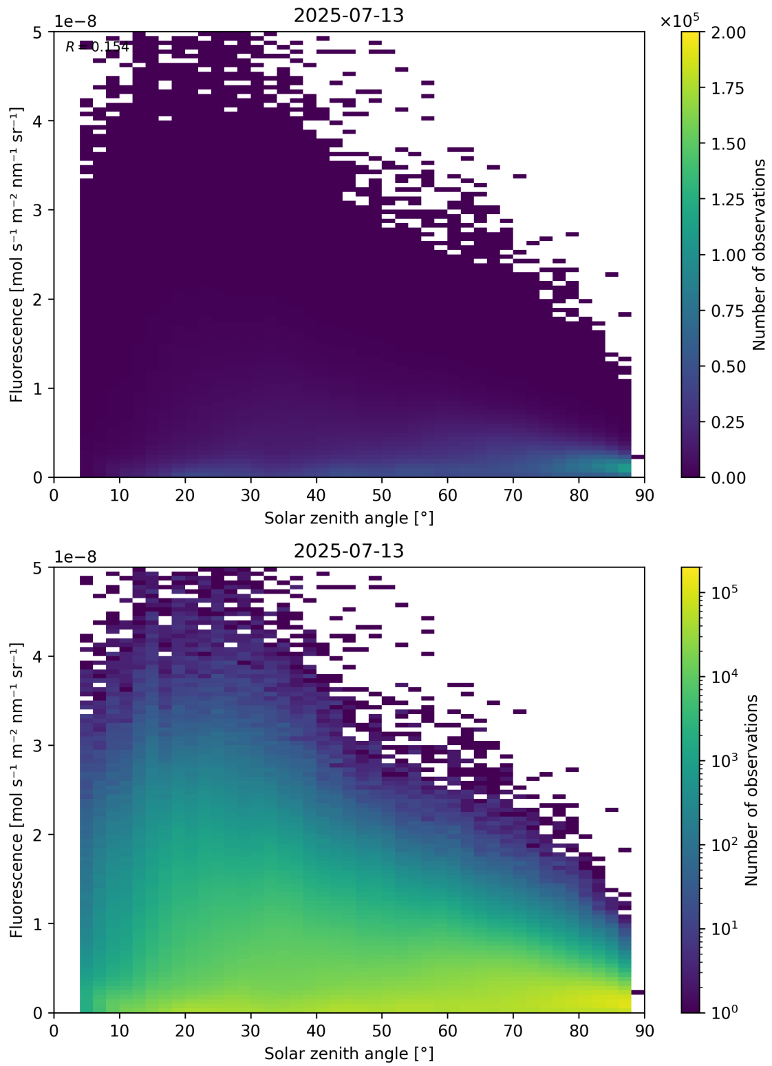
Figure 112: Scatter density plot of “Solar zenith angle” against “Fluorescence” for 2025-07-13 to 2025-07-14.
