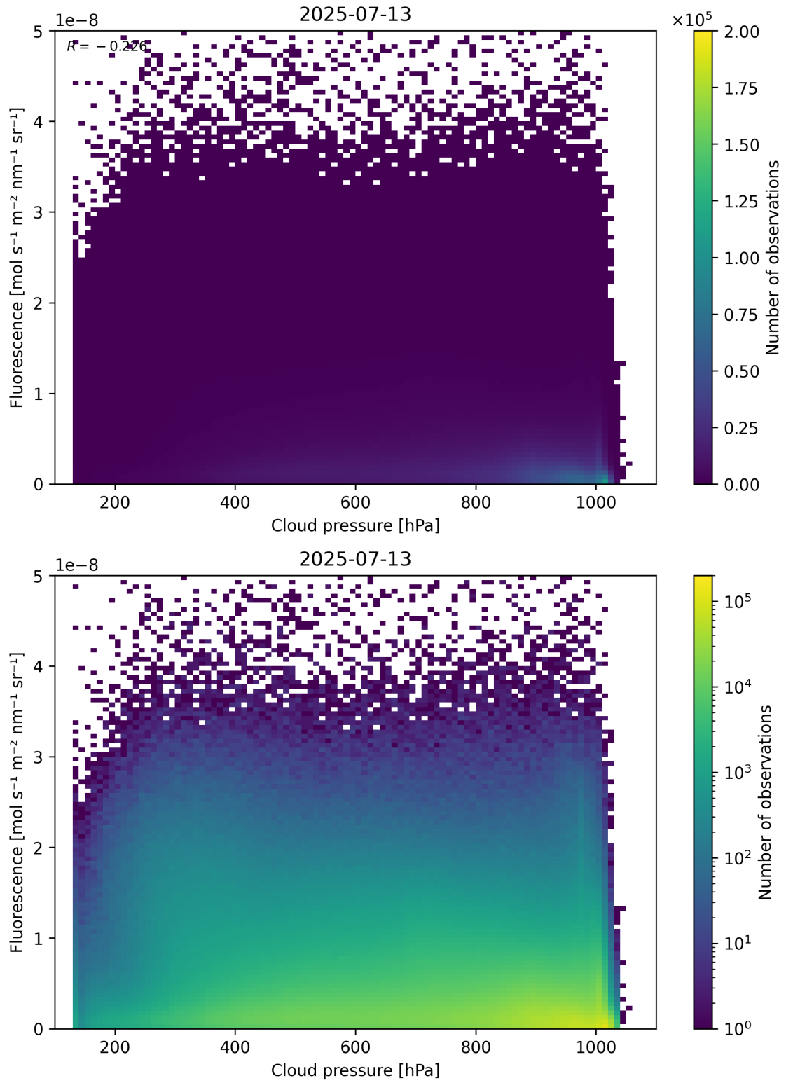
Figure 80: Scatter density plot of “Cloud pressure” against “Fluorescence” for 2025-07-13 to 2025-07-14.
