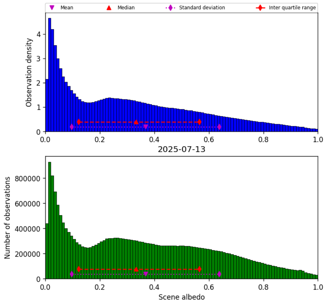
Figure 34: Histogram of “Scene albedo” for 2025-07-13 to 2025-07-14
