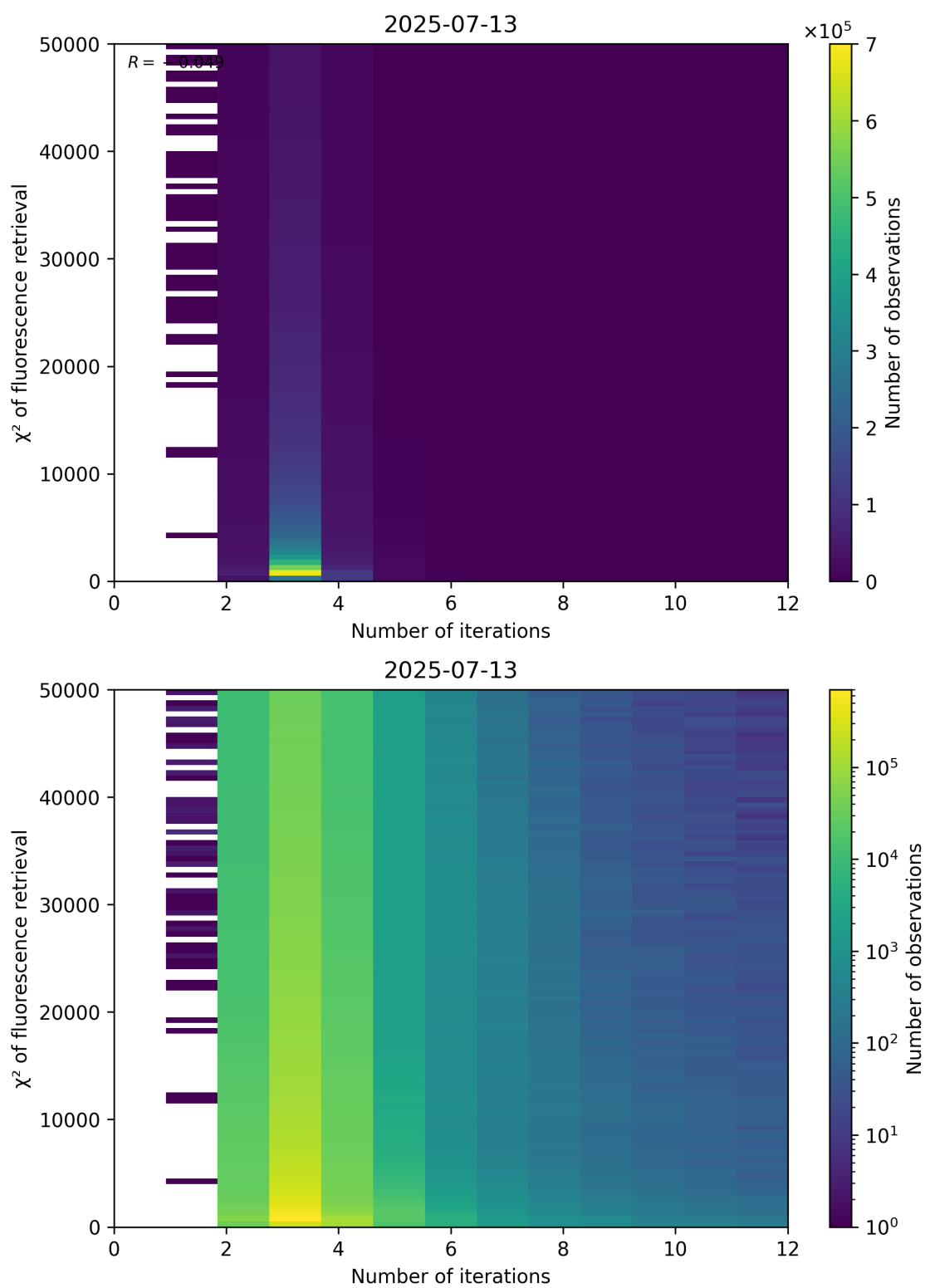
Figure 97: Scatter density plot of “Number of iterations” against “ \chi^2 of fluorescence retrieval” for 2025-07-13 to 2025-07-14.
