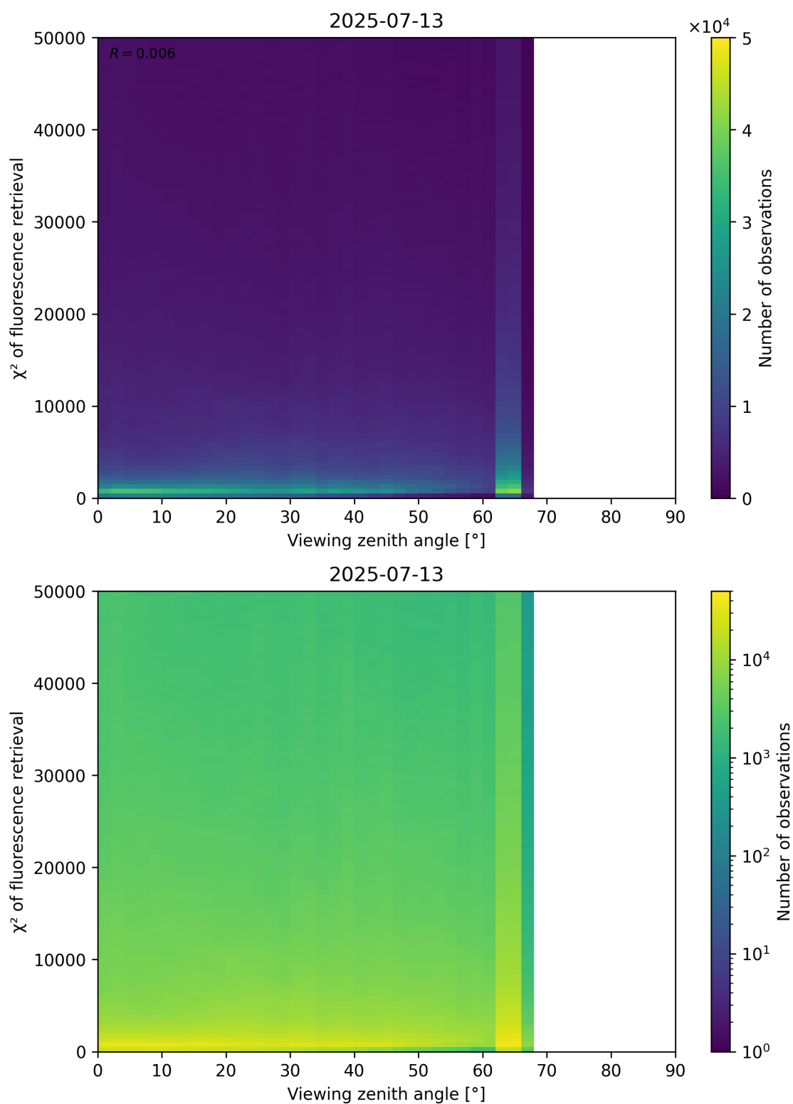
Figure 119: Scatter density plot of “Viewing zenith angle” against “ \chi^2 of fluorescence retrieval” for 2025-07-13 to 2025-07-14.
