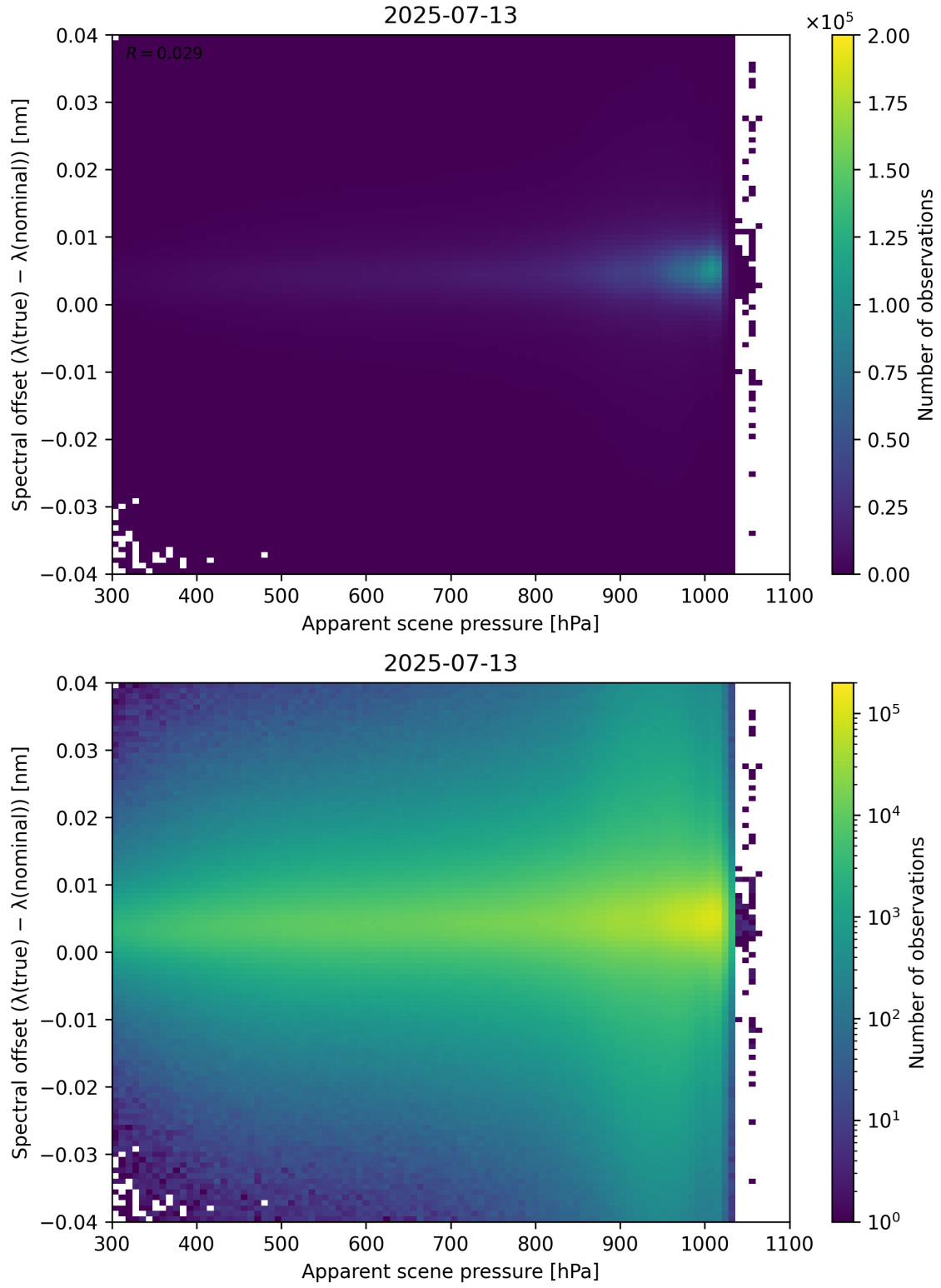
Figure 67: Scatter density plot of “Apparent scene pressure” against “Spectral offset ( \lambda_{\text{true}} - \lambda_{\text{nominal}} )” for 2025-07-13 to 2025-07-14.
