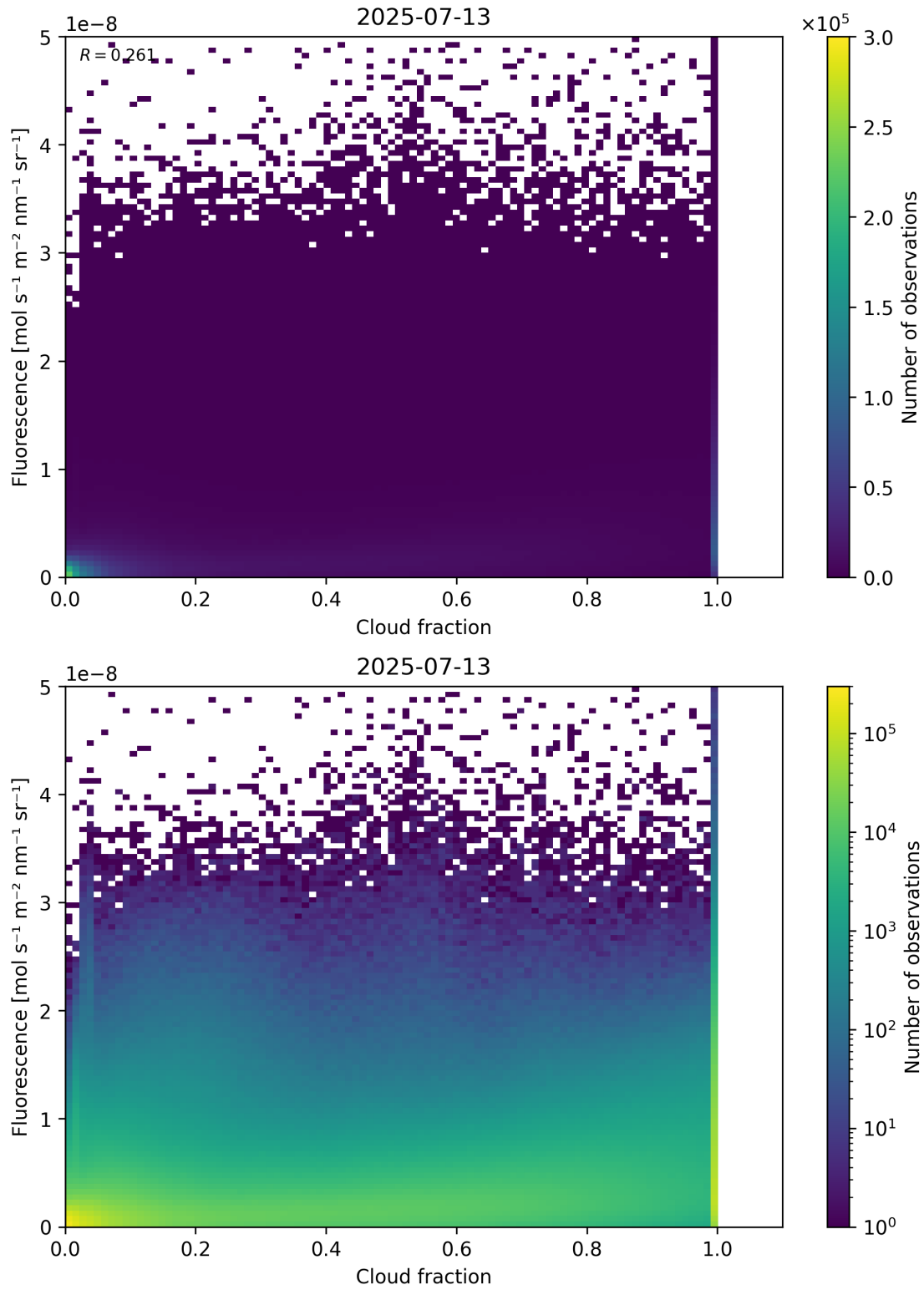
Figure 72: Scatter density plot of “Cloud fraction” against “Fluorescence” for 2025-07-13 to 2025-07-14.
