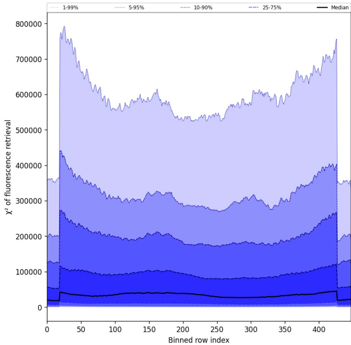
Figure 59: Along track statistics of “ \chi^2 of fluorescence retrieval” for 2025-07-13 to 2025-07-14
