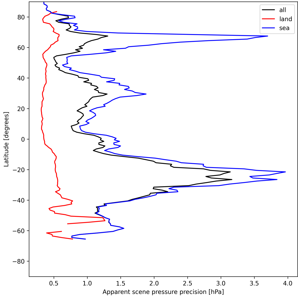
Figure 20: Zonal average of “Apparent scene pressure precision” for 2025-07-13 to 2025-07-14.
