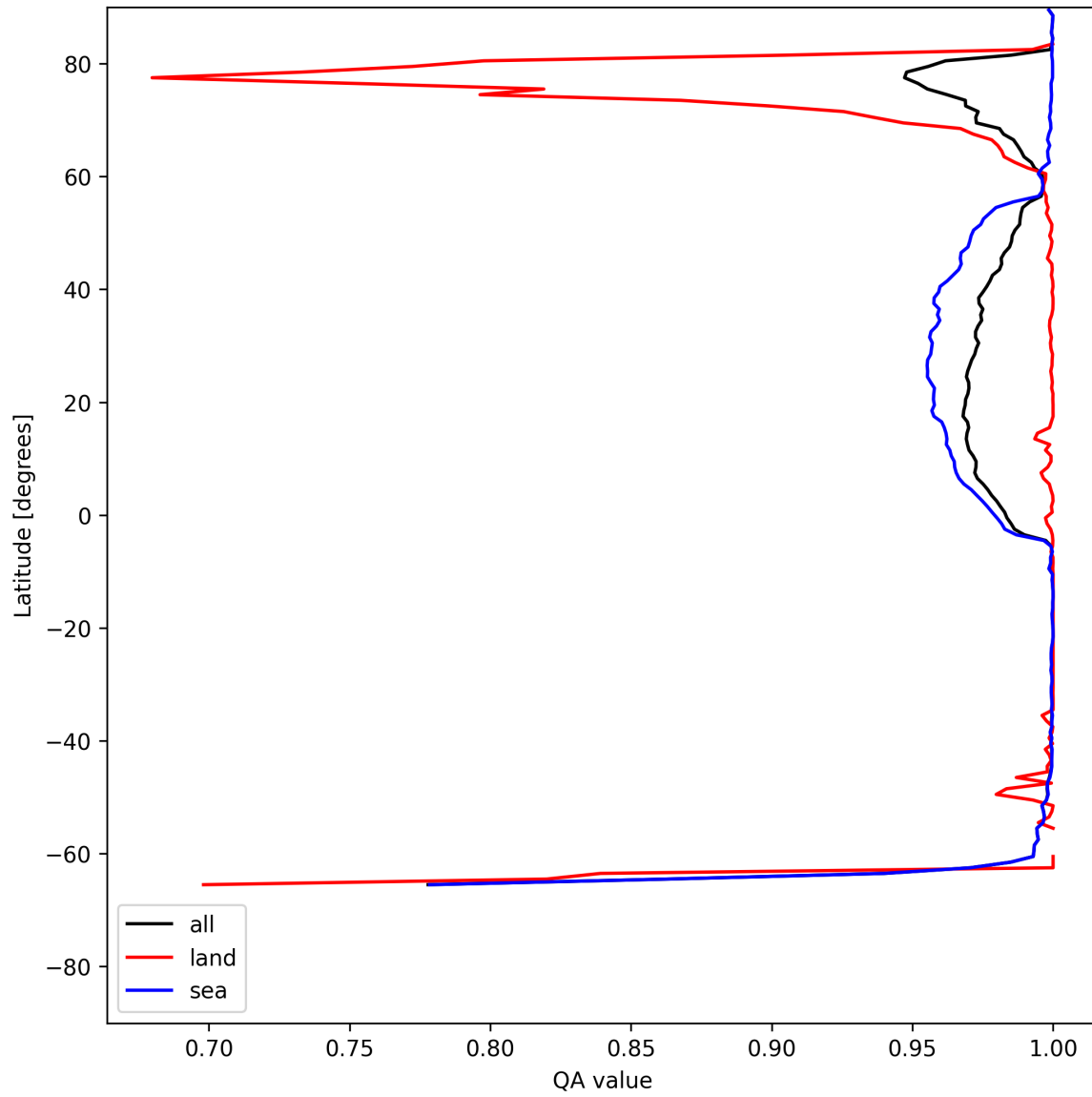
Figure 12: Zonal average of “QA value” for 2025-07-13 to 2025-07-14.
