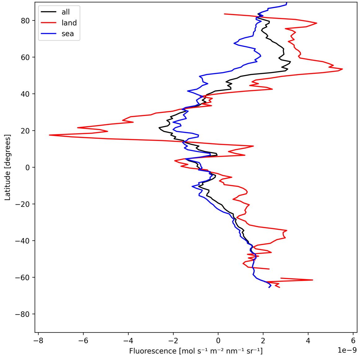
Figure 23: Zonal average of “Fluorescence” for 2025-07-13 to 2025-07-14.
