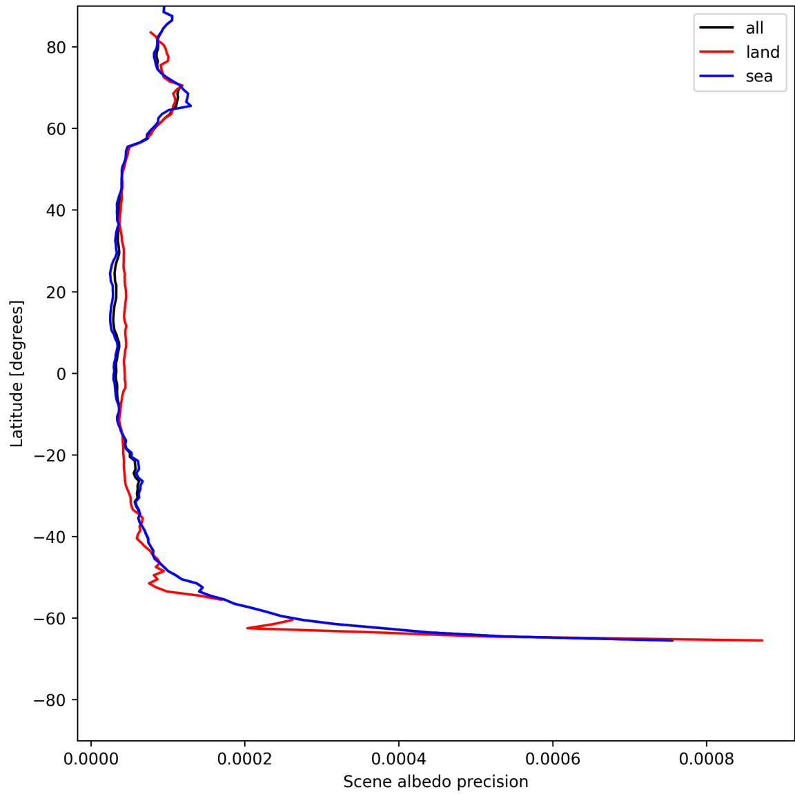
Figure 18: Zonal average of “Scene albedo precision” for 2025-07-13 to 2025-07-14.
