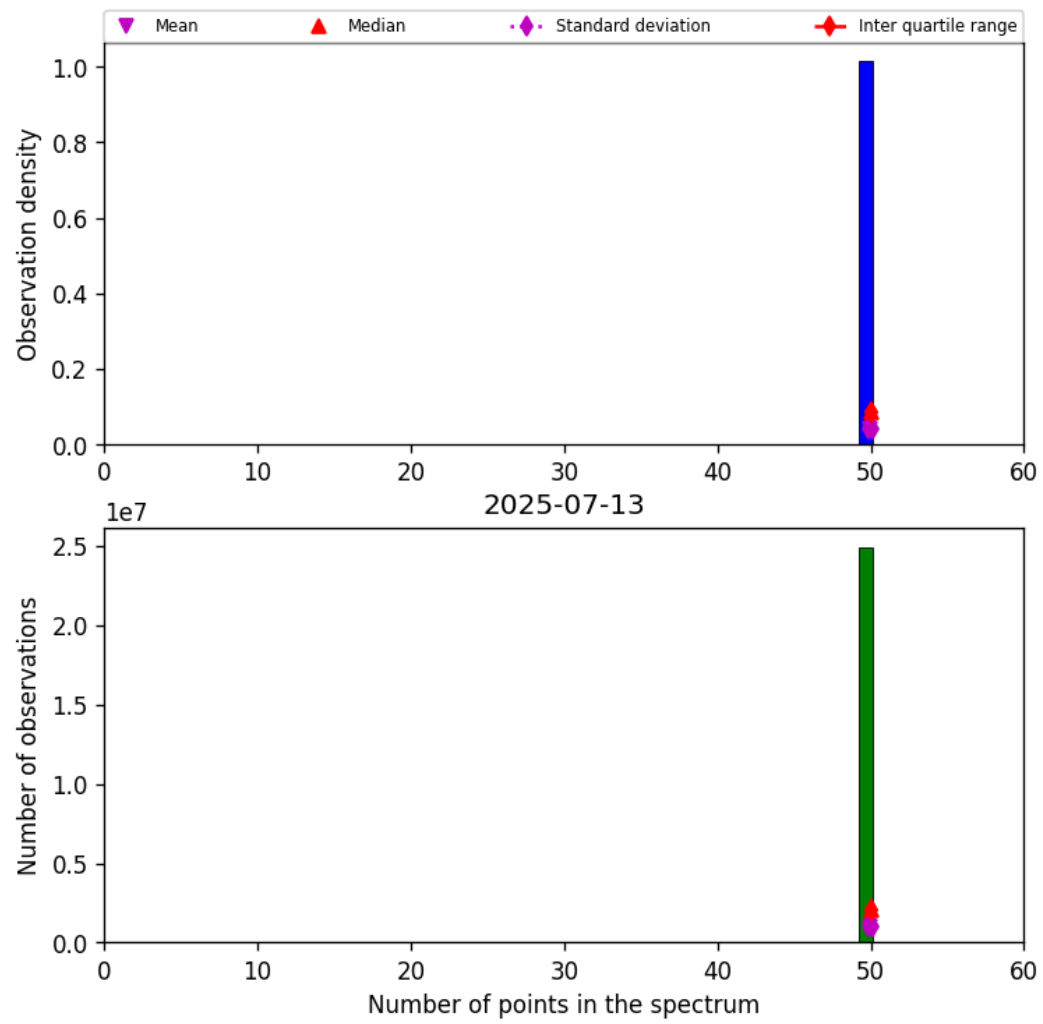
Figure 44: Histogram of “Number of points in the spectrum” for 2025-07-13 to 2025-07-14
