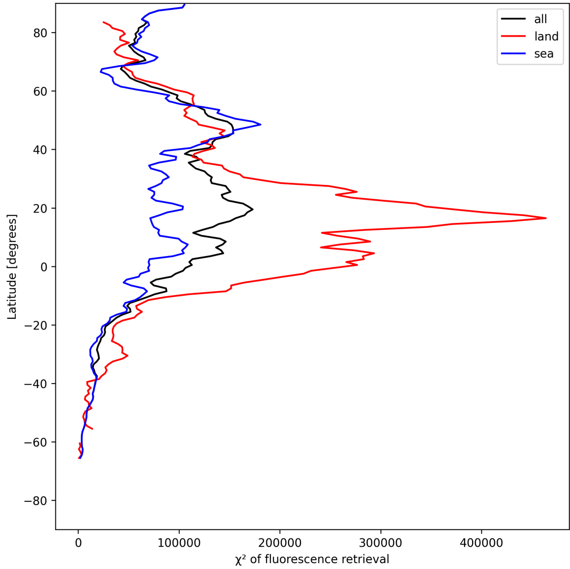
Figure 25: Zonal average of “ \chi^2 of fluorescence retrieval” for 2025-07-13 to 2025-07-14.
