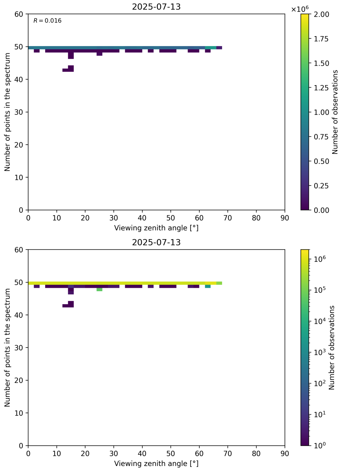
Figure 125: Scatter density plot of “Viewing zenith angle” against “Number of points in the spectrum” for 2025-07-13 to 2025-07-14.
