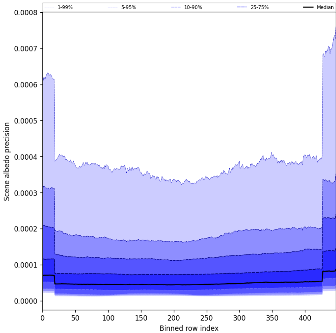
Figure 52: Along track statistics of “Scene albedo precision” for 2025-07-13 to 2025-07-14
