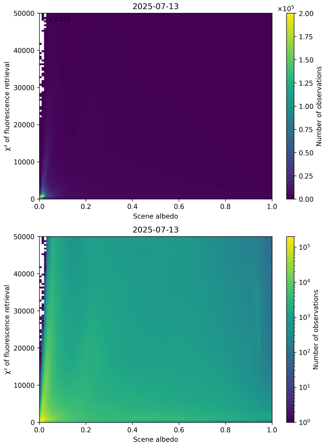
Figure 103: Scatter density plot of “Scene albedo” against “ \chi^2 of fluorescence retrieval” for 2025-07-13 to 2025-07-14.
