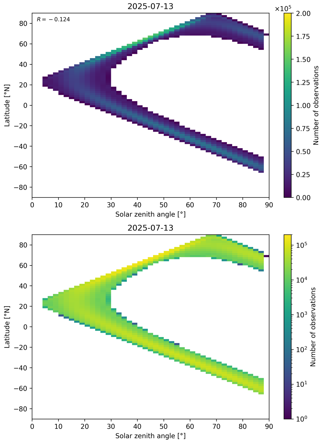
Figure 113: Scatter density plot of “Solar zenith angle” against “Latitude” for 2025-07-13 to 2025-07-14.
