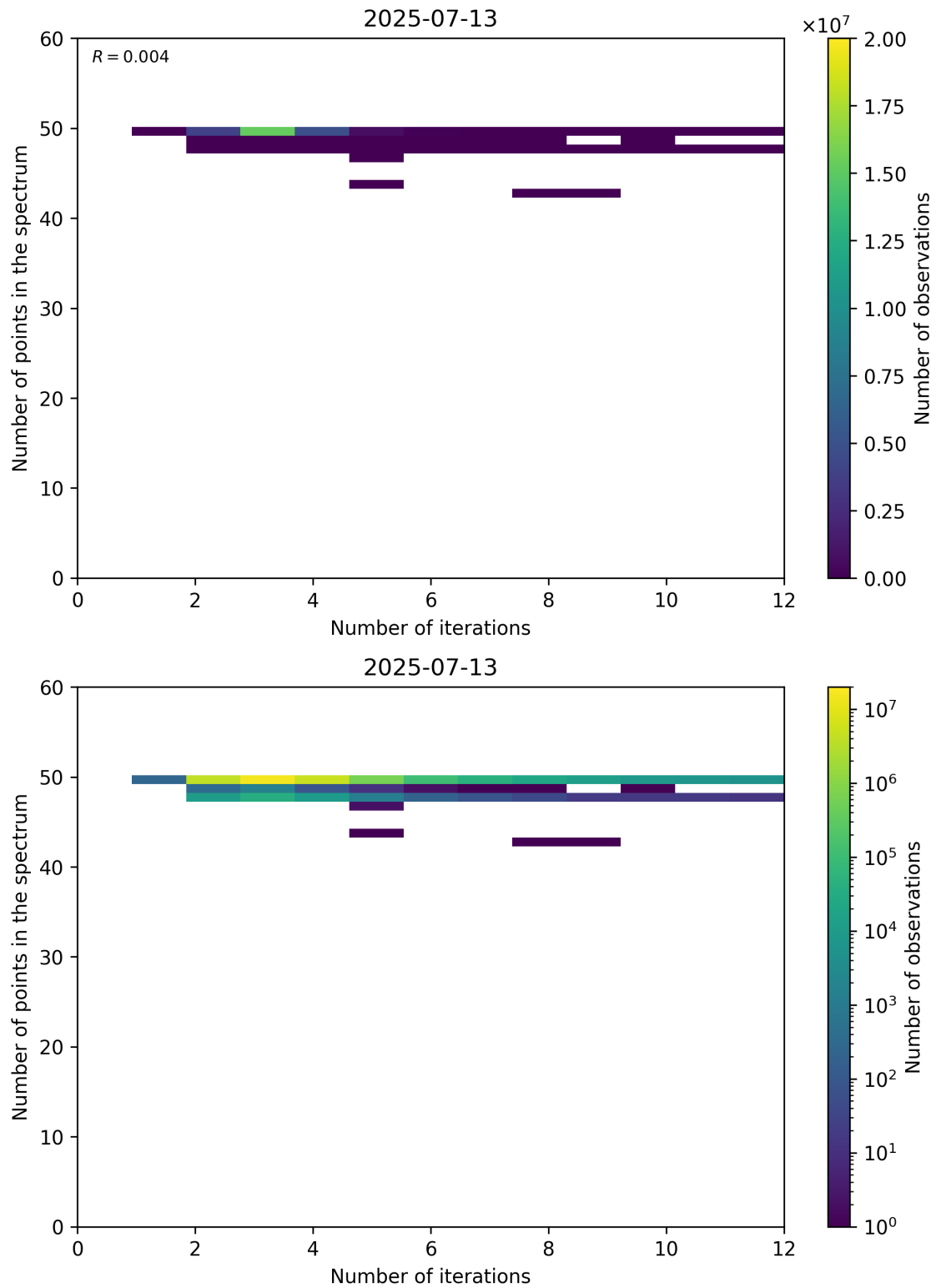
Figure 99: Scatter density plot of “Number of iterations” against “Number of points in the spectrum” for 2025-07-13 to 2025-07-14.
