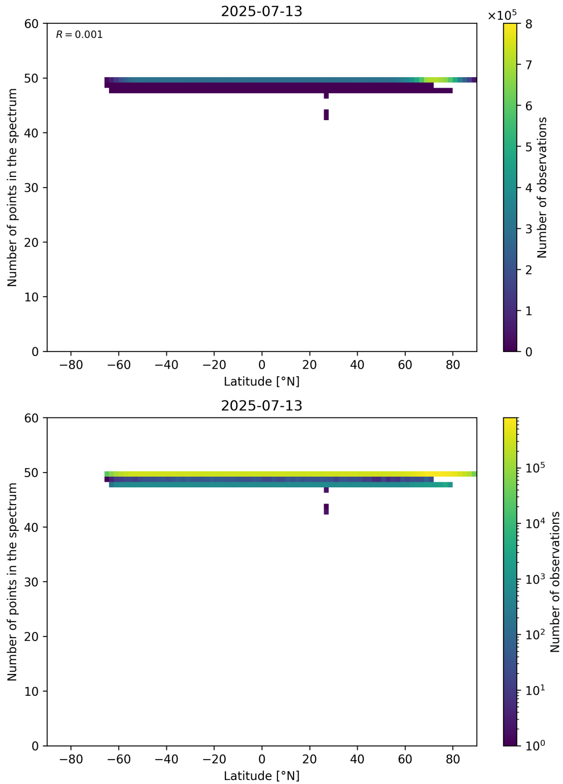
Figure 94: Scatter density plot of “Latitude” against “Number of points in the spectrum” for 2025-07-13 to 2025-07-14.
