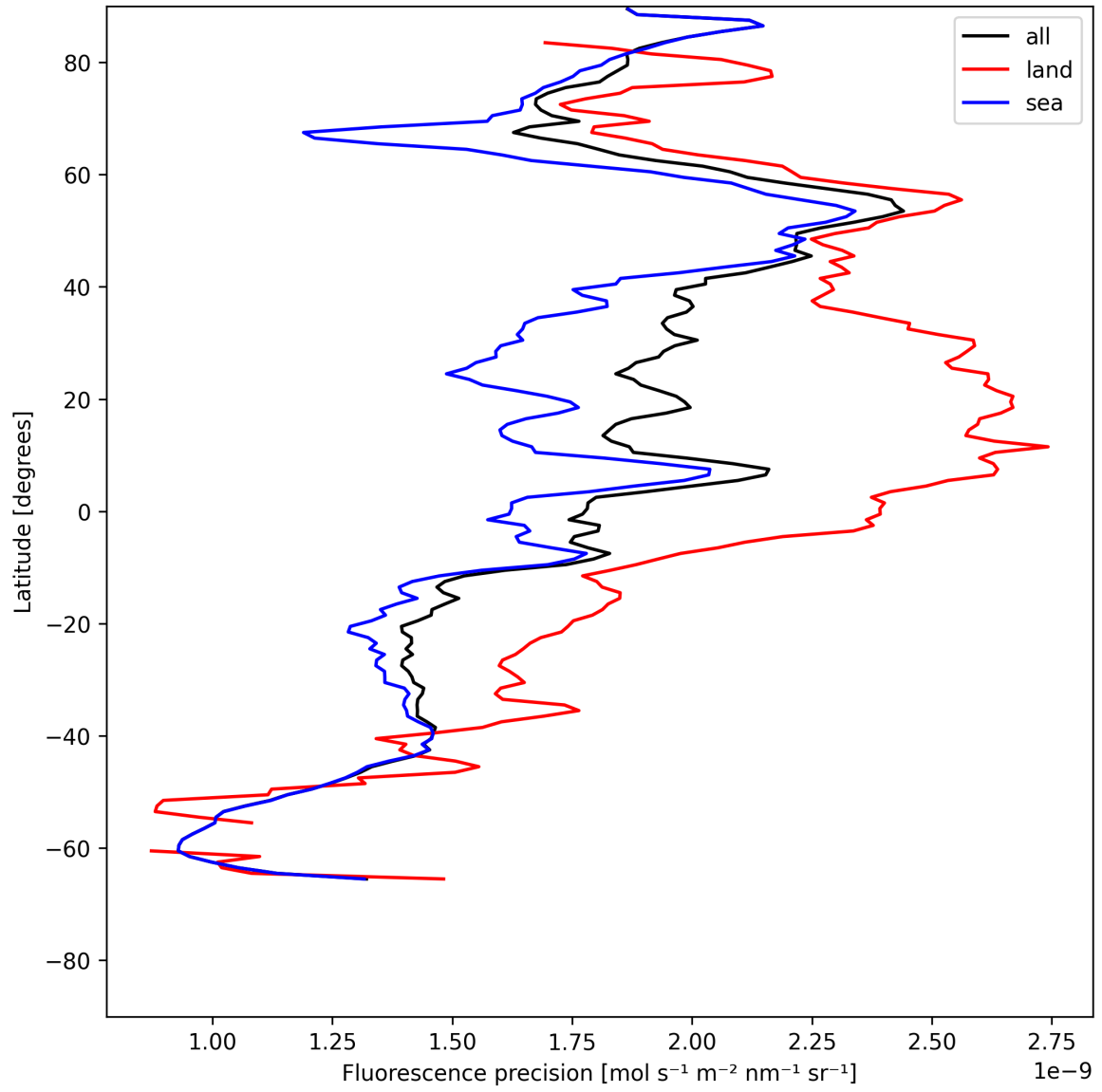
Figure 24: Zonal average of “Fluorescence precision” for 2025-07-13 to 2025-07-14.
