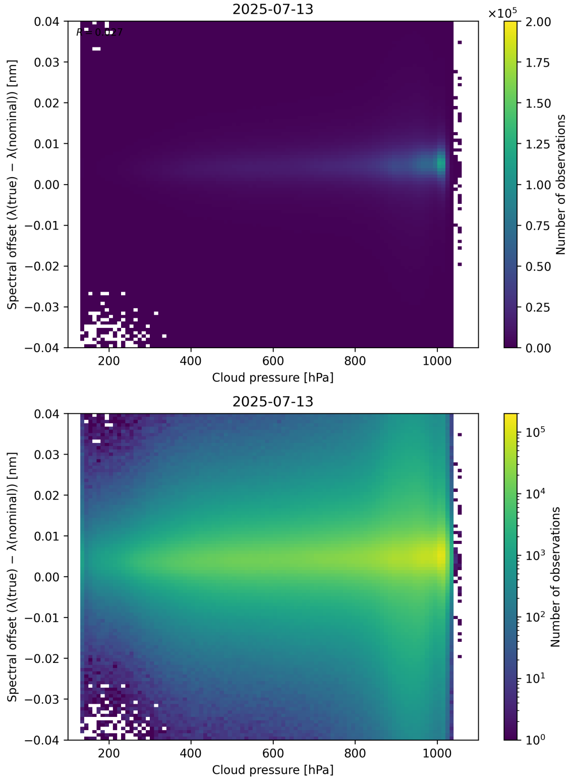
Figure 84: Scatter density plot of “Cloud pressure” against “Spectral offset ( \lambda_{\text{true}} - \lambda_{\text{nominal}} )” for 2025-07-13 to 2025-07-14.
