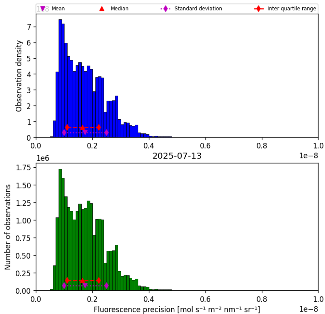
Figure 41: Histogram of “Fluorescence precision” for 2025-07-13 to 2025-07-14
