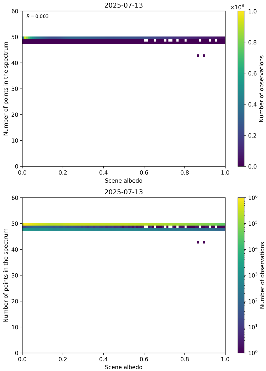
Figure 106: Scatter density plot of “Scene albedo” against “Number of points in the spectrum” for 2025-07-13 to 2025-07-14.
