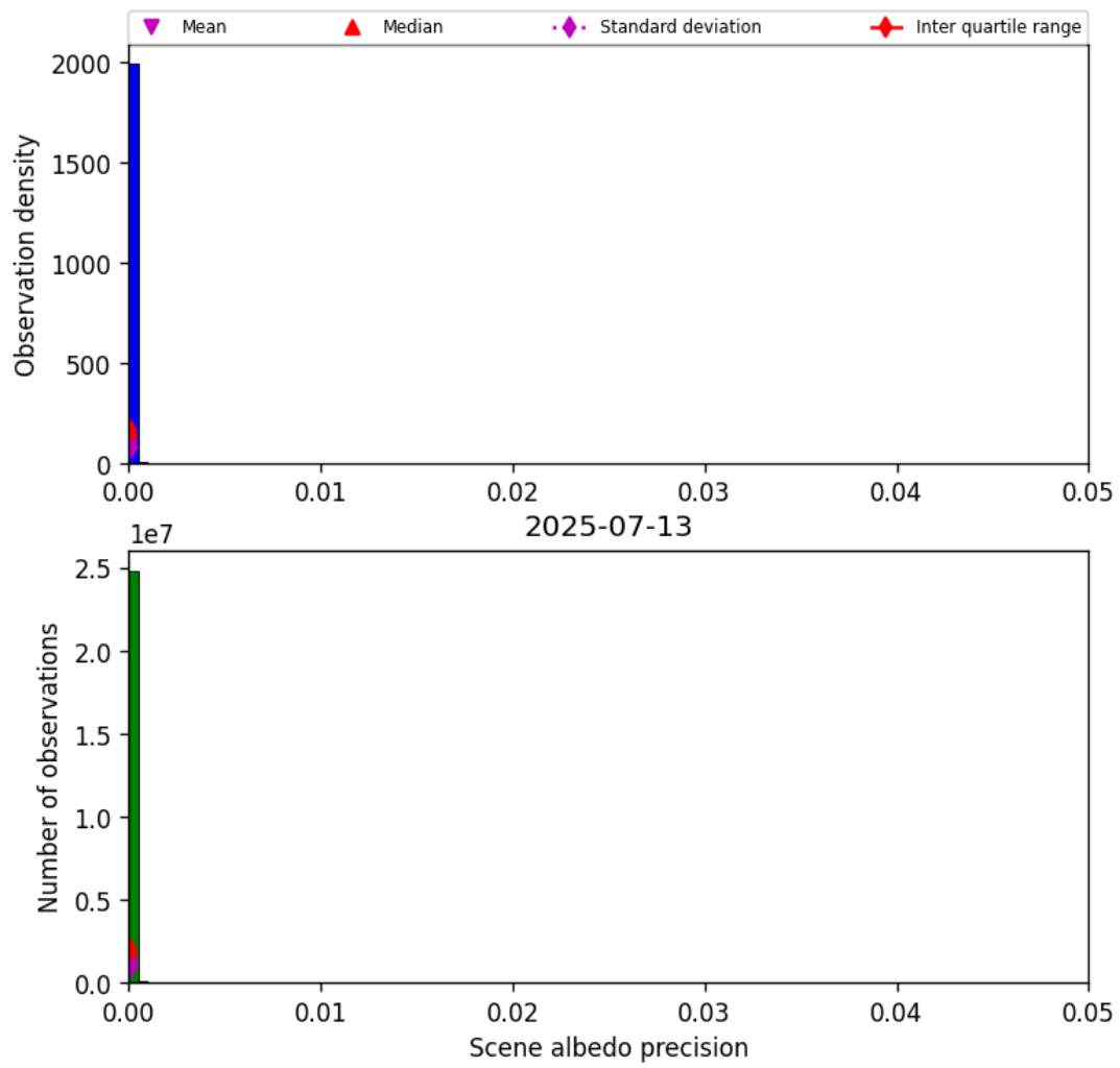
Figure 35: Histogram of “Scene albedo precision” for 2025-07-13 to 2025-07-14
