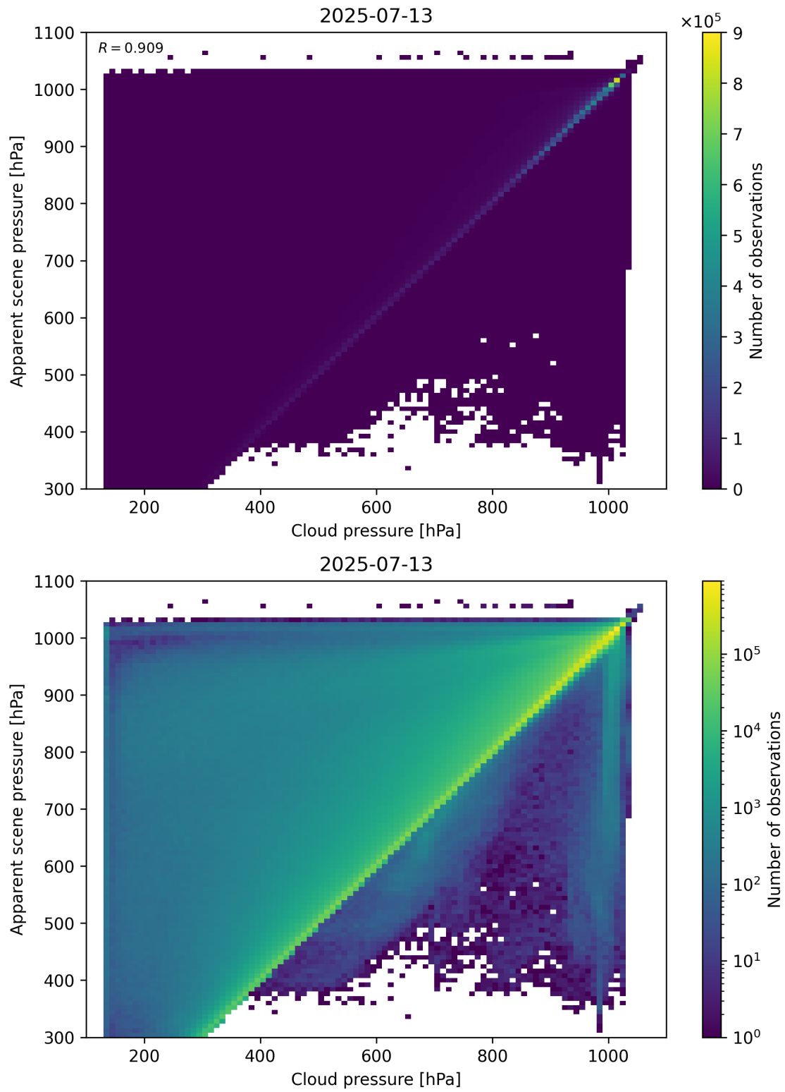
Figure 77: Scatter density plot of “Cloud pressure” against “Apparent scene pressure” for 2025-07-13 to 2025-07-14.
