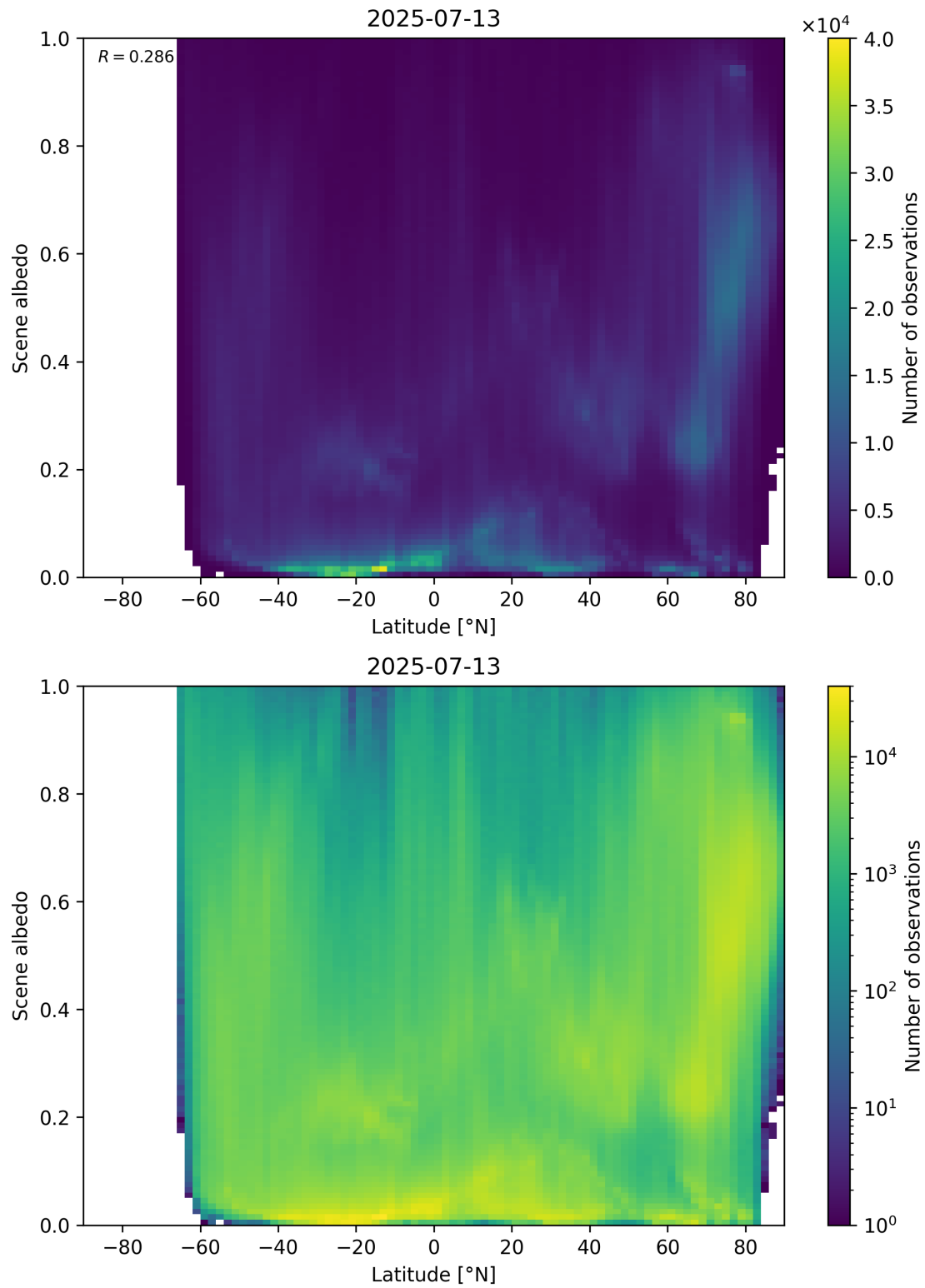
Figure 95: Scatter density plot of “Latitude” against “Scene albedo” for 2025-07-13 to 2025-07-14.
