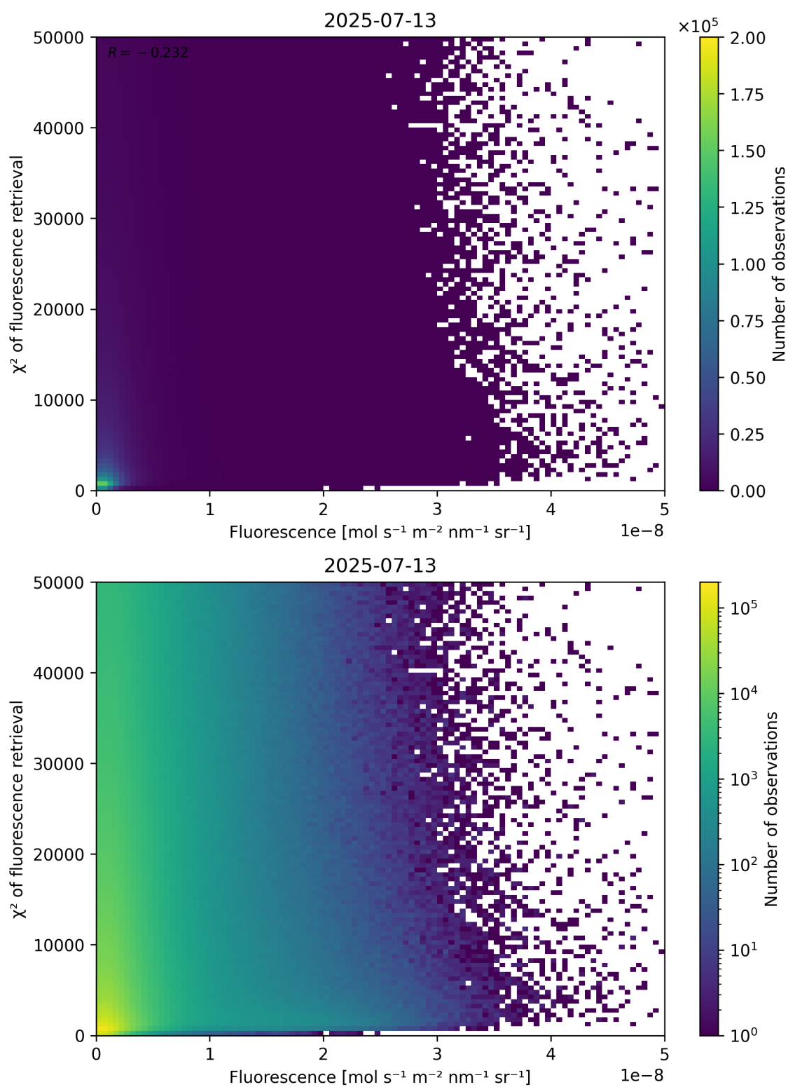
Figure 85: Scatter density plot of “Fluorescence” against “ \chi^2 of fluorescence retrieval” for 2025-07-13 to 2025-07-14.
