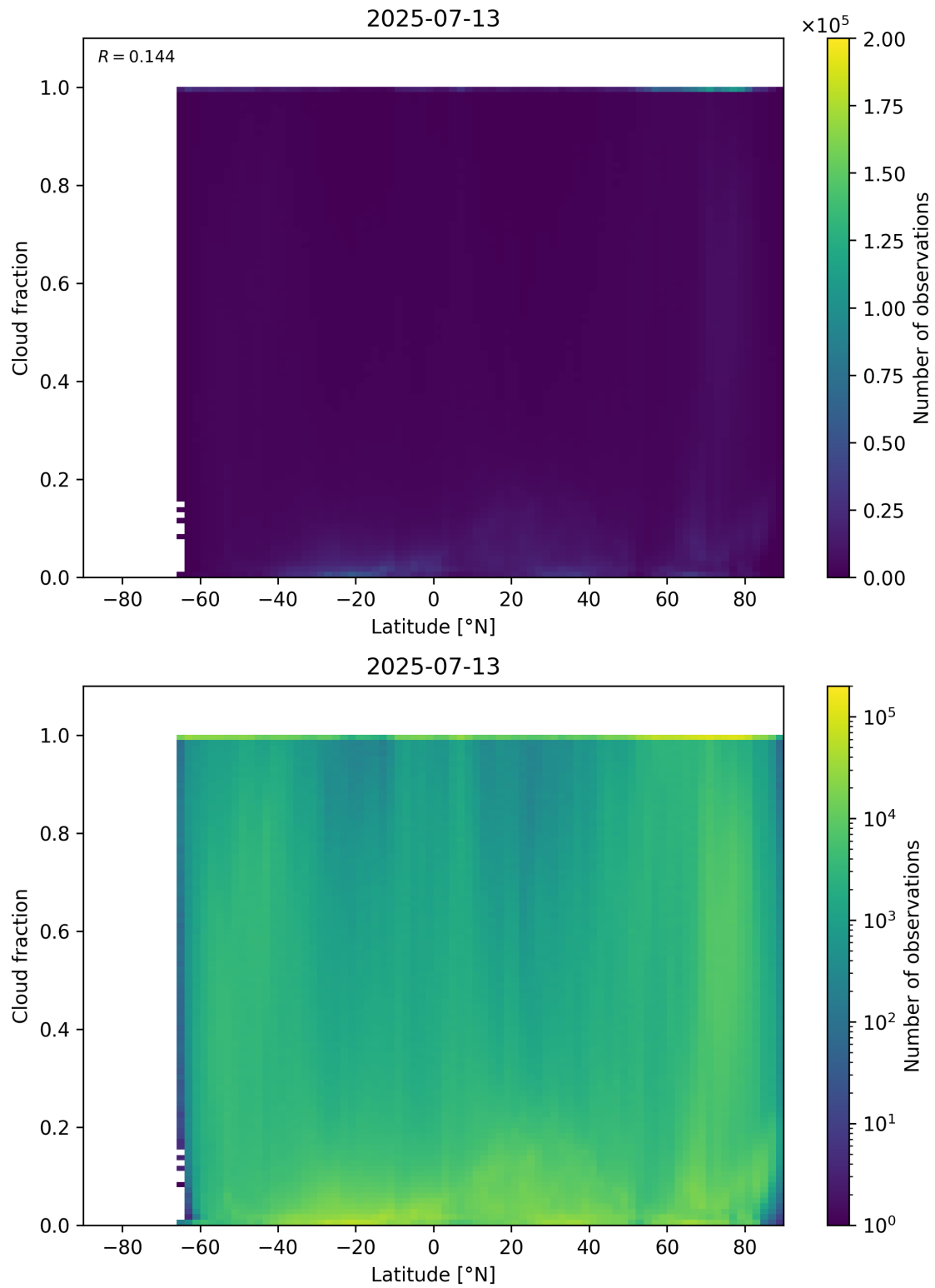
Figure 90: Scatter density plot of “Latitude” against “Cloud fraction” for 2025-07-13 to 2025-07-14.
