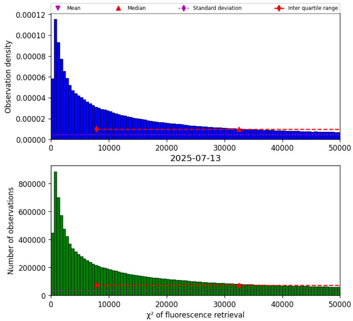
Figure 42: Histogram of “ \chi^2 of fluorescence retrieval” for 2025-07-13 to 2025-07-14
