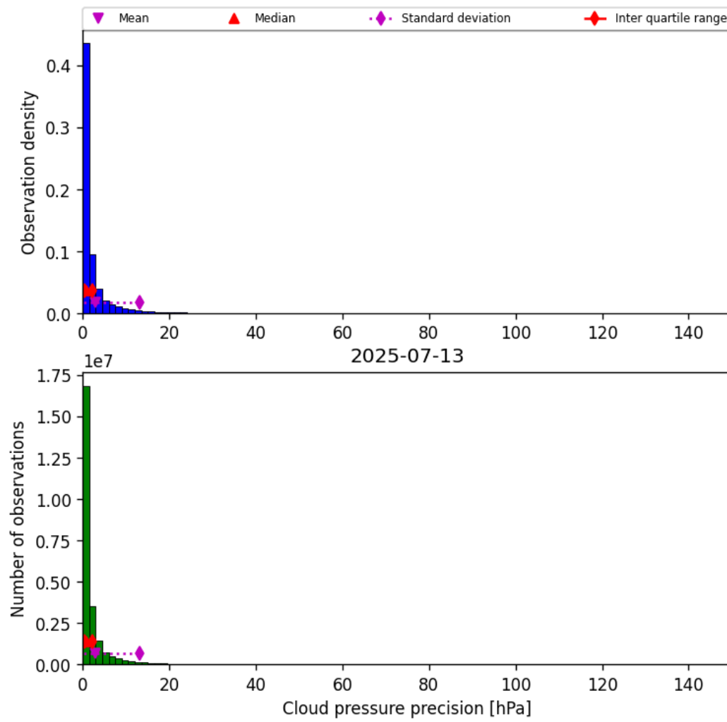
Figure 31: Histogram of “Cloud pressure precision” for 2025-07-13 to 2025-07-14
