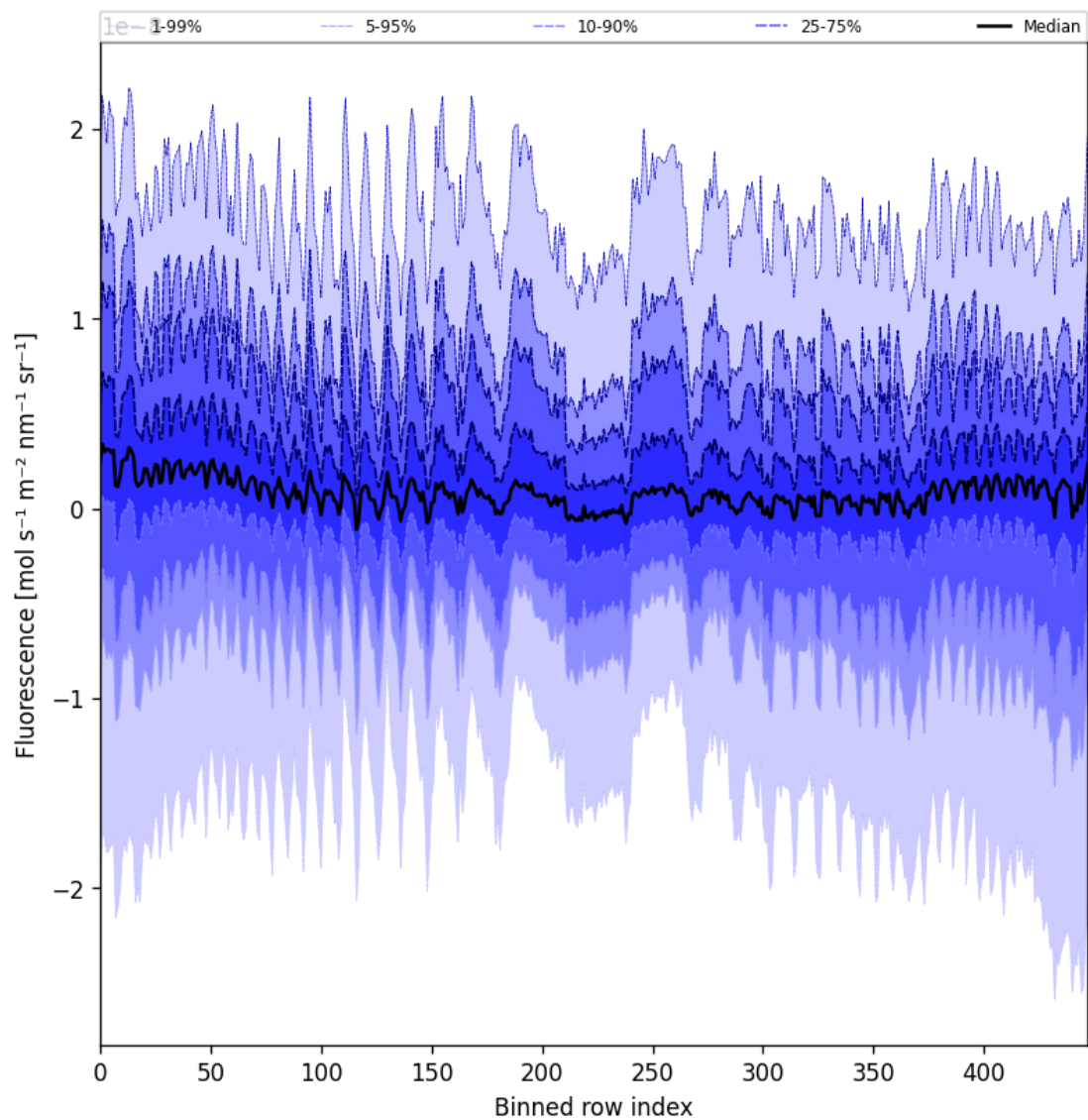
Figure 57: Along track statistics of “Fluorescence” for 2025-07-13 to 2025-07-14
