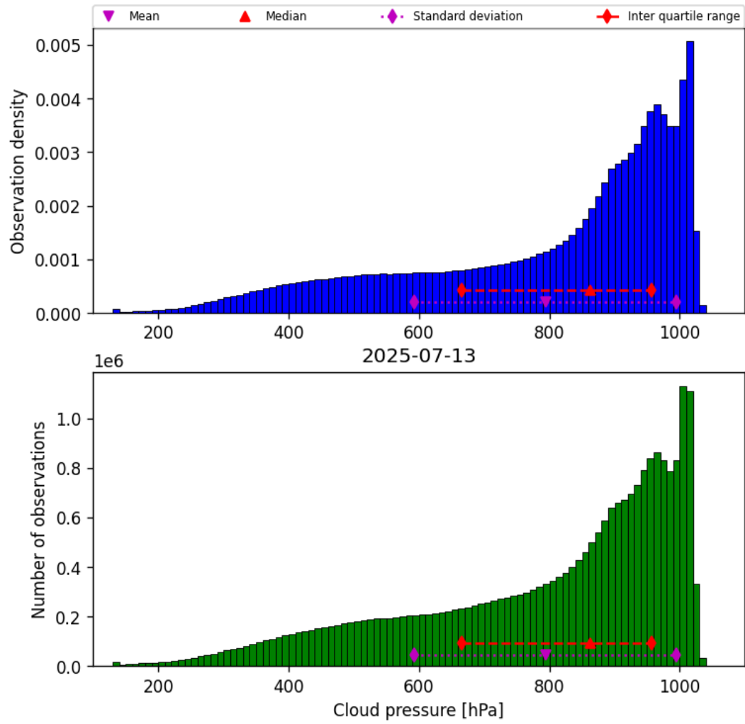
Figure 30: Histogram of “Cloud pressure” for 2025-07-13 to 2025-07-14
