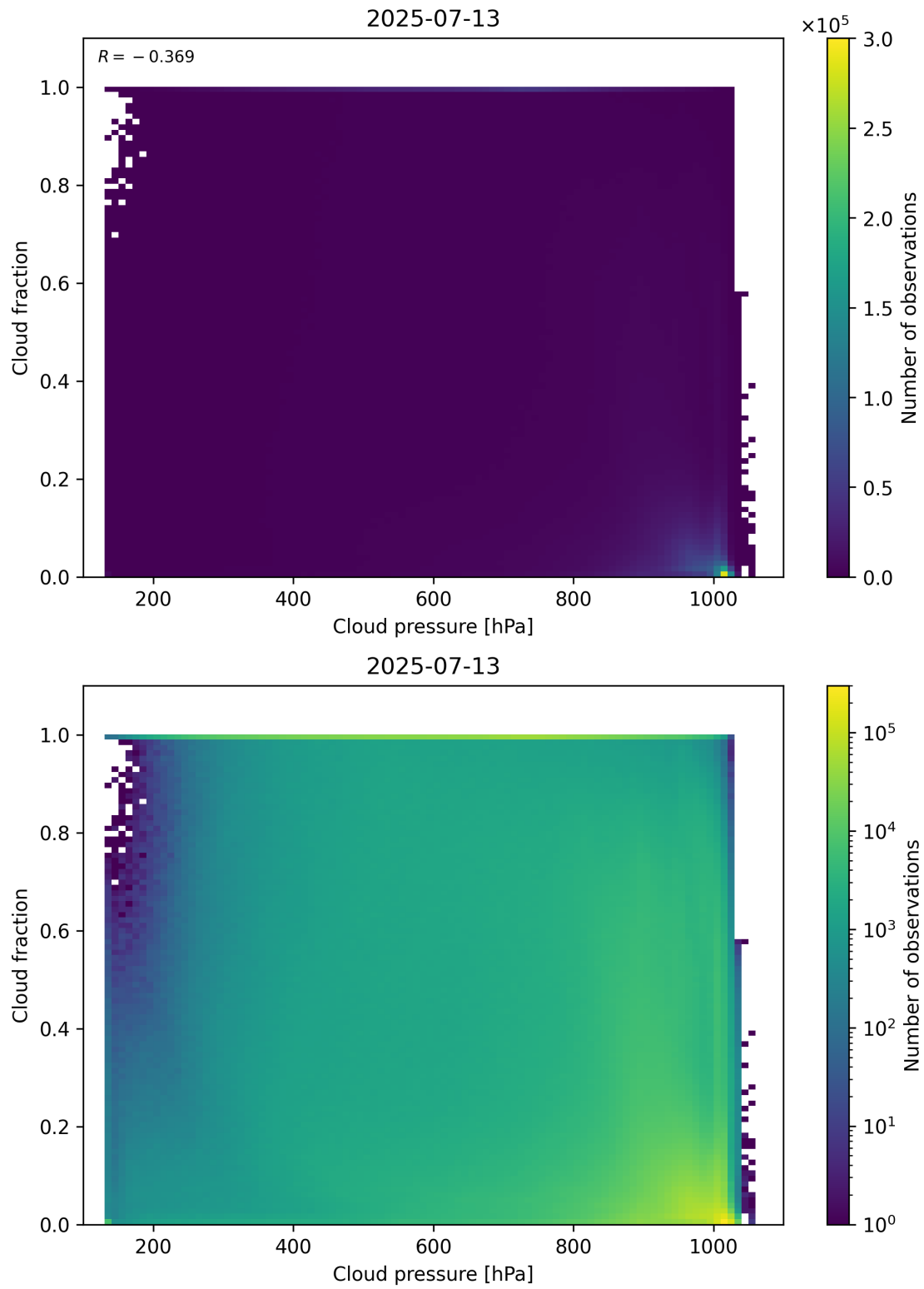
Figure 79: Scatter density plot of “Cloud pressure” against “Cloud fraction” for 2025-07-13 to 2025-07-14.
