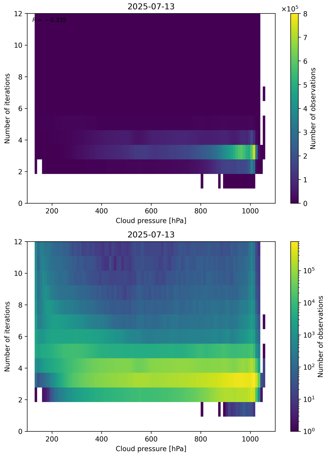
Figure 81: Scatter density plot of “Cloud pressure” against “Number of iterations” for 2025-07-13 to 2025-07-14.
