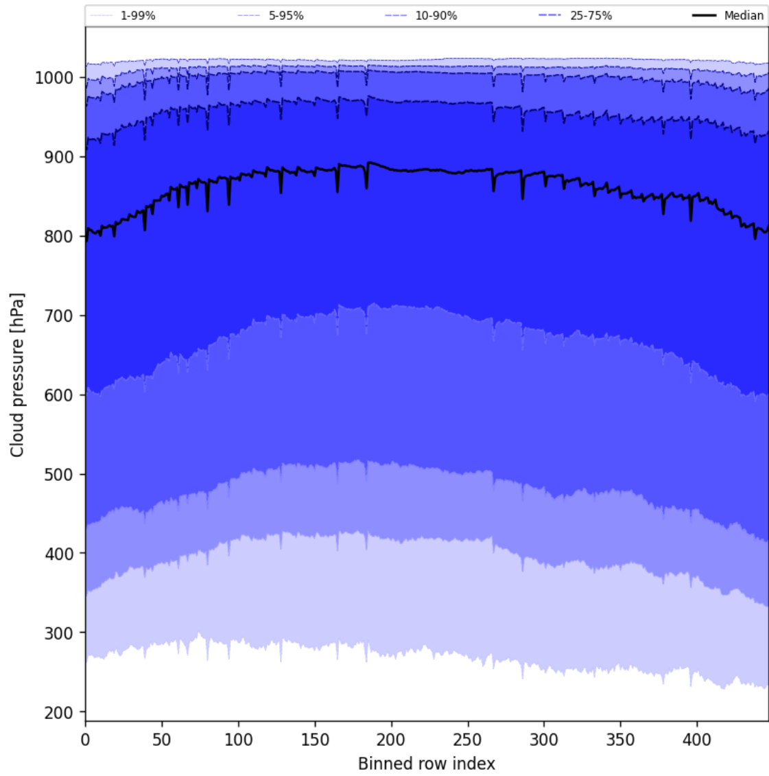
Figure 47: Along track statistics of “Cloud pressure” for 2025-07-13 to 2025-07-14
