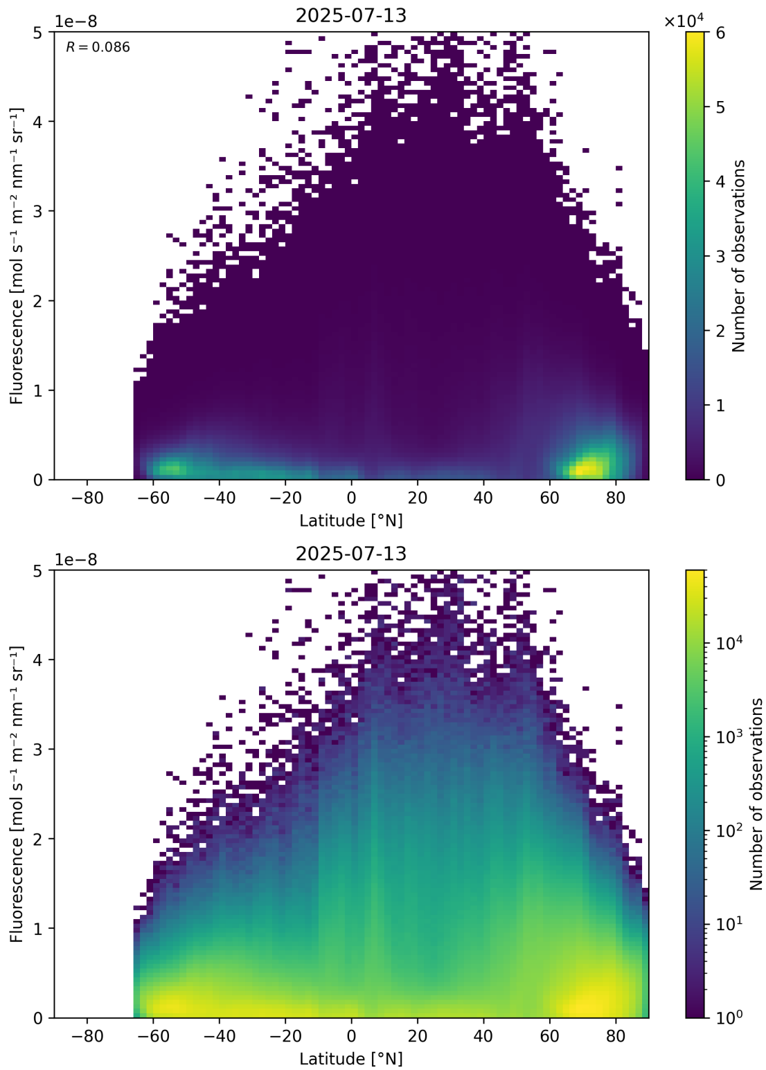
Figure 92: Scatter density plot of “Latitude” against “Fluorescence” for 2025-07-13 to 2025-07-14.
