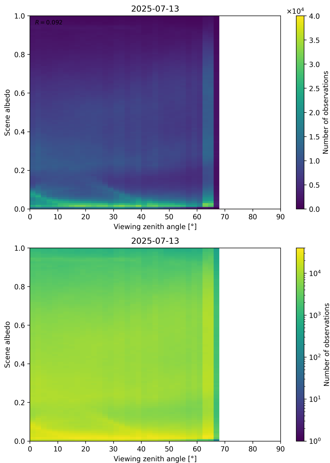
Figure 126: Scatter density plot of “Viewing zenith angle” against “Scene albedo” for 2025-07-13 to 2025-07-14.
