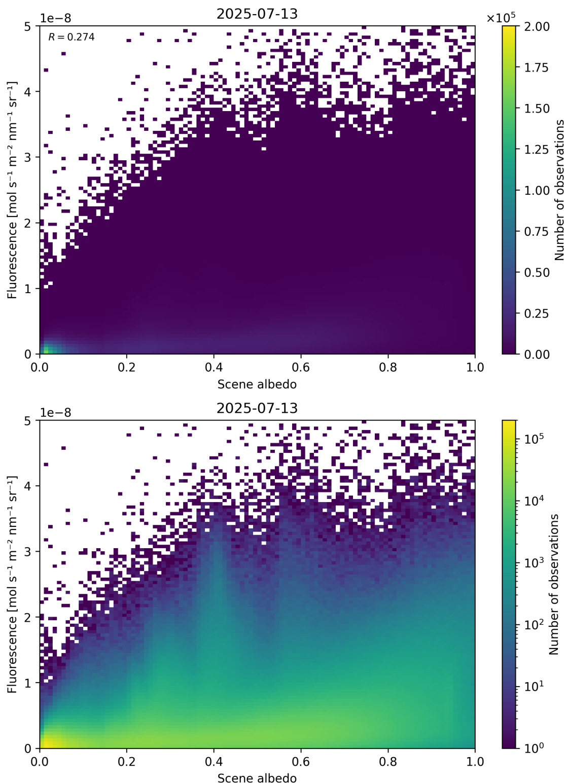
Figure 104: Scatter density plot of “Scene albedo” against “Fluorescence” for 2025-07-13 to 2025-07-14.
