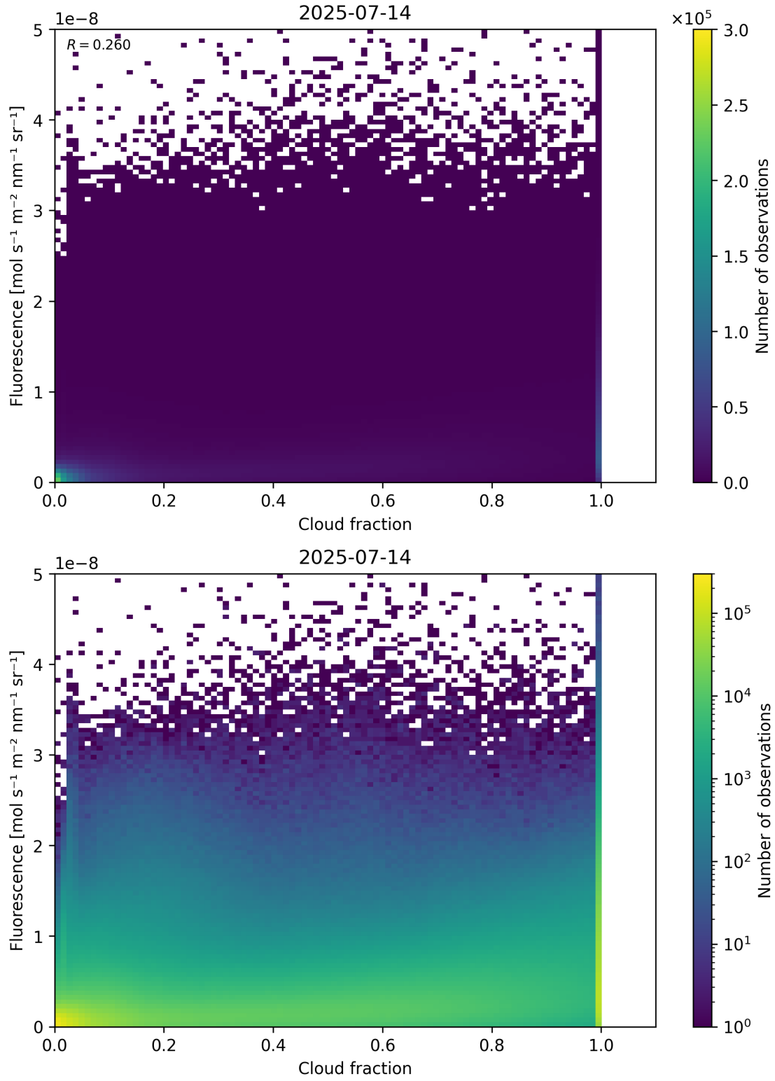
Figure 72: Scatter density plot of “Cloud fraction” against “Fluorescence” for 2025-07-13 to 2025-07-15.
