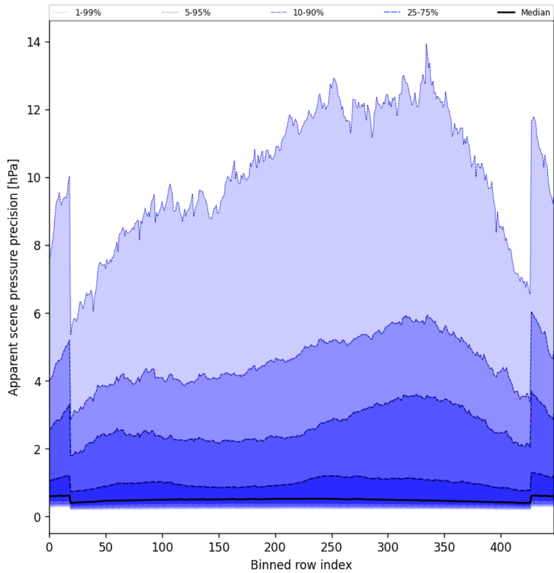
Figure 54: Along track statistics of “Apparent scene pressure precision” for 2025-07-13 to 2025-07-15
