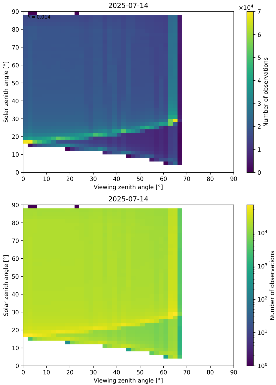
Figure 127: Scatter density plot of “Viewing zenith angle” against “Solar zenith angle” for 2025-07-13 to 2025-07-15.
