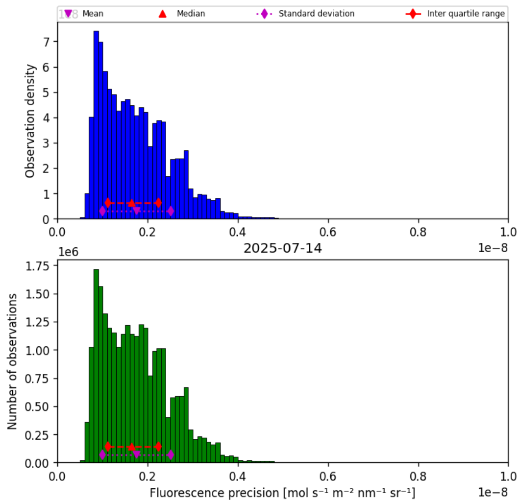
Figure 41: Histogram of “Fluorescence precision” for 2025-07-13 to 2025-07-15
