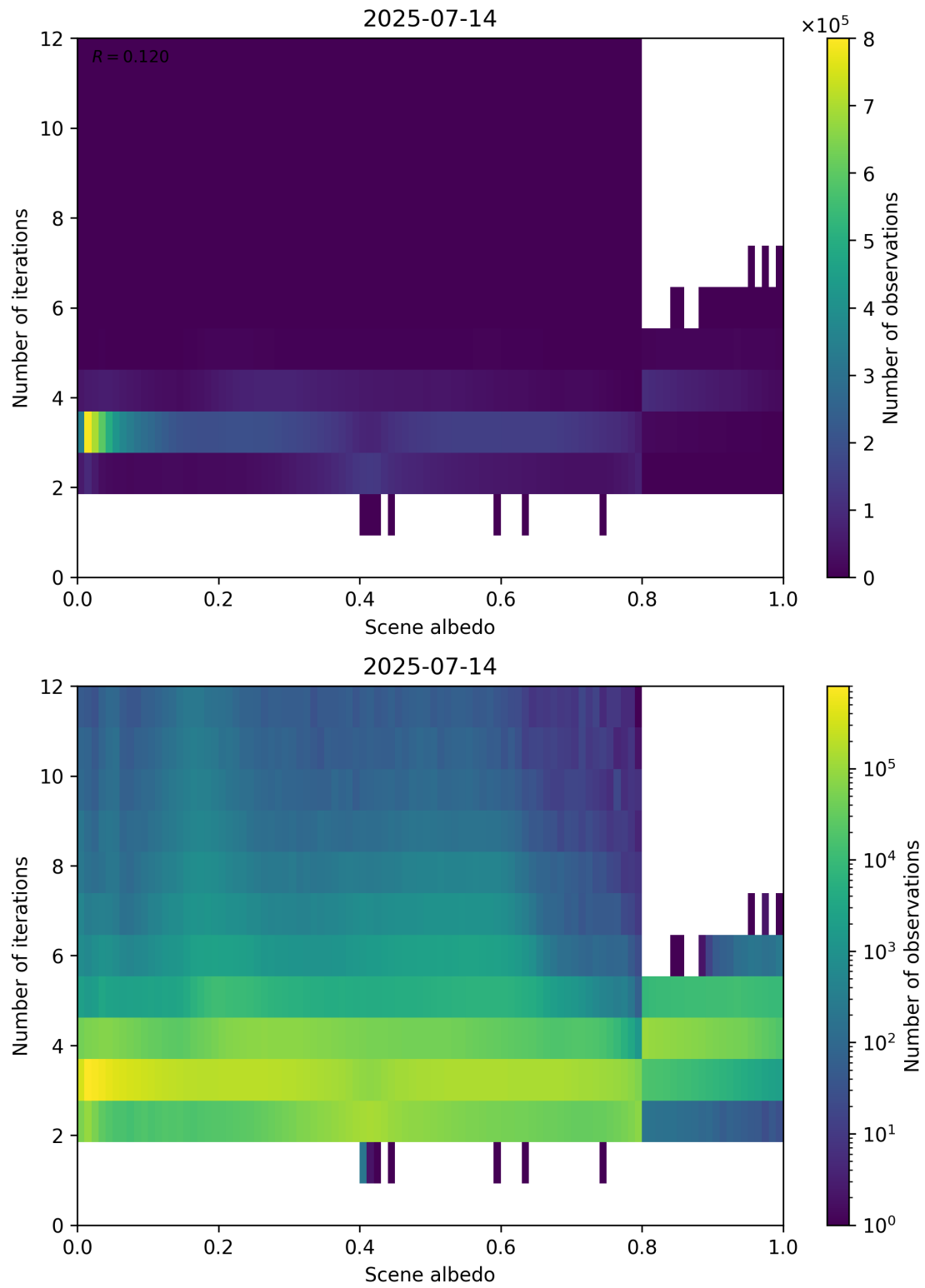
Figure 105: Scatter density plot of “Scene albedo” against “Number of iterations” for 2025-07-13 to 2025-07-15.
