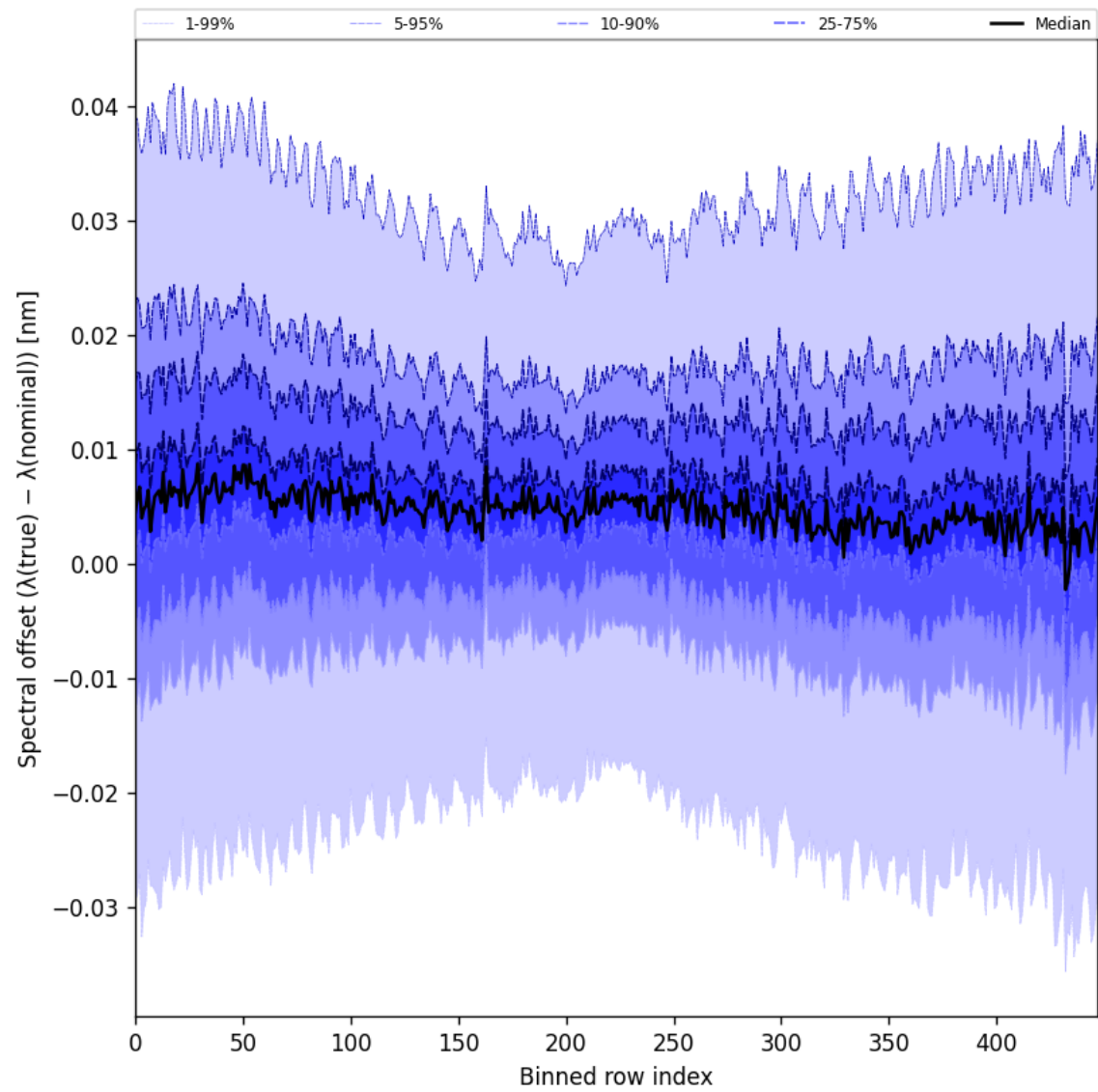
Figure 62: Along track statistics of “Spectral offset ( \lambda_{\text{true}} - \lambda_{\text{nominal}} )” for 2025-07-13 to 2025-07-15
