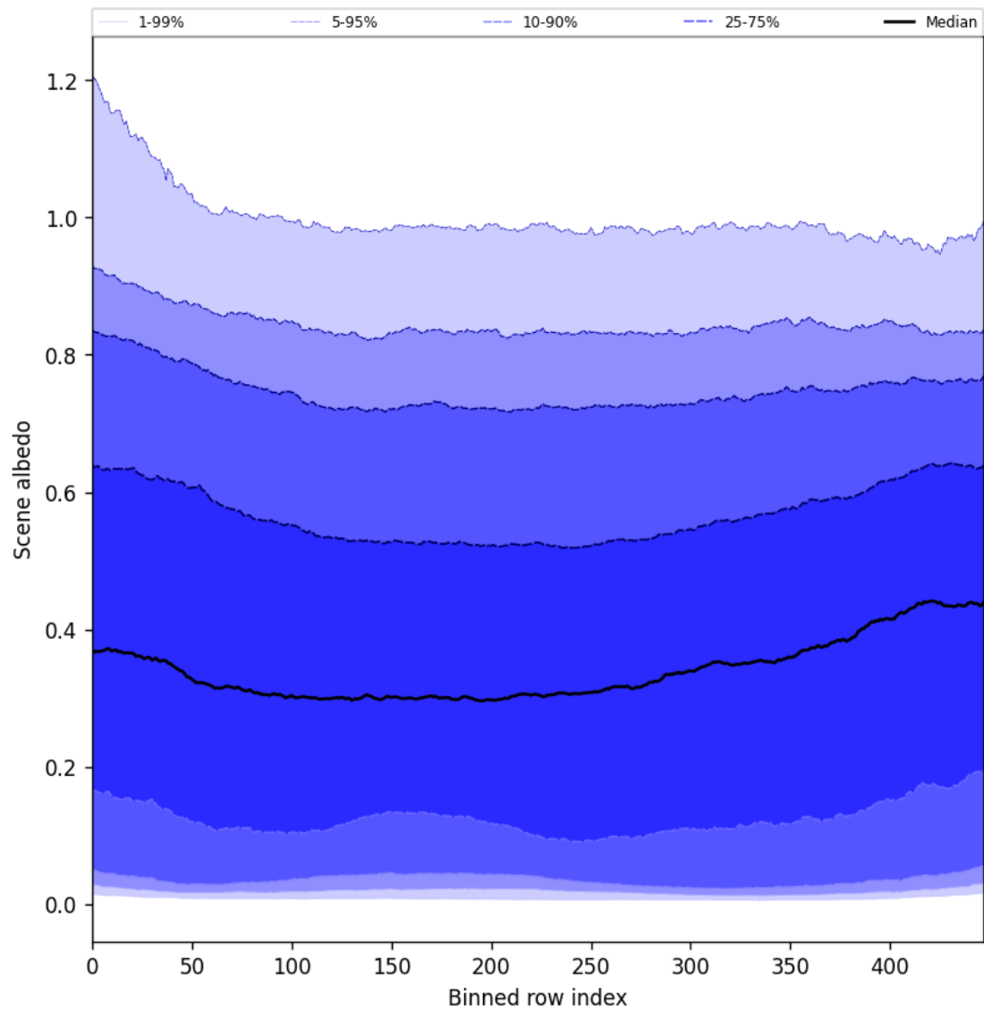
Figure 51: Along track statistics of “Scene albedo” for 2025-07-13 to 2025-07-15
