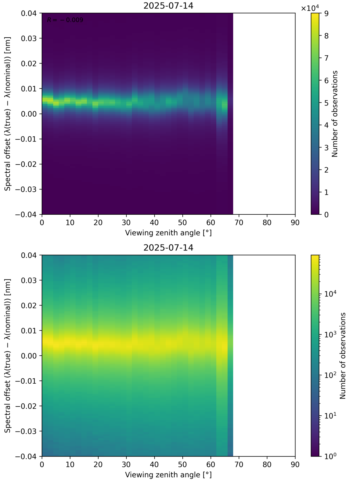
Figure 128: Scatter density plot of “Viewing zenith angle” against “Spectral offset ( \lambda_{\text{true}} - \lambda_{\text{nominal}} )” for 2025-07-13 to 2025-07-15.
