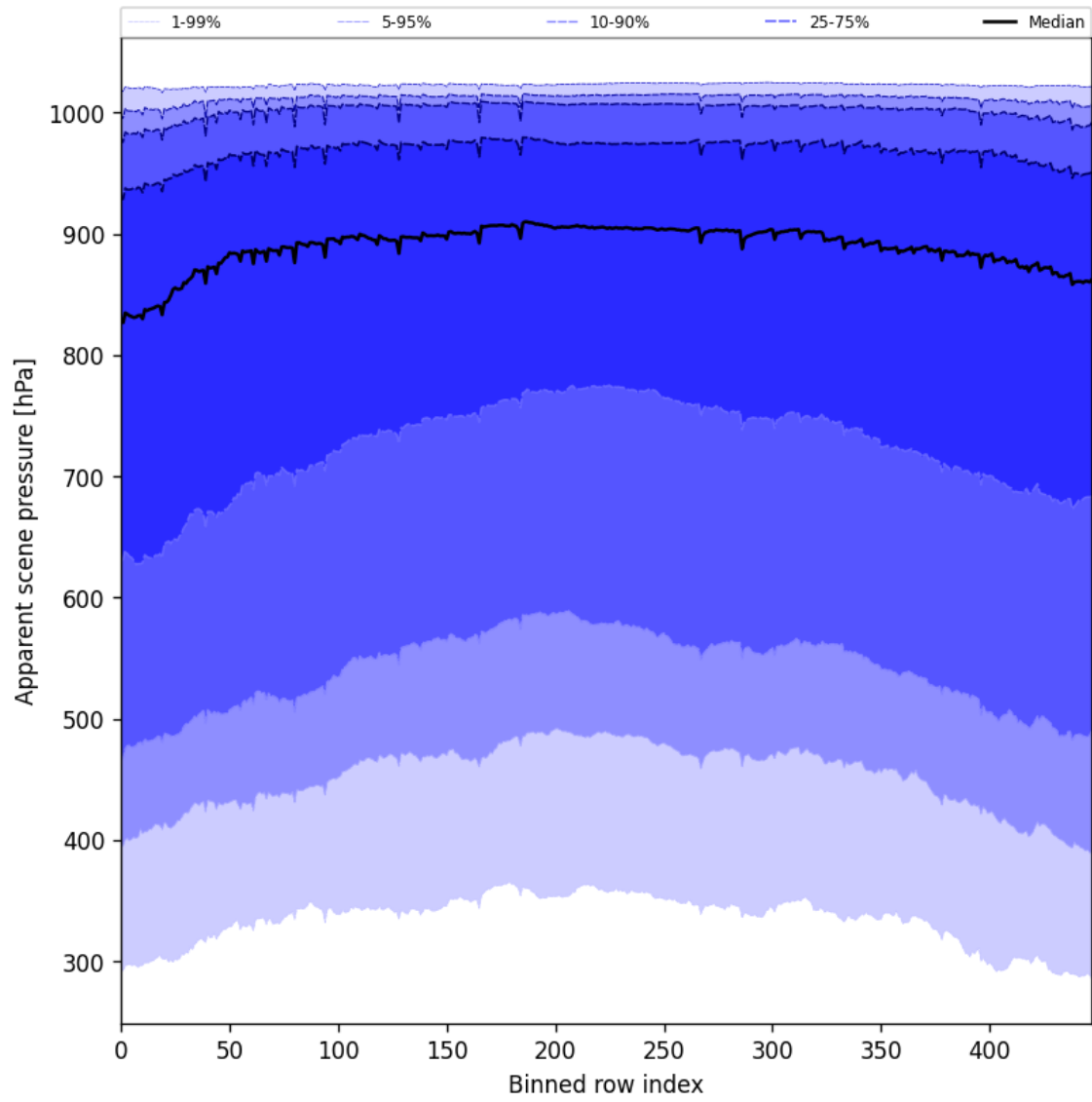
Figure 53: Along track statistics of “Apparent scene pressure” for 2025-07-13 to 2025-07-15
