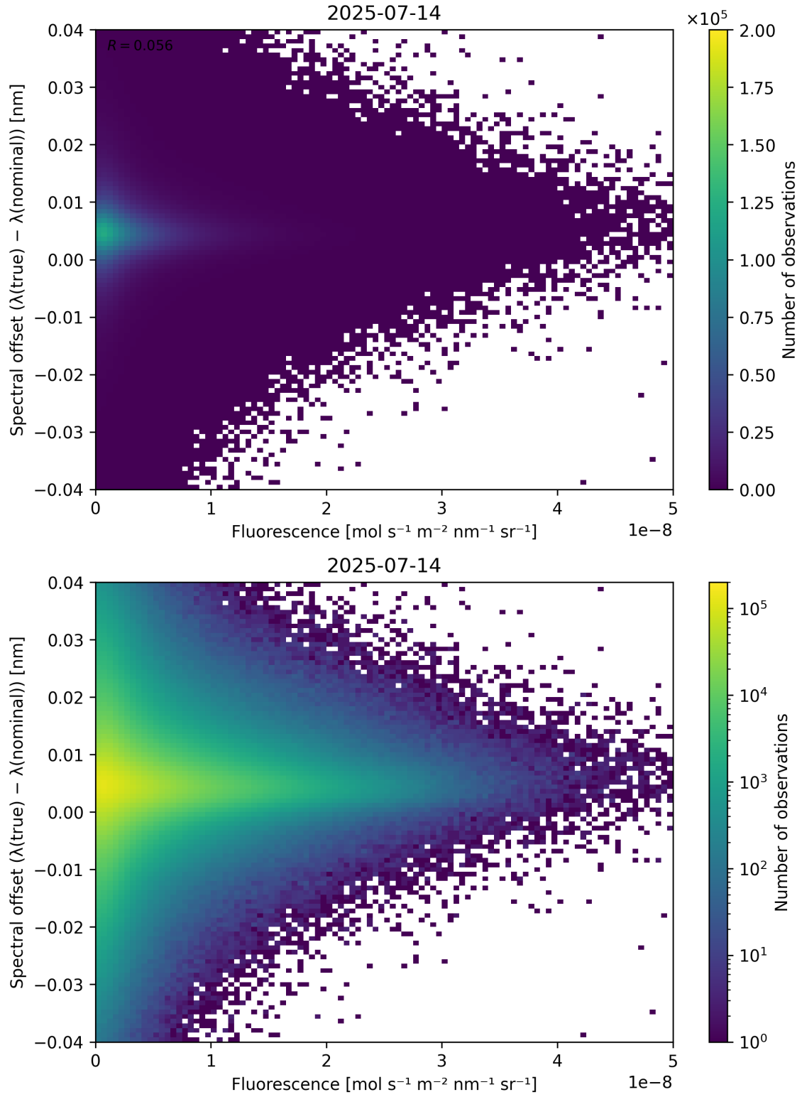
Figure 87: Scatter density plot of “Fluorescence” against “Spectral offset ( \lambda_{\text{true}} - \lambda_{\text{nominal}} )” for 2025-07-13 to 2025-07-15.
