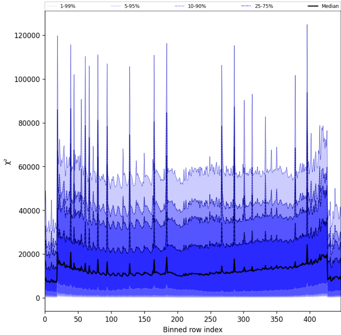
Figure 55: Along track statistics of “ \chi^2 ” for 2025-07-13 to 2025-07-15
