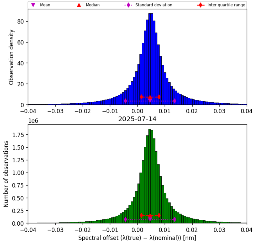
Figure 45: Histogram of “Spectral offset ( \lambda_{\text{true}} - \lambda_{\text{nominal}} )” for 2025-07-13 to 2025-07-15
