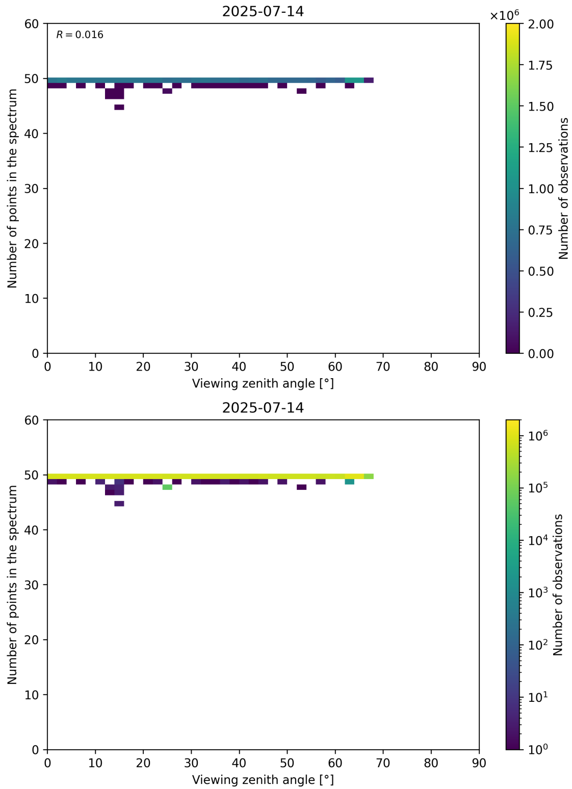
Figure 125: Scatter density plot of “Viewing zenith angle” against “Number of points in the spectrum” for 2025-07-13 to 2025-07-15.
