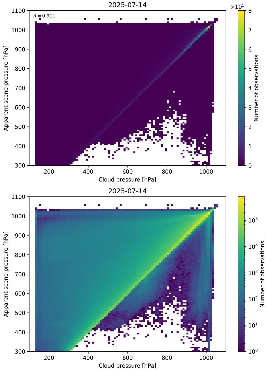
Figure 77: Scatter density plot of “Cloud pressure” against “Apparent scene pressure” for 2025-07-13 to 2025-07-15.
