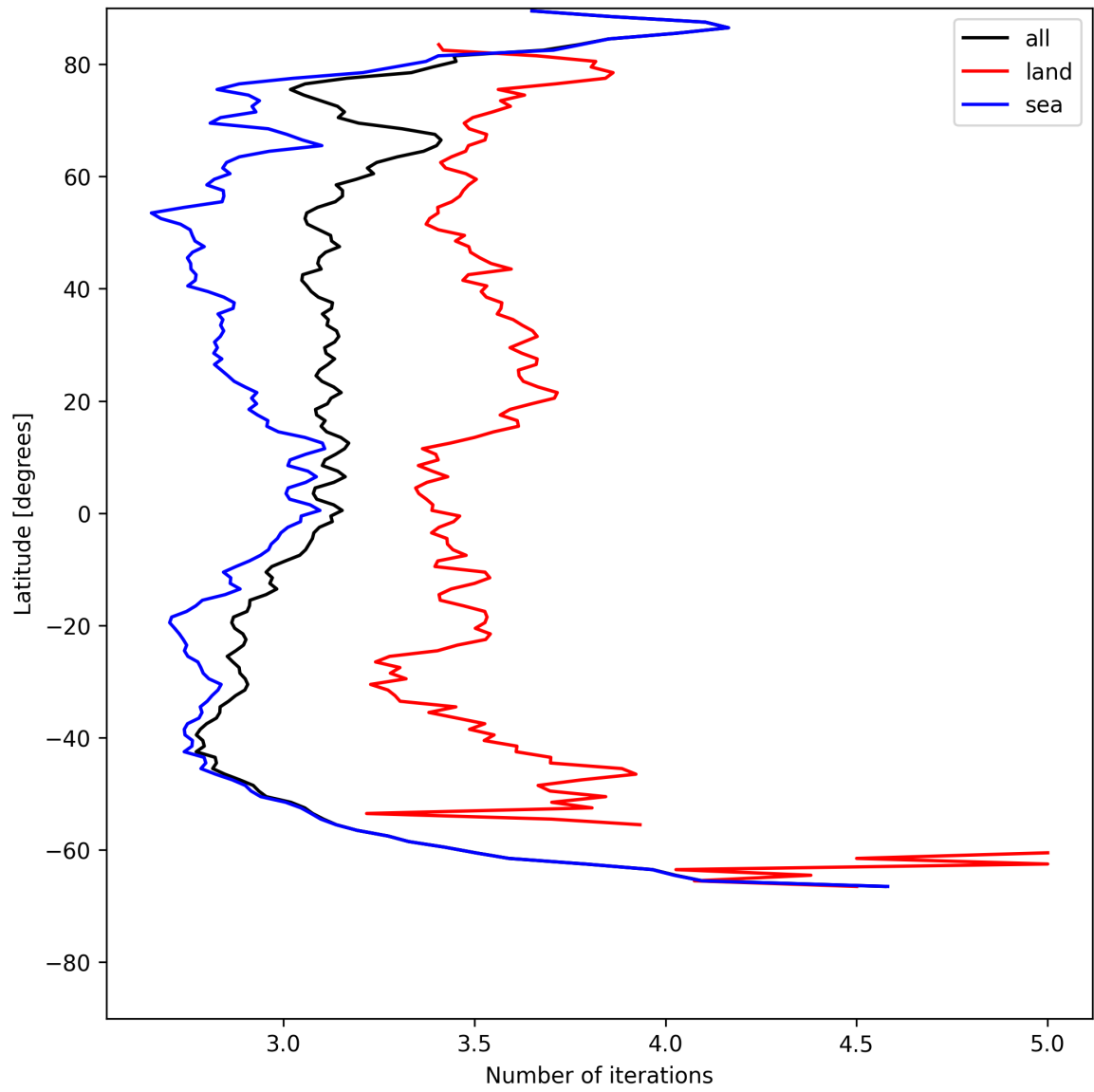
Figure 22: Zonal average of “Number of iterations” for 2025-07-13 to 2025-07-15.
