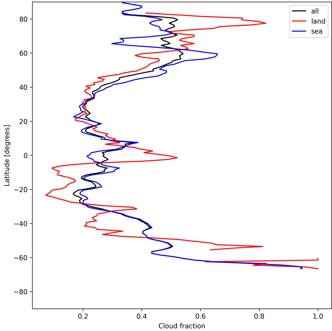
Figure 15: Zonal average of “Cloud fraction” for 2025-07-13 to 2025-07-15.
