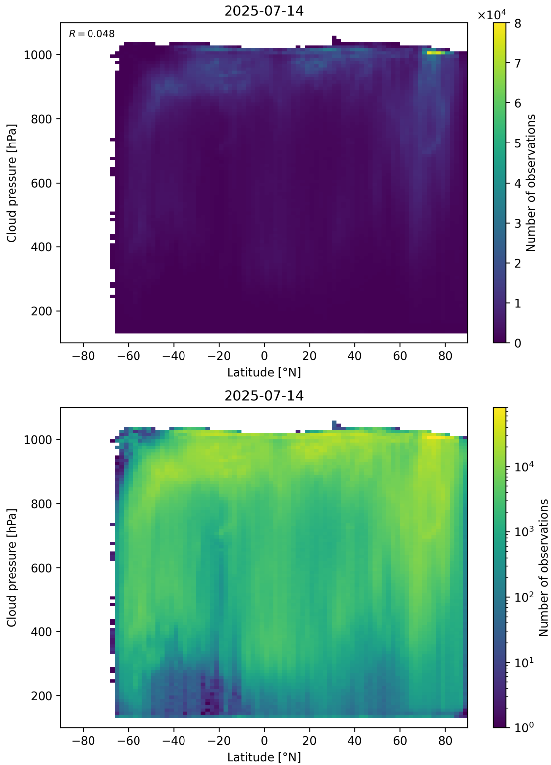
Figure 91: Scatter density plot of “Latitude” against “Cloud pressure” for 2025-07-13 to 2025-07-15.
