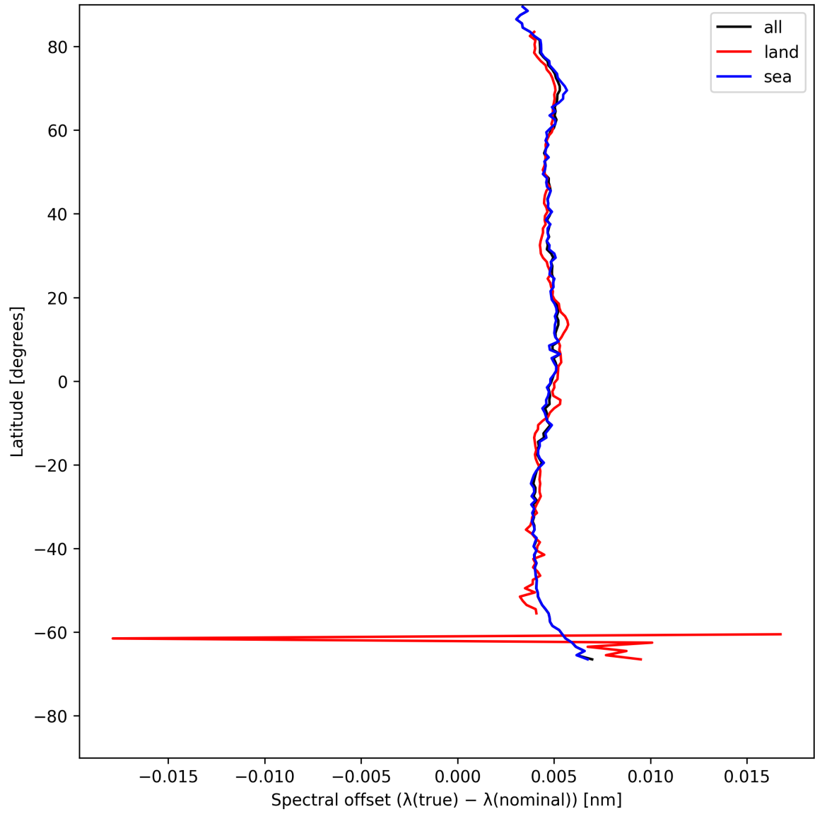
Figure 28: Zonal average of “Spectral offset ( \lambda_{\text{true}} - \lambda_{\text{nominal}} )” for 2025-07-13 to 2025-07-15.
