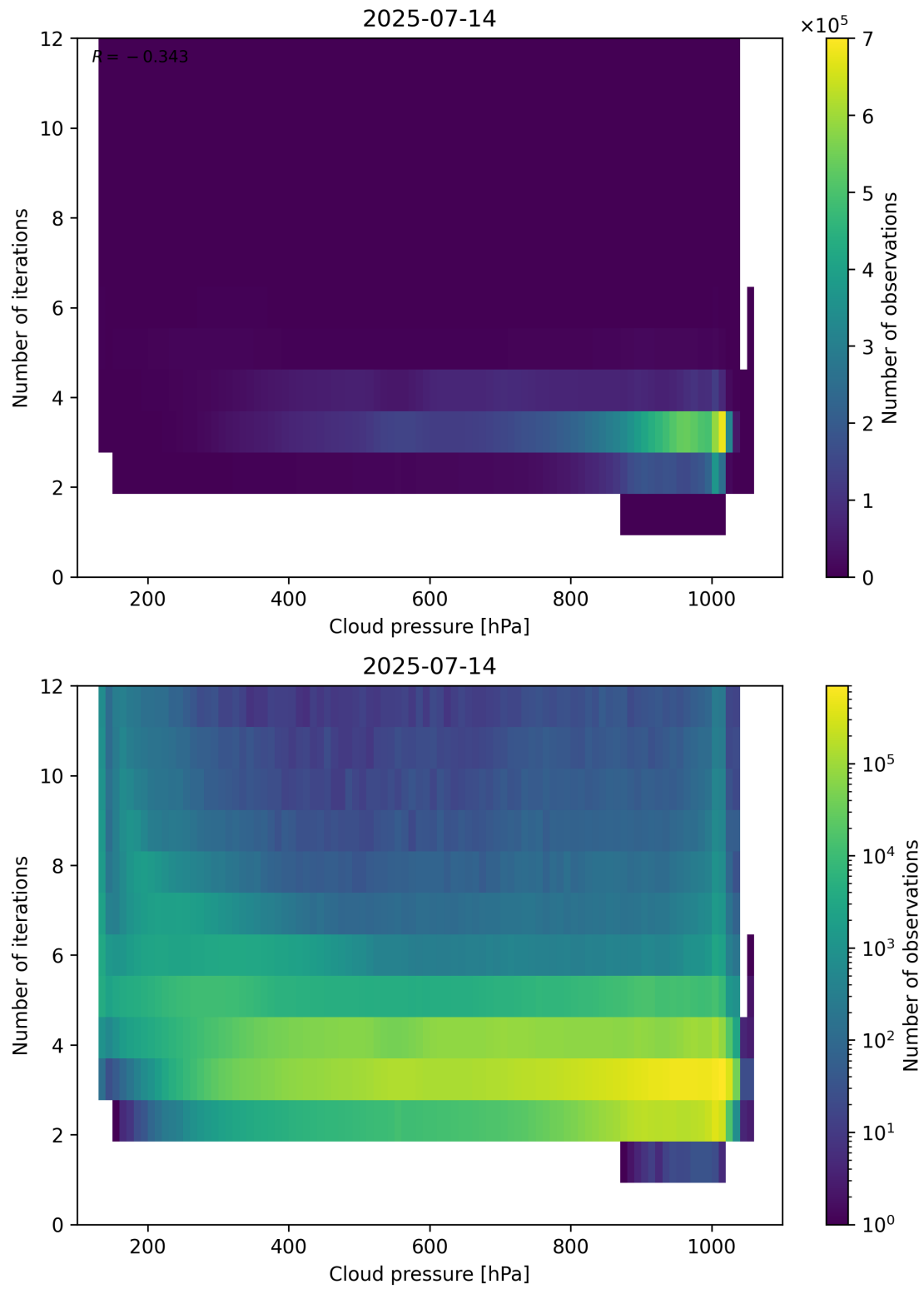
Figure 81: Scatter density plot of “Cloud pressure” against “Number of iterations” for 2025-07-13 to 2025-07-15.
