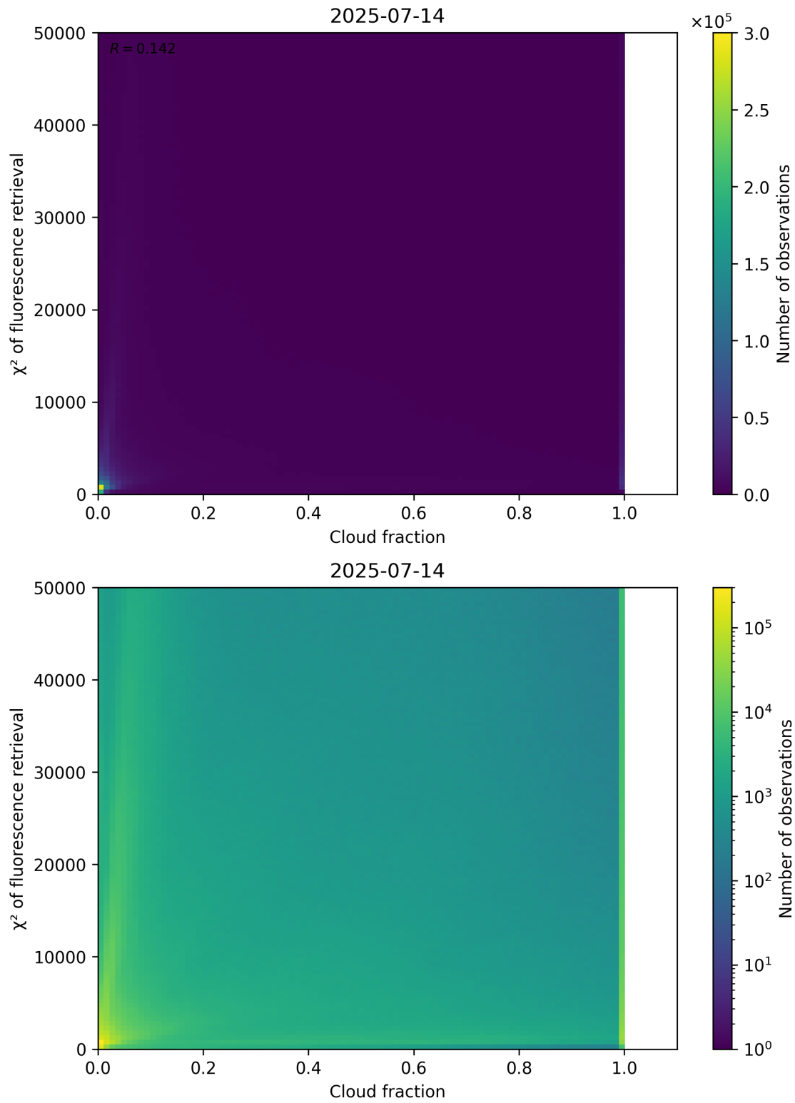
Figure 71: Scatter density plot of “Cloud fraction” against “ \chi^2 of fluorescence retrieval” for 2025-07-13 to 2025-07-15.
