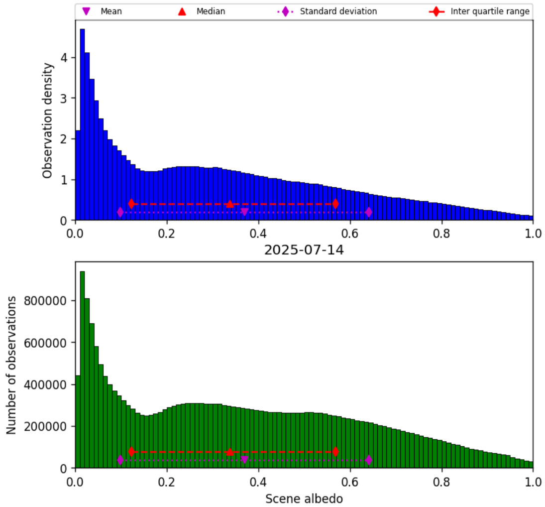
Figure 34: Histogram of “Scene albedo” for 2025-07-13 to 2025-07-15
