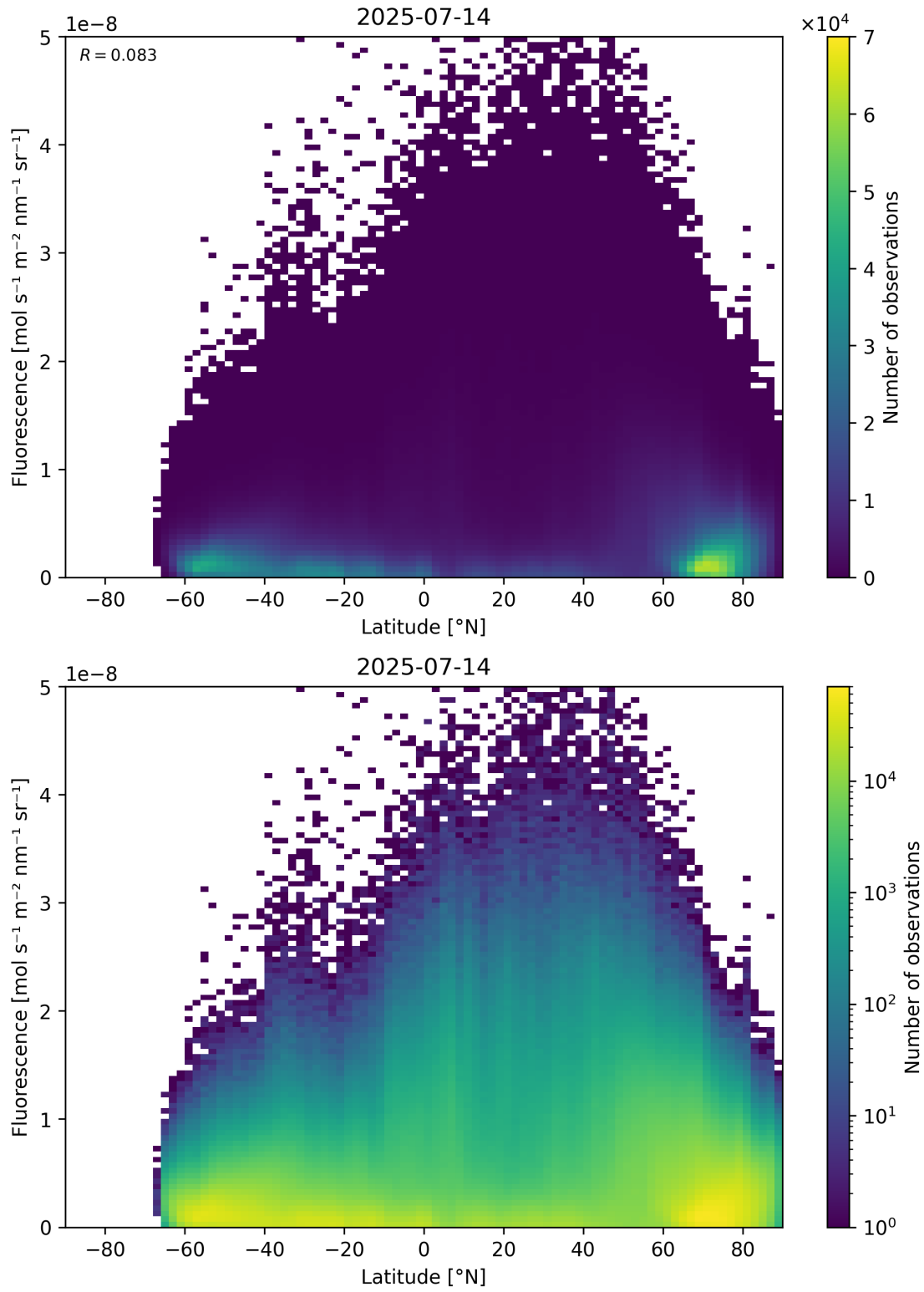
Figure 92: Scatter density plot of “Latitude” against “Fluorescence” for 2025-07-13 to 2025-07-15.
