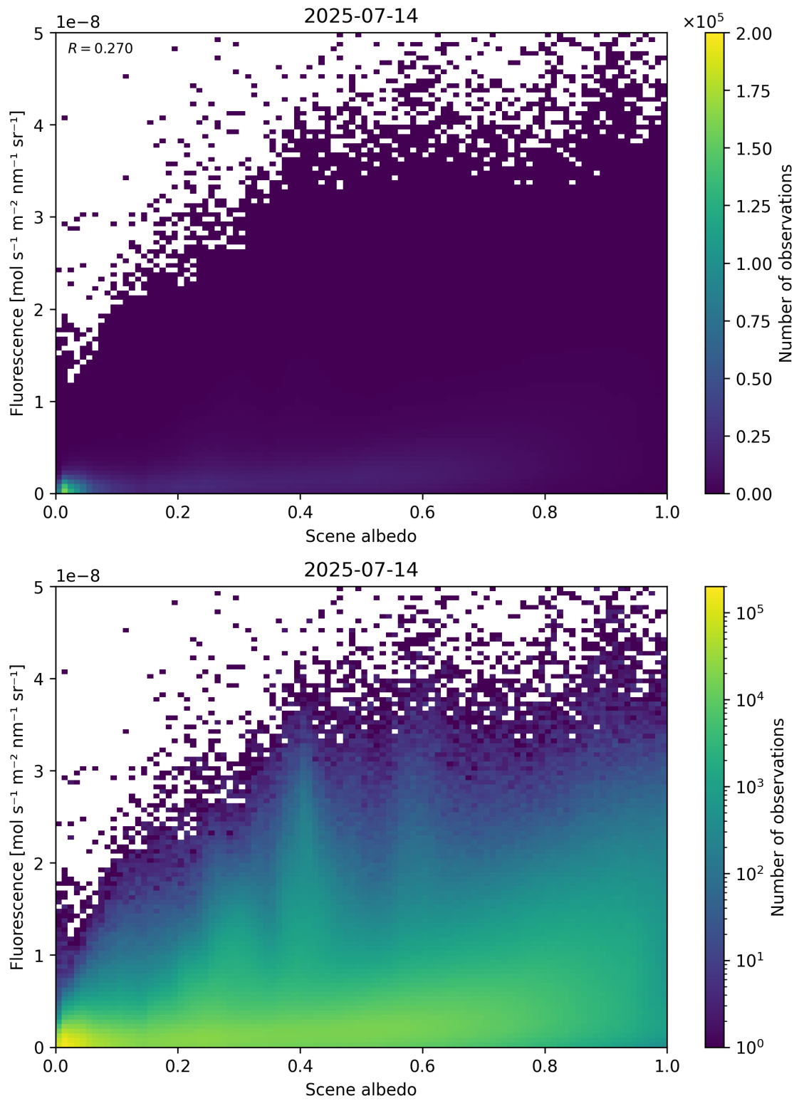
Figure 104: Scatter density plot of “Scene albedo” against “Fluorescence” for 2025-07-13 to 2025-07-15.
