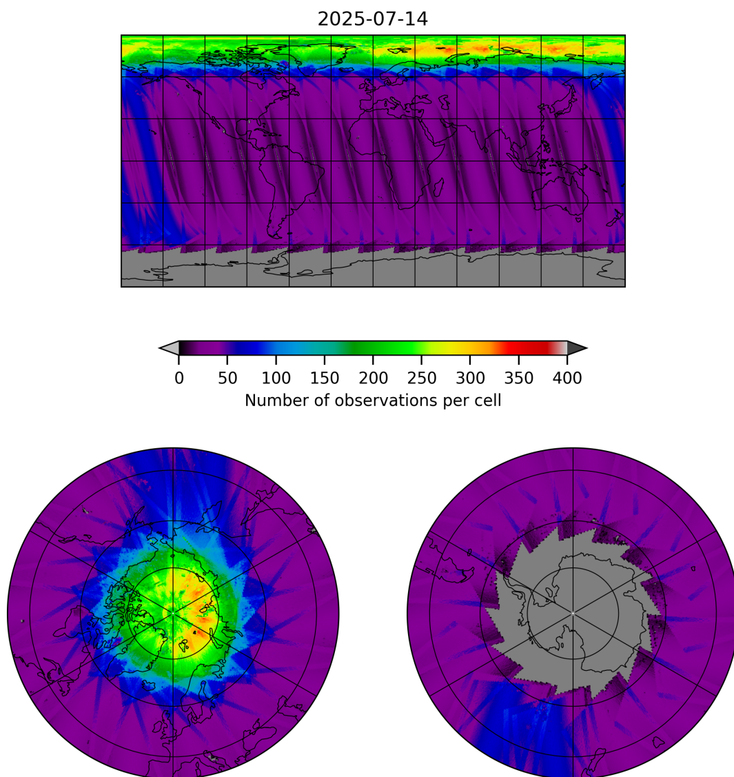
Figure 11: Map of the number of observations for 2025-07-13 to 2025-07-15
