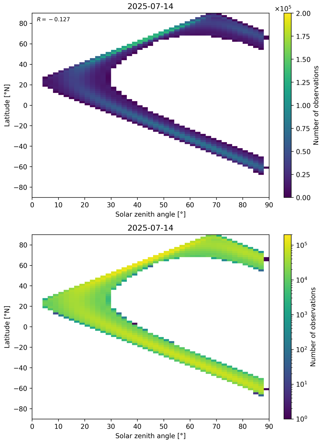
Figure 113: Scatter density plot of “Solar zenith angle” against “Latitude” for 2025-07-13 to 2025-07-15.
