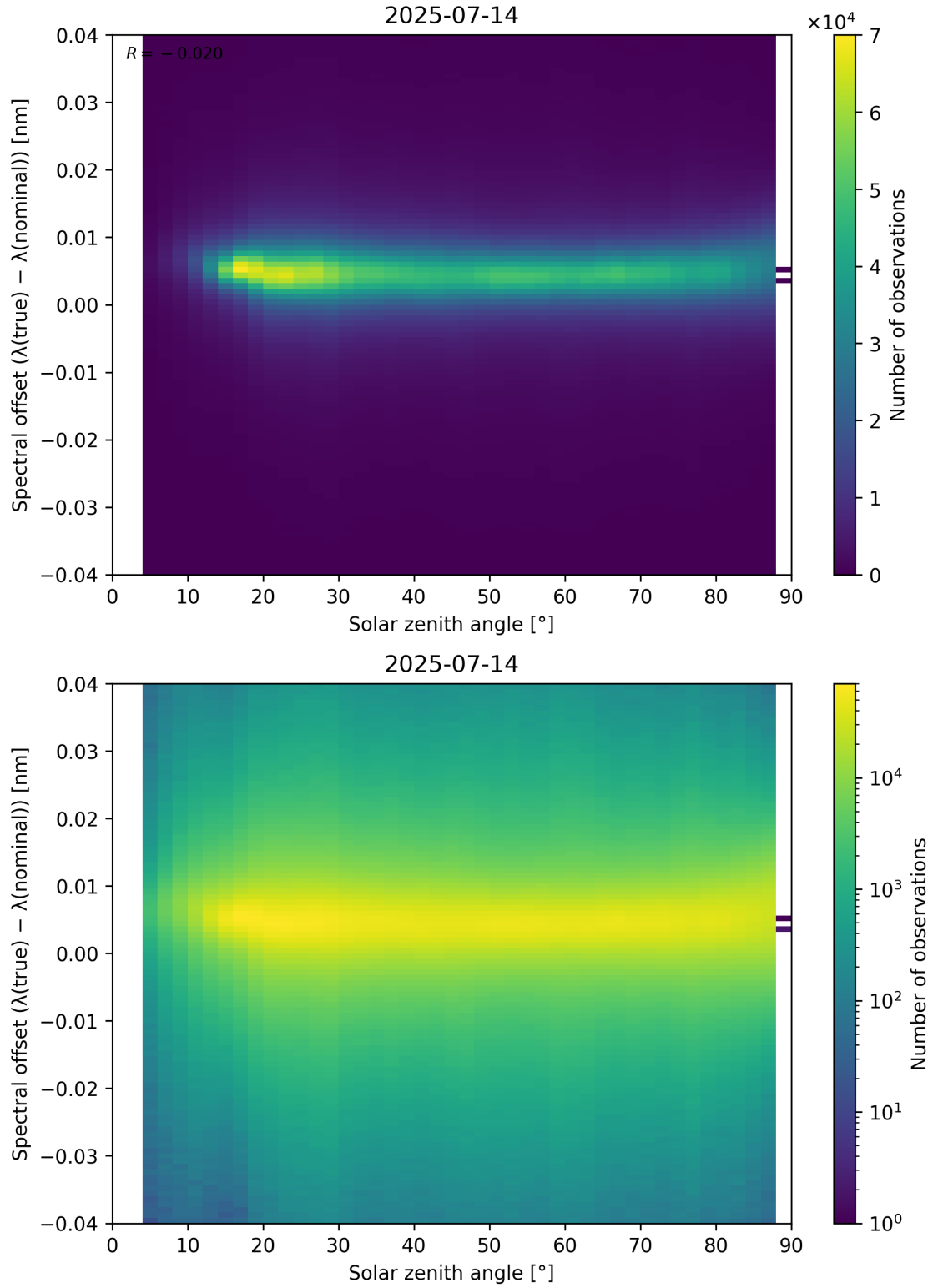
Figure 117: Scatter density plot of “Solar zenith angle” against “Spectral offset ( \lambda_{\text{true}} - \lambda_{\text{nominal}} )” for 2025-07-13 to 2025-07-15.
