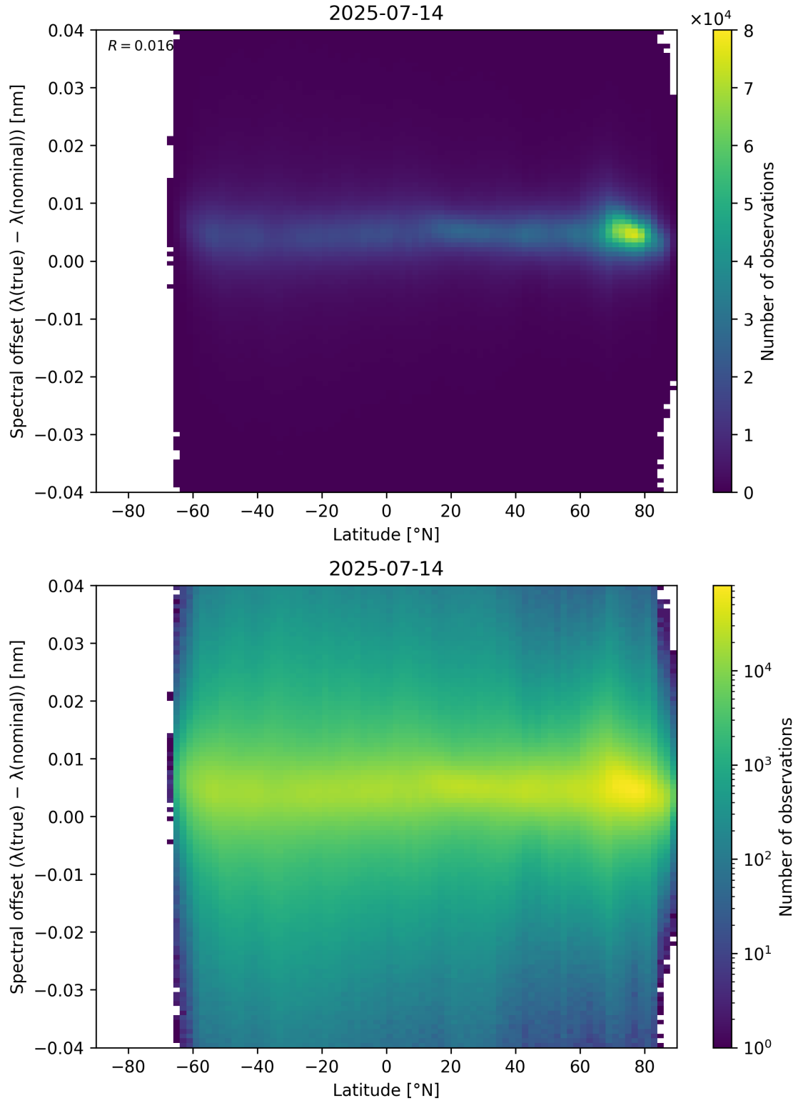
Figure 96: Scatter density plot of “Latitude” against “Spectral offset ( \lambda_{\text{true}} - \lambda_{\text{nominal}} )” for 2025-07-13 to 2025-07-15.
