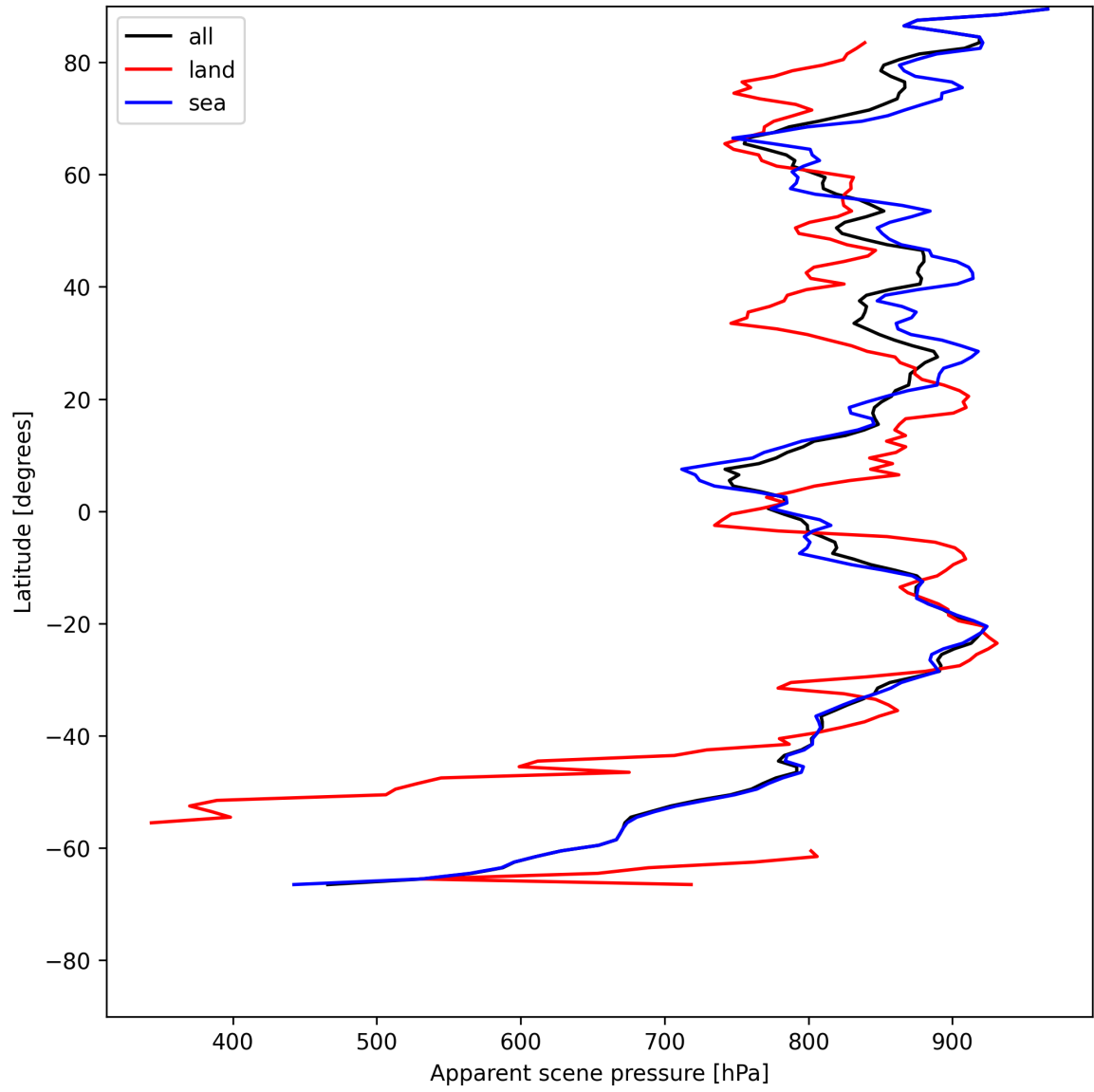
Figure 19: Zonal average of “Apparent scene pressure” for 2025-07-13 to 2025-07-15.
