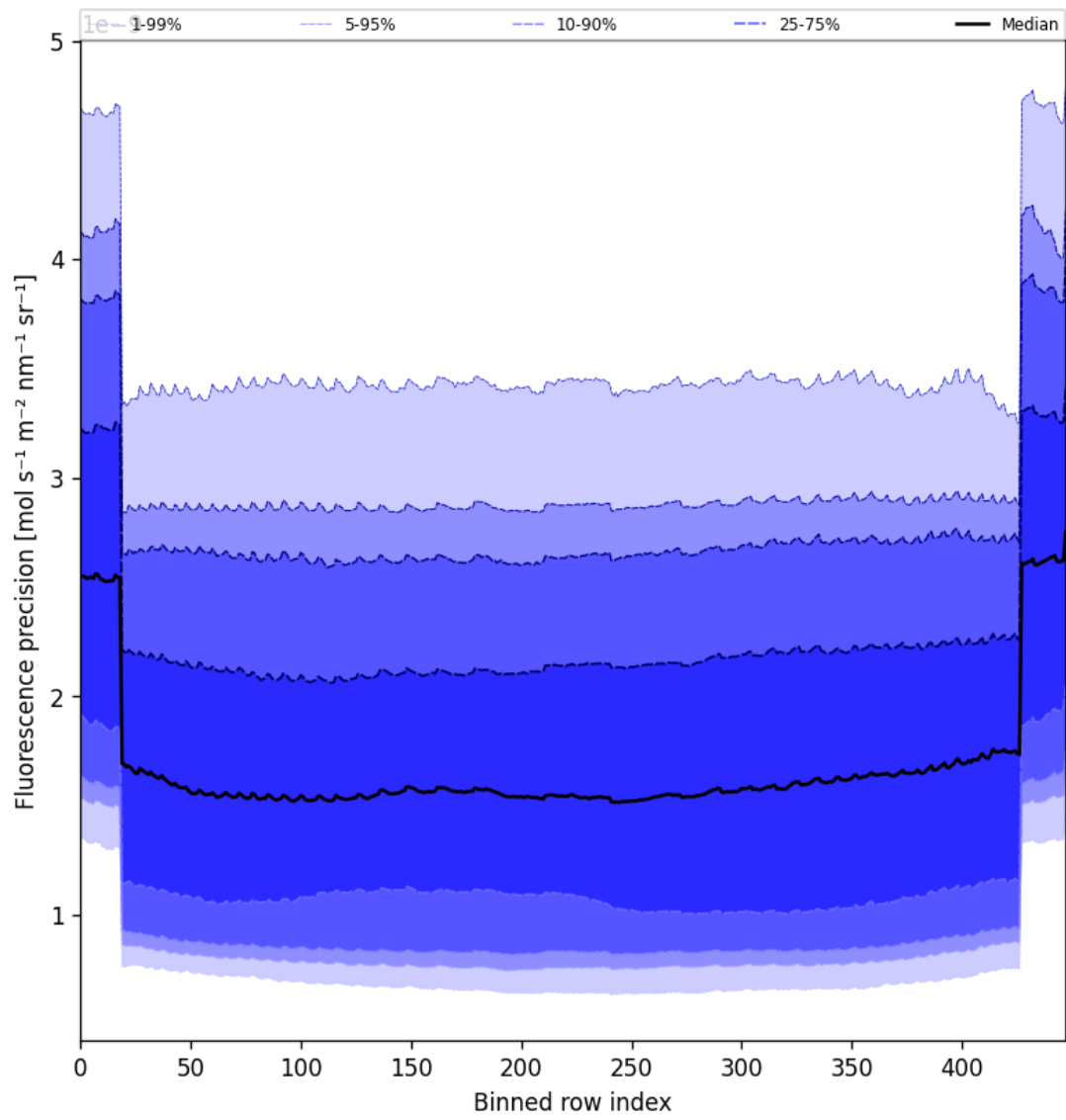
Figure 58: Along track statistics of “Fluorescence precision” for 2025-07-13 to 2025-07-15
