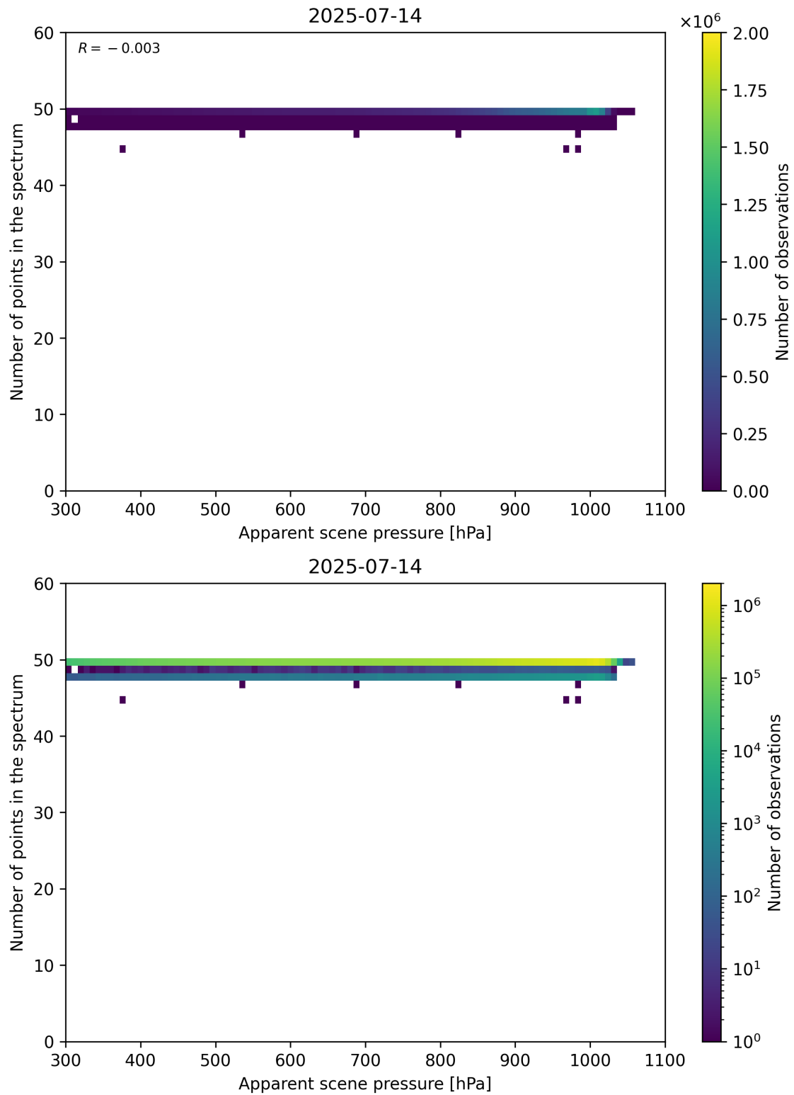
Figure 66: Scatter density plot of “Apparent scene pressure” against “Number of points in the spectrum” for 2025-07-13 to 2025-07-15.
