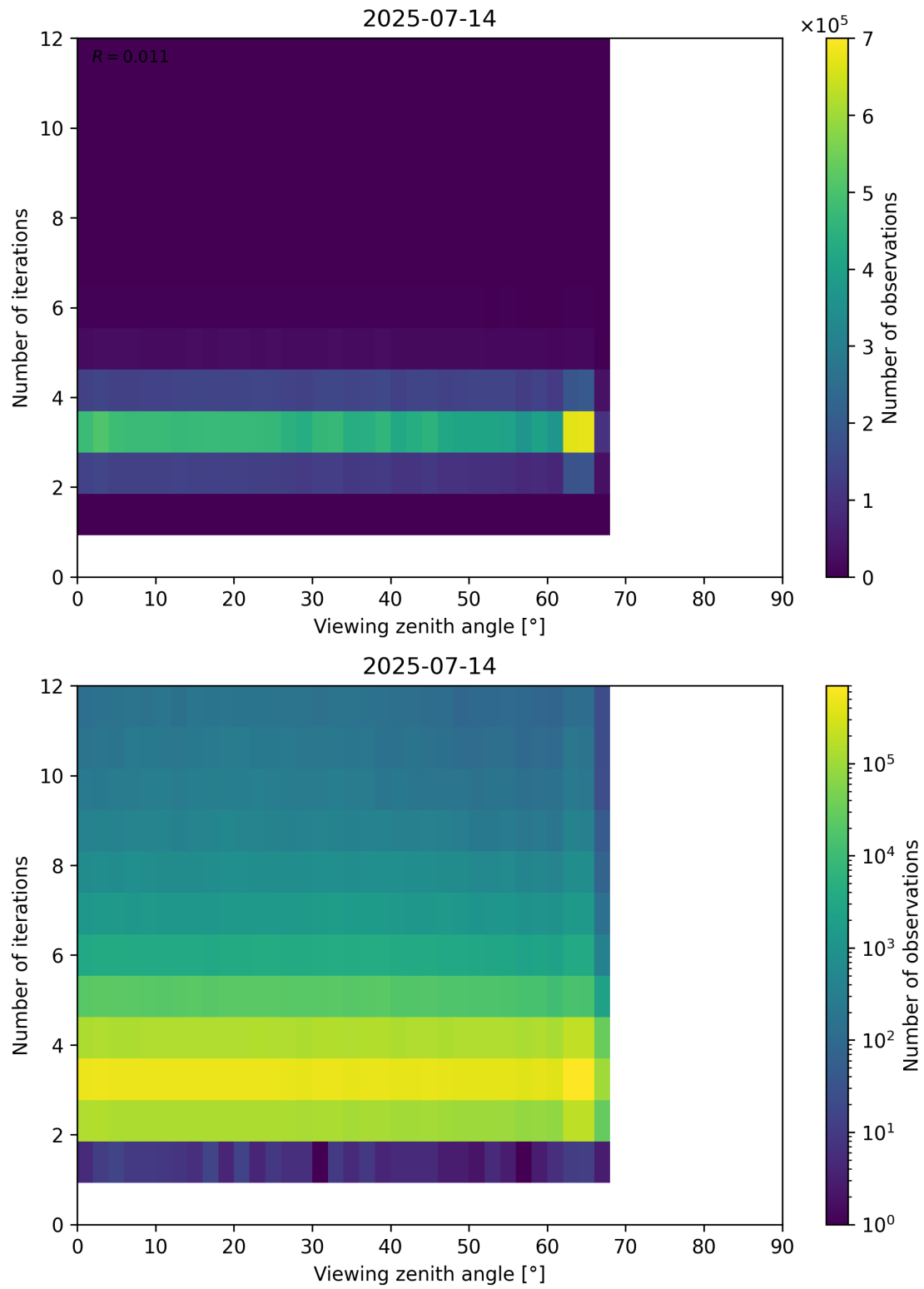
Figure 124: Scatter density plot of “Viewing zenith angle” against “Number of iterations” for 2025-07-13 to 2025-07-15.
