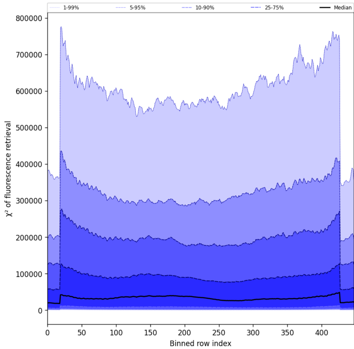
Figure 59: Along track statistics of “ \chi^2 of fluorescence retrieval” for 2025-07-13 to 2025-07-15
