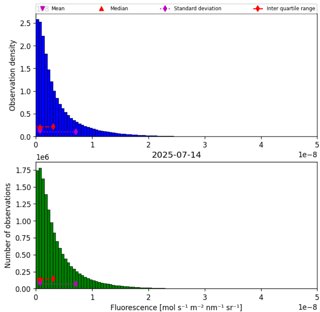
Figure 40: Histogram of “Fluorescence” for 2025-07-13 to 2025-07-15
