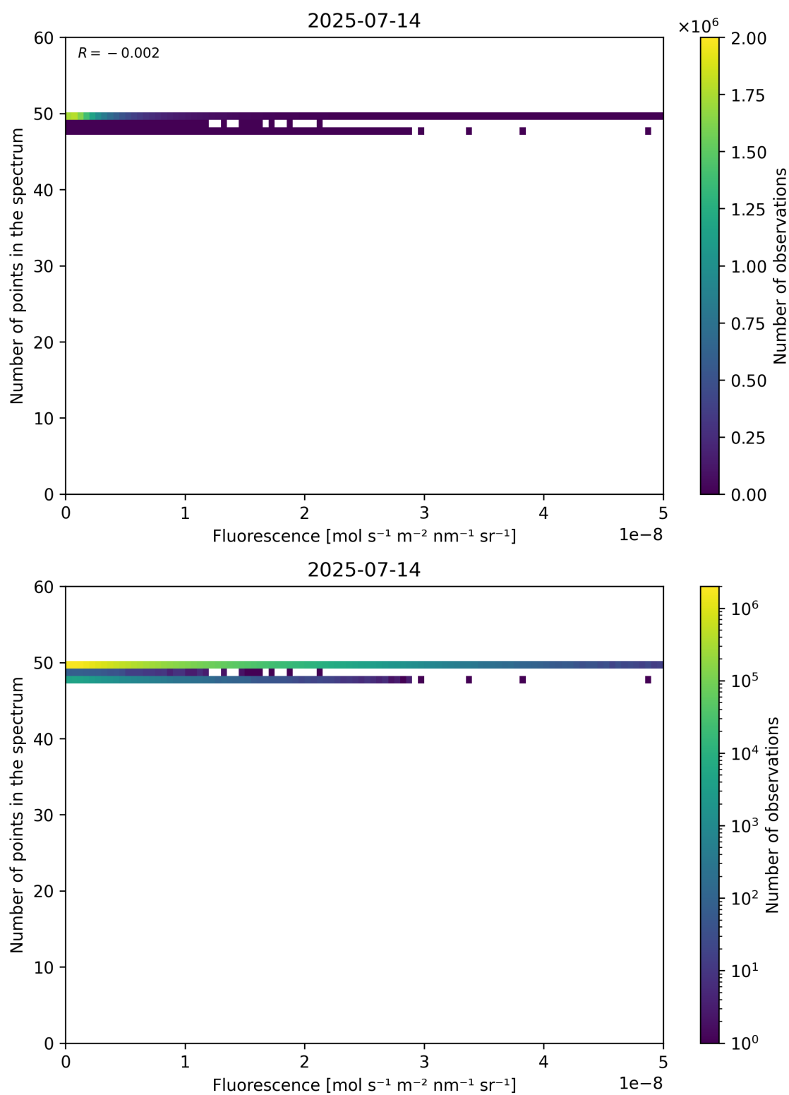
Figure 86: Scatter density plot of “Fluorescence” against “Number of points in the spectrum” for 2025-07-13 to 2025-07-15.
