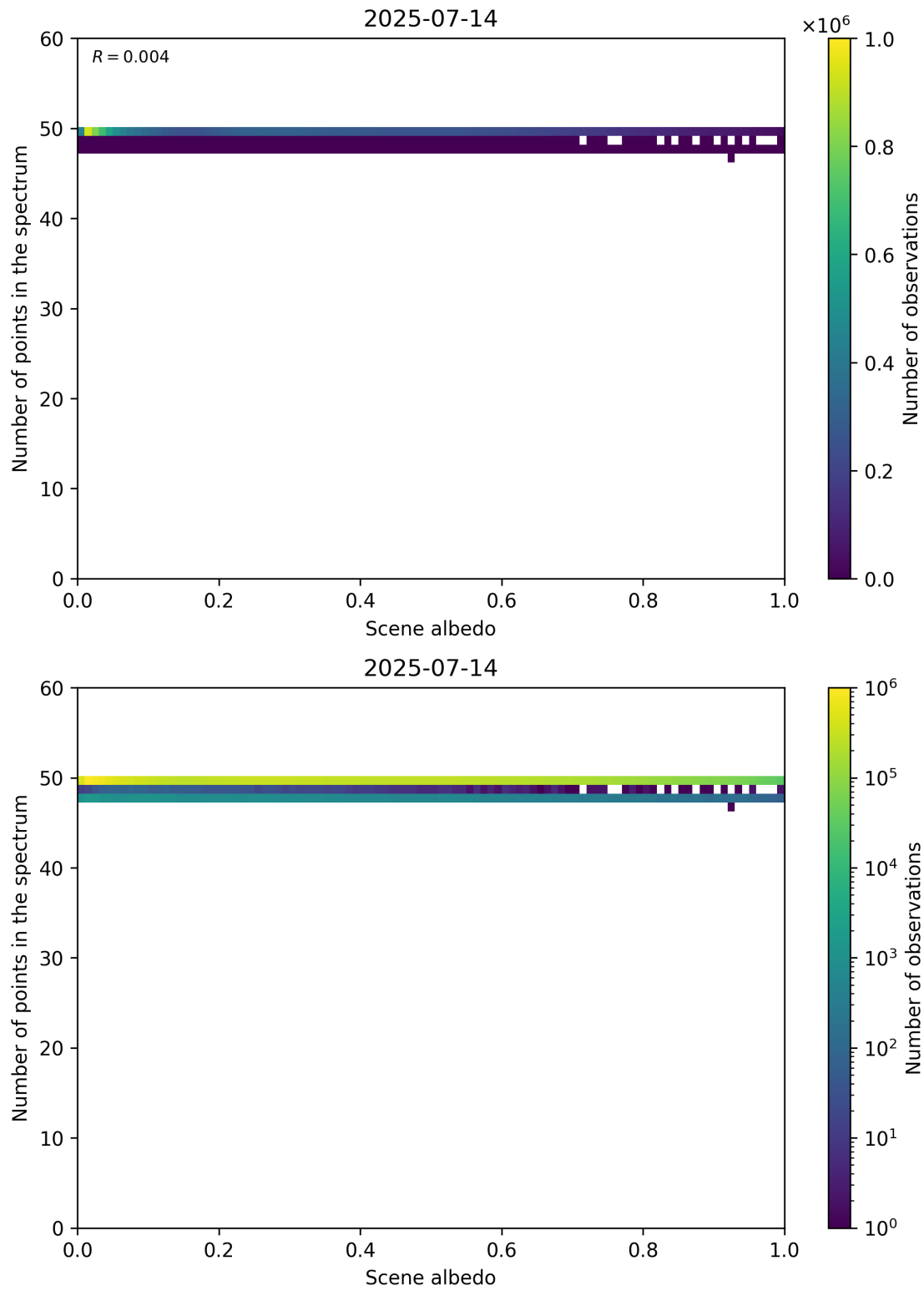
Figure 106: Scatter density plot of “Scene albedo” against “Number of points in the spectrum” for 2025-07-13 to 2025-07-15.
