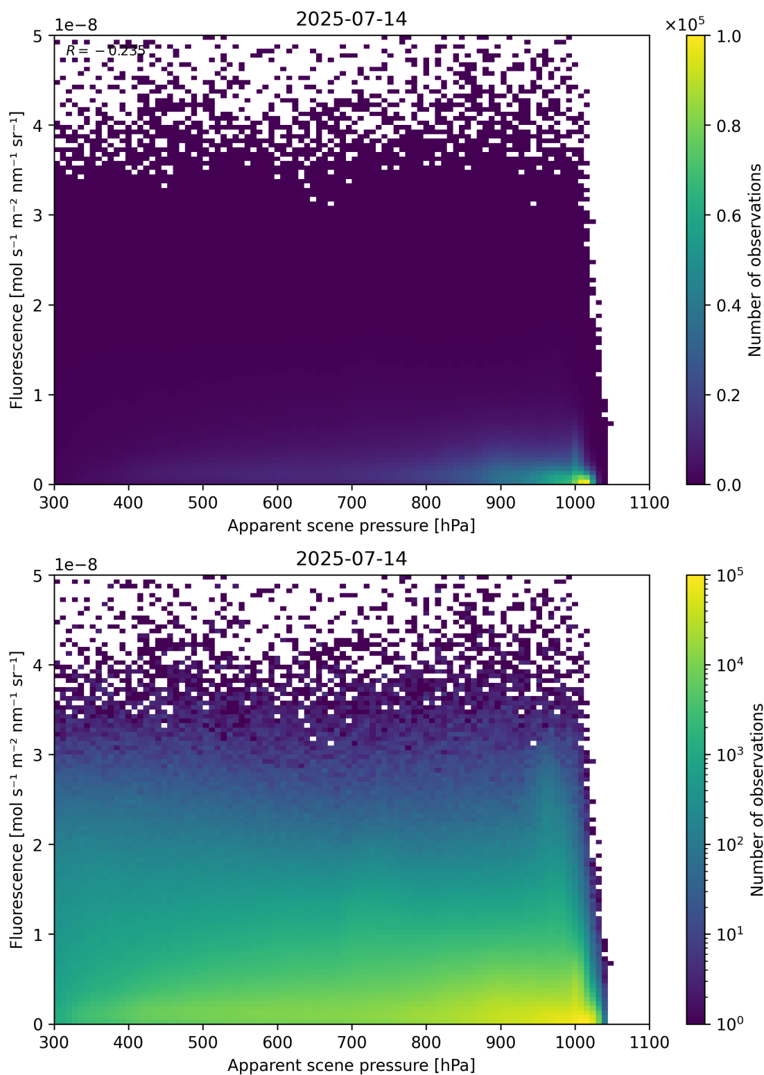
Figure 64: Scatter density plot of “Apparent scene pressure” against “Fluorescence” for 2025-07-13 to 2025-07-15.
