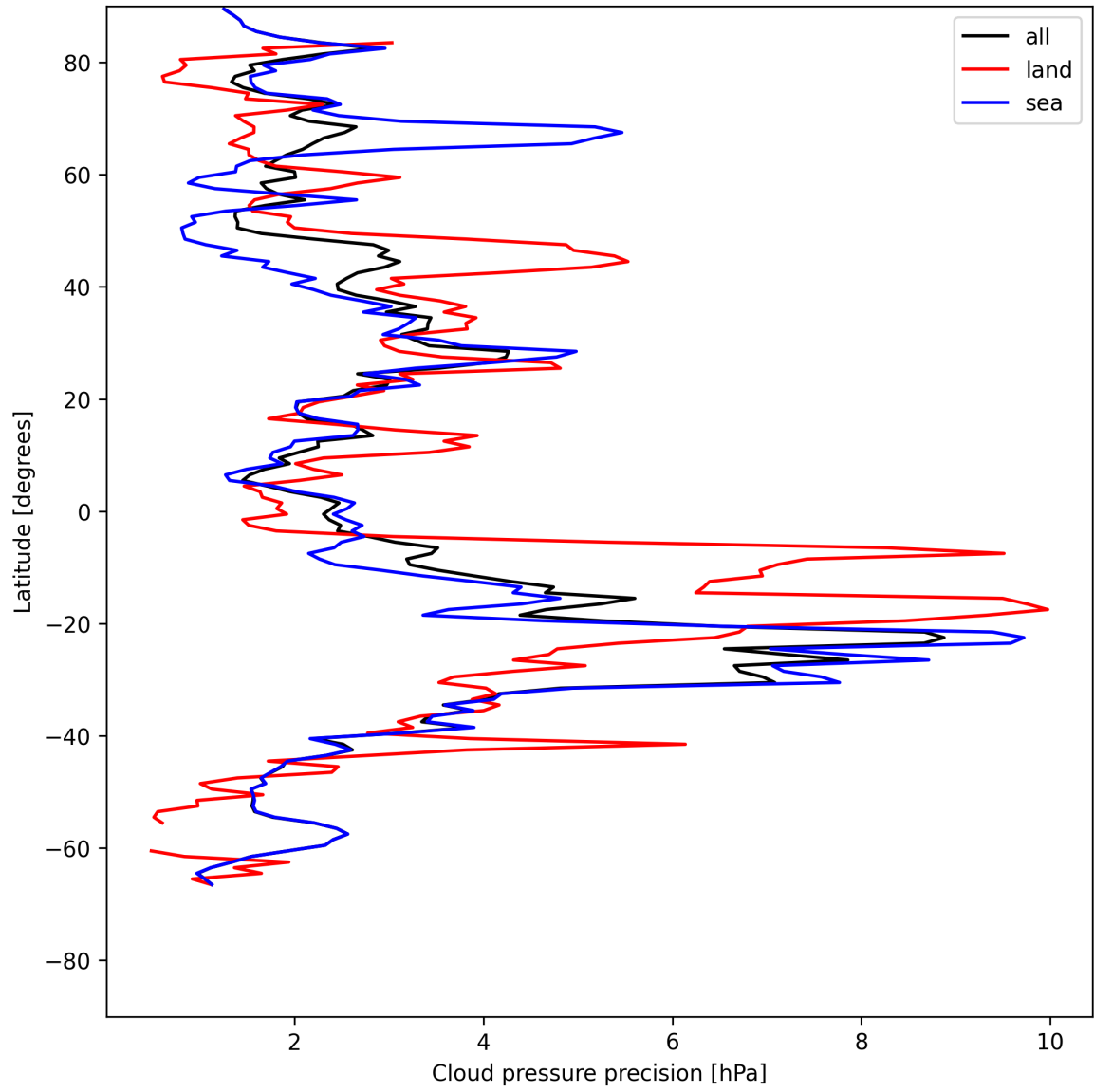
Figure 14: Zonal average of "Cloud pressure precision" for 2025-07-13 to 2025-07-15.
