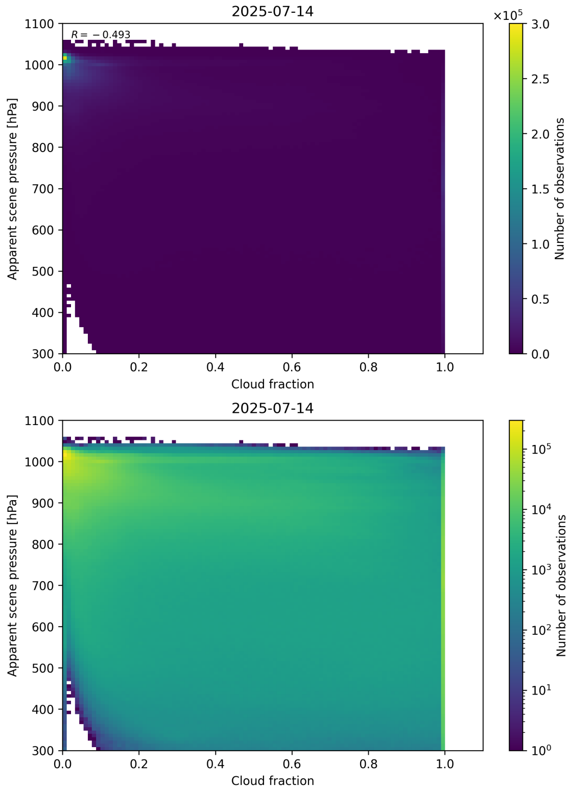
Figure 70: Scatter density plot of “Cloud fraction” against “Apparent scene pressure” for 2025-07-13 to 2025-07-15.
