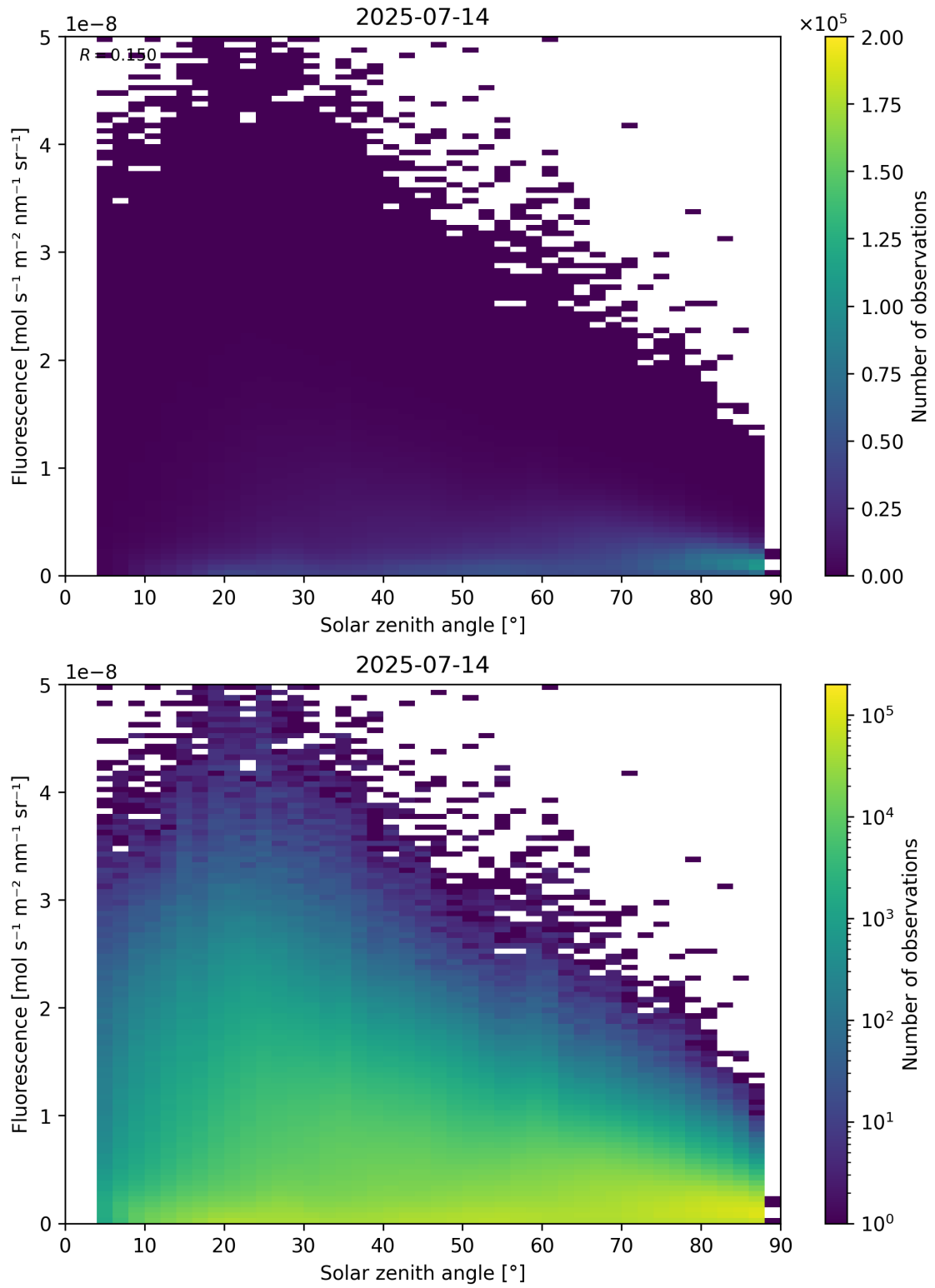
Figure 112: Scatter density plot of “Solar zenith angle” against “Fluorescence” for 2025-07-13 to 2025-07-15.
