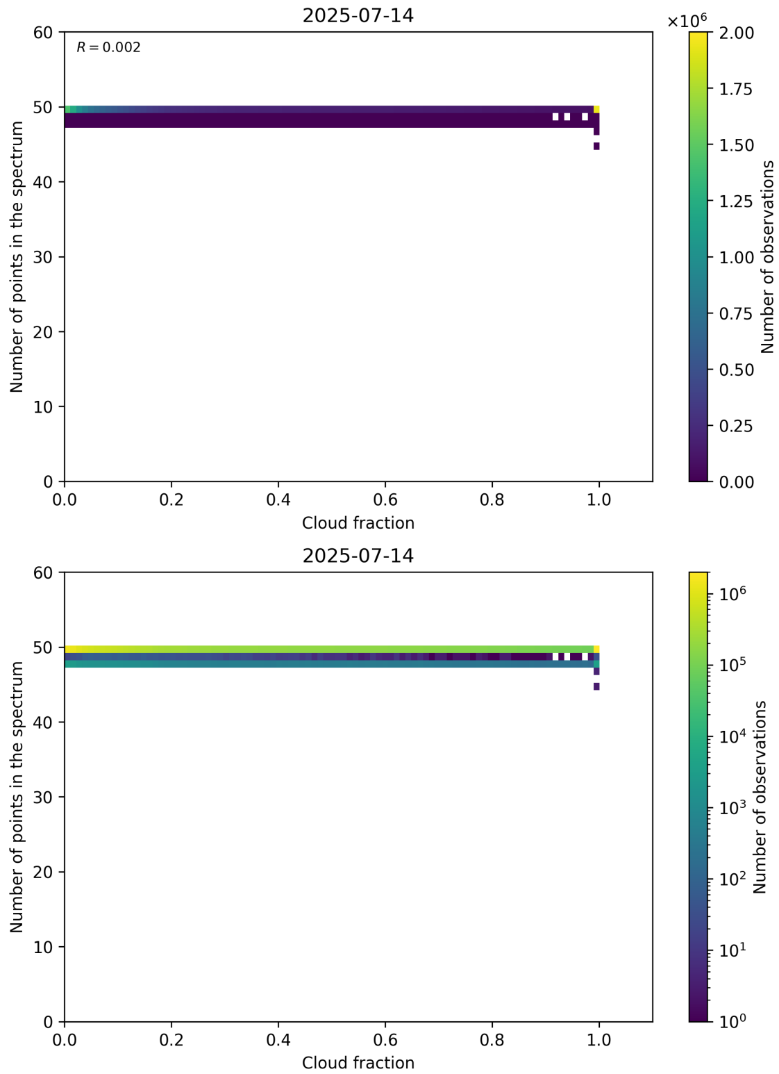
Figure 74: Scatter density plot of “Cloud fraction” against “Number of points in the spectrum” for 2025-07-13 to 2025-07-15.
