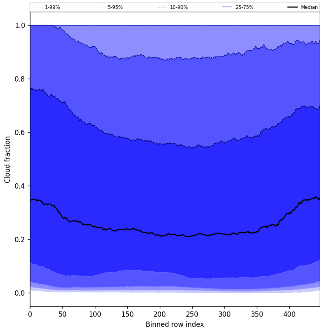
Figure 49: Along track statistics of “Cloud fraction” for 2025-07-13 to 2025-07-15
