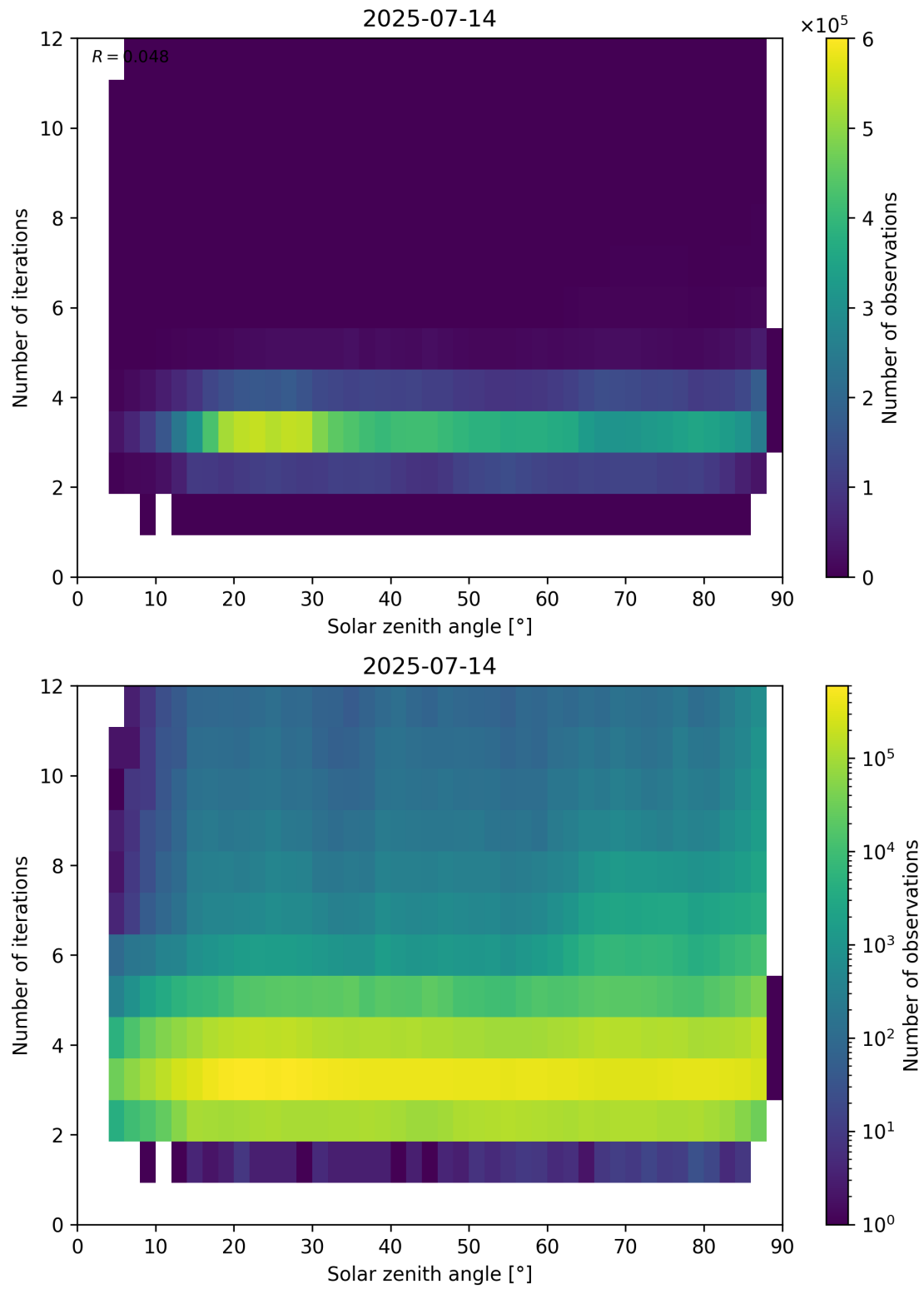
Figure 114: Scatter density plot of “Solar zenith angle” against “Number of iterations” for 2025-07-13 to 2025-07-15.
