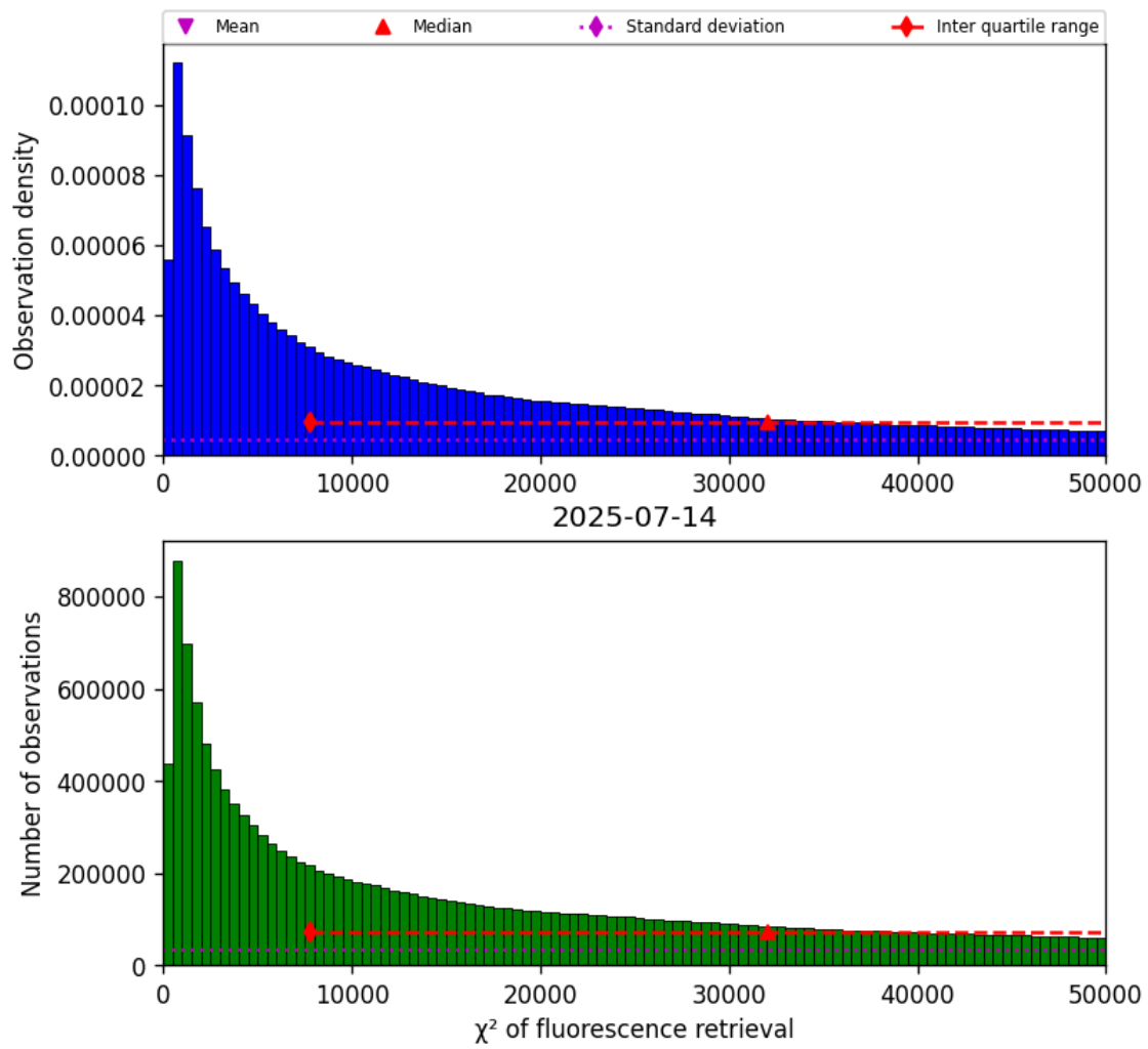
Figure 42: Histogram of “ \chi^2 of fluorescence retrieval” for 2025-07-13 to 2025-07-15
