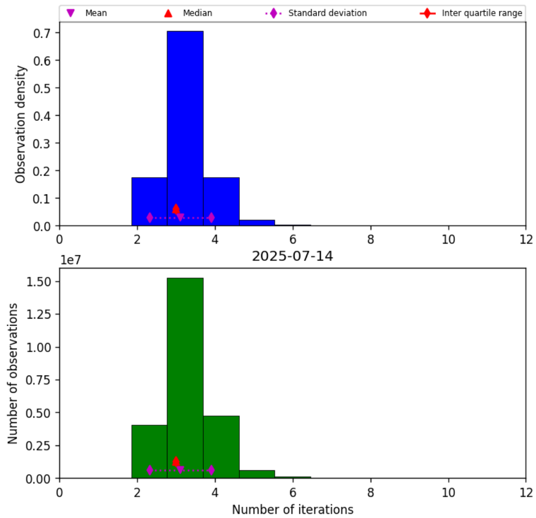
Figure 39: Histogram of “Number of iterations” for 2025-07-13 to 2025-07-15
