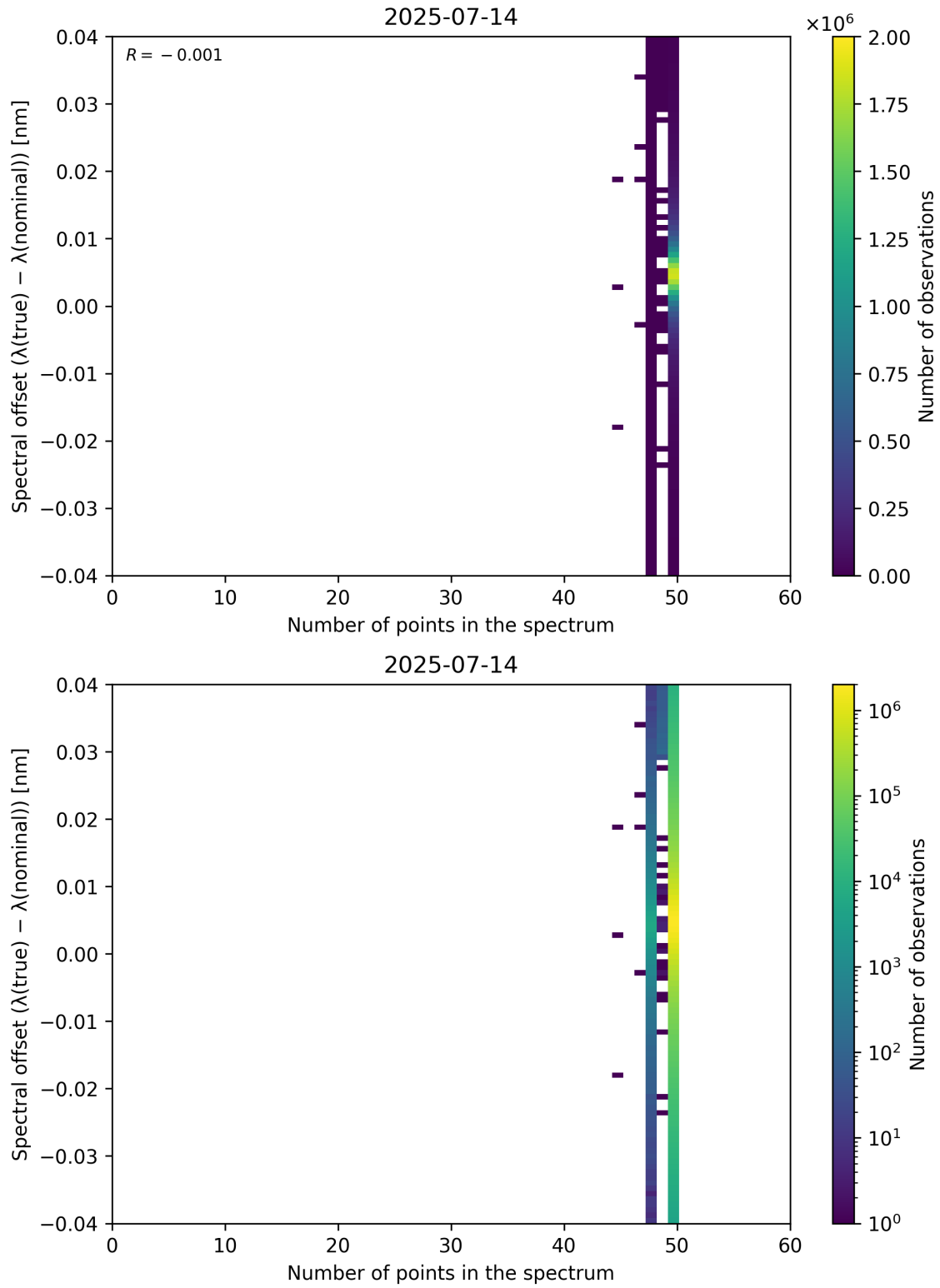
Figure 101: Scatter density plot of “Number of points in the spectrum” against “Spectral offset ( \lambda_{\text{true}} - \lambda_{\text{nominal}} )” for 2025-07-13 to 2025-07-15.
