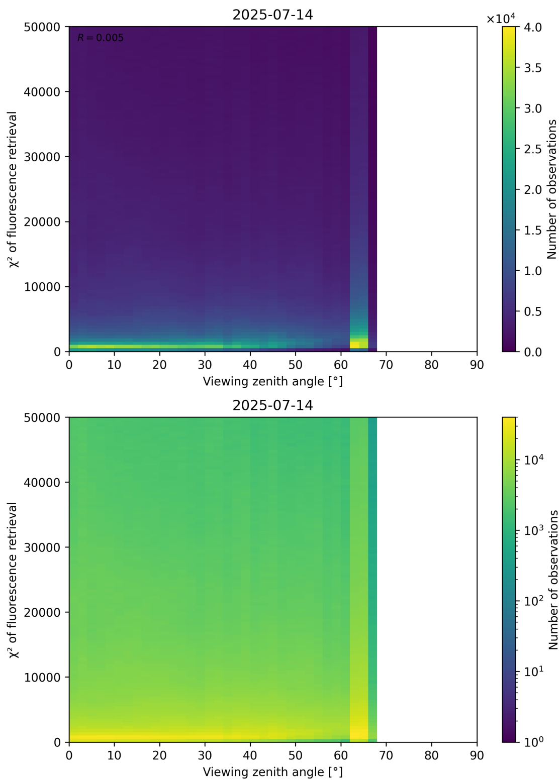
Figure 119: Scatter density plot of “Viewing zenith angle” against “ \chi^2 of fluorescence retrieval” for 2025-07-13 to 2025-07-15.
