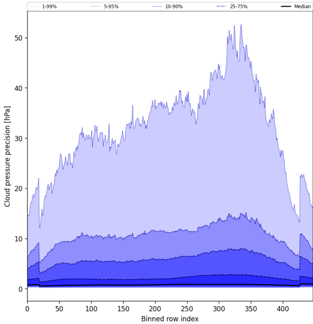
Figure 48: Along track statistics of “Cloud pressure precision” for 2025-07-13 to 2025-07-15
