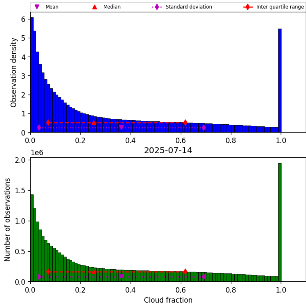
Figure 32: Histogram of “Cloud fraction” for 2025-07-13 to 2025-07-15
