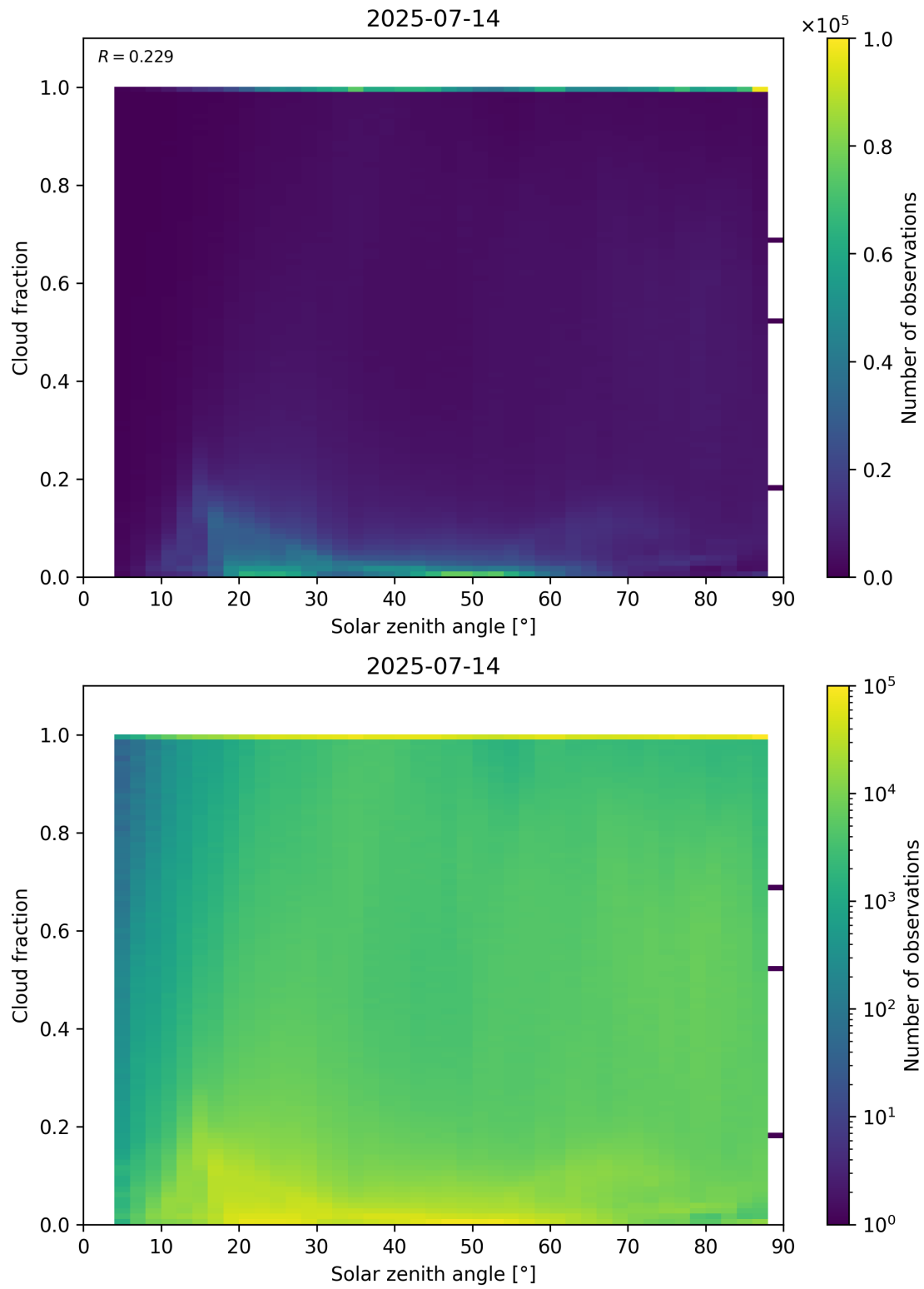
Figure 110: Scatter density plot of “Solar zenith angle” against “Cloud fraction” for 2025-07-13 to 2025-07-15.
