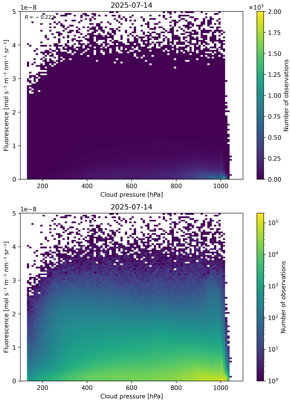
Figure 80: Scatter density plot of “Cloud pressure” against “Fluorescence” for 2025-07-13 to 2025-07-15.
