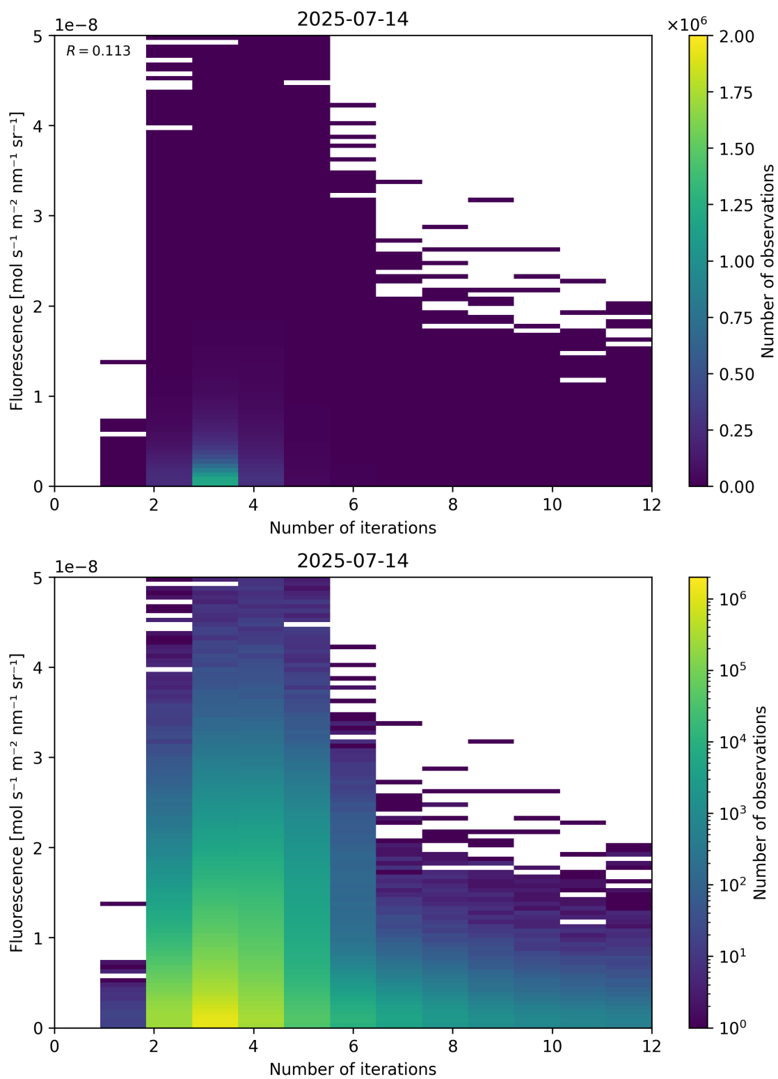
Figure 98: Scatter density plot of “Number of iterations” against “Fluorescence” for 2025-07-13 to 2025-07-15.
