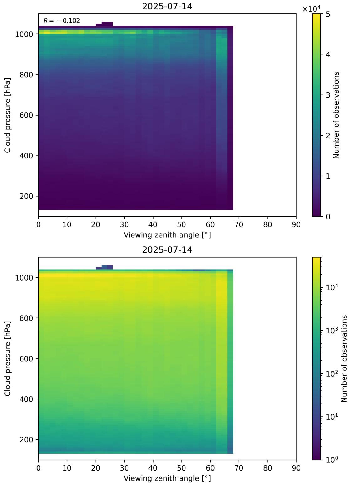
Figure 121: Scatter density plot of “Viewing zenith angle” against “Cloud pressure” for 2025-07-13 to 2025-07-15.
