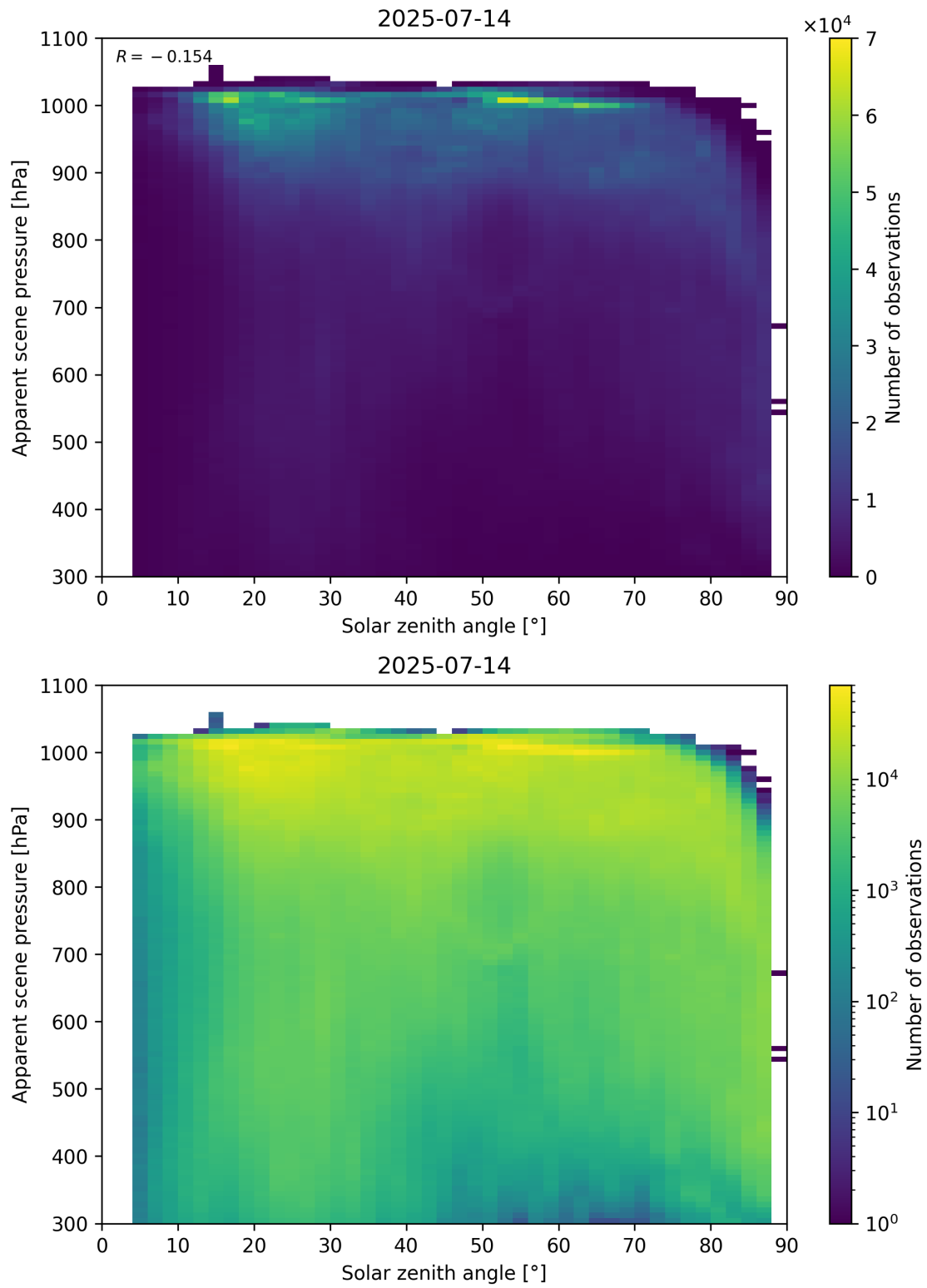
Figure 108: Scatter density plot of “Solar zenith angle” against “Apparent scene pressure” for 2025-07-13 to 2025-07-15.
