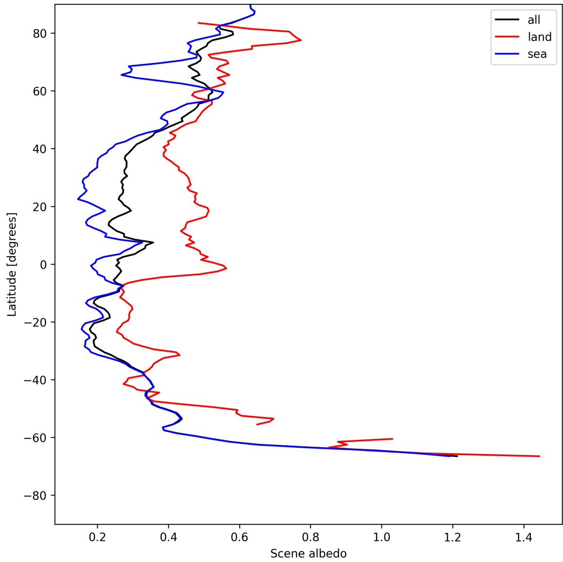
Figure 17: Zonal average of “Scene albedo” for 2025-07-13 to 2025-07-15.
