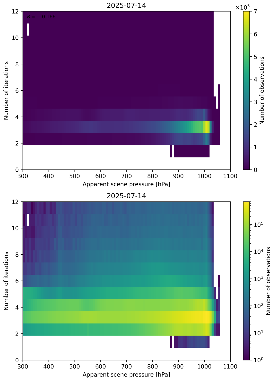
Figure 65: Scatter density plot of “Apparent scene pressure” against “Number of iterations” for 2025-07-13 to 2025-07-15.
