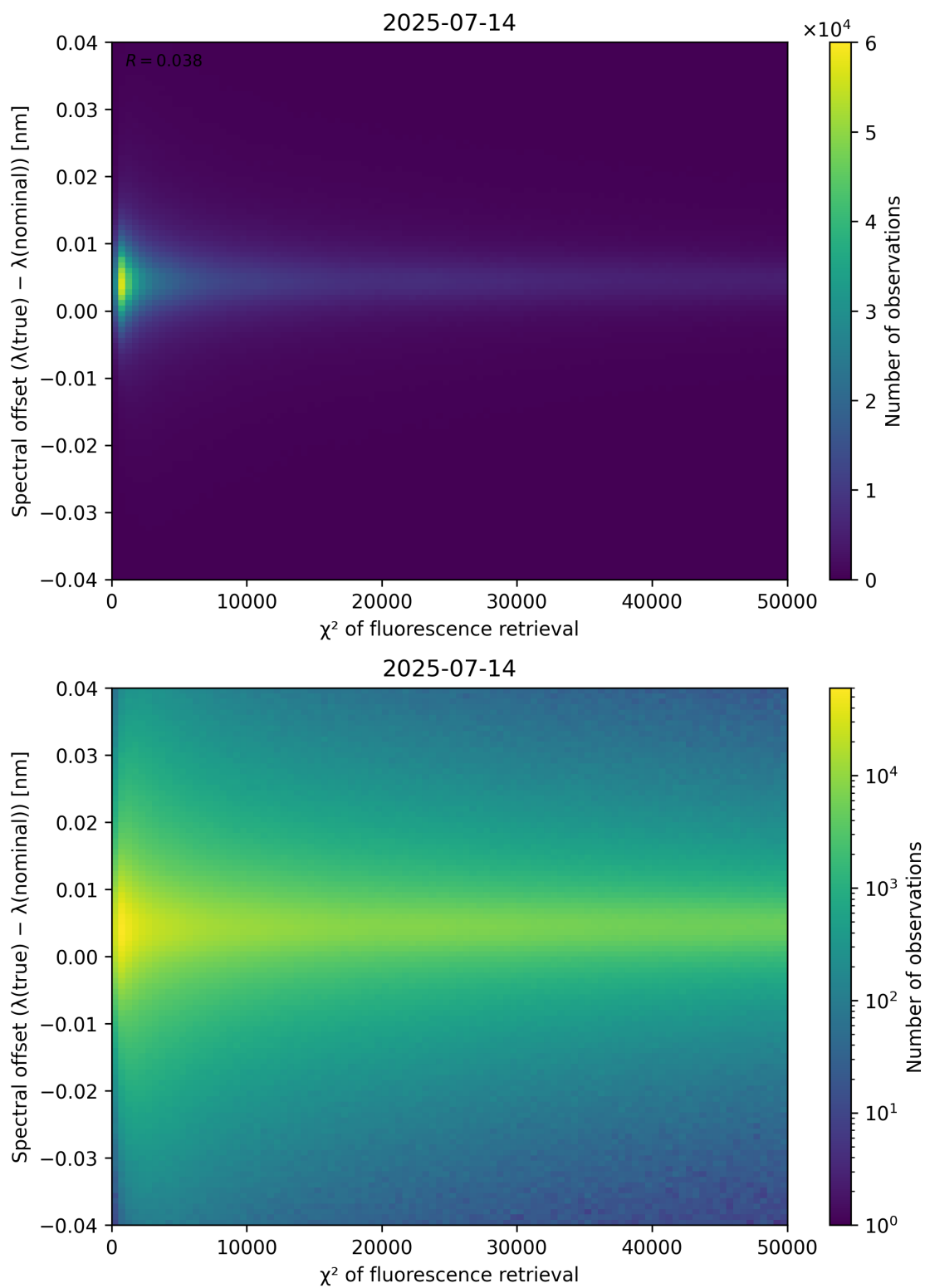
Figure 69: Scatter density plot of “ \chi^2 of fluorescence retrieval” against “Spectral offset ( \lambda_{\text{true}} - \lambda_{\text{nominal}} )” for 2025-07-13 to 2025-07-15.
