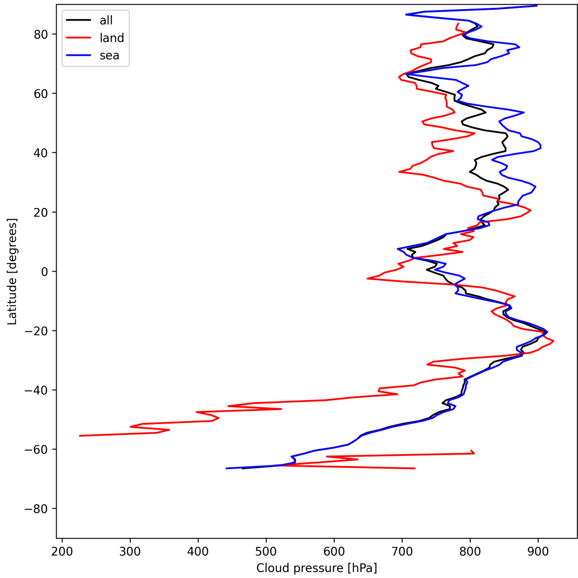
Figure 13: Zonal average of “Cloud pressure” for 2025-07-13 to 2025-07-15.
