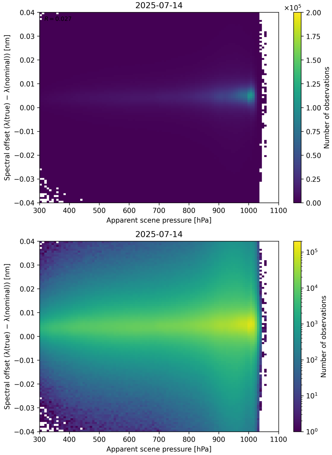
Figure 67: Scatter density plot of “Apparent scene pressure” against “Spectral offset ( \lambda_{\text{true}} - \lambda_{\text{nominal}} )” for 2025-07-13 to 2025-07-15.
