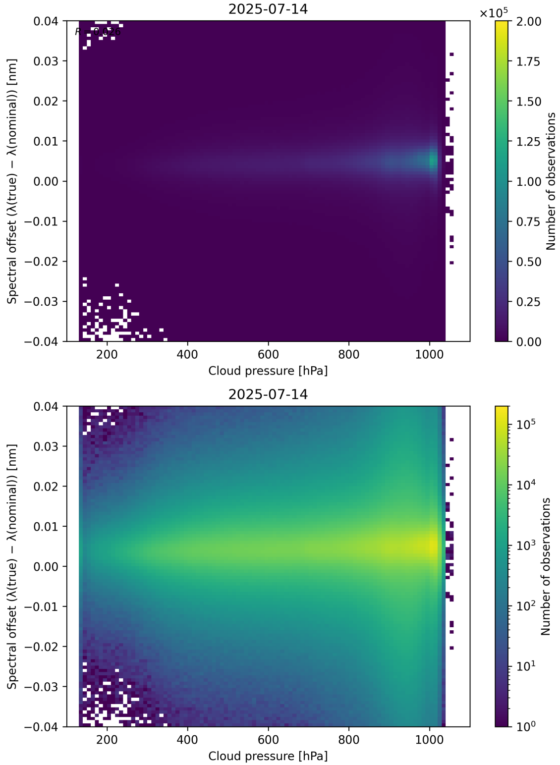
Figure 84: Scatter density plot of “Cloud pressure” against “Spectral offset ( \lambda_{\text{true}} - \lambda_{\text{nominal}} )” for 2025-07-13 to 2025-07-15.
