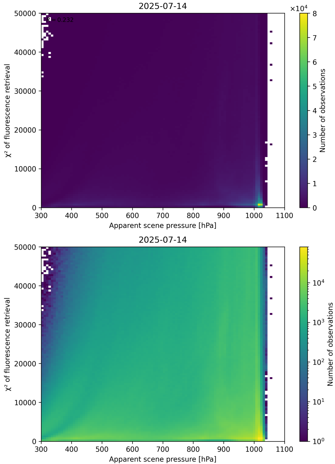
Figure 63: Scatter density plot of “Apparent scene pressure” against “ \chi^2 of fluorescence retrieval” for 2025-07-13 to 2025-07-15.
