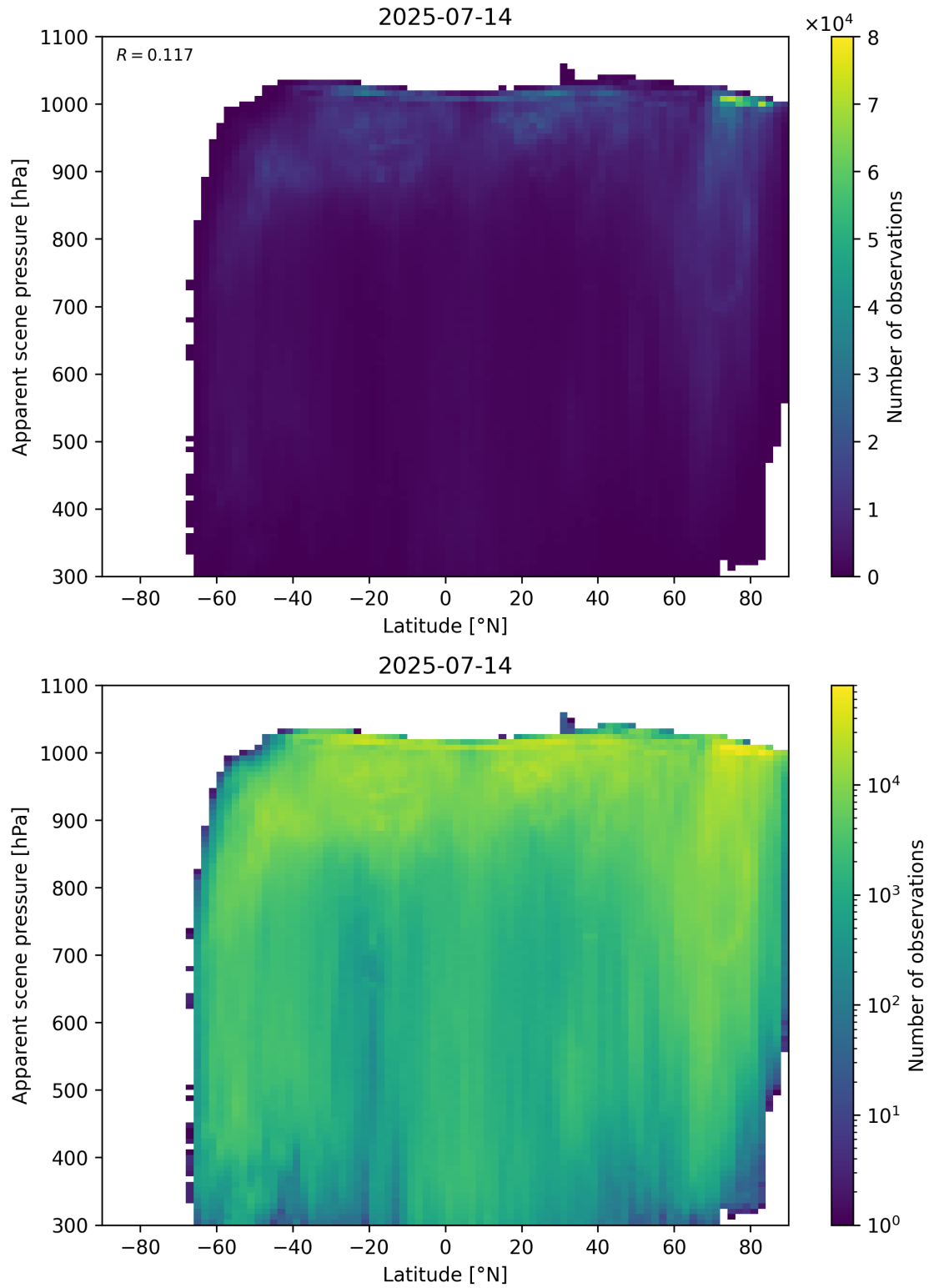
Figure 88: Scatter density plot of “Latitude” against “Apparent scene pressure” for 2025-07-13 to 2025-07-15.
