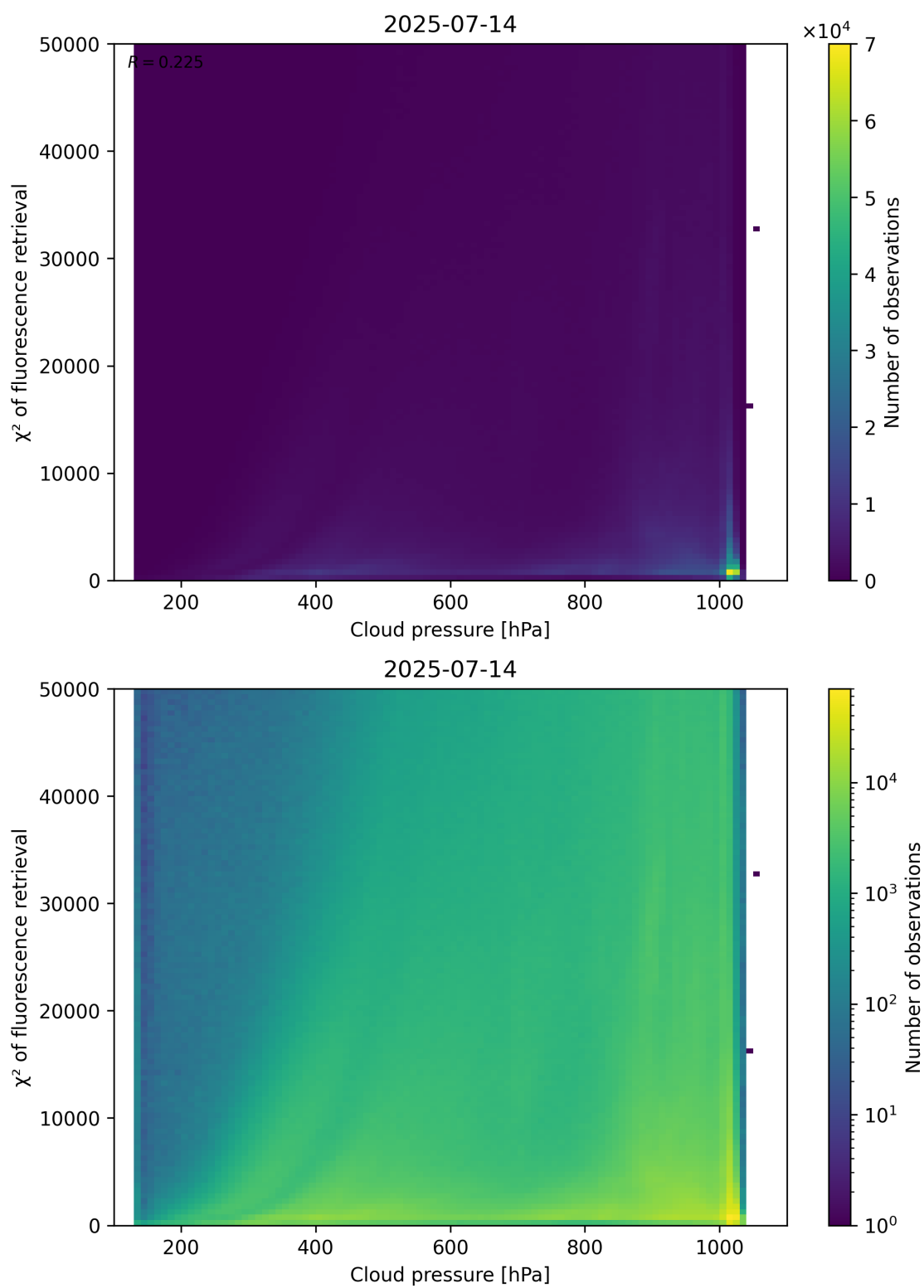
Figure 78: Scatter density plot of “Cloud pressure” against “ \chi^2 of fluorescence retrieval” for 2025-07-13 to 2025-07-15.
