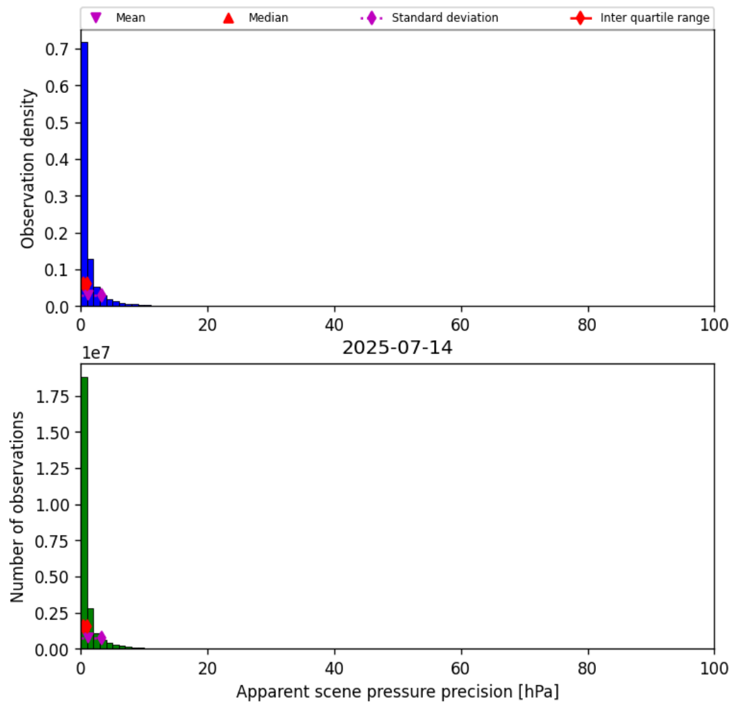
Figure 37: Histogram of “Apparent scene pressure precision” for 2025-07-13 to 2025-07-15
