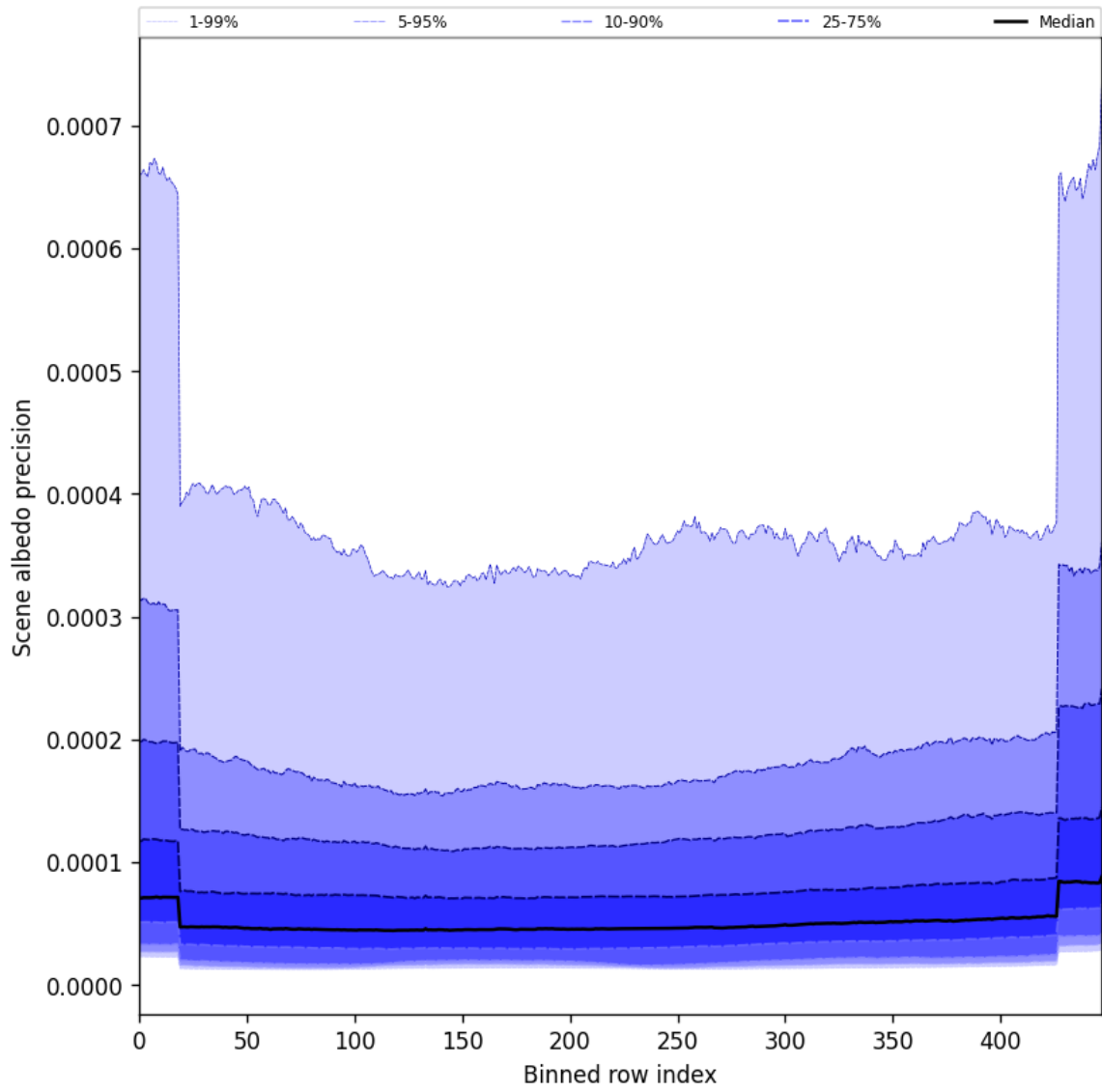
Figure 52: Along track statistics of “Scene albedo precision” for 2025-07-13 to 2025-07-15
