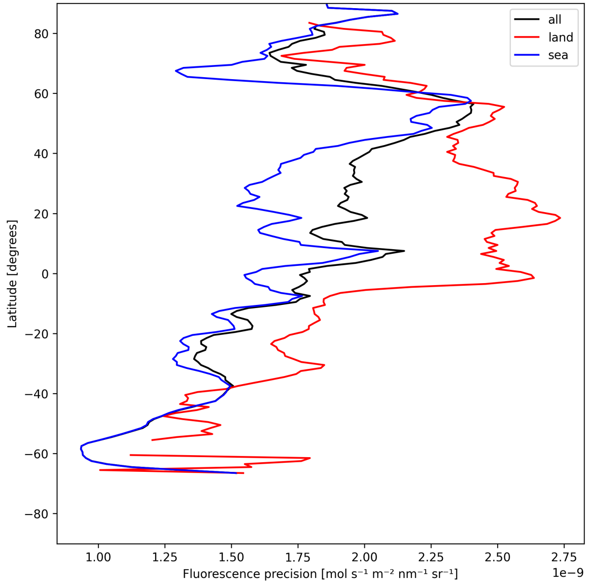
Figure 24: Zonal average of “Fluorescence precision” for 2025-07-13 to 2025-07-15.
