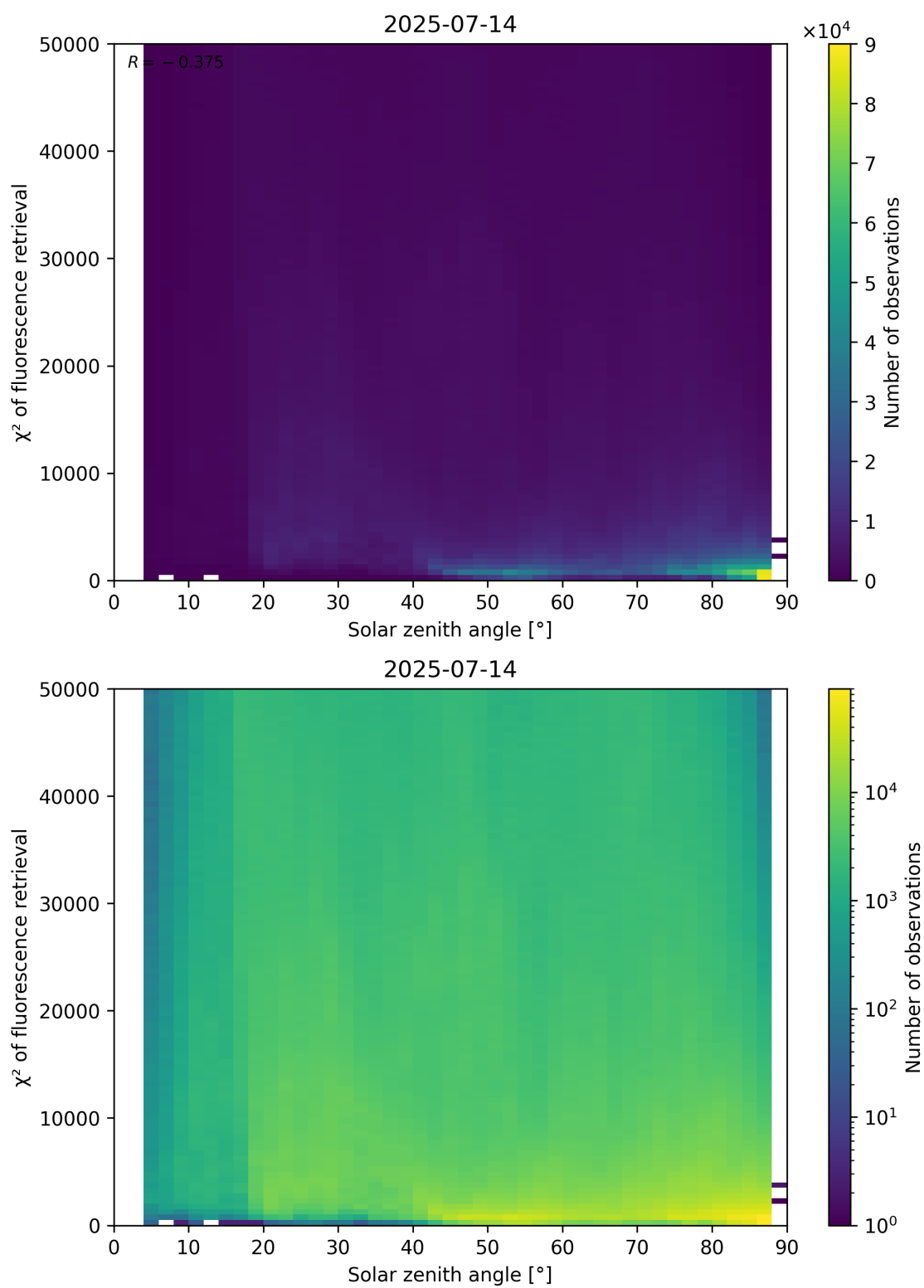
Figure 109: Scatter density plot of “Solar zenith angle” against “ \chi^2 of fluorescence retrieval” for 2025-07-13 to 2025-07-15.
