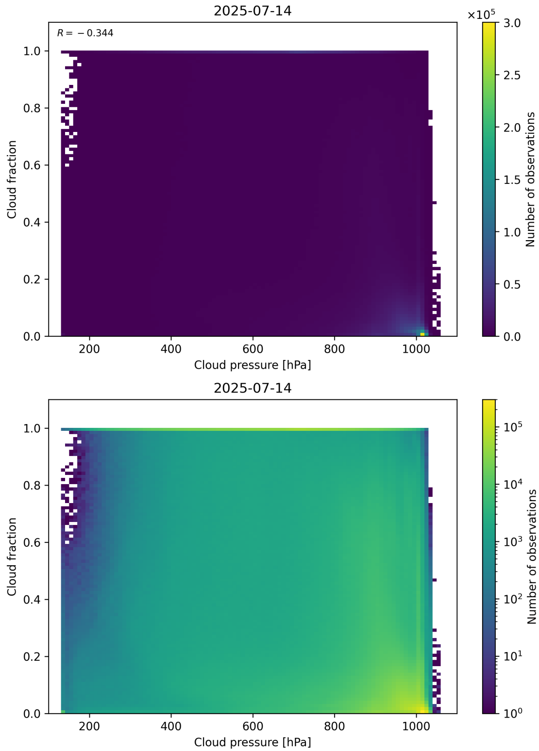
Figure 79: Scatter density plot of “Cloud pressure” against “Cloud fraction” for 2025-07-13 to 2025-07-15.
