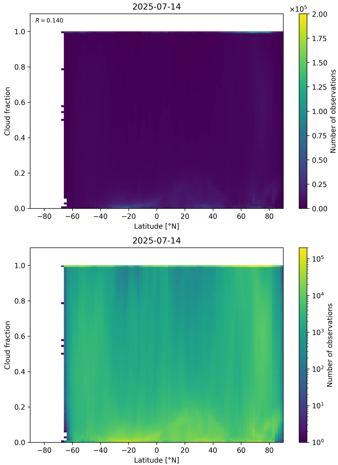
Figure 90: Scatter density plot of “Latitude” against “Cloud fraction” for 2025-07-13 to 2025-07-15.
