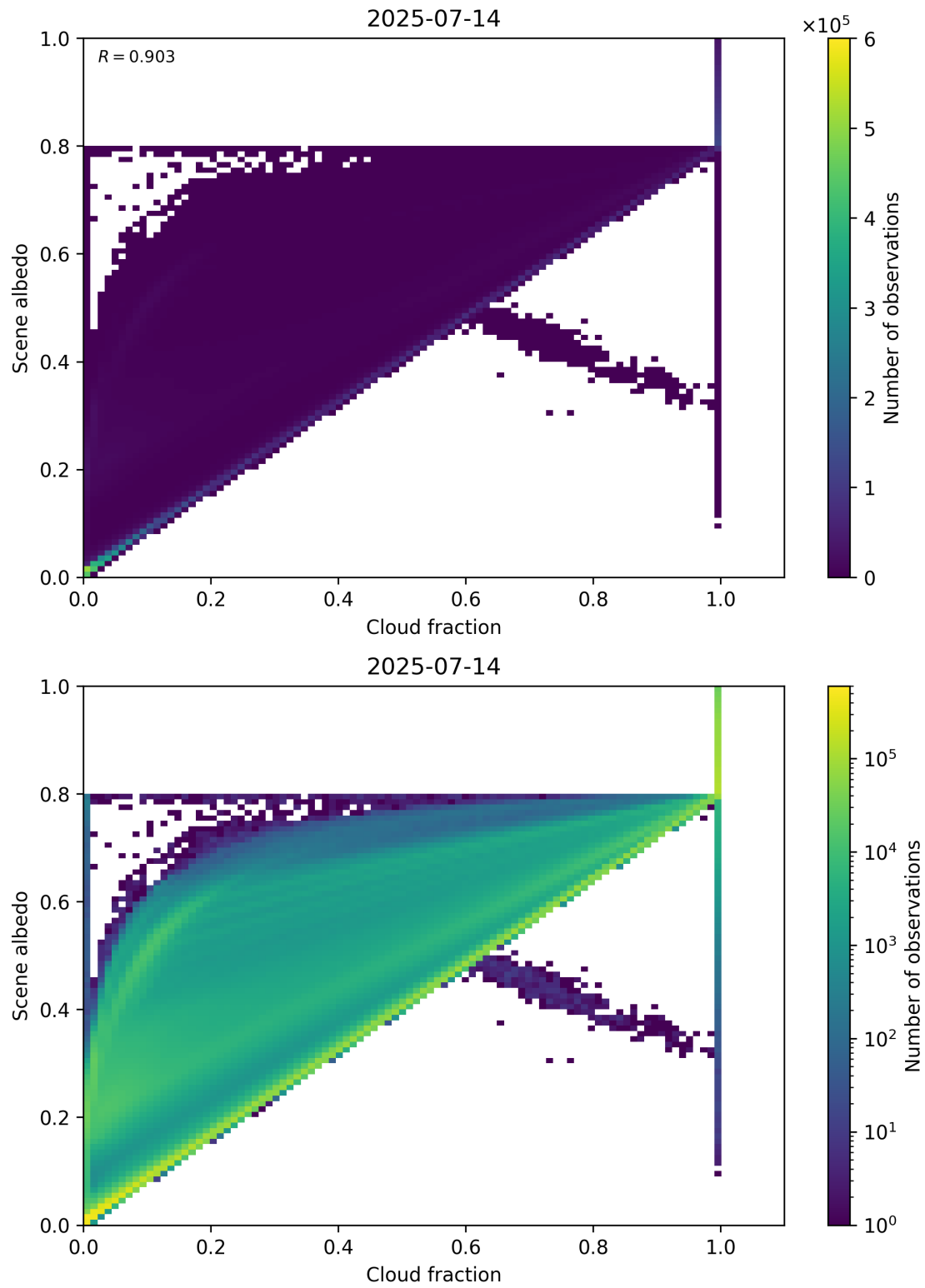
Figure 75: Scatter density plot of “Cloud fraction” against “Scene albedo” for 2025-07-13 to 2025-07-15.
