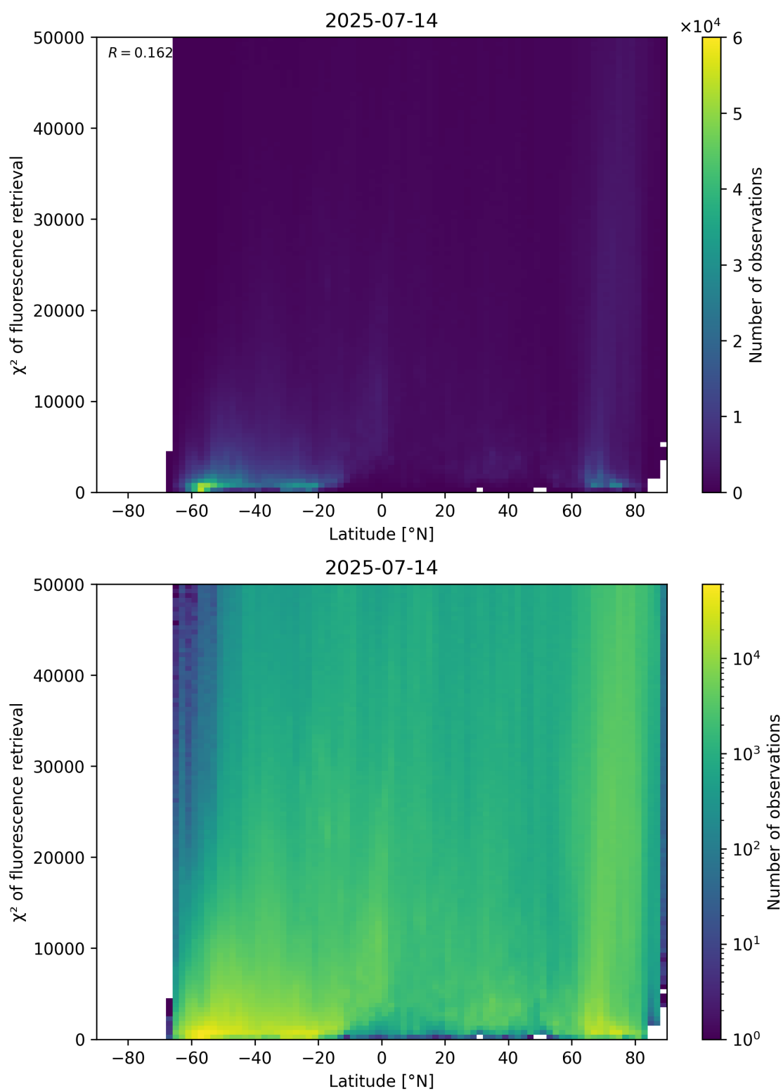
Figure 89: Scatter density plot of “Latitude” against “ \chi^2 of fluorescence retrieval” for 2025-07-13 to 2025-07-15.
