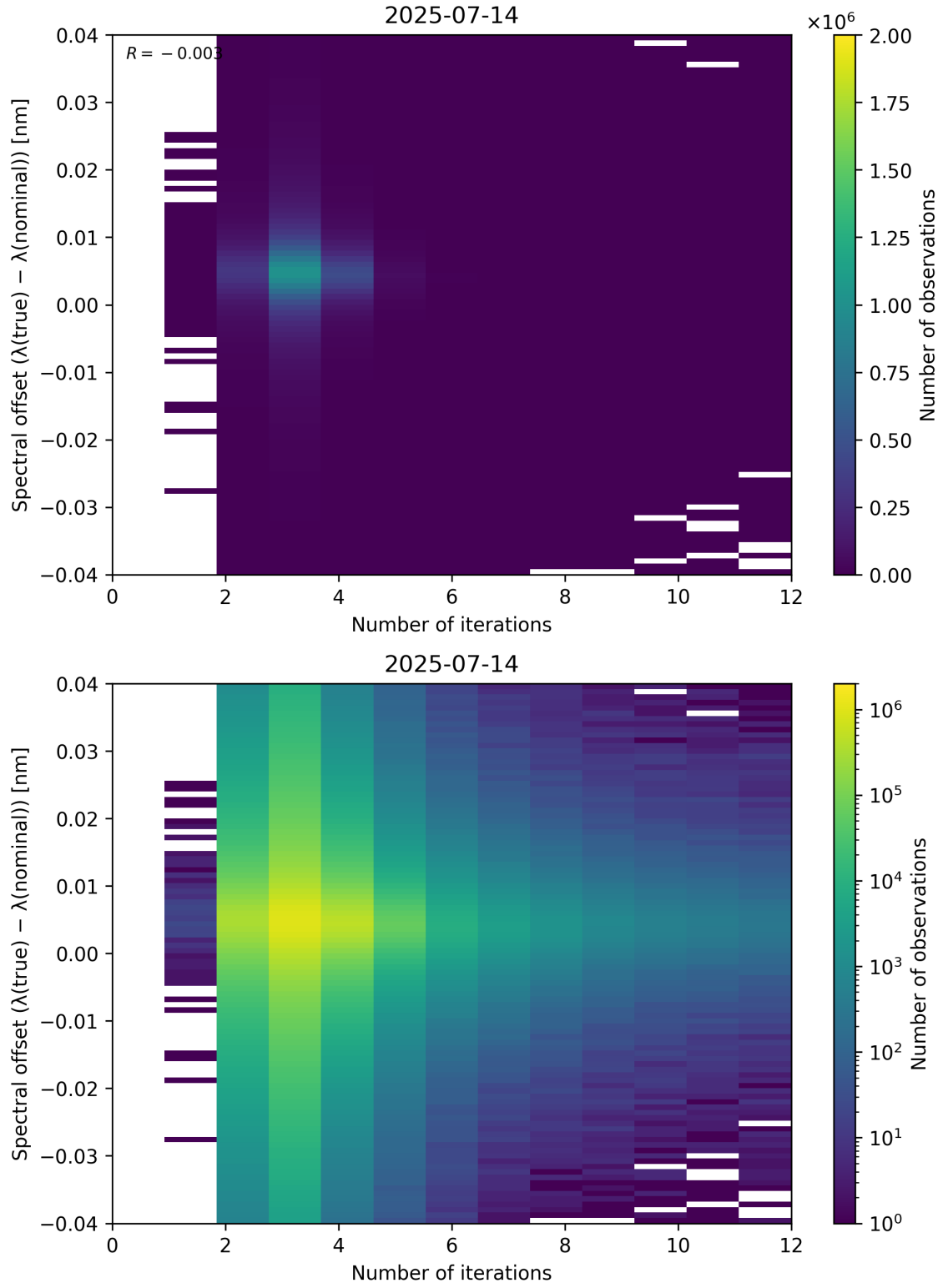
Figure 100: Scatter density plot of “Number of iterations” against “Spectral offset ( \lambda_{\text{true}} - \lambda_{\text{nominal}} )” for 2025-07-13 to 2025-07-15.
