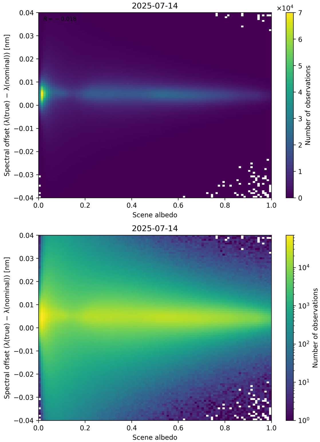
Figure 107: Scatter density plot of “Scene albedo” against “Spectral offset ( \lambda_{\text{true}} - \lambda_{\text{nominal}} )” for 2025-07-13 to 2025-07-15.
