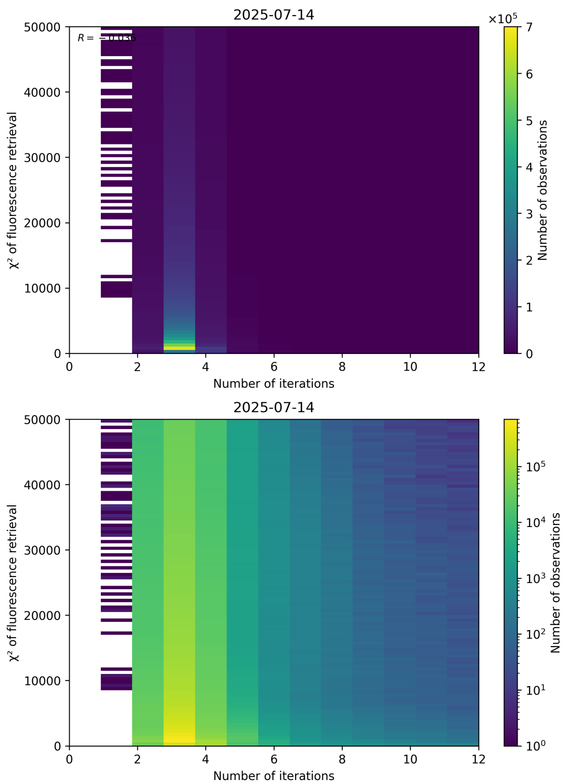
Figure 97: Scatter density plot of “Number of iterations” against “ \chi^2 of fluorescence retrieval” for 2025-07-13 to 2025-07-15.
