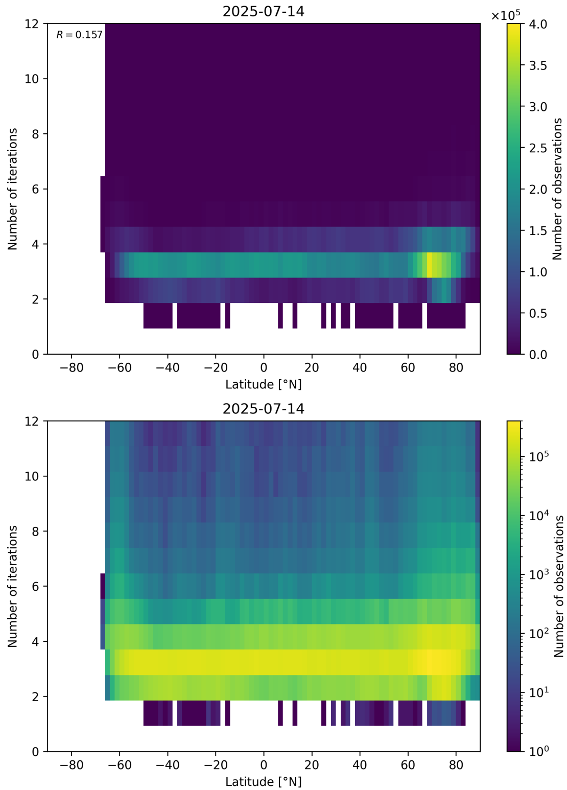
Figure 93: Scatter density plot of “Latitude” against “Number of iterations” for 2025-07-13 to 2025-07-15.
