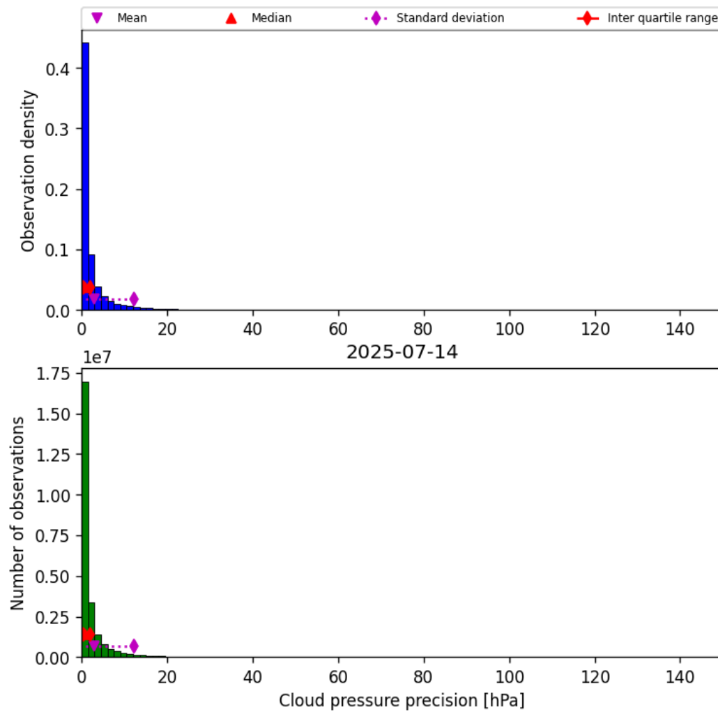
Figure 31: Histogram of “Cloud pressure precision” for 2025-07-13 to 2025-07-15
