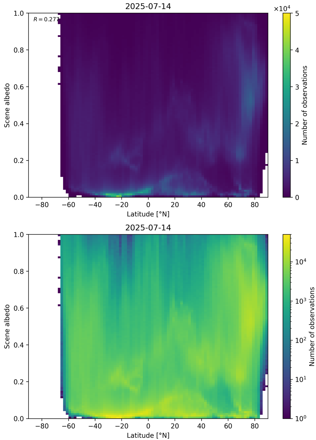
Figure 95: Scatter density plot of “Latitude” against “Scene albedo” for 2025-07-13 to 2025-07-15.
