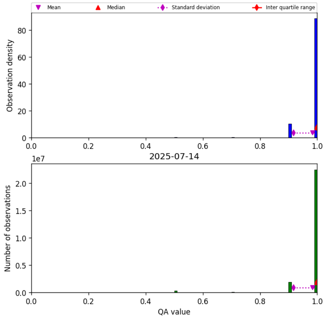
Figure 29: Histogram of “QA value” for 2025-07-13 to 2025-07-15
