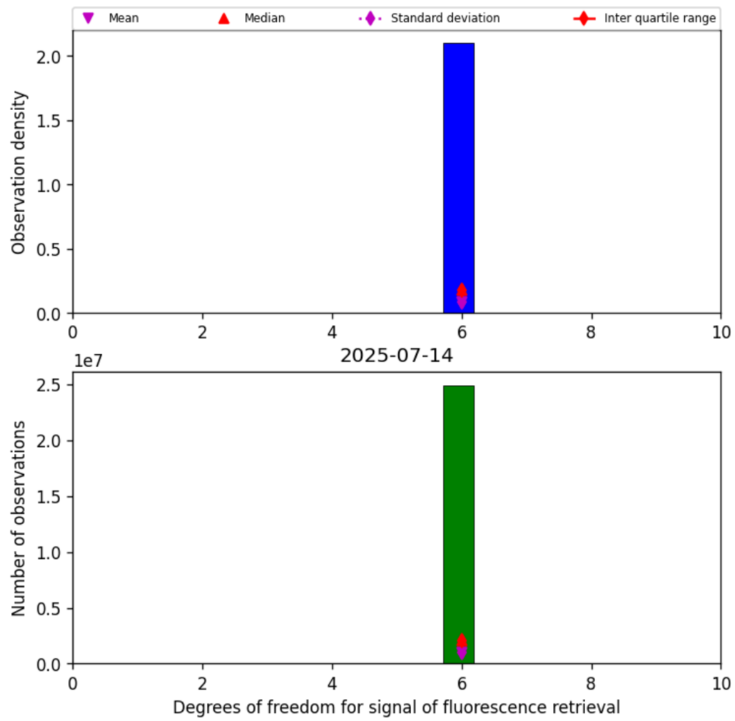
Figure 43: Histogram of “Degrees of freedom for signal of fluorescence retrieval” for 2025-07-13 to 2025-07-15
