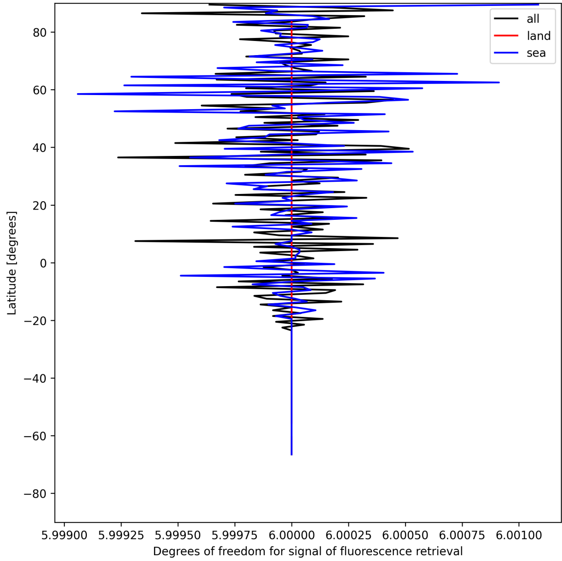
Figure 26: Zonal average of “Degrees of freedom for signal of fluorescence retrieval” for 2025-07-13 to 2025-07-15.
