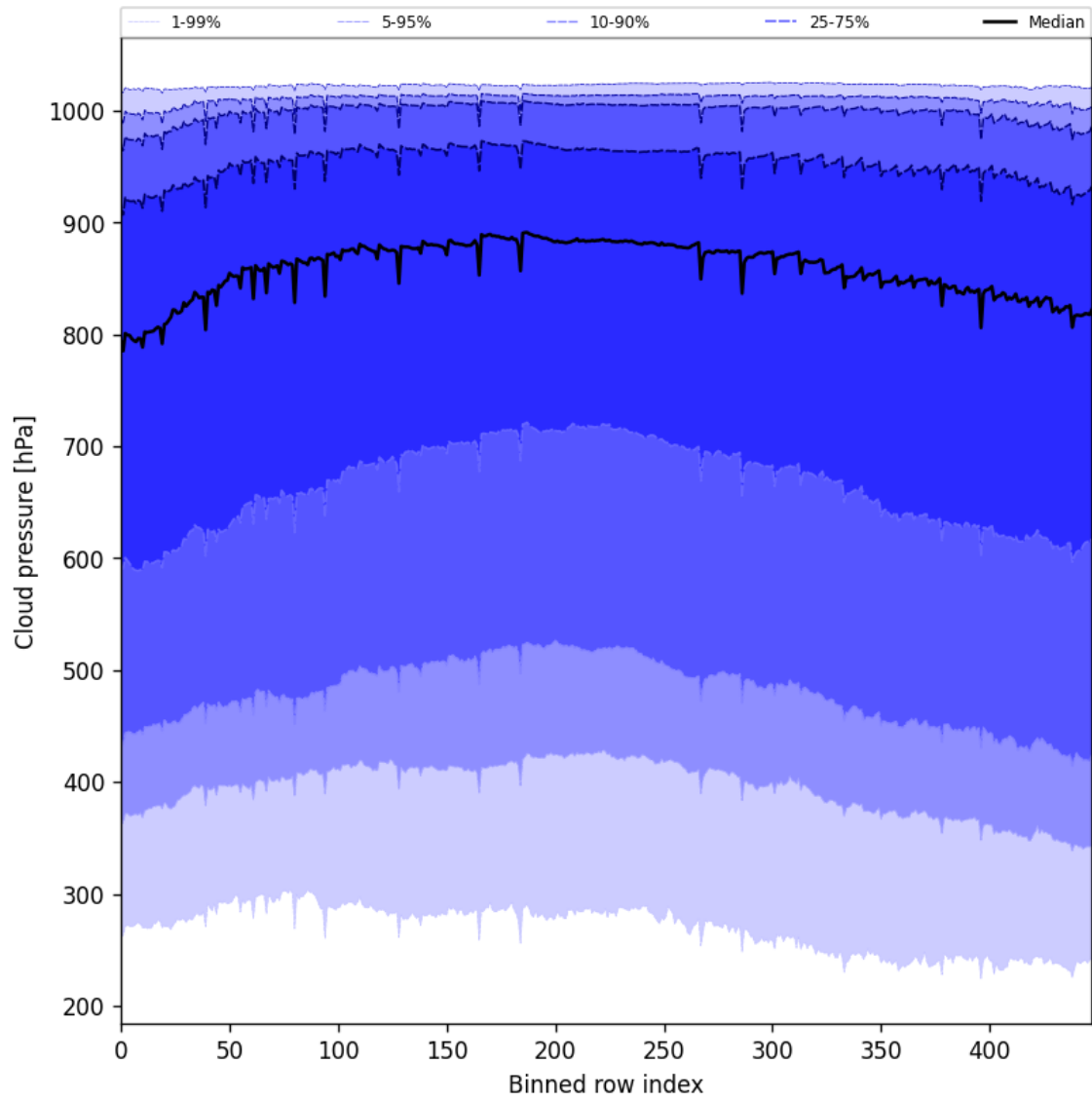
Figure 47: Along track statistics of “Cloud pressure” for 2025-07-13 to 2025-07-15
