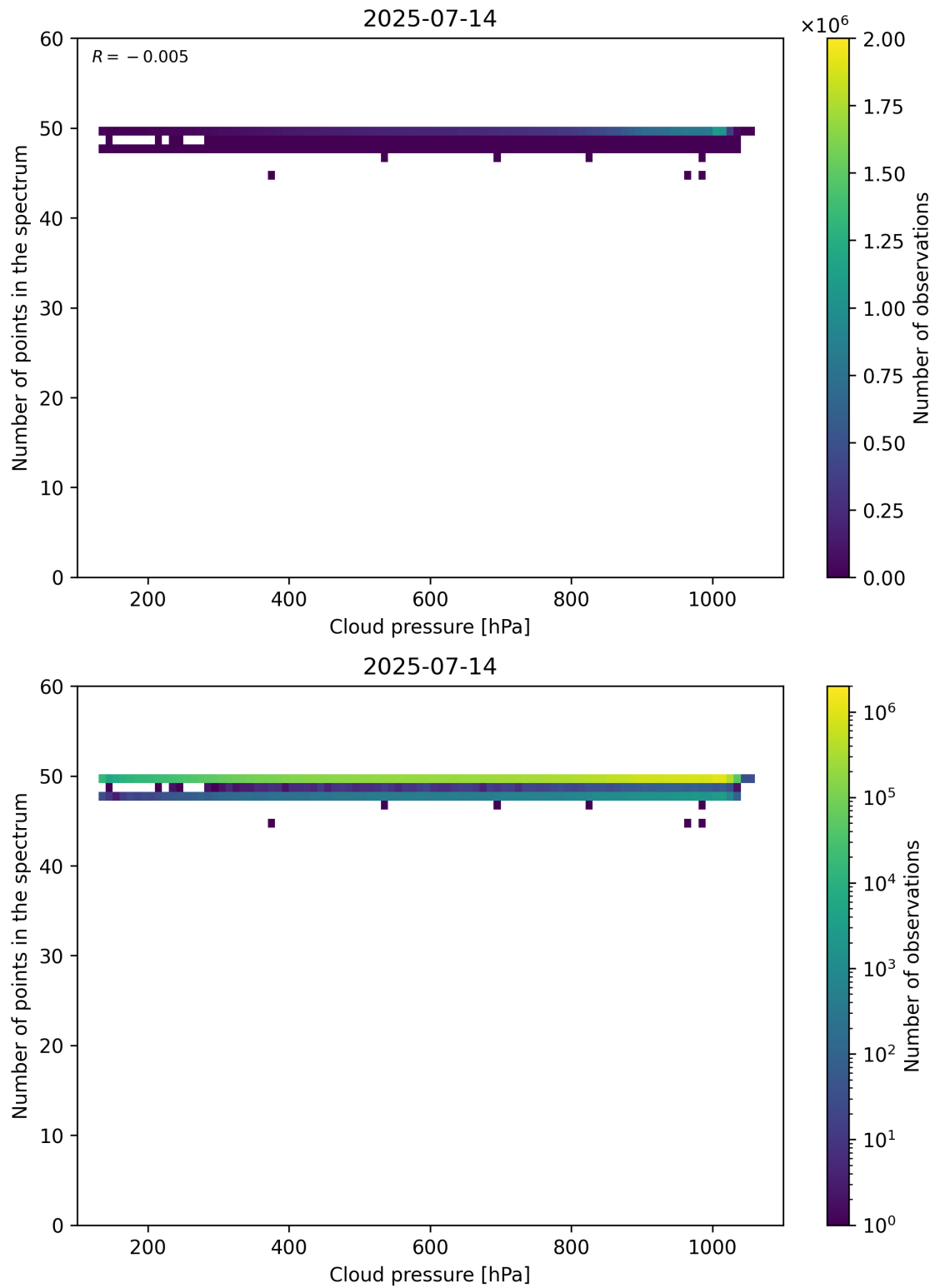
Figure 82: Scatter density plot of “Cloud pressure” against “Number of points in the spectrum” for 2025-07-13 to 2025-07-15.
