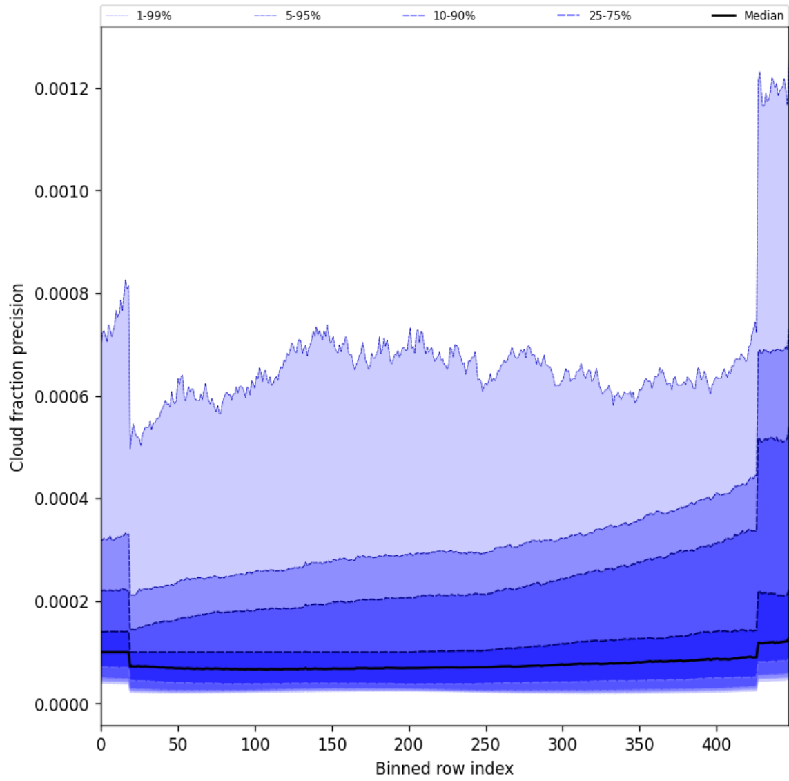
Figure 50: Along track statistics of “Cloud fraction precision” for 2025-07-13 to 2025-07-15
