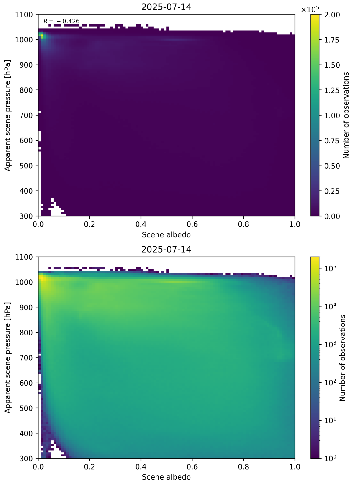
Figure 102: Scatter density plot of “Scene albedo” against “Apparent scene pressure” for 2025-07-13 to 2025-07-15.
