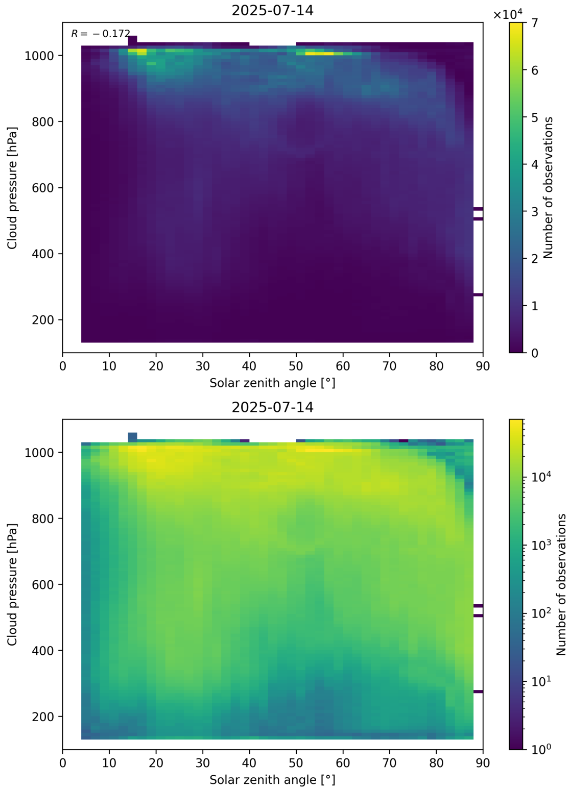
Figure 111: Scatter density plot of “Solar zenith angle” against “Cloud pressure” for 2025-07-13 to 2025-07-15.
