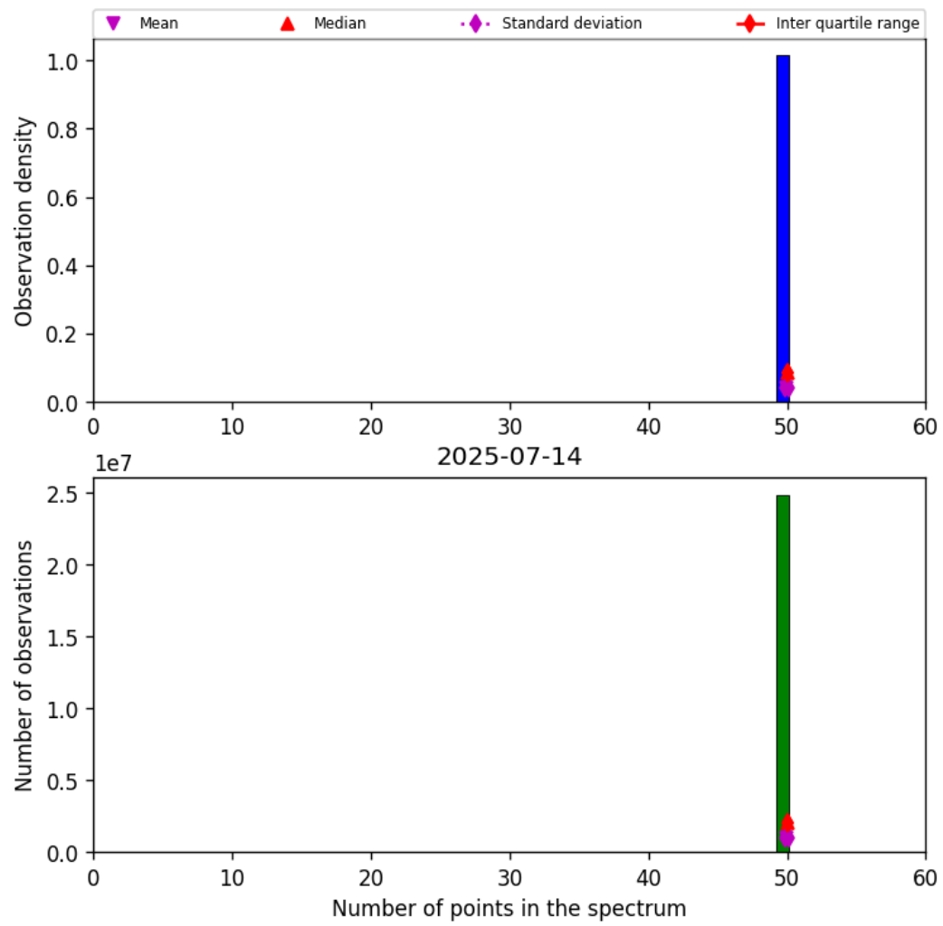
Figure 44: Histogram of “Number of points in the spectrum” for 2025-07-13 to 2025-07-15
