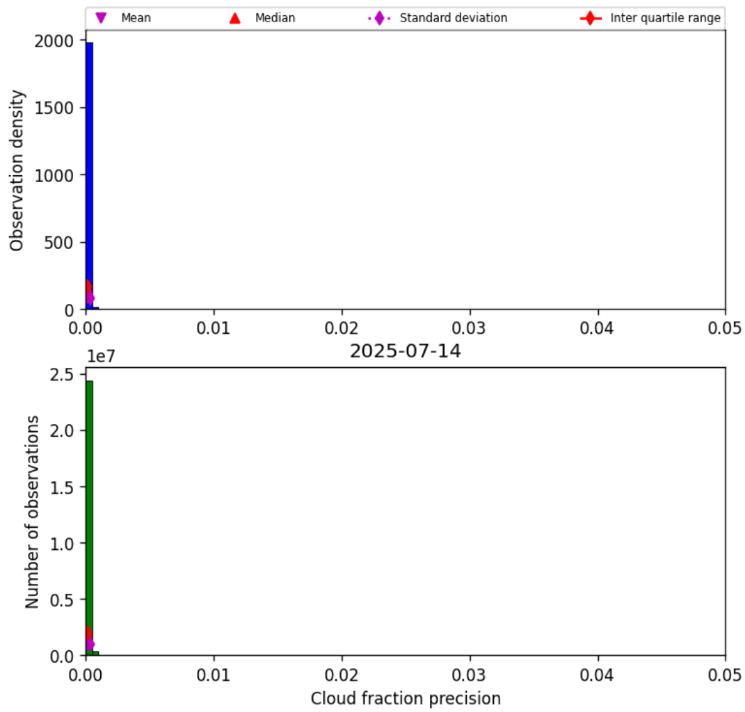
Figure 33: Histogram of “Cloud fraction precision” for 2025-07-13 to 2025-07-15
