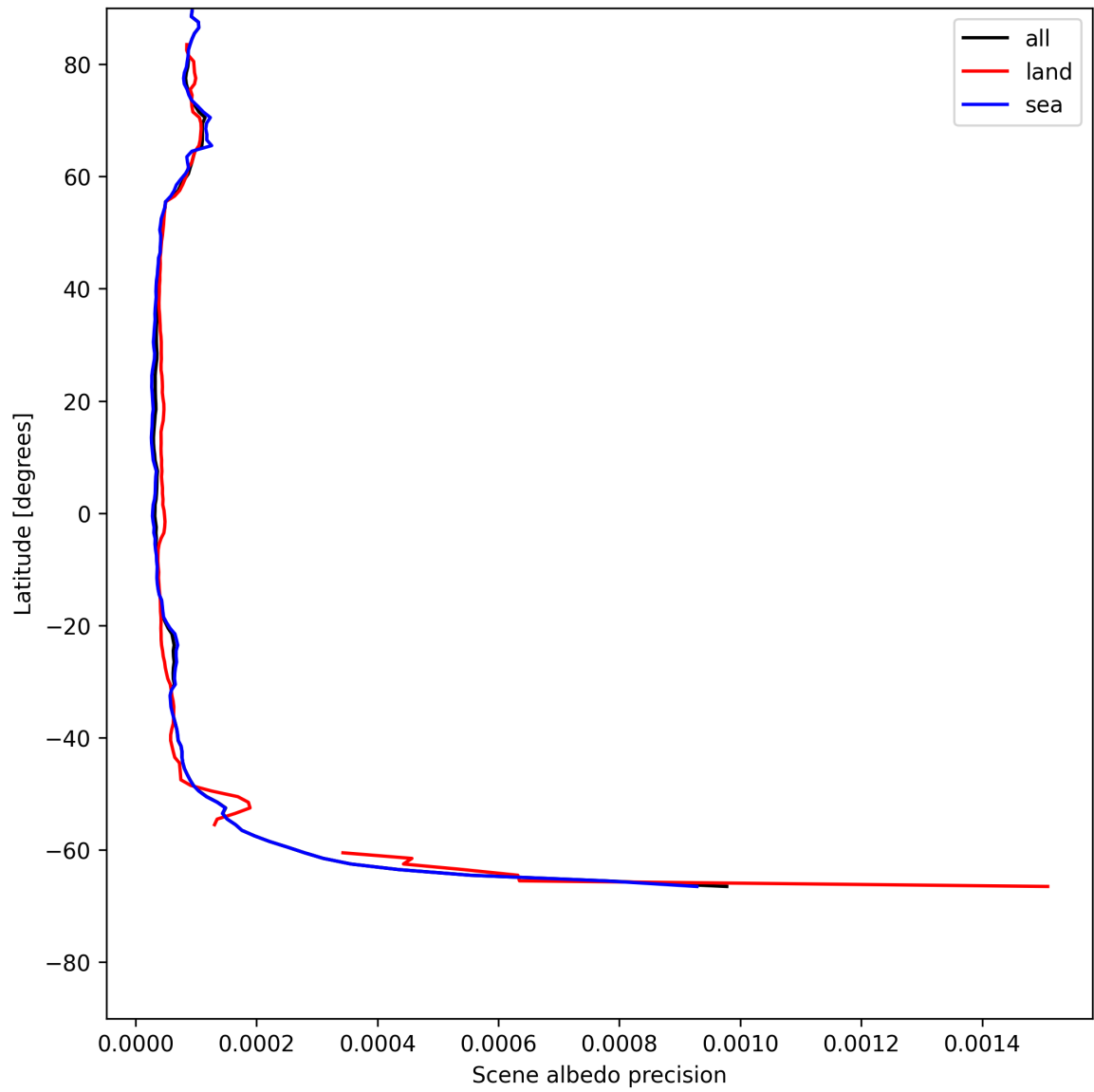
Figure 18: Zonal average of “Scene albedo precision” for 2025-07-13 to 2025-07-15.
