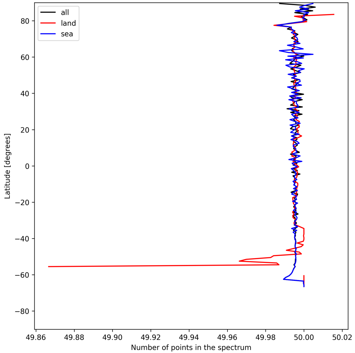
Figure 27: Zonal average of “Number of points in the spectrum” for 2025-07-13 to 2025-07-15.
