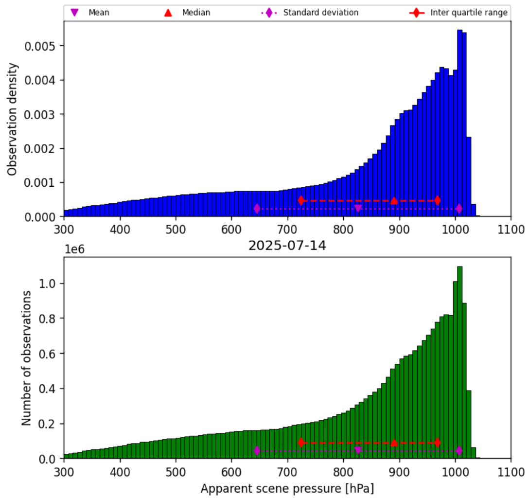
Figure 36: Histogram of “Apparent scene pressure” for 2025-07-13 to 2025-07-15
