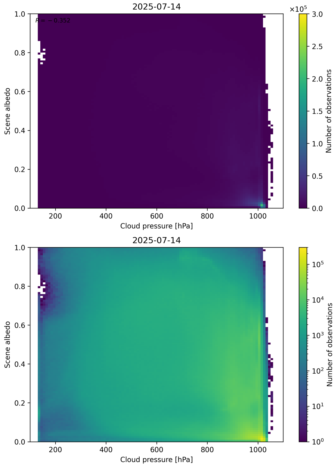
Figure 83: Scatter density plot of “Cloud pressure” against “Scene albedo” for 2025-07-13 to 2025-07-15.
