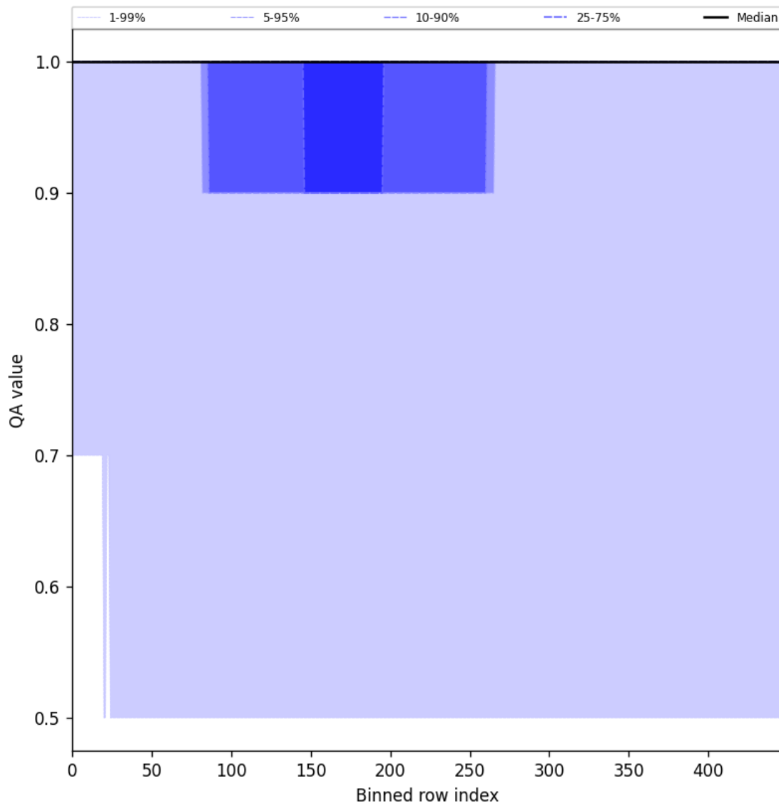
Figure 46: Along track statistics of “QA value” for 2025-07-13 to 2025-07-15
