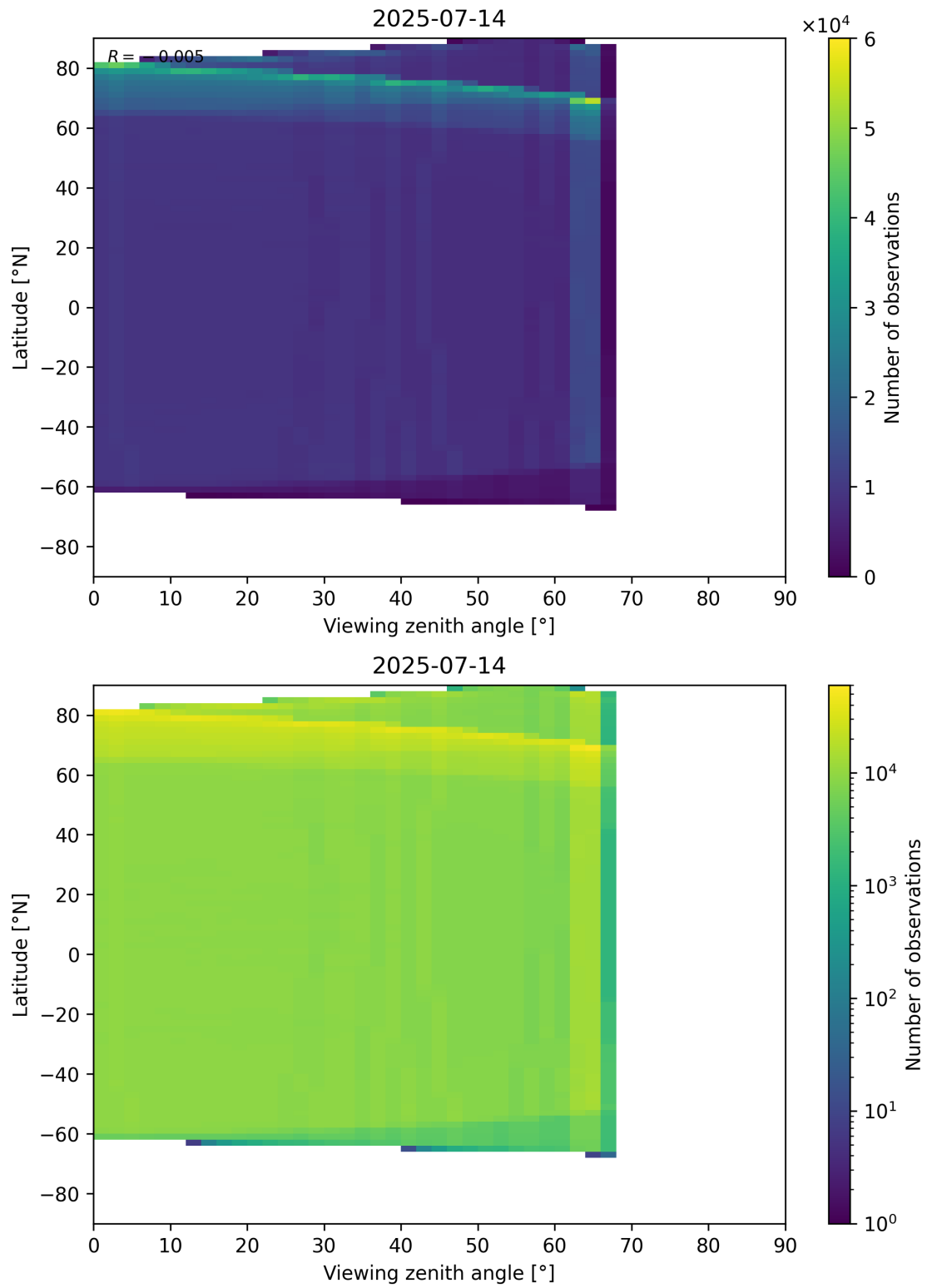
Figure 123: Scatter density plot of “Viewing zenith angle” against “Latitude” for 2025-07-13 to 2025-07-15.
