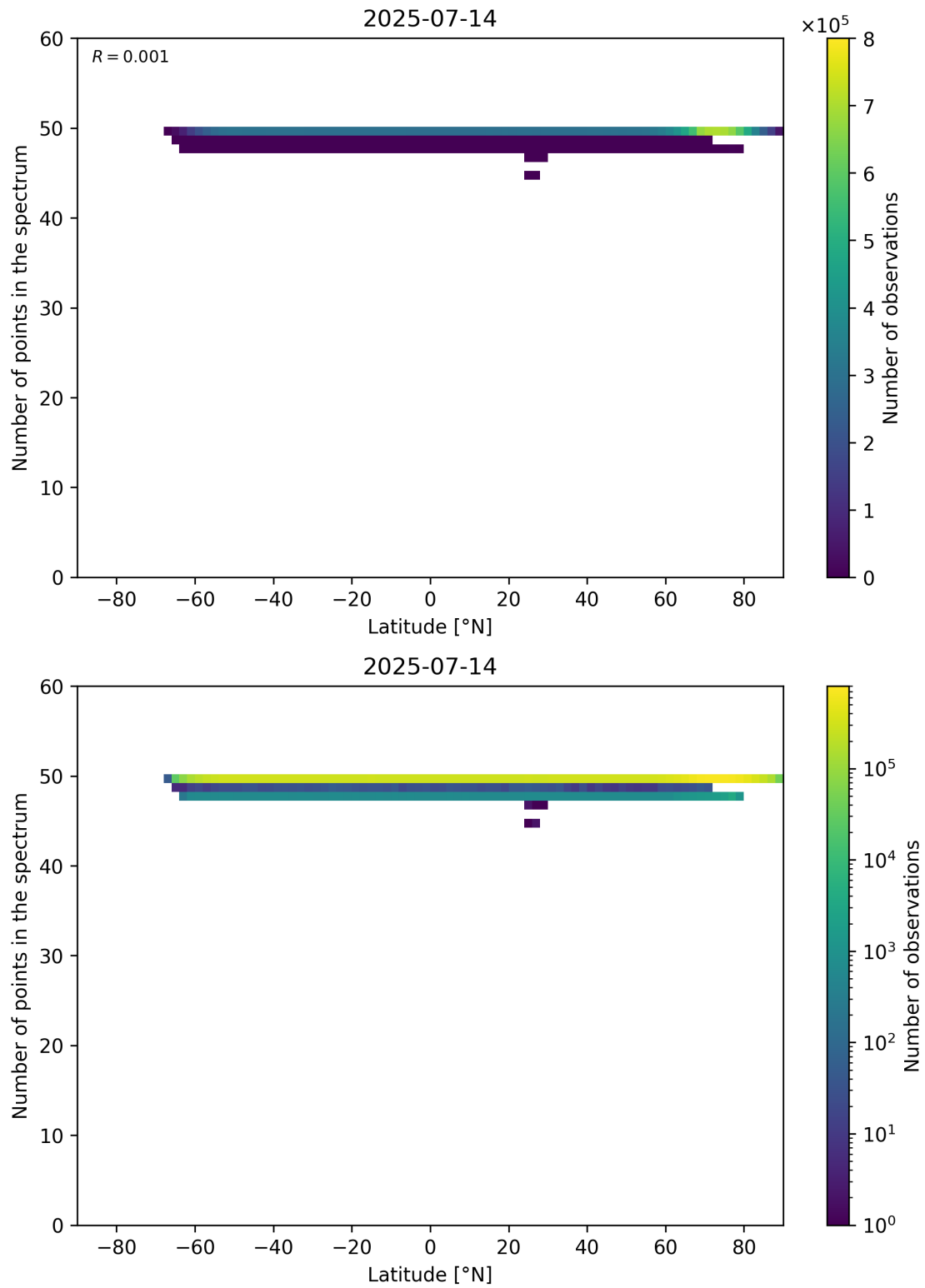
Figure 94: Scatter density plot of “Latitude” against “Number of points in the spectrum” for 2025-07-13 to 2025-07-15.
