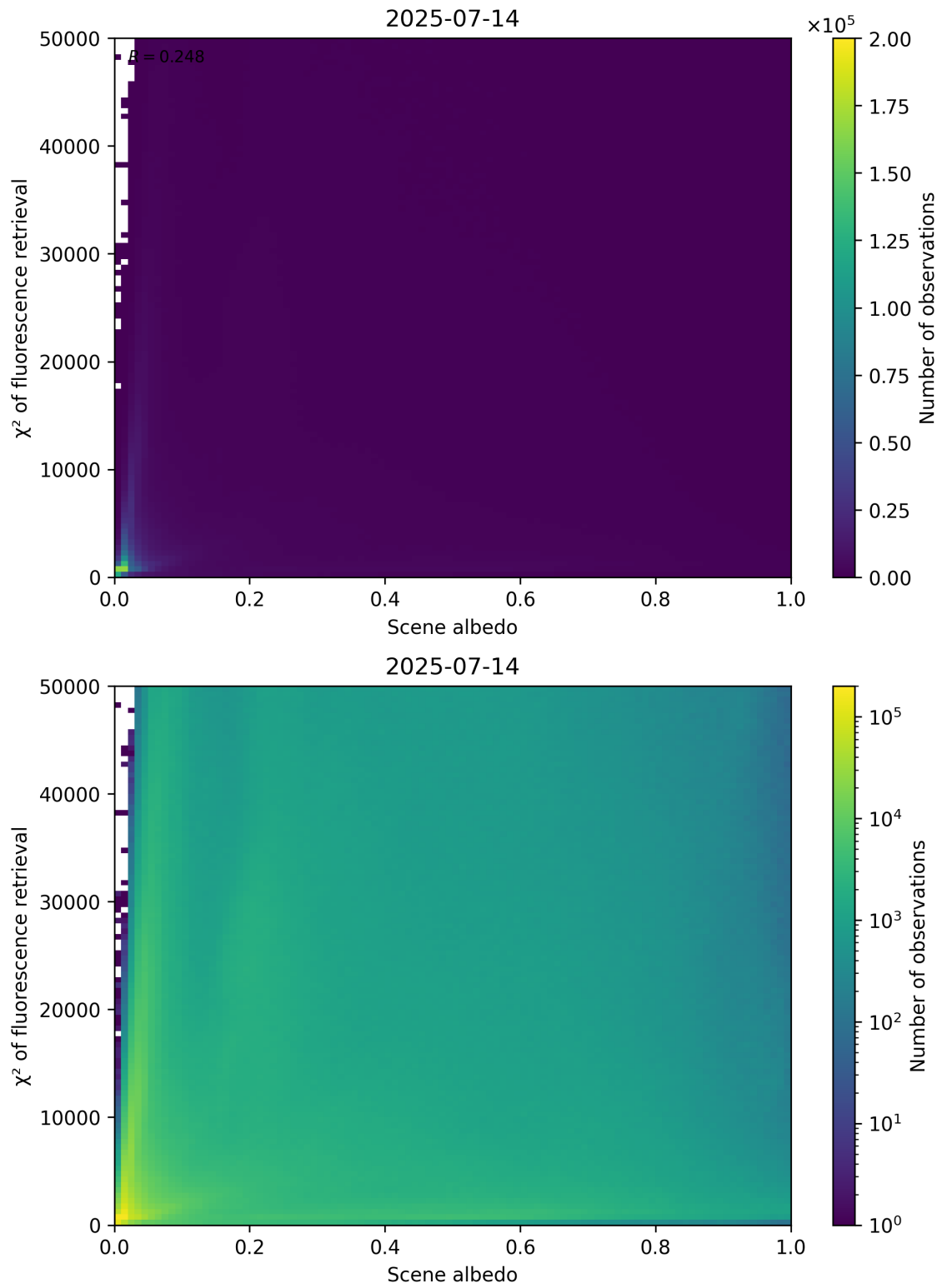
Figure 103: Scatter density plot of “Scene albedo” against “ \chi^2 of fluorescence retrieval” for 2025-07-13 to 2025-07-15.
