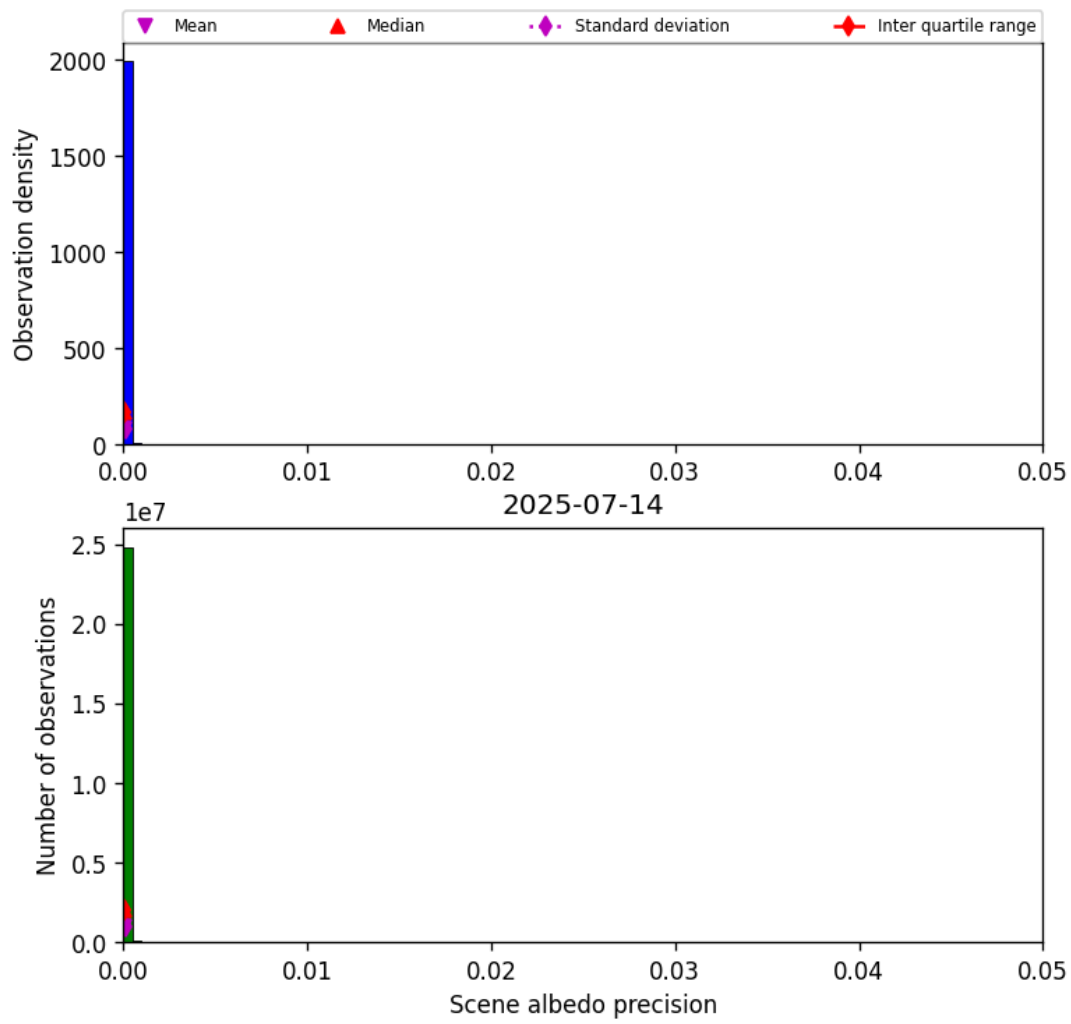
Figure 35: Histogram of “Scene albedo precision” for 2025-07-13 to 2025-07-15
