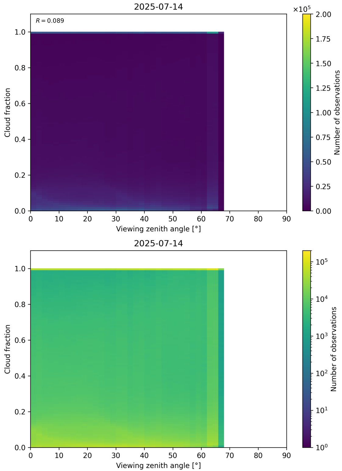
Figure 120: Scatter density plot of “Viewing zenith angle” against “Cloud fraction” for 2025-07-13 to 2025-07-15.
