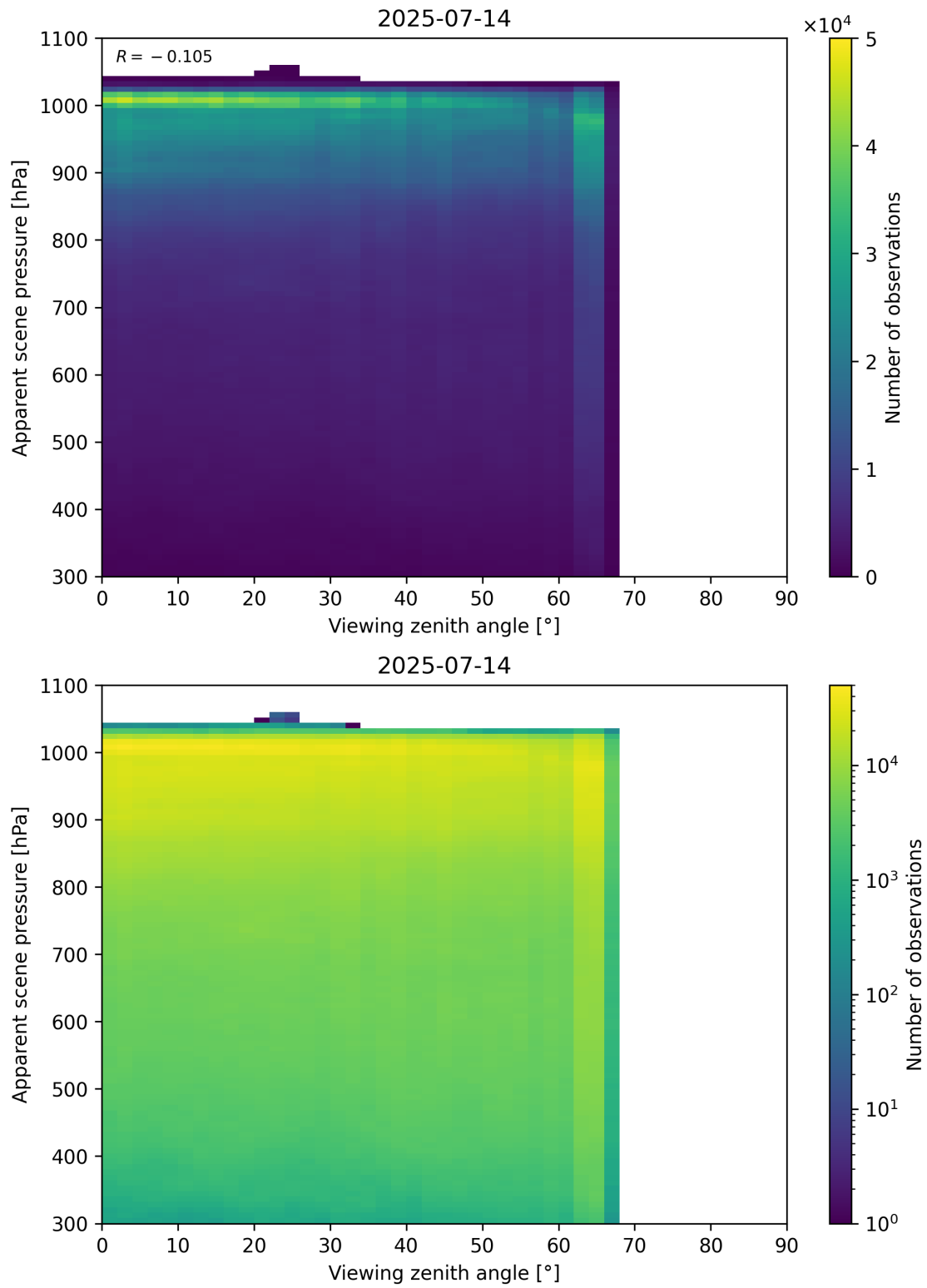
Figure 118: Scatter density plot of “Viewing zenith angle” against “Apparent scene pressure” for 2025-07-13 to 2025-07-15.
