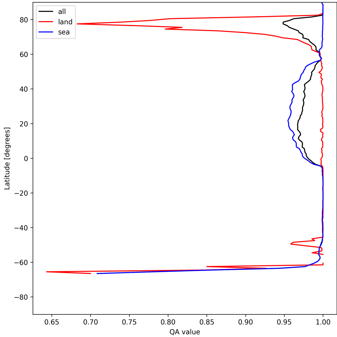
Figure 12: Zonal average of “QA value” for 2025-07-13 to 2025-07-15.
