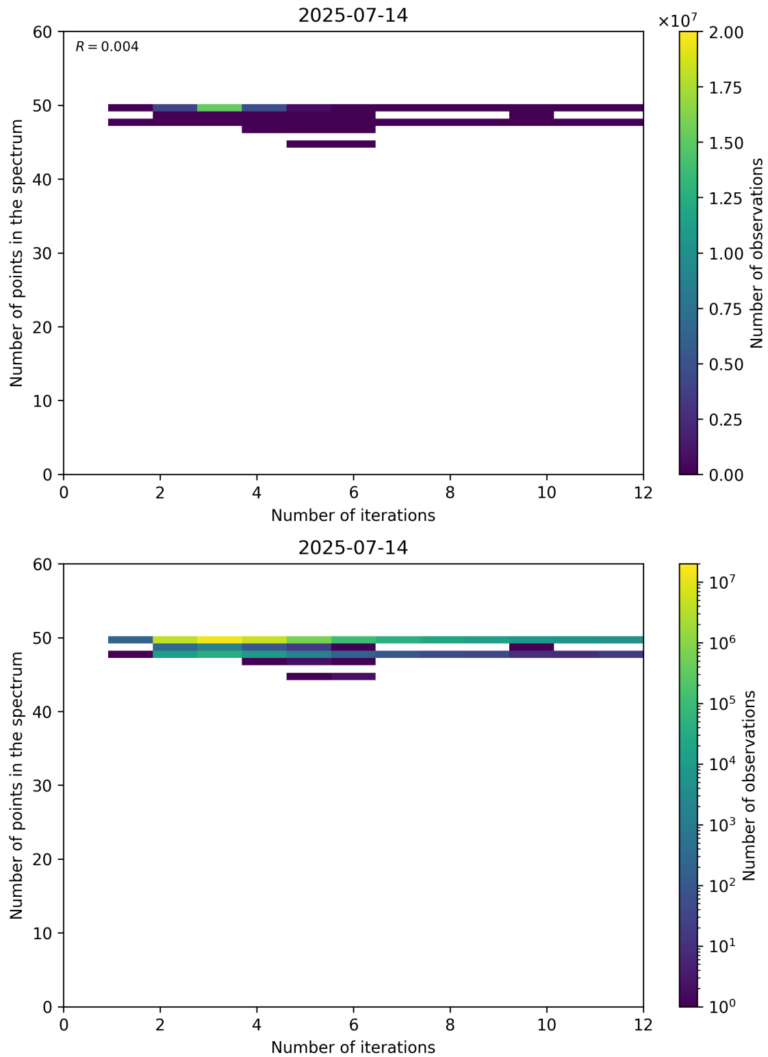
Figure 99: Scatter density plot of “Number of iterations” against “Number of points in the spectrum” for 2025-07-13 to 2025-07-15.
