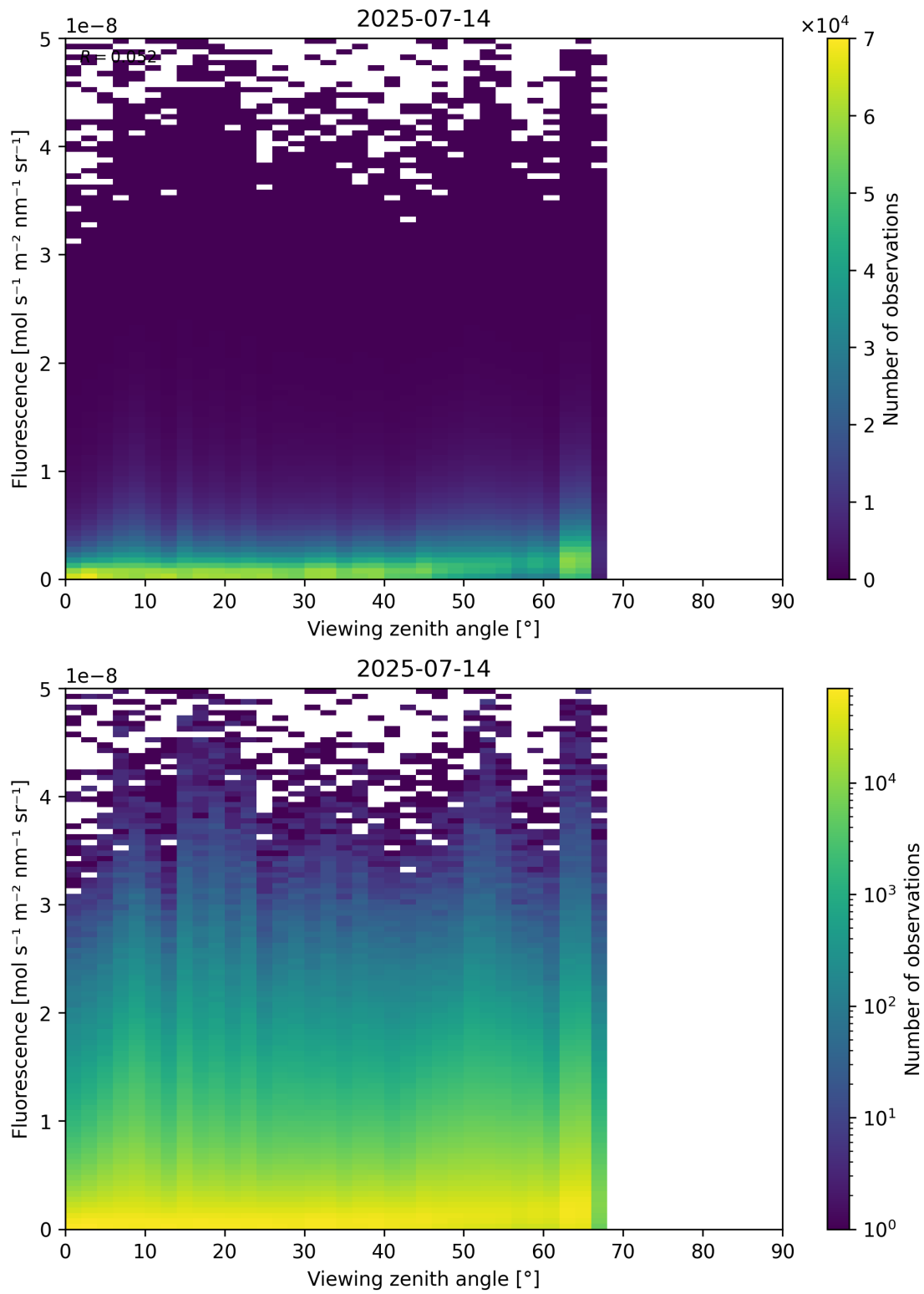
Figure 122: Scatter density plot of “Viewing zenith angle” against “Fluorescence” for 2025-07-13 to 2025-07-15.
