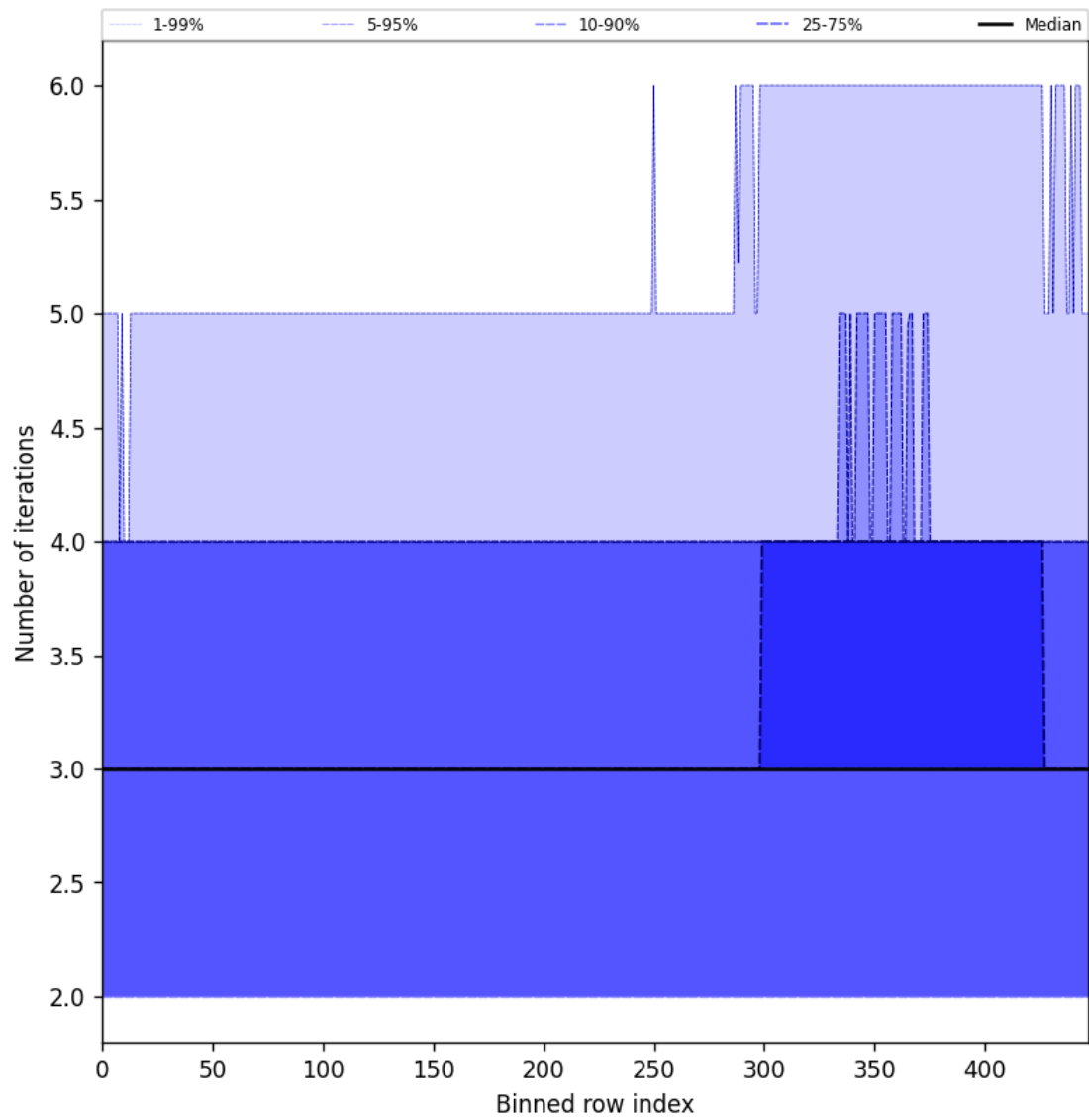
Figure 56: Along track statistics of “Number of iterations” for 2025-07-13 to 2025-07-15
