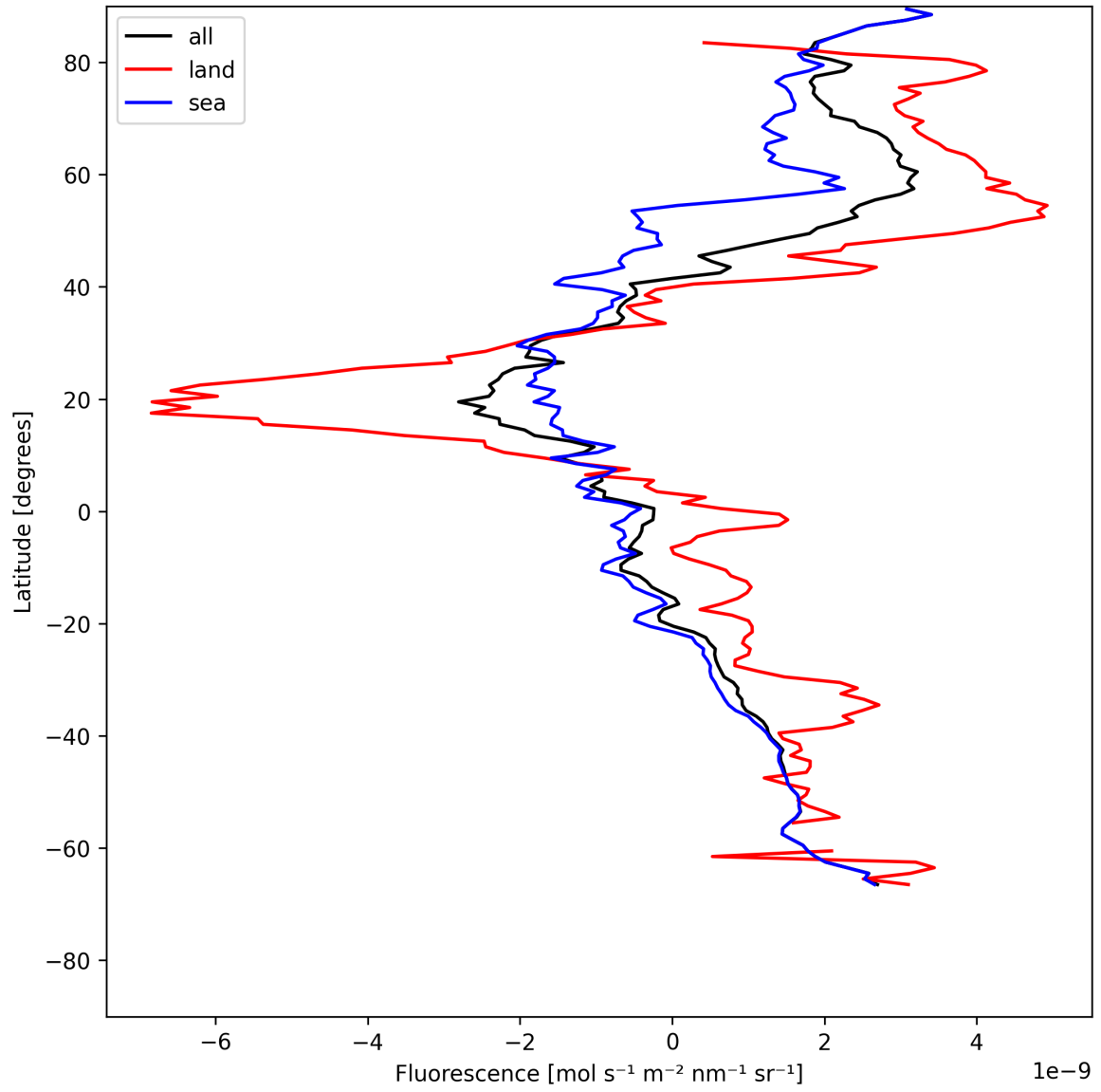
Figure 23: Zonal average of “Fluorescence” for 2025-07-13 to 2025-07-15.
