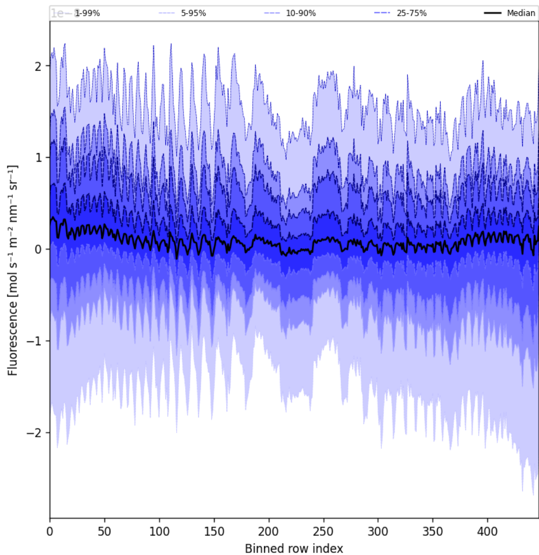
Figure 57: Along track statistics of “Fluorescence” for 2025-07-13 to 2025-07-15
