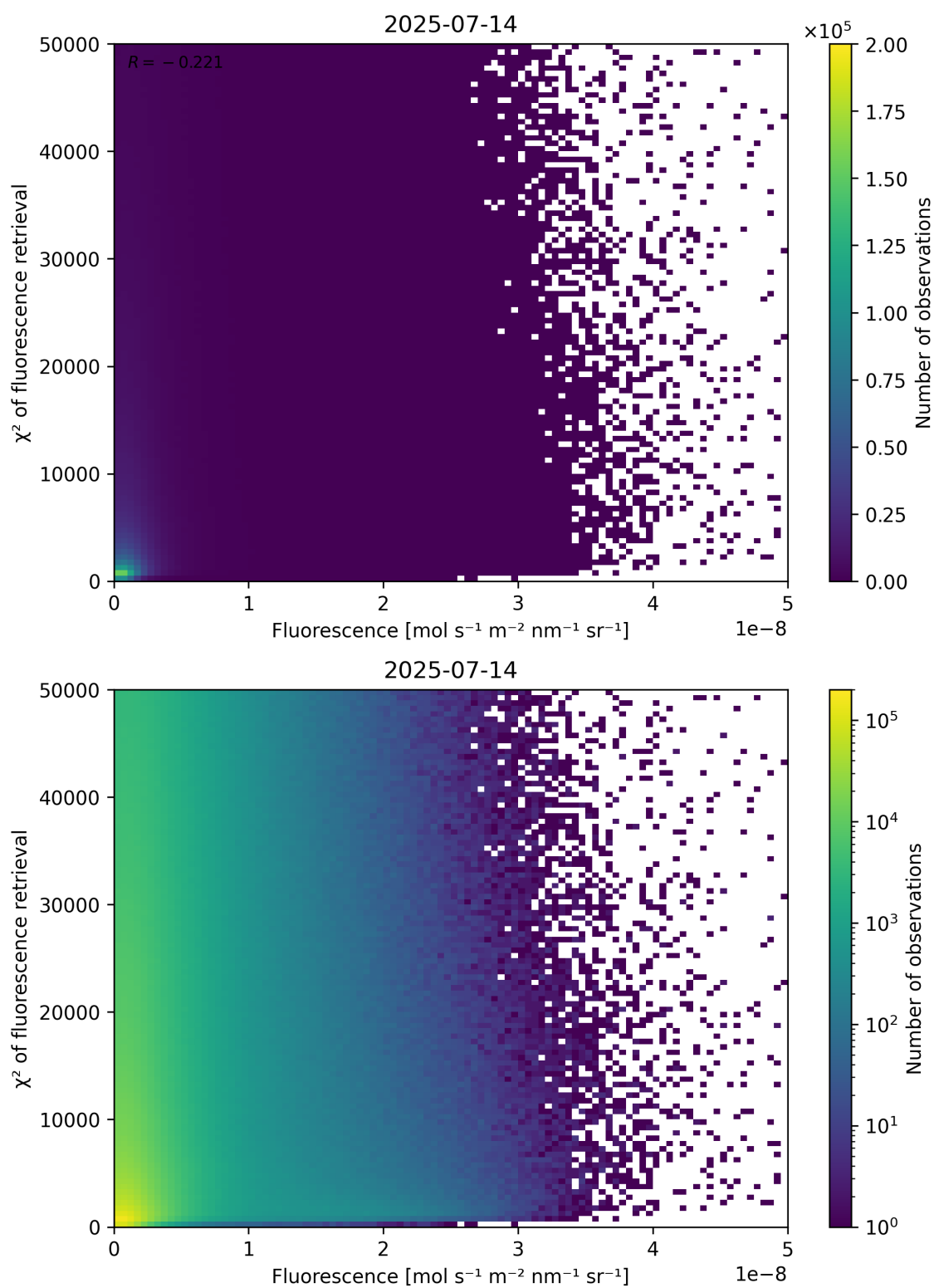
Figure 85: Scatter density plot of “Fluorescence” against “ \chi^2 of fluorescence retrieval” for 2025-07-13 to 2025-07-15.
