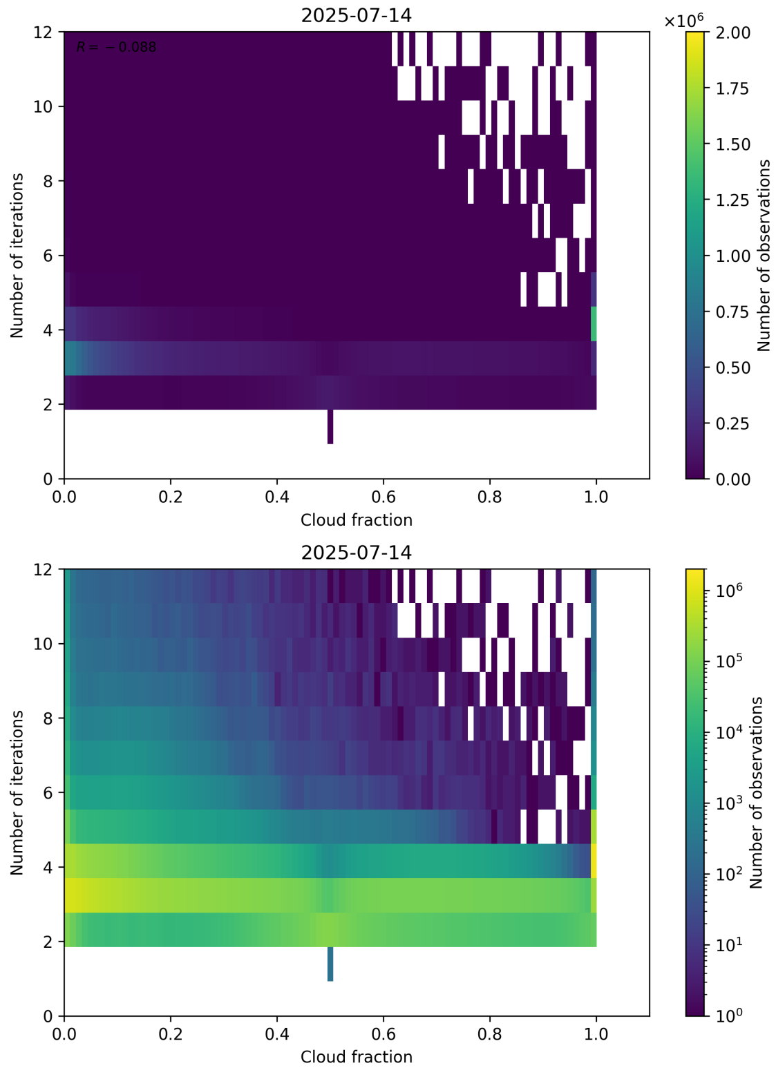
Figure 73: Scatter density plot of “Cloud fraction” against “Number of iterations” for 2025-07-13 to 2025-07-15.
