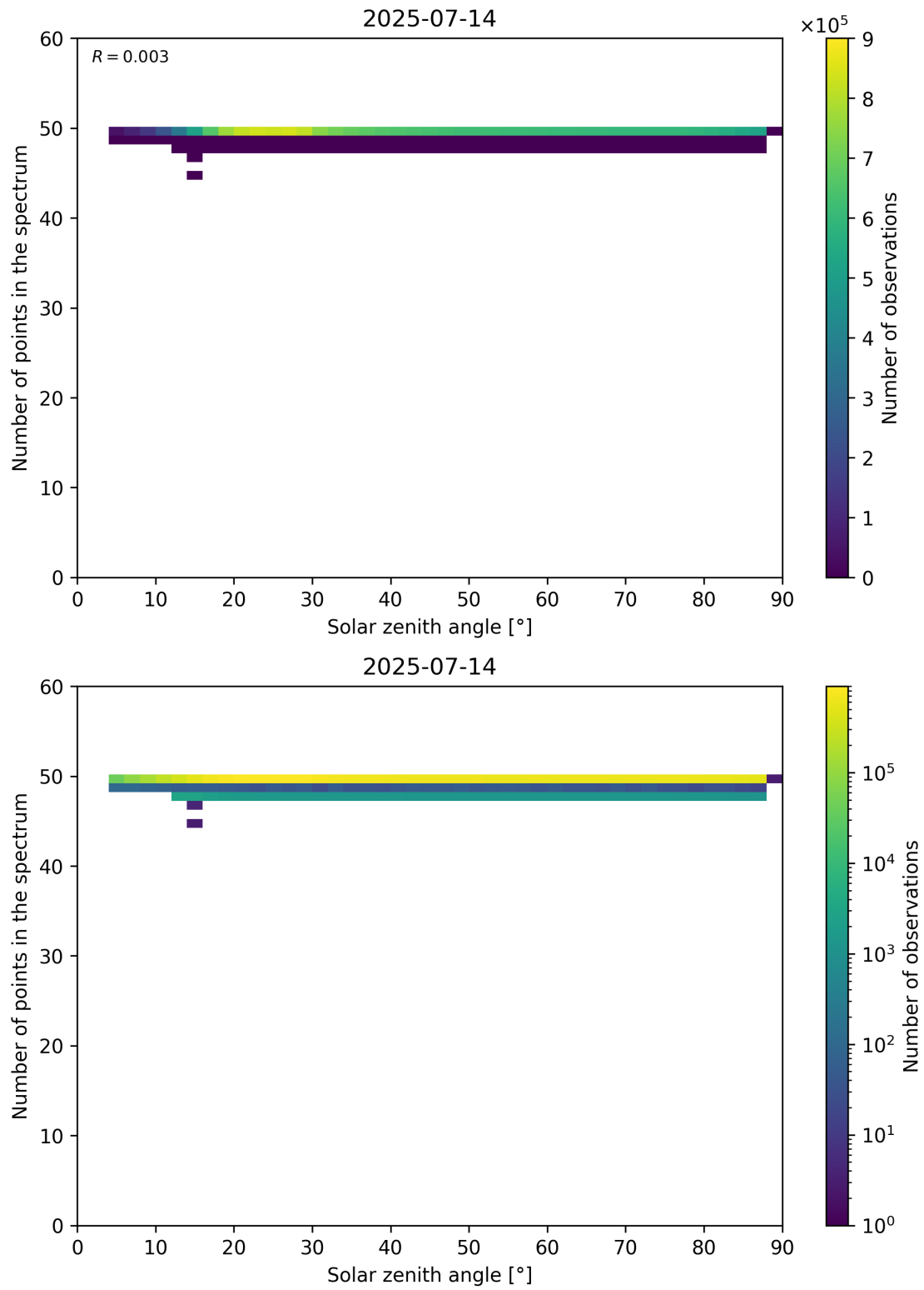
Figure 115: Scatter density plot of “Solar zenith angle” against “Number of points in the spectrum” for 2025-07-13 to 2025-07-15.
