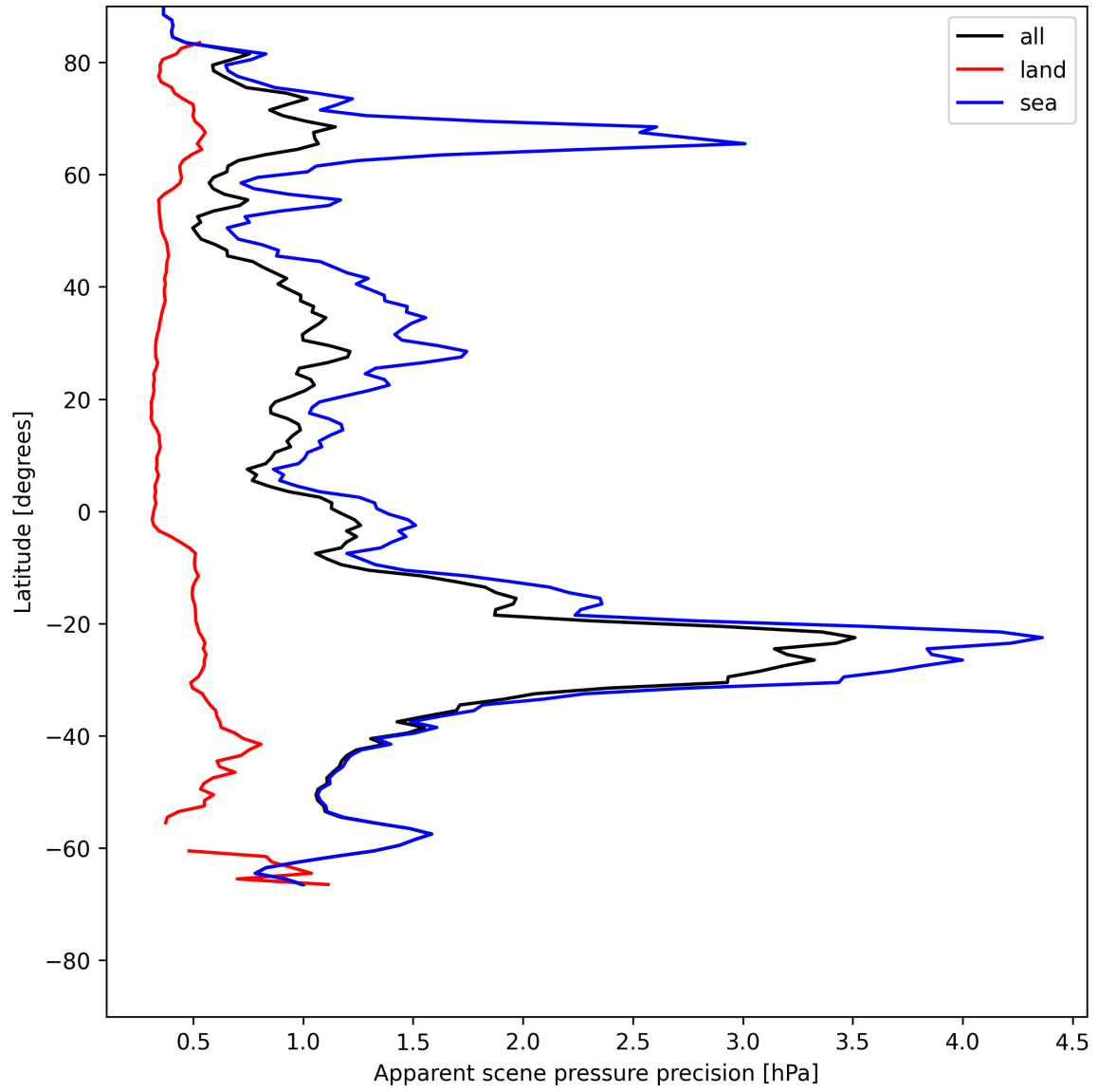
Figure 20: Zonal average of “Apparent scene pressure precision” for 2025-07-13 to 2025-07-15.
