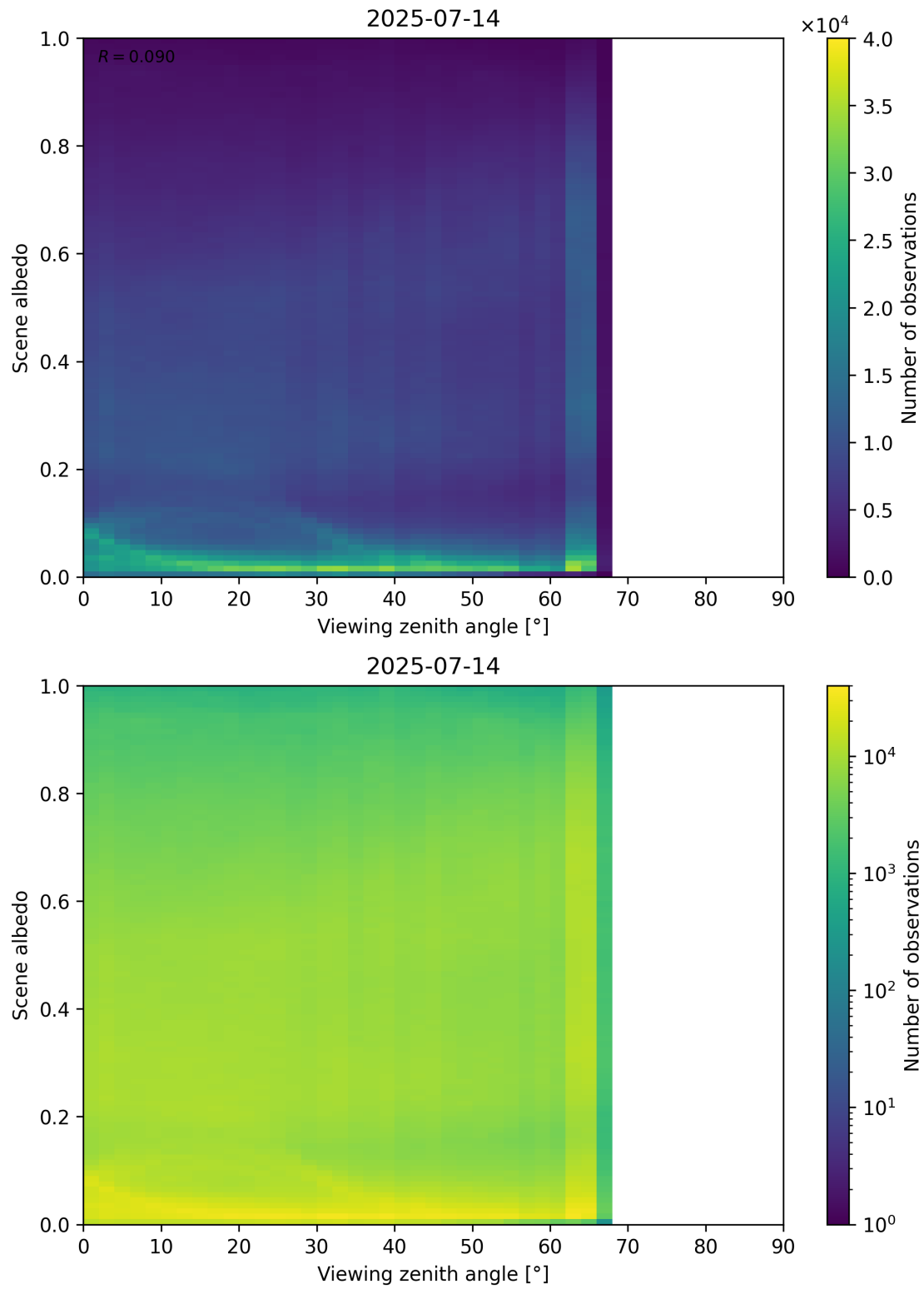
Figure 126: Scatter density plot of “Viewing zenith angle” against “Scene albedo” for 2025-07-13 to 2025-07-15.
