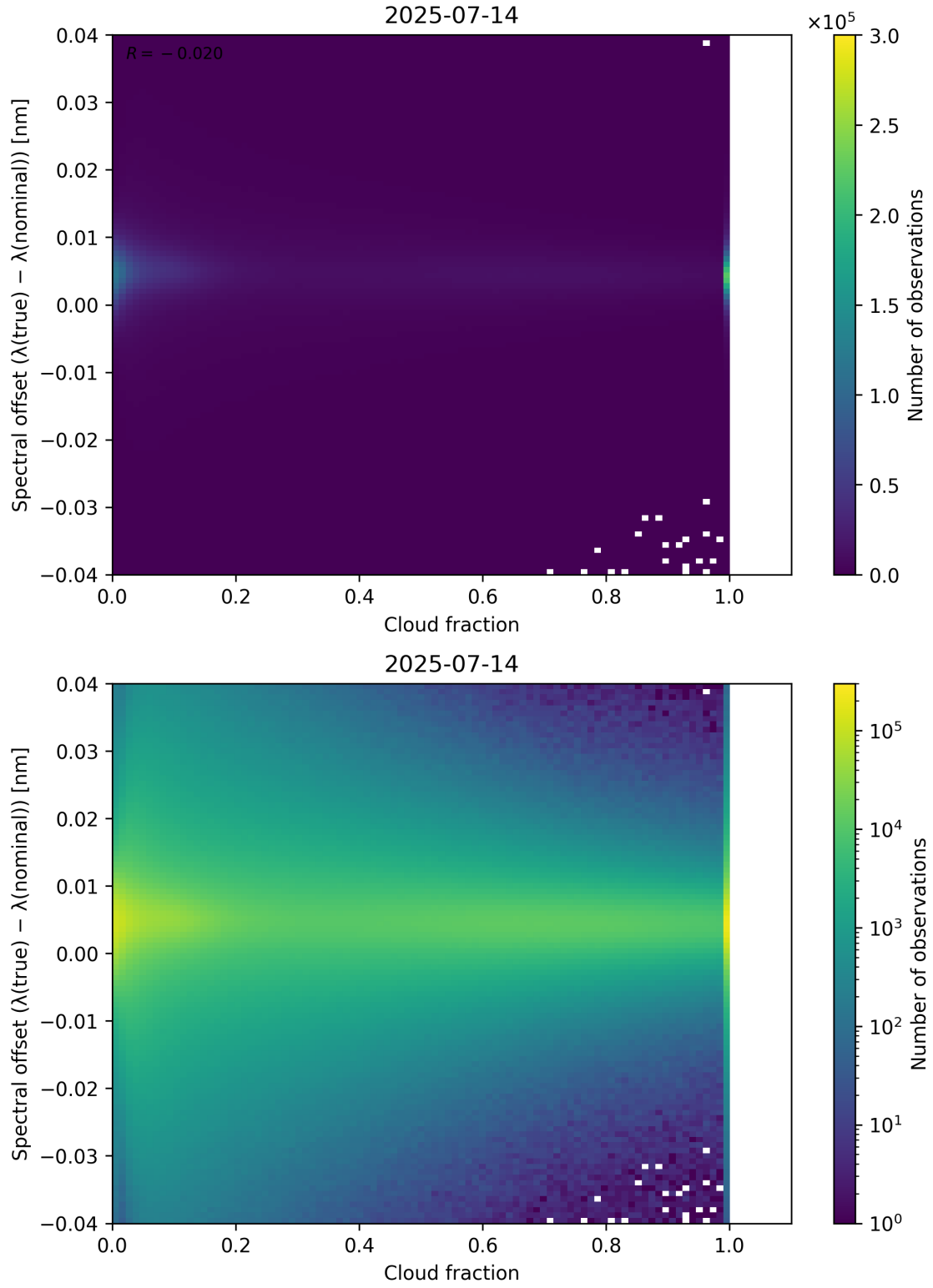
Figure 76: Scatter density plot of “Cloud fraction” against “Spectral offset ( \lambda_{\text{true}} - \lambda_{\text{nominal}} )” for 2025-07-13 to 2025-07-15.
