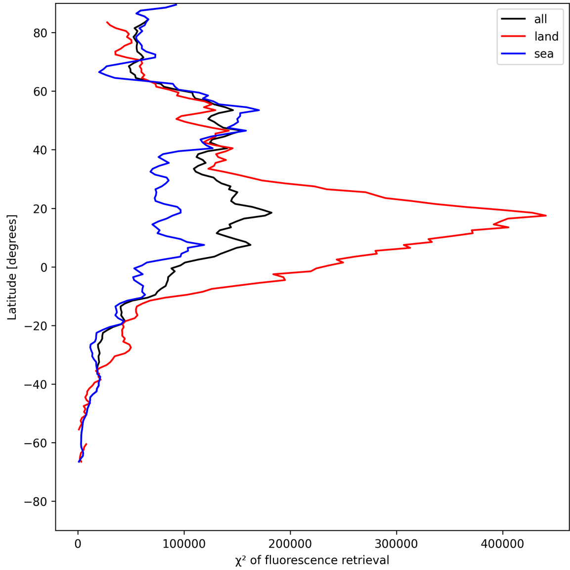
Figure 25: Zonal average of “ \chi^2 of fluorescence retrieval” for 2025-07-13 to 2025-07-15.
