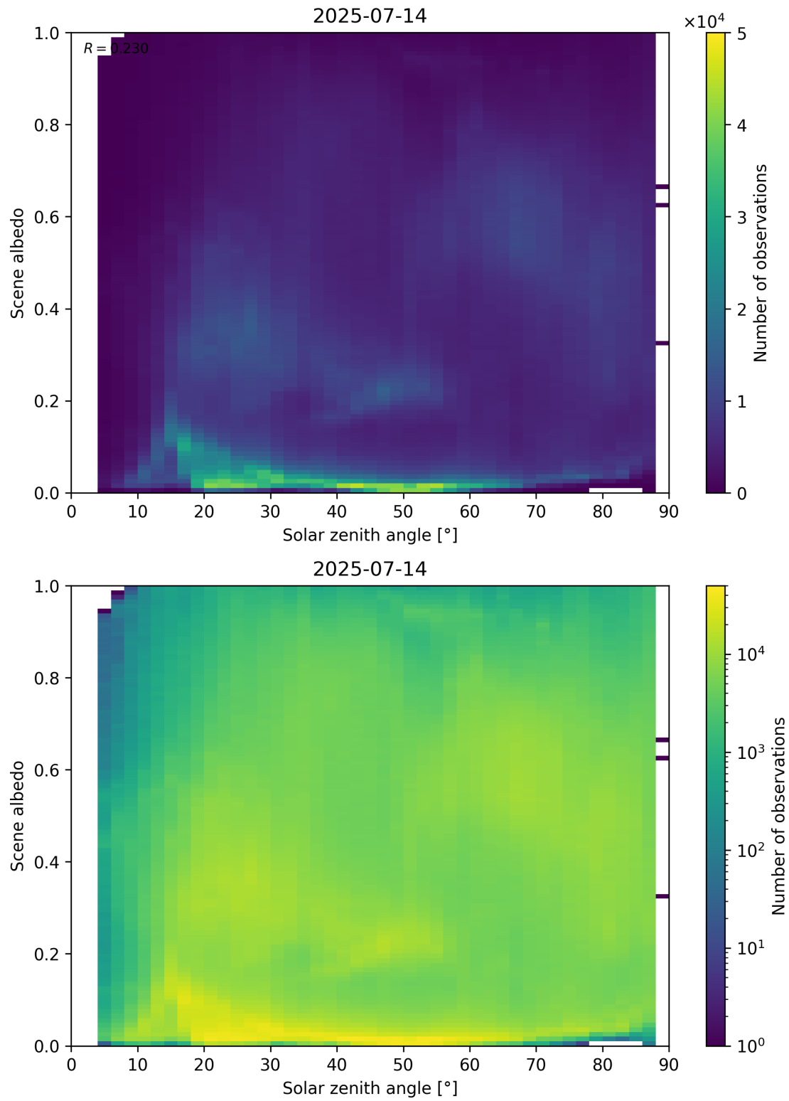
Figure 116: Scatter density plot of “Solar zenith angle” against “Scene albedo” for 2025-07-13 to 2025-07-15.
