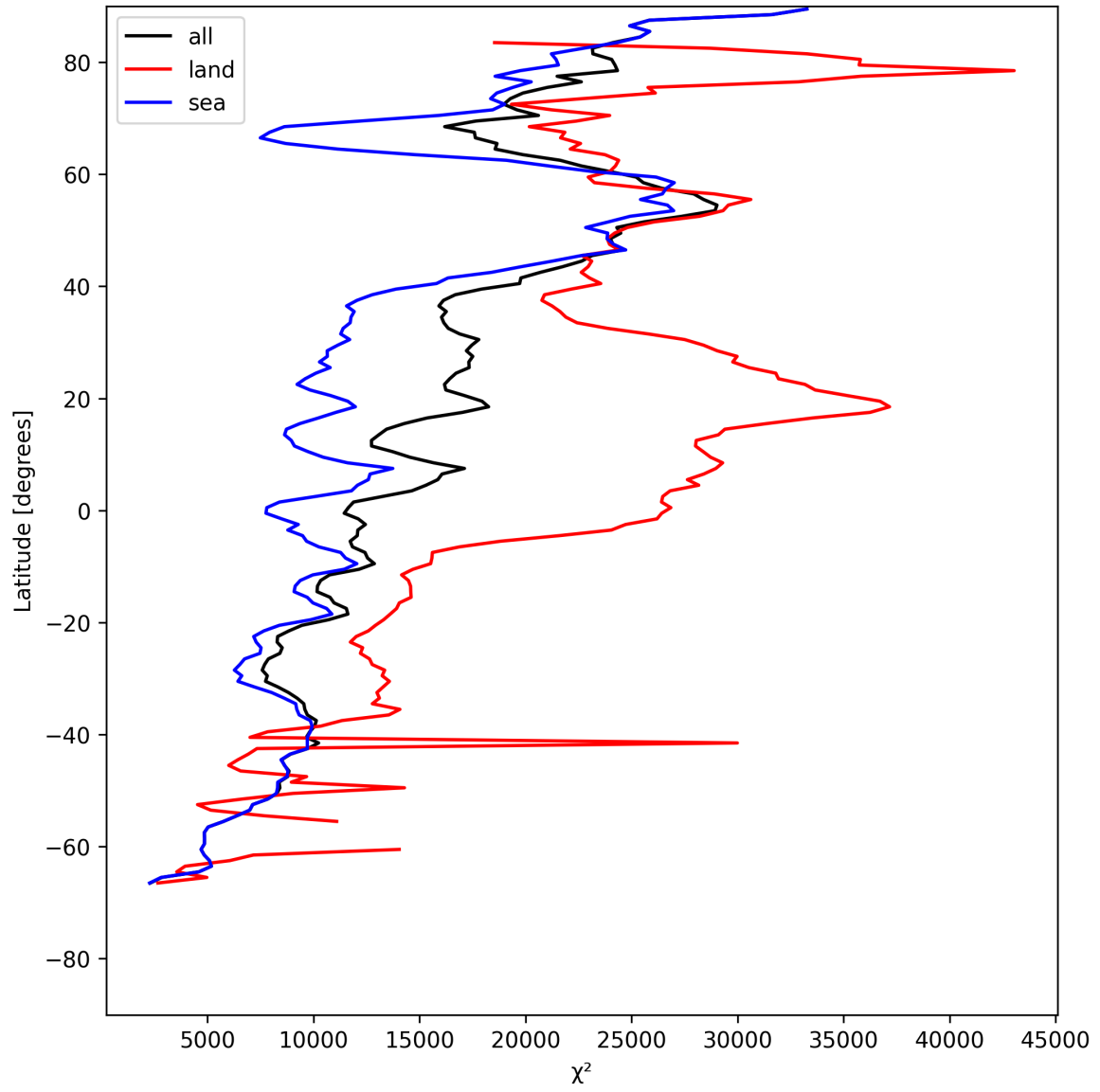
Figure 21: Zonal average of “ \chi^2 ” for 2025-07-13 to 2025-07-15.
