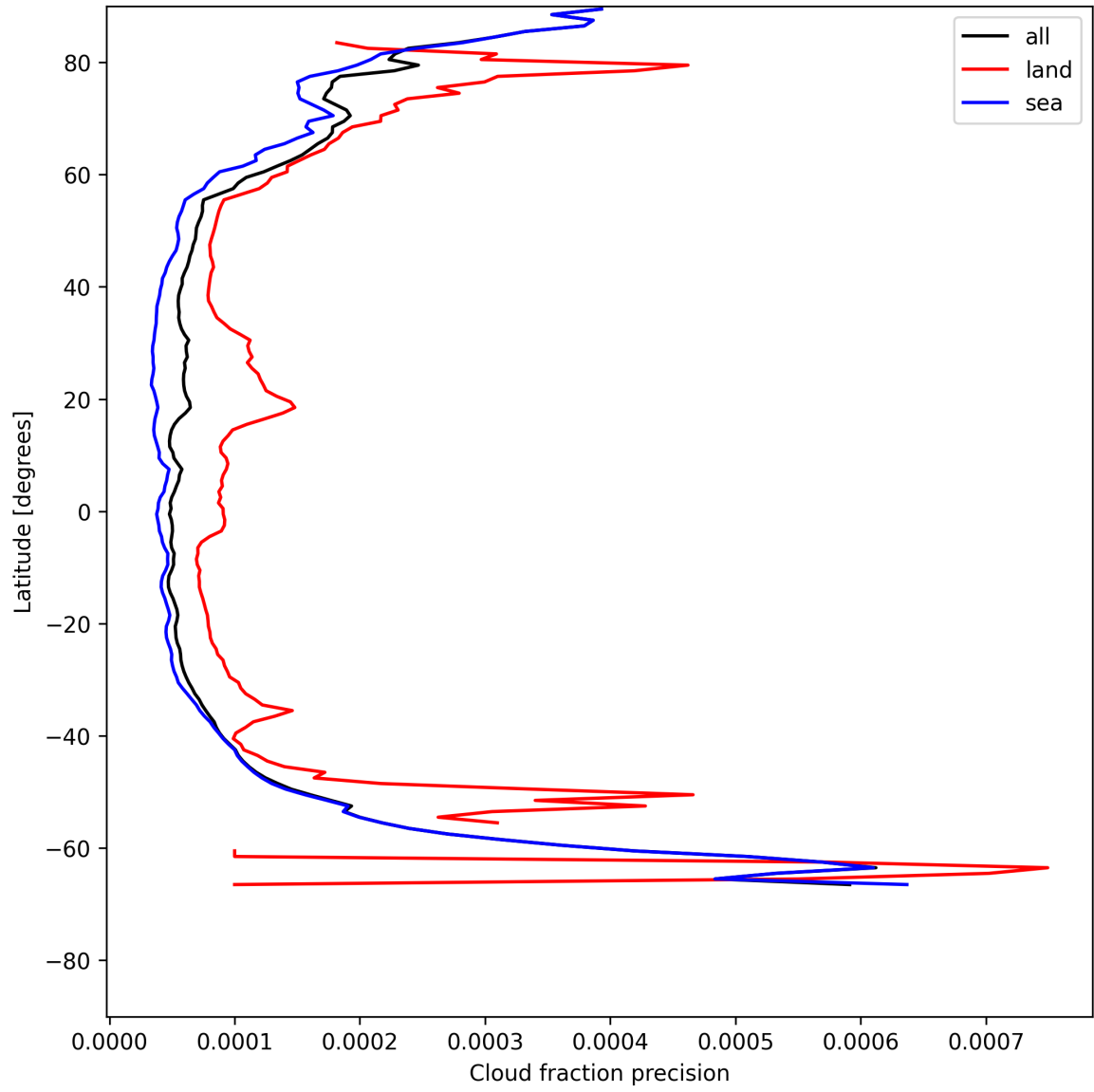
Figure 16: Zonal average of “Cloud fraction precision” for 2025-07-13 to 2025-07-15.
