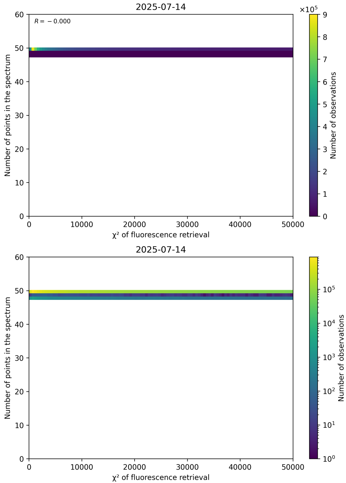
Figure 68: Scatter density plot of " \chi^2 of fluorescence retrieval" against "Number of points in the spectrum" for 2025-07-13 to 2025-07-15.
