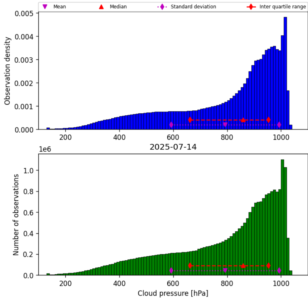
Figure 30: Histogram of “Cloud pressure” for 2025-07-13 to 2025-07-15
