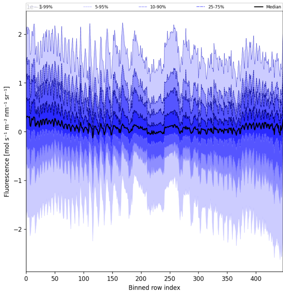
Figure 57: Along track statistics of “Fluorescence” for 2025-07-14 to 2025-07-16
