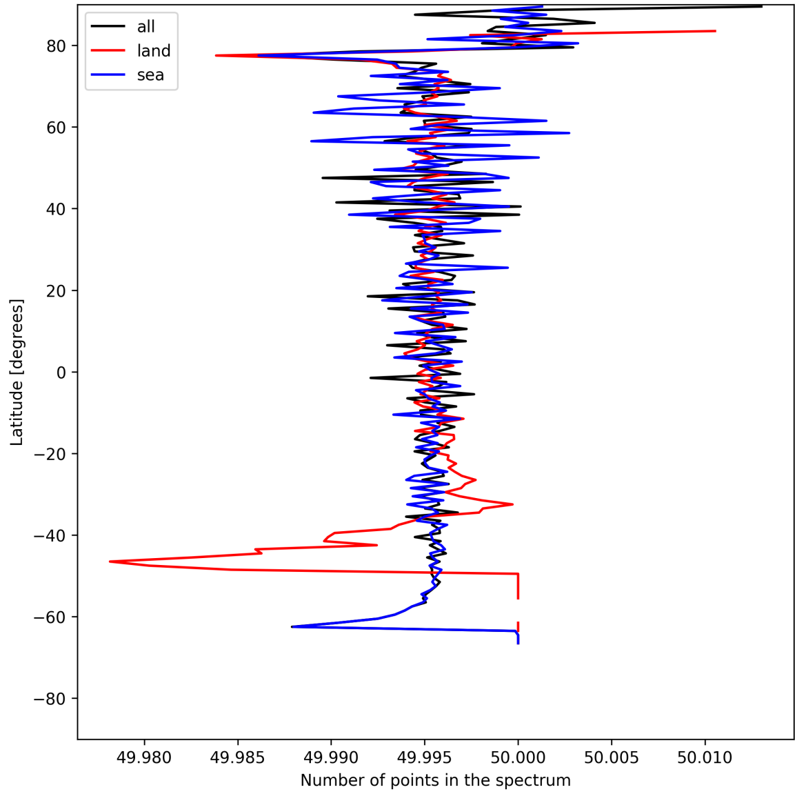
Figure 27: Zonal average of “Number of points in the spectrum” for 2025-07-14 to 2025-07-16.
