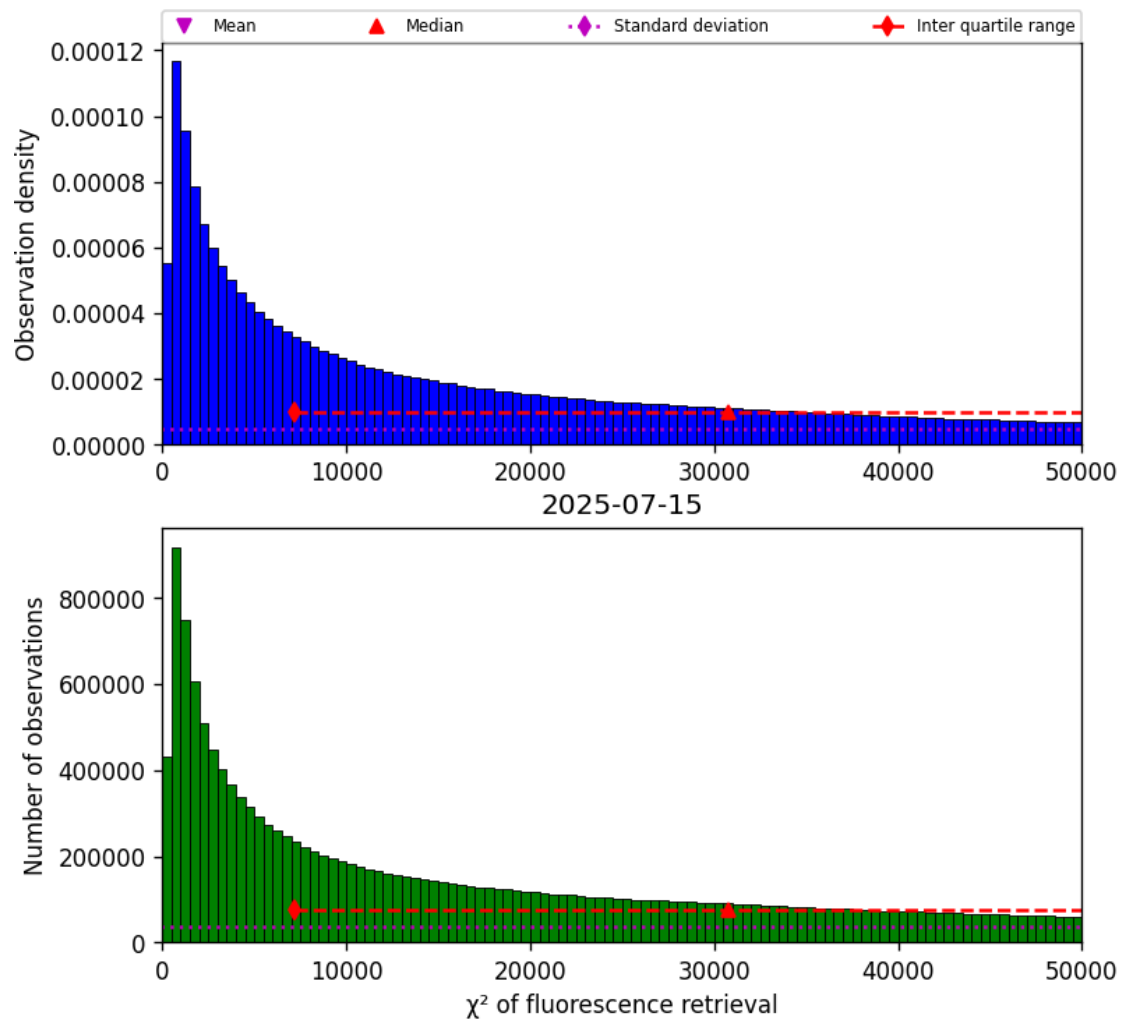
Figure 42: Histogram of “ \chi^2 of fluorescence retrieval” for 2025-07-14 to 2025-07-16
