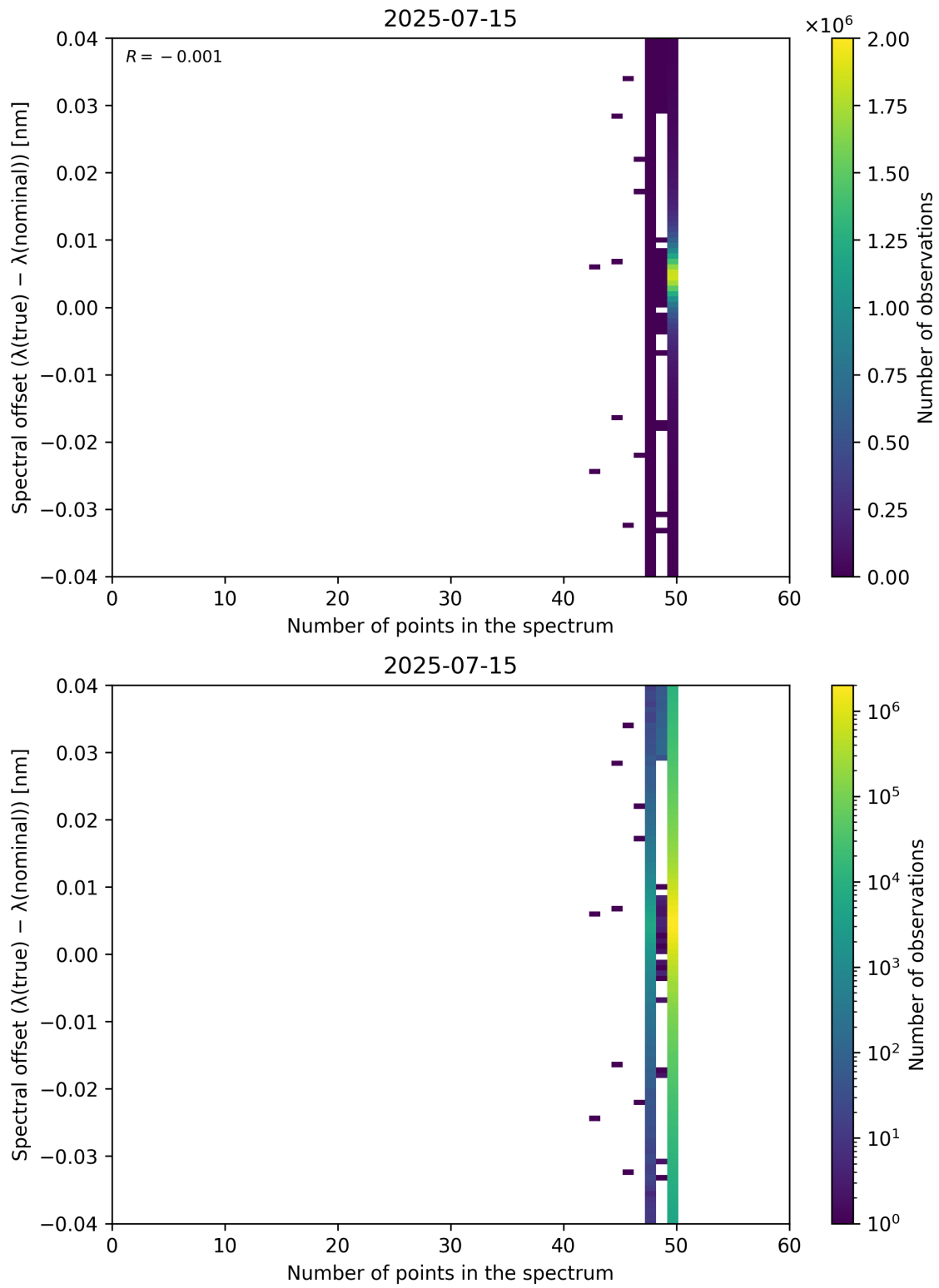
Figure 101: Scatter density plot of “Number of points in the spectrum” against “Spectral offset ( \lambda_{\text{true}} - \lambda_{\text{nominal}} )” for 2025-07-14 to 2025-07-16.
