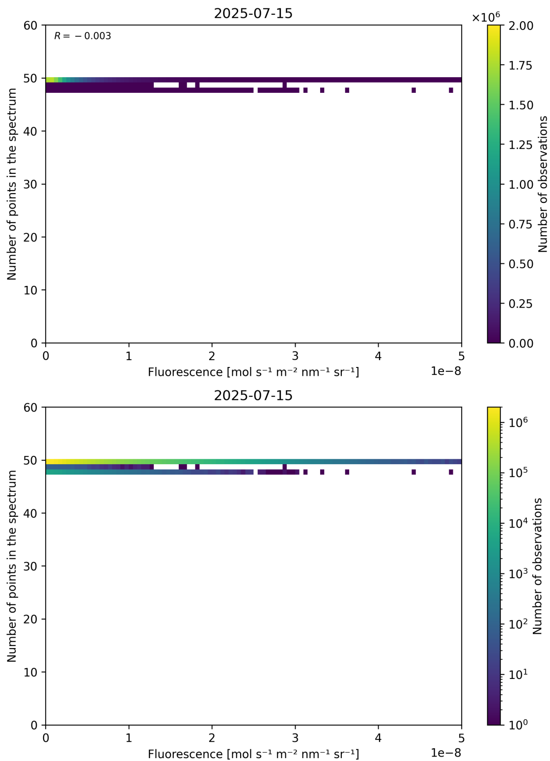
Figure 86: Scatter density plot of “Fluorescence” against “Number of points in the spectrum” for 2025-07-14 to 2025-07-16.
