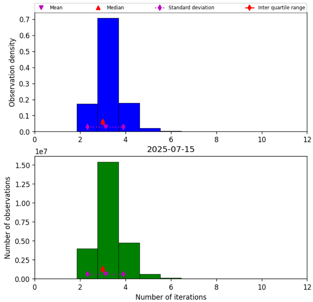
Figure 39: Histogram of “Number of iterations” for 2025-07-14 to 2025-07-16
