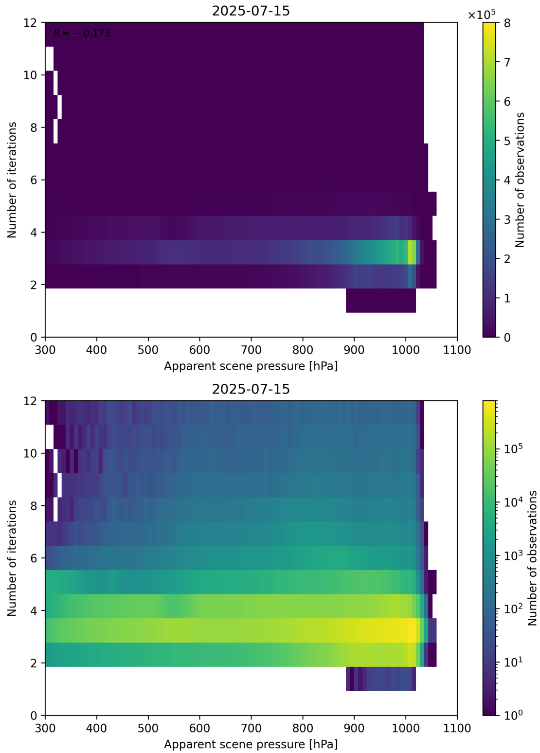
Figure 65: Scatter density plot of “Apparent scene pressure” against “Number of iterations” for 2025-07-14 to 2025-07-16.
