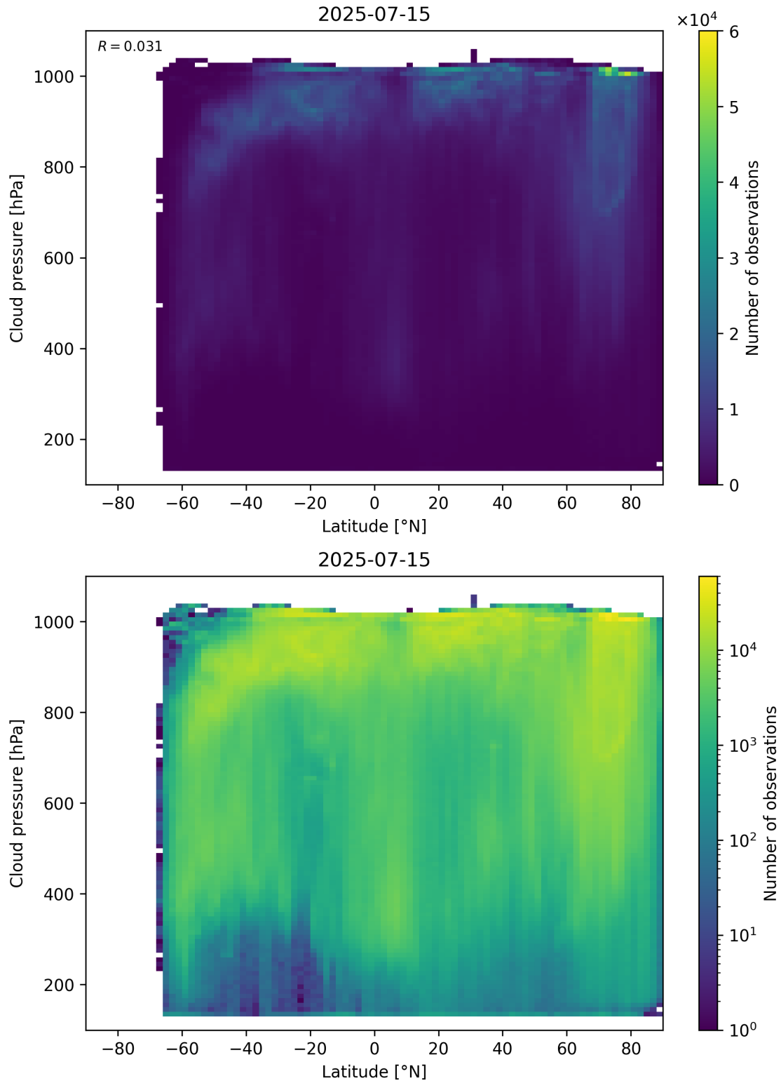
Figure 91: Scatter density plot of “Latitude” against “Cloud pressure” for 2025-07-14 to 2025-07-16.
