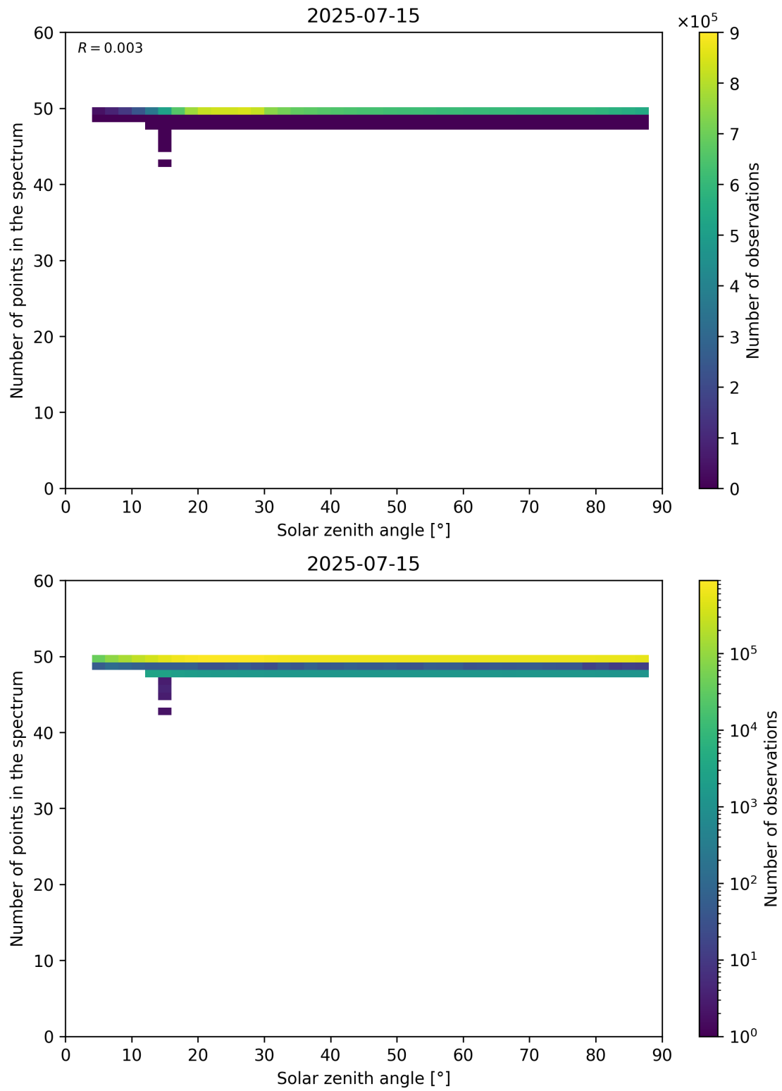
Figure 115: Scatter density plot of “Solar zenith angle” against “Number of points in the spectrum” for 2025-07-14 to 2025-07-16.
