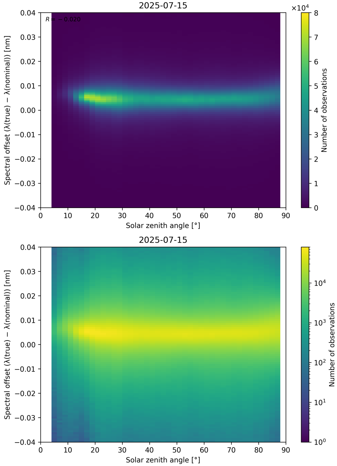
Figure 117: Scatter density plot of “Solar zenith angle” against “Spectral offset ( \lambda_{\text{true}} - \lambda_{\text{nominal}} )” for 2025-07-14 to 2025-07-16.
