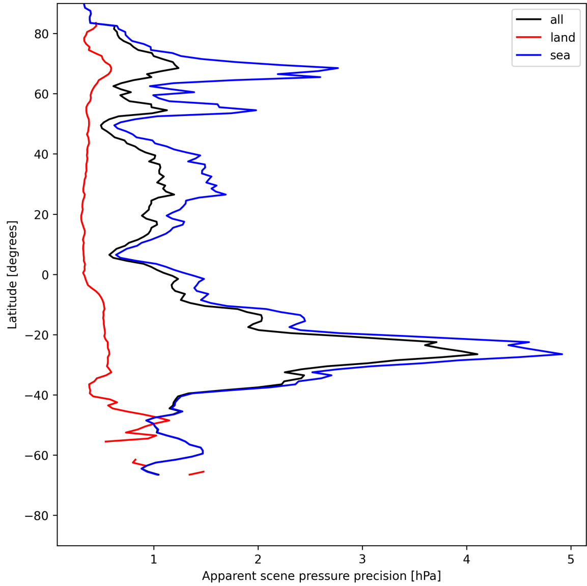
Figure 20: Zonal average of “Apparent scene pressure precision” for 2025-07-14 to 2025-07-16.
