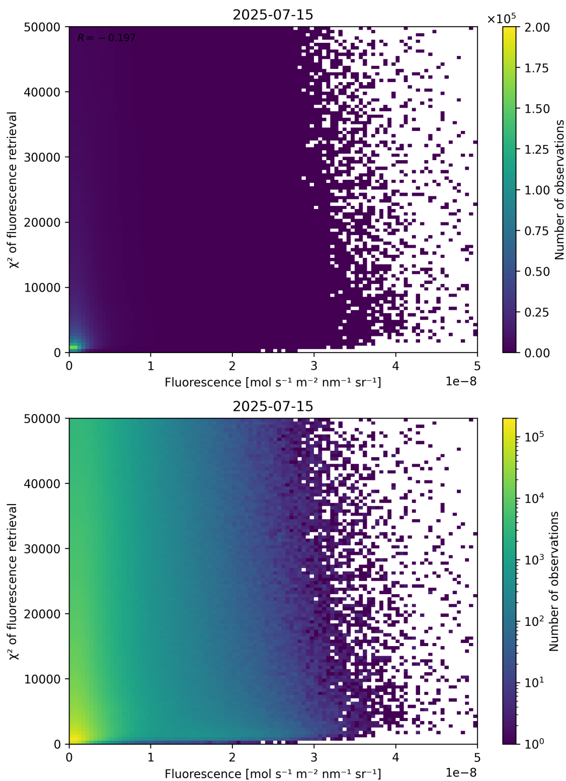
Figure 85: Scatter density plot of “Fluorescence” against “ \chi^2 of fluorescence retrieval” for 2025-07-14 to 2025-07-16.
