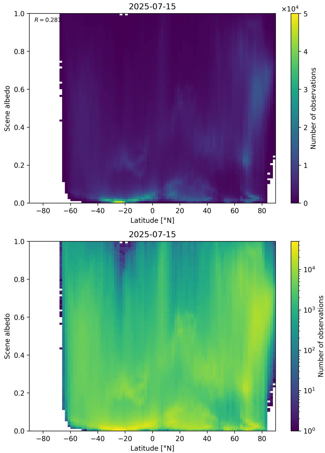
Figure 95: Scatter density plot of “Latitude” against “Scene albedo” for 2025-07-14 to 2025-07-16.
