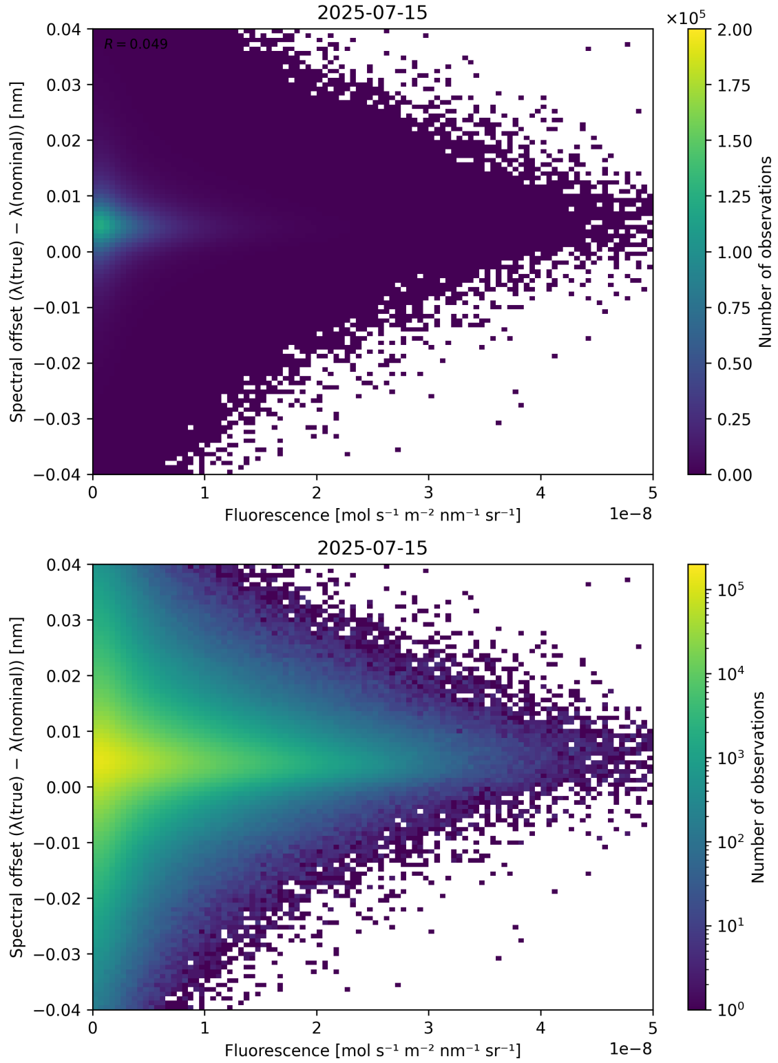
Figure 87: Scatter density plot of “Fluorescence” against “Spectral offset ( \lambda_{\text{true}} - \lambda_{\text{nominal}} )” for 2025-07-14 to 2025-07-16.
