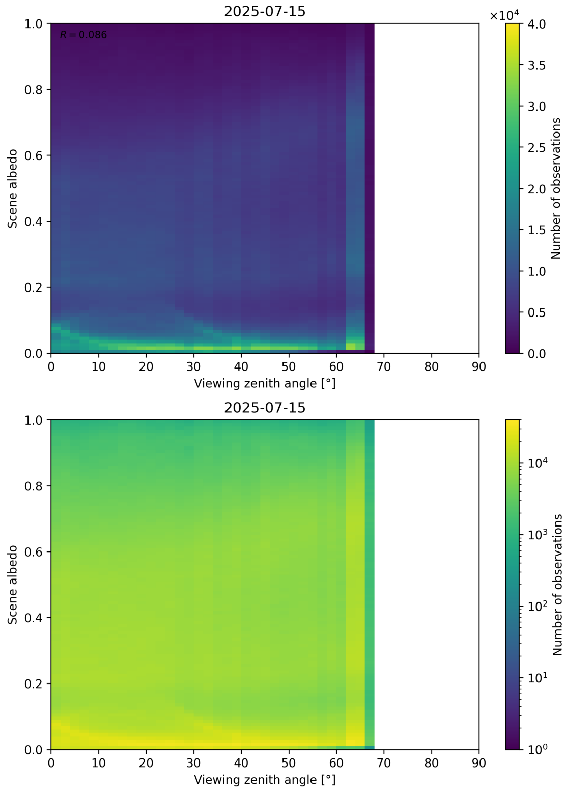
Figure 126: Scatter density plot of “Viewing zenith angle” against “Scene albedo” for 2025-07-14 to 2025-07-16.
