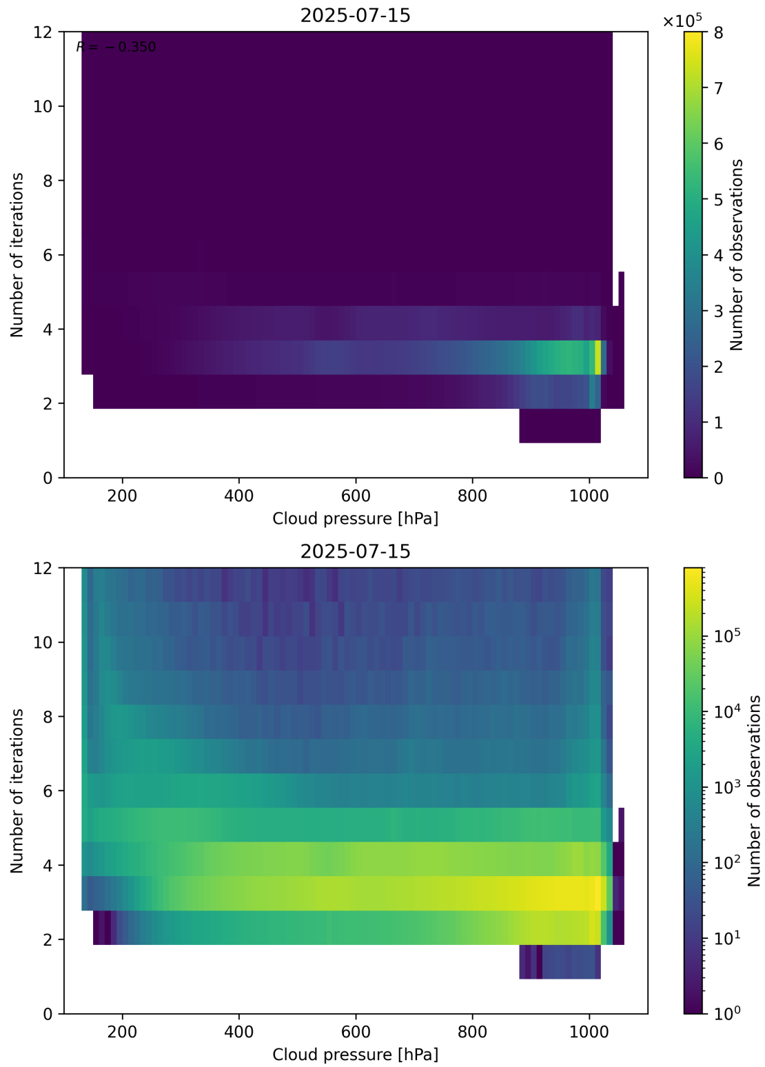
Figure 81: Scatter density plot of “Cloud pressure” against “Number of iterations” for 2025-07-14 to 2025-07-16.
