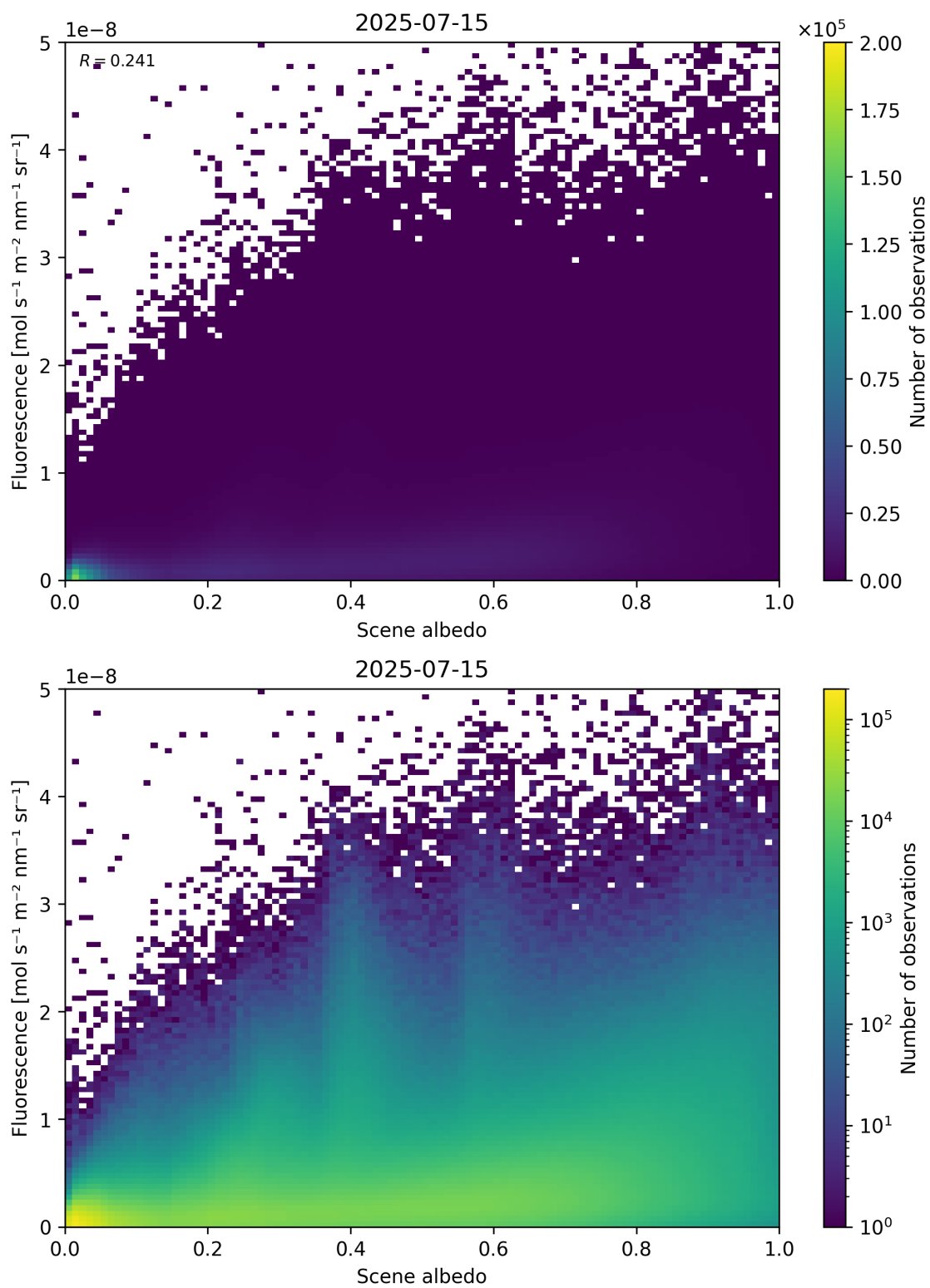
Figure 104: Scatter density plot of “Scene albedo” against “Fluorescence” for 2025-07-14 to 2025-07-16.
