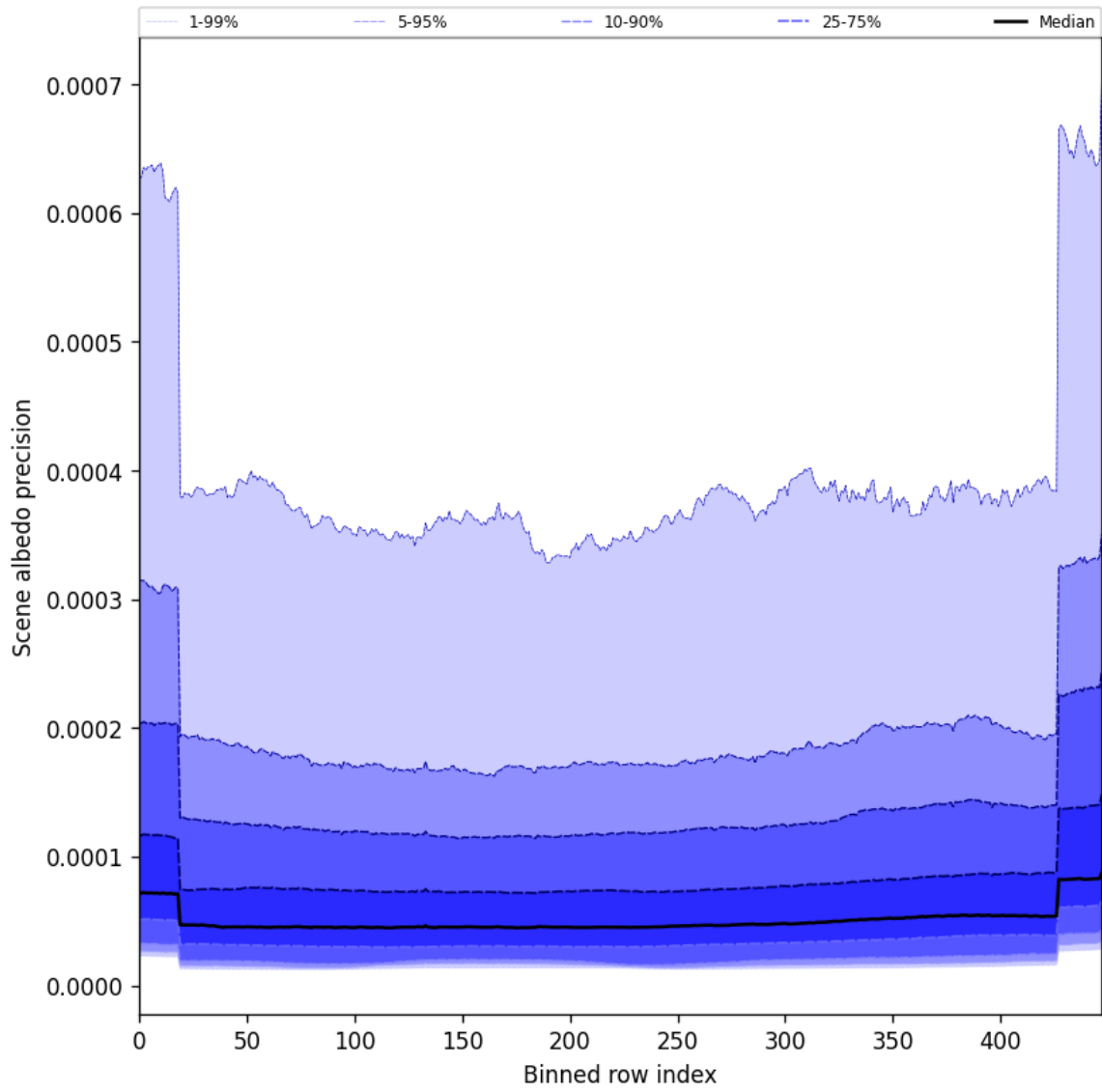
Figure 52: Along track statistics of “Scene albedo precision” for 2025-07-14 to 2025-07-16
