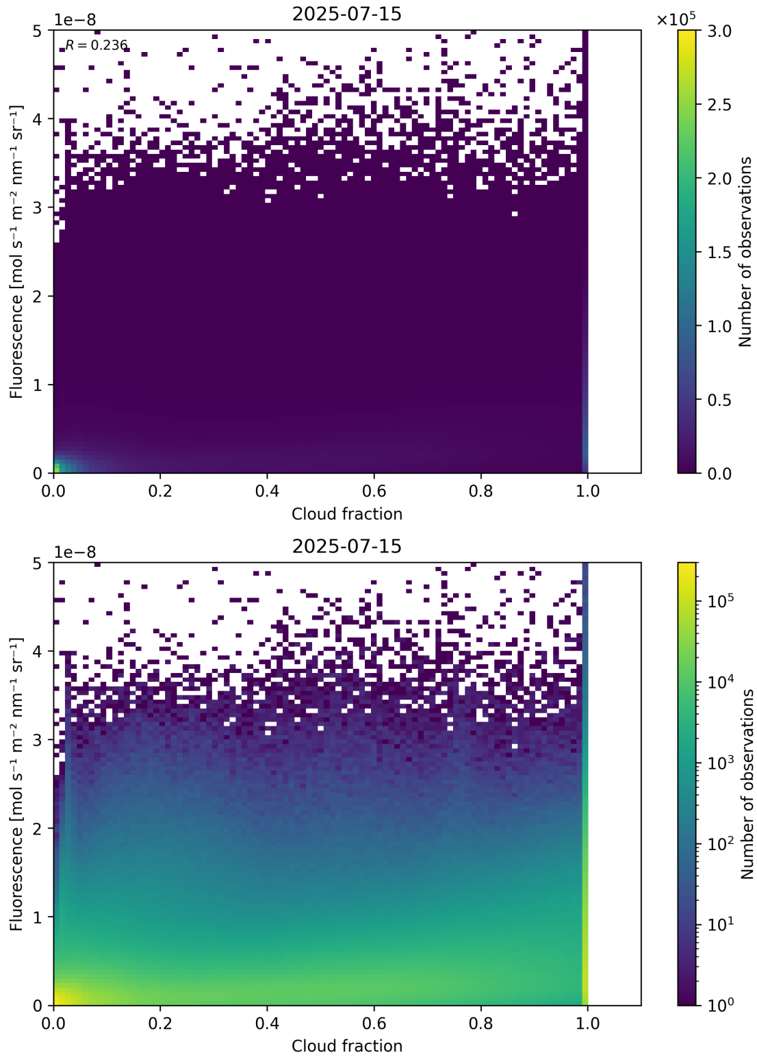
Figure 72: Scatter density plot of “Cloud fraction” against “Fluorescence” for 2025-07-14 to 2025-07-16.
