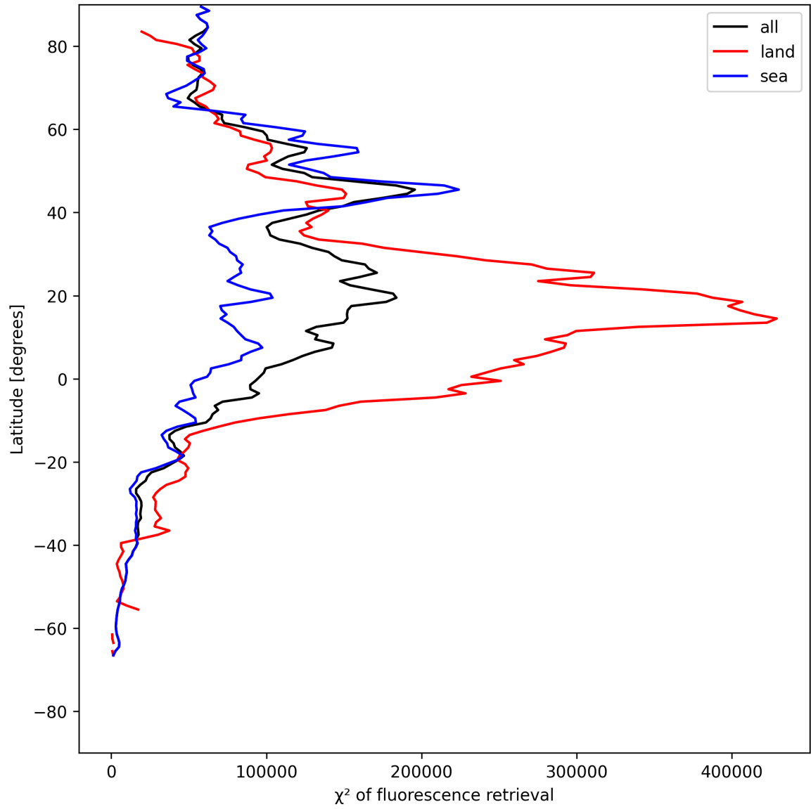
Figure 25: Zonal average of “ \chi^2 of fluorescence retrieval” for 2025-07-14 to 2025-07-16.
