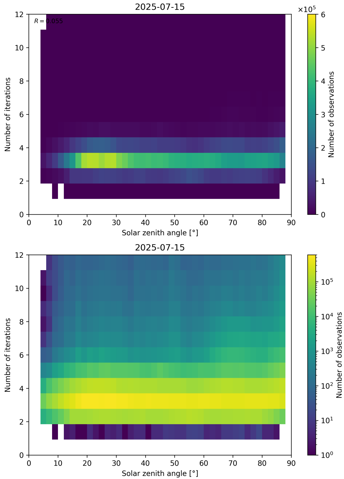
Figure 114: Scatter density plot of “Solar zenith angle” against “Number of iterations” for 2025-07-14 to 2025-07-16.
