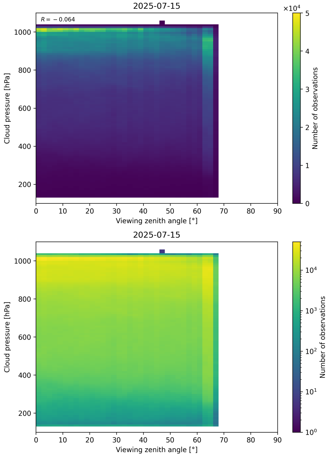
Figure 121: Scatter density plot of “Viewing zenith angle” against “Cloud pressure” for 2025-07-14 to 2025-07-16.
