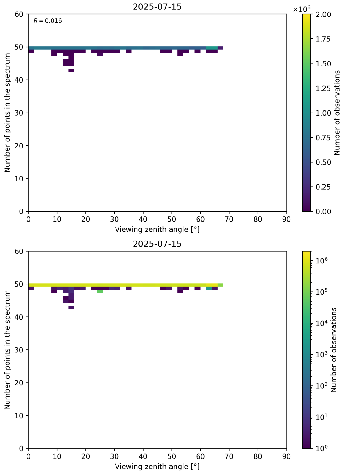
Figure 125: Scatter density plot of “Viewing zenith angle” against “Number of points in the spectrum” for 2025-07-14 to 2025-07-16.
