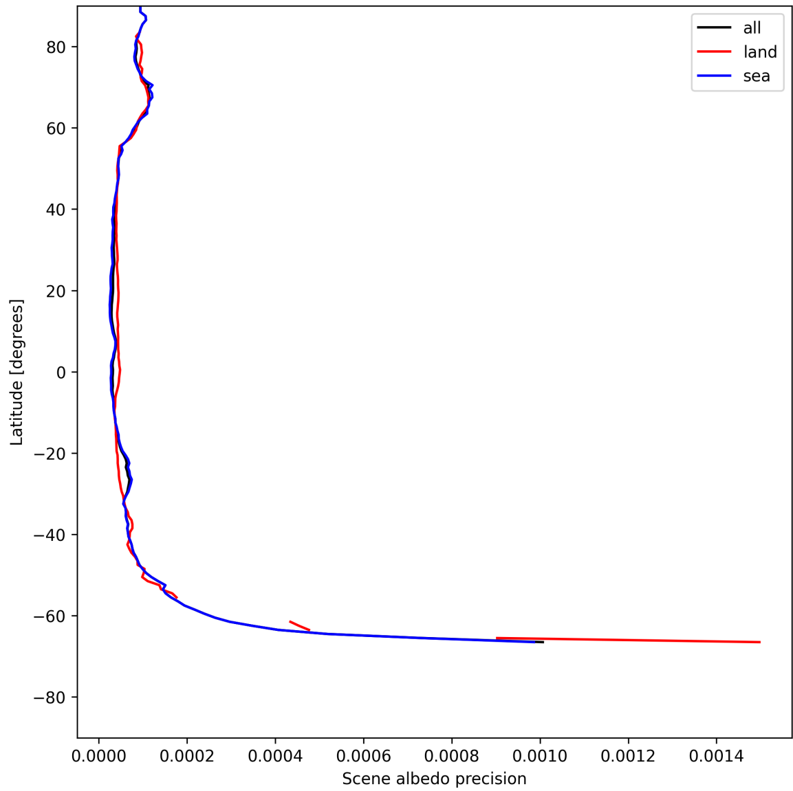
Figure 18: Zonal average of “Scene albedo precision” for 2025-07-14 to 2025-07-16.
