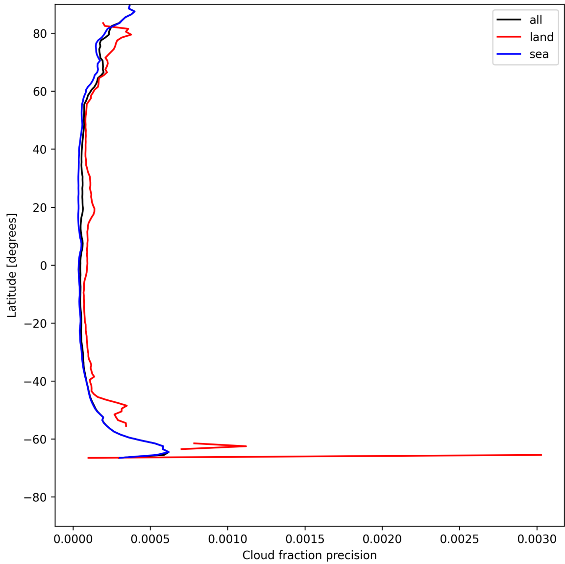
Figure 16: Zonal average of “Cloud fraction precision” for 2025-07-14 to 2025-07-16.
