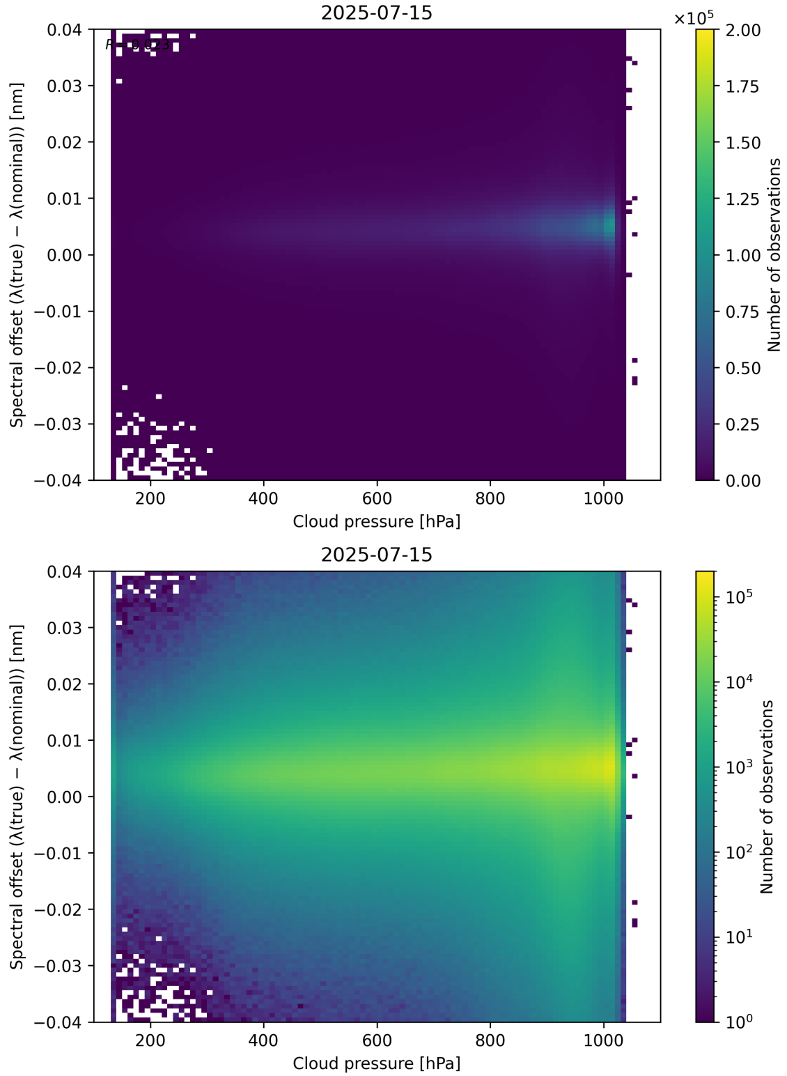
Figure 84: Scatter density plot of “Cloud pressure” against “Spectral offset ( \lambda_{\text{true}} - \lambda_{\text{nominal}} )” for 2025-07-14 to 2025-07-16.
