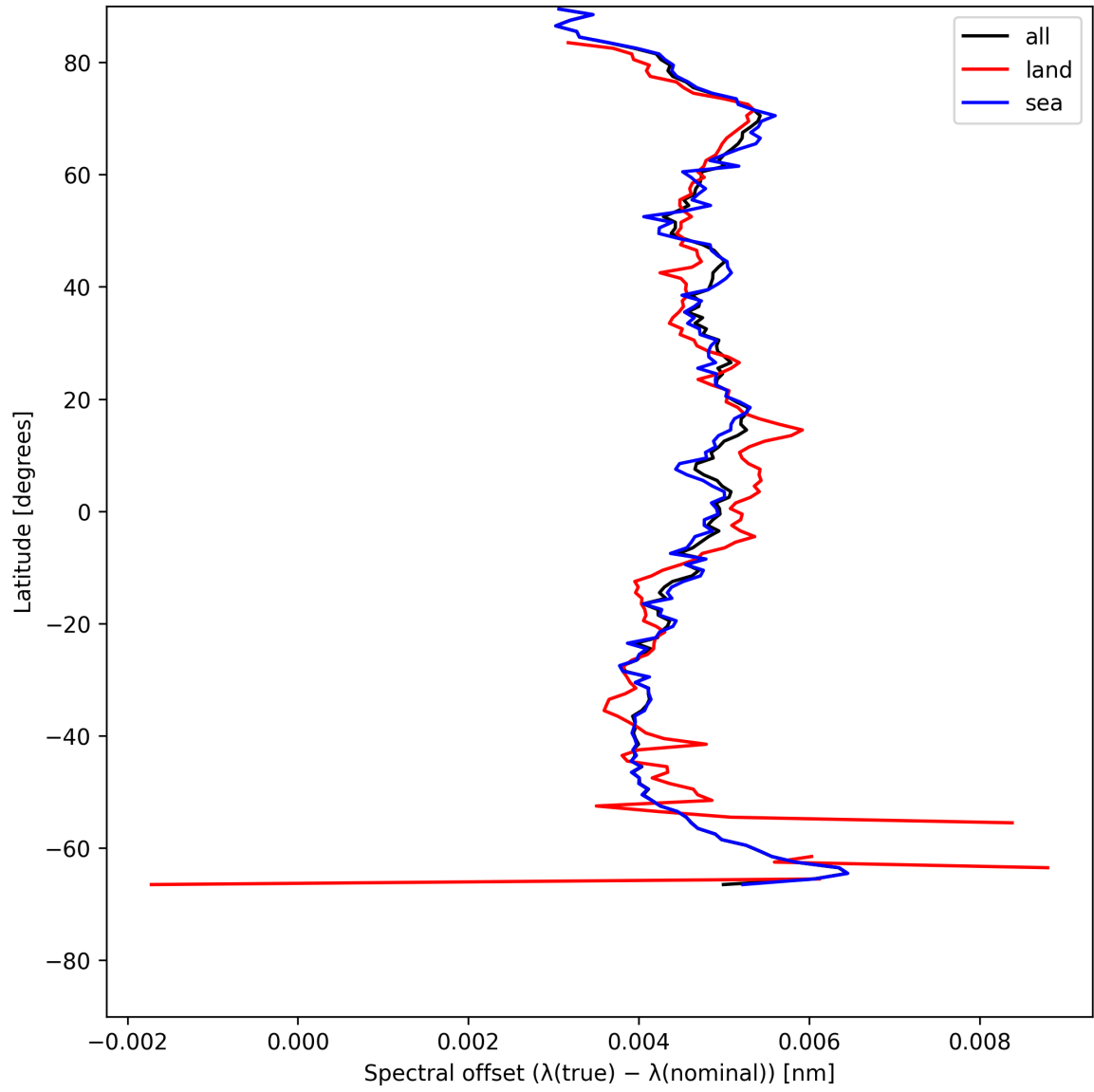
Figure 28: Zonal average of “Spectral offset ( \lambda_{\text{true}} - \lambda_{\text{nominal}} )” for 2025-07-14 to 2025-07-16.
