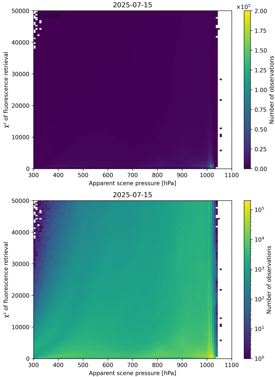
Figure 63: Scatter density plot of “Apparent scene pressure” against “ \chi^2 of fluorescence retrieval” for 2025-07-14 to 2025-07-16.
