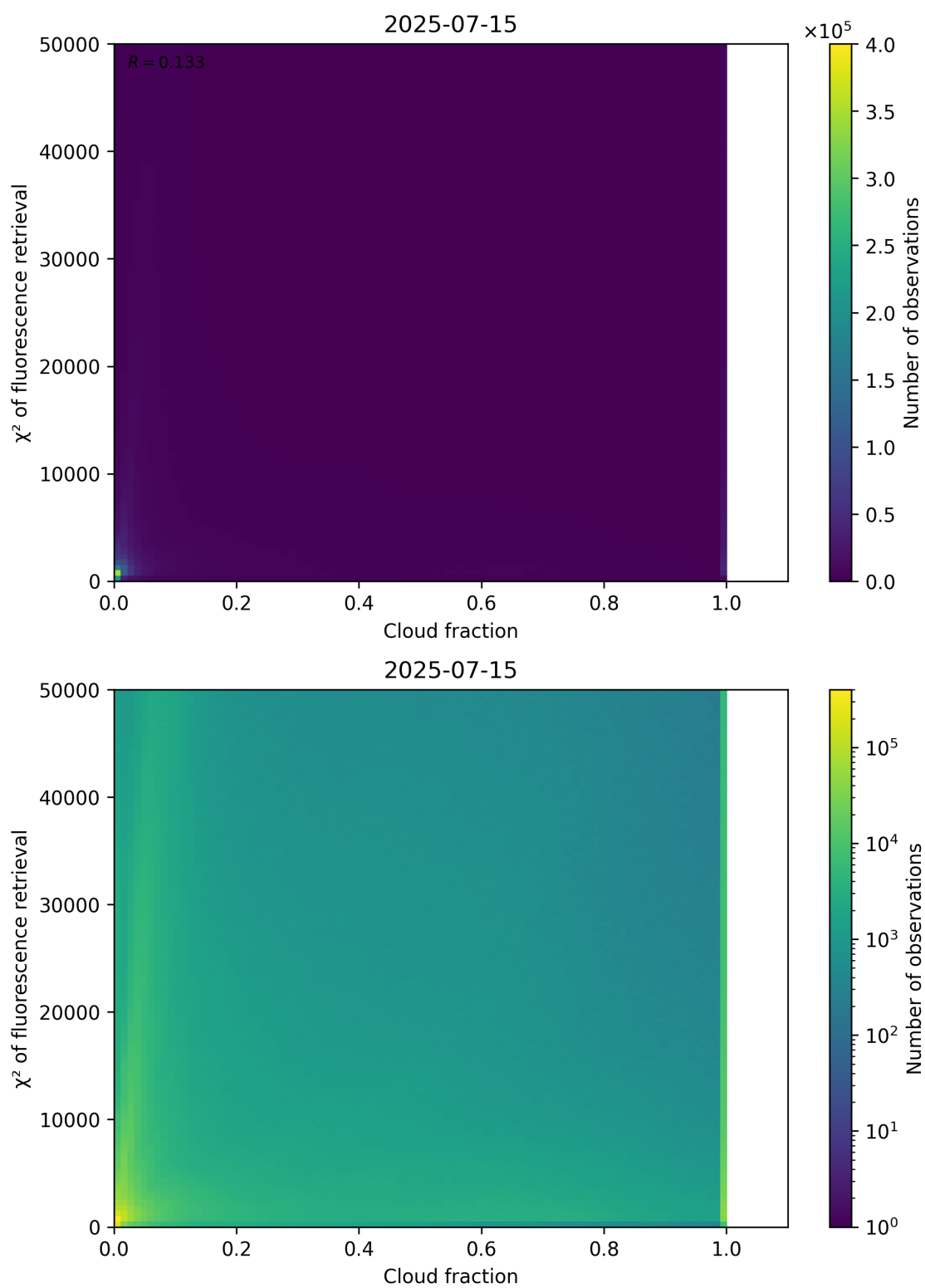
Figure 71: Scatter density plot of “Cloud fraction” against “ \chi^2 of fluorescence retrieval” for 2025-07-14 to 2025-07-16.
