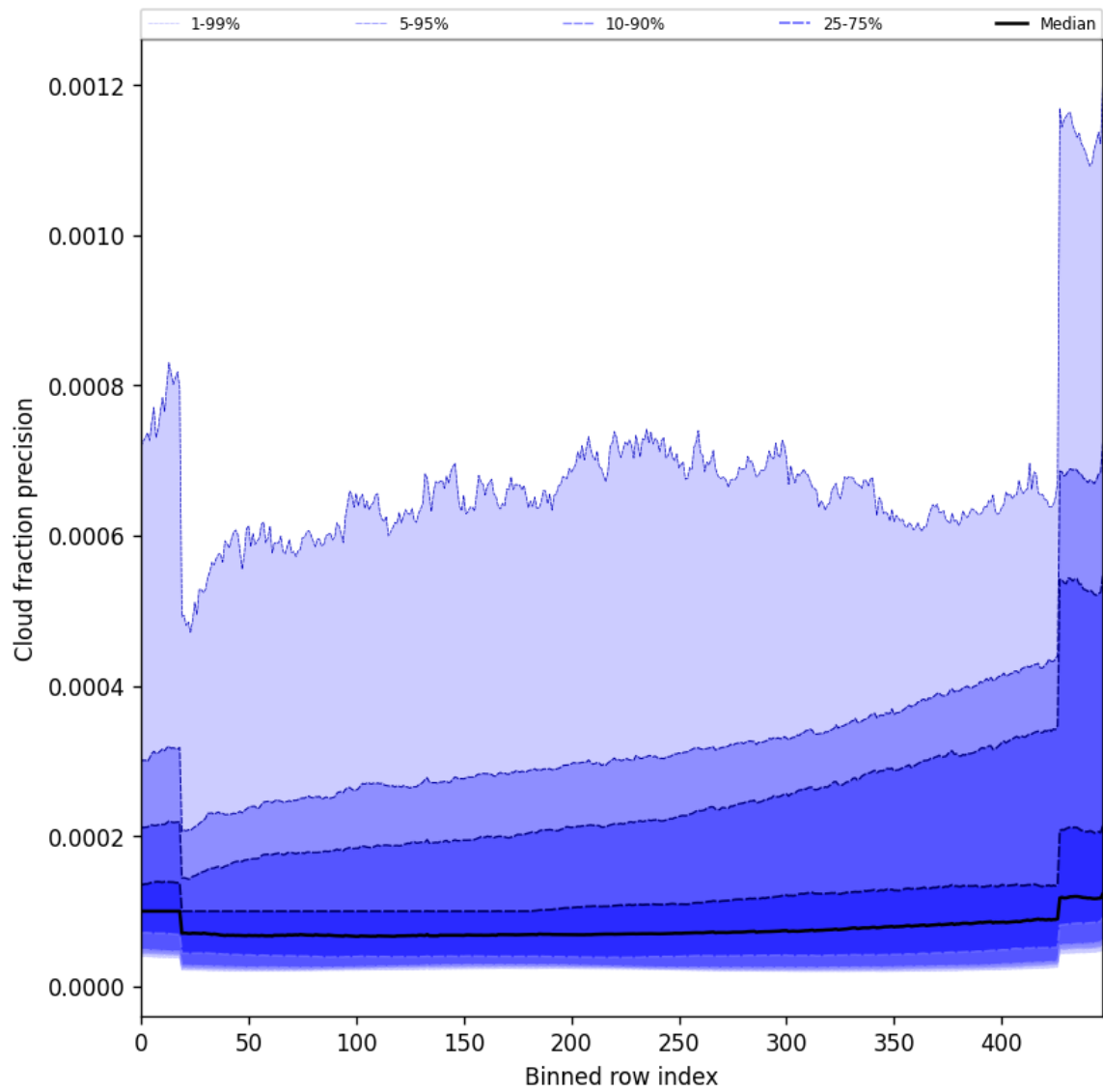
Figure 50: Along track statistics of “Cloud fraction precision” for 2025-07-14 to 2025-07-16
