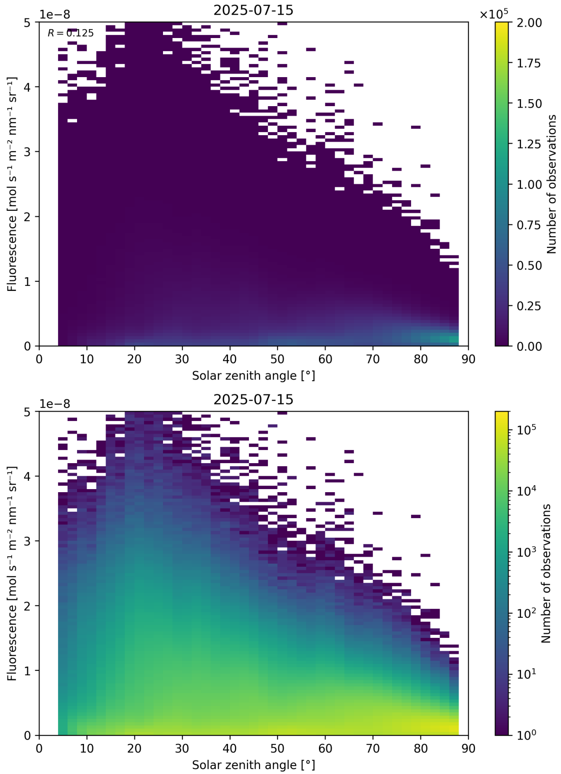
Figure 112: Scatter density plot of “Solar zenith angle” against “Fluorescence” for 2025-07-14 to 2025-07-16.
