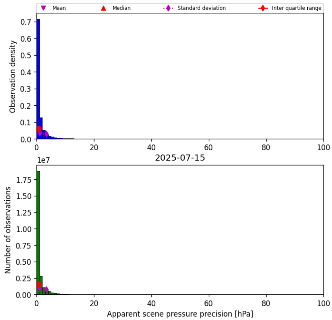
Figure 37: Histogram of “Apparent scene pressure precision” for 2025-07-14 to 2025-07-16
