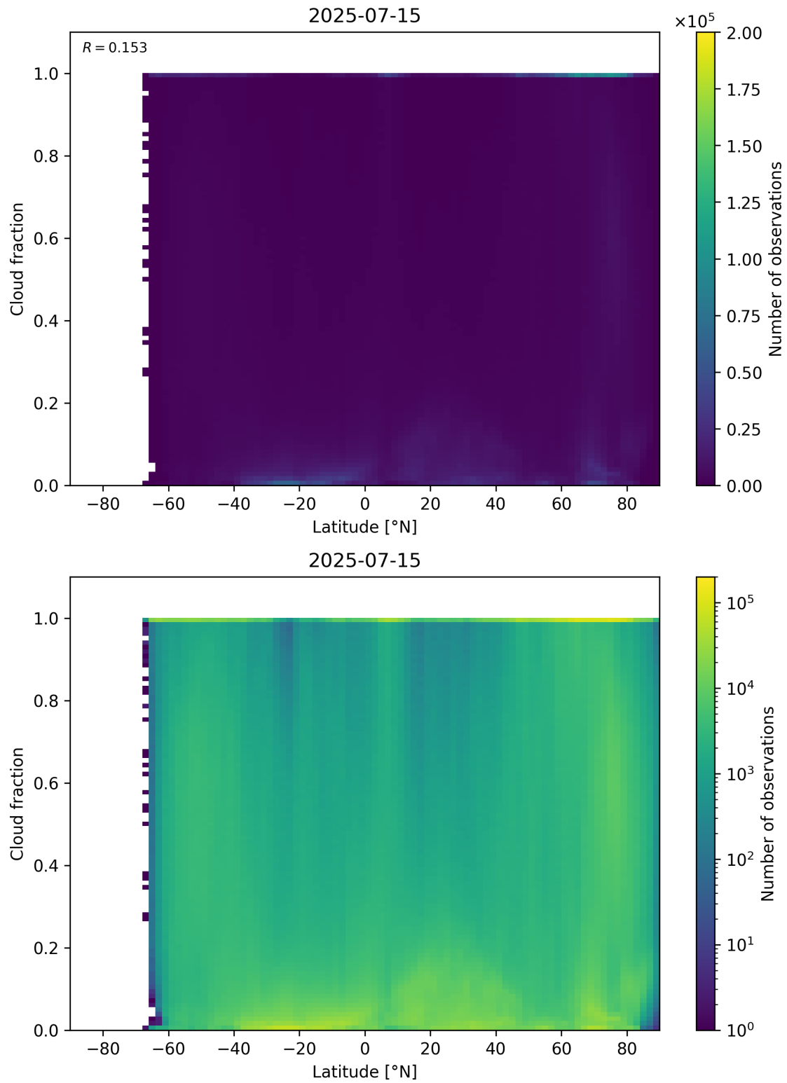
Figure 90: Scatter density plot of “Latitude” against “Cloud fraction” for 2025-07-14 to 2025-07-16.
