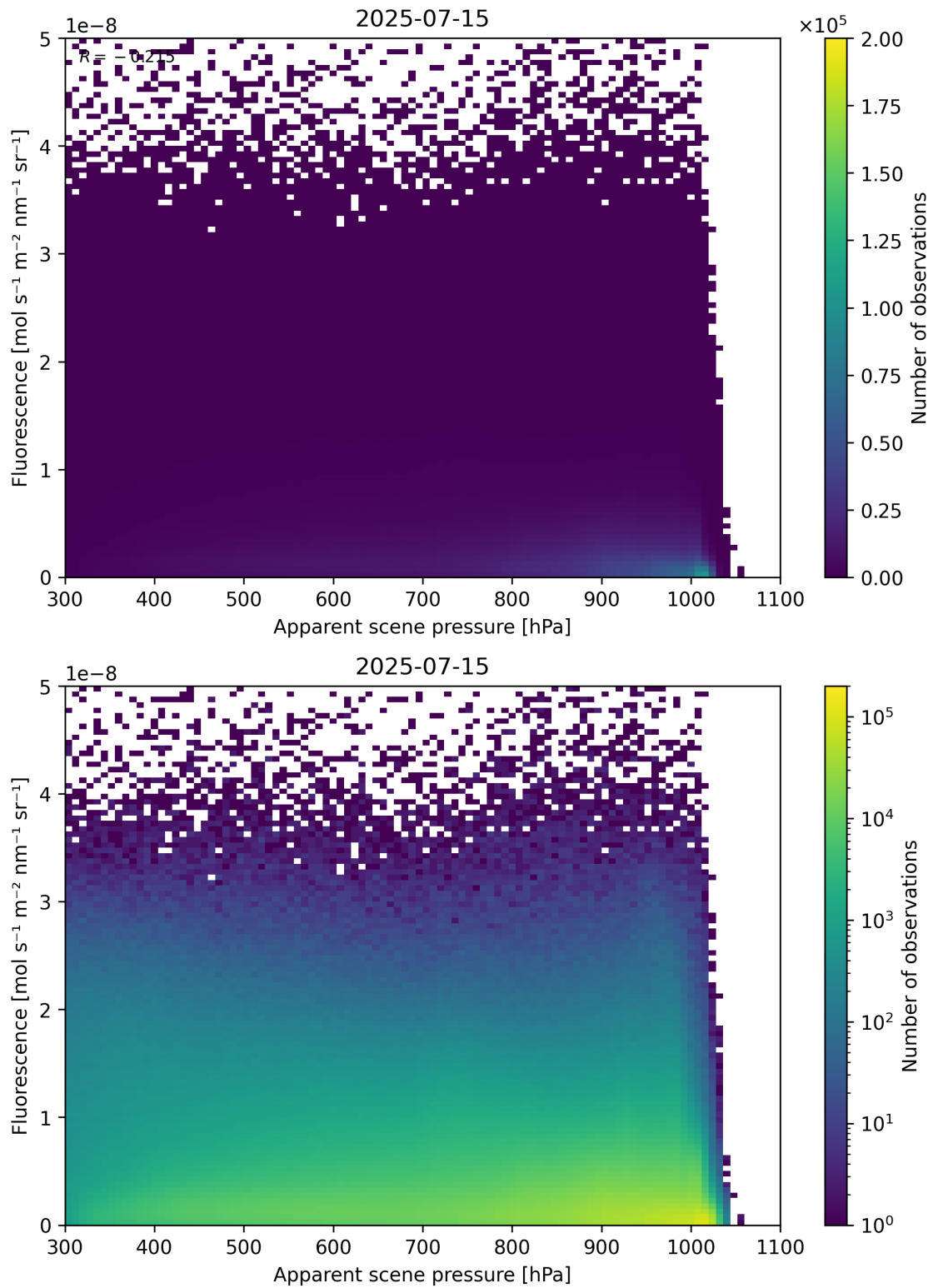
Figure 64: Scatter density plot of “Apparent scene pressure” against “Fluorescence” for 2025-07-14 to 2025-07-16.
