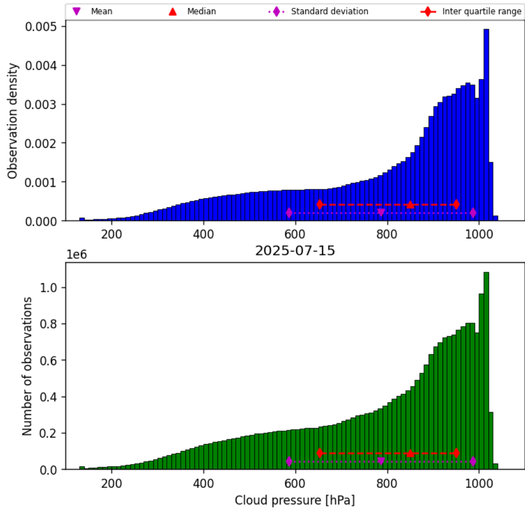
Figure 30: Histogram of “Cloud pressure” for 2025-07-14 to 2025-07-16
