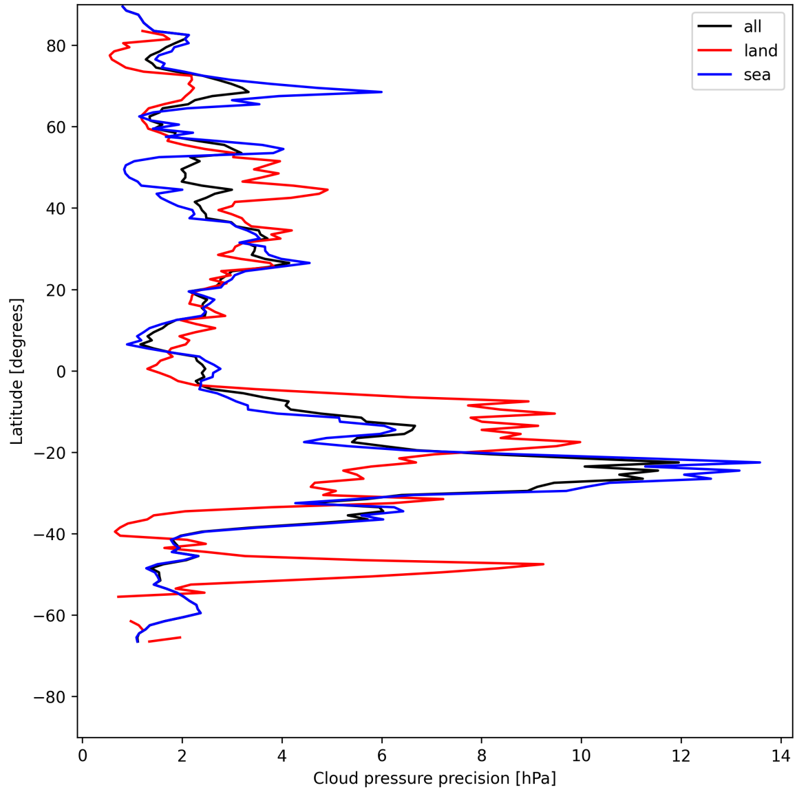
Figure 14: Zonal average of “Cloud pressure precision” for 2025-07-14 to 2025-07-16.
