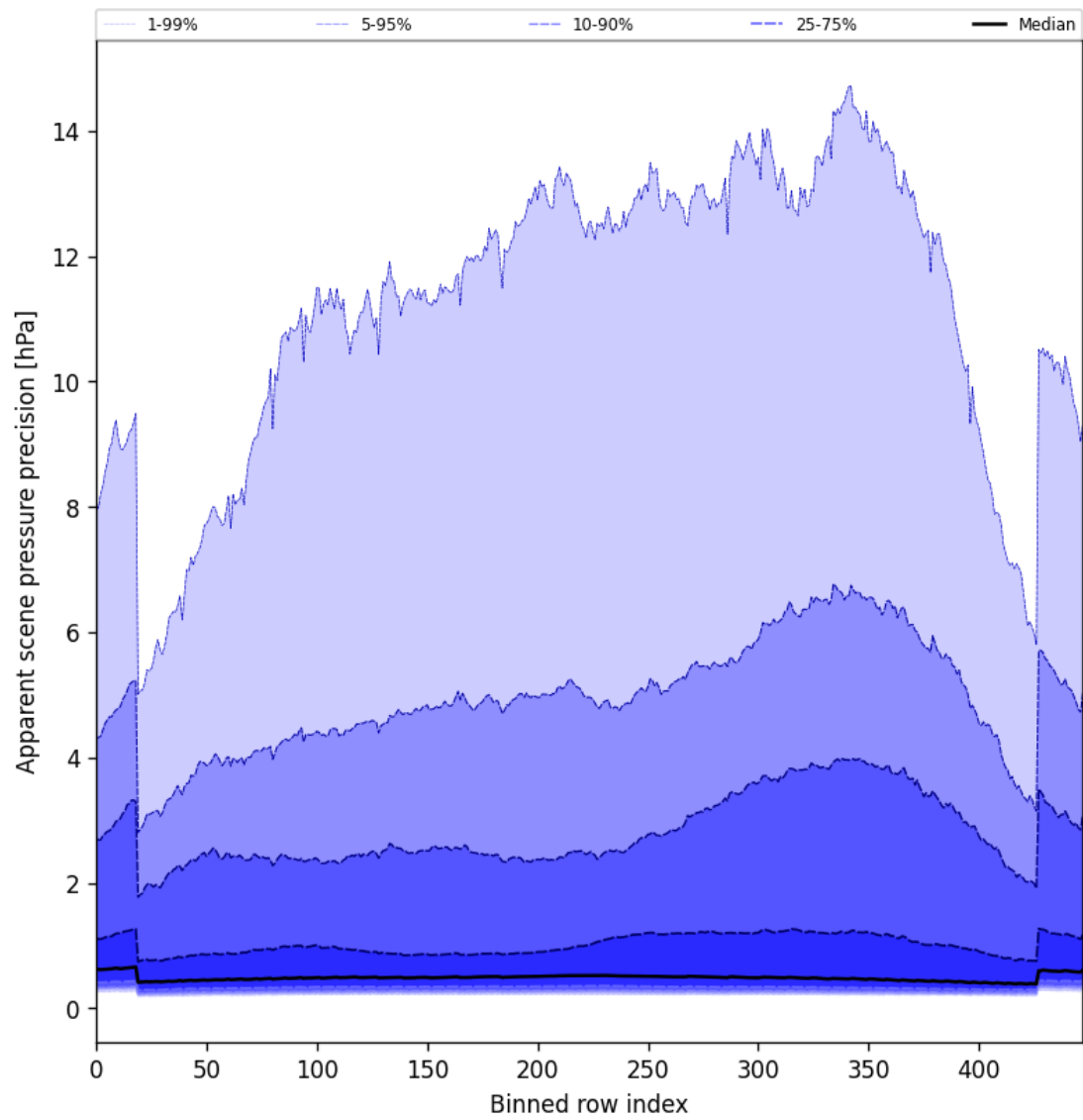
Figure 54: Along track statistics of “Apparent scene pressure precision” for 2025-07-14 to 2025-07-16
