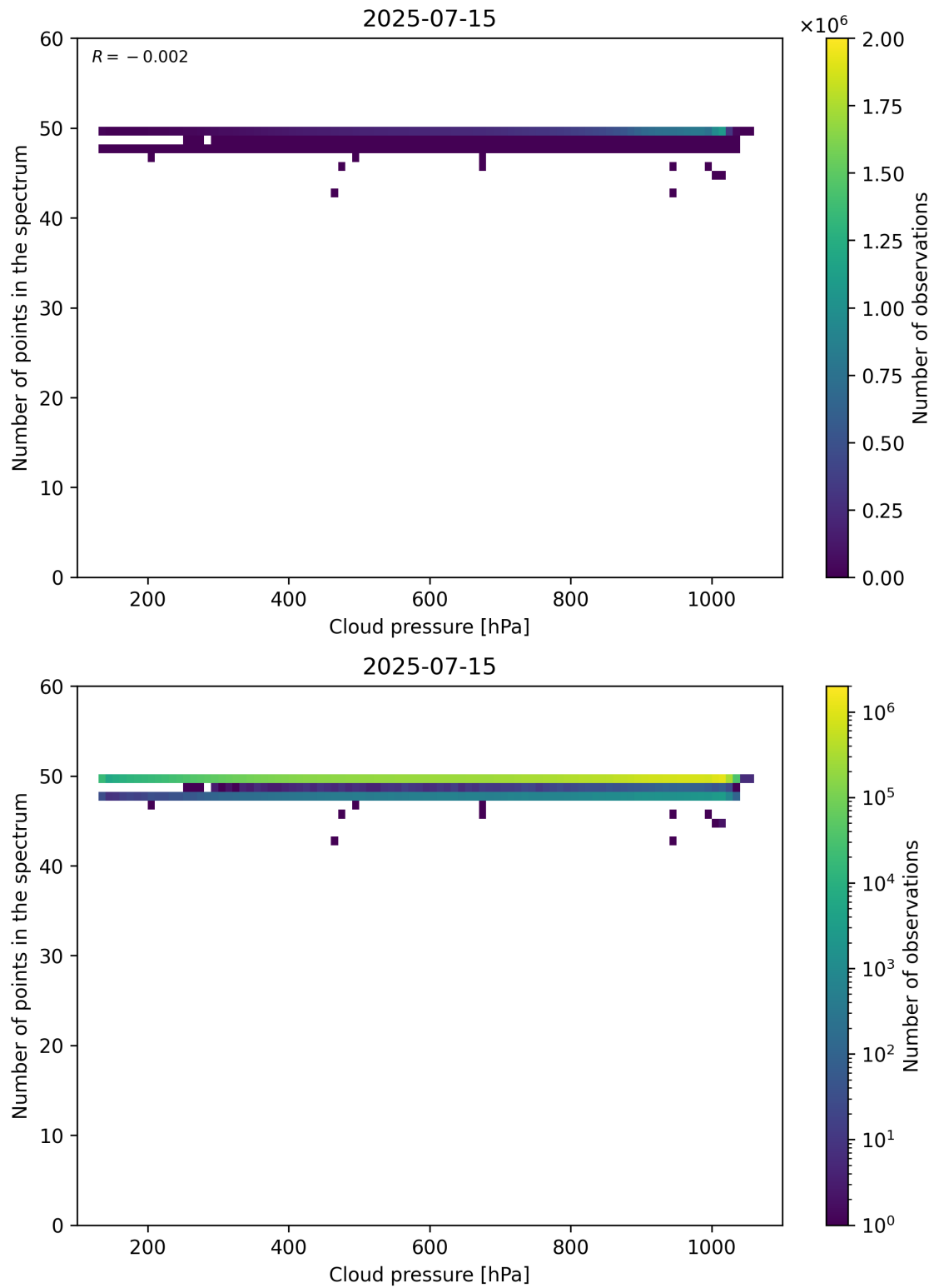
Figure 82: Scatter density plot of “Cloud pressure” against “Number of points in the spectrum” for 2025-07-14 to 2025-07-16.
