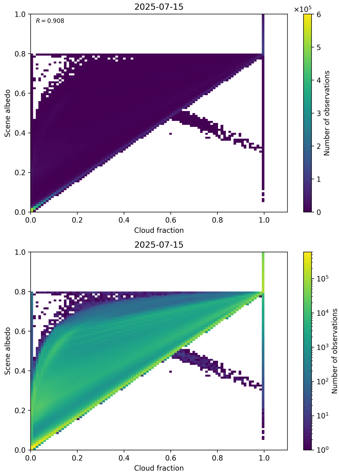
Figure 75: Scatter density plot of “Cloud fraction” against “Scene albedo” for 2025-07-14 to 2025-07-16.
