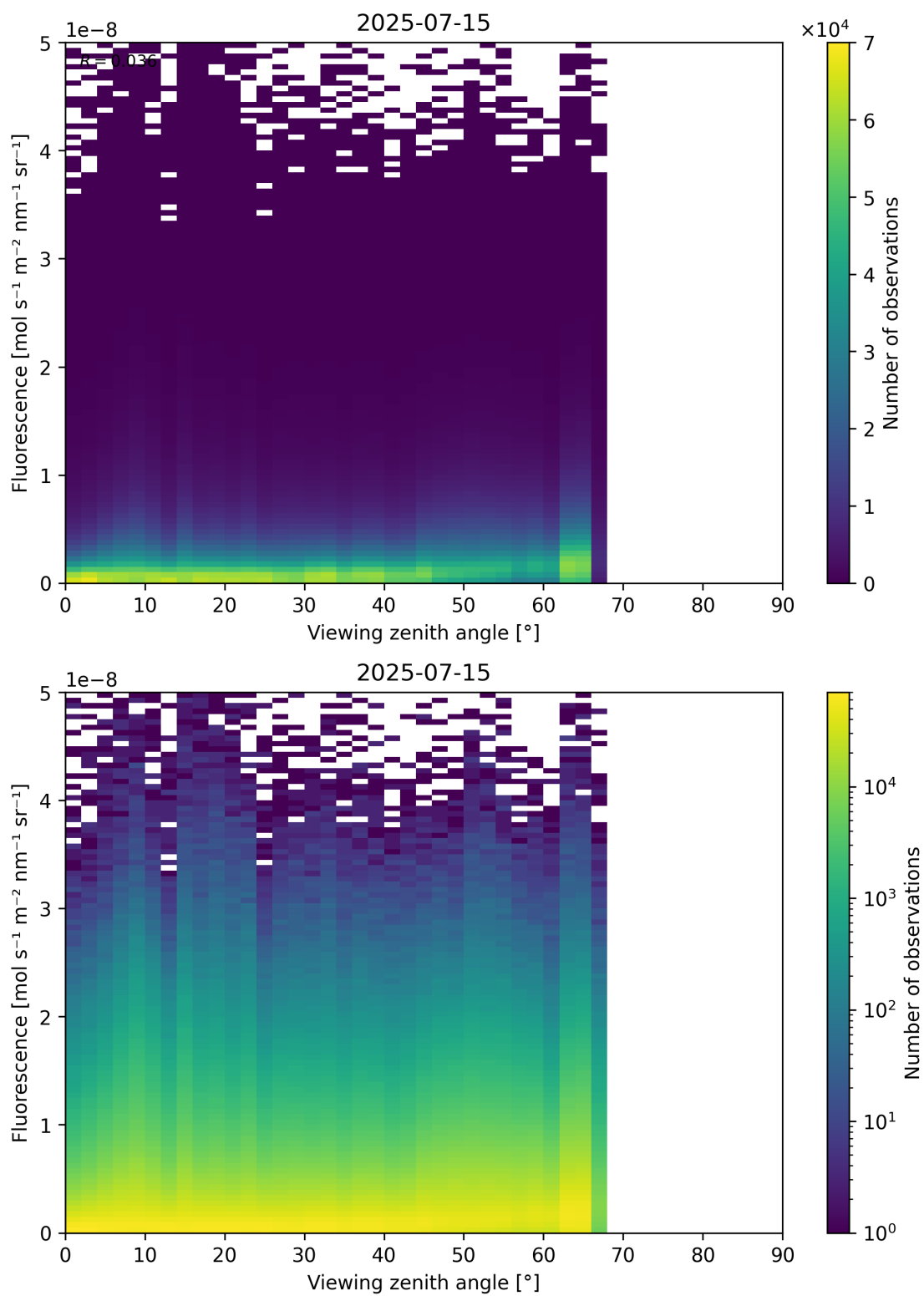
Figure 122: Scatter density plot of “Viewing zenith angle” against “Fluorescence” for 2025-07-14 to 2025-07-16.
