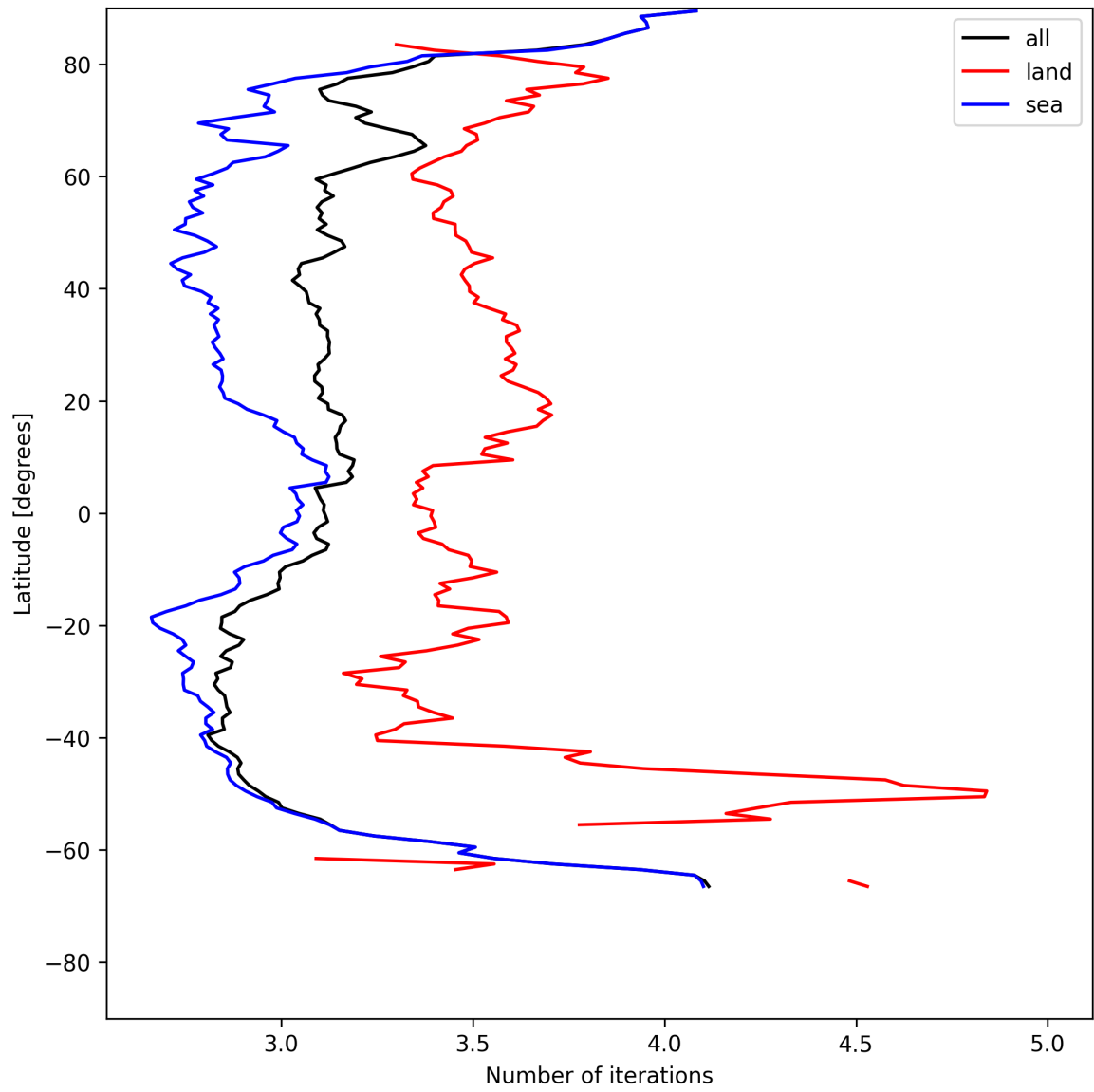
Figure 22: Zonal average of “Number of iterations” for 2025-07-14 to 2025-07-16.
