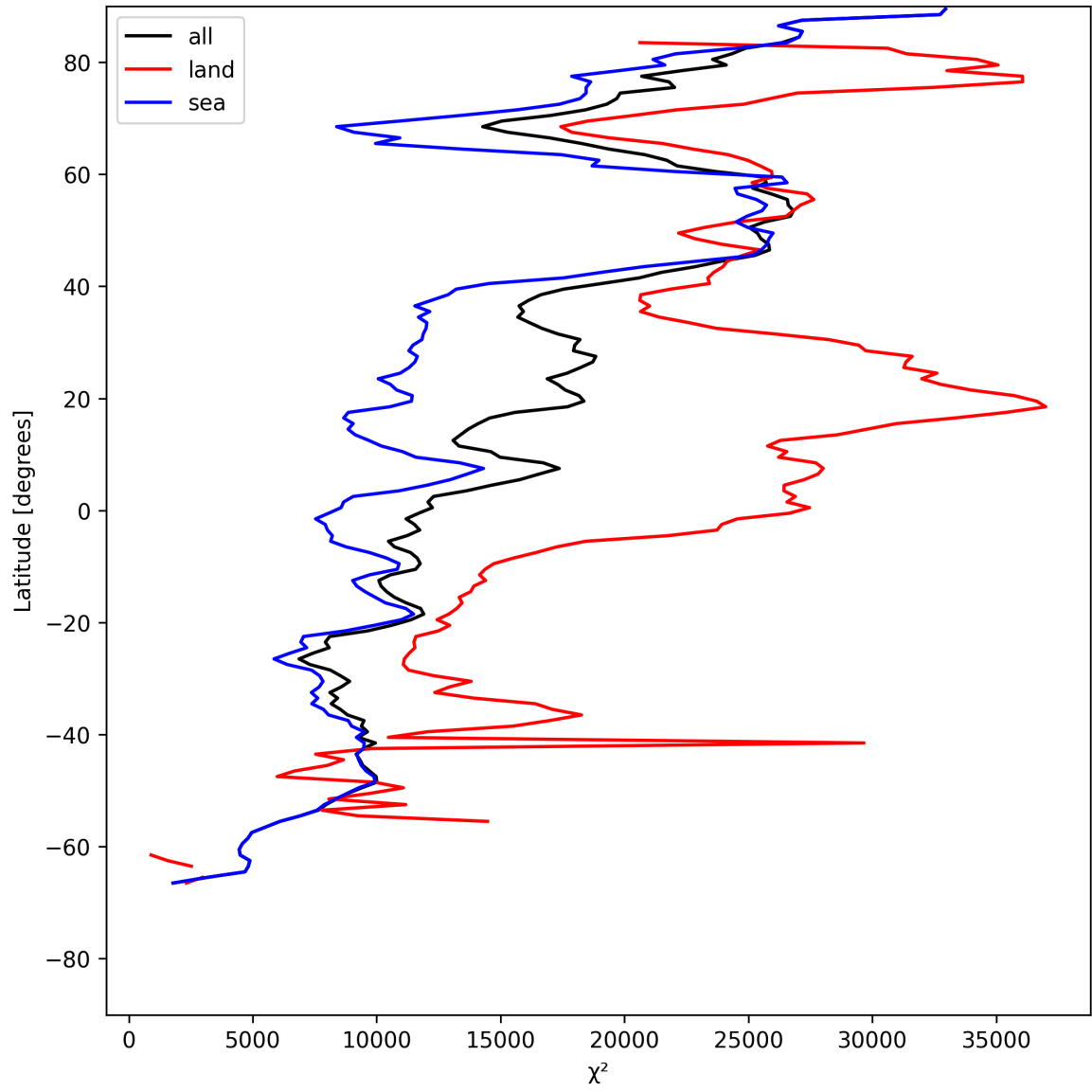
Figure 21: Zonal average of “ \chi^2 ” for 2025-07-14 to 2025-07-16.
