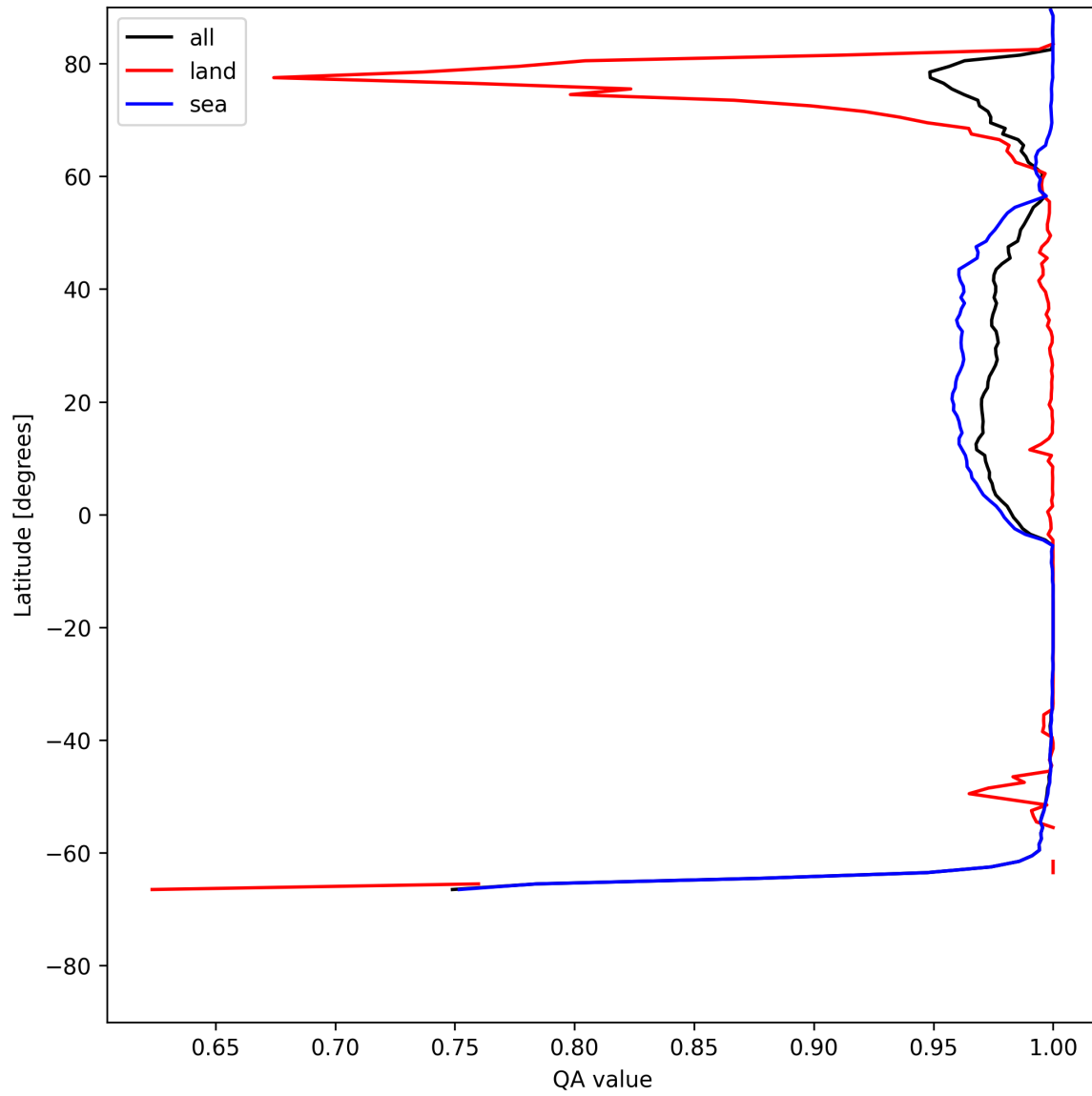
Figure 12: Zonal average of “QA value” for 2025-07-14 to 2025-07-16.
