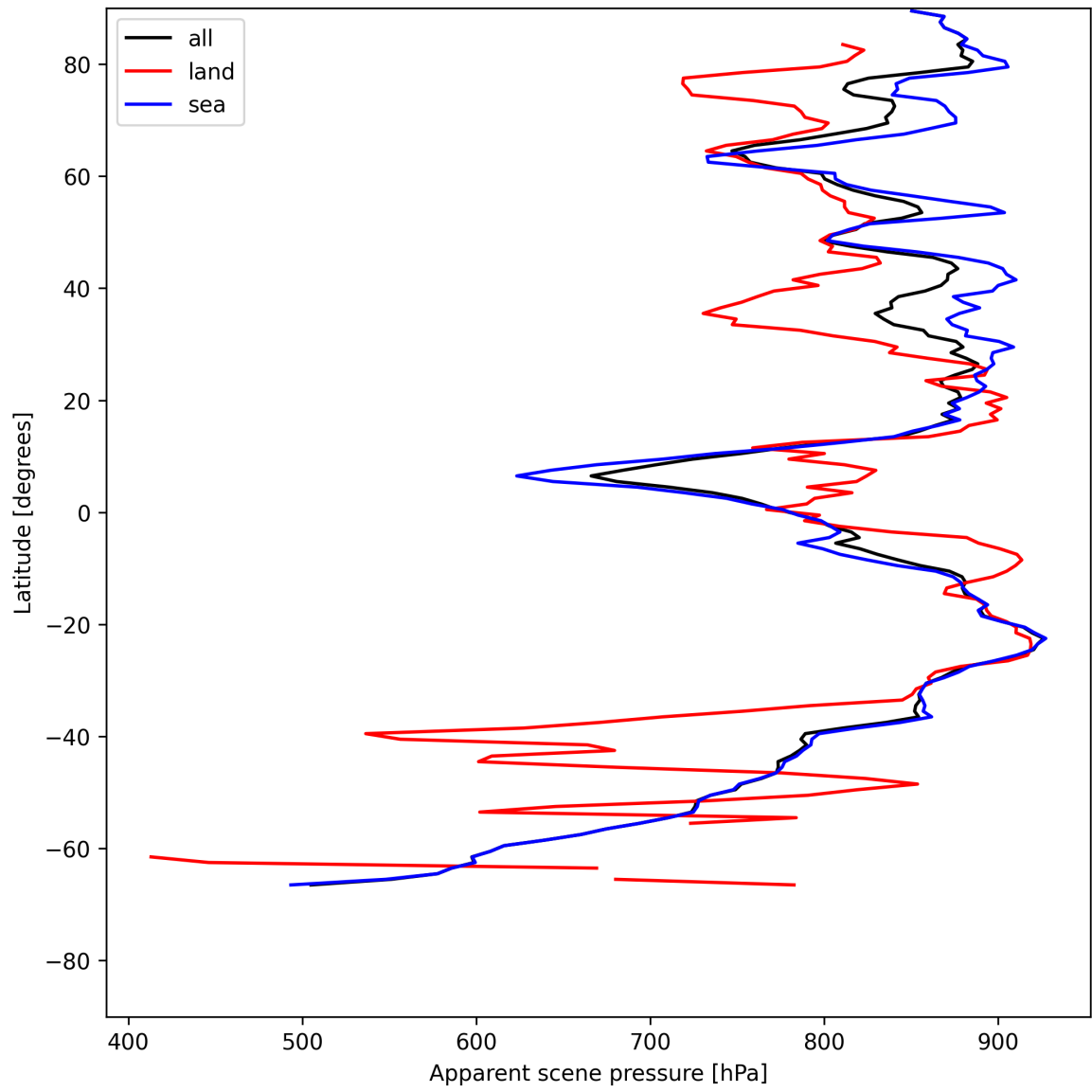
Figure 19: Zonal average of “Apparent scene pressure” for 2025-07-14 to 2025-07-16.
