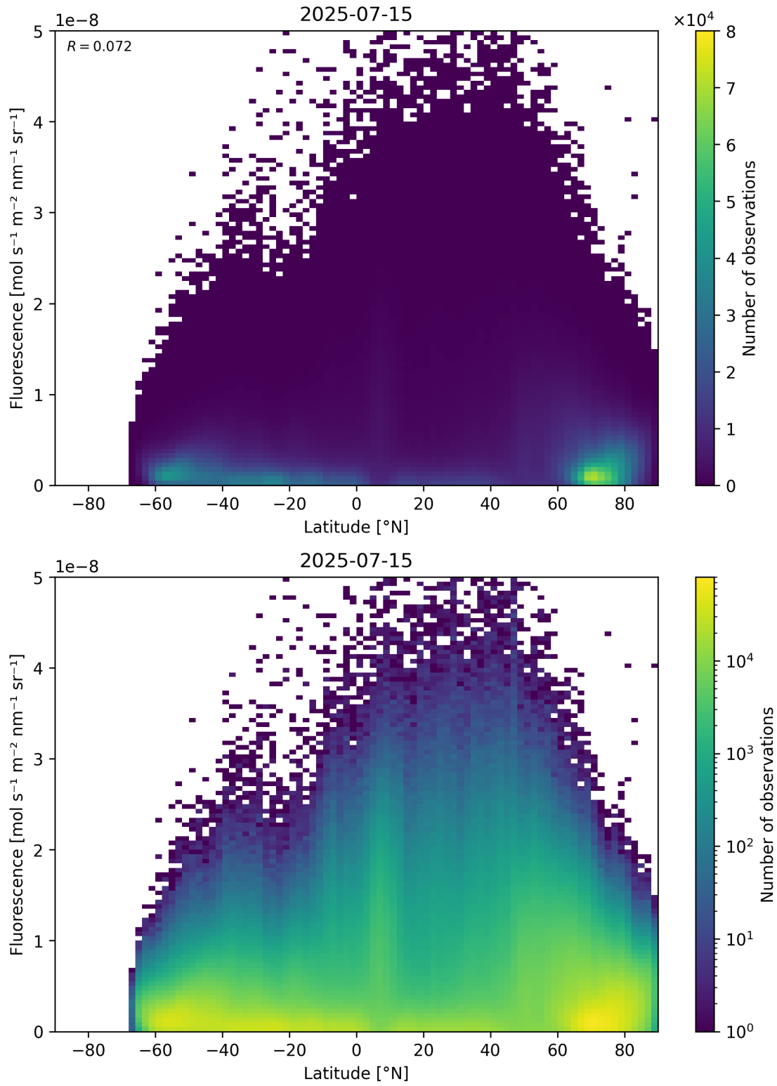
Figure 92: Scatter density plot of “Latitude” against “Fluorescence” for 2025-07-14 to 2025-07-16.
