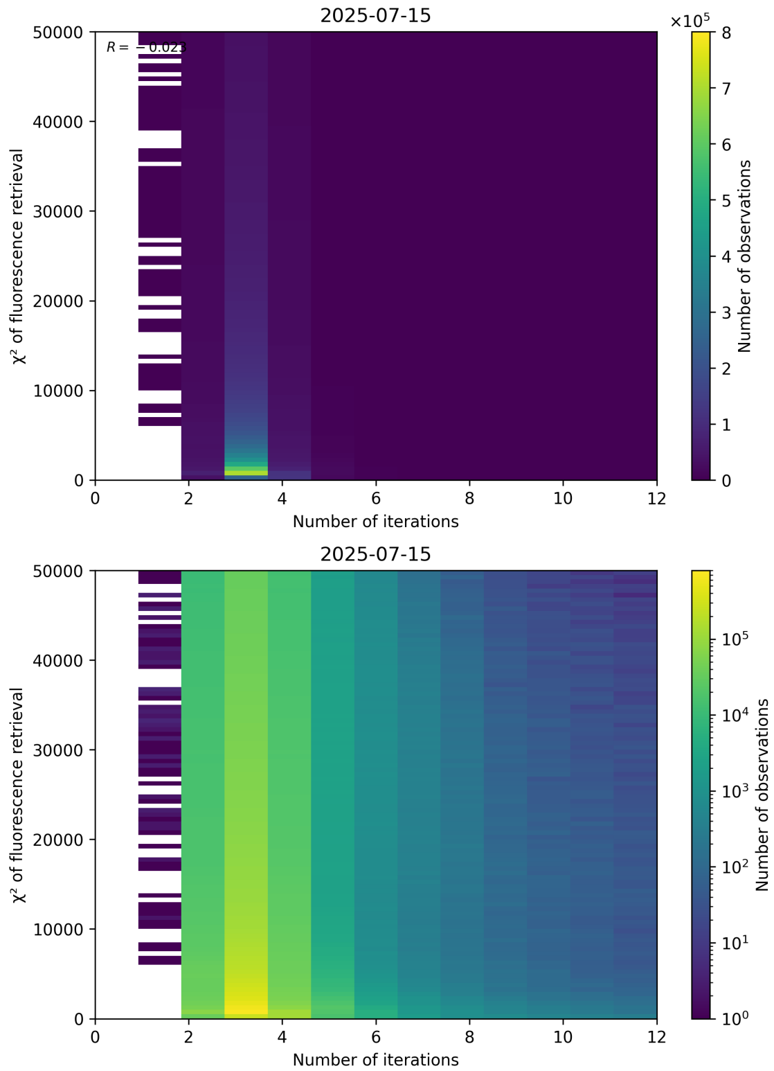
Figure 97: Scatter density plot of “Number of iterations” against “ \chi^2 of fluorescence retrieval” for 2025-07-14 to 2025-07-16.
