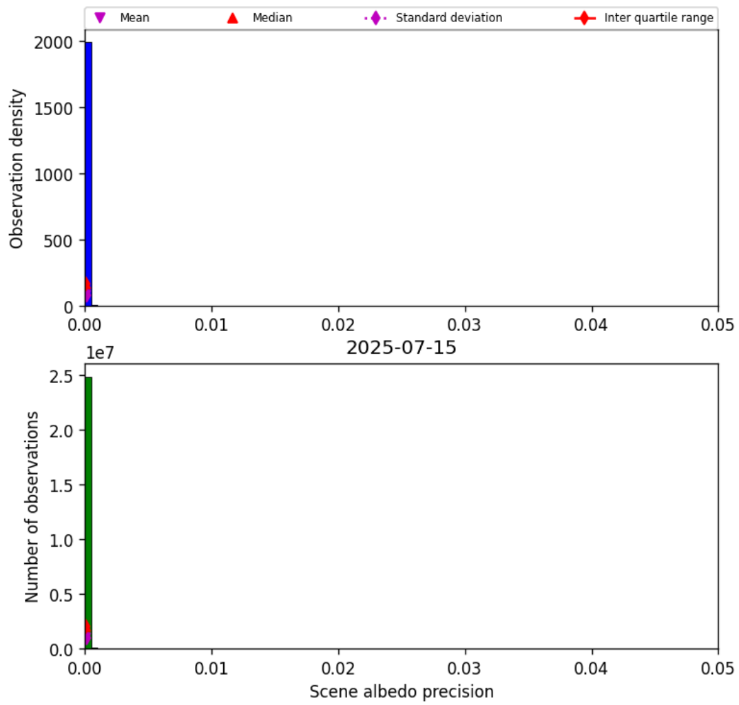
Figure 35: Histogram of “Scene albedo precision” for 2025-07-14 to 2025-07-16
