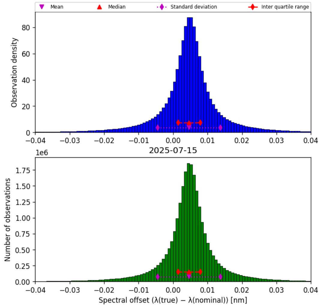
Figure 45: Histogram of “Spectral offset ( \lambda_{\text{true}} - \lambda_{\text{nominal}} )” for 2025-07-14 to 2025-07-16
