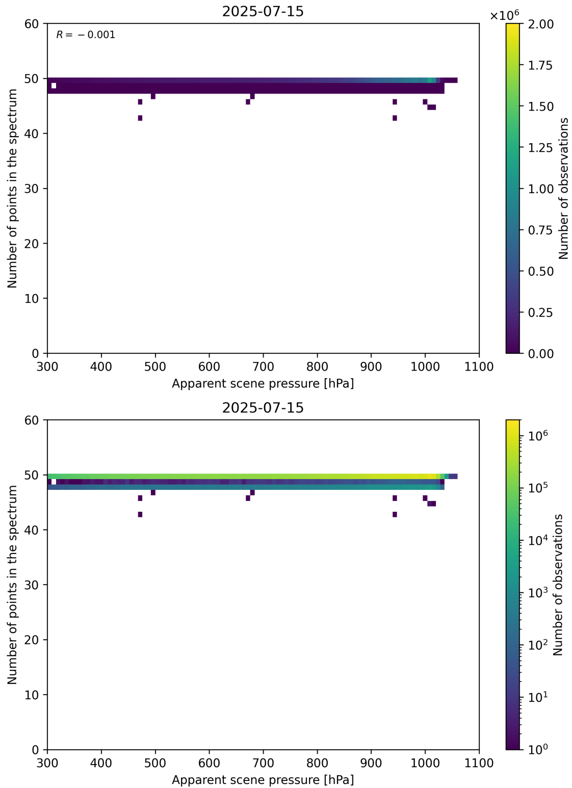
Figure 66: Scatter density plot of “Apparent scene pressure” against “Number of points in the spectrum” for 2025-07-14 to 2025-07-16.
