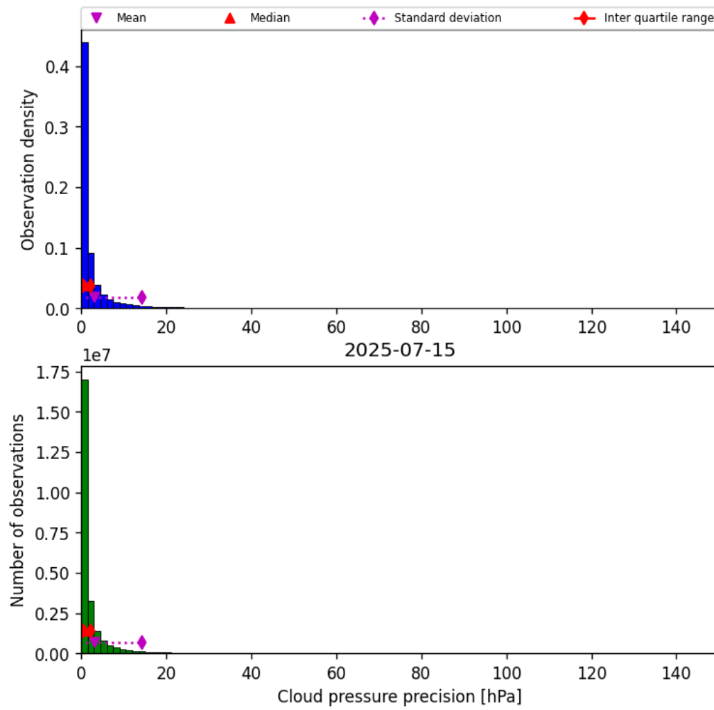
Figure 31: Histogram of “Cloud pressure precision” for 2025-07-14 to 2025-07-16
