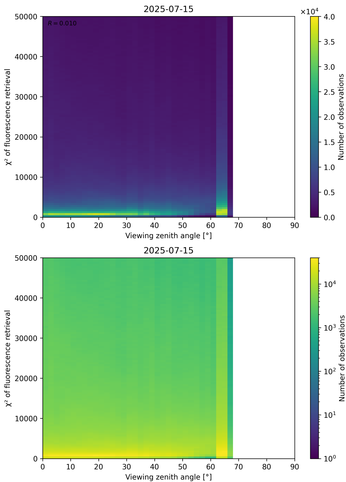
Figure 119: Scatter density plot of “Viewing zenith angle” against “ \chi^2 of fluorescence retrieval” for 2025-07-14 to 2025-07-16.
