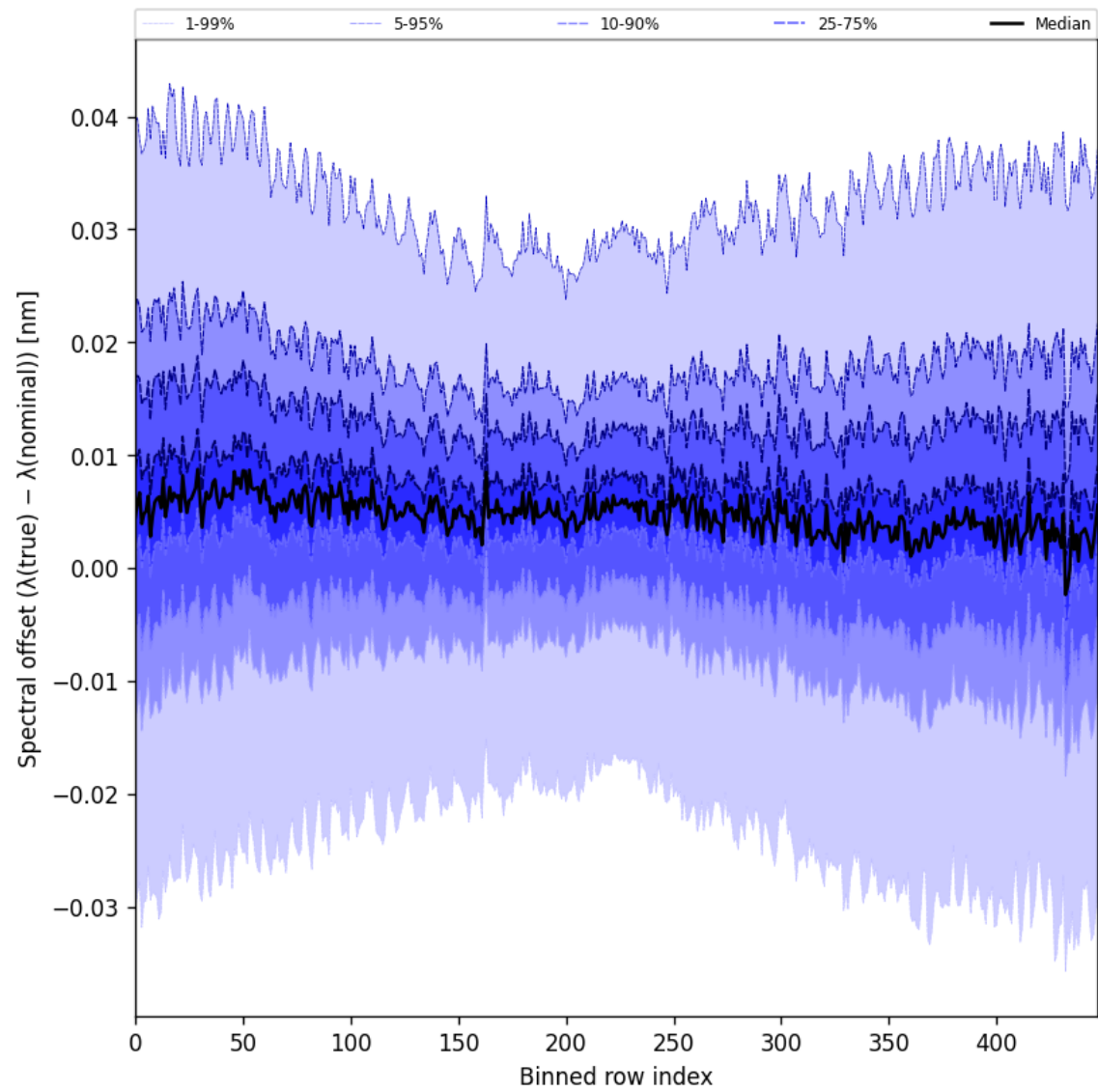
Figure 62: Along track statistics of “Spectral offset ( \lambda_{\text{true}} - \lambda_{\text{nominal}} )” for 2025-07-14 to 2025-07-16
