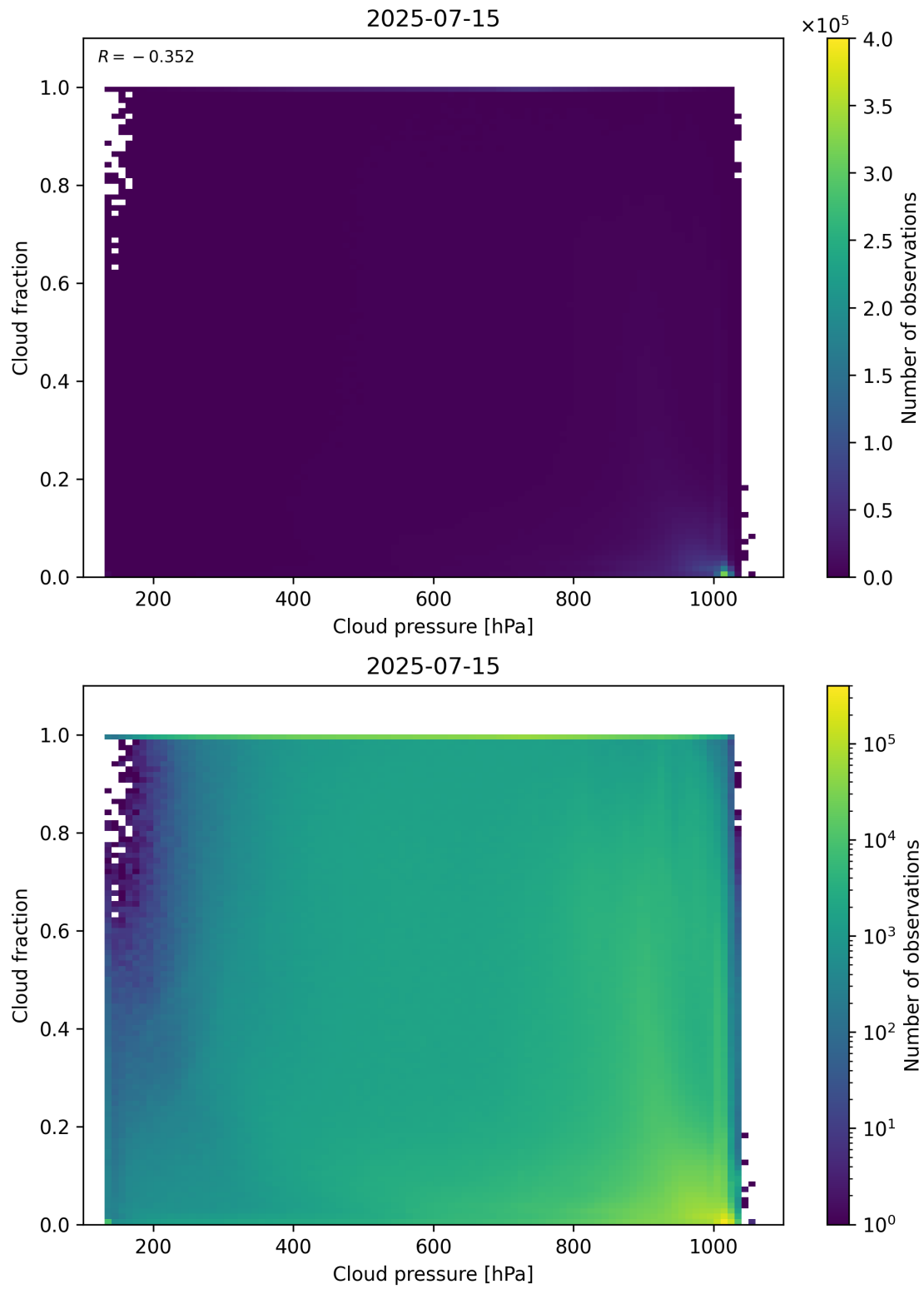
Figure 79: Scatter density plot of “Cloud pressure” against “Cloud fraction” for 2025-07-14 to 2025-07-16.
