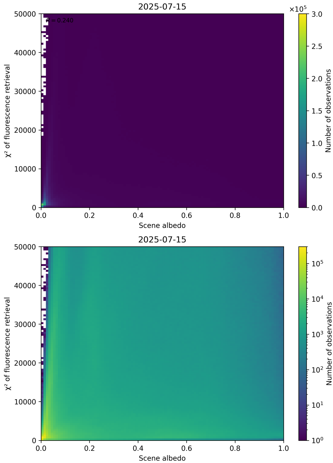
Figure 103: Scatter density plot of “Scene albedo” against “ \chi^2 of fluorescence retrieval” for 2025-07-14 to 2025-07-16.
