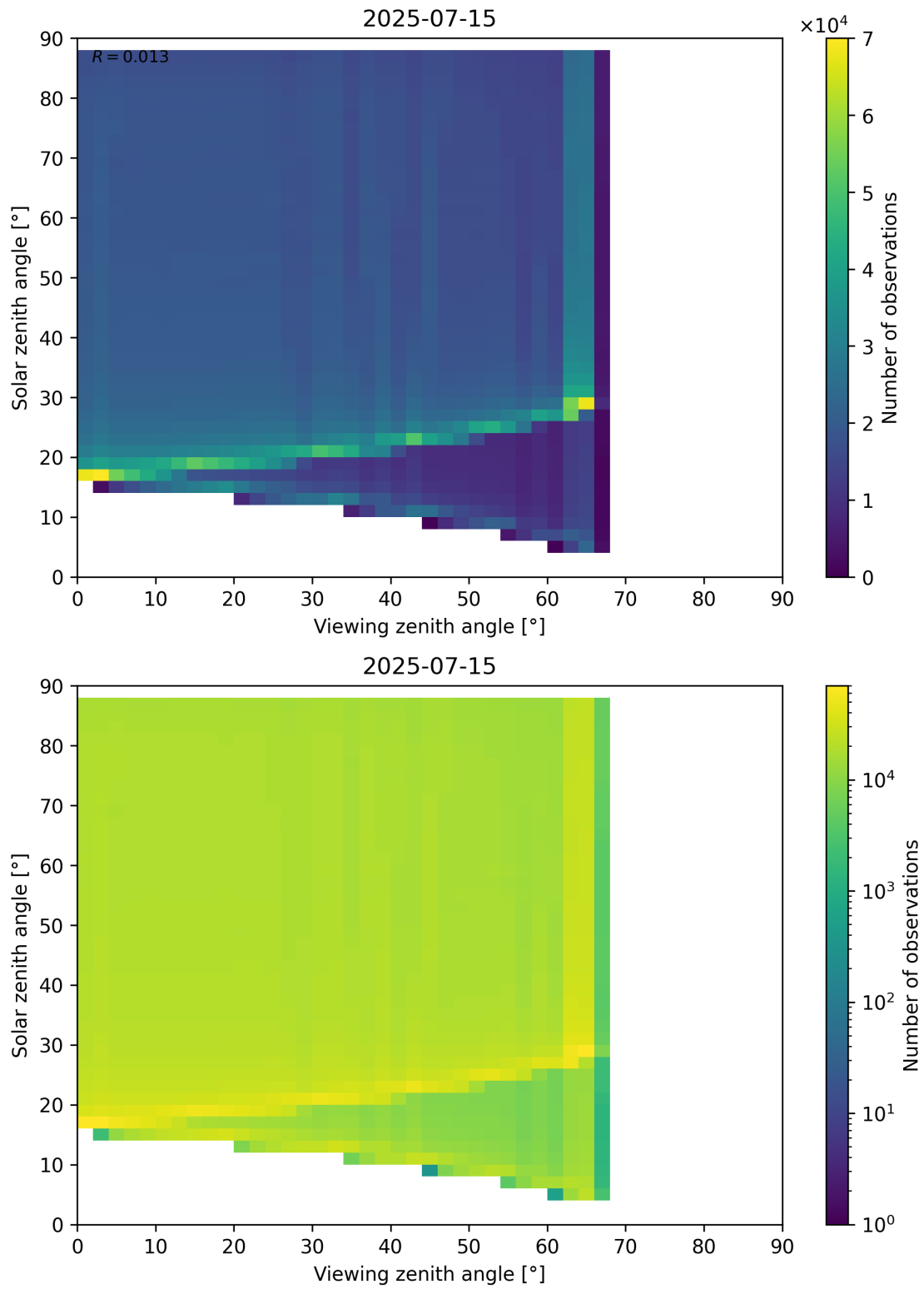
Figure 127: Scatter density plot of “Viewing zenith angle” against “Solar zenith angle” for 2025-07-14 to 2025-07-16.
