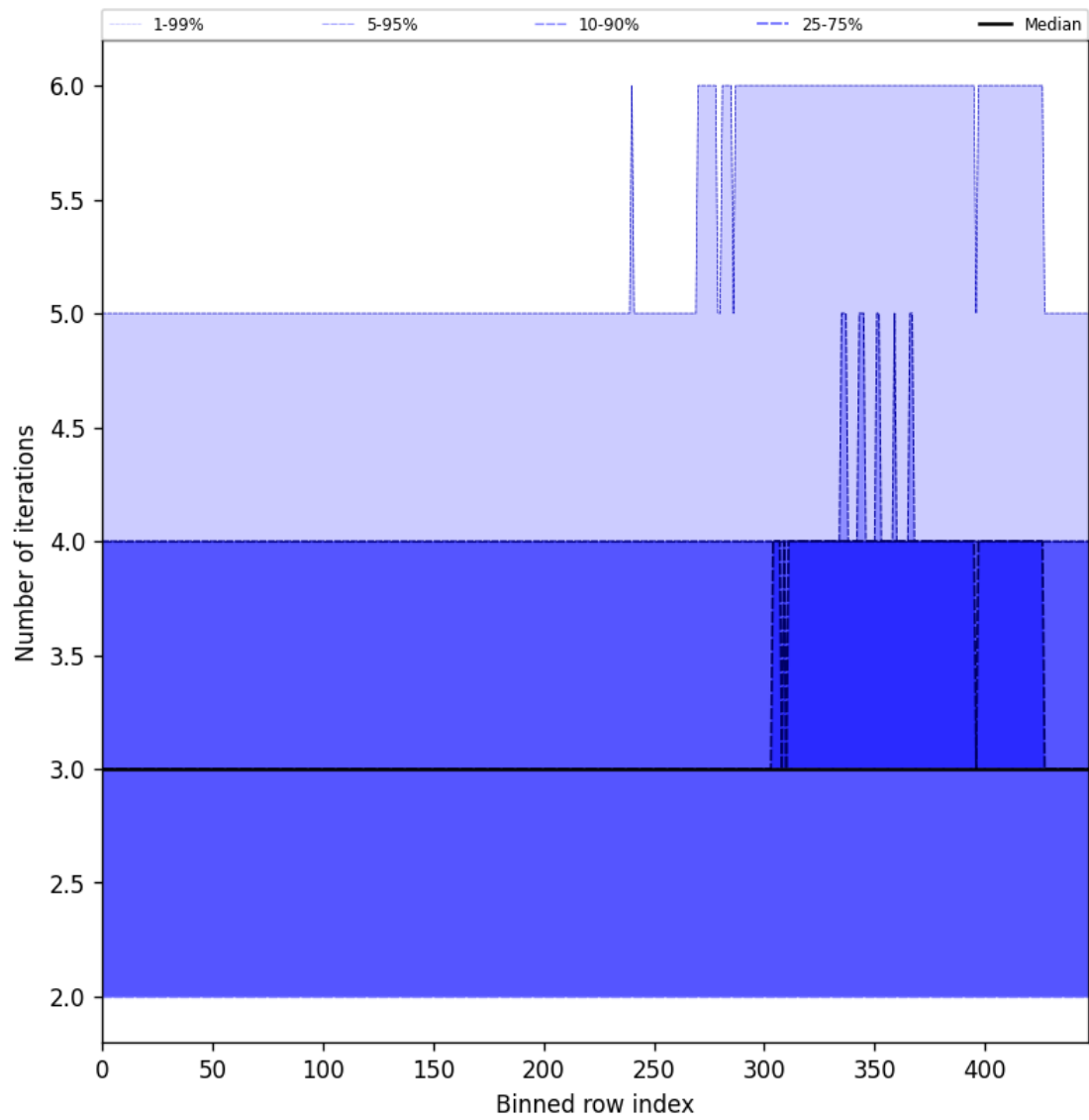
Figure 56: Along track statistics of "Number of iterations" for 2025-07-14 to 2025-07-16
