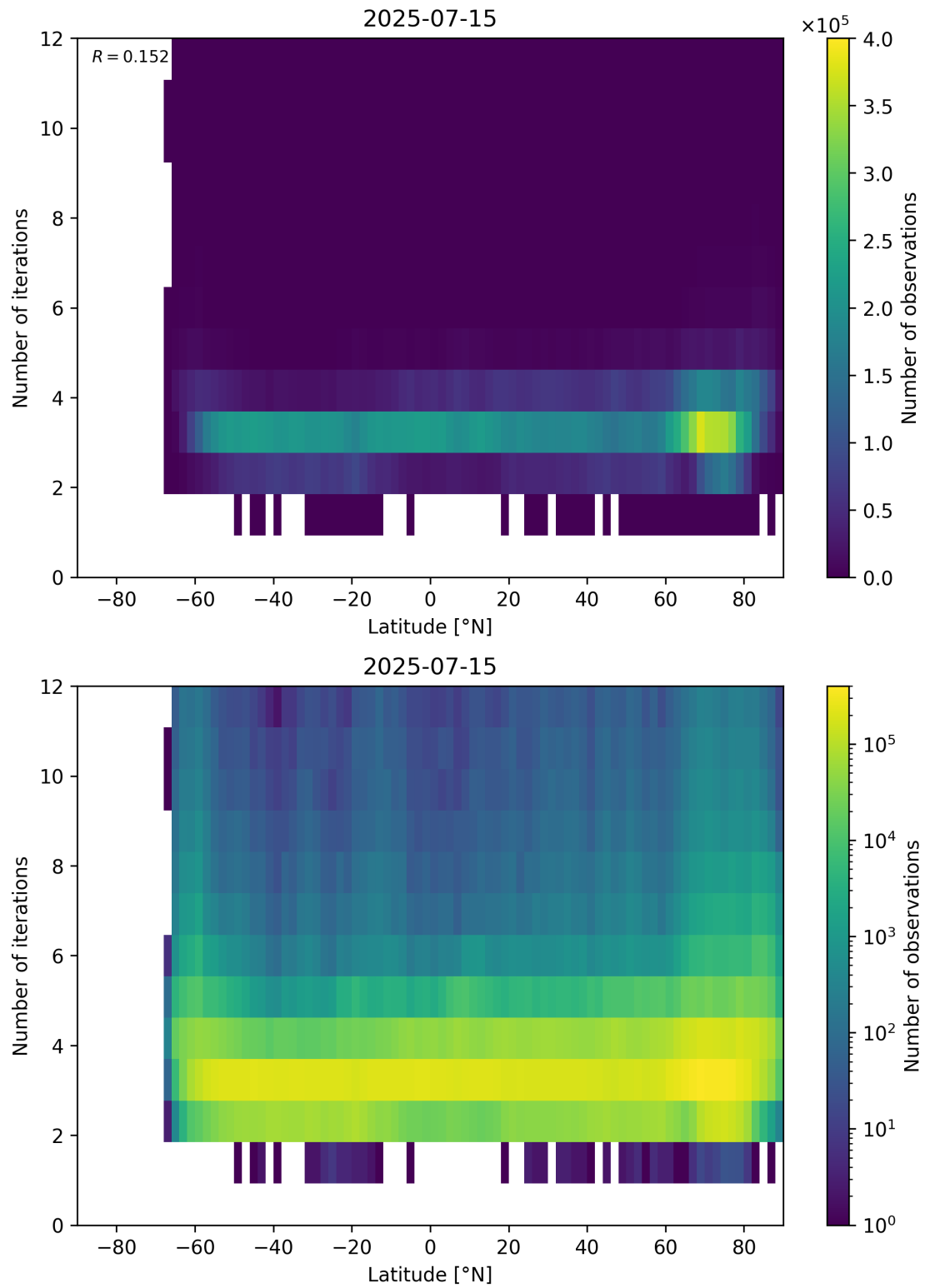
Figure 93: Scatter density plot of “Latitude” against “Number of iterations” for 2025-07-14 to 2025-07-16.
