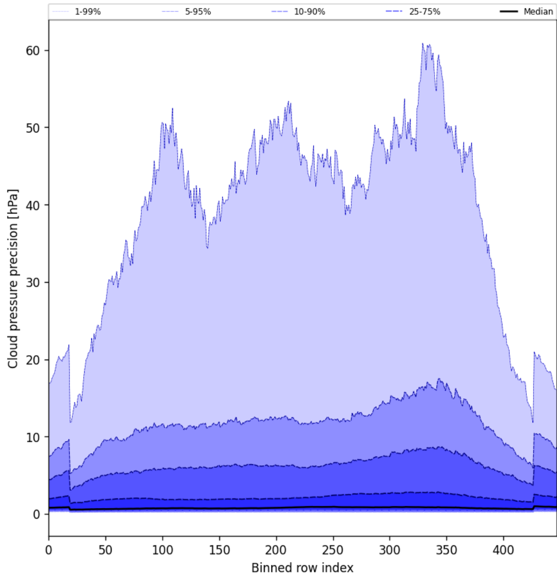
Figure 48: Along track statistics of “Cloud pressure precision” for 2025-07-14 to 2025-07-16
