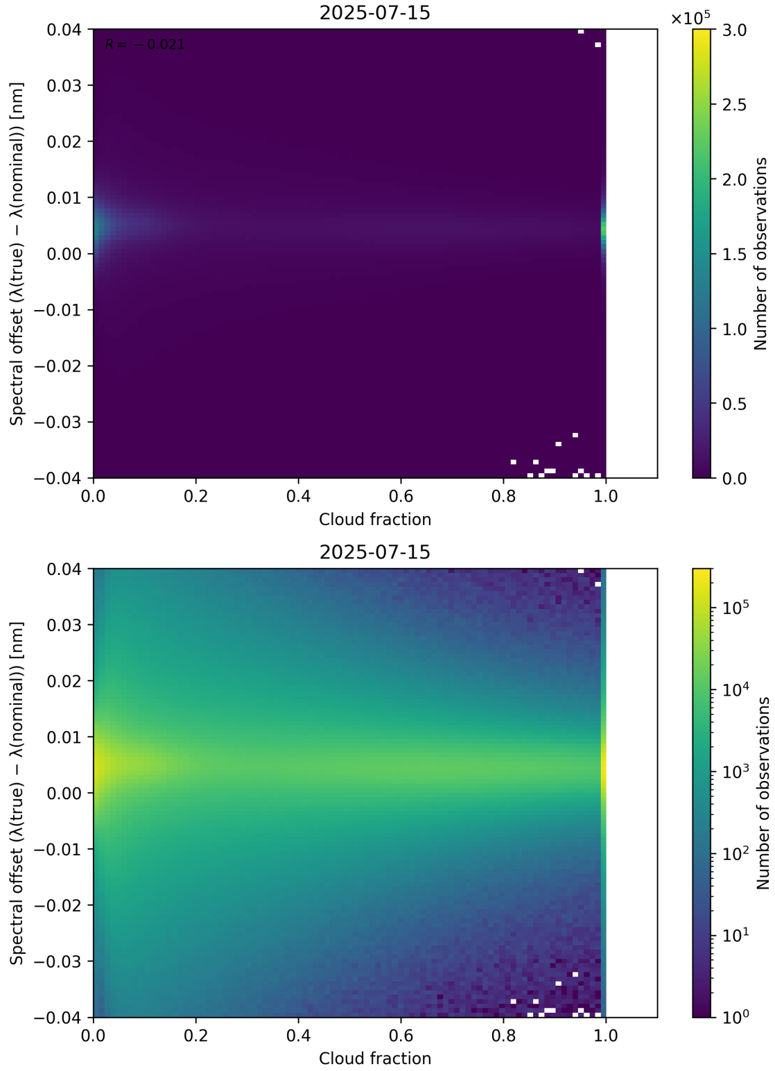
Figure 76: Scatter density plot of “Cloud fraction” against “Spectral offset ( \lambda_{\text{true}} - \lambda_{\text{nominal}} )” for 2025-07-14 to 2025-07-16.
