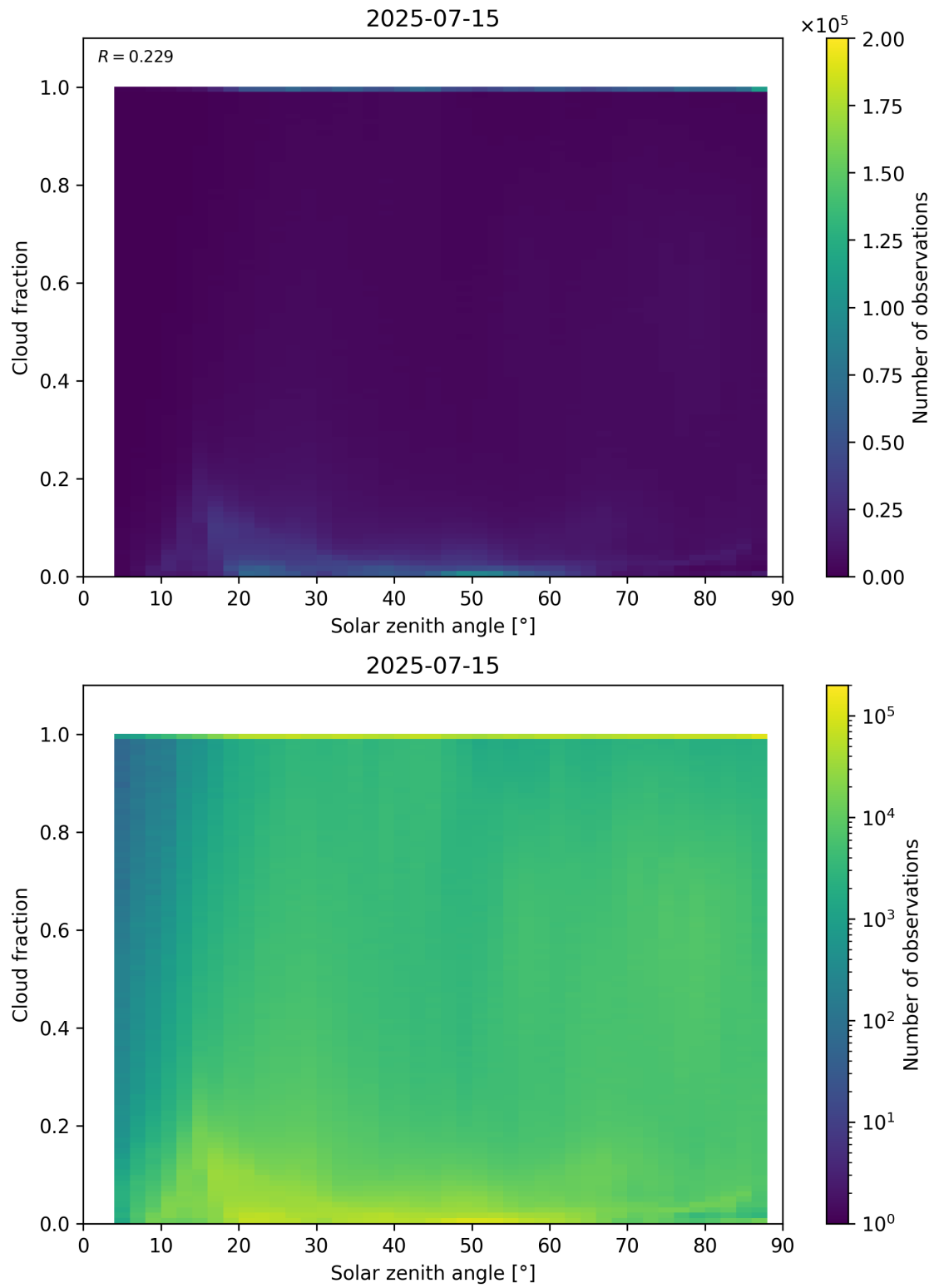
Figure 110: Scatter density plot of “Solar zenith angle” against “Cloud fraction” for 2025-07-14 to 2025-07-16.
