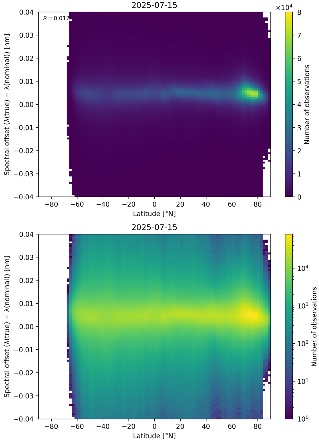
Figure 96: Scatter density plot of “Latitude” against “Spectral offset ( \lambda_{\text{true}} - \lambda_{\text{nominal}} )” for 2025-07-14 to 2025-07-16.
