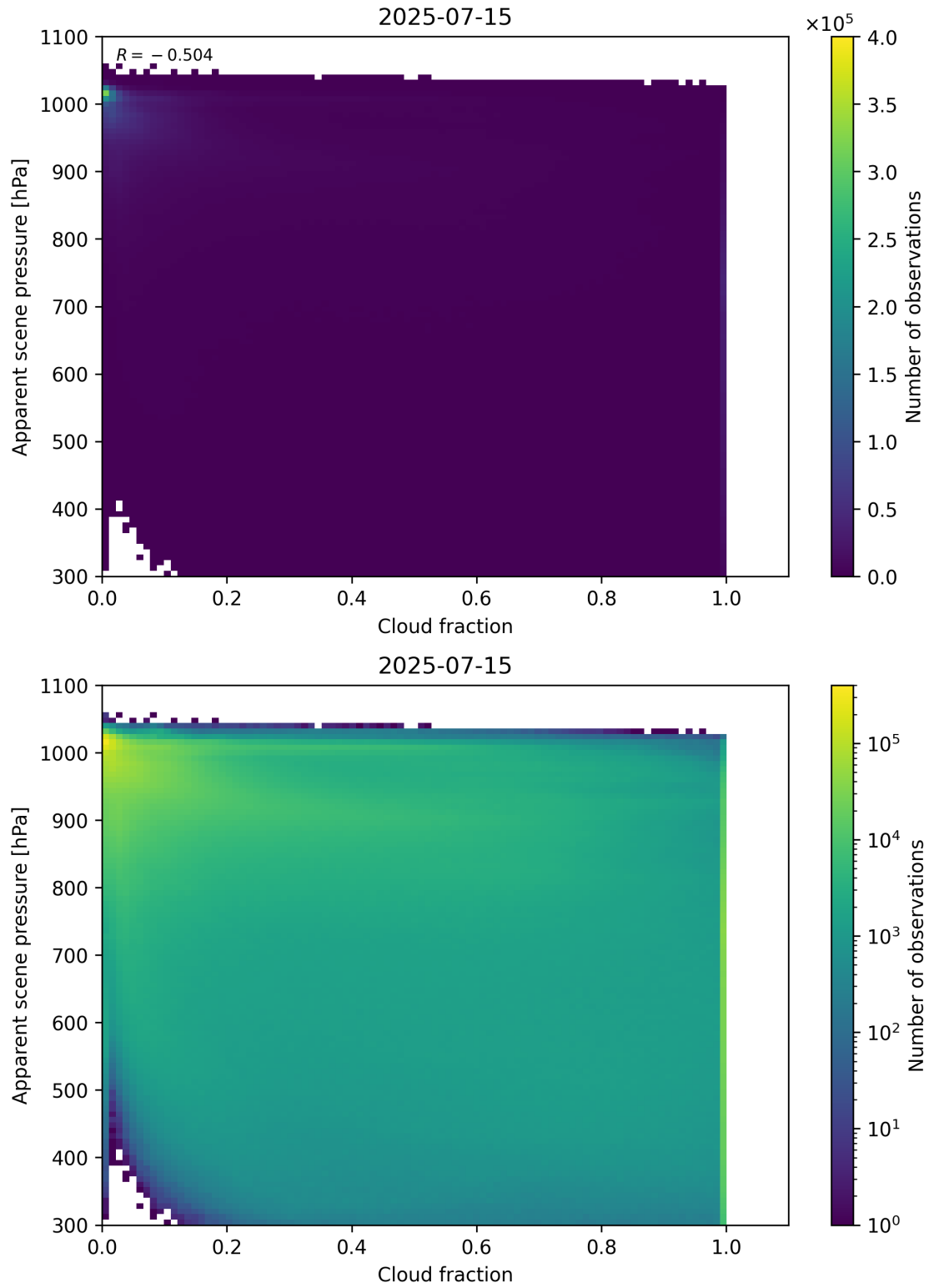
Figure 70: Scatter density plot of “Cloud fraction” against “Apparent scene pressure” for 2025-07-14 to 2025-07-16.
