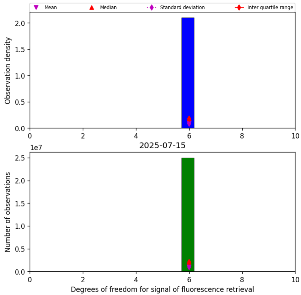
Figure 43: Histogram of “Degrees of freedom for signal of fluorescence retrieval” for 2025-07-14 to 2025-07-16
