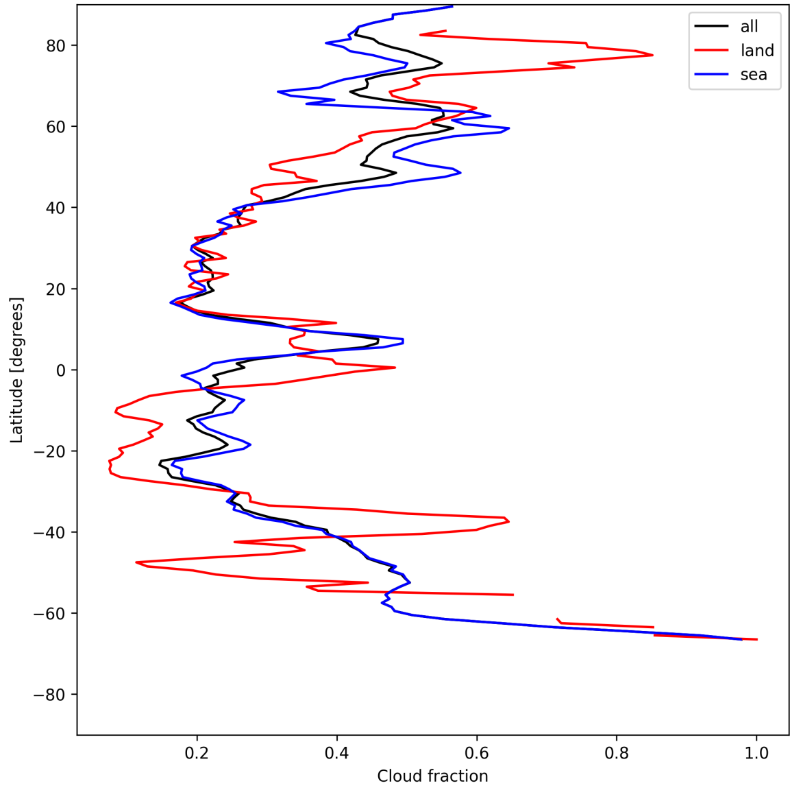
Figure 15: Zonal average of “Cloud fraction” for 2025-07-14 to 2025-07-16.
