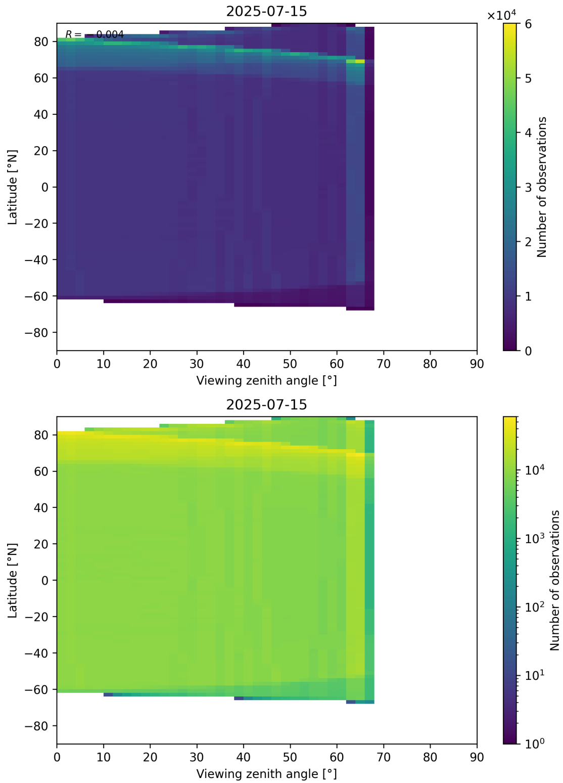
Figure 123: Scatter density plot of “Viewing zenith angle” against “Latitude” for 2025-07-14 to 2025-07-16.
