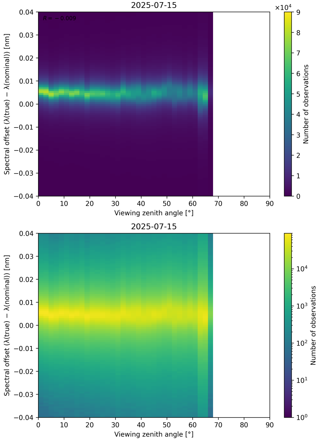
Figure 128: Scatter density plot of “Viewing zenith angle” against “Spectral offset ( \lambda_{\text{true}} - \lambda_{\text{nominal}} )” for 2025-07-14 to 2025-07-16.
