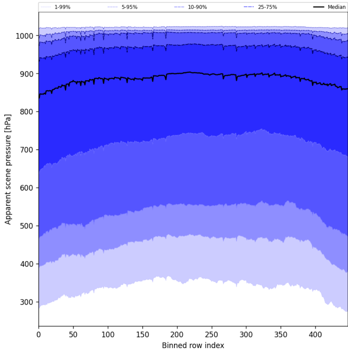
Figure 53: Along track statistics of “Apparent scene pressure” for 2025-07-14 to 2025-07-16
