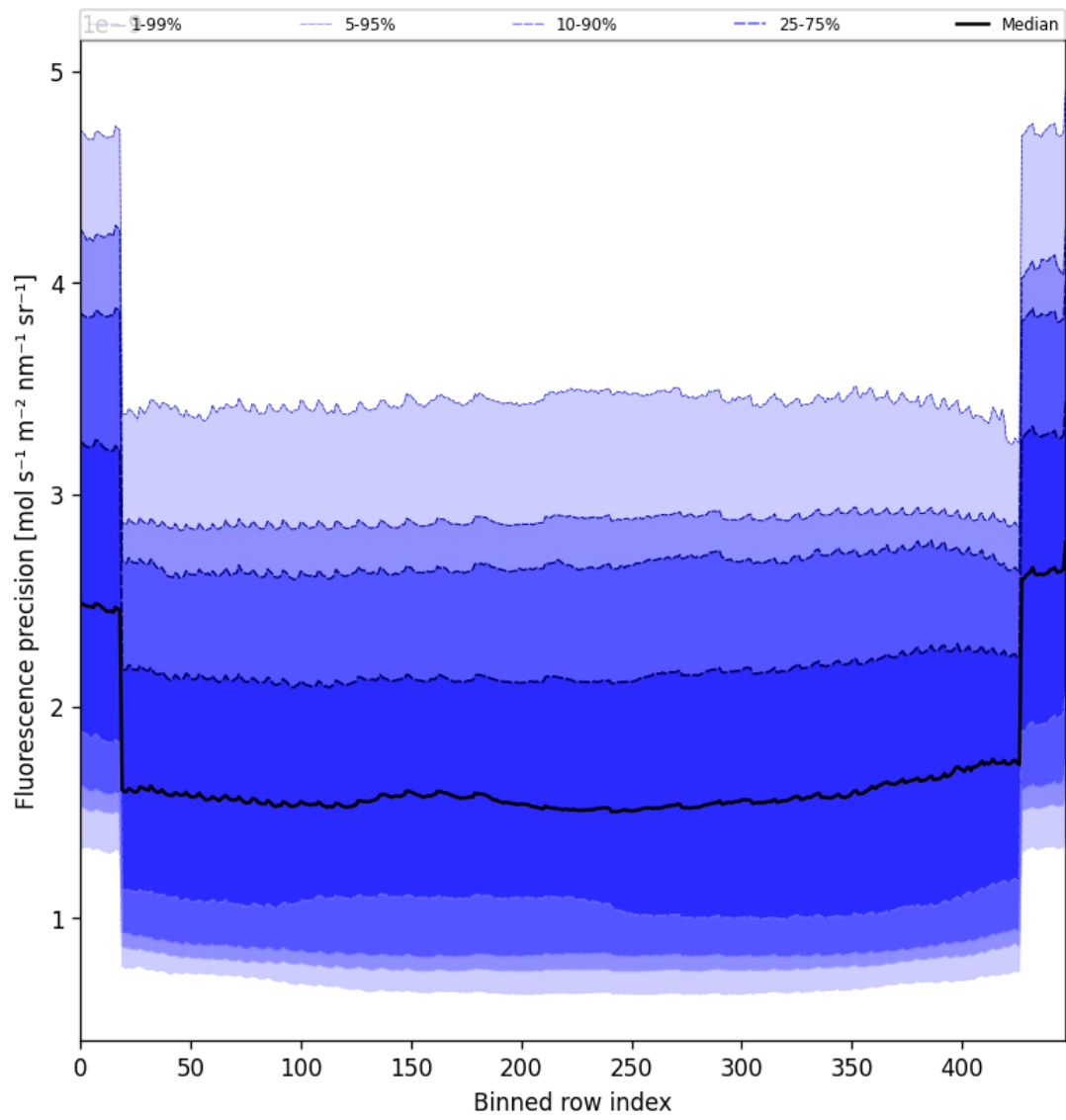
Figure 58: Along track statistics of “Fluorescence precision” for 2025-07-14 to 2025-07-16
