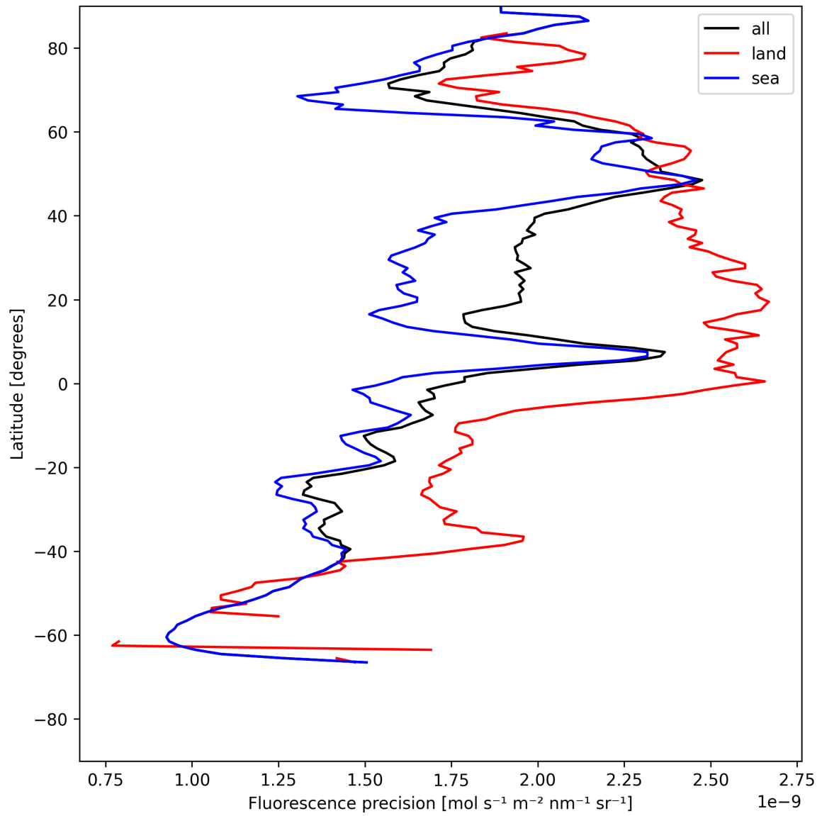
Figure 24: Zonal average of “Fluorescence precision” for 2025-07-14 to 2025-07-16.
