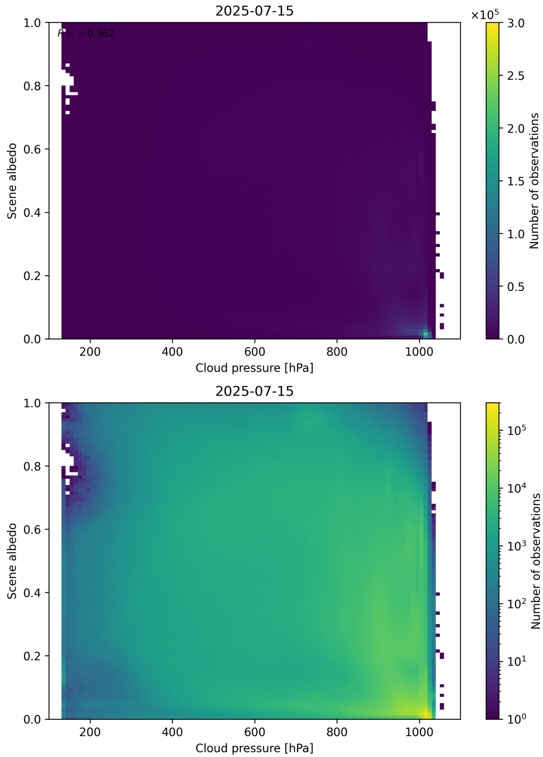
Figure 83: Scatter density plot of “Cloud pressure” against “Scene albedo” for 2025-07-14 to 2025-07-16.
