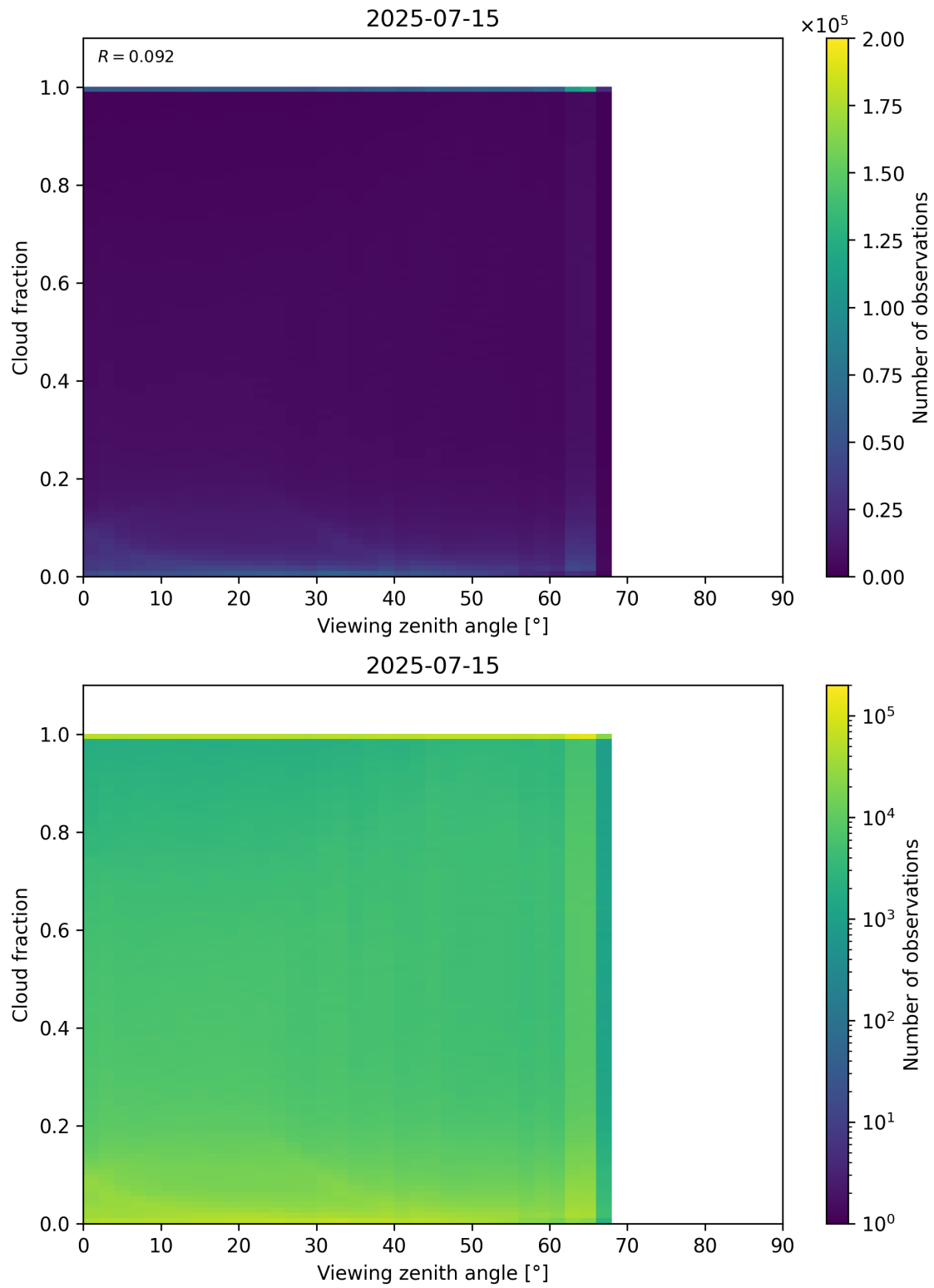
Figure 120: Scatter density plot of “Viewing zenith angle” against “Cloud fraction” for 2025-07-14 to 2025-07-16.
