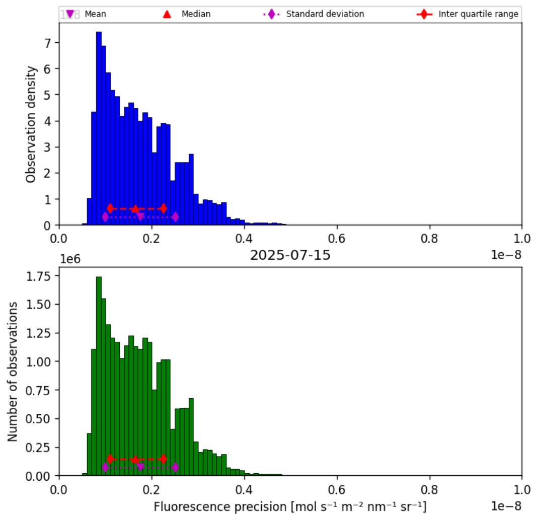
Figure 41: Histogram of “Fluorescence precision” for 2025-07-14 to 2025-07-16
