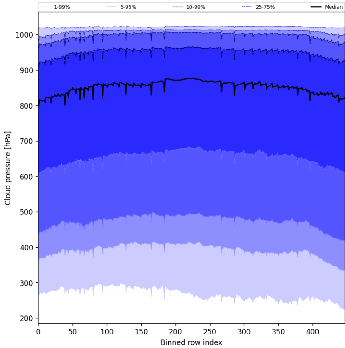
Figure 47: Along track statistics of “Cloud pressure” for 2025-07-14 to 2025-07-16
