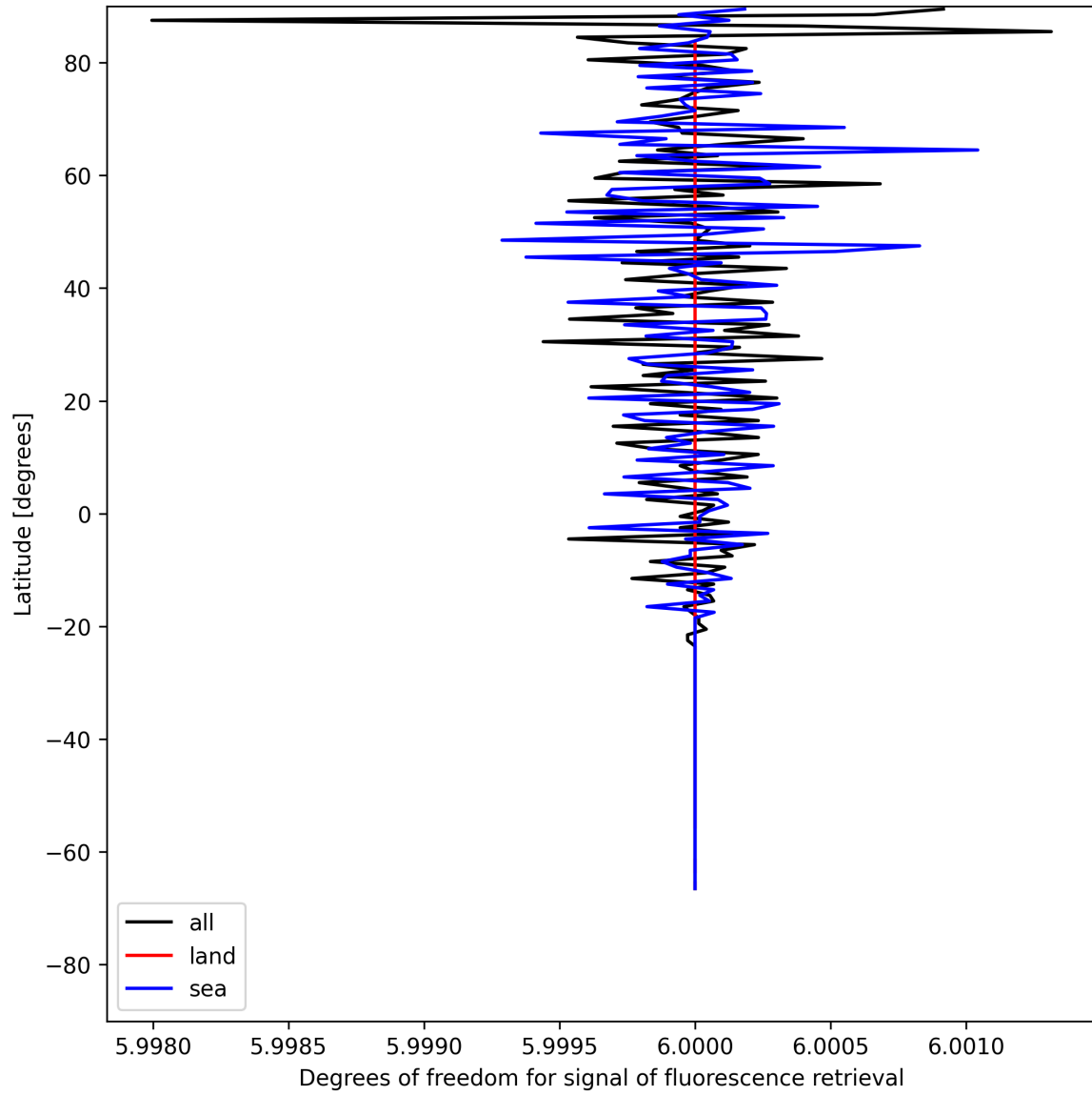
Figure 26: Zonal average of “Degrees of freedom for signal of fluorescence retrieval” for 2025-07-14 to 2025-07-16.
