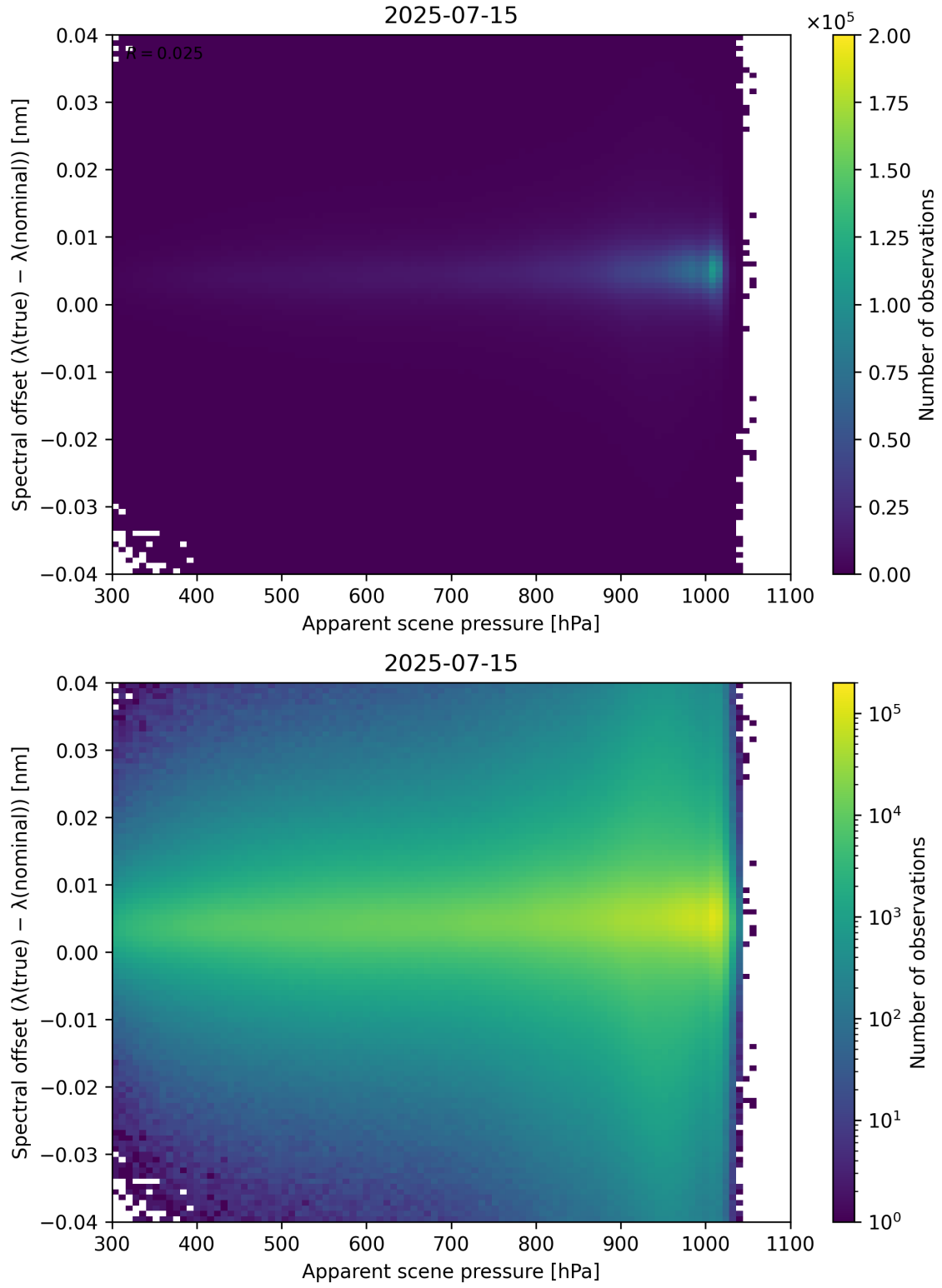
Figure 67: Scatter density plot of “Apparent scene pressure” against “Spectral offset ( \lambda_{\text{true}} - \lambda_{\text{nominal}} )” for 2025-07-14 to 2025-07-16.
