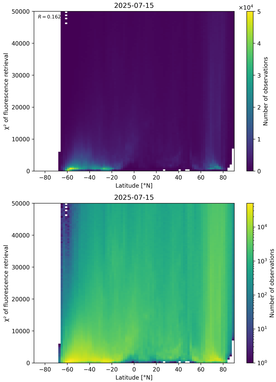
Figure 89: Scatter density plot of “Latitude” against “ \chi^2 of fluorescence retrieval” for 2025-07-14 to 2025-07-16.
