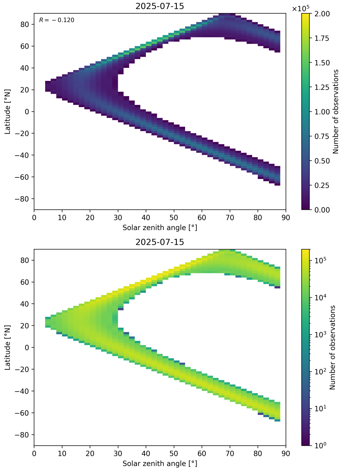
Figure 113: Scatter density plot of “Solar zenith angle” against “Latitude” for 2025-07-14 to 2025-07-16.
