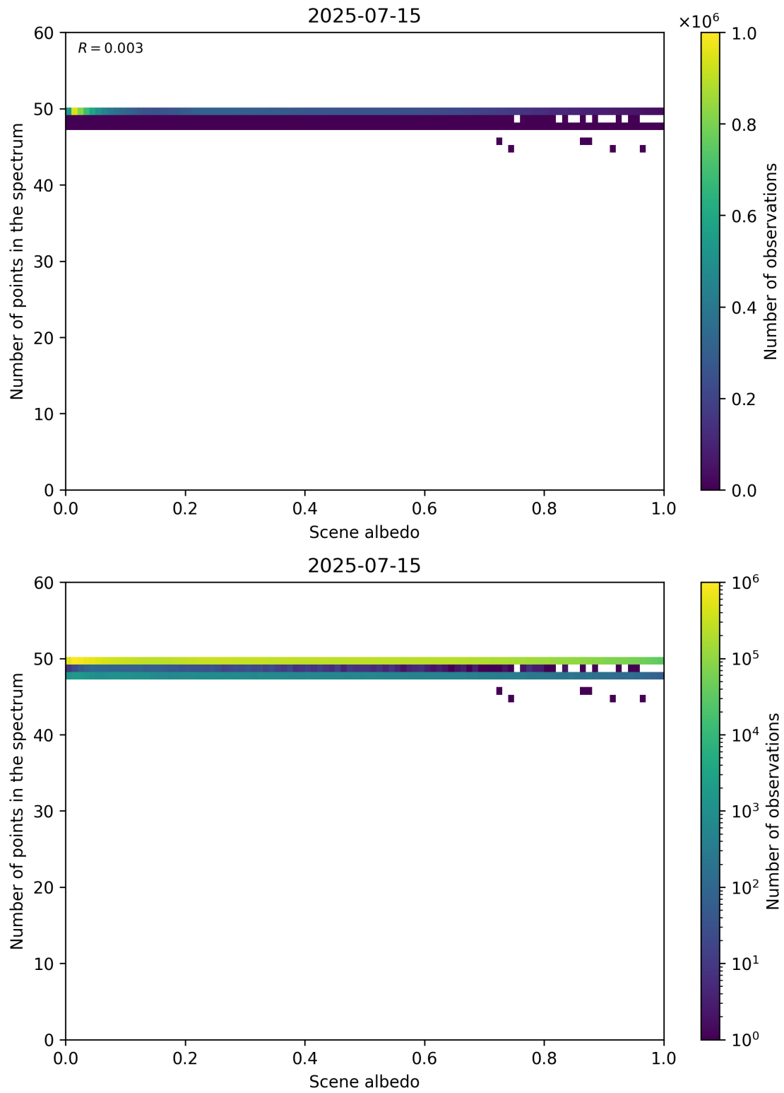
Figure 106: Scatter density plot of “Scene albedo” against “Number of points in the spectrum” for 2025-07-14 to 2025-07-16.
