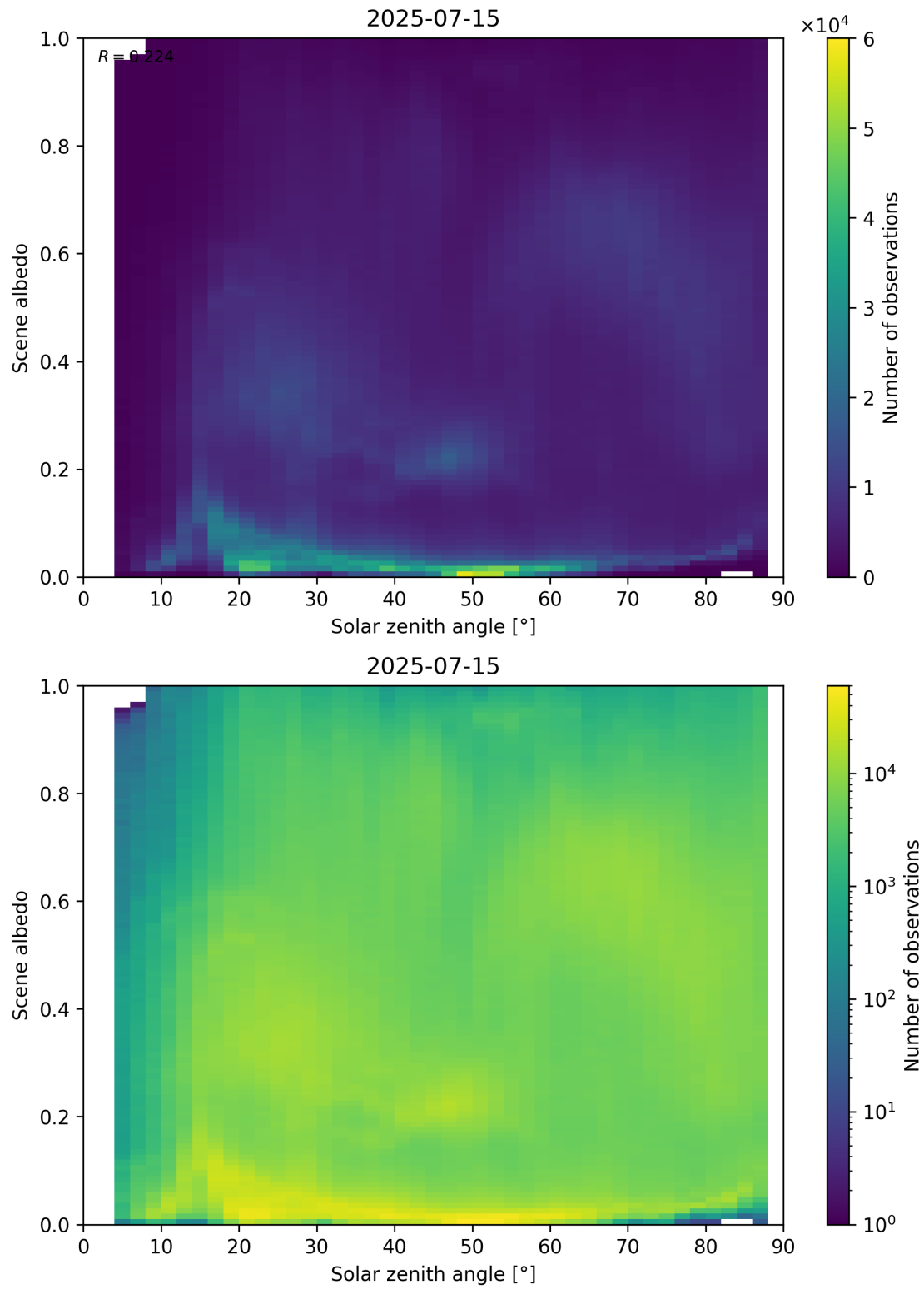
Figure 116: Scatter density plot of “Solar zenith angle” against “Scene albedo” for 2025-07-14 to 2025-07-16.
