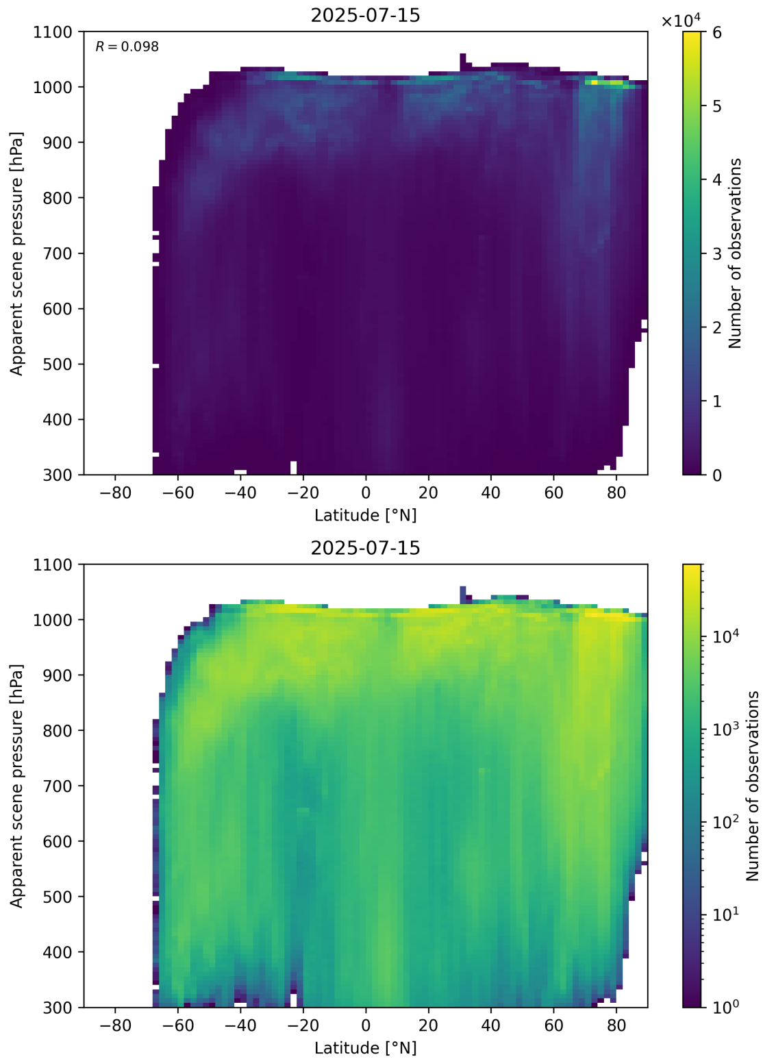
Figure 88: Scatter density plot of “Latitude” against “Apparent scene pressure” for 2025-07-14 to 2025-07-16.
