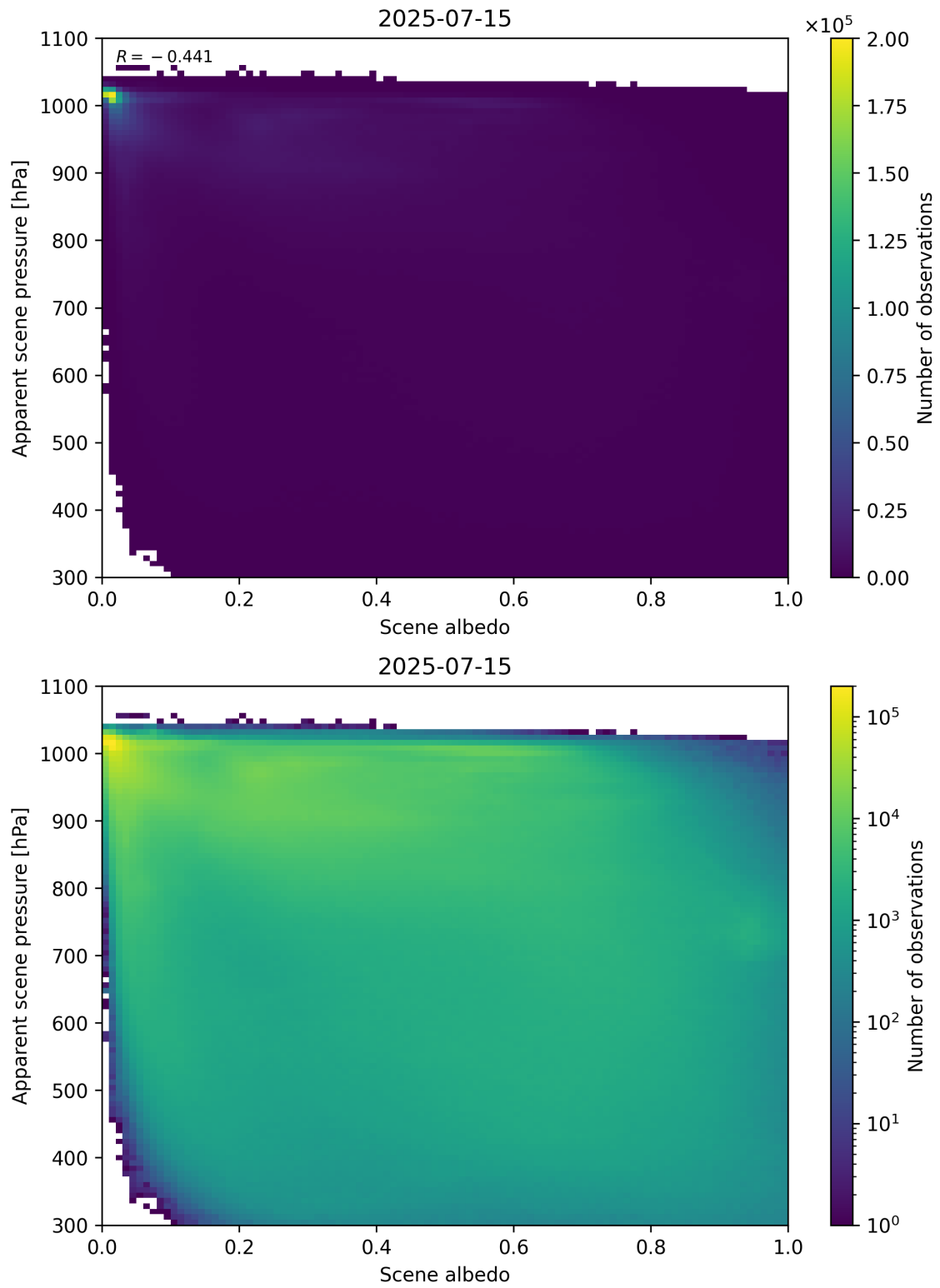
Figure 102: Scatter density plot of “Scene albedo” against “Apparent scene pressure” for 2025-07-14 to 2025-07-16.
