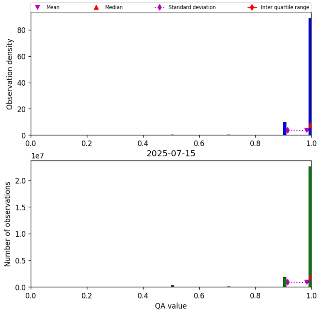
Figure 29: Histogram of “QA value” for 2025-07-14 to 2025-07-16
