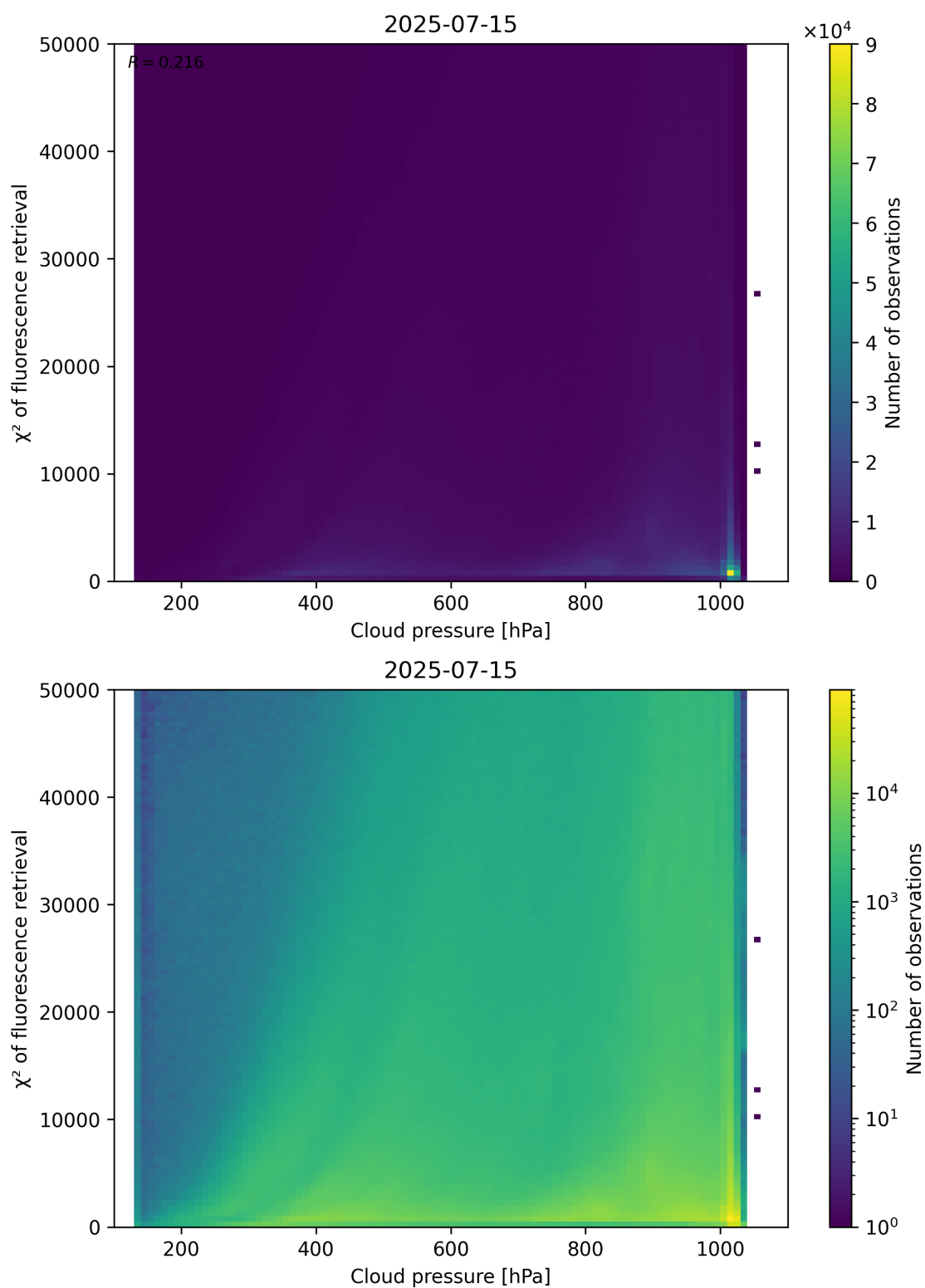
Figure 78: Scatter density plot of “Cloud pressure” against “ \chi^2 of fluorescence retrieval” for 2025-07-14 to 2025-07-16.
