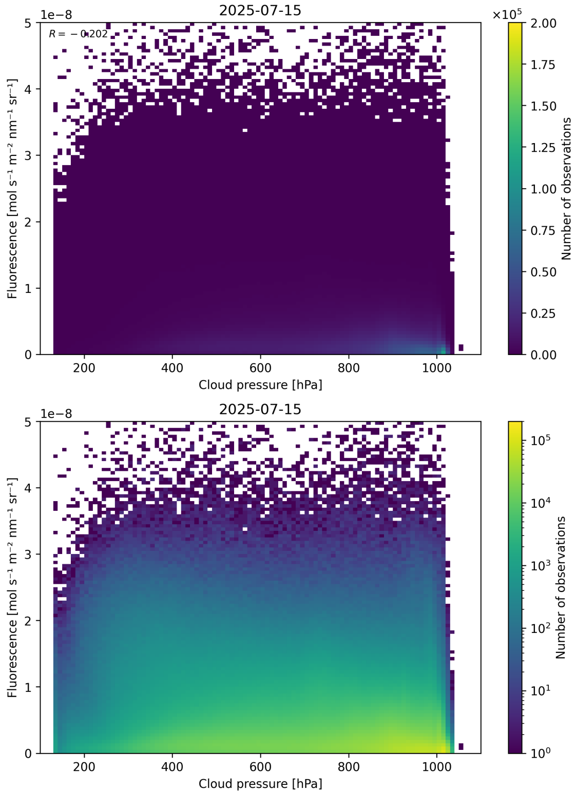
Figure 80: Scatter density plot of “Cloud pressure” against “Fluorescence” for 2025-07-14 to 2025-07-16.
