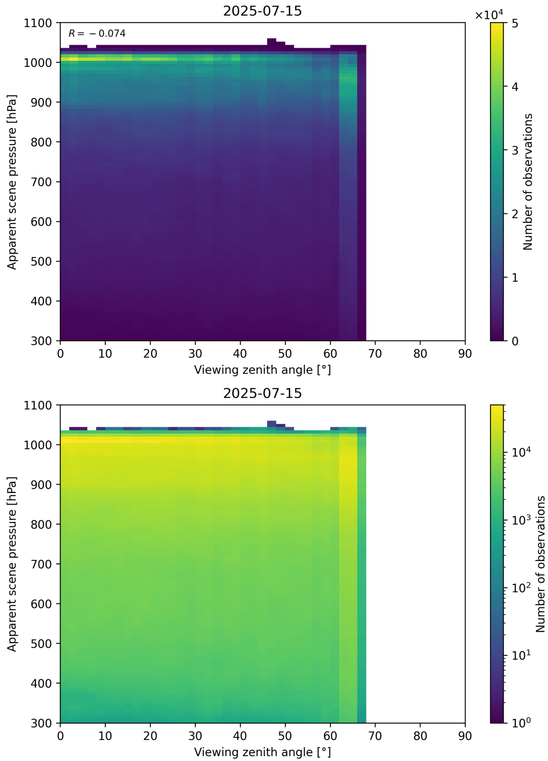
Figure 118: Scatter density plot of “Viewing zenith angle” against “Apparent scene pressure” for 2025-07-14 to 2025-07-16.
