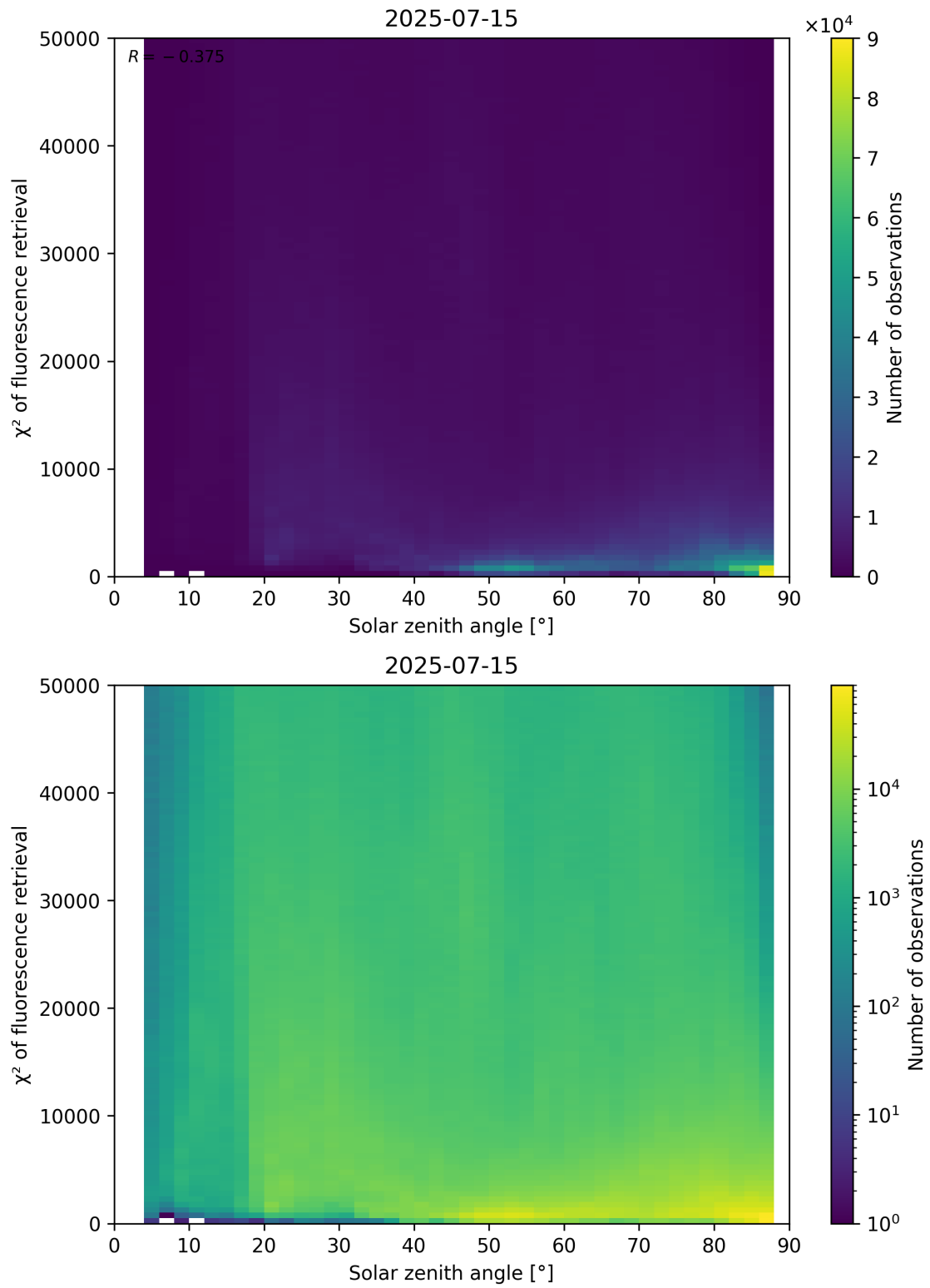
Figure 109: Scatter density plot of “Solar zenith angle” against “ \chi^2 of fluorescence retrieval” for 2025-07-14 to 2025-07-16.
