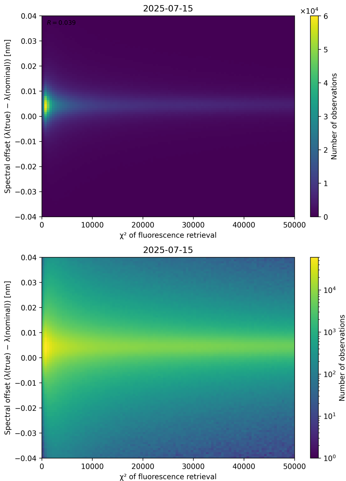
Figure 69: Scatter density plot of “ \chi^2 of fluorescence retrieval” against “Spectral offset ( \lambda_{\text{true}} - \lambda_{\text{nominal}} )” for 2025-07-14 to 2025-07-16.
