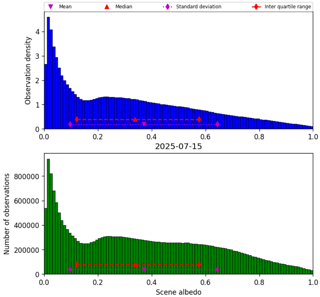
Figure 34: Histogram of “Scene albedo” for 2025-07-14 to 2025-07-16
