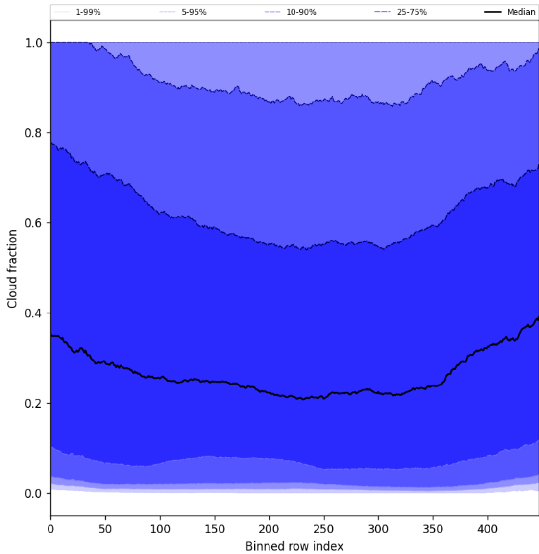
Figure 49: Along track statistics of “Cloud fraction” for 2025-07-14 to 2025-07-16
