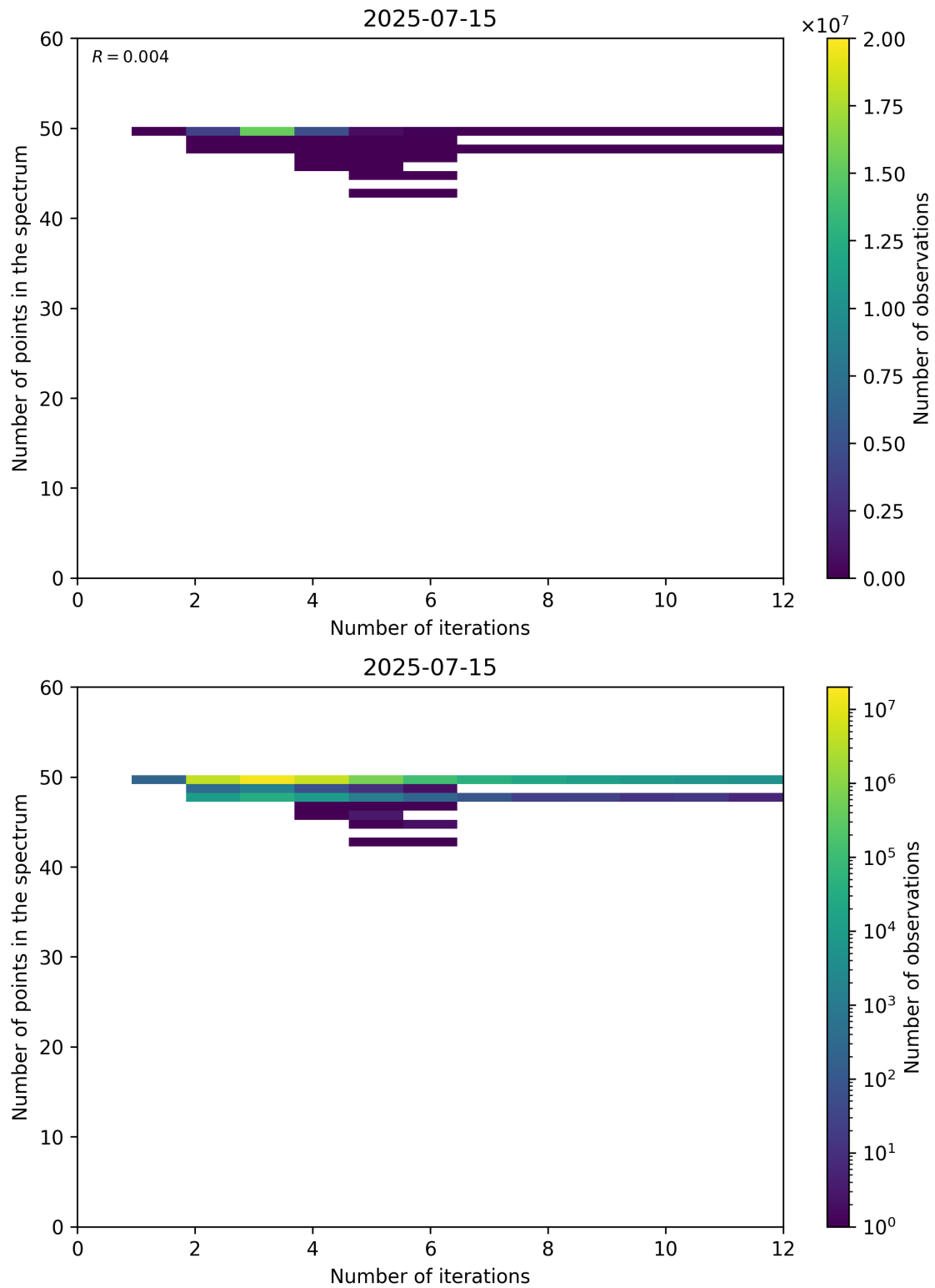
Figure 99: Scatter density plot of “Number of iterations” against “Number of points in the spectrum” for 2025-07-14 to 2025-07-16.
