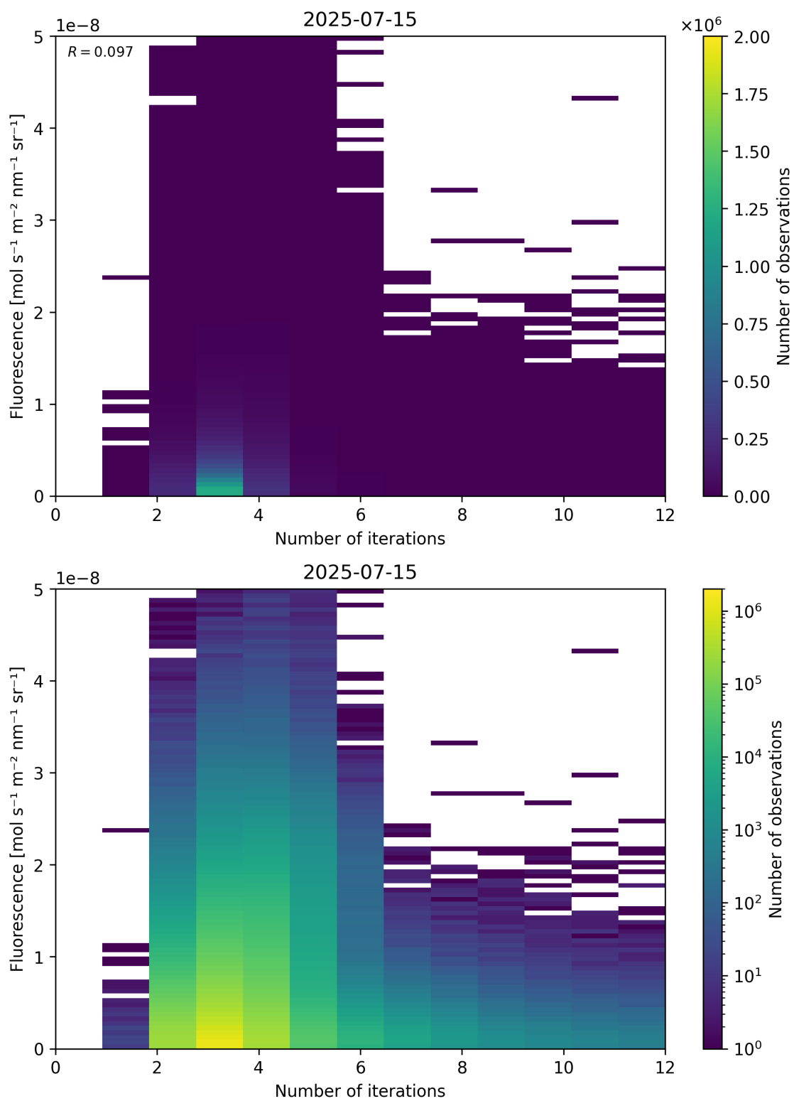
Figure 98: Scatter density plot of “Number of iterations” against “Fluorescence” for 2025-07-14 to 2025-07-16.
