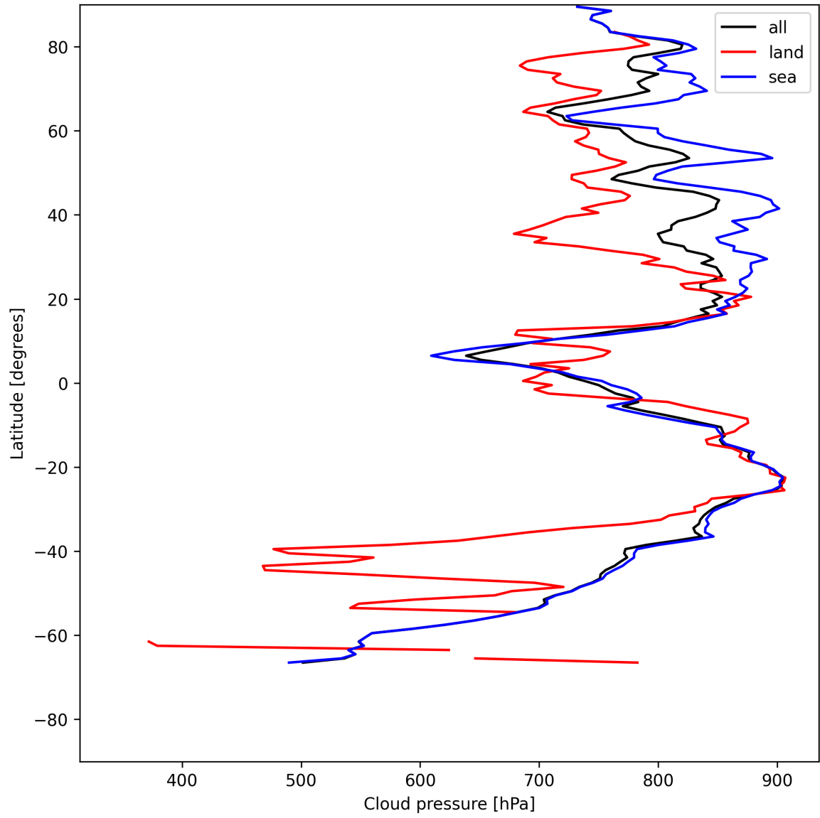
Figure 13: Zonal average of “Cloud pressure” for 2025-07-14 to 2025-07-16.
