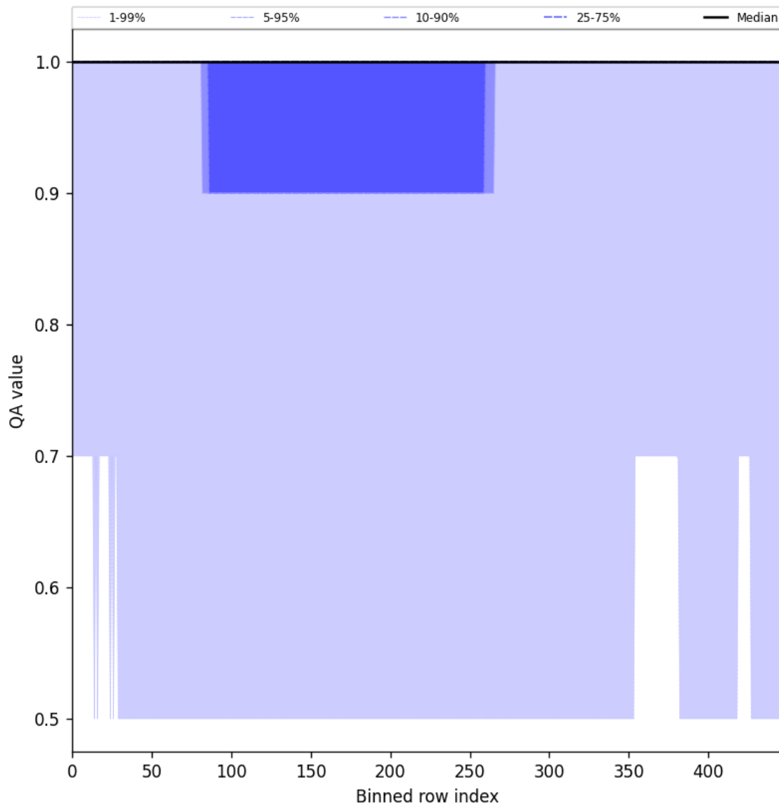
Figure 46: Along track statistics of “QA value” for 2025-07-14 to 2025-07-16
