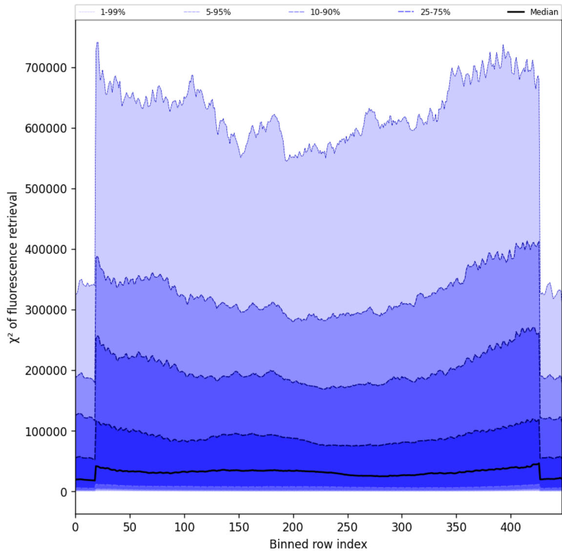
Figure 59: Along track statistics of “ \chi^2 of fluorescence retrieval” for 2025-07-14 to 2025-07-16
