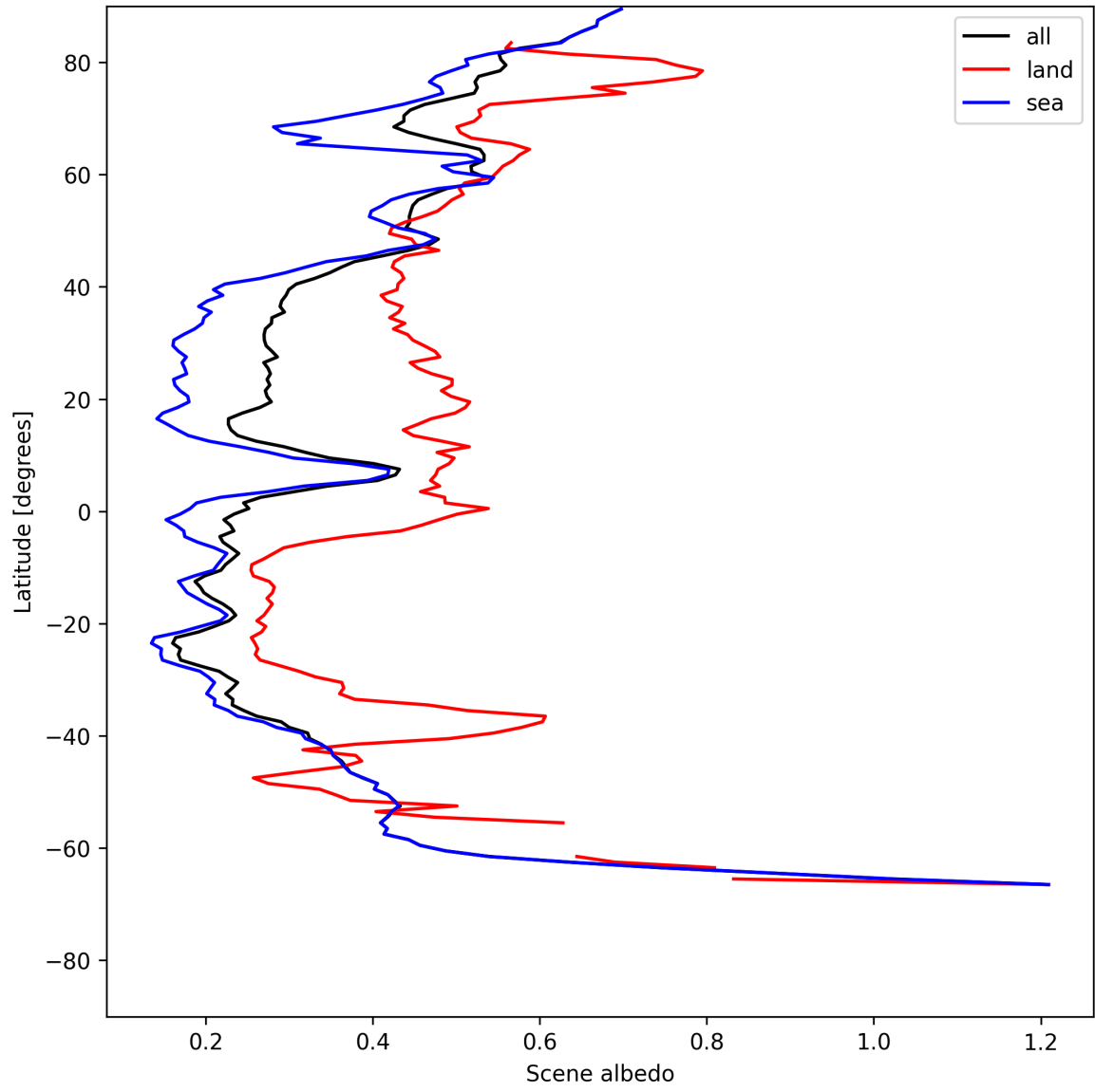
Figure 17: Zonal average of “Scene albedo” for 2025-07-14 to 2025-07-16.
