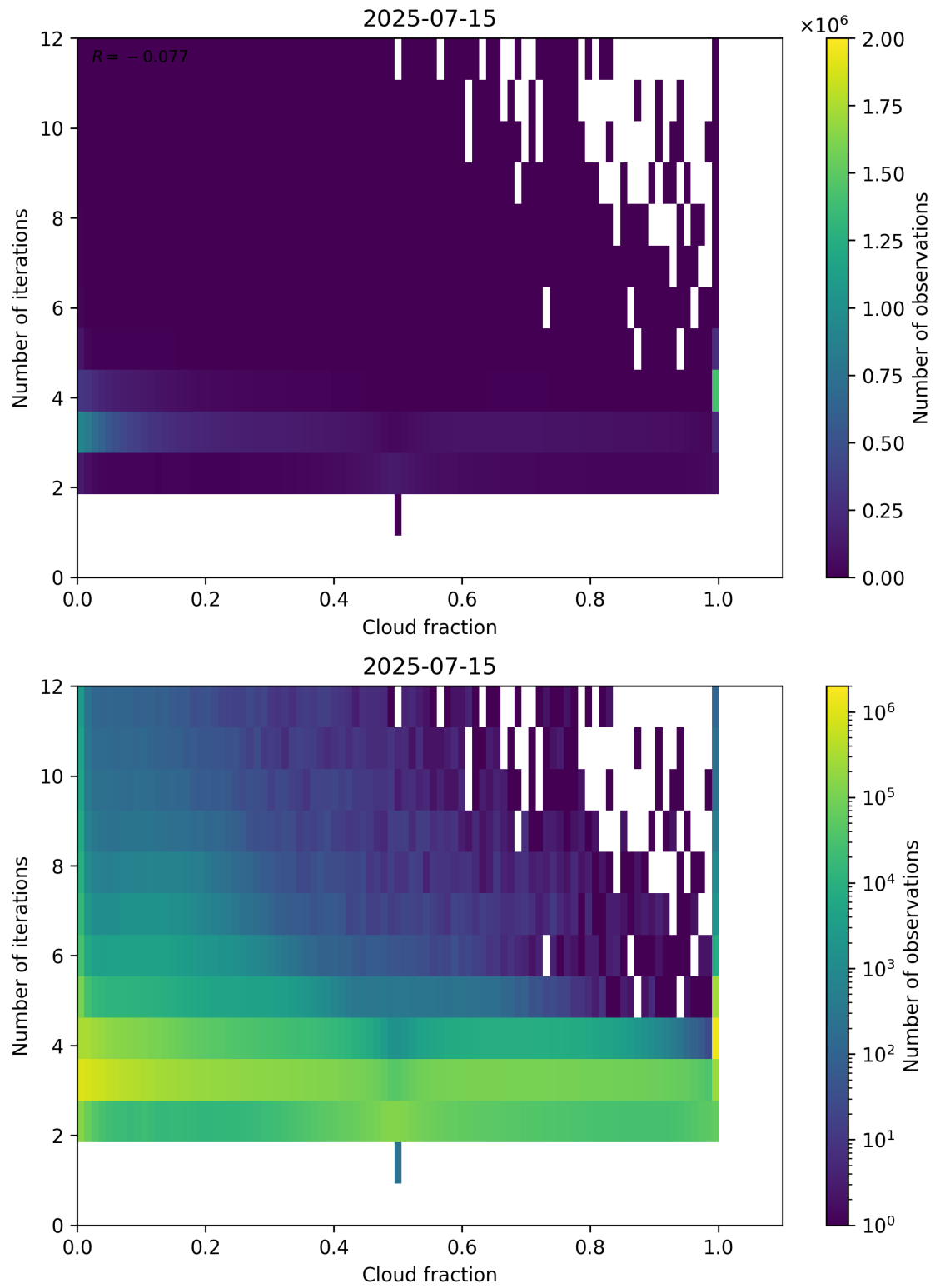
Figure 73: Scatter density plot of “Cloud fraction” against “Number of iterations” for 2025-07-14 to 2025-07-16.
