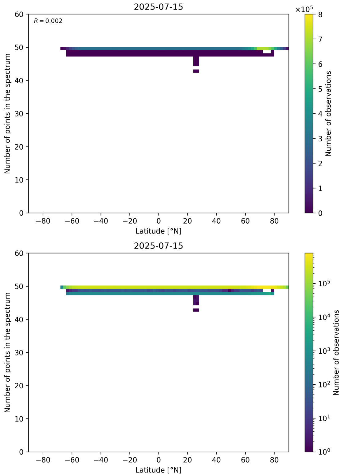
Figure 94: Scatter density plot of “Latitude” against “Number of points in the spectrum” for 2025-07-14 to 2025-07-16.
