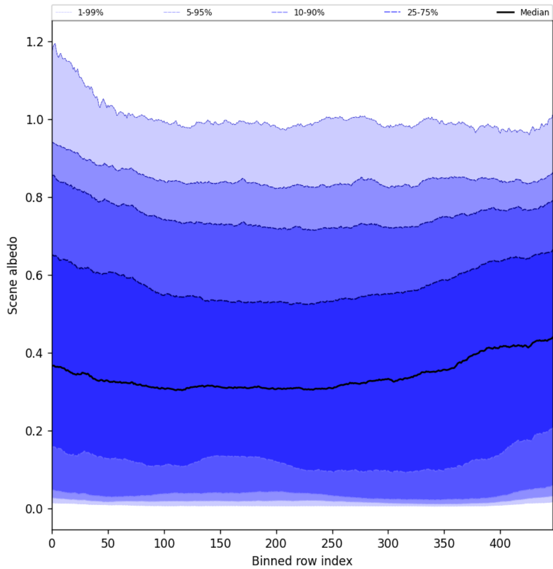
Figure 51: Along track statistics of “Scene albedo” for 2025-07-14 to 2025-07-16
