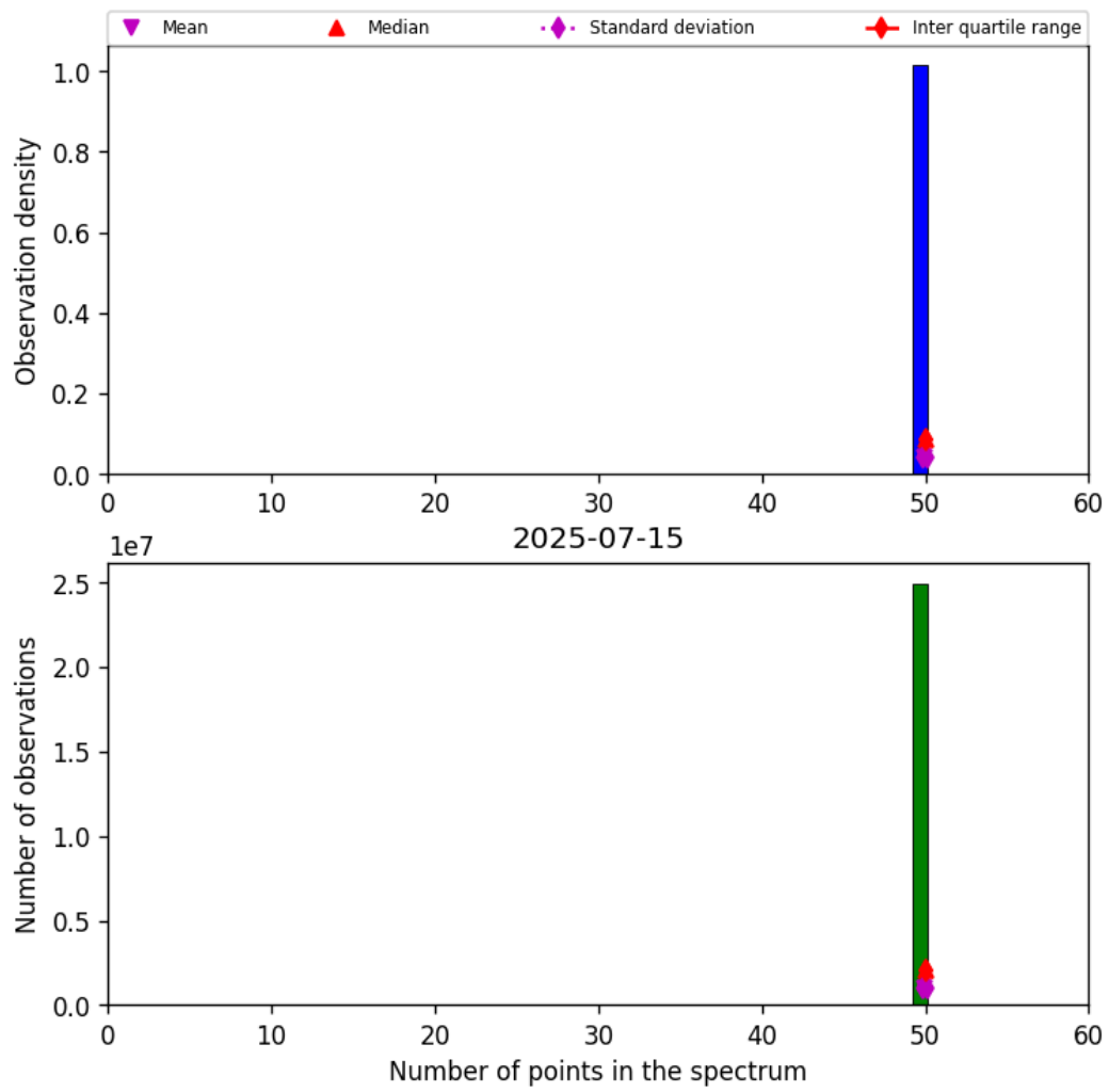
Figure 44: Histogram of “Number of points in the spectrum” for 2025-07-14 to 2025-07-16
