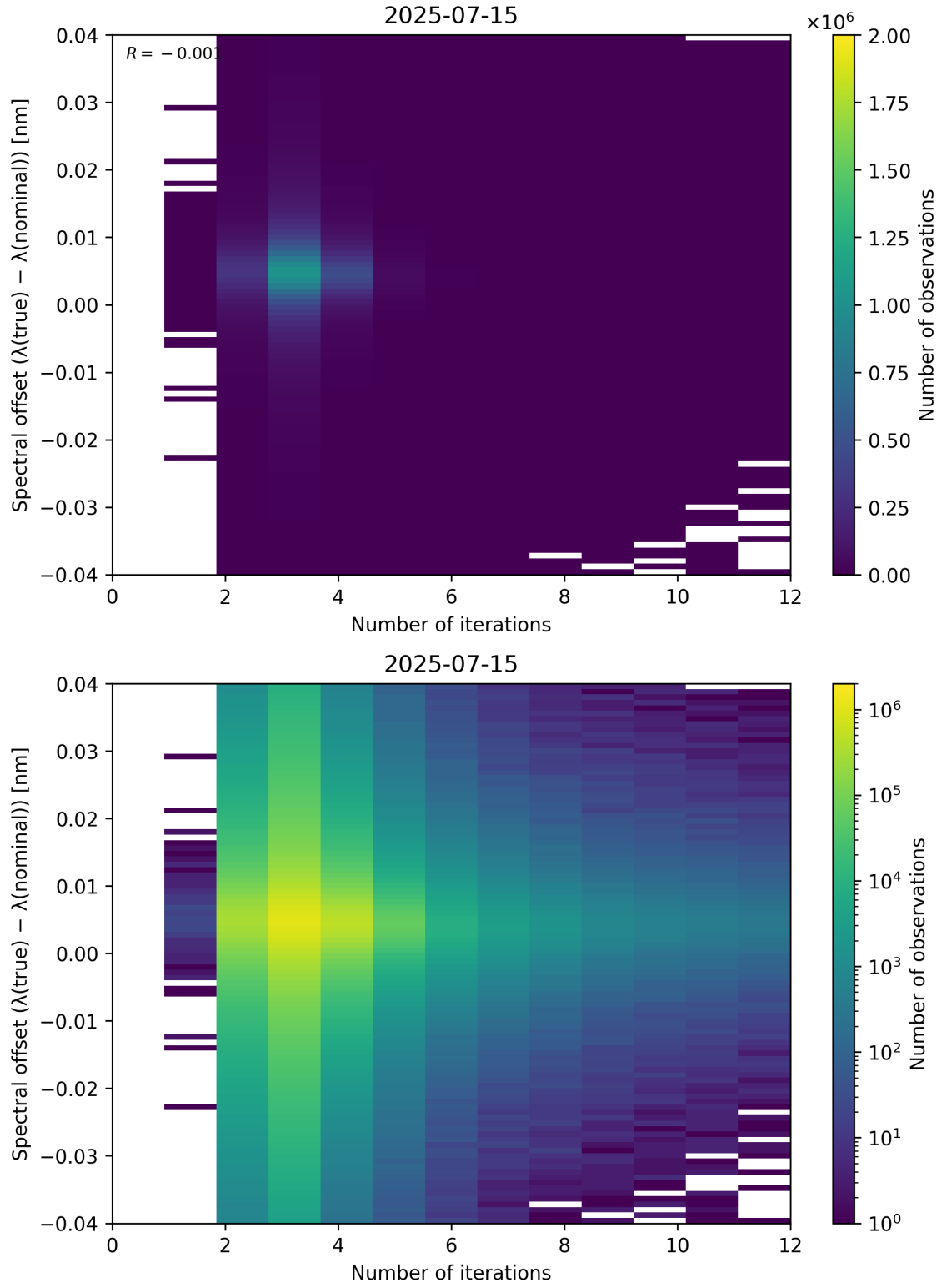
Figure 100: Scatter density plot of “Number of iterations” against “Spectral offset ( \lambda_{\text{true}} - \lambda_{\text{nominal}} )” for 2025-07-14 to 2025-07-16.
