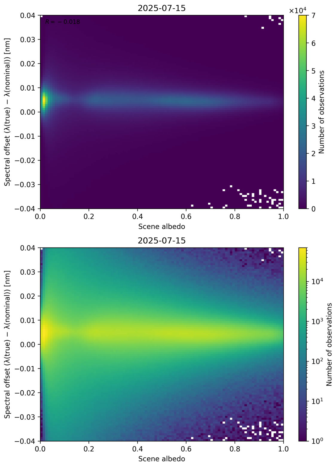
Figure 107: Scatter density plot of “Scene albedo” against “Spectral offset ( \lambda_{\text{true}} - \lambda_{\text{nominal}} )” for 2025-07-14 to 2025-07-16.
