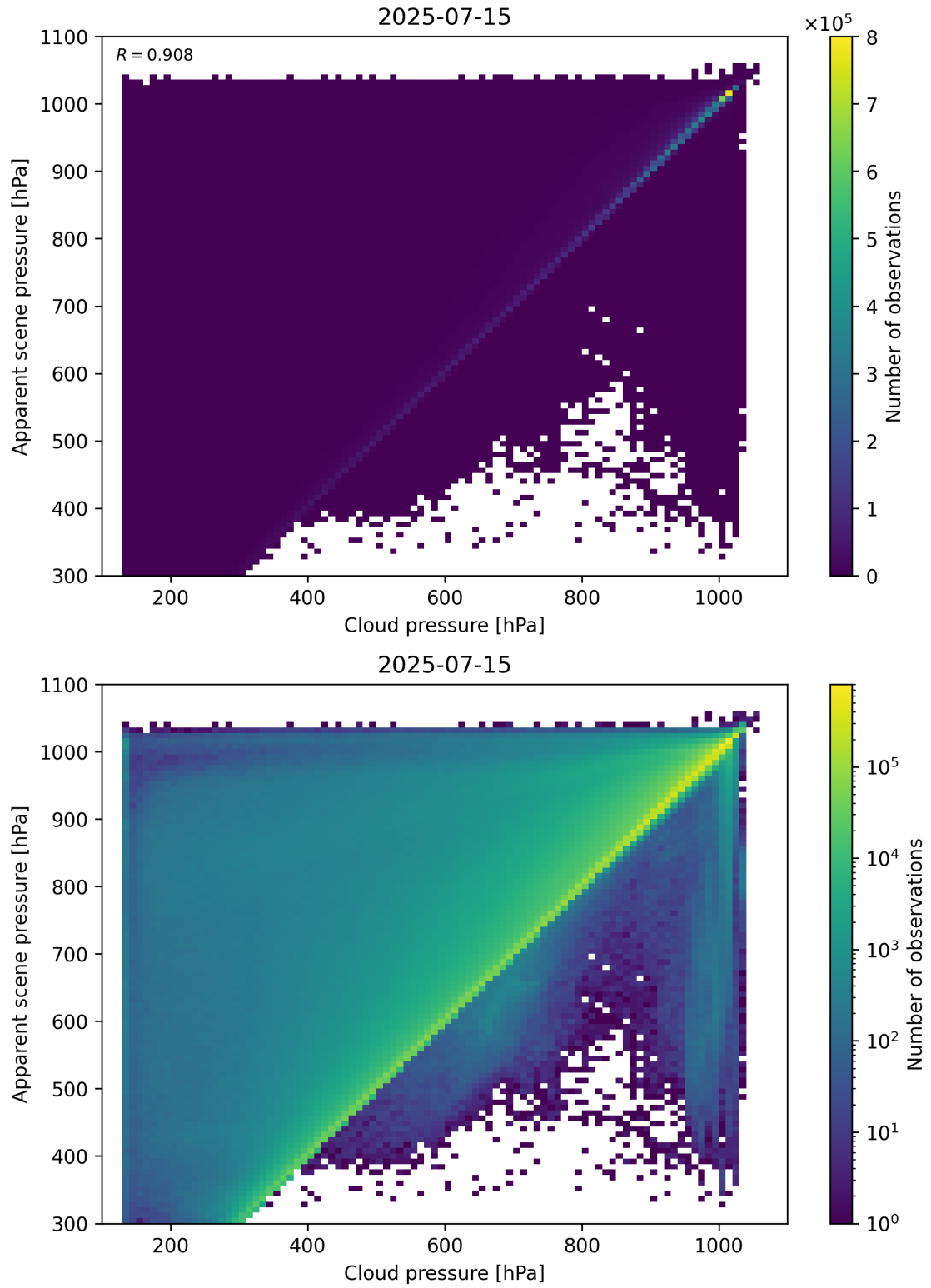
Figure 77: Scatter density plot of “Cloud pressure” against “Apparent scene pressure” for 2025-07-14 to 2025-07-16.
