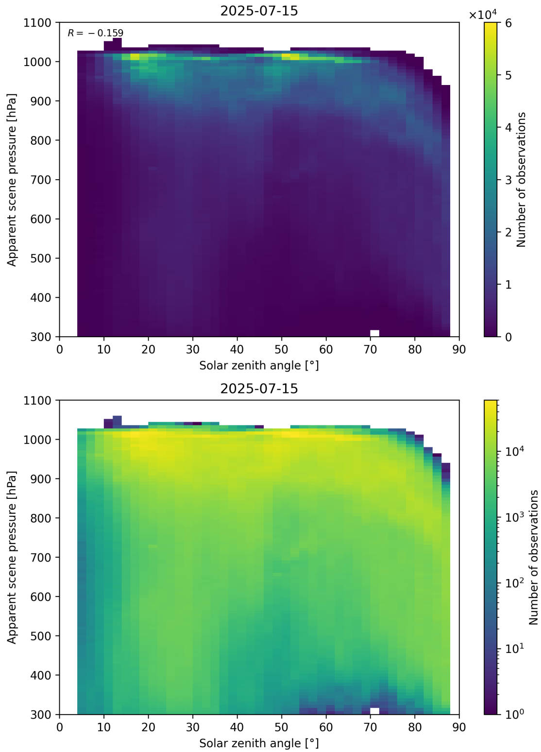
Figure 108: Scatter density plot of “Solar zenith angle” against “Apparent scene pressure” for 2025-07-14 to 2025-07-16.
