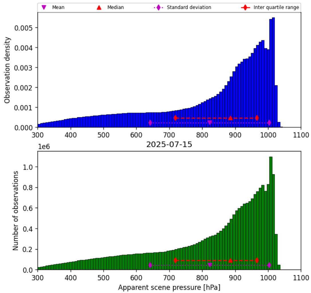
Figure 36: Histogram of “Apparent scene pressure” for 2025-07-14 to 2025-07-16
