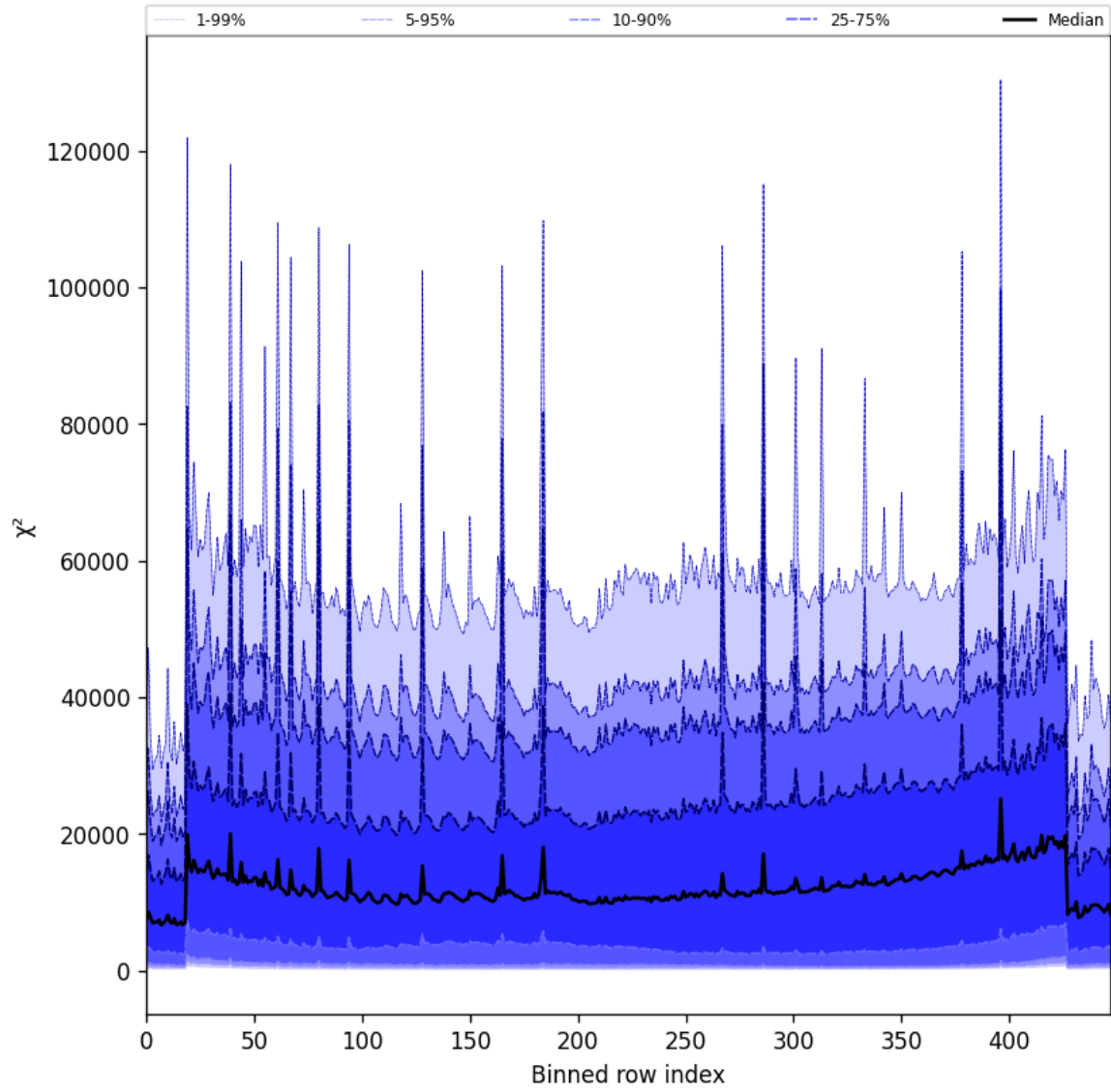
Figure 55: Along track statistics of “ \chi^2 ” for 2025-07-14 to 2025-07-16
