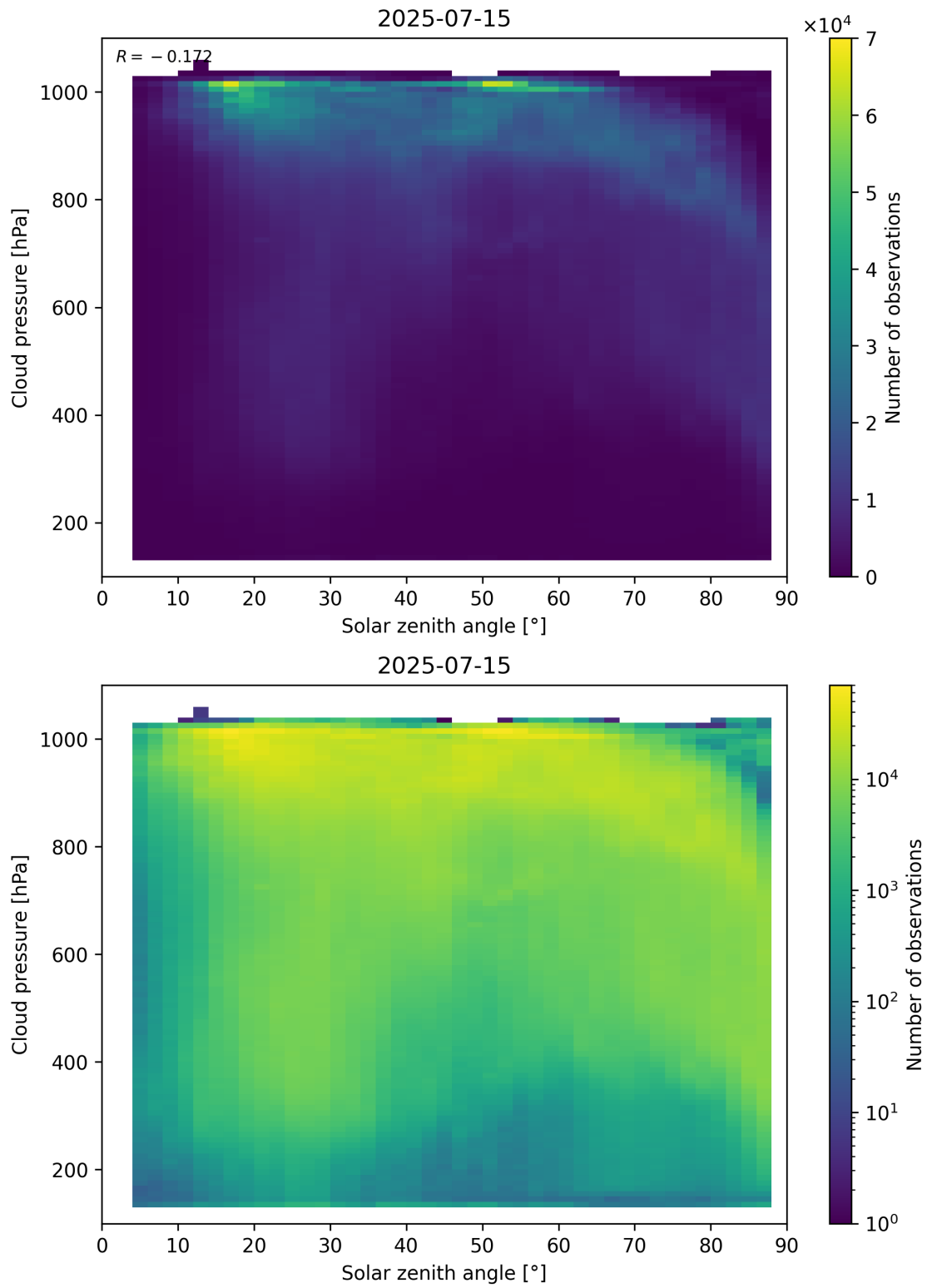
Figure 111: Scatter density plot of “Solar zenith angle” against “Cloud pressure” for 2025-07-14 to 2025-07-16.
