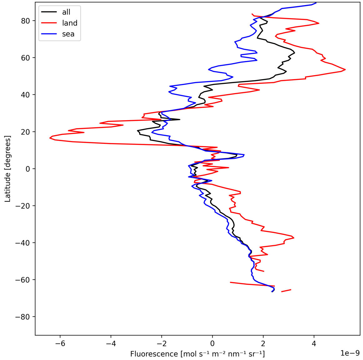
Figure 23: Zonal average of “Fluorescence” for 2025-07-14 to 2025-07-16.
