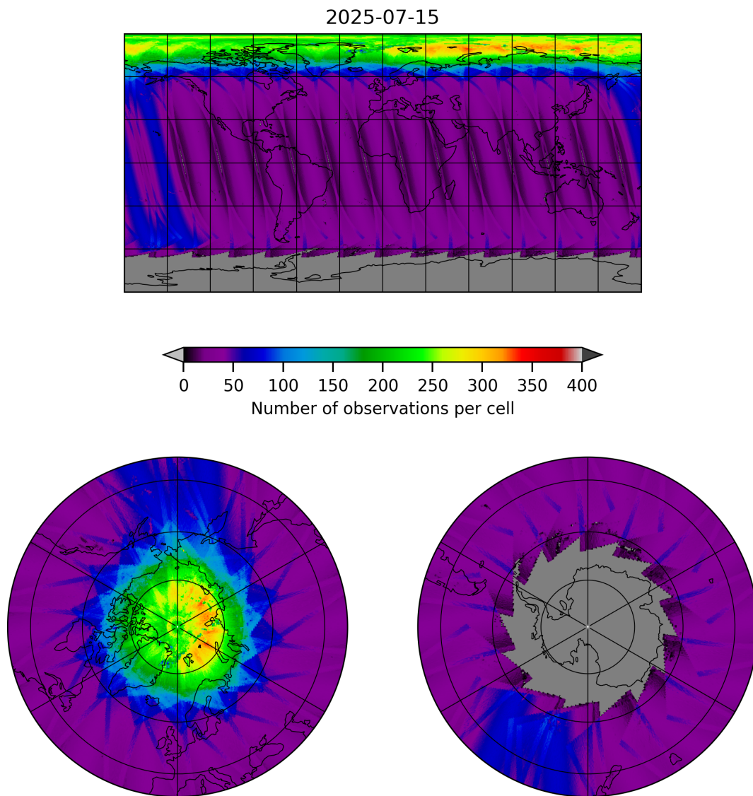
Figure 11: Map of the number of observations for 2025-07-14 to 2025-07-16
