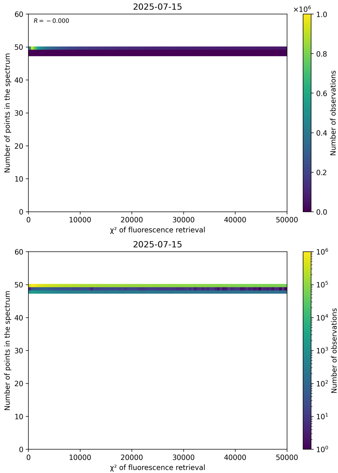
Figure 68: Scatter density plot of " \chi^2 of fluorescence retrieval" against "Number of points in the spectrum" for 2025-07-14 to 2025-07-16.
