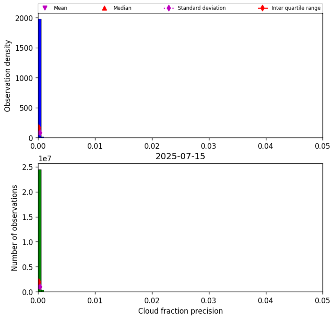
Figure 33: Histogram of “Cloud fraction precision” for 2025-07-14 to 2025-07-16
