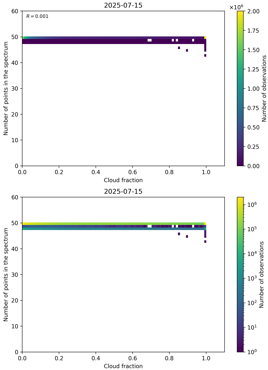
Figure 74: Scatter density plot of “Cloud fraction” against “Number of points in the spectrum” for 2025-07-14 to 2025-07-16.
