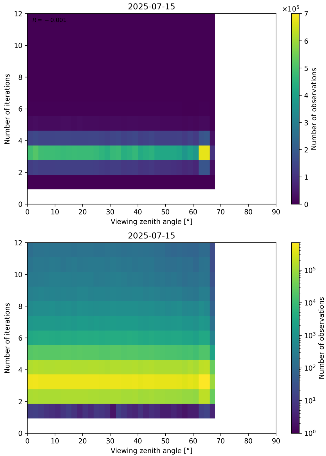
Figure 124: Scatter density plot of “Viewing zenith angle” against “Number of iterations” for 2025-07-14 to 2025-07-16.
