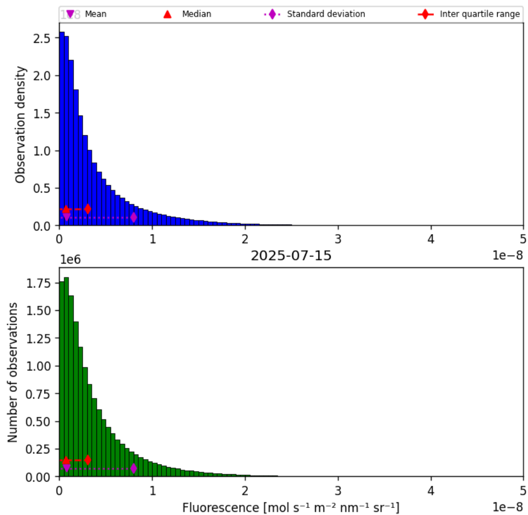
Figure 40: Histogram of “Fluorescence” for 2025-07-14 to 2025-07-16
