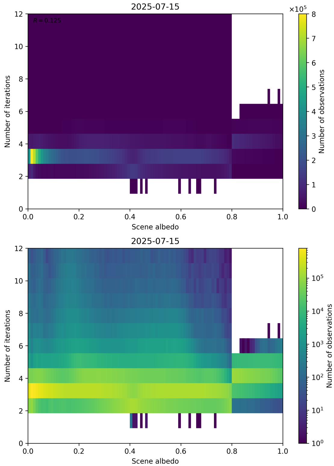
Figure 105: Scatter density plot of “Scene albedo” against “Number of iterations” for 2025-07-14 to 2025-07-16.
