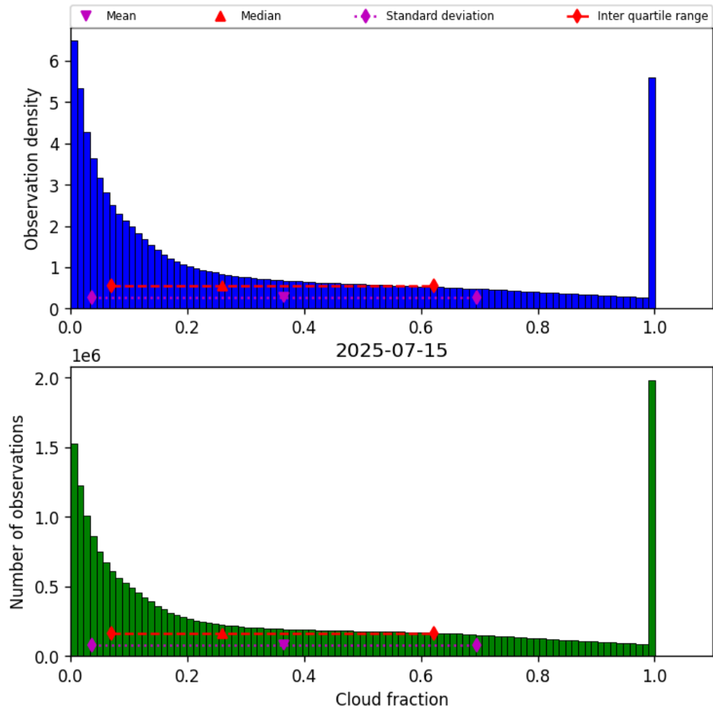
Figure 32: Histogram of “Cloud fraction” for 2025-07-14 to 2025-07-16
