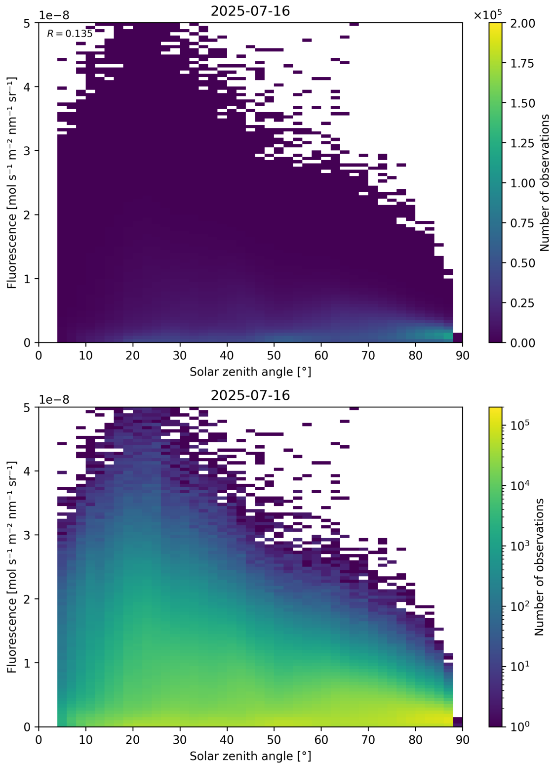
Figure 112: Scatter density plot of “Solar zenith angle” against “Fluorescence” for 2025-07-15 to 2025-07-17.
