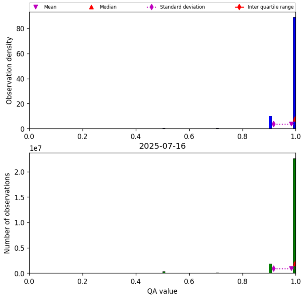
Figure 29: Histogram of “QA value” for 2025-07-15 to 2025-07-17
