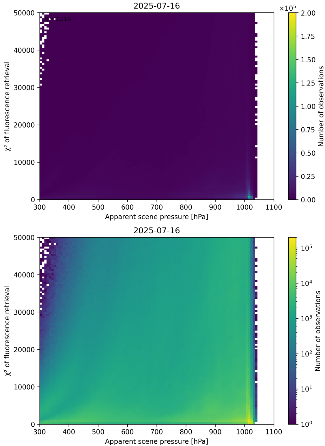
Figure 63: Scatter density plot of “Apparent scene pressure” against “ \chi^2 of fluorescence retrieval” for 2025-07-15 to 2025-07-17.
