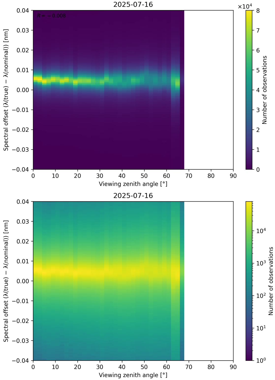
Figure 128: Scatter density plot of “Viewing zenith angle” against “Spectral offset ( \lambda_{\text{true}} - \lambda_{\text{nominal}} )” for 2025-07-15 to 2025-07-17.
