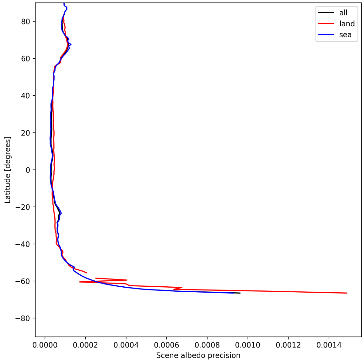
Figure 18: Zonal average of “Scene albedo precision” for 2025-07-15 to 2025-07-17.
