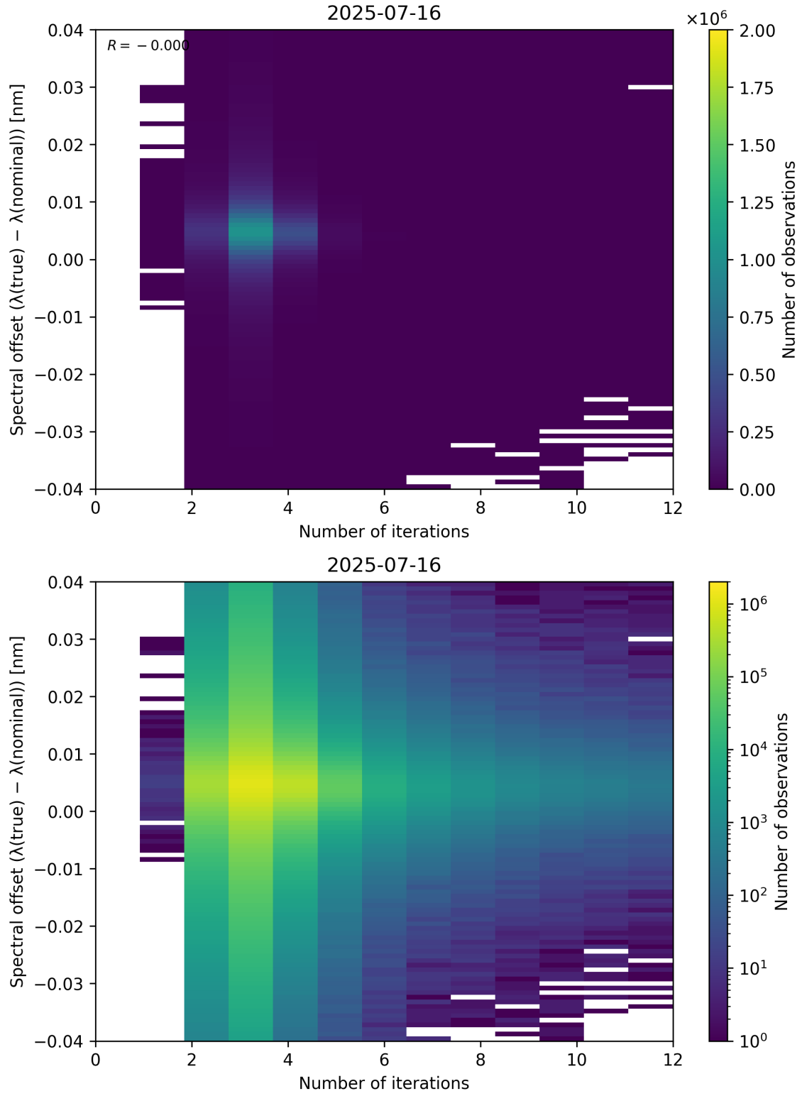
Figure 100: Scatter density plot of “Number of iterations” against “Spectral offset ( \lambda_{\text{true}} - \lambda_{\text{nominal}} )” for 2025-07-15 to 2025-07-17.
