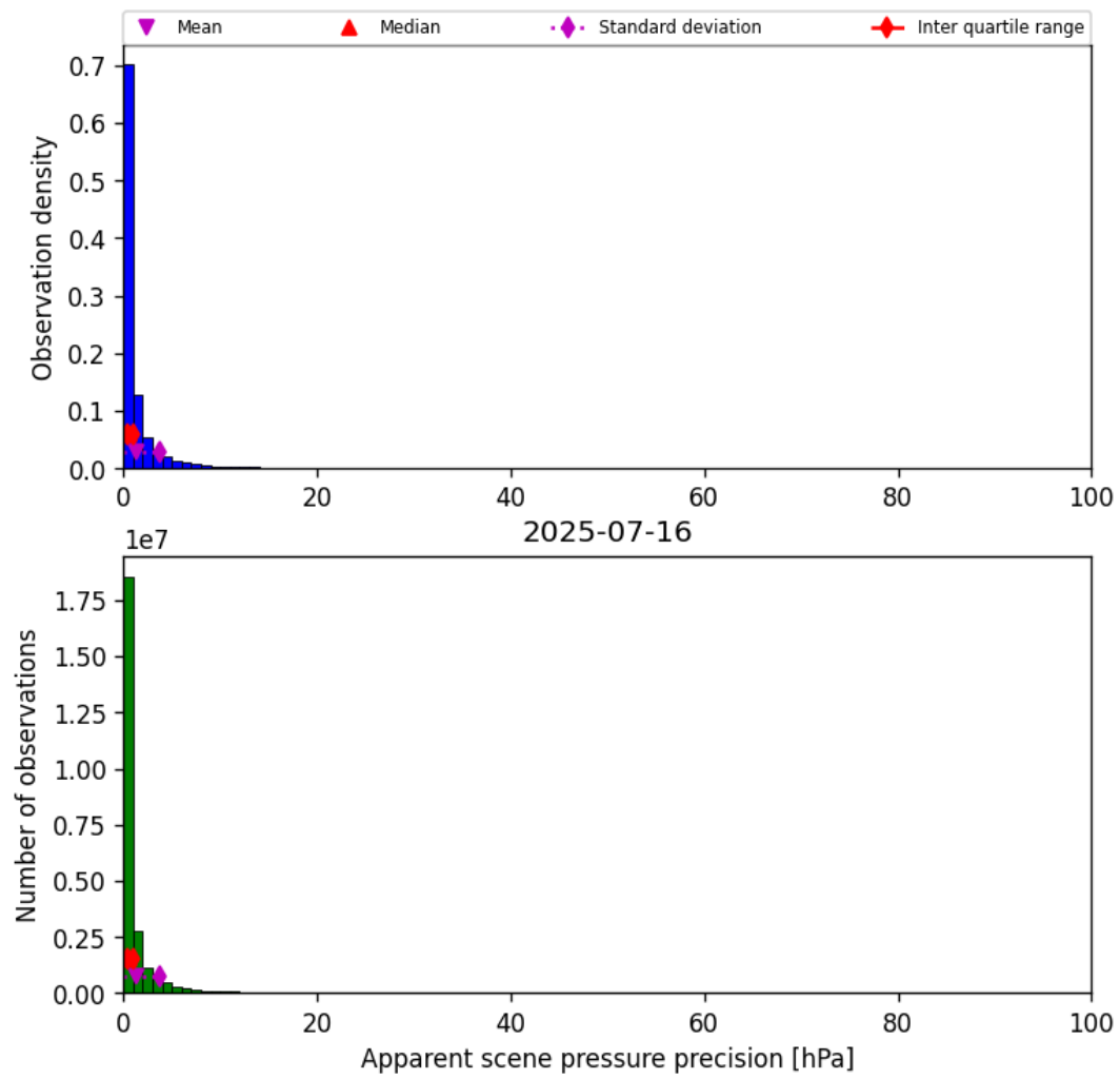
Figure 37: Histogram of “Apparent scene pressure precision” for 2025-07-15 to 2025-07-17
