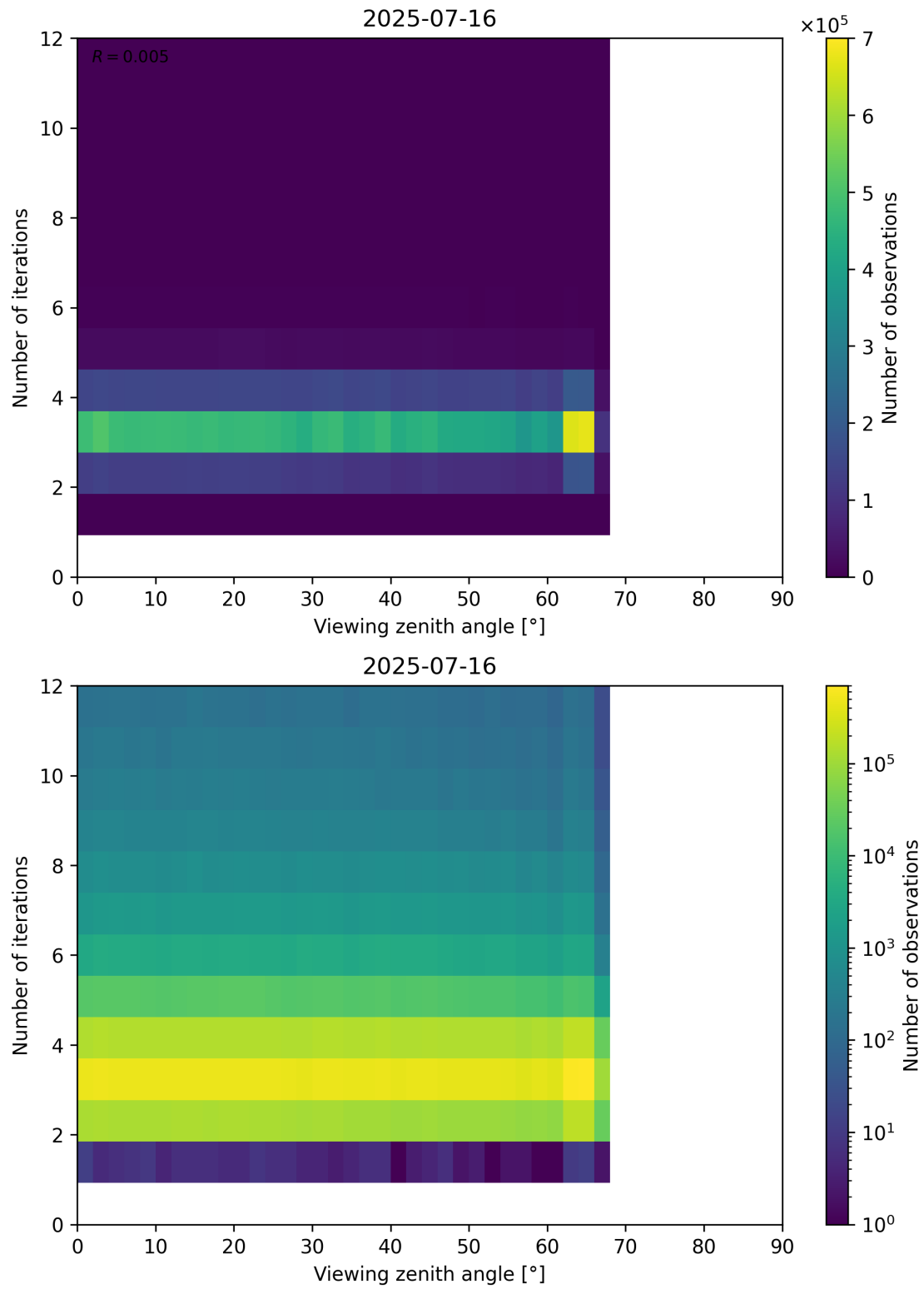
Figure 124: Scatter density plot of “Viewing zenith angle” against “Number of iterations” for 2025-07-15 to 2025-07-17.
