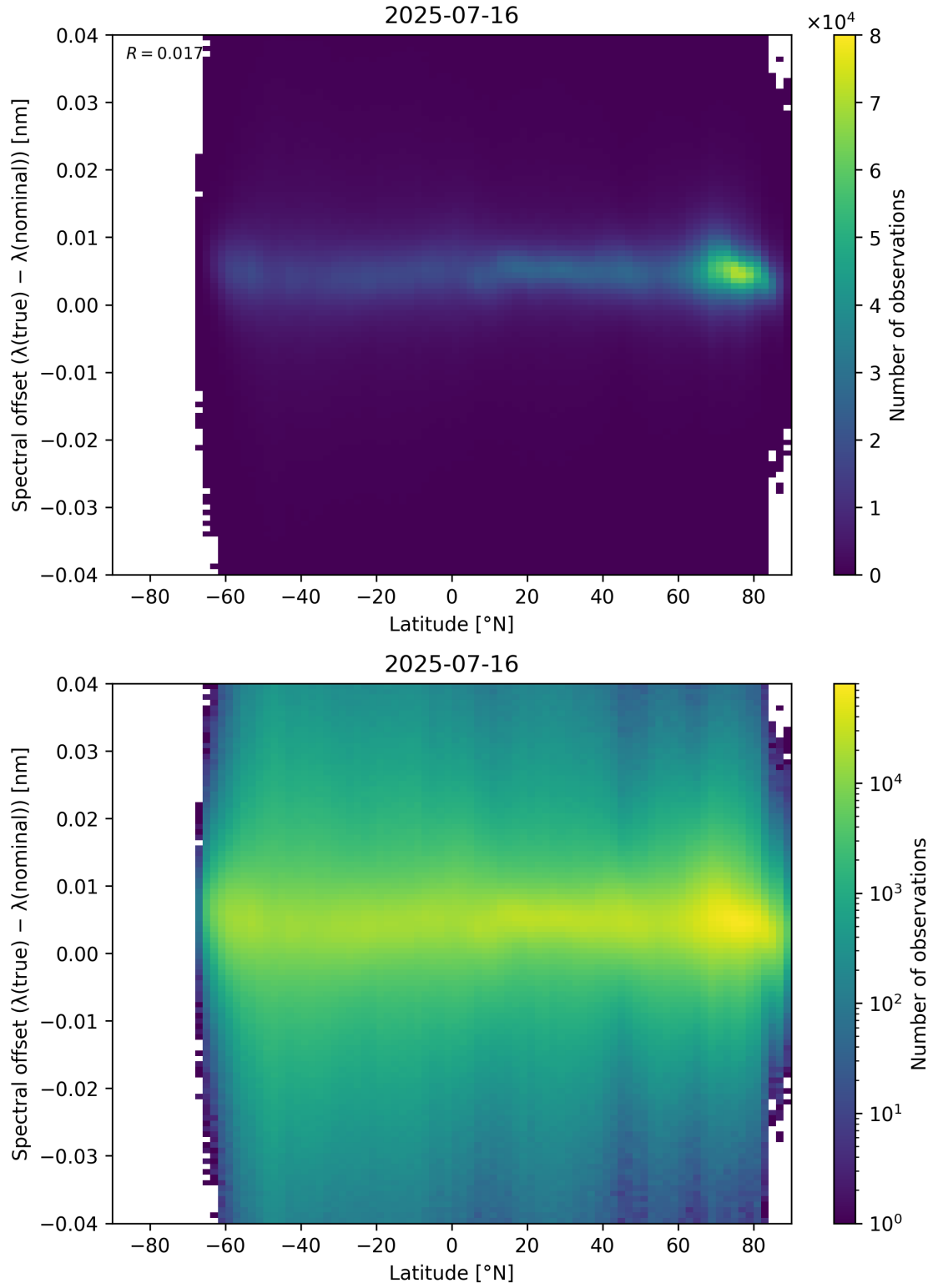
Figure 96: Scatter density plot of “Latitude” against “Spectral offset ( \lambda_{\text{true}} - \lambda_{\text{nominal}} )” for 2025-07-15 to 2025-07-17.
