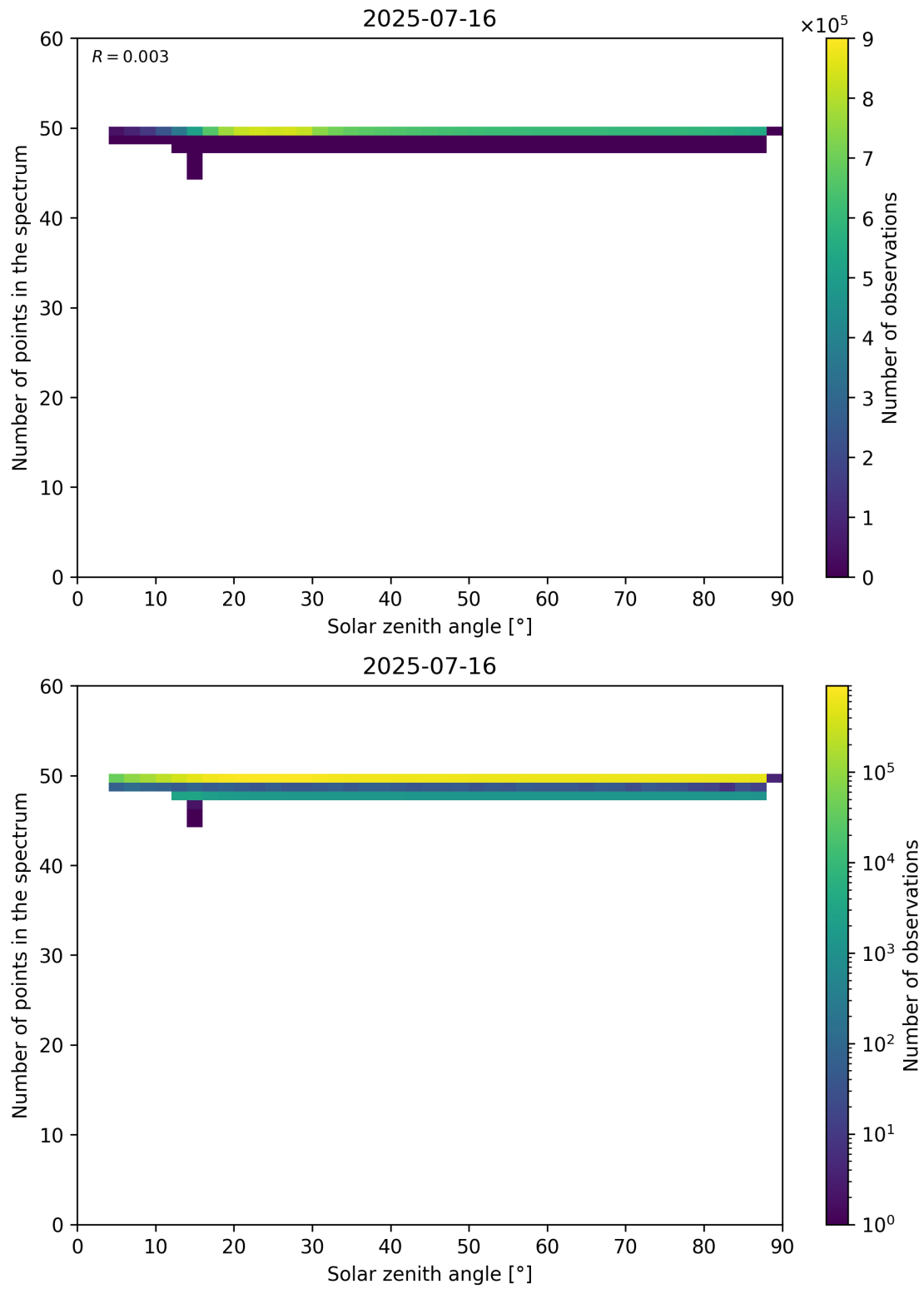
Figure 115: Scatter density plot of “Solar zenith angle” against “Number of points in the spectrum” for 2025-07-15 to 2025-07-17.
