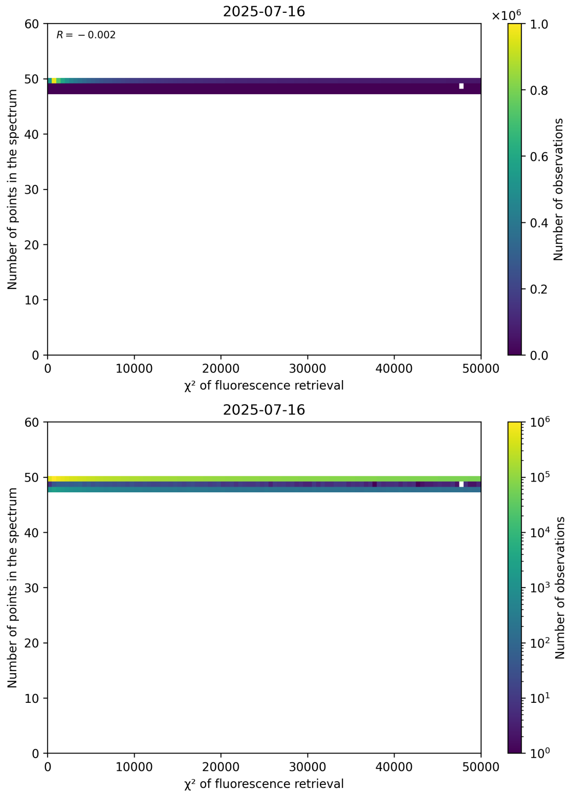
Figure 68: Scatter density plot of " \chi^2 of fluorescence retrieval" against "Number of points in the spectrum" for 2025-07-15 to 2025-07-17.
