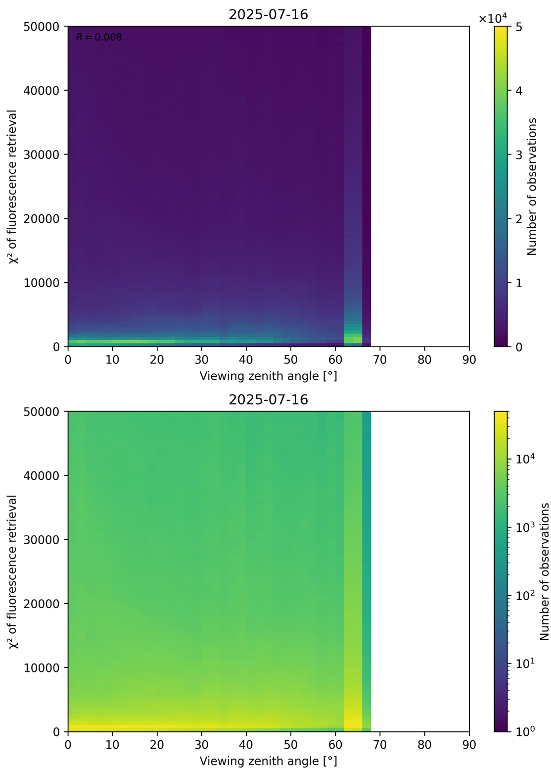
Figure 119: Scatter density plot of “Viewing zenith angle” against “ \chi^2 of fluorescence retrieval” for 2025-07-15 to 2025-07-17.
