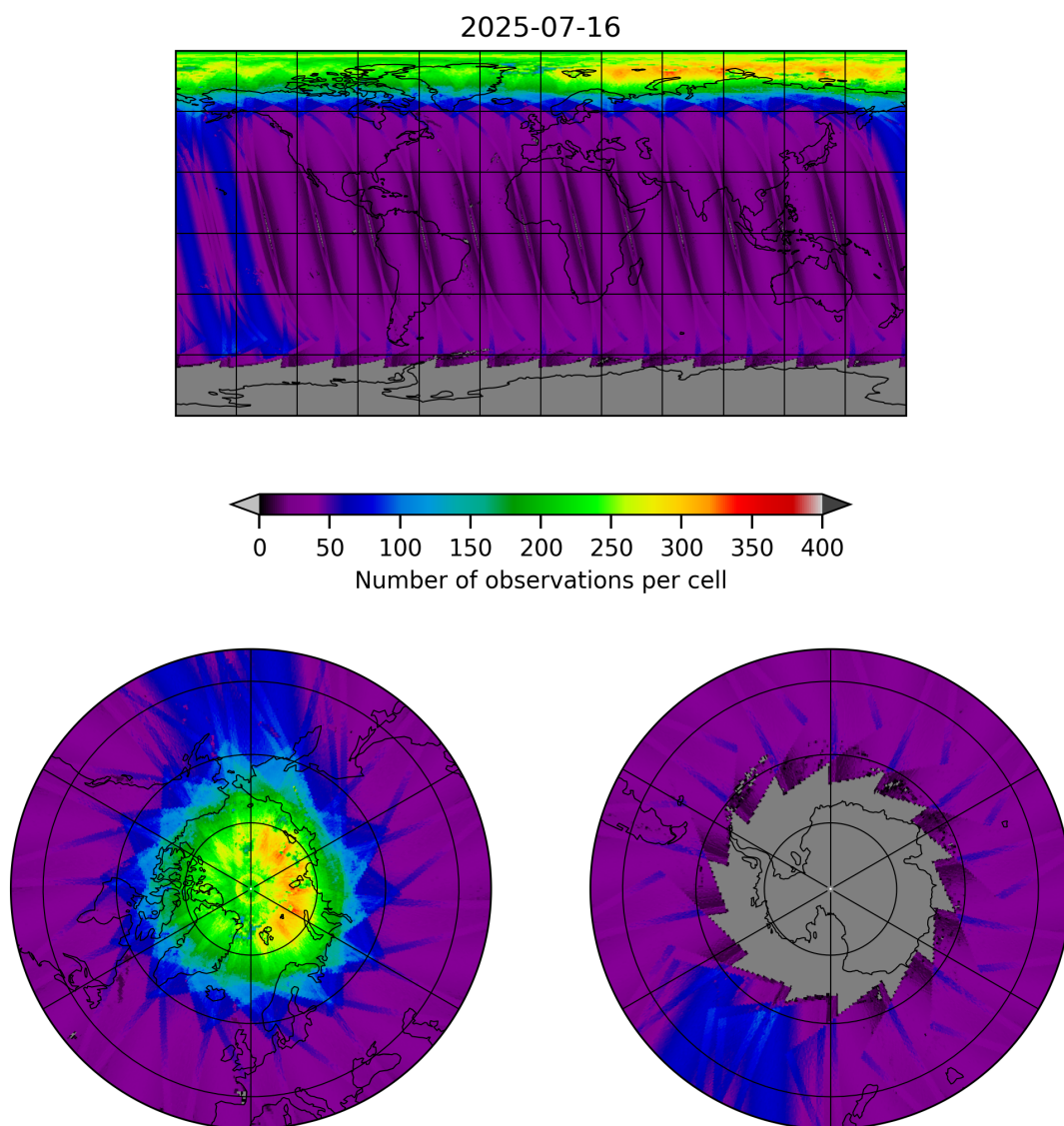
Figure 11: Map of the number of observations for 2025-07-15 to 2025-07-17
