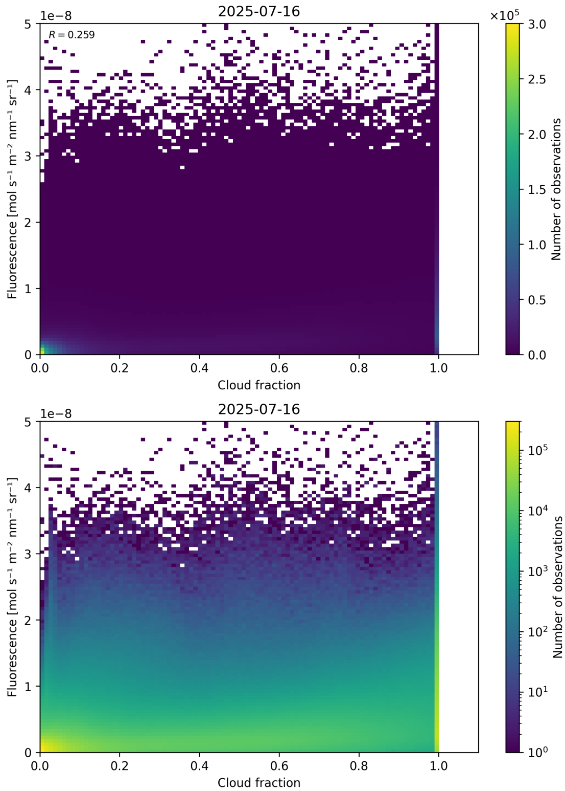
Figure 72: Scatter density plot of “Cloud fraction” against “Fluorescence” for 2025-07-15 to 2025-07-17.
