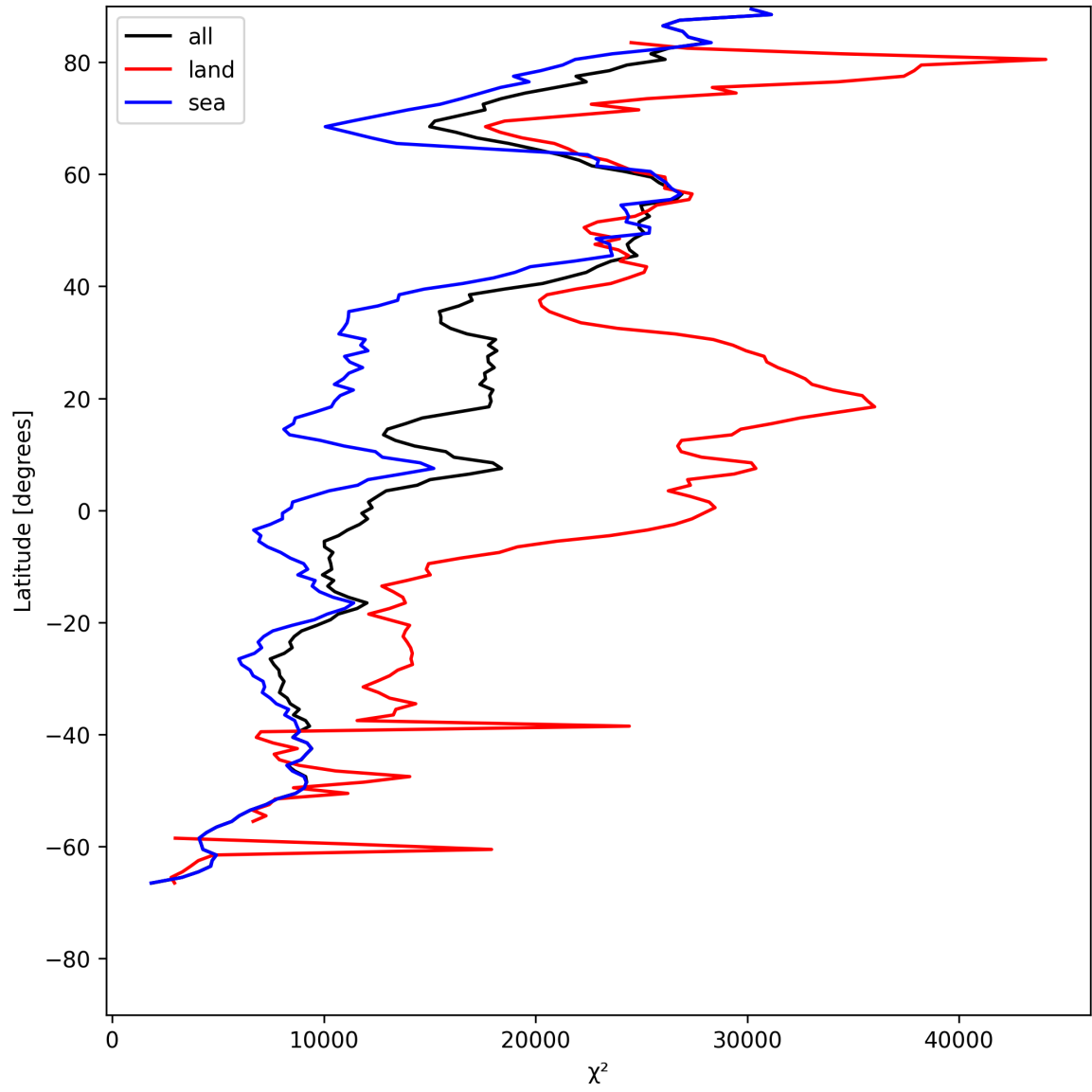
Figure 21: Zonal average of “ \chi^2 ” for 2025-07-15 to 2025-07-17.
