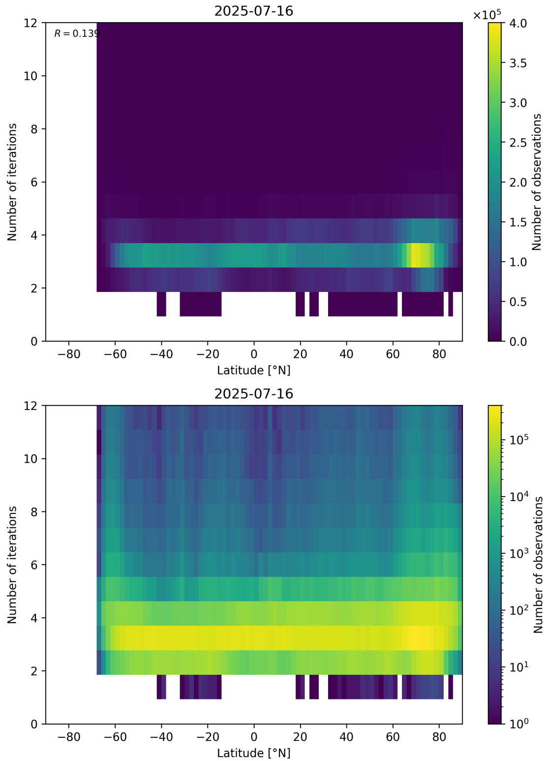
Figure 93: Scatter density plot of “Latitude” against “Number of iterations” for 2025-07-15 to 2025-07-17.
