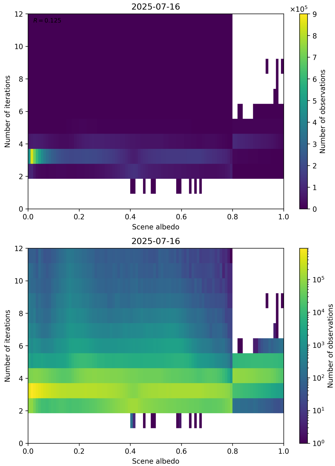
Figure 105: Scatter density plot of “Scene albedo” against “Number of iterations” for 2025-07-15 to 2025-07-17.
