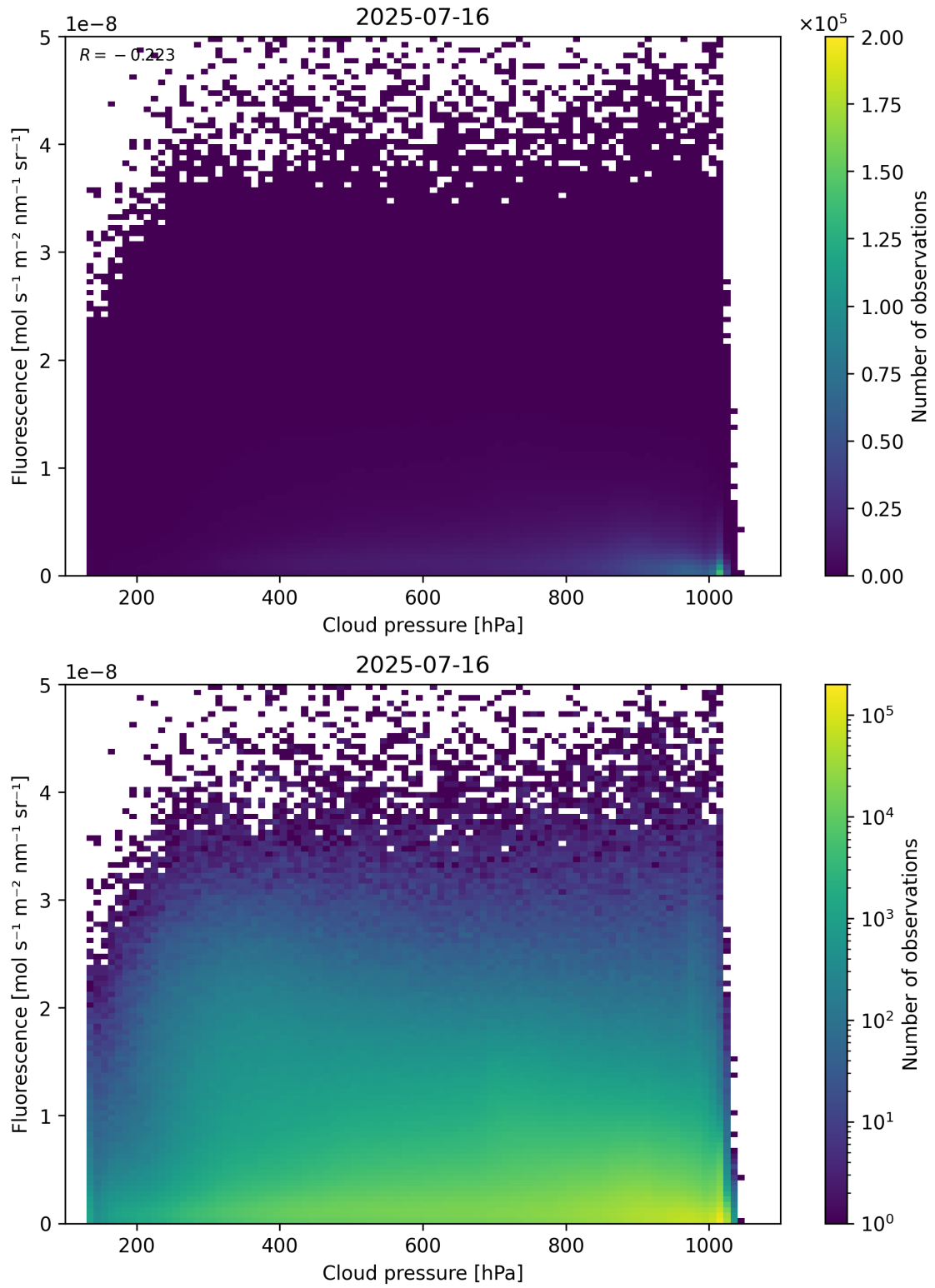
Figure 80: Scatter density plot of “Cloud pressure” against “Fluorescence” for 2025-07-15 to 2025-07-17.
