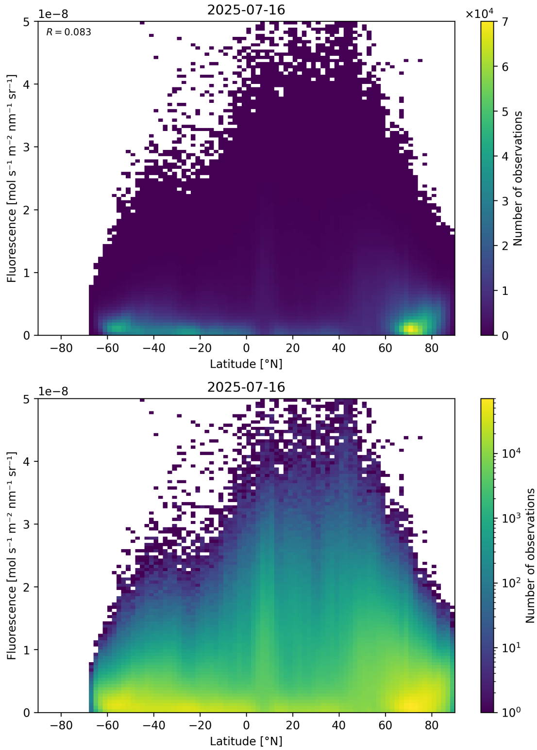
Figure 92: Scatter density plot of “Latitude” against “Fluorescence” for 2025-07-15 to 2025-07-17.
