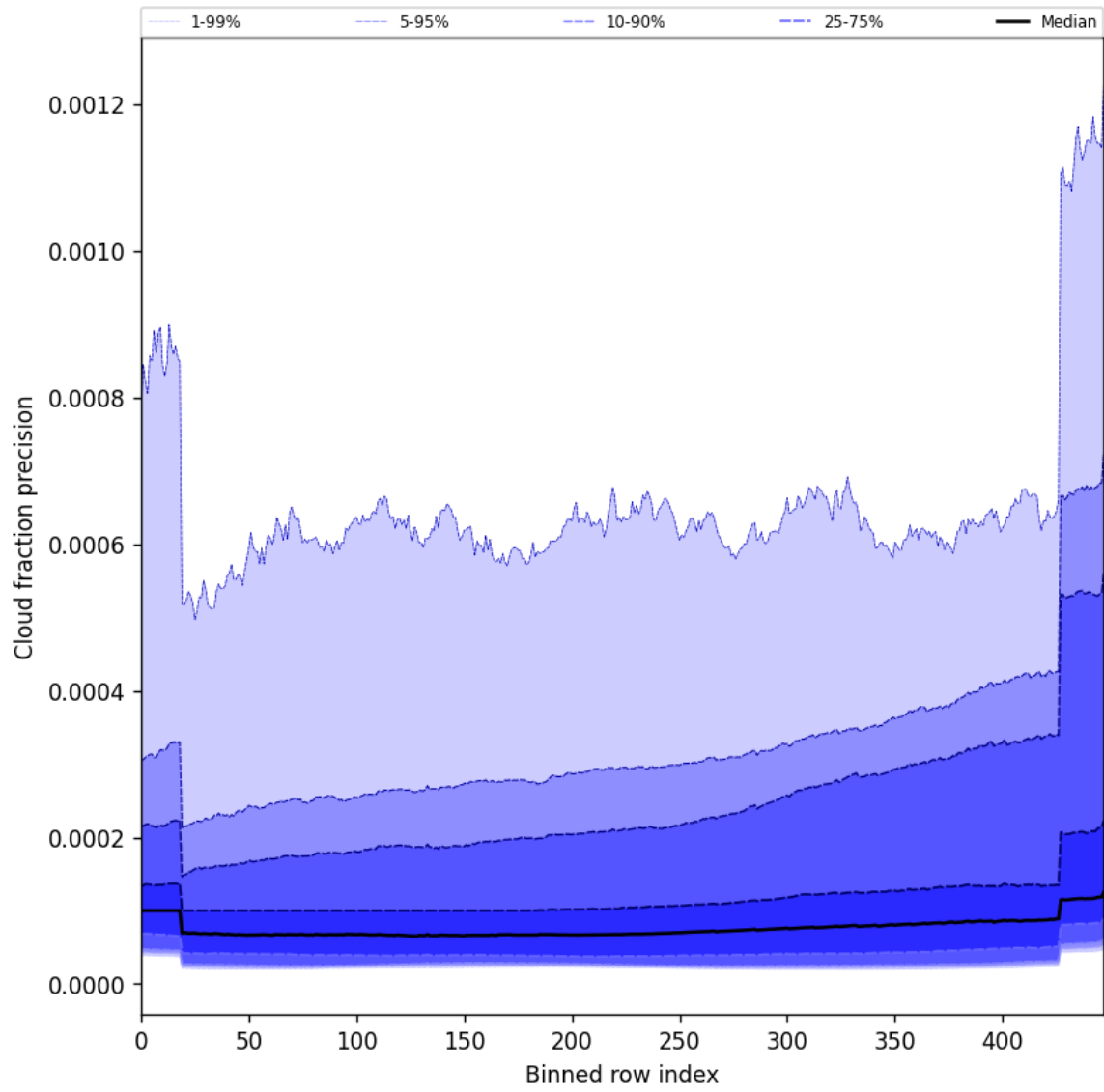
Figure 50: Along track statistics of “Cloud fraction precision” for 2025-07-15 to 2025-07-17
