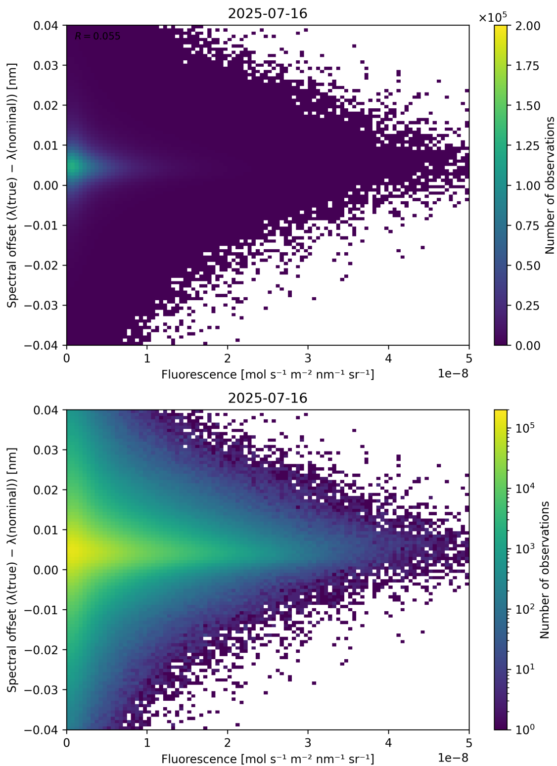
Figure 87: Scatter density plot of “Fluorescence” against “Spectral offset ( \lambda_{\text{true}} - \lambda_{\text{nominal}} )” for 2025-07-15 to 2025-07-17.
