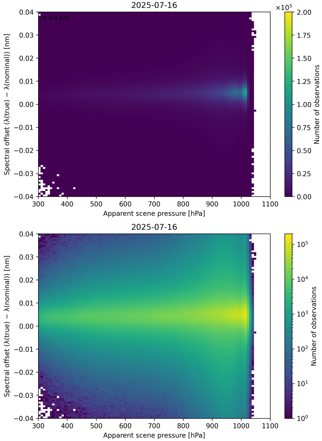
Figure 67: Scatter density plot of “Apparent scene pressure” against “Spectral offset ( \lambda_{\text{true}} - \lambda_{\text{nominal}} )” for 2025-07-15 to 2025-07-17.
