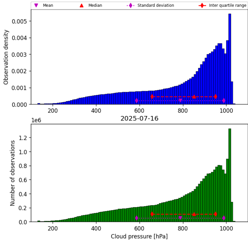
Figure 30: Histogram of “Cloud pressure” for 2025-07-15 to 2025-07-17
