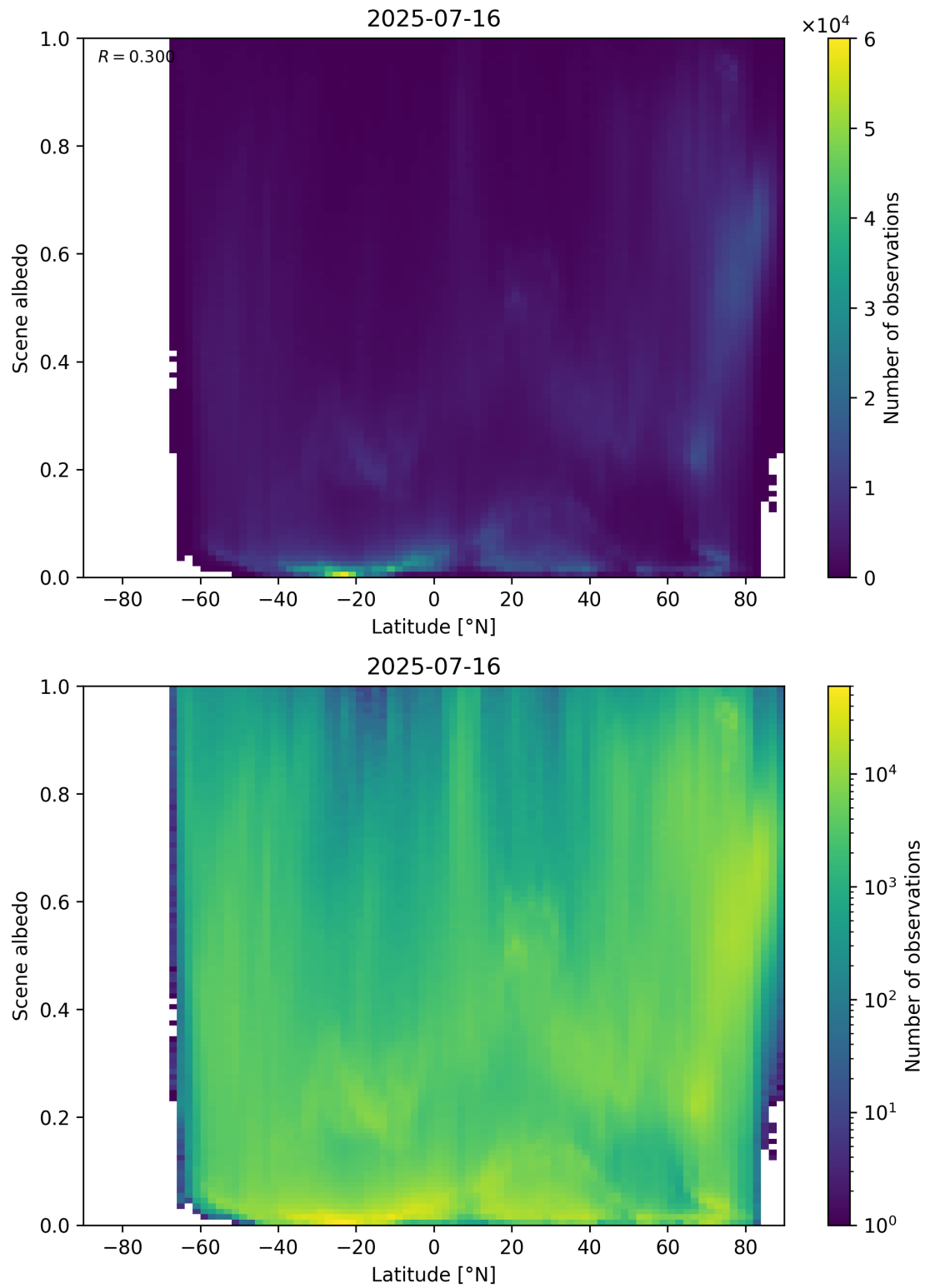
Figure 95: Scatter density plot of “Latitude” against “Scene albedo” for 2025-07-15 to 2025-07-17.
