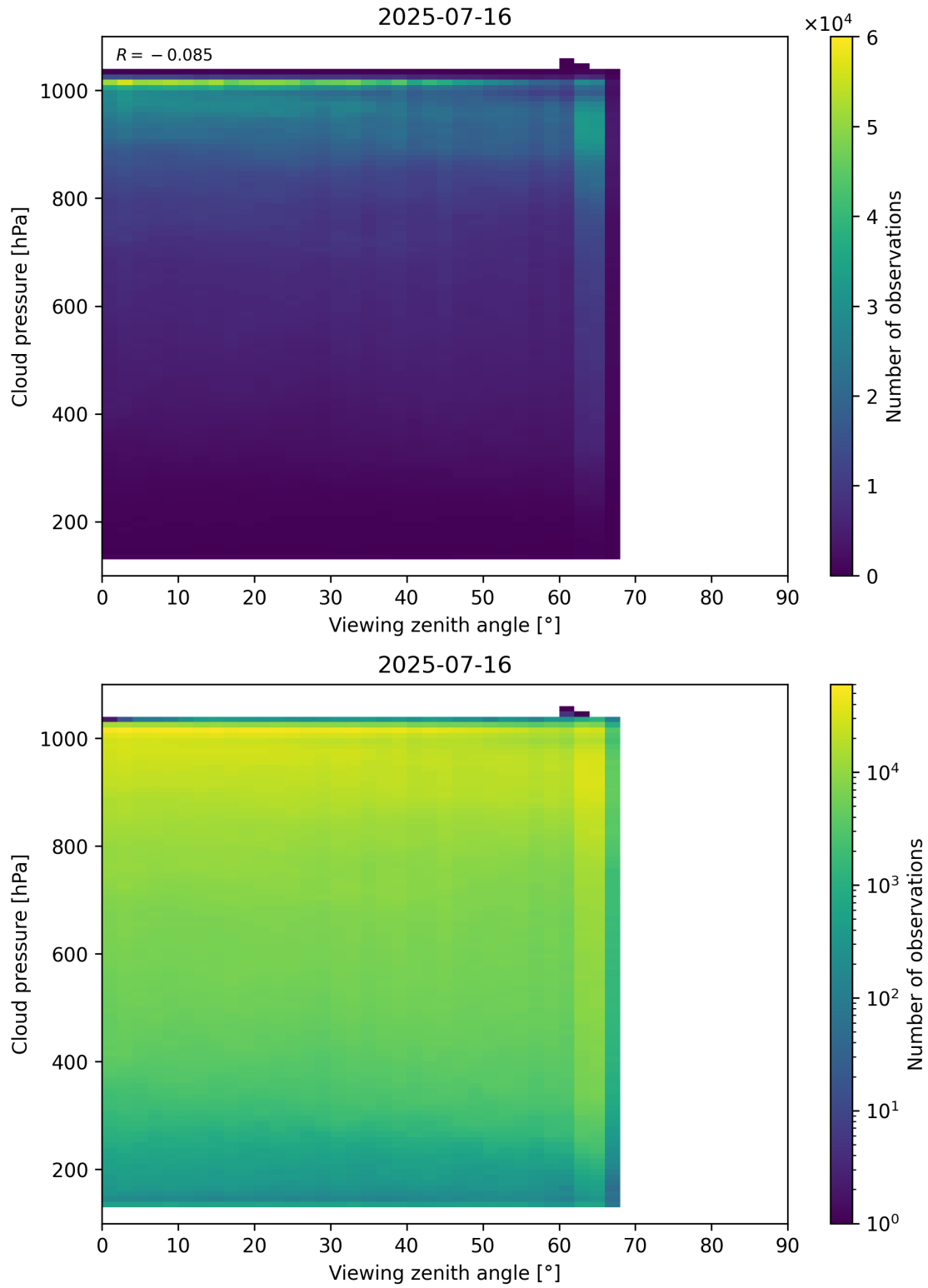
Figure 121: Scatter density plot of “Viewing zenith angle” against “Cloud pressure” for 2025-07-15 to 2025-07-17.
