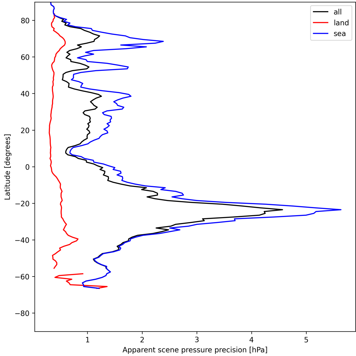
Figure 20: Zonal average of “Apparent scene pressure precision” for 2025-07-15 to 2025-07-17.
