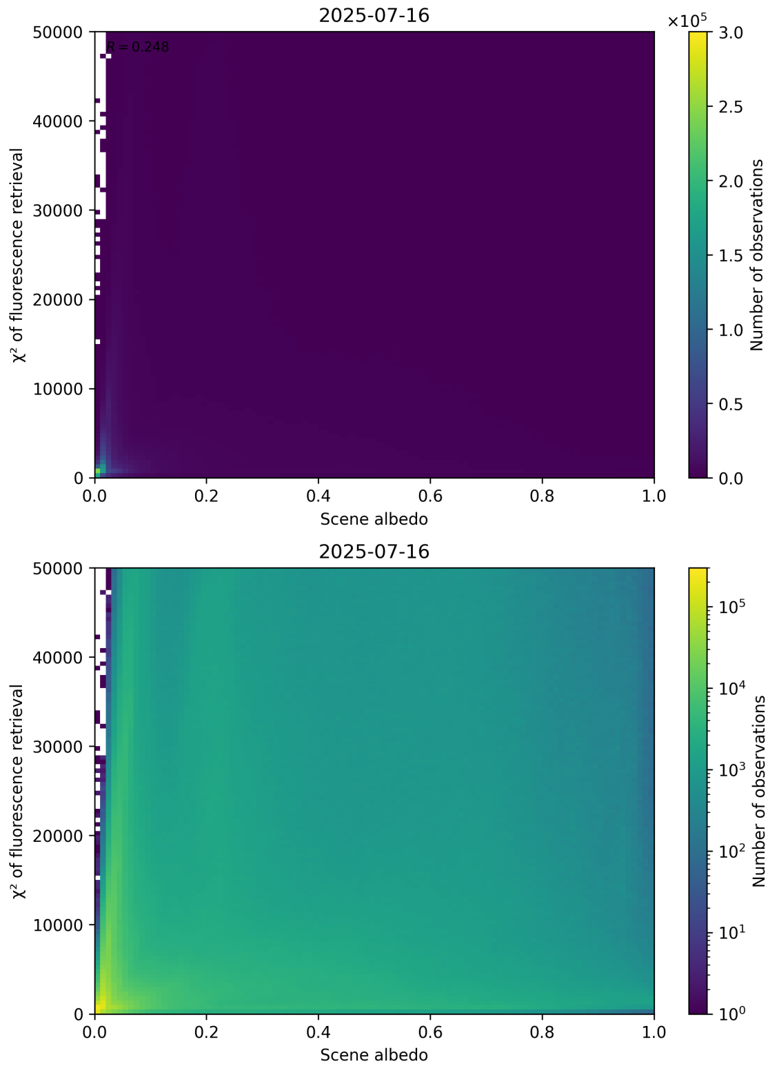
Figure 103: Scatter density plot of “Scene albedo” against “ \chi^2 of fluorescence retrieval” for 2025-07-15 to 2025-07-17.
