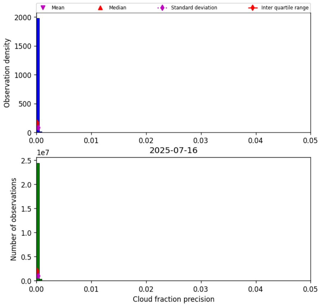
Figure 33: Histogram of “Cloud fraction precision” for 2025-07-15 to 2025-07-17
