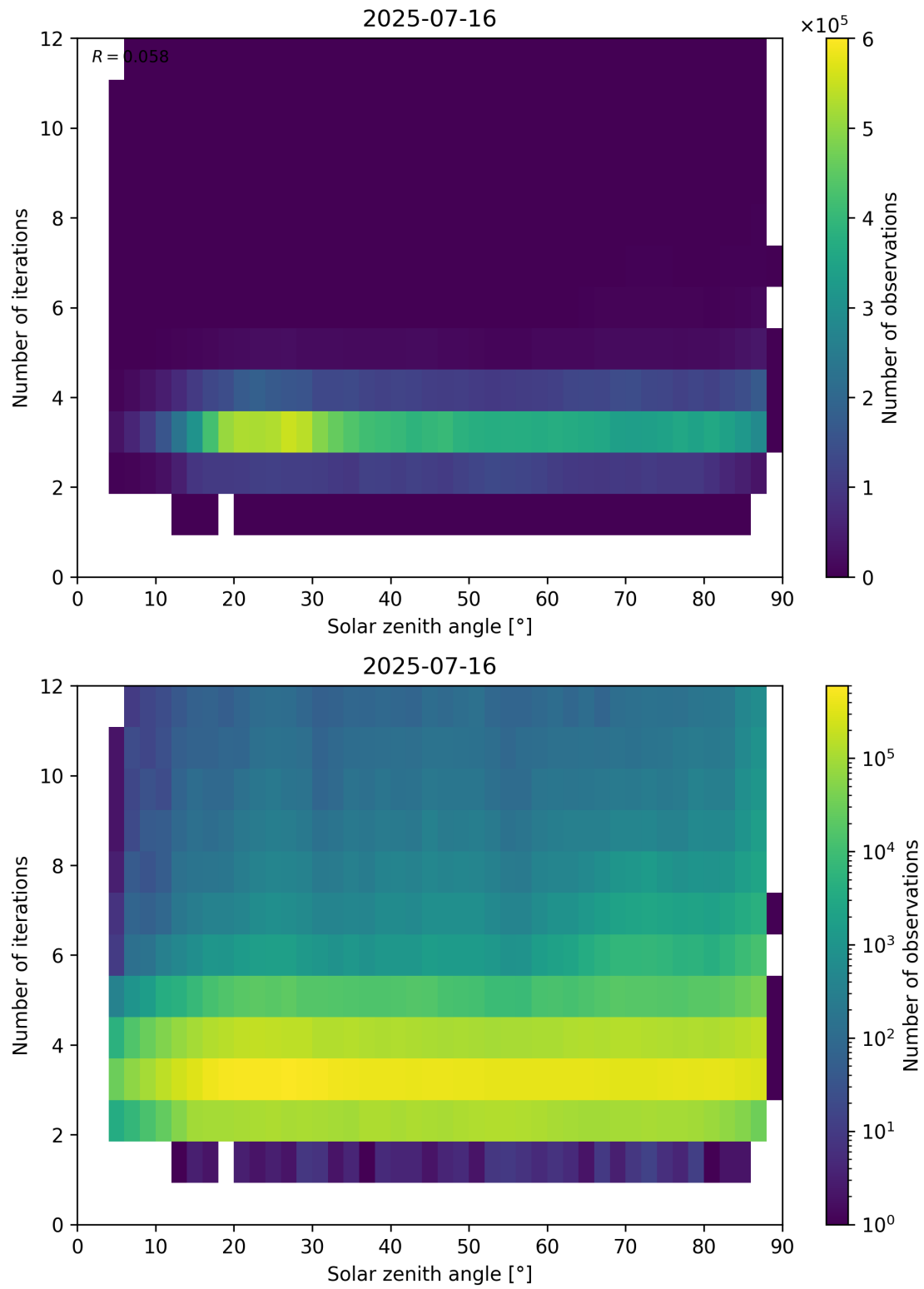
Figure 114: Scatter density plot of “Solar zenith angle” against “Number of iterations” for 2025-07-15 to 2025-07-17.
