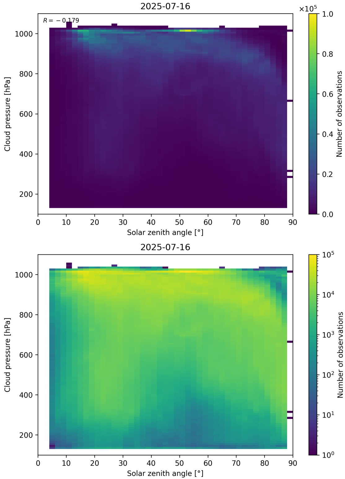
Figure 111: Scatter density plot of “Solar zenith angle” against “Cloud pressure” for 2025-07-15 to 2025-07-17.
