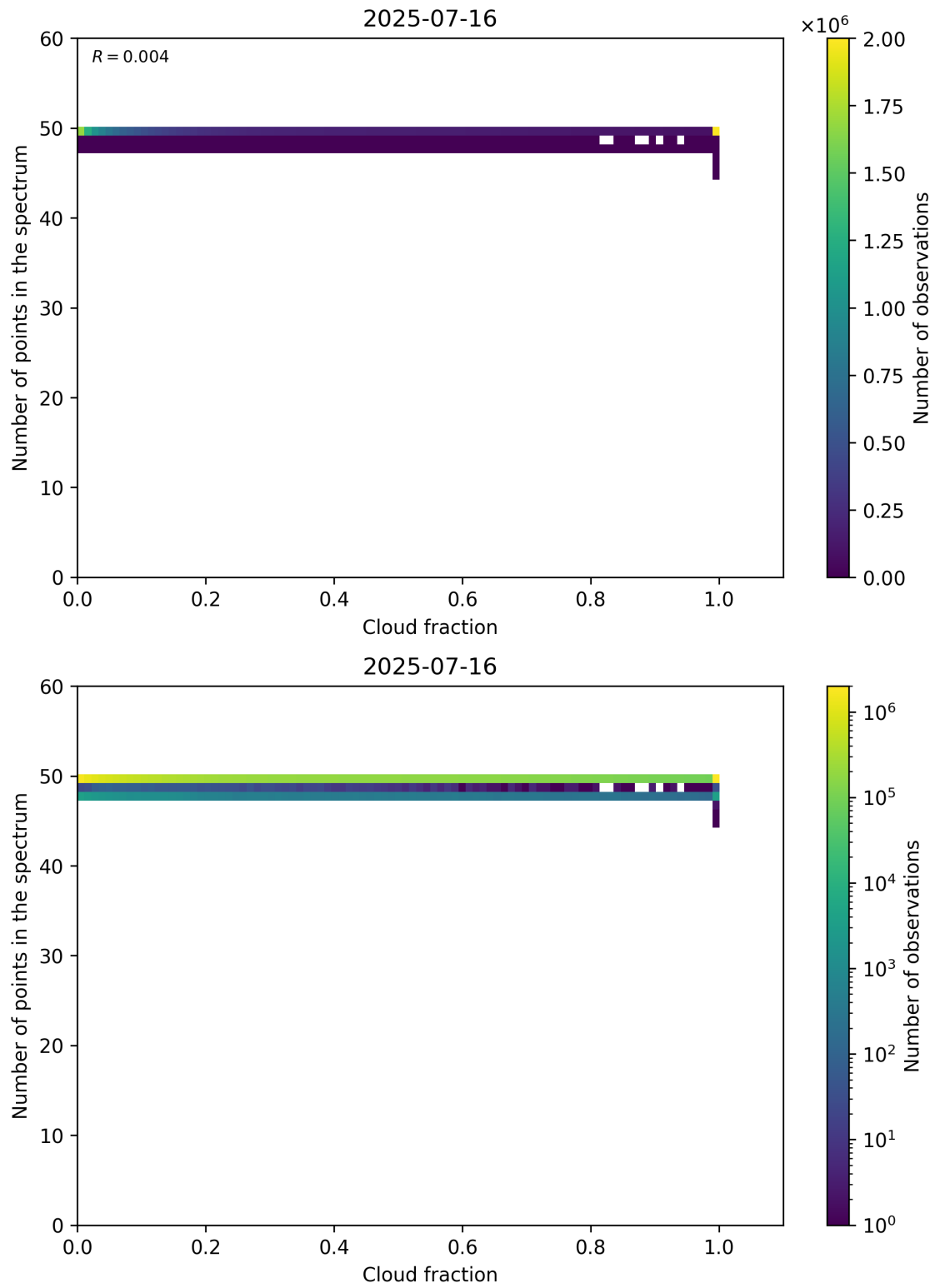
Figure 74: Scatter density plot of “Cloud fraction” against “Number of points in the spectrum” for 2025-07-15 to 2025-07-17.
