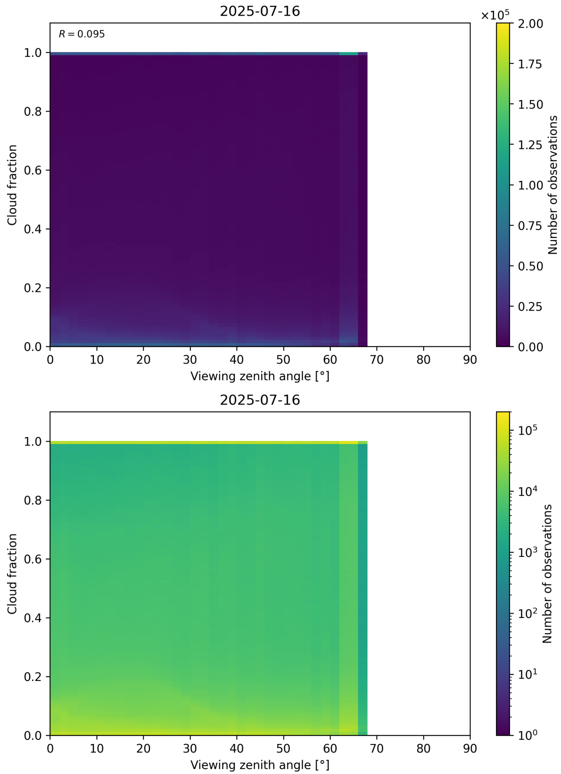
Figure 120: Scatter density plot of “Viewing zenith angle” against “Cloud fraction” for 2025-07-15 to 2025-07-17.
