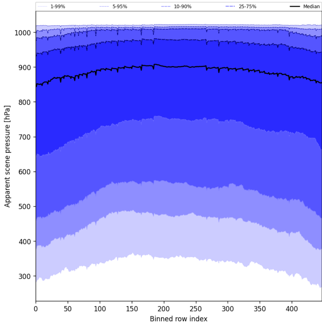
Figure 53: Along track statistics of “Apparent scene pressure” for 2025-07-15 to 2025-07-17
