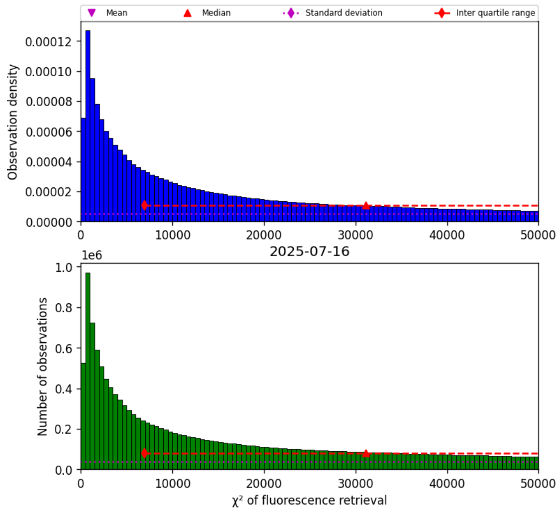
Figure 42: Histogram of “ \chi^2 of fluorescence retrieval” for 2025-07-15 to 2025-07-17
