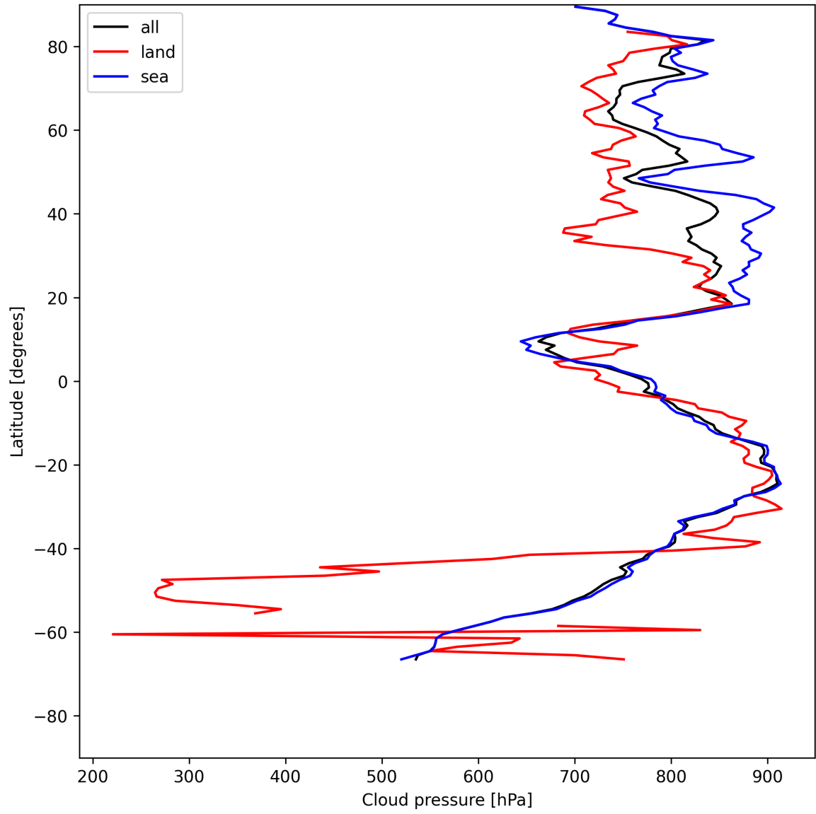
Figure 13: Zonal average of “Cloud pressure” for 2025-07-15 to 2025-07-17.
