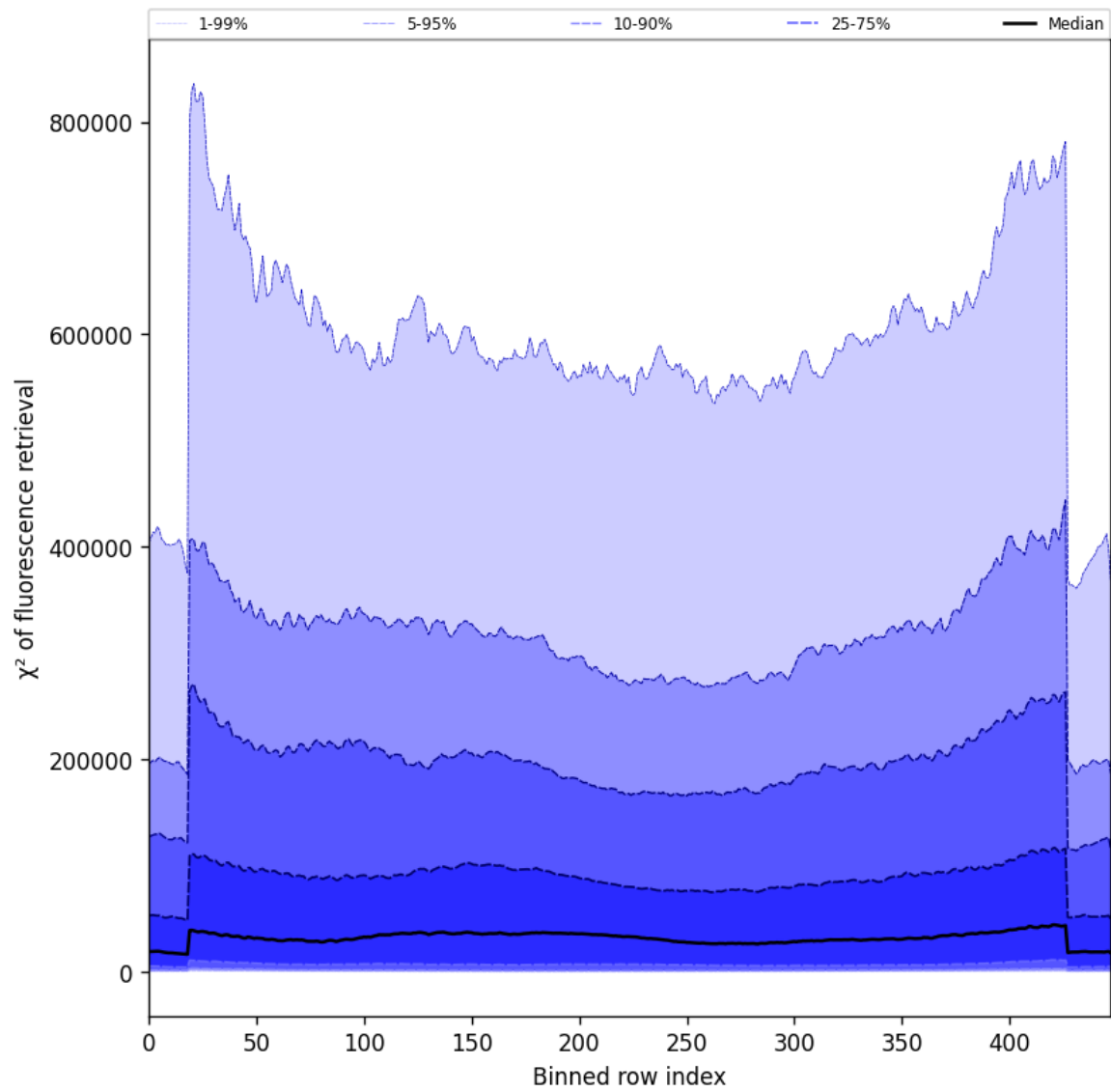
Figure 59: Along track statistics of “ \chi^2 of fluorescence retrieval” for 2025-07-15 to 2025-07-17
