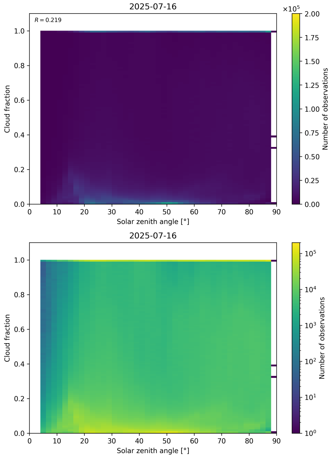
Figure 110: Scatter density plot of “Solar zenith angle” against “Cloud fraction” for 2025-07-15 to 2025-07-17.
