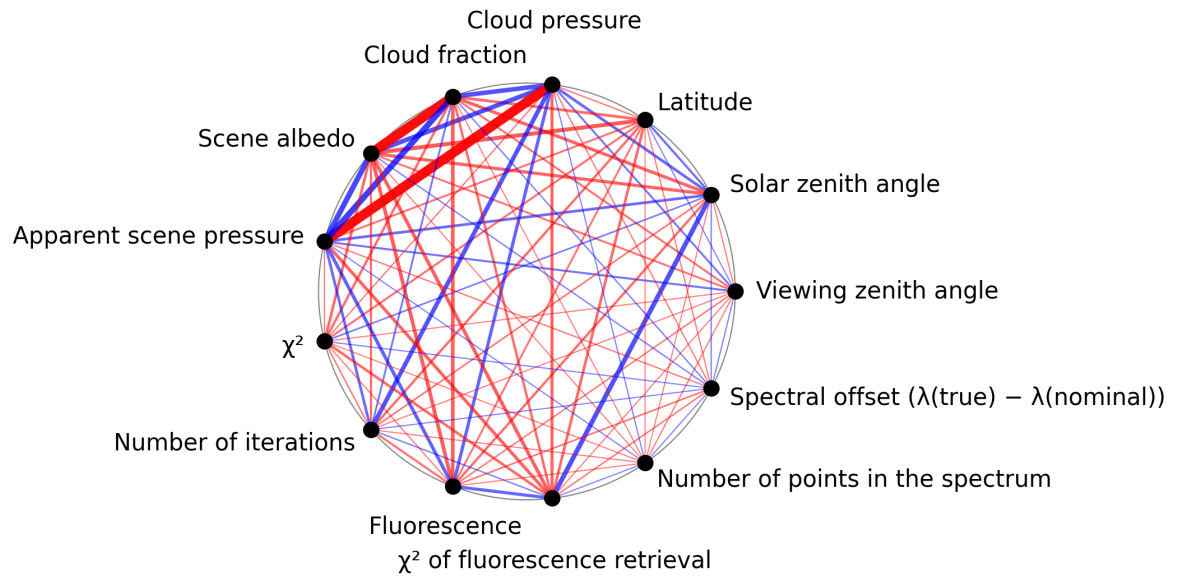
Figure 1: Map of correlation graph for 2025-07-15 to 2025-07-17.
