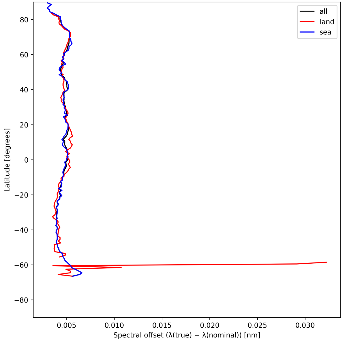
Figure 28: Zonal average of “Spectral offset ( \lambda_{\text{true}} - \lambda_{\text{nominal}} )” for 2025-07-15 to 2025-07-17.
