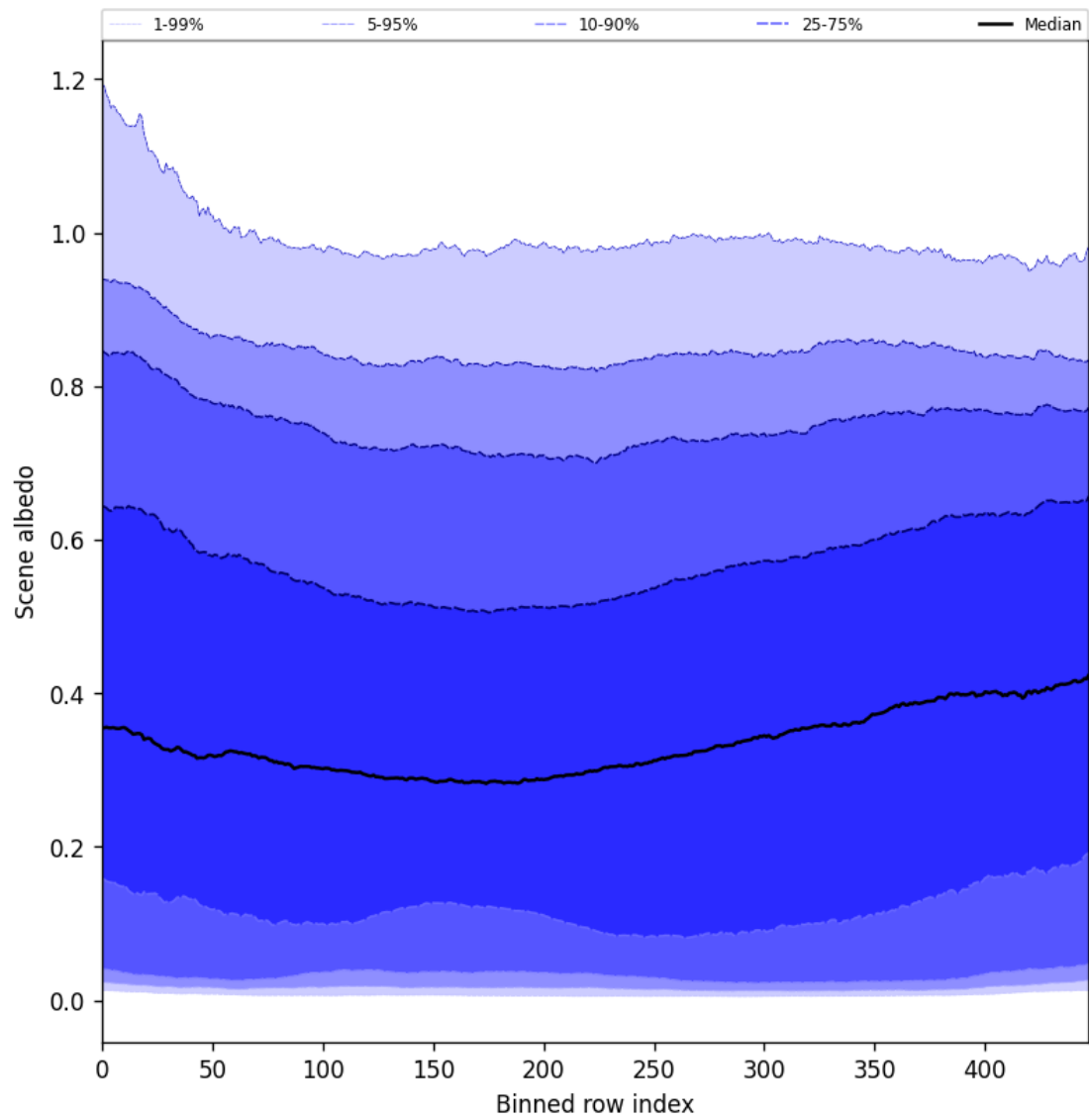
Figure 51: Along track statistics of “Scene albedo” for 2025-07-15 to 2025-07-17
