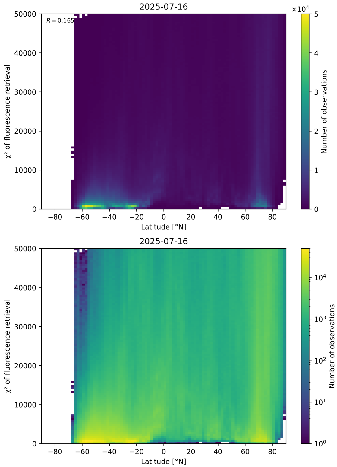
Figure 89: Scatter density plot of “Latitude” against “ \chi^2 of fluorescence retrieval” for 2025-07-15 to 2025-07-17.
