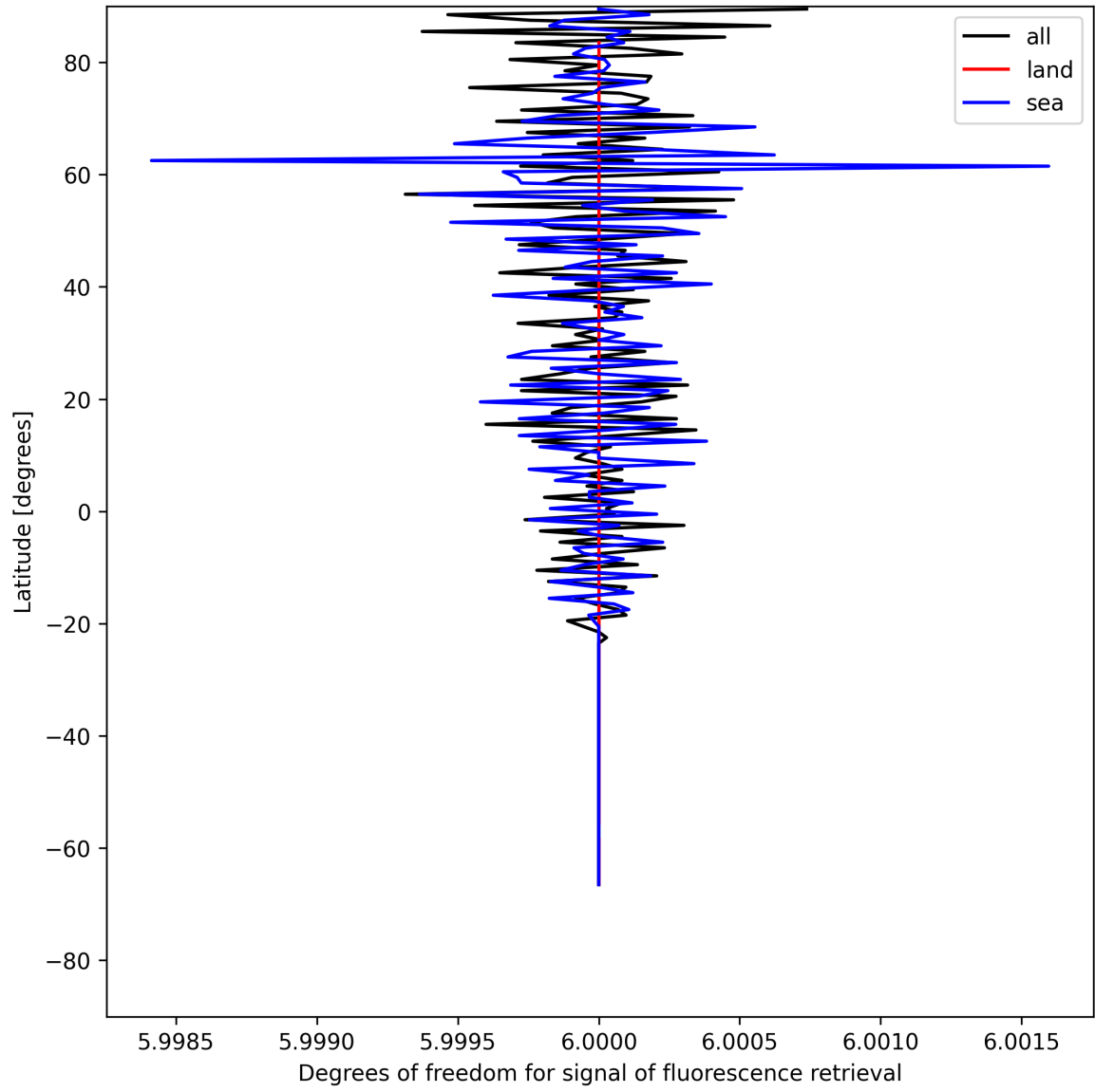
Figure 26: Zonal average of “Degrees of freedom for signal of fluorescence retrieval” for 2025-07-15 to 2025-07-17.
