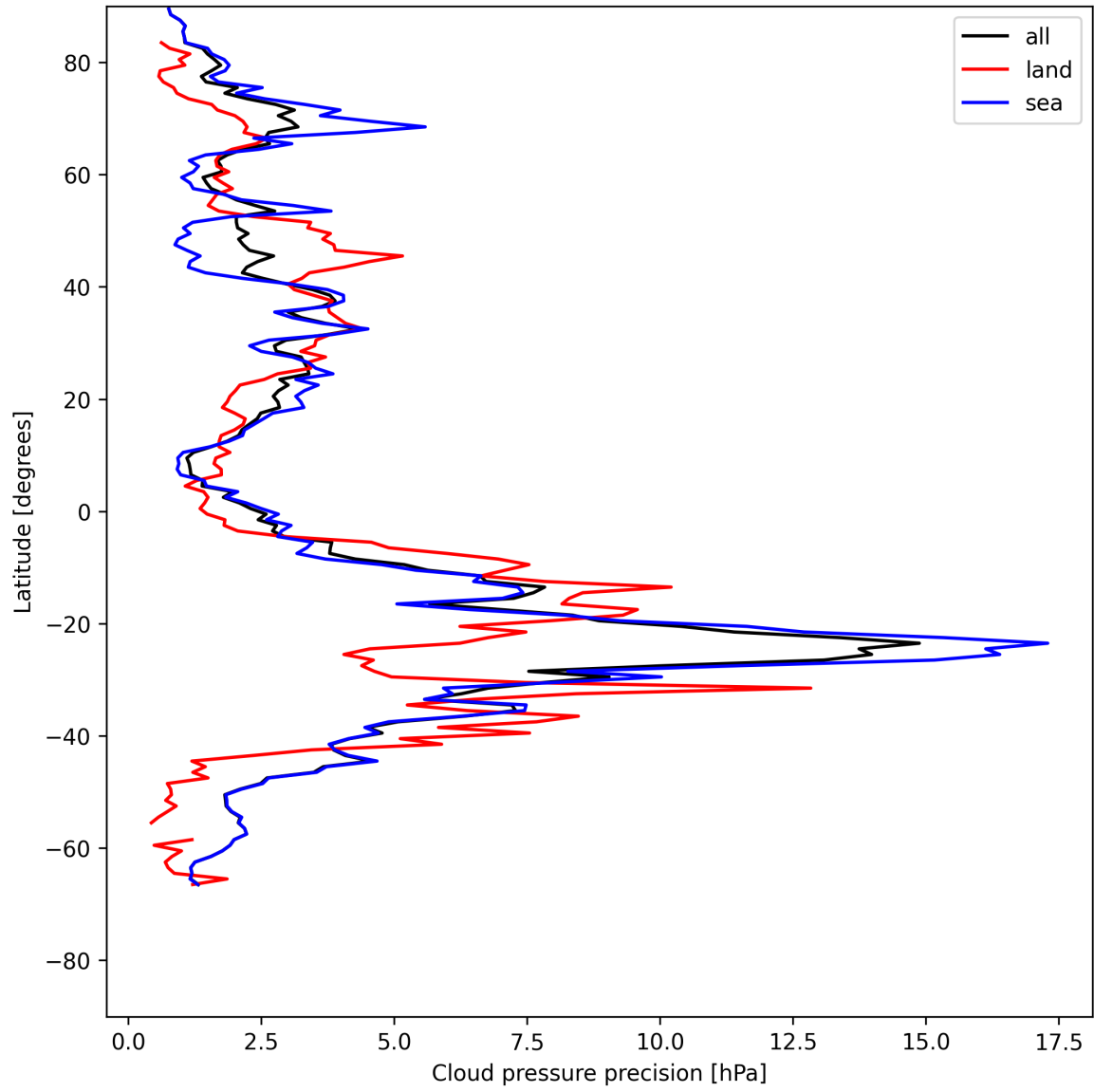
Figure 14: Zonal average of “Cloud pressure precision” for 2025-07-15 to 2025-07-17.
