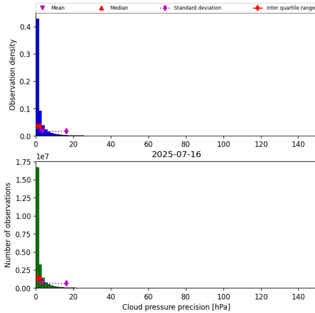
Figure 31: Histogram of “Cloud pressure precision” for 2025-07-15 to 2025-07-17
