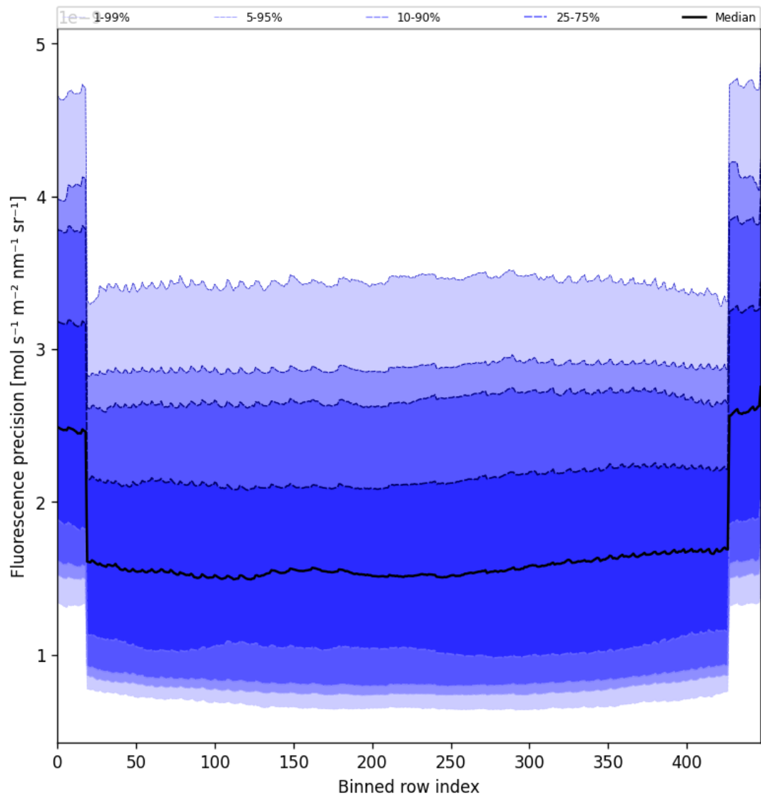
Figure 58: Along track statistics of “Fluorescence precision” for 2025-07-15 to 2025-07-17
