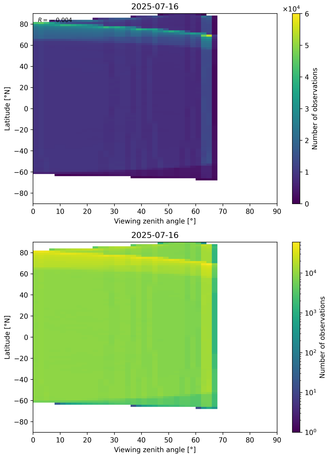
Figure 123: Scatter density plot of “Viewing zenith angle” against “Latitude” for 2025-07-15 to 2025-07-17.
