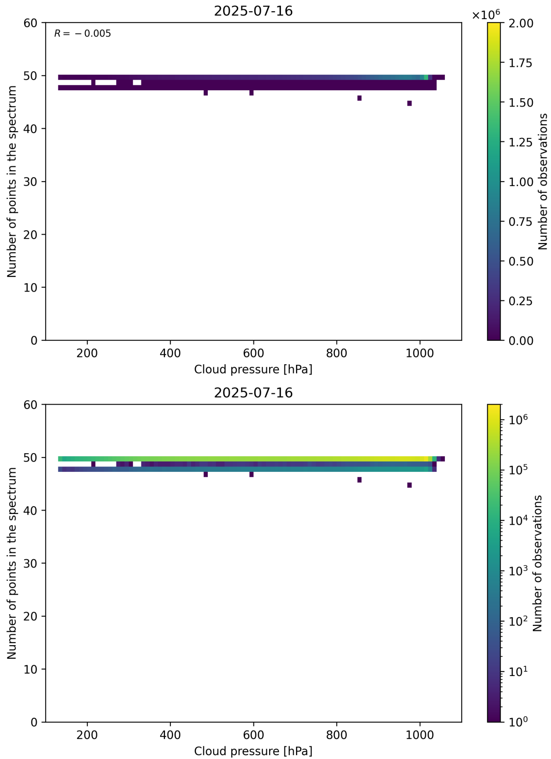
Figure 82: Scatter density plot of “Cloud pressure” against “Number of points in the spectrum” for 2025-07-15 to 2025-07-17.
