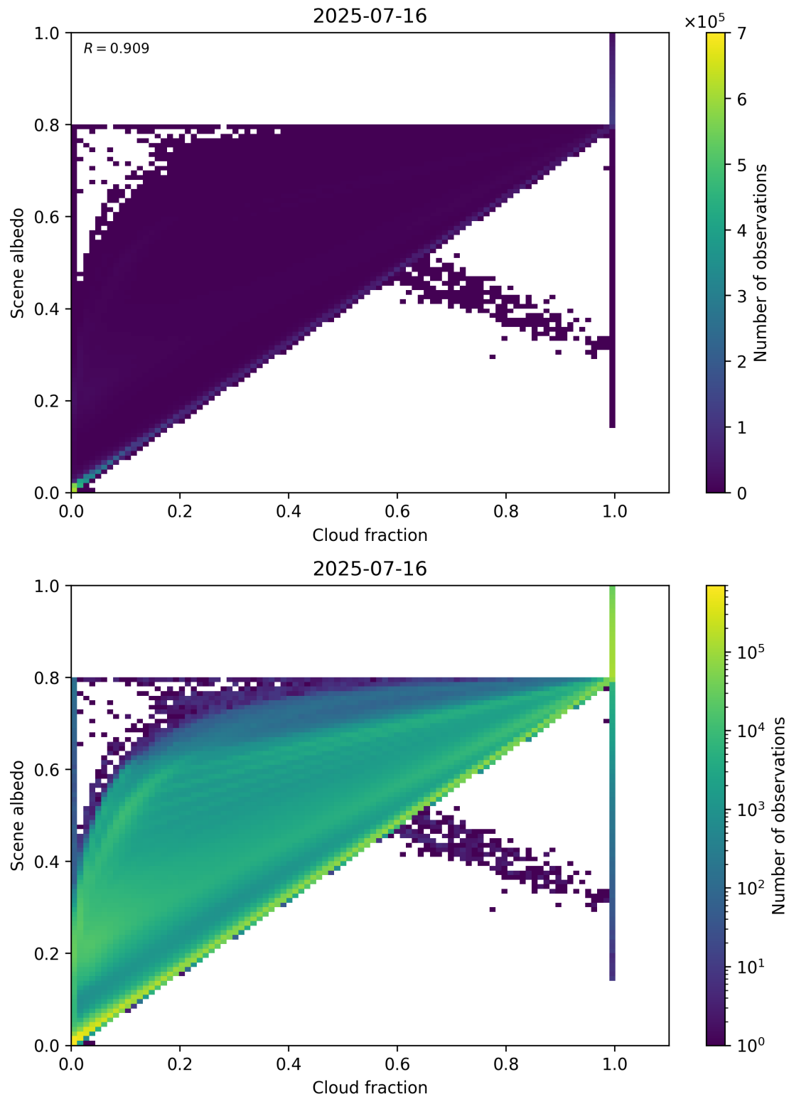
Figure 75: Scatter density plot of “Cloud fraction” against “Scene albedo” for 2025-07-15 to 2025-07-17.
