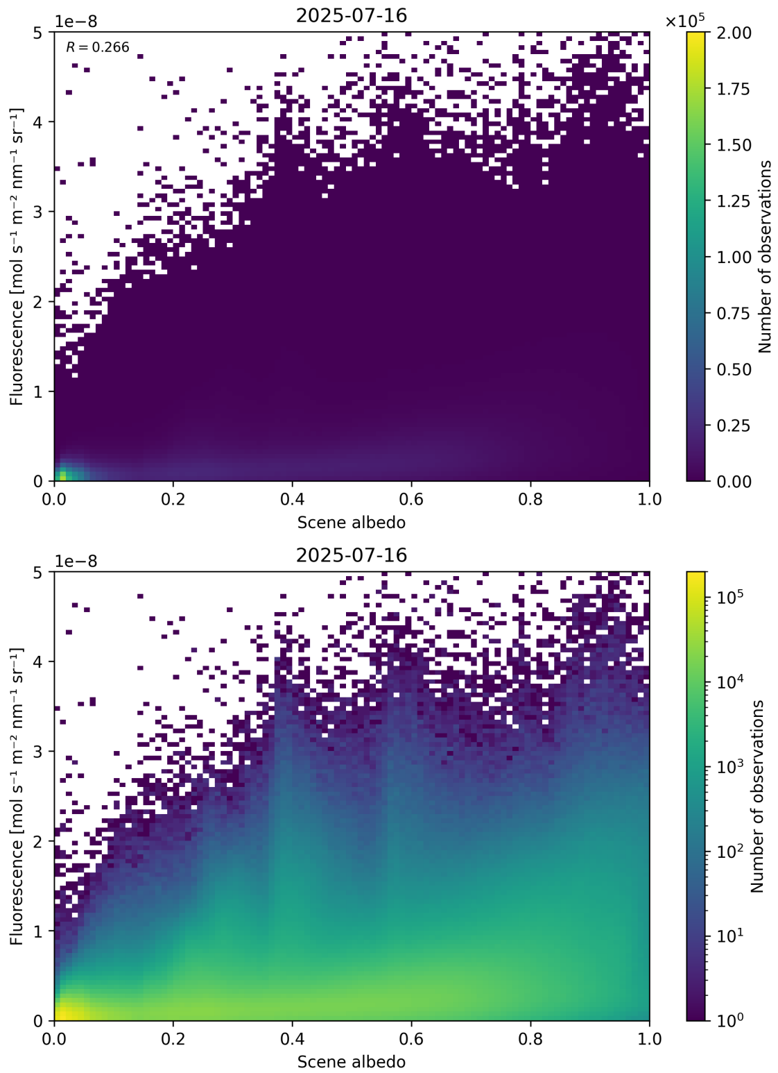
Figure 104: Scatter density plot of “Scene albedo” against “Fluorescence” for 2025-07-15 to 2025-07-17.
