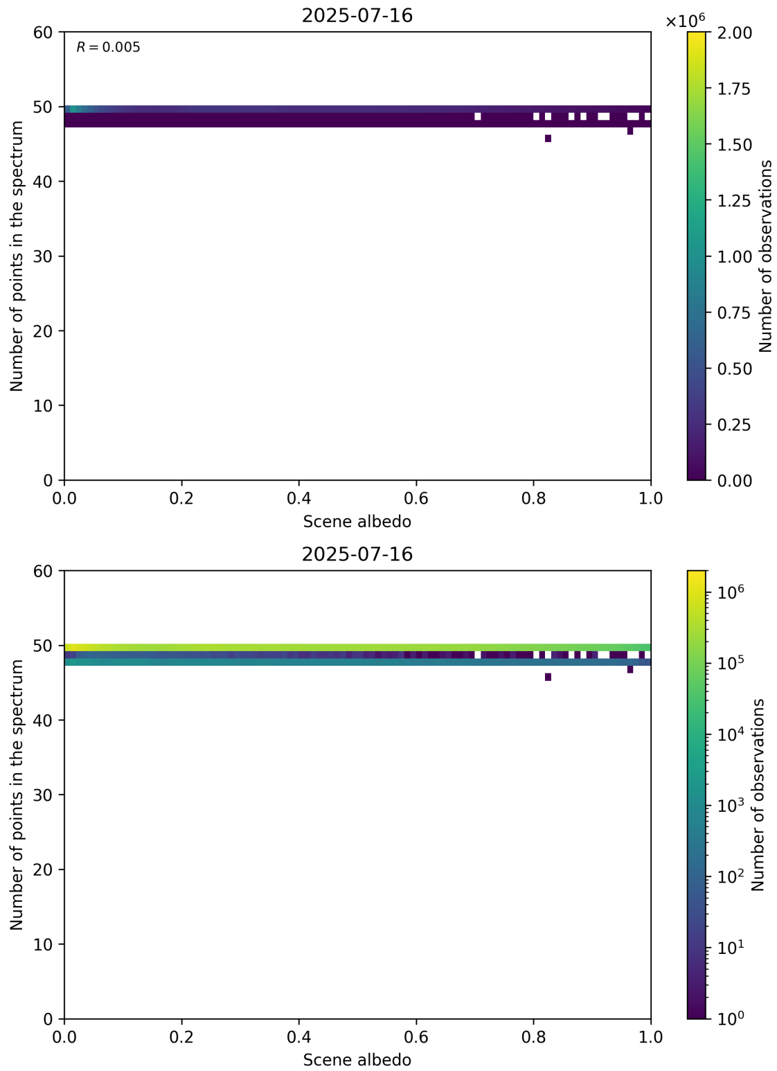
Figure 106: Scatter density plot of “Scene albedo” against “Number of points in the spectrum” for 2025-07-15 to 2025-07-17.
