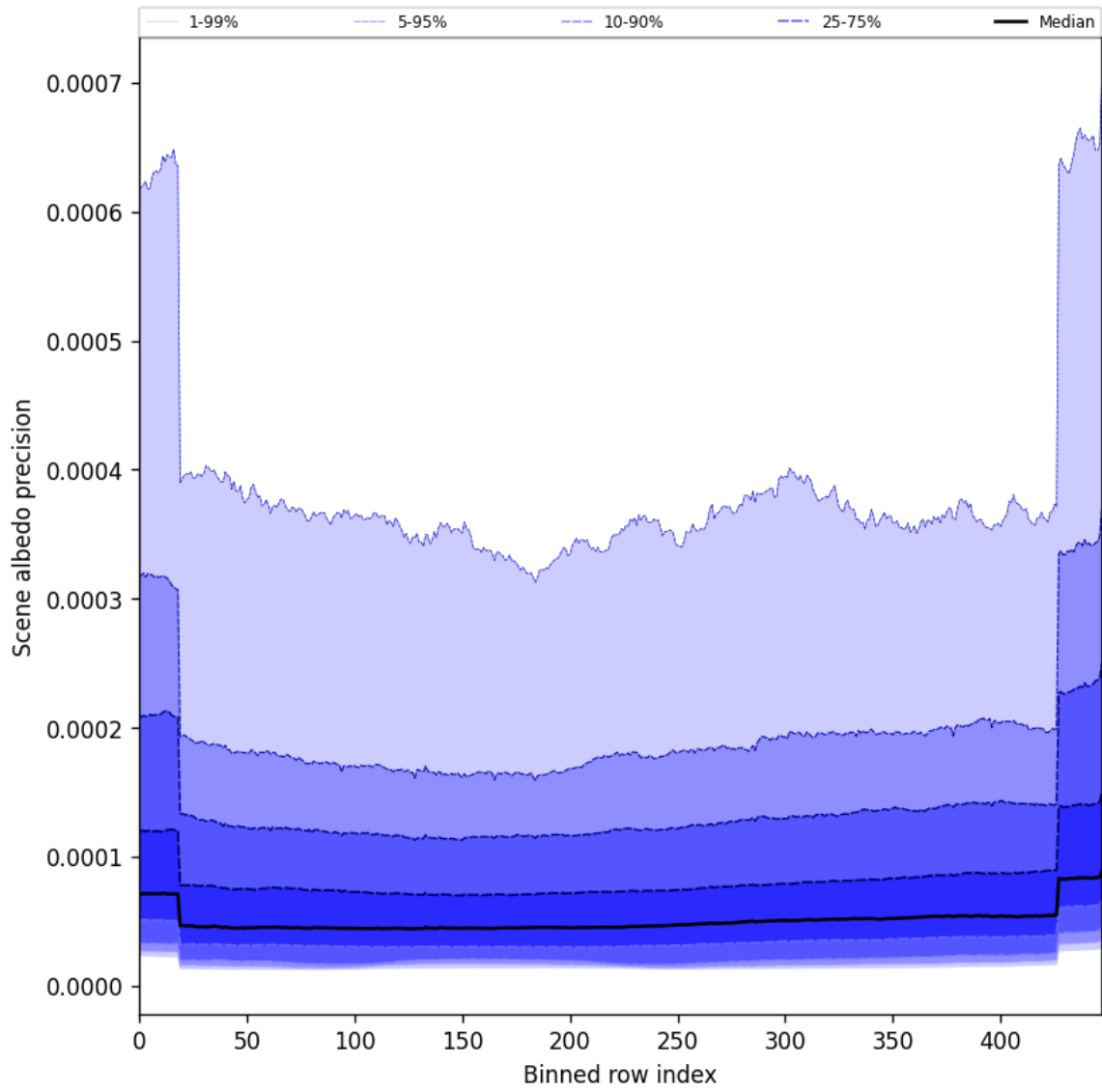
Figure 52: Along track statistics of “Scene albedo precision” for 2025-07-15 to 2025-07-17
