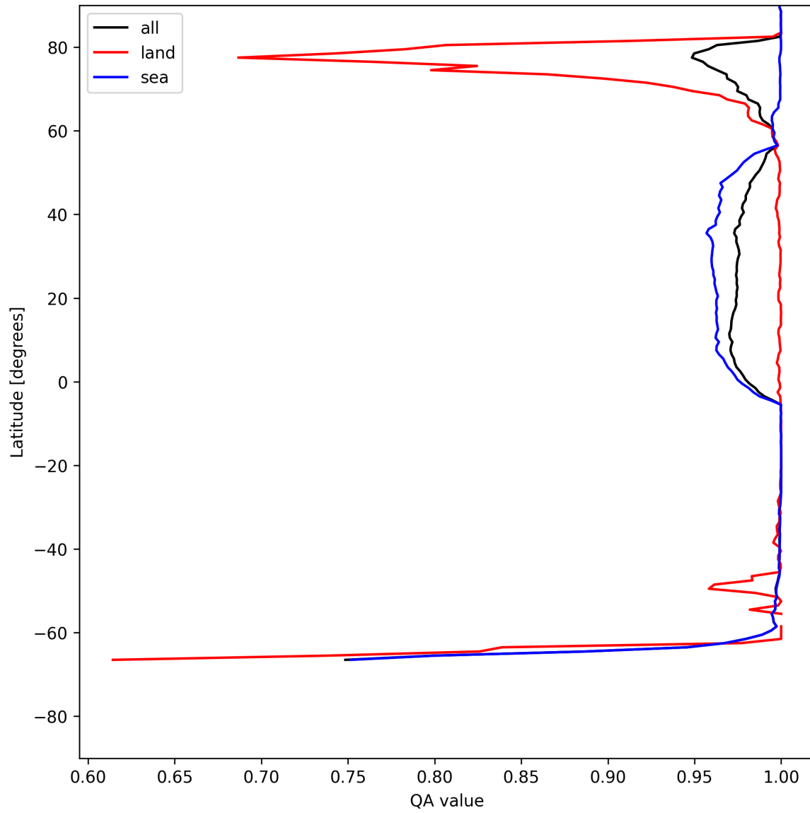
Figure 12: Zonal average of “QA value” for 2025-07-15 to 2025-07-17.
