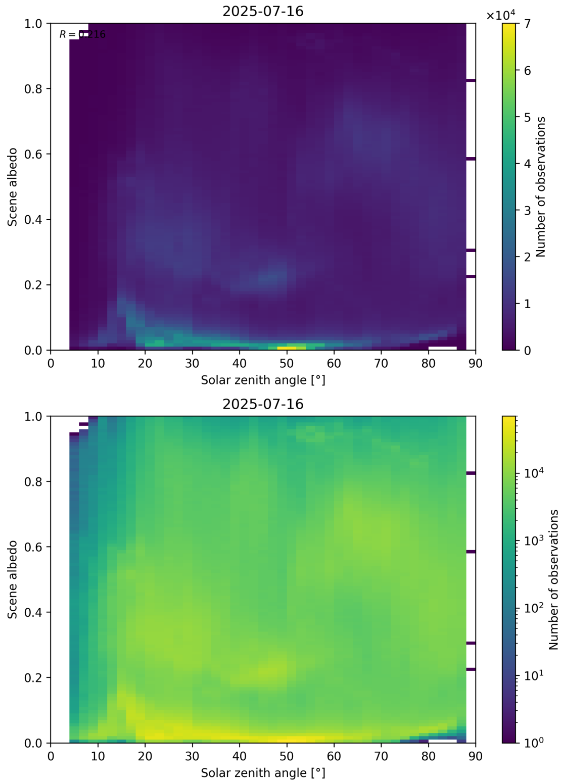
Figure 116: Scatter density plot of “Solar zenith angle” against “Scene albedo” for 2025-07-15 to 2025-07-17.
