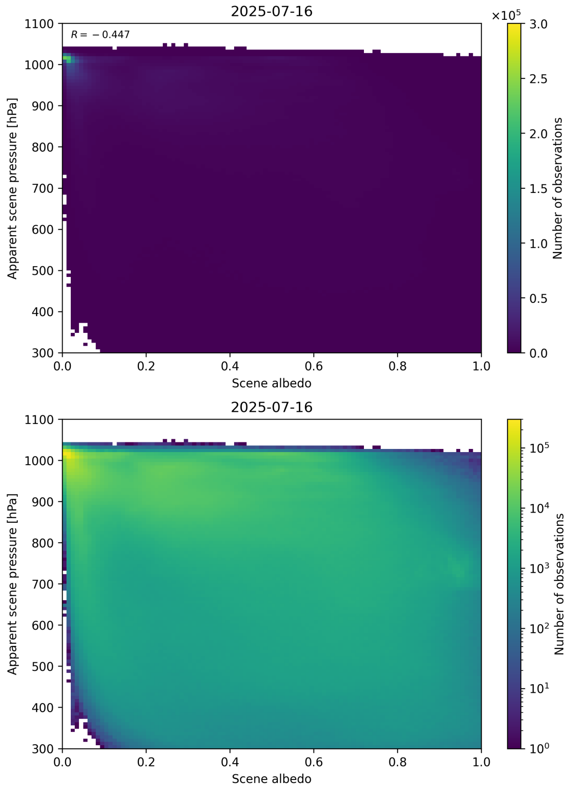
Figure 102: Scatter density plot of “Scene albedo” against “Apparent scene pressure” for 2025-07-15 to 2025-07-17.
