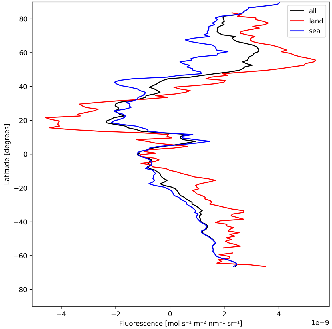
Figure 23: Zonal average of “Fluorescence” for 2025-07-15 to 2025-07-17.
