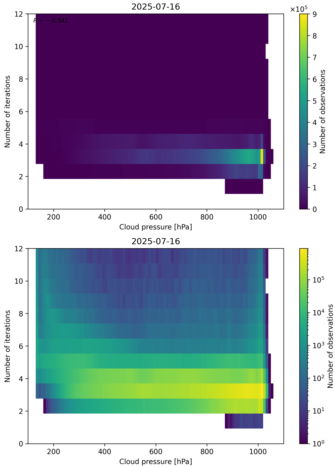
Figure 81: Scatter density plot of “Cloud pressure” against “Number of iterations” for 2025-07-15 to 2025-07-17.
