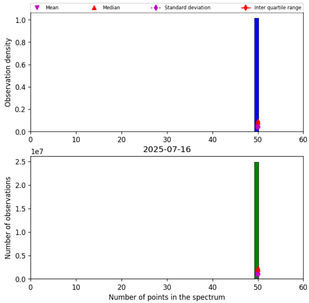
Figure 44: Histogram of "Number of points in the spectrum" for 2025-07-15 to 2025-07-17
