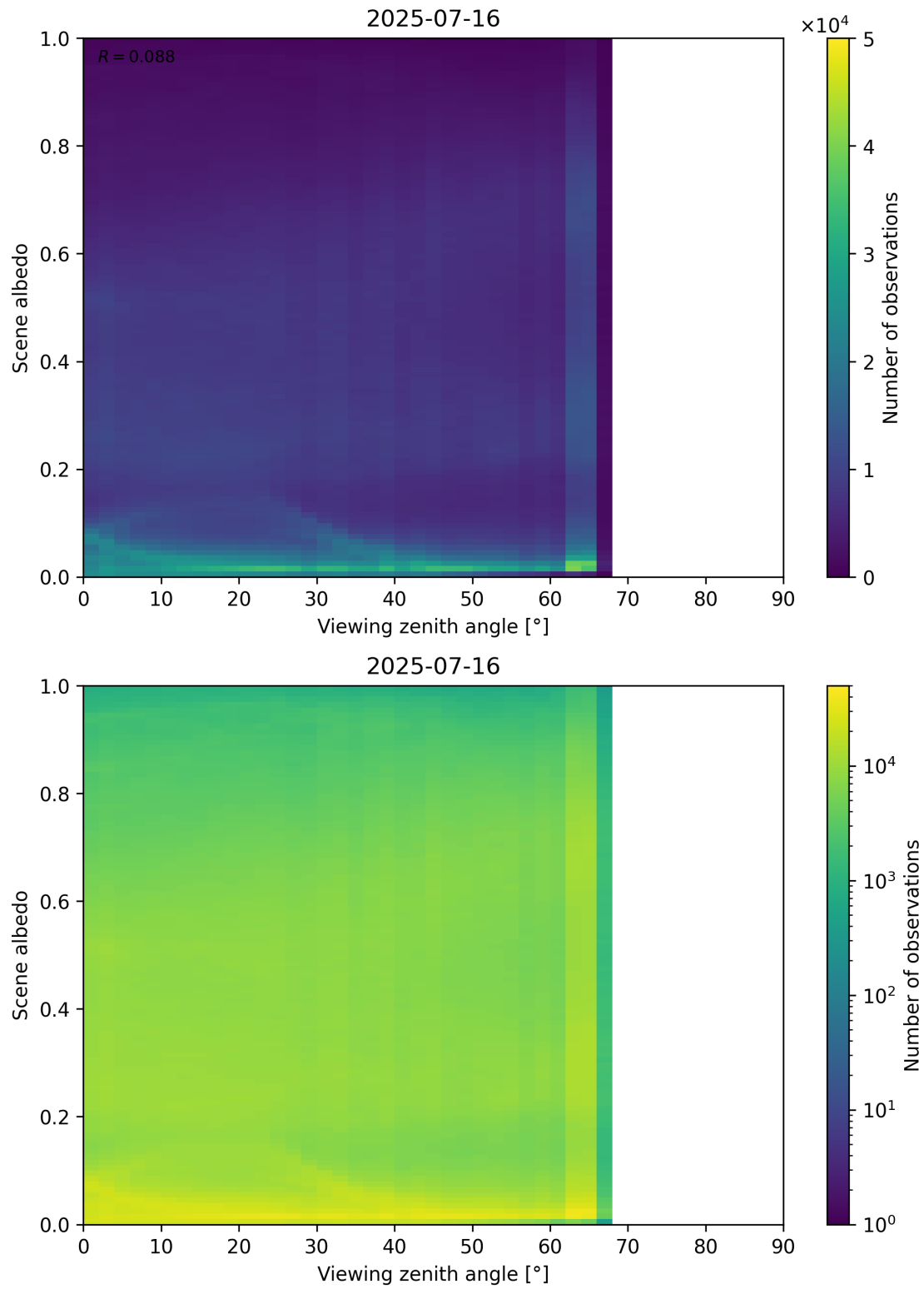
Figure 126: Scatter density plot of “Viewing zenith angle” against “Scene albedo” for 2025-07-15 to 2025-07-17.
