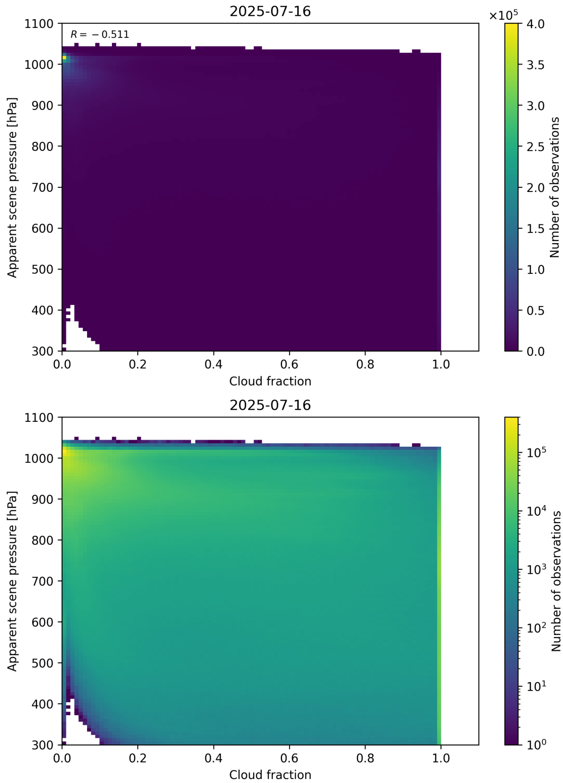
Figure 70: Scatter density plot of “Cloud fraction” against “Apparent scene pressure” for 2025-07-15 to 2025-07-17.
