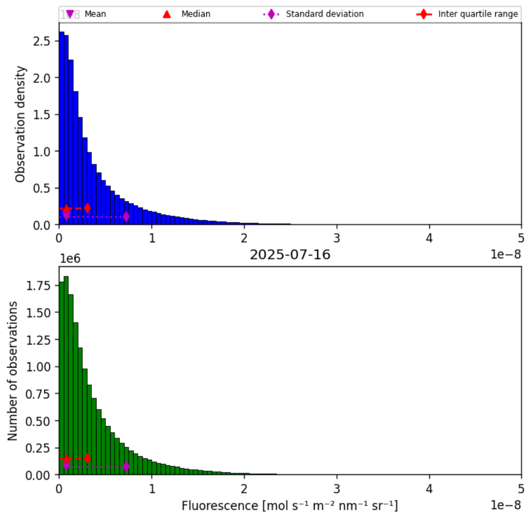
Figure 40: Histogram of “Fluorescence” for 2025-07-15 to 2025-07-17
