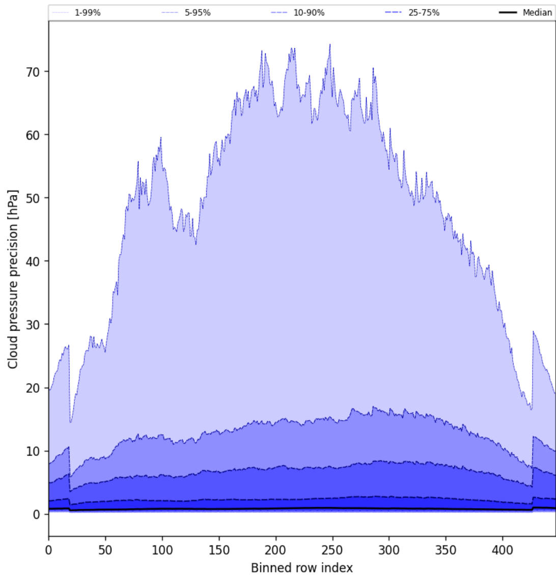
Figure 48: Along track statistics of “Cloud pressure precision” for 2025-07-15 to 2025-07-17
