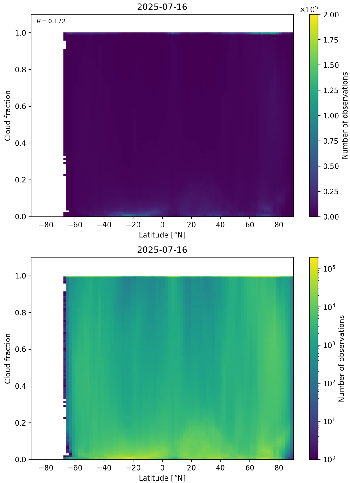
Figure 90: Scatter density plot of “Latitude” against “Cloud fraction” for 2025-07-15 to 2025-07-17.
