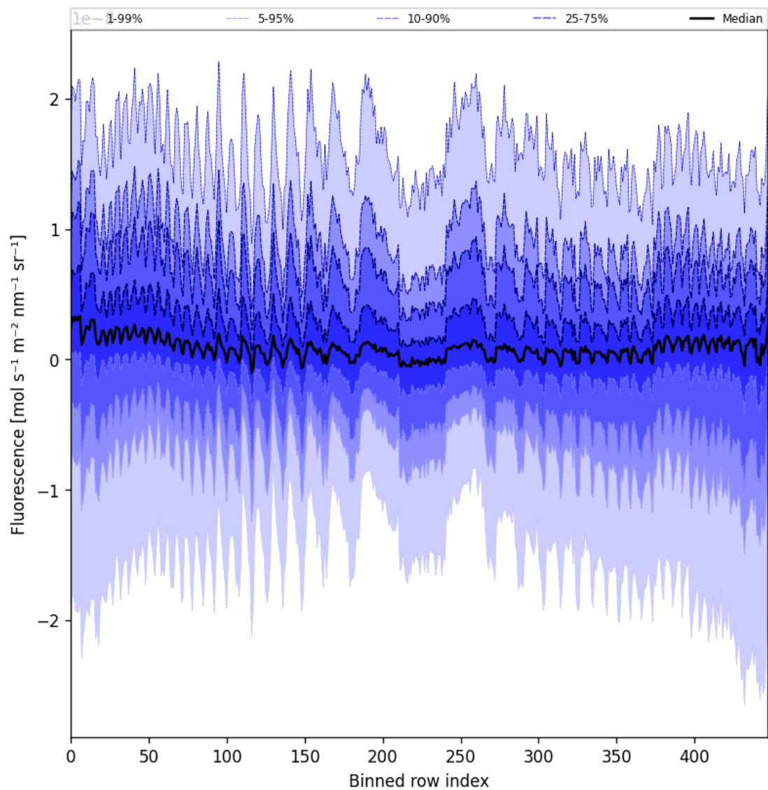
Figure 57: Along track statistics of "Fluorescence" for 2025-07-15 to 2025-07-17
