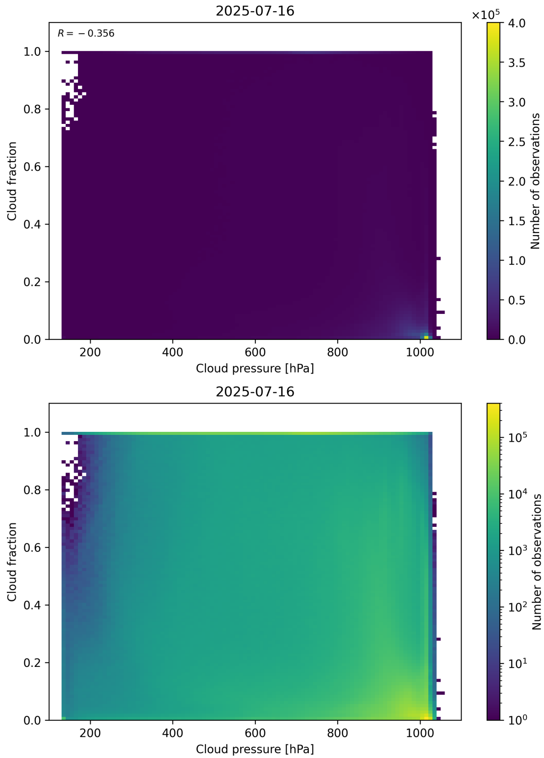
Figure 79: Scatter density plot of “Cloud pressure” against “Cloud fraction” for 2025-07-15 to 2025-07-17.
