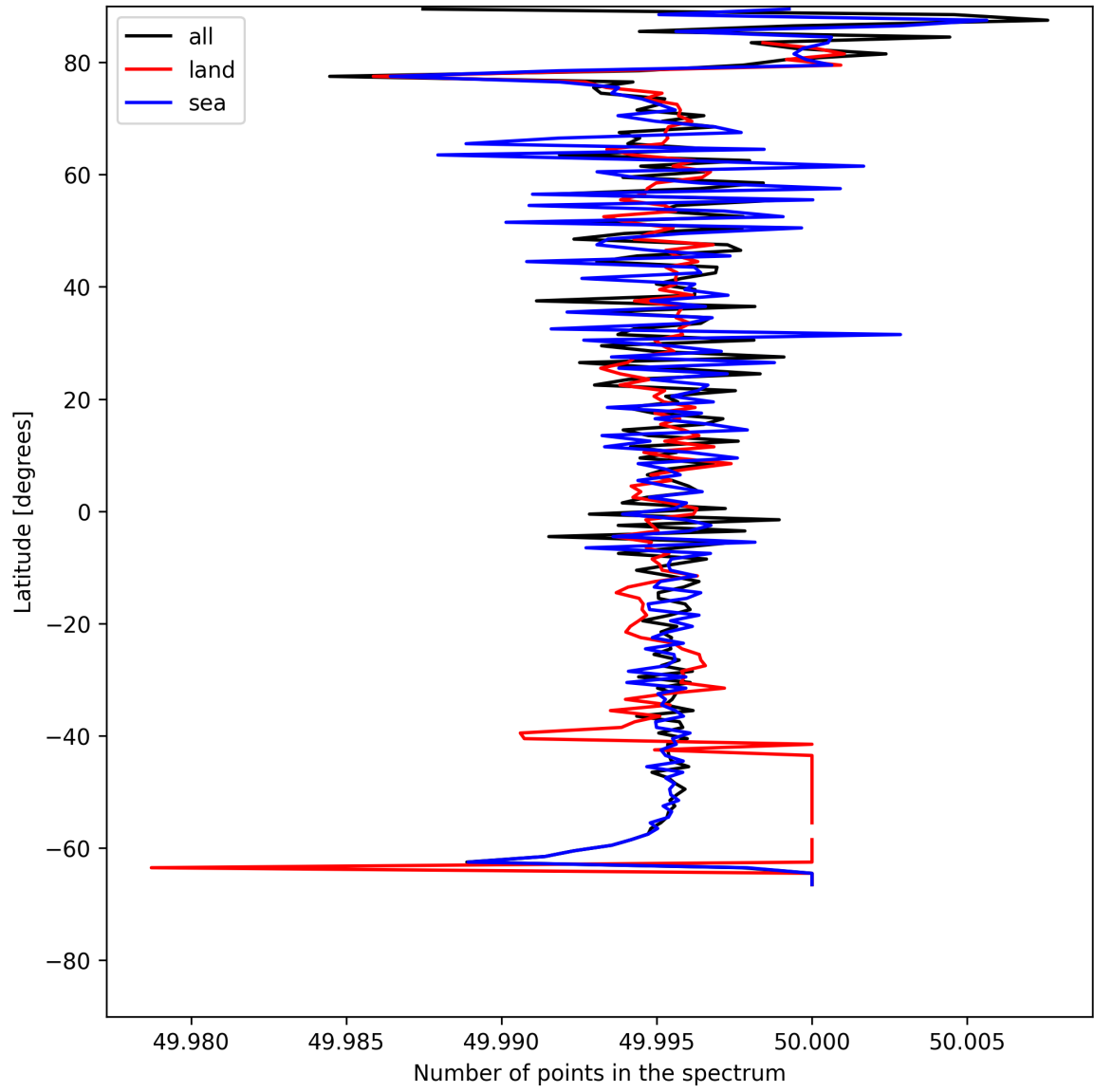
Figure 27: Zonal average of “Number of points in the spectrum” for 2025-07-15 to 2025-07-17.
