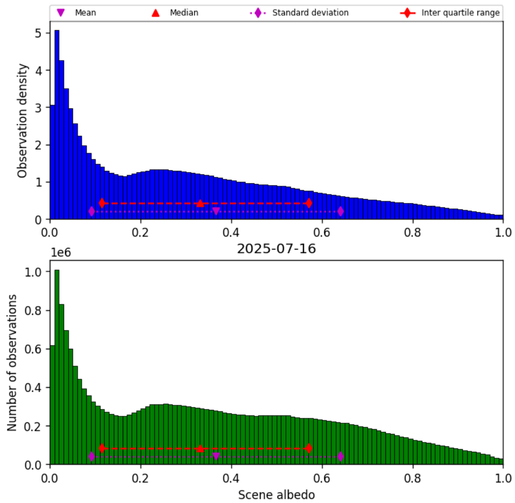
Figure 34: Histogram of “Scene albedo” for 2025-07-15 to 2025-07-17
