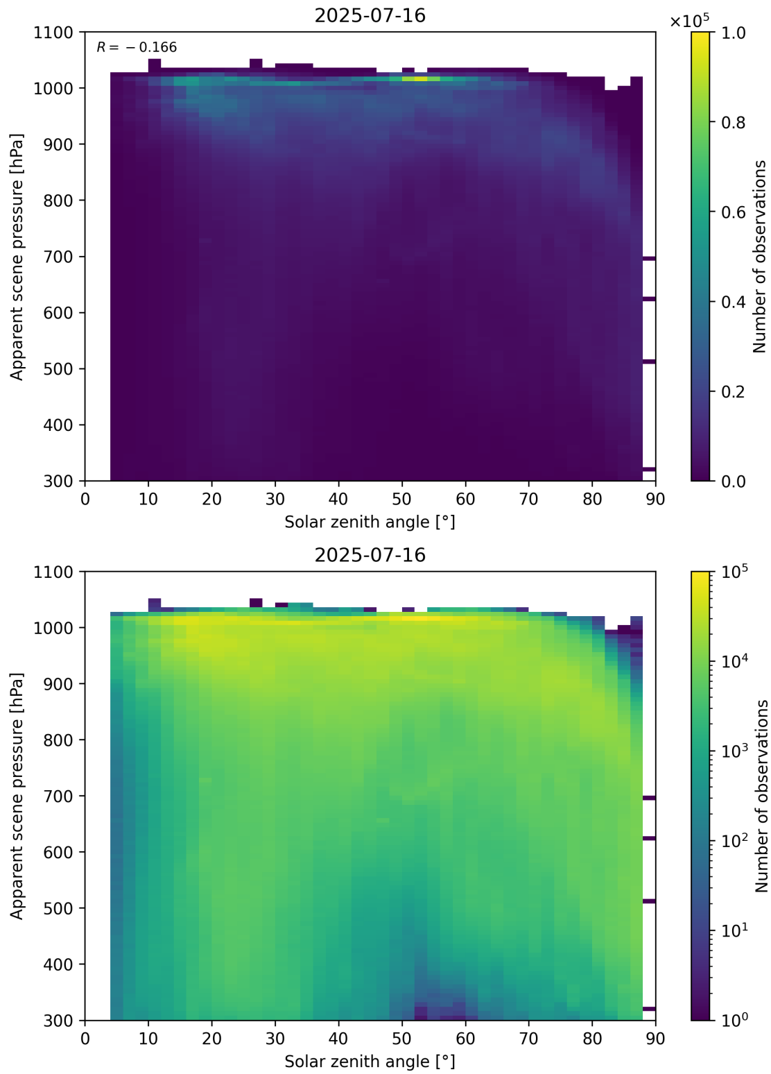
Figure 108: Scatter density plot of “Solar zenith angle” against “Apparent scene pressure” for 2025-07-15 to 2025-07-17.
