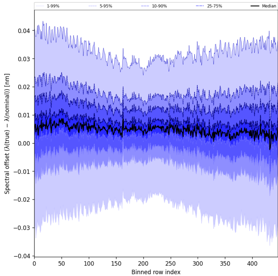
Figure 62: Along track statistics of “Spectral offset ( \lambda_{\text{true}} - \lambda_{\text{nominal}} )” for 2025-07-15 to 2025-07-17
