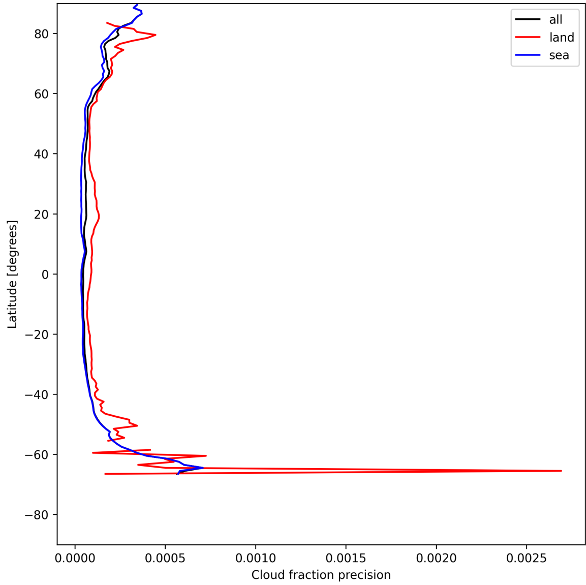
Figure 16: Zonal average of “Cloud fraction precision” for 2025-07-15 to 2025-07-17.
