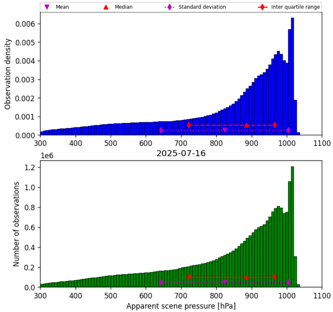
Figure 36: Histogram of “Apparent scene pressure” for 2025-07-15 to 2025-07-17
