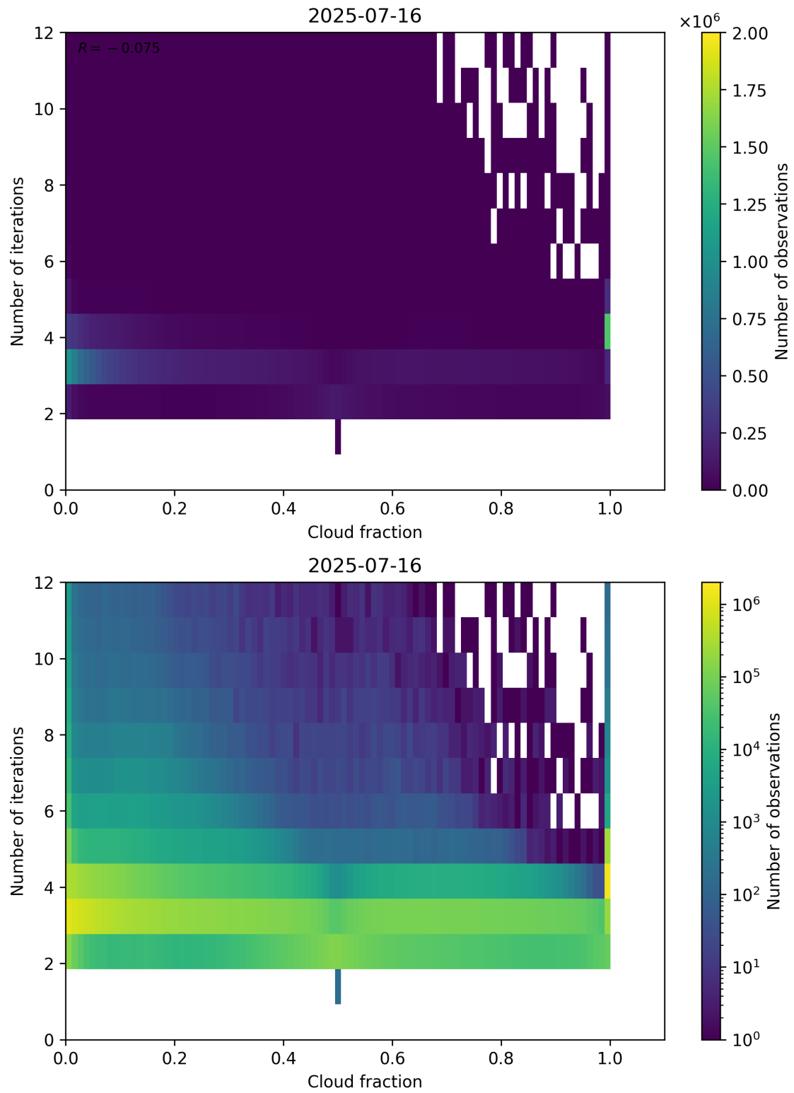
Figure 73: Scatter density plot of “Cloud fraction” against “Number of iterations” for 2025-07-15 to 2025-07-17.
