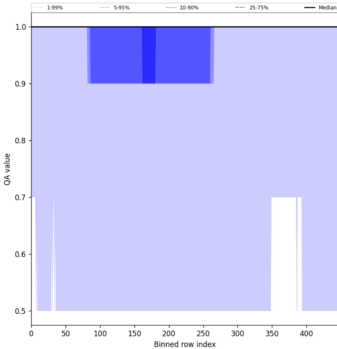
Figure 46: Along track statistics of “QA value” for 2025-07-15 to 2025-07-17
