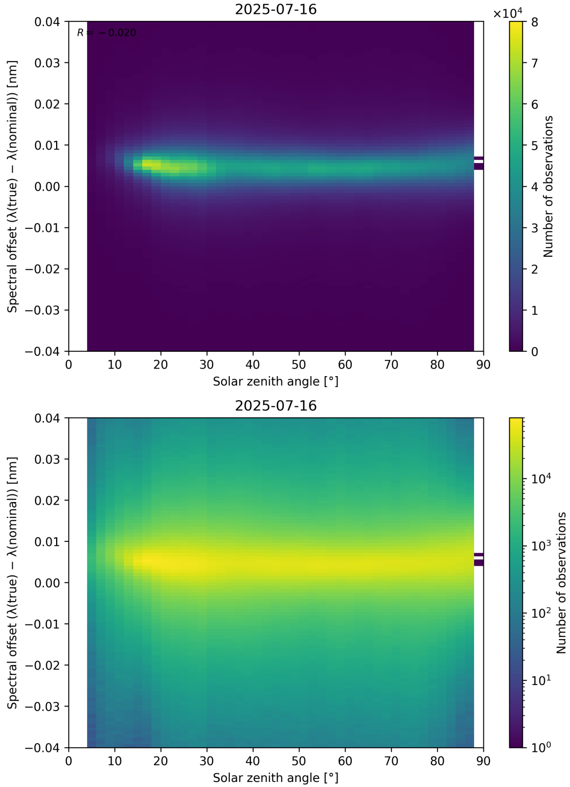
Figure 117: Scatter density plot of “Solar zenith angle” against “Spectral offset ( \lambda_{\text{true}} - \lambda_{\text{nominal}} )” for 2025-07-15 to 2025-07-17.
