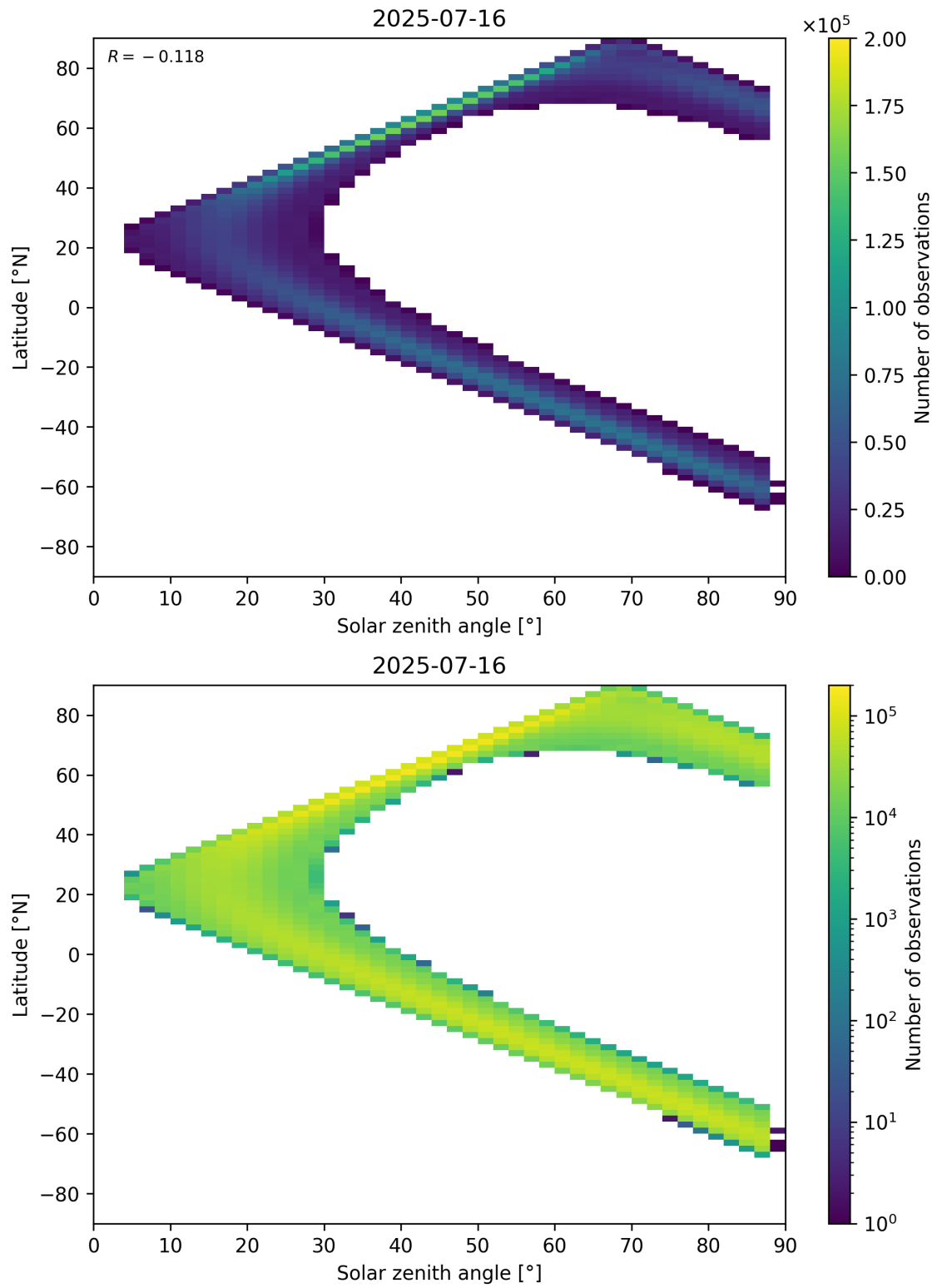
Figure 113: Scatter density plot of “Solar zenith angle” against “Latitude” for 2025-07-15 to 2025-07-17.
