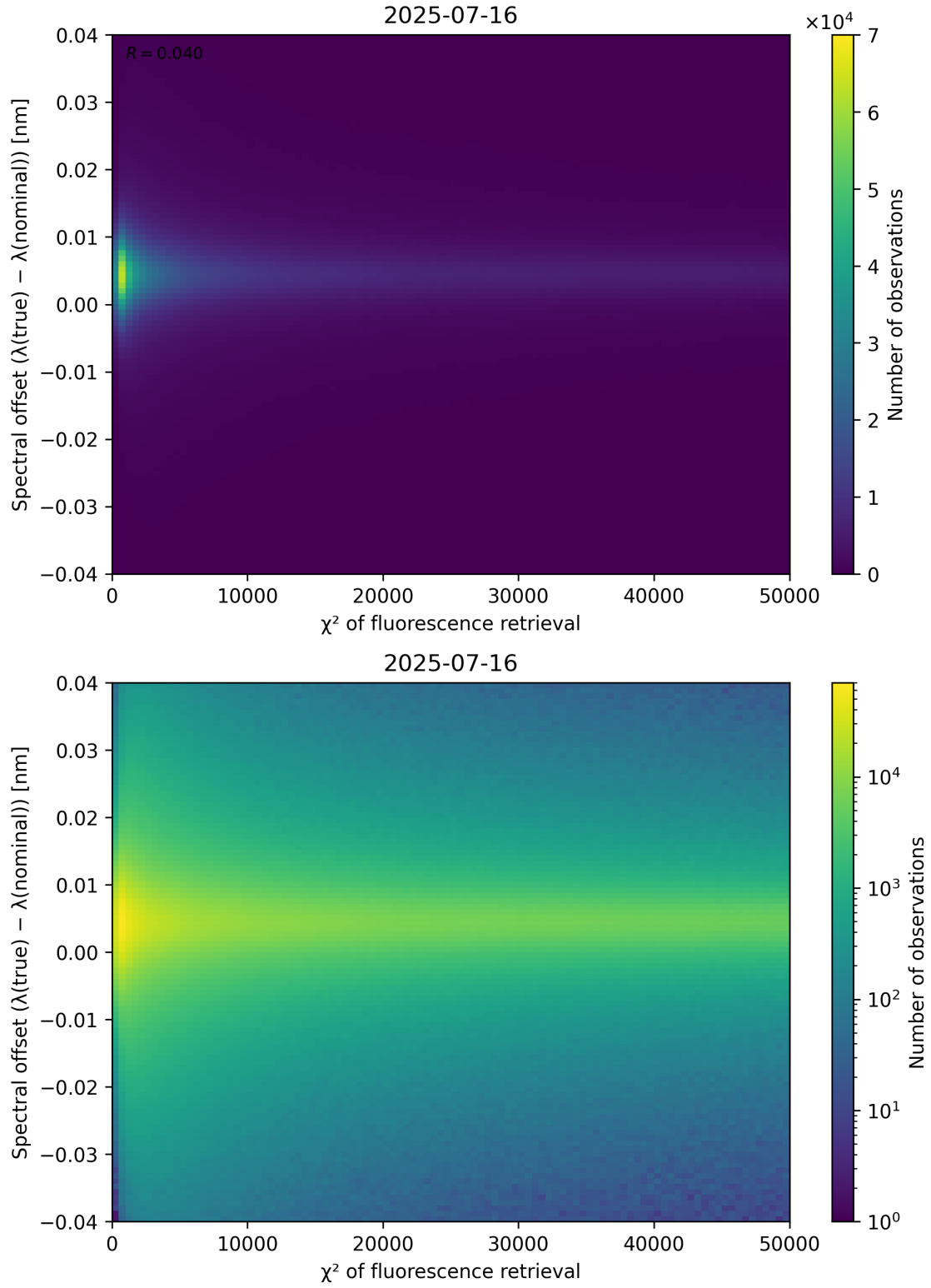
Figure 69: Scatter density plot of “ \chi^2 of fluorescence retrieval” against “Spectral offset ( \lambda_{\text{true}} - \lambda_{\text{nominal}} )” for 2025-07-15 to 2025-07-17.
