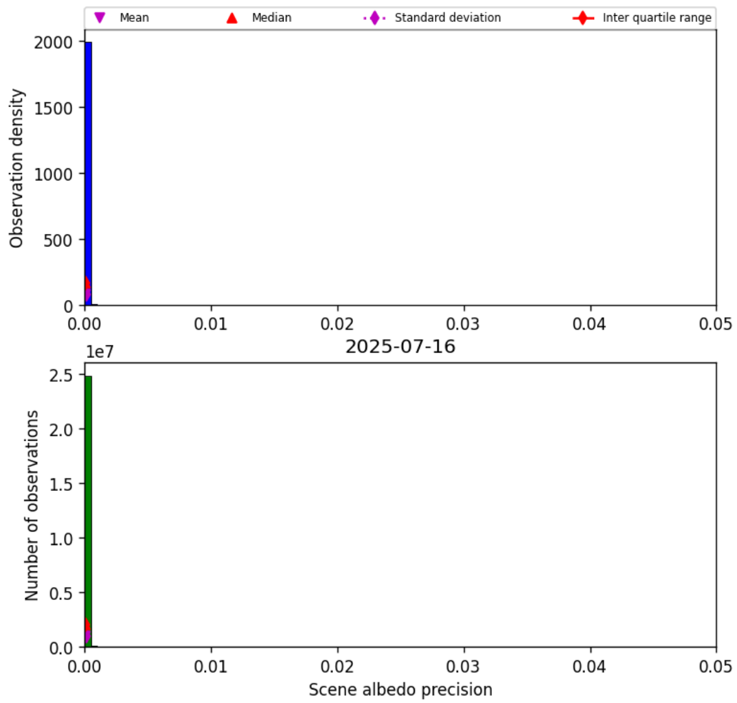
Figure 35: Histogram of “Scene albedo precision” for 2025-07-15 to 2025-07-17
