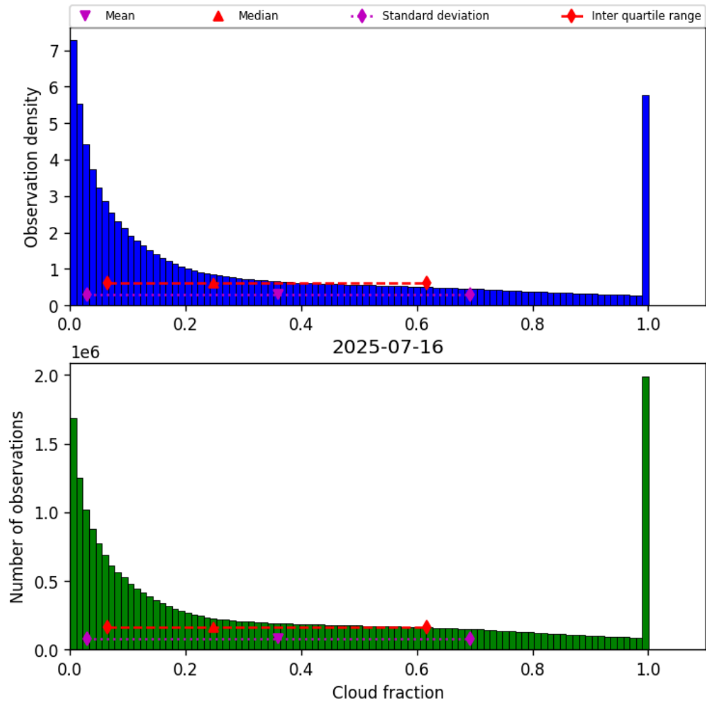
Figure 32: Histogram of “Cloud fraction” for 2025-07-15 to 2025-07-17
