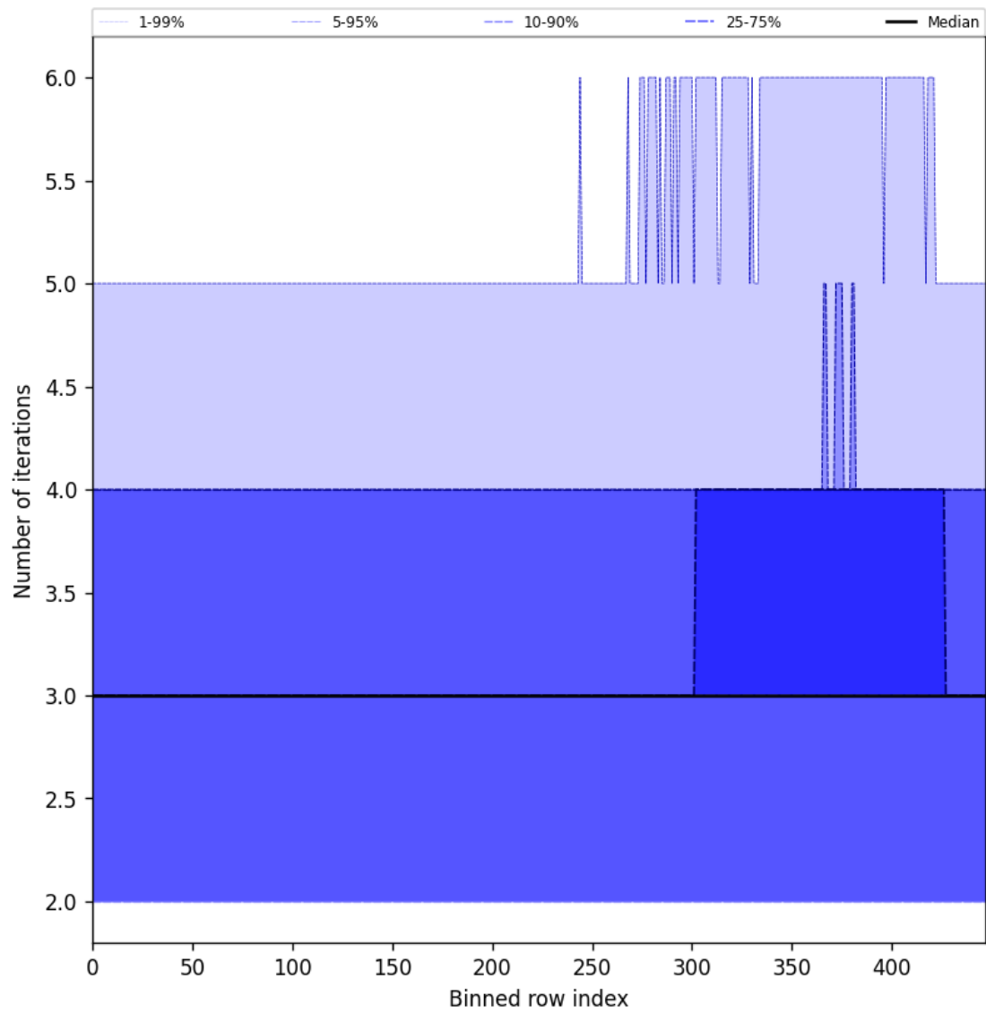
Figure 56: Along track statistics of “Number of iterations” for 2025-07-15 to 2025-07-17
