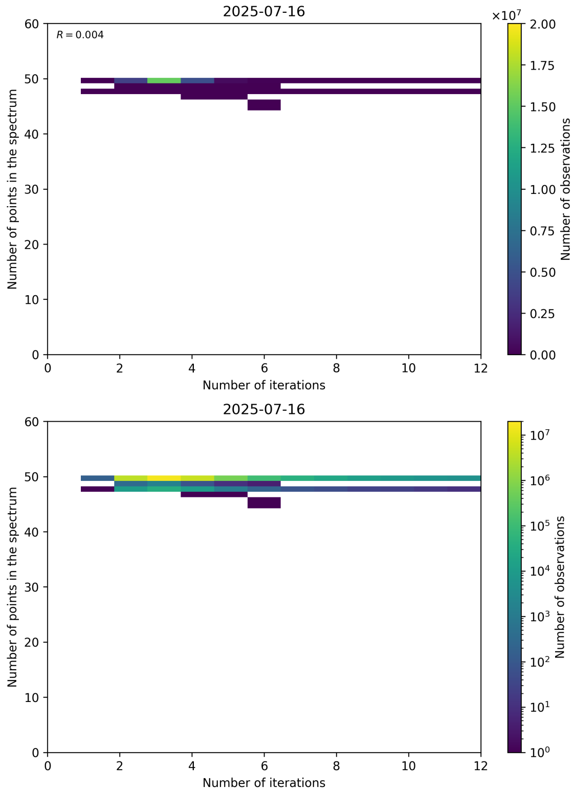
Figure 99: Scatter density plot of “Number of iterations” against “Number of points in the spectrum” for 2025-07-15 to 2025-07-17.
