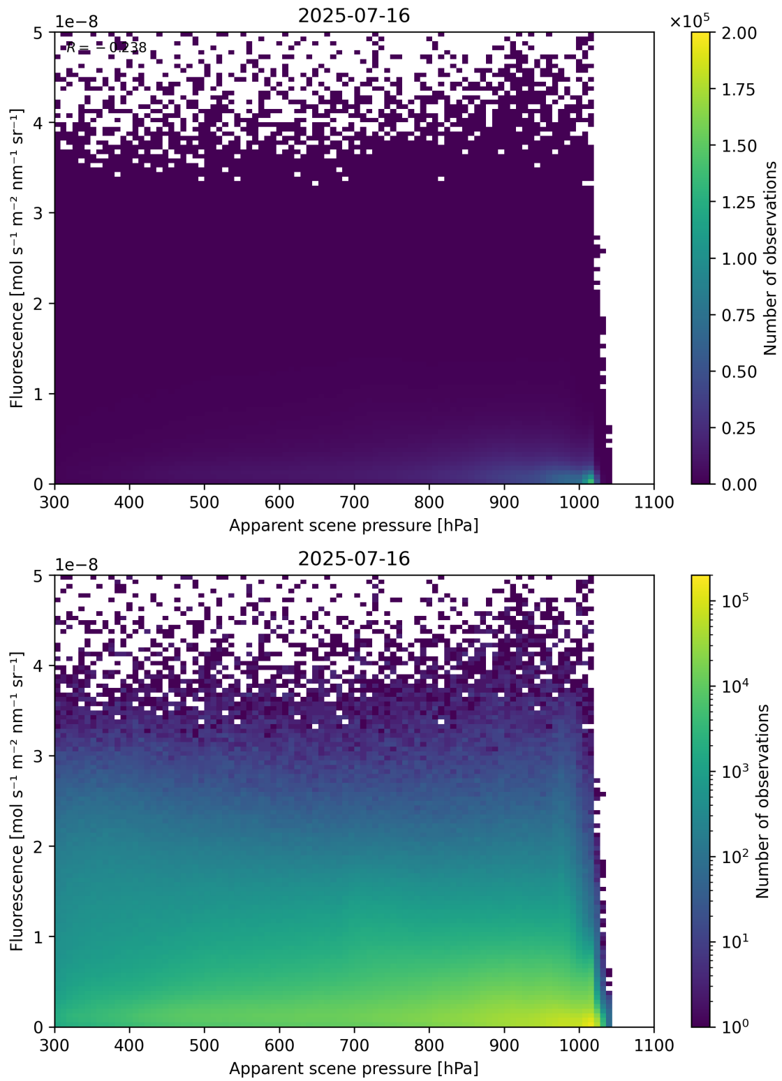
Figure 64: Scatter density plot of “Apparent scene pressure” against “Fluorescence” for 2025-07-15 to 2025-07-17.
