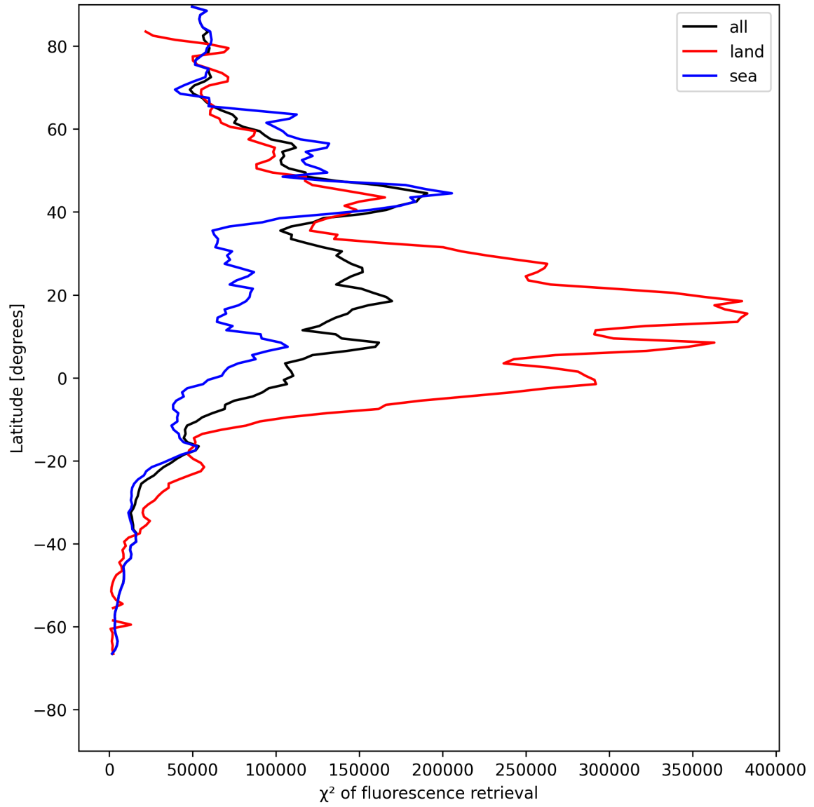
Figure 25: Zonal average of “ \chi^2 of fluorescence retrieval” for 2025-07-15 to 2025-07-17.
