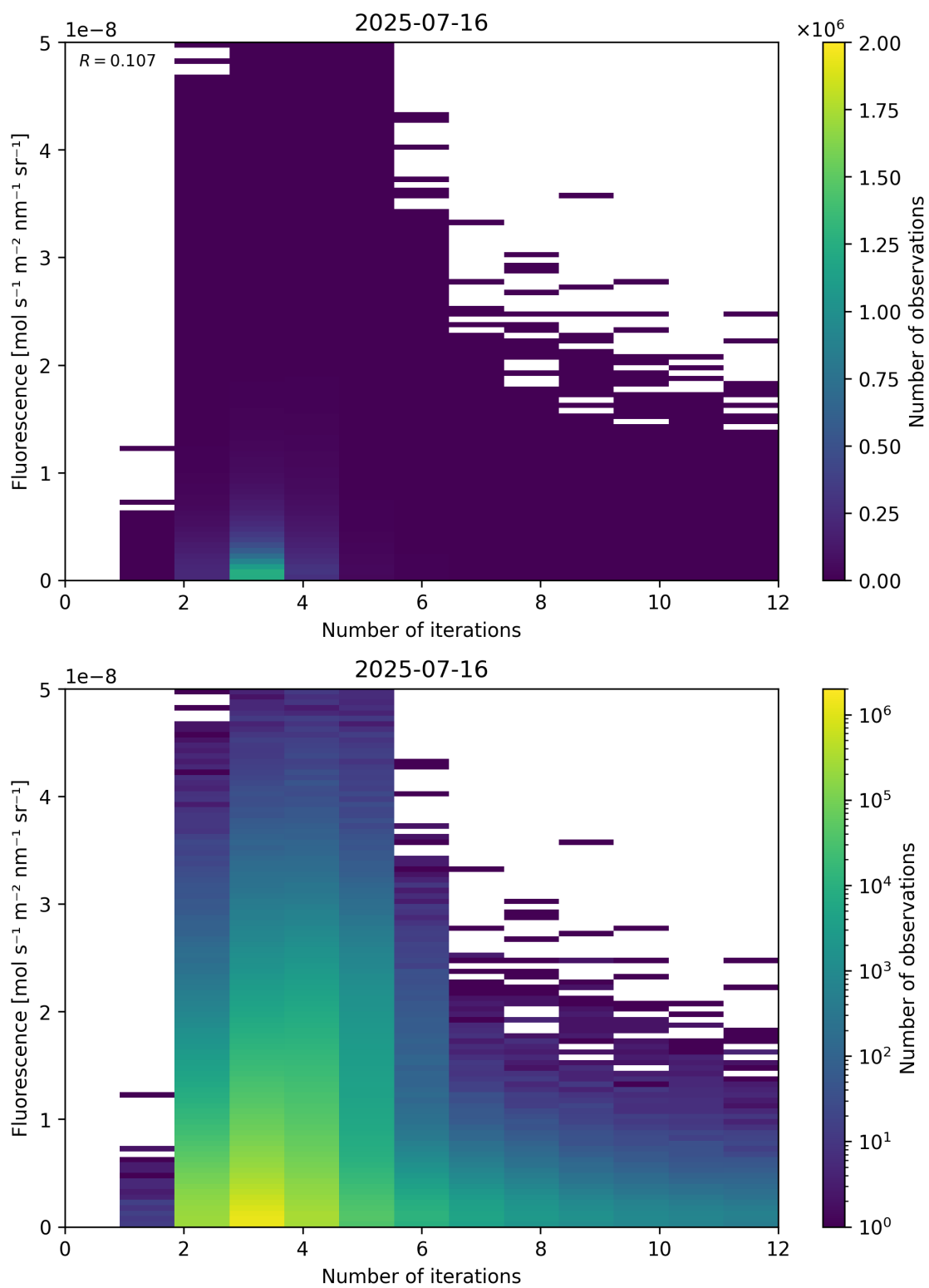
Figure 98: Scatter density plot of “Number of iterations” against “Fluorescence” for 2025-07-15 to 2025-07-17.
