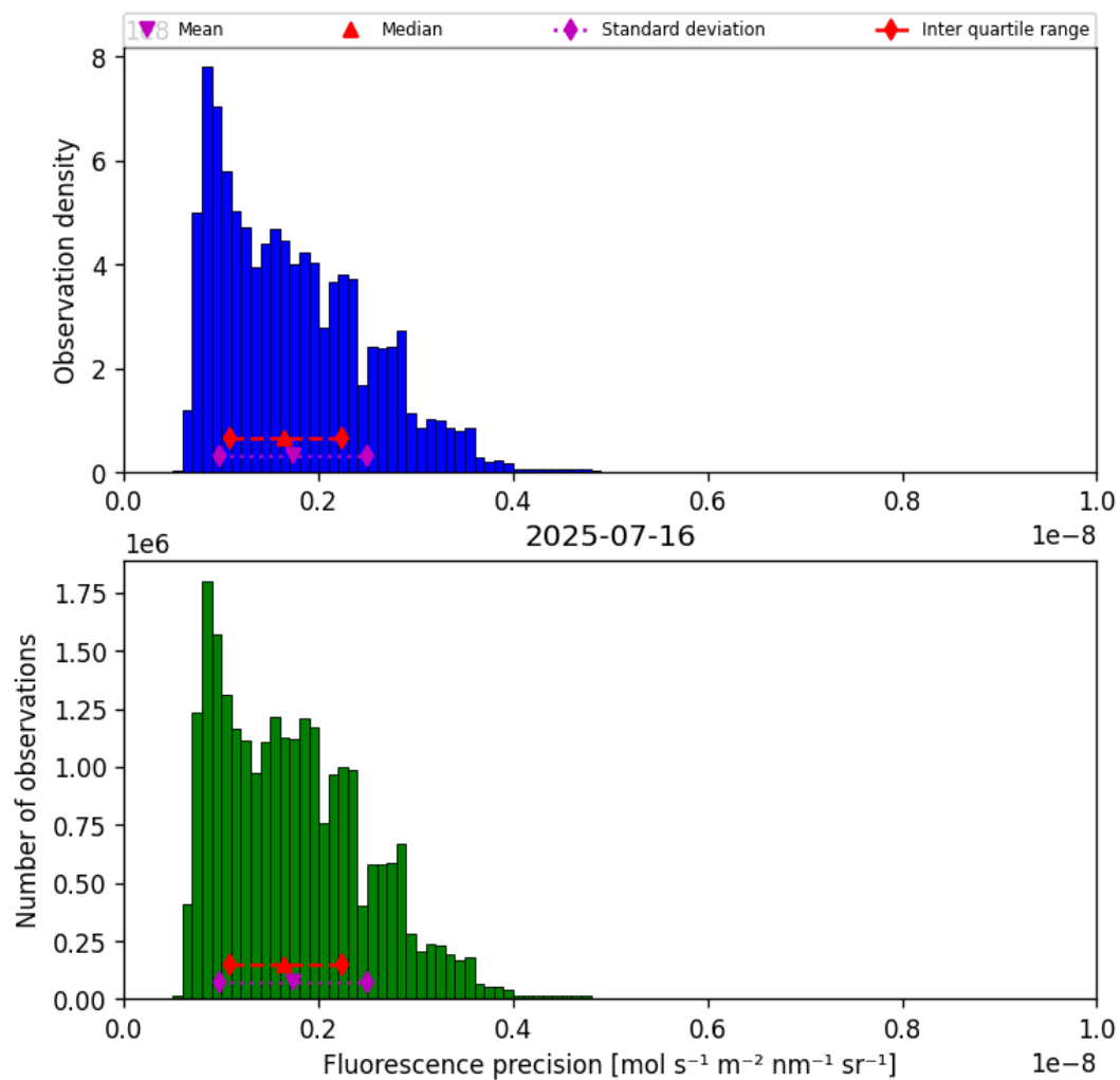
Figure 41: Histogram of “Fluorescence precision” for 2025-07-15 to 2025-07-17
