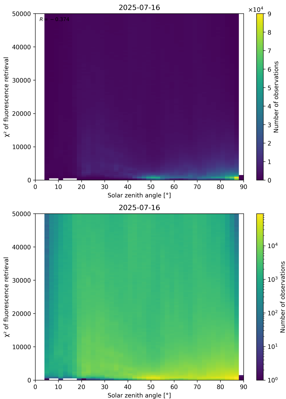
Figure 109: Scatter density plot of “Solar zenith angle” against “ \chi^2 of fluorescence retrieval” for 2025-07-15 to 2025-07-17.
