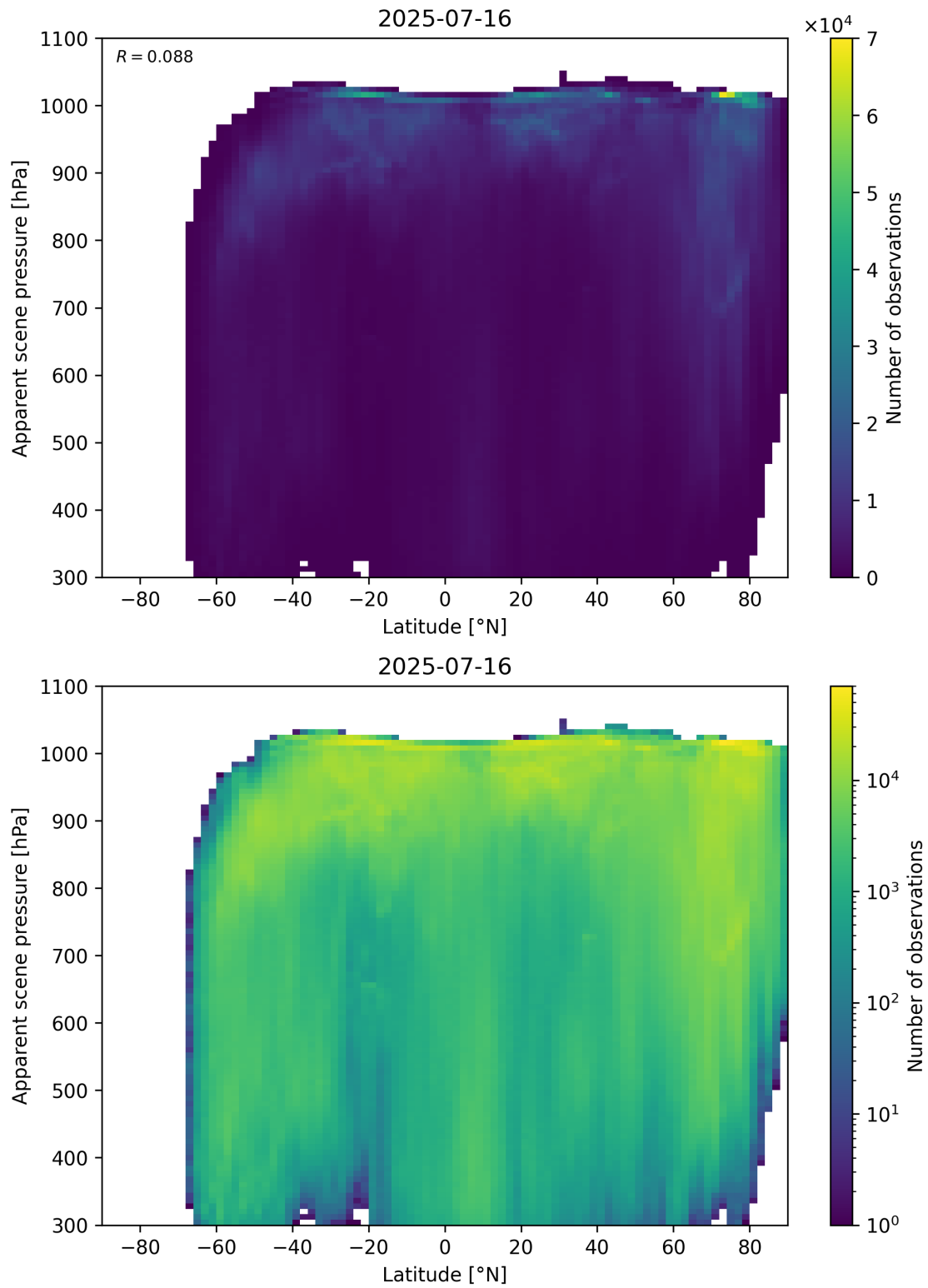
Figure 88: Scatter density plot of “Latitude” against “Apparent scene pressure” for 2025-07-15 to 2025-07-17.
