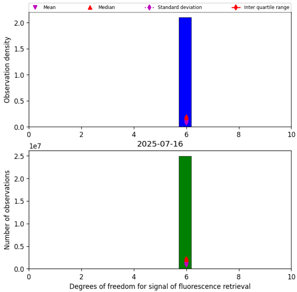
Figure 43: Histogram of "Degrees of freedom for signal of fluorescence retrieval" for 2025-07-15 to 2025-07-17
