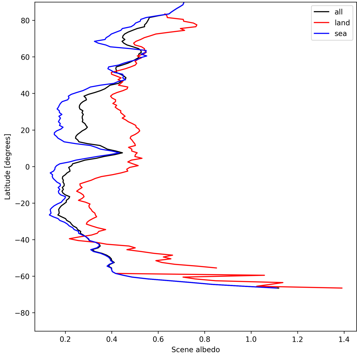
Figure 17: Zonal average of “Scene albedo” for 2025-07-15 to 2025-07-17.
