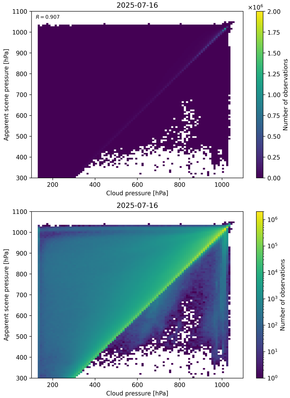
Figure 77: Scatter density plot of “Cloud pressure” against “Apparent scene pressure” for 2025-07-15 to 2025-07-17.
