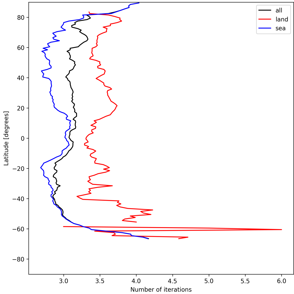
Figure 22: Zonal average of “Number of iterations” for 2025-07-15 to 2025-07-17.
