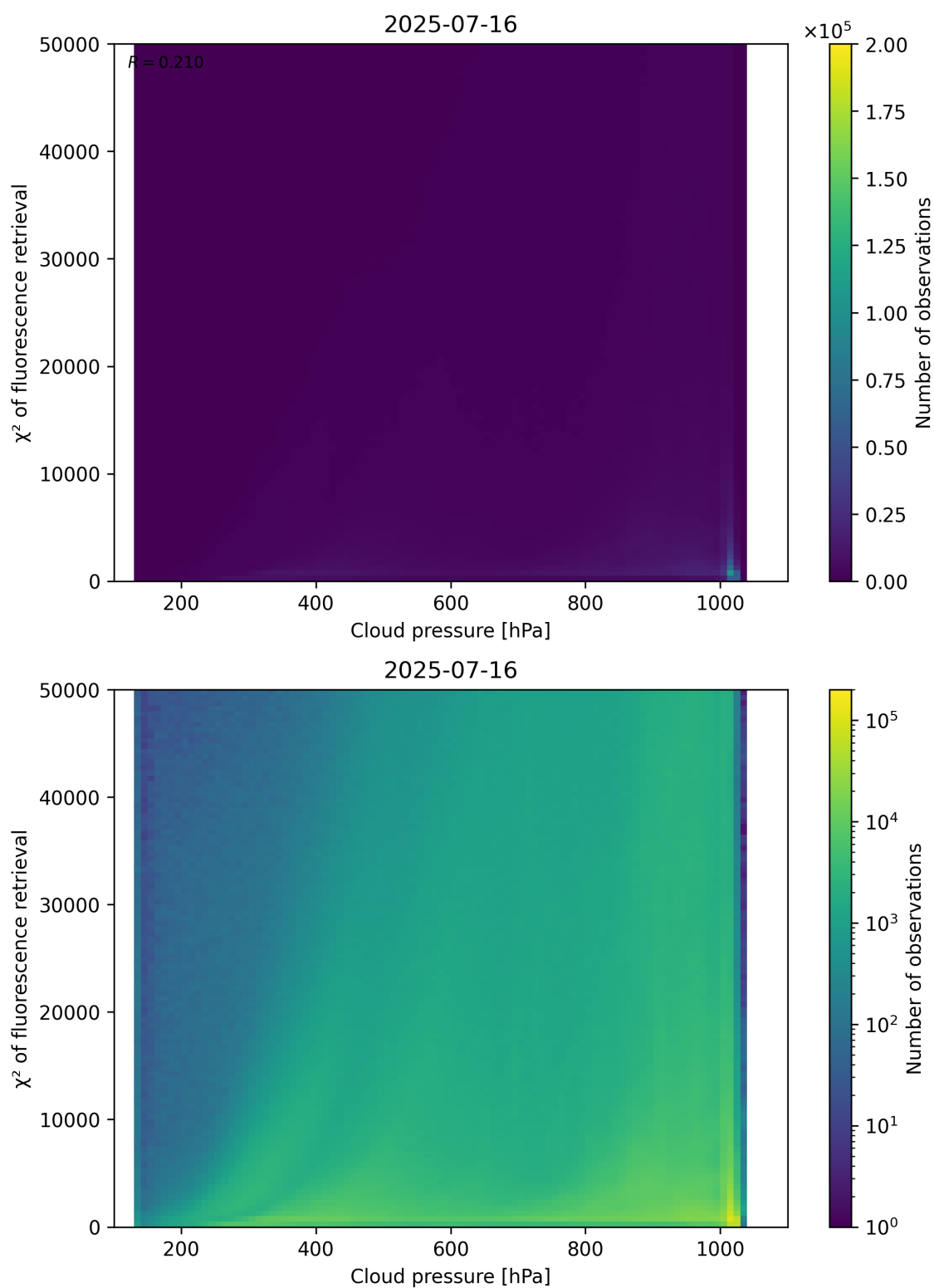
Figure 78: Scatter density plot of “Cloud pressure” against “ \chi^2 of fluorescence retrieval” for 2025-07-15 to 2025-07-17.
