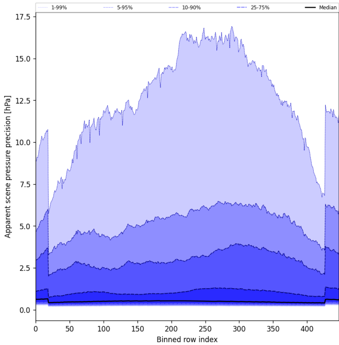
Figure 54: Along track statistics of “Apparent scene pressure precision” for 2025-07-15 to 2025-07-17
