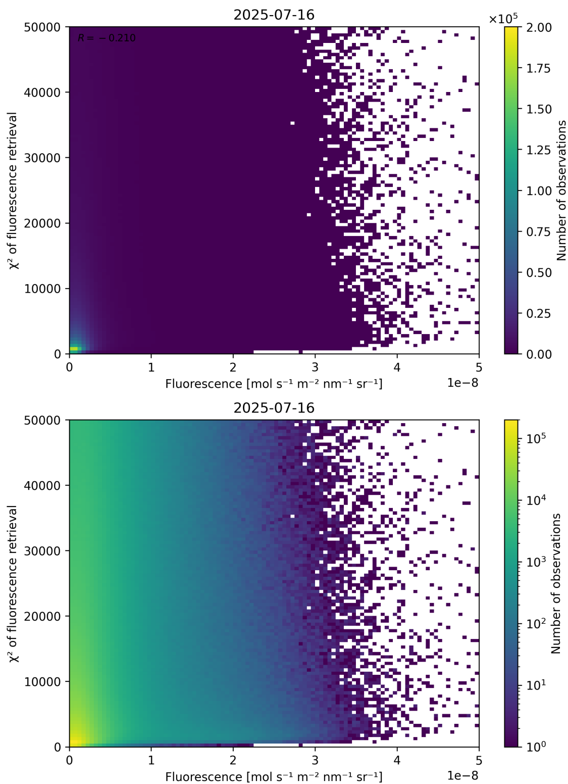
Figure 85: Scatter density plot of “Fluorescence” against “ \chi^2 of fluorescence retrieval” for 2025-07-15 to 2025-07-17.
