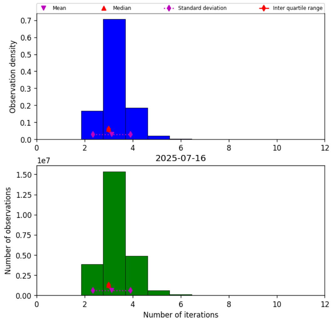
Figure 39: Histogram of “Number of iterations” for 2025-07-15 to 2025-07-17
