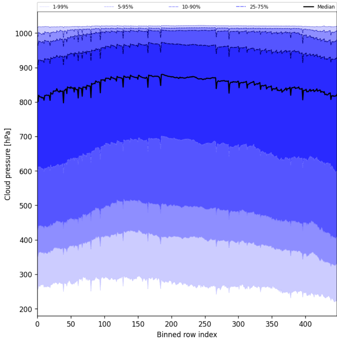
Figure 47: Along track statistics of “Cloud pressure” for 2025-07-15 to 2025-07-17
