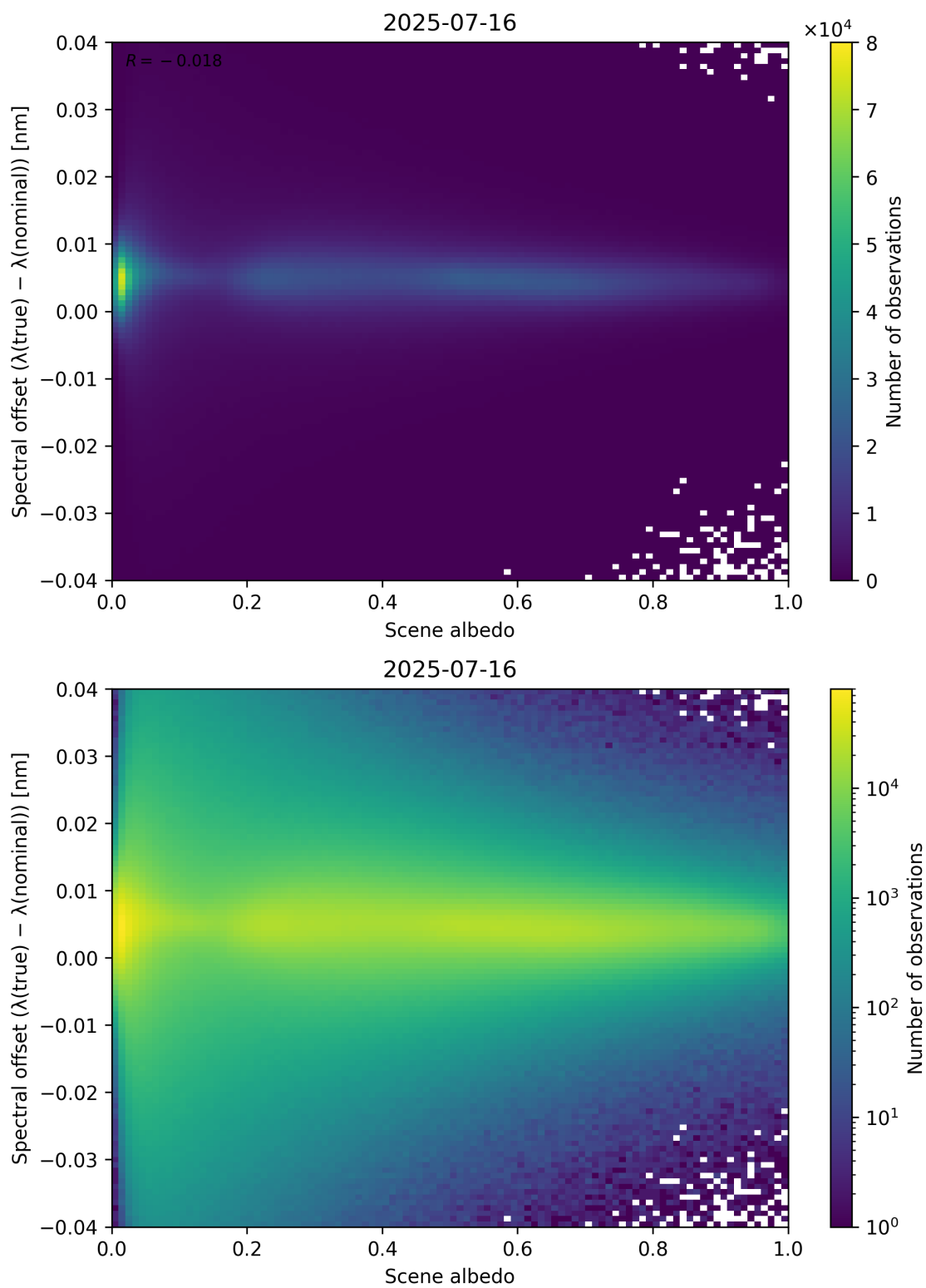
Figure 107: Scatter density plot of “Scene albedo” against “Spectral offset ( \lambda_{\text{true}} - \lambda_{\text{nominal}} )” for 2025-07-15 to 2025-07-17.
