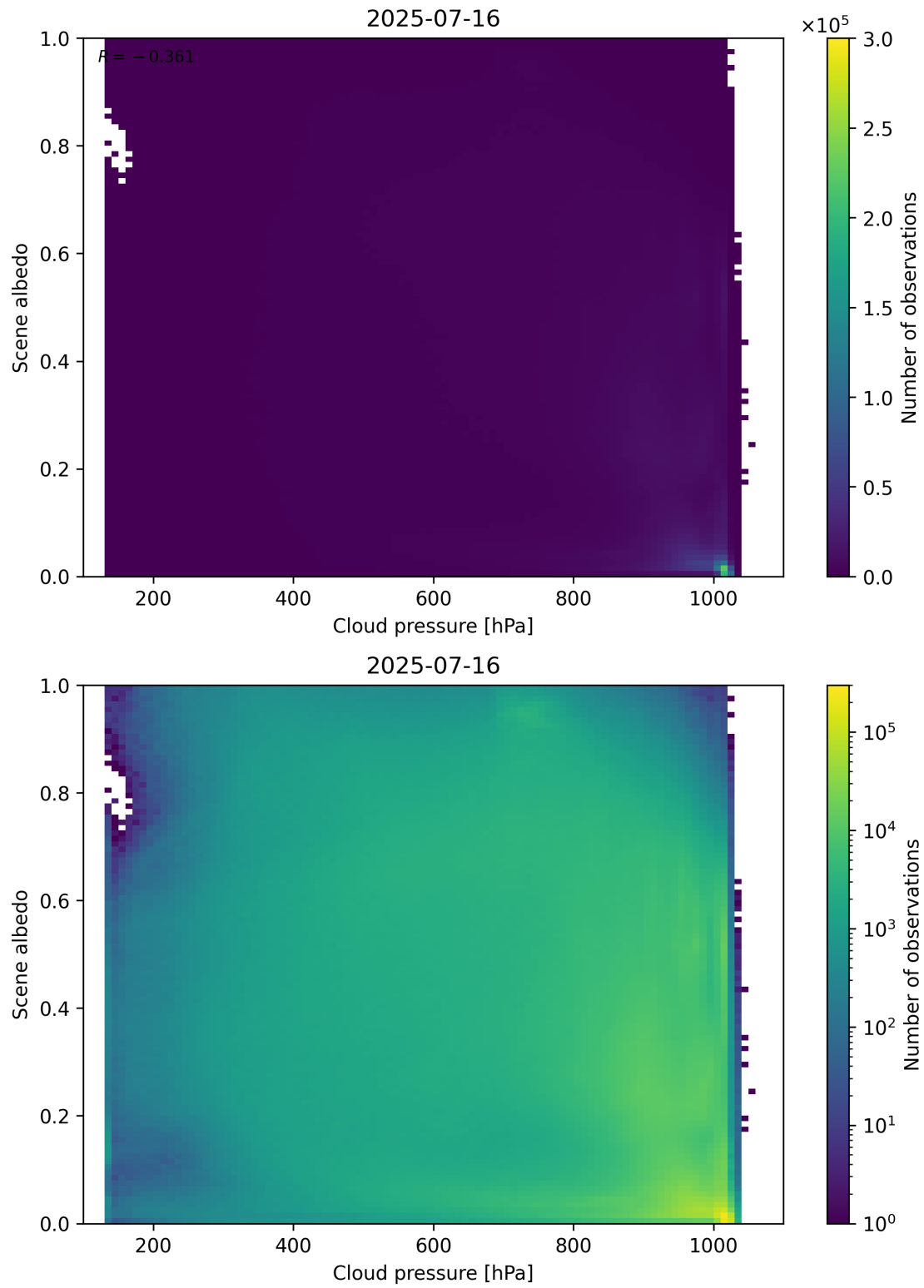
Figure 83: Scatter density plot of “Cloud pressure” against “Scene albedo” for 2025-07-15 to 2025-07-17.
