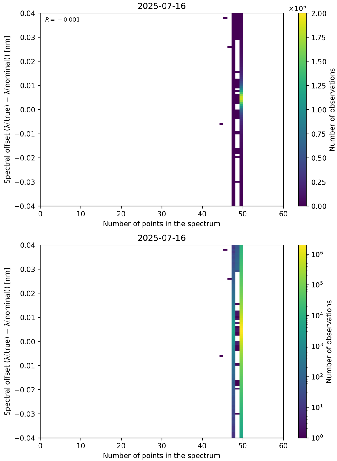
Figure 101: Scatter density plot of “Number of points in the spectrum” against “Spectral offset ( \lambda_{\text{true}} - \lambda_{\text{nominal}} )” for 2025-07-15 to 2025-07-17.
