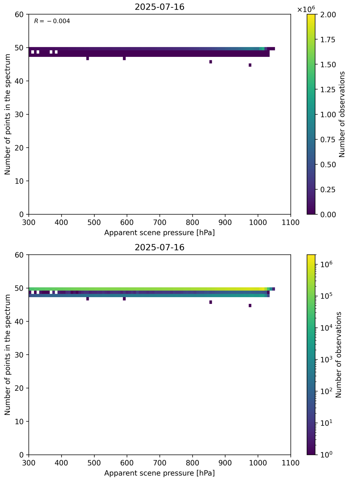
Figure 66: Scatter density plot of “Apparent scene pressure” against “Number of points in the spectrum” for 2025-07-15 to 2025-07-17.
