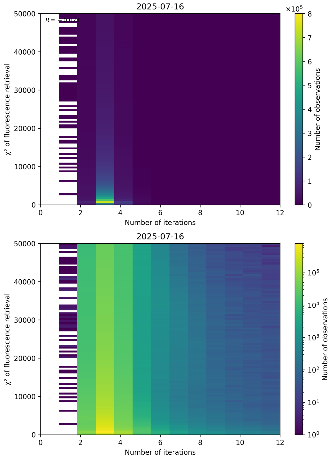
Figure 97: Scatter density plot of “Number of iterations” against “ \chi^2 of fluorescence retrieval” for 2025-07-15 to 2025-07-17.
