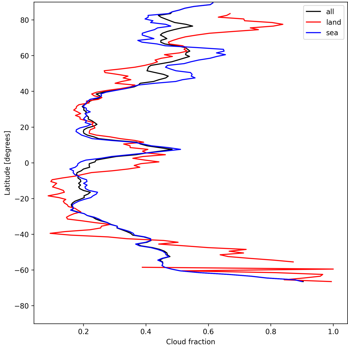
Figure 15: Zonal average of “Cloud fraction” for 2025-07-15 to 2025-07-17.
