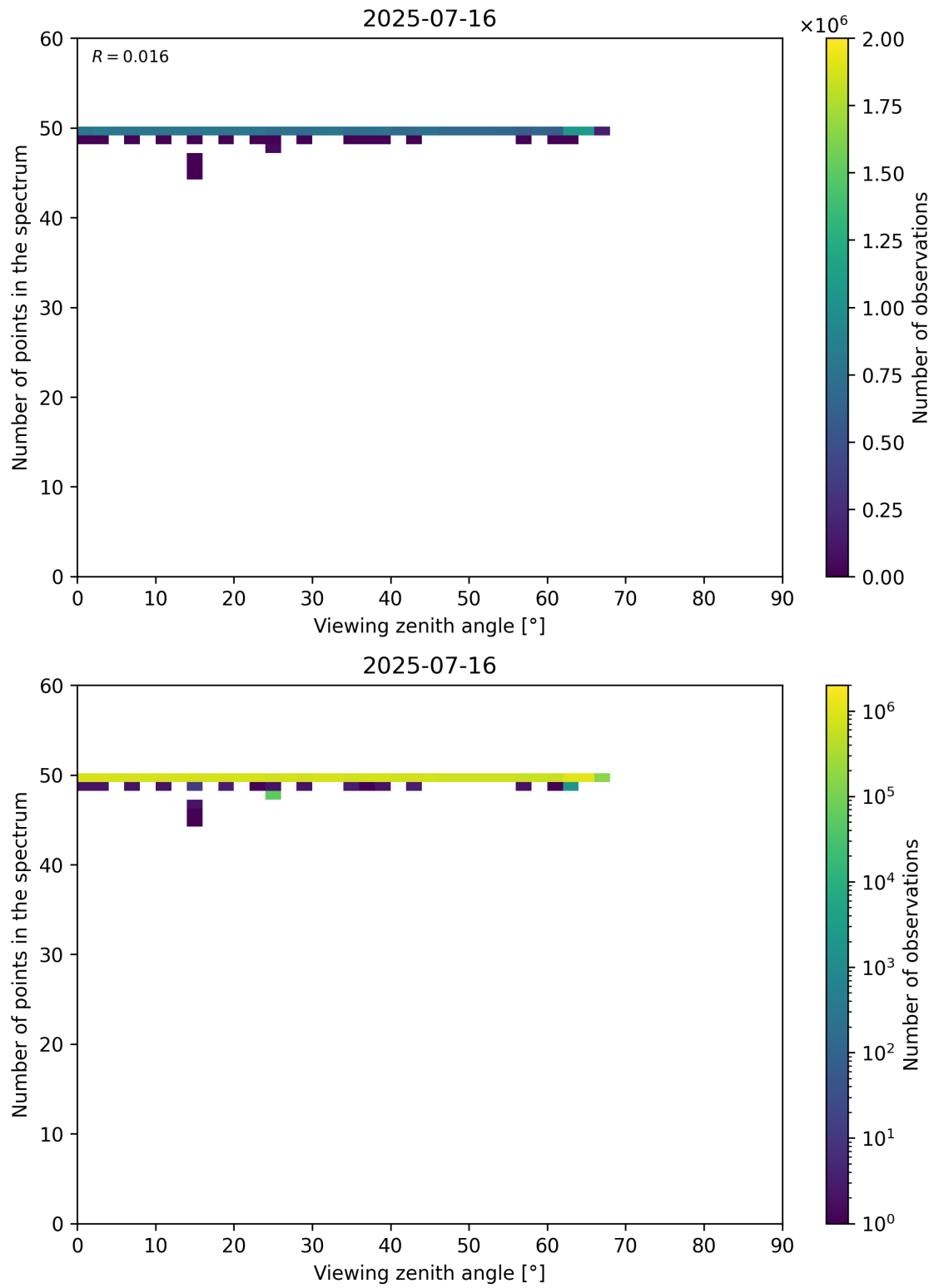
Figure 125: Scatter density plot of “Viewing zenith angle” against “Number of points in the spectrum” for 2025-07-15 to 2025-07-17.
