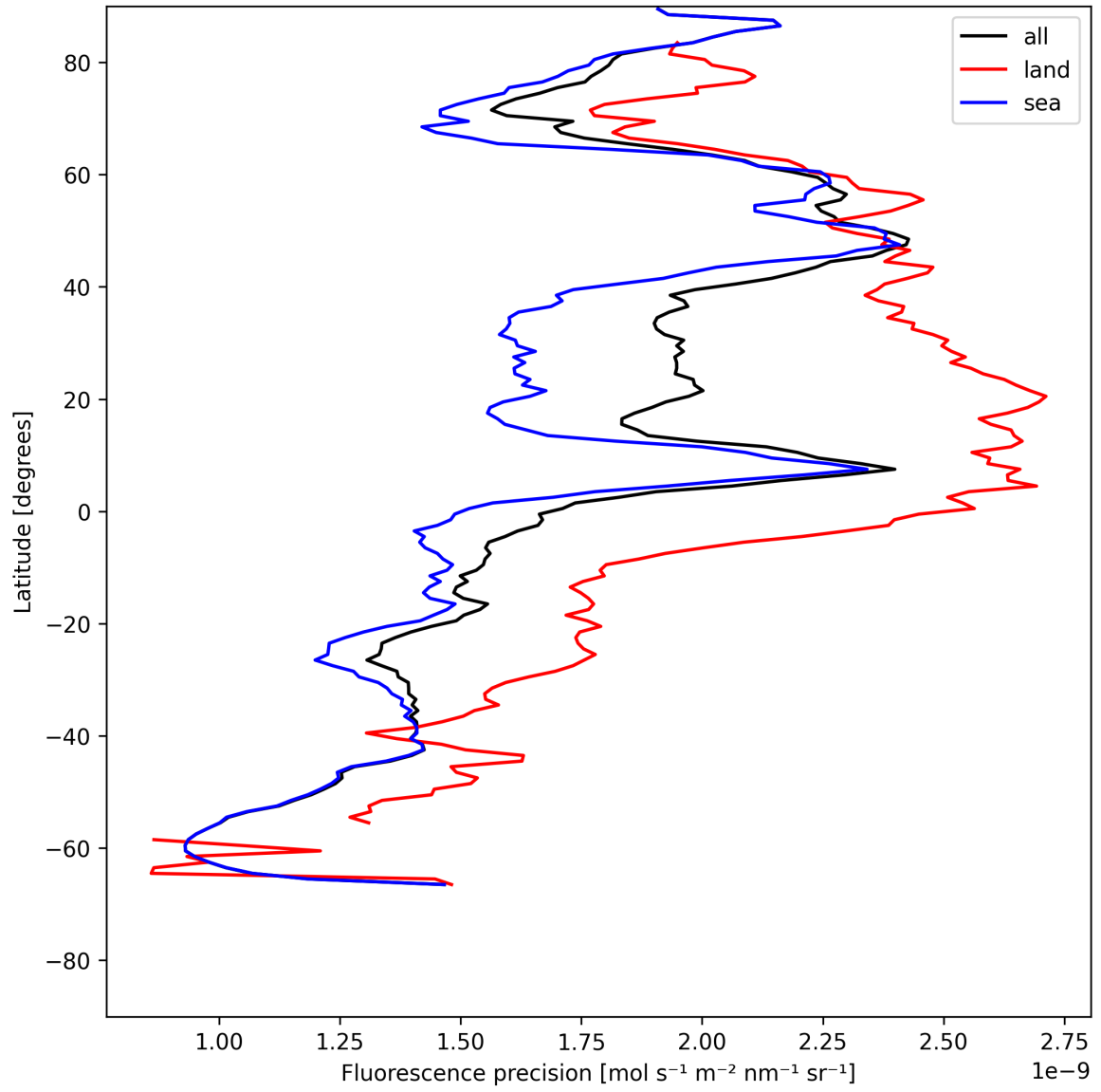
Figure 24: Zonal average of “Fluorescence precision” for 2025-07-15 to 2025-07-17.
