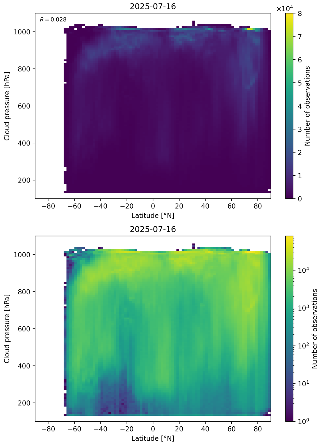
Figure 91: Scatter density plot of “Latitude” against “Cloud pressure” for 2025-07-15 to 2025-07-17.
