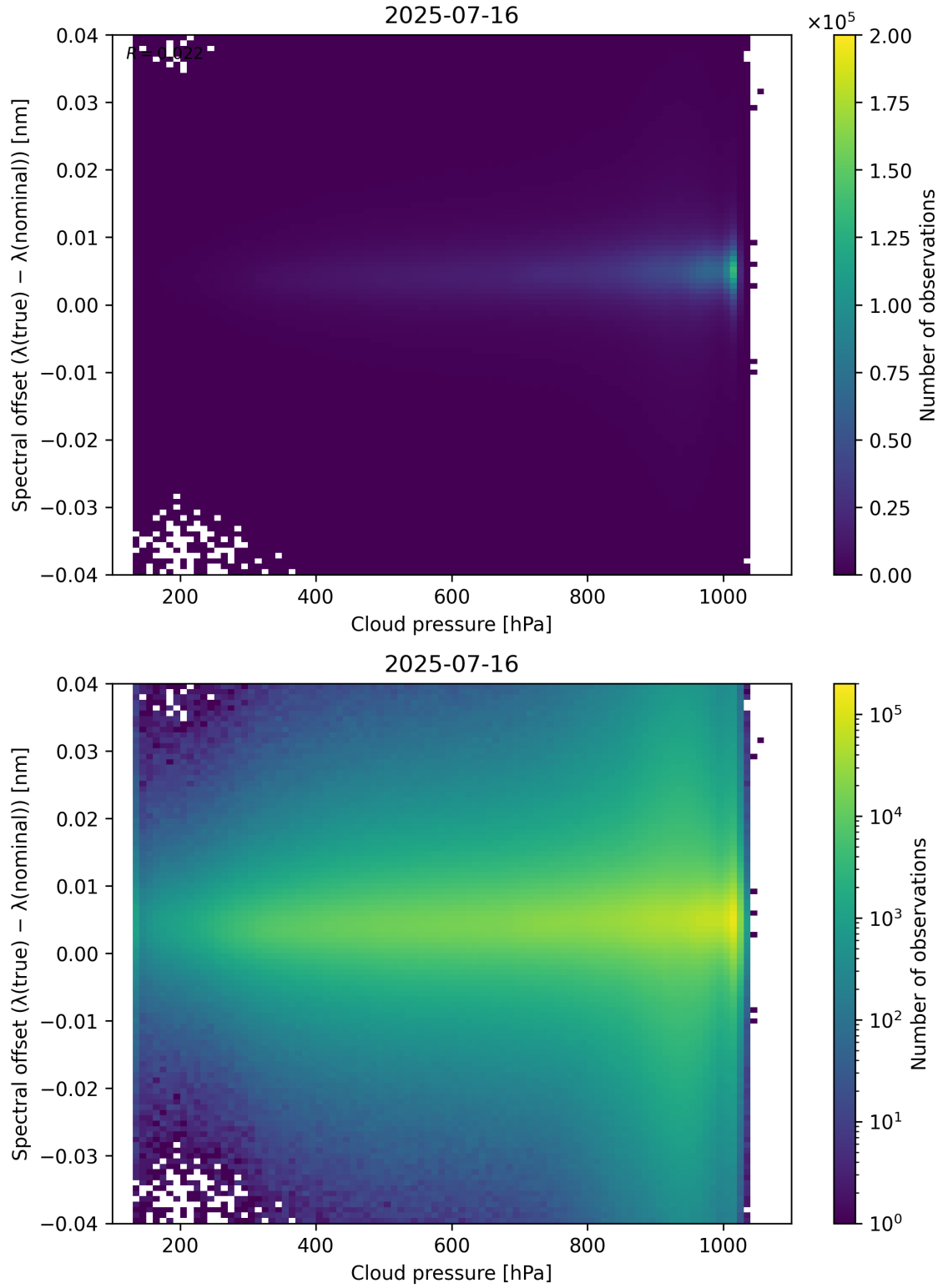
Figure 84: Scatter density plot of “Cloud pressure” against “Spectral offset ( \lambda_{\text{true}} - \lambda_{\text{nominal}} )” for 2025-07-15 to 2025-07-17.
