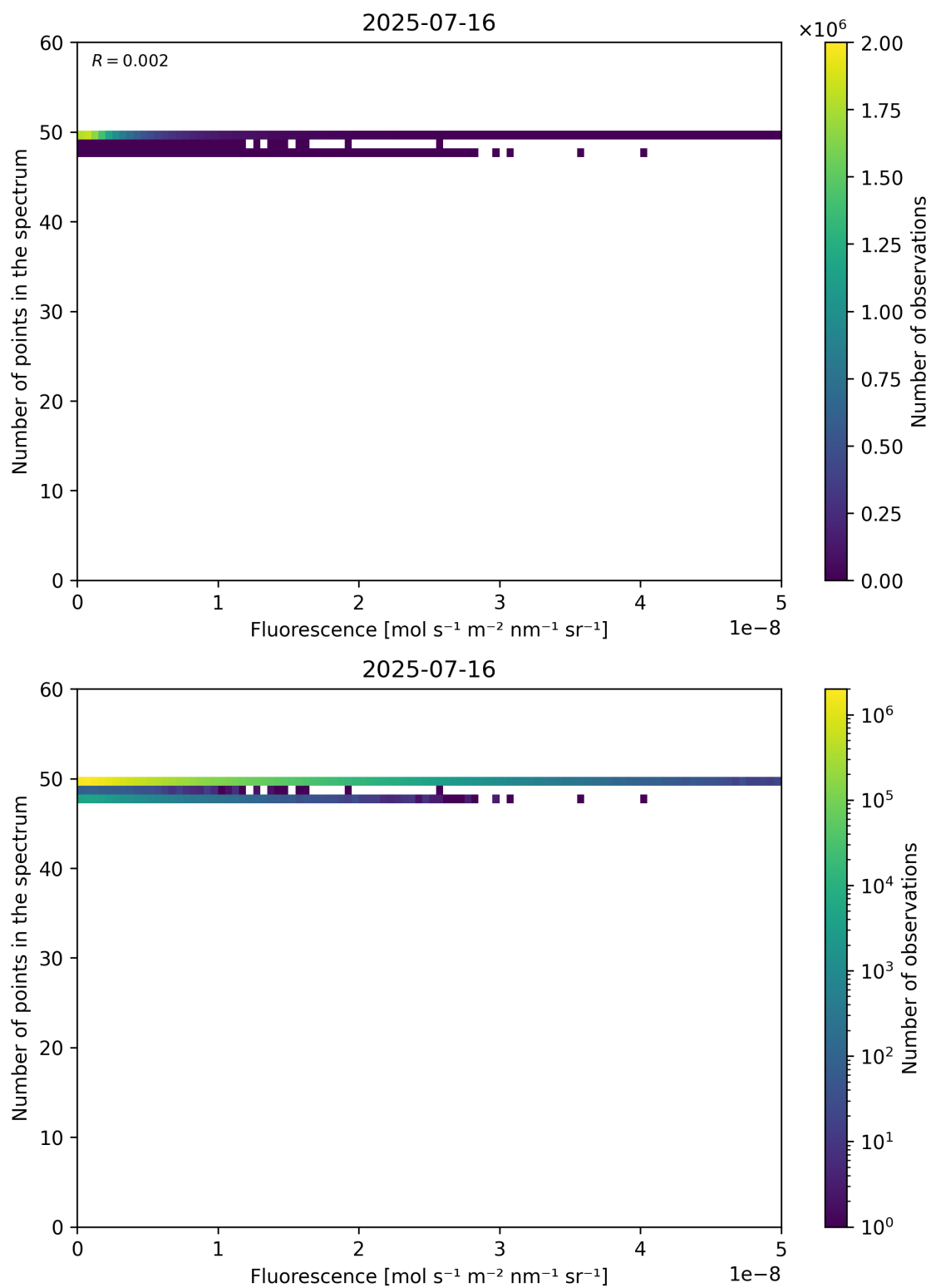
Figure 86: Scatter density plot of “Fluorescence” against “Number of points in the spectrum” for 2025-07-15 to 2025-07-17.
