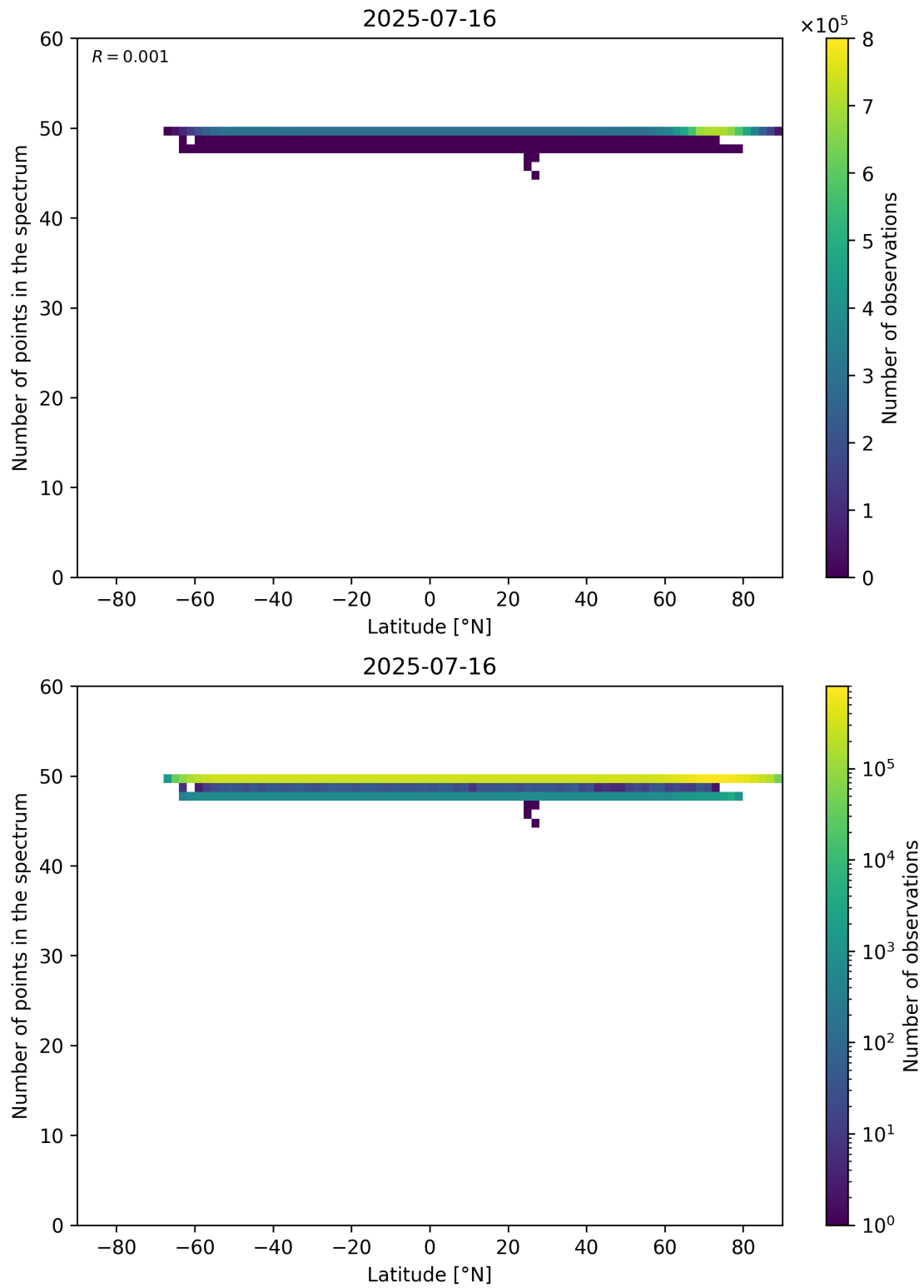
Figure 94: Scatter density plot of “Latitude” against “Number of points in the spectrum” for 2025-07-15 to 2025-07-17.
