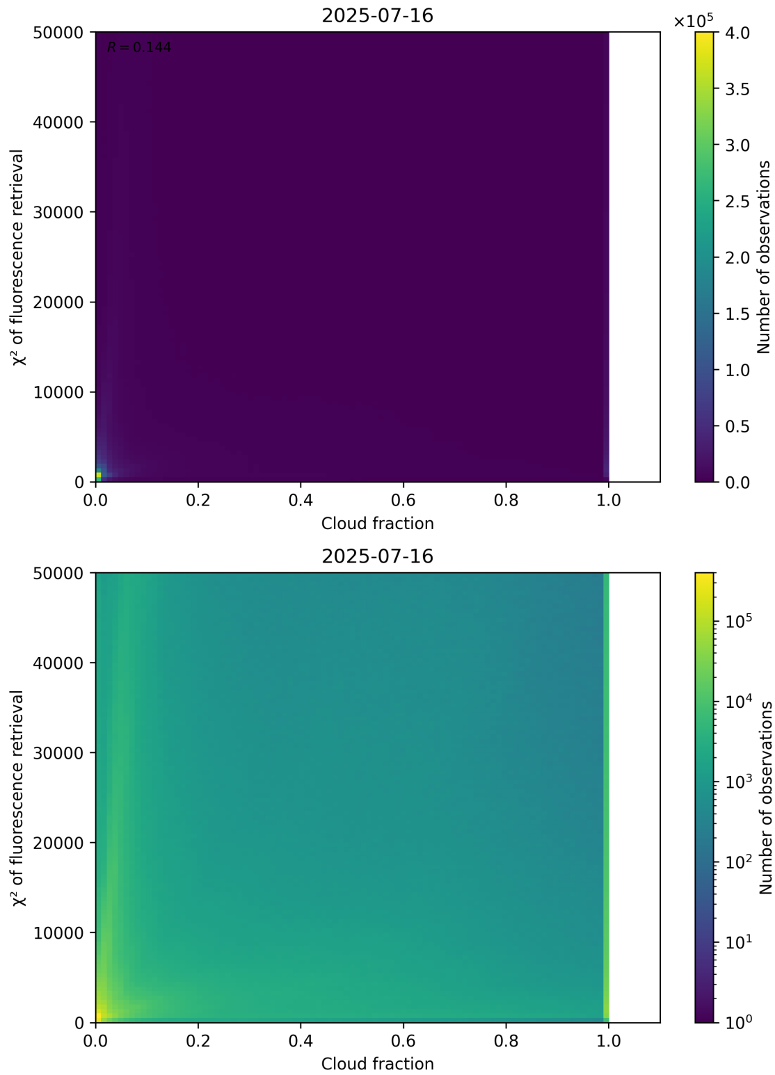
Figure 71: Scatter density plot of “Cloud fraction” against “ \chi^2 of fluorescence retrieval” for 2025-07-15 to 2025-07-17.
