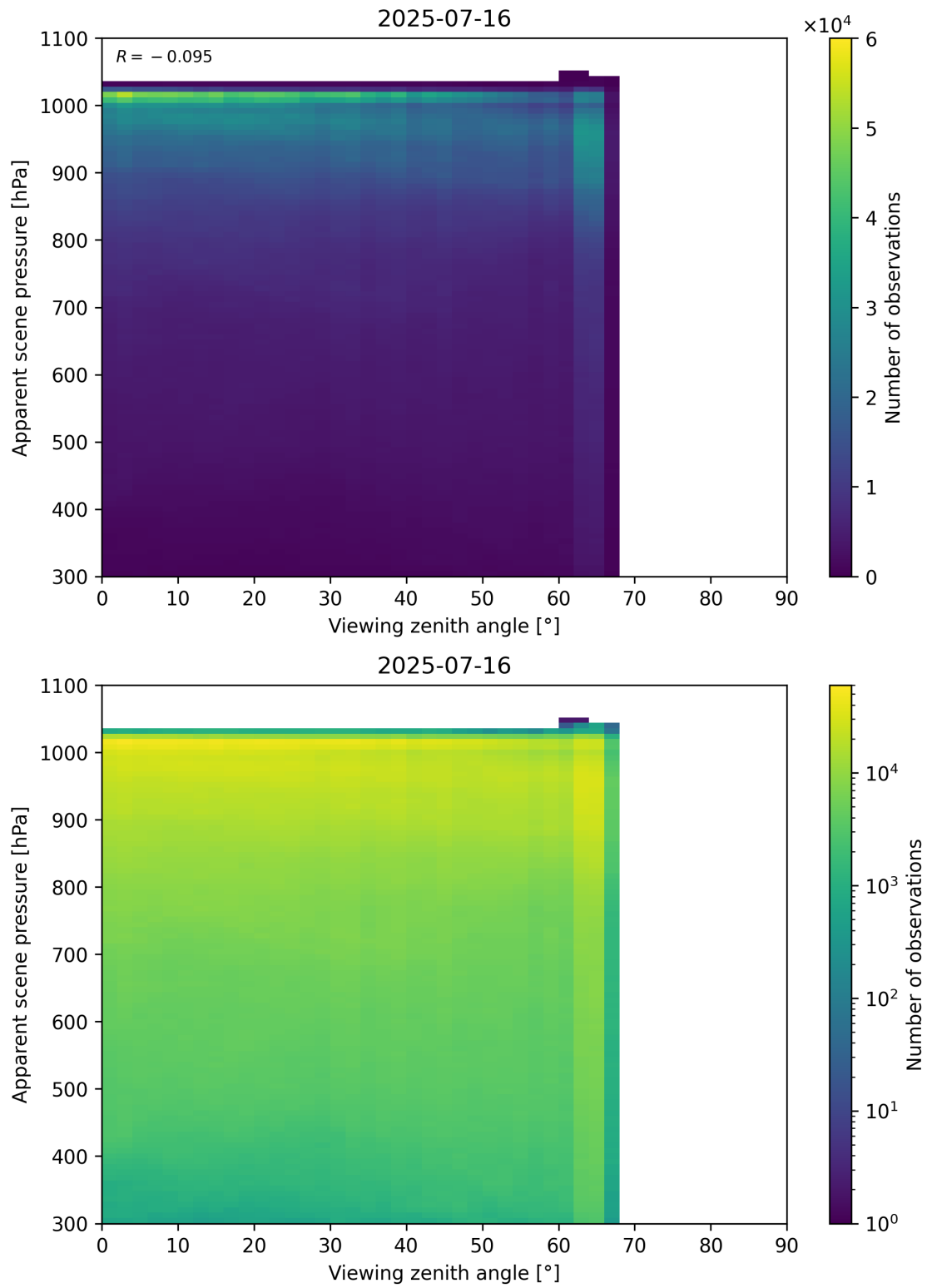
Figure 118: Scatter density plot of “Viewing zenith angle” against “Apparent scene pressure” for 2025-07-15 to 2025-07-17.
