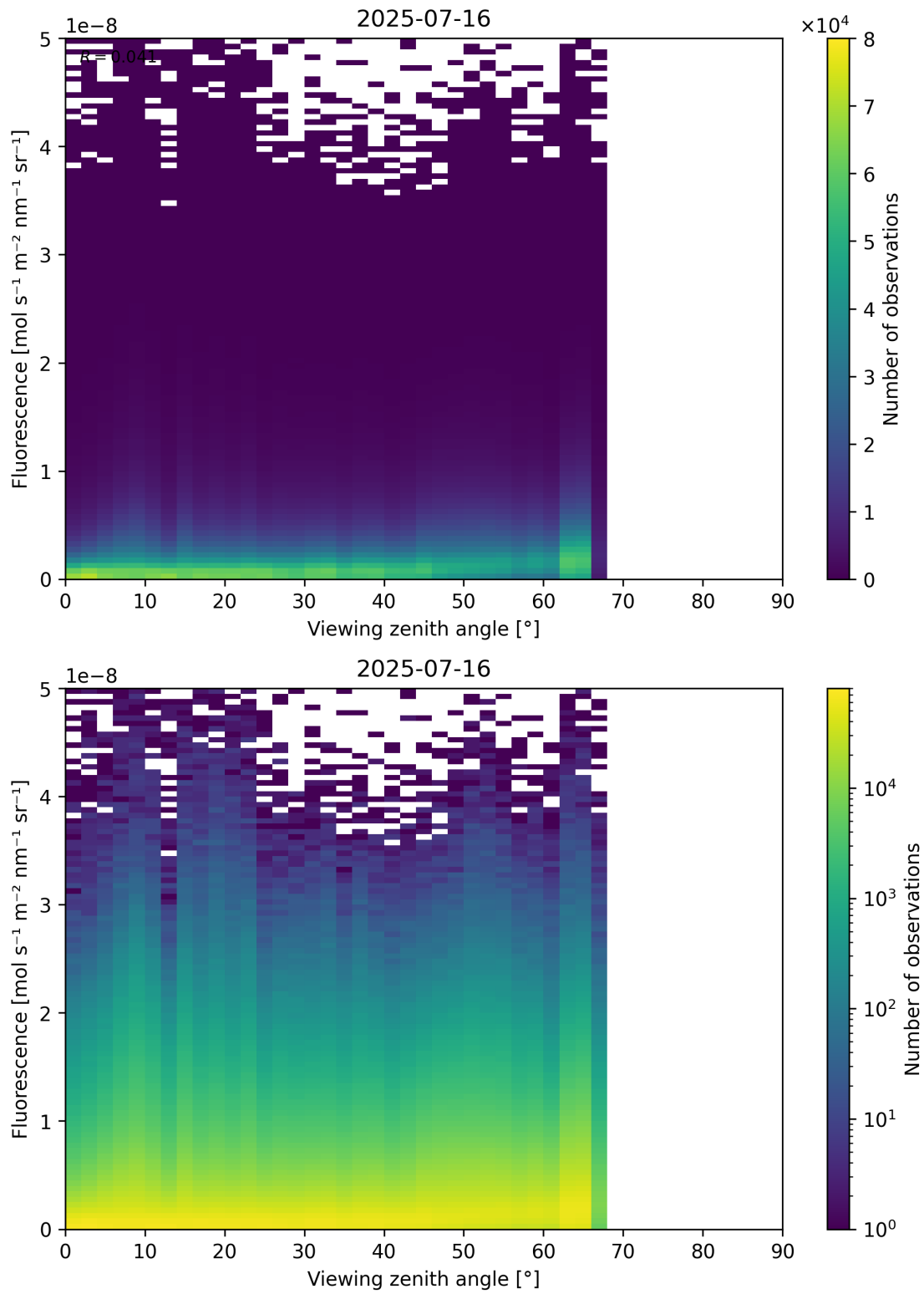
Figure 122: Scatter density plot of “Viewing zenith angle” against “Fluorescence” for 2025-07-15 to 2025-07-17.
