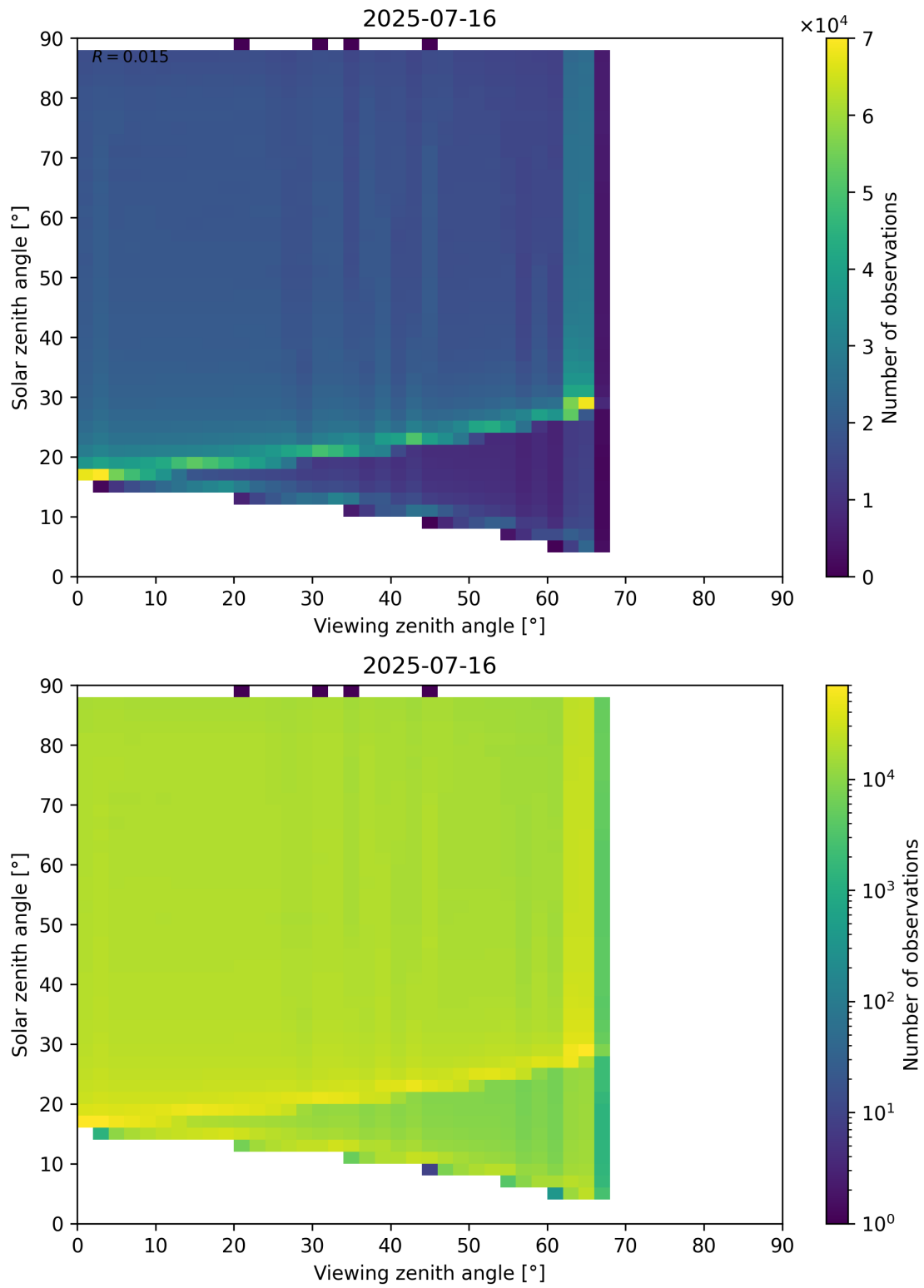
Figure 127: Scatter density plot of “Viewing zenith angle” against “Solar zenith angle” for 2025-07-15 to 2025-07-17.
