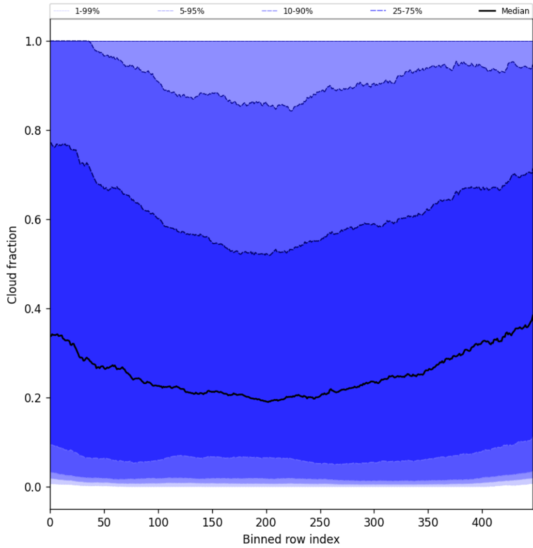
Figure 49: Along track statistics of “Cloud fraction” for 2025-07-15 to 2025-07-17
