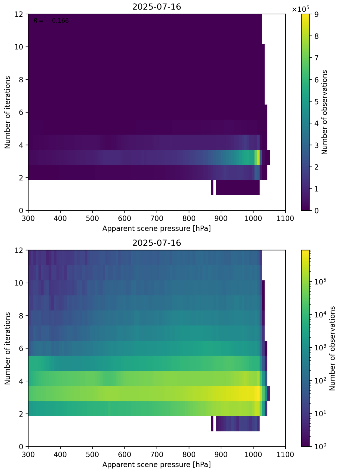
Figure 65: Scatter density plot of “Apparent scene pressure” against “Number of iterations” for 2025-07-15 to 2025-07-17.
