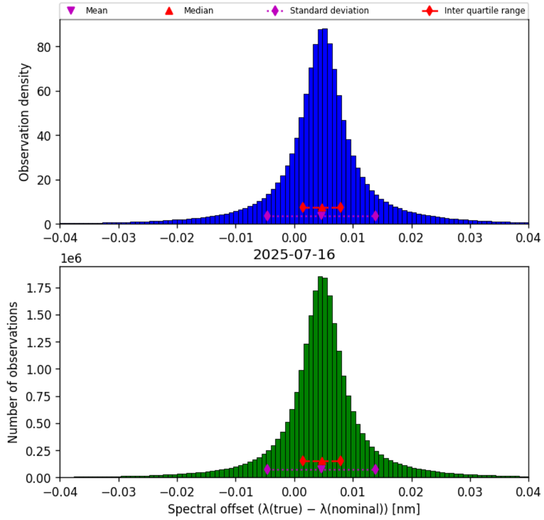
Figure 45: Histogram of “Spectral offset ( \lambda_{\text{true}} - \lambda_{\text{nominal}} )” for 2025-07-15 to 2025-07-17
