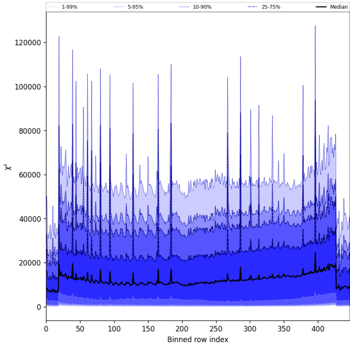
Figure 55: Along track statistics of " \chi^2 " for 2025-07-15 to 2025-07-17
