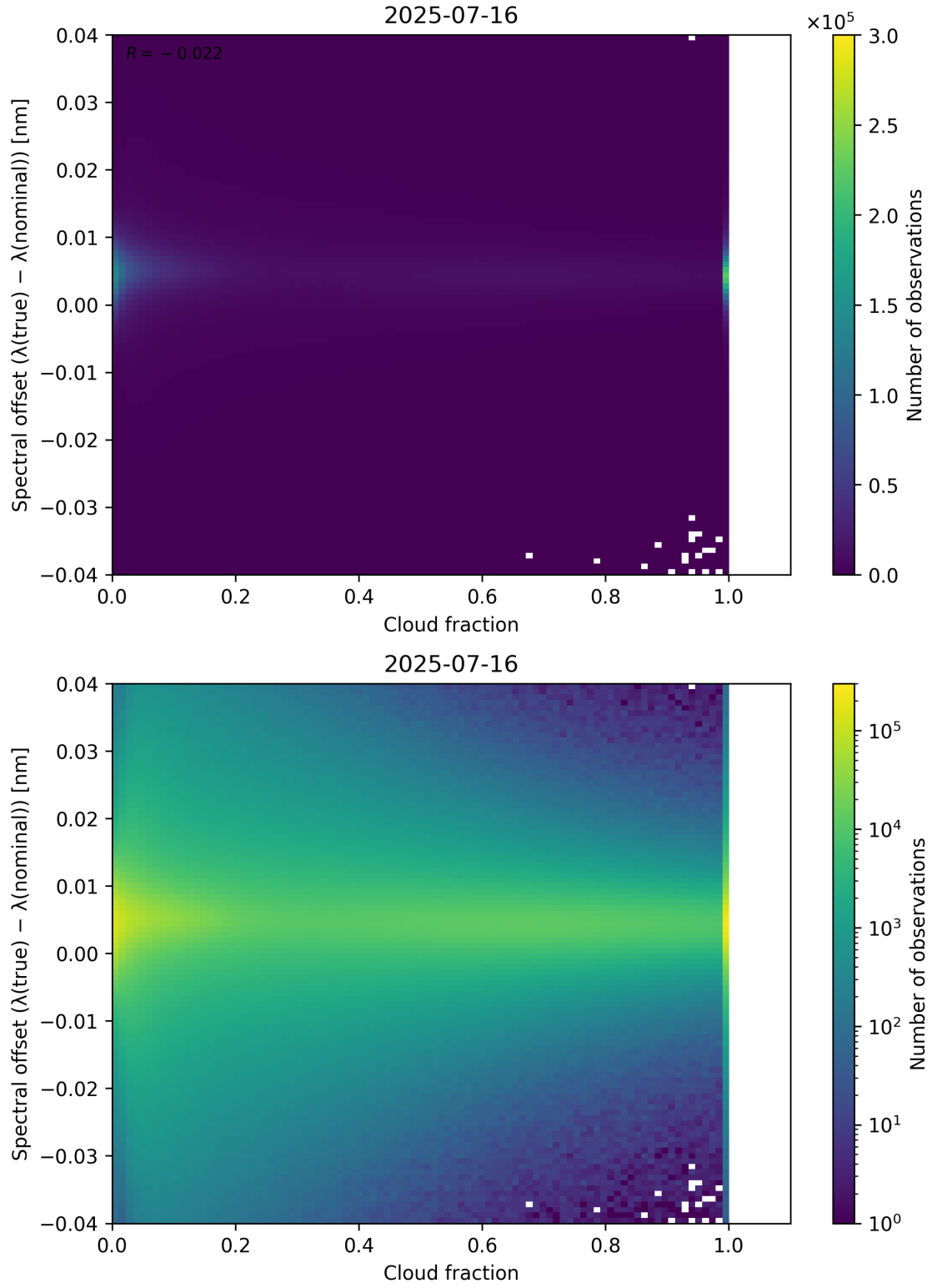
Figure 76: Scatter density plot of “Cloud fraction” against “Spectral offset ( \lambda_{\text{true}} - \lambda_{\text{nominal}} )” for 2025-07-15 to 2025-07-17.
