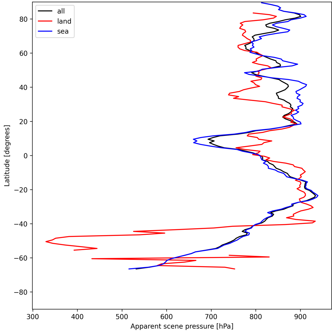
Figure 19: Zonal average of “Apparent scene pressure” for 2025-07-15 to 2025-07-17.
