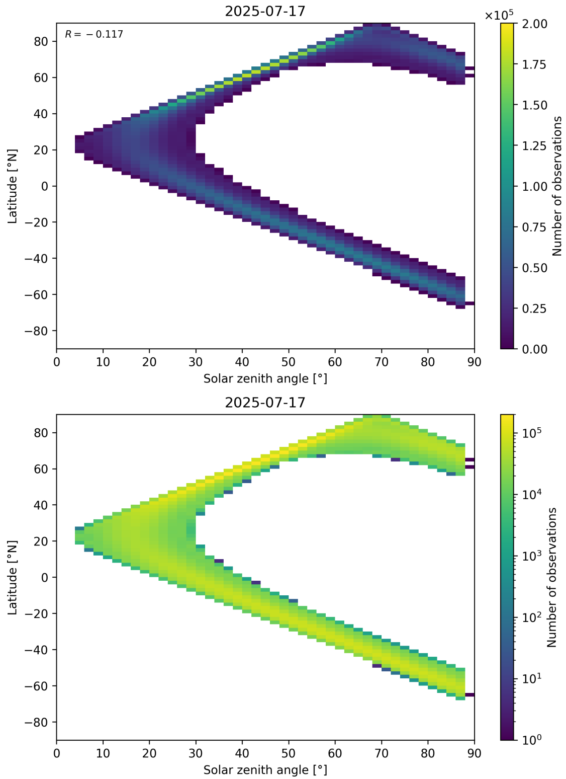
Figure 113: Scatter density plot of “Solar zenith angle” against “Latitude” for 2025-07-16 to 2025-07-18.
