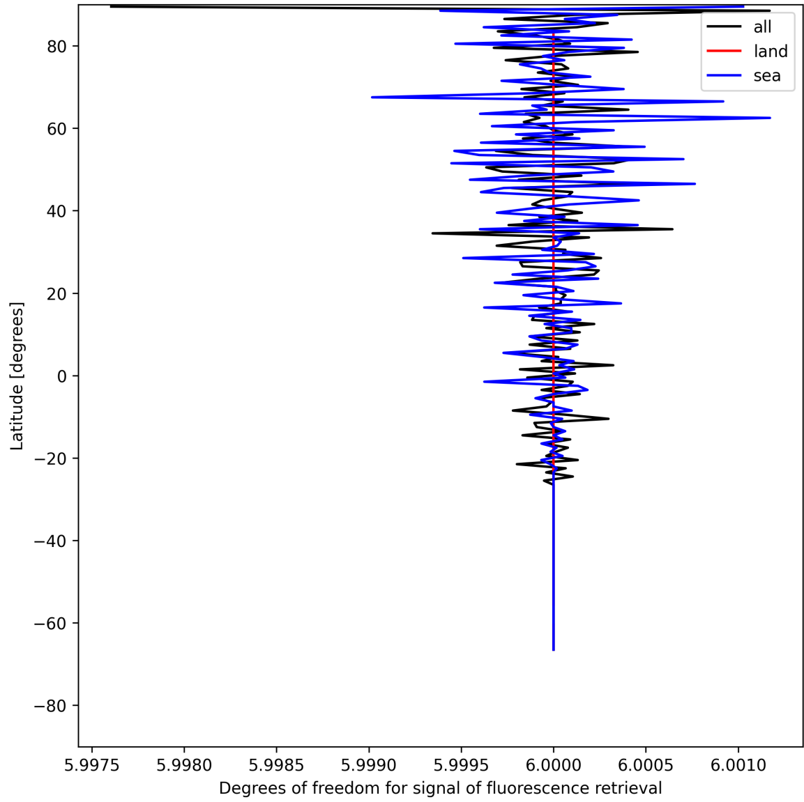
Figure 26: Zonal average of “Degrees of freedom for signal of fluorescence retrieval” for 2025-07-16 to 2025-07-18.
