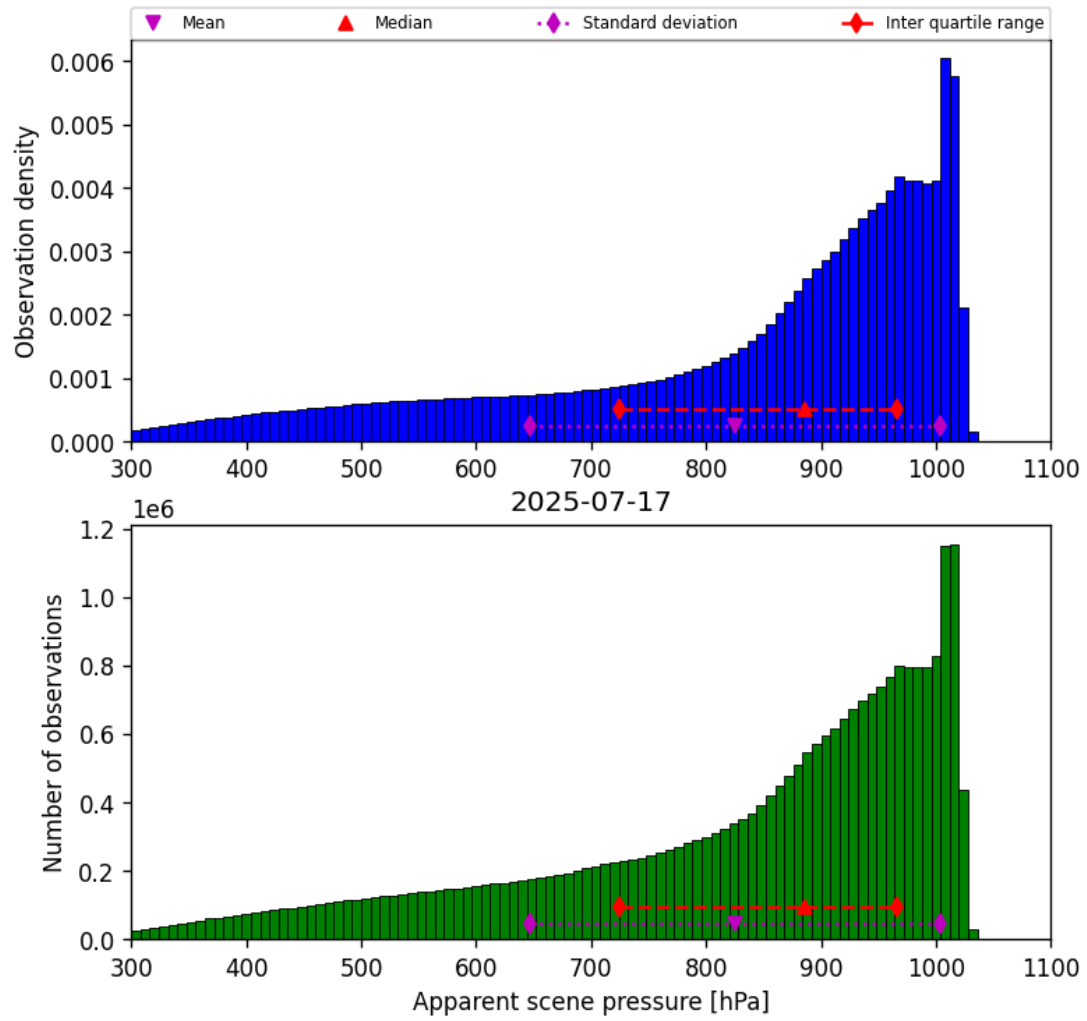
Figure 36: Histogram of “Apparent scene pressure” for 2025-07-16 to 2025-07-18
