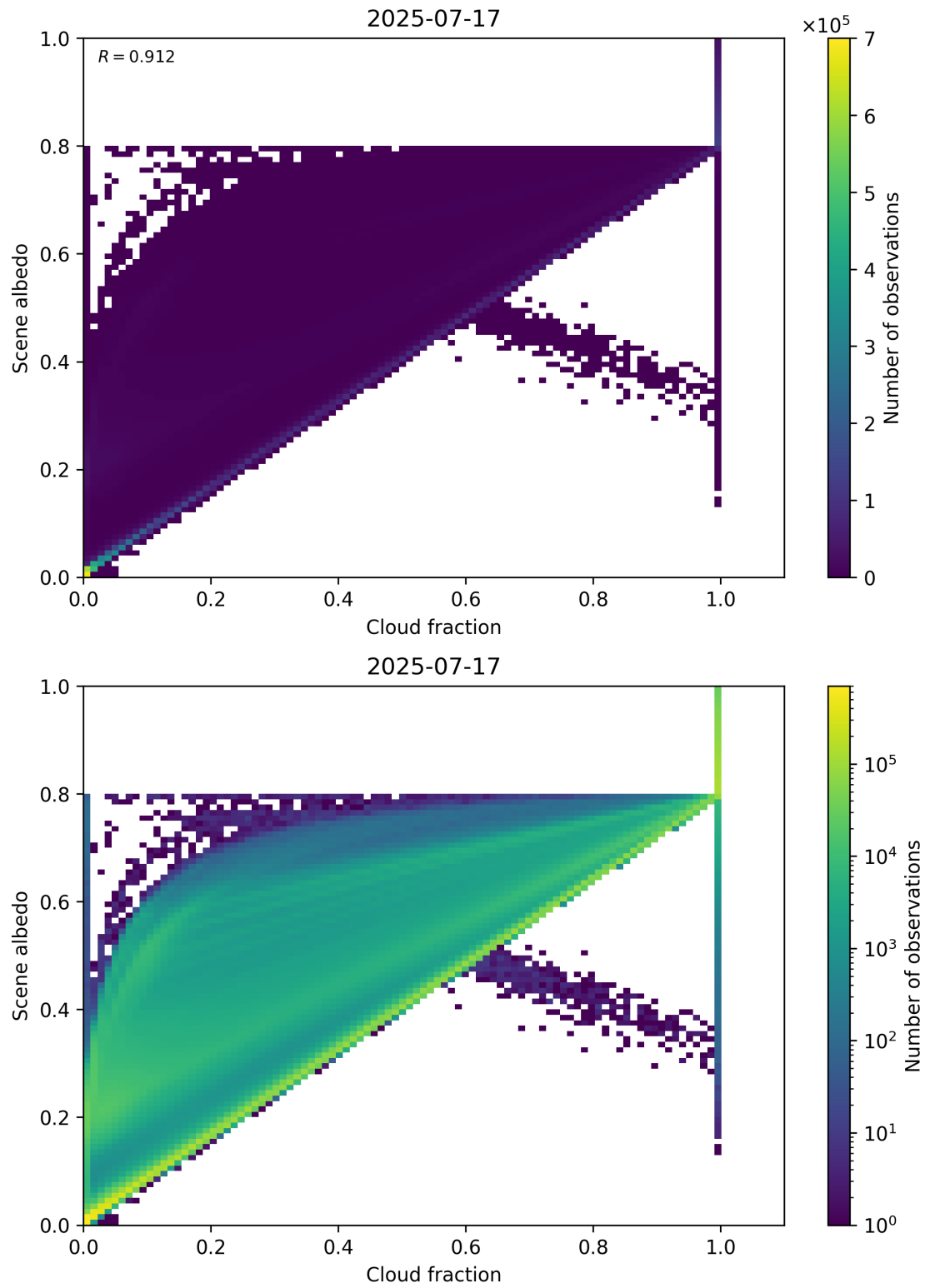
Figure 75: Scatter density plot of “Cloud fraction” against “Scene albedo” for 2025-07-16 to 2025-07-18.
