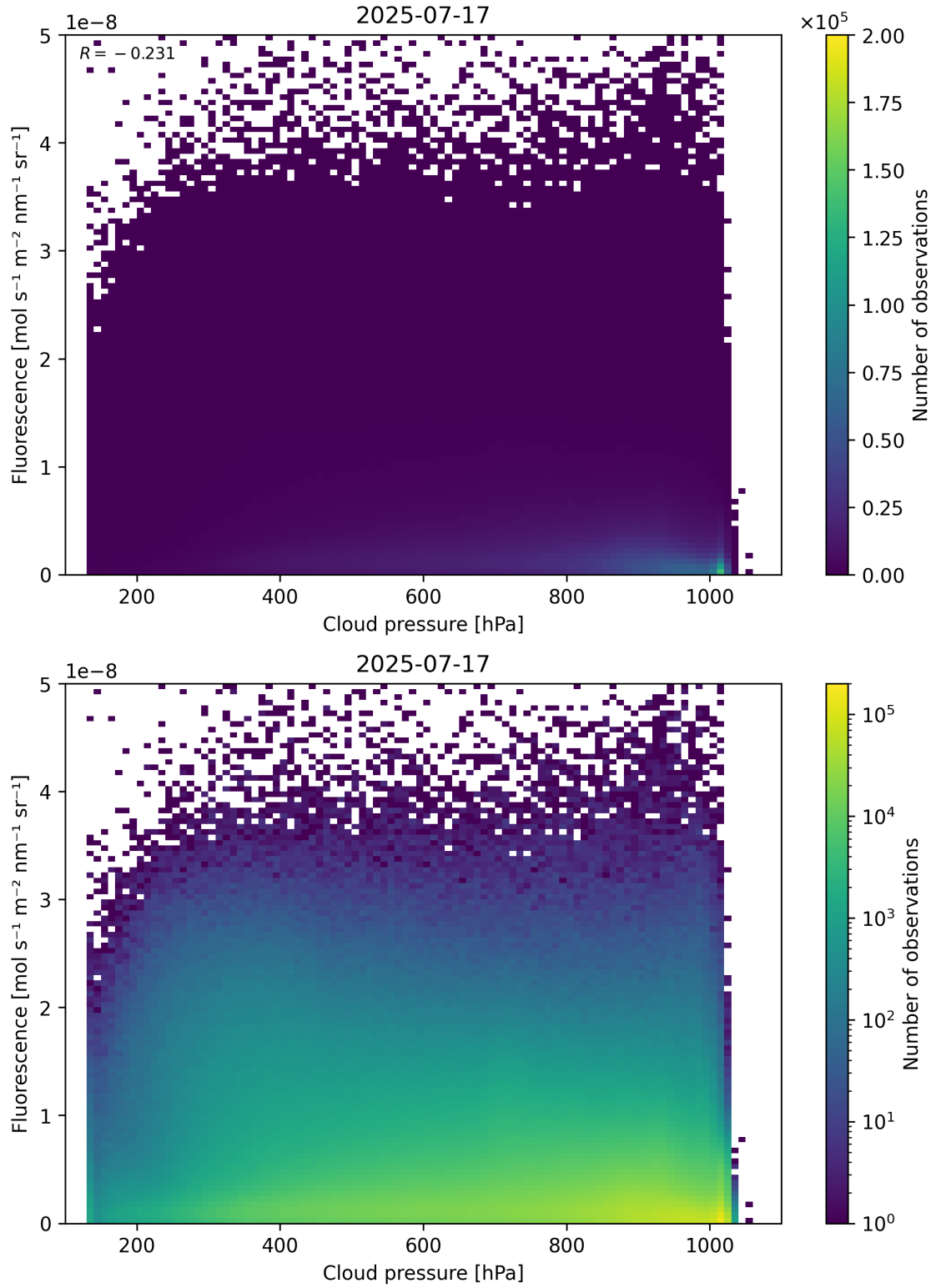
Figure 80: Scatter density plot of “Cloud pressure” against “Fluorescence” for 2025-07-16 to 2025-07-18.
