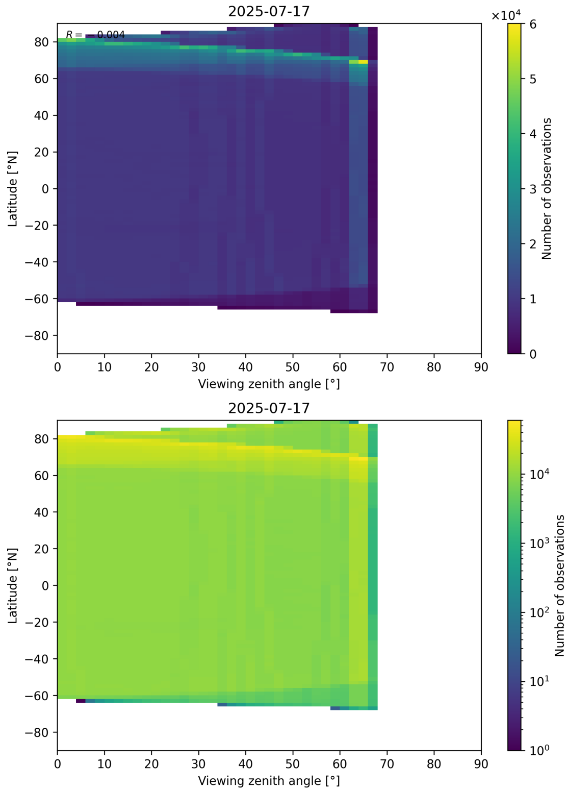
Figure 123: Scatter density plot of “Viewing zenith angle” against “Latitude” for 2025-07-16 to 2025-07-18.
