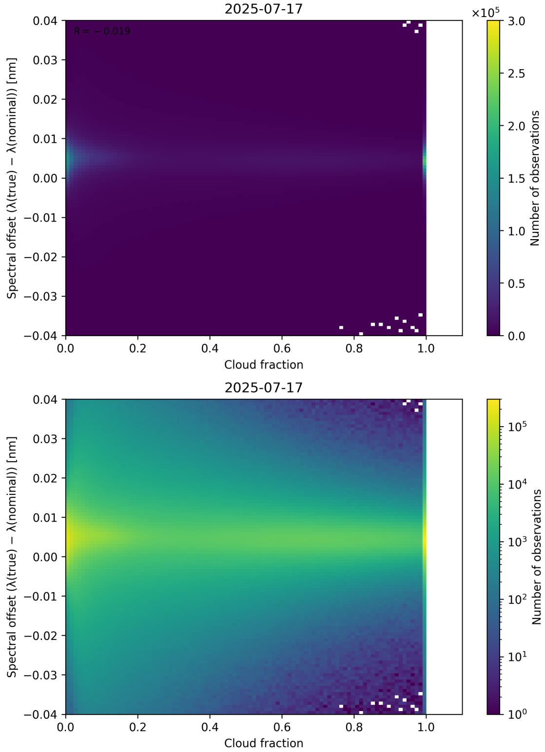
Figure 76: Scatter density plot of “Cloud fraction” against “Spectral offset ( \lambda_{\text{true}} - \lambda_{\text{nominal}} )” for 2025-07-16 to 2025-07-18.
