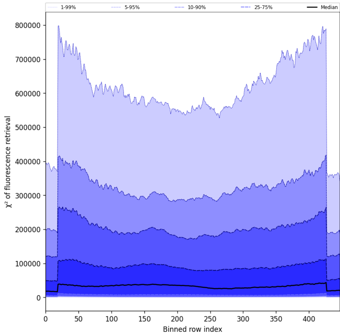
Figure 59: Along track statistics of “ \chi^2 of fluorescence retrieval” for 2025-07-16 to 2025-07-18
