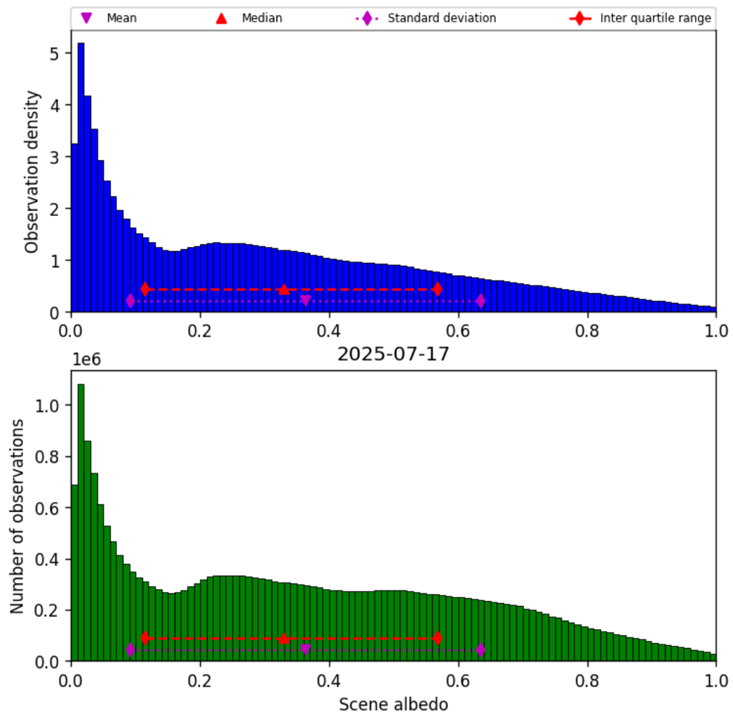
Figure 34: Histogram of “Scene albedo” for 2025-07-16 to 2025-07-18
