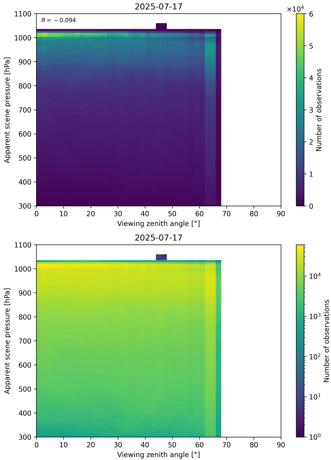
Figure 118: Scatter density plot of “Viewing zenith angle” against “Apparent scene pressure” for 2025-07-16 to 2025-07-18.
