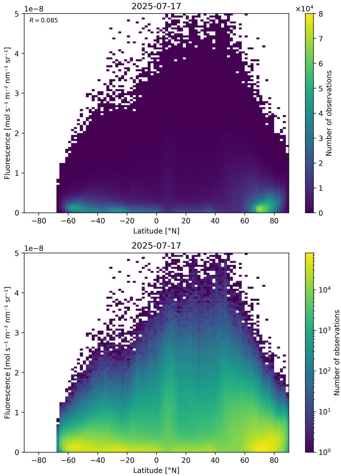
Figure 92: Scatter density plot of “Latitude” against “Fluorescence” for 2025-07-16 to 2025-07-18.
