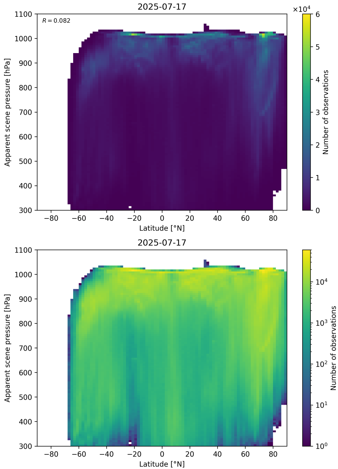
Figure 88: Scatter density plot of “Latitude” against “Apparent scene pressure” for 2025-07-16 to 2025-07-18.
