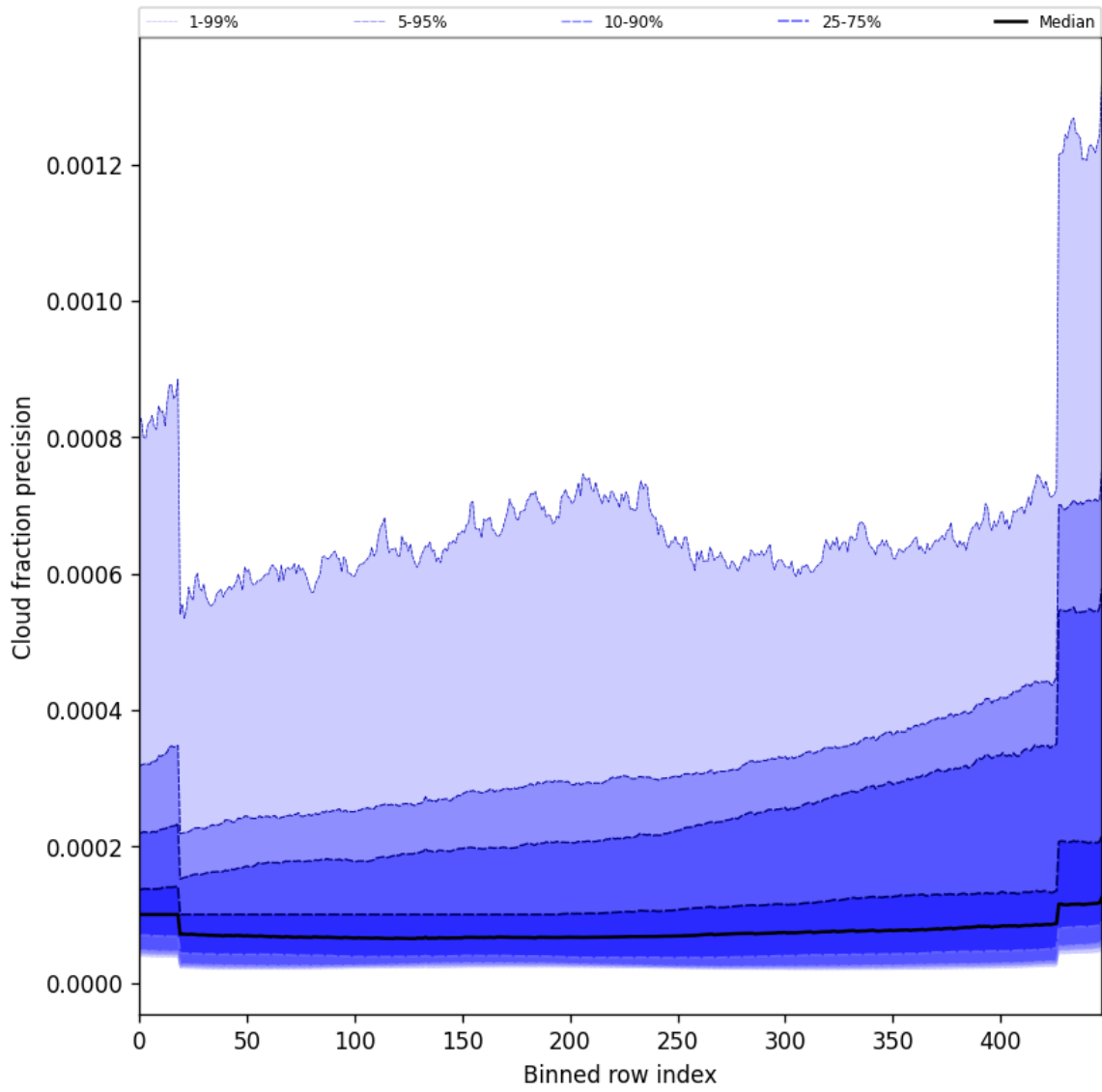
Figure 50: Along track statistics of “Cloud fraction precision” for 2025-07-16 to 2025-07-18
