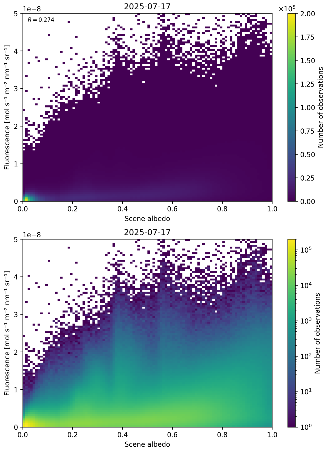
Figure 104: Scatter density plot of “Scene albedo” against “Fluorescence” for 2025-07-16 to 2025-07-18.
