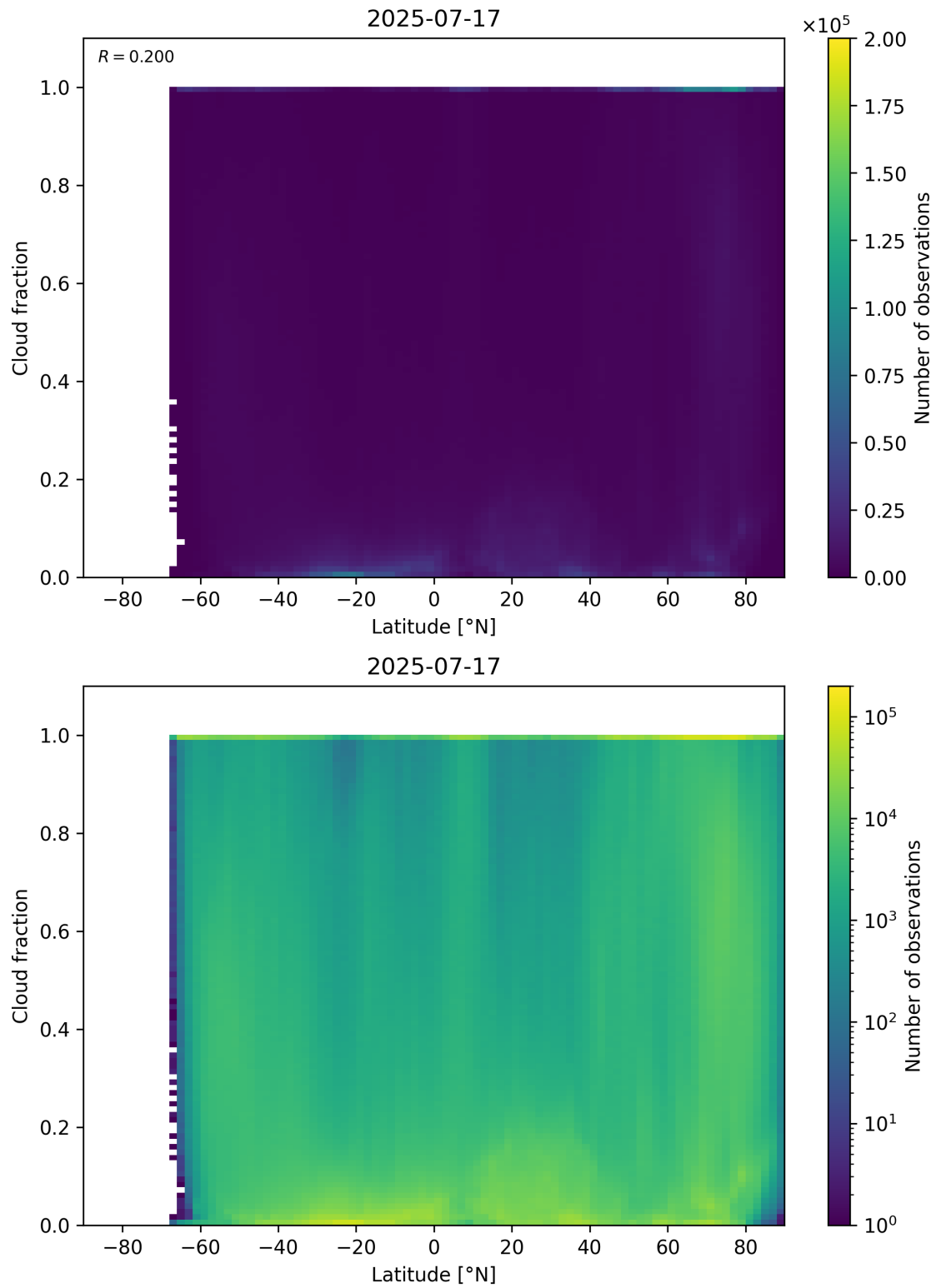
Figure 90: Scatter density plot of “Latitude” against “Cloud fraction” for 2025-07-16 to 2025-07-18.
