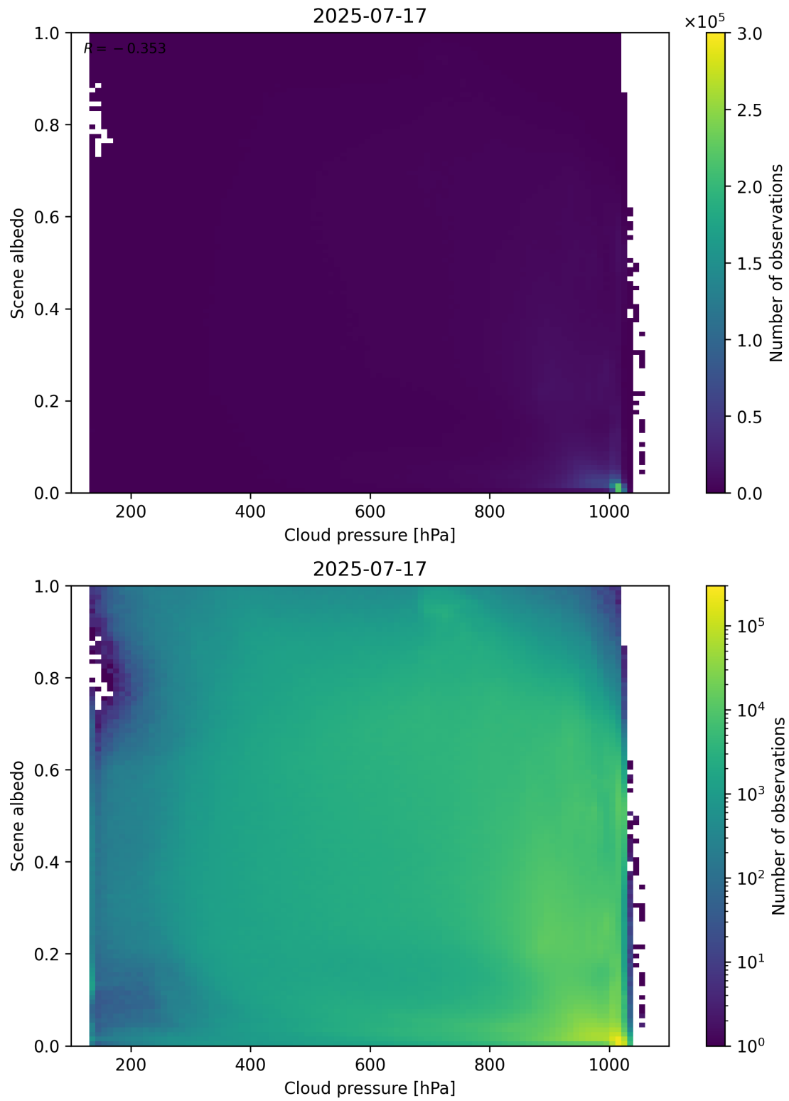
Figure 83: Scatter density plot of “Cloud pressure” against “Scene albedo” for 2025-07-16 to 2025-07-18.
