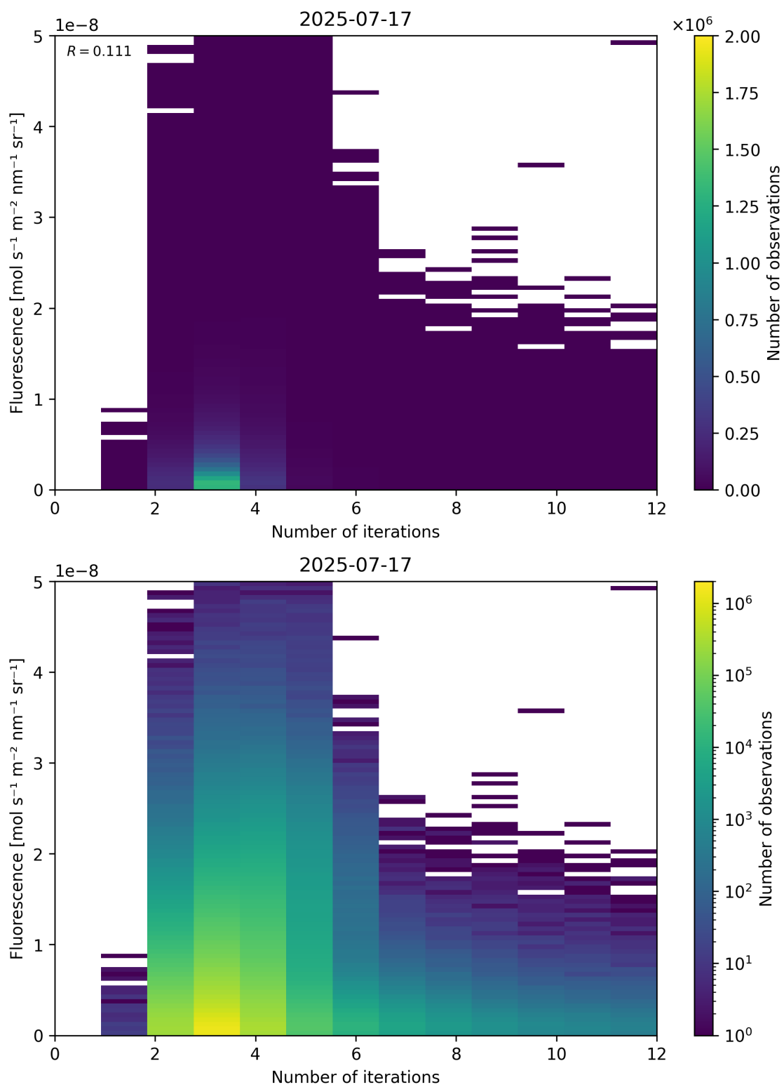
Figure 98: Scatter density plot of “Number of iterations” against “Fluorescence” for 2025-07-16 to 2025-07-18.
