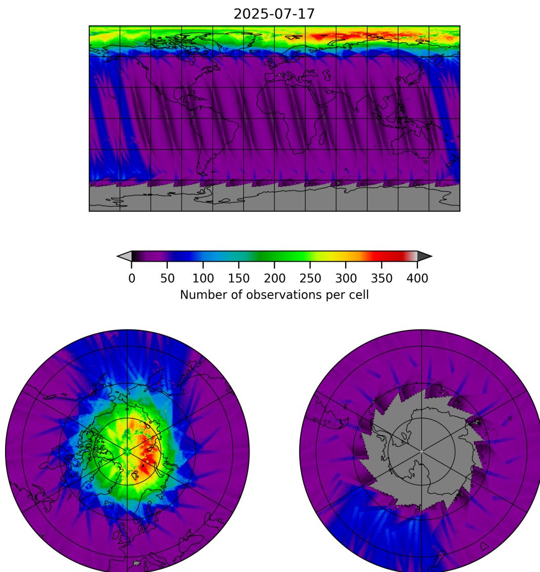
Figure 11: Map of the number of observations for 2025-07-16 to 2025-07-18
