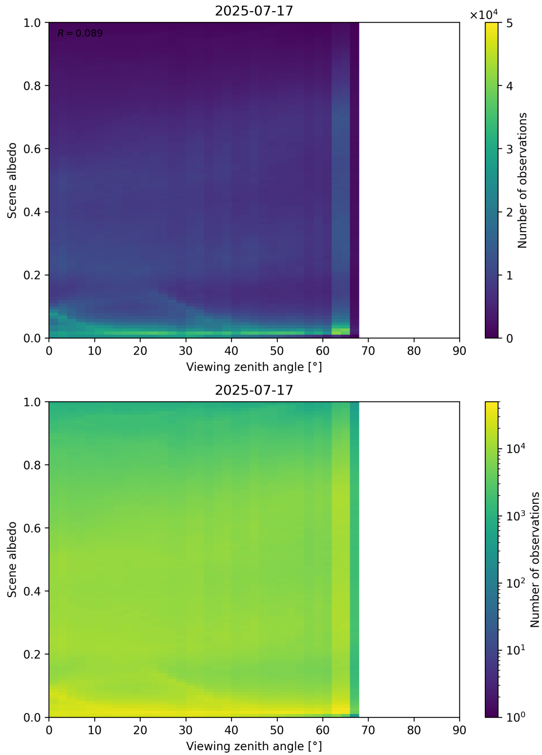
Figure 126: Scatter density plot of “Viewing zenith angle” against “Scene albedo” for 2025-07-16 to 2025-07-18.
