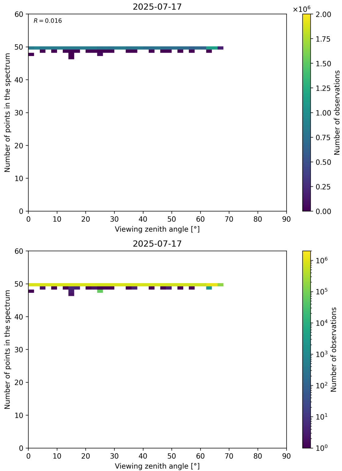
Figure 125: Scatter density plot of “Viewing zenith angle” against “Number of points in the spectrum” for 2025-07-16 to 2025-07-18.
