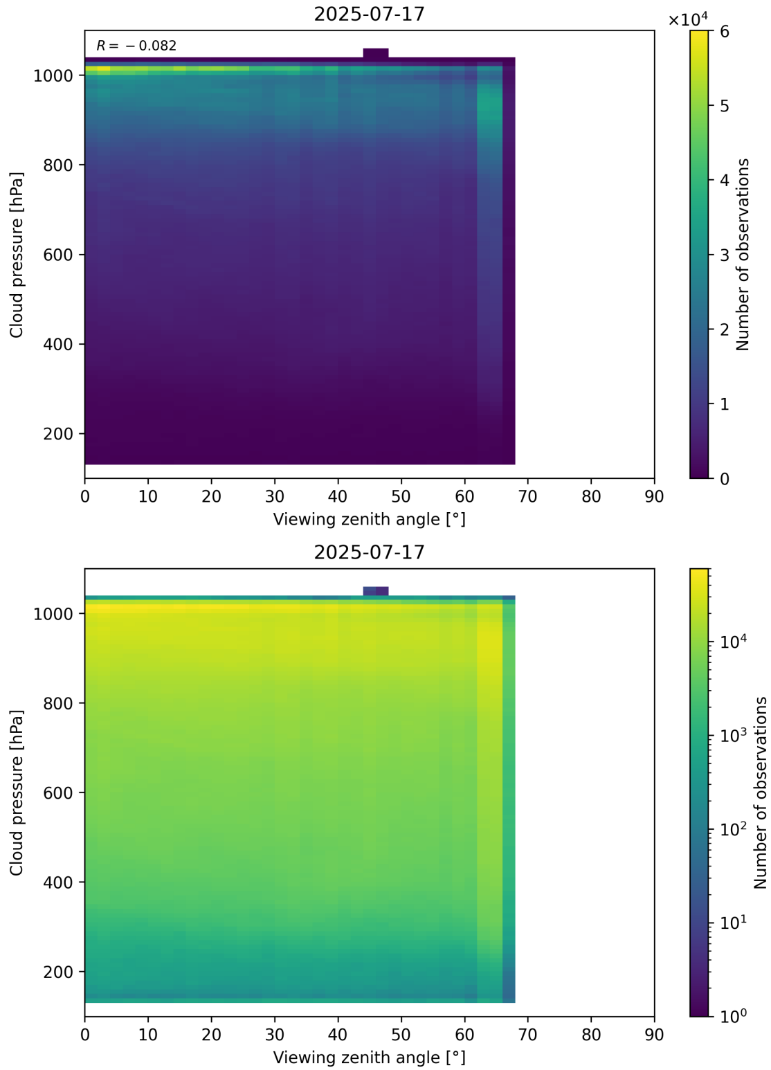
Figure 121: Scatter density plot of “Viewing zenith angle” against “Cloud pressure” for 2025-07-16 to 2025-07-18.
