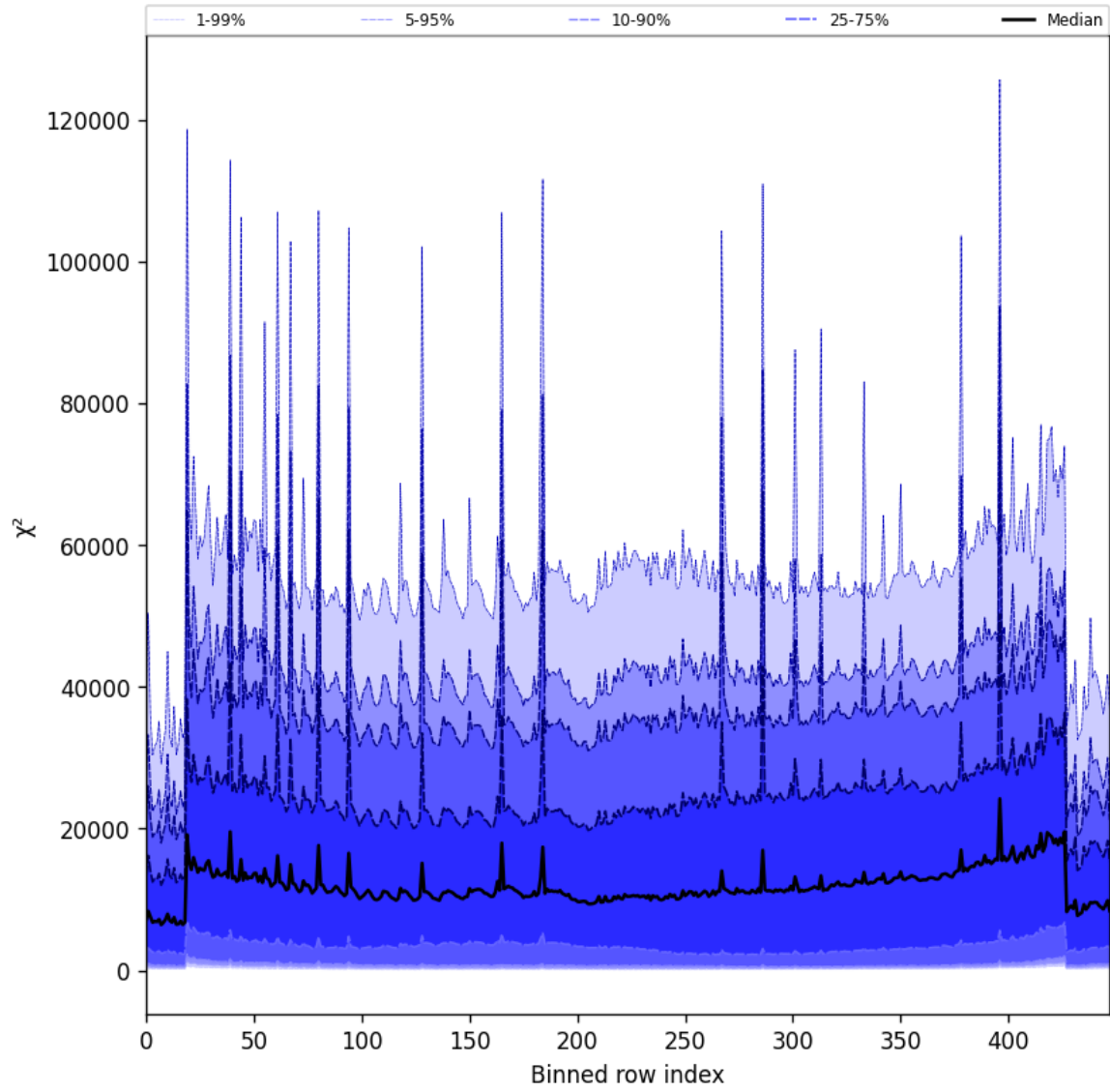
Figure 55: Along track statistics of “ \chi^2 ” for 2025-07-16 to 2025-07-18
