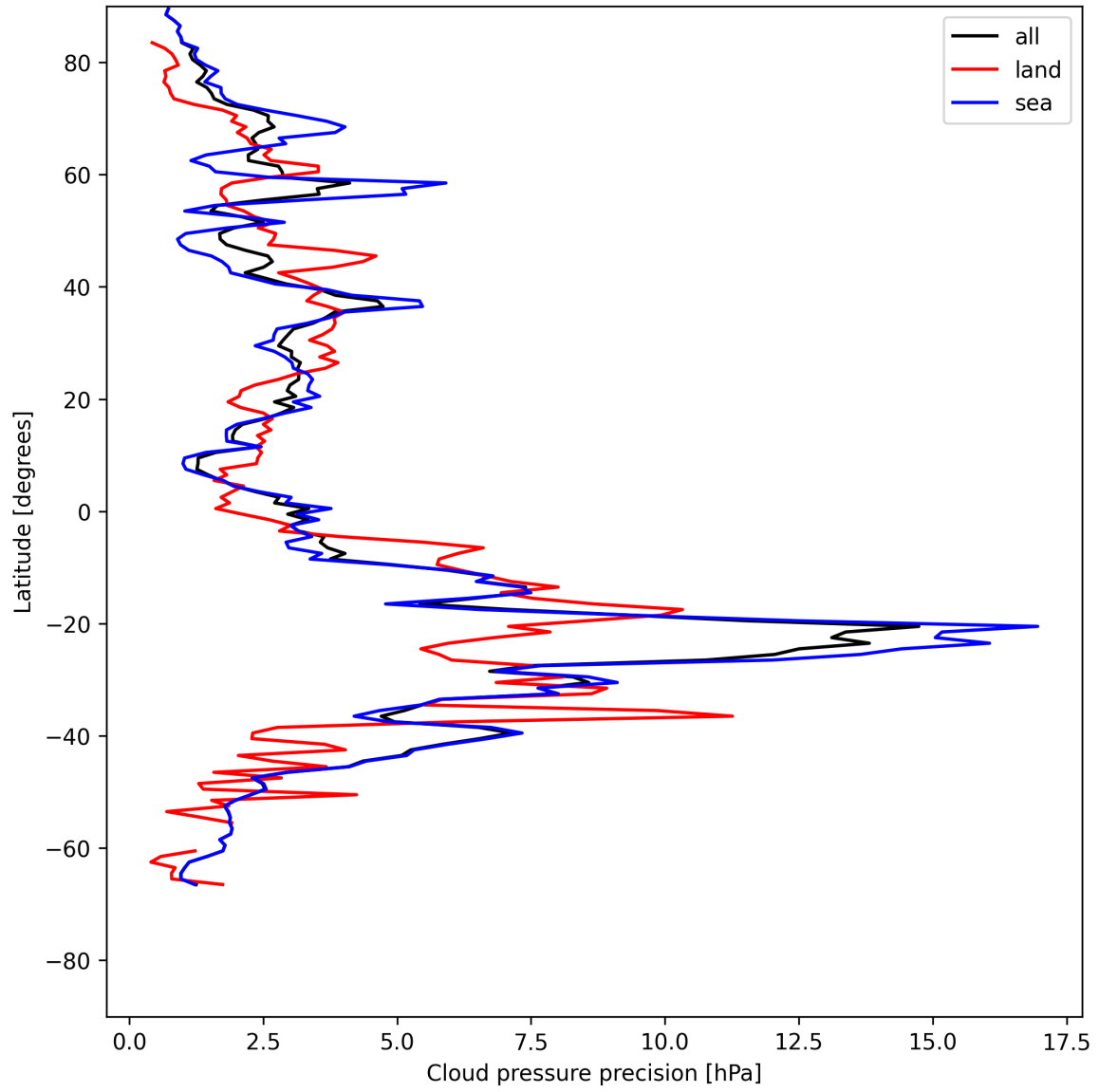
Figure 14: Zonal average of "Cloud pressure precision" for 2025-07-16 to 2025-07-18.
