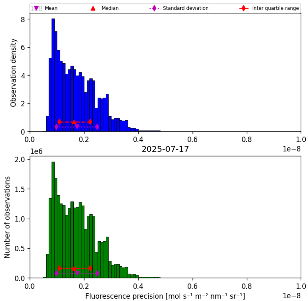
Figure 41: Histogram of “Fluorescence precision” for 2025-07-16 to 2025-07-18
