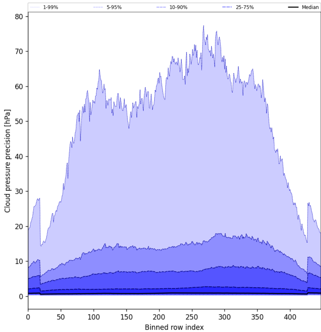
Figure 48: Along track statistics of “Cloud pressure precision” for 2025-07-16 to 2025-07-18
