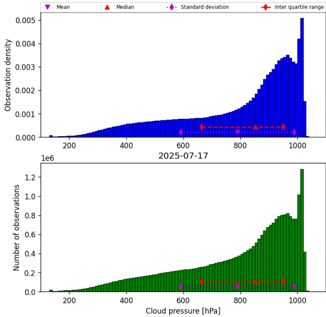
Figure 30: Histogram of “Cloud pressure” for 2025-07-16 to 2025-07-18
