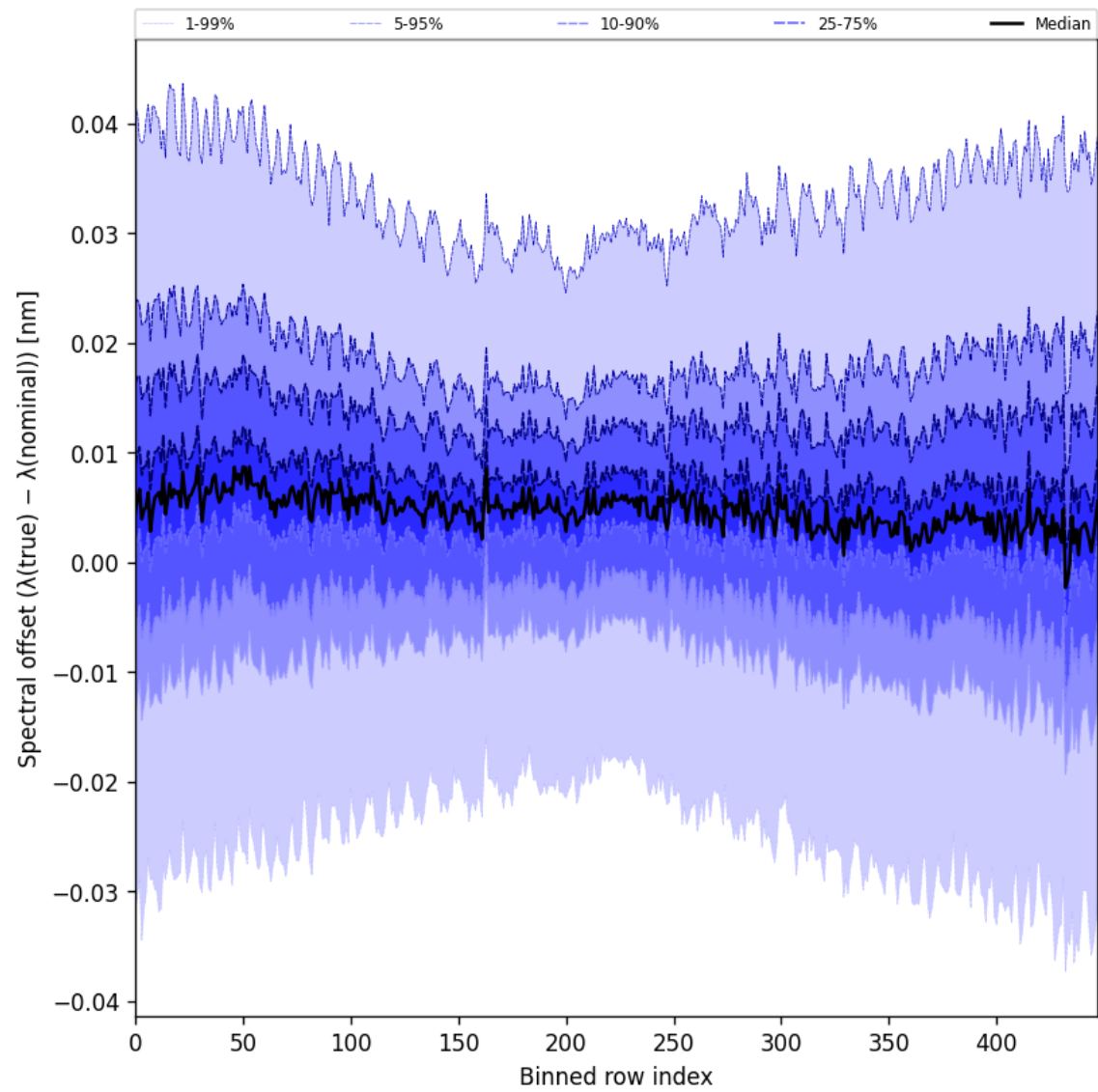
Figure 62: Along track statistics of “Spectral offset ( \lambda_{\text{true}} - \lambda_{\text{nominal}} )” for 2025-07-16 to 2025-07-18
