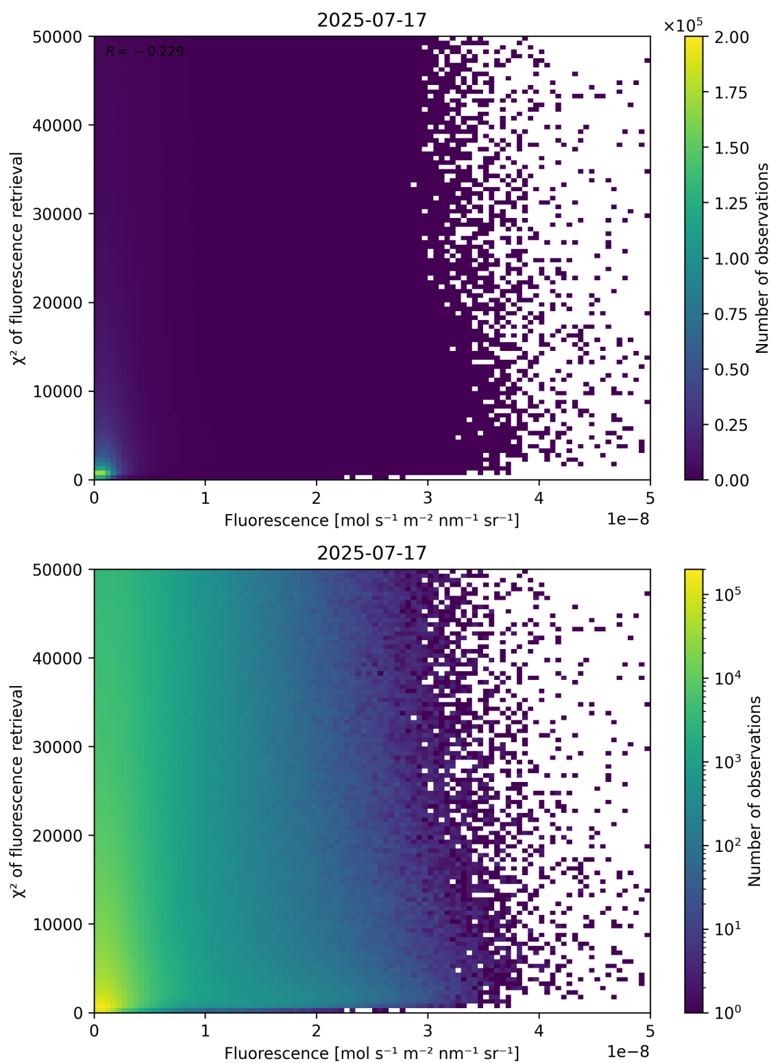
Figure 85: Scatter density plot of “Fluorescence” against “ \chi^2 of fluorescence retrieval” for 2025-07-16 to 2025-07-18.
