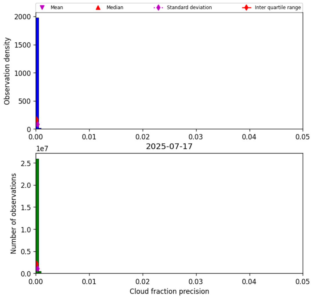
Figure 33: Histogram of “Cloud fraction precision” for 2025-07-16 to 2025-07-18
