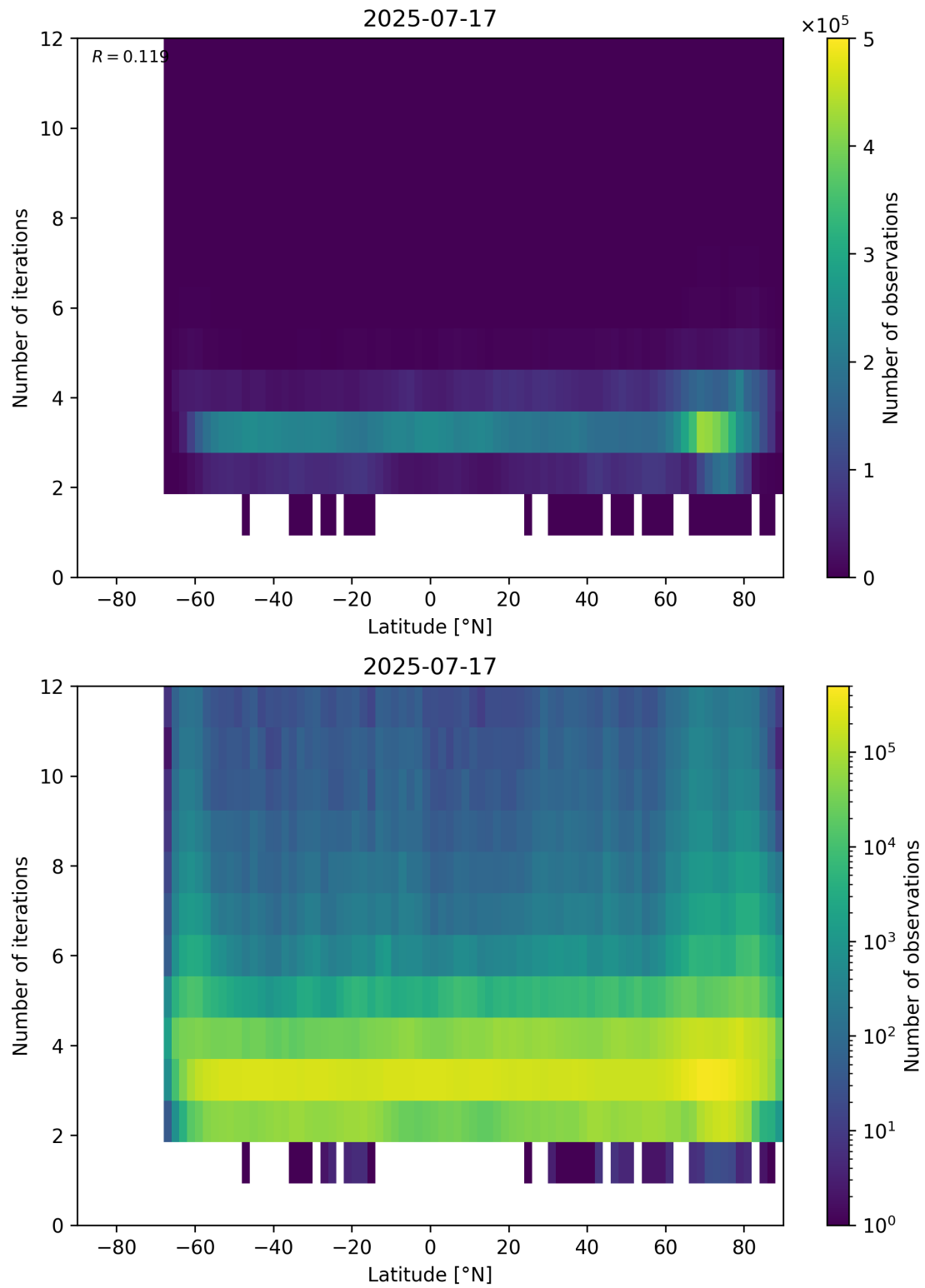
Figure 93: Scatter density plot of “Latitude” against “Number of iterations” for 2025-07-16 to 2025-07-18.
