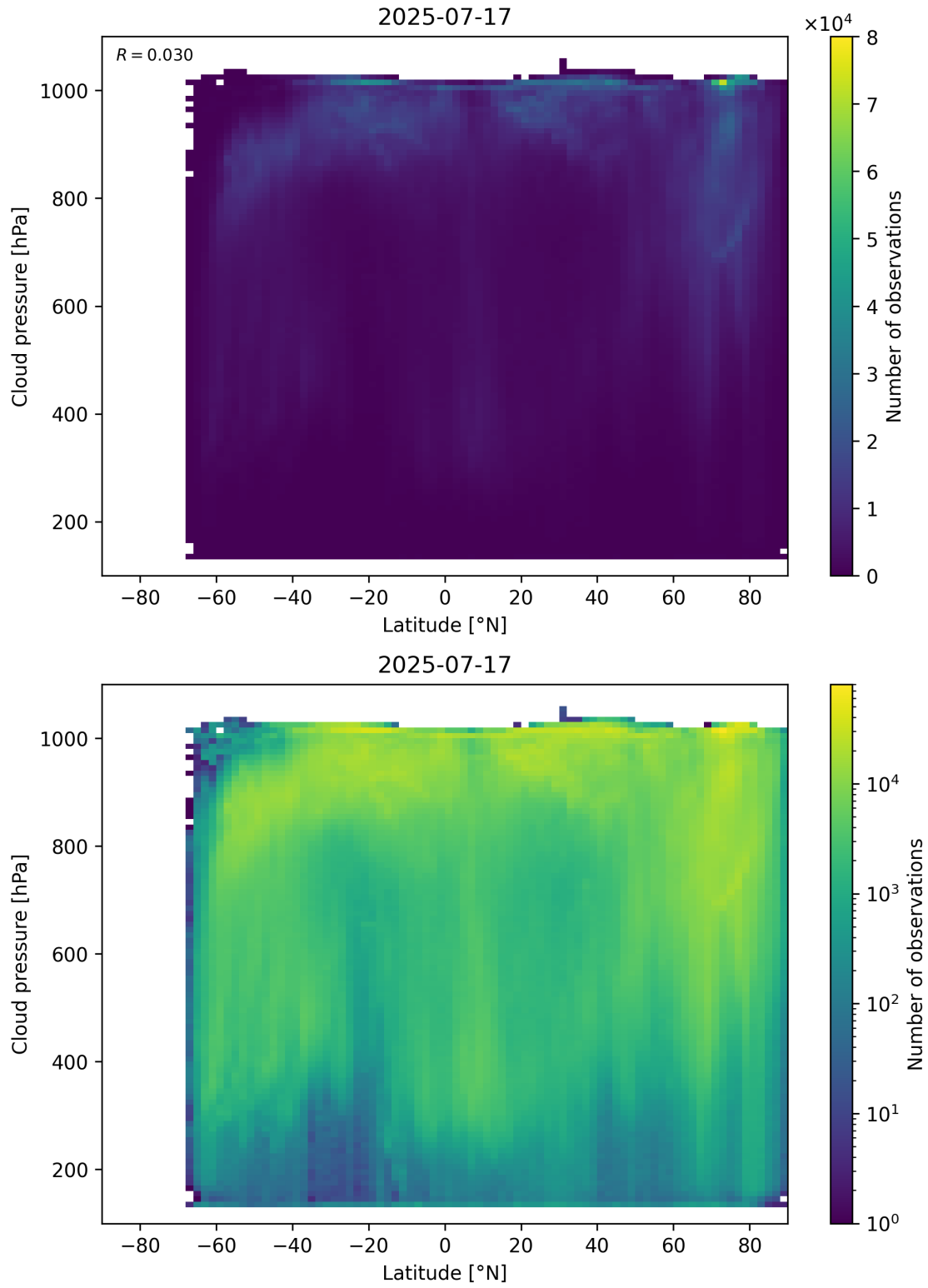
Figure 91: Scatter density plot of “Latitude” against “Cloud pressure” for 2025-07-16 to 2025-07-18.
