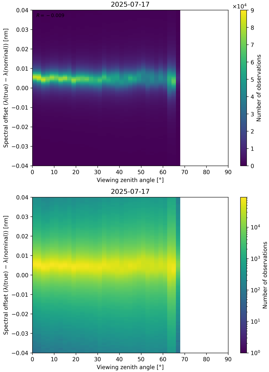
Figure 128: Scatter density plot of “Viewing zenith angle” against “Spectral offset ( \lambda_{\text{true}} - \lambda_{\text{nominal}} )” for 2025-07-16 to 2025-07-18.
