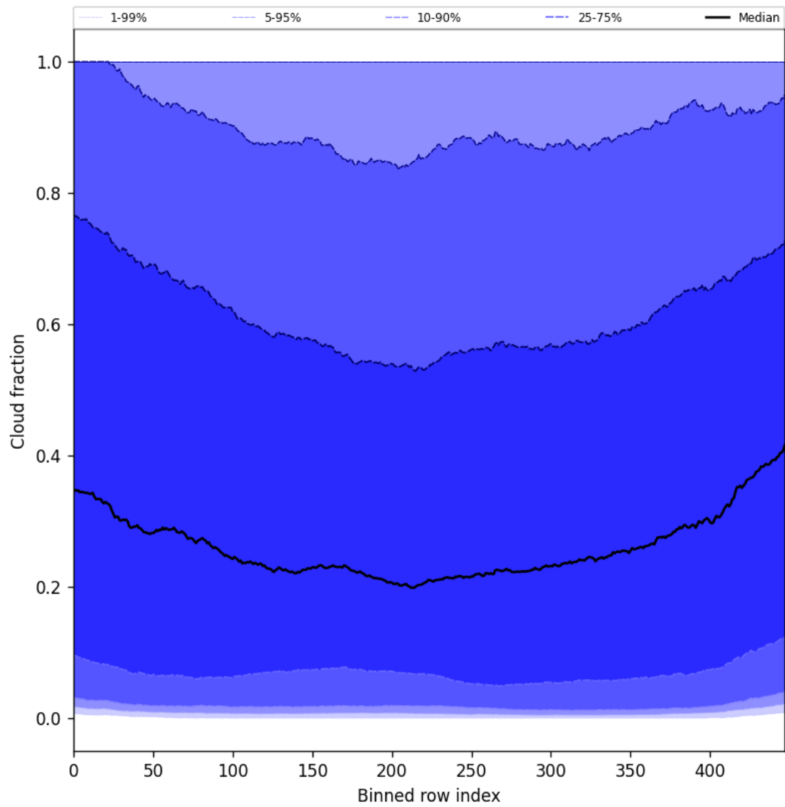
Figure 49: Along track statistics of “Cloud fraction” for 2025-07-16 to 2025-07-18
