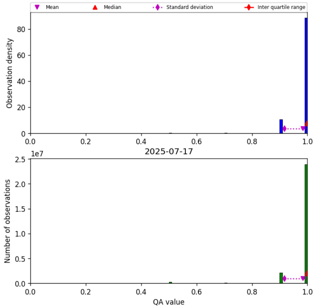
Figure 29: Histogram of “QA value” for 2025-07-16 to 2025-07-18
