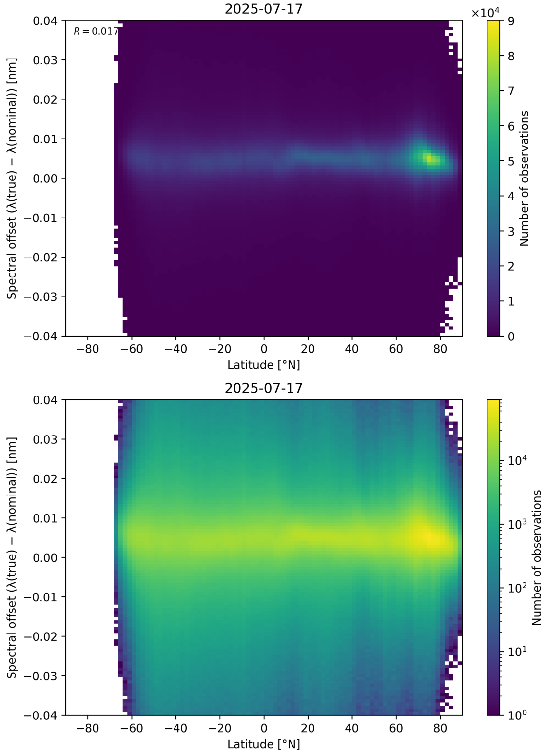
Figure 96: Scatter density plot of “Latitude” against “Spectral offset ( \lambda_{\text{true}} - \lambda_{\text{nominal}} )” for 2025-07-16 to 2025-07-18.
