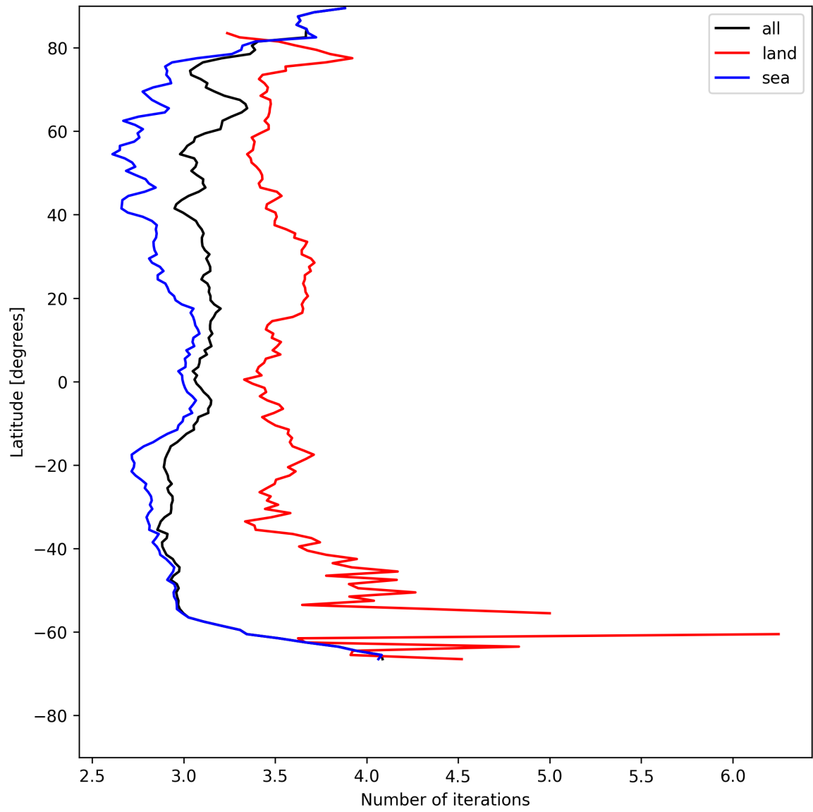
Figure 22: Zonal average of “Number of iterations” for 2025-07-16 to 2025-07-18.
