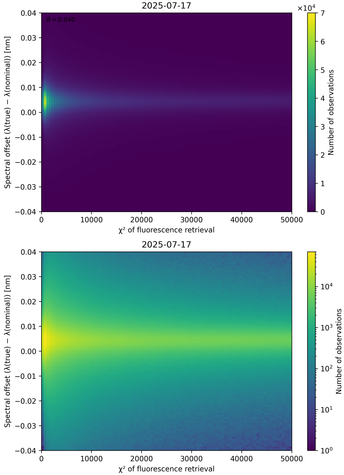
Figure 69: Scatter density plot of “ \chi^2 of fluorescence retrieval” against “Spectral offset ( \lambda_{\text{true}} - \lambda_{\text{nominal}} )” for 2025-07-16 to 2025-07-18.
