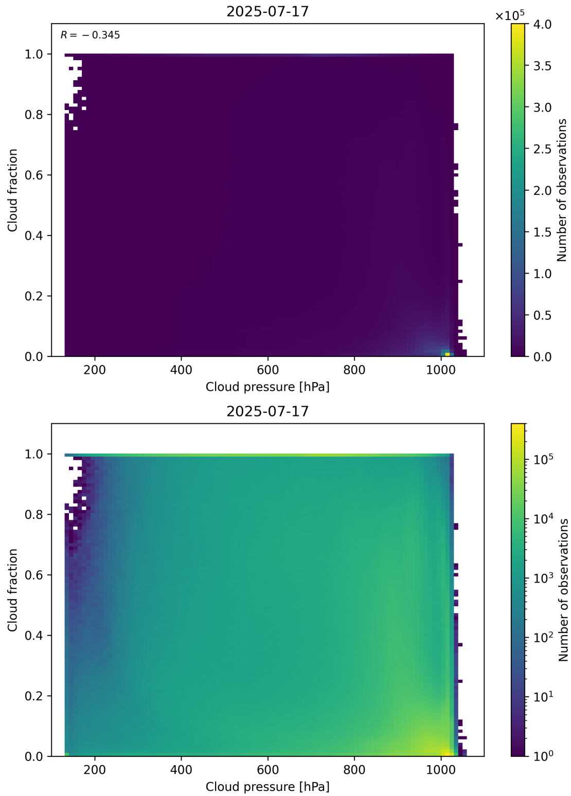
Figure 79: Scatter density plot of “Cloud pressure” against “Cloud fraction” for 2025-07-16 to 2025-07-18.
