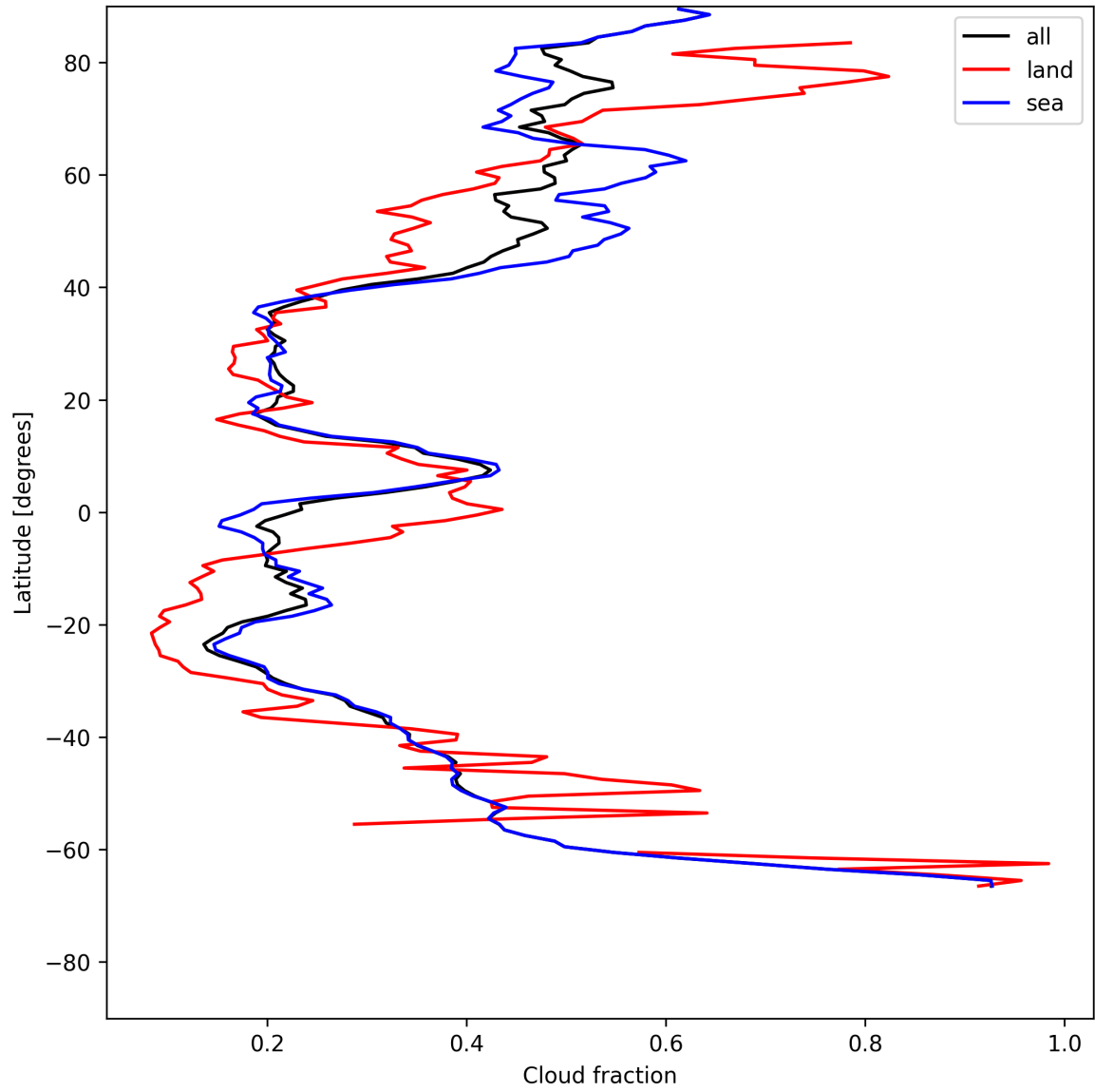
Figure 15: Zonal average of “Cloud fraction” for 2025-07-16 to 2025-07-18.
