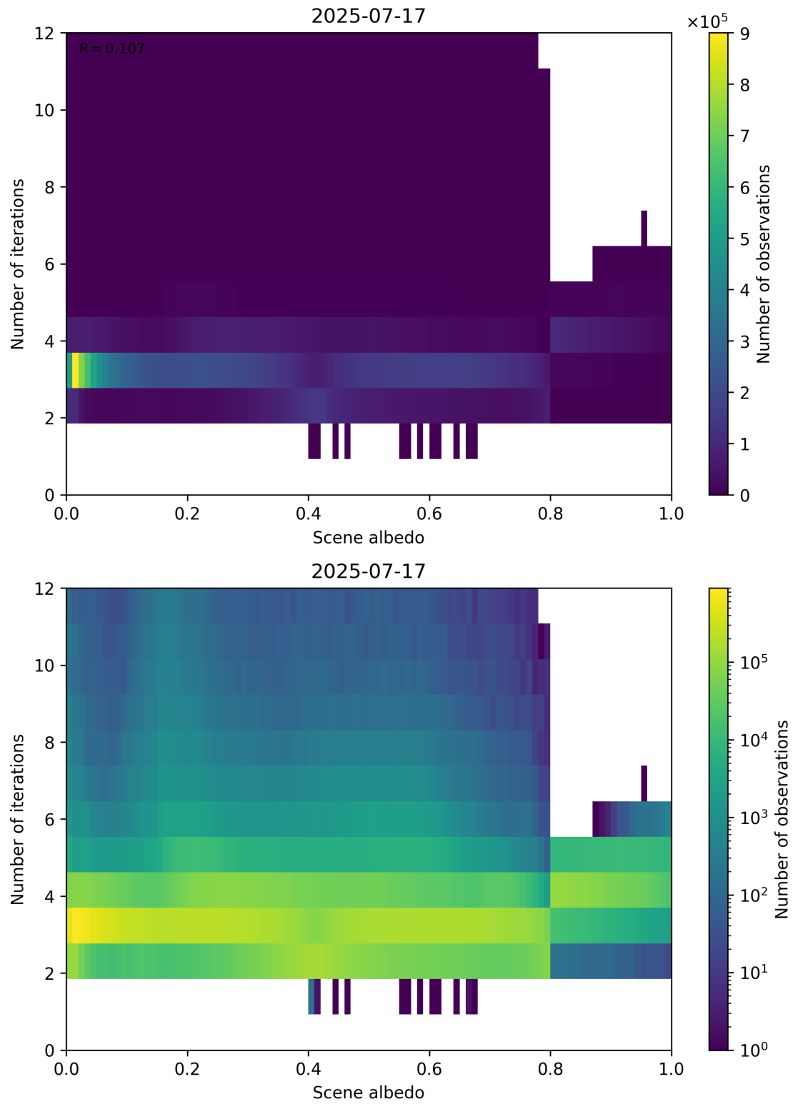
Figure 105: Scatter density plot of “Scene albedo” against “Number of iterations” for 2025-07-16 to 2025-07-18.
