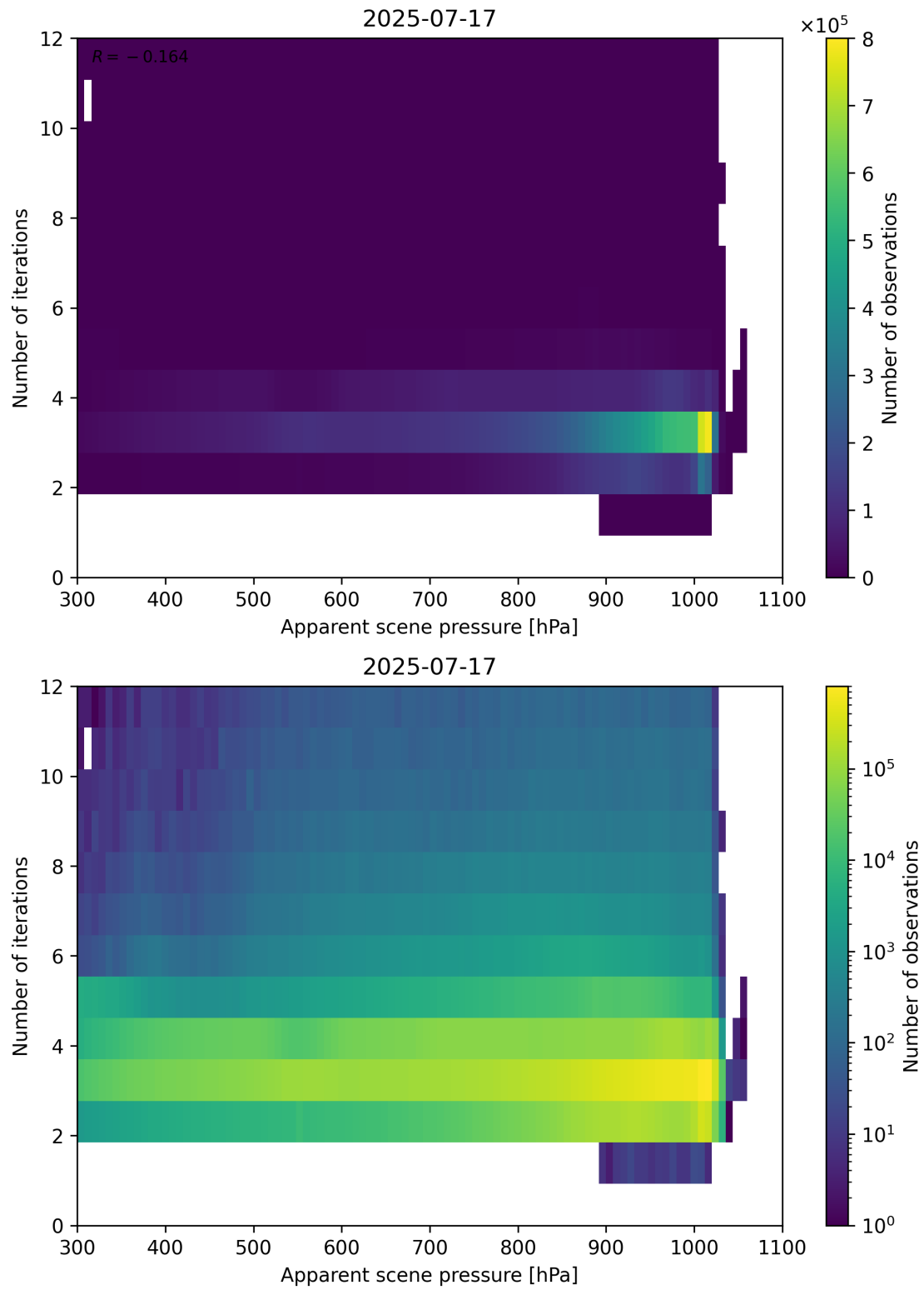
Figure 65: Scatter density plot of “Apparent scene pressure” against “Number of iterations” for 2025-07-16 to 2025-07-18.
