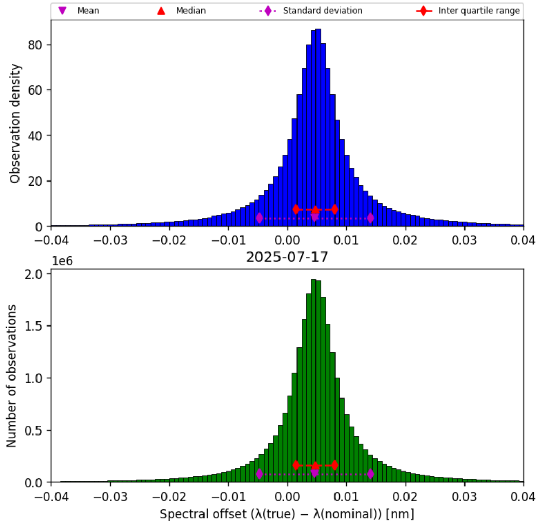
Figure 45: Histogram of “Spectral offset ( \lambda_{\text{true}} - \lambda_{\text{nominal}} )” for 2025-07-16 to 2025-07-18
