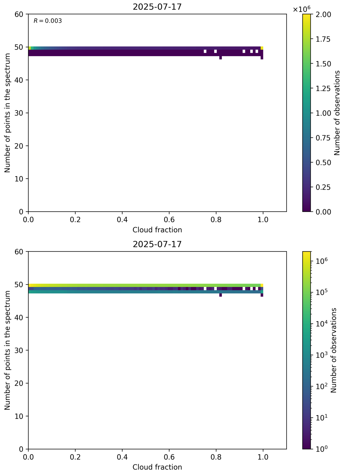
Figure 74: Scatter density plot of “Cloud fraction” against “Number of points in the spectrum” for 2025-07-16 to 2025-07-18.
