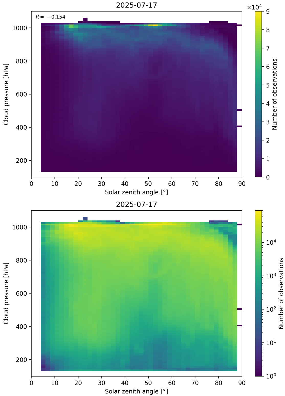
Figure 111: Scatter density plot of “Solar zenith angle” against “Cloud pressure” for 2025-07-16 to 2025-07-18.
