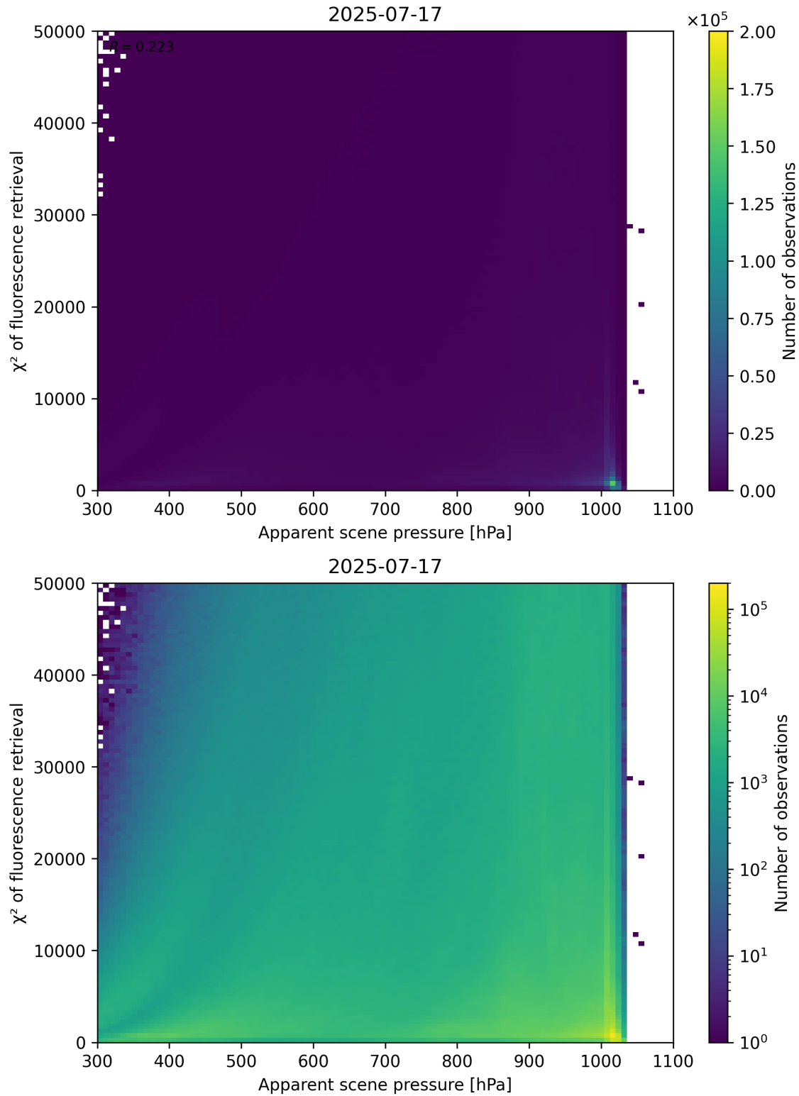
Figure 63: Scatter density plot of “Apparent scene pressure” against “ \chi^2 of fluorescence retrieval” for 2025-07-16 to 2025-07-18.
