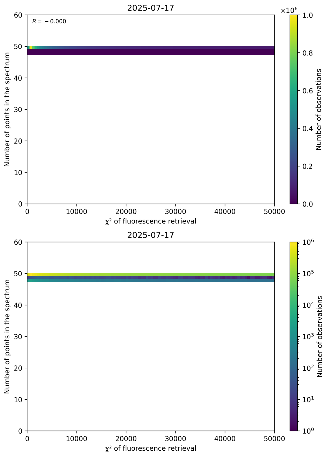
Figure 68: Scatter density plot of “ \chi^2 of fluorescence retrieval” against “Number of points in the spectrum” for 2025-07-16 to 2025-07-18.
