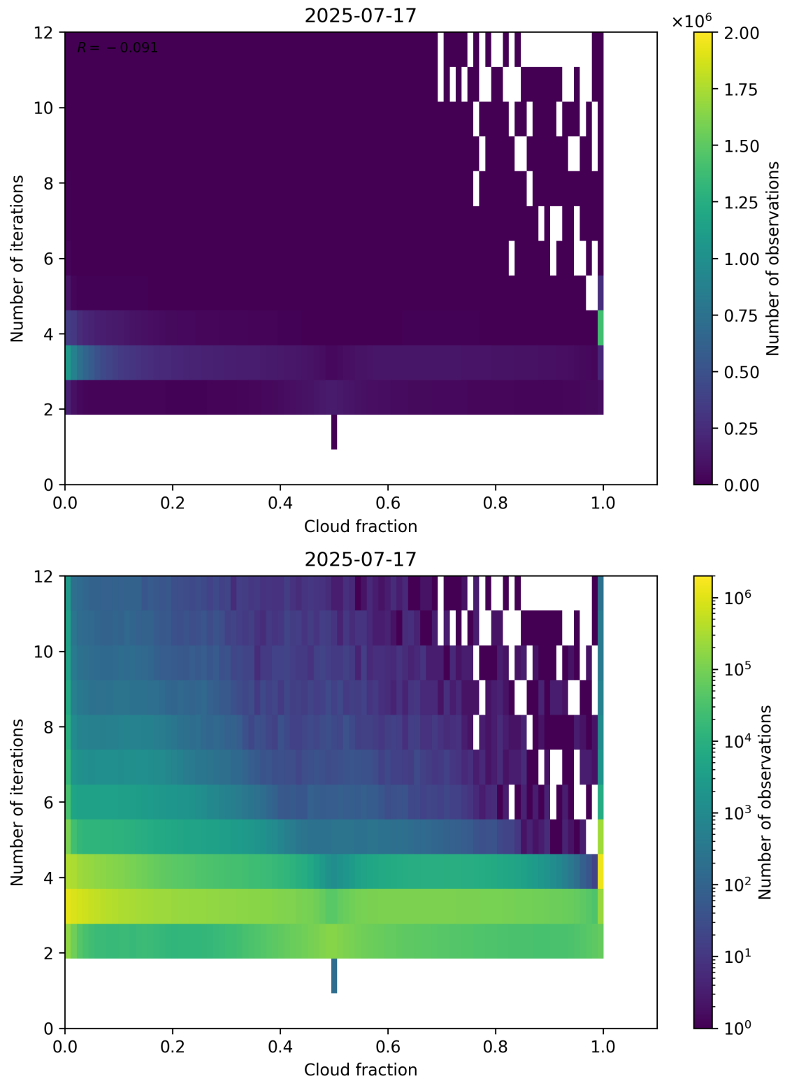
Figure 73: Scatter density plot of “Cloud fraction” against “Number of iterations” for 2025-07-16 to 2025-07-18.
