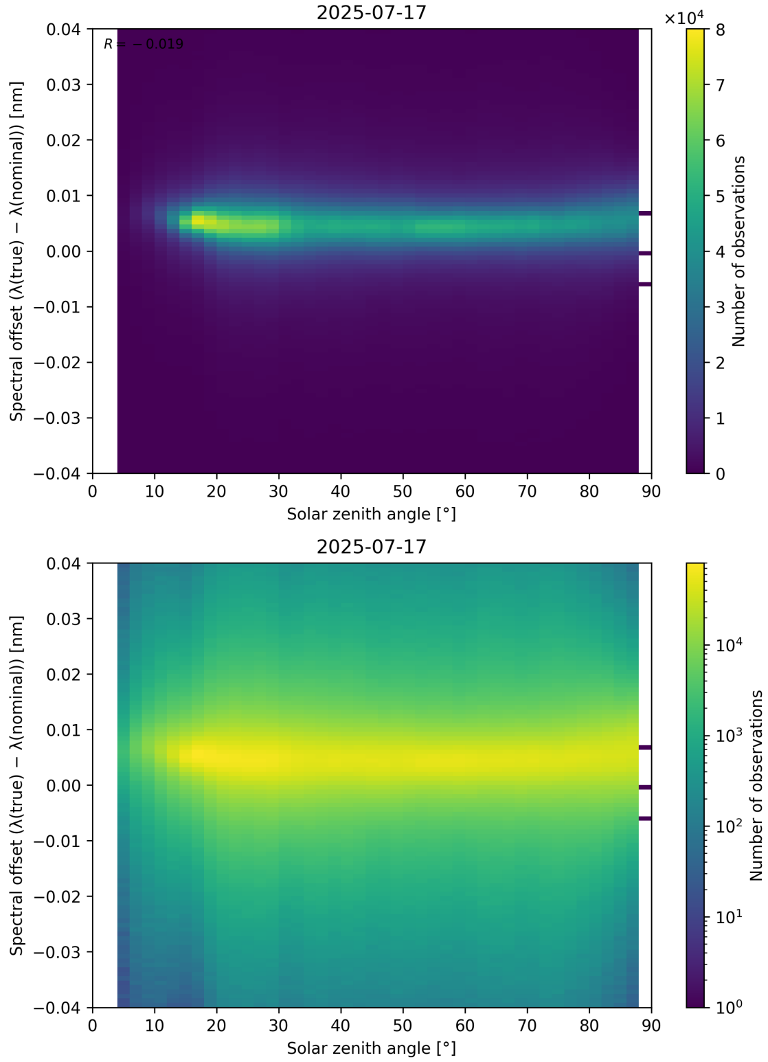
Figure 117: Scatter density plot of “Solar zenith angle” against “Spectral offset ( \lambda_{\text{true}} - \lambda_{\text{nominal}} )” for 2025-07-16 to 2025-07-18.
