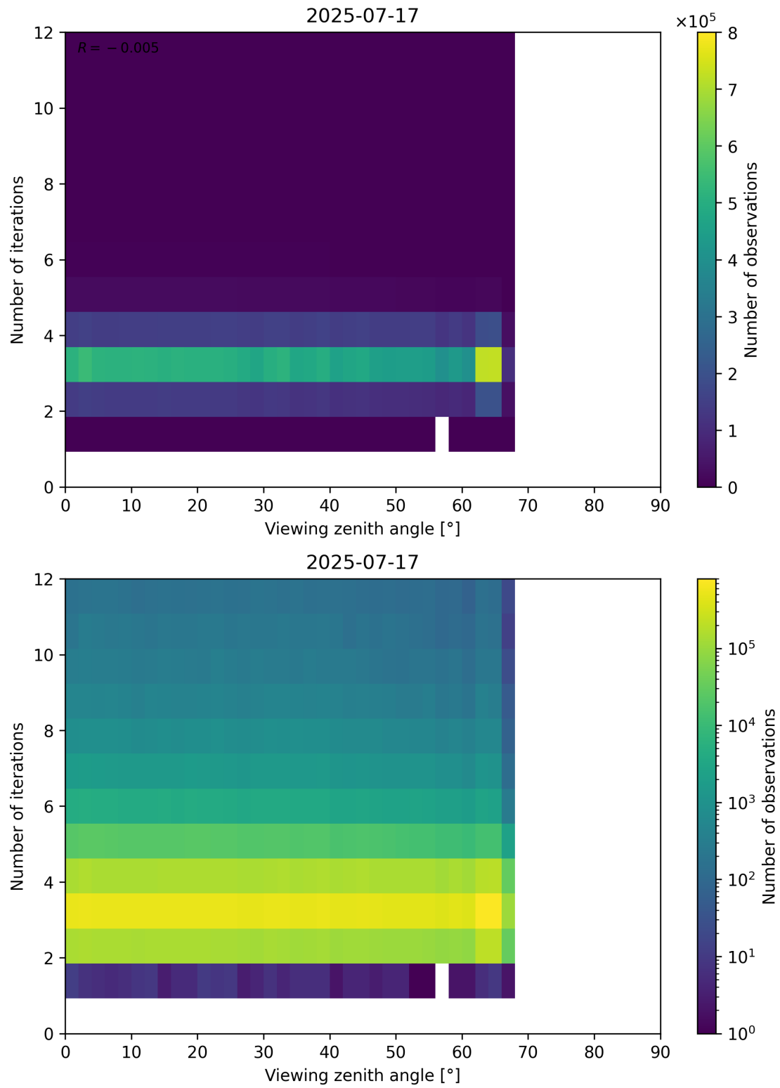
Figure 124: Scatter density plot of “Viewing zenith angle” against “Number of iterations” for 2025-07-16 to 2025-07-18.
