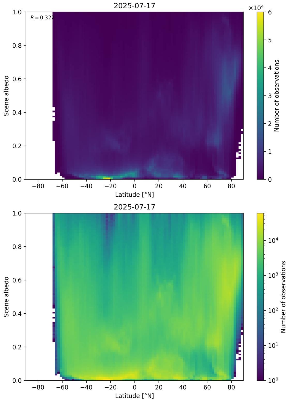
Figure 95: Scatter density plot of “Latitude” against “Scene albedo” for 2025-07-16 to 2025-07-18.
