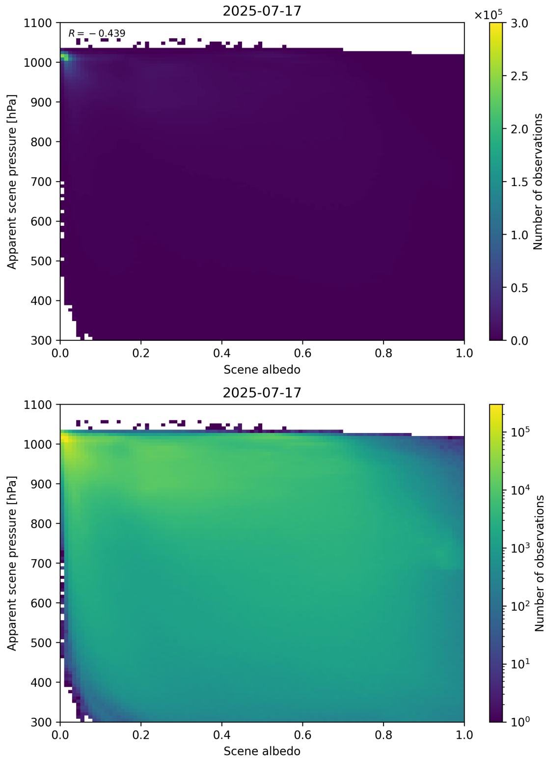
Figure 102: Scatter density plot of “Scene albedo” against “Apparent scene pressure” for 2025-07-16 to 2025-07-18.
