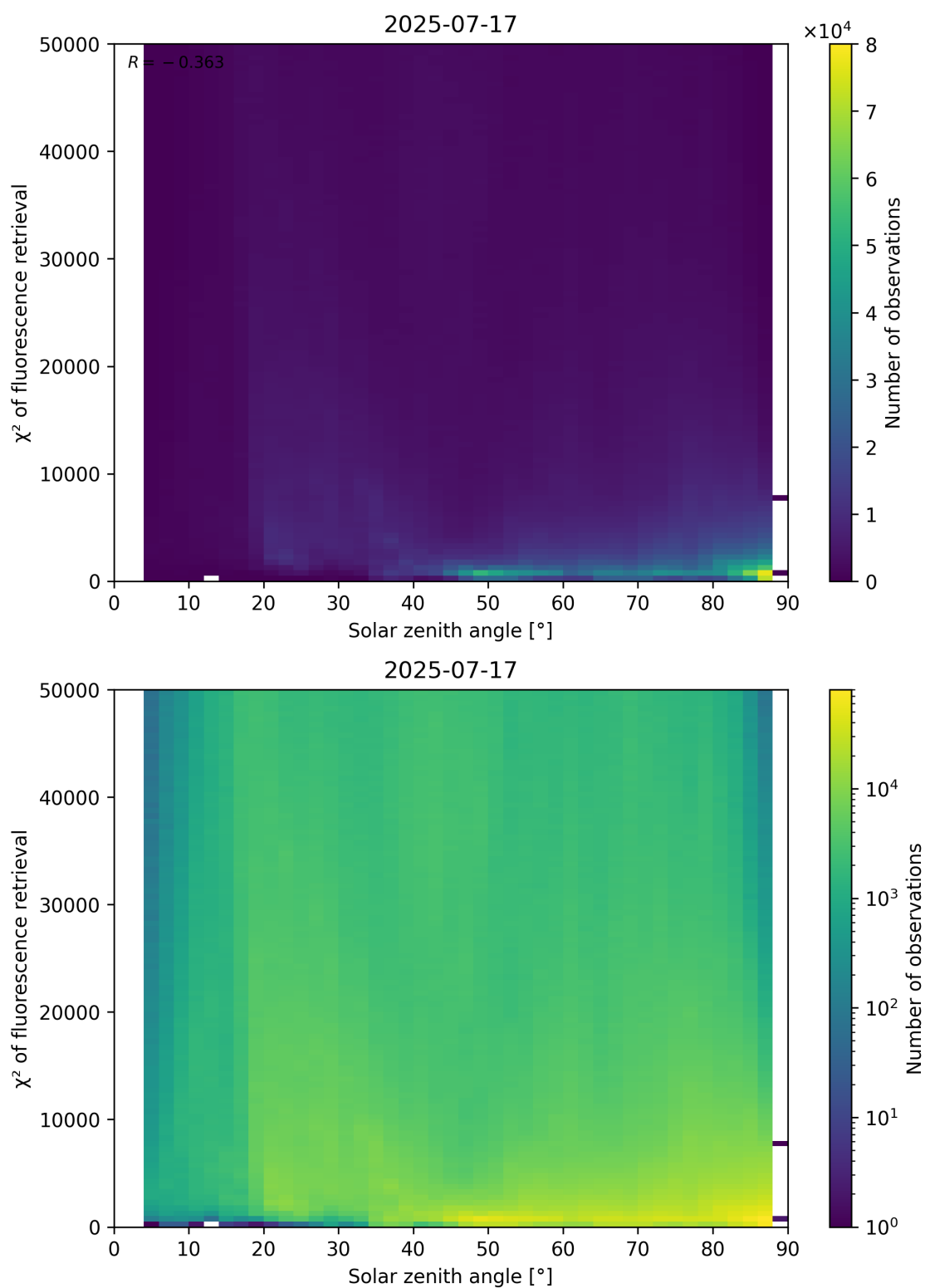
Figure 109: Scatter density plot of “Solar zenith angle” against “ \chi^2 of fluorescence retrieval” for 2025-07-16 to 2025-07-18.
