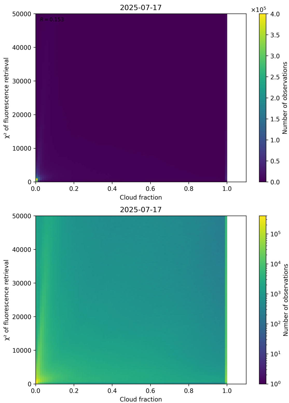
Figure 71: Scatter density plot of “Cloud fraction” against “ \chi^2 of fluorescence retrieval” for 2025-07-16 to 2025-07-18.
