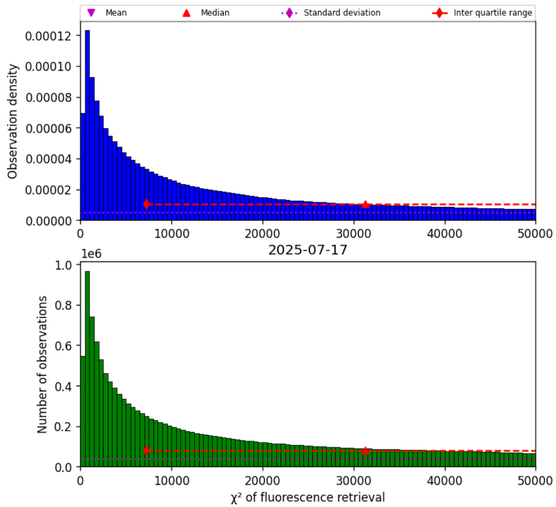
Figure 42: Histogram of “ \chi^2 of fluorescence retrieval” for 2025-07-16 to 2025-07-18
