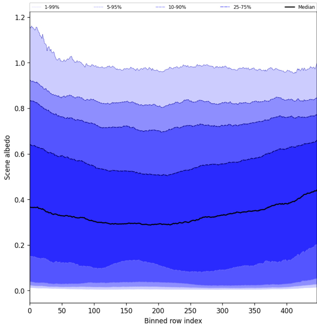
Figure 51: Along track statistics of “Scene albedo” for 2025-07-16 to 2025-07-18
