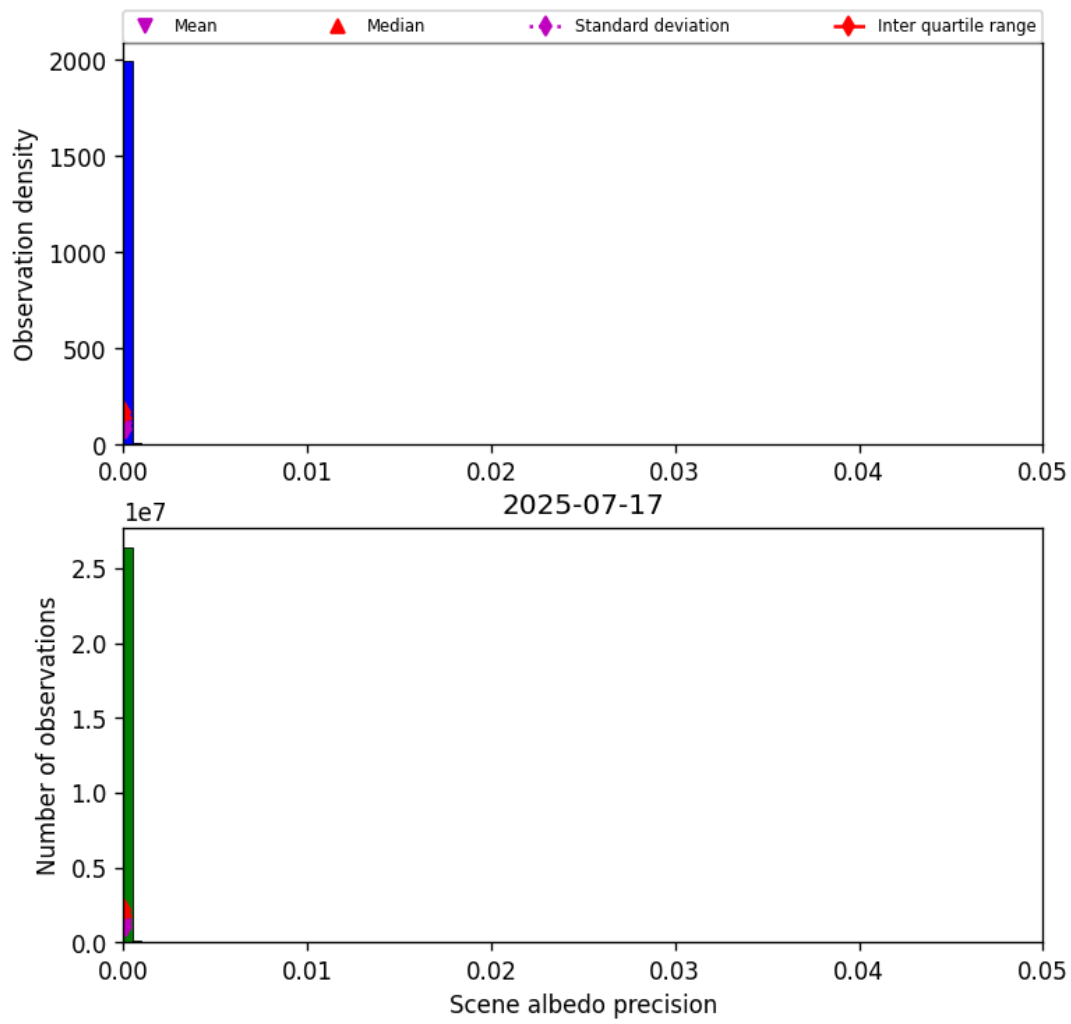
Figure 35: Histogram of “Scene albedo precision” for 2025-07-16 to 2025-07-18
