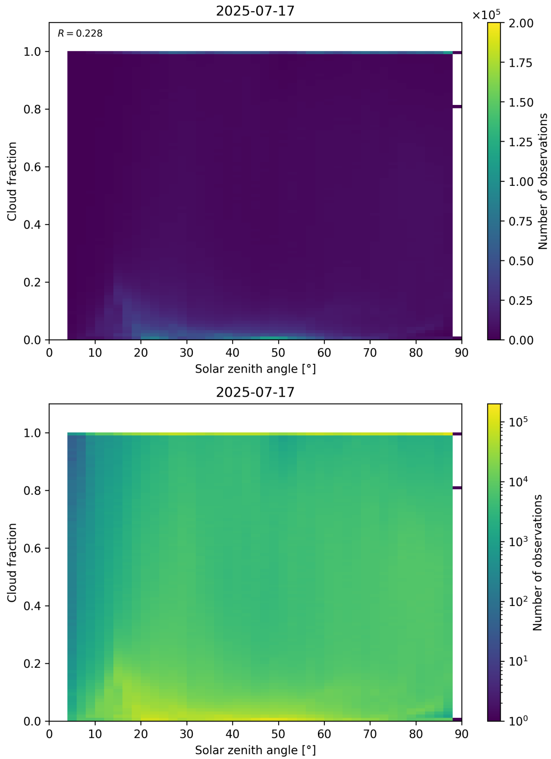
Figure 110: Scatter density plot of “Solar zenith angle” against “Cloud fraction” for 2025-07-16 to 2025-07-18.
