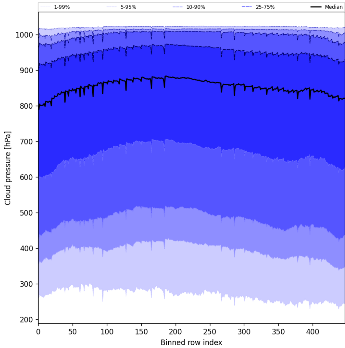
Figure 47: Along track statistics of “Cloud pressure” for 2025-07-16 to 2025-07-18
