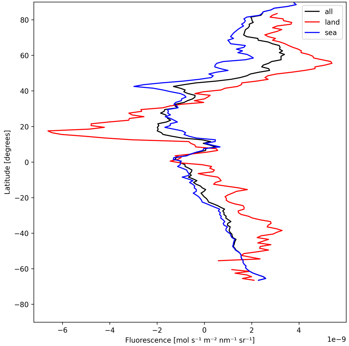
Figure 23: Zonal average of “Fluorescence” for 2025-07-16 to 2025-07-18.
