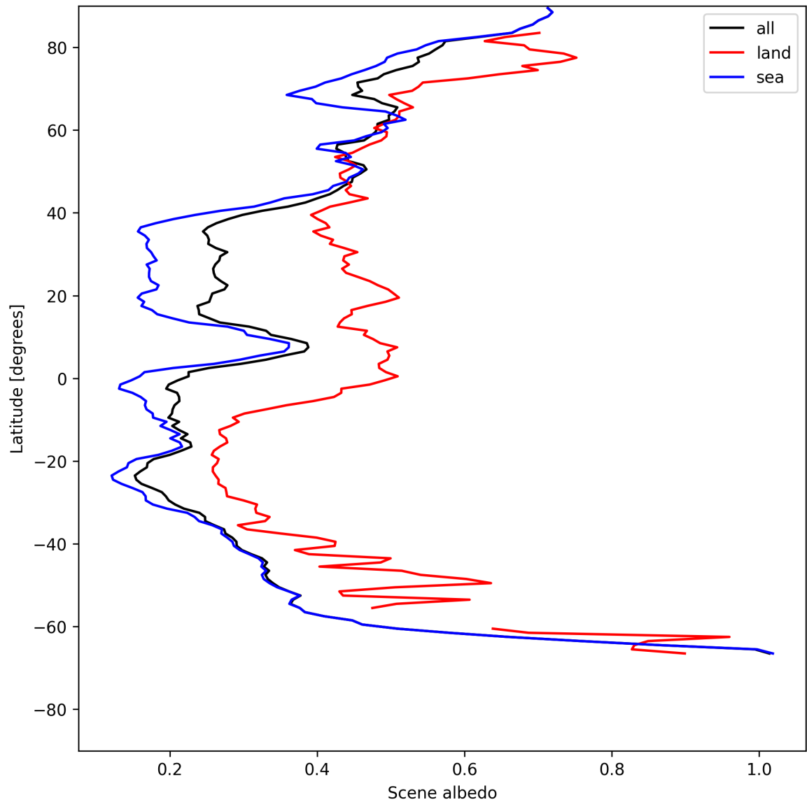
Figure 17: Zonal average of “Scene albedo” for 2025-07-16 to 2025-07-18.
