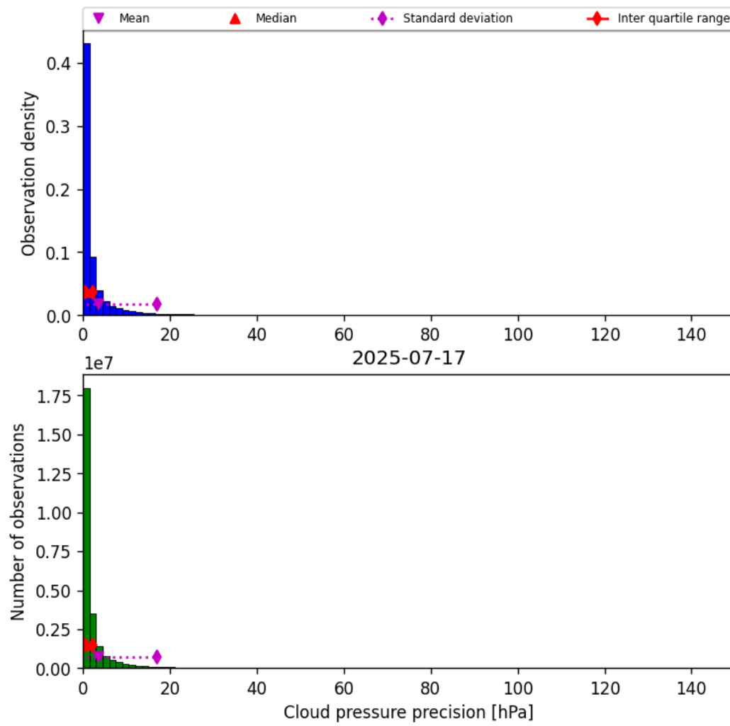
Figure 31: Histogram of “Cloud pressure precision” for 2025-07-16 to 2025-07-18
