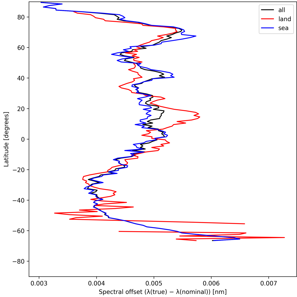
Figure 28: Zonal average of “Spectral offset ( \lambda_{\text{true}} - \lambda_{\text{nominal}} )” for 2025-07-16 to 2025-07-18.
