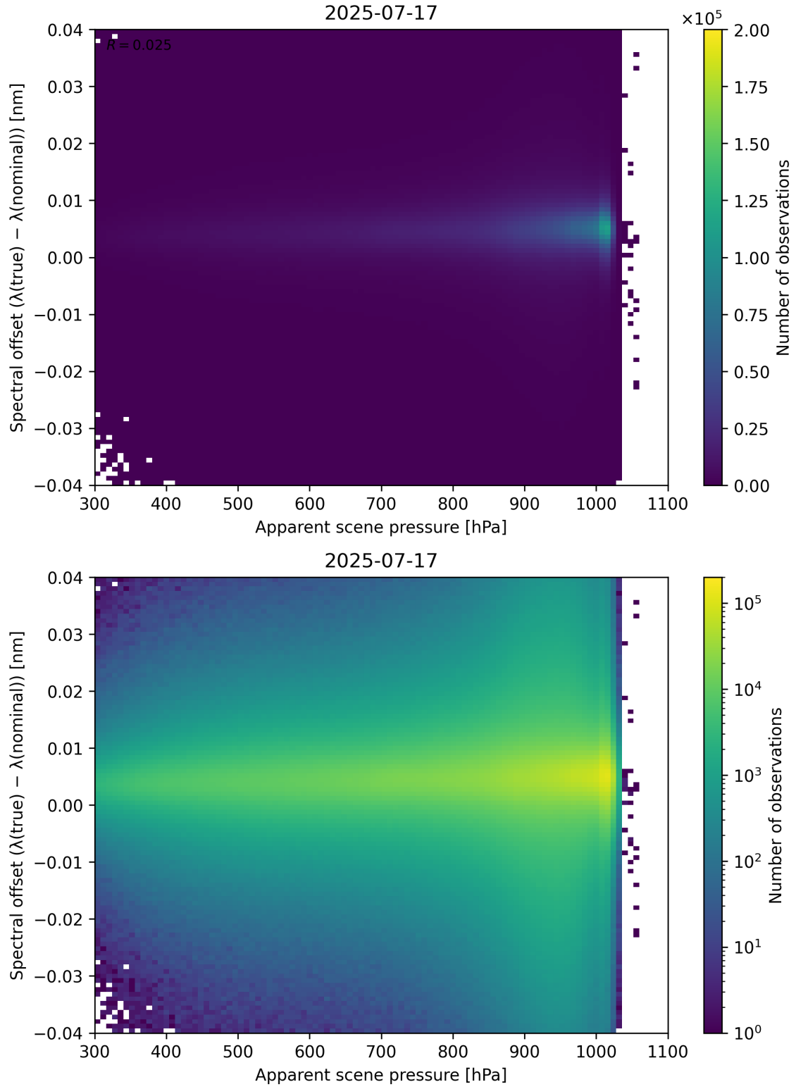
Figure 67: Scatter density plot of “Apparent scene pressure” against “Spectral offset ( \lambda_{\text{true}} - \lambda_{\text{nominal}} )” for 2025-07-16 to 2025-07-18.
