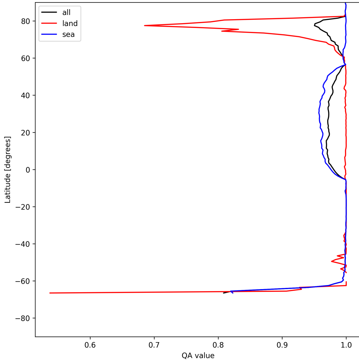
Figure 12: Zonal average of "QA value" for 2025-07-16 to 2025-07-18.
