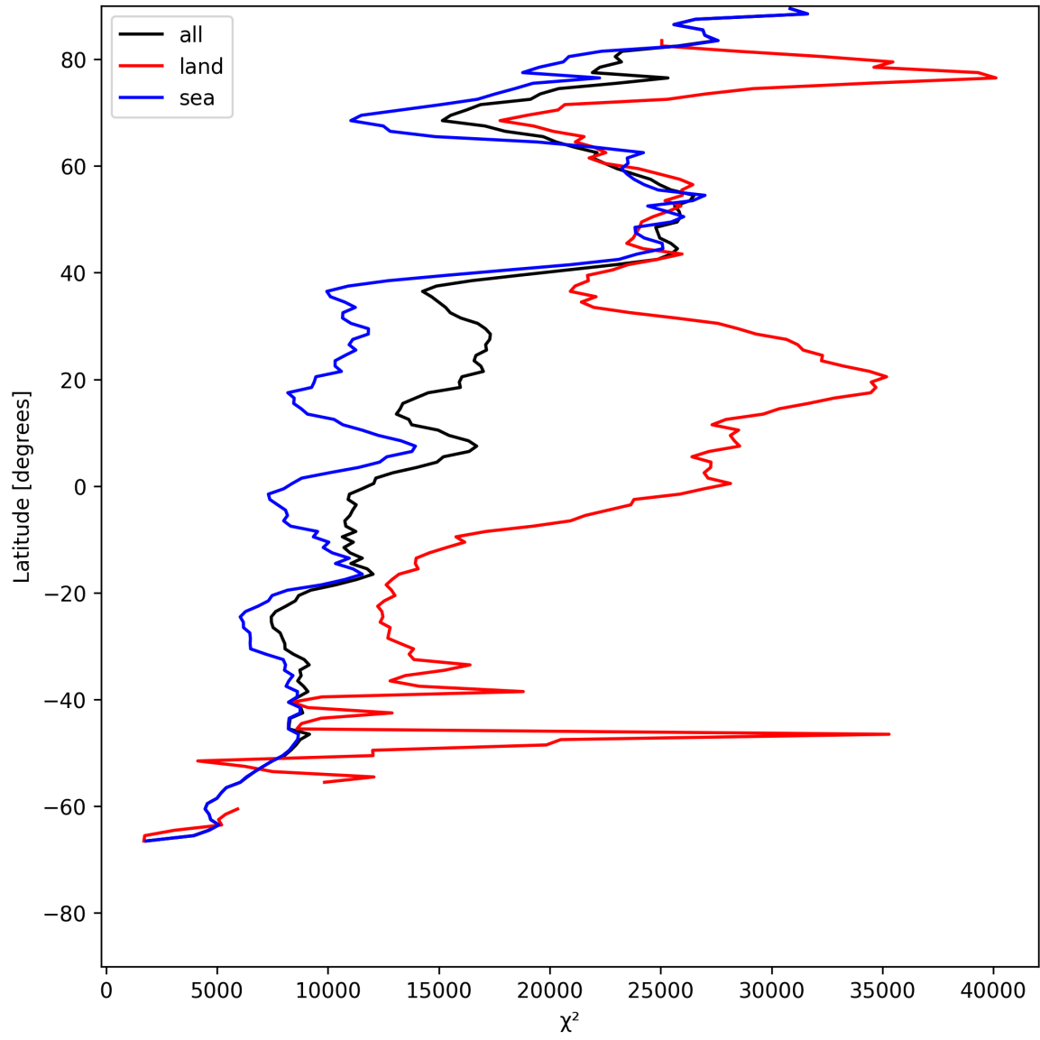
Figure 21: Zonal average of “ \chi^2 ” for 2025-07-16 to 2025-07-18.
