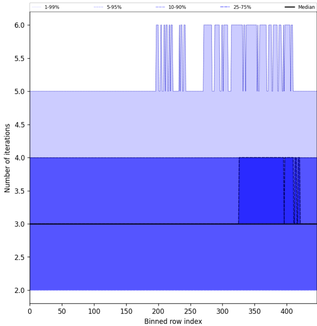
Figure 56: Along track statistics of “Number of iterations” for 2025-07-16 to 2025-07-18
