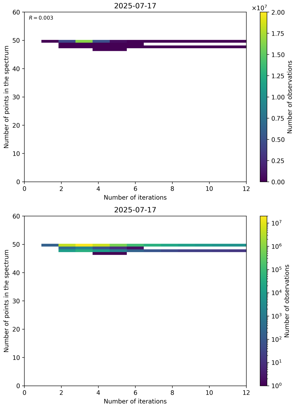
Figure 99: Scatter density plot of “Number of iterations” against “Number of points in the spectrum” for 2025-07-16 to 2025-07-18.
