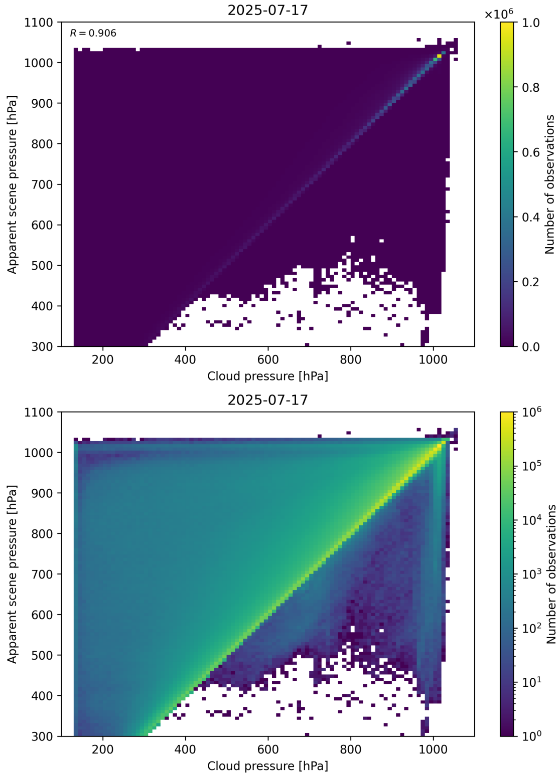
Figure 77: Scatter density plot of “Cloud pressure” against “Apparent scene pressure” for 2025-07-16 to 2025-07-18.
