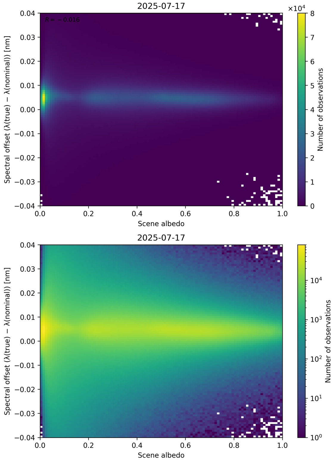
Figure 107: Scatter density plot of “Scene albedo” against “Spectral offset ( \lambda_{\text{true}} - \lambda_{\text{nominal}} )” for 2025-07-16 to 2025-07-18.
