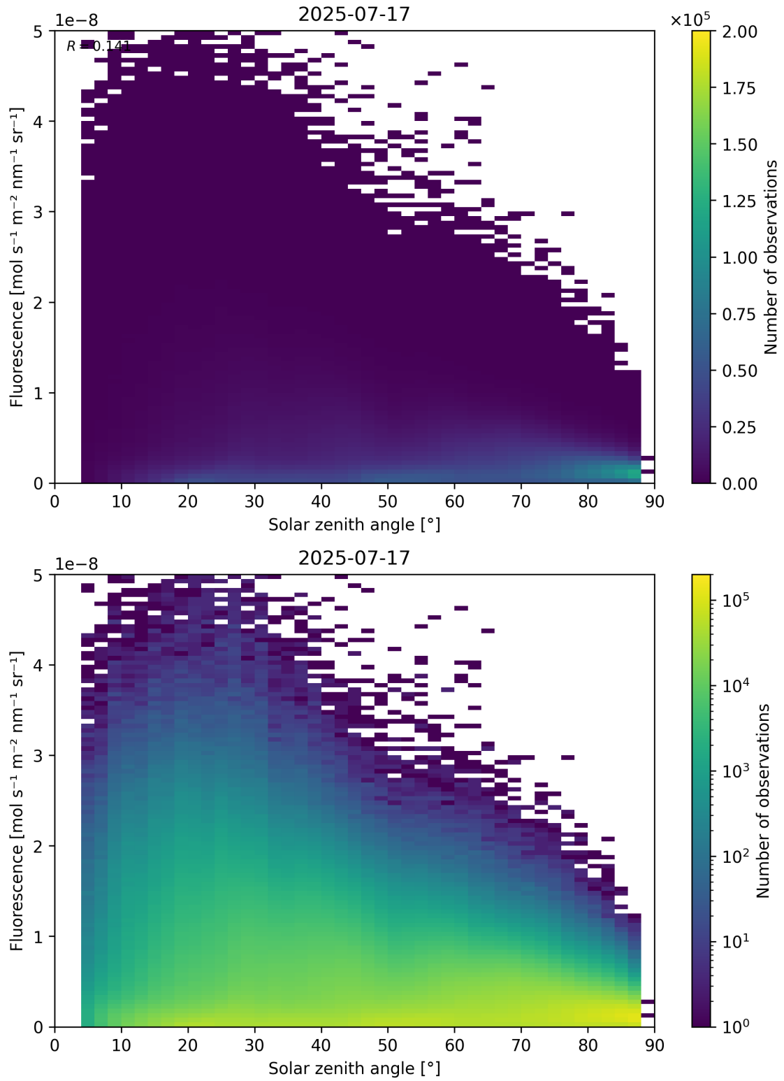
Figure 112: Scatter density plot of “Solar zenith angle” against “Fluorescence” for 2025-07-16 to 2025-07-18.
