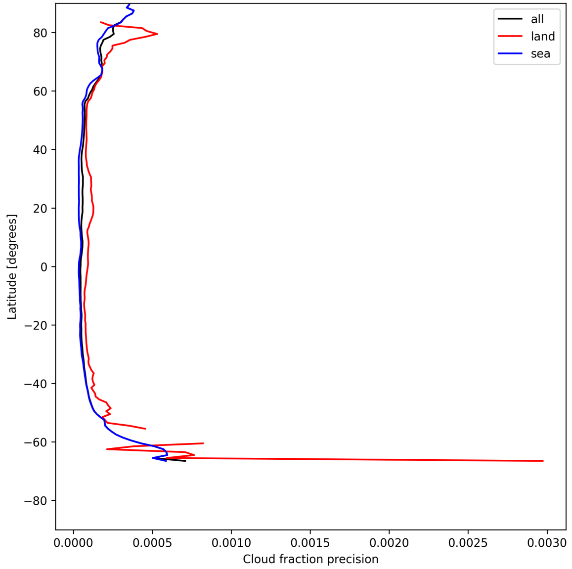
Figure 16: Zonal average of “Cloud fraction precision” for 2025-07-16 to 2025-07-18.
