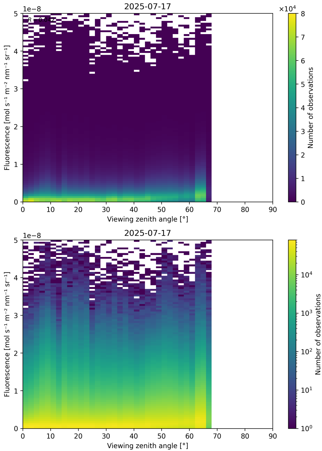
Figure 122: Scatter density plot of “Viewing zenith angle” against “Fluorescence” for 2025-07-16 to 2025-07-18.
