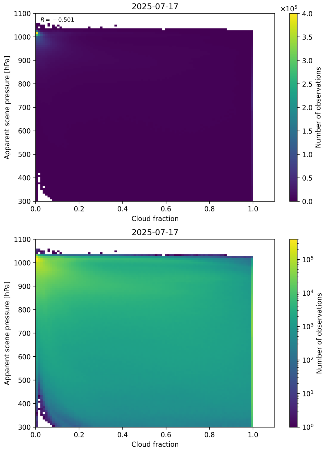
Figure 70: Scatter density plot of “Cloud fraction” against “Apparent scene pressure” for 2025-07-16 to 2025-07-18.
