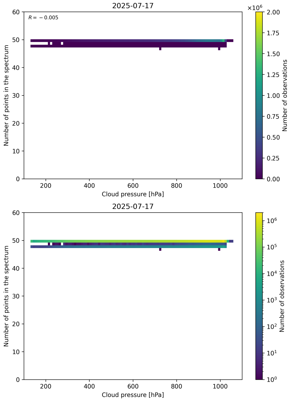
Figure 82: Scatter density plot of “Cloud pressure” against “Number of points in the spectrum” for 2025-07-16 to 2025-07-18.
