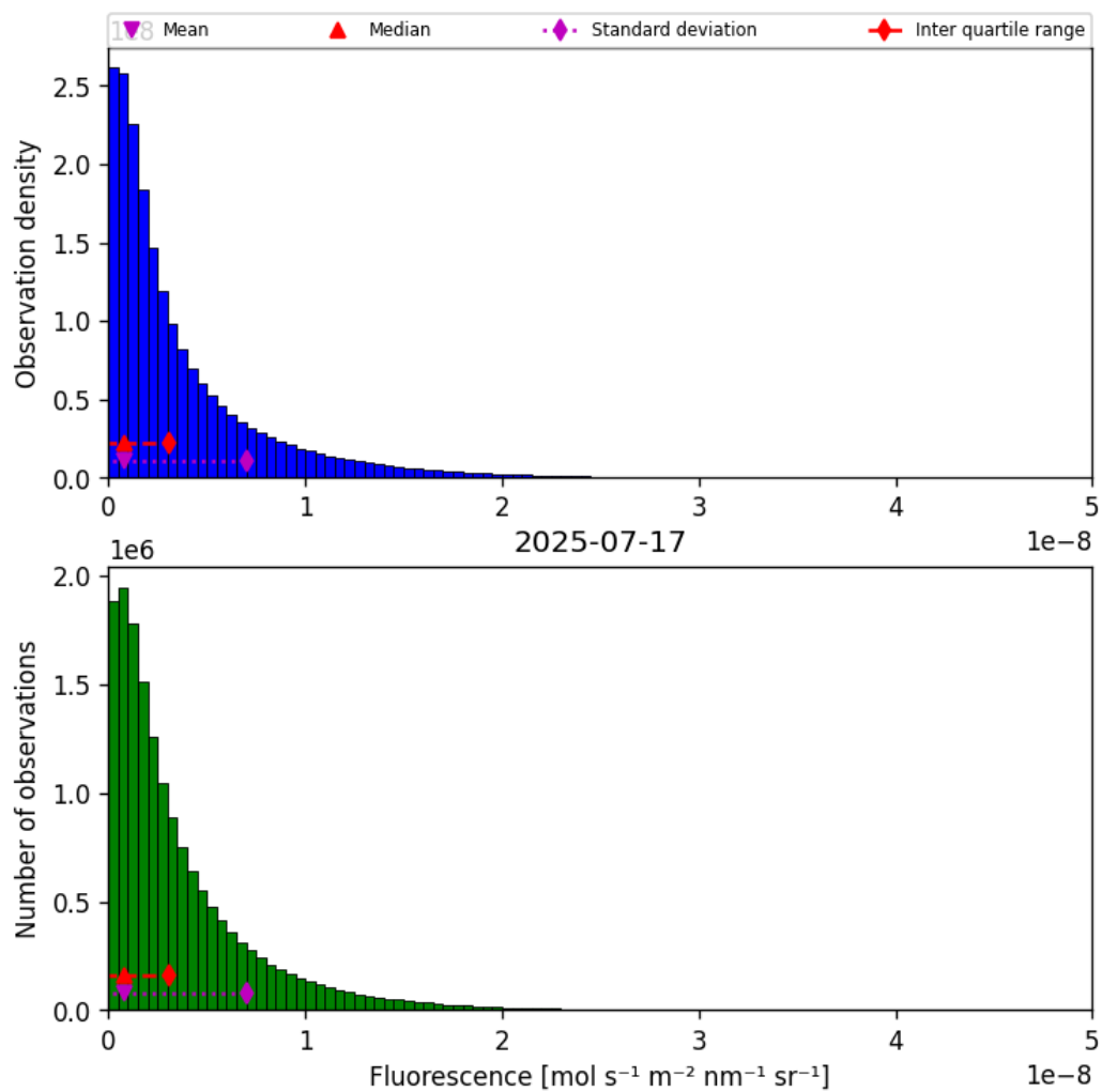
Figure 40: Histogram of “Fluorescence” for 2025-07-16 to 2025-07-18
