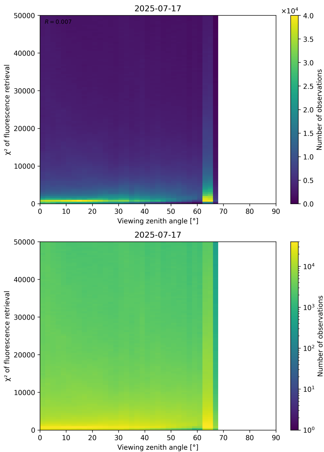
Figure 119: Scatter density plot of “Viewing zenith angle” against “ \chi^2 of fluorescence retrieval” for 2025-07-16 to 2025-07-18.
