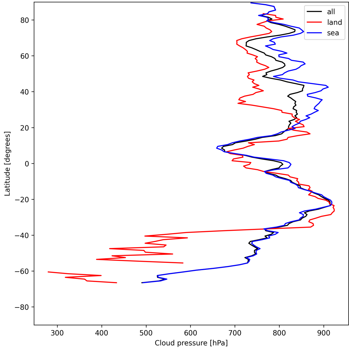
Figure 13: Zonal average of “Cloud pressure” for 2025-07-16 to 2025-07-18.
