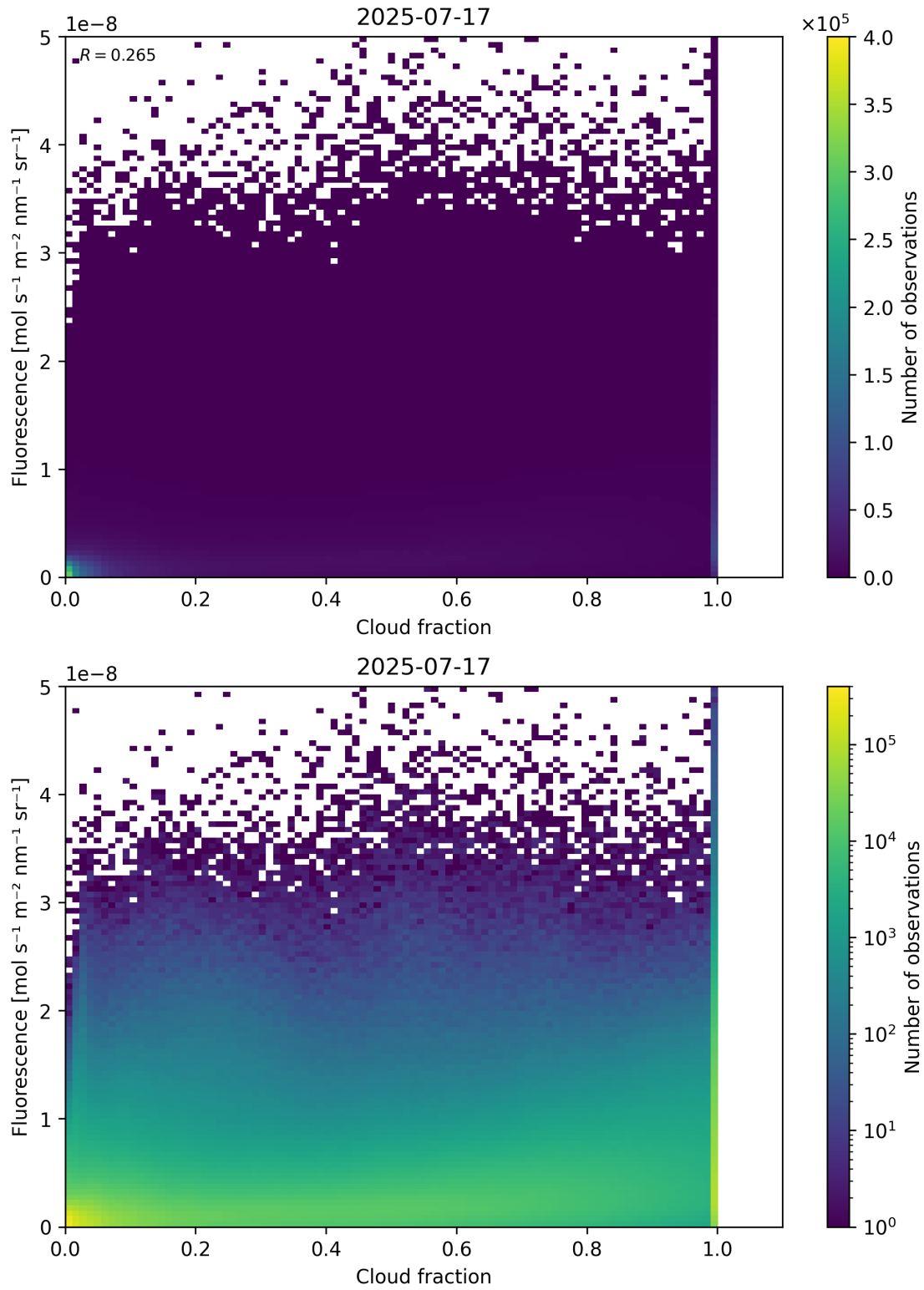
Figure 72: Scatter density plot of “Cloud fraction” against “Fluorescence” for 2025-07-16 to 2025-07-18.
