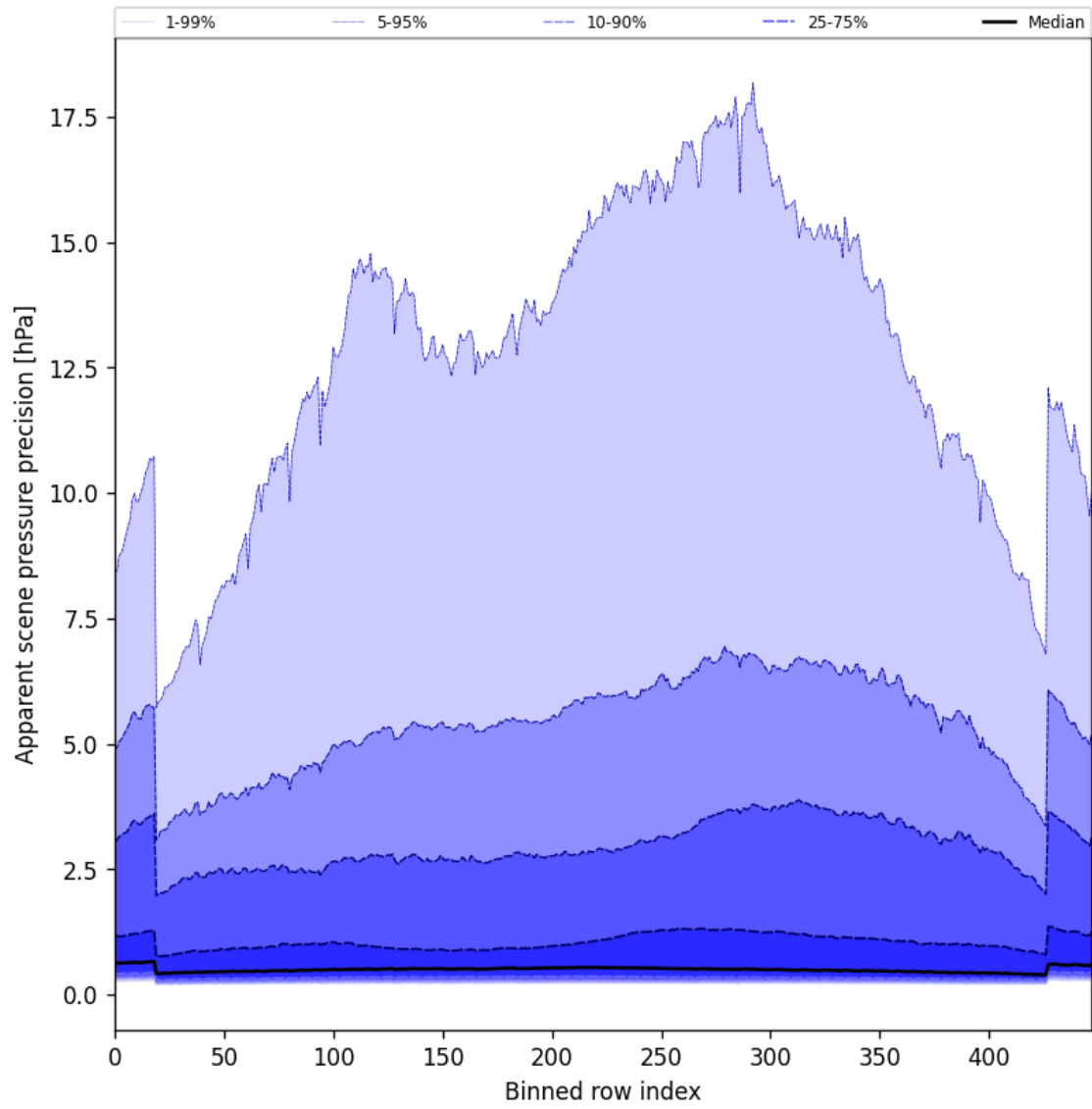
Figure 54: Along track statistics of “Apparent scene pressure precision” for 2025-07-16 to 2025-07-18
