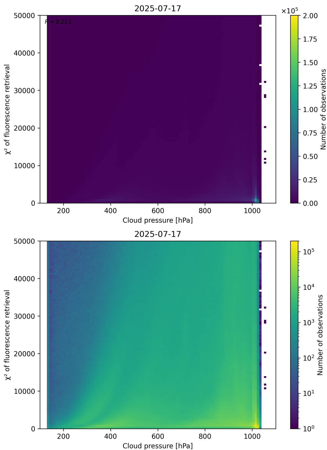
Figure 78: Scatter density plot of “Cloud pressure” against “ \chi^2 of fluorescence retrieval” for 2025-07-16 to 2025-07-18.
