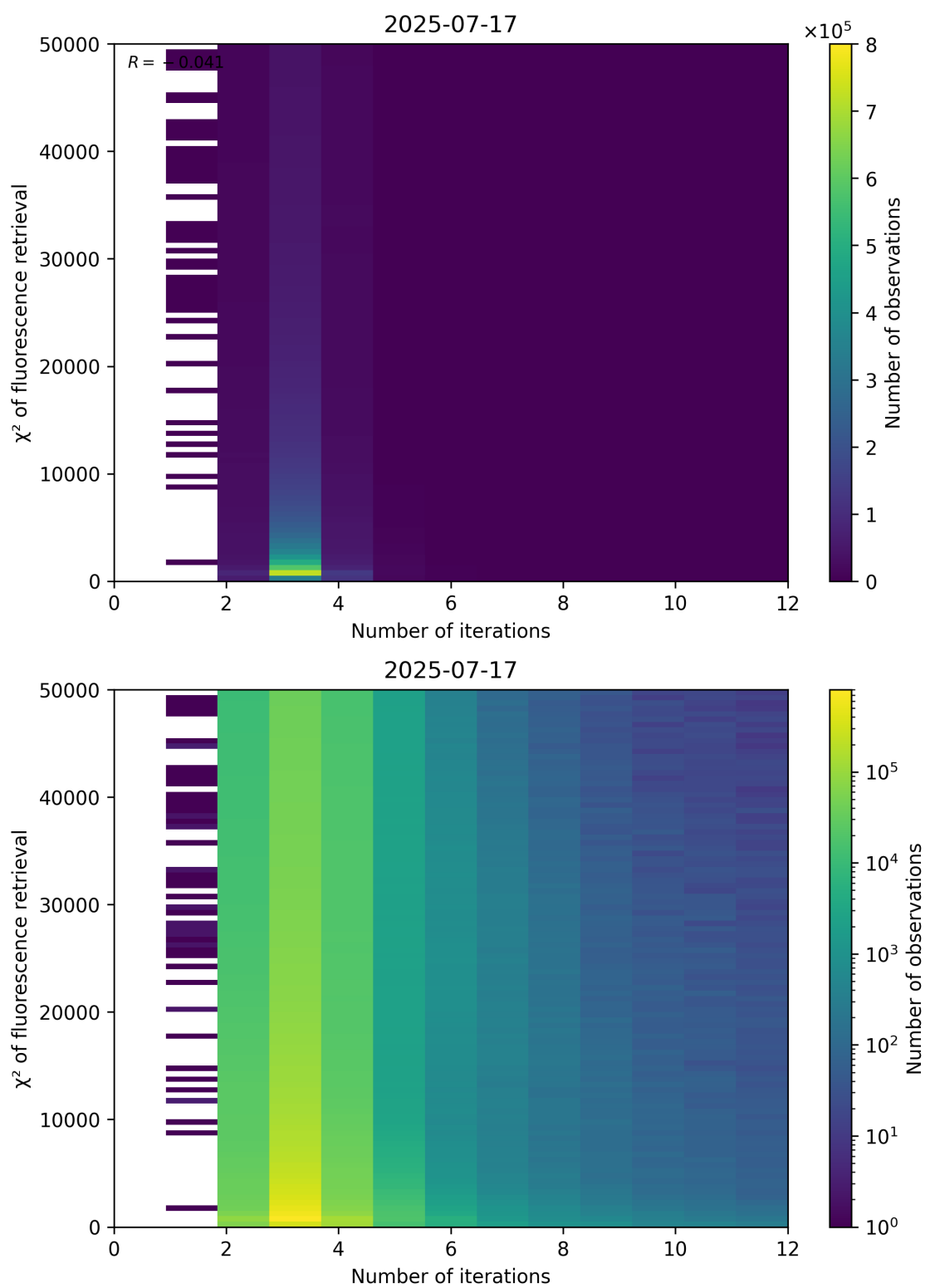
Figure 97: Scatter density plot of “Number of iterations” against “ \chi^2 of fluorescence retrieval” for 2025-07-16 to 2025-07-18.
