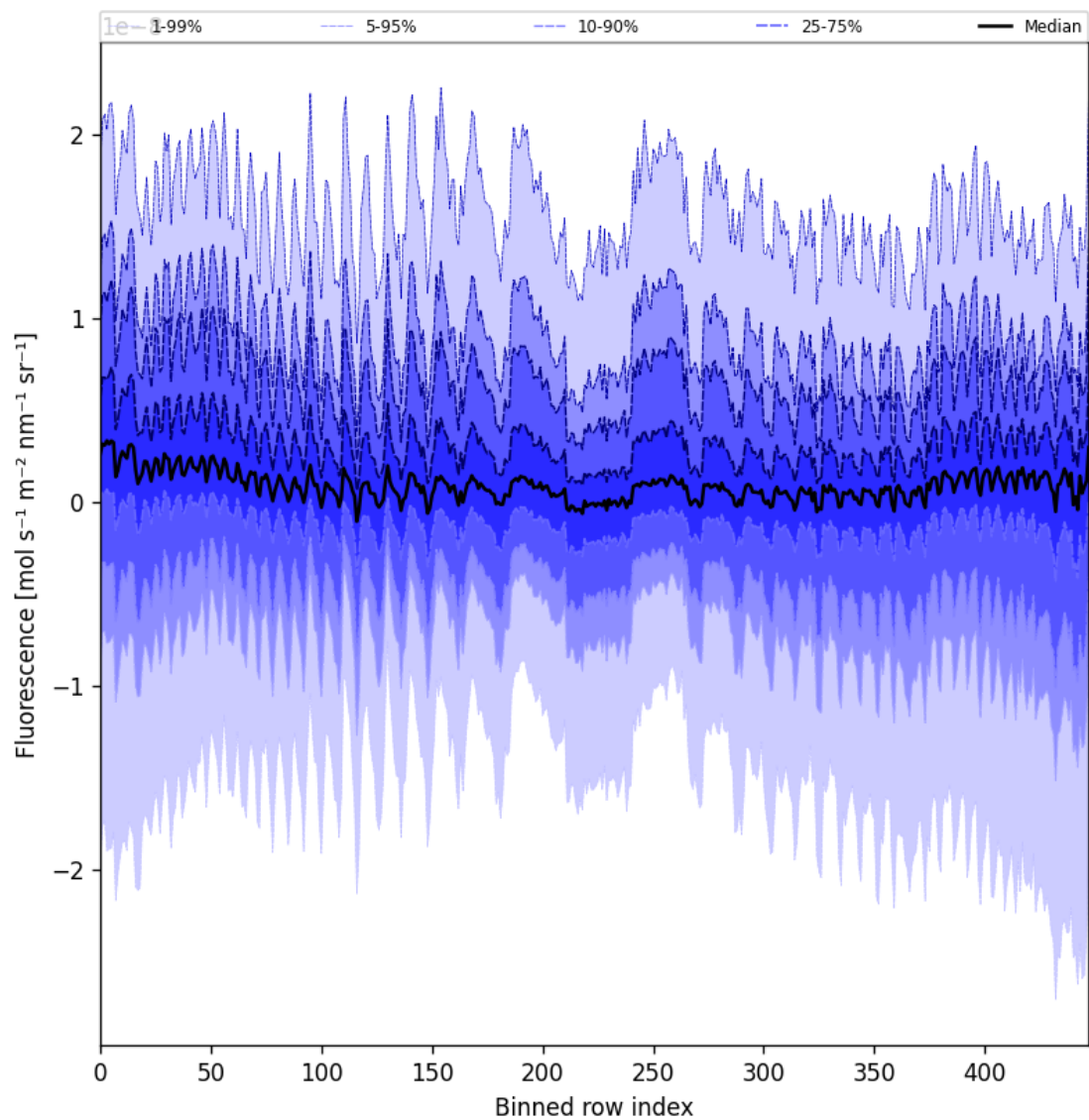
Figure 57: Along track statistics of “Fluorescence” for 2025-07-16 to 2025-07-18
