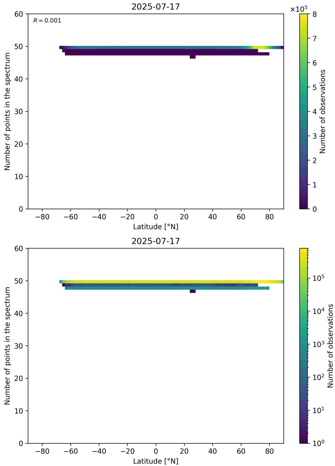
Figure 94: Scatter density plot of “Latitude” against “Number of points in the spectrum” for 2025-07-16 to 2025-07-18.
