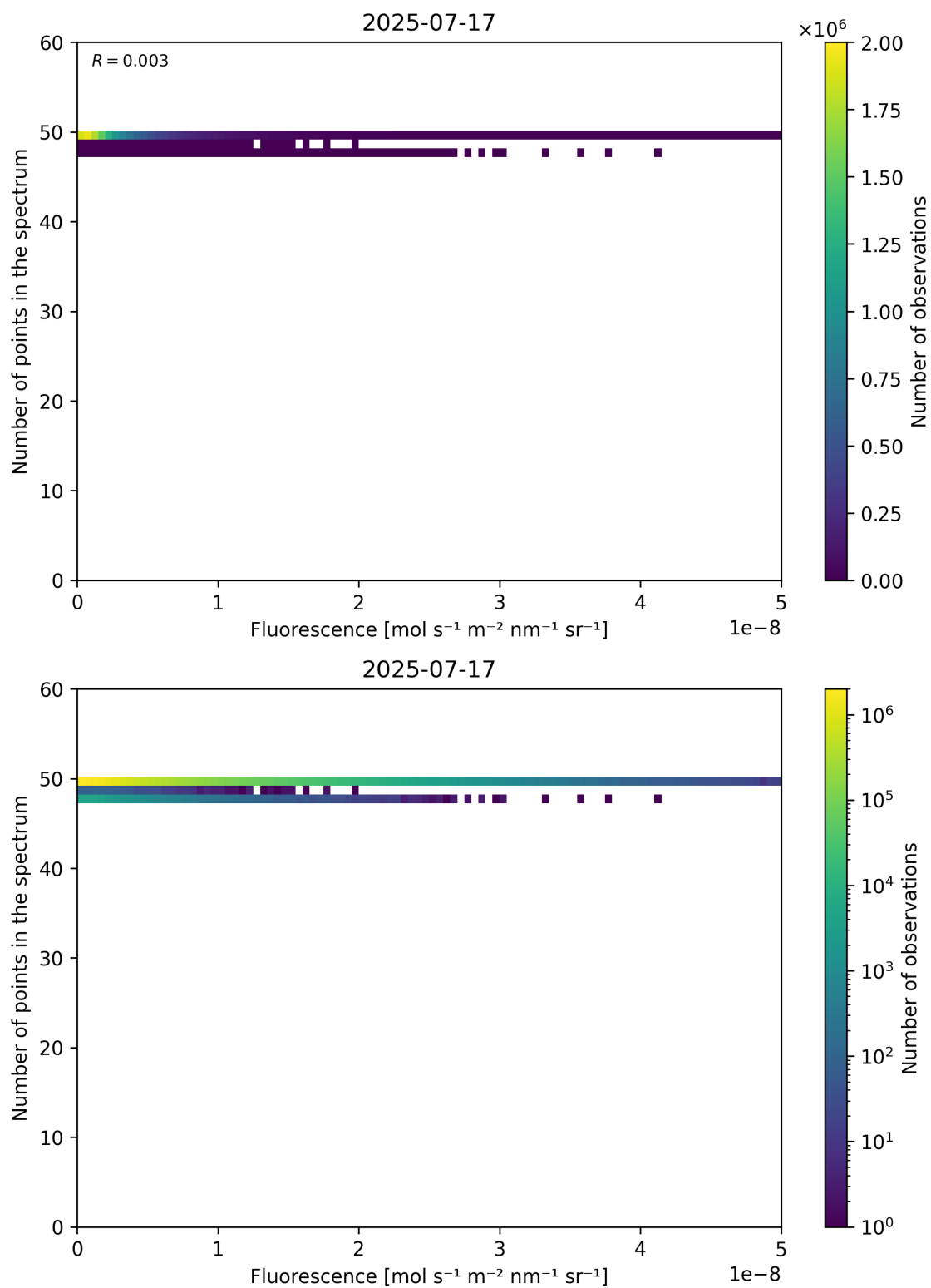
Figure 86: Scatter density plot of “Fluorescence” against “Number of points in the spectrum” for 2025-07-16 to 2025-07-18.
