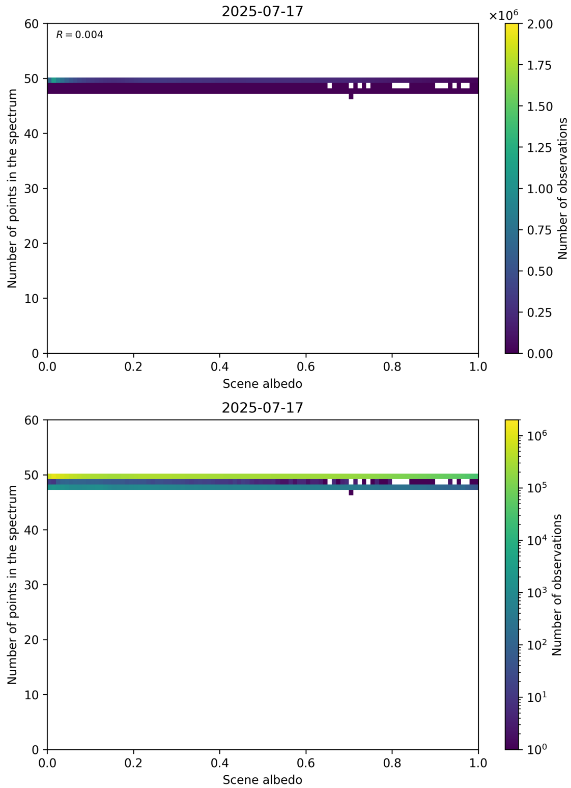
Figure 106: Scatter density plot of “Scene albedo” against “Number of points in the spectrum” for 2025-07-16 to 2025-07-18.
