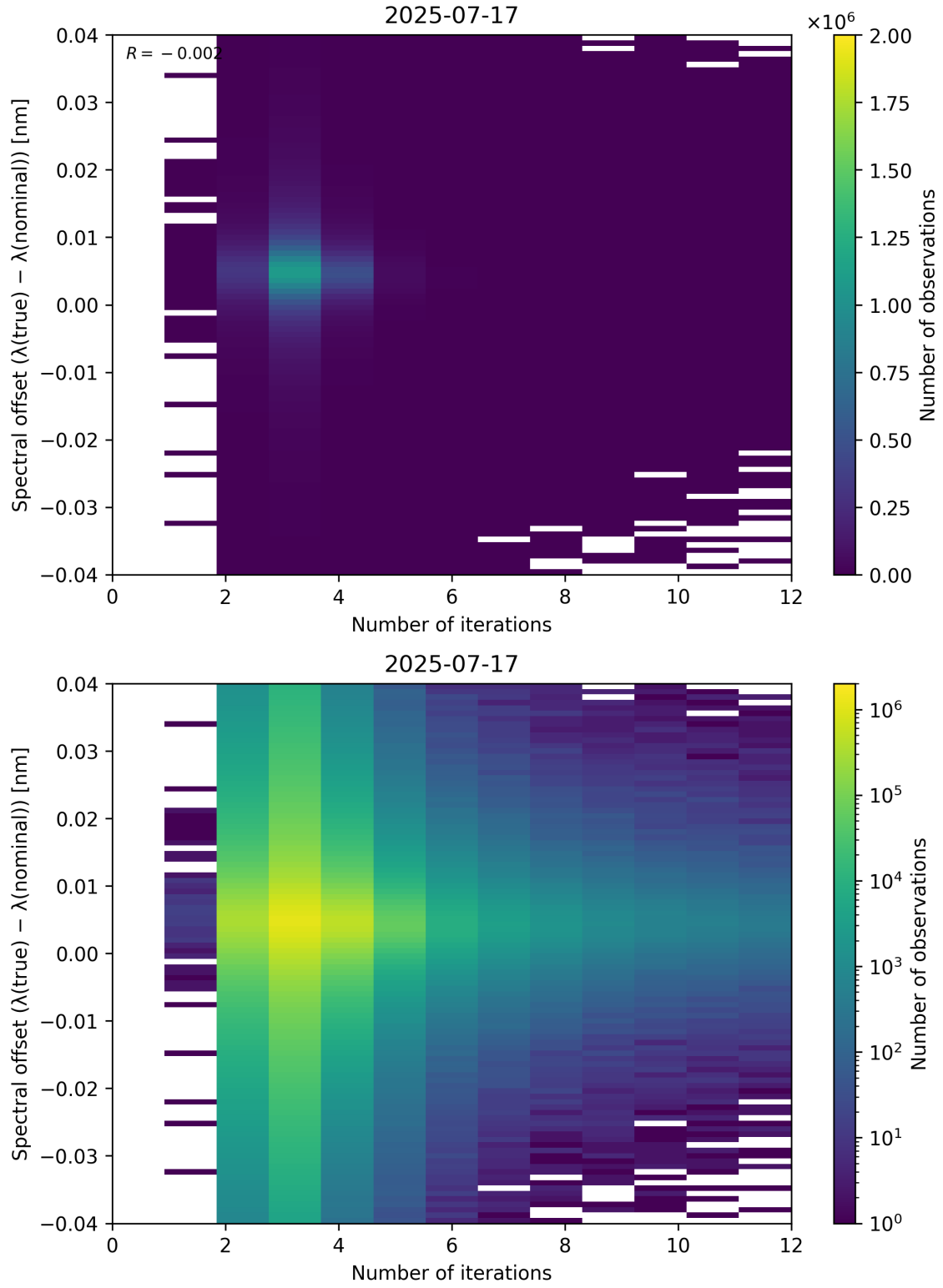
Figure 100: Scatter density plot of “Number of iterations” against “Spectral offset ( \lambda_{\text{true}} - \lambda_{\text{nominal}} )” for 2025-07-16 to 2025-07-18.
