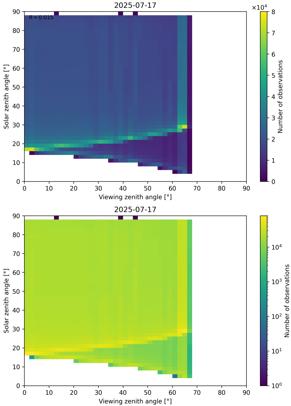
Figure 127: Scatter density plot of “Viewing zenith angle” against “Solar zenith angle” for 2025-07-16 to 2025-07-18.
