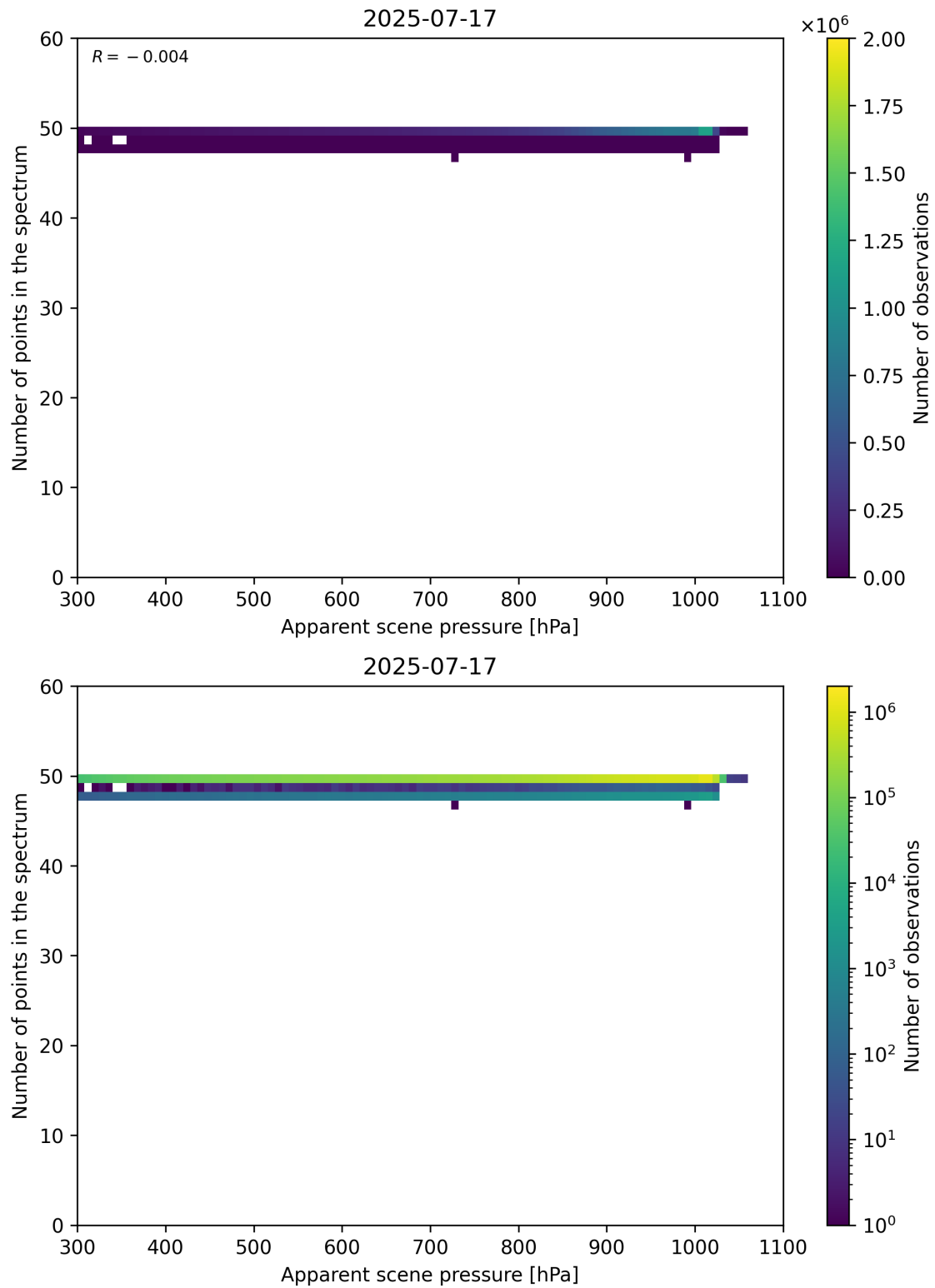
Figure 66: Scatter density plot of “Apparent scene pressure” against “Number of points in the spectrum” for 2025-07-16 to 2025-07-18.
