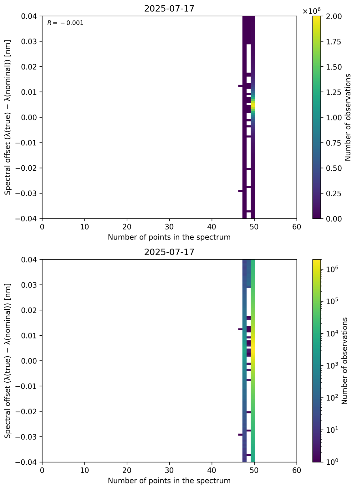
Figure 101: Scatter density plot of “Number of points in the spectrum” against “Spectral offset ( \lambda_{\text{true}} - \lambda_{\text{nominal}} )” for 2025-07-16 to 2025-07-18.
