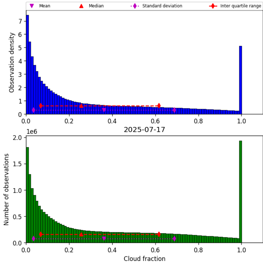
Figure 32: Histogram of “Cloud fraction” for 2025-07-16 to 2025-07-18
