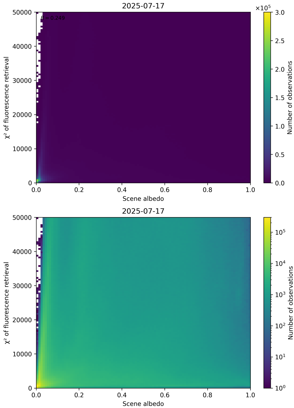
Figure 103: Scatter density plot of “Scene albedo” against “ \chi^2 of fluorescence retrieval” for 2025-07-16 to 2025-07-18.
