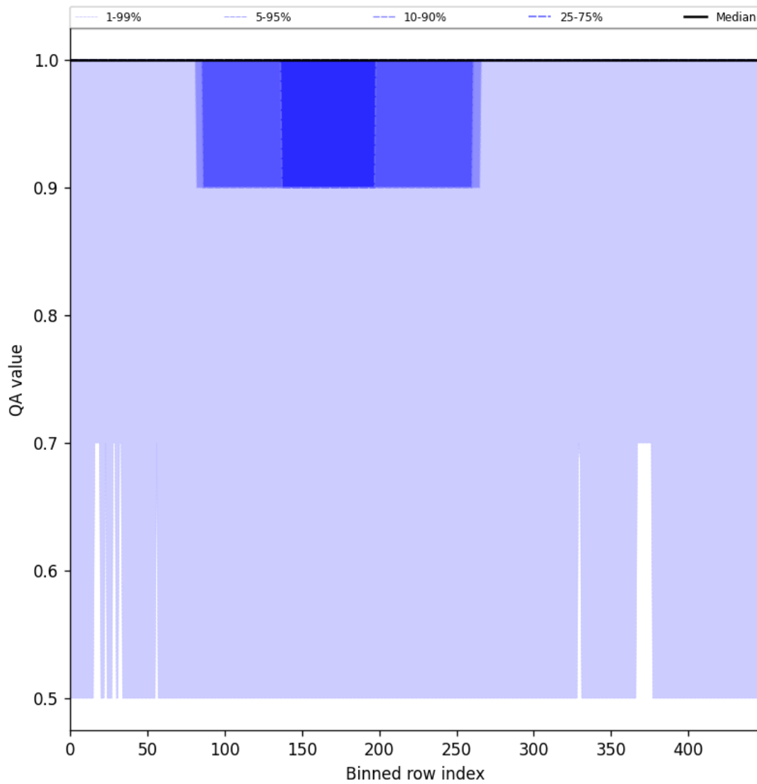
Figure 46: Along track statistics of “QA value” for 2025-07-16 to 2025-07-18
