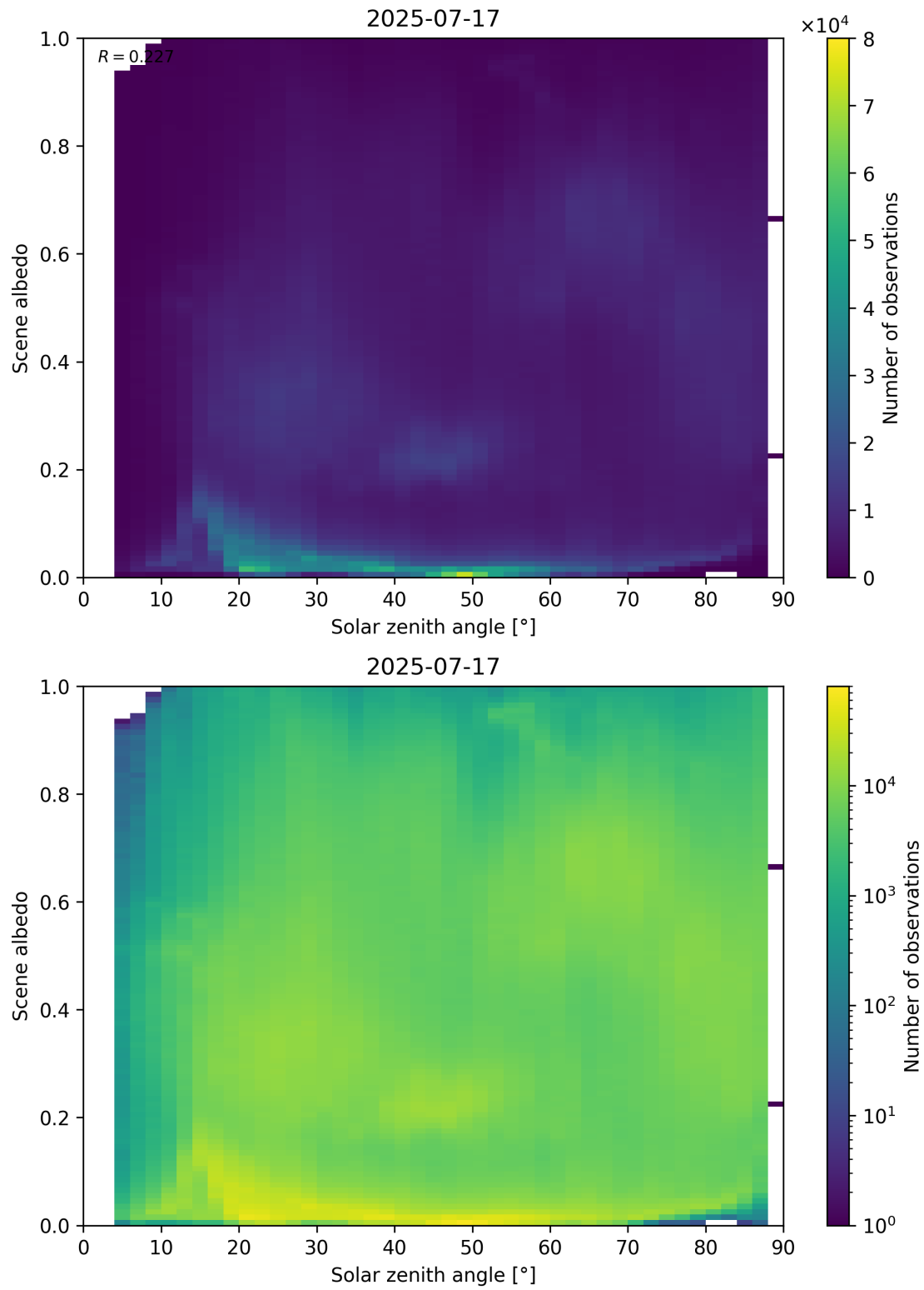
Figure 116: Scatter density plot of “Solar zenith angle” against “Scene albedo” for 2025-07-16 to 2025-07-18.
