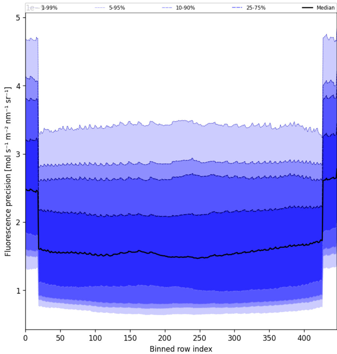
Figure 58: Along track statistics of “Fluorescence precision” for 2025-07-16 to 2025-07-18
