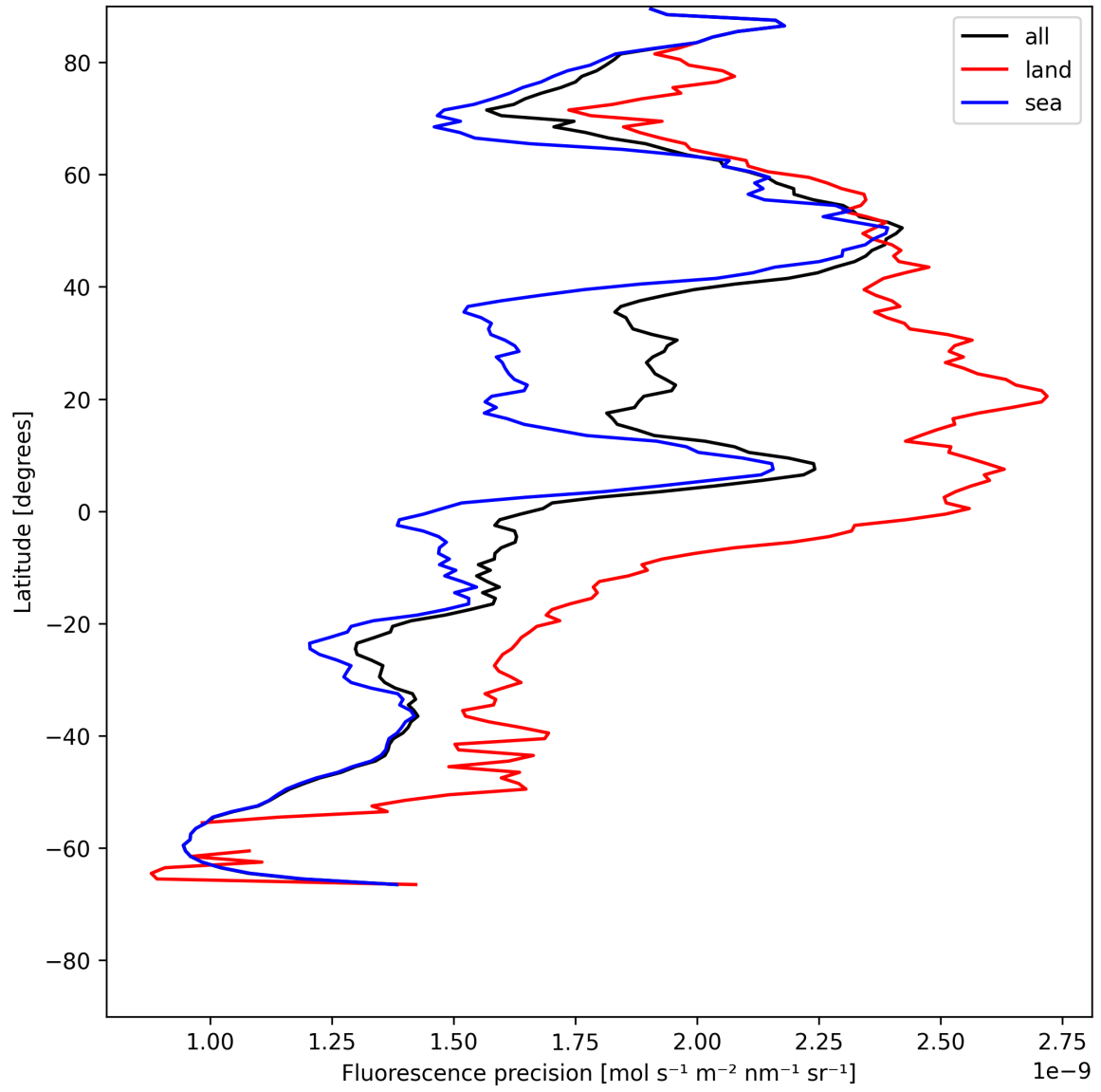
Figure 24: Zonal average of “Fluorescence precision” for 2025-07-16 to 2025-07-18.
