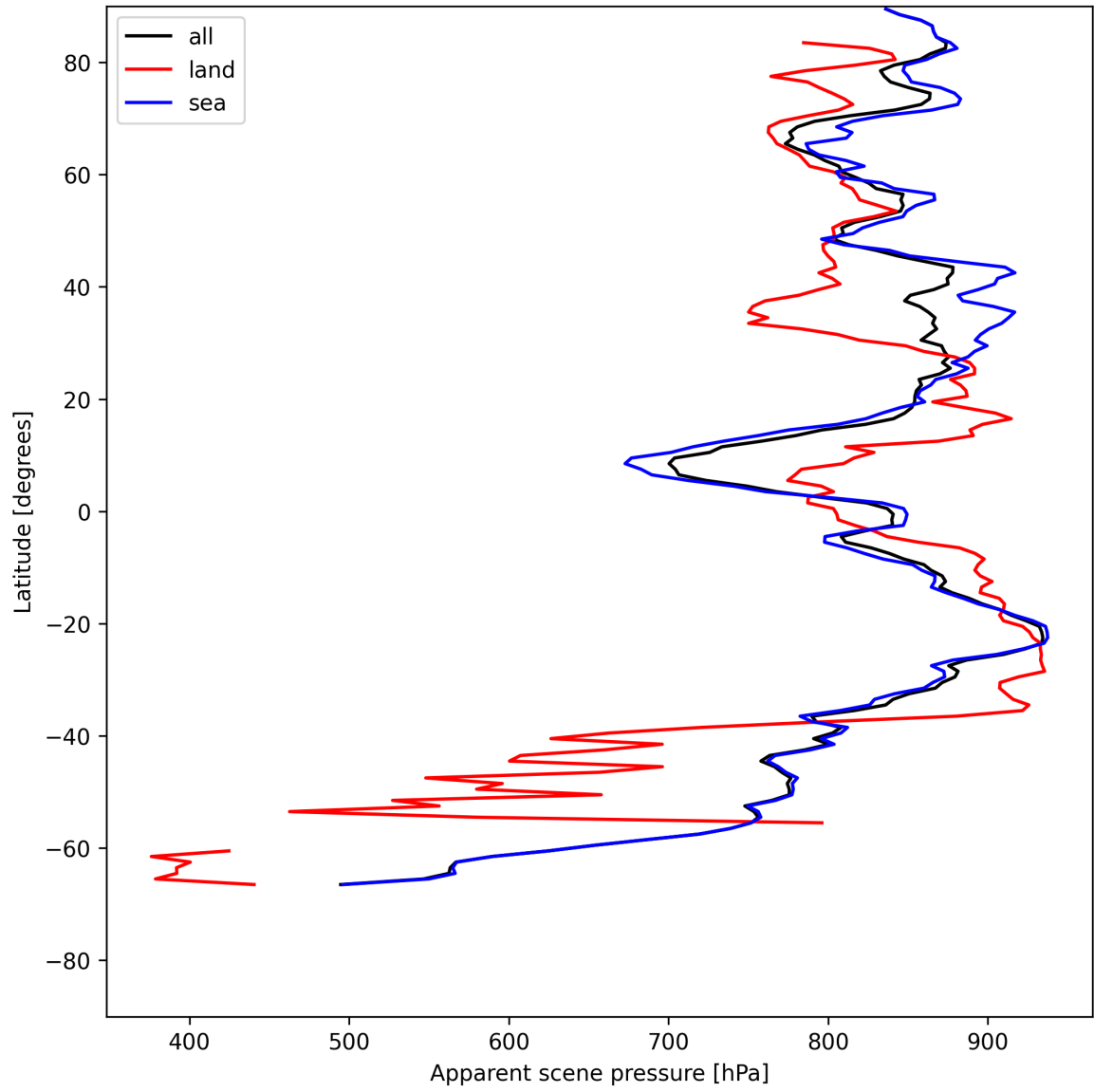
Figure 19: Zonal average of “Apparent scene pressure” for 2025-07-16 to 2025-07-18.
