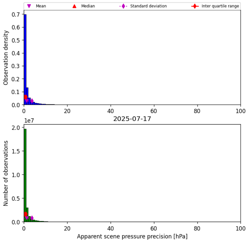
Figure 37: Histogram of “Apparent scene pressure precision” for 2025-07-16 to 2025-07-18
