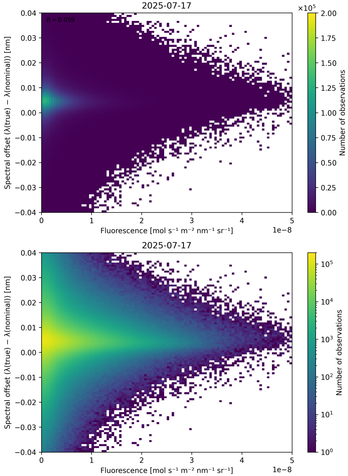
Figure 87: Scatter density plot of “Fluorescence” against “Spectral offset ( \lambda_{\text{true}} - \lambda_{\text{nominal}} )” for 2025-07-16 to 2025-07-18.
