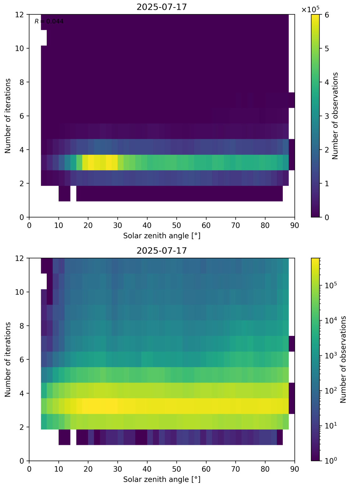
Figure 114: Scatter density plot of “Solar zenith angle” against “Number of iterations” for 2025-07-16 to 2025-07-18.
