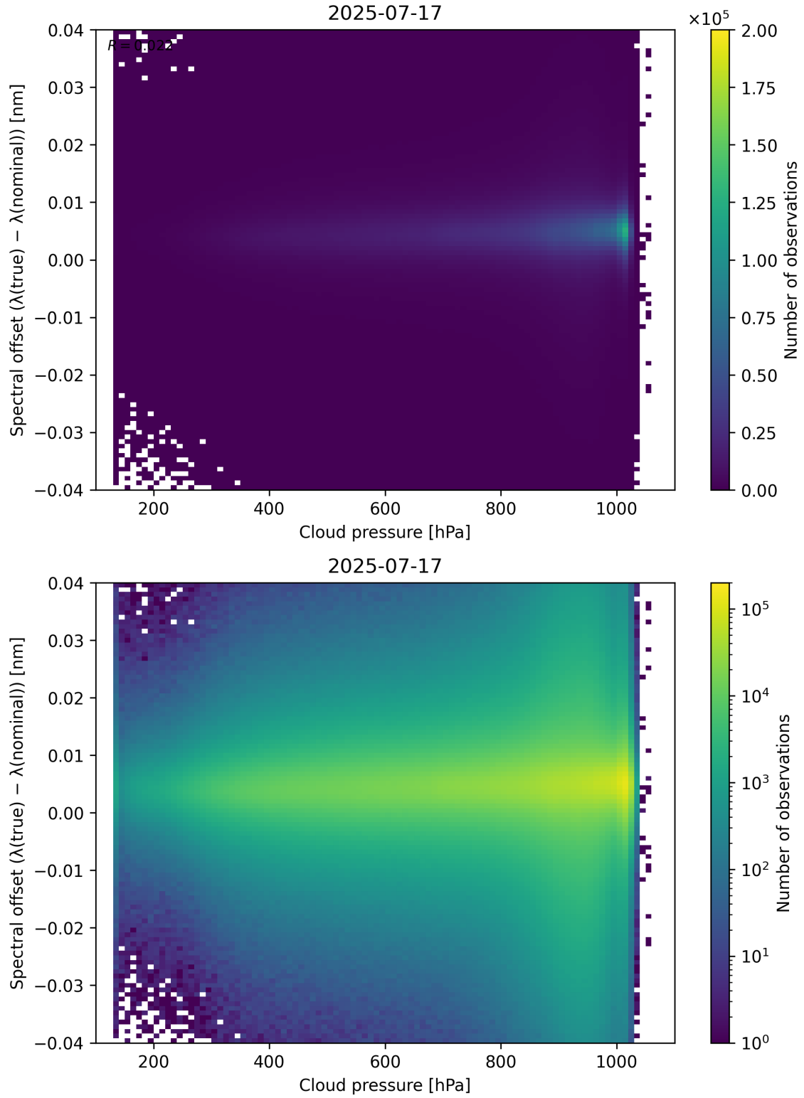
Figure 84: Scatter density plot of “Cloud pressure” against “Spectral offset ( \lambda_{\text{true}} - \lambda_{\text{nominal}} )” for 2025-07-16 to 2025-07-18.
