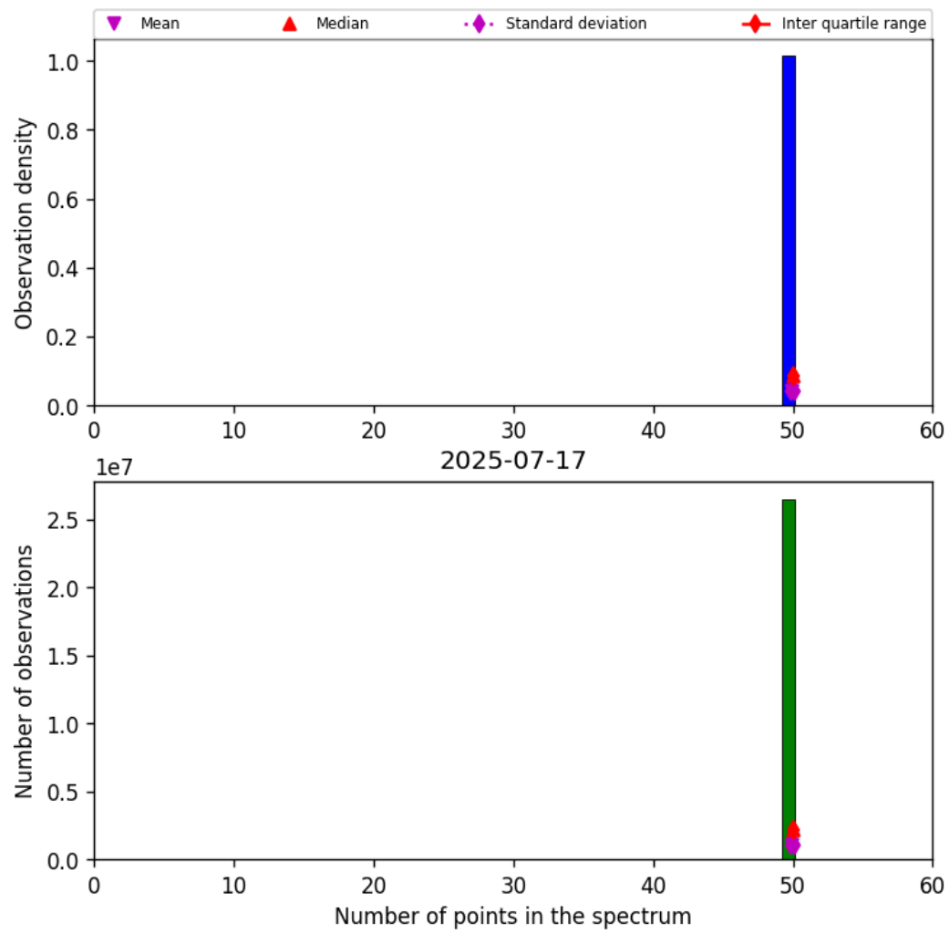
Figure 44: Histogram of "Number of points in the spectrum" for 2025-07-16 to 2025-07-18
