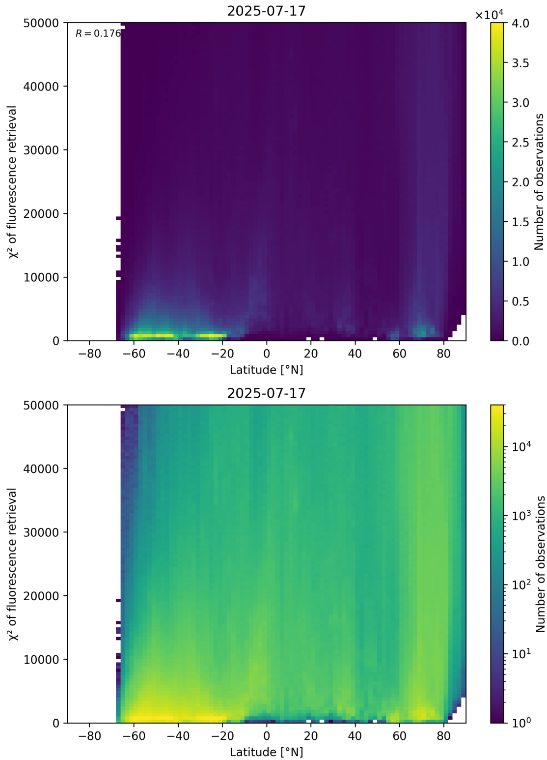
Figure 89: Scatter density plot of “Latitude” against “ \chi^2 of fluorescence retrieval” for 2025-07-16 to 2025-07-18.
