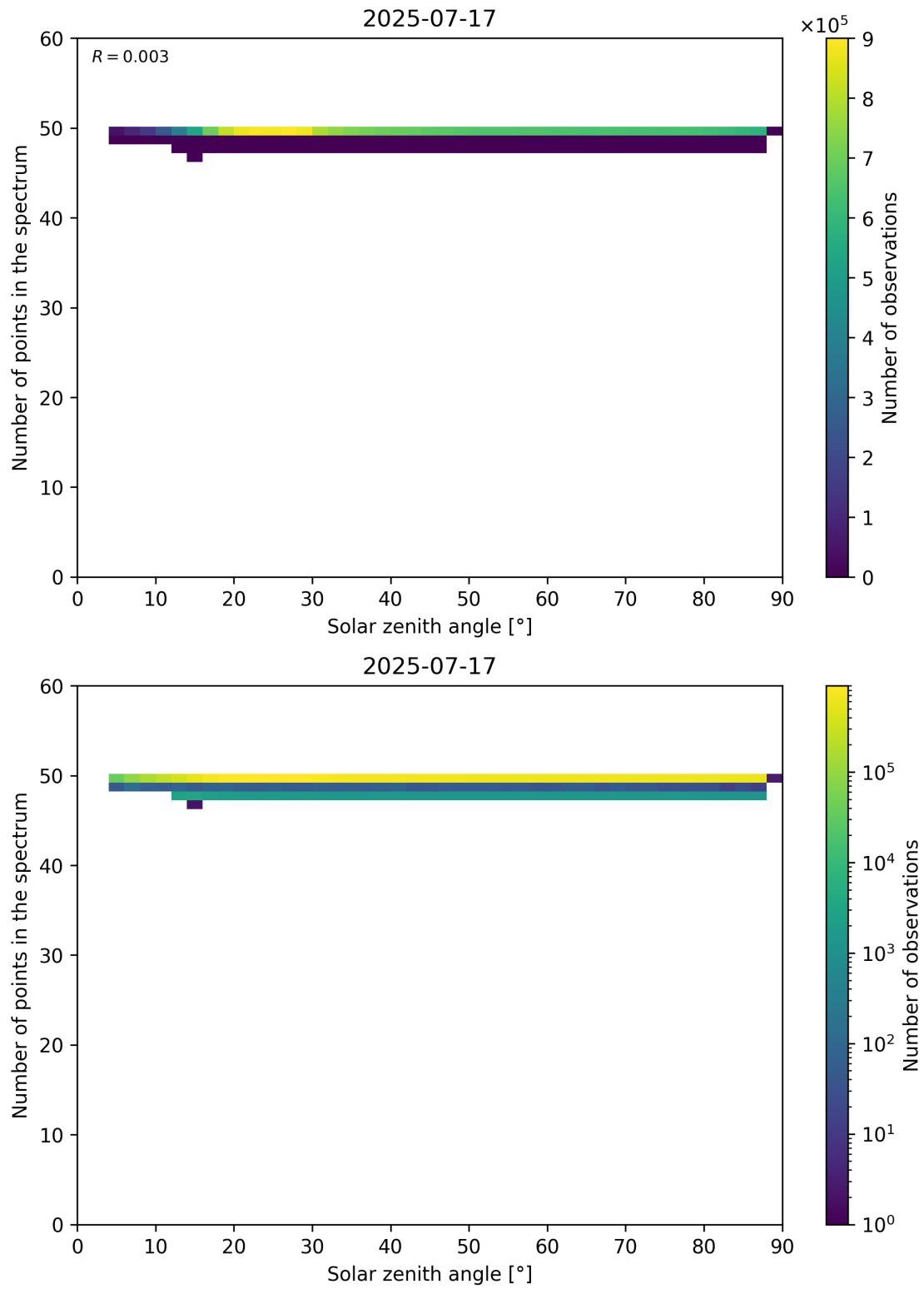
Figure 115: Scatter density plot of “Solar zenith angle” against “Number of points in the spectrum” for 2025-07-16 to 2025-07-18.
