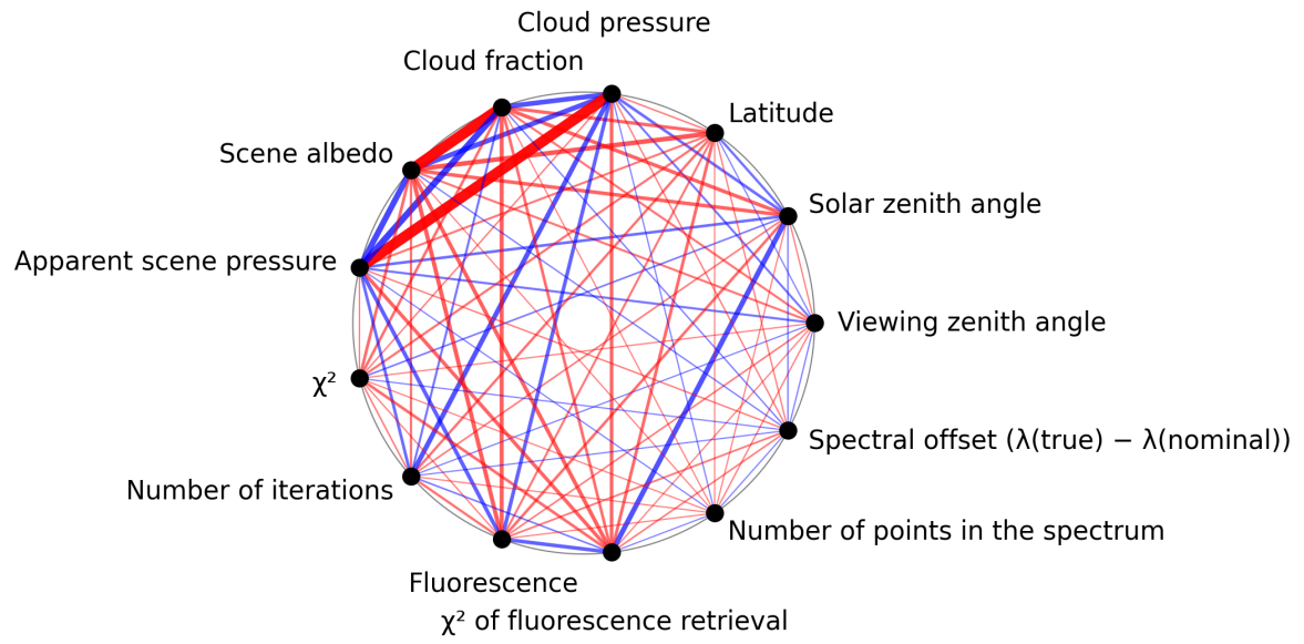
Figure 1: Map of correlation graph for 2025-07-16 to 2025-07-18.
