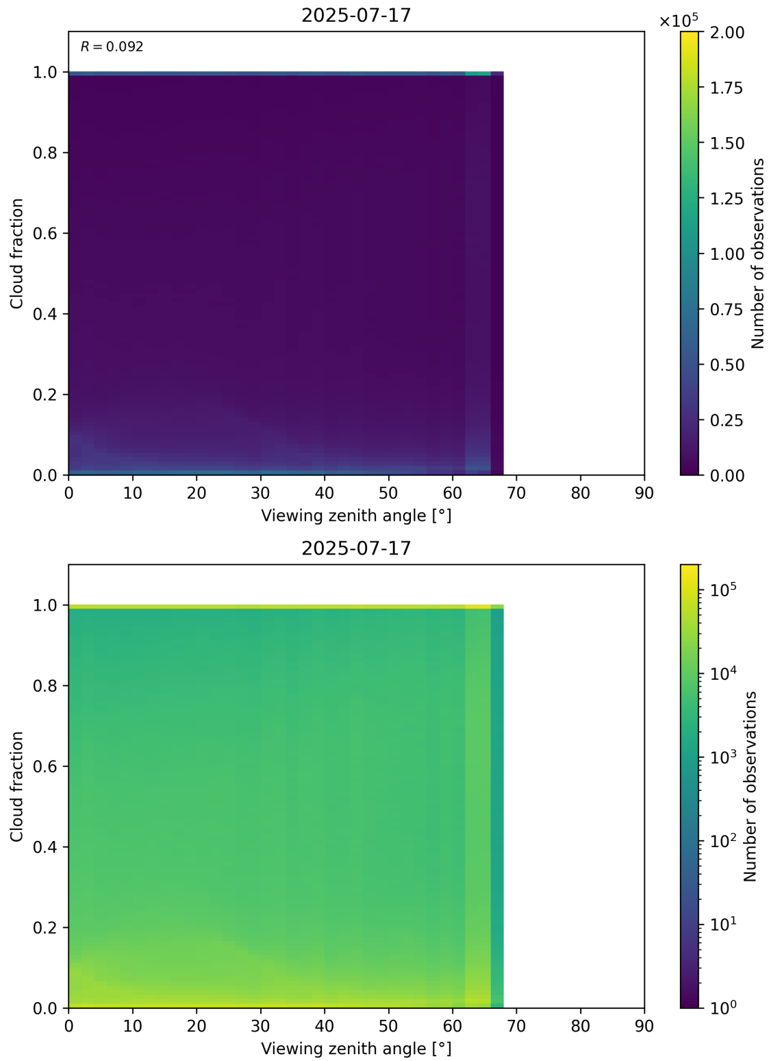
Figure 120: Scatter density plot of “Viewing zenith angle” against “Cloud fraction” for 2025-07-16 to 2025-07-18.
