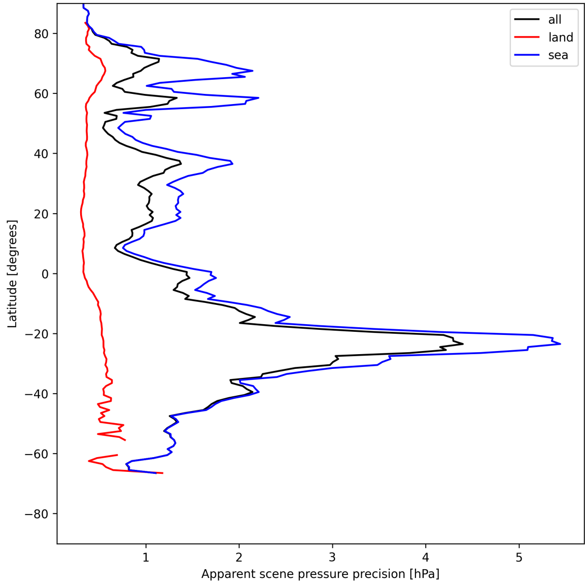
Figure 20: Zonal average of “Apparent scene pressure precision” for 2025-07-16 to 2025-07-18.
