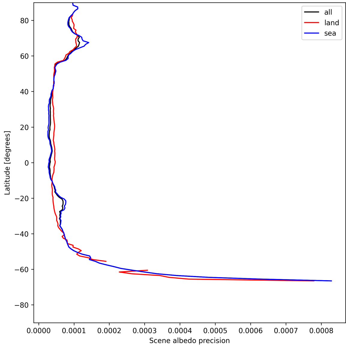
Figure 18: Zonal average of "Scene albedo precision" for 2025-07-16 to 2025-07-18.
