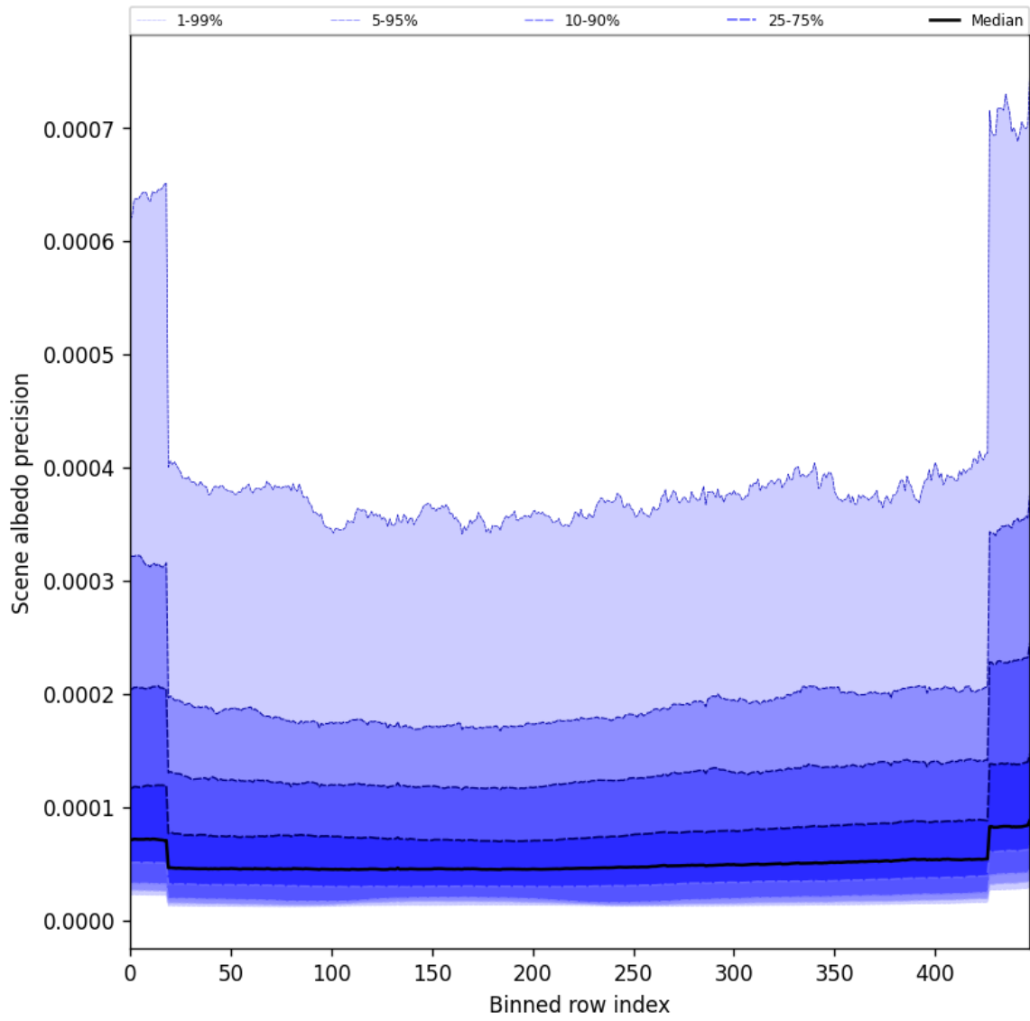
Figure 52: Along track statistics of “Scene albedo precision” for 2025-07-16 to 2025-07-18
