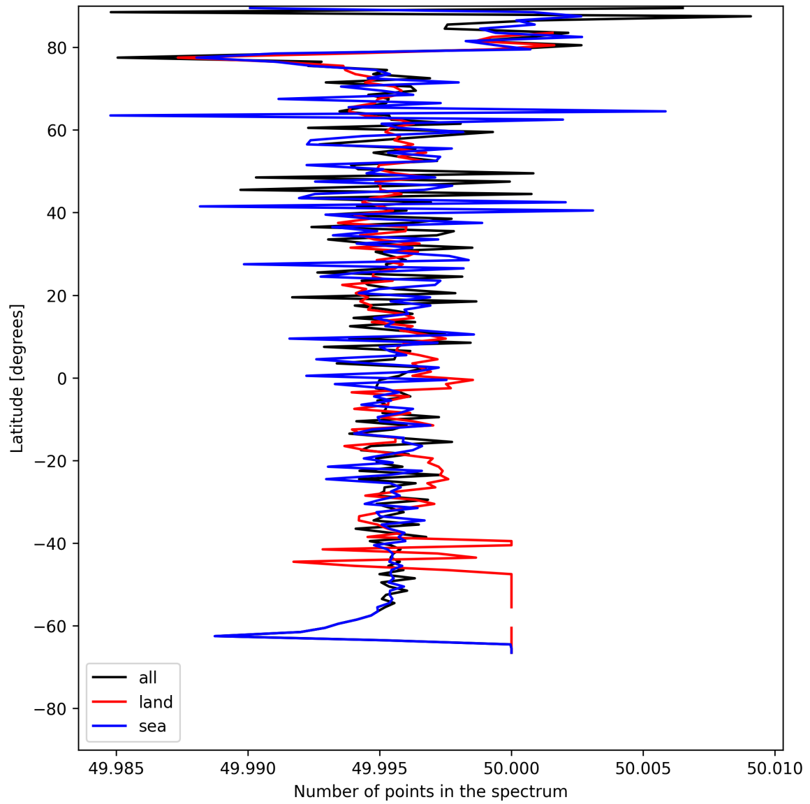
Figure 27: Zonal average of “Number of points in the spectrum” for 2025-07-16 to 2025-07-18.
