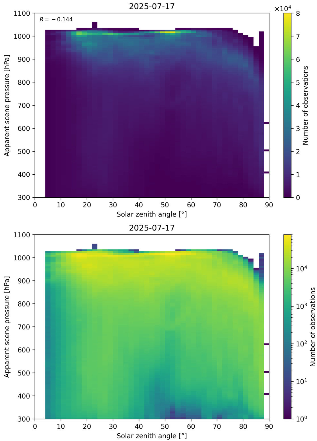
Figure 108: Scatter density plot of “Solar zenith angle” against “Apparent scene pressure” for 2025-07-16 to 2025-07-18.
