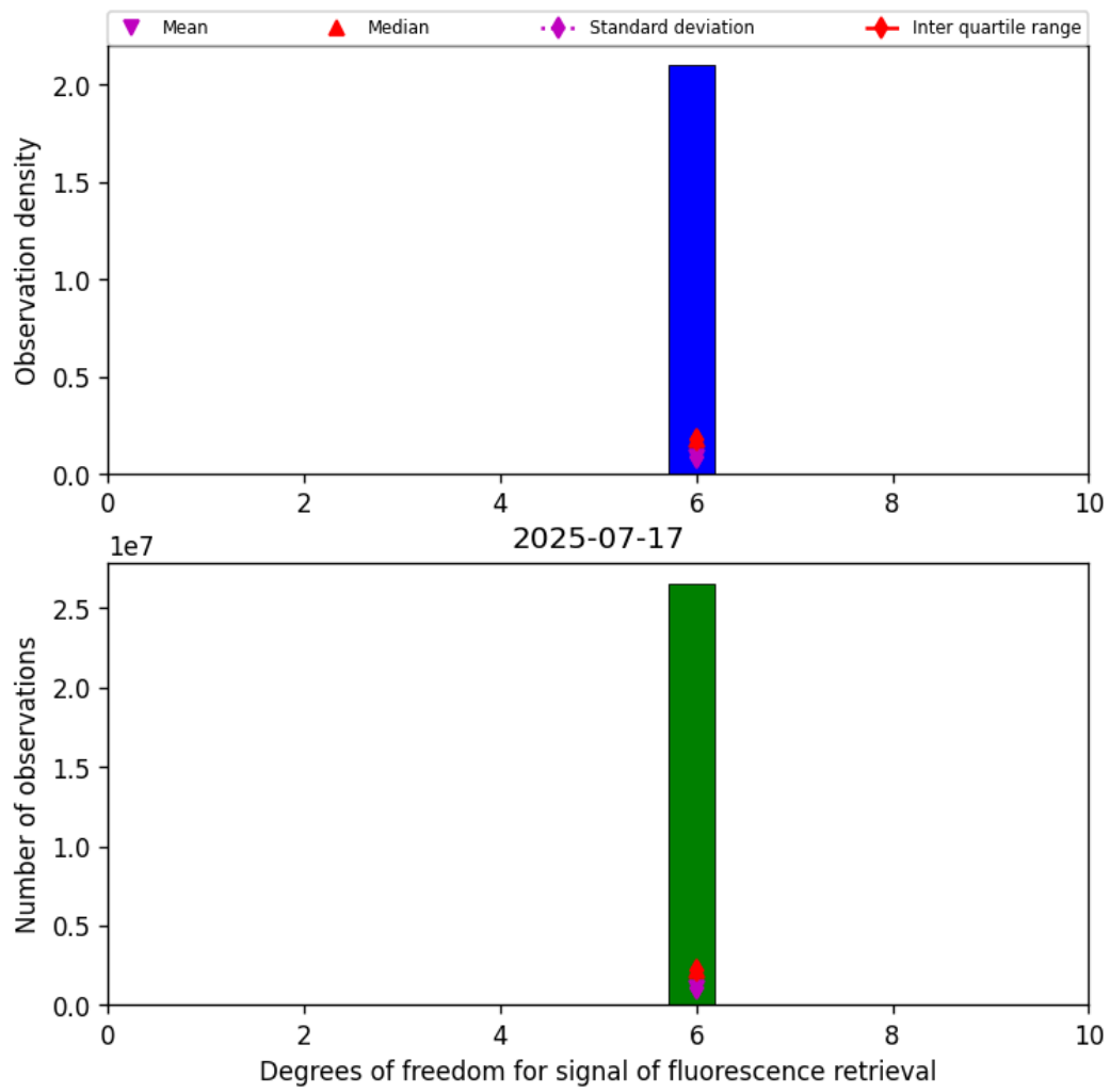
Figure 43: Histogram of "Degrees of freedom for signal of fluorescence retrieval" for 2025-07-16 to 2025-07-18
