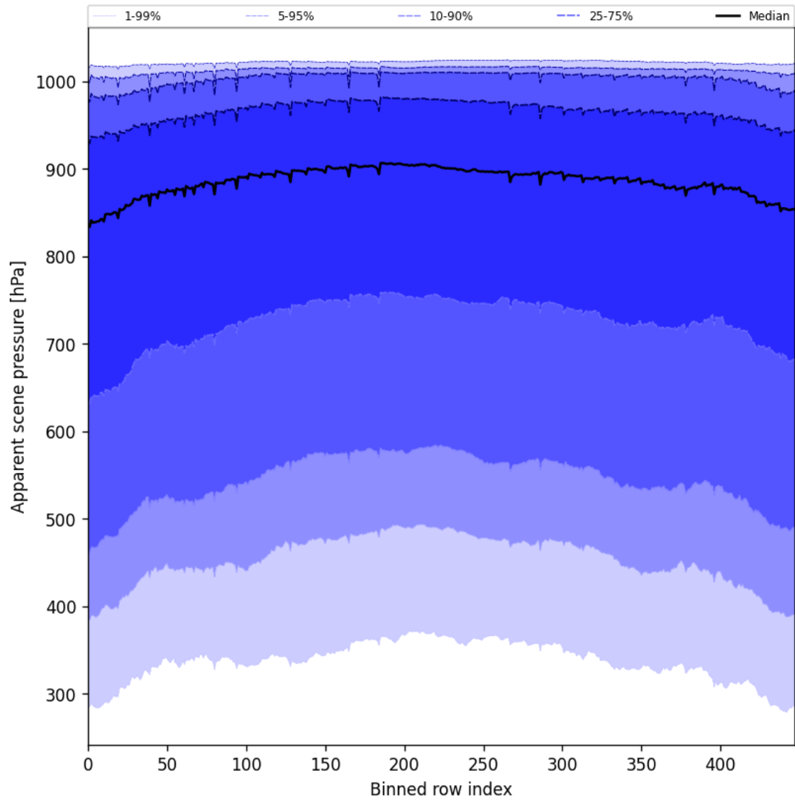
Figure 53: Along track statistics of “Apparent scene pressure” for 2025-07-16 to 2025-07-18
