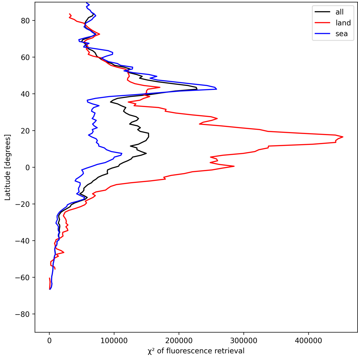
Figure 25: Zonal average of “ \chi^2 of fluorescence retrieval” for 2025-07-16 to 2025-07-18.
