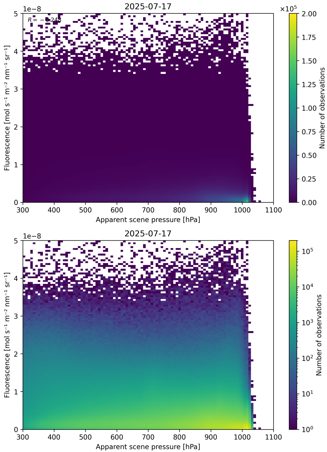
Figure 64: Scatter density plot of “Apparent scene pressure” against “Fluorescence” for 2025-07-16 to 2025-07-18.
