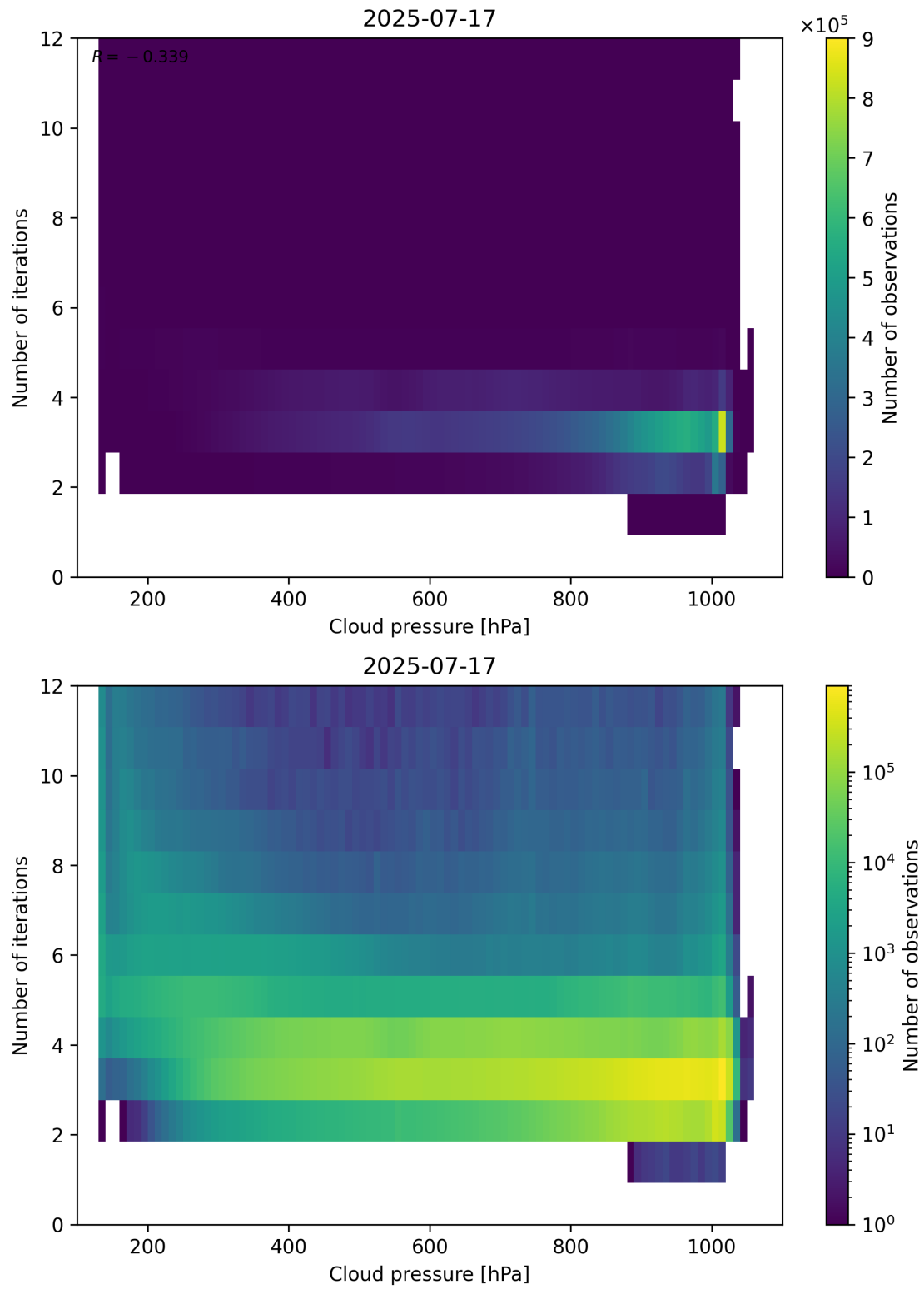
Figure 81: Scatter density plot of “Cloud pressure” against “Number of iterations” for 2025-07-16 to 2025-07-18.
