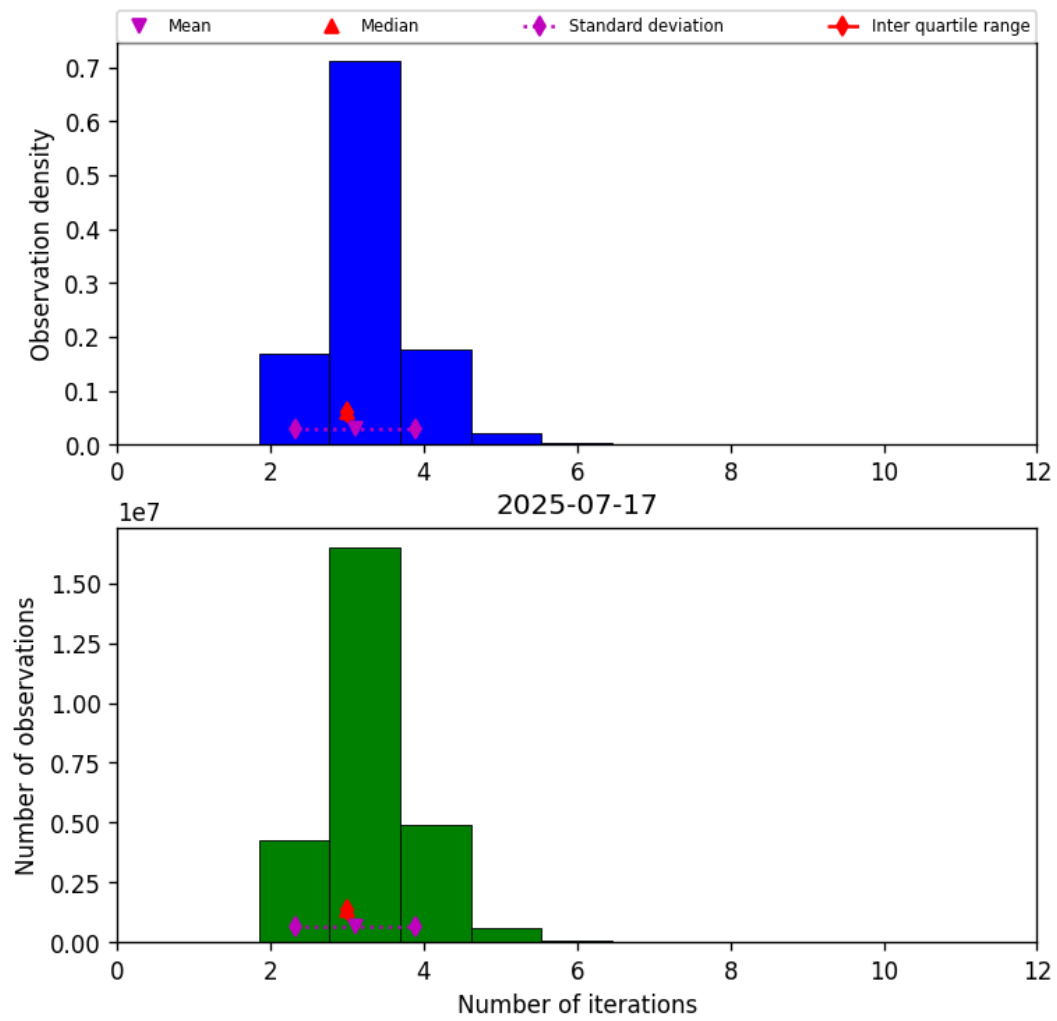
Figure 39: Histogram of “Number of iterations” for 2025-07-16 to 2025-07-18
