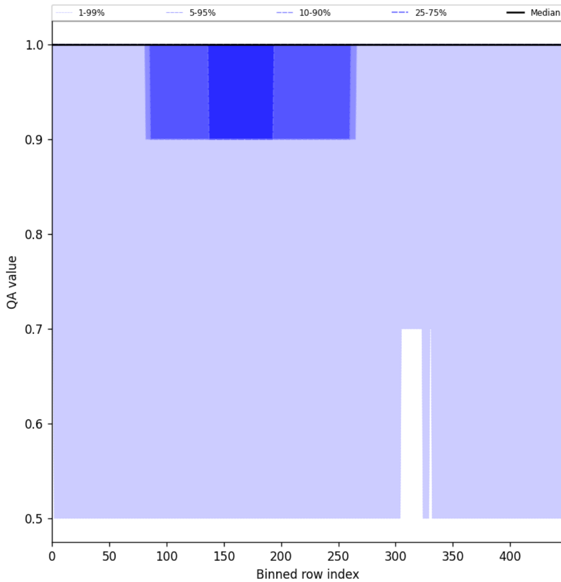
Figure 46: Along track statistics of “QA value” for 2025-07-18 to 2025-07-19
