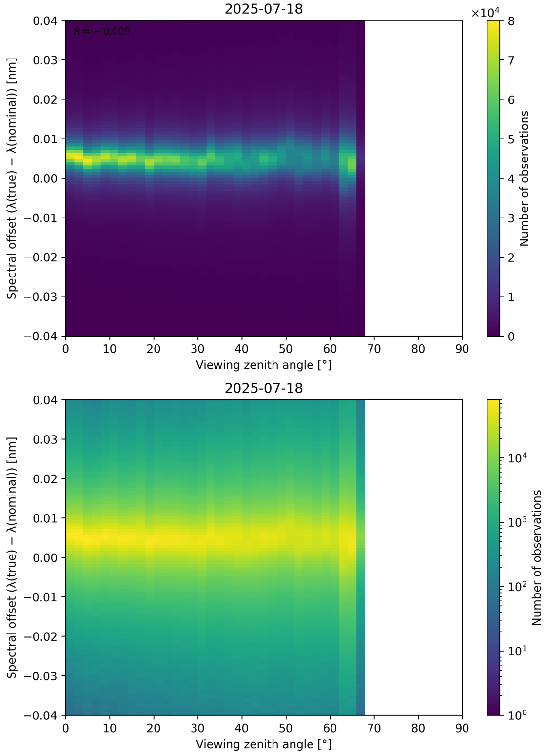
Figure 128: Scatter density plot of “Viewing zenith angle” against “Spectral offset ( \lambda_{\text{true}} - \lambda_{\text{nominal}} )” for 2025-07-18 to 2025-07-19.
