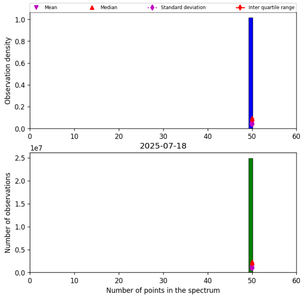
Figure 44: Histogram of "Number of points in the spectrum" for 2025-07-18 to 2025-07-19
