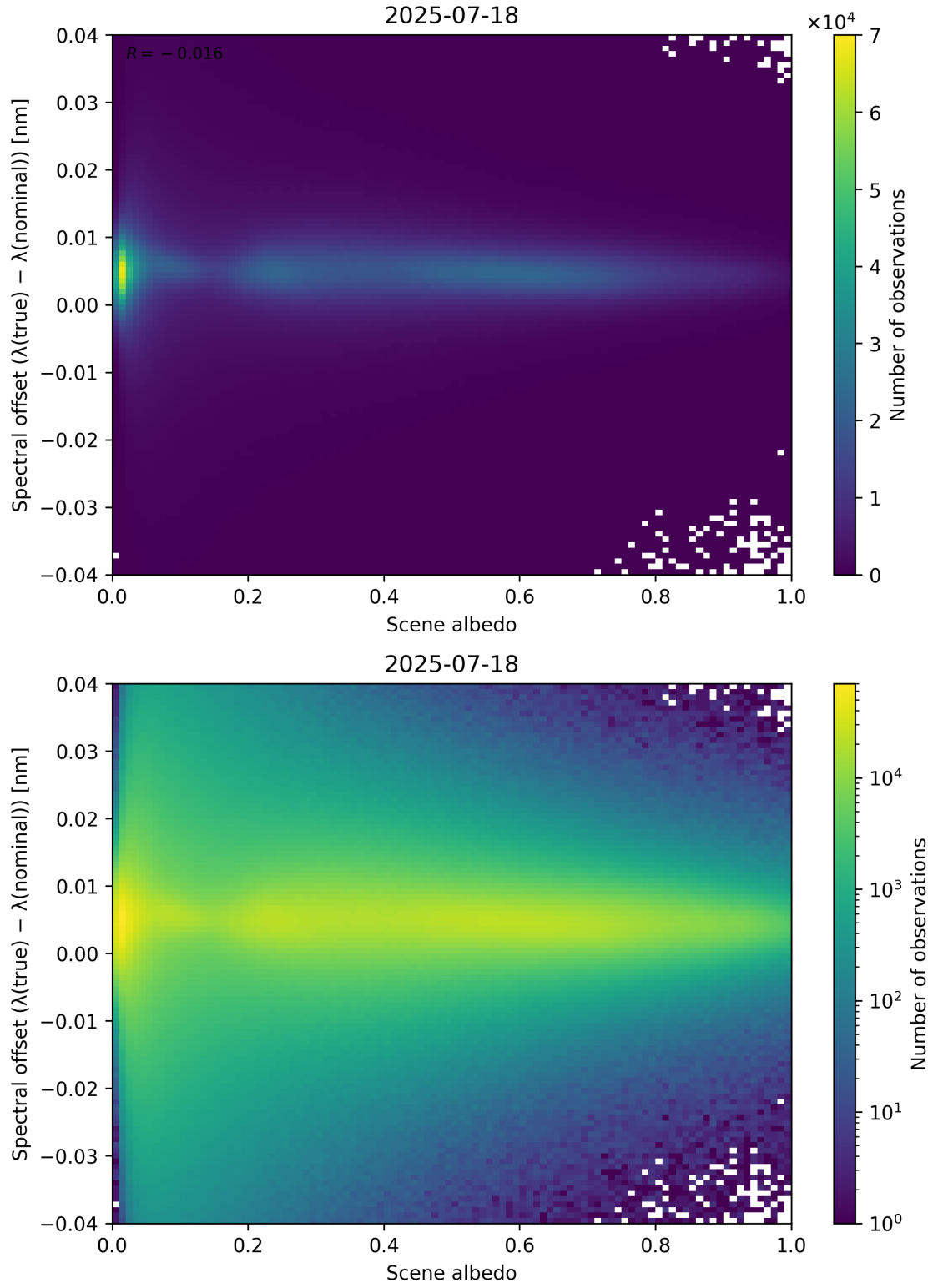
Figure 107: Scatter density plot of “Scene albedo” against “Spectral offset ( \lambda_{\text{true}} - \lambda_{\text{nominal}} )” for 2025-07-18 to 2025-07-19.
