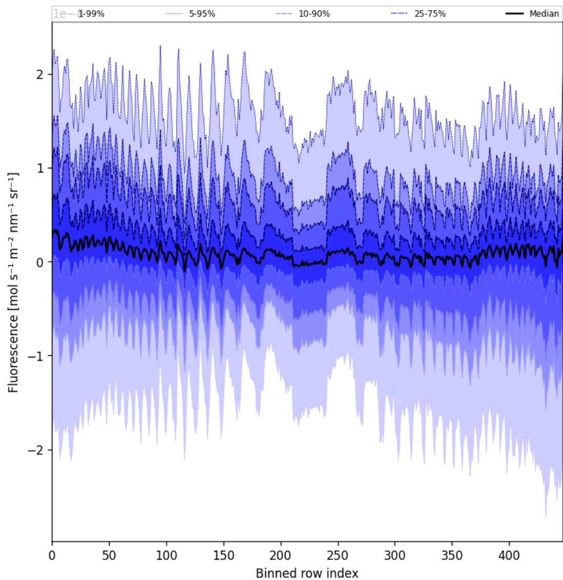
Figure 57: Along track statistics of “Fluorescence” for 2025-07-18 to 2025-07-19
