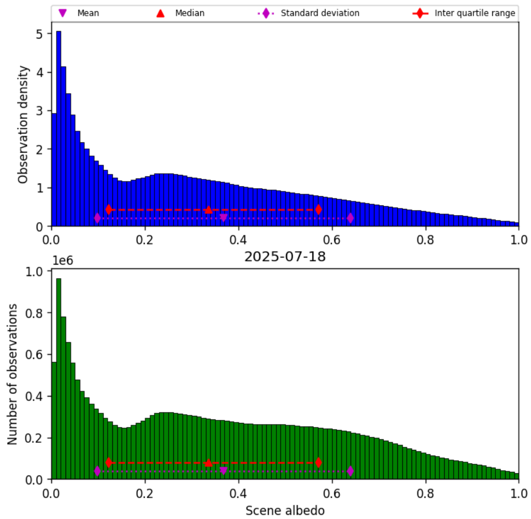
Figure 34: Histogram of “Scene albedo” for 2025-07-18 to 2025-07-19
