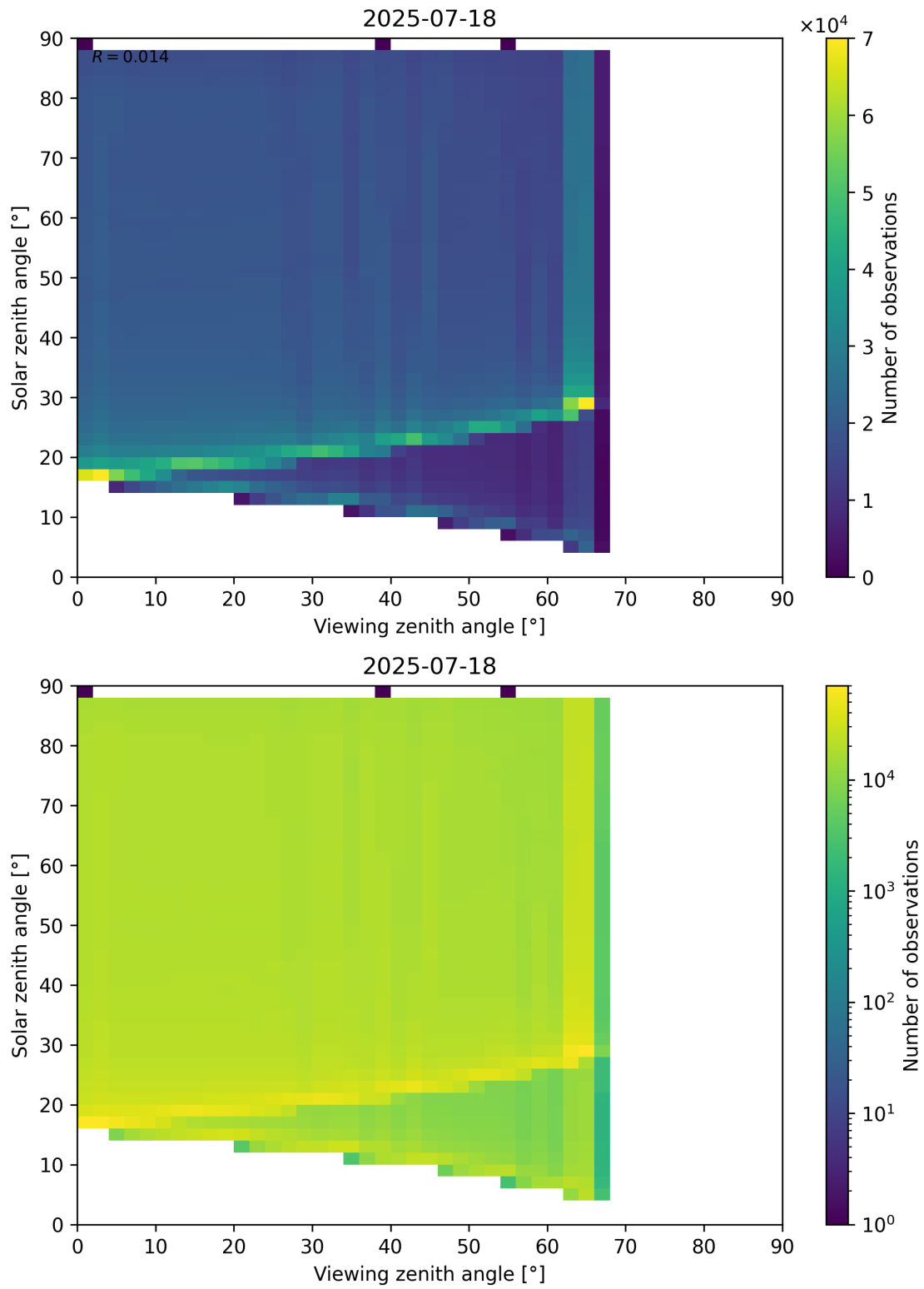
Figure 127: Scatter density plot of “Viewing zenith angle” against “Solar zenith angle” for 2025-07-18 to 2025-07-19.
