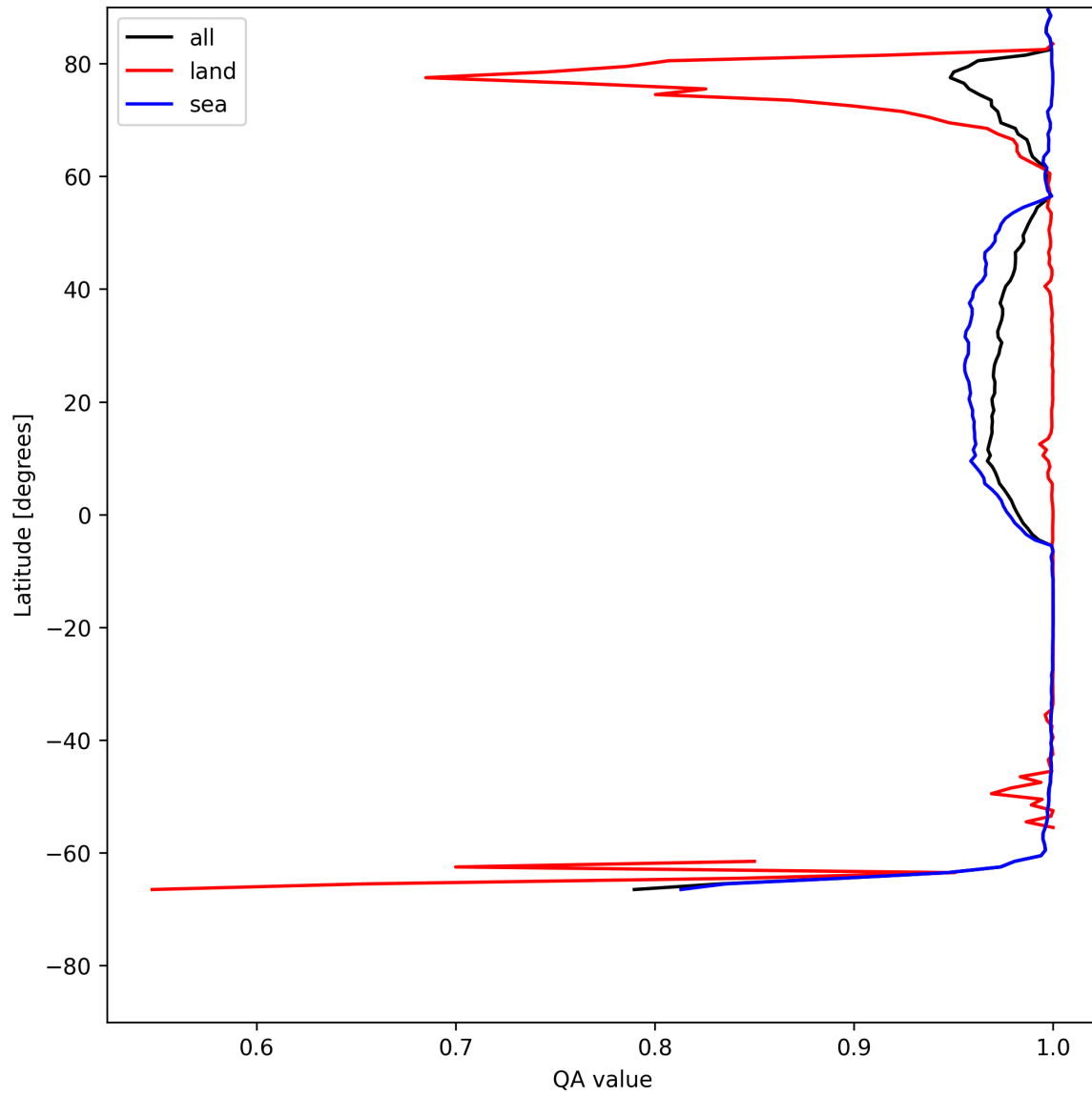
Figure 12: Zonal average of “QA value” for 2025-07-18 to 2025-07-19.
