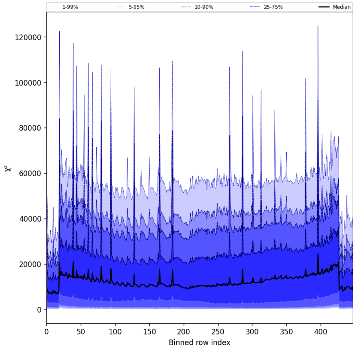
Figure 55: Along track statistics of “ \chi^2 ” for 2025-07-18 to 2025-07-19
