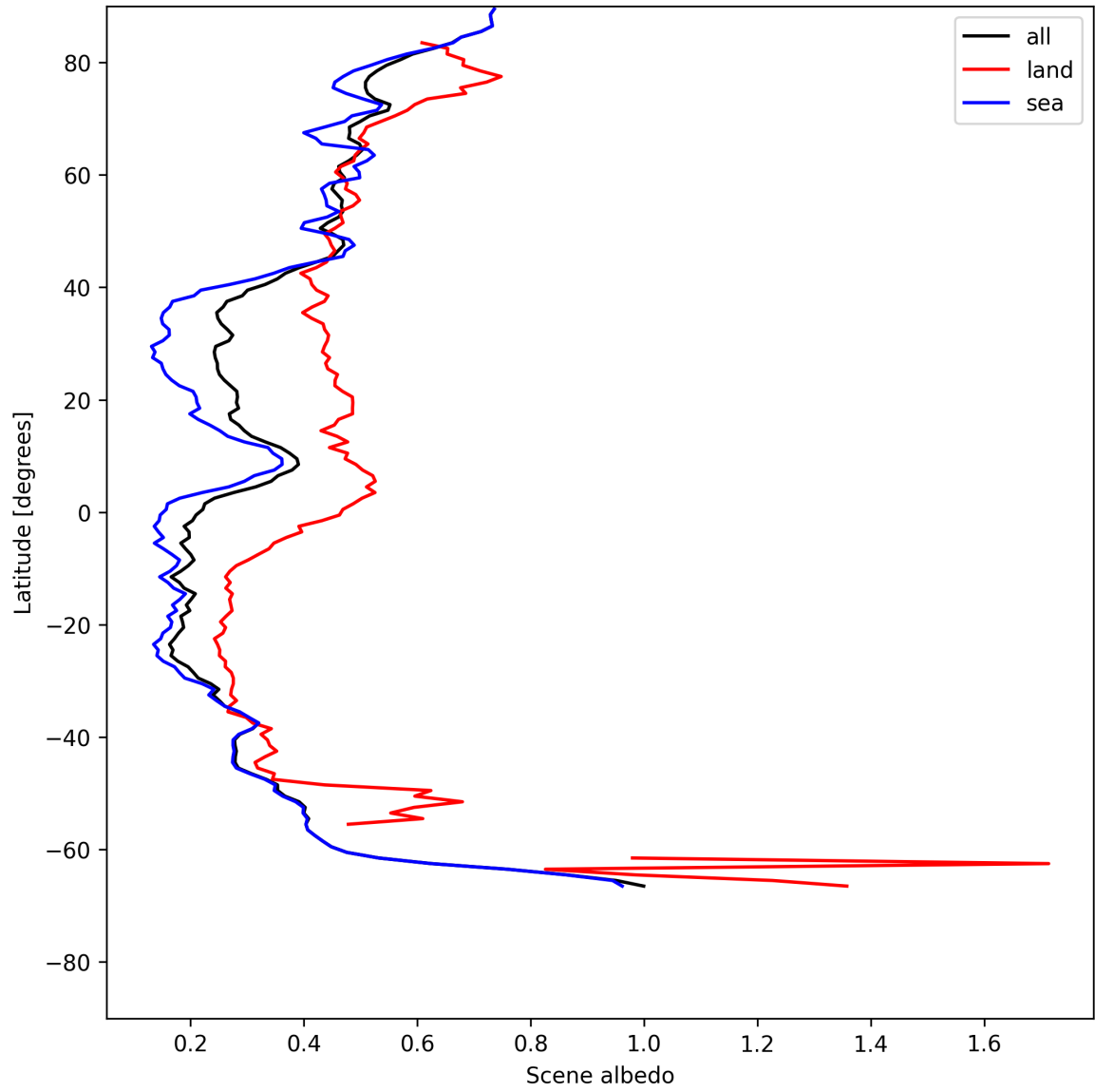
Figure 17: Zonal average of “Scene albedo” for 2025-07-18 to 2025-07-19.
