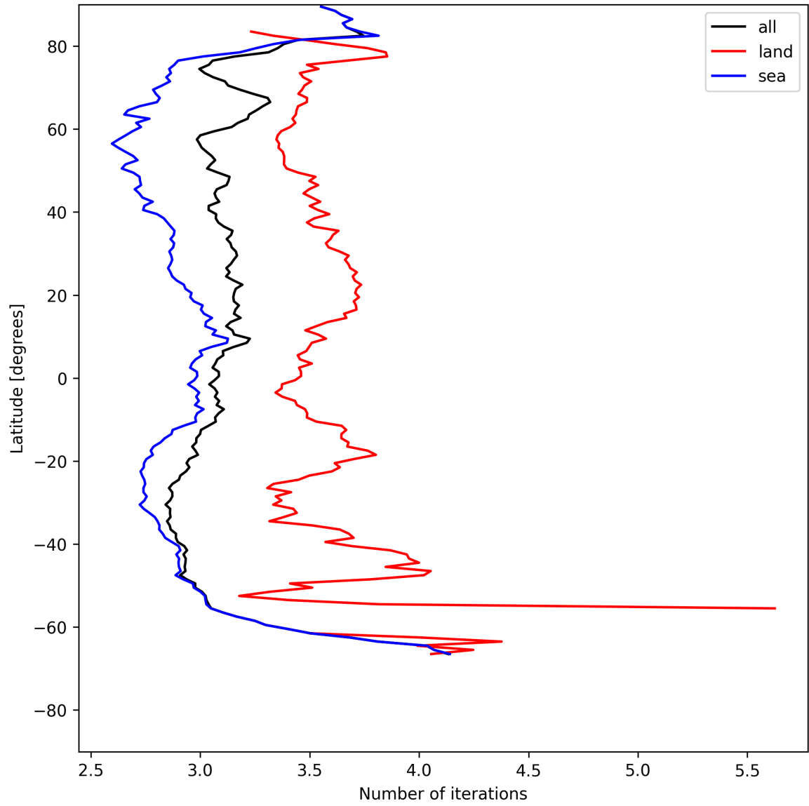
Figure 22: Zonal average of “Number of iterations” for 2025-07-18 to 2025-07-19.
