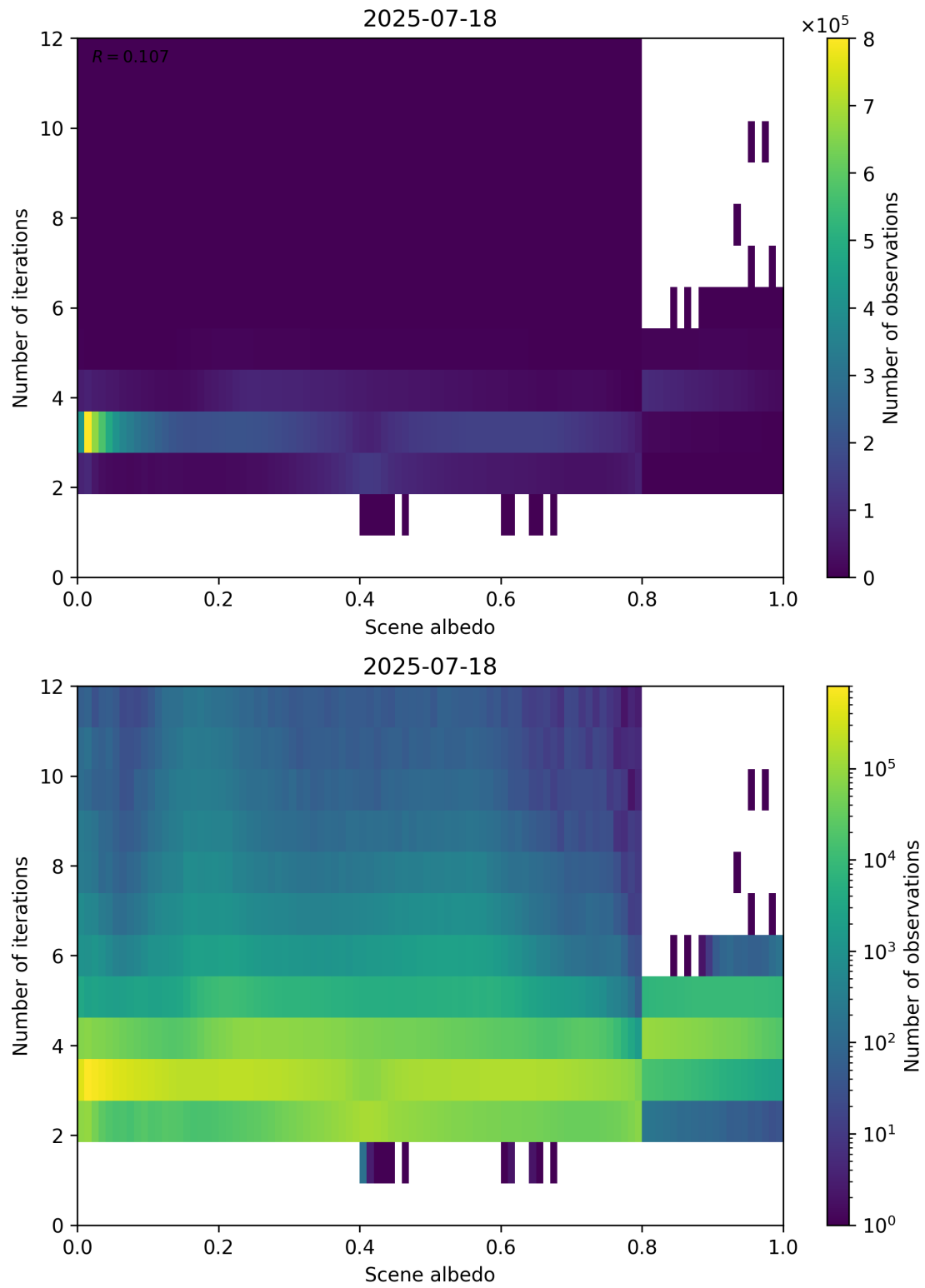
Figure 105: Scatter density plot of “Scene albedo” against “Number of iterations” for 2025-07-18 to 2025-07-19.
