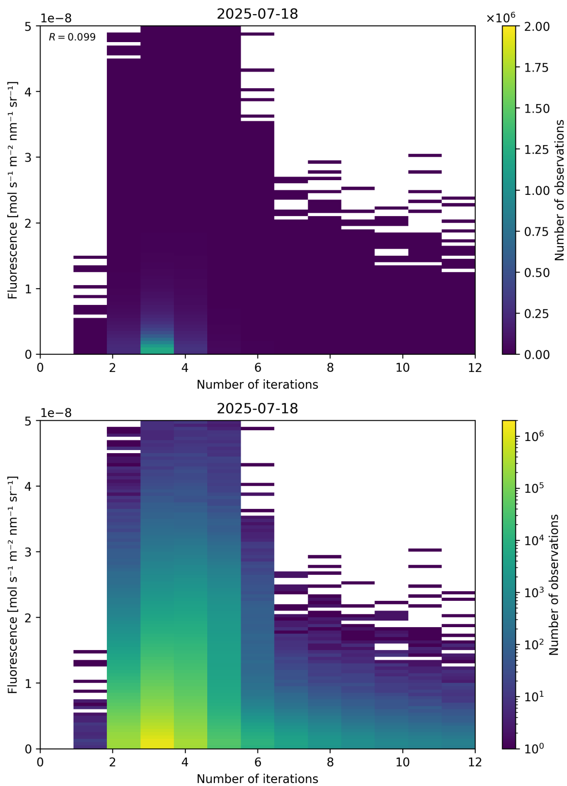
Figure 98: Scatter density plot of “Number of iterations” against “Fluorescence” for 2025-07-18 to 2025-07-19.
