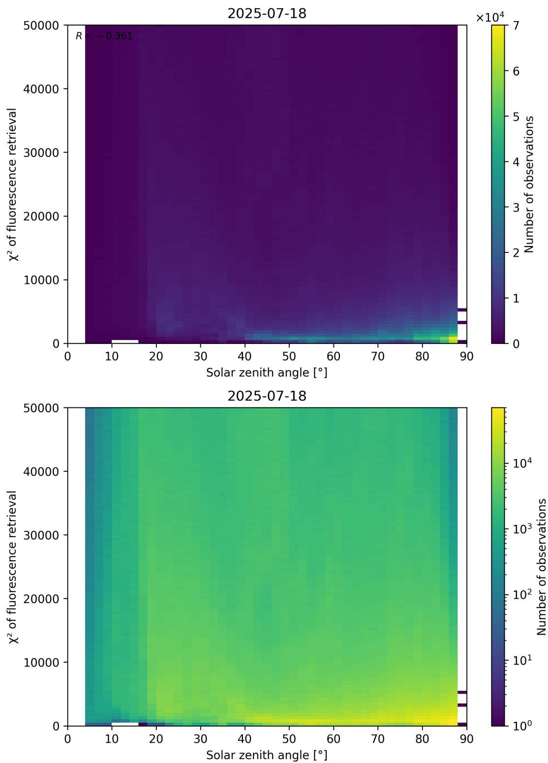
Figure 109: Scatter density plot of “Solar zenith angle” against “ \chi^2 of fluorescence retrieval” for 2025-07-18 to 2025-07-19.
