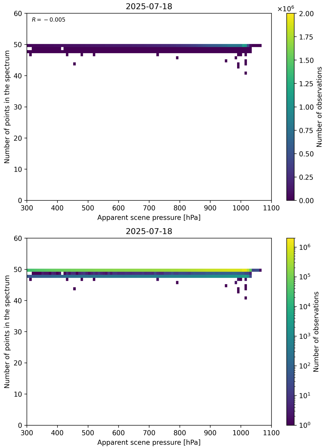
Figure 66: Scatter density plot of “Apparent scene pressure” against “Number of points in the spectrum” for 2025-07-18 to 2025-07-19.
