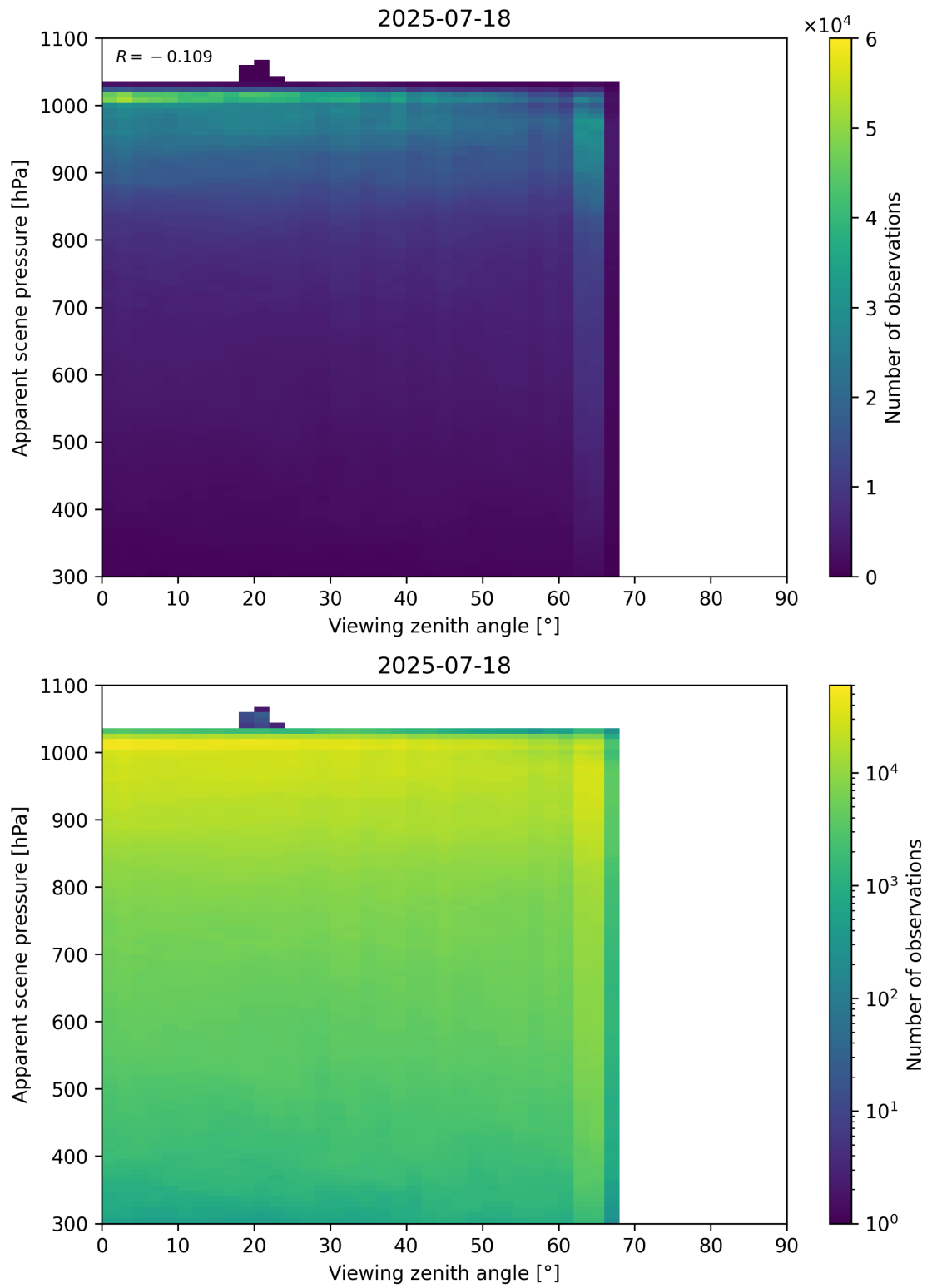
Figure 118: Scatter density plot of “Viewing zenith angle” against “Apparent scene pressure” for 2025-07-18 to 2025-07-19.
