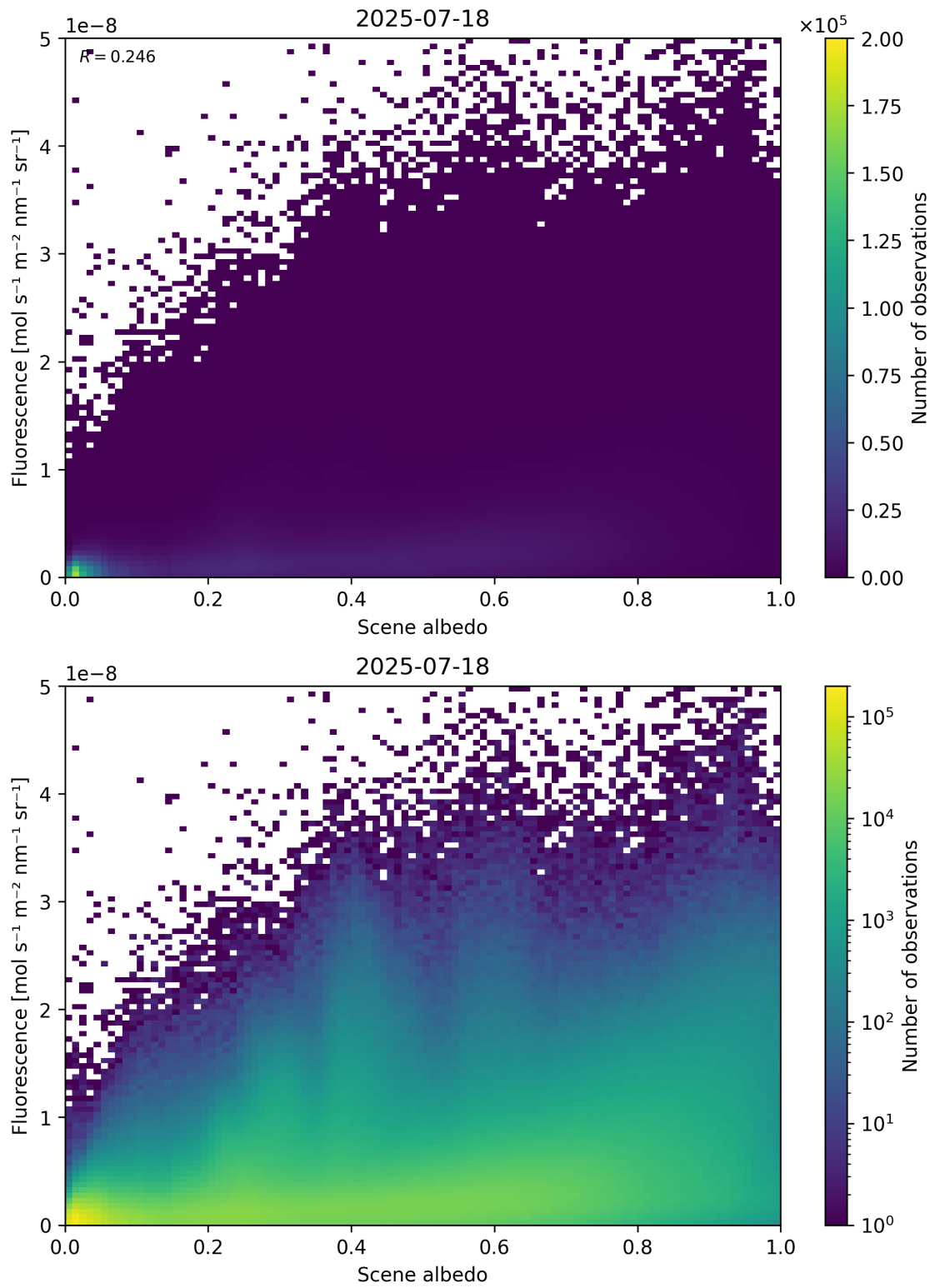
Figure 104: Scatter density plot of “Scene albedo” against “Fluorescence” for 2025-07-18 to 2025-07-19.
