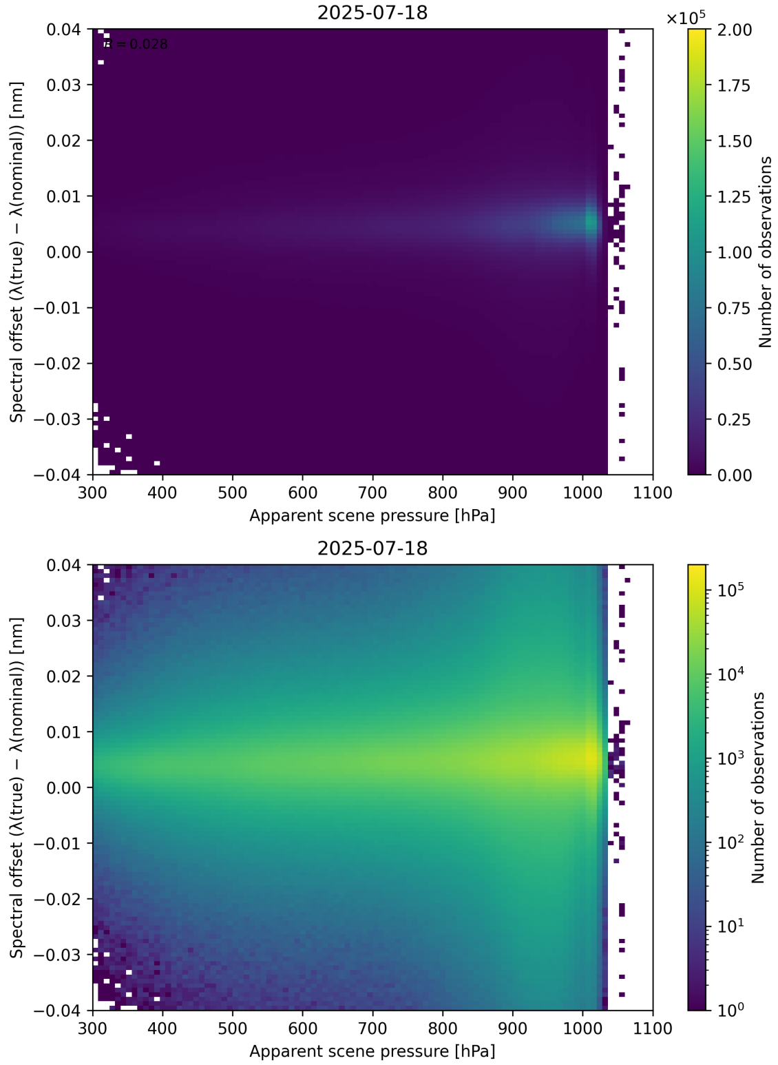
Figure 67: Scatter density plot of “Apparent scene pressure” against “Spectral offset ( \lambda_{\text{true}} - \lambda_{\text{nominal}} )” for 2025-07-18 to 2025-07-19.
