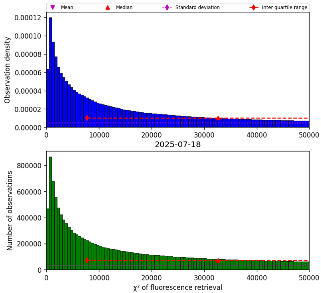
Figure 42: Histogram of “ \chi^2 of fluorescence retrieval” for 2025-07-18 to 2025-07-19
