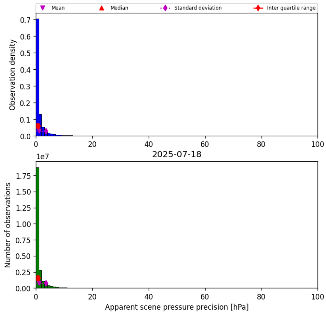
Figure 37: Histogram of “Apparent scene pressure precision” for 2025-07-18 to 2025-07-19
