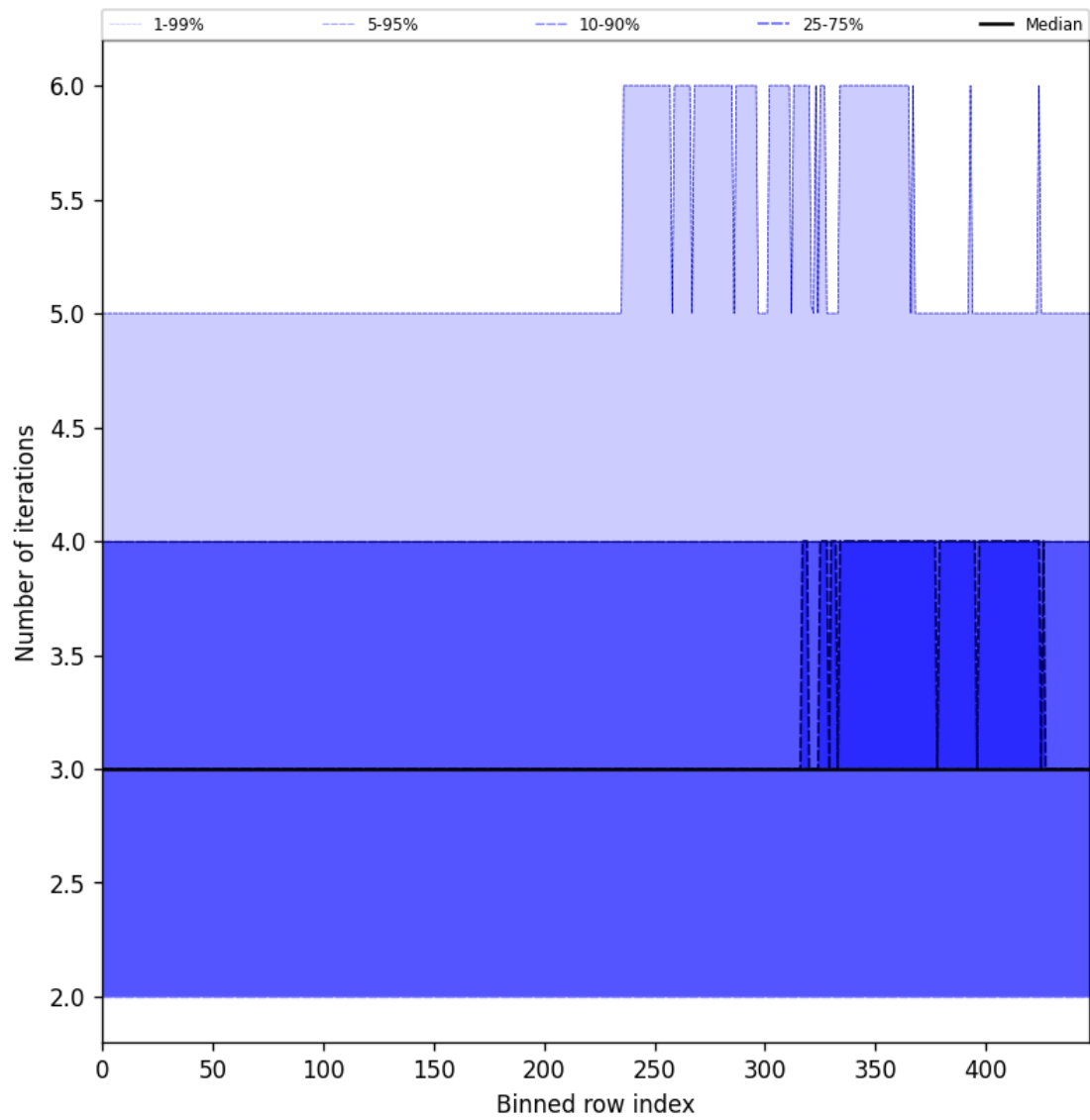
Figure 56: Along track statistics of "Number of iterations" for 2025-07-18 to 2025-07-19
