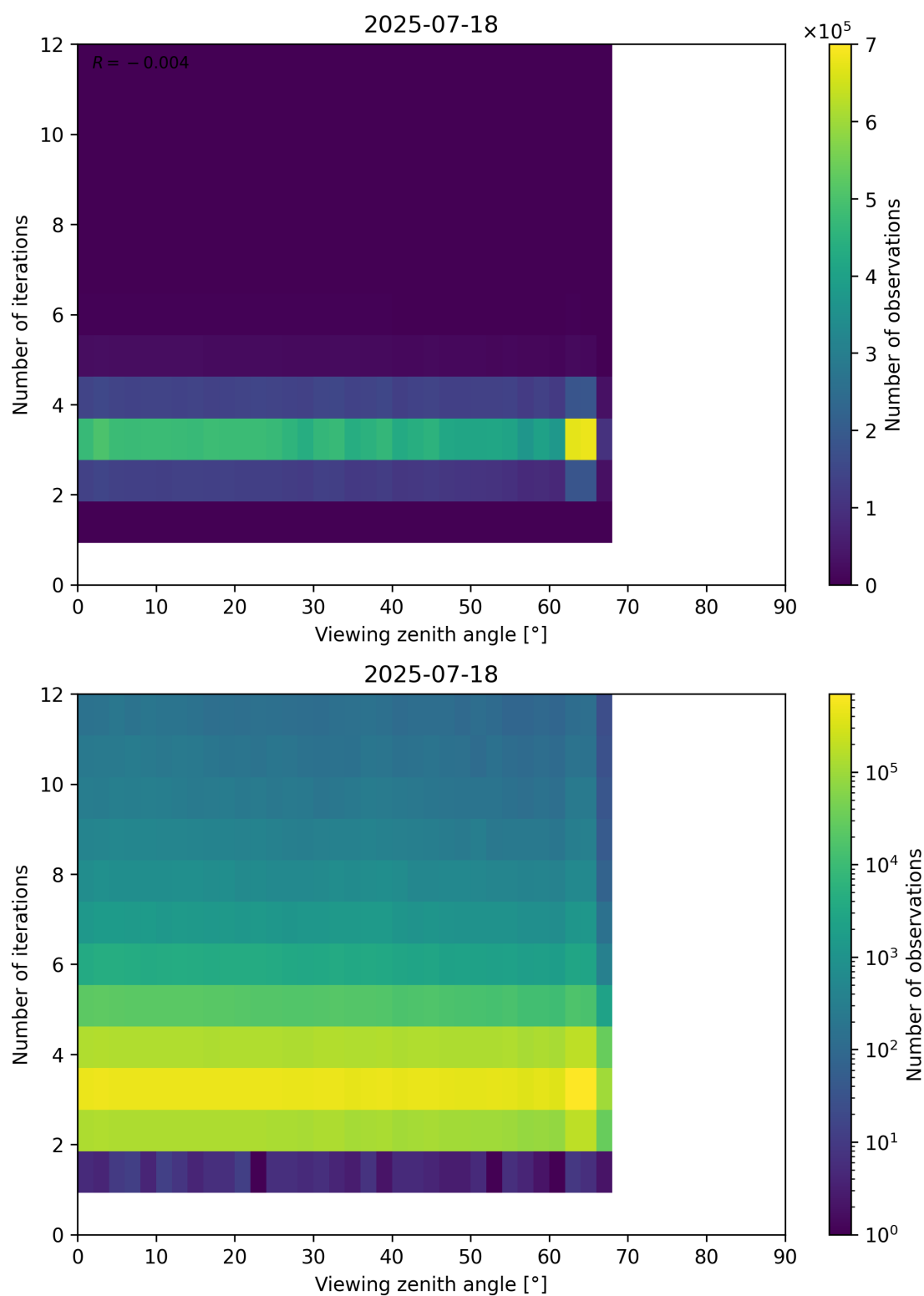
Figure 124: Scatter density plot of “Viewing zenith angle” against “Number of iterations” for 2025-07-18 to 2025-07-19.
