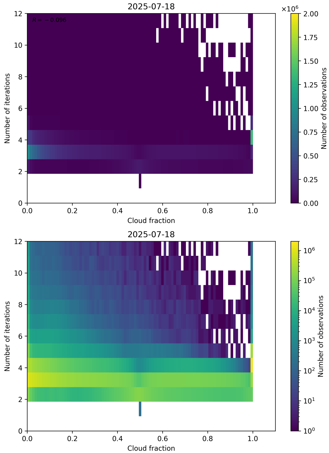
Figure 73: Scatter density plot of “Cloud fraction” against “Number of iterations” for 2025-07-18 to 2025-07-19.
