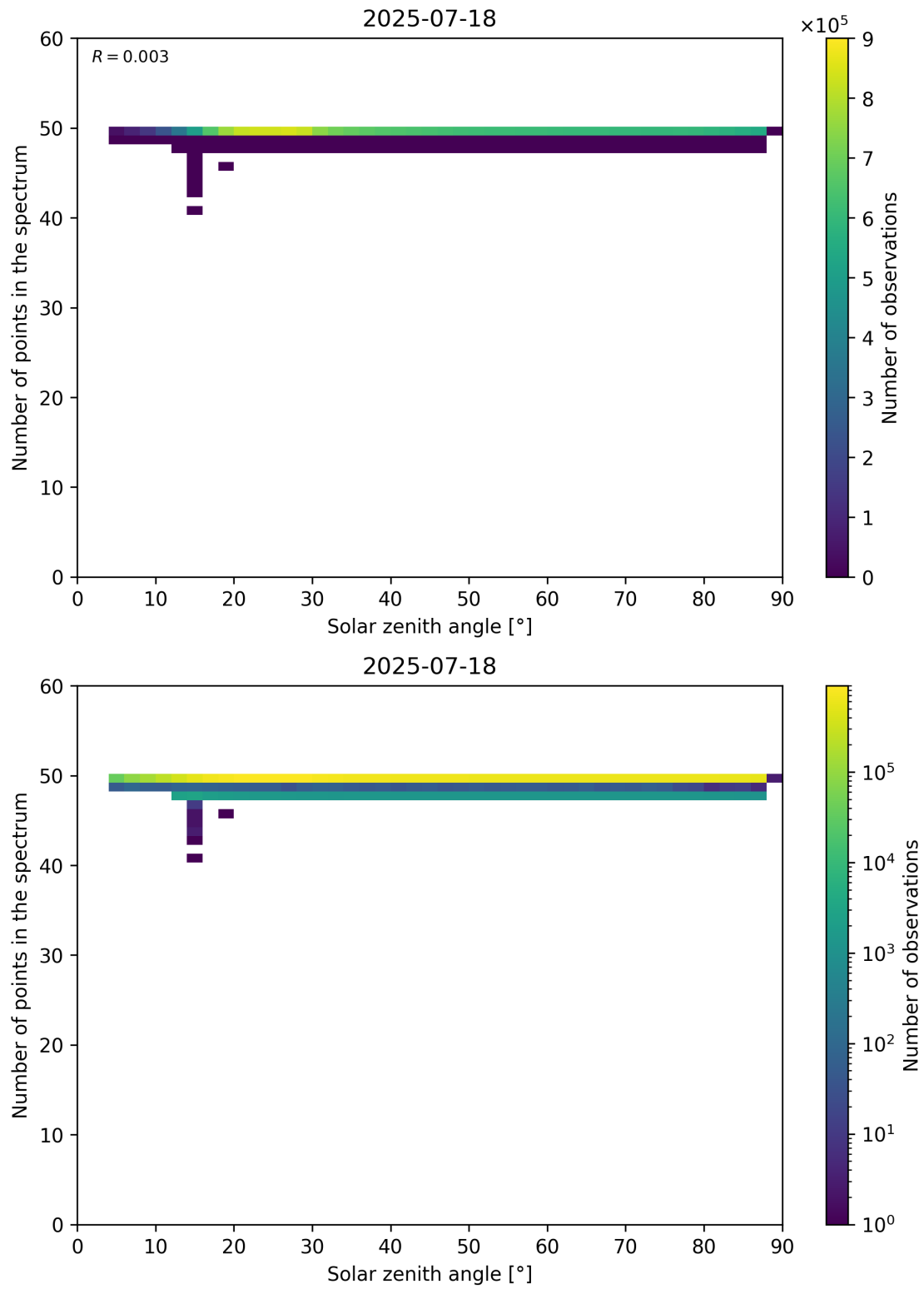
Figure 115: Scatter density plot of “Solar zenith angle” against “Number of points in the spectrum” for 2025-07-18 to 2025-07-19.
