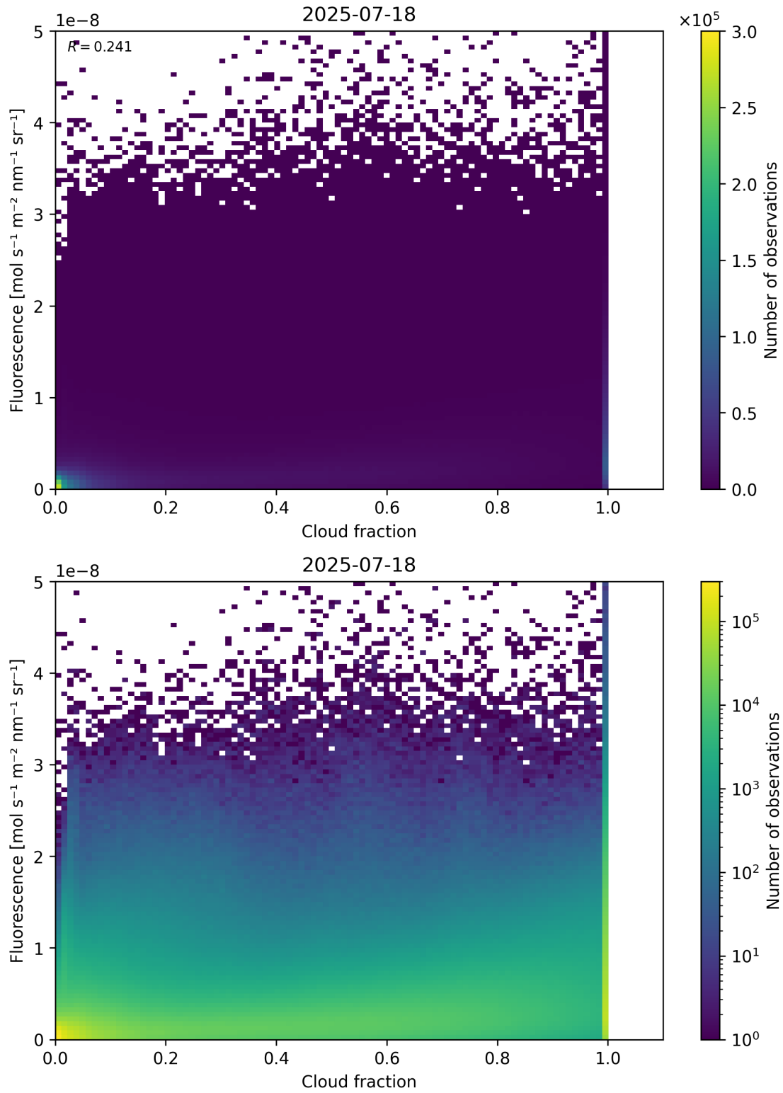
Figure 72: Scatter density plot of “Cloud fraction” against “Fluorescence” for 2025-07-18 to 2025-07-19.
