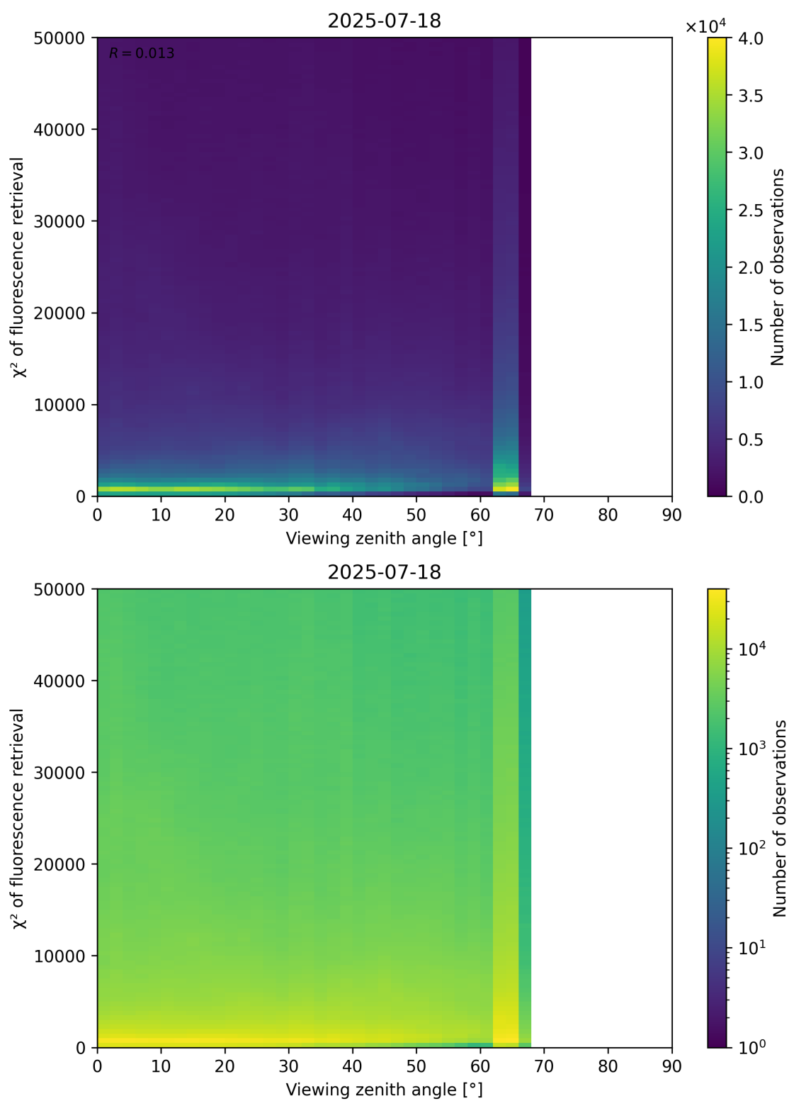
Figure 119: Scatter density plot of “Viewing zenith angle” against “ \chi^2 of fluorescence retrieval” for 2025-07-18 to 2025-07-19.
