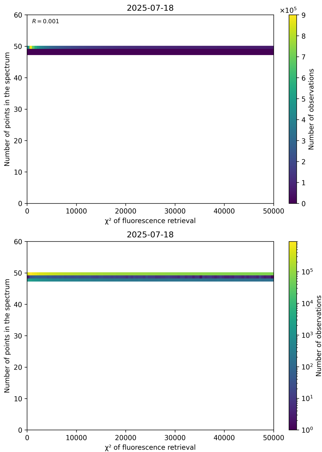
Figure 68: Scatter density plot of “ \chi^2 of fluorescence retrieval” against “Number of points in the spectrum” for 2025-07-18 to 2025-07-19.
