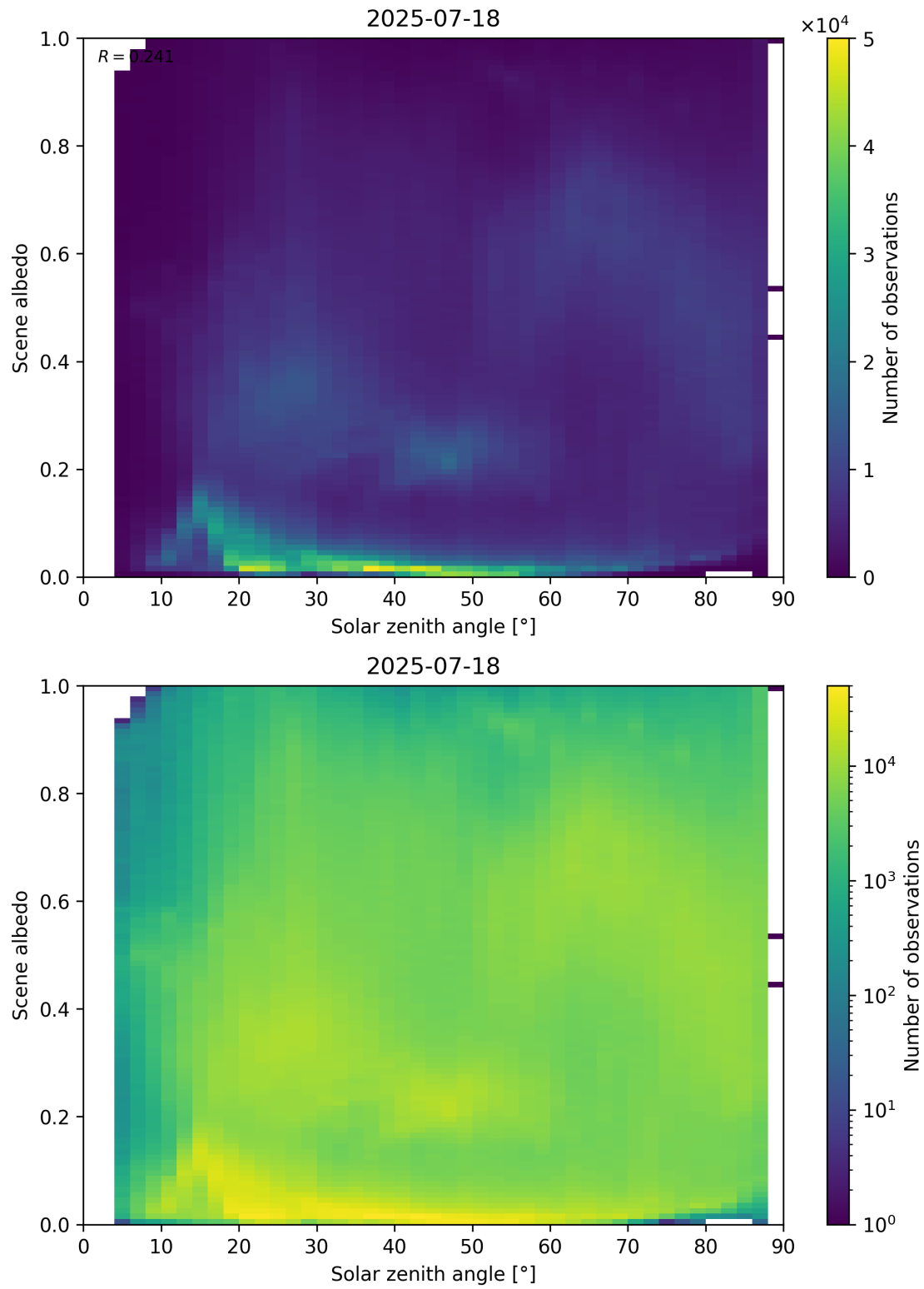
Figure 116: Scatter density plot of “Solar zenith angle” against “Scene albedo” for 2025-07-18 to 2025-07-19.
