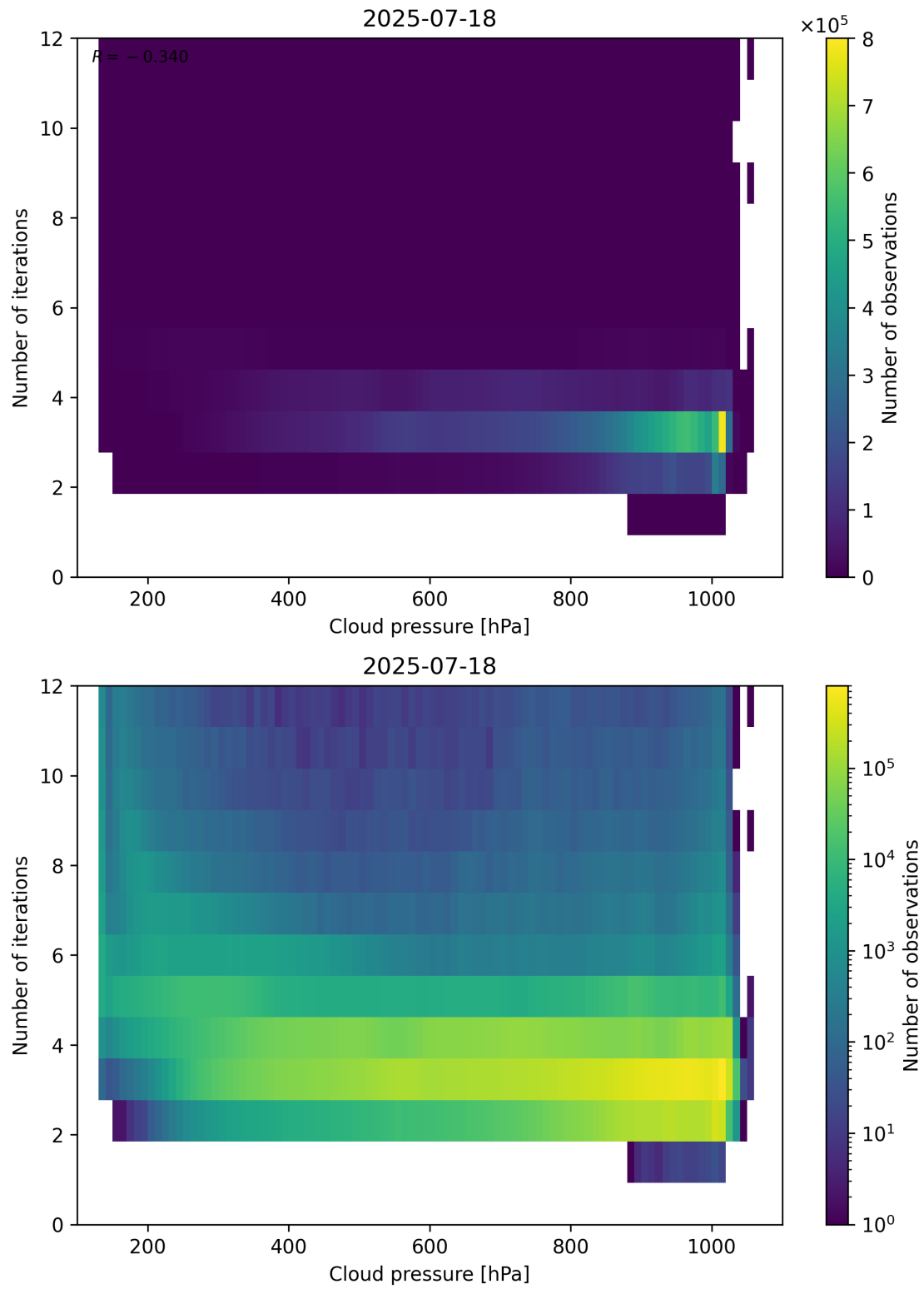
Figure 81: Scatter density plot of “Cloud pressure” against “Number of iterations” for 2025-07-18 to 2025-07-19.
