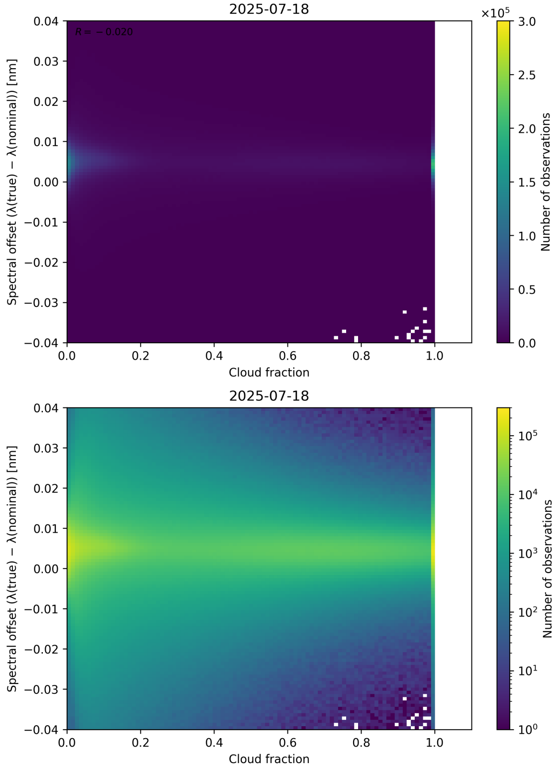
Figure 76: Scatter density plot of “Cloud fraction” against “Spectral offset ( \lambda_{\text{true}} - \lambda_{\text{nominal}} )” for 2025-07-18 to 2025-07-19.
