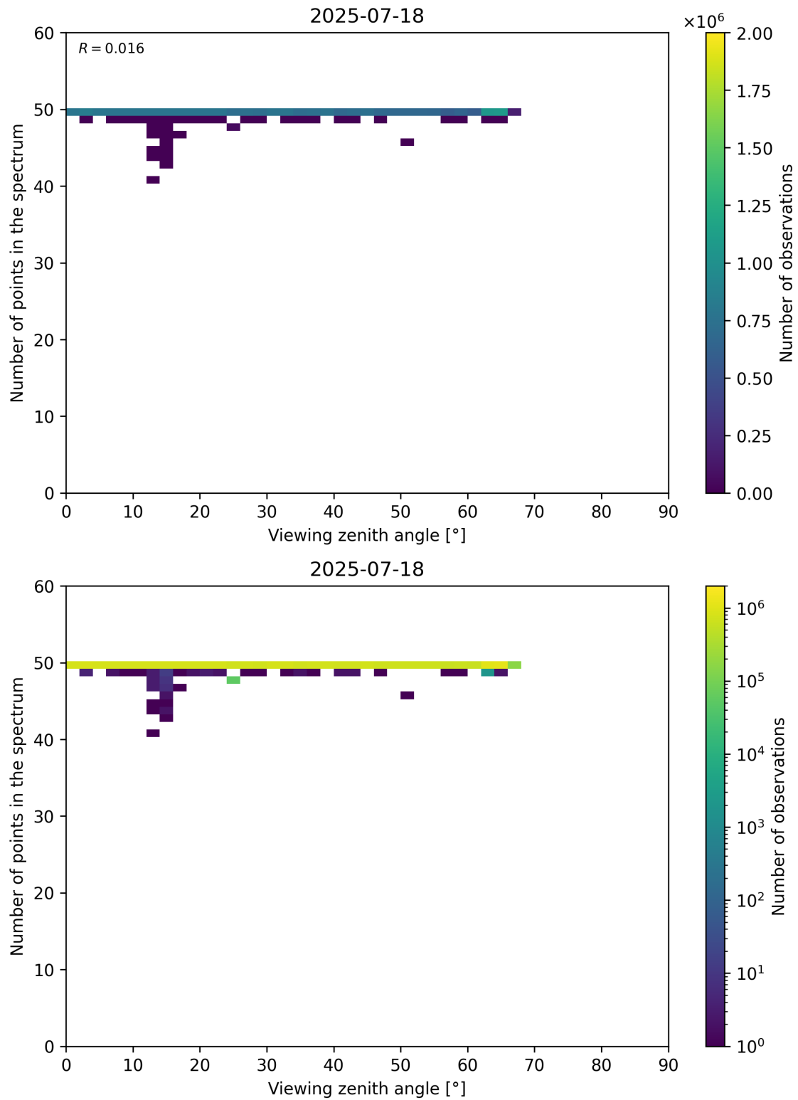
Figure 125: Scatter density plot of “Viewing zenith angle” against “Number of points in the spectrum” for 2025-07-18 to 2025-07-19.
