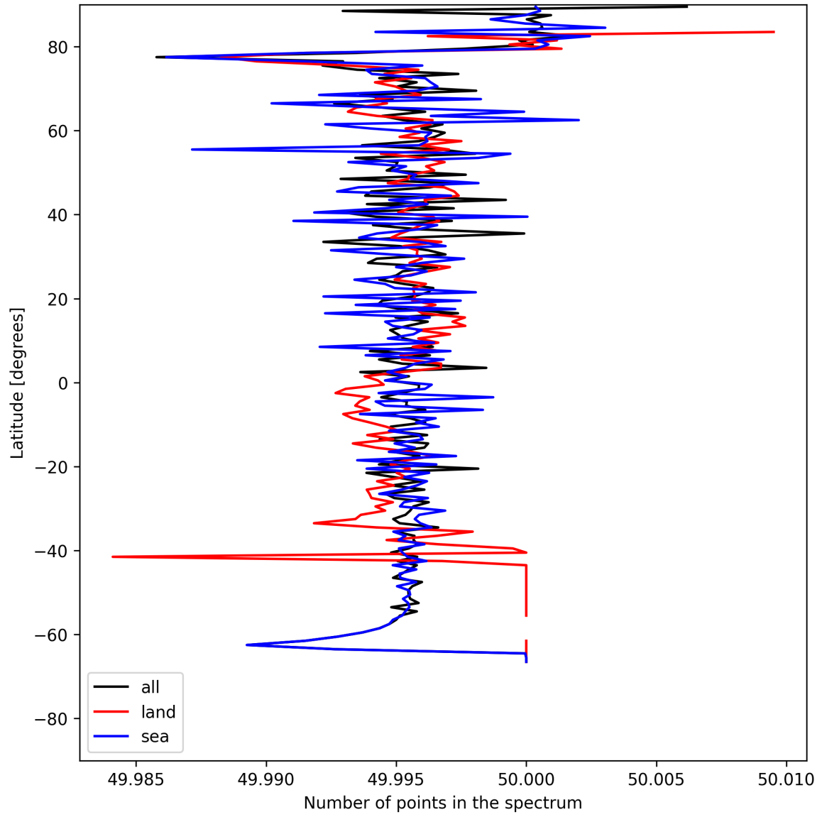
Figure 27: Zonal average of “Number of points in the spectrum” for 2025-07-18 to 2025-07-19.
