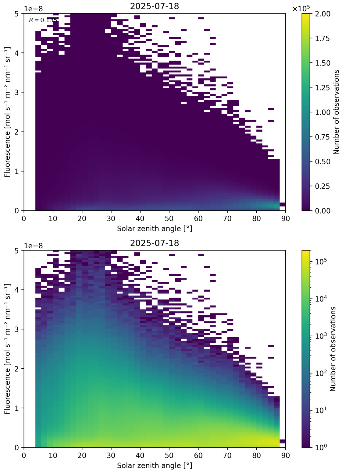
Figure 112: Scatter density plot of “Solar zenith angle” against “Fluorescence” for 2025-07-18 to 2025-07-19.
