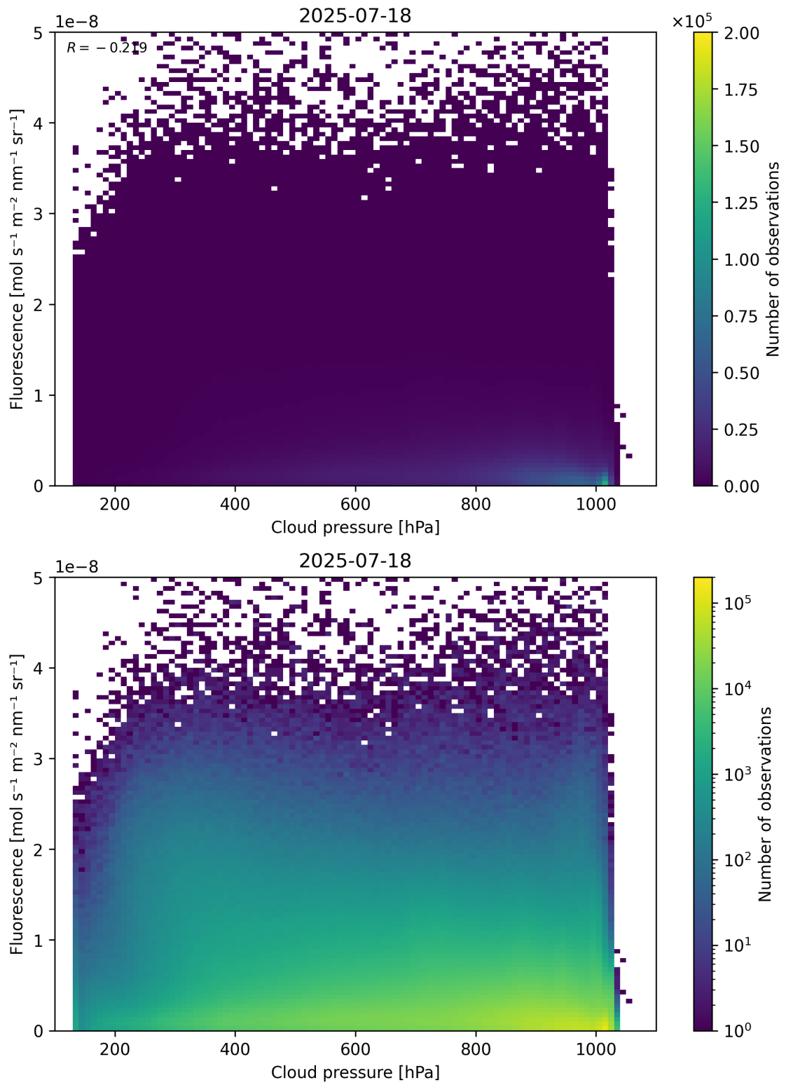
Figure 80: Scatter density plot of “Cloud pressure” against “Fluorescence” for 2025-07-18 to 2025-07-19.
