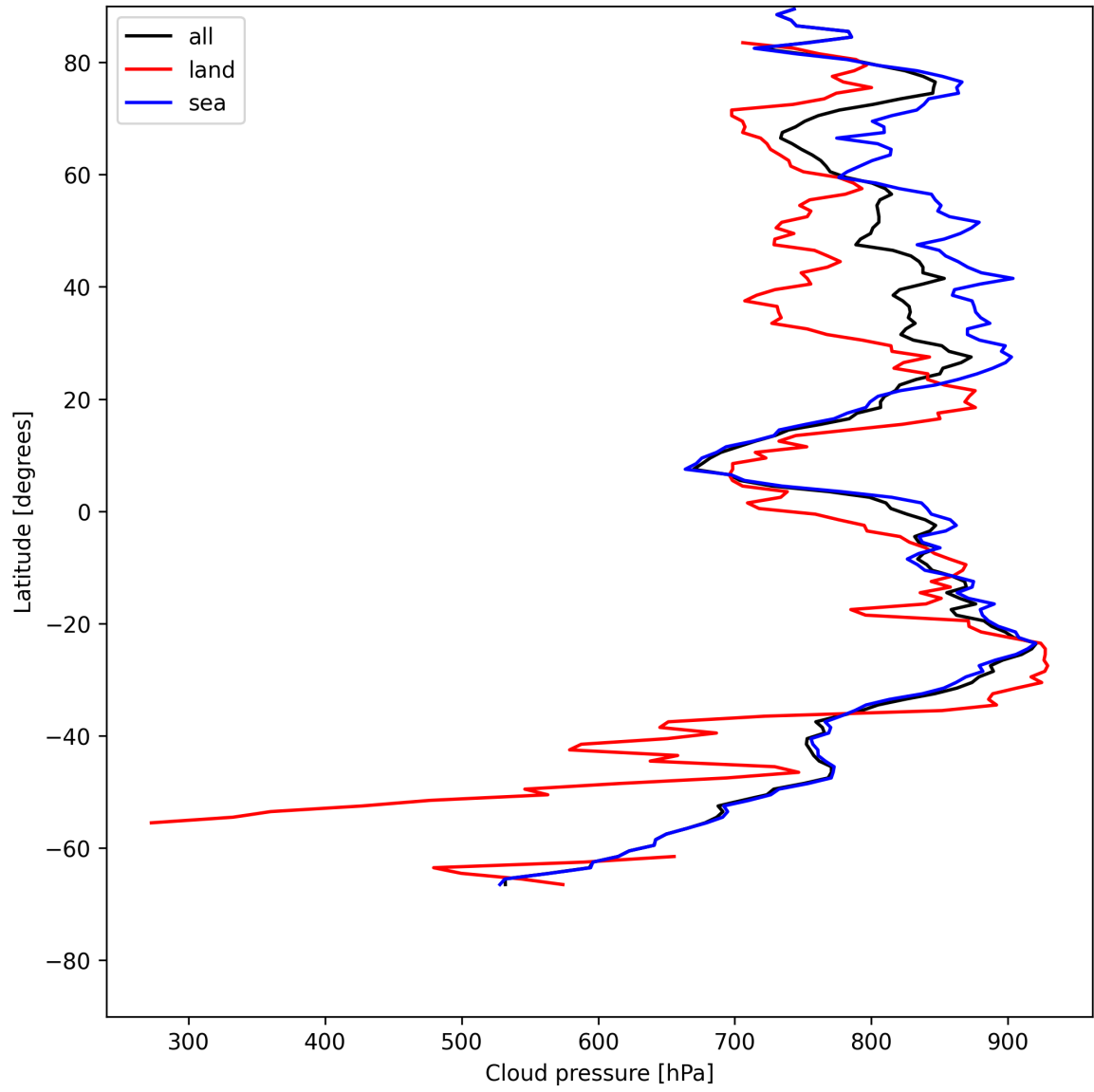
Figure 13: Zonal average of “Cloud pressure” for 2025-07-18 to 2025-07-19.
