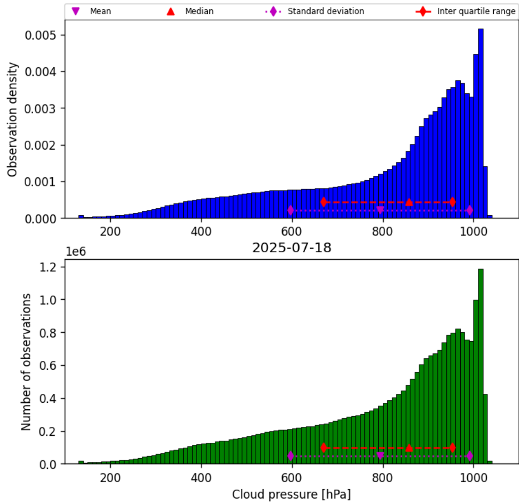
Figure 30: Histogram of “Cloud pressure” for 2025-07-18 to 2025-07-19
