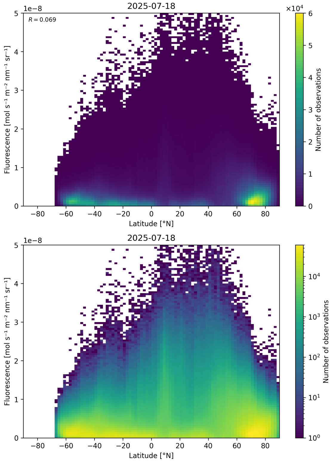
Figure 92: Scatter density plot of “Latitude” against “Fluorescence” for 2025-07-18 to 2025-07-19.
