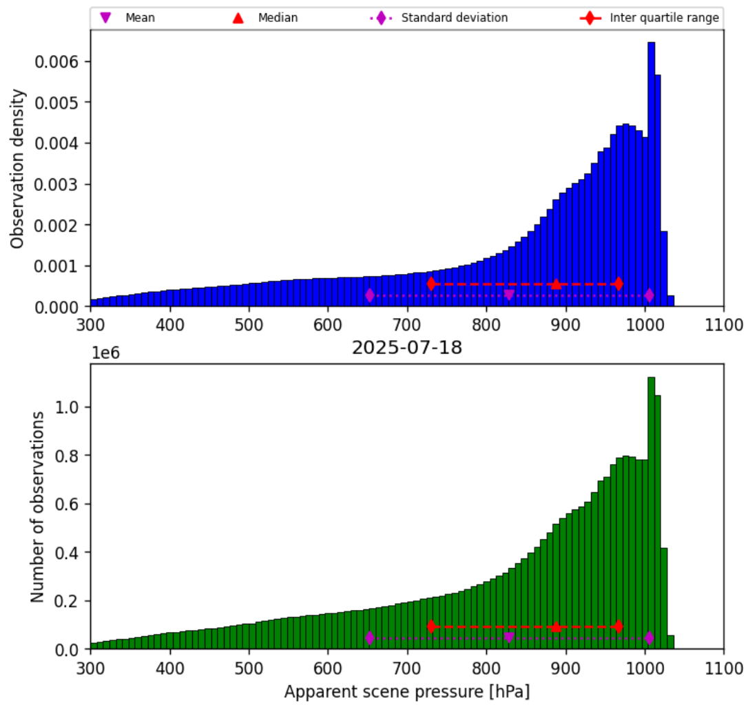
Figure 36: Histogram of “Apparent scene pressure” for 2025-07-18 to 2025-07-19
