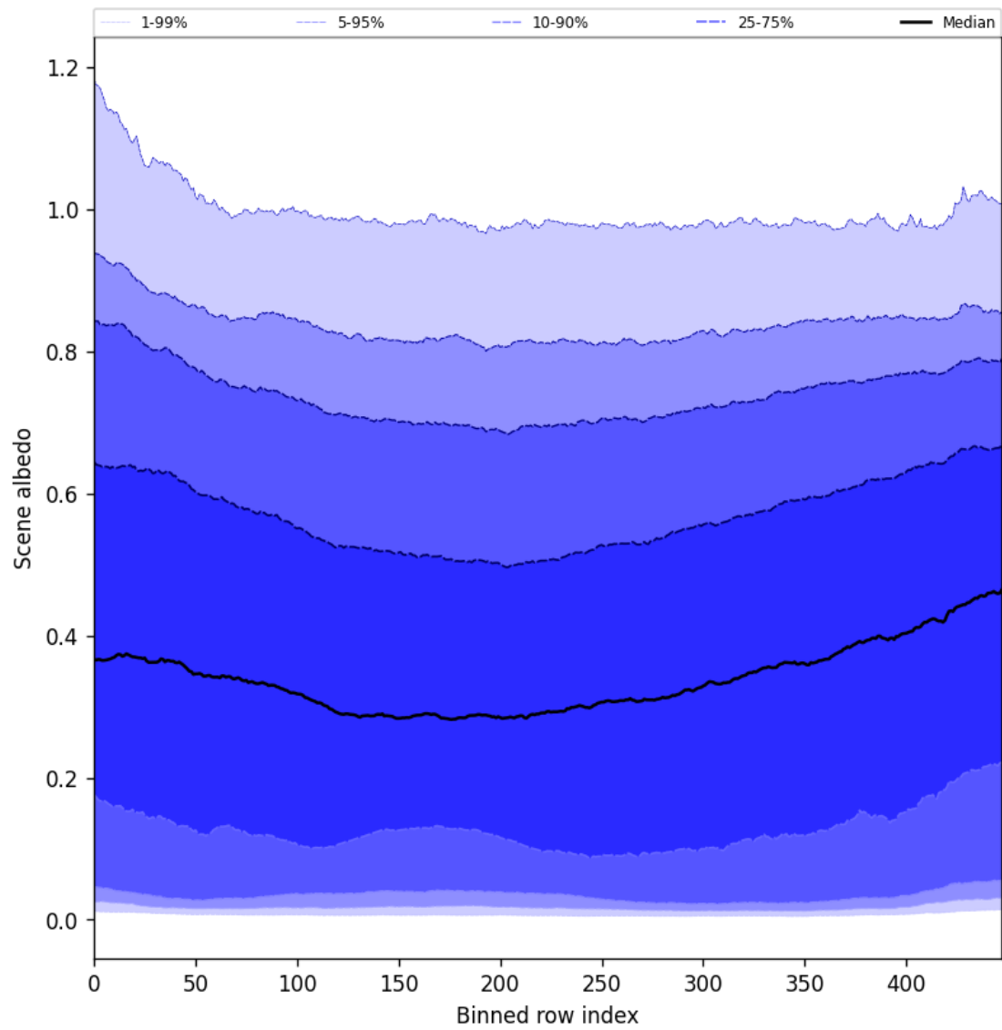
Figure 51: Along track statistics of “Scene albedo” for 2025-07-18 to 2025-07-19
