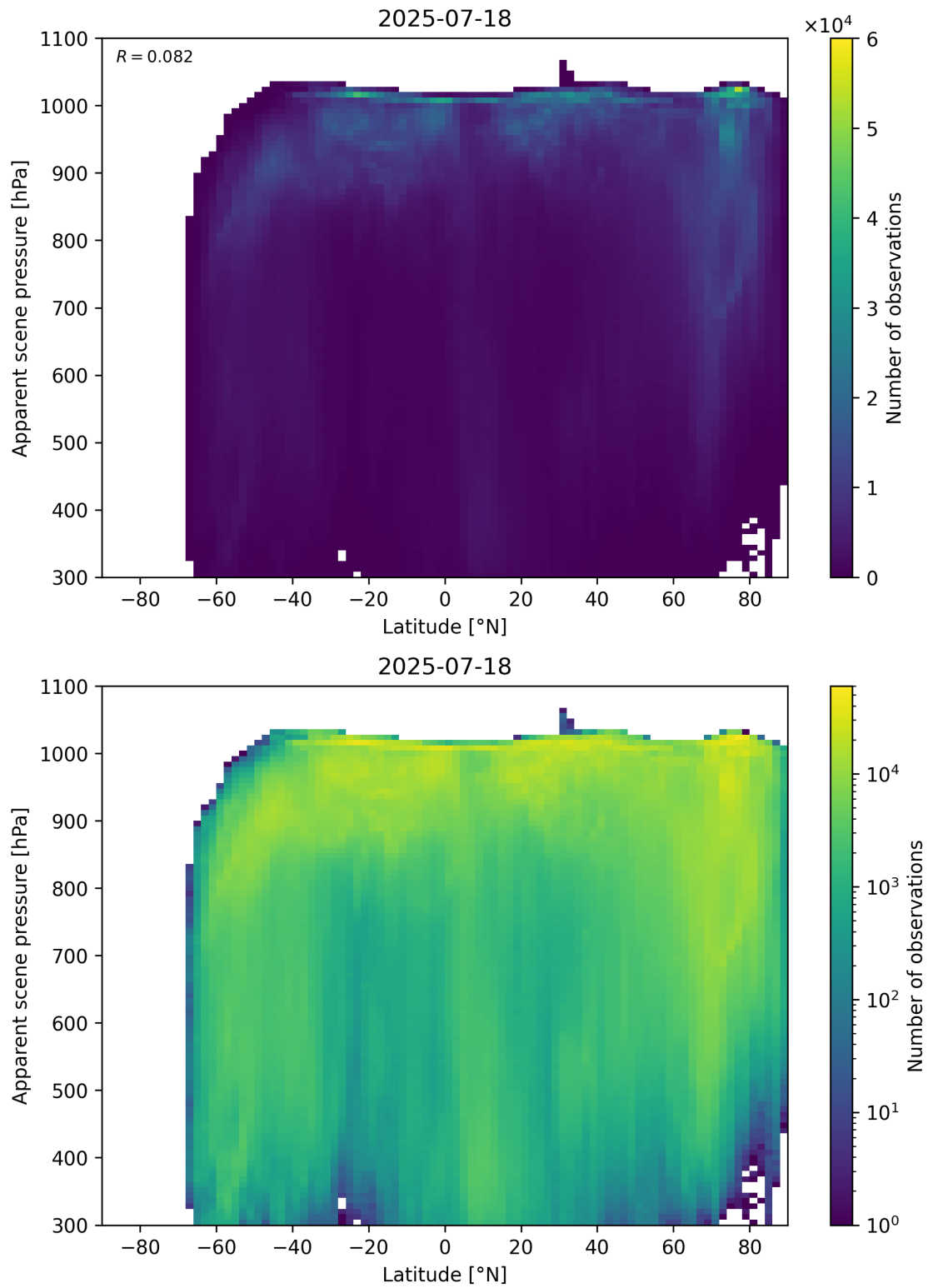
Figure 88: Scatter density plot of “Latitude” against “Apparent scene pressure” for 2025-07-18 to 2025-07-19.
