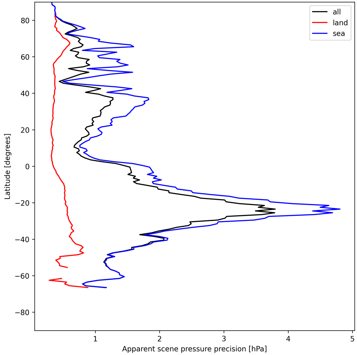
Figure 20: Zonal average of “Apparent scene pressure precision” for 2025-07-18 to 2025-07-19.
