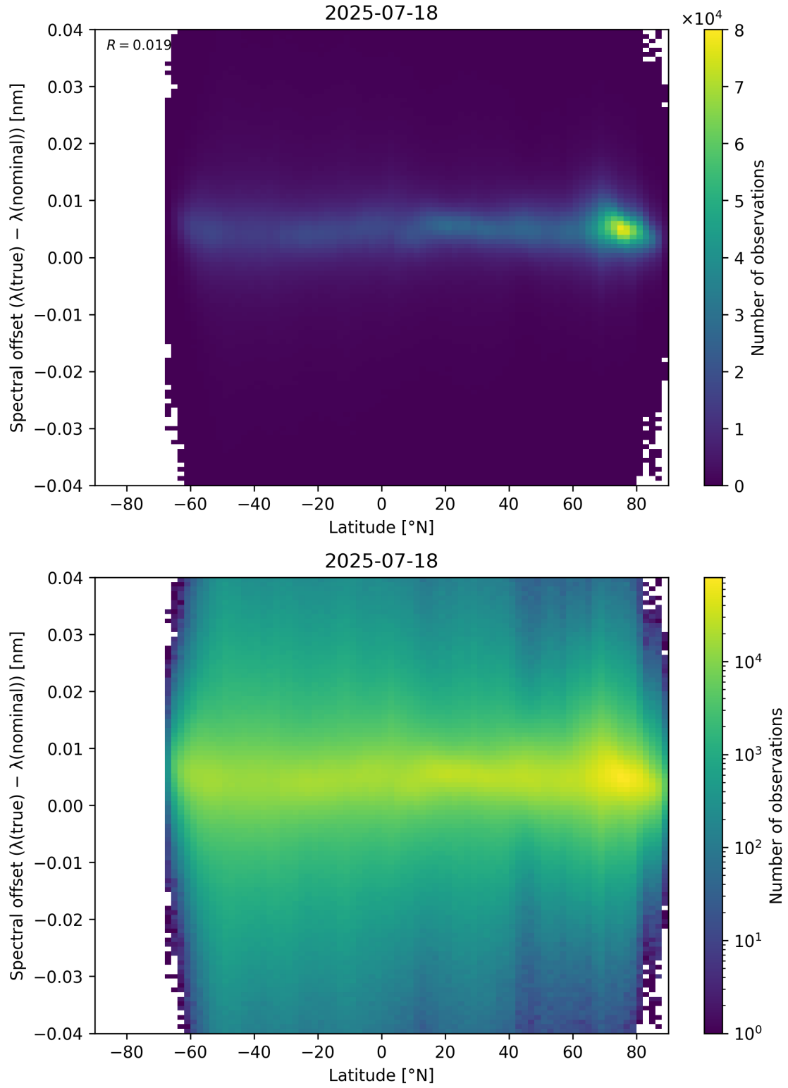
Figure 96: Scatter density plot of “Latitude” against “Spectral offset ( \lambda_{\text{true}} - \lambda_{\text{nominal}} )” for 2025-07-18 to 2025-07-19.
