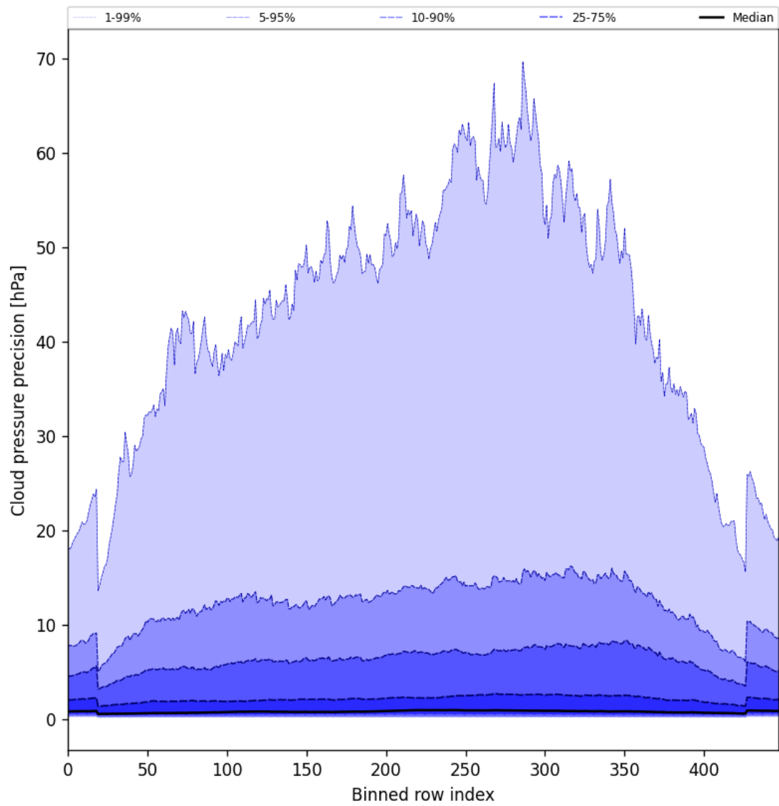
Figure 48: Along track statistics of “Cloud pressure precision” for 2025-07-18 to 2025-07-19
