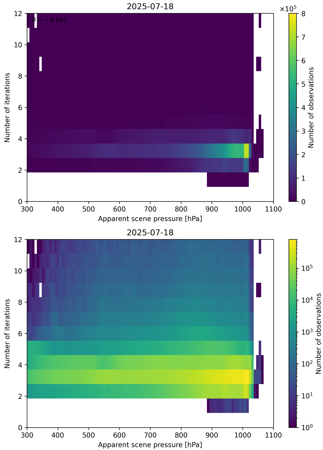
Figure 65: Scatter density plot of “Apparent scene pressure” against “Number of iterations” for 2025-07-18 to 2025-07-19.
