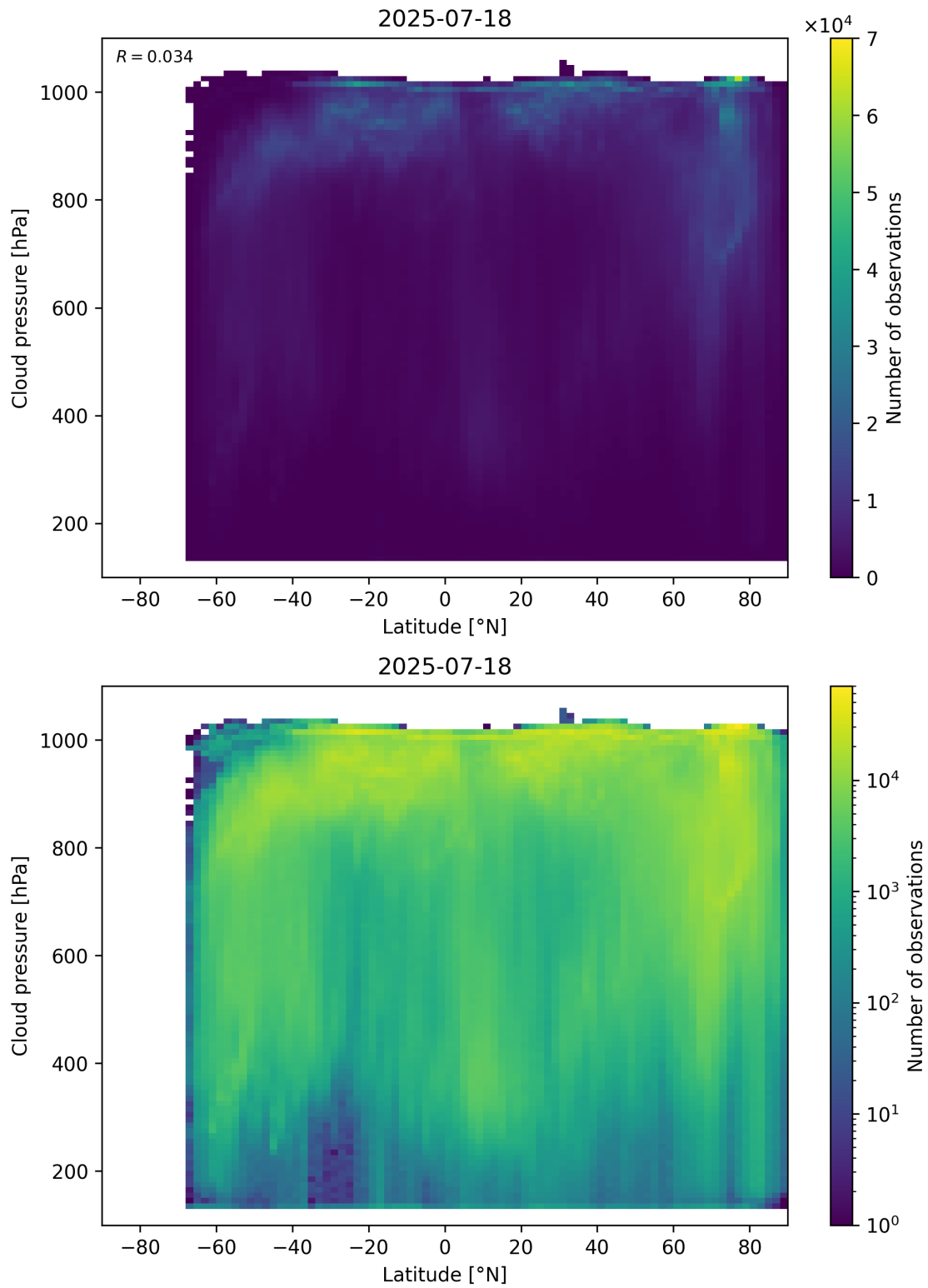
Figure 91: Scatter density plot of “Latitude” against “Cloud pressure” for 2025-07-18 to 2025-07-19.
