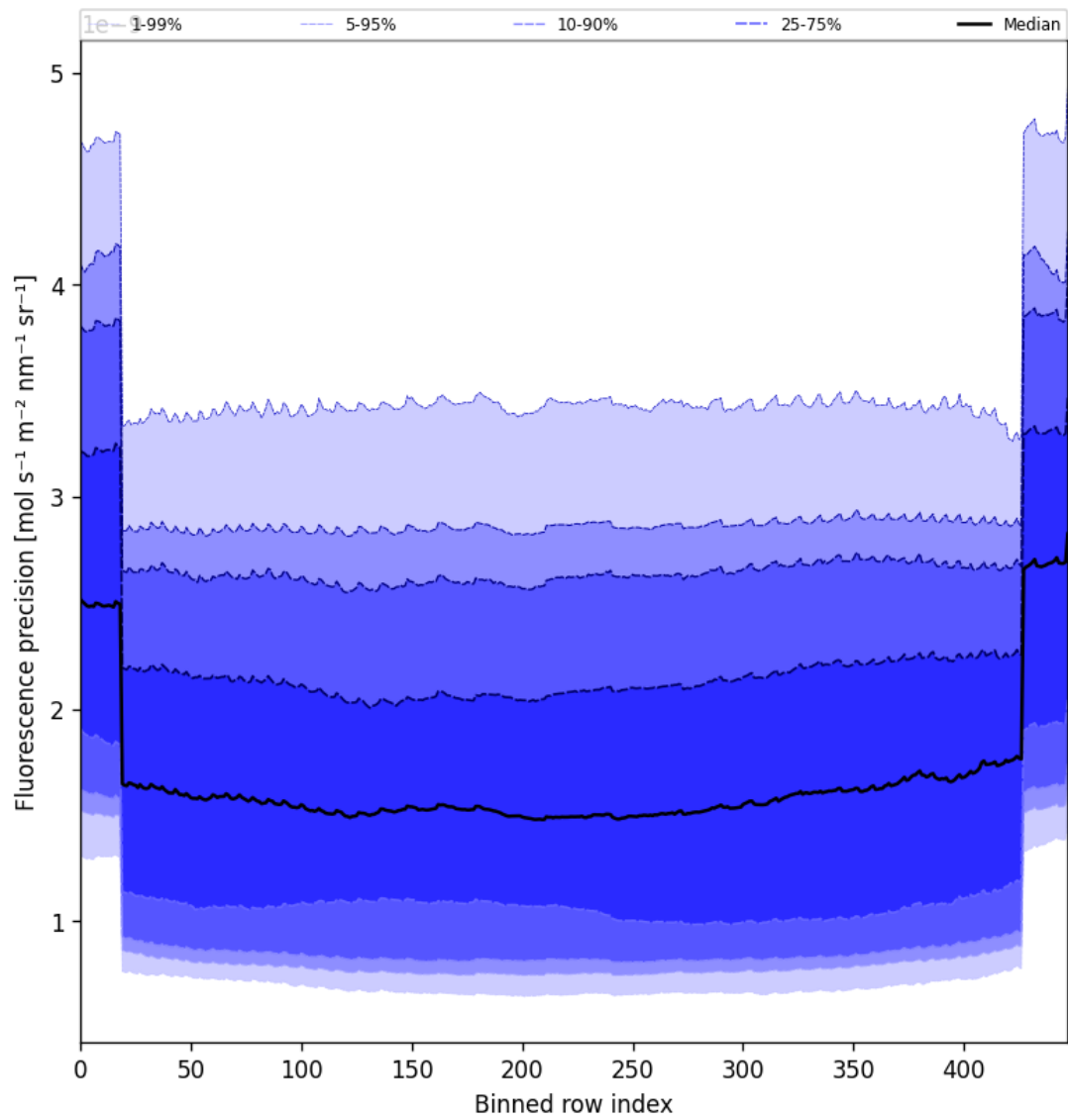
Figure 58: Along track statistics of “Fluorescence precision” for 2025-07-18 to 2025-07-19
