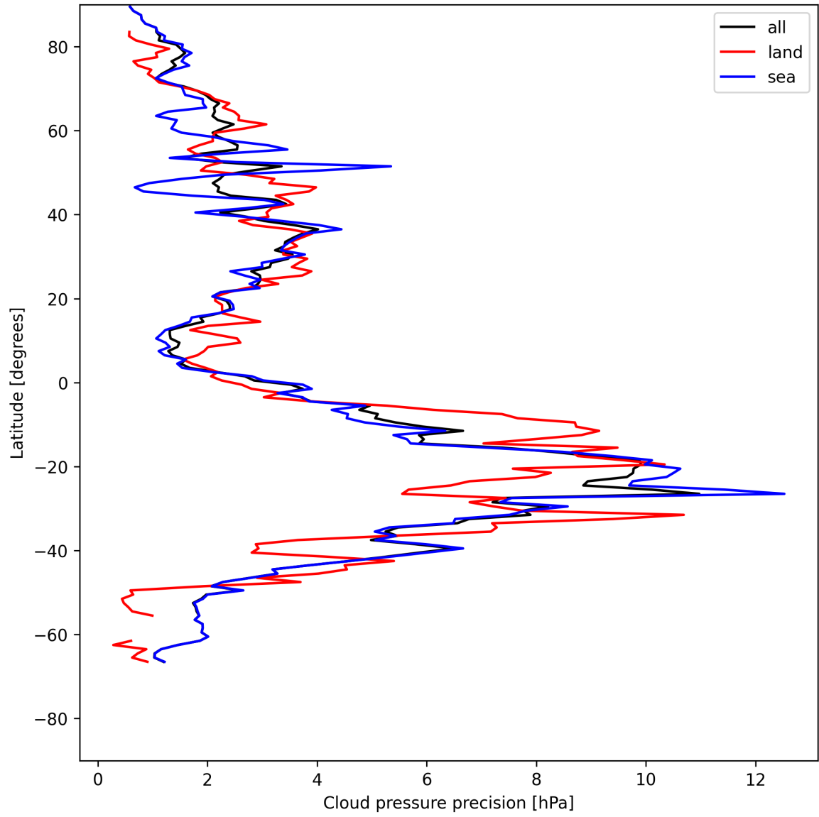
Figure 14: Zonal average of "Cloud pressure precision" for 2025-07-18 to 2025-07-19.
