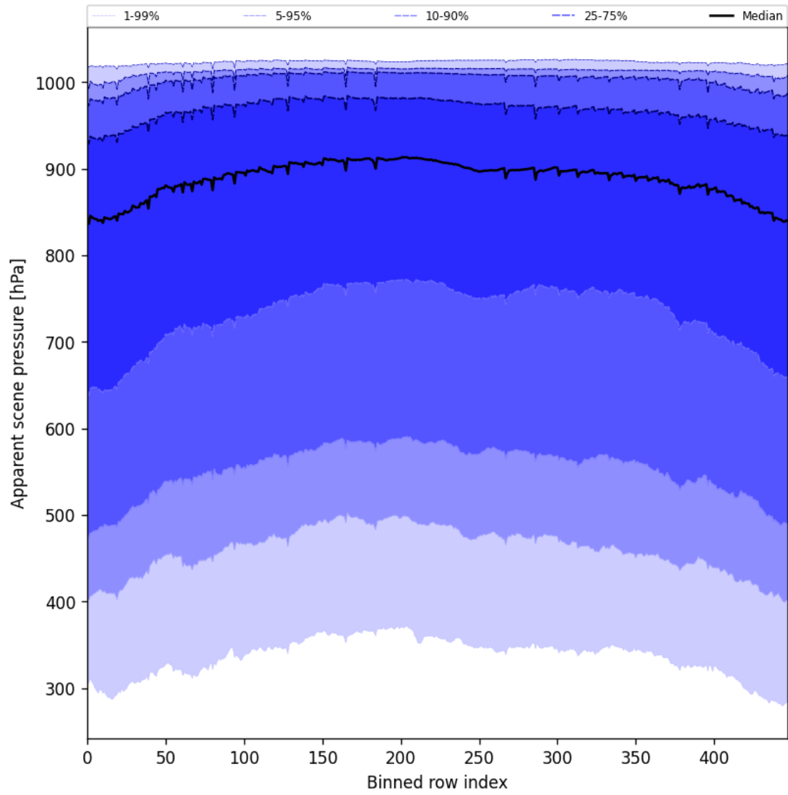
Figure 53: Along track statistics of “Apparent scene pressure” for 2025-07-18 to 2025-07-19
