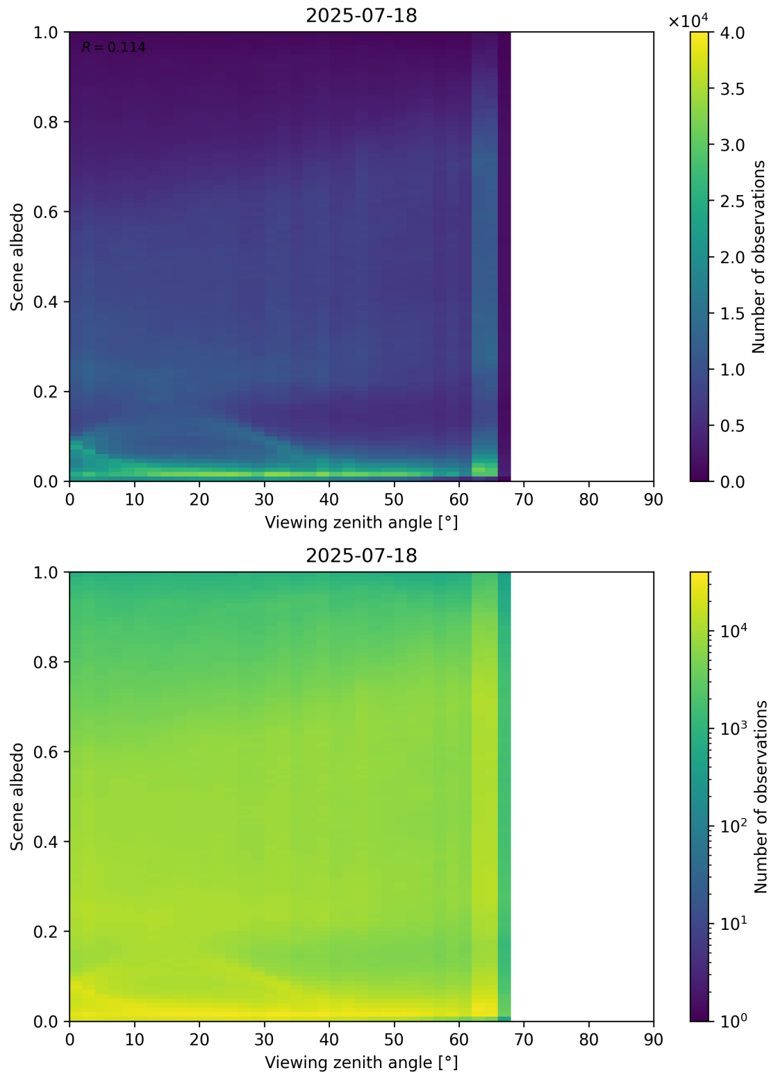
Figure 126: Scatter density plot of “Viewing zenith angle” against “Scene albedo” for 2025-07-18 to 2025-07-19.
