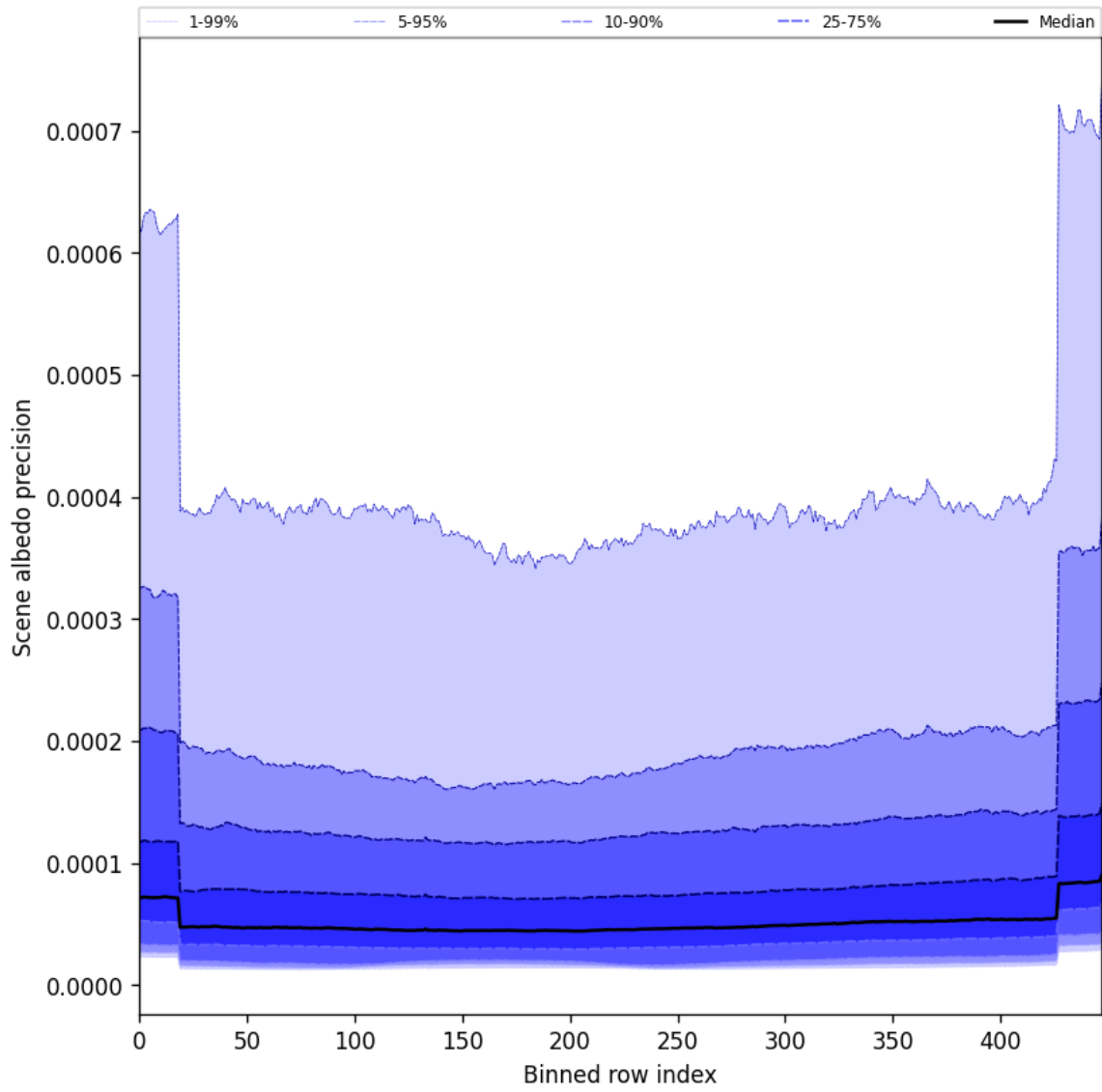
Figure 52: Along track statistics of “Scene albedo precision” for 2025-07-18 to 2025-07-19
