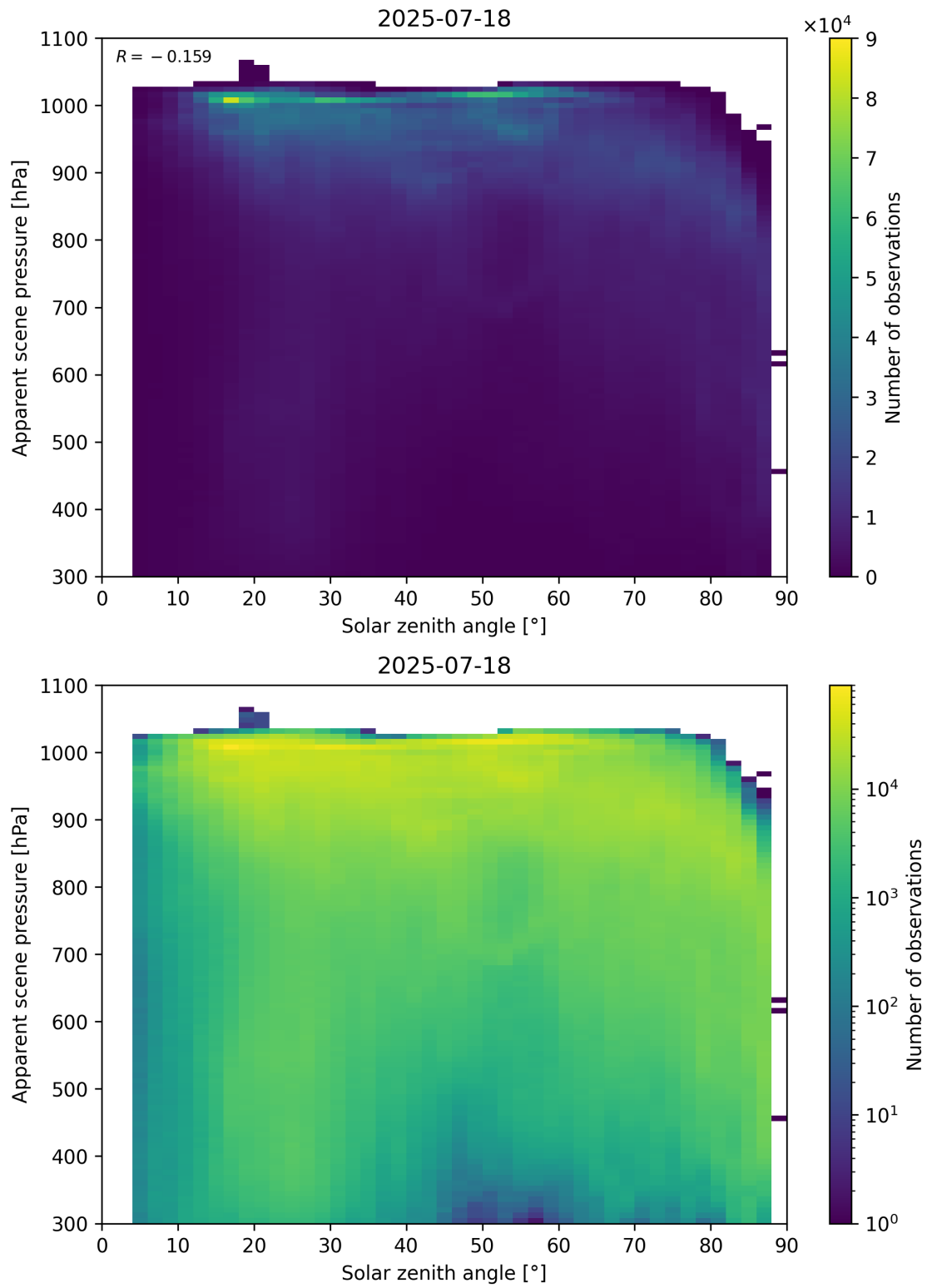
Figure 108: Scatter density plot of “Solar zenith angle” against “Apparent scene pressure” for 2025-07-18 to 2025-07-19.
