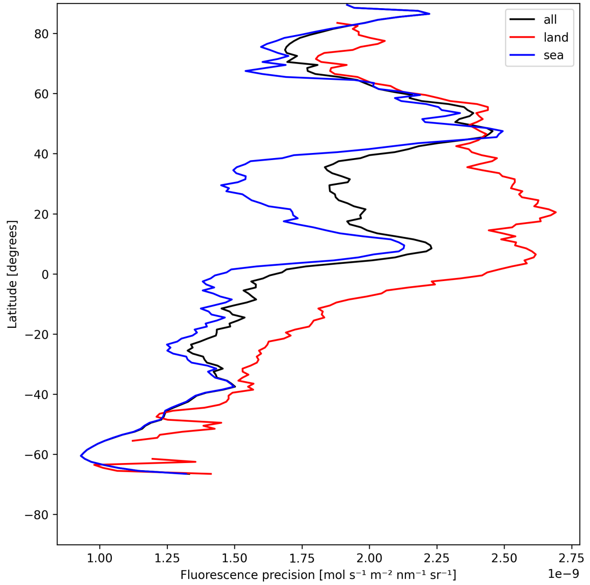
Figure 24: Zonal average of “Fluorescence precision” for 2025-07-18 to 2025-07-19.
