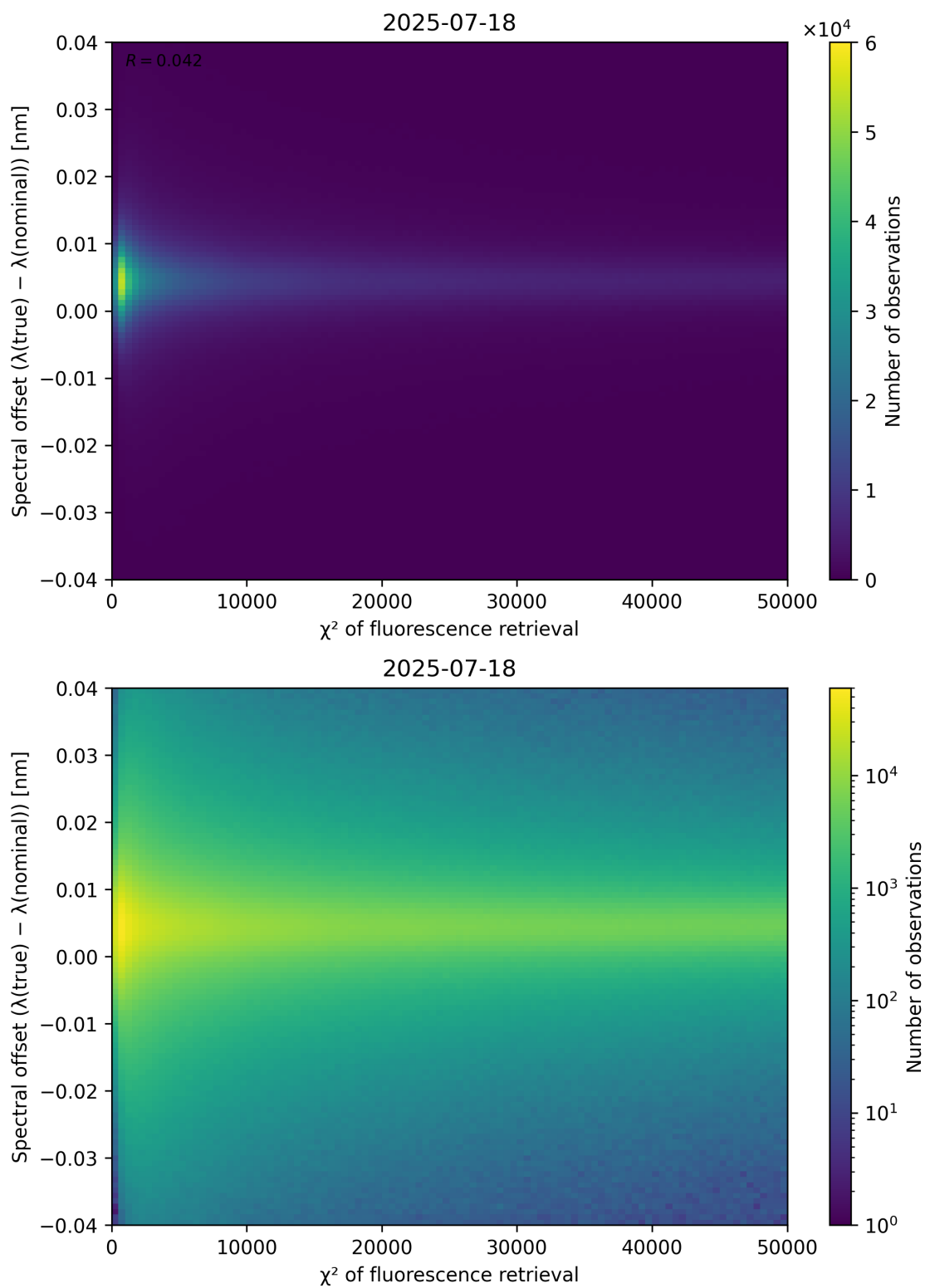
Figure 69: Scatter density plot of “ \chi^2 of fluorescence retrieval” against “Spectral offset ( \lambda_{\text{true}} - \lambda_{\text{nominal}} )” for 2025-07-18 to 2025-07-19.
