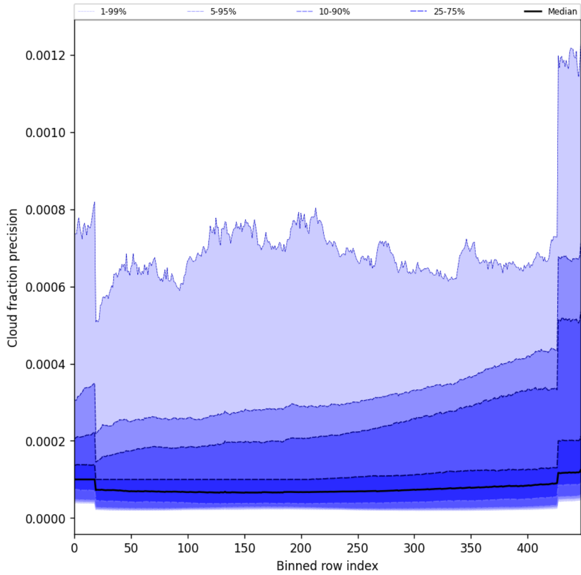
Figure 50: Along track statistics of “Cloud fraction precision” for 2025-07-18 to 2025-07-19
