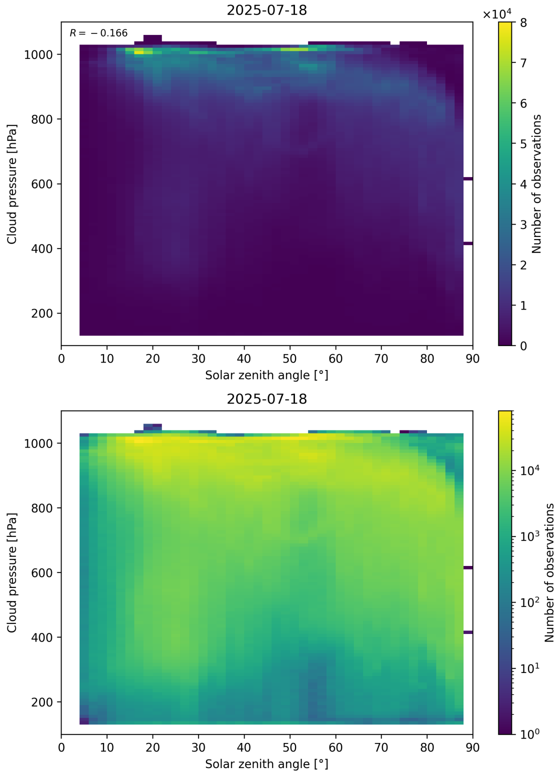
Figure 111: Scatter density plot of “Solar zenith angle” against “Cloud pressure” for 2025-07-18 to 2025-07-19.
