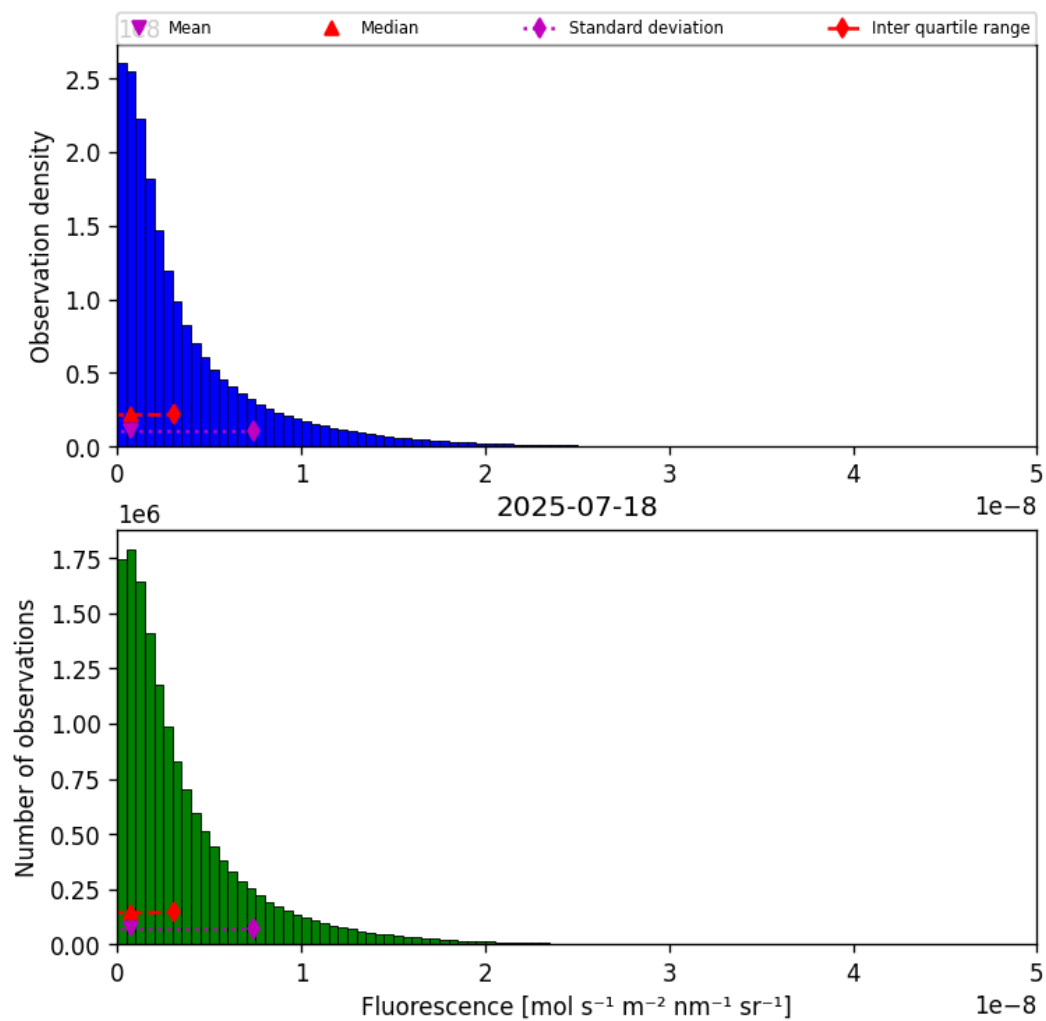
Figure 40: Histogram of “Fluorescence” for 2025-07-18 to 2025-07-19
