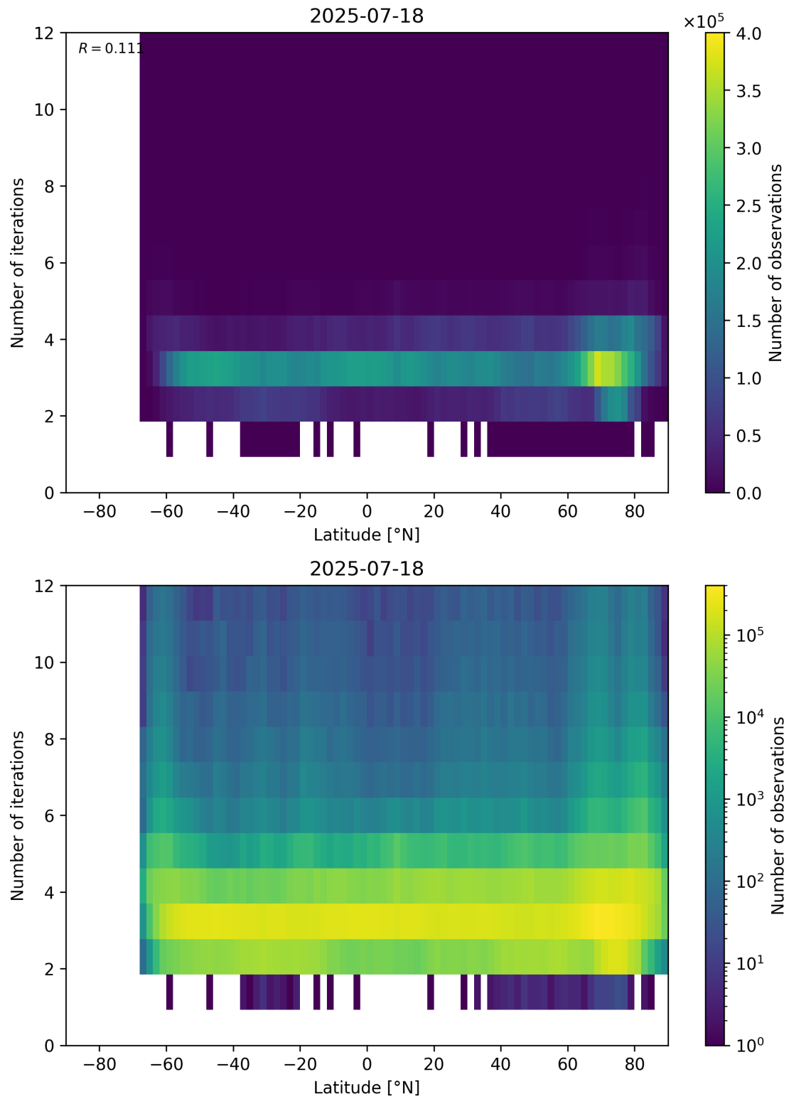
Figure 93: Scatter density plot of “Latitude” against “Number of iterations” for 2025-07-18 to 2025-07-19.
