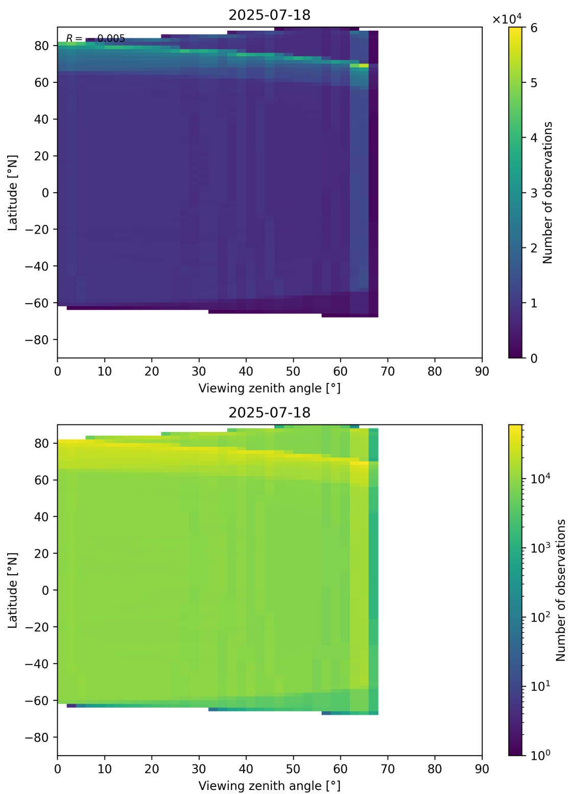
Figure 123: Scatter density plot of “Viewing zenith angle” against “Latitude” for 2025-07-18 to 2025-07-19.
