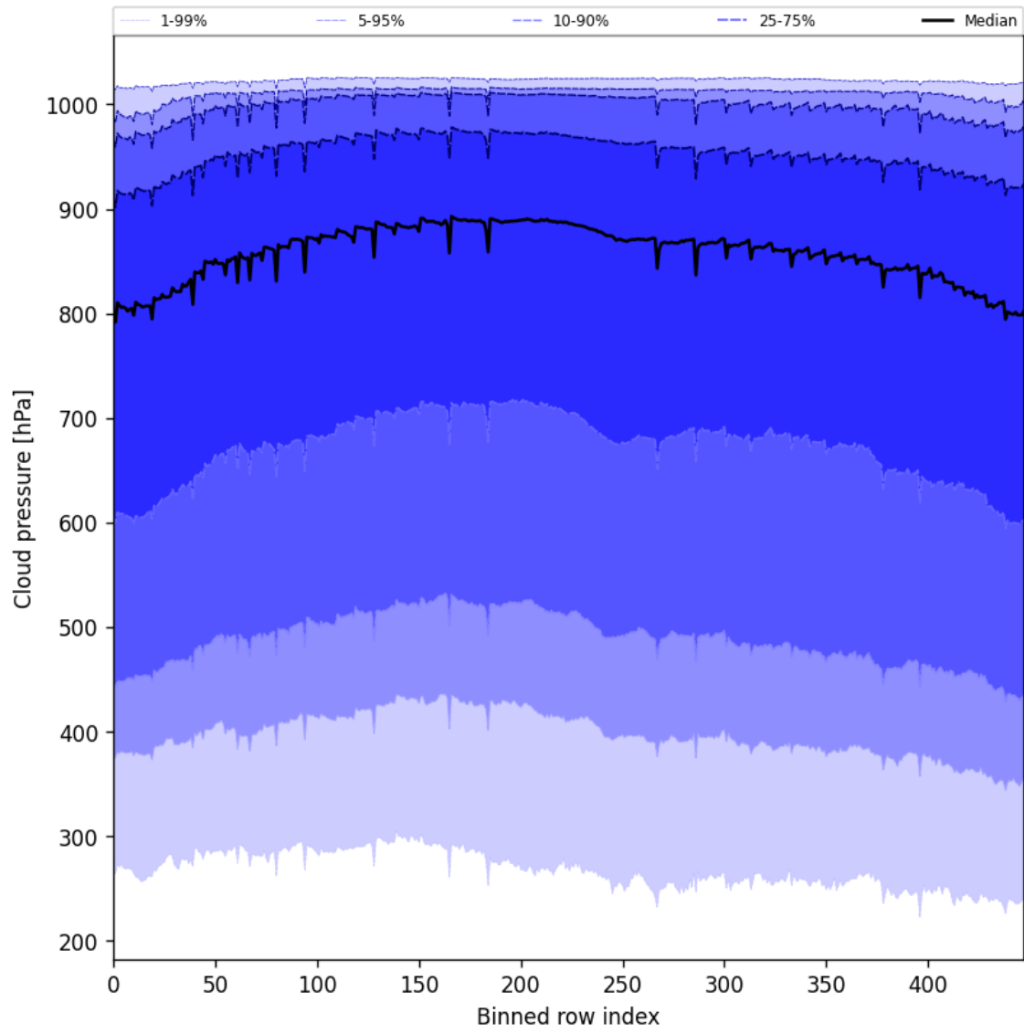
Figure 47: Along track statistics of “Cloud pressure” for 2025-07-18 to 2025-07-19
