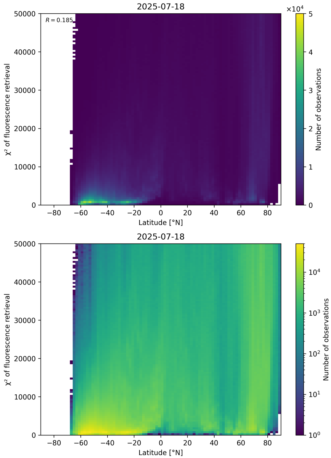
Figure 89: Scatter density plot of “Latitude” against “ \chi^2 of fluorescence retrieval” for 2025-07-18 to 2025-07-19.
