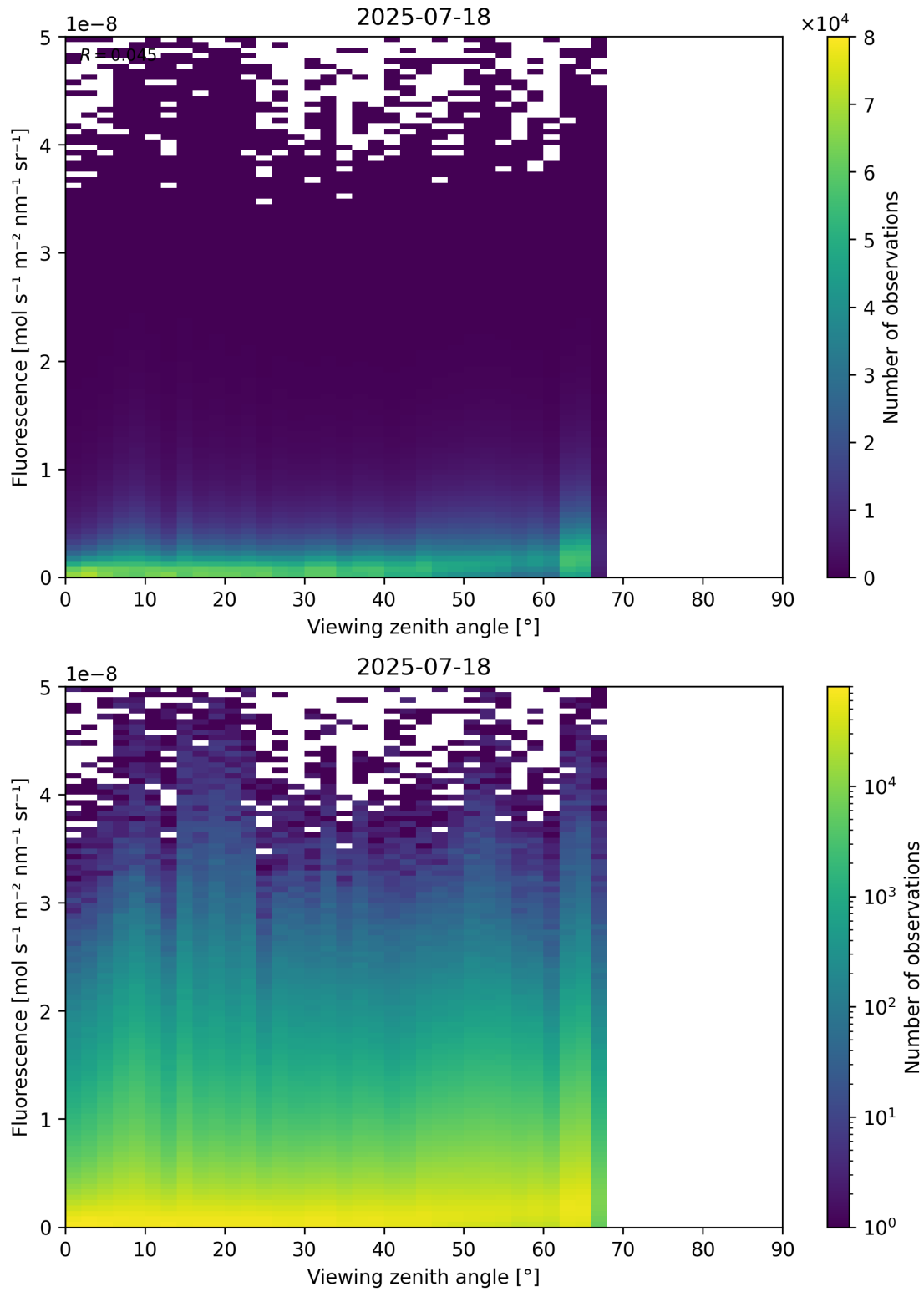
Figure 122: Scatter density plot of “Viewing zenith angle” against “Fluorescence” for 2025-07-18 to 2025-07-19.
