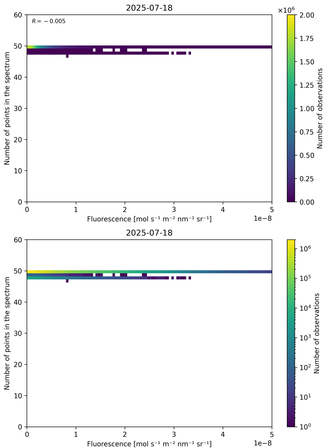
Figure 86: Scatter density plot of “Fluorescence” against “Number of points in the spectrum” for 2025-07-18 to 2025-07-19.
