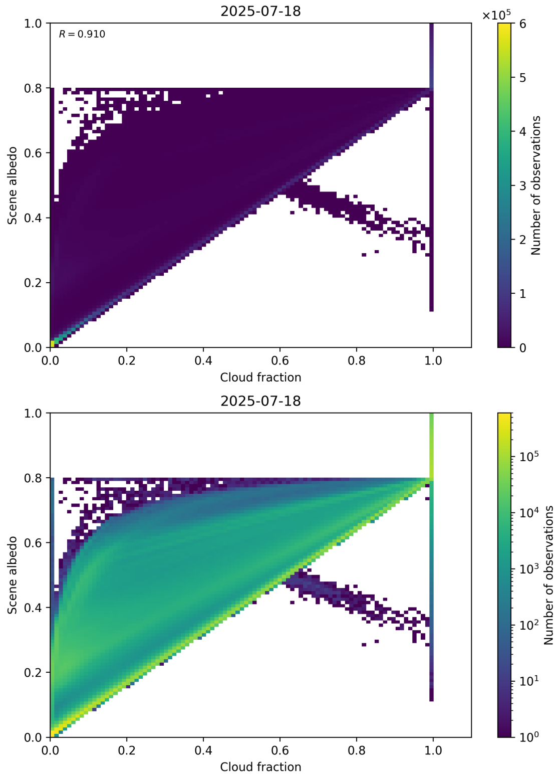
Figure 75: Scatter density plot of “Cloud fraction” against “Scene albedo” for 2025-07-18 to 2025-07-19.
