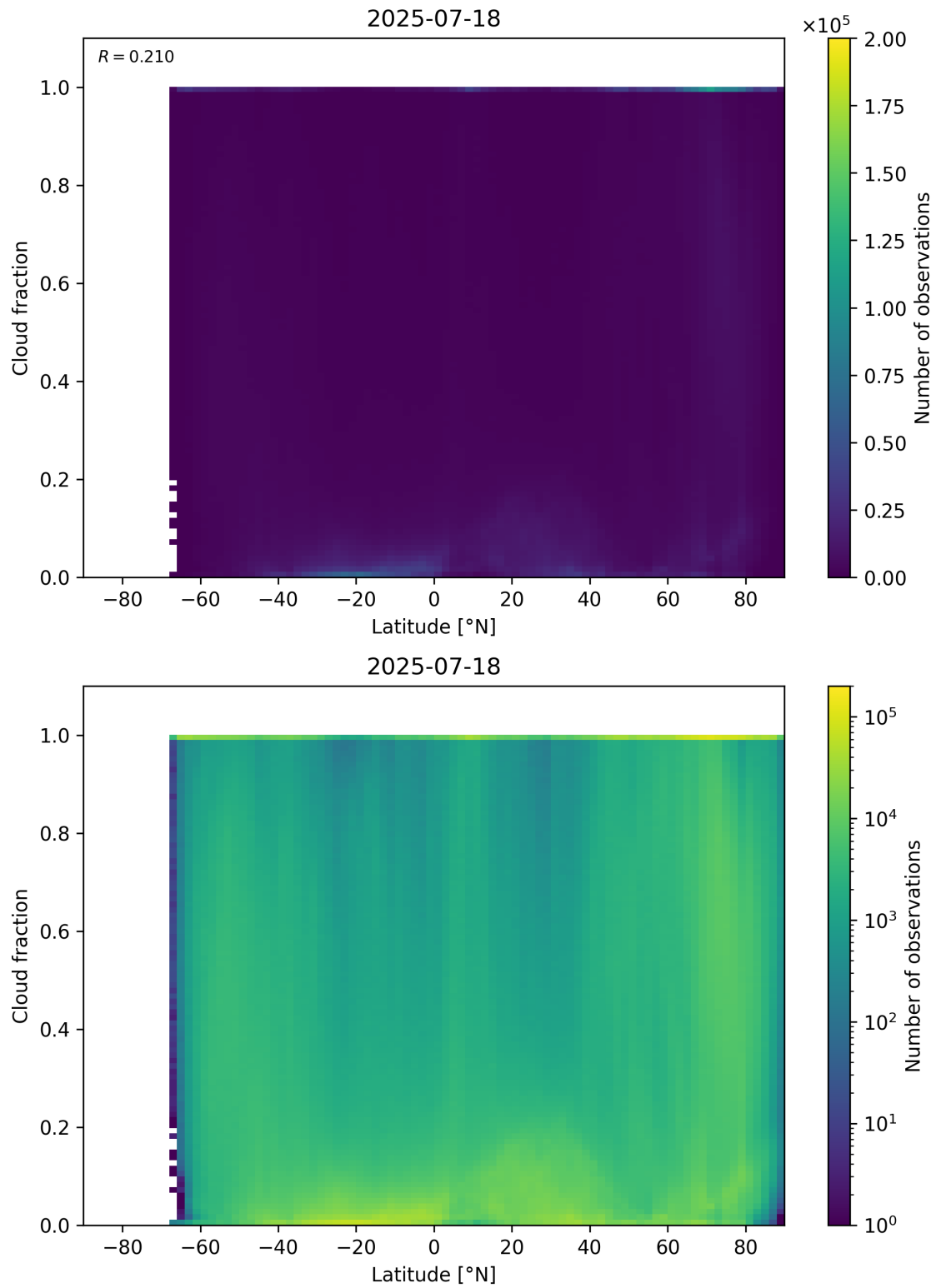
Figure 90: Scatter density plot of “Latitude” against “Cloud fraction” for 2025-07-18 to 2025-07-19.
