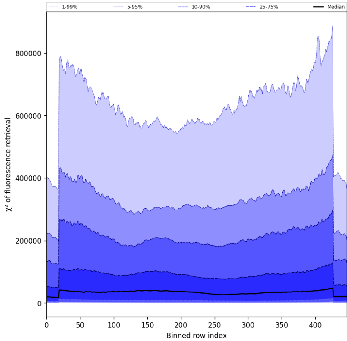
Figure 59: Along track statistics of “ \chi^2 of fluorescence retrieval” for 2025-07-18 to 2025-07-19
