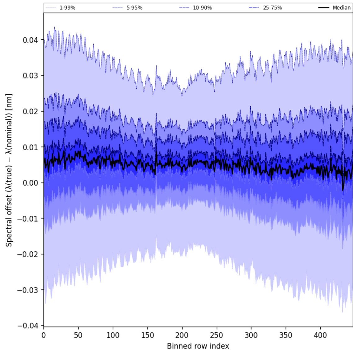
Figure 62: Along track statistics of “Spectral offset ( \lambda_{\text{true}} - \lambda_{\text{nominal}} )” for 2025-07-18 to 2025-07-19
