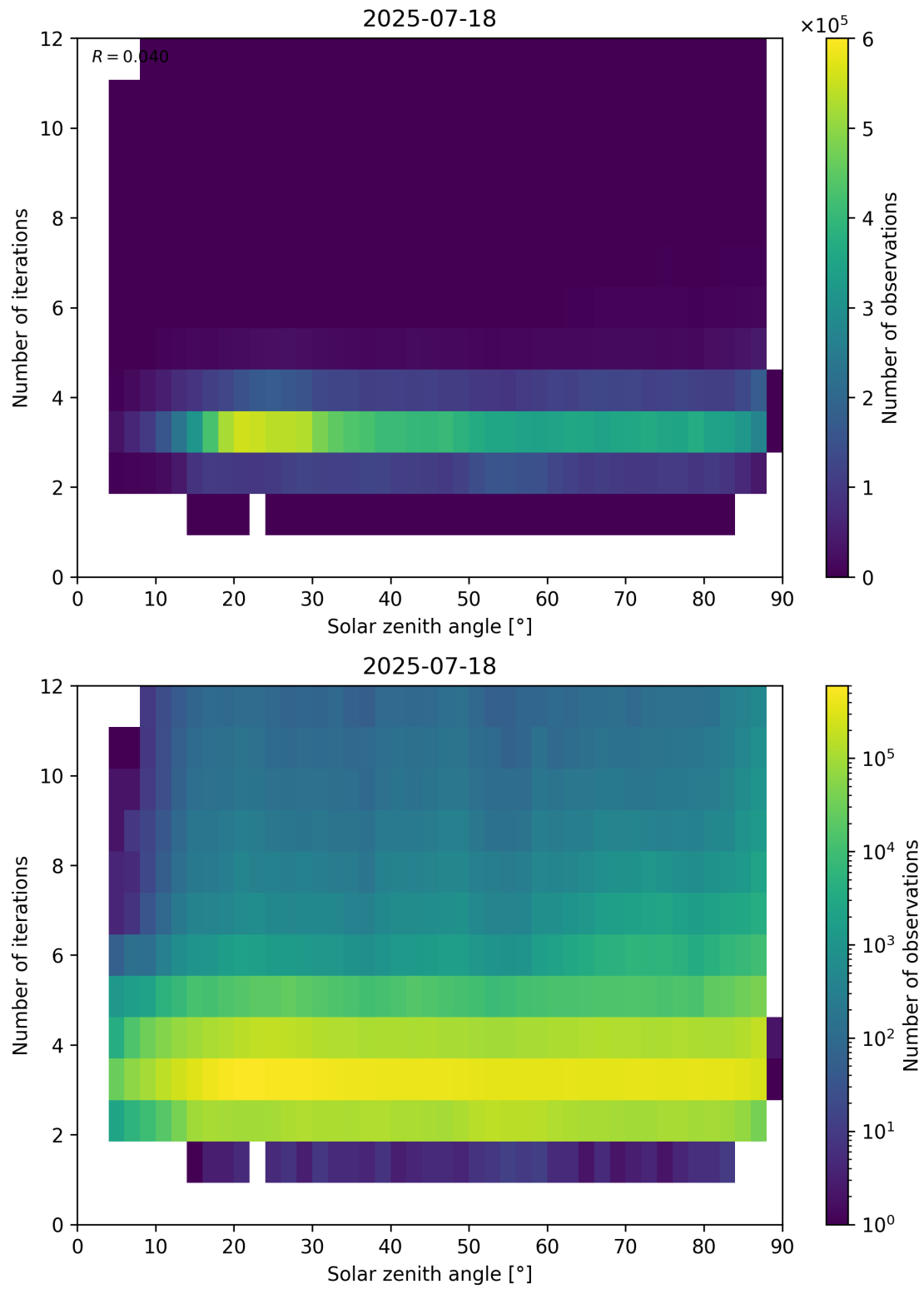
Figure 114: Scatter density plot of “Solar zenith angle” against “Number of iterations” for 2025-07-18 to 2025-07-19.
