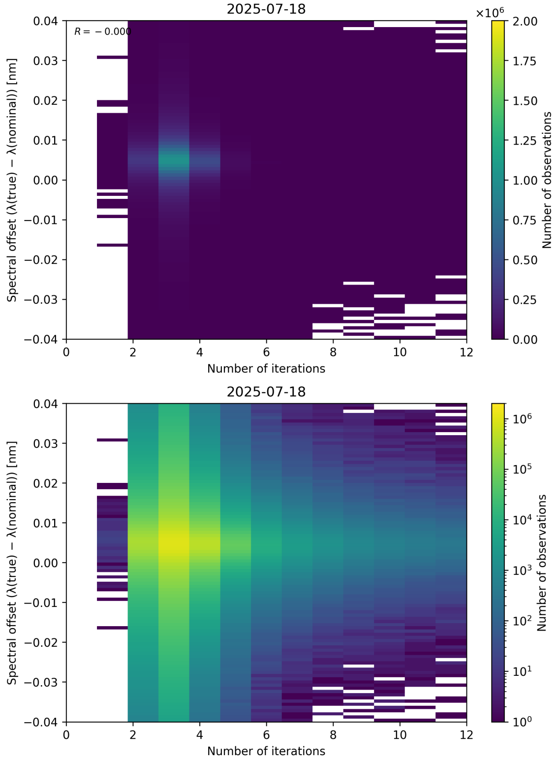
Figure 100: Scatter density plot of “Number of iterations” against “Spectral offset ( \lambda_{\text{true}} - \lambda_{\text{nominal}} )” for 2025-07-18 to 2025-07-19.
