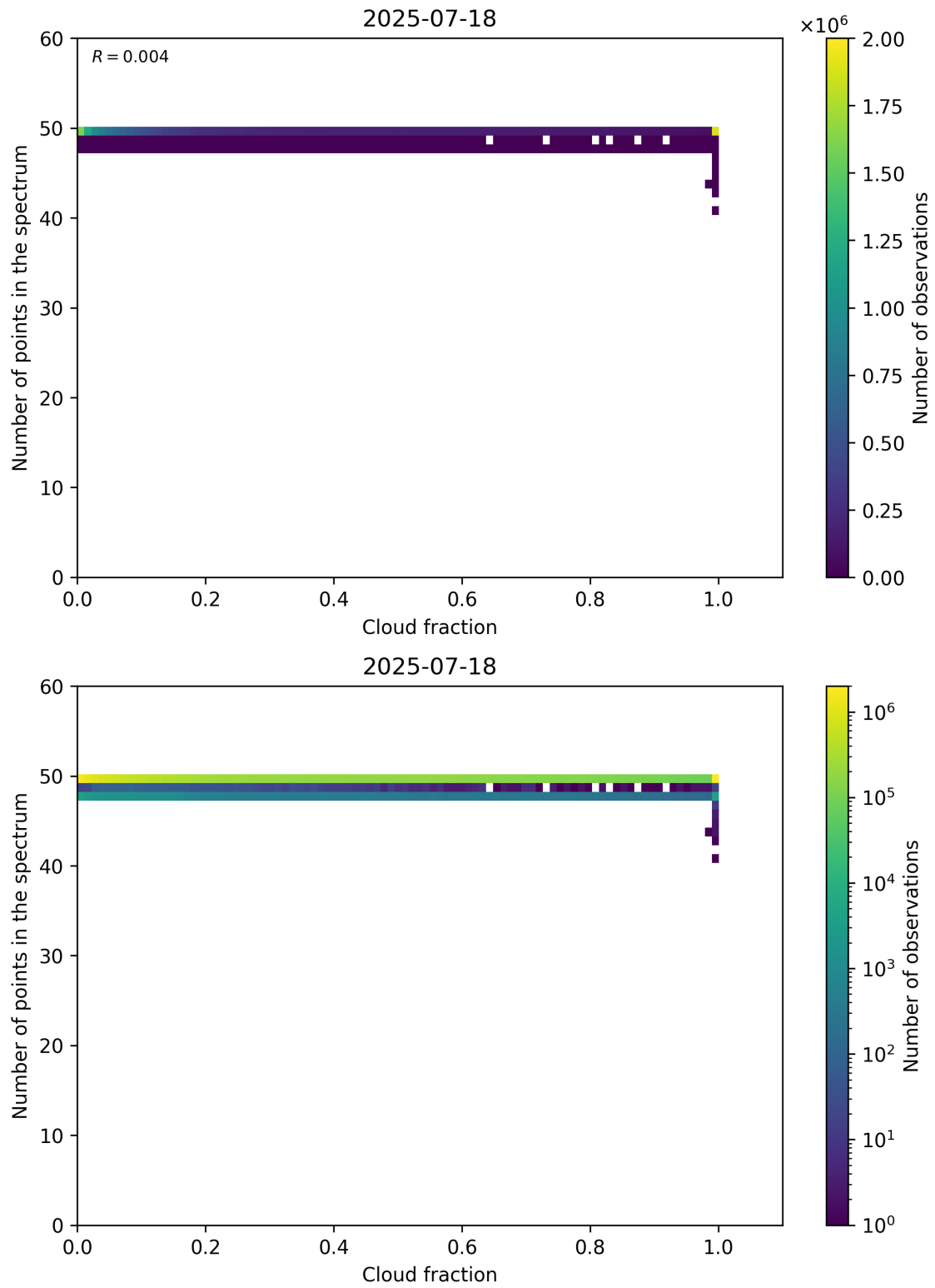
Figure 74: Scatter density plot of “Cloud fraction” against “Number of points in the spectrum” for 2025-07-18 to 2025-07-19.
