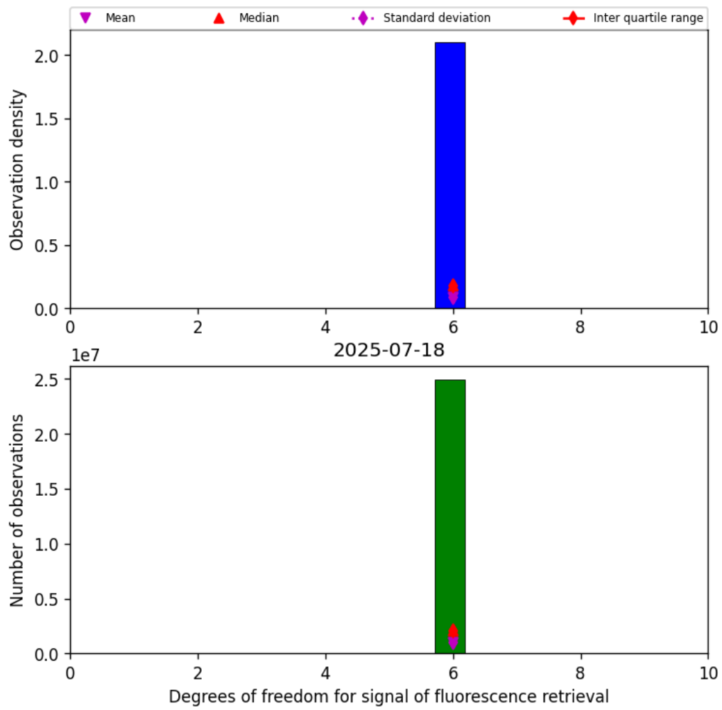
Figure 43: Histogram of “Degrees of freedom for signal of fluorescence retrieval” for 2025-07-18 to 2025-07-19
