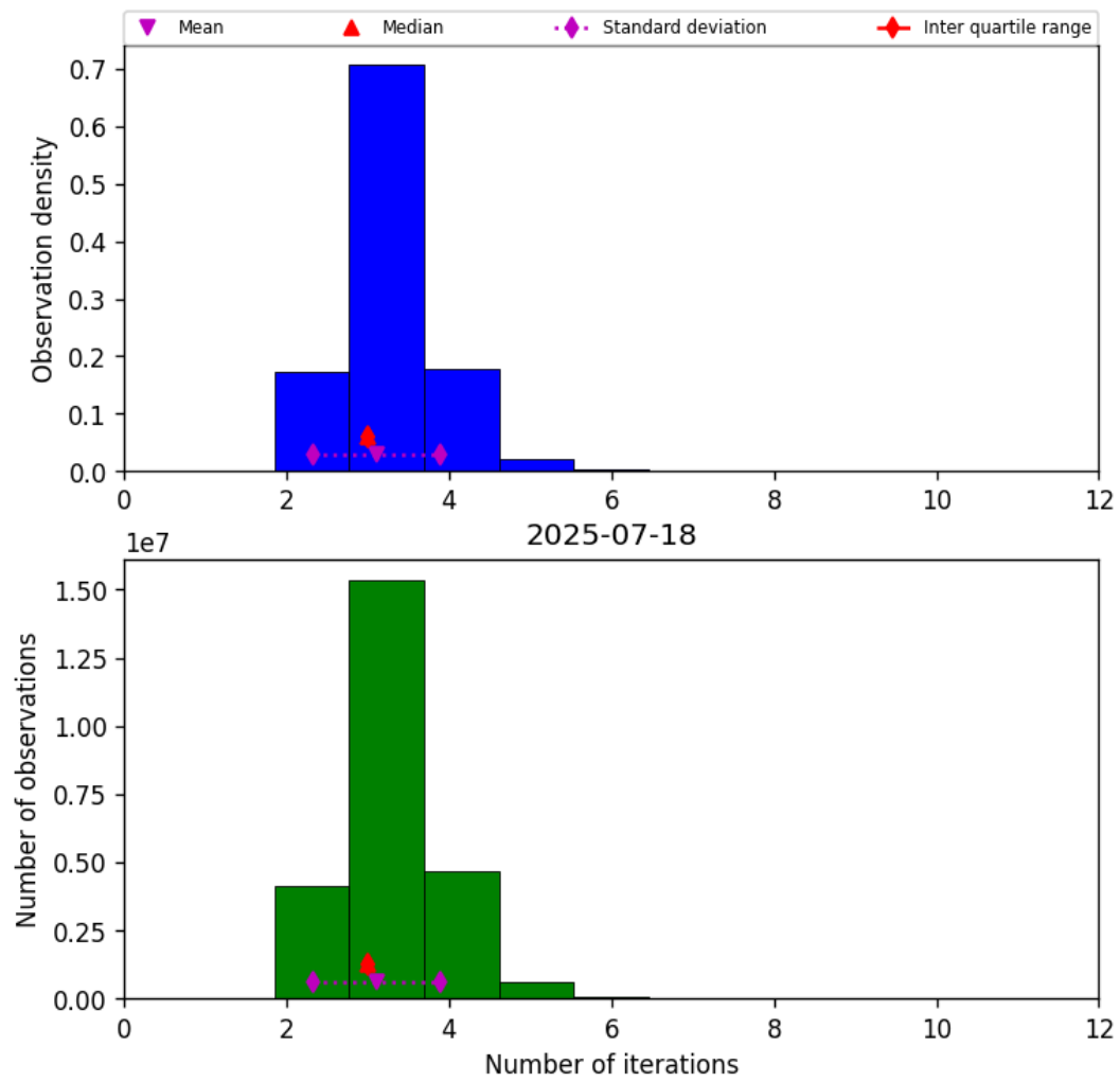
Figure 39: Histogram of “Number of iterations” for 2025-07-18 to 2025-07-19
