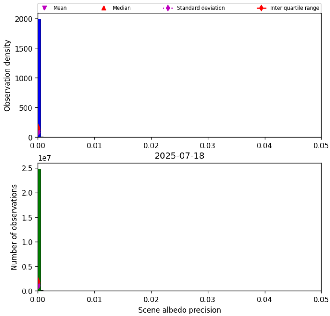
Figure 35: Histogram of “Scene albedo precision” for 2025-07-18 to 2025-07-19
