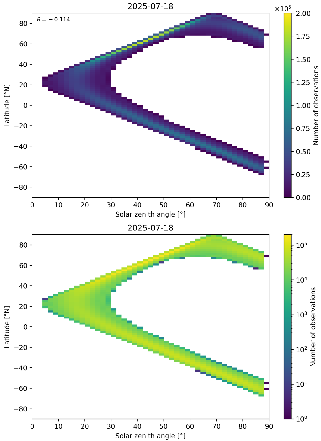
Figure 113: Scatter density plot of “Solar zenith angle” against “Latitude” for 2025-07-18 to 2025-07-19.
