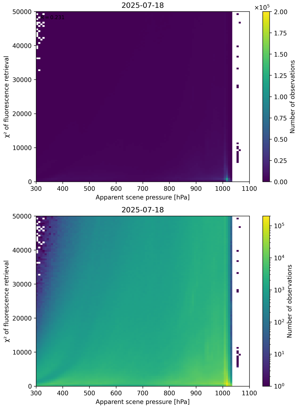
Figure 63: Scatter density plot of “Apparent scene pressure” against “ \chi^2 of fluorescence retrieval” for 2025-07-18 to 2025-07-19.
