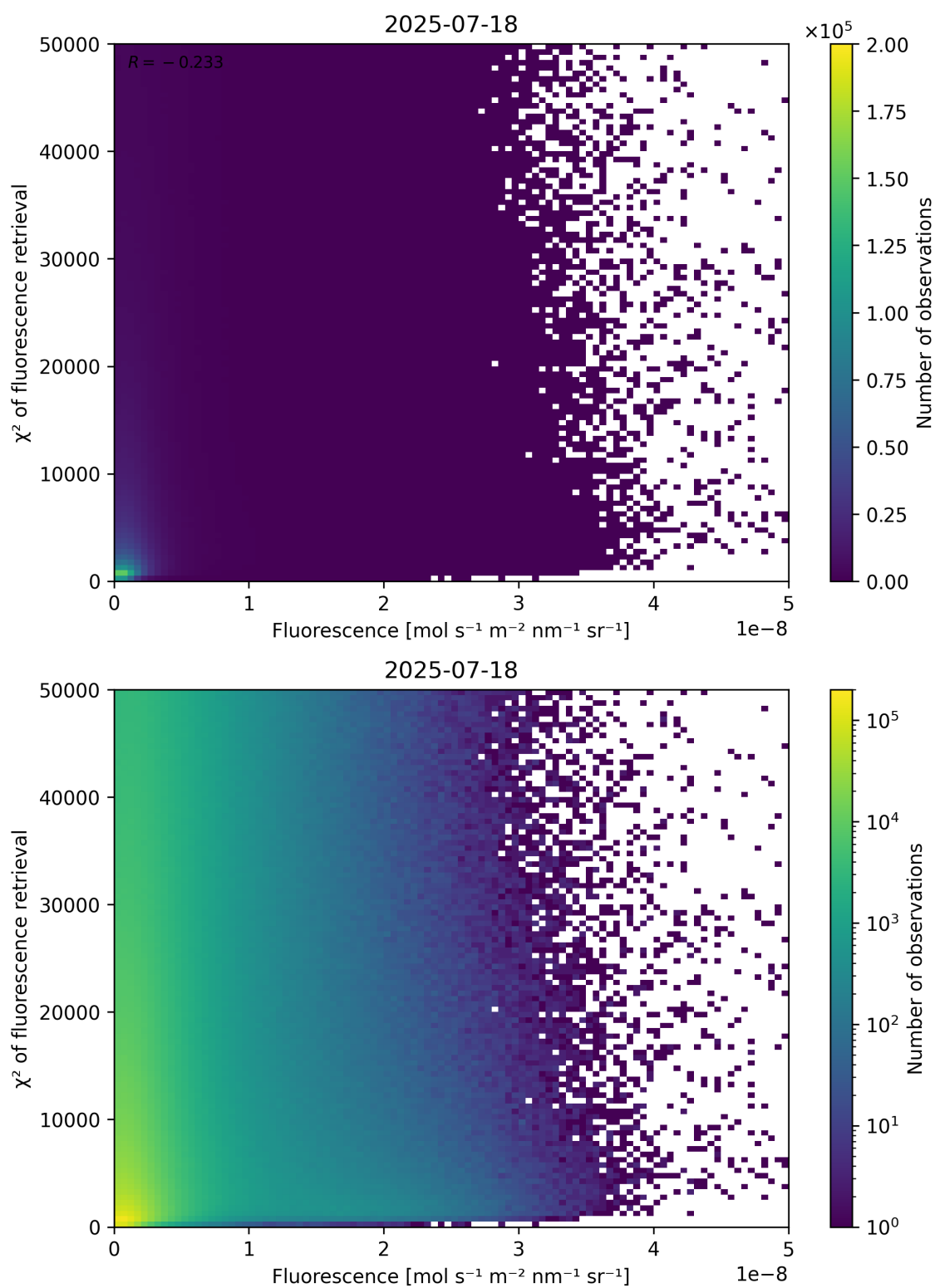
Figure 85: Scatter density plot of “Fluorescence” against “ \chi^2 of fluorescence retrieval” for 2025-07-18 to 2025-07-19.
