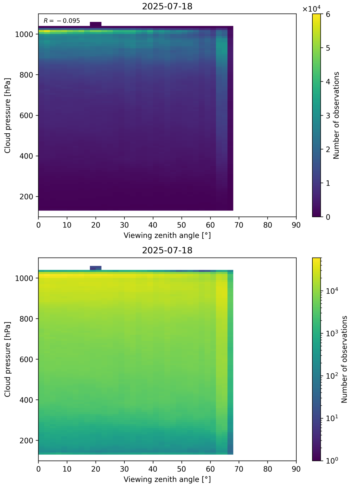
Figure 121: Scatter density plot of “Viewing zenith angle” against “Cloud pressure” for 2025-07-18 to 2025-07-19.
