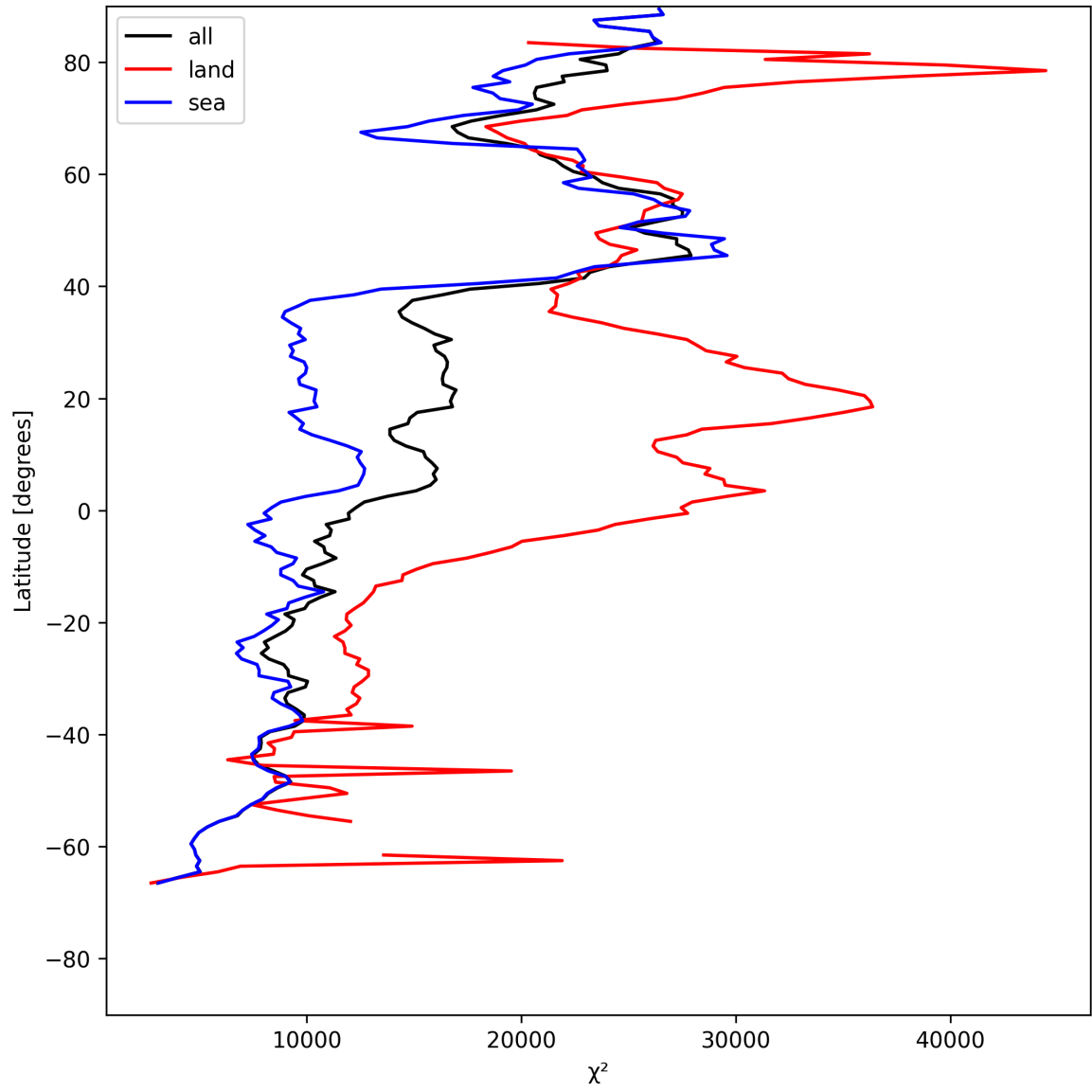
Figure 21: Zonal average of “ \chi^2 ” for 2025-07-18 to 2025-07-19.
