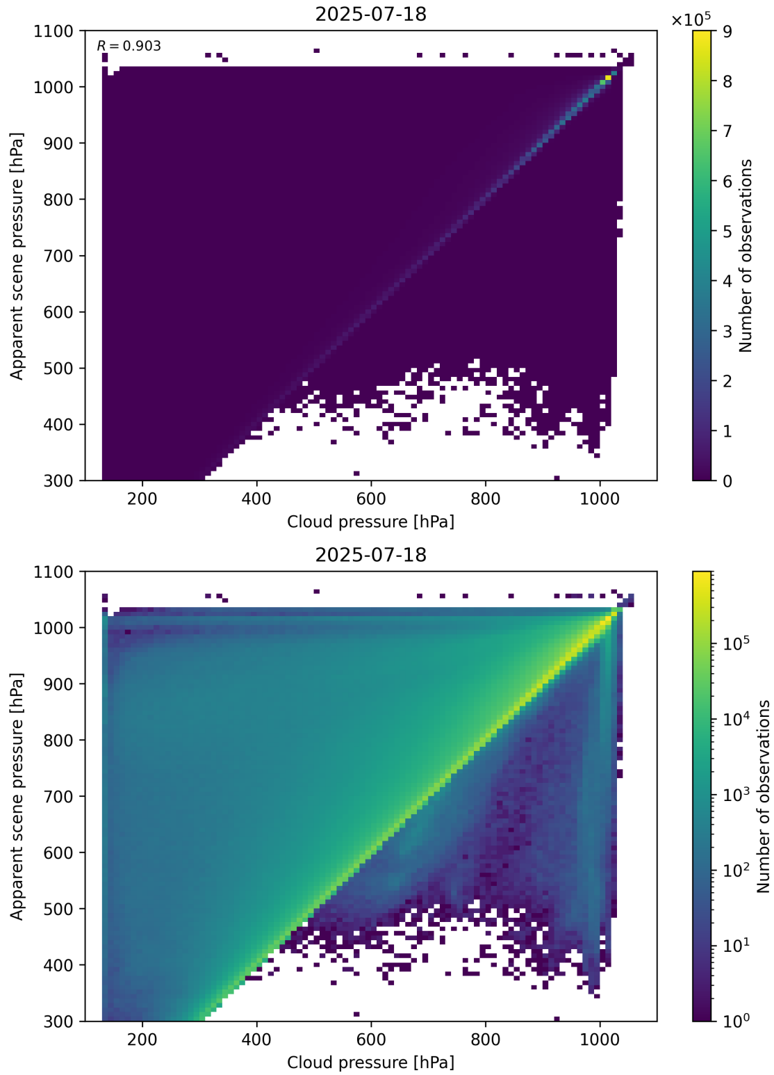
Figure 77: Scatter density plot of “Cloud pressure” against “Apparent scene pressure” for 2025-07-18 to 2025-07-19.
