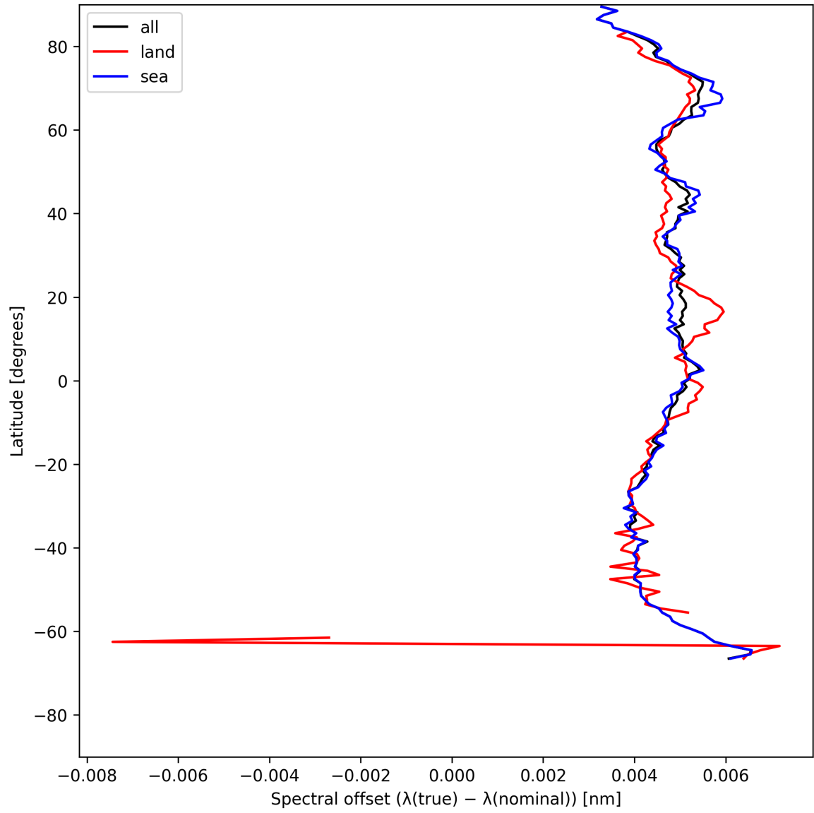
Figure 28: Zonal average of “Spectral offset ( \lambda_{\text{true}} - \lambda_{\text{nominal}} )” for 2025-07-18 to 2025-07-19.
