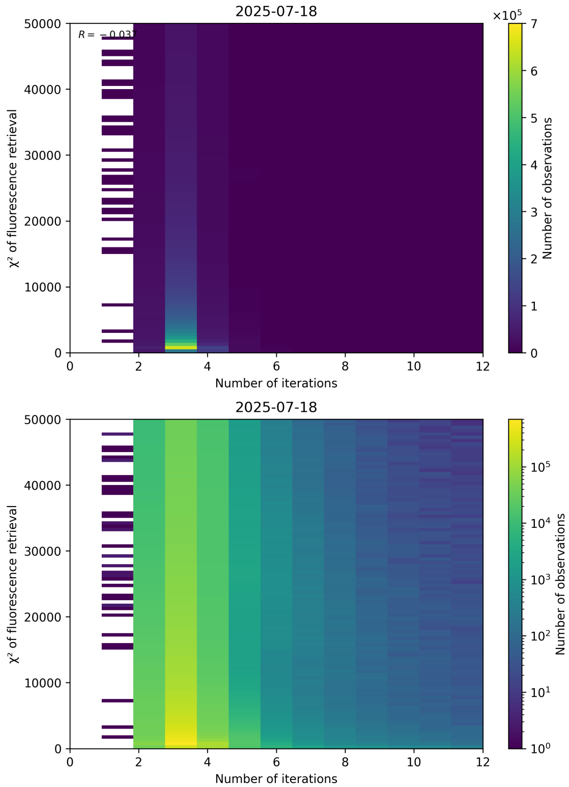
Figure 97: Scatter density plot of “Number of iterations” against “ \chi^2 of fluorescence retrieval” for 2025-07-18 to 2025-07-19.
