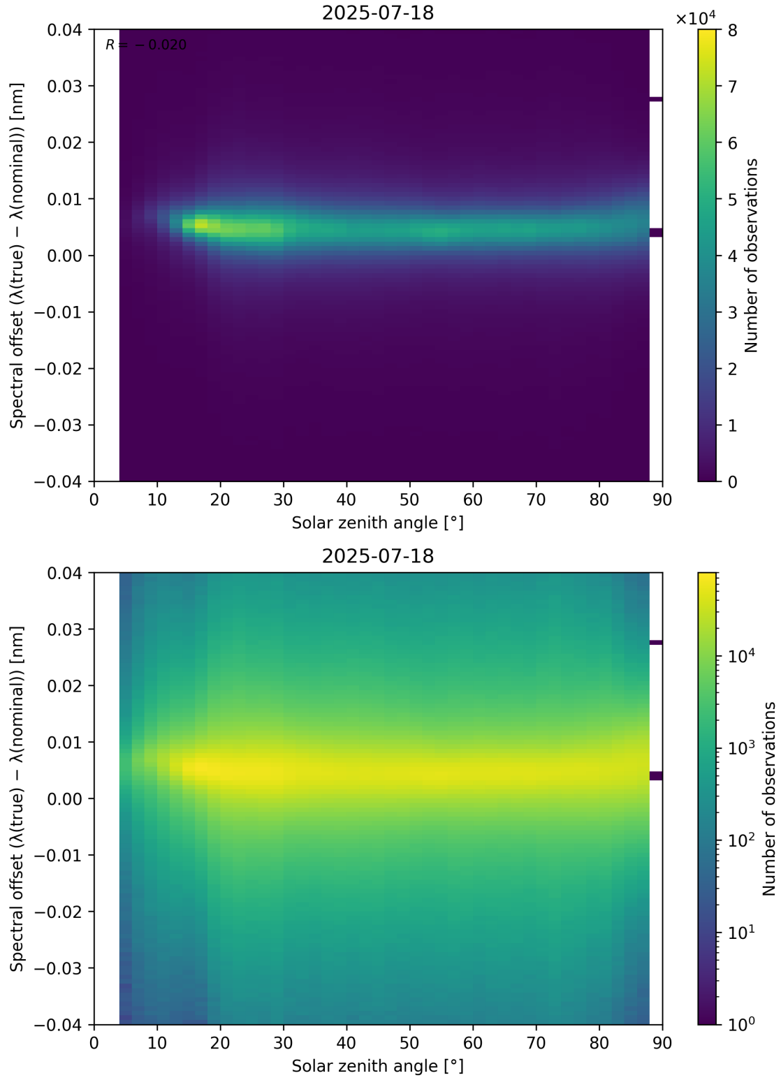
Figure 117: Scatter density plot of “Solar zenith angle” against “Spectral offset ( \lambda_{\text{true}} - \lambda_{\text{nominal}} )” for 2025-07-18 to 2025-07-19.
