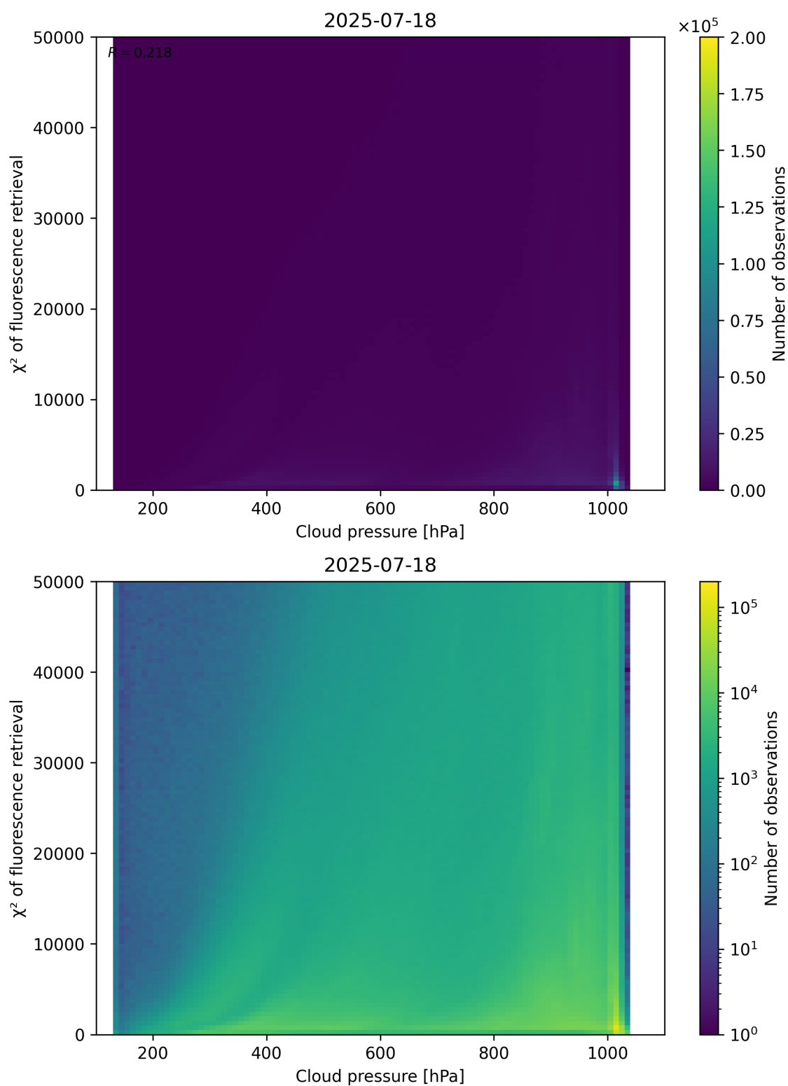
Figure 78: Scatter density plot of “Cloud pressure” against “ \chi^2 of fluorescence retrieval” for 2025-07-18 to 2025-07-19.
