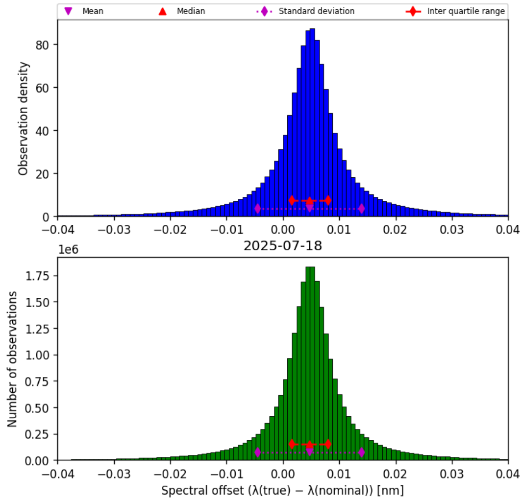
Figure 45: Histogram of “Spectral offset ( \lambda_{\text{true}} - \lambda_{\text{nominal}} )” for 2025-07-18 to 2025-07-19
