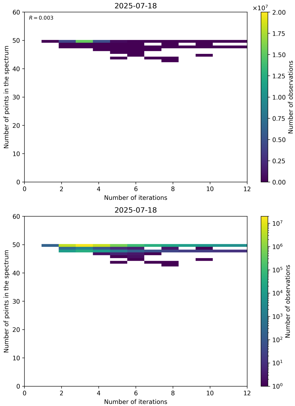
Figure 99: Scatter density plot of “Number of iterations” against “Number of points in the spectrum” for 2025-07-18 to 2025-07-19.
