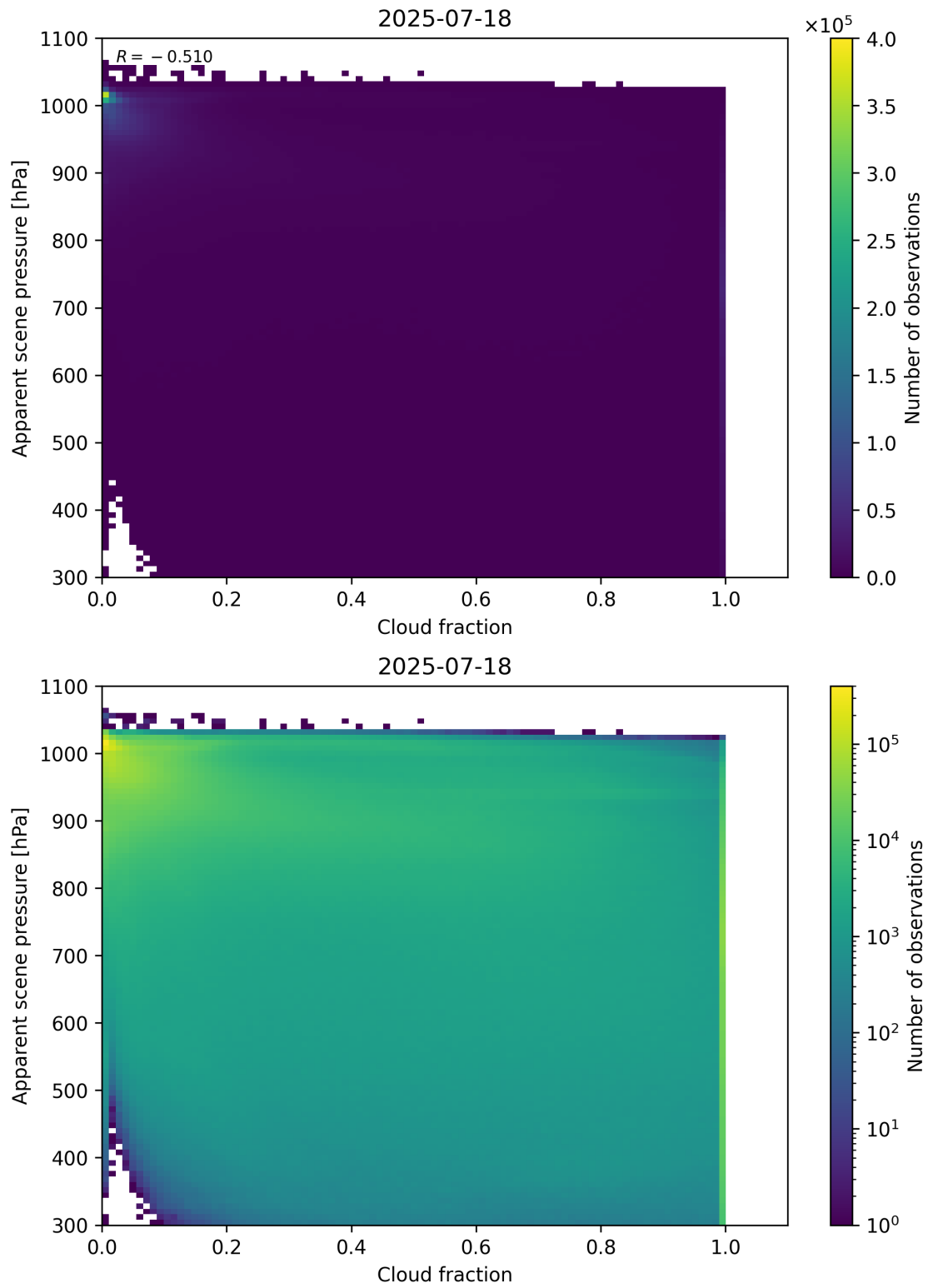
Figure 70: Scatter density plot of “Cloud fraction” against “Apparent scene pressure” for 2025-07-18 to 2025-07-19.
