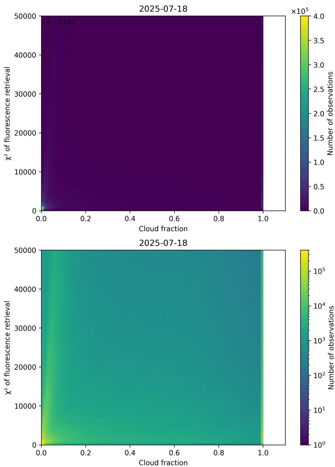
Figure 71: Scatter density plot of “Cloud fraction” against “ \chi^2 of fluorescence retrieval” for 2025-07-18 to 2025-07-19.
