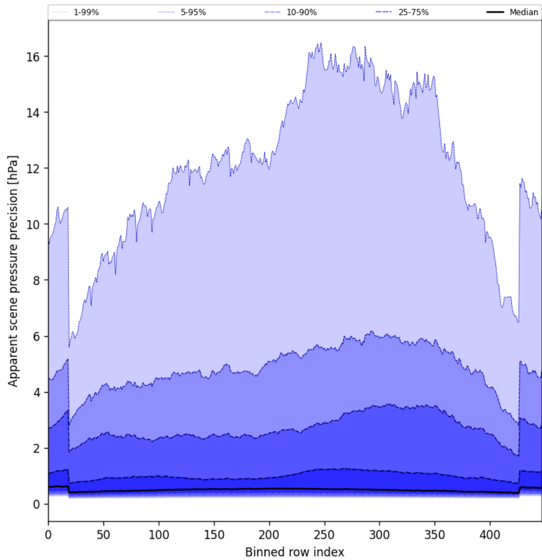
Figure 54: Along track statistics of “Apparent scene pressure precision” for 2025-07-18 to 2025-07-19
