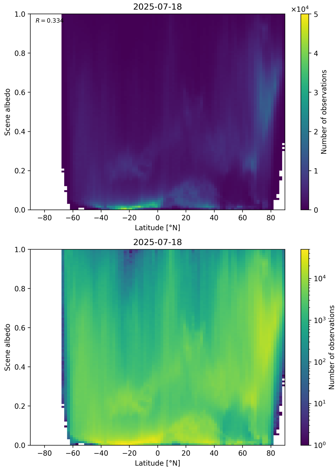
Figure 95: Scatter density plot of “Latitude” against “Scene albedo” for 2025-07-18 to 2025-07-19.
