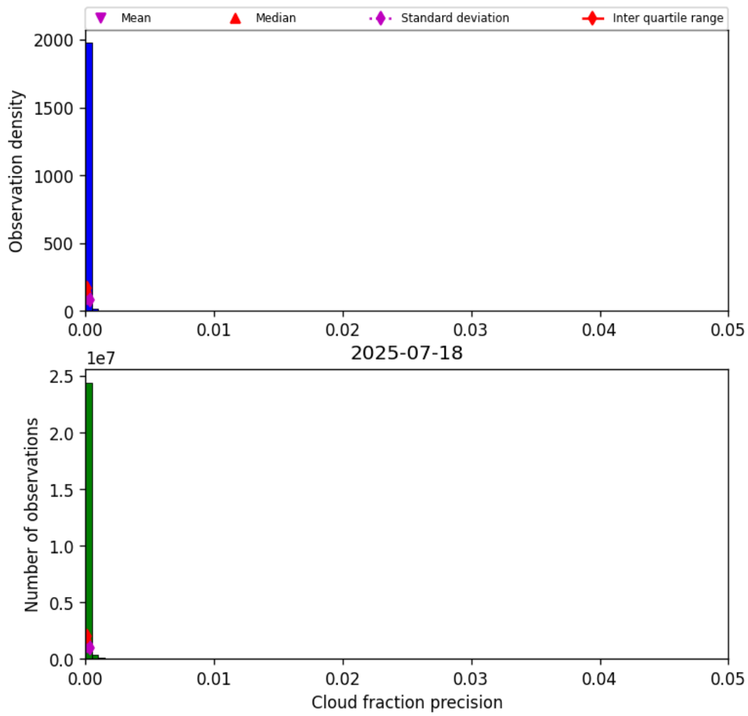
Figure 33: Histogram of “Cloud fraction precision” for 2025-07-18 to 2025-07-19
