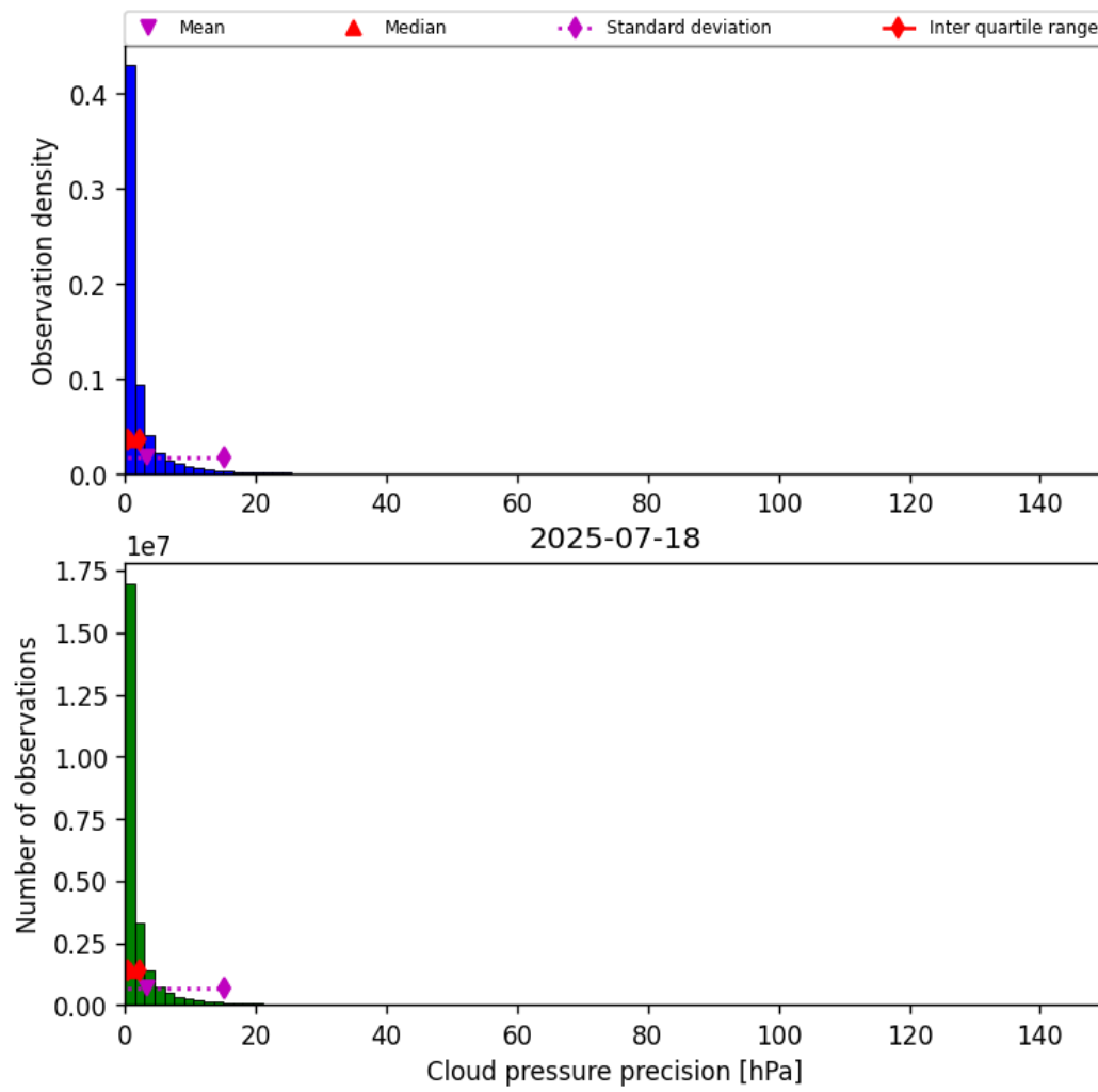
Figure 31: Histogram of “Cloud pressure precision” for 2025-07-18 to 2025-07-19
