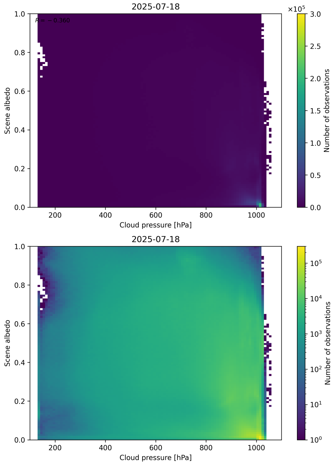
Figure 83: Scatter density plot of “Cloud pressure” against “Scene albedo” for 2025-07-18 to 2025-07-19.
