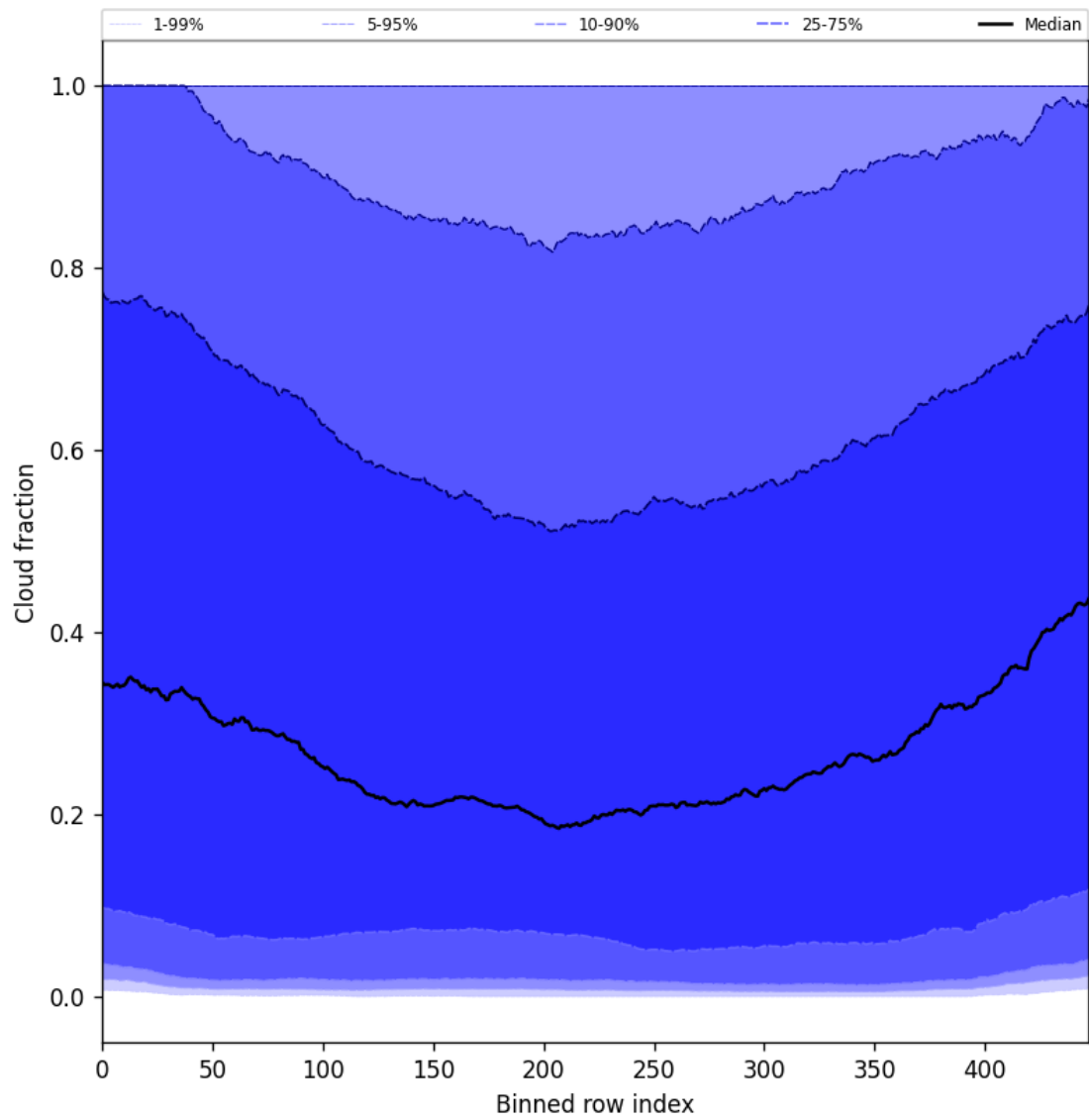
Figure 49: Along track statistics of “Cloud fraction” for 2025-07-18 to 2025-07-19
