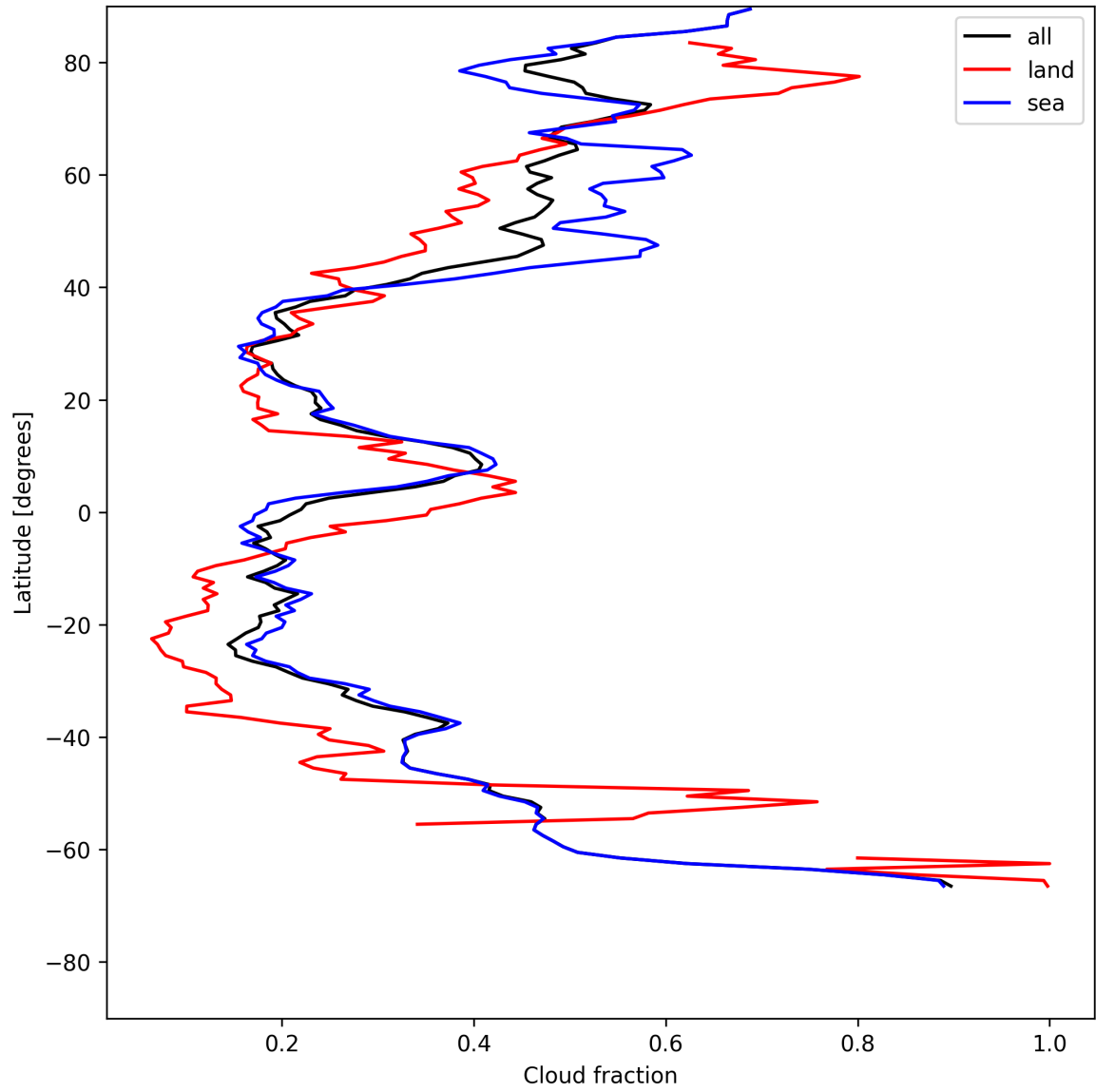
Figure 15: Zonal average of “Cloud fraction” for 2025-07-18 to 2025-07-19.
