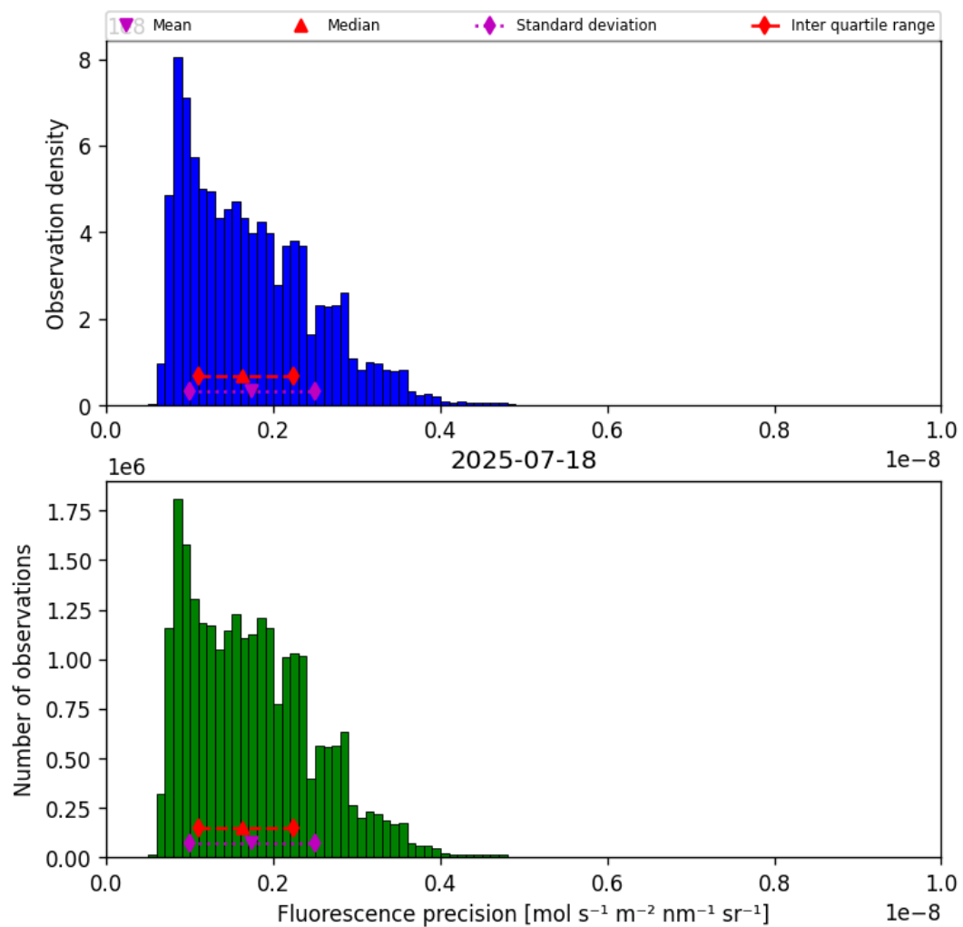
Figure 41: Histogram of “Fluorescence precision” for 2025-07-18 to 2025-07-19
