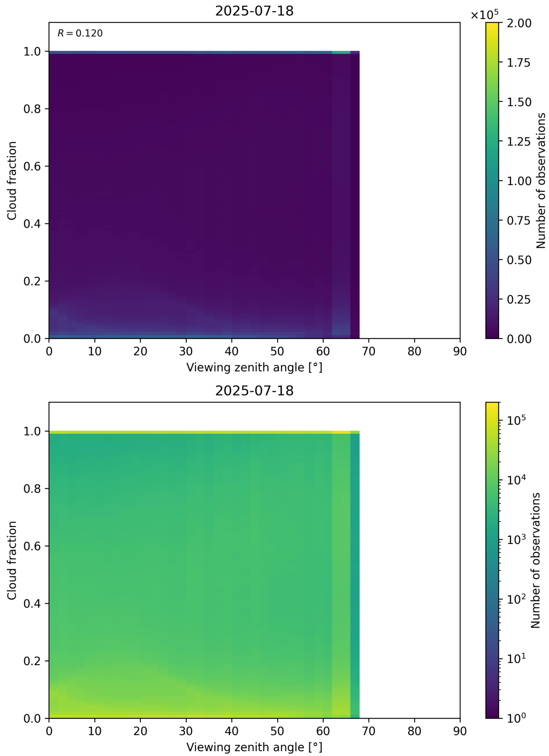
Figure 120: Scatter density plot of “Viewing zenith angle” against “Cloud fraction” for 2025-07-18 to 2025-07-19.
