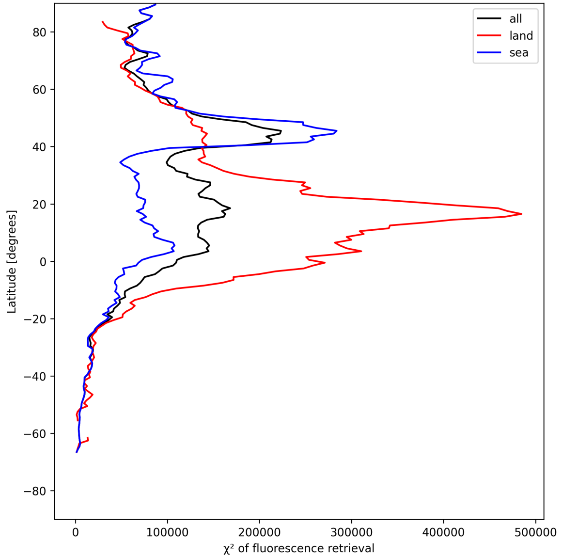
Figure 25: Zonal average of “ \chi^2 of fluorescence retrieval” for 2025-07-18 to 2025-07-19.
