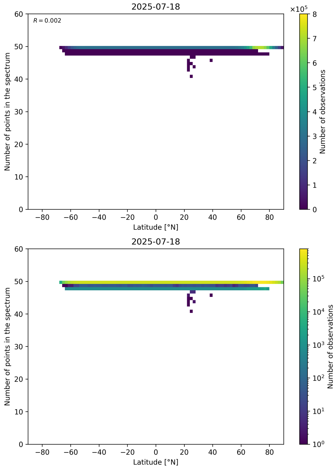
Figure 94: Scatter density plot of “Latitude” against “Number of points in the spectrum” for 2025-07-18 to 2025-07-19.
