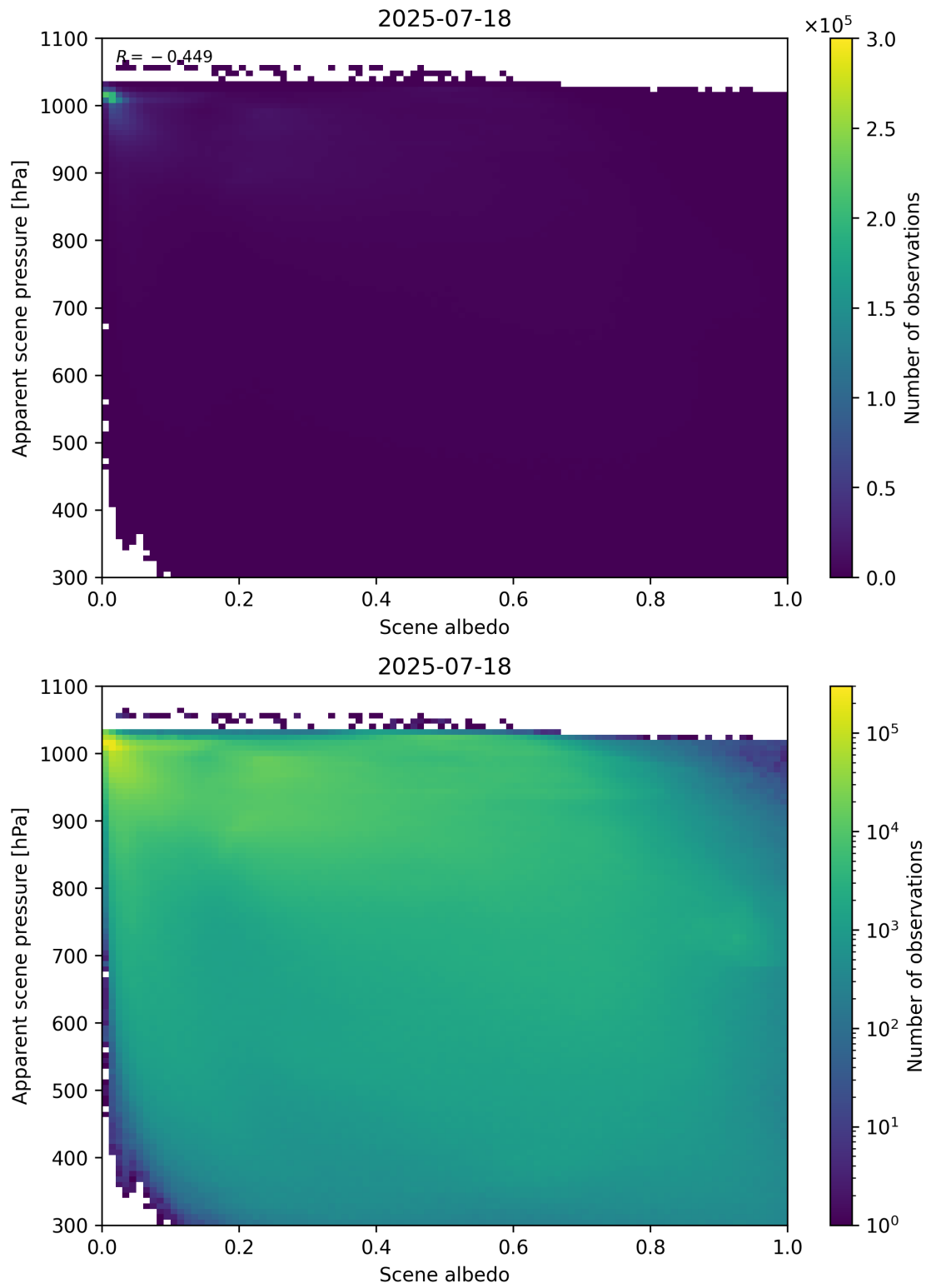
Figure 102: Scatter density plot of “Scene albedo” against “Apparent scene pressure” for 2025-07-18 to 2025-07-19.
