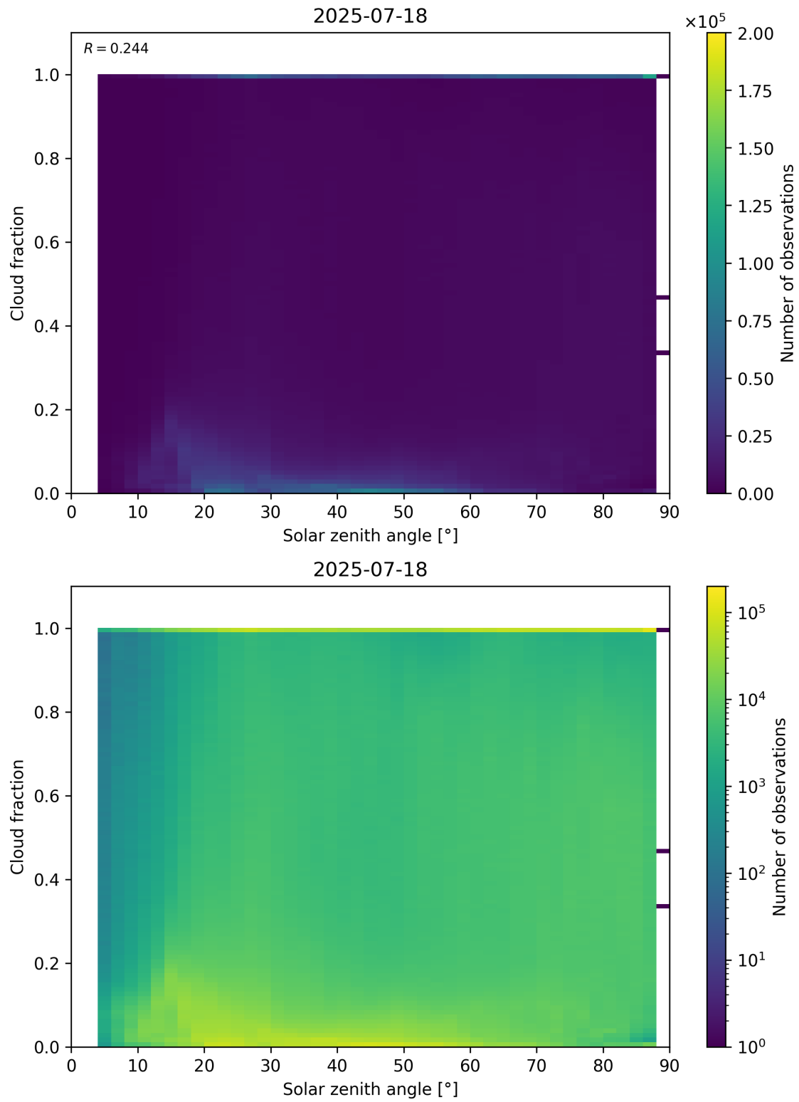
Figure 110: Scatter density plot of “Solar zenith angle” against “Cloud fraction” for 2025-07-18 to 2025-07-19.
