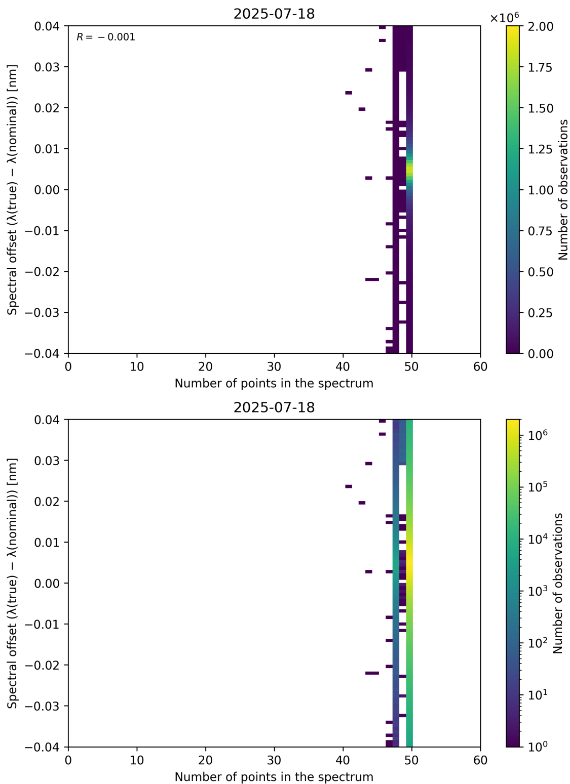
Figure 101: Scatter density plot of “Number of points in the spectrum” against “Spectral offset ( \lambda_{\text{true}} - \lambda_{\text{nominal}} )” for 2025-07-18 to 2025-07-19.
