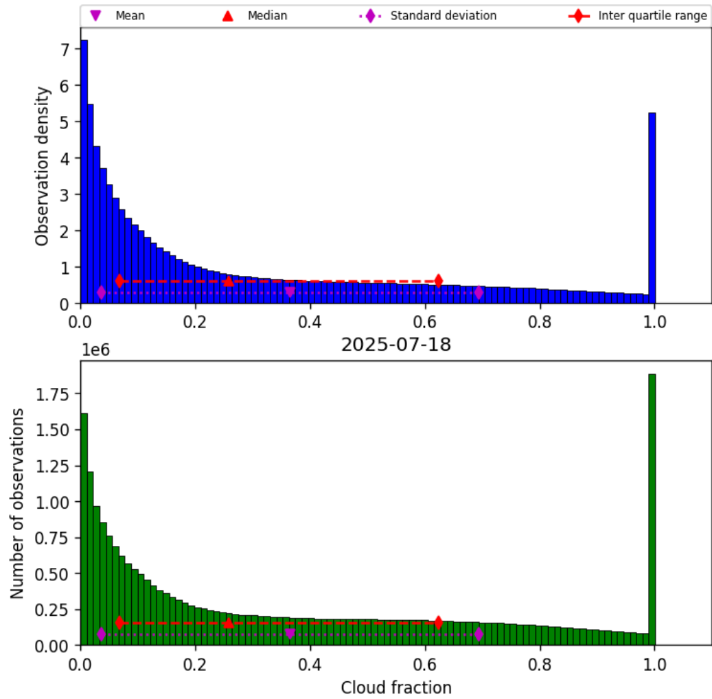
Figure 32: Histogram of “Cloud fraction” for 2025-07-18 to 2025-07-19
