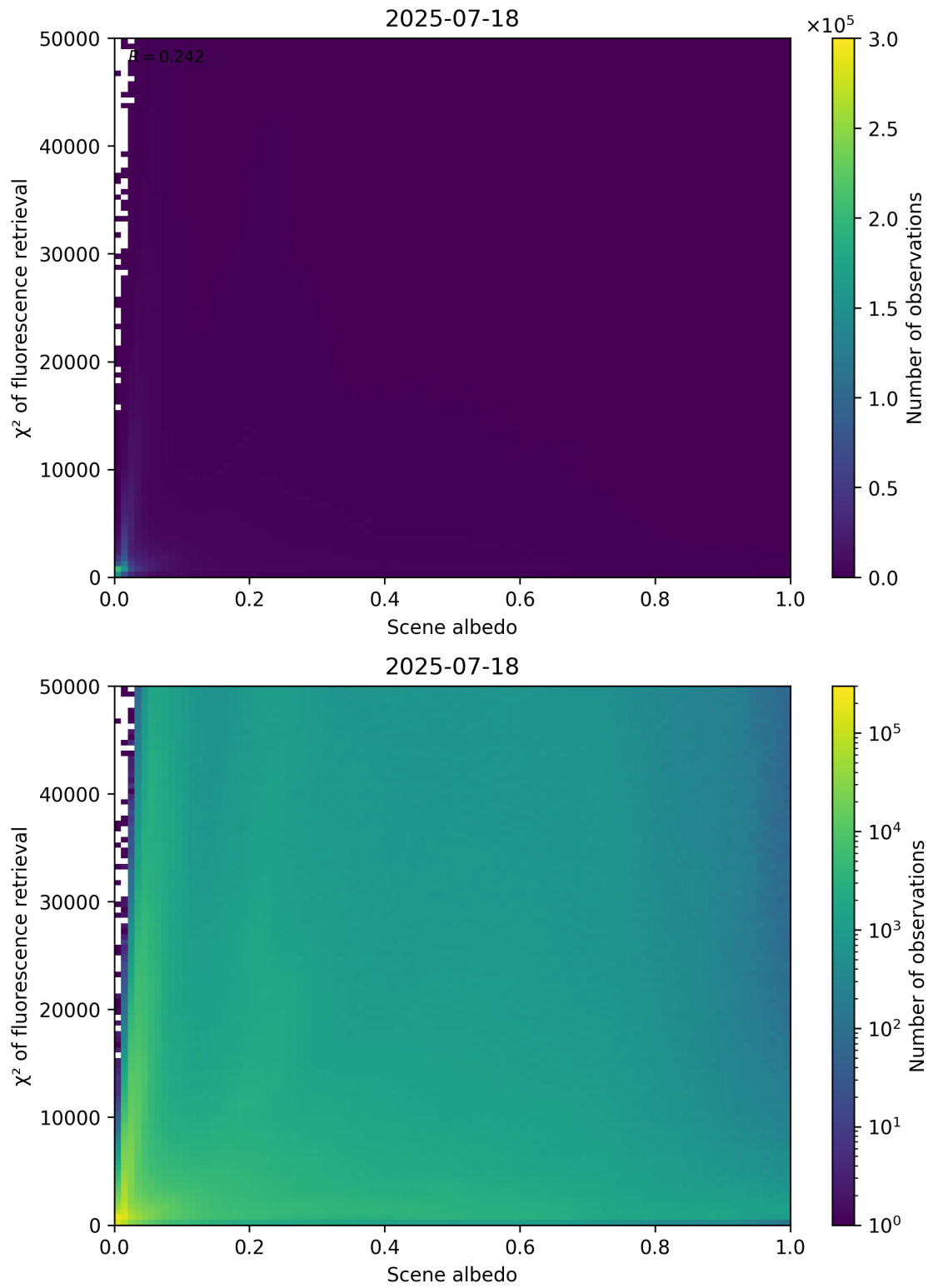
Figure 103: Scatter density plot of “Scene albedo” against “ \chi^2 of fluorescence retrieval” for 2025-07-18 to 2025-07-19.
