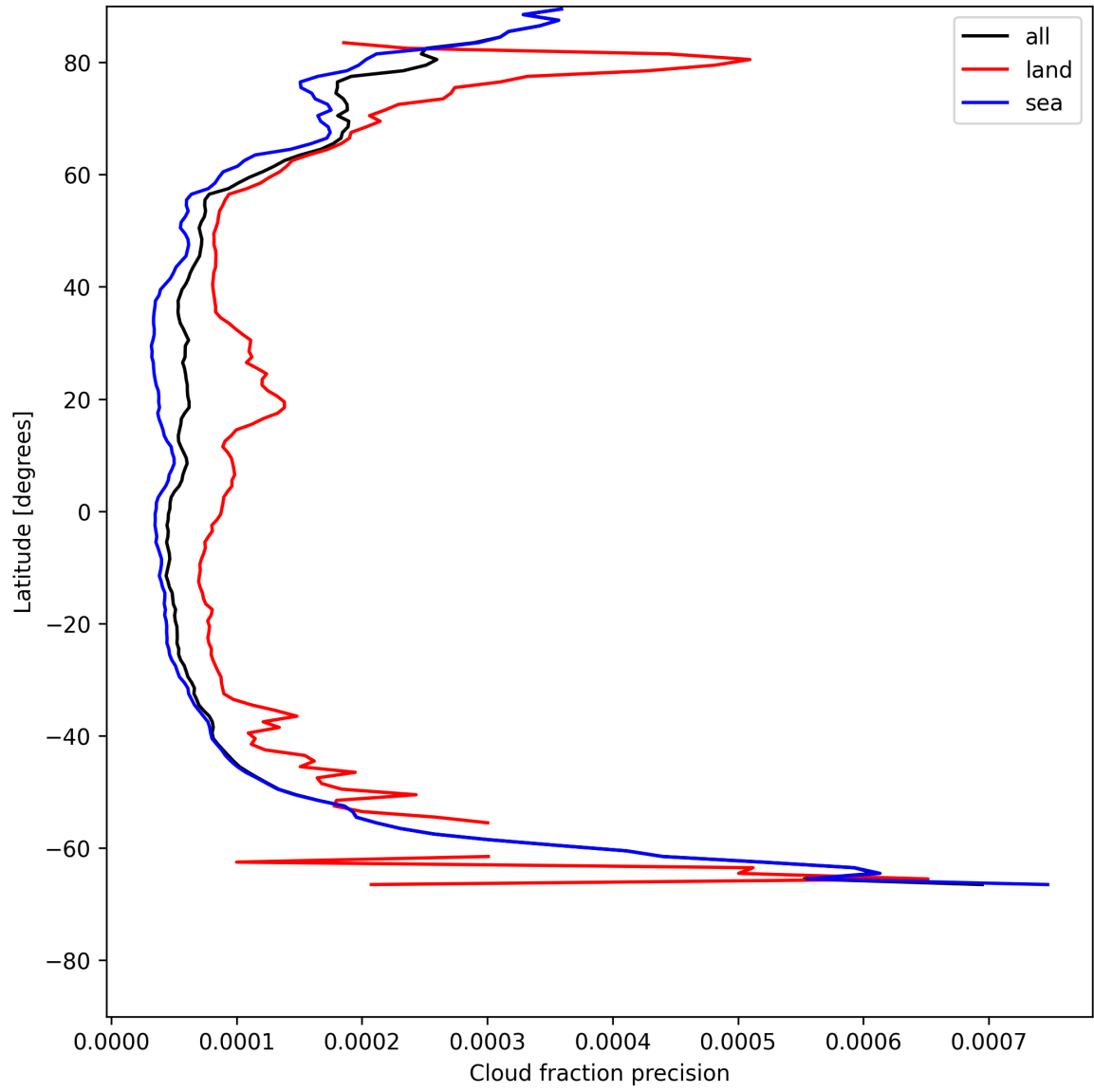
Figure 16: Zonal average of “Cloud fraction precision” for 2025-07-18 to 2025-07-19.
