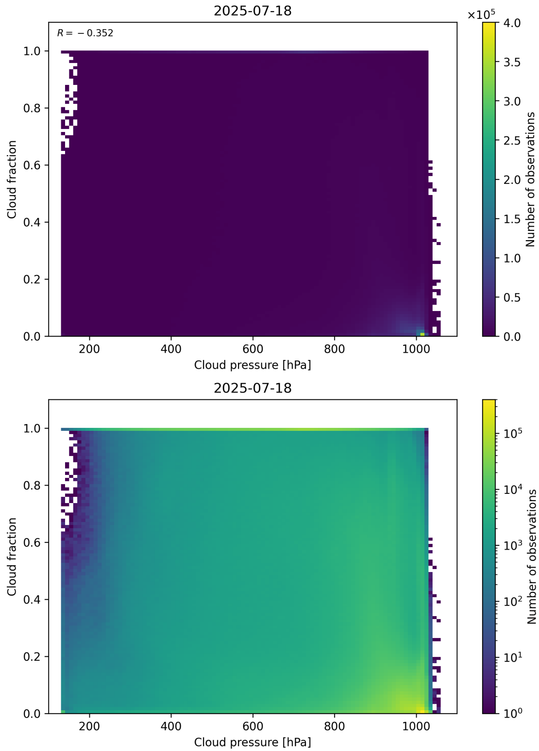
Figure 79: Scatter density plot of “Cloud pressure” against “Cloud fraction” for 2025-07-18 to 2025-07-19.
