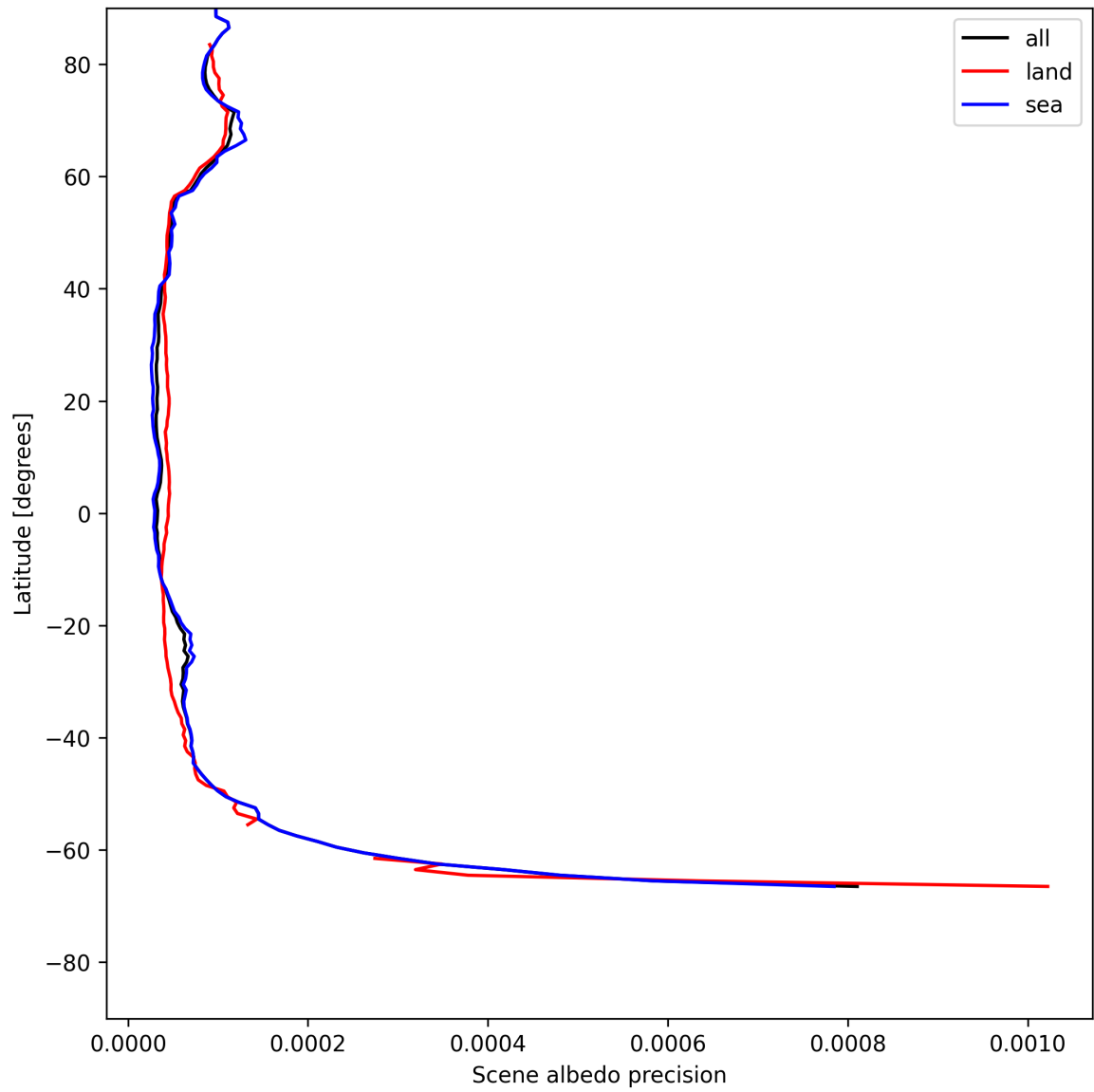
Figure 18: Zonal average of “Scene albedo precision” for 2025-07-18 to 2025-07-19.
