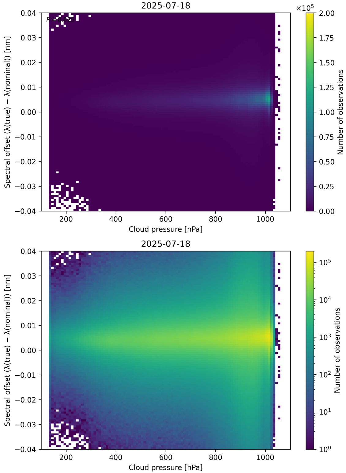
Figure 84: Scatter density plot of “Cloud pressure” against “Spectral offset ( \lambda_{\text{true}} - \lambda_{\text{nominal}} )” for 2025-07-18 to 2025-07-19.
