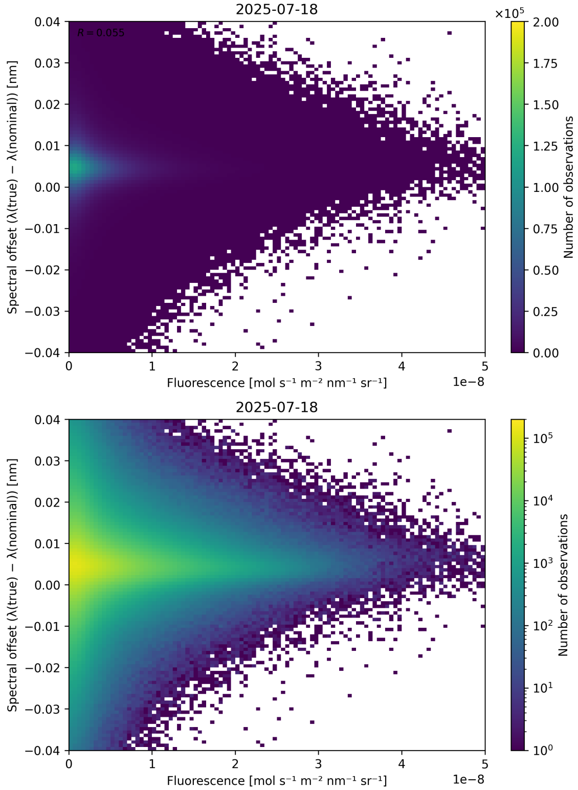
Figure 87: Scatter density plot of “Fluorescence” against “Spectral offset ( \lambda_{\text{true}} - \lambda_{\text{nominal}} )” for 2025-07-18 to 2025-07-19.
