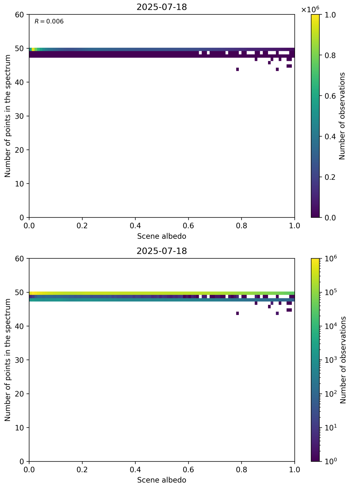
Figure 106: Scatter density plot of “Scene albedo” against “Number of points in the spectrum” for 2025-07-18 to 2025-07-19.
