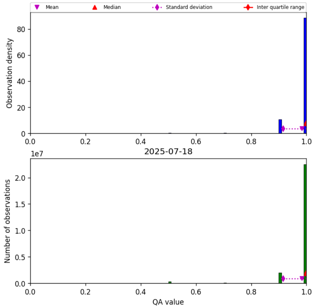
Figure 29: Histogram of “QA value” for 2025-07-18 to 2025-07-19
