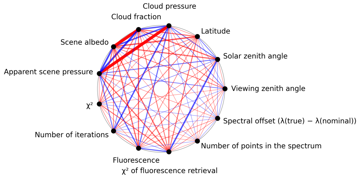
Figure 1: Map of correlation graph for 2025-07-18 to 2025-07-19.
