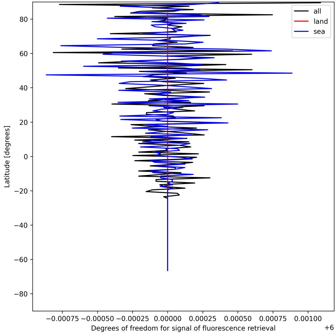
Figure 26: Zonal average of “Degrees of freedom for signal of fluorescence retrieval” for 2025-07-18 to 2025-07-19.
