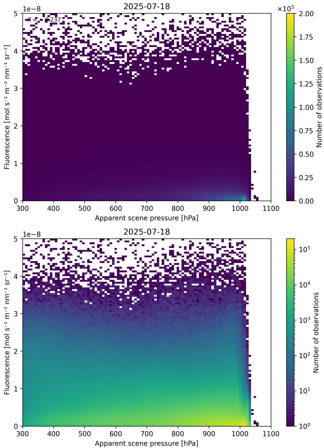
Figure 64: Scatter density plot of “Apparent scene pressure” against “Fluorescence” for 2025-07-18 to 2025-07-19.
