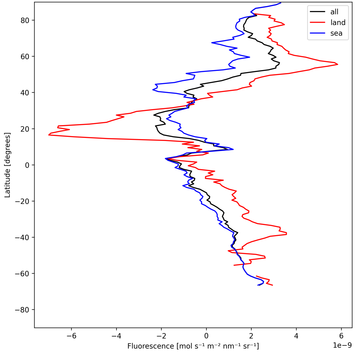
Figure 23: Zonal average of “Fluorescence” for 2025-07-18 to 2025-07-19.
