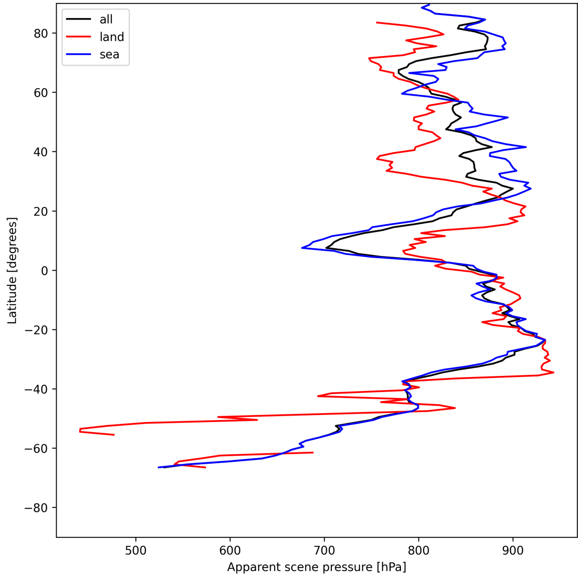
Figure 19: Zonal average of “Apparent scene pressure” for 2025-07-18 to 2025-07-19.
