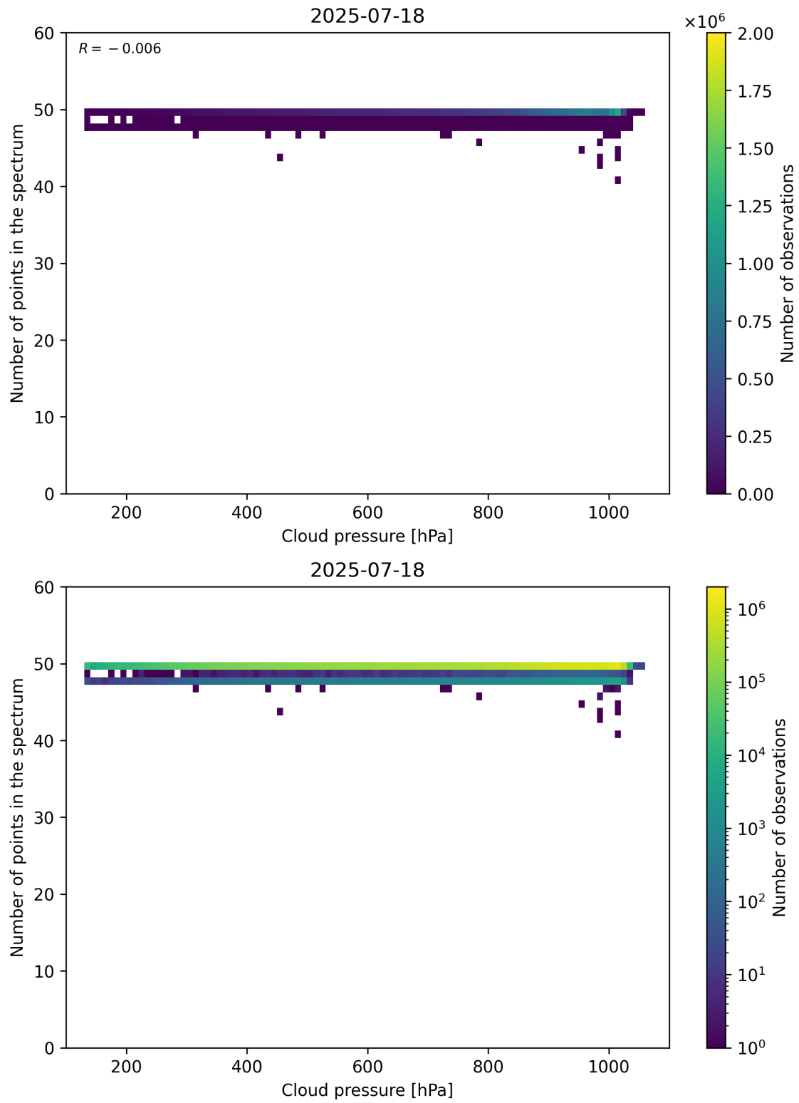
Figure 82: Scatter density plot of “Cloud pressure” against “Number of points in the spectrum” for 2025-07-18 to 2025-07-19.
