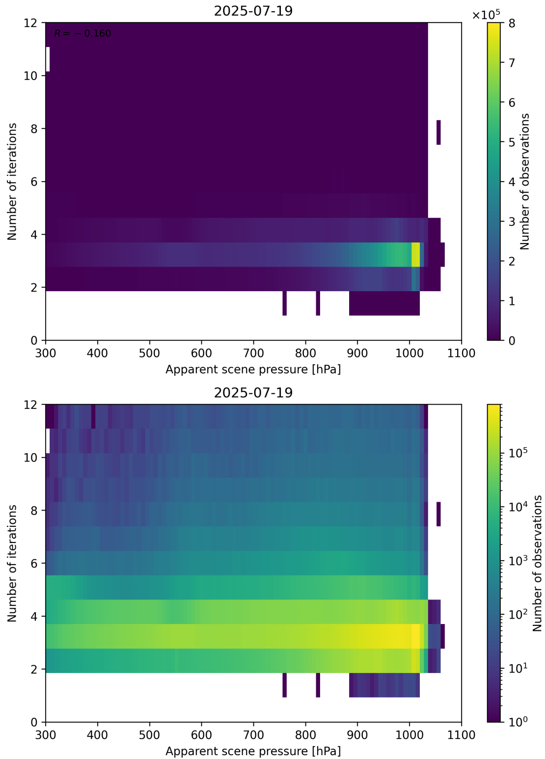
Figure 65: Scatter density plot of “Apparent scene pressure” against “Number of iterations” for 2025-07-19 to 2025-07-20.
