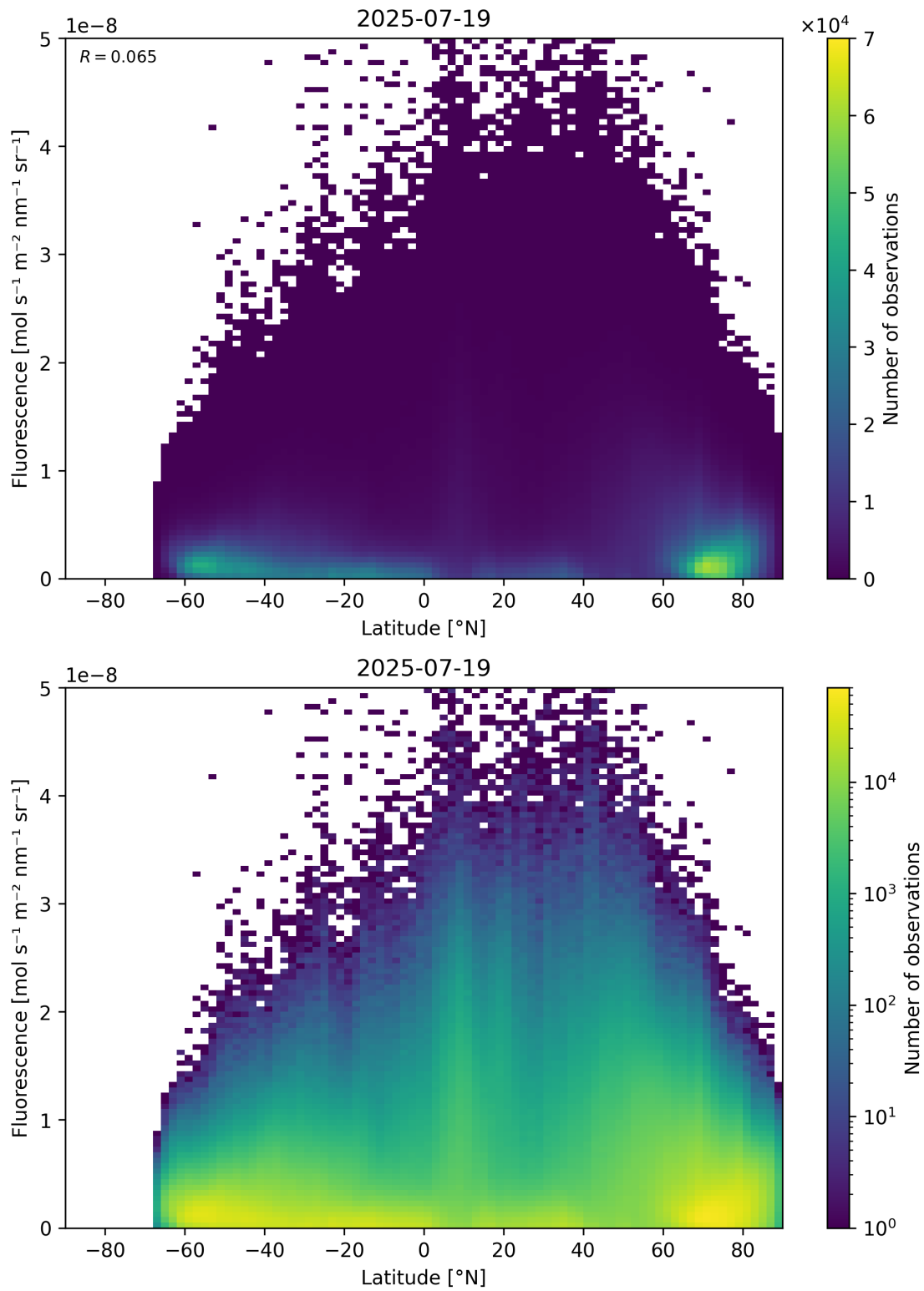
Figure 92: Scatter density plot of “Latitude” against “Fluorescence” for 2025-07-19 to 2025-07-20.
