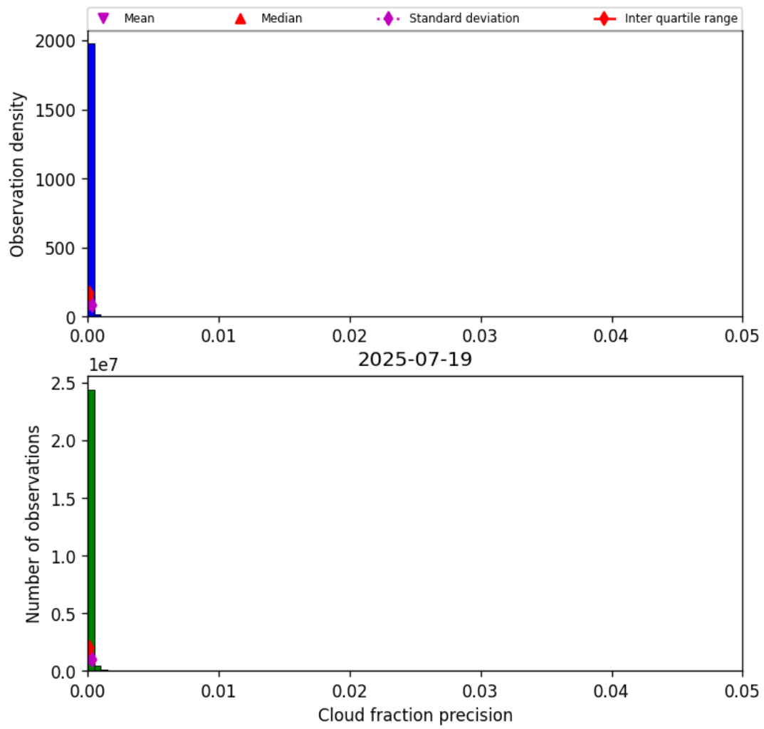
Figure 33: Histogram of “Cloud fraction precision” for 2025-07-19 to 2025-07-20
