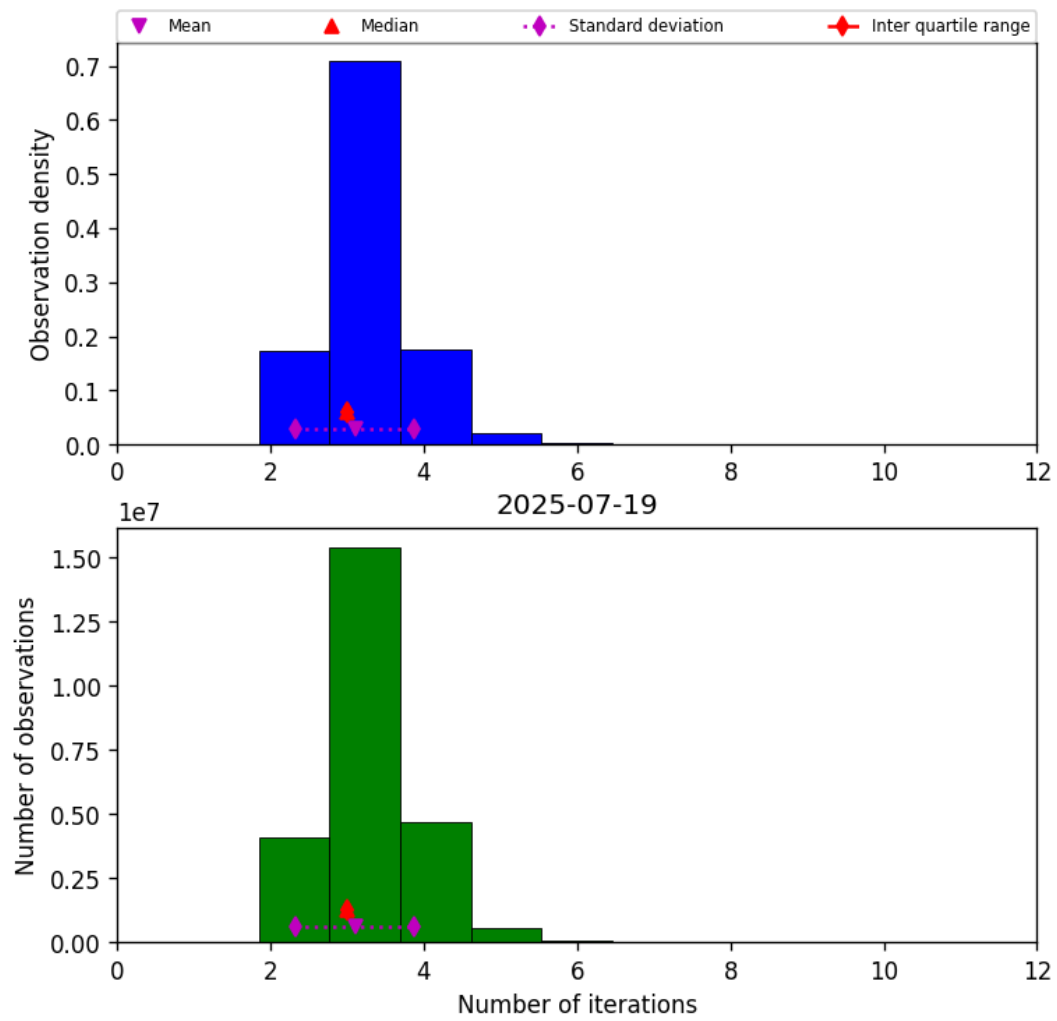
Figure 39: Histogram of “Number of iterations” for 2025-07-19 to 2025-07-20
