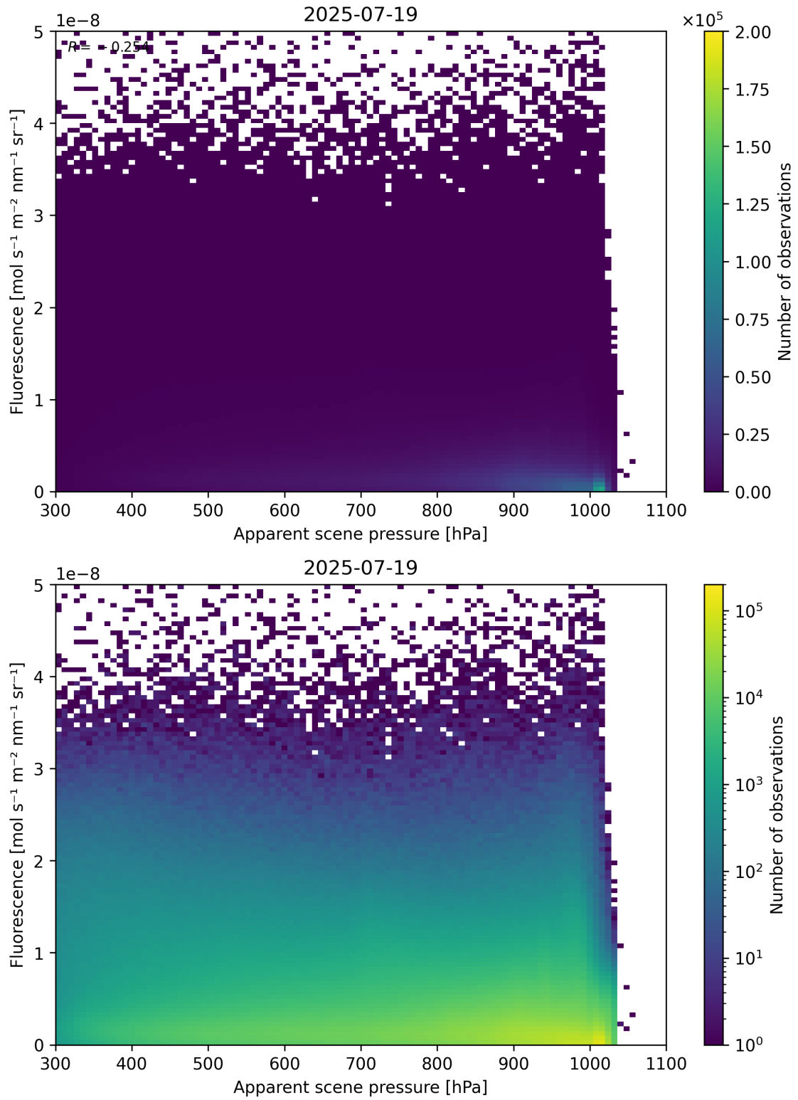
Figure 64: Scatter density plot of “Apparent scene pressure” against “Fluorescence” for 2025-07-19 to 2025-07-20.
