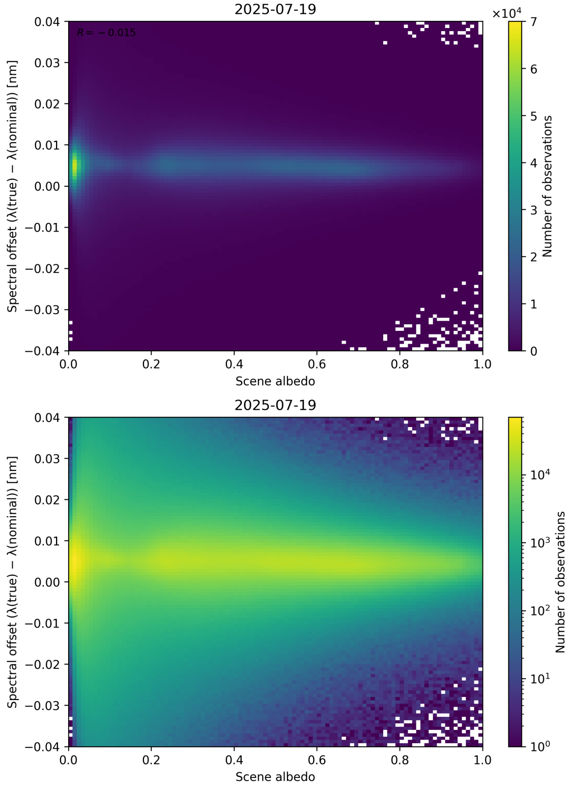
Figure 107: Scatter density plot of “Scene albedo” against “Spectral offset ( \lambda_{\text{true}} - \lambda_{\text{nominal}} )” for 2025-07-19 to 2025-07-20.
