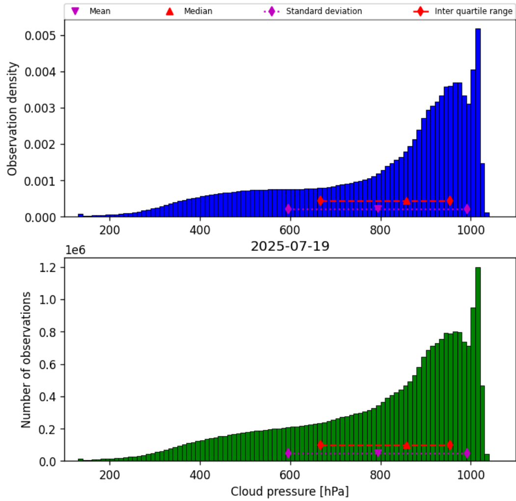
Figure 30: Histogram of “Cloud pressure” for 2025-07-19 to 2025-07-20
