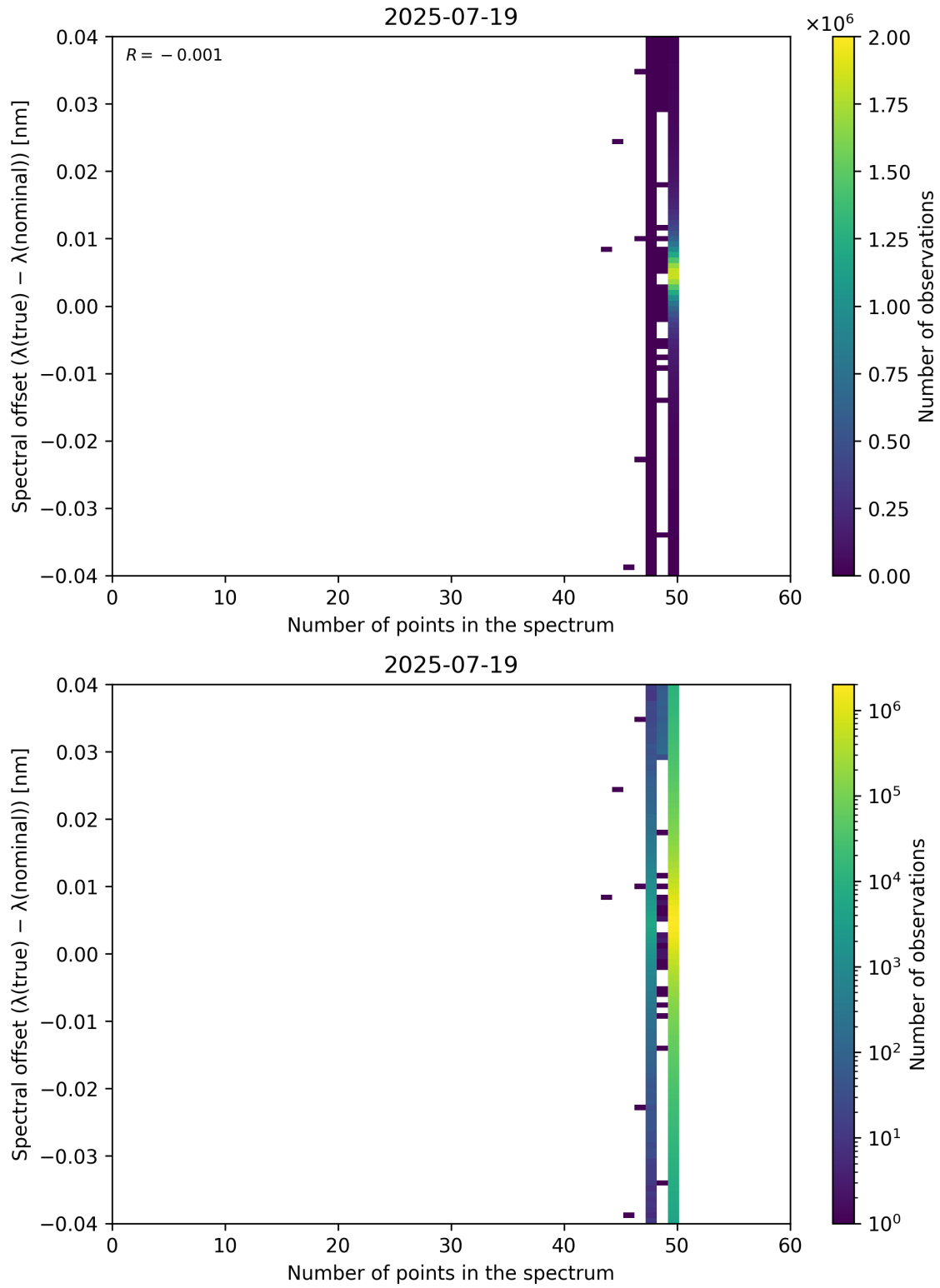
Figure 101: Scatter density plot of “Number of points in the spectrum” against “Spectral offset ( \lambda_{\text{true}} - \lambda_{\text{nominal}} )” for 2025-07-19 to 2025-07-20.
