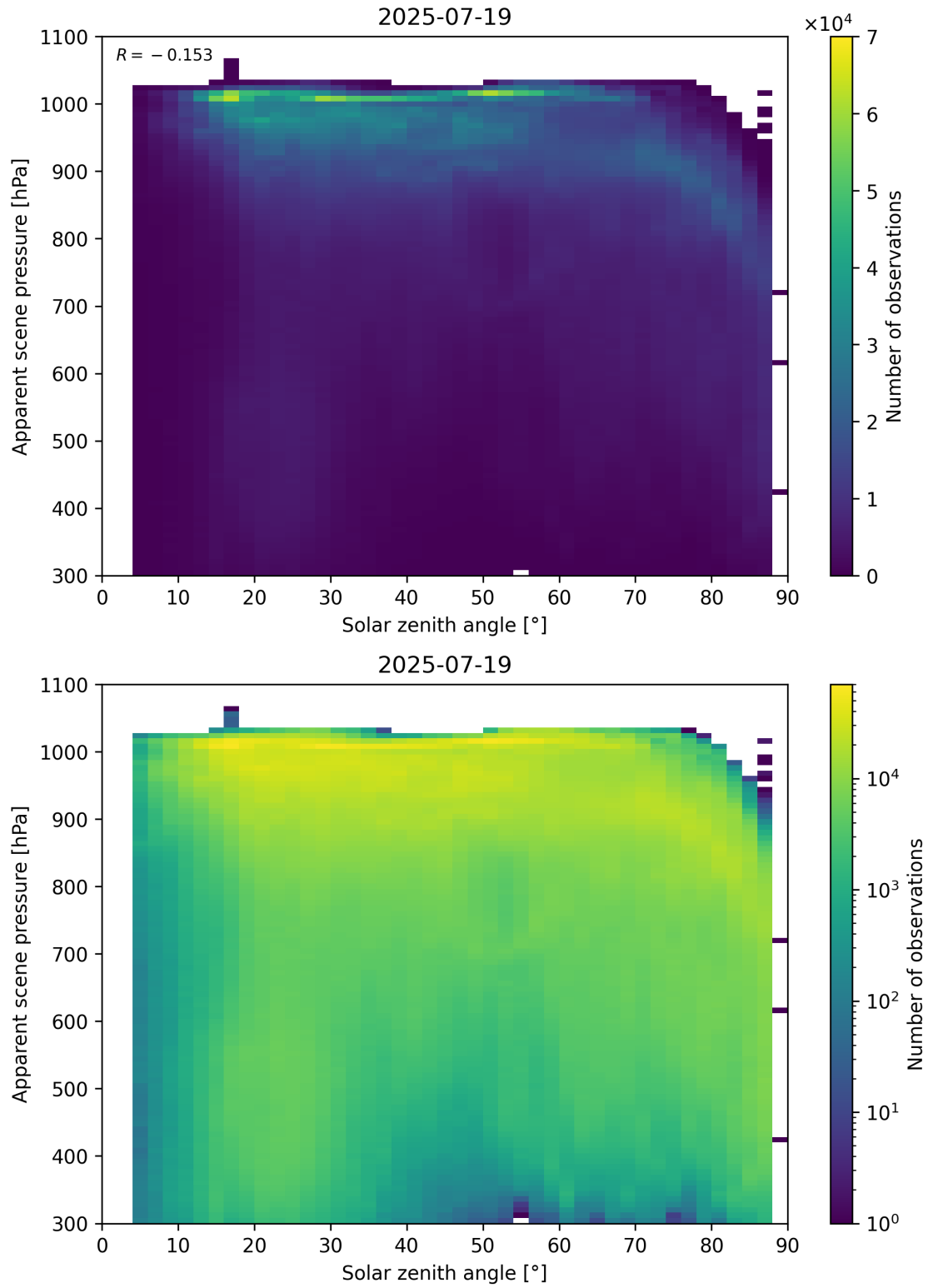
Figure 108: Scatter density plot of “Solar zenith angle” against “Apparent scene pressure” for 2025-07-19 to 2025-07-20.
