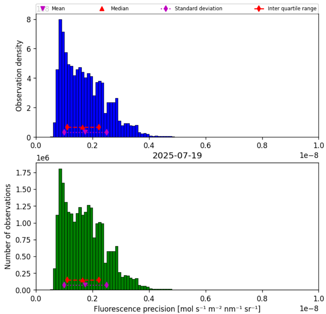
Figure 41: Histogram of “Fluorescence precision” for 2025-07-19 to 2025-07-20
