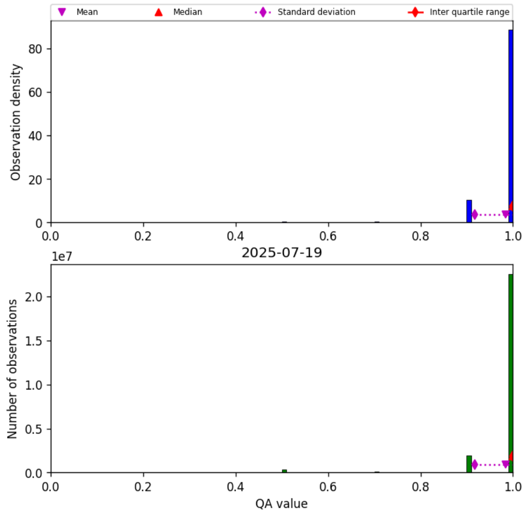
Figure 29: Histogram of “QA value” for 2025-07-19 to 2025-07-20
