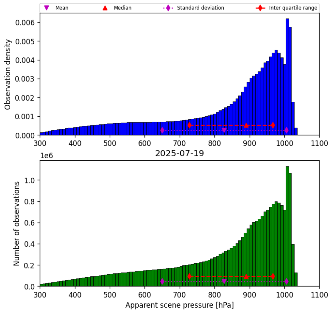
Figure 36: Histogram of “Apparent scene pressure” for 2025-07-19 to 2025-07-20
