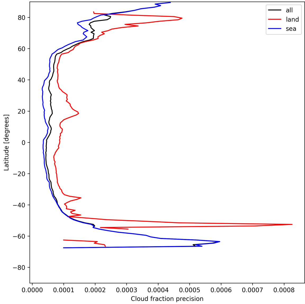
Figure 16: Zonal average of “Cloud fraction precision” for 2025-07-19 to 2025-07-20.
