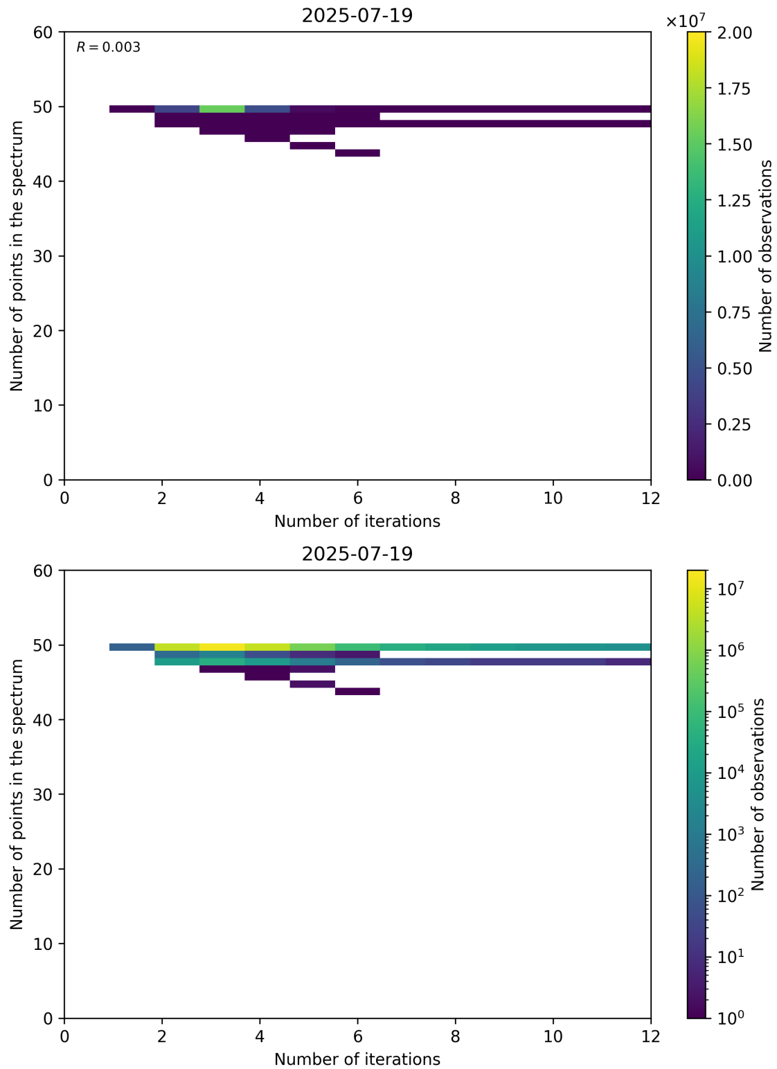
Figure 99: Scatter density plot of “Number of iterations” against “Number of points in the spectrum” for 2025-07-19 to 2025-07-20.
