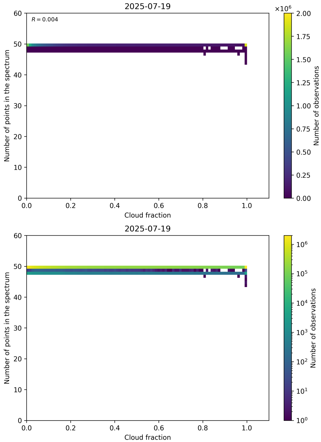
Figure 74: Scatter density plot of “Cloud fraction” against “Number of points in the spectrum” for 2025-07-19 to 2025-07-20.
