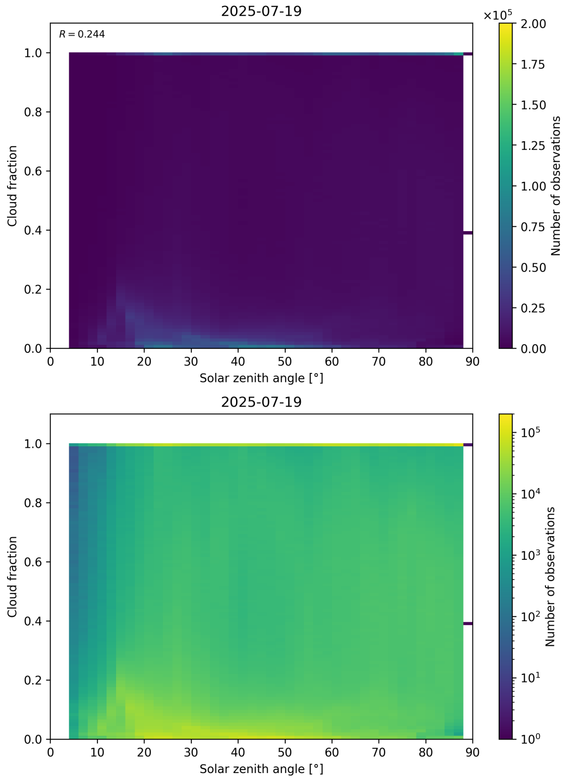
Figure 110: Scatter density plot of “Solar zenith angle” against “Cloud fraction” for 2025-07-19 to 2025-07-20.
