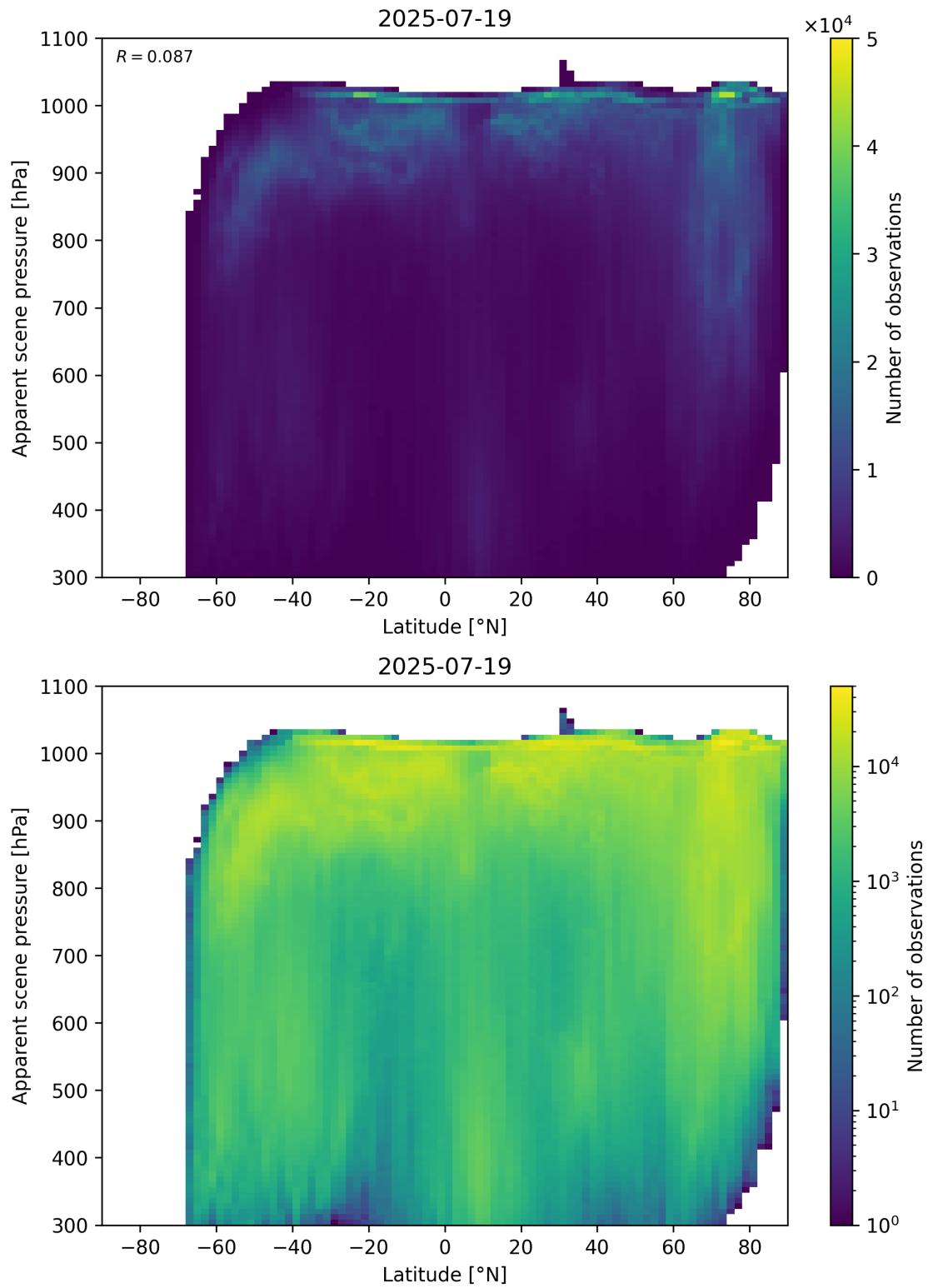
Figure 88: Scatter density plot of “Latitude” against “Apparent scene pressure” for 2025-07-19 to 2025-07-20.
