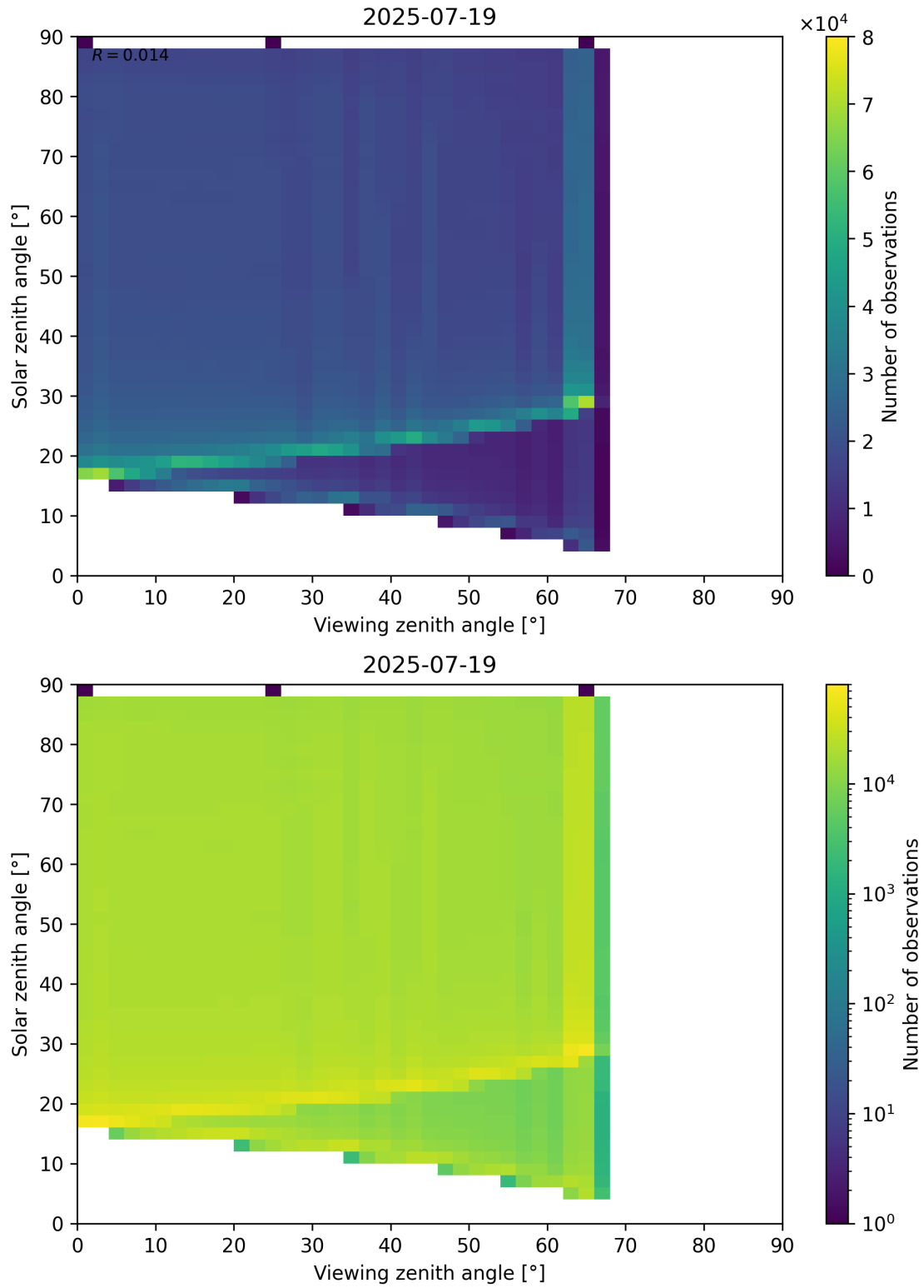
Figure 127: Scatter density plot of “Viewing zenith angle” against “Solar zenith angle” for 2025-07-19 to 2025-07-20.
