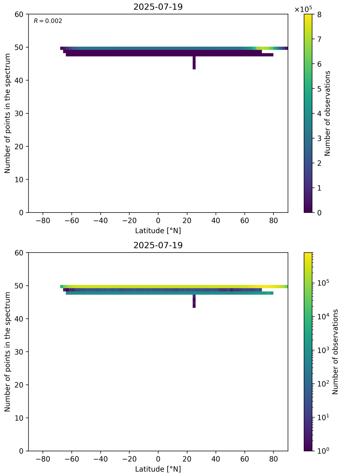
Figure 94: Scatter density plot of “Latitude” against “Number of points in the spectrum” for 2025-07-19 to 2025-07-20.
