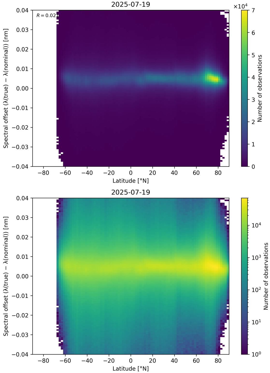
Figure 96: Scatter density plot of “Latitude” against “Spectral offset ( \lambda_{\text{true}} - \lambda_{\text{nominal}} )” for 2025-07-19 to 2025-07-20.
