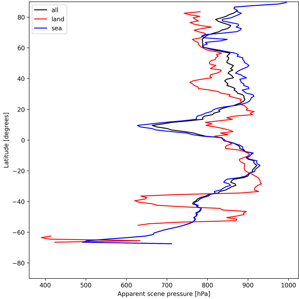
Figure 19: Zonal average of “Apparent scene pressure” for 2025-07-19 to 2025-07-20.
