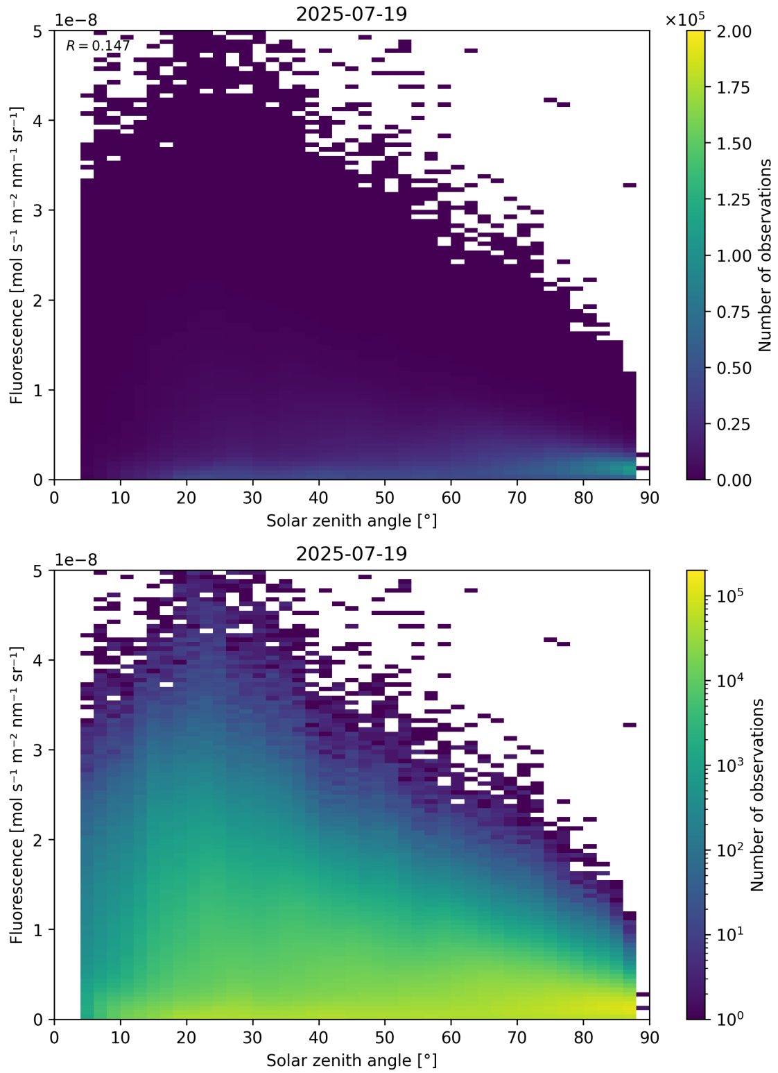
Figure 112: Scatter density plot of “Solar zenith angle” against “Fluorescence” for 2025-07-19 to 2025-07-20.
