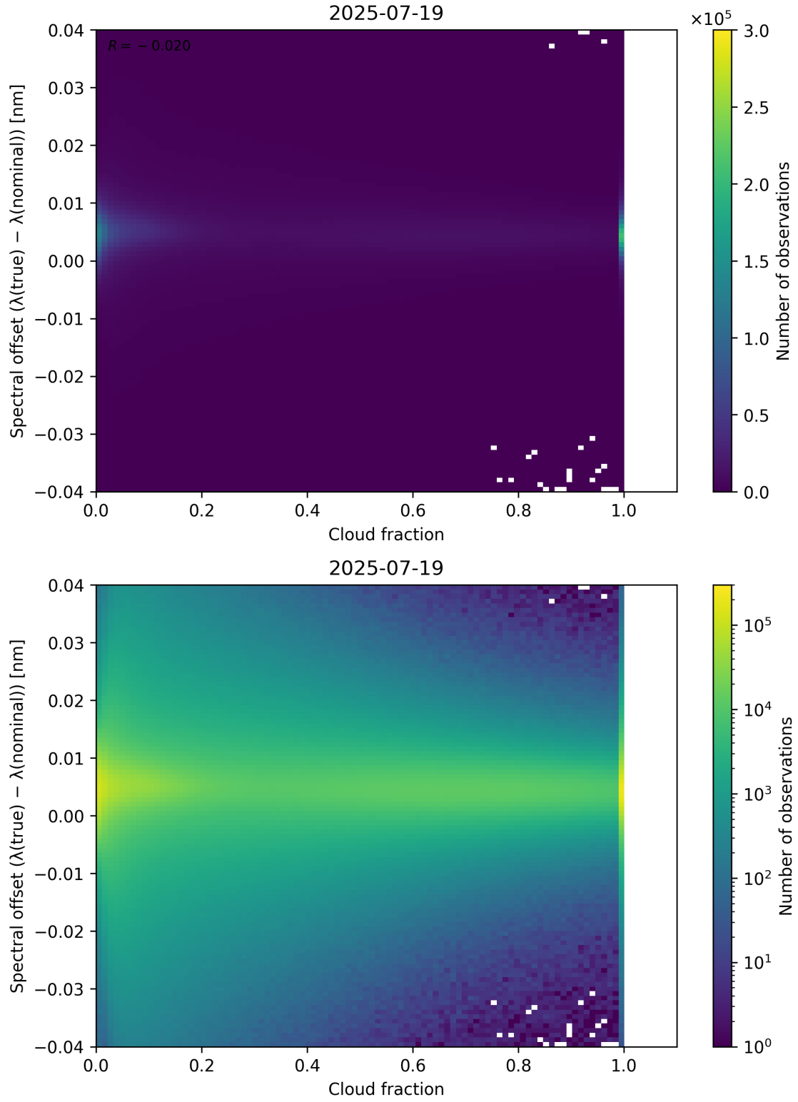
Figure 76: Scatter density plot of “Cloud fraction” against “Spectral offset ( \lambda_{\text{true}} - \lambda_{\text{nominal}} )” for 2025-07-19 to 2025-07-20.
