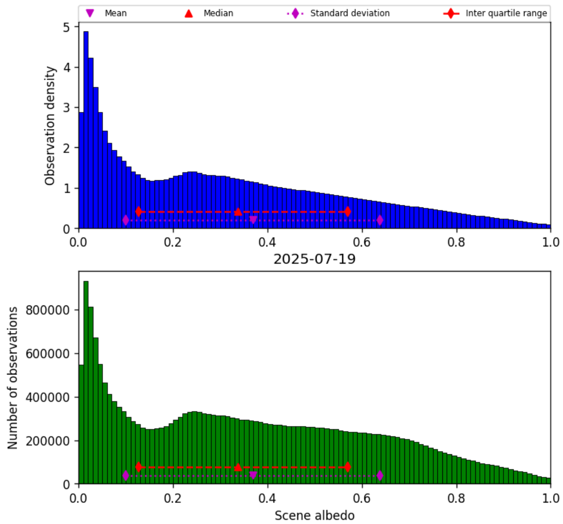
Figure 34: Histogram of “Scene albedo” for 2025-07-19 to 2025-07-20
