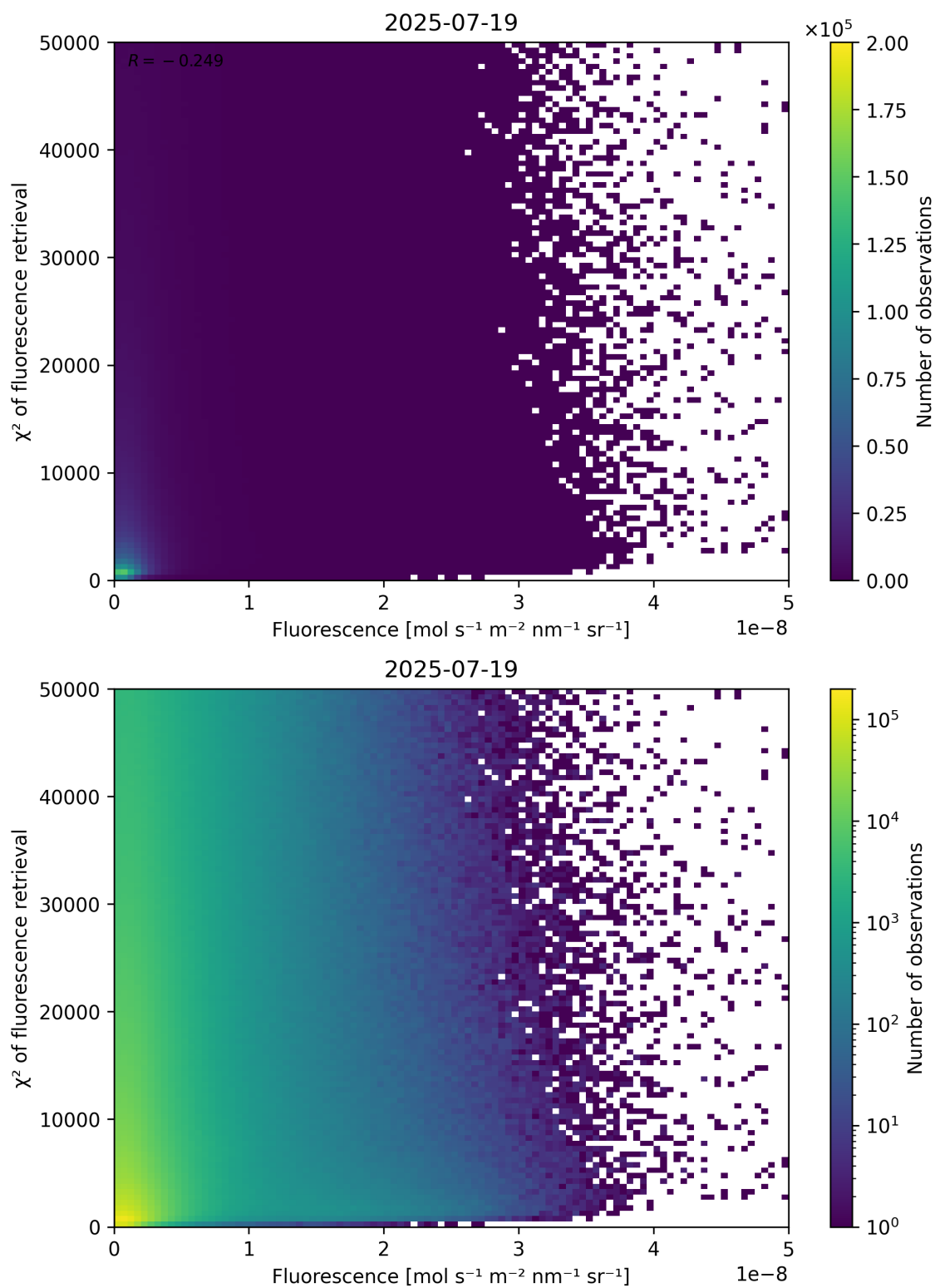
Figure 85: Scatter density plot of “Fluorescence” against “ \chi^2 of fluorescence retrieval” for 2025-07-19 to 2025-07-20.
