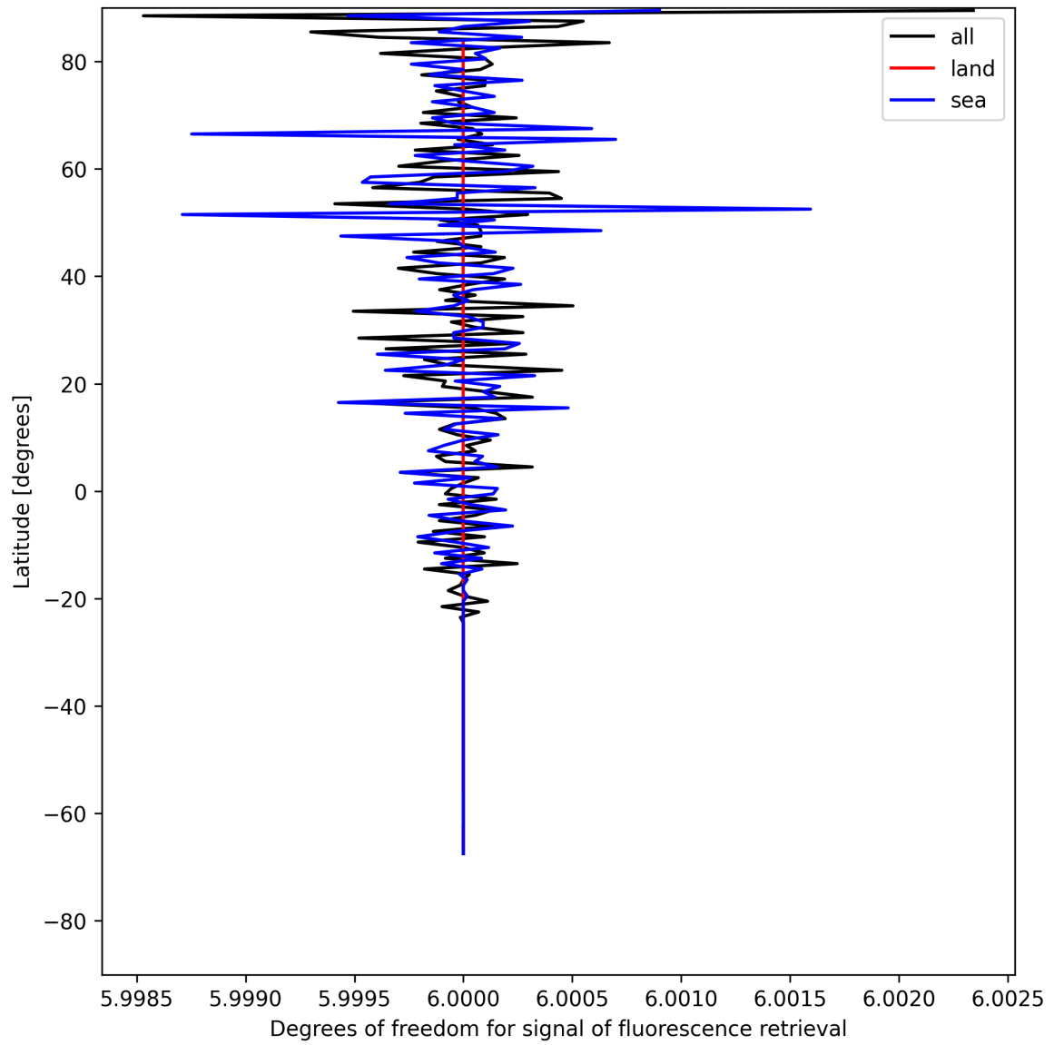
Figure 26: Zonal average of “Degrees of freedom for signal of fluorescence retrieval” for 2025-07-19 to 2025-07-20.
