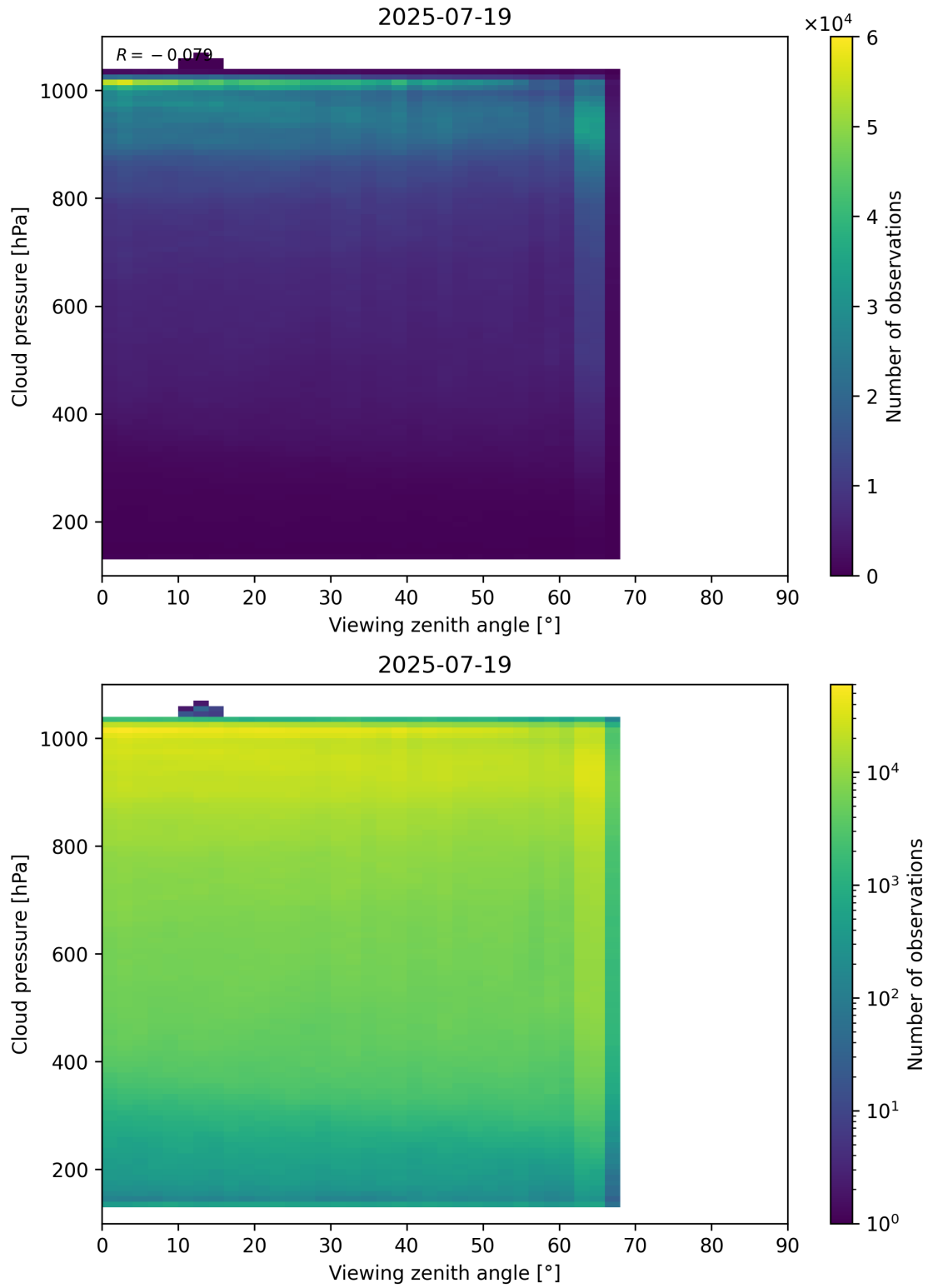
Figure 121: Scatter density plot of “Viewing zenith angle” against “Cloud pressure” for 2025-07-19 to 2025-07-20.
