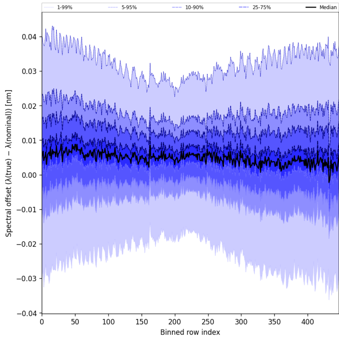
Figure 62: Along track statistics of “Spectral offset ( \lambda_{\text{true}} - \lambda_{\text{nominal}} )” for 2025-07-19 to 2025-07-20
