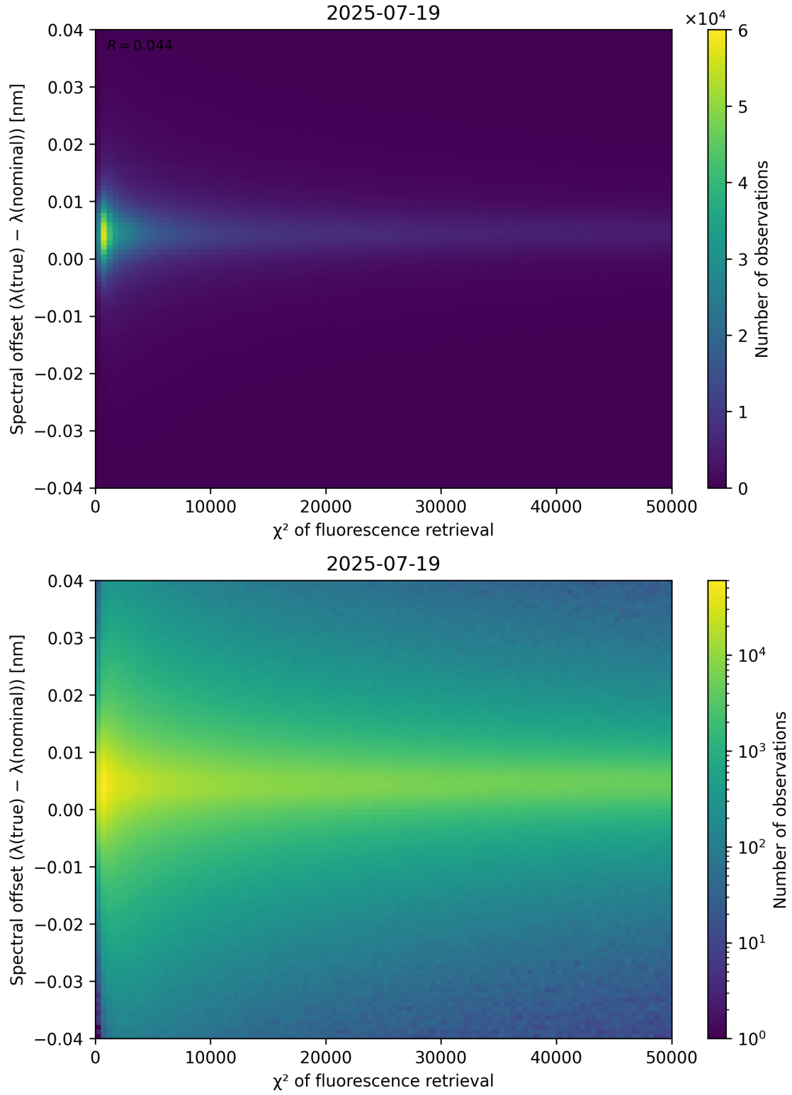
Figure 69: Scatter density plot of “ \chi^2 of fluorescence retrieval” against “Spectral offset ( \lambda_{\text{true}} - \lambda_{\text{nominal}} )” for 2025-07-19 to 2025-07-20.
