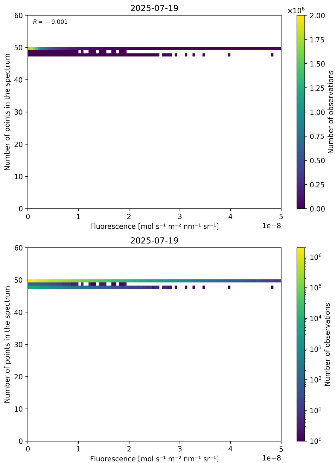
Figure 86: Scatter density plot of “Fluorescence” against “Number of points in the spectrum” for 2025-07-19 to 2025-07-20.
