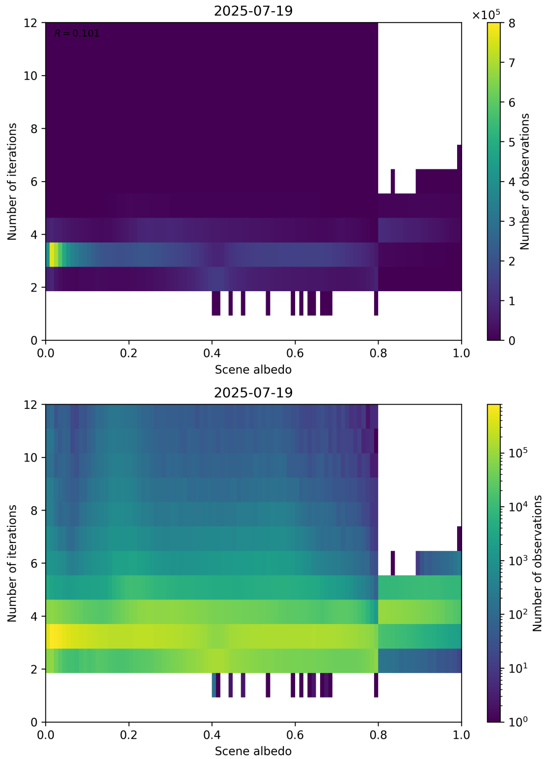
Figure 105: Scatter density plot of “Scene albedo” against “Number of iterations” for 2025-07-19 to 2025-07-20.
