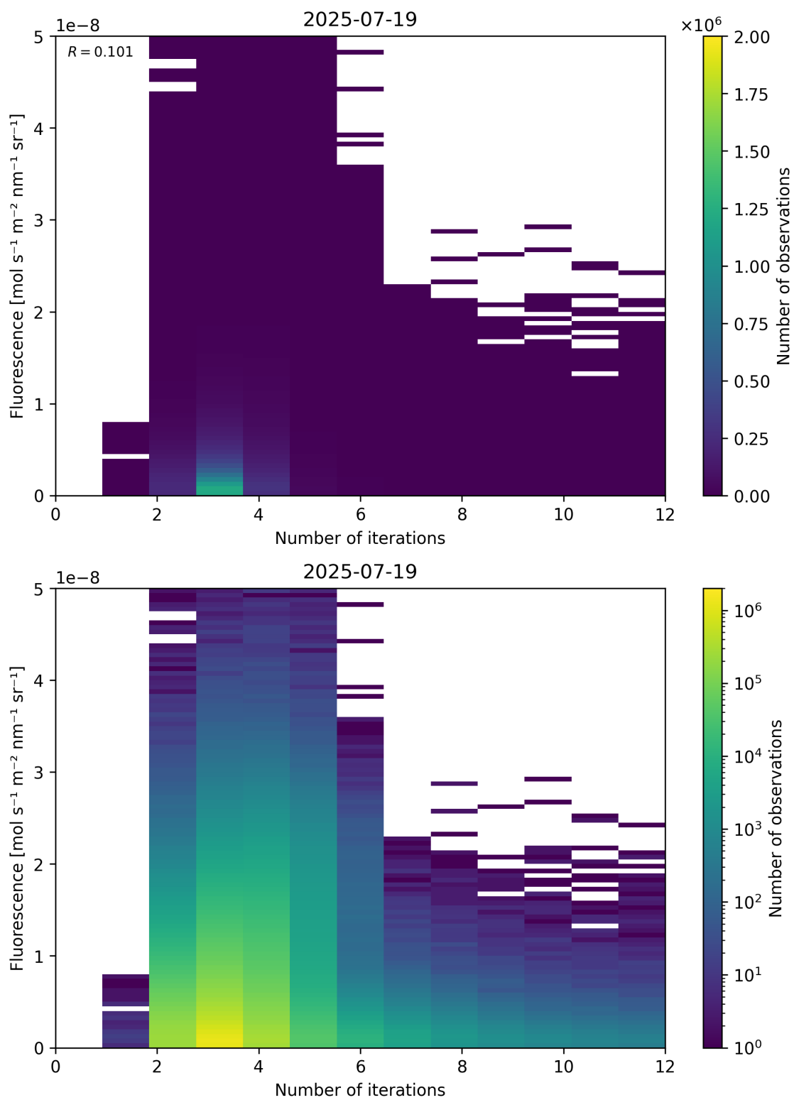
Figure 98: Scatter density plot of “Number of iterations” against “Fluorescence” for 2025-07-19 to 2025-07-20.
