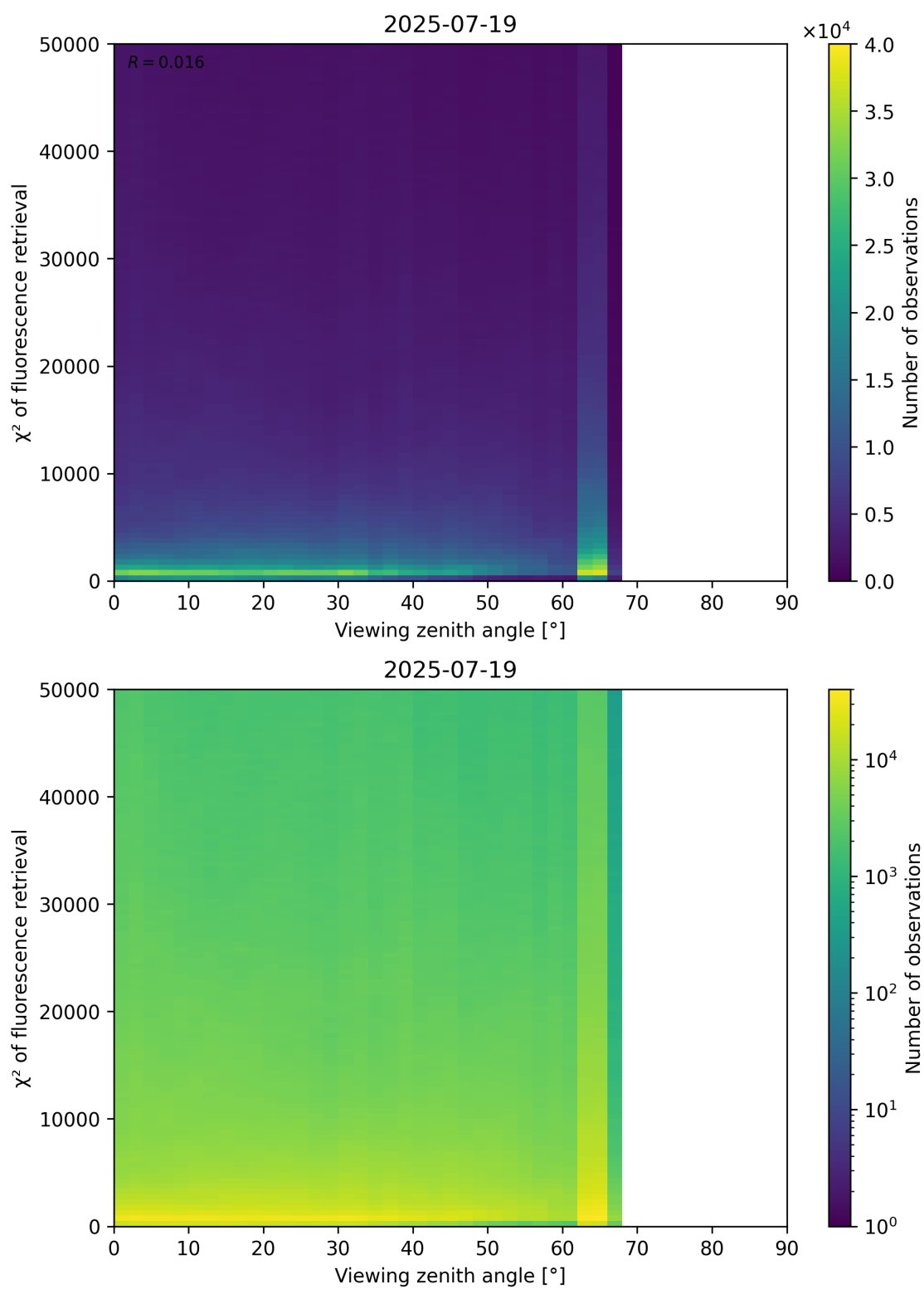
Figure 119: Scatter density plot of “Viewing zenith angle” against “ \chi^2 of fluorescence retrieval” for 2025-07-19 to 2025-07-20.
