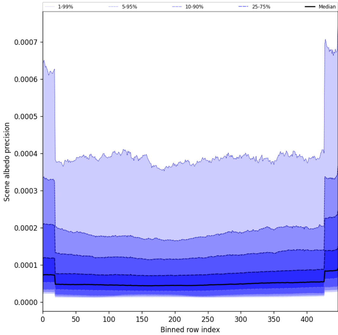
Figure 52: Along track statistics of “Scene albedo precision” for 2025-07-19 to 2025-07-20
