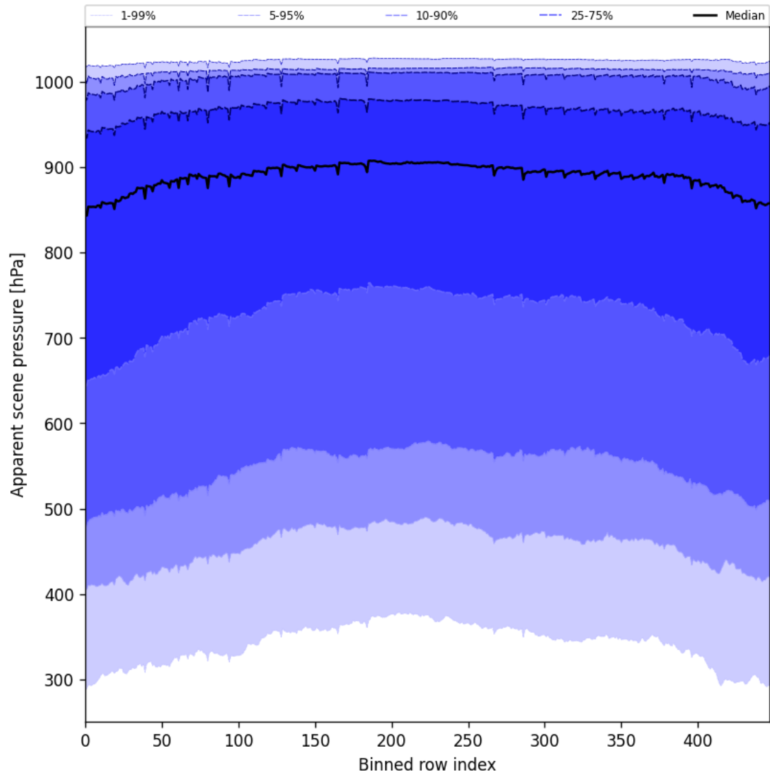
Figure 53: Along track statistics of “Apparent scene pressure” for 2025-07-19 to 2025-07-20
