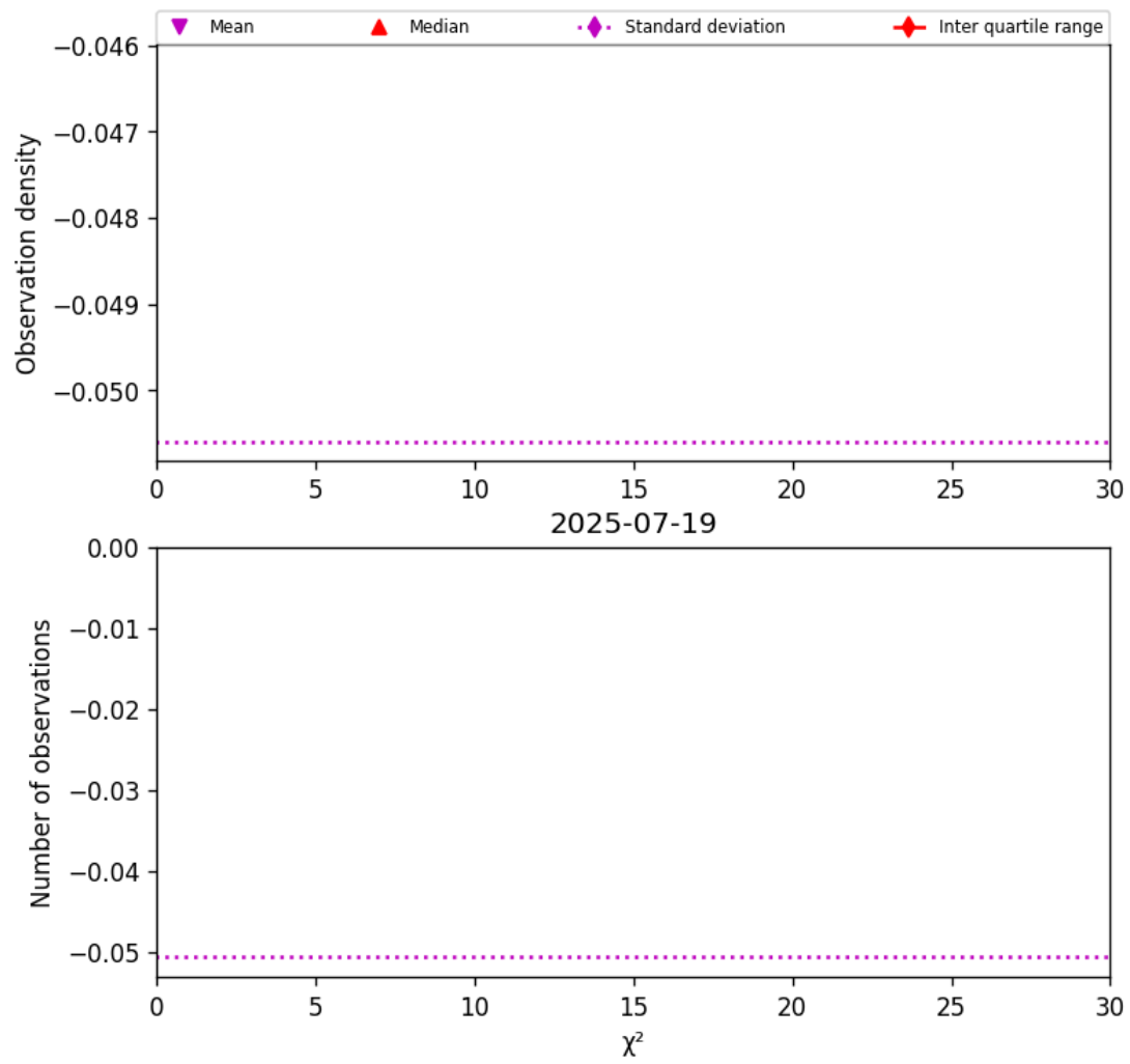
Figure 38: Histogram of “ \chi^2 ” for 2025-07-19 to 2025-07-20
