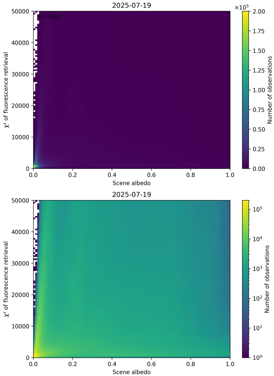
Figure 103: Scatter density plot of “Scene albedo” against “ \chi^2 of fluorescence retrieval” for 2025-07-19 to 2025-07-20.
