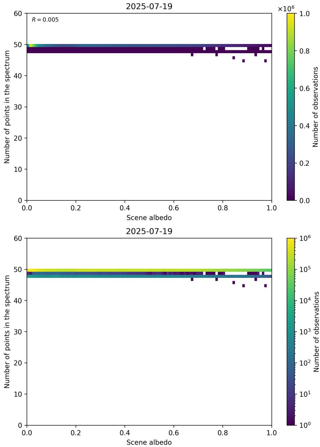
Figure 106: Scatter density plot of “Scene albedo” against “Number of points in the spectrum” for 2025-07-19 to 2025-07-20.
