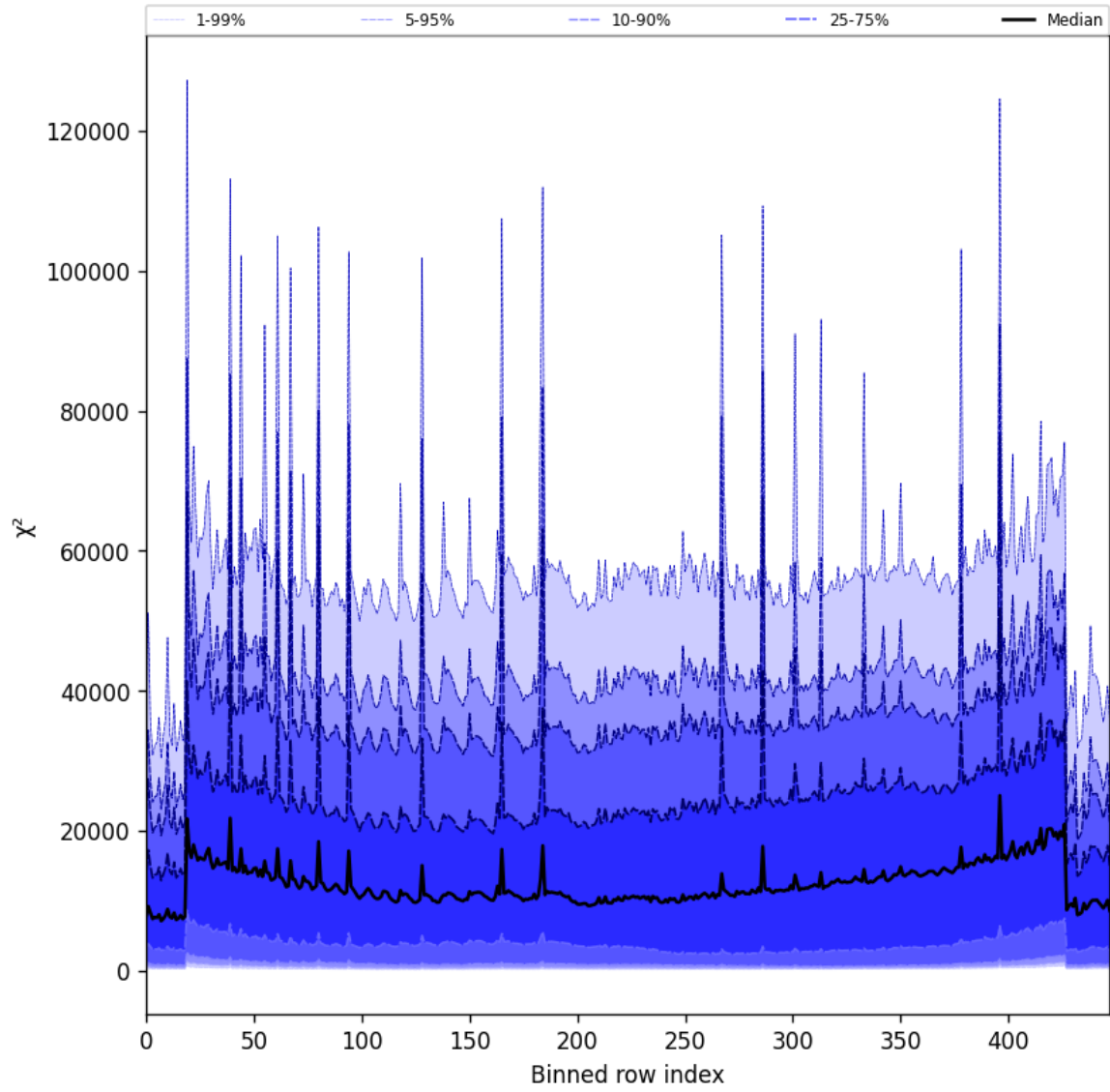
Figure 55: Along track statistics of “ \chi^2 ” for 2025-07-19 to 2025-07-20
