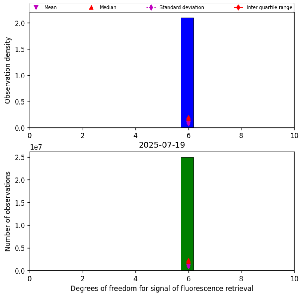
Figure 43: Histogram of “Degrees of freedom for signal of fluorescence retrieval” for 2025-07-19 to 2025-07-20
