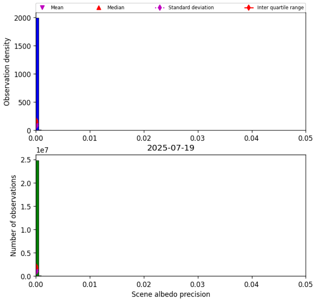
Figure 35: Histogram of “Scene albedo precision” for 2025-07-19 to 2025-07-20
