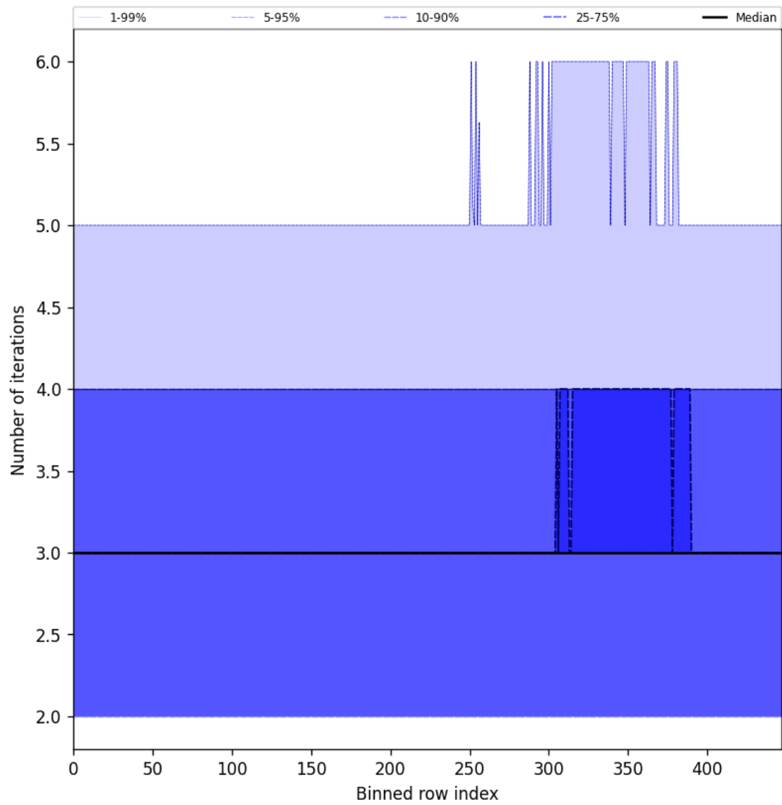
Figure 56: Along track statistics of “Number of iterations” for 2025-07-19 to 2025-07-20
