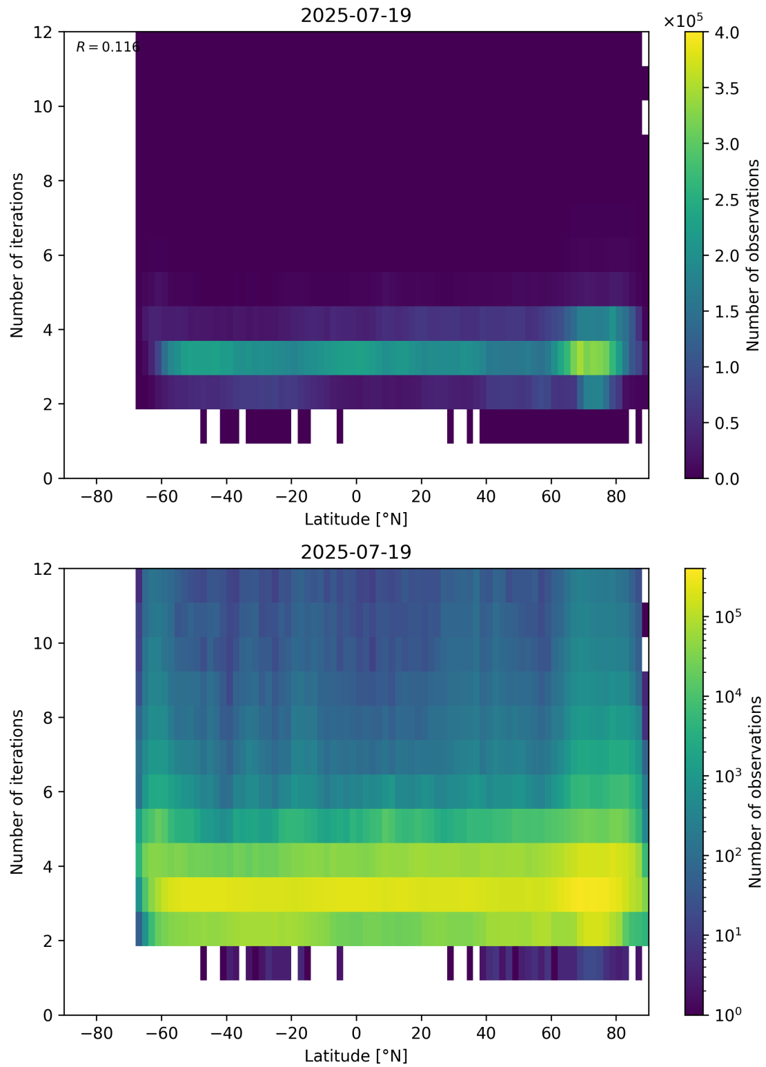
Figure 93: Scatter density plot of “Latitude” against “Number of iterations” for 2025-07-19 to 2025-07-20.
