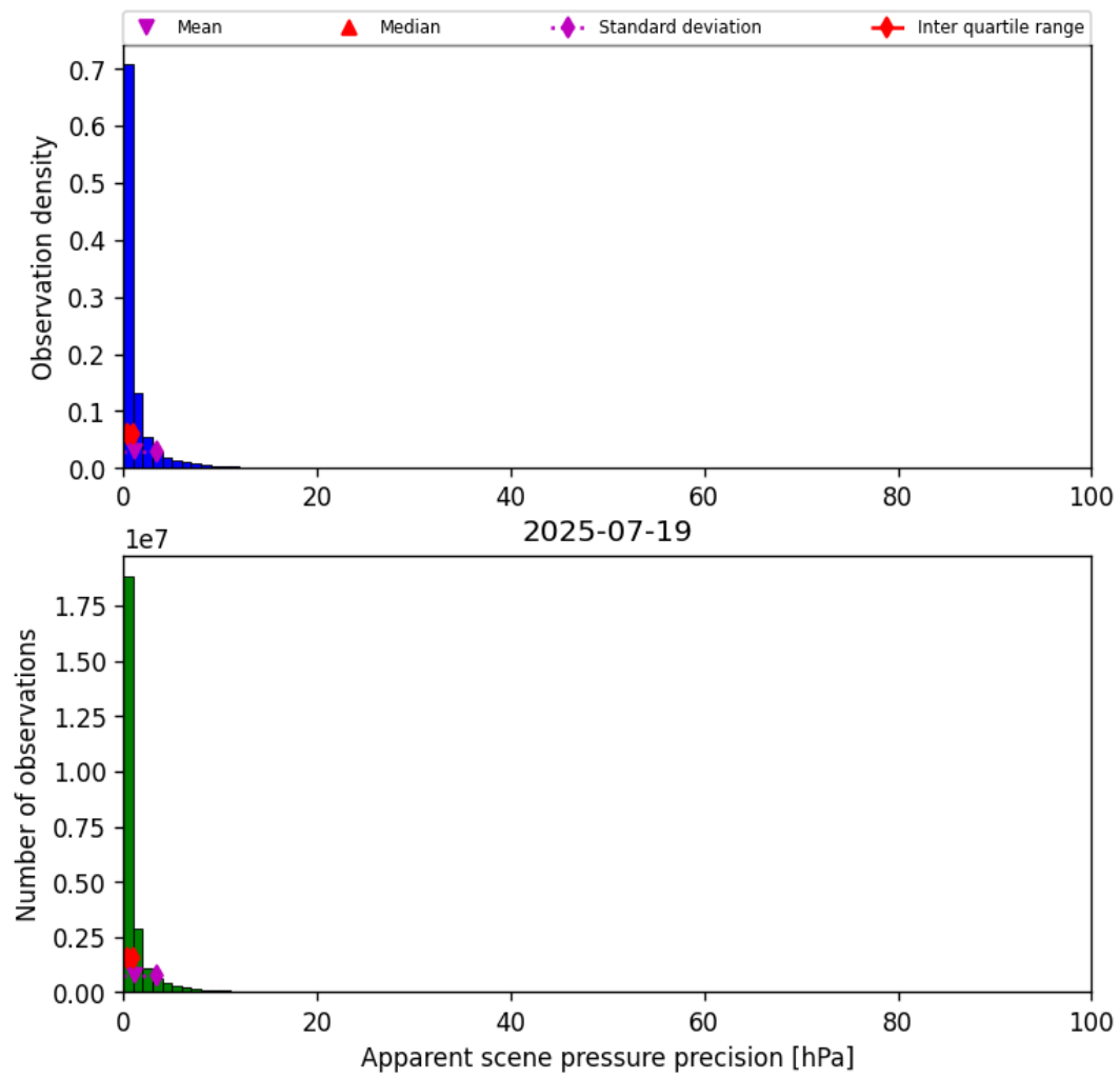
Figure 37: Histogram of “Apparent scene pressure precision” for 2025-07-19 to 2025-07-20
