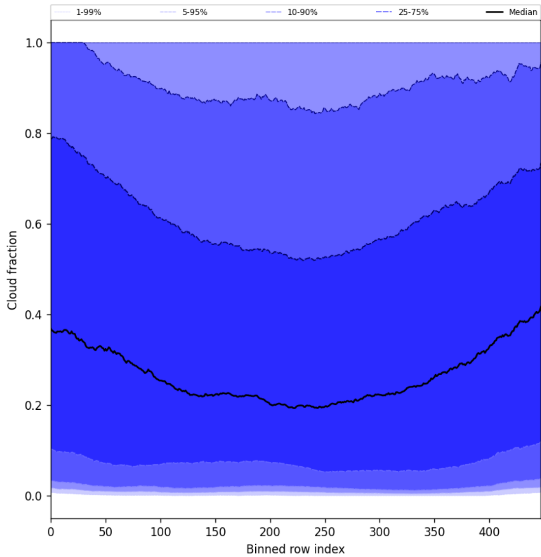
Figure 49: Along track statistics of “Cloud fraction” for 2025-07-19 to 2025-07-20
