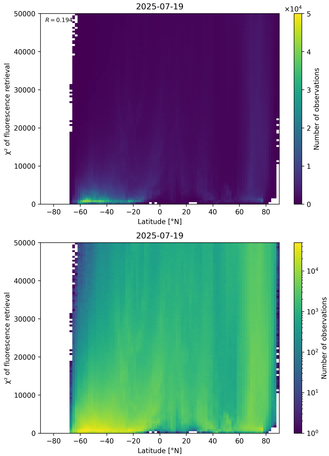
Figure 89: Scatter density plot of “Latitude” against “ \chi^2 of fluorescence retrieval” for 2025-07-19 to 2025-07-20.
