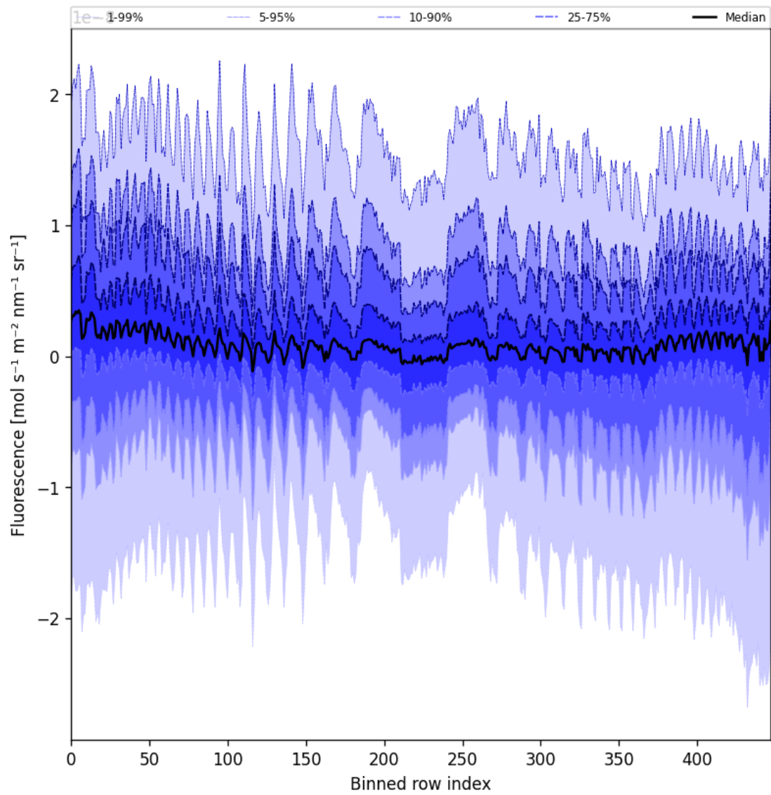
Figure 57: Along track statistics of “Fluorescence” for 2025-07-19 to 2025-07-20
