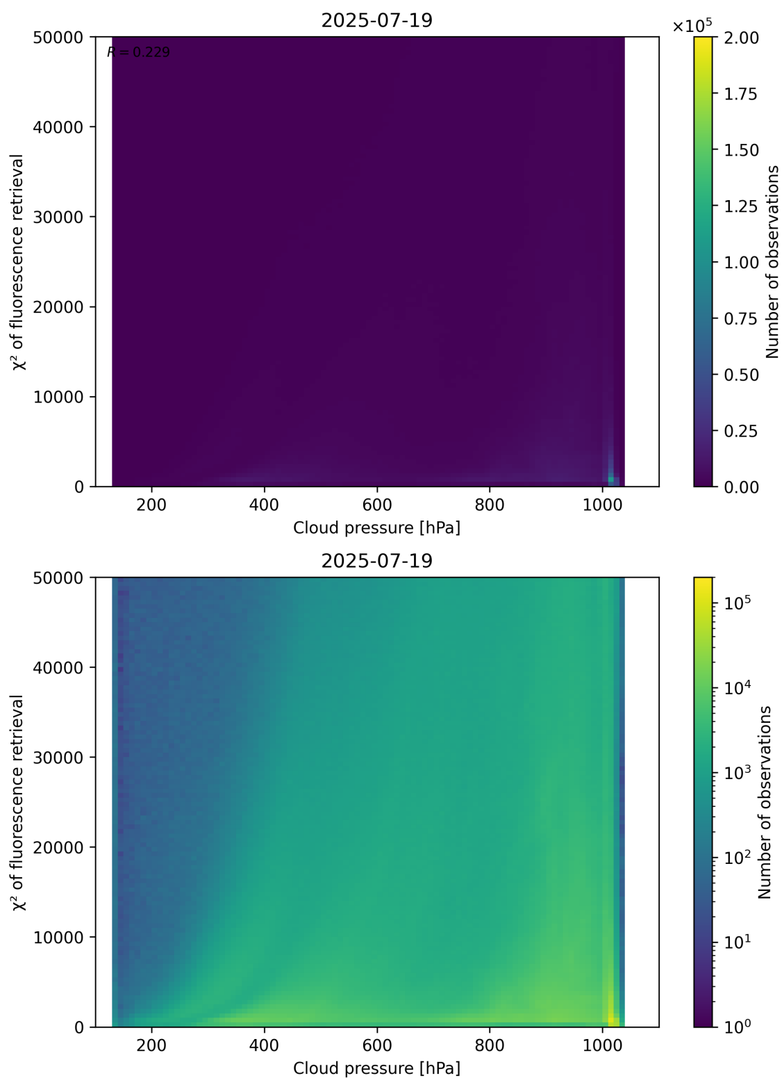
Figure 78: Scatter density plot of “Cloud pressure” against “ \chi^2 of fluorescence retrieval” for 2025-07-19 to 2025-07-20.
