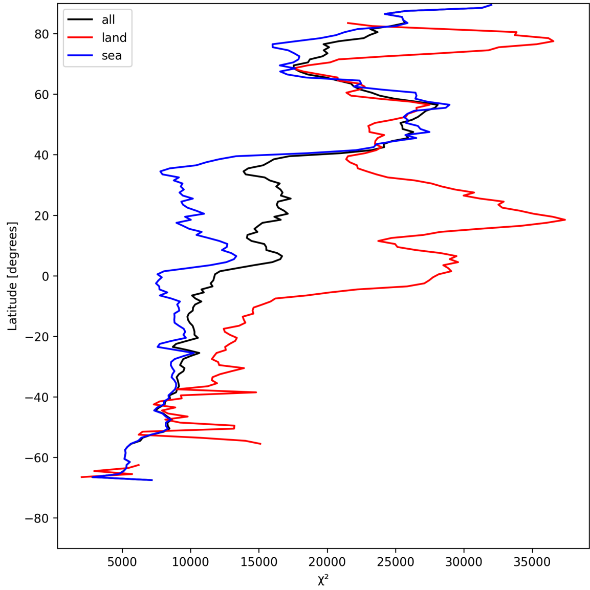
Figure 21: Zonal average of “ \chi^2 ” for 2025-07-19 to 2025-07-20.
