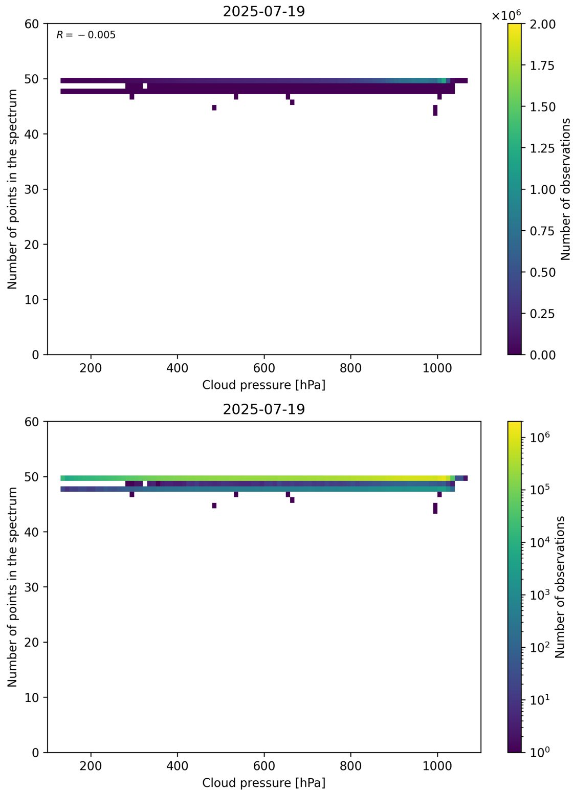
Figure 82: Scatter density plot of “Cloud pressure” against “Number of points in the spectrum” for 2025-07-19 to 2025-07-20.
