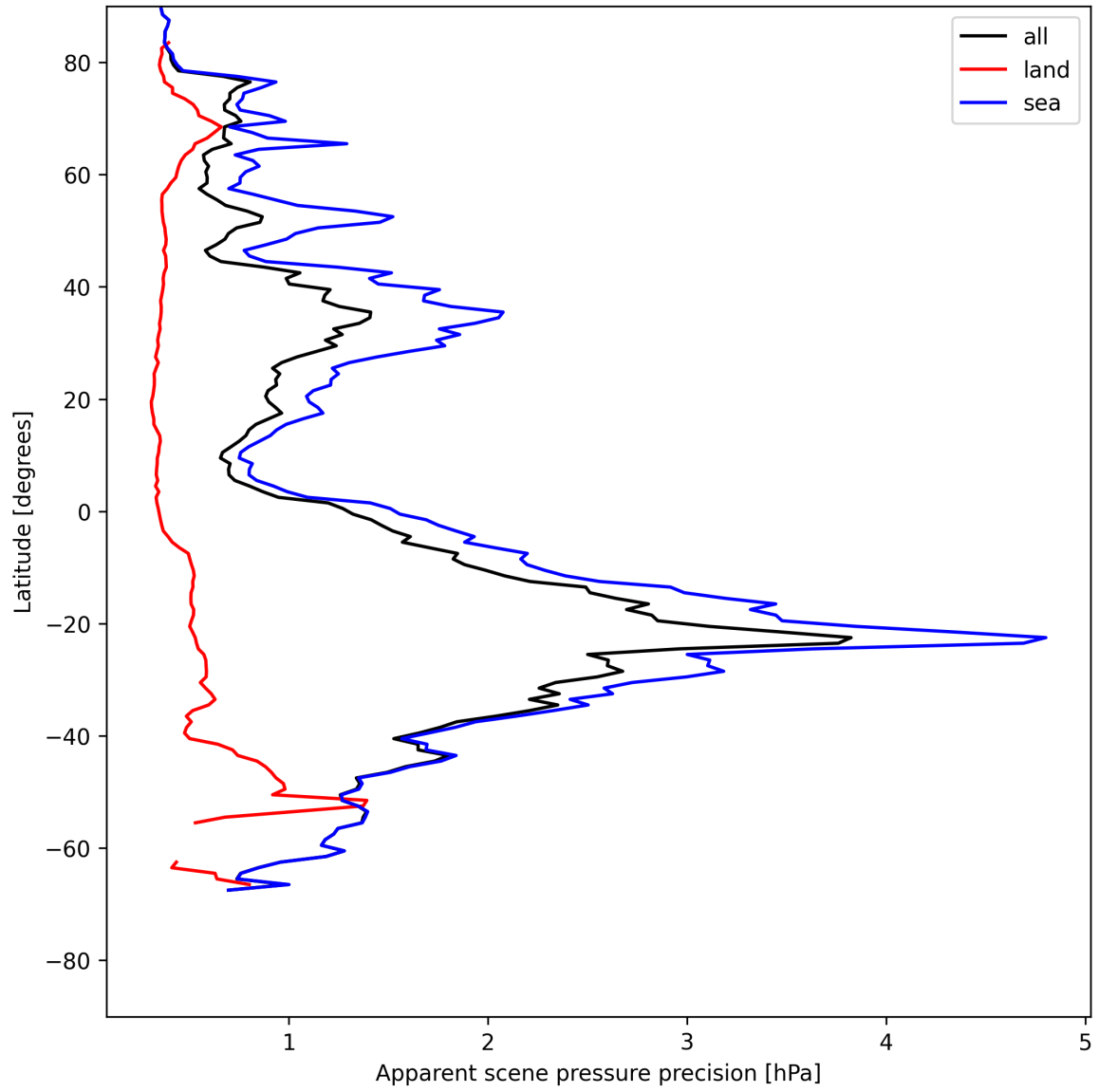
Figure 20: Zonal average of “Apparent scene pressure precision” for 2025-07-19 to 2025-07-20.
