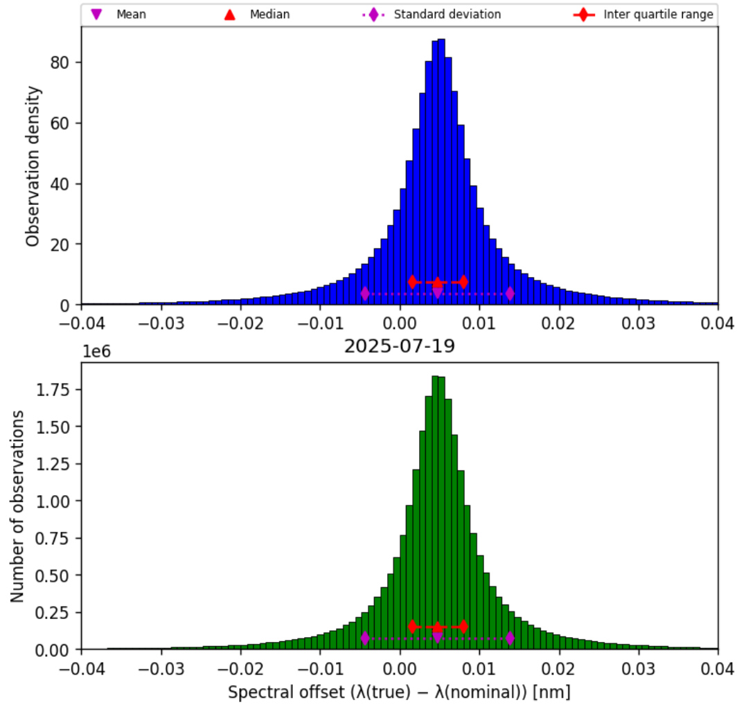
Figure 45: Histogram of “Spectral offset ( \lambda_{\text{true}} - \lambda_{\text{nominal}} )” for 2025-07-19 to 2025-07-20
