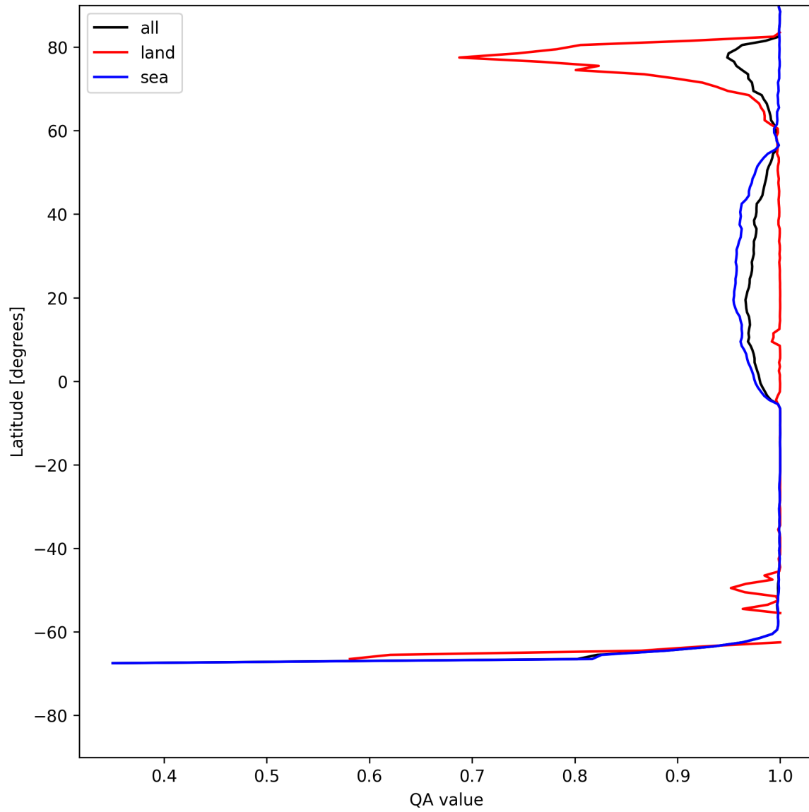
Figure 12: Zonal average of “QA value” for 2025-07-19 to 2025-07-20.
