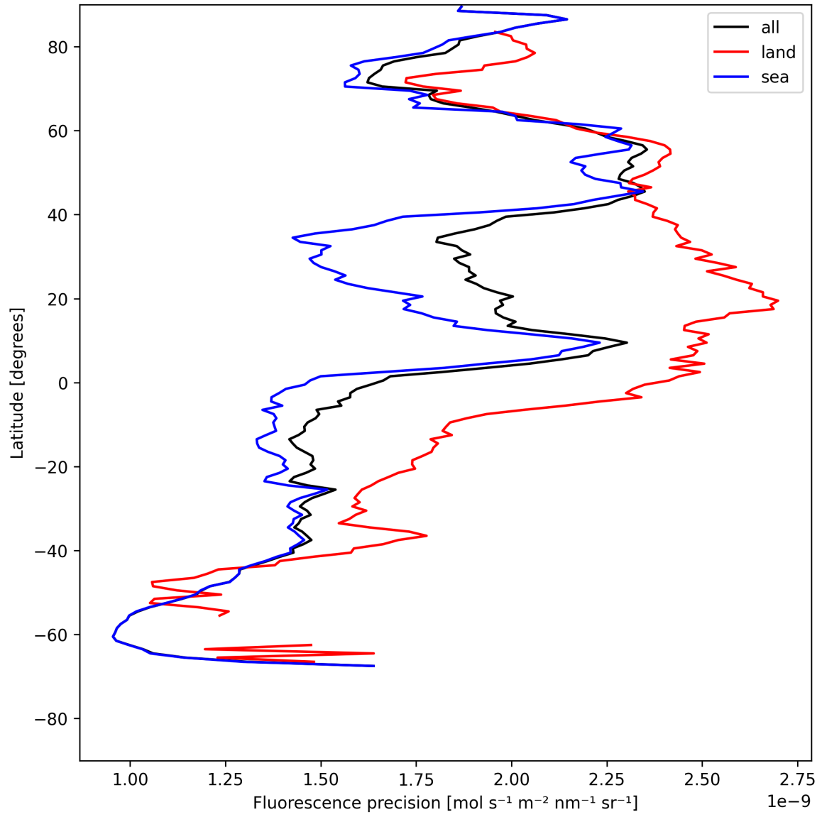
Figure 24: Zonal average of “Fluorescence precision” for 2025-07-19 to 2025-07-20.
