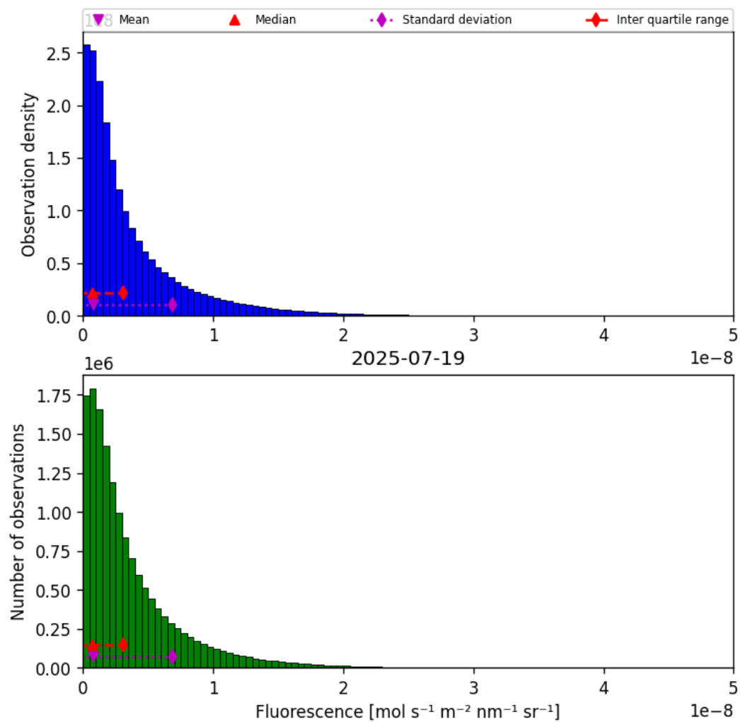
Figure 40: Histogram of “Fluorescence” for 2025-07-19 to 2025-07-20
