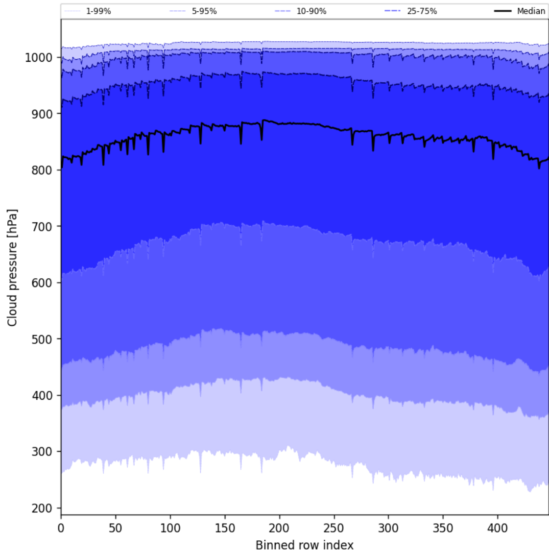
Figure 47: Along track statistics of “Cloud pressure” for 2025-07-19 to 2025-07-20
