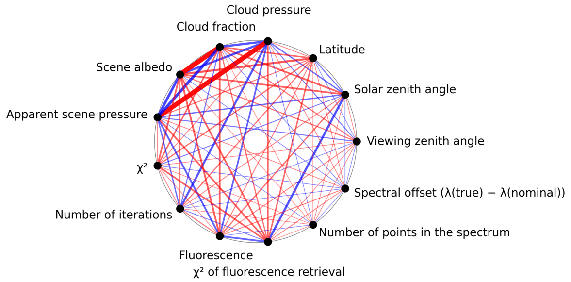
Figure 1: Map of correlation graph for 2025-07-19 to 2025-07-20.
