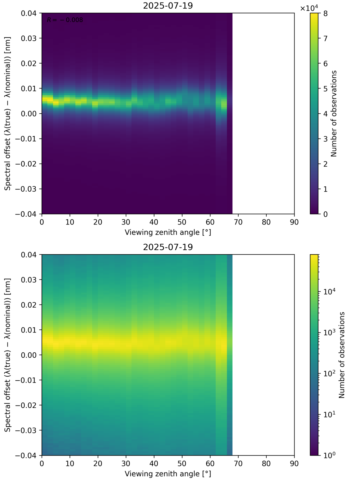
Figure 128: Scatter density plot of “Viewing zenith angle” against “Spectral offset ( \lambda_{\text{true}} - \lambda_{\text{nominal}} )” for 2025-07-19 to 2025-07-20.
