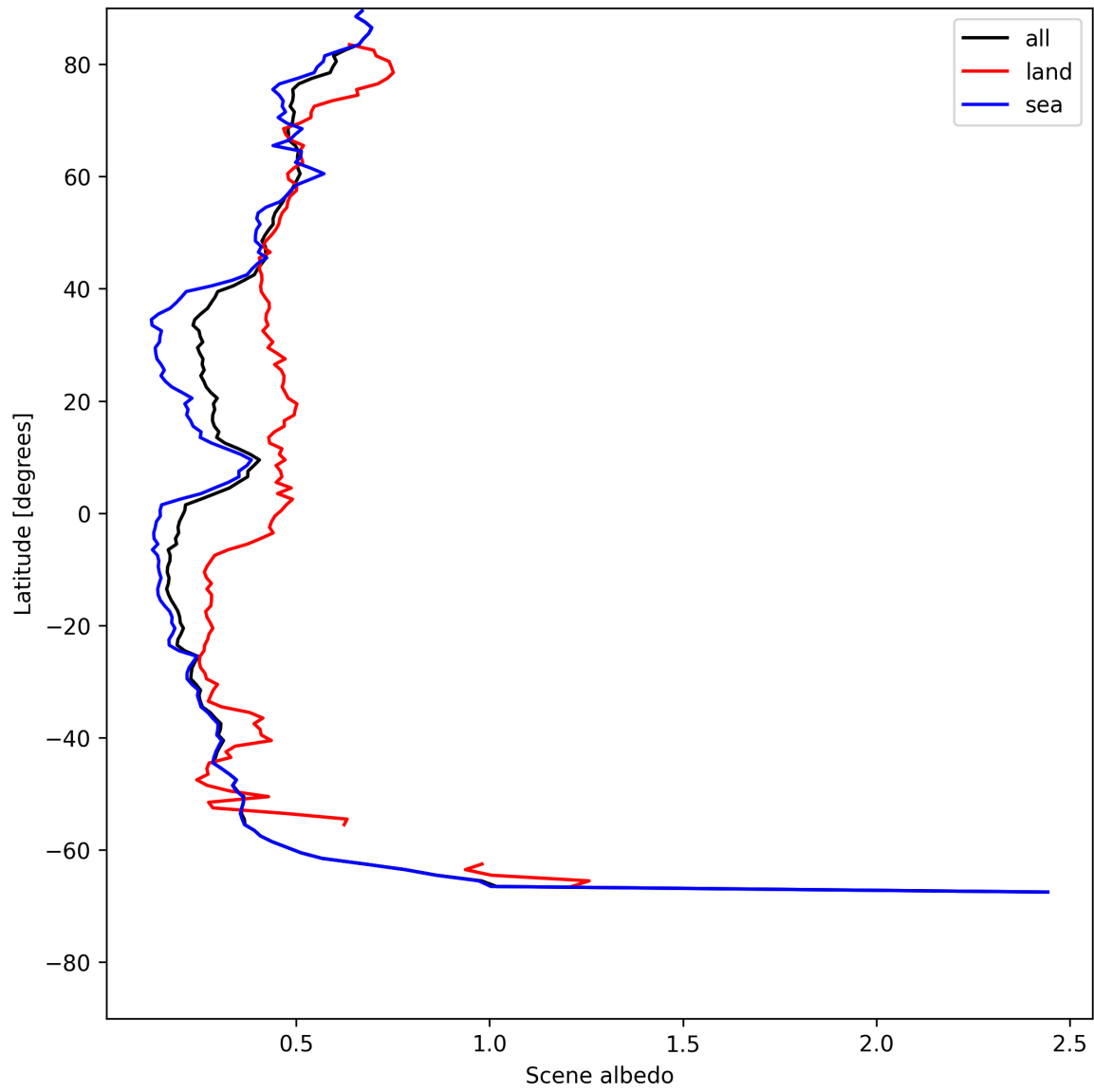
Figure 17: Zonal average of “Scene albedo” for 2025-07-19 to 2025-07-20.
