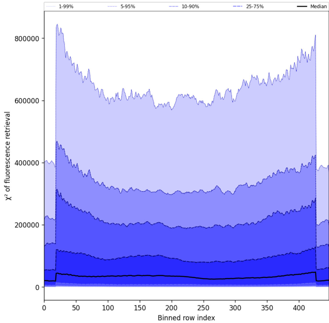
Figure 59: Along track statistics of “ \chi^2 of fluorescence retrieval” for 2025-07-19 to 2025-07-20
