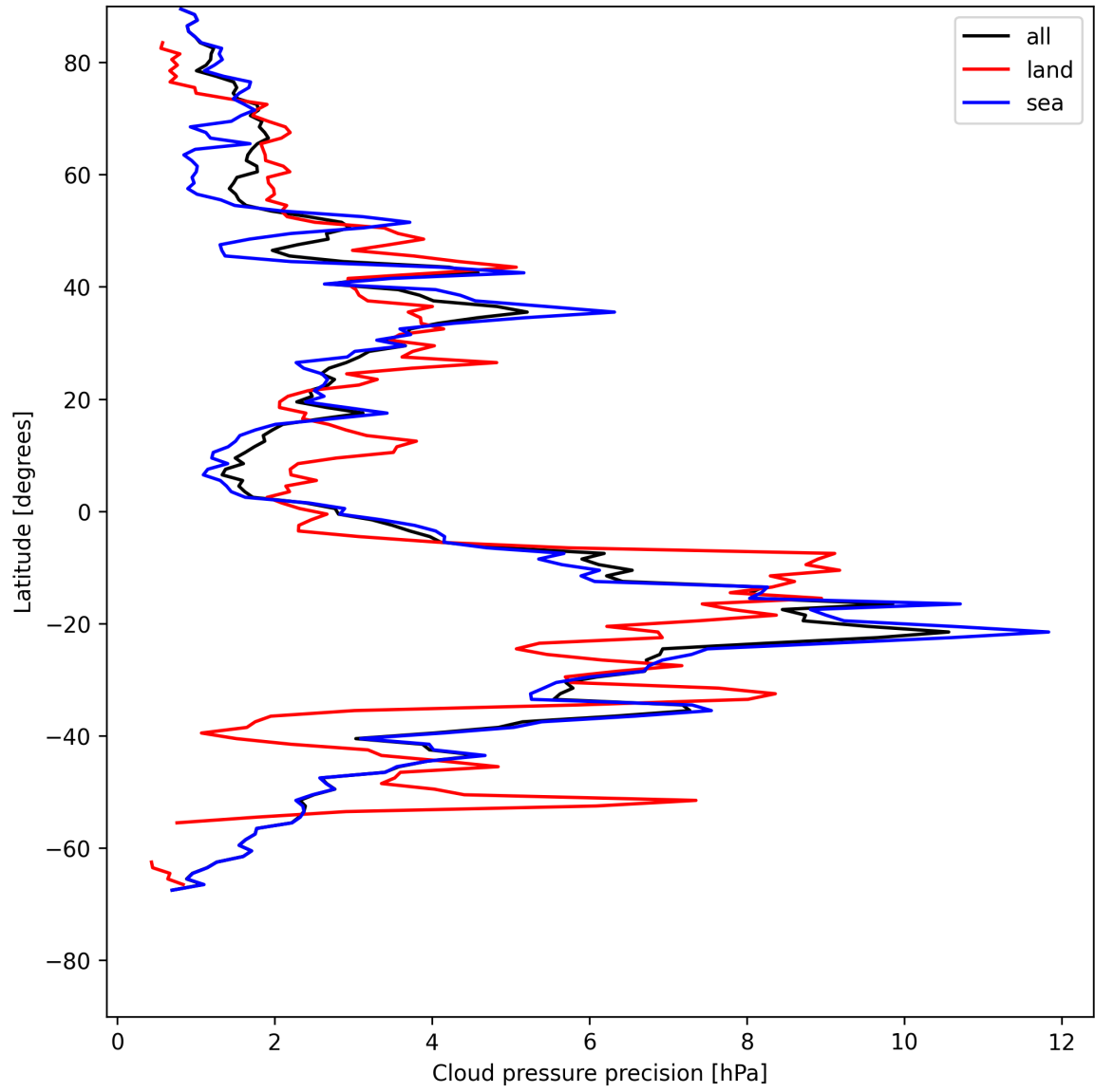
Figure 14: Zonal average of “Cloud pressure precision” for 2025-07-19 to 2025-07-20.
