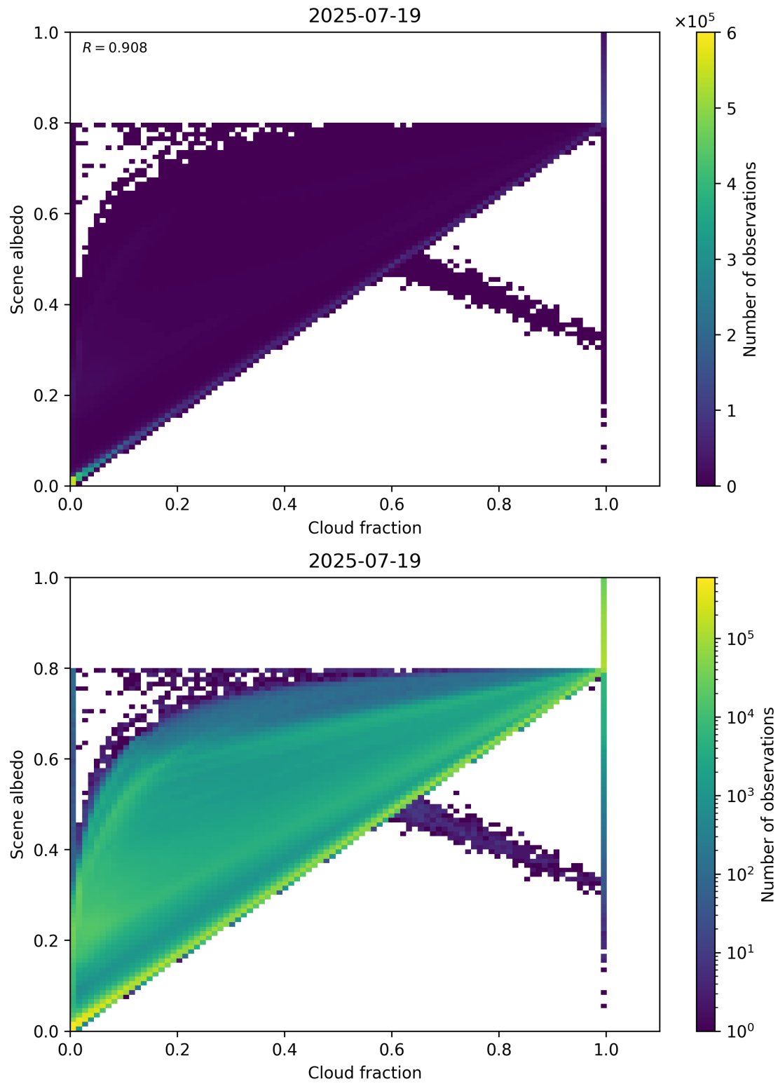
Figure 75: Scatter density plot of “Cloud fraction” against “Scene albedo” for 2025-07-19 to 2025-07-20.
