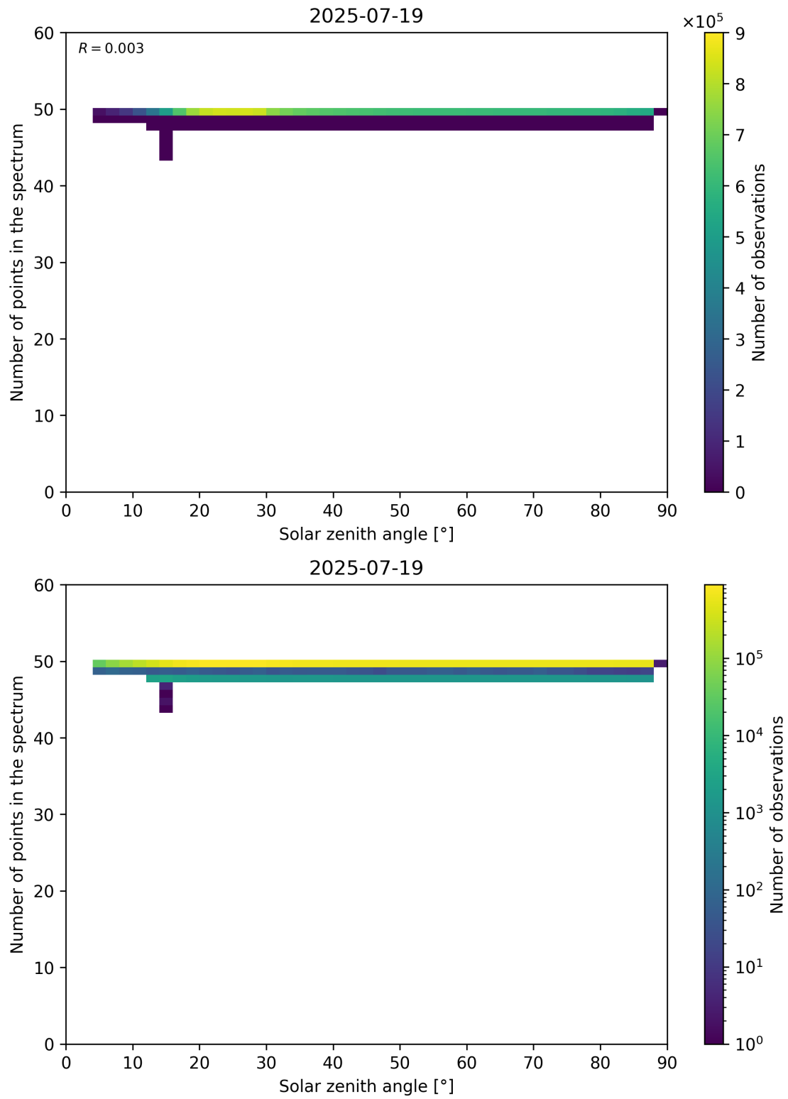
Figure 115: Scatter density plot of “Solar zenith angle” against “Number of points in the spectrum” for 2025-07-19 to 2025-07-20.
