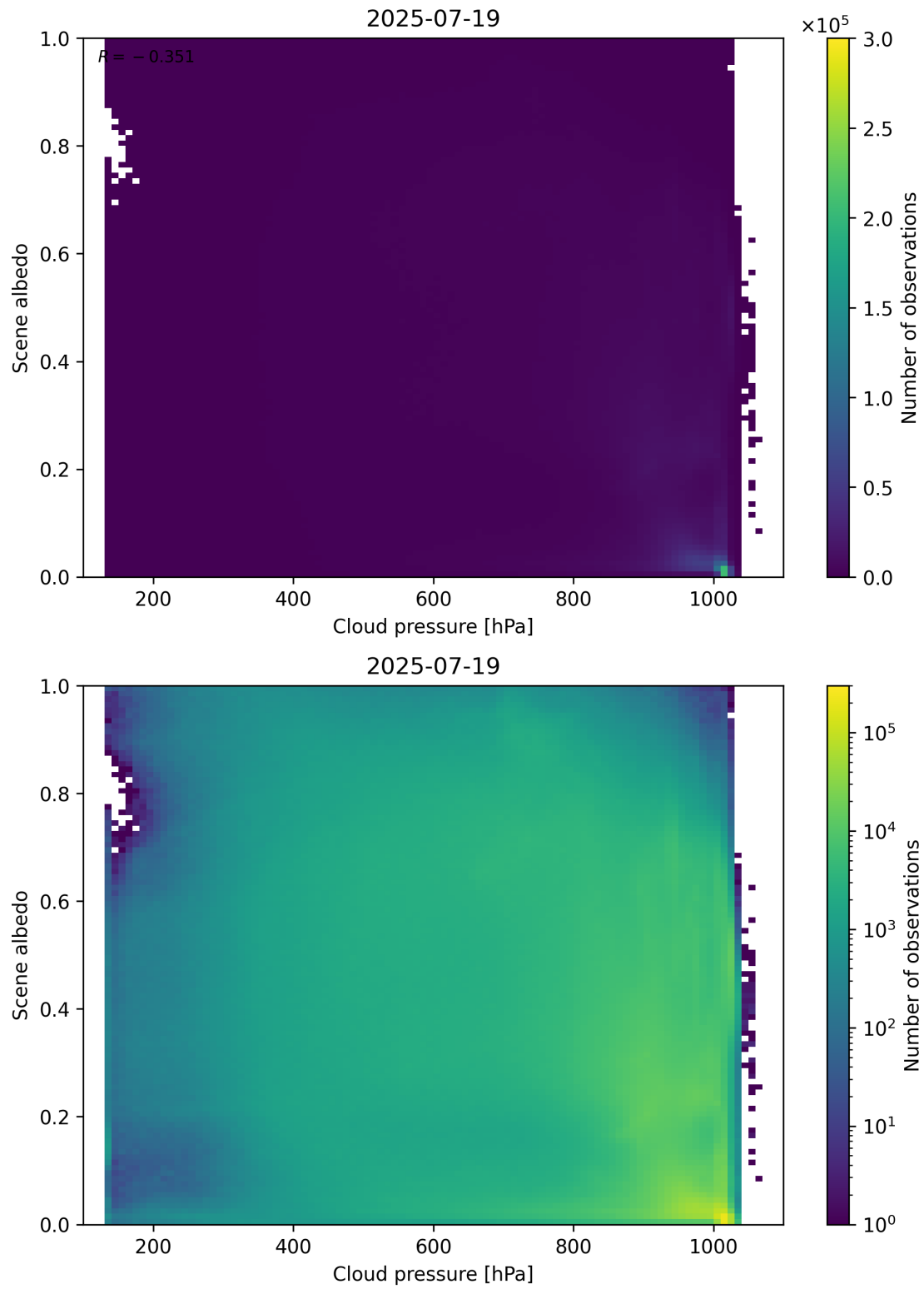
Figure 83: Scatter density plot of “Cloud pressure” against “Scene albedo” for 2025-07-19 to 2025-07-20.
