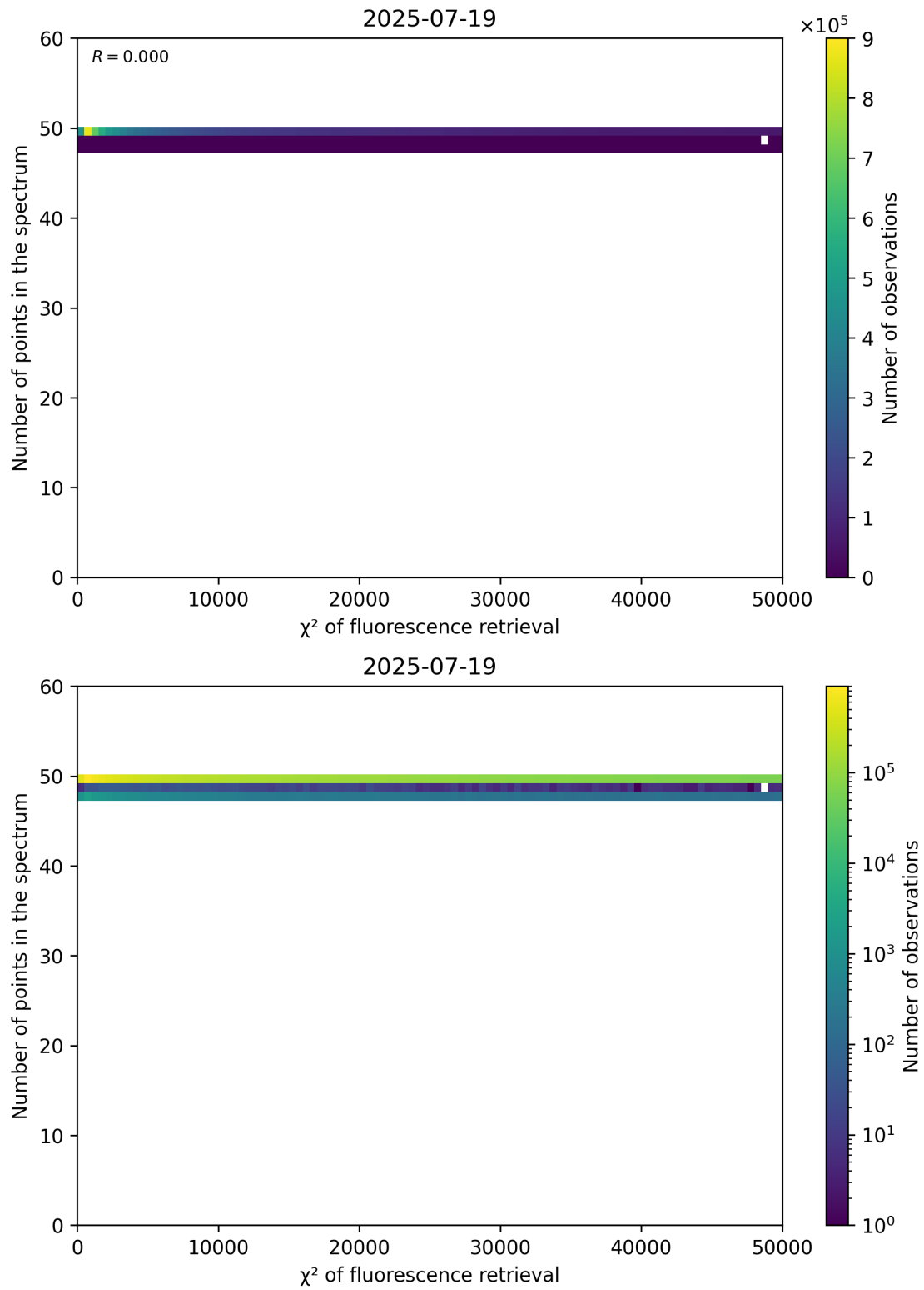
Figure 68: Scatter density plot of " \chi^2 of fluorescence retrieval" against "Number of points in the spectrum" for 2025-07-19 to 2025-07-20.
