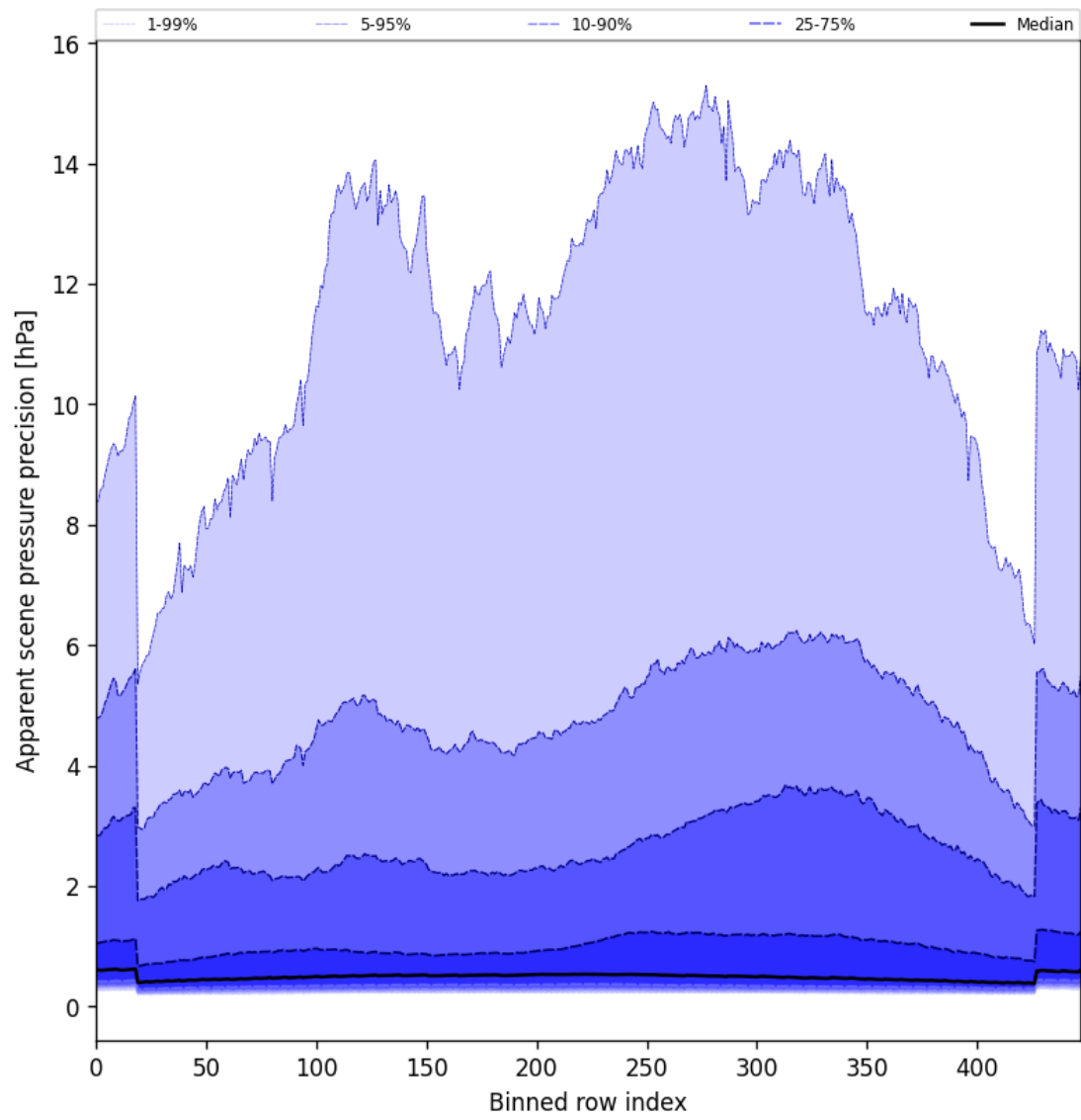
Figure 54: Along track statistics of “Apparent scene pressure precision” for 2025-07-19 to 2025-07-20
