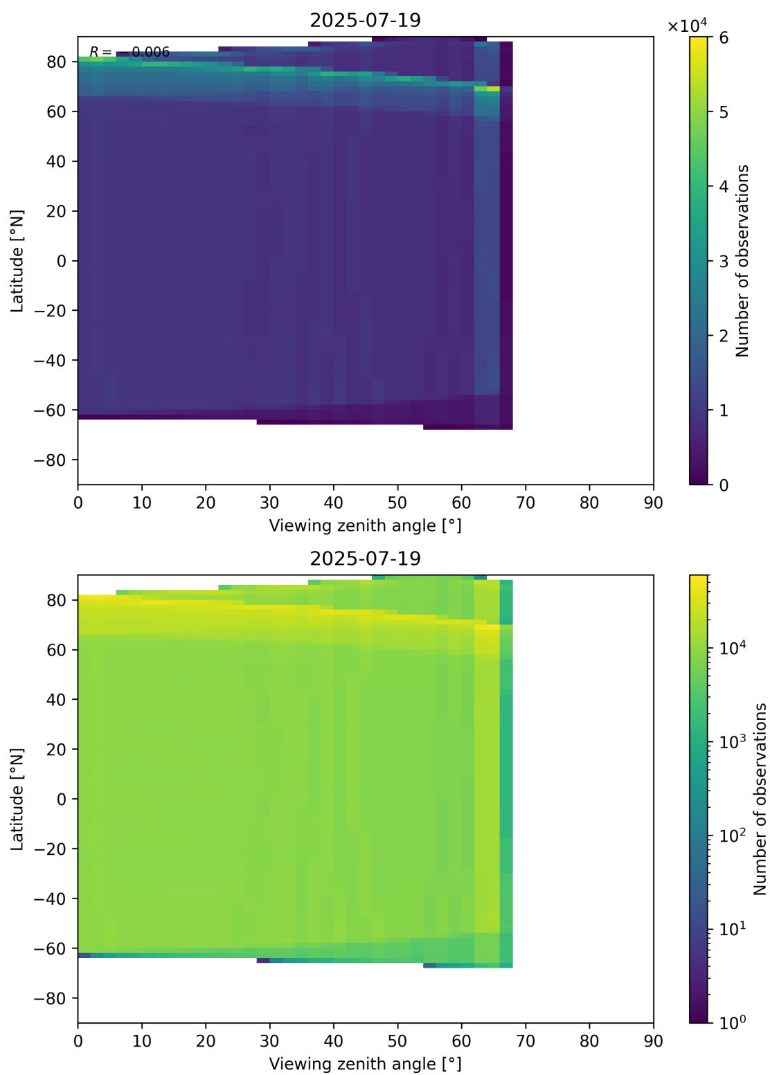
Figure 123: Scatter density plot of “Viewing zenith angle” against “Latitude” for 2025-07-19 to 2025-07-20.
