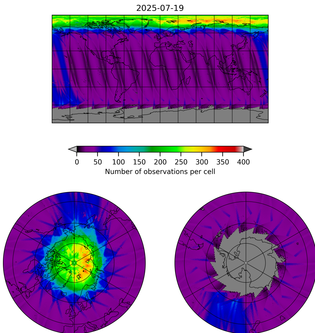
Figure 11: Map of the number of observations for 2025-07-19 to 2025-07-20
