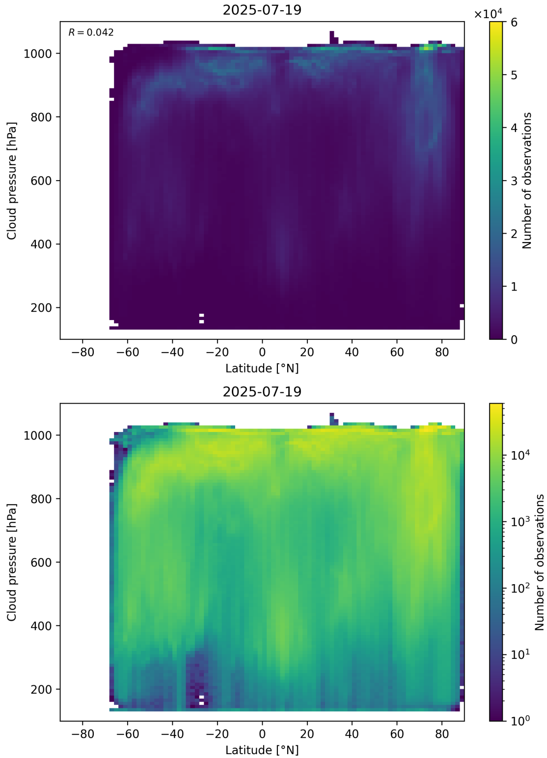
Figure 91: Scatter density plot of “Latitude” against “Cloud pressure” for 2025-07-19 to 2025-07-20.
