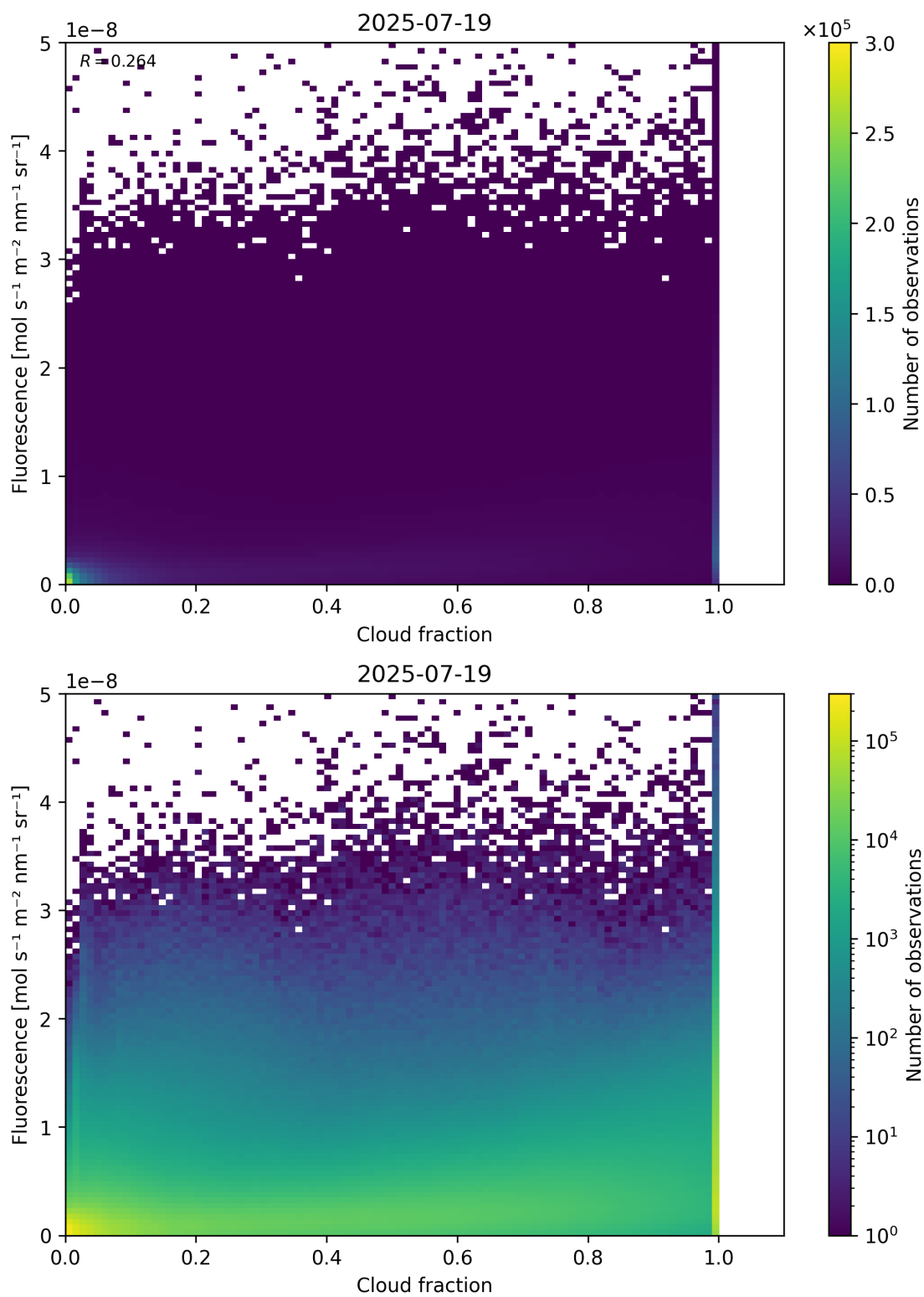
Figure 72: Scatter density plot of “Cloud fraction” against “Fluorescence” for 2025-07-19 to 2025-07-20.
