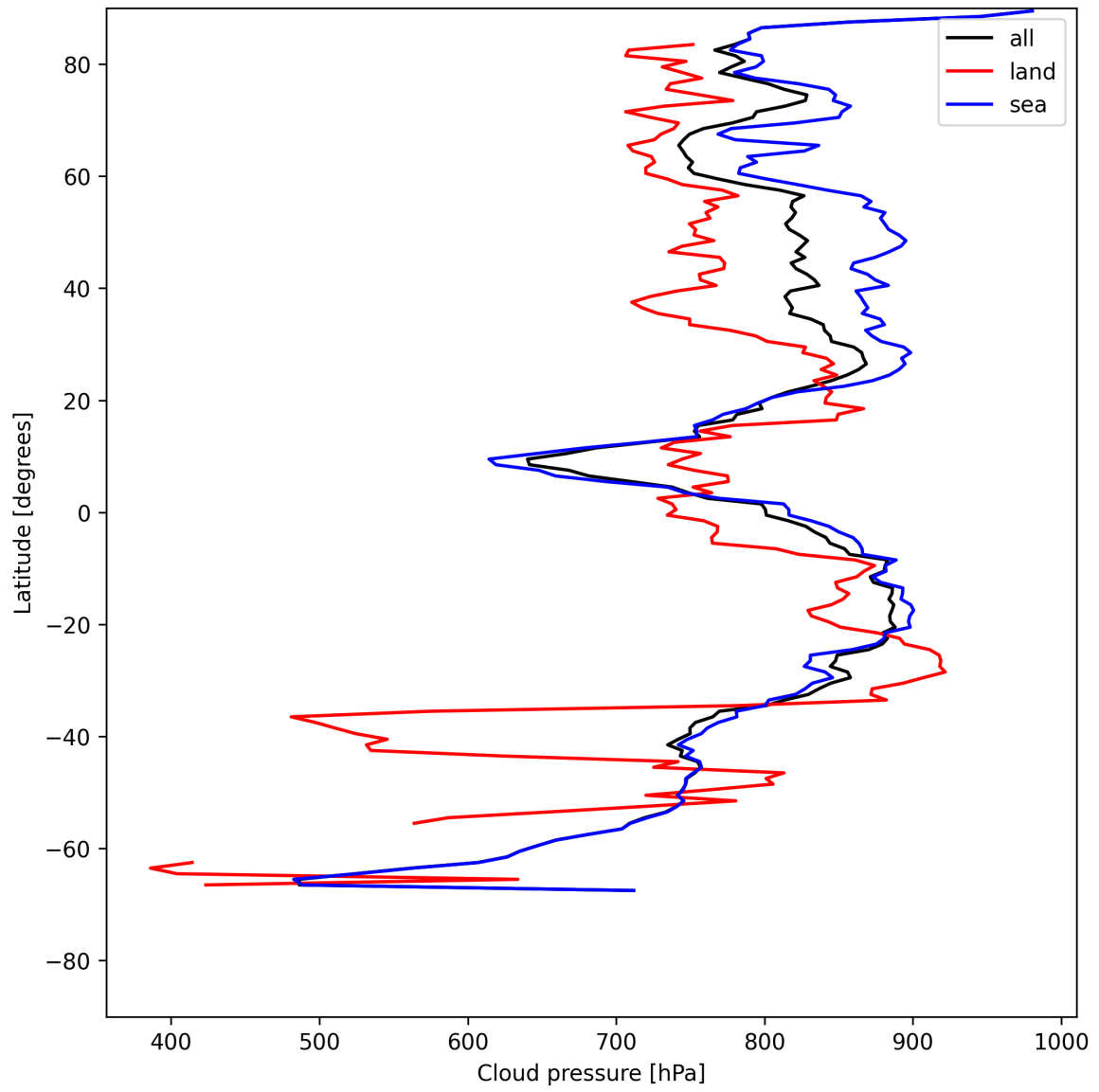
Figure 13: Zonal average of “Cloud pressure” for 2025-07-19 to 2025-07-20.
