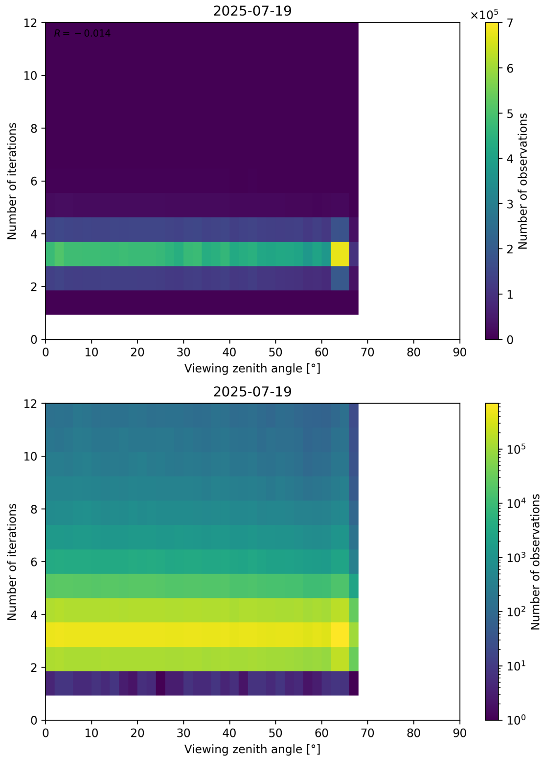
Figure 124: Scatter density plot of “Viewing zenith angle” against “Number of iterations” for 2025-07-19 to 2025-07-20.
