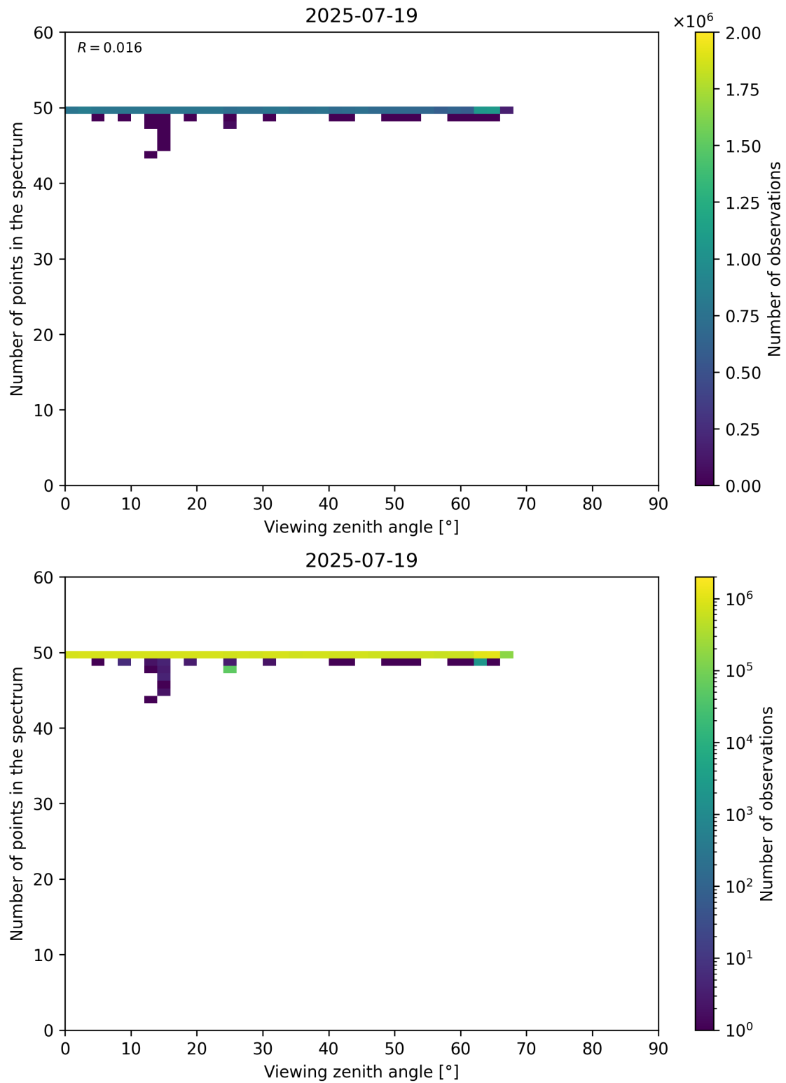
Figure 125: Scatter density plot of “Viewing zenith angle” against “Number of points in the spectrum” for 2025-07-19 to 2025-07-20.
