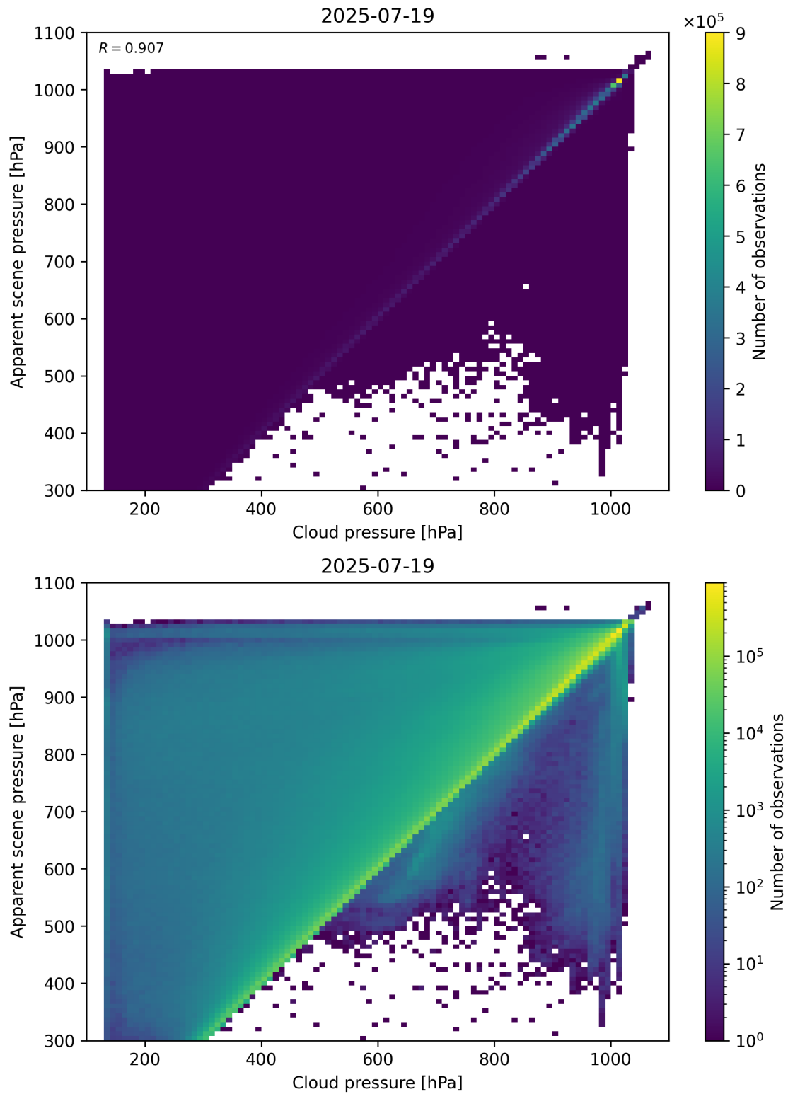
Figure 77: Scatter density plot of “Cloud pressure” against “Apparent scene pressure” for 2025-07-19 to 2025-07-20.
