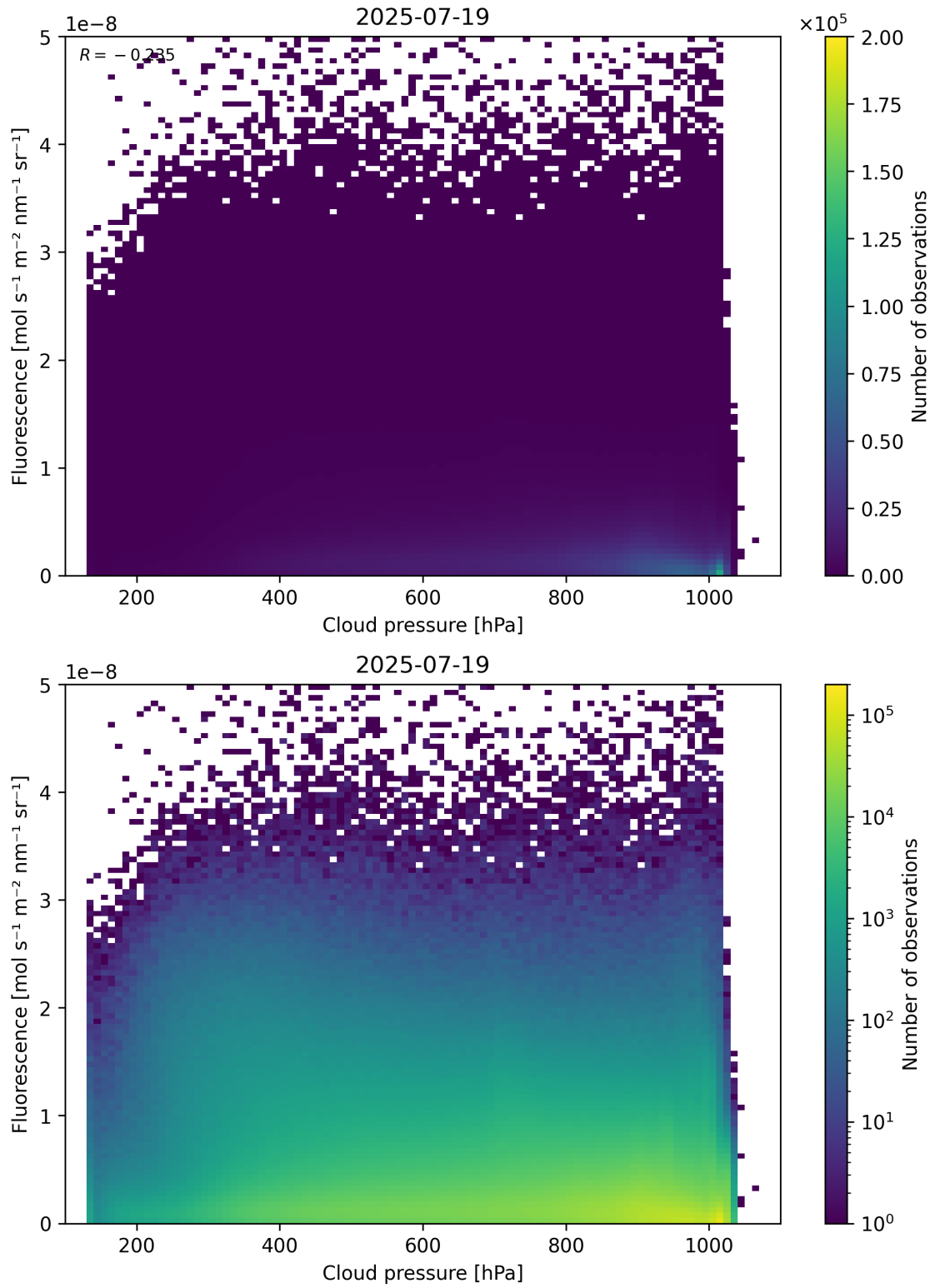
Figure 80: Scatter density plot of “Cloud pressure” against “Fluorescence” for 2025-07-19 to 2025-07-20.
