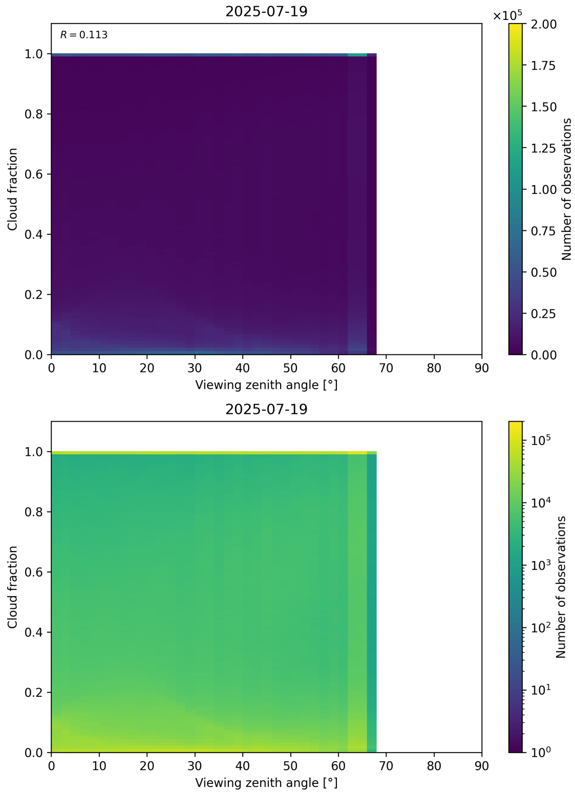
Figure 120: Scatter density plot of “Viewing zenith angle” against “Cloud fraction” for 2025-07-19 to 2025-07-20.
