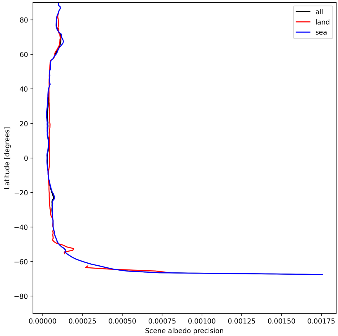
Figure 18: Zonal average of “Scene albedo precision” for 2025-07-19 to 2025-07-20.
