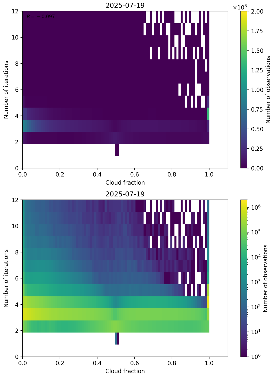
Figure 73: Scatter density plot of “Cloud fraction” against “Number of iterations” for 2025-07-19 to 2025-07-20.
