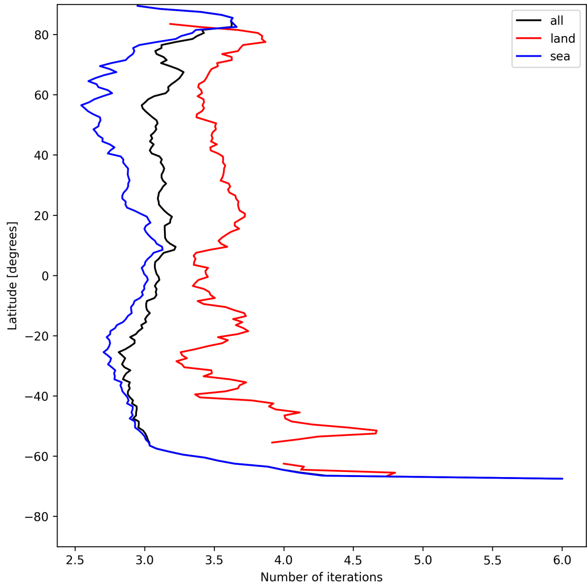
Figure 22: Zonal average of “Number of iterations” for 2025-07-19 to 2025-07-20.
