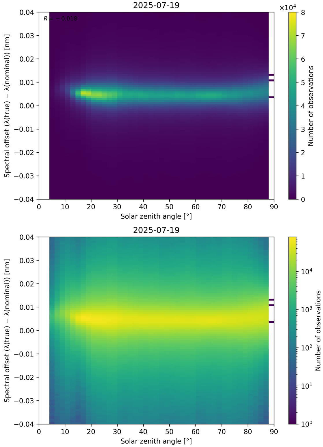
Figure 117: Scatter density plot of “Solar zenith angle” against “Spectral offset ( \lambda_{\text{true}} - \lambda_{\text{nominal}} )” for 2025-07-19 to 2025-07-20.
