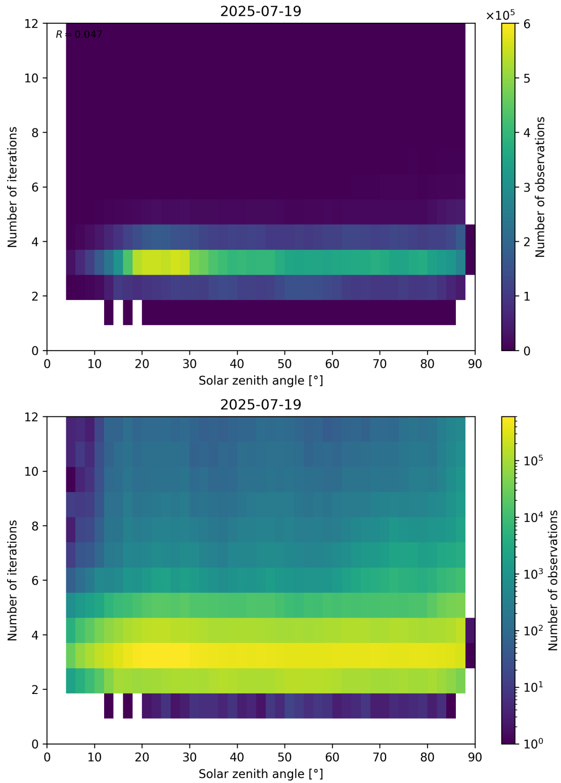
Figure 114: Scatter density plot of “Solar zenith angle” against “Number of iterations” for 2025-07-19 to 2025-07-20.
