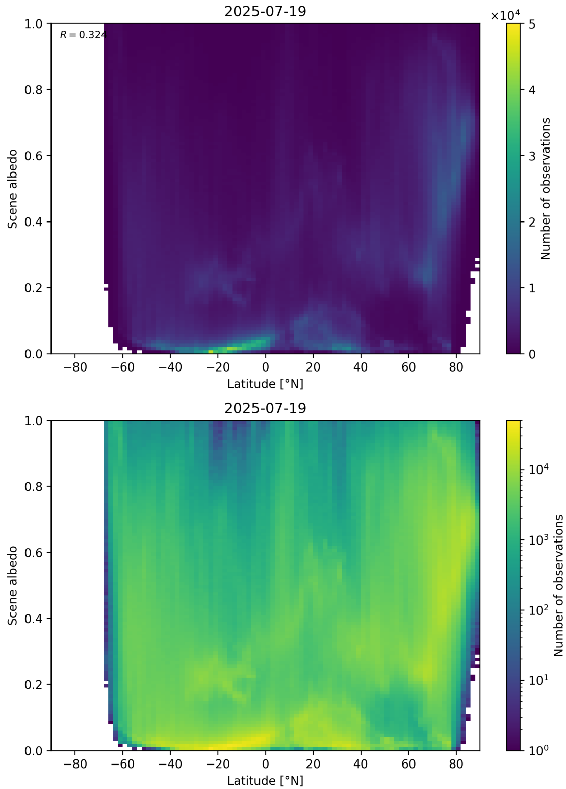
Figure 95: Scatter density plot of “Latitude” against “Scene albedo” for 2025-07-19 to 2025-07-20.
