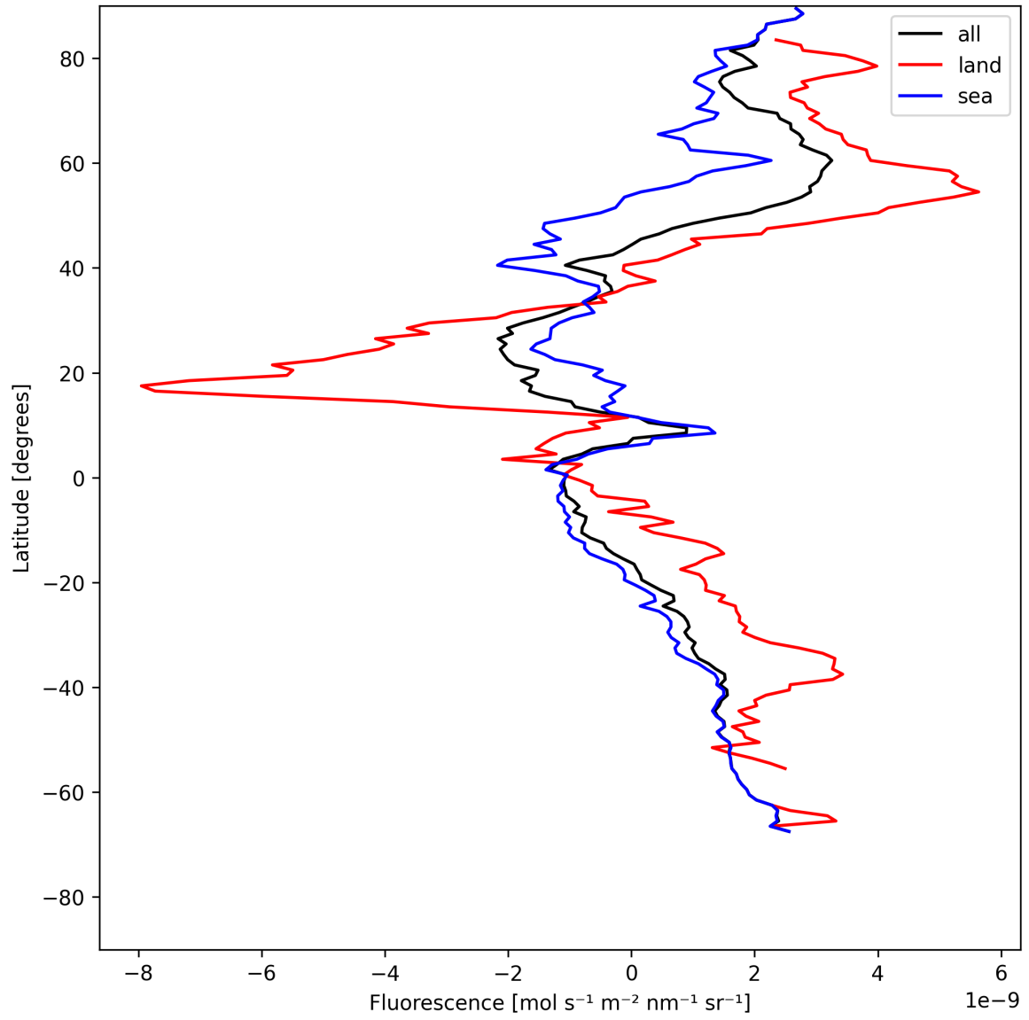
Figure 23: Zonal average of “Fluorescence” for 2025-07-19 to 2025-07-20.
