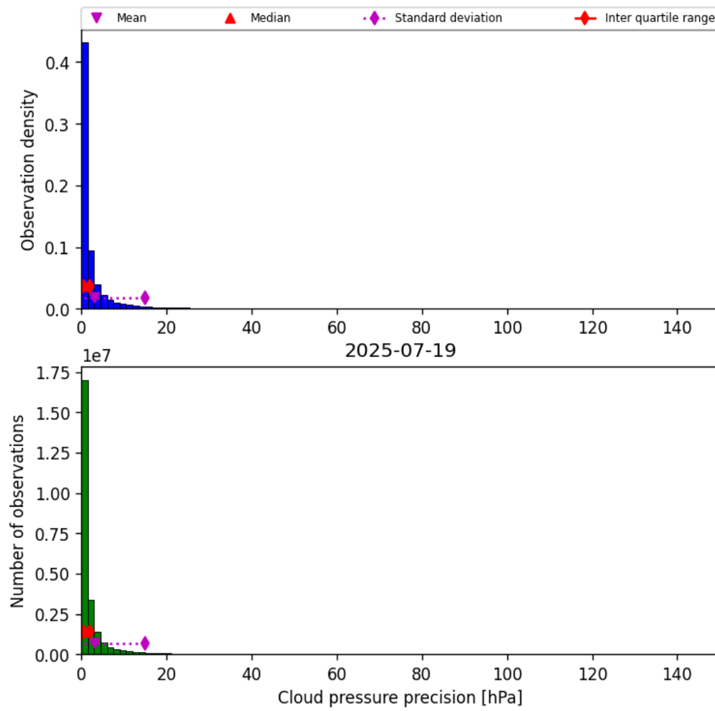
Figure 31: Histogram of “Cloud pressure precision” for 2025-07-19 to 2025-07-20
