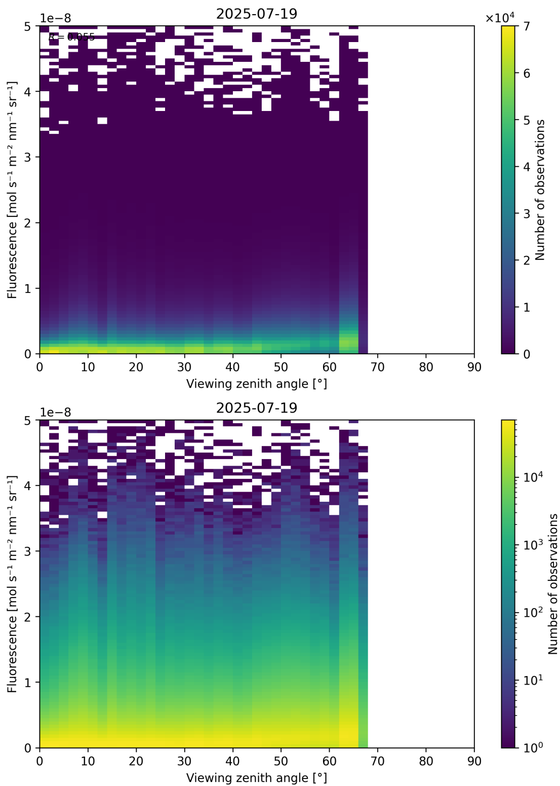
Figure 122: Scatter density plot of “Viewing zenith angle” against “Fluorescence” for 2025-07-19 to 2025-07-20.
