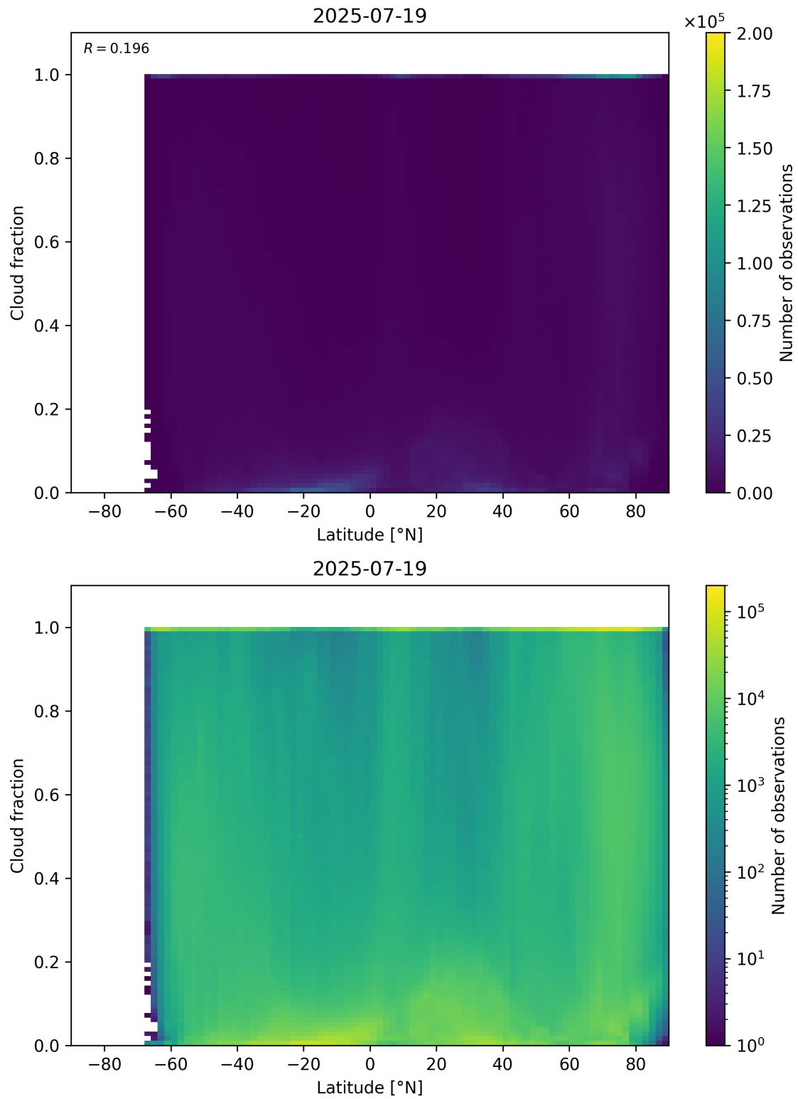
Figure 90: Scatter density plot of “Latitude” against “Cloud fraction” for 2025-07-19 to 2025-07-20.
