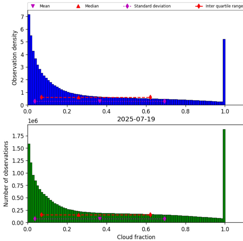
Figure 32: Histogram of “Cloud fraction” for 2025-07-19 to 2025-07-20
