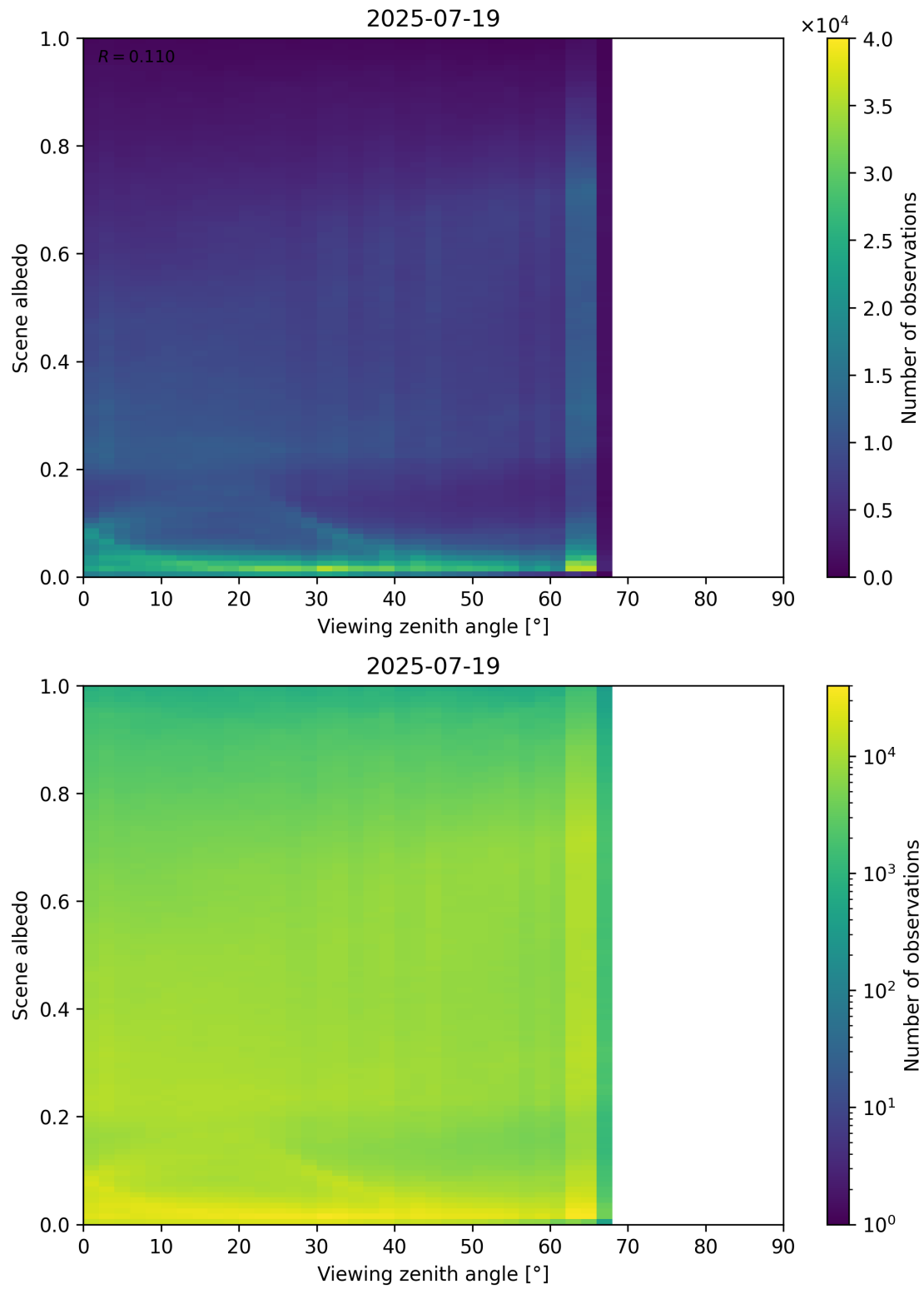
Figure 126: Scatter density plot of “Viewing zenith angle” against “Scene albedo” for 2025-07-19 to 2025-07-20.
