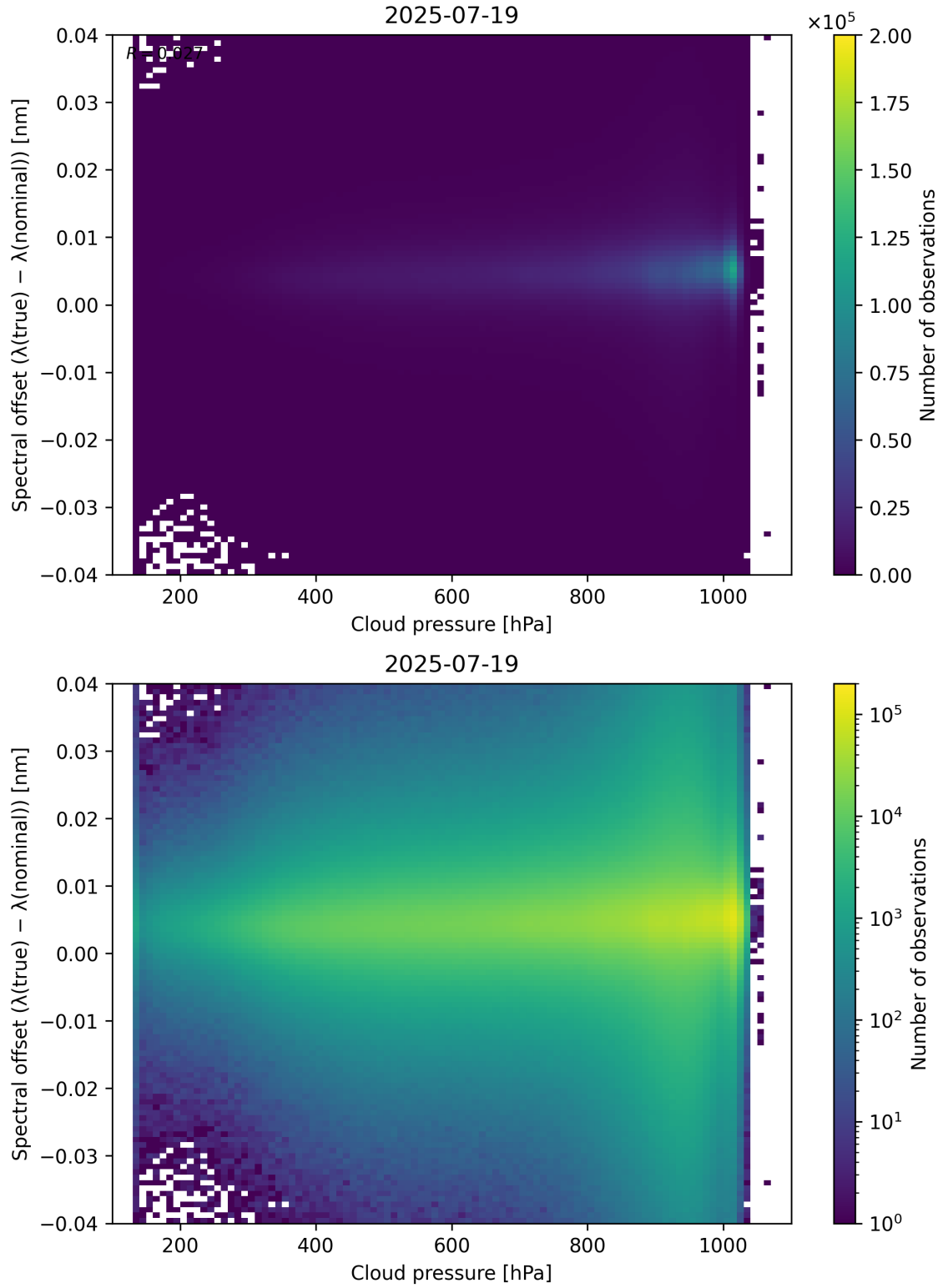
Figure 84: Scatter density plot of “Cloud pressure” against “Spectral offset ( \lambda_{\text{true}} - \lambda_{\text{nominal}} )” for 2025-07-19 to 2025-07-20.
