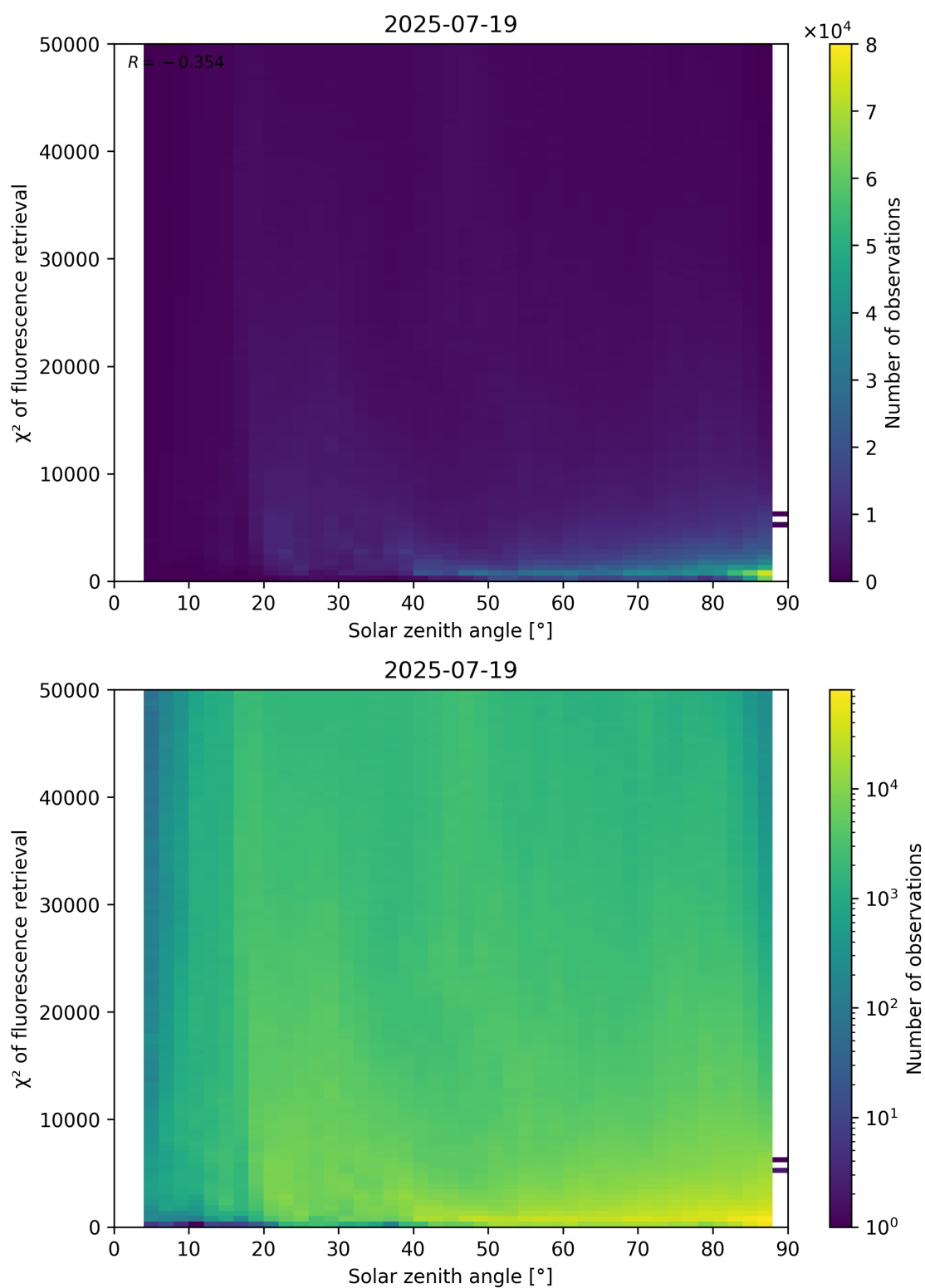
Figure 109: Scatter density plot of “Solar zenith angle” against “ \chi^2 of fluorescence retrieval” for 2025-07-19 to 2025-07-20.
