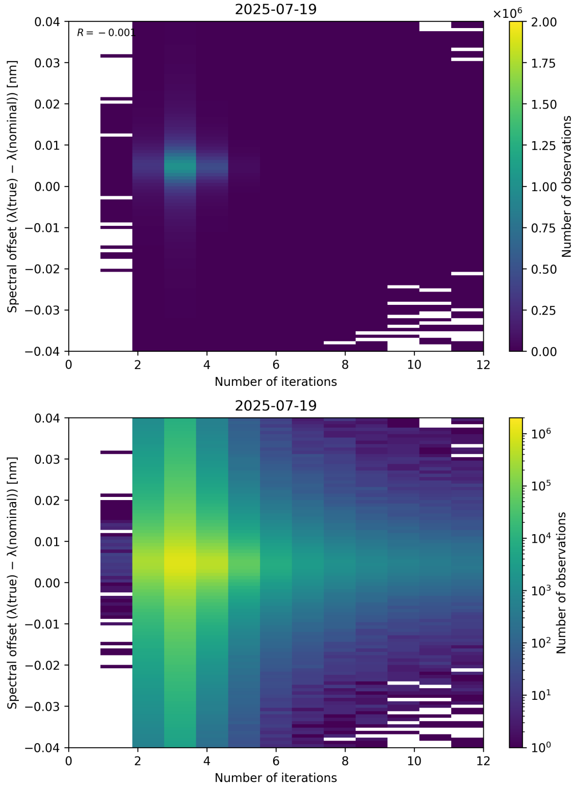
Figure 100: Scatter density plot of “Number of iterations” against “Spectral offset ( \lambda_{\text{true}} - \lambda_{\text{nominal}} )” for 2025-07-19 to 2025-07-20.
