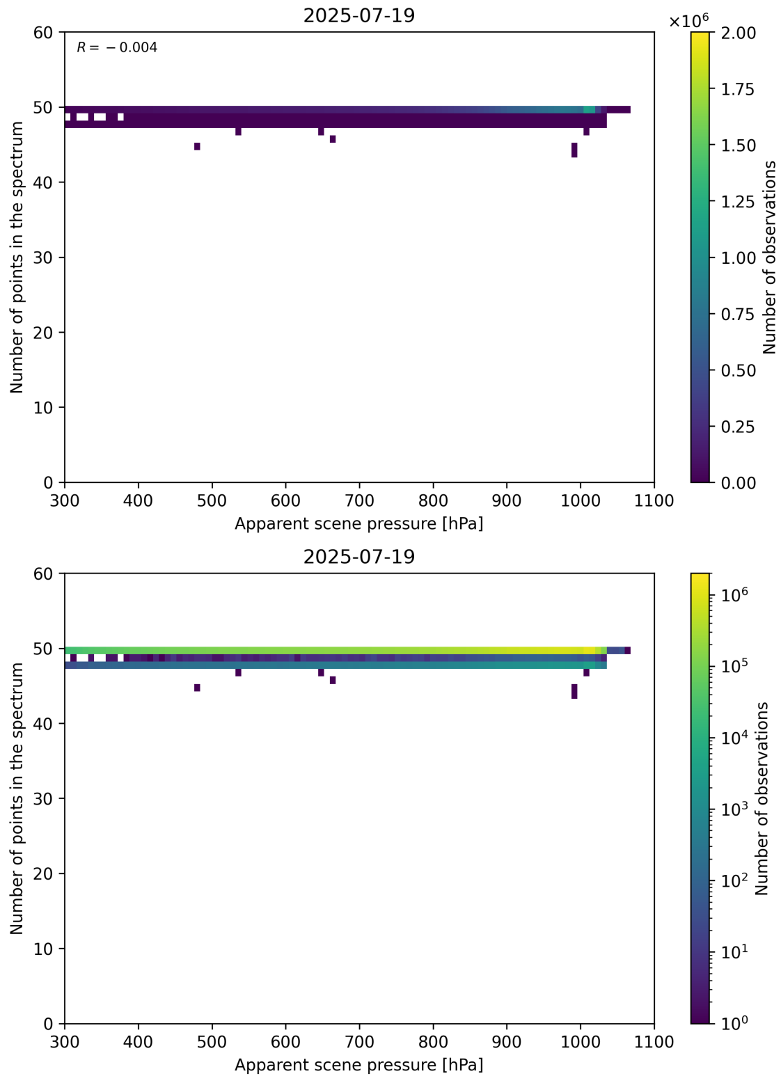
Figure 66: Scatter density plot of “Apparent scene pressure” against “Number of points in the spectrum” for 2025-07-19 to 2025-07-20.
