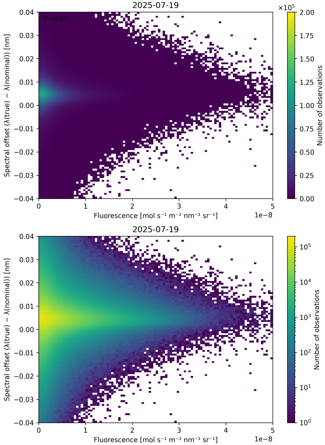
Figure 87: Scatter density plot of “Fluorescence” against “Spectral offset ( \lambda_{\text{true}} - \lambda_{\text{nominal}} )” for 2025-07-19 to 2025-07-20.
