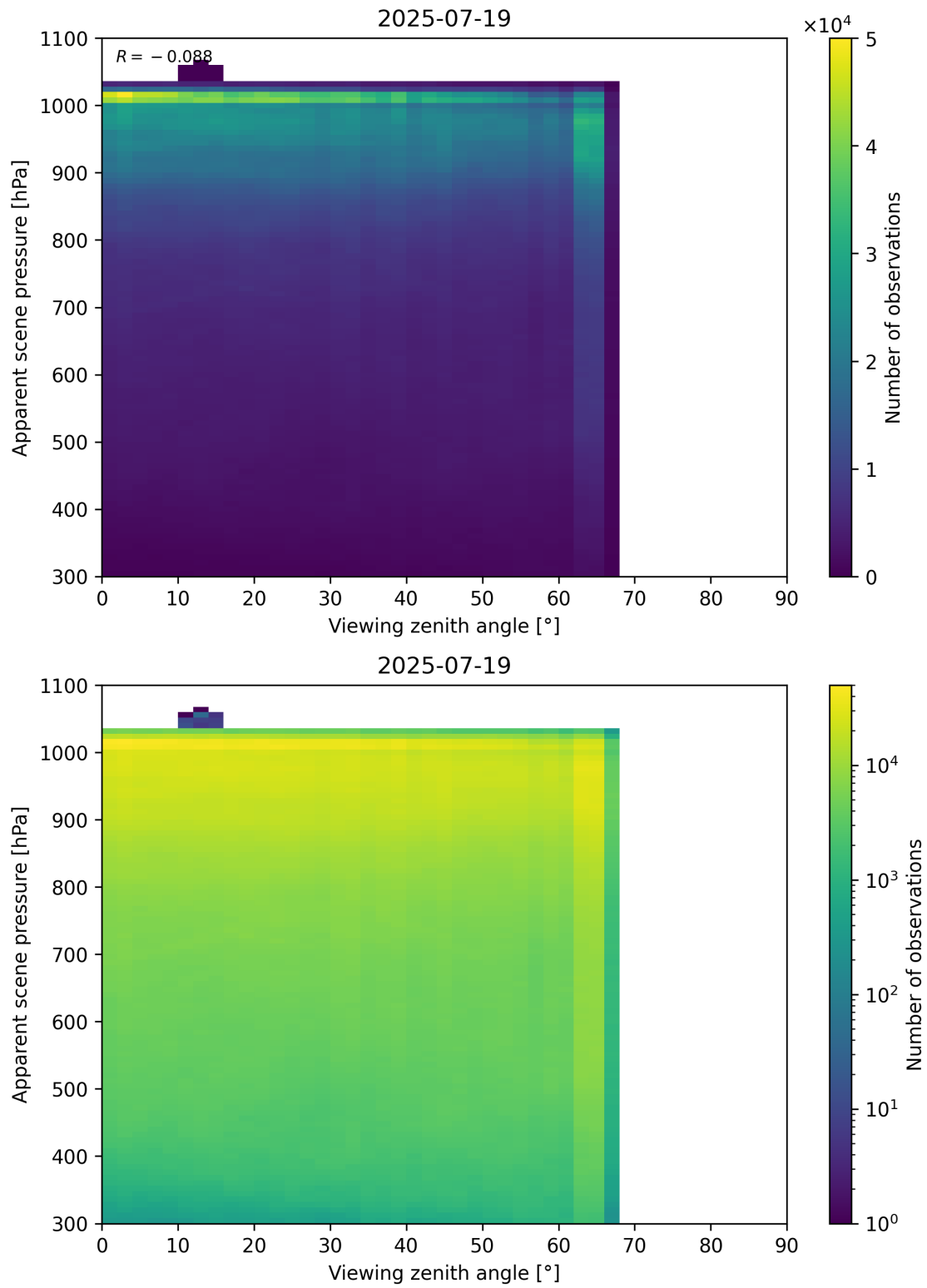
Figure 118: Scatter density plot of “Viewing zenith angle” against “Apparent scene pressure” for 2025-07-19 to 2025-07-20.
