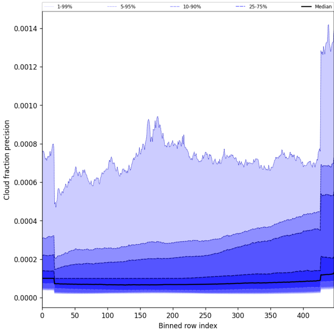
Figure 50: Along track statistics of “Cloud fraction precision” for 2025-07-19 to 2025-07-20
