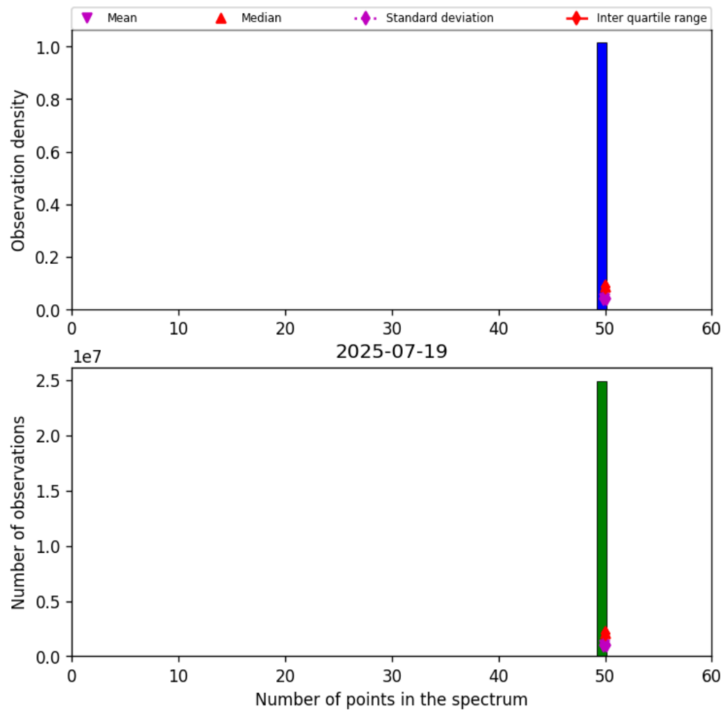
Figure 44: Histogram of “Number of points in the spectrum” for 2025-07-19 to 2025-07-20
