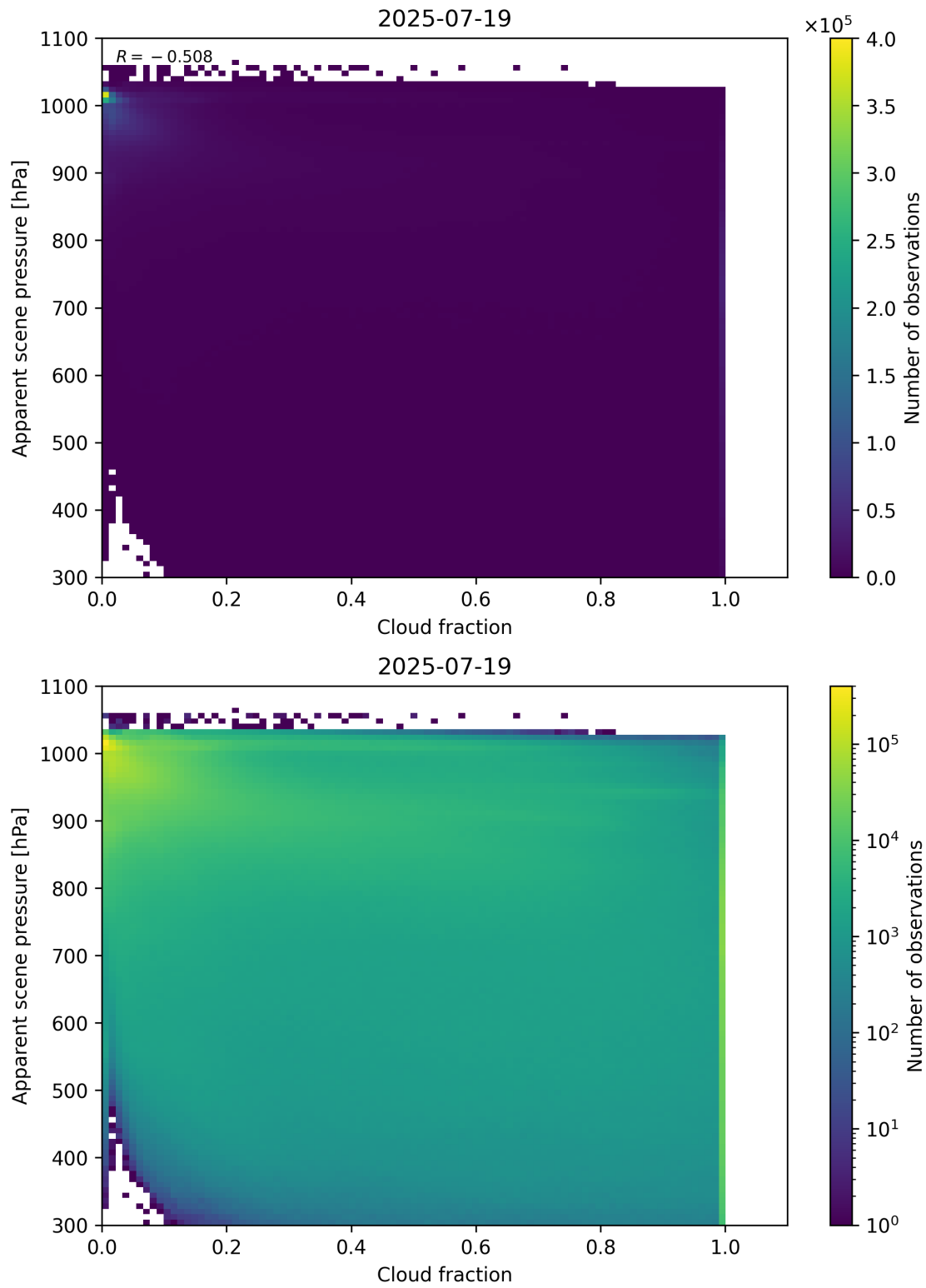
Figure 70: Scatter density plot of “Cloud fraction” against “Apparent scene pressure” for 2025-07-19 to 2025-07-20.
