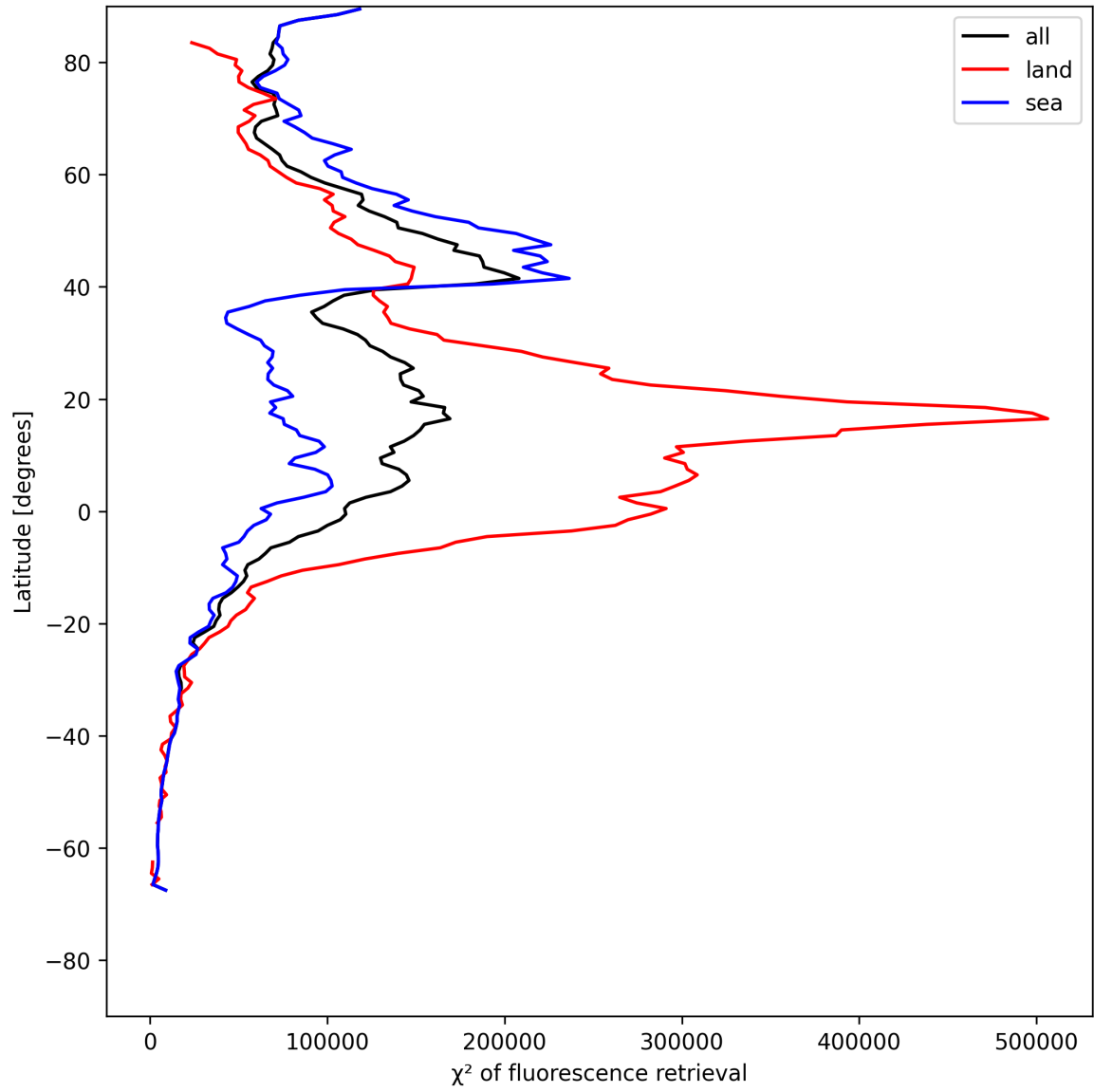
Figure 25: Zonal average of “ \chi^2 of fluorescence retrieval” for 2025-07-19 to 2025-07-20.
