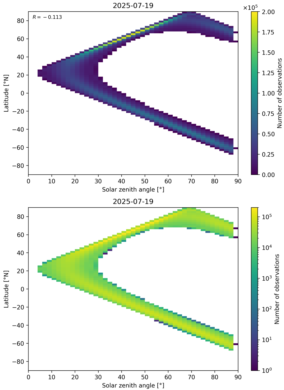
Figure 113: Scatter density plot of “Solar zenith angle” against “Latitude” for 2025-07-19 to 2025-07-20.
