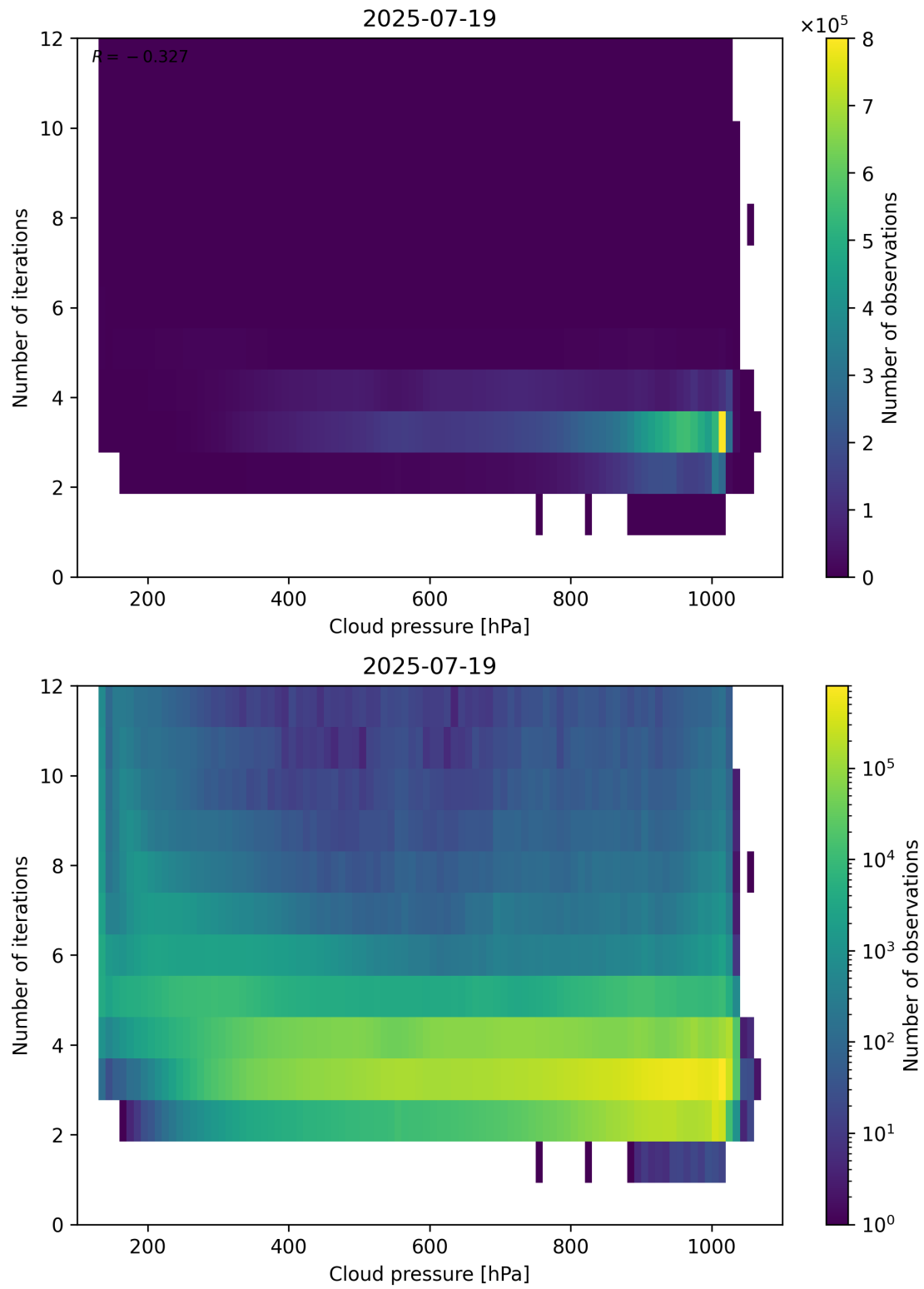
Figure 81: Scatter density plot of “Cloud pressure” against “Number of iterations” for 2025-07-19 to 2025-07-20.
