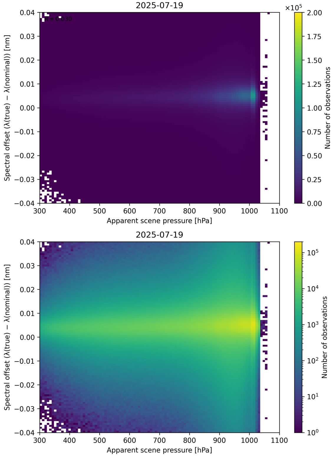
Figure 67: Scatter density plot of “Apparent scene pressure” against “Spectral offset ( \lambda_{\text{true}} - \lambda_{\text{nominal}} )” for 2025-07-19 to 2025-07-20.
