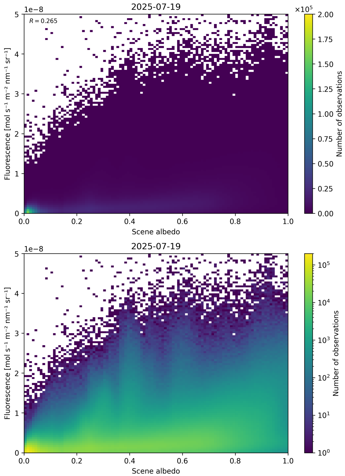
Figure 104: Scatter density plot of “Scene albedo” against “Fluorescence” for 2025-07-19 to 2025-07-20.
