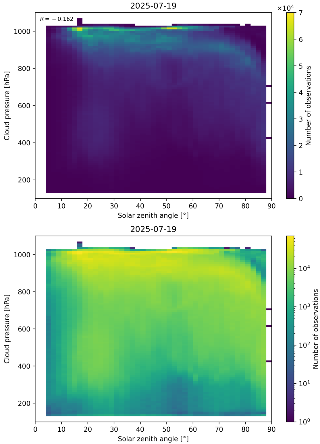
Figure 111: Scatter density plot of “Solar zenith angle” against “Cloud pressure” for 2025-07-19 to 2025-07-20.
