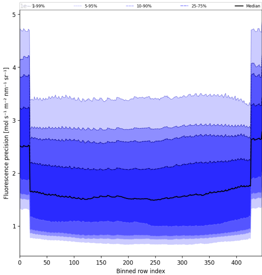
Figure 58: Along track statistics of “Fluorescence precision” for 2025-07-19 to 2025-07-20
