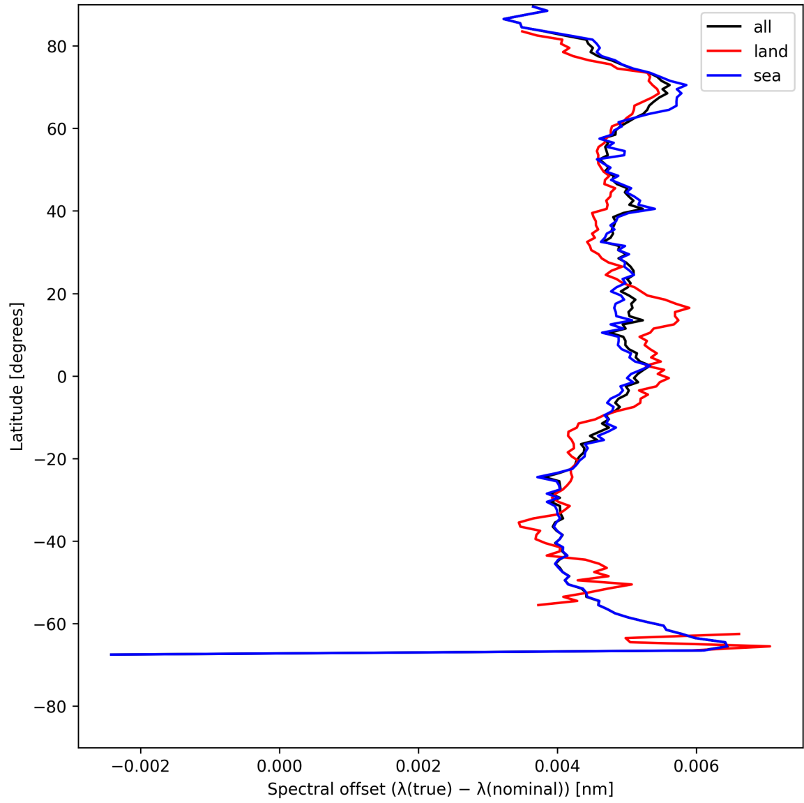
Figure 28: Zonal average of “Spectral offset ( \lambda_{\text{true}} - \lambda_{\text{nominal}} )” for 2025-07-19 to 2025-07-20.
