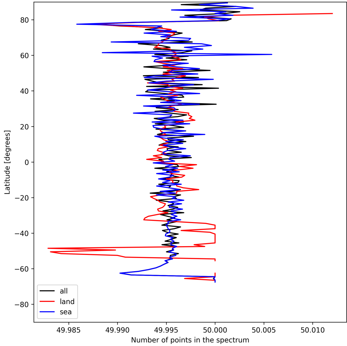
Figure 27: Zonal average of “Number of points in the spectrum” for 2025-07-19 to 2025-07-20.
