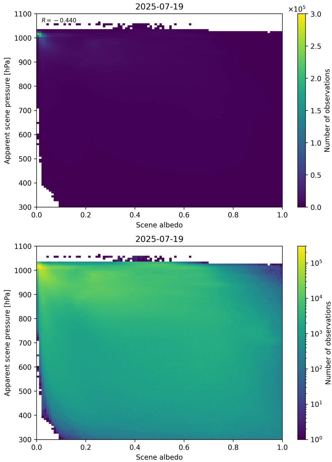
Figure 102: Scatter density plot of “Scene albedo” against “Apparent scene pressure” for 2025-07-19 to 2025-07-20.
