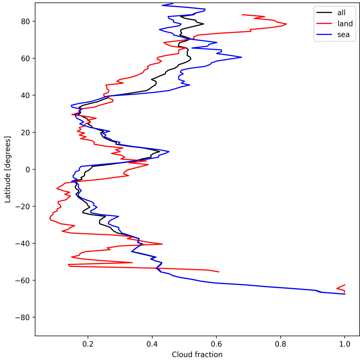
Figure 15: Zonal average of “Cloud fraction” for 2025-07-19 to 2025-07-20.
