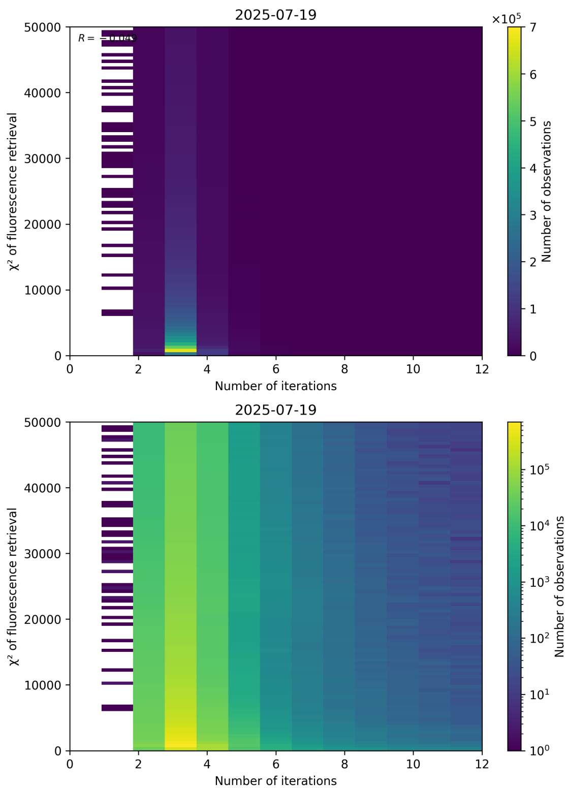
Figure 97: Scatter density plot of “Number of iterations” against “ \chi^2 of fluorescence retrieval” for 2025-07-19 to 2025-07-20.
