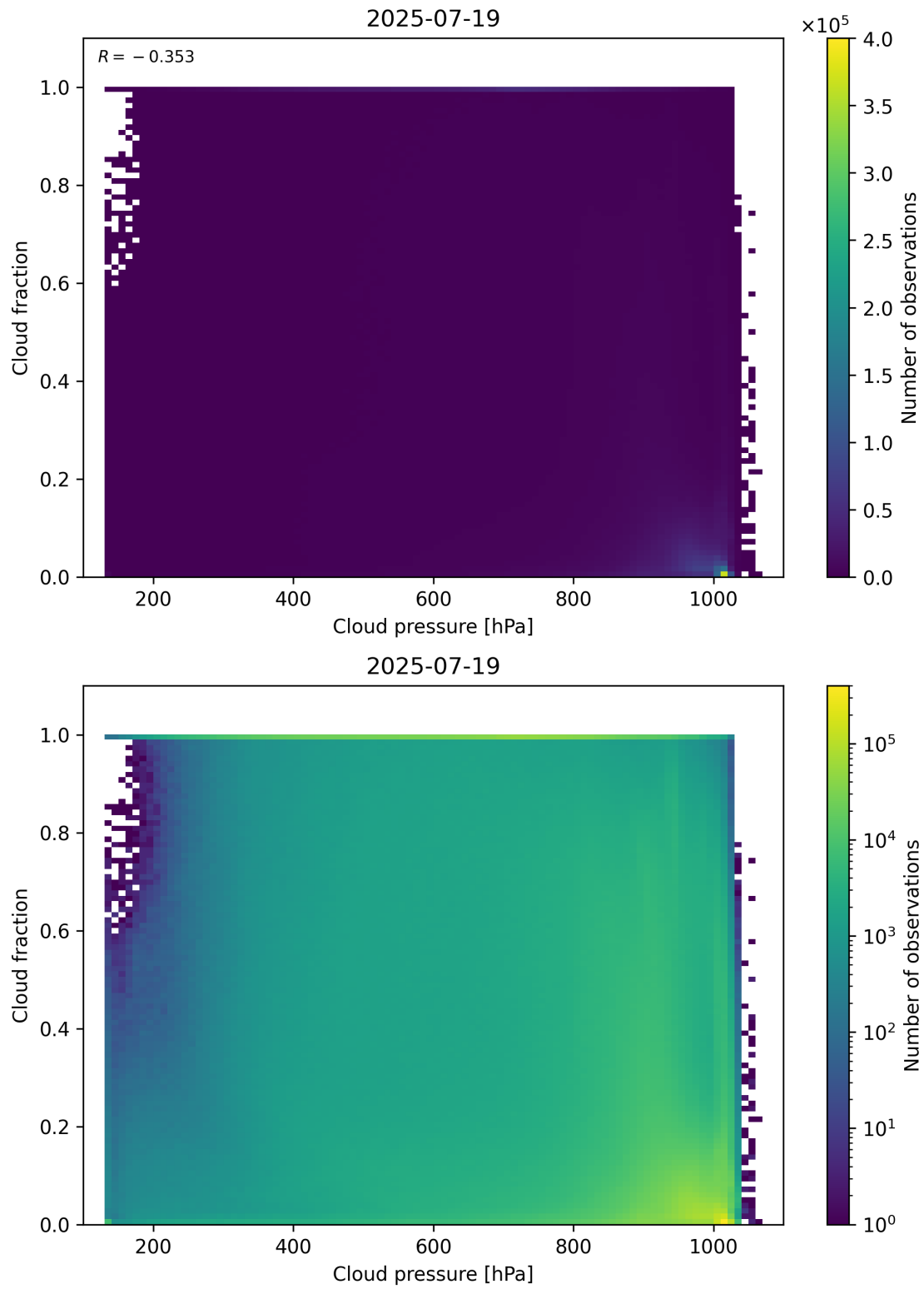
Figure 79: Scatter density plot of “Cloud pressure” against “Cloud fraction” for 2025-07-19 to 2025-07-20.
