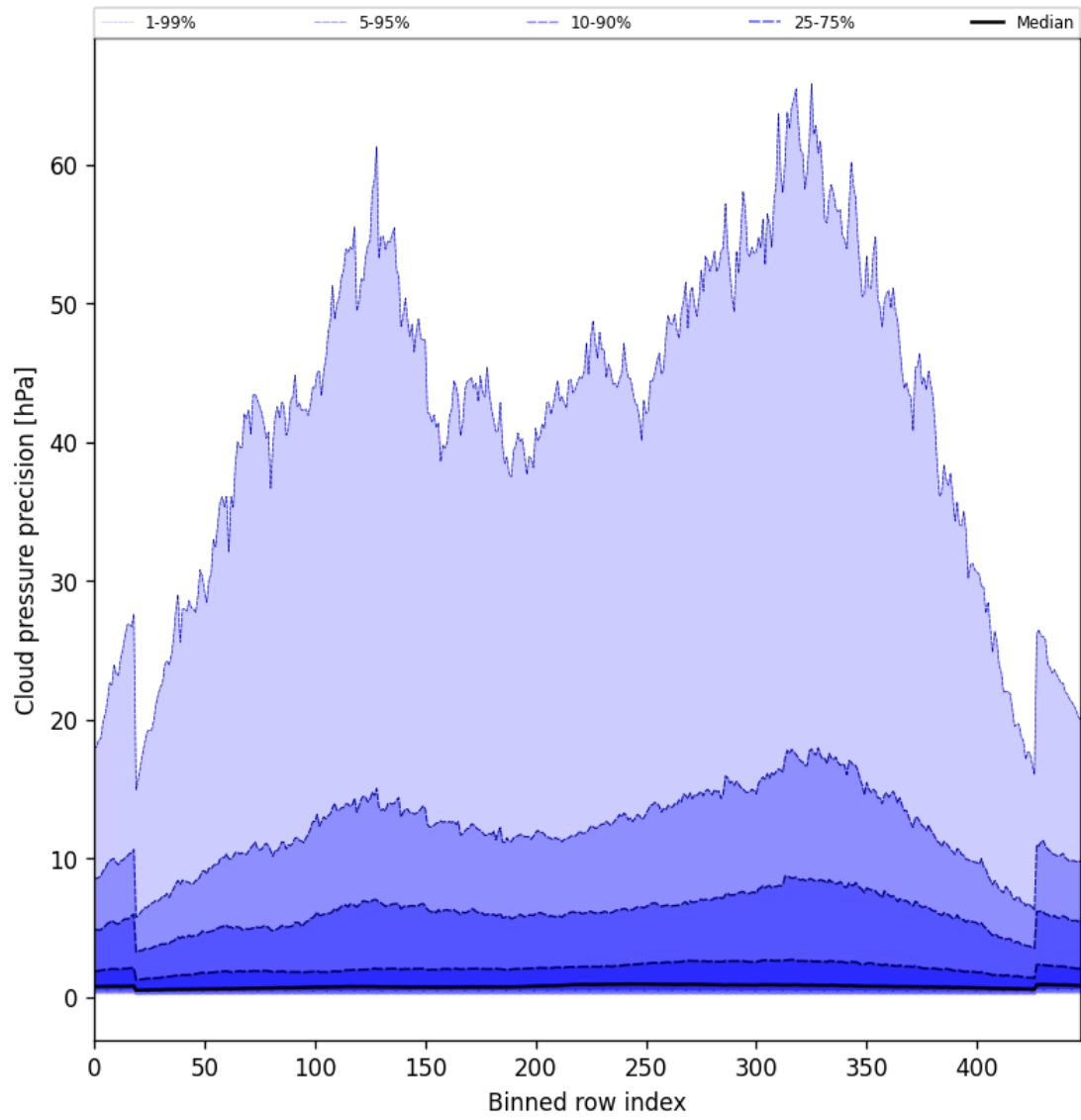
Figure 48: Along track statistics of “Cloud pressure precision” for 2025-07-19 to 2025-07-20
