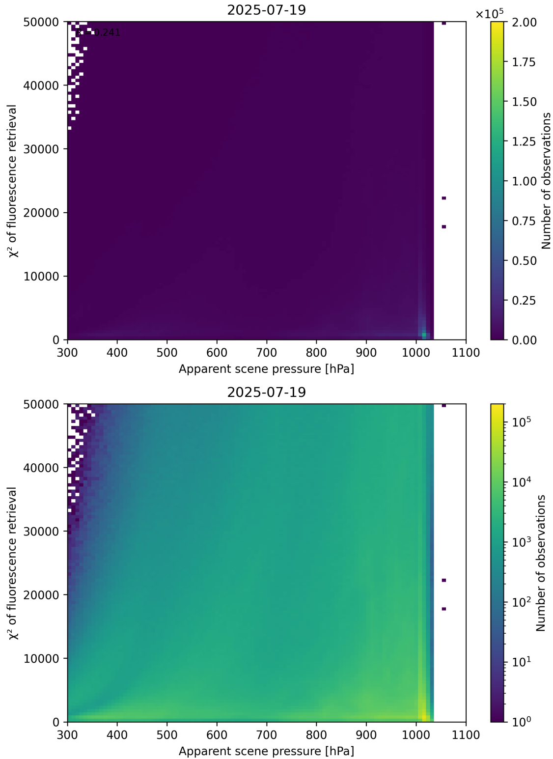
Figure 63: Scatter density plot of “Apparent scene pressure” against “ \chi^2 of fluorescence retrieval” for 2025-07-19 to 2025-07-20.
