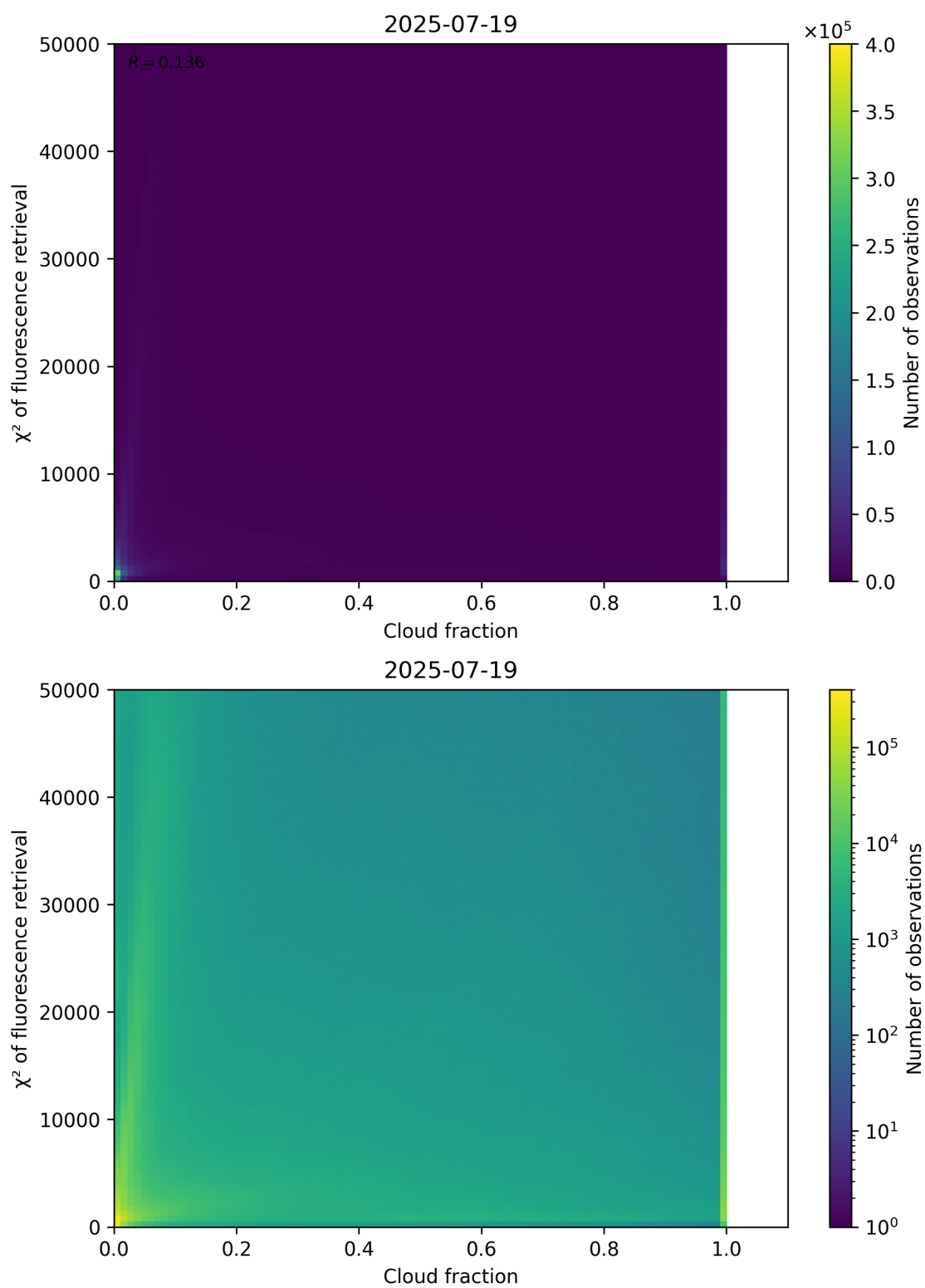
Figure 71: Scatter density plot of “Cloud fraction” against “ \chi^2 of fluorescence retrieval” for 2025-07-19 to 2025-07-20.
