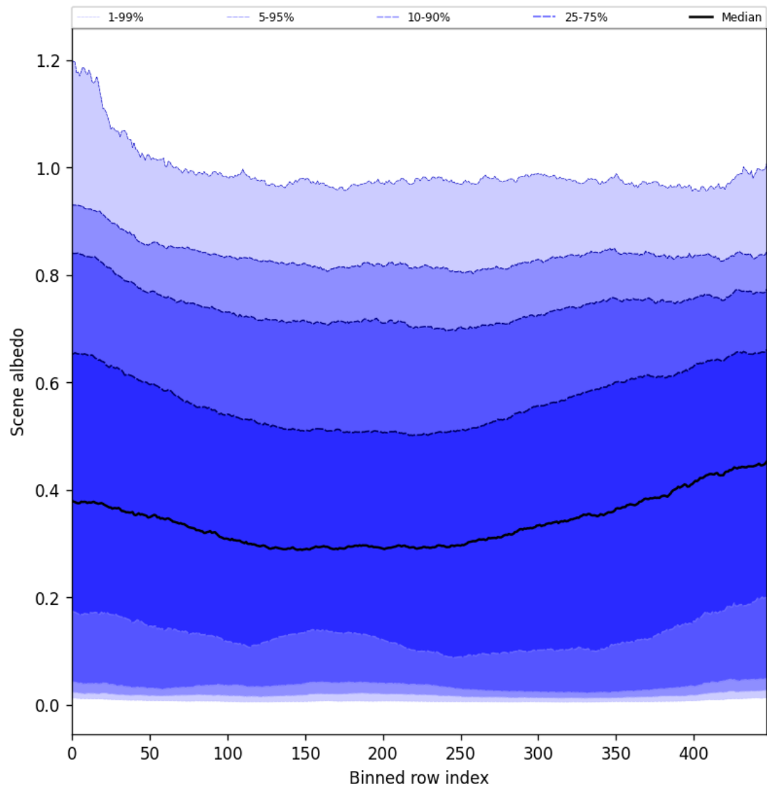
Figure 51: Along track statistics of “Scene albedo” for 2025-07-19 to 2025-07-20
