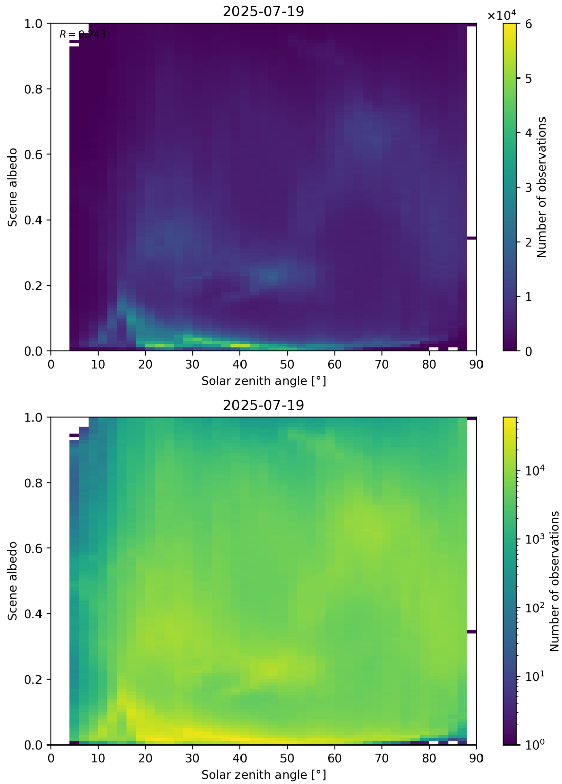
Figure 116: Scatter density plot of “Solar zenith angle” against “Scene albedo” for 2025-07-19 to 2025-07-20.
