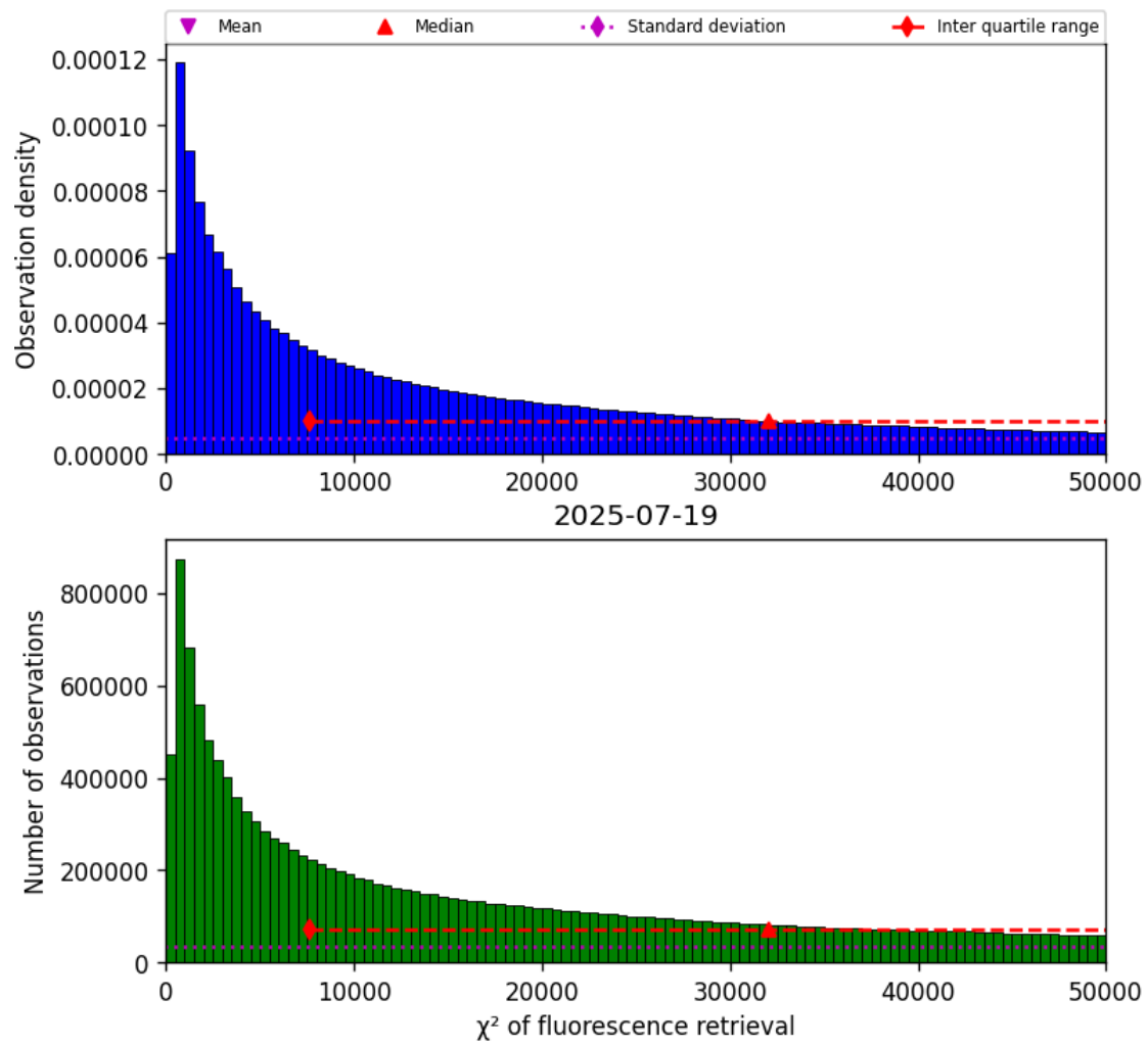
Figure 42: Histogram of “ \chi^2 of fluorescence retrieval” for 2025-07-19 to 2025-07-20
