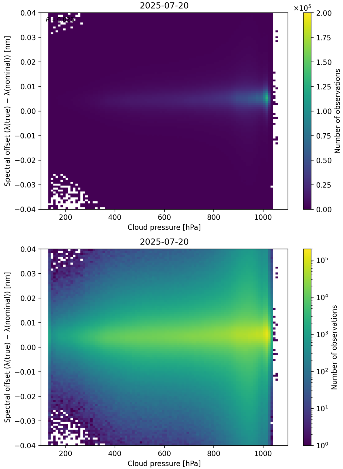
Figure 84: Scatter density plot of “Cloud pressure” against “Spectral offset ( \lambda_{\text{true}} - \lambda_{\text{nominal}} )” for 2025-07-19 to 2025-07-21.
