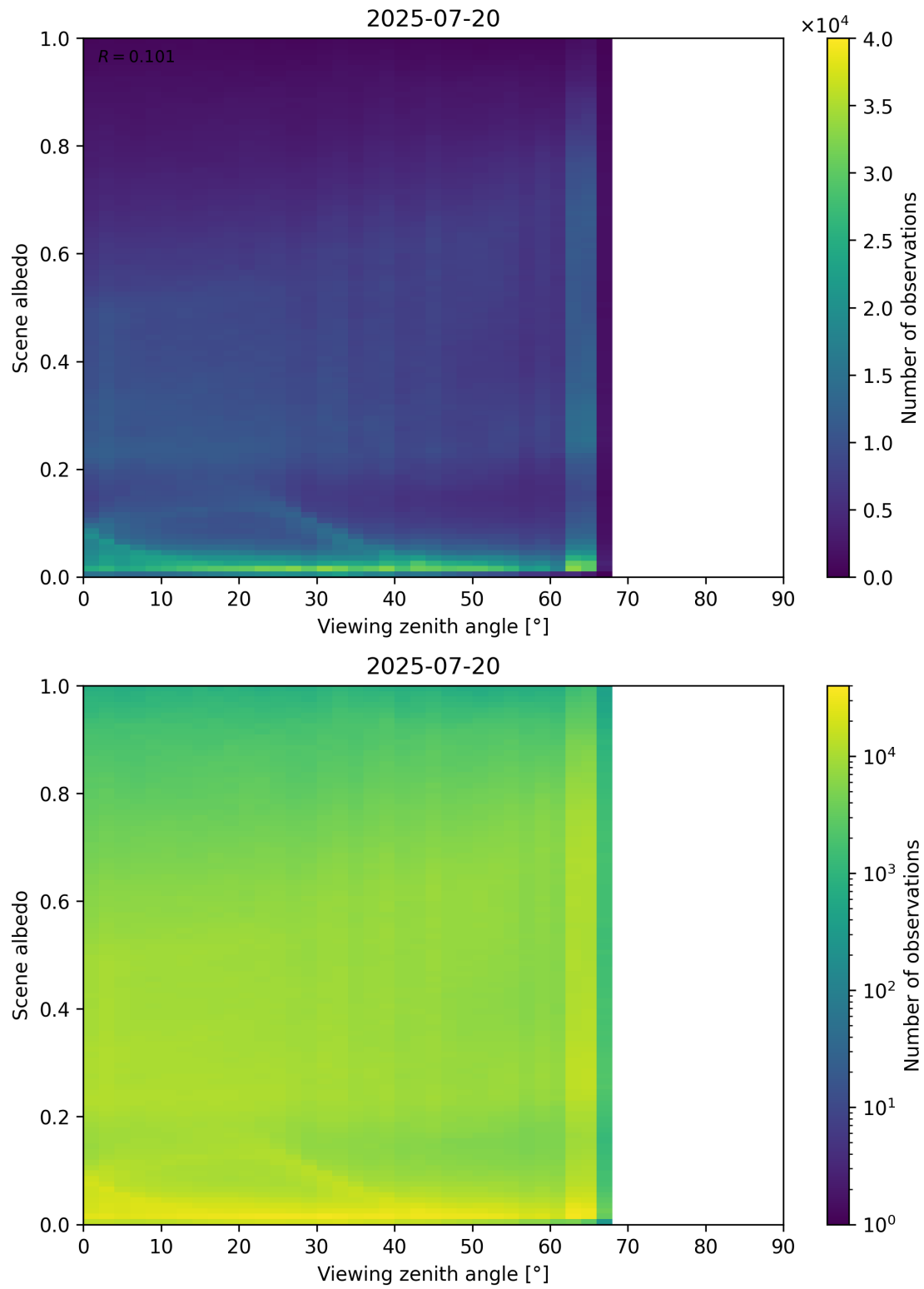
Figure 126: Scatter density plot of “Viewing zenith angle” against “Scene albedo” for 2025-07-19 to 2025-07-21.
