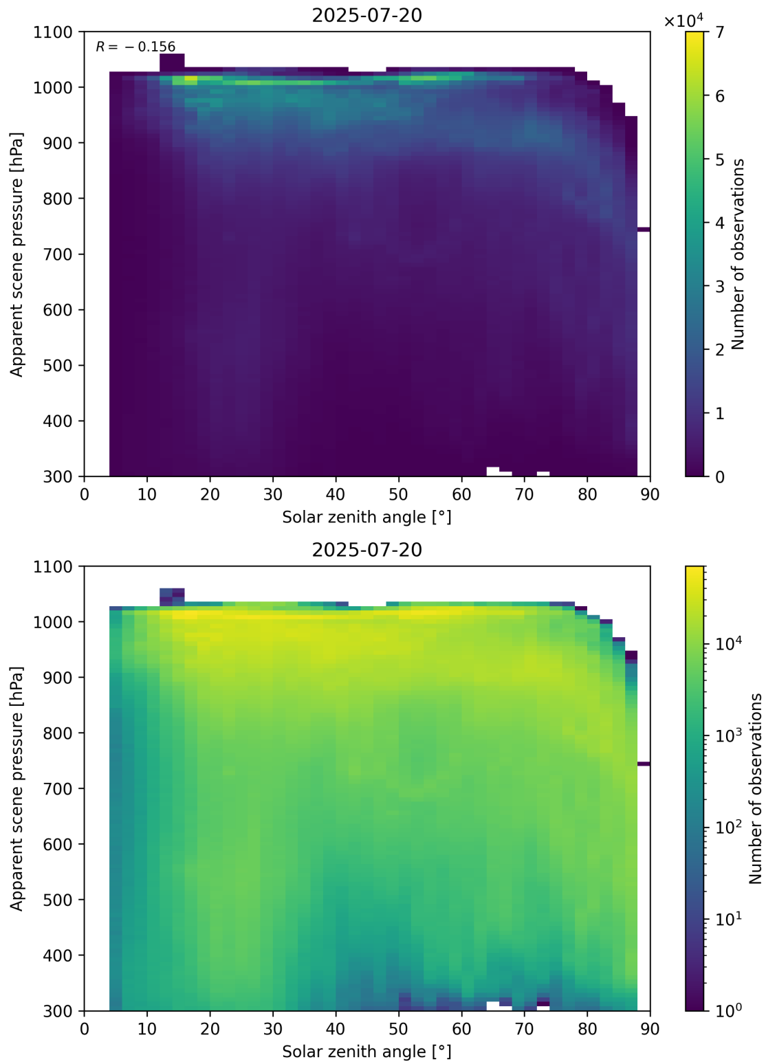
Figure 108: Scatter density plot of “Solar zenith angle” against “Apparent scene pressure” for 2025-07-19 to 2025-07-21.
