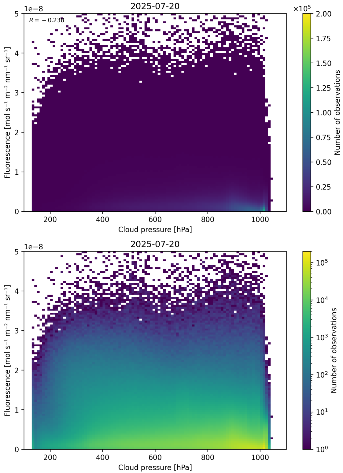
Figure 80: Scatter density plot of “Cloud pressure” against “Fluorescence” for 2025-07-19 to 2025-07-21.
