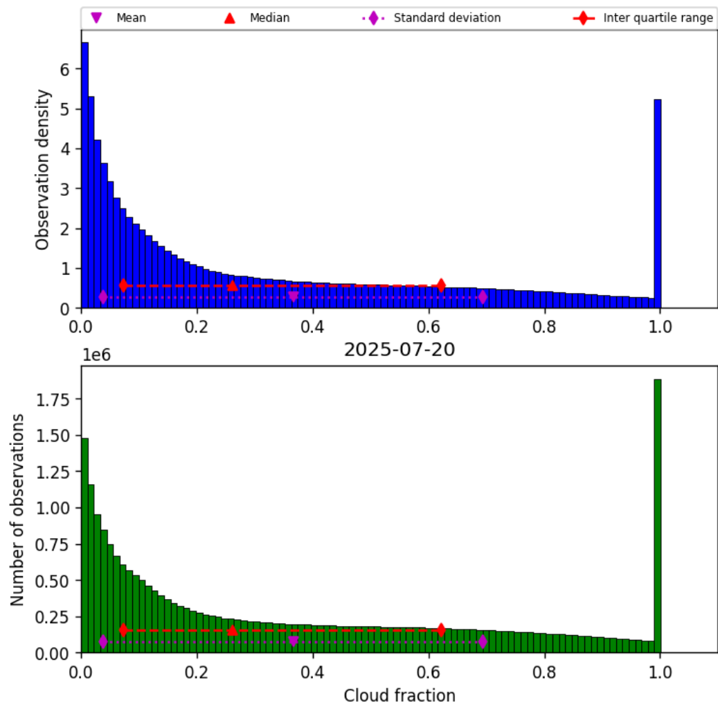
Figure 32: Histogram of “Cloud fraction” for 2025-07-19 to 2025-07-21
