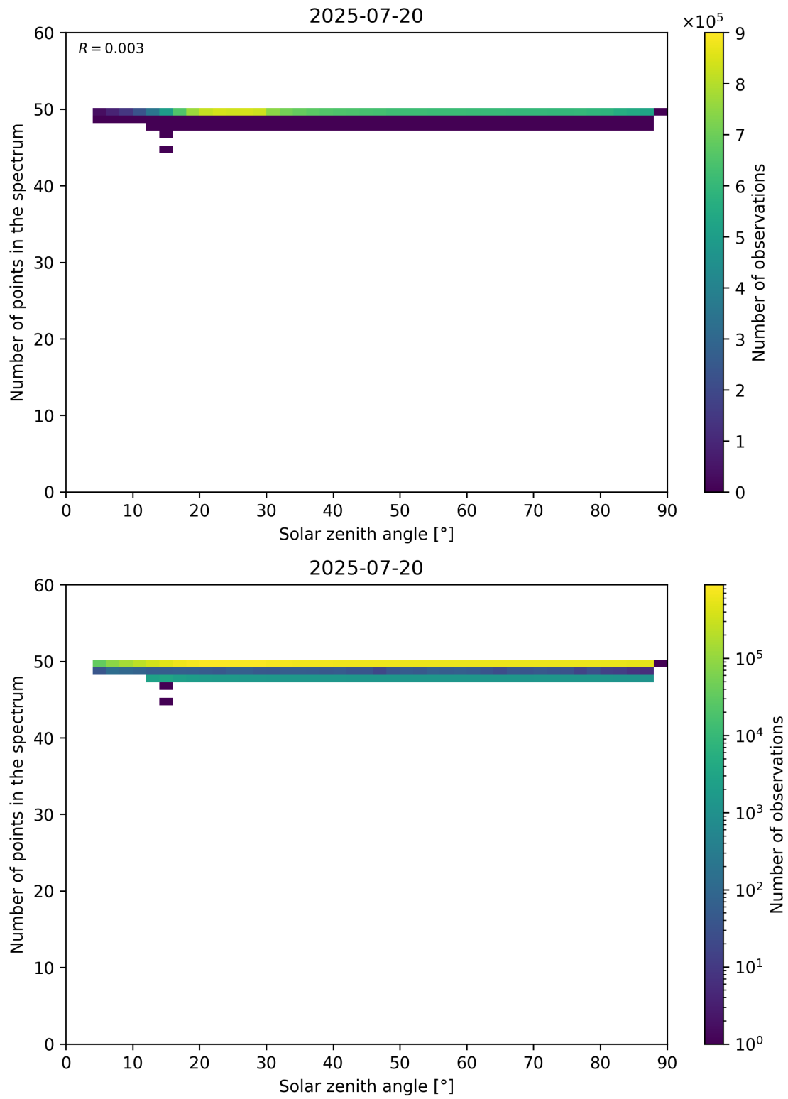
Figure 115: Scatter density plot of “Solar zenith angle” against “Number of points in the spectrum” for 2025-07-19 to 2025-07-21.
