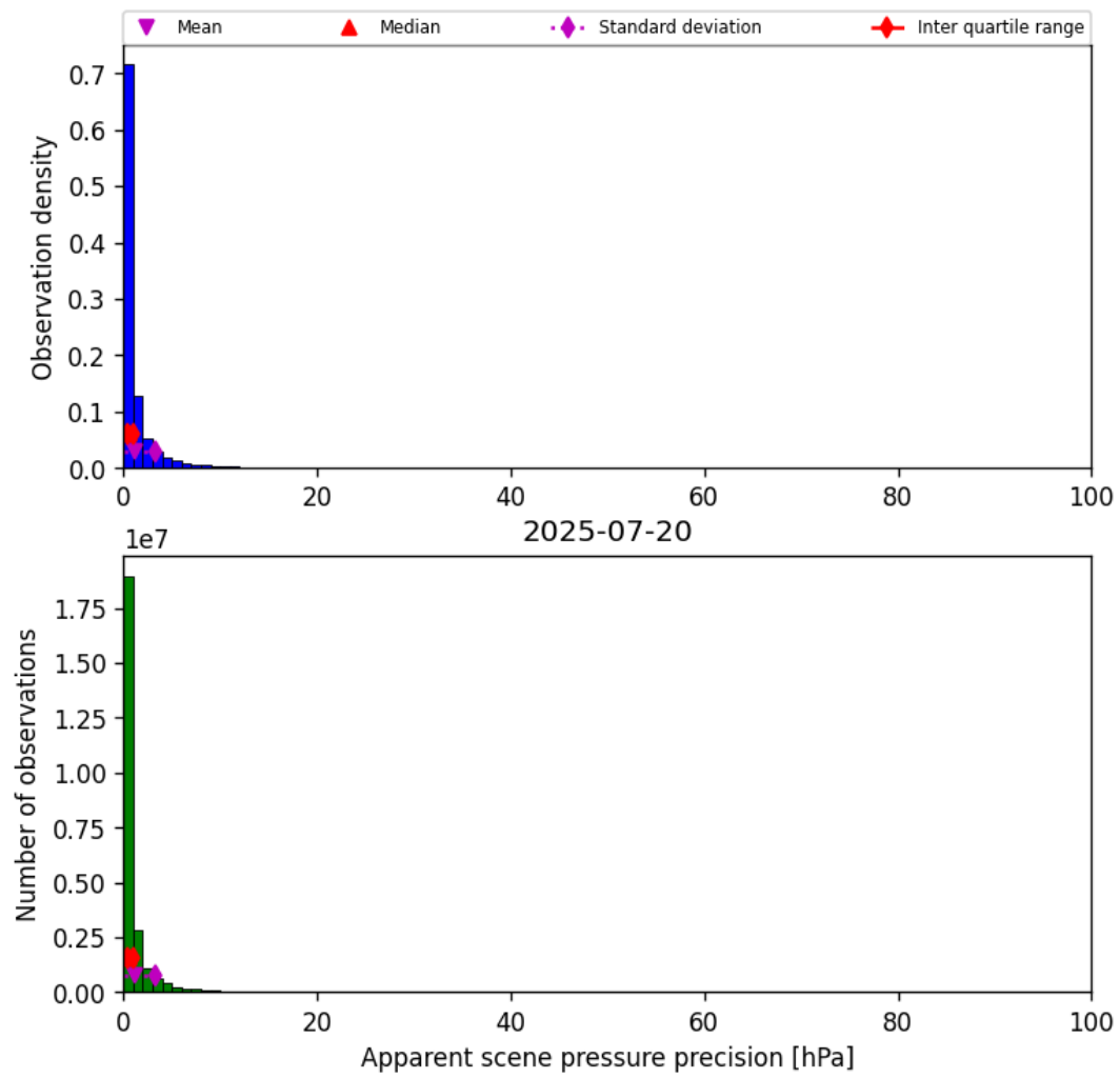
Figure 37: Histogram of “Apparent scene pressure precision” for 2025-07-19 to 2025-07-21
