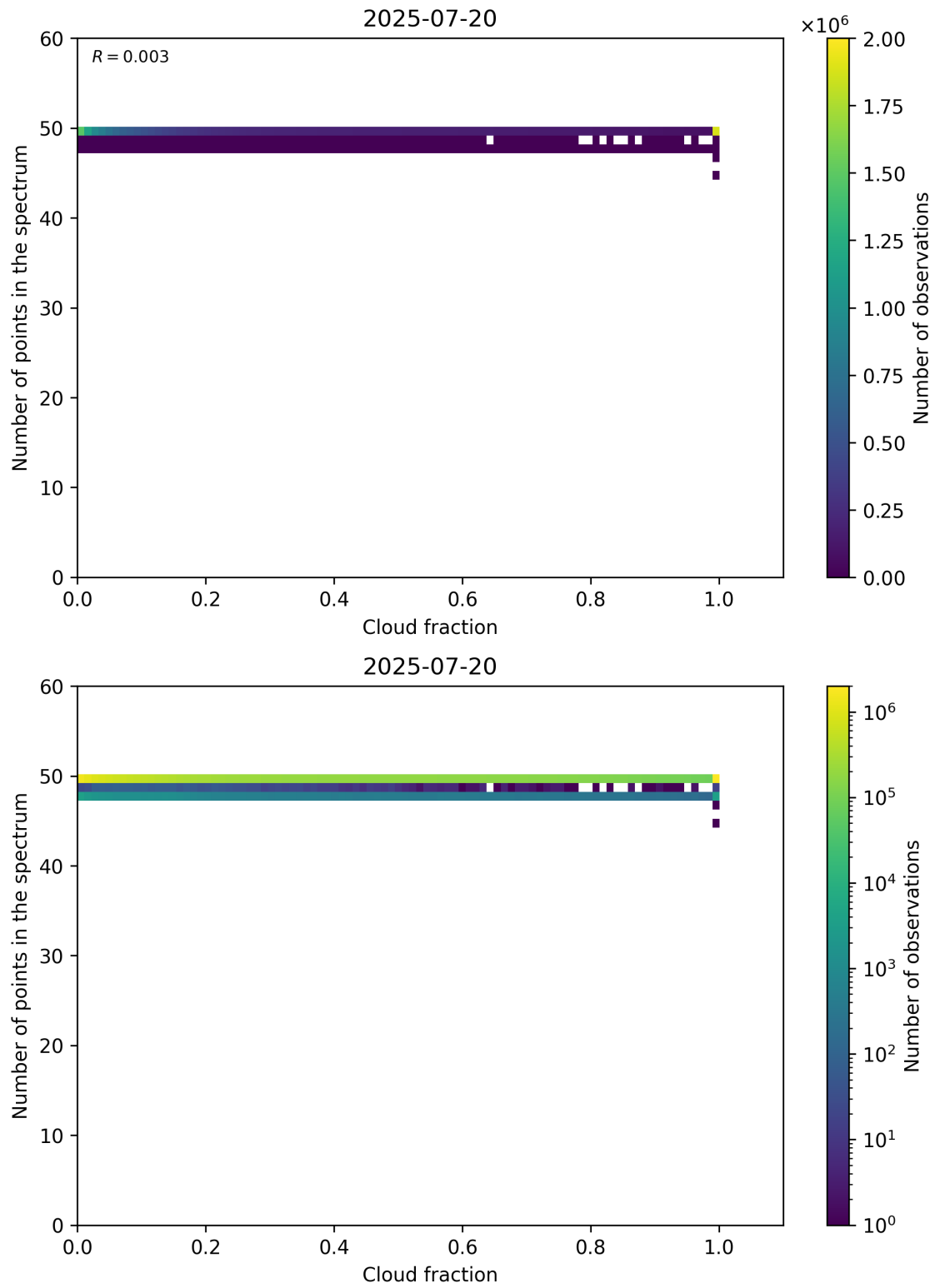
Figure 74: Scatter density plot of “Cloud fraction” against “Number of points in the spectrum” for 2025-07-19 to 2025-07-21.
