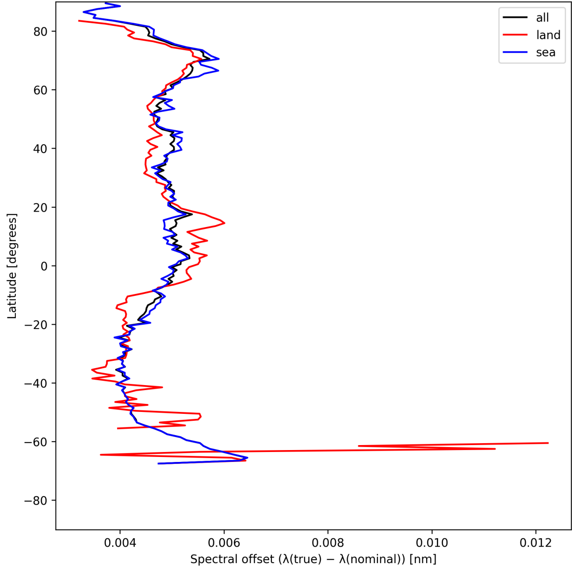
Figure 28: Zonal average of “Spectral offset ( \lambda_{\text{true}} - \lambda_{\text{nominal}} )” for 2025-07-19 to 2025-07-21.
