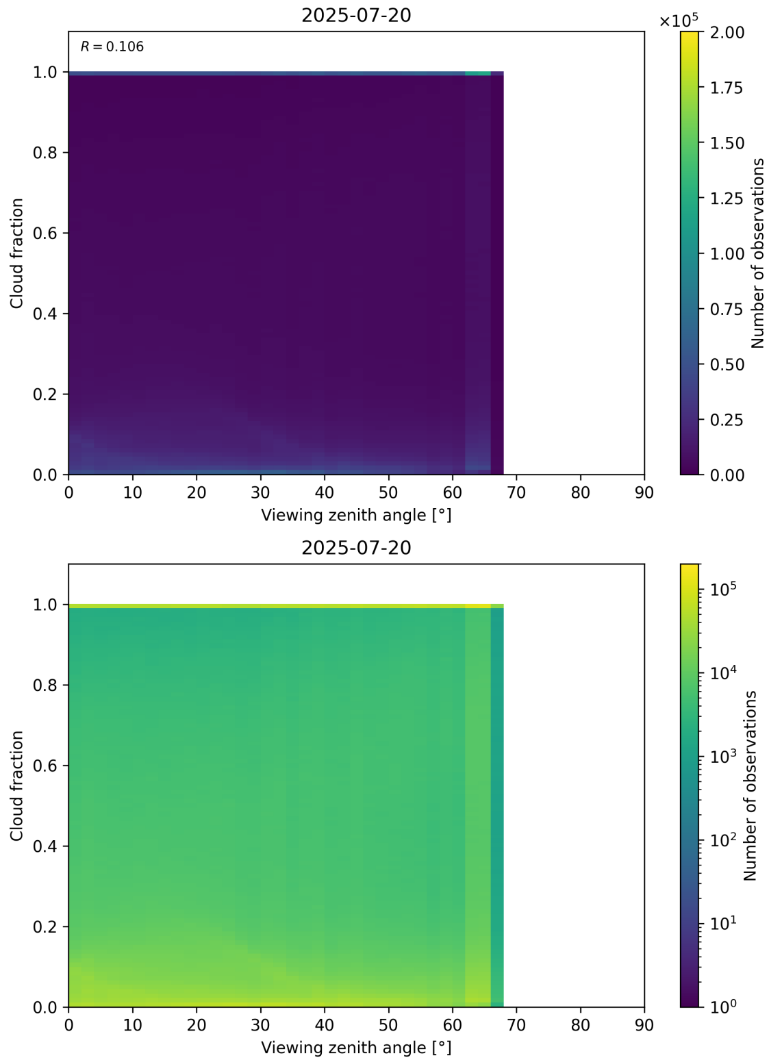
Figure 120: Scatter density plot of “Viewing zenith angle” against “Cloud fraction” for 2025-07-19 to 2025-07-21.
