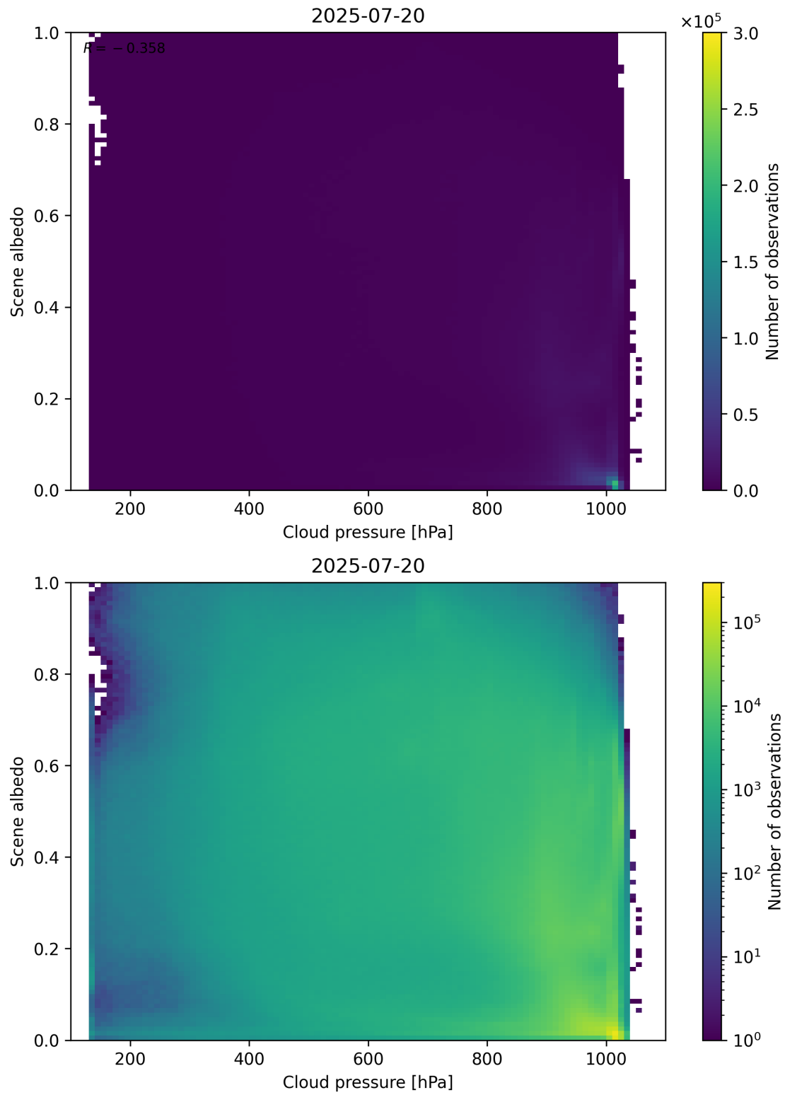
Figure 83: Scatter density plot of “Cloud pressure” against “Scene albedo” for 2025-07-19 to 2025-07-21.
