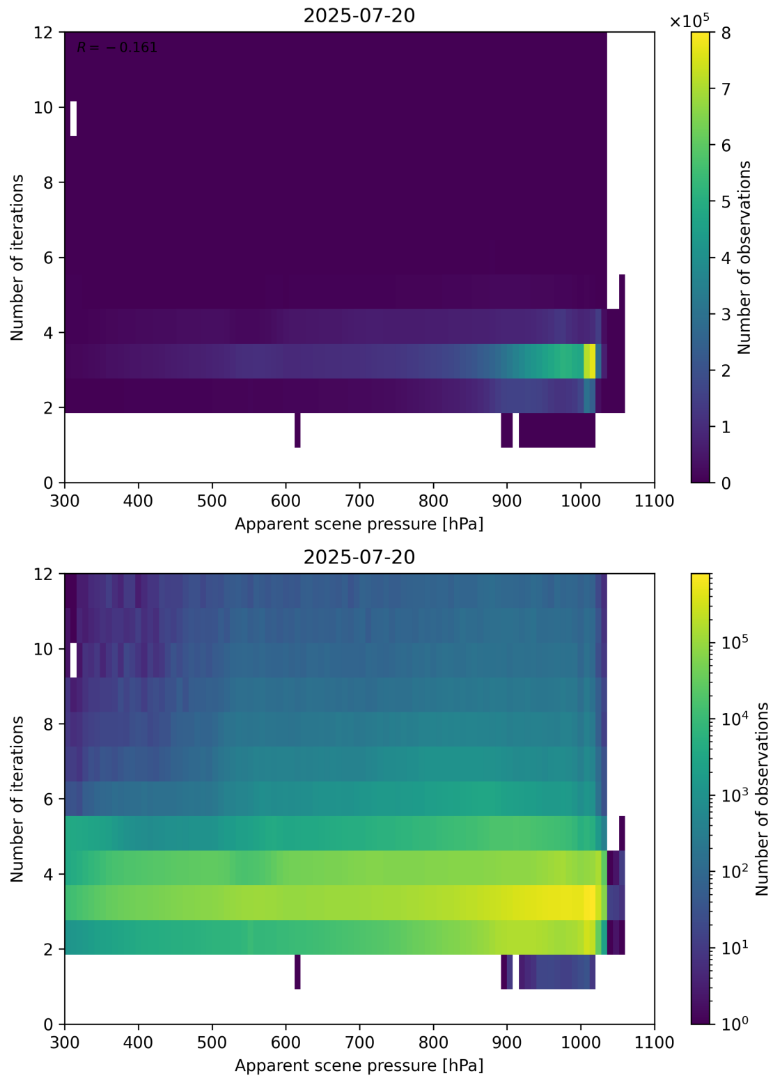
Figure 65: Scatter density plot of “Apparent scene pressure” against “Number of iterations” for 2025-07-19 to 2025-07-21.
