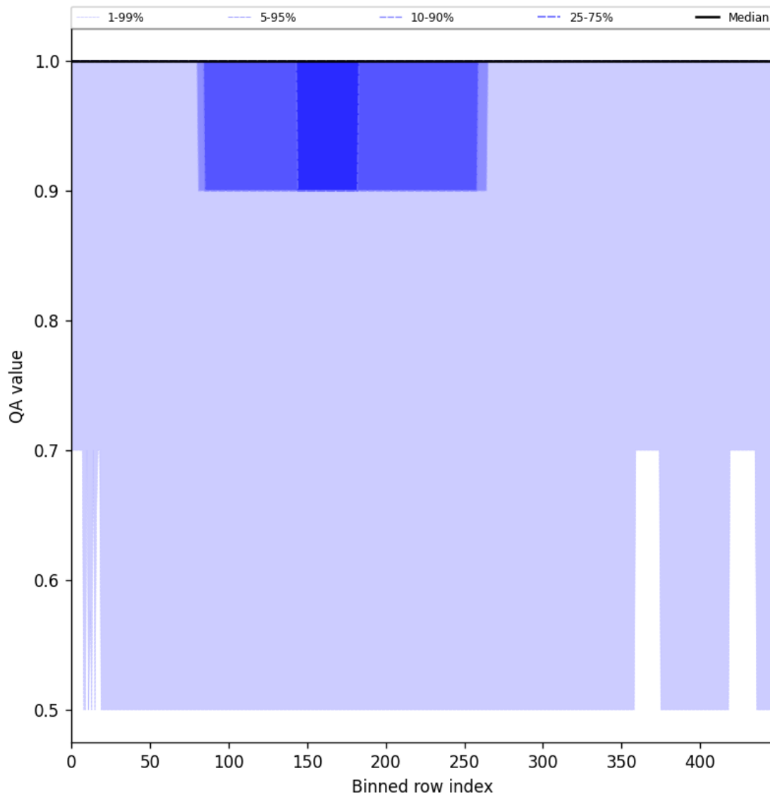
Figure 46: Along track statistics of “QA value” for 2025-07-19 to 2025-07-21
