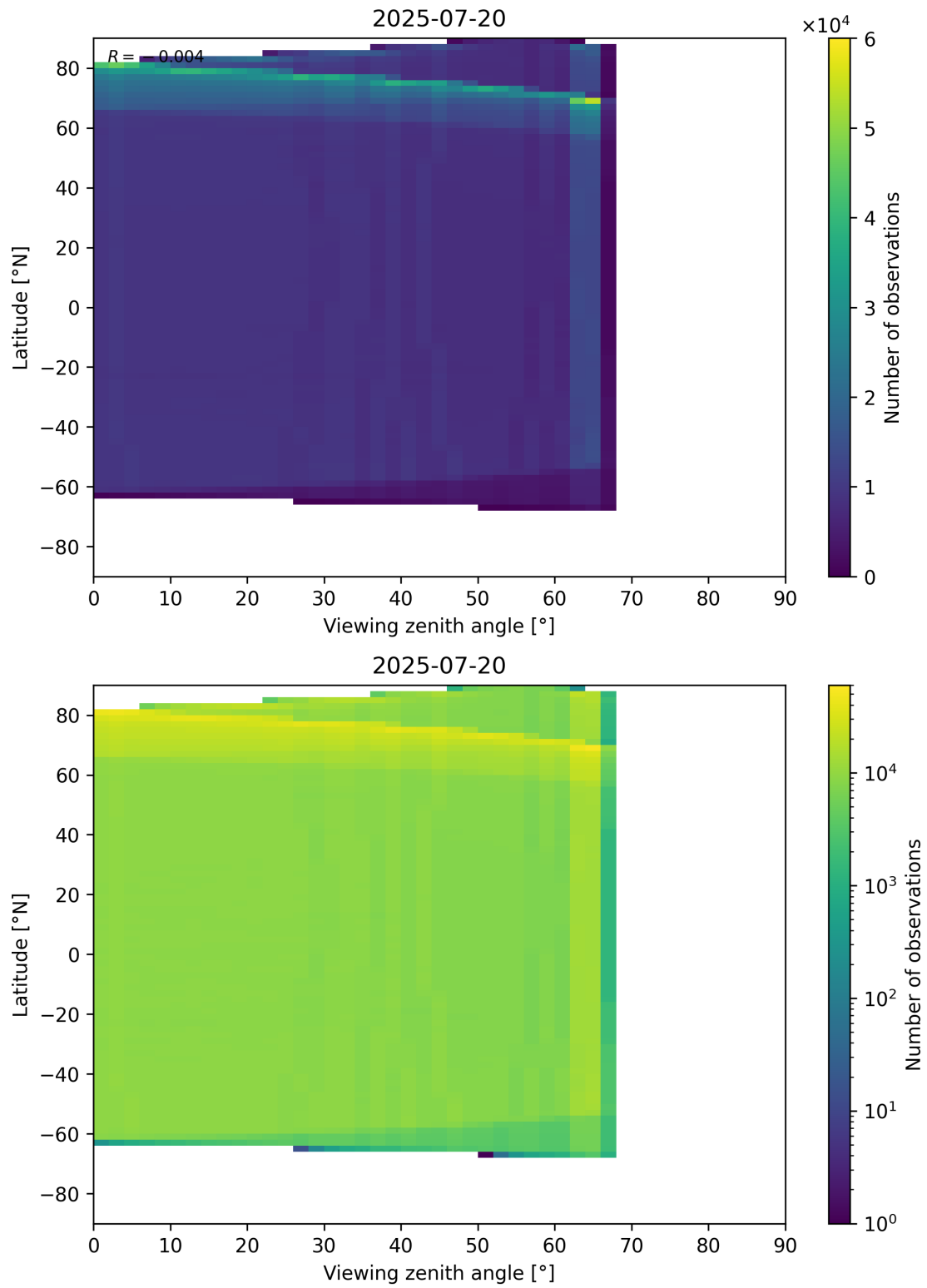
Figure 123: Scatter density plot of “Viewing zenith angle” against “Latitude” for 2025-07-19 to 2025-07-21.
