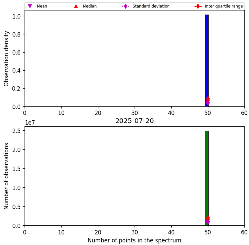
Figure 44: Histogram of “Number of points in the spectrum” for 2025-07-19 to 2025-07-21
