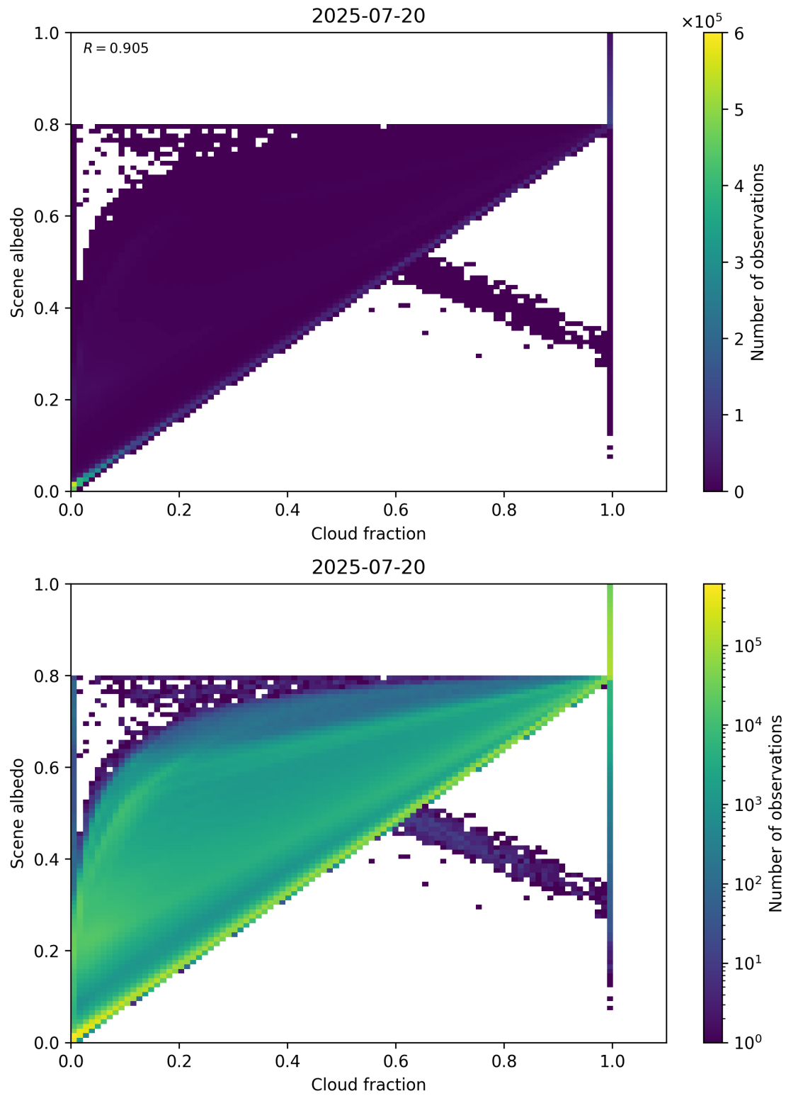
Figure 75: Scatter density plot of “Cloud fraction” against “Scene albedo” for 2025-07-19 to 2025-07-21.
