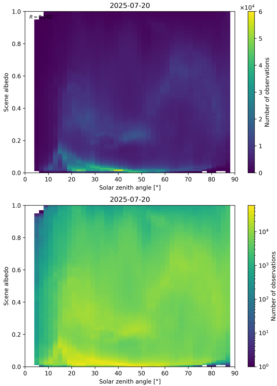
Figure 116: Scatter density plot of “Solar zenith angle” against “Scene albedo” for 2025-07-19 to 2025-07-21.
