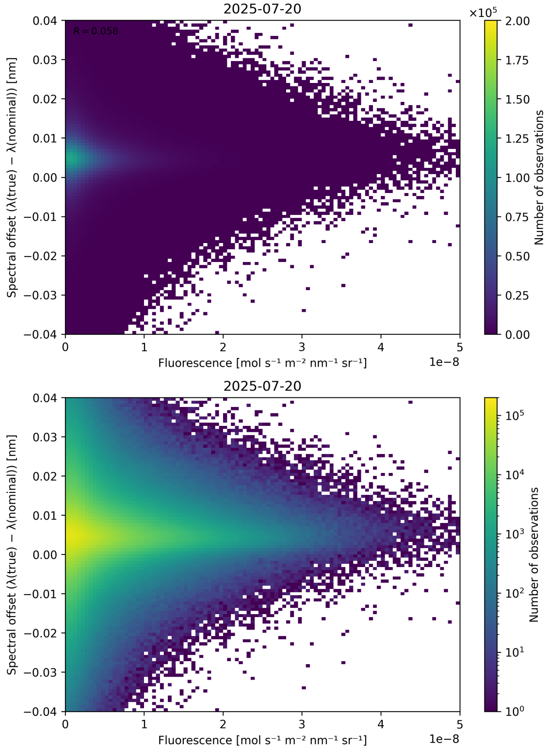
Figure 87: Scatter density plot of “Fluorescence” against “Spectral offset ( \lambda_{\text{true}} - \lambda_{\text{nominal}} )” for 2025-07-19 to 2025-07-21.
