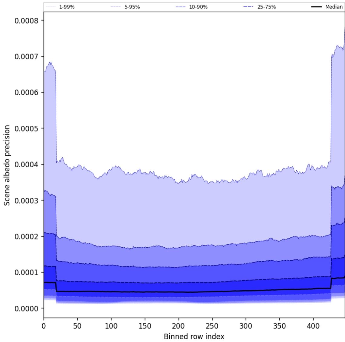
Figure 52: Along track statistics of “Scene albedo precision” for 2025-07-19 to 2025-07-21
