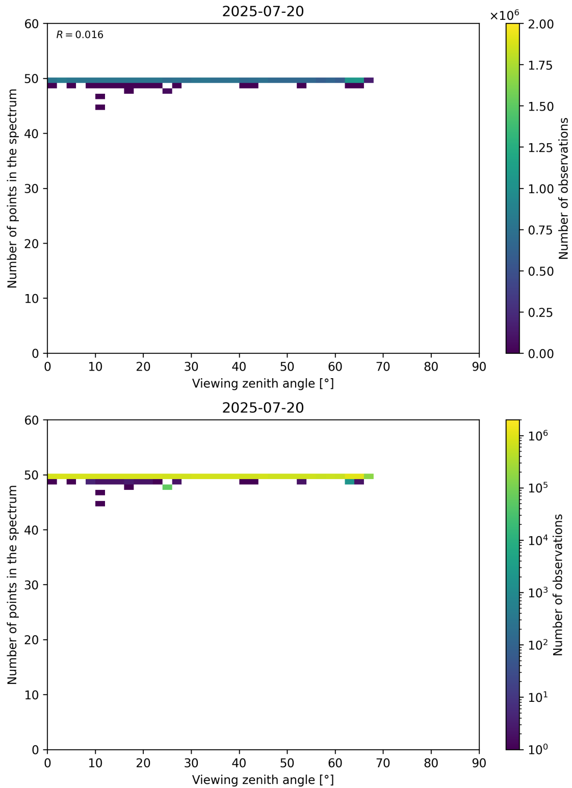
Figure 125: Scatter density plot of “Viewing zenith angle” against “Number of points in the spectrum” for 2025-07-19 to 2025-07-21.
