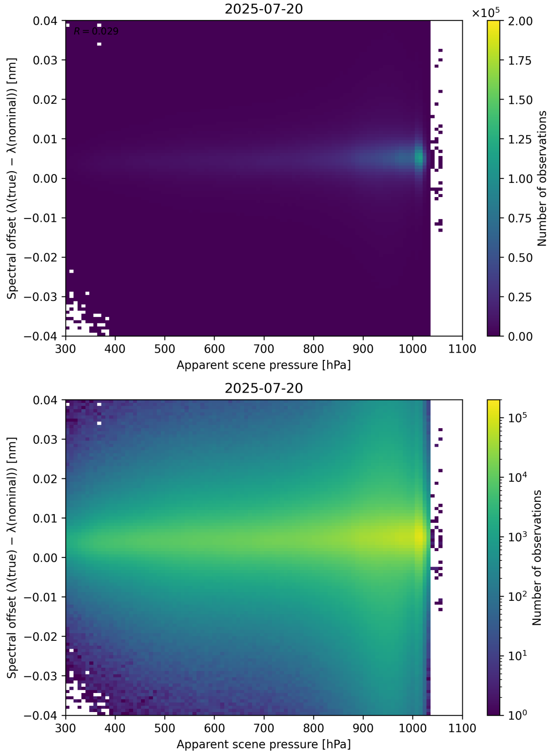
Figure 67: Scatter density plot of “Apparent scene pressure” against “Spectral offset ( \lambda_{\text{true}} - \lambda_{\text{nominal}} )” for 2025-07-19 to 2025-07-21.
