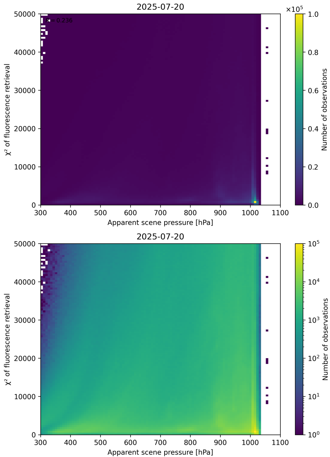
Figure 63: Scatter density plot of “Apparent scene pressure” against “ \chi^2 of fluorescence retrieval” for 2025-07-19 to 2025-07-21.
