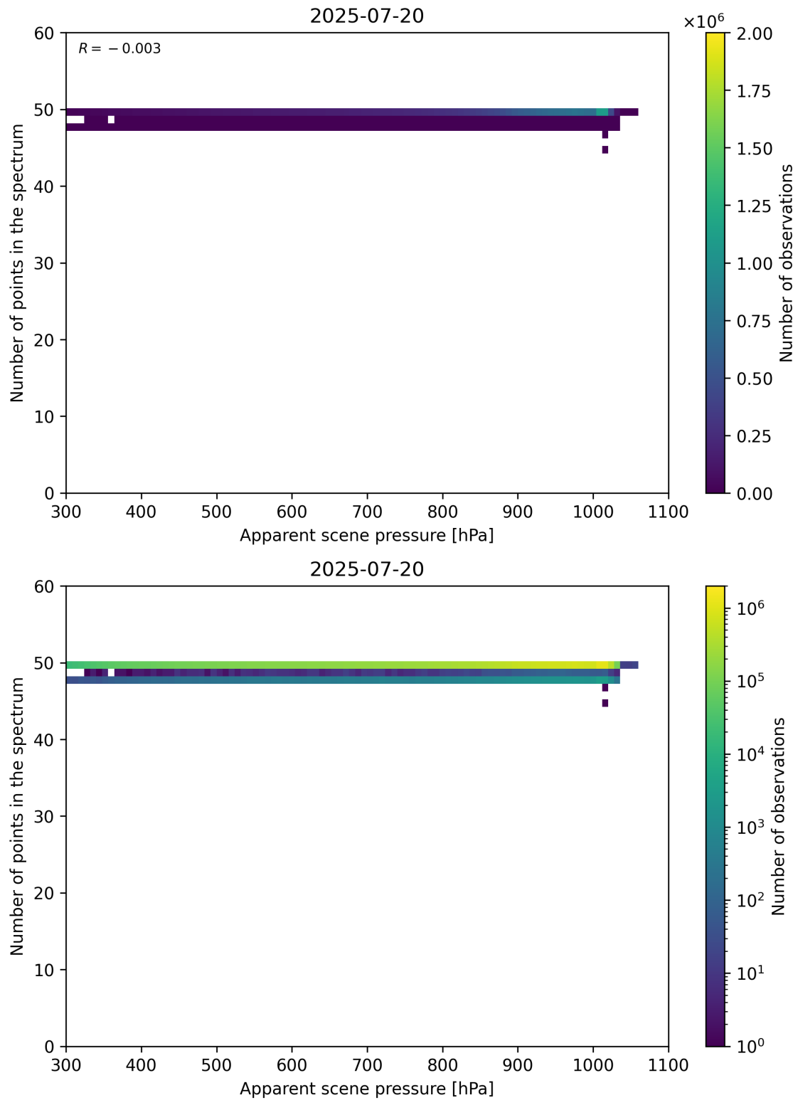
Figure 66: Scatter density plot of “Apparent scene pressure” against “Number of points in the spectrum” for 2025-07-19 to 2025-07-21.
