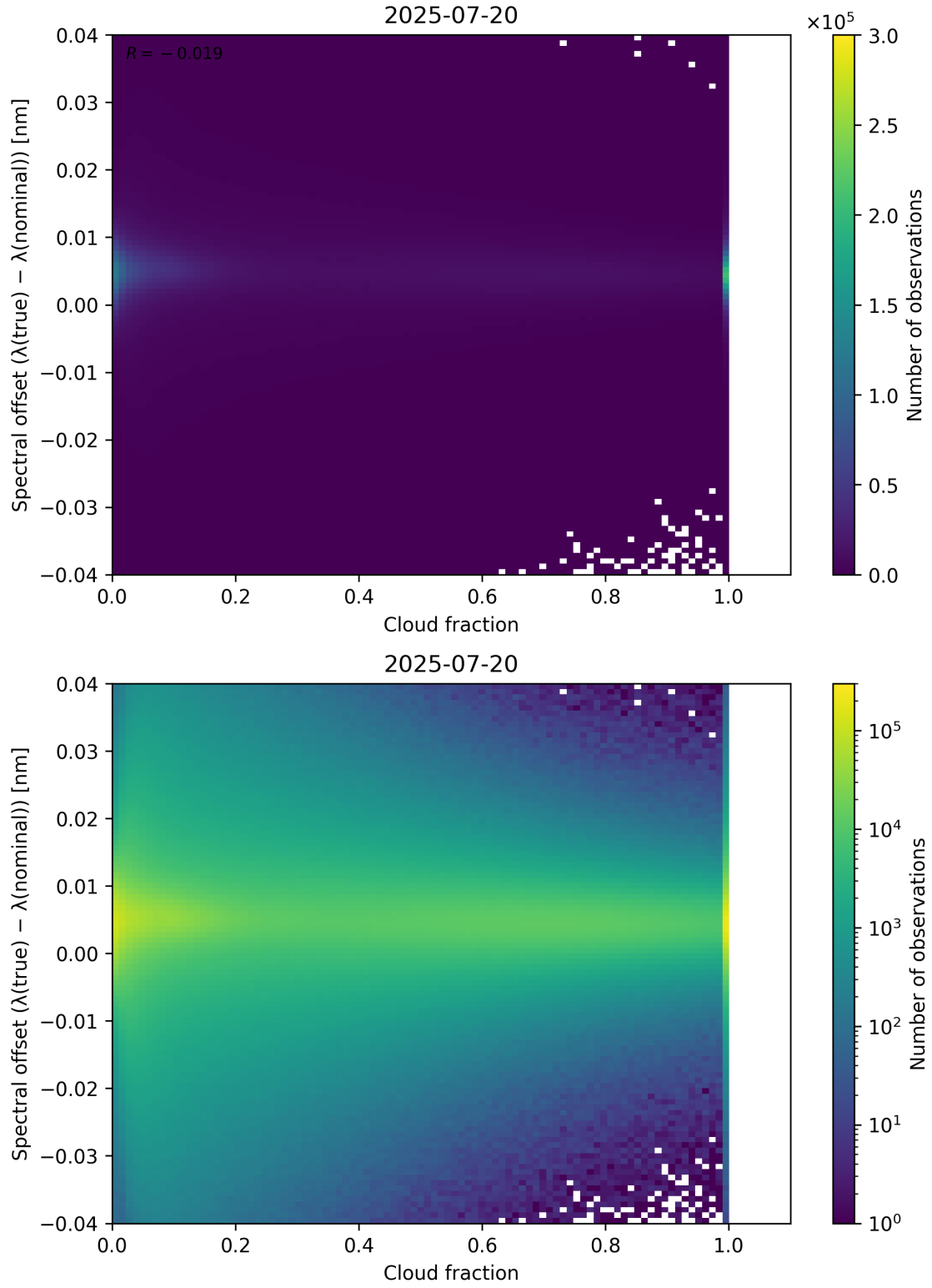
Figure 76: Scatter density plot of “Cloud fraction” against “Spectral offset ( \lambda_{\text{true}} - \lambda_{\text{nominal}} )” for 2025-07-19 to 2025-07-21.
