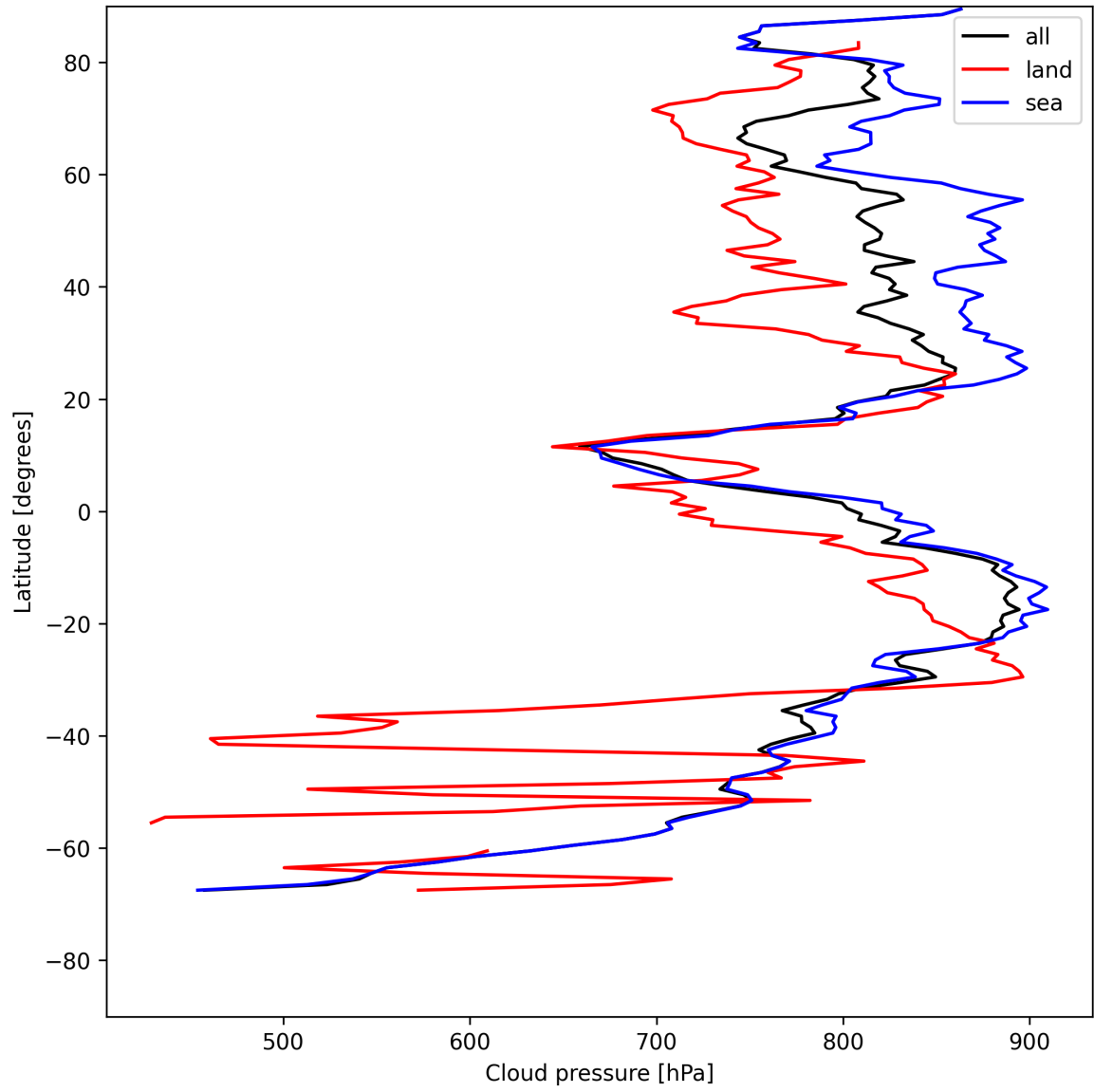
Figure 13: Zonal average of “Cloud pressure” for 2025-07-19 to 2025-07-21.
