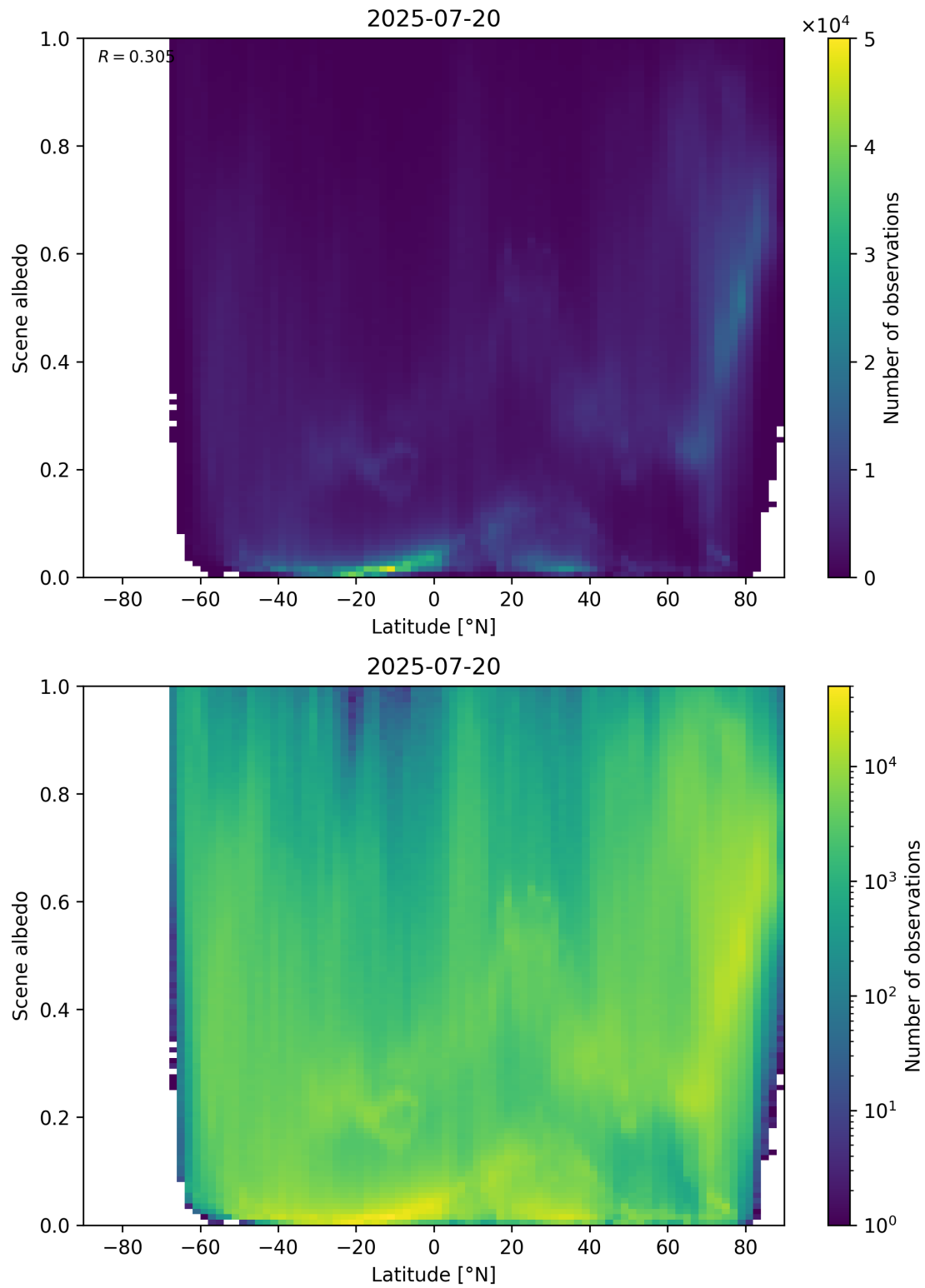
Figure 95: Scatter density plot of “Latitude” against “Scene albedo” for 2025-07-19 to 2025-07-21.
