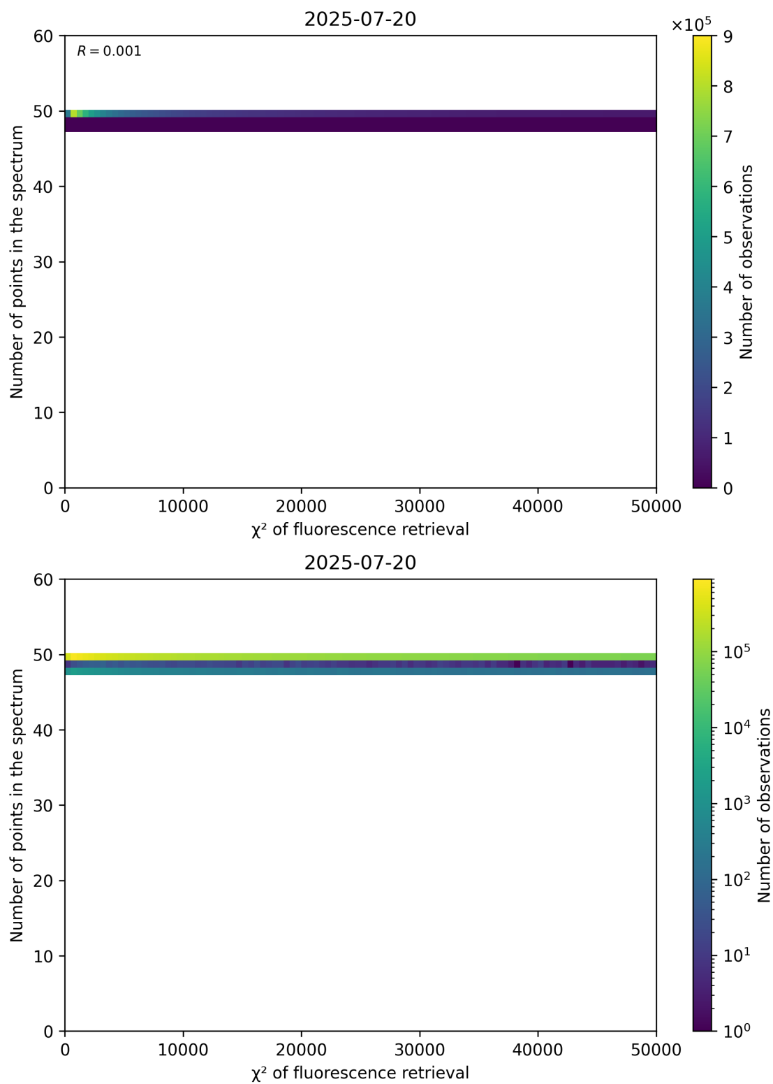
Figure 68: Scatter density plot of “ \chi^2 of fluorescence retrieval” against “Number of points in the spectrum” for 2025-07-19 to 2025-07-21.
