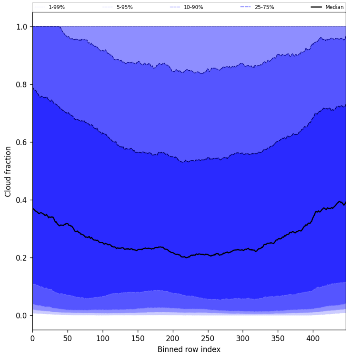
Figure 49: Along track statistics of “Cloud fraction” for 2025-07-19 to 2025-07-21
