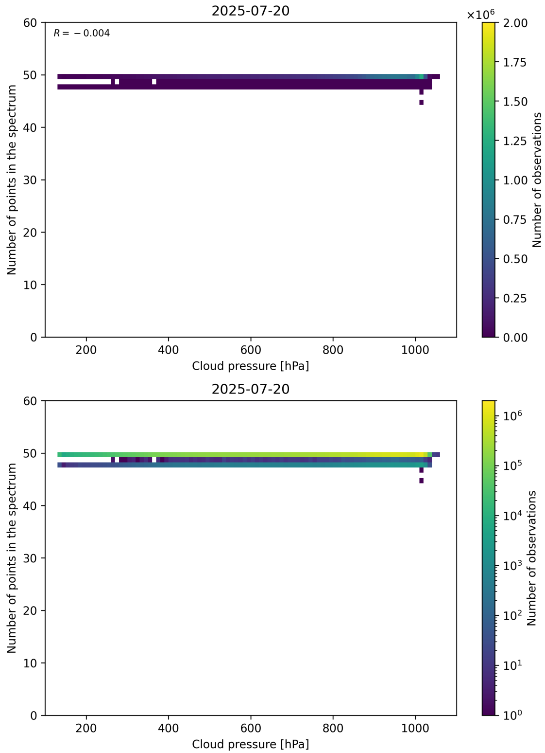
Figure 82: Scatter density plot of “Cloud pressure” against “Number of points in the spectrum” for 2025-07-19 to 2025-07-21.
