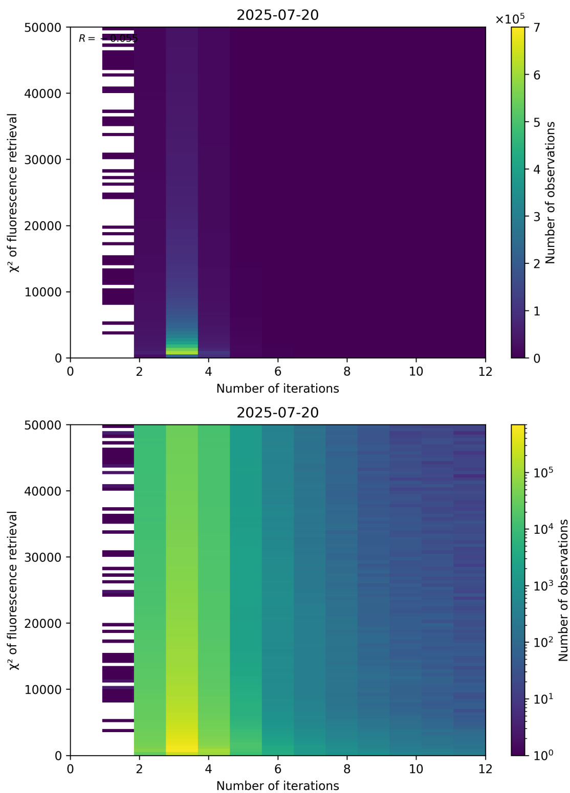
Figure 97: Scatter density plot of “Number of iterations” against “ \chi^2 of fluorescence retrieval” for 2025-07-19 to 2025-07-21.
