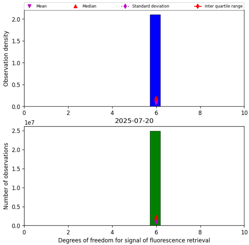
Figure 43: Histogram of "Degrees of freedom for signal of fluorescence retrieval" for 2025-07-19 to 2025-07-21
