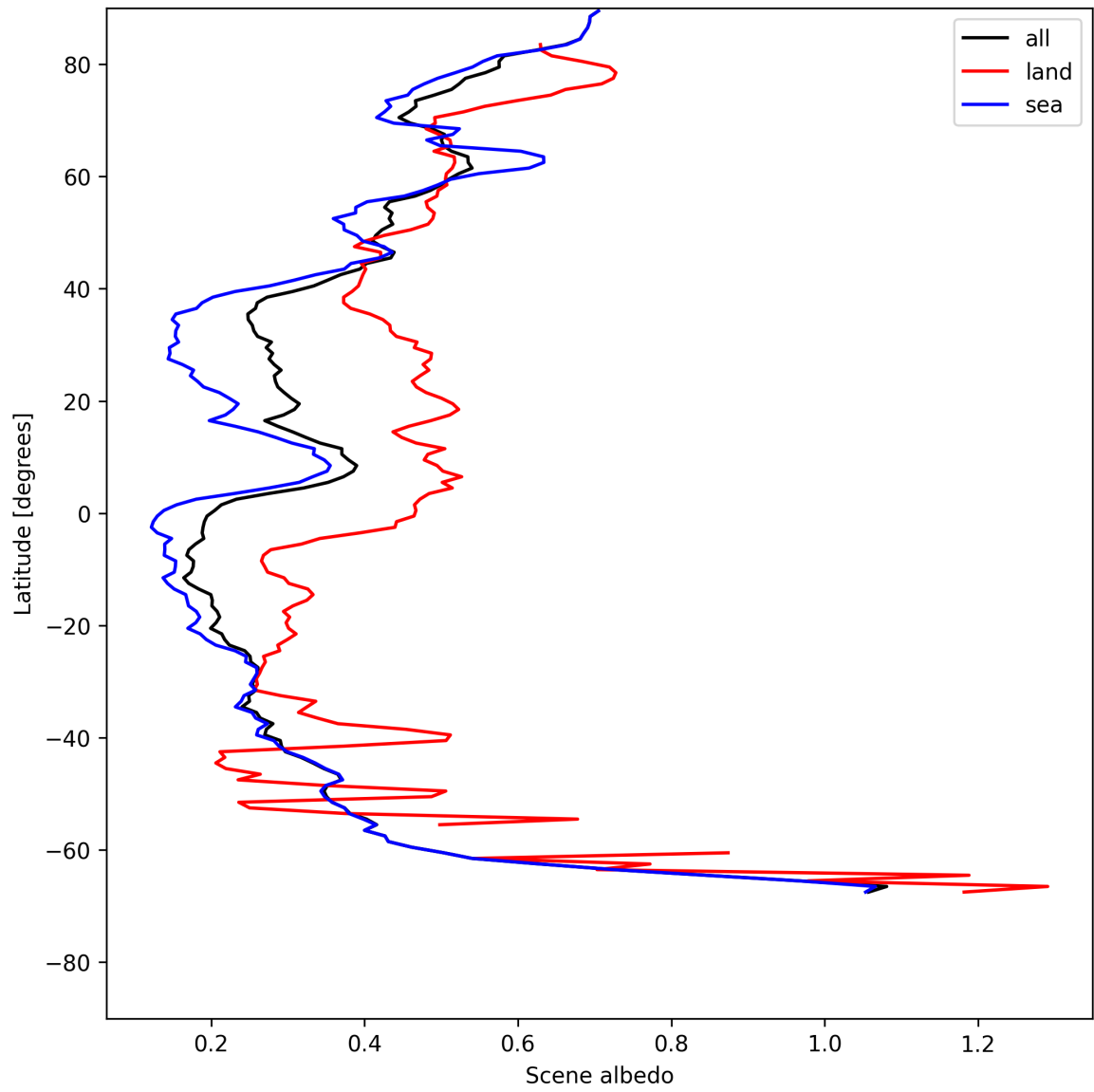
Figure 17: Zonal average of “Scene albedo” for 2025-07-19 to 2025-07-21.
