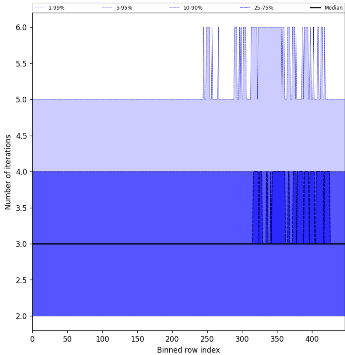
Figure 56: Along track statistics of "Number of iterations" for 2025-07-19 to 2025-07-21
