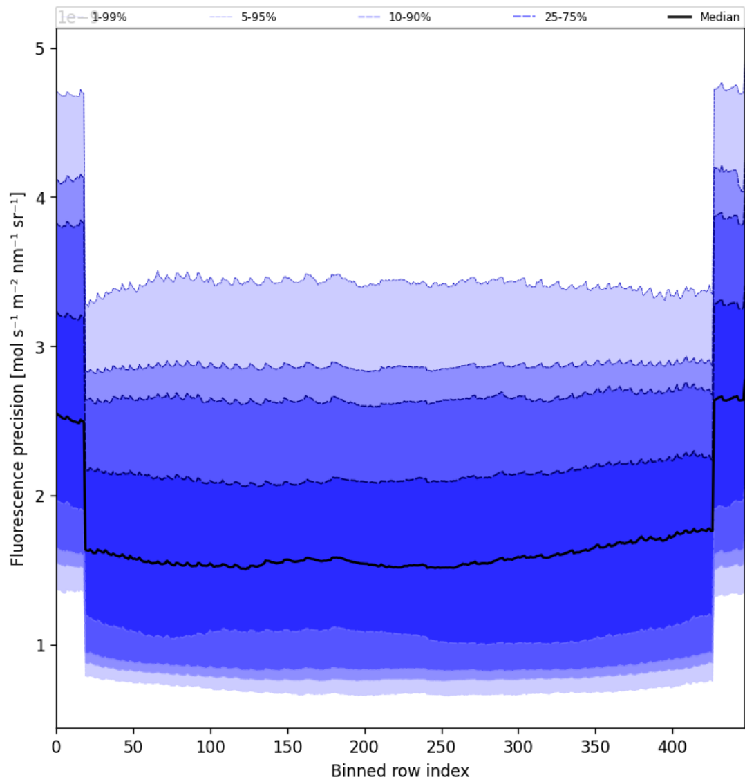
Figure 58: Along track statistics of “Fluorescence precision” for 2025-07-19 to 2025-07-21
