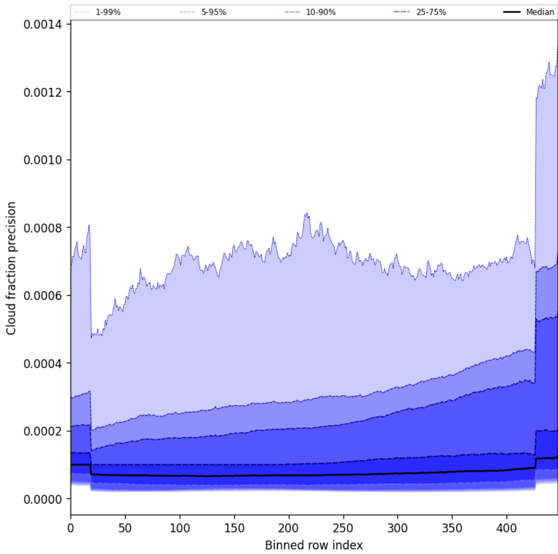
Figure 50: Along track statistics of “Cloud fraction precision” for 2025-07-19 to 2025-07-21
