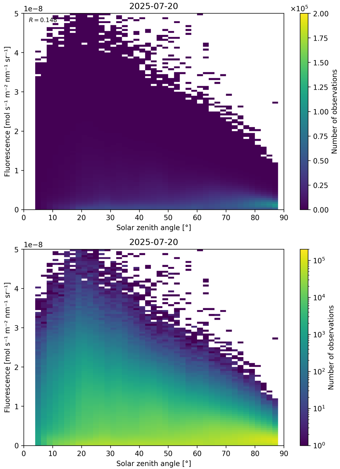
Figure 112: Scatter density plot of “Solar zenith angle” against “Fluorescence” for 2025-07-19 to 2025-07-21.
