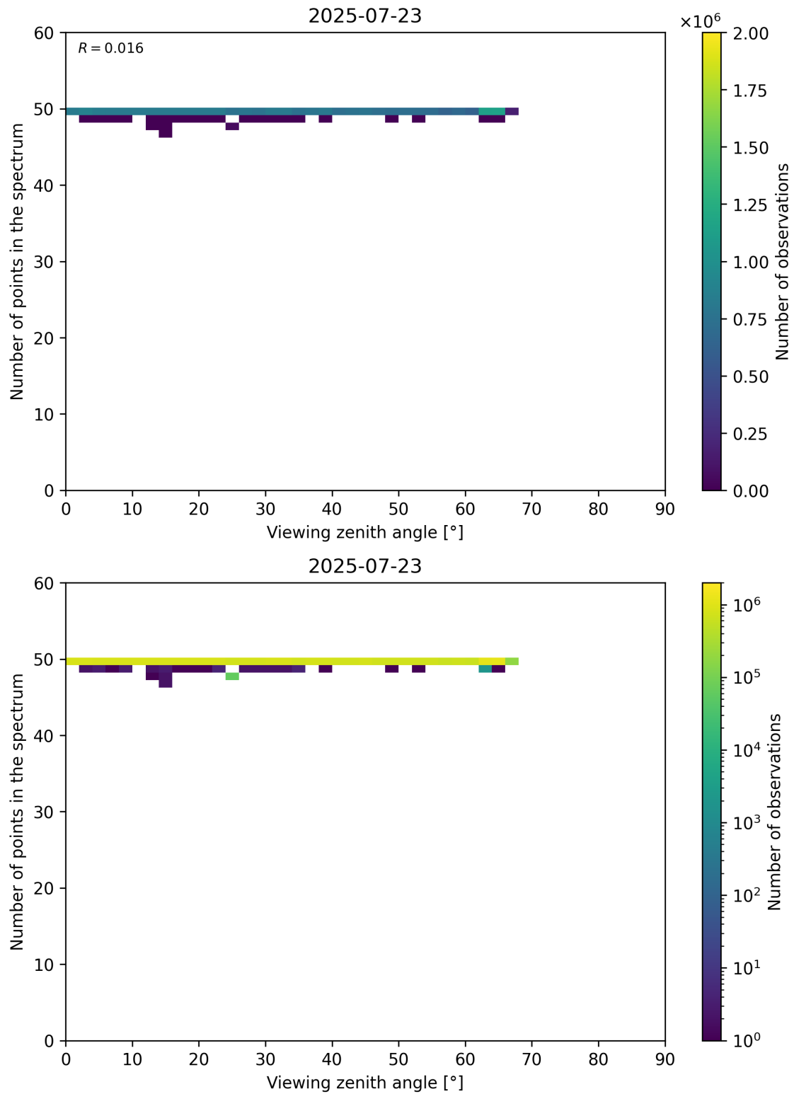
Figure 125: Scatter density plot of “Viewing zenith angle” against “Number of points in the spectrum” for 2025-07-22 to 2025-07-24.
