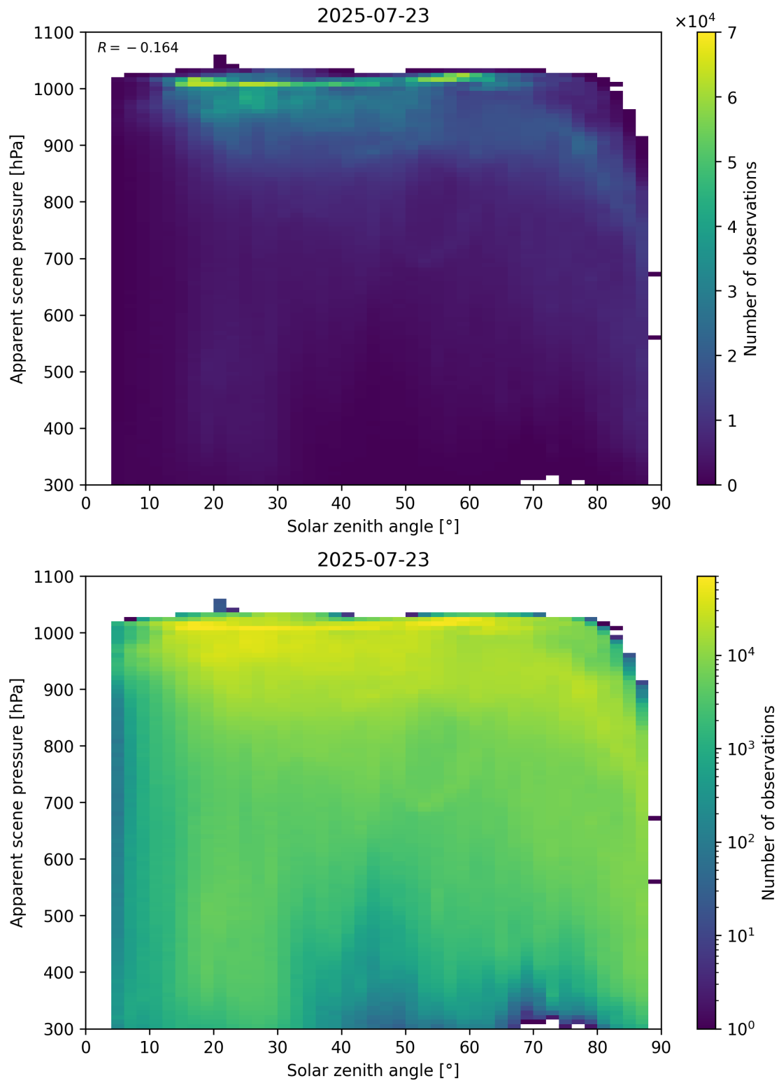
Figure 108: Scatter density plot of “Solar zenith angle” against “Apparent scene pressure” for 2025-07-22 to 2025-07-24.
