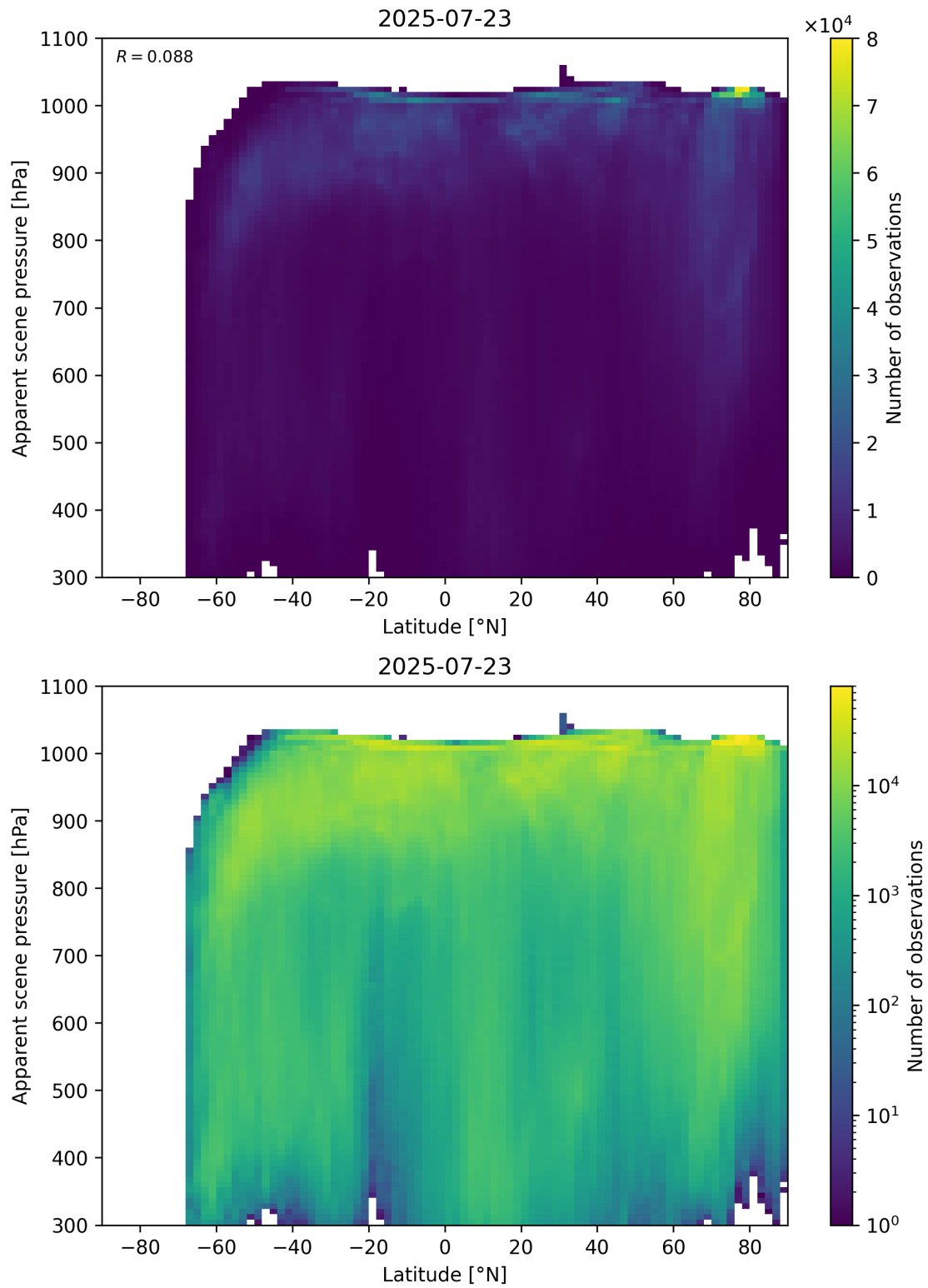
Figure 88: Scatter density plot of “Latitude” against “Apparent scene pressure” for 2025-07-22 to 2025-07-24.
