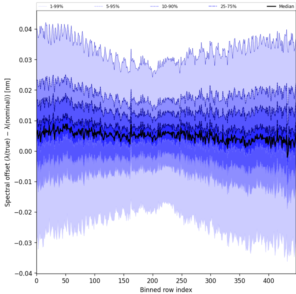
Figure 62: Along track statistics of “Spectral offset ( \lambda_{\text{true}} - \lambda_{\text{nominal}} )” for 2025-07-22 to 2025-07-24
