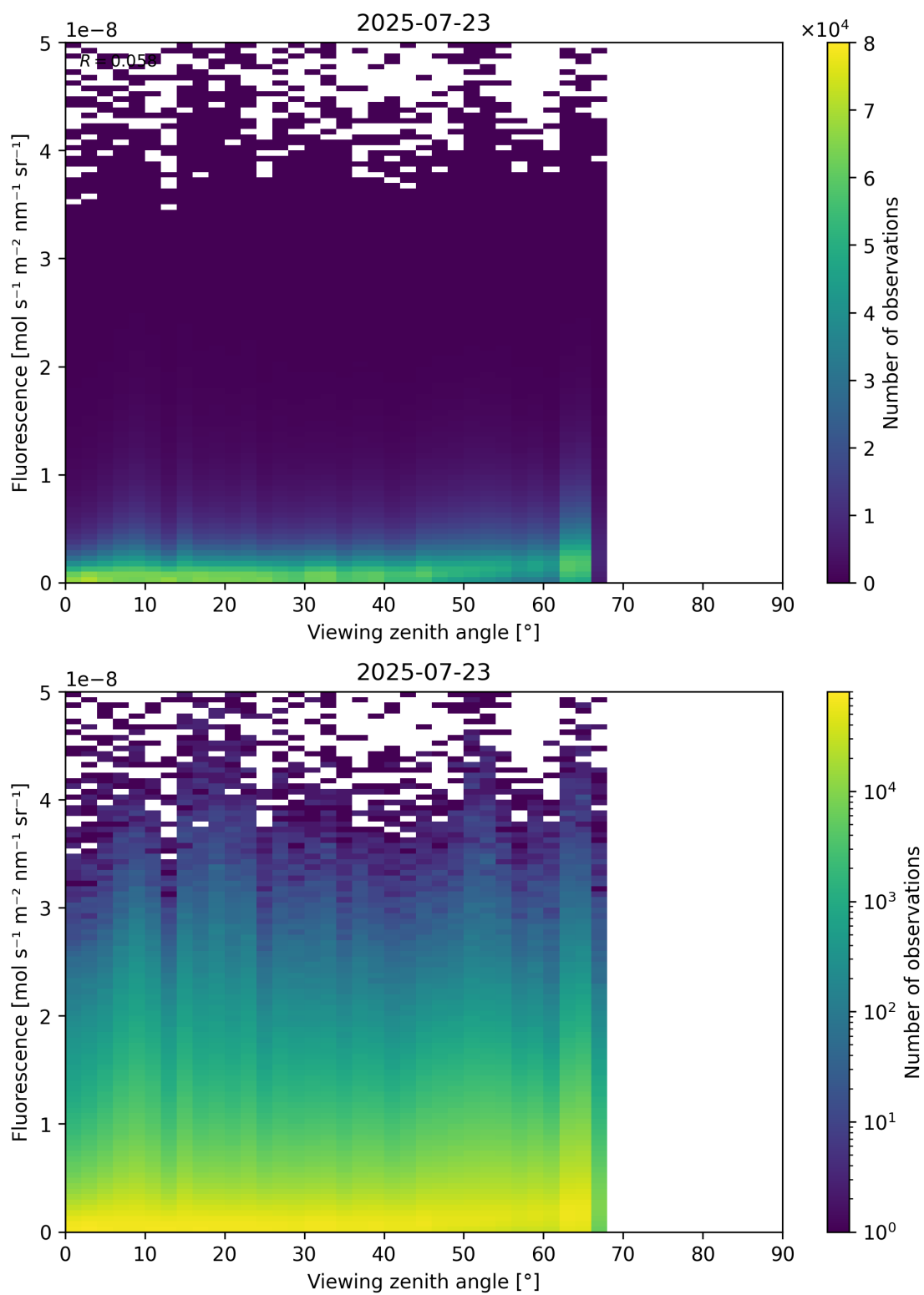
Figure 122: Scatter density plot of “Viewing zenith angle” against “Fluorescence” for 2025-07-22 to 2025-07-24.
