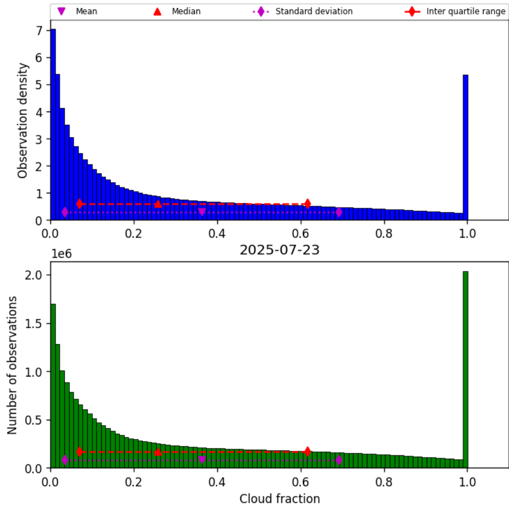
Figure 32: Histogram of “Cloud fraction” for 2025-07-22 to 2025-07-24
