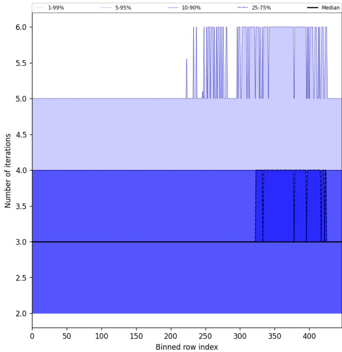
Figure 56: Along track statistics of “Number of iterations” for 2025-07-22 to 2025-07-24
