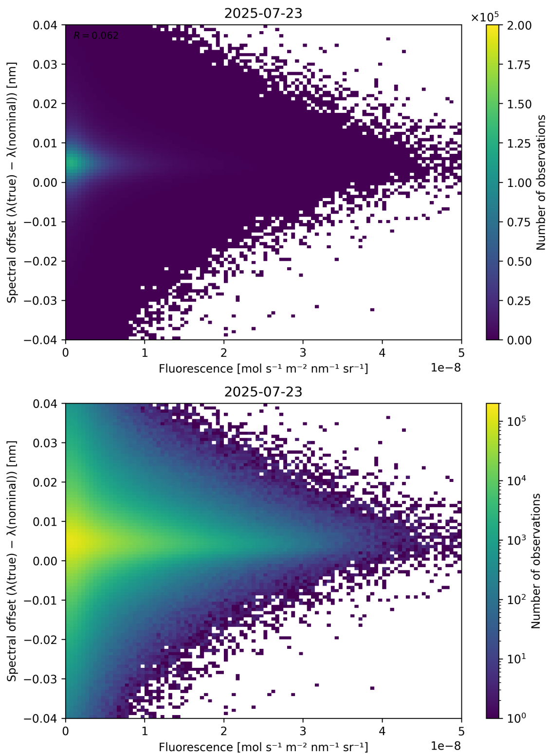
Figure 87: Scatter density plot of “Fluorescence” against “Spectral offset ( \lambda_{\text{true}} - \lambda_{\text{nominal}} )” for 2025-07-22 to 2025-07-24.
