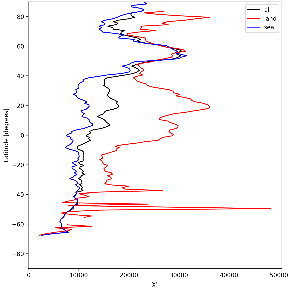
Figure 21: Zonal average of “ \chi^2 ” for 2025-07-22 to 2025-07-24.
