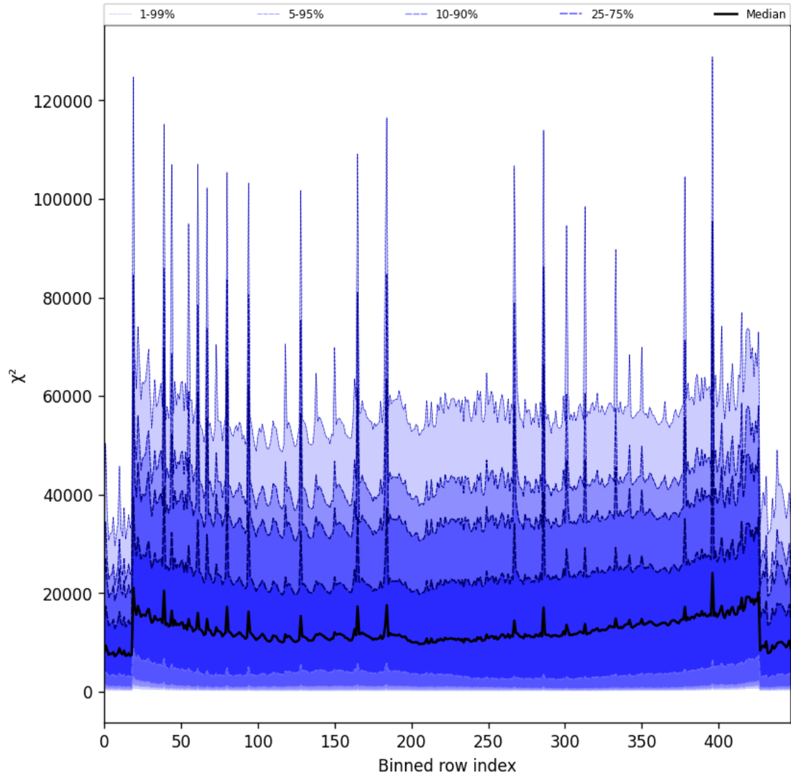
Figure 55: Along track statistics of “ \chi^2 ” for 2025-07-22 to 2025-07-24
