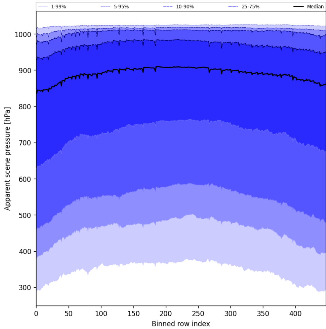
Figure 53: Along track statistics of “Apparent scene pressure” for 2025-07-22 to 2025-07-24
