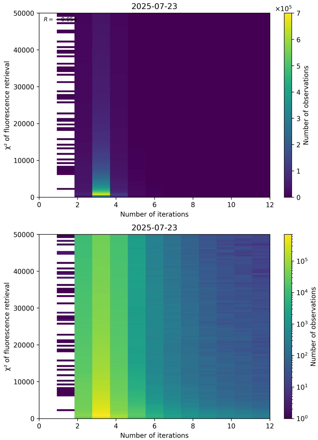
Figure 97: Scatter density plot of “Number of iterations” against “ \chi^2 of fluorescence retrieval” for 2025-07-22 to 2025-07-24.
