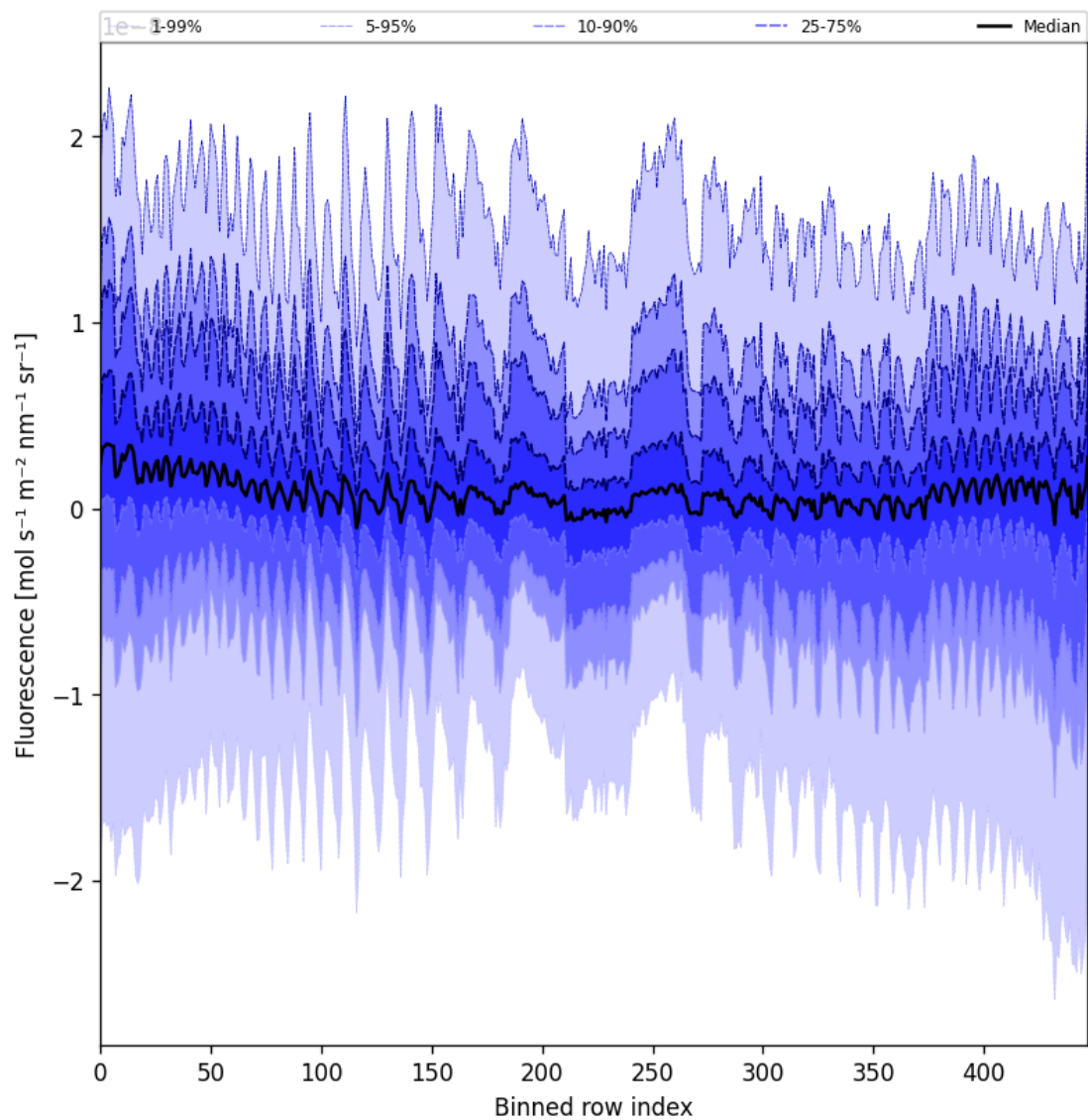
Figure 57: Along track statistics of “Fluorescence” for 2025-07-22 to 2025-07-24
