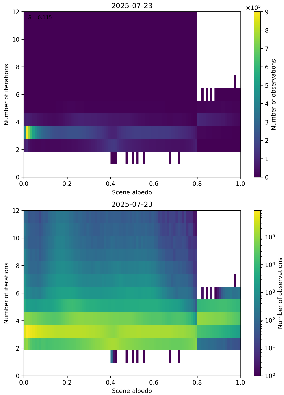
Figure 105: Scatter density plot of “Scene albedo” against “Number of iterations” for 2025-07-22 to 2025-07-24.
