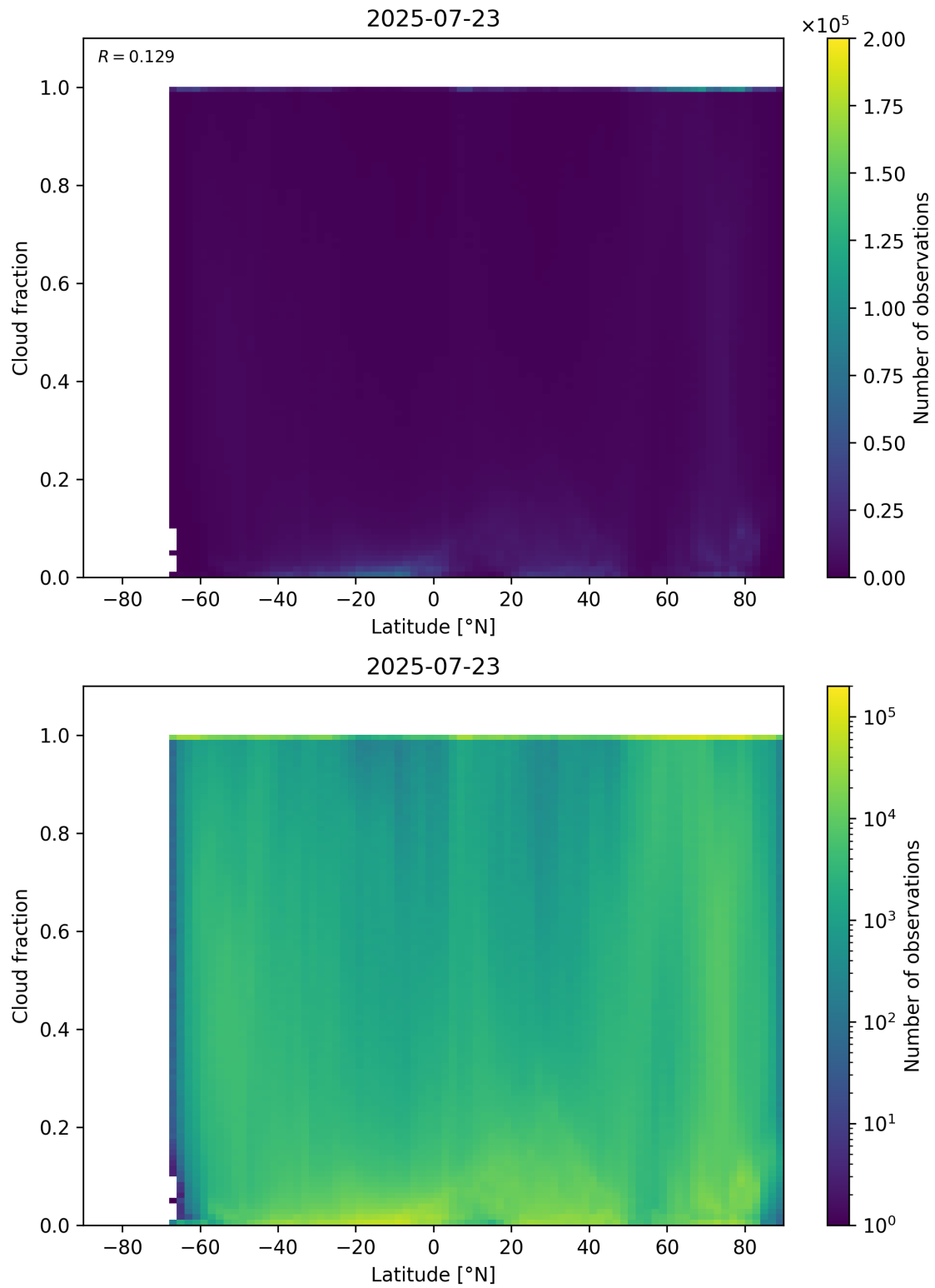
Figure 90: Scatter density plot of “Latitude” against “Cloud fraction” for 2025-07-22 to 2025-07-24.
