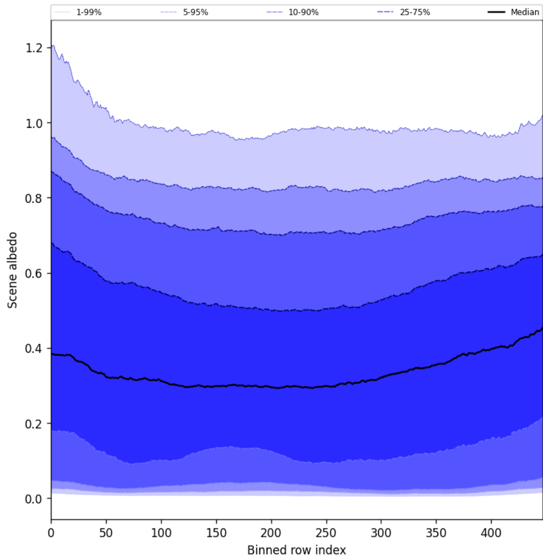
Figure 51: Along track statistics of “Scene albedo” for 2025-07-22 to 2025-07-24
