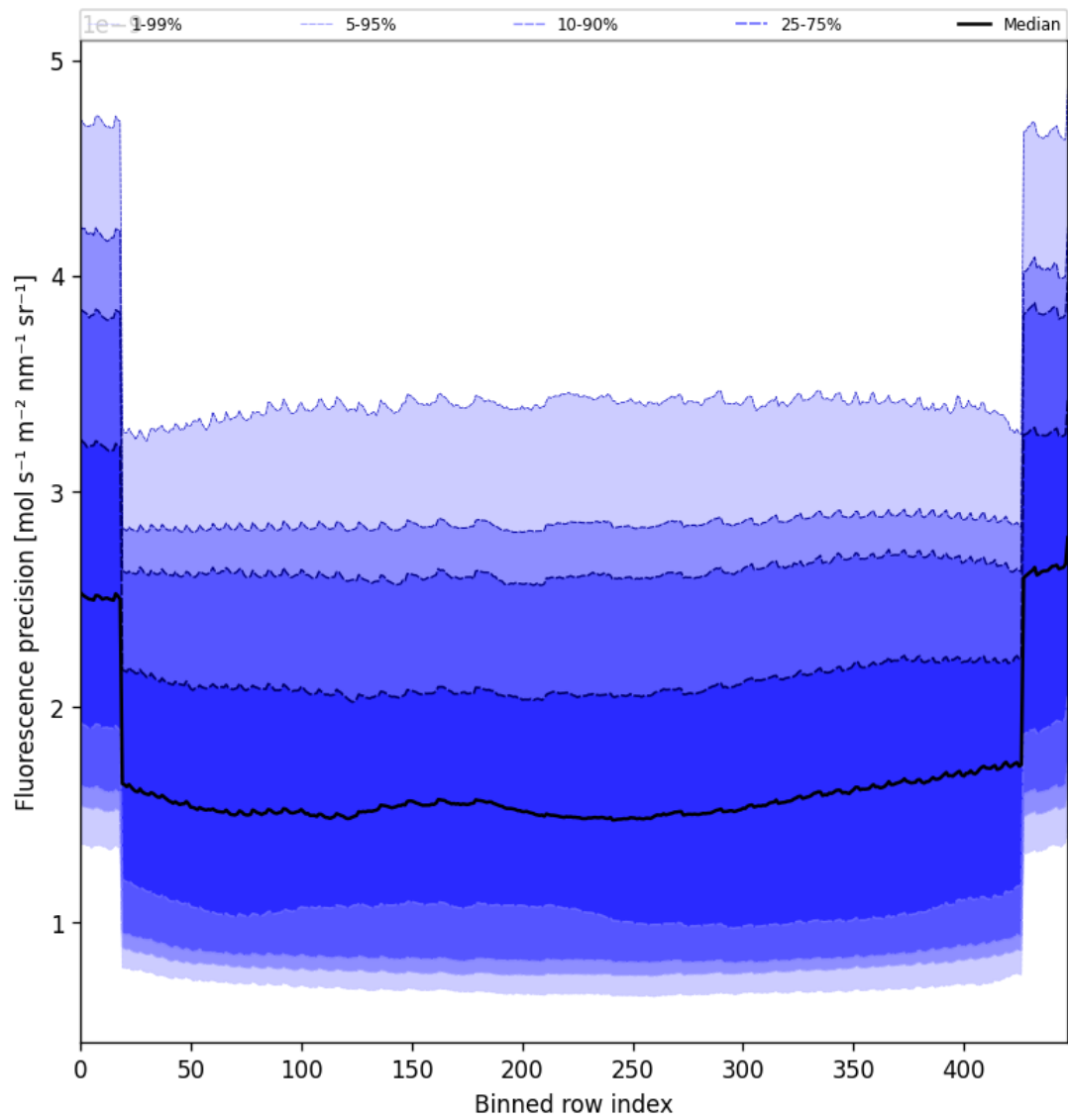
Figure 58: Along track statistics of “Fluorescence precision” for 2025-07-22 to 2025-07-24
