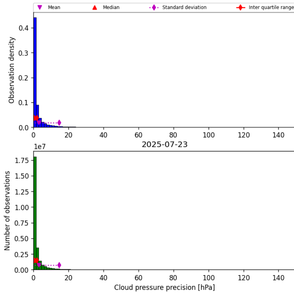
Figure 31: Histogram of “Cloud pressure precision” for 2025-07-22 to 2025-07-24
