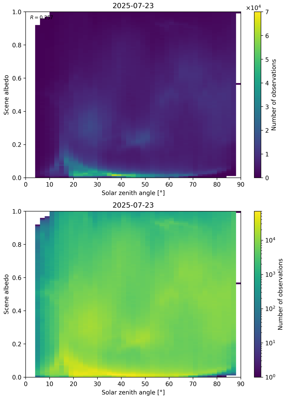
Figure 116: Scatter density plot of “Solar zenith angle” against “Scene albedo” for 2025-07-22 to 2025-07-24.
