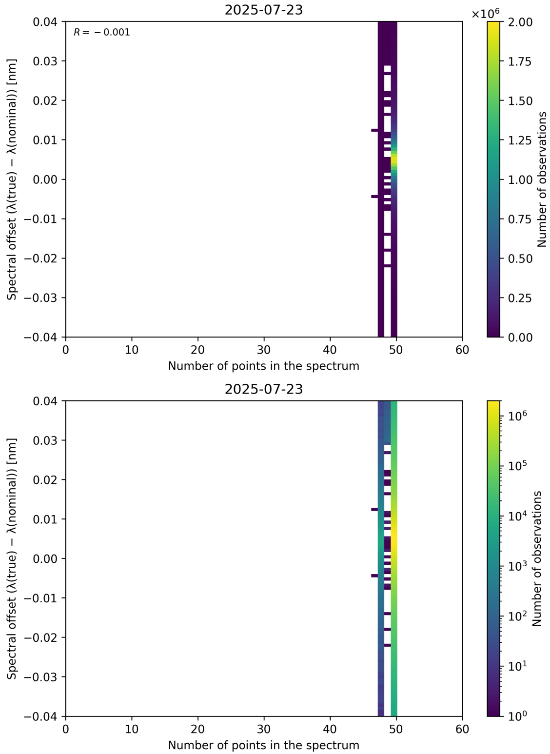
Figure 101: Scatter density plot of “Number of points in the spectrum” against “Spectral offset ( \lambda_{\text{true}} - \lambda_{\text{nominal}} )” for 2025-07-22 to 2025-07-24.
