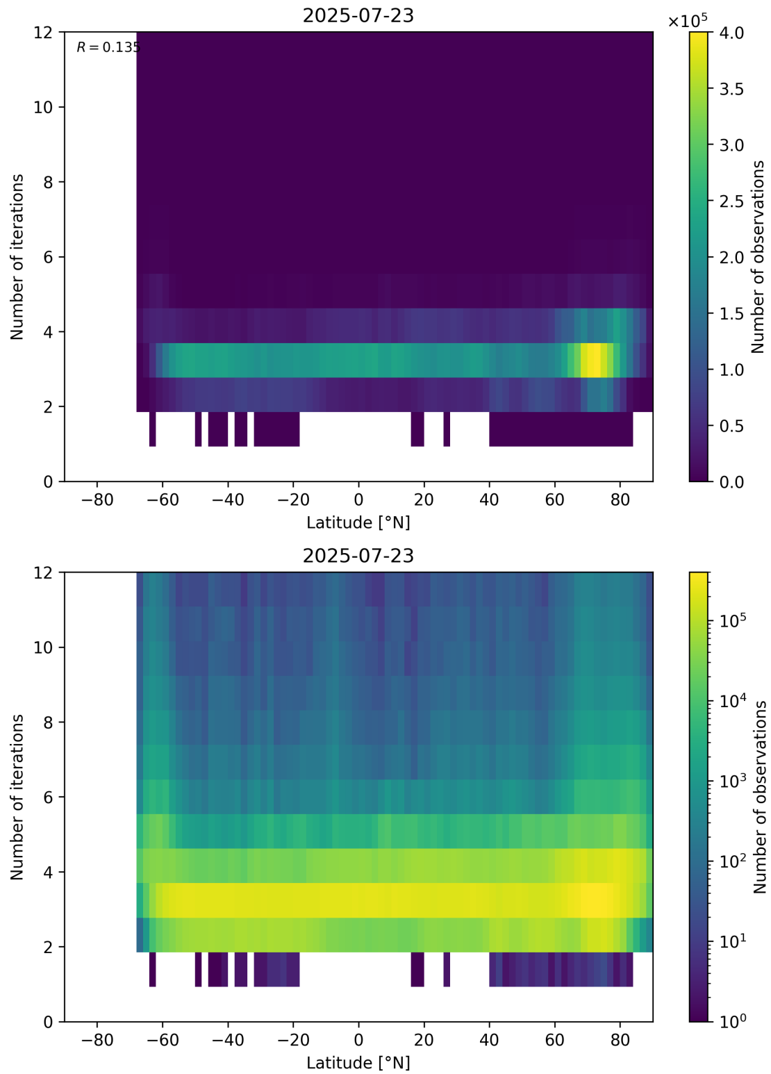
Figure 93: Scatter density plot of “Latitude” against “Number of iterations” for 2025-07-22 to 2025-07-24.
