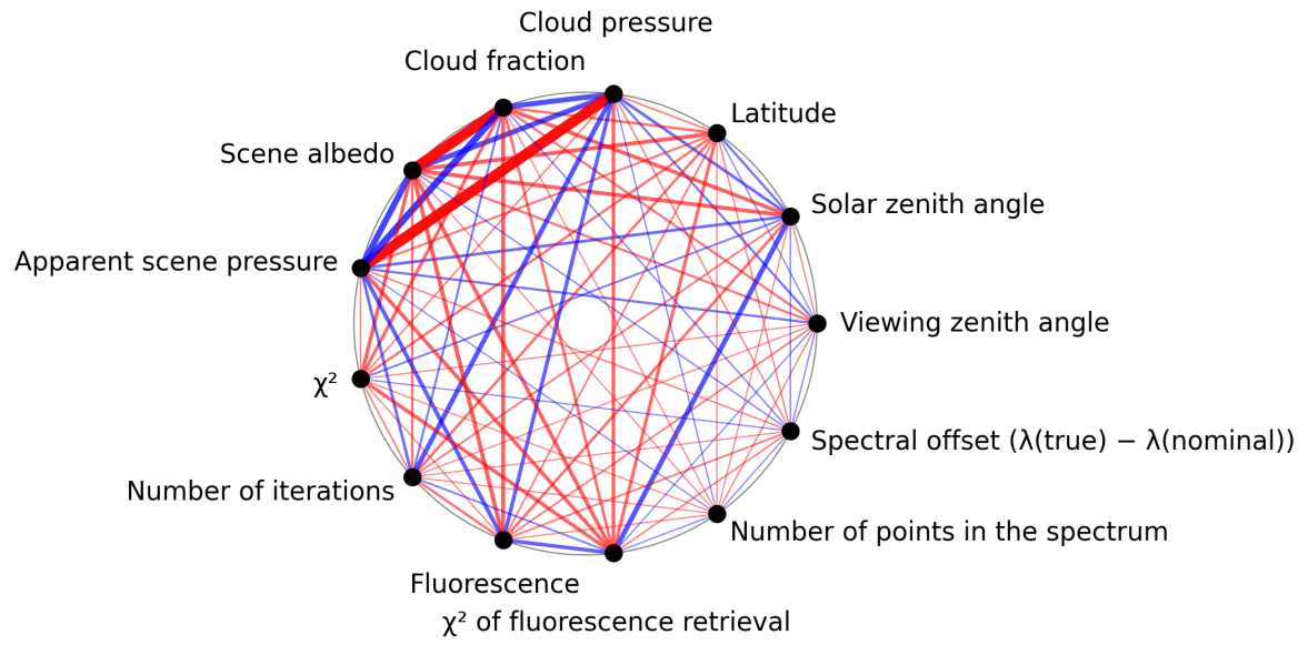
Figure 1: Map of correlation graph for 2025-07-22 to 2025-07-24.
