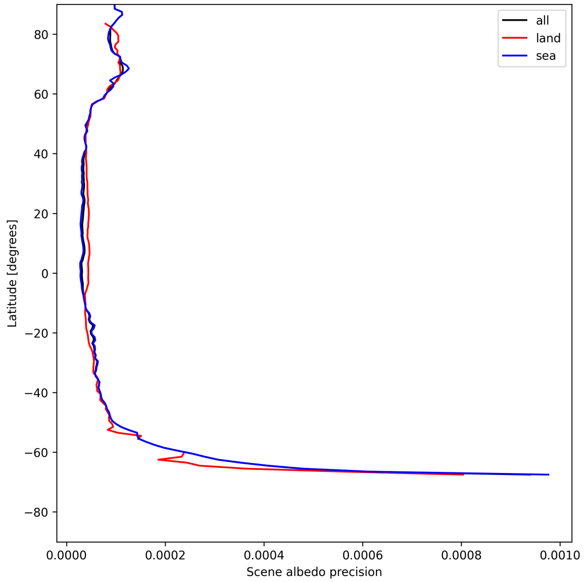
Figure 18: Zonal average of “Scene albedo precision” for 2025-07-22 to 2025-07-24.
