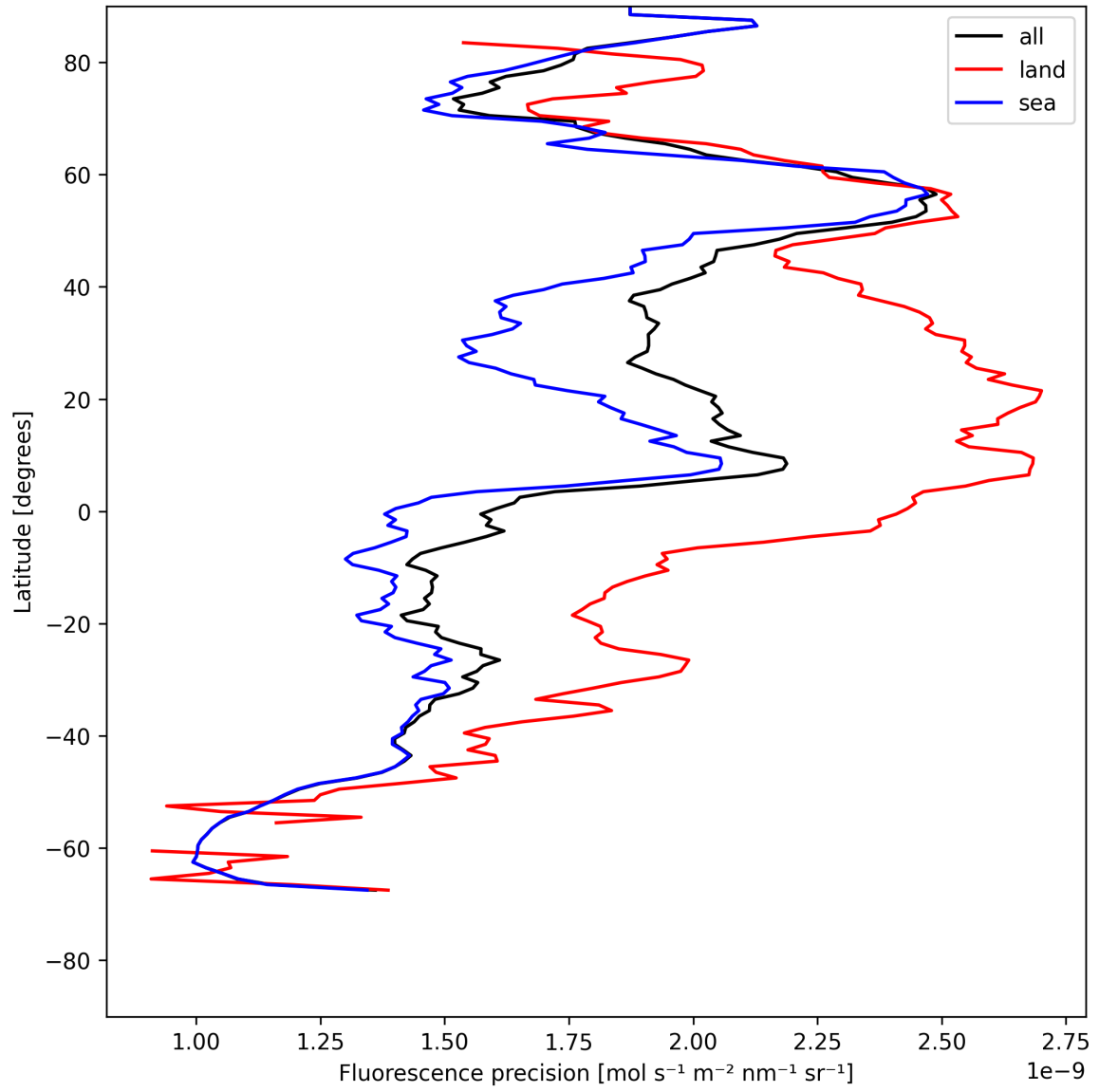
Figure 24: Zonal average of “Fluorescence precision” for 2025-07-22 to 2025-07-24.
