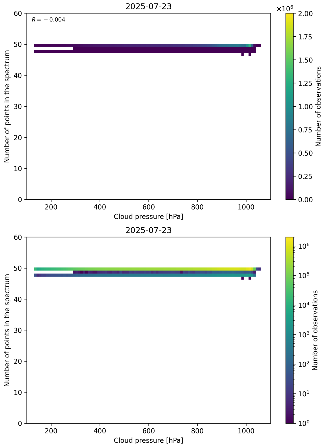
Figure 82: Scatter density plot of “Cloud pressure” against “Number of points in the spectrum” for 2025-07-22 to 2025-07-24.
