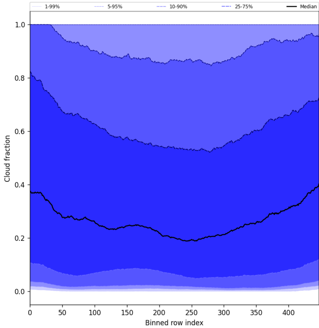
Figure 49: Along track statistics of “Cloud fraction” for 2025-07-22 to 2025-07-24
