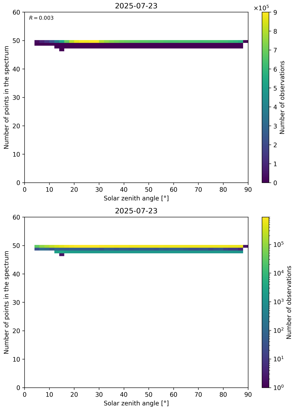
Figure 115: Scatter density plot of “Solar zenith angle” against “Number of points in the spectrum” for 2025-07-22 to 2025-07-24.
