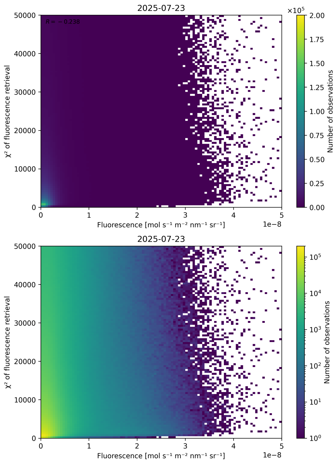
Figure 85: Scatter density plot of “Fluorescence” against “ \chi^2 of fluorescence retrieval” for 2025-07-22 to 2025-07-24.
