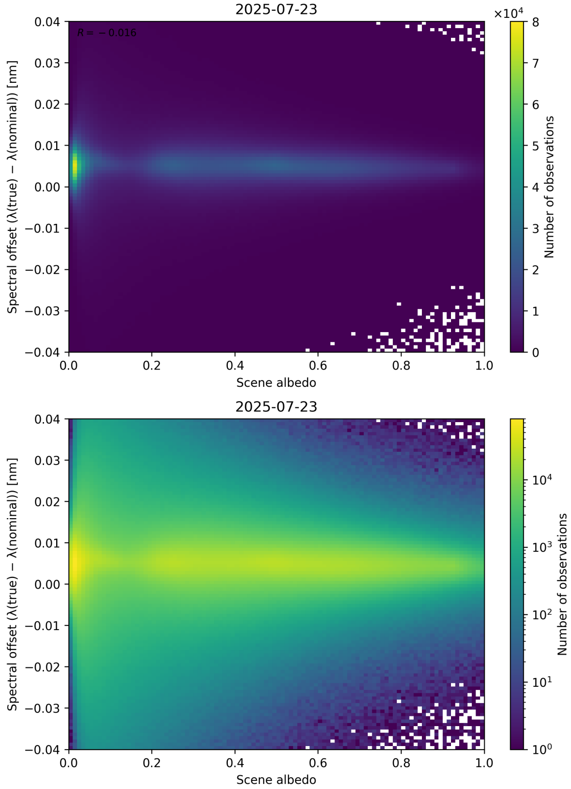
Figure 107: Scatter density plot of “Scene albedo” against “Spectral offset ( \lambda_{\text{true}} - \lambda_{\text{nominal}} )” for 2025-07-22 to 2025-07-24.
