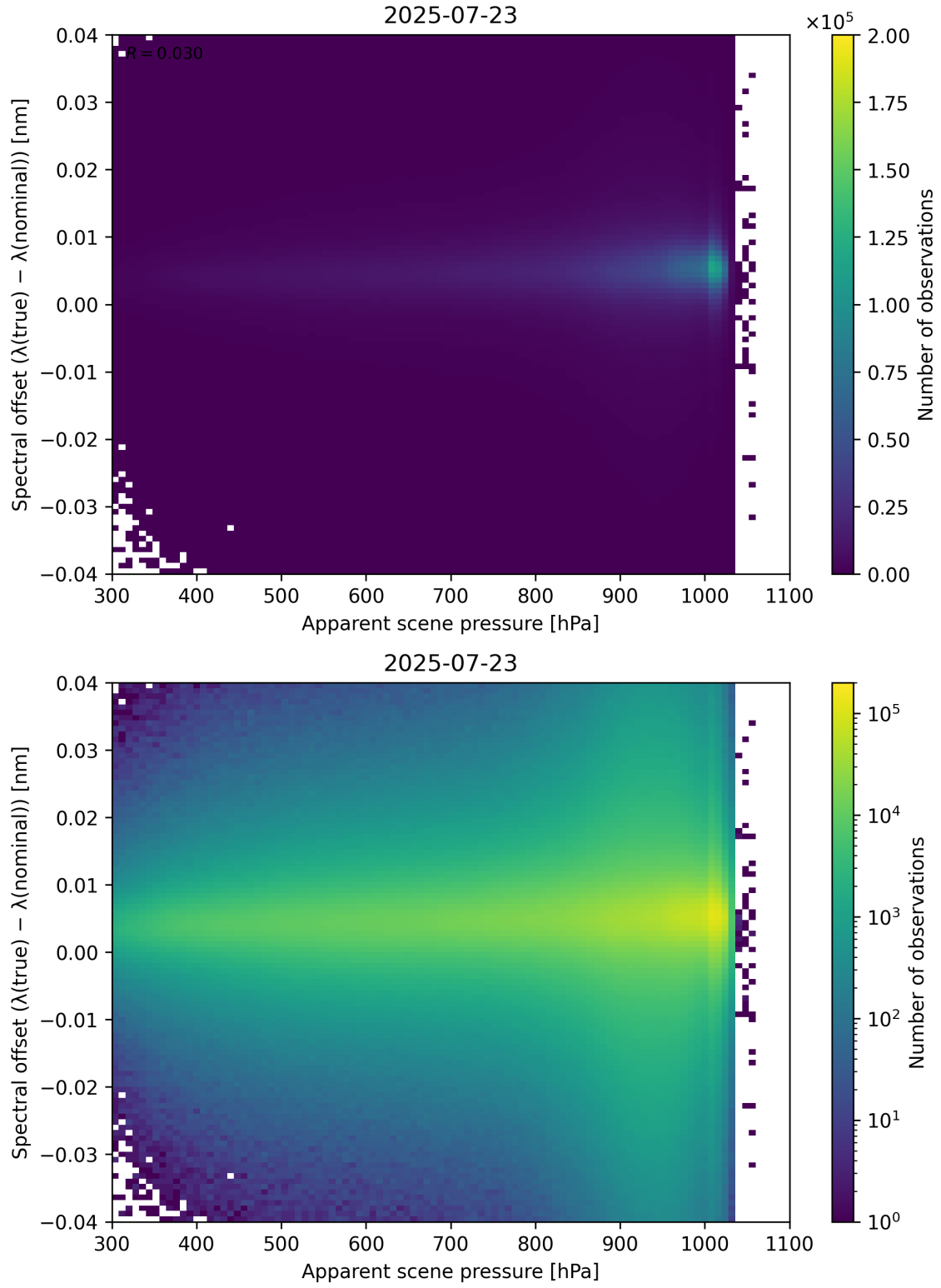
Figure 67: Scatter density plot of “Apparent scene pressure” against “Spectral offset ( \lambda_{\text{true}} - \lambda_{\text{nominal}} )” for 2025-07-22 to 2025-07-24.
