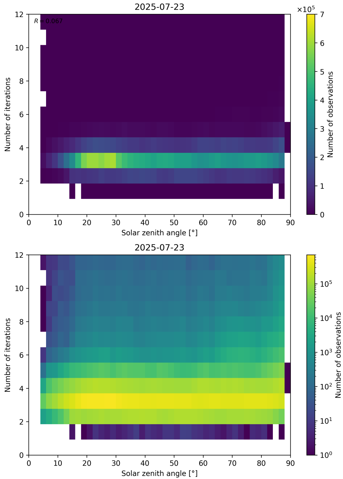
Figure 114: Scatter density plot of “Solar zenith angle” against “Number of iterations” for 2025-07-22 to 2025-07-24.
