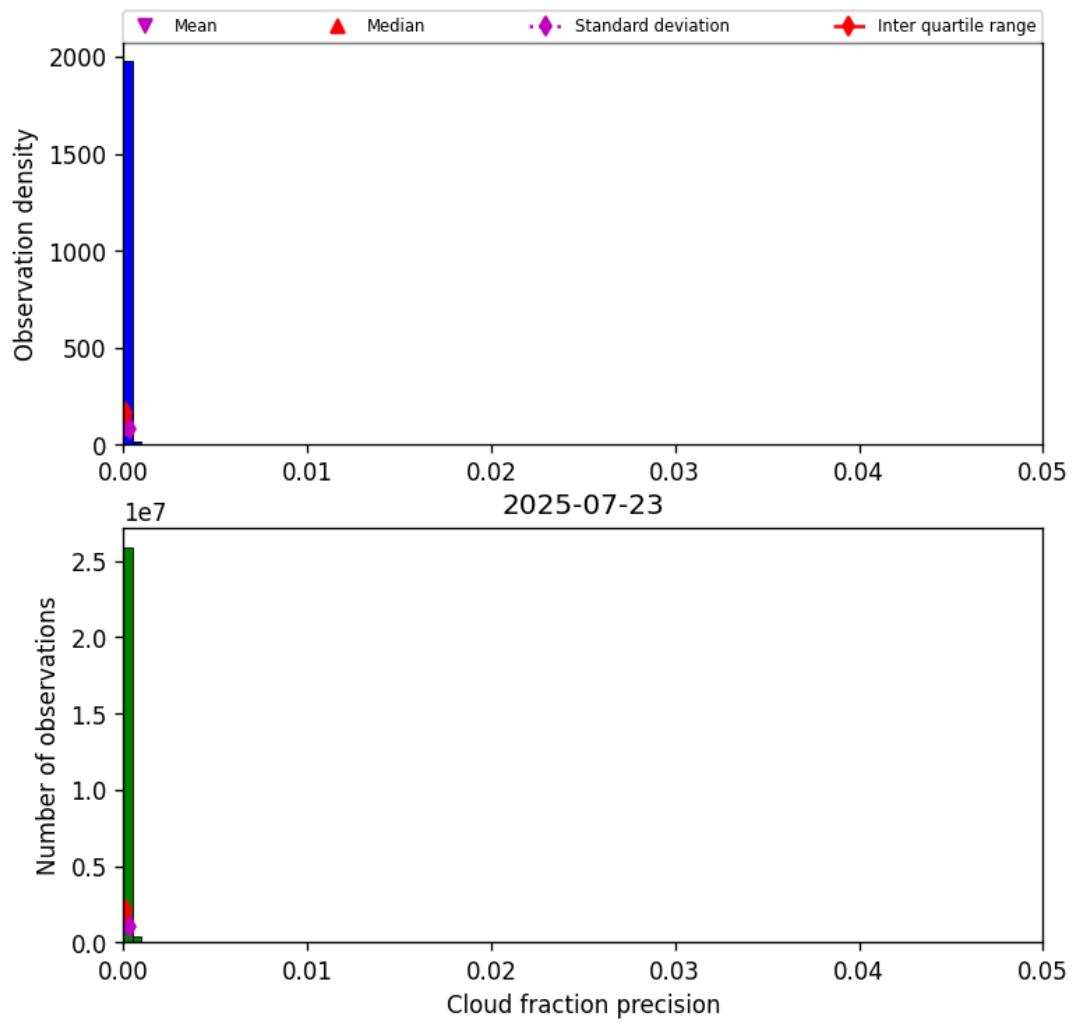
Figure 33: Histogram of “Cloud fraction precision” for 2025-07-22 to 2025-07-24
