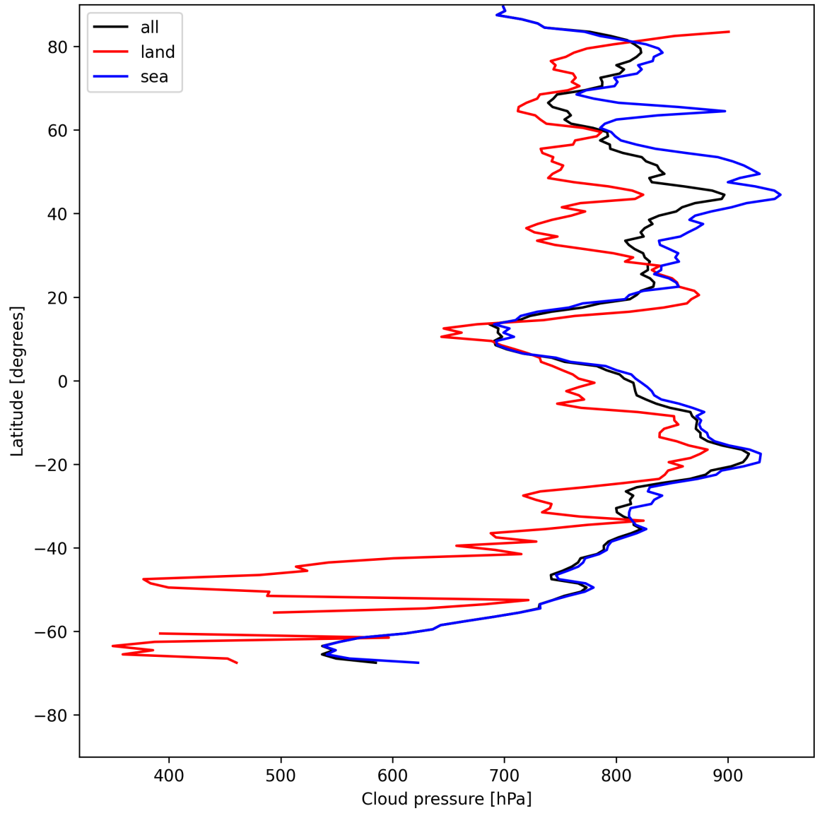
Figure 13: Zonal average of “Cloud pressure” for 2025-07-22 to 2025-07-24.
