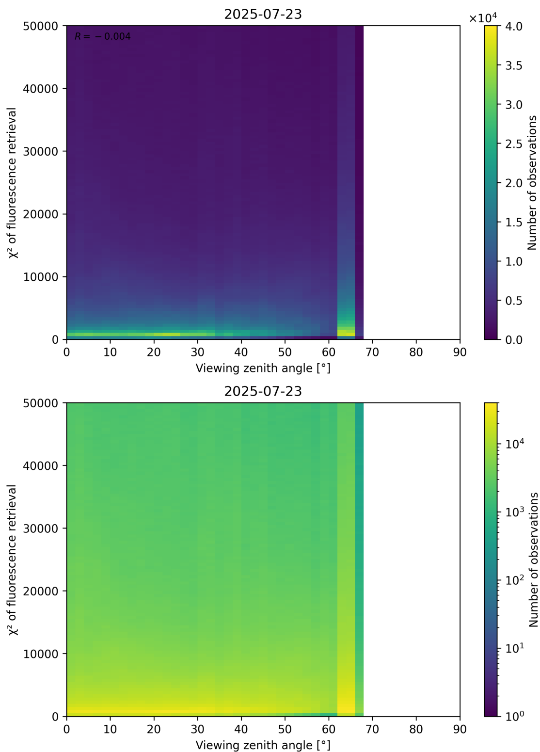
Figure 119: Scatter density plot of “Viewing zenith angle” against “ \chi^2 of fluorescence retrieval” for 2025-07-22 to 2025-07-24.
