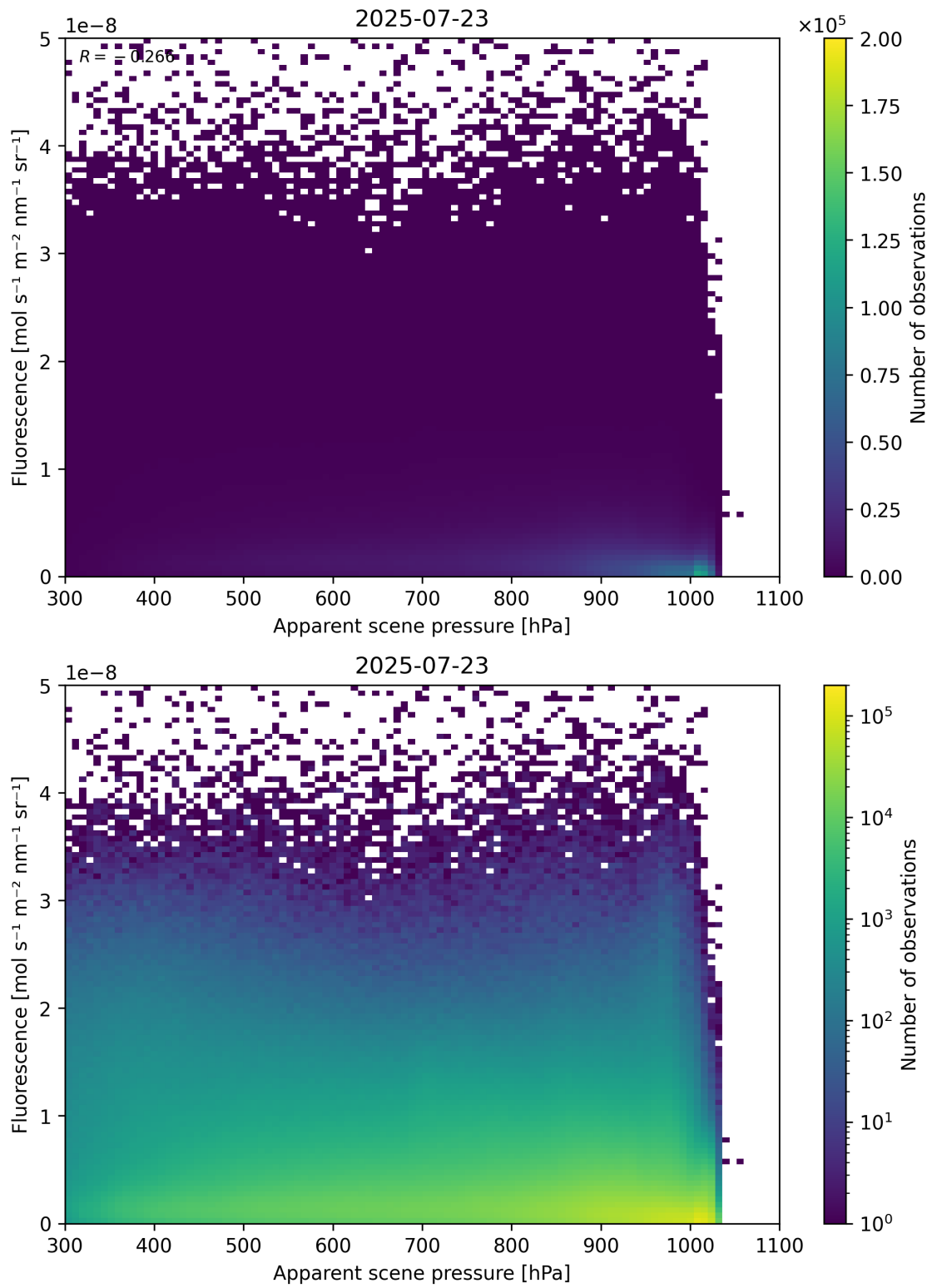
Figure 64: Scatter density plot of “Apparent scene pressure” against “Fluorescence” for 2025-07-22 to 2025-07-24.
