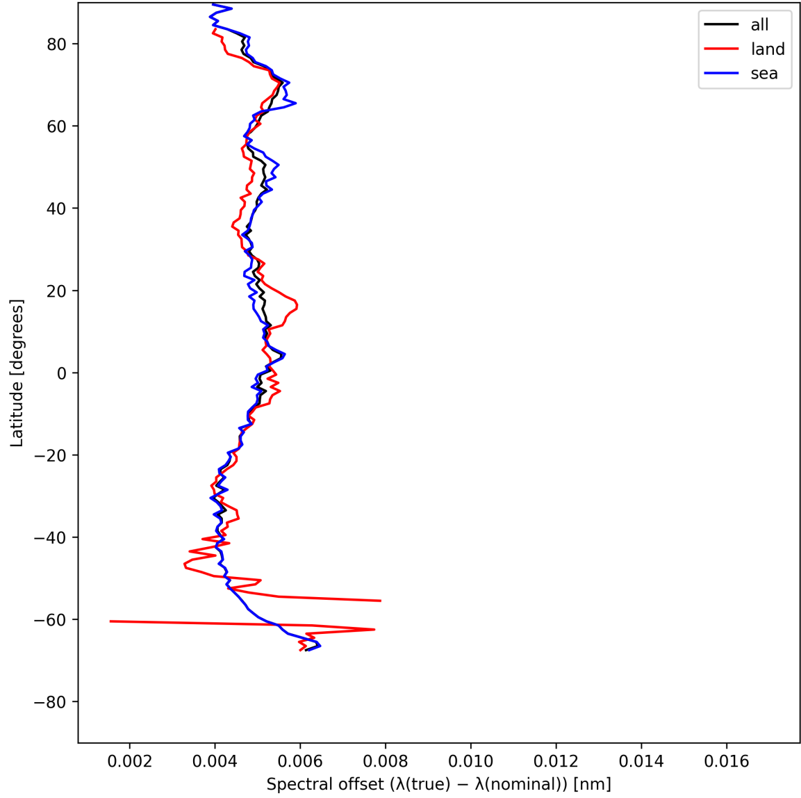
Figure 28: Zonal average of “Spectral offset ( \lambda_{\text{true}} - \lambda_{\text{nominal}} )” for 2025-07-22 to 2025-07-24.
