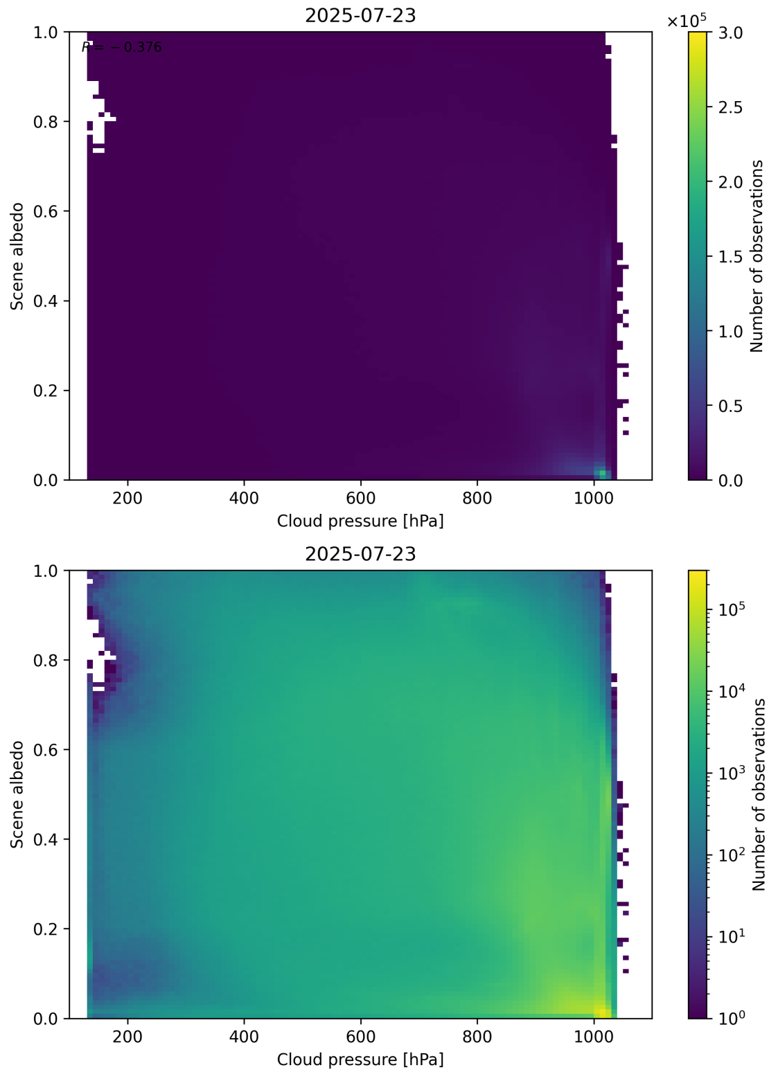
Figure 83: Scatter density plot of “Cloud pressure” against “Scene albedo” for 2025-07-22 to 2025-07-24.
