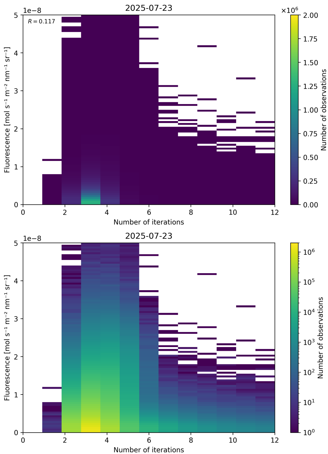
Figure 98: Scatter density plot of “Number of iterations” against “Fluorescence” for 2025-07-22 to 2025-07-24.
