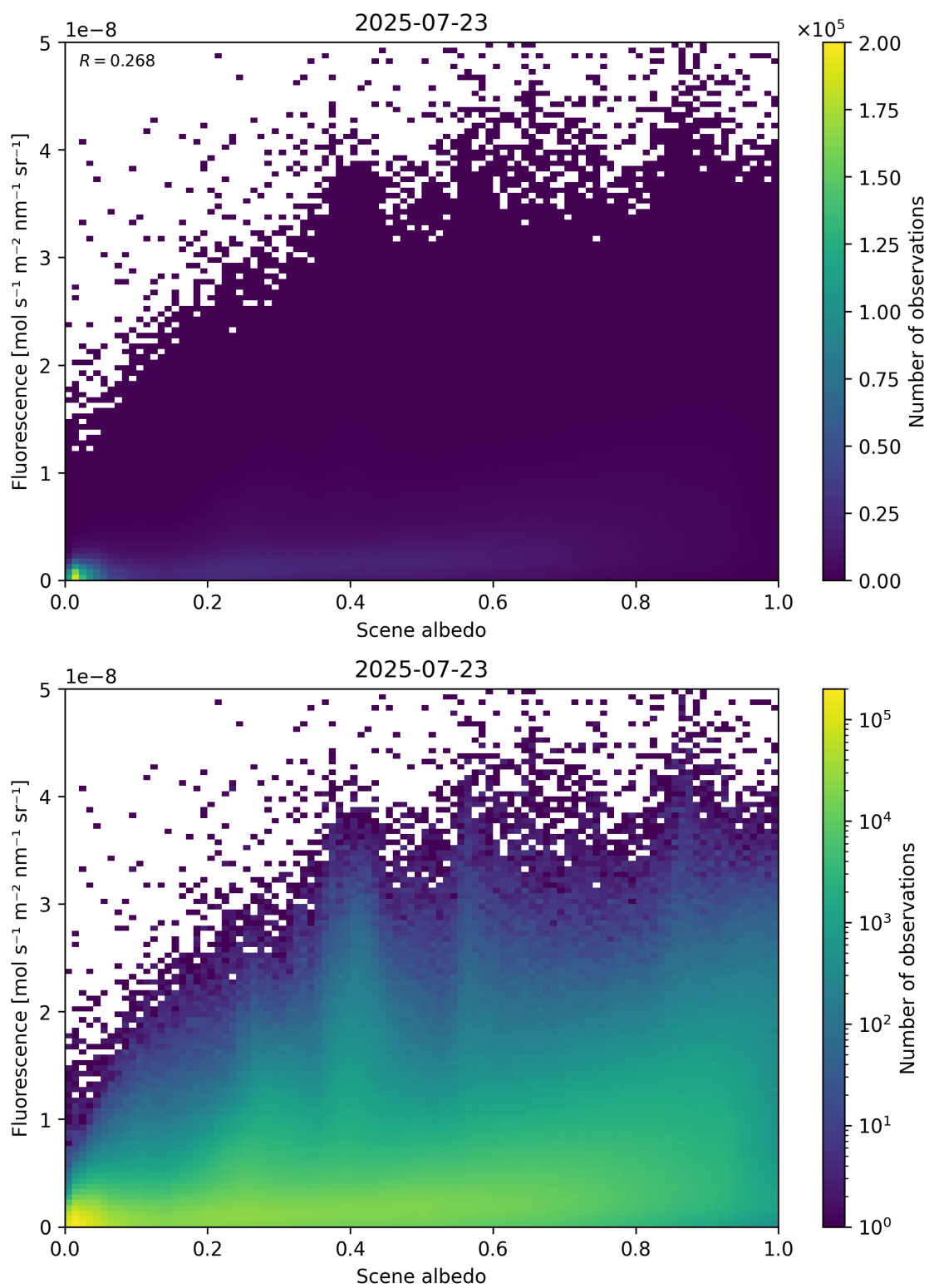
Figure 104: Scatter density plot of “Scene albedo” against “Fluorescence” for 2025-07-22 to 2025-07-24.
