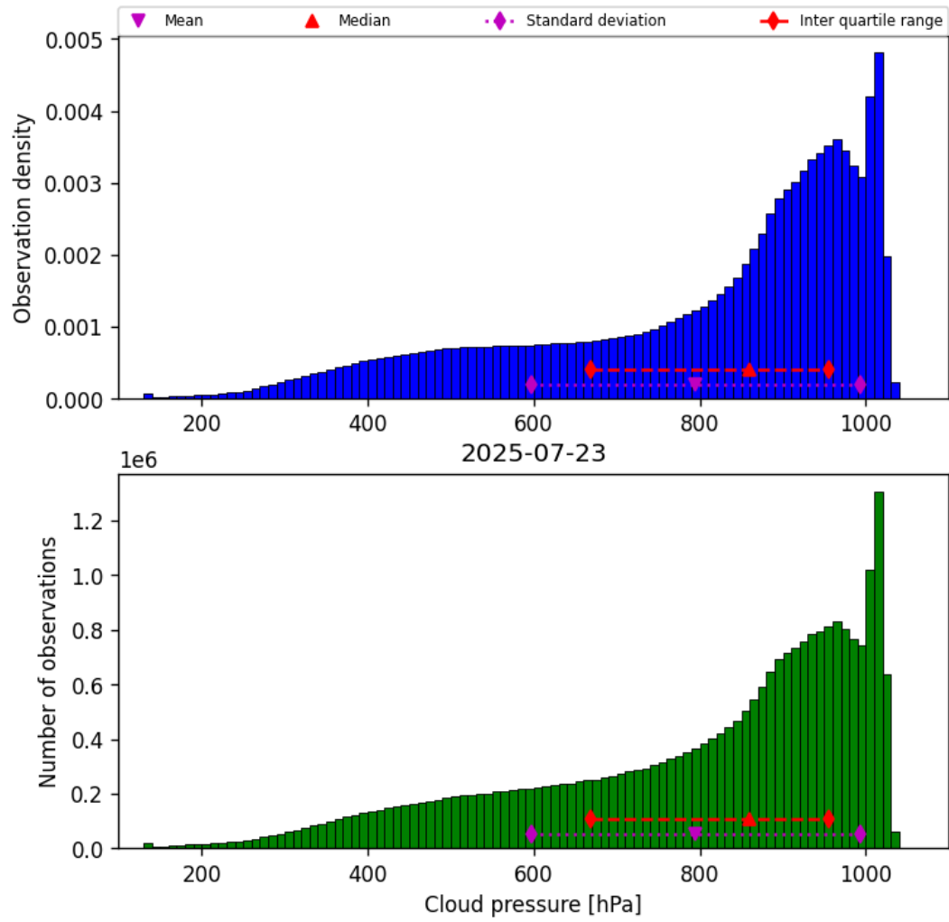
Figure 30: Histogram of “Cloud pressure” for 2025-07-22 to 2025-07-24
