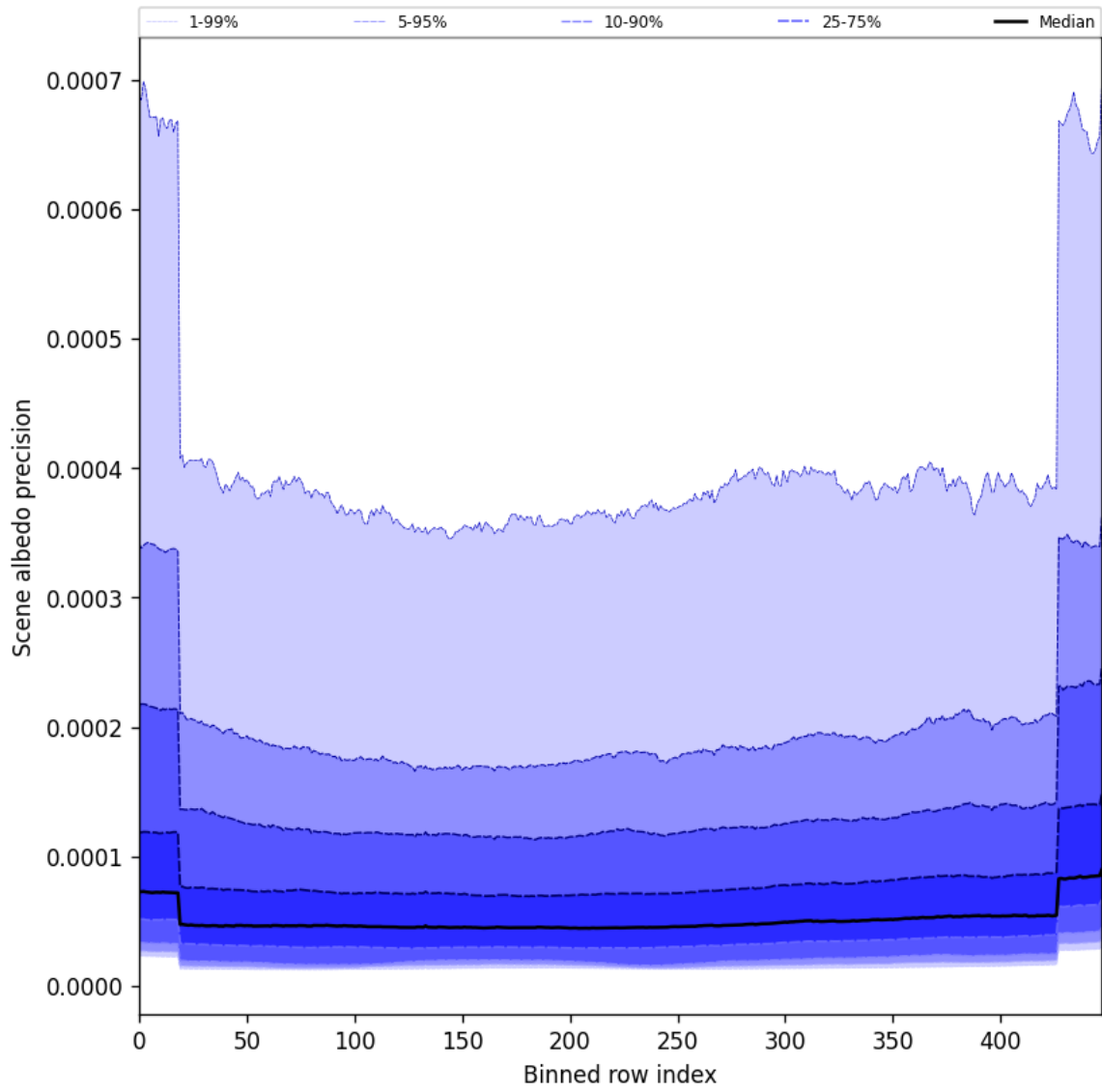
Figure 52: Along track statistics of “Scene albedo precision” for 2025-07-22 to 2025-07-24
