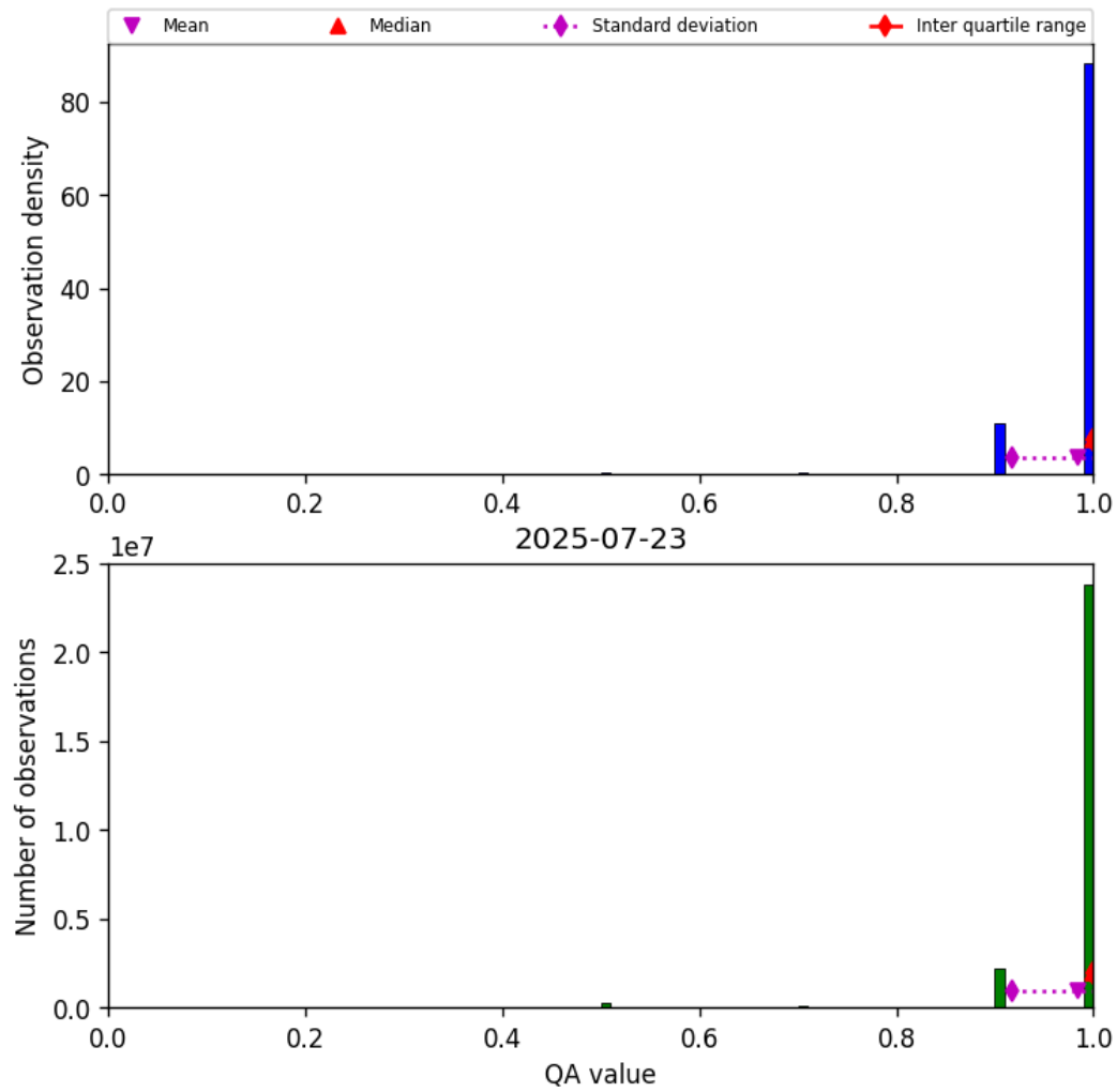
Figure 29: Histogram of “QA value” for 2025-07-22 to 2025-07-24
