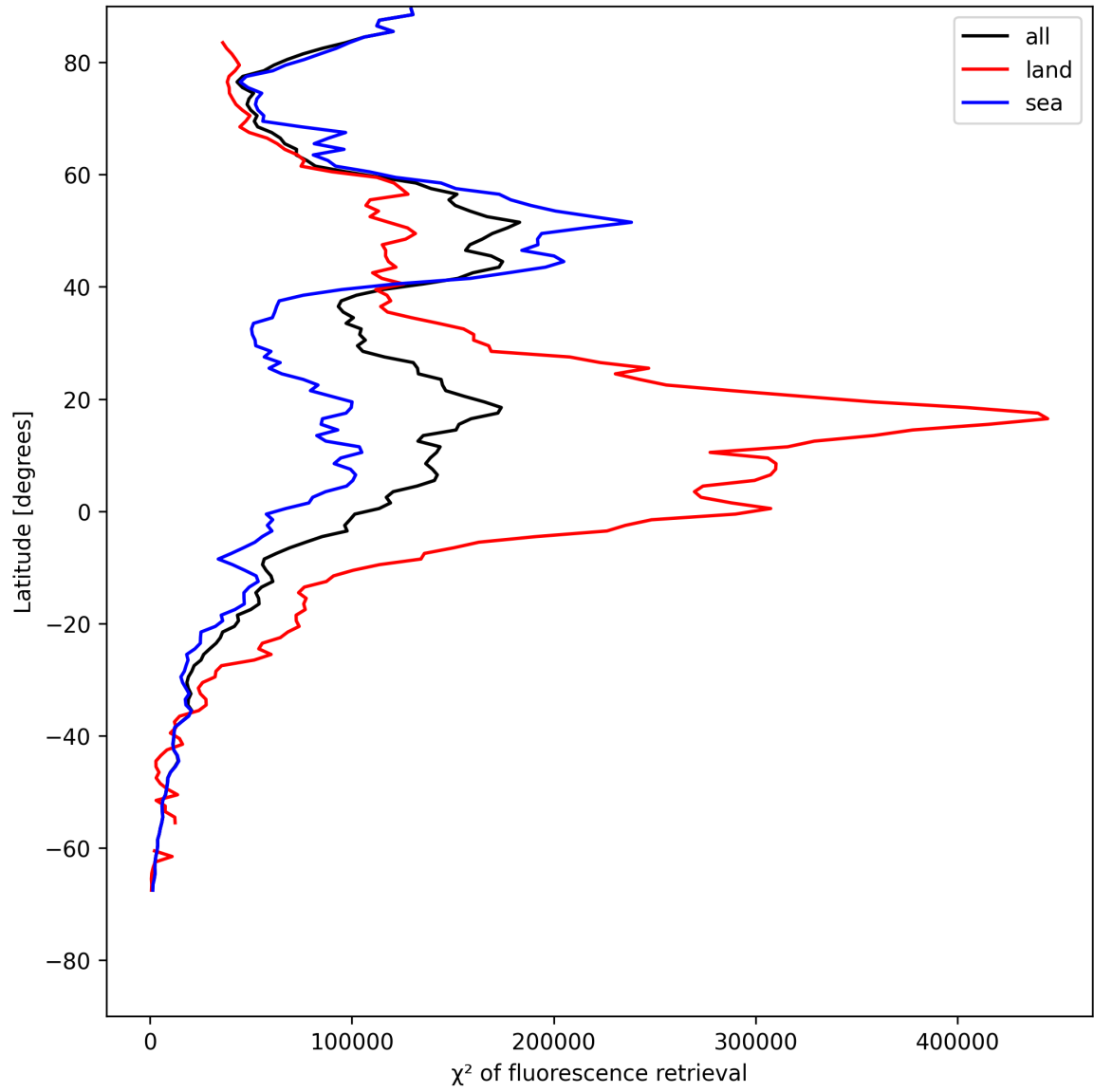
Figure 25: Zonal average of “ \chi^2 of fluorescence retrieval” for 2025-07-22 to 2025-07-24.
