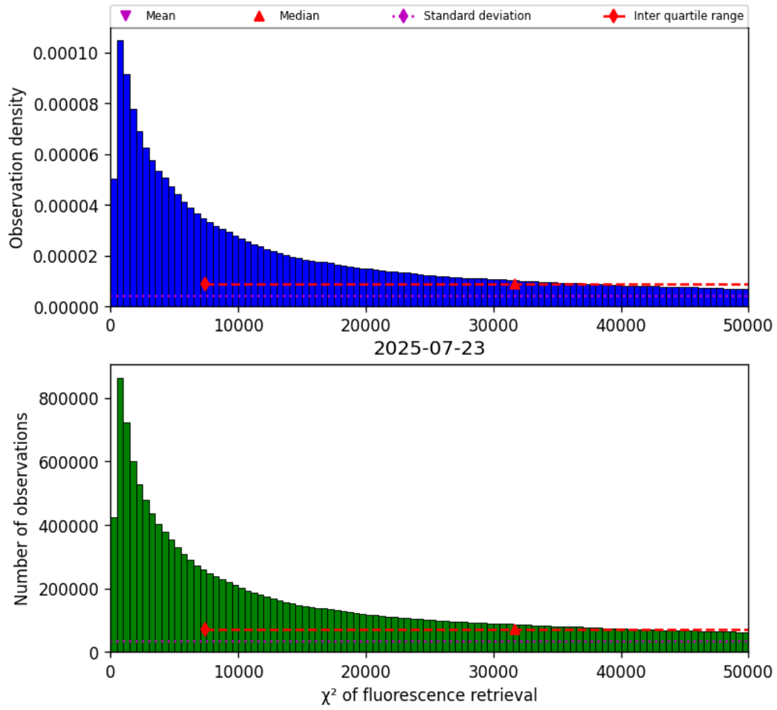
Figure 42: Histogram of “ \chi^2 of fluorescence retrieval” for 2025-07-22 to 2025-07-24
