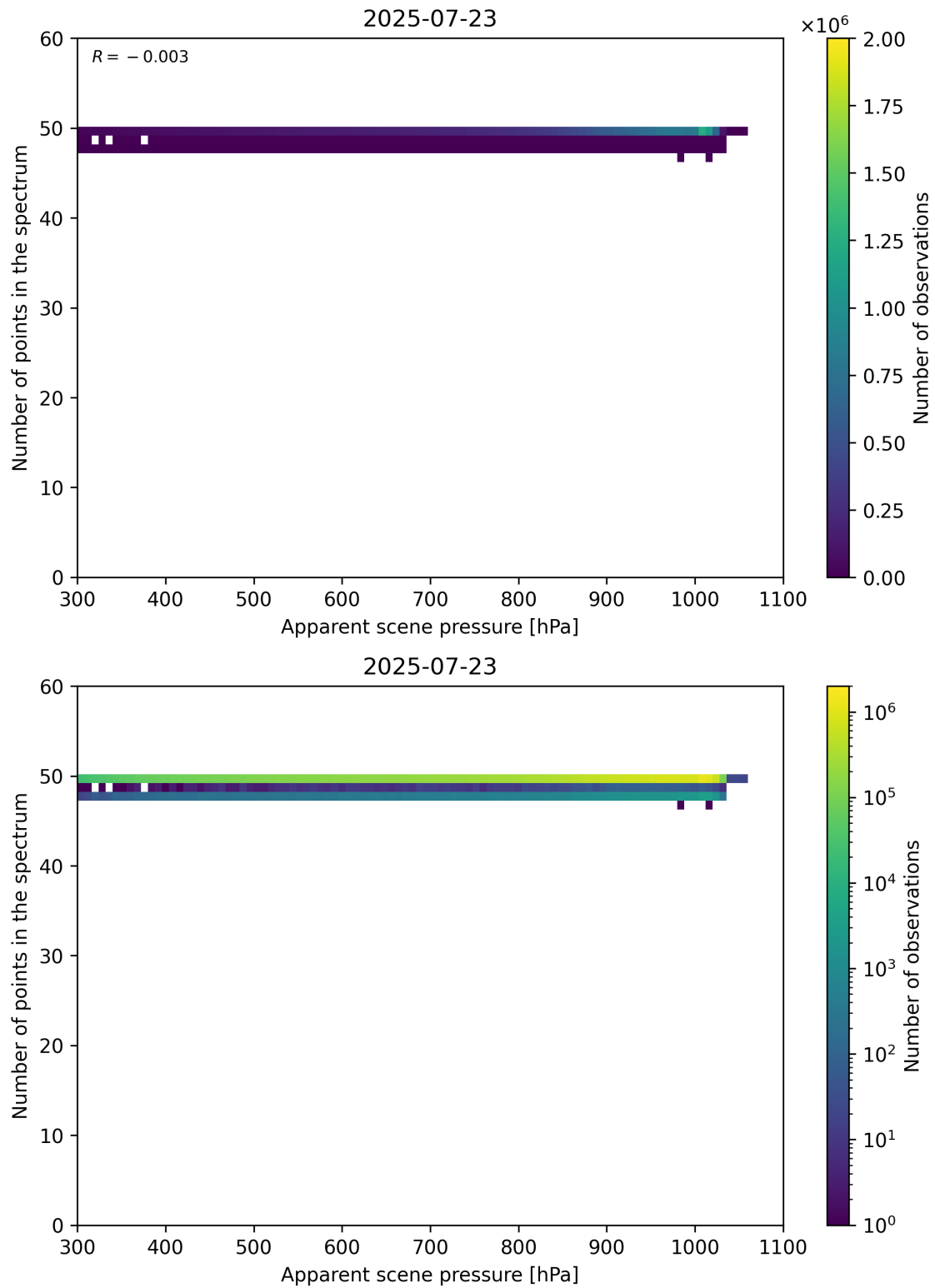
Figure 66: Scatter density plot of “Apparent scene pressure” against “Number of points in the spectrum” for 2025-07-22 to 2025-07-24.
