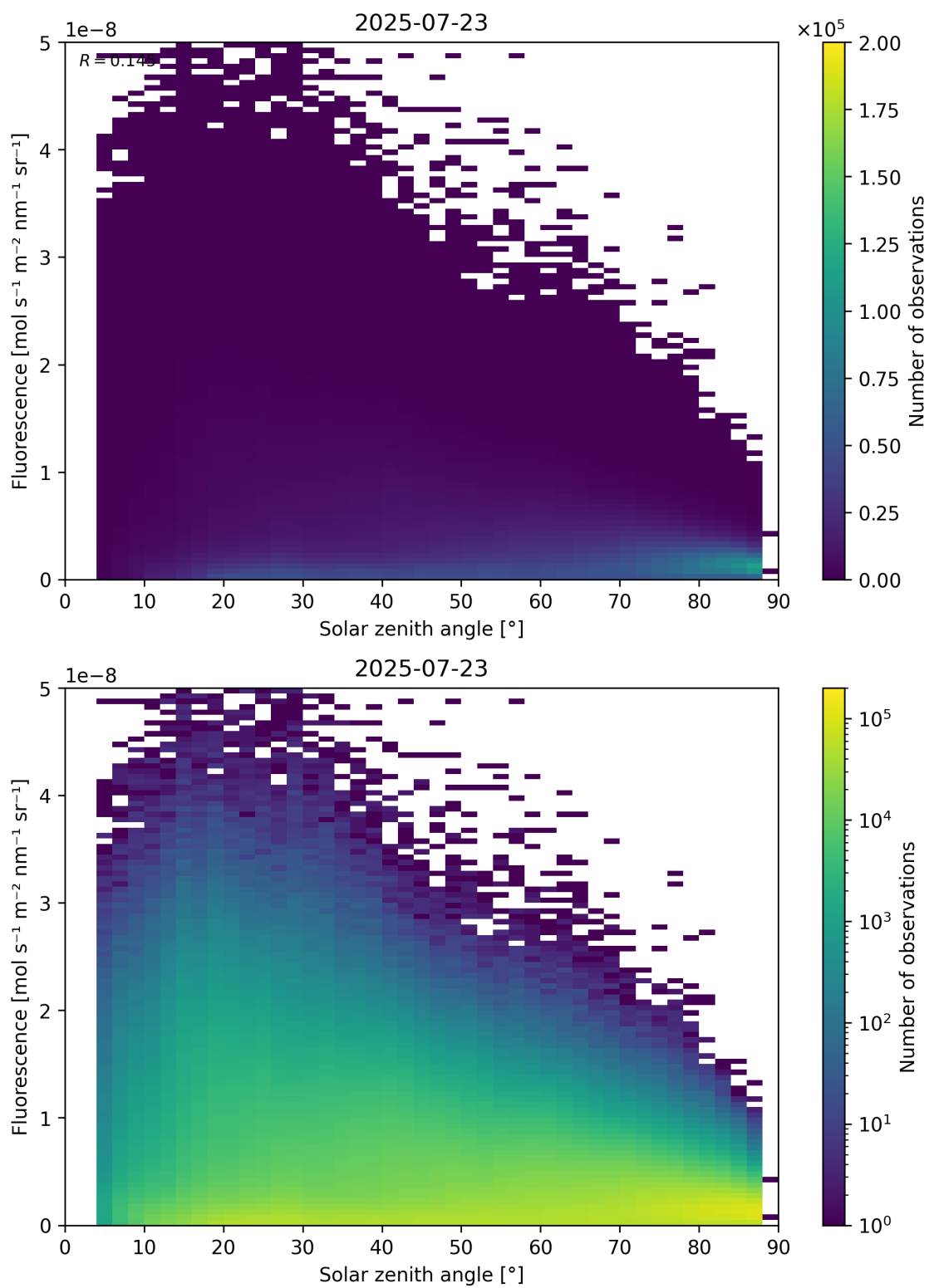
Figure 112: Scatter density plot of “Solar zenith angle” against “Fluorescence” for 2025-07-22 to 2025-07-24.
