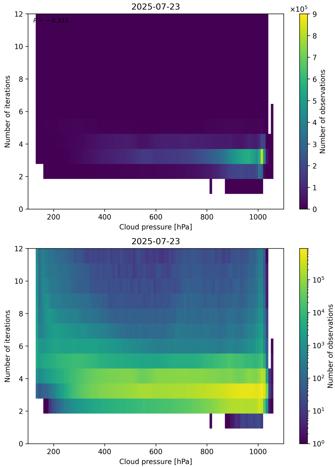
Figure 81: Scatter density plot of “Cloud pressure” against “Number of iterations” for 2025-07-22 to 2025-07-24.
