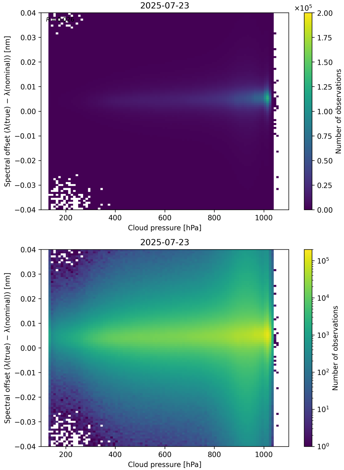
Figure 84: Scatter density plot of “Cloud pressure” against “Spectral offset ( \lambda_{\text{true}} - \lambda_{\text{nominal}} )” for 2025-07-22 to 2025-07-24.
