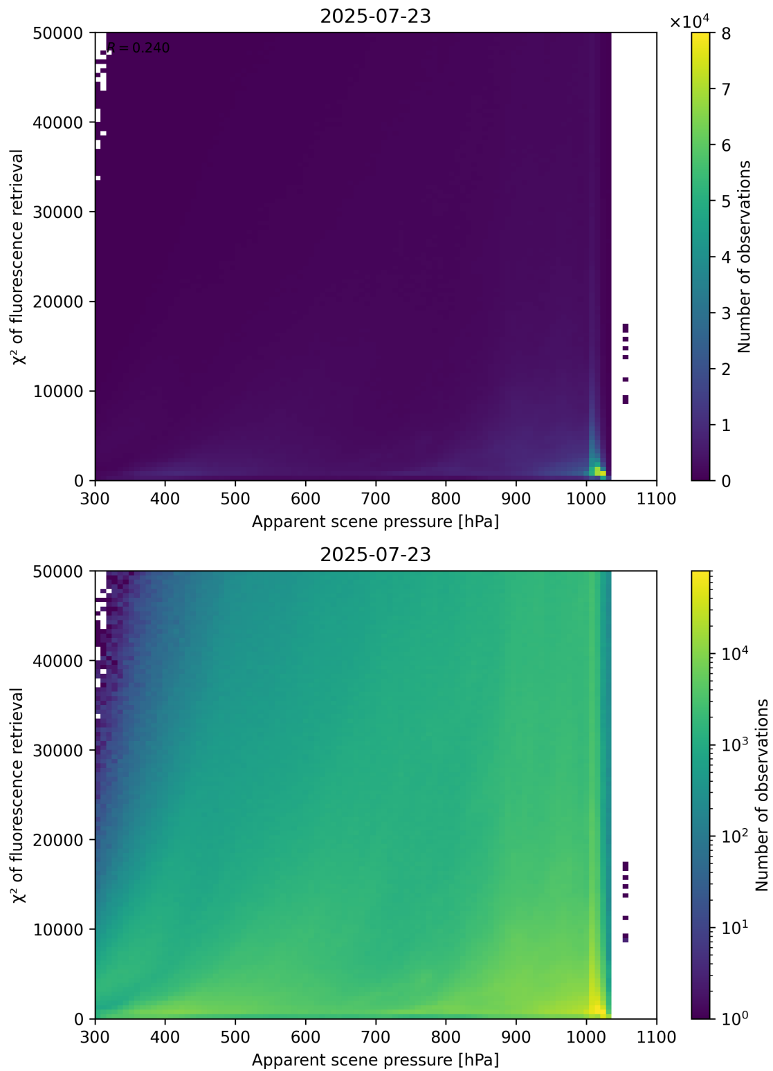
Figure 63: Scatter density plot of “Apparent scene pressure” against “ \chi^2 of fluorescence retrieval” for 2025-07-22 to 2025-07-24.
