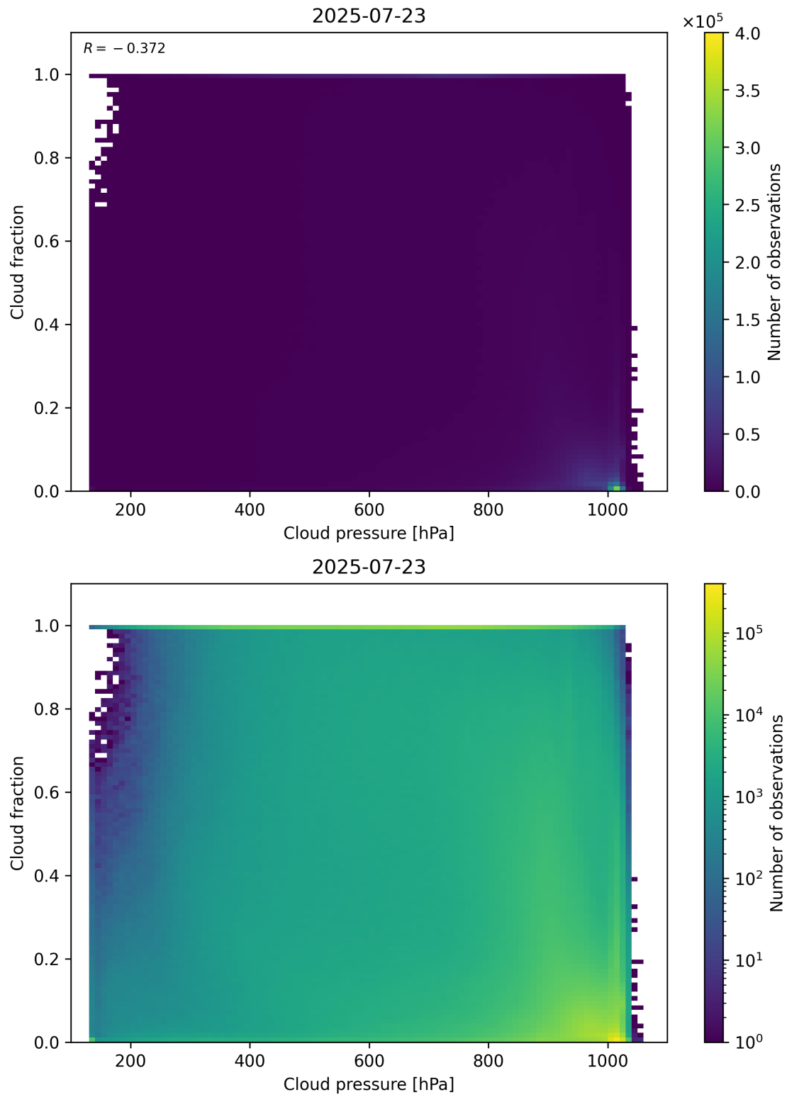
Figure 79: Scatter density plot of “Cloud pressure” against “Cloud fraction” for 2025-07-22 to 2025-07-24.
