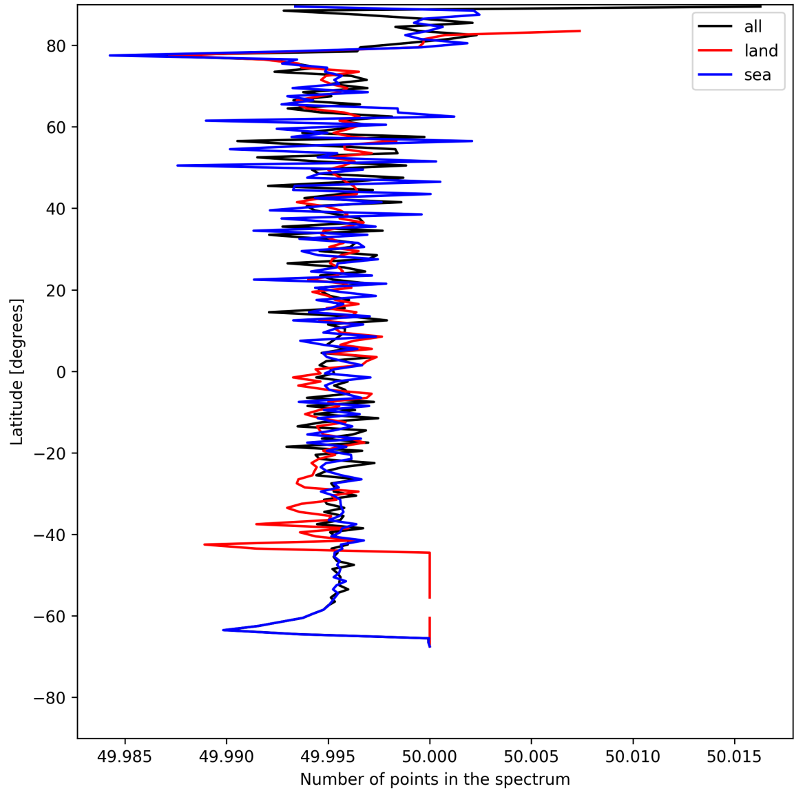
Figure 27: Zonal average of “Number of points in the spectrum” for 2025-07-22 to 2025-07-24.
