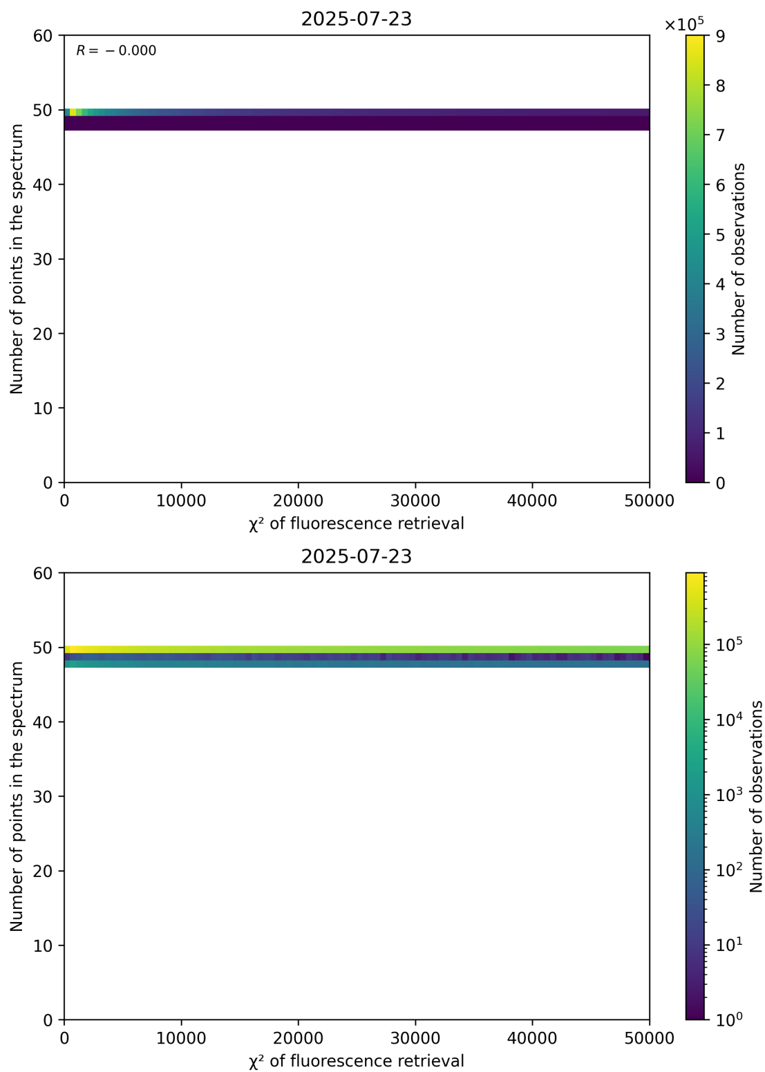
Figure 68: Scatter density plot of “ \chi^2 of fluorescence retrieval” against “Number of points in the spectrum” for 2025-07-22 to 2025-07-24.
