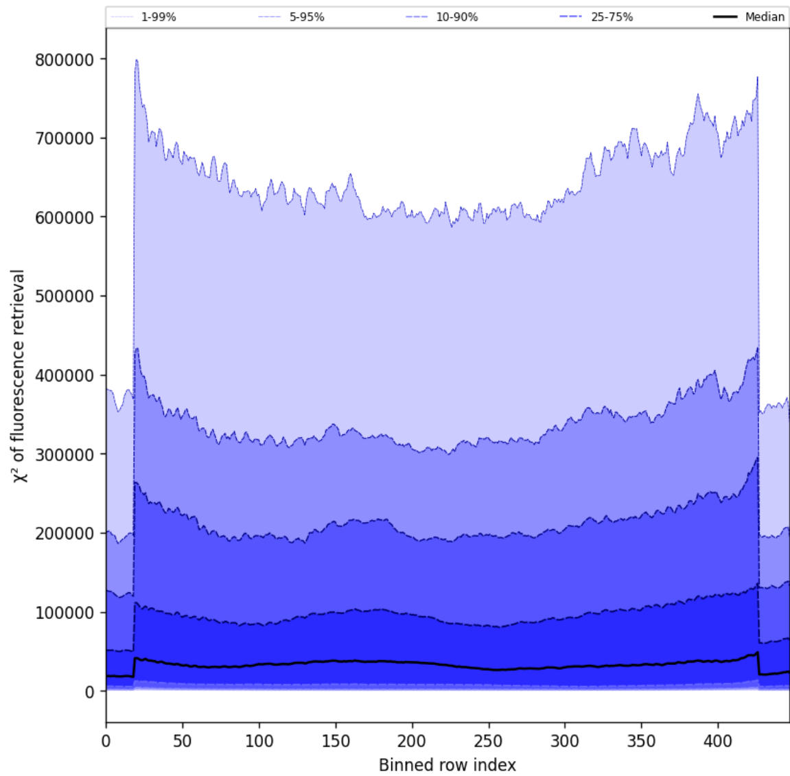
Figure 59: Along track statistics of “ \chi^2 of fluorescence retrieval” for 2025-07-22 to 2025-07-24
