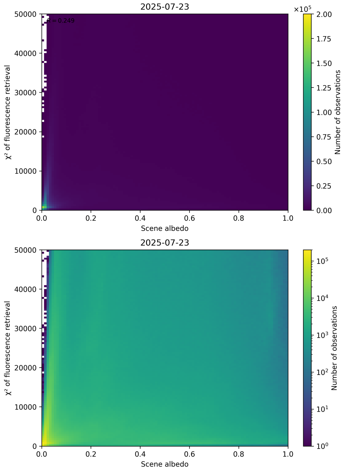
Figure 103: Scatter density plot of “Scene albedo” against “ \chi^2 of fluorescence retrieval” for 2025-07-22 to 2025-07-24.
