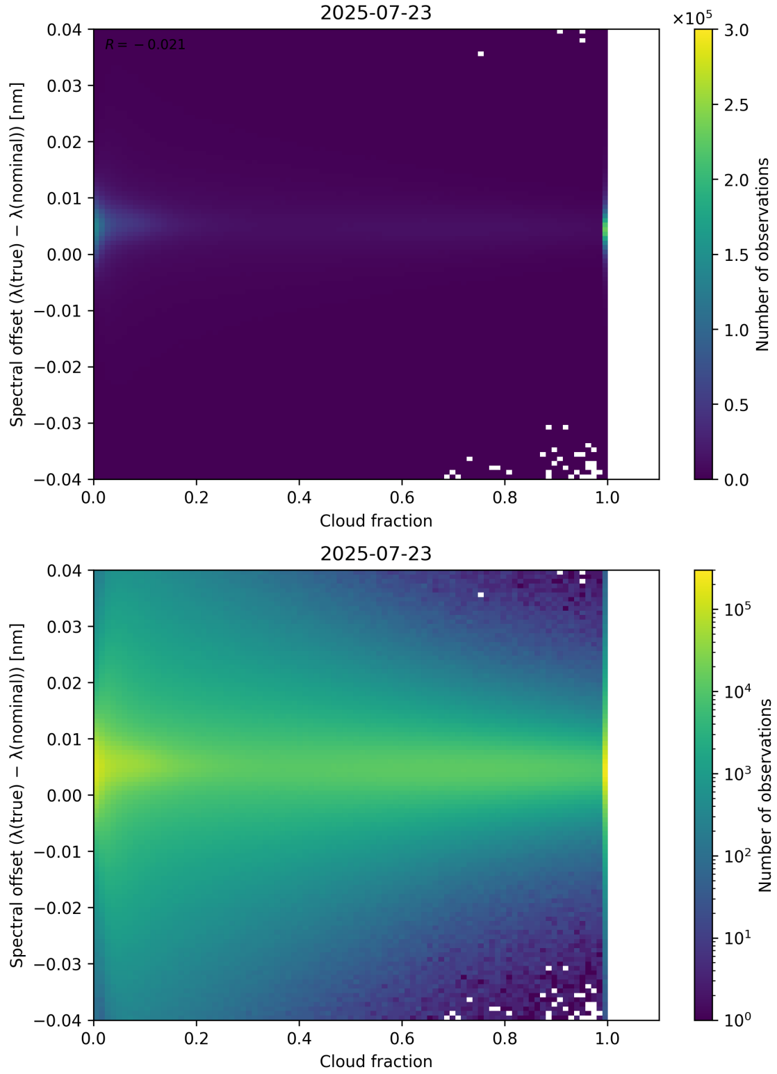
Figure 76: Scatter density plot of “Cloud fraction” against “Spectral offset ( \lambda_{\text{true}} - \lambda_{\text{nominal}} )” for 2025-07-22 to 2025-07-24.
