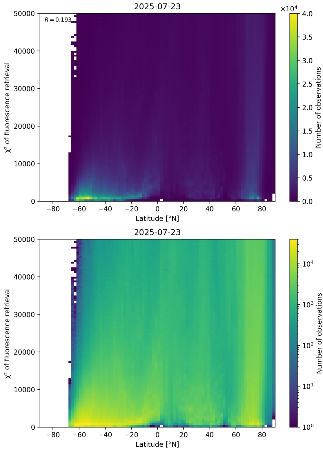
Figure 89: Scatter density plot of “Latitude” against “ \chi^2 of fluorescence retrieval” for 2025-07-22 to 2025-07-24.
