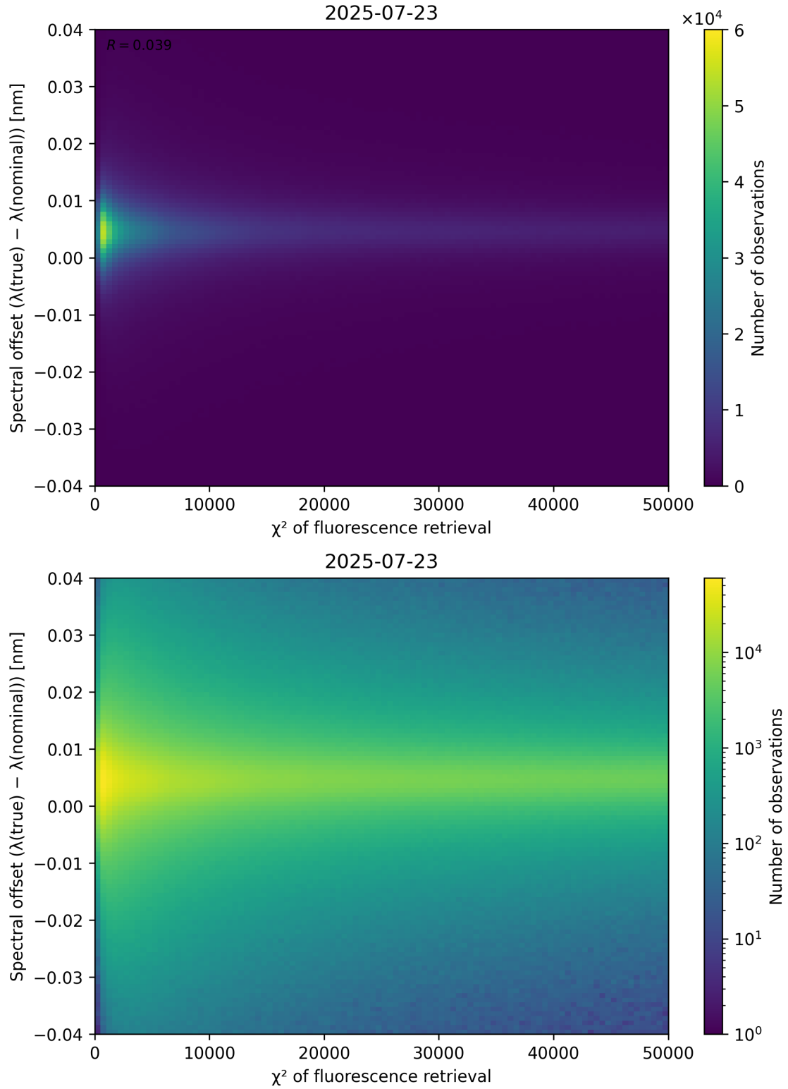
Figure 69: Scatter density plot of “ \chi^2 of fluorescence retrieval” against “Spectral offset ( \lambda_{\text{true}} - \lambda_{\text{nominal}} )” for 2025-07-22 to 2025-07-24.
