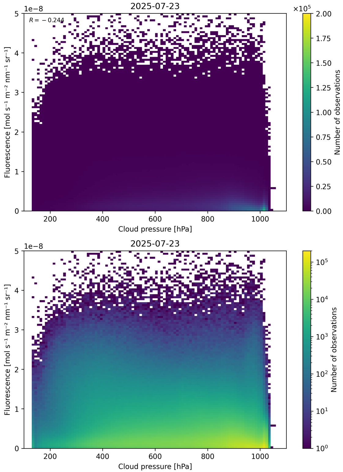
Figure 80: Scatter density plot of “Cloud pressure” against “Fluorescence” for 2025-07-22 to 2025-07-24.
