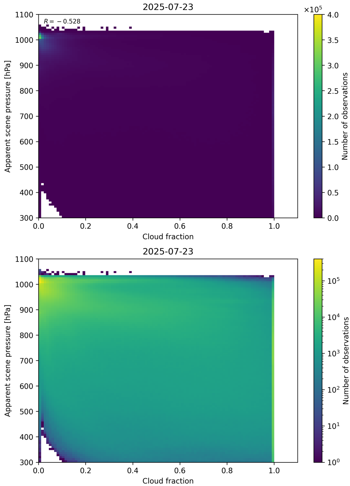
Figure 70: Scatter density plot of “Cloud fraction” against “Apparent scene pressure” for 2025-07-22 to 2025-07-24.
