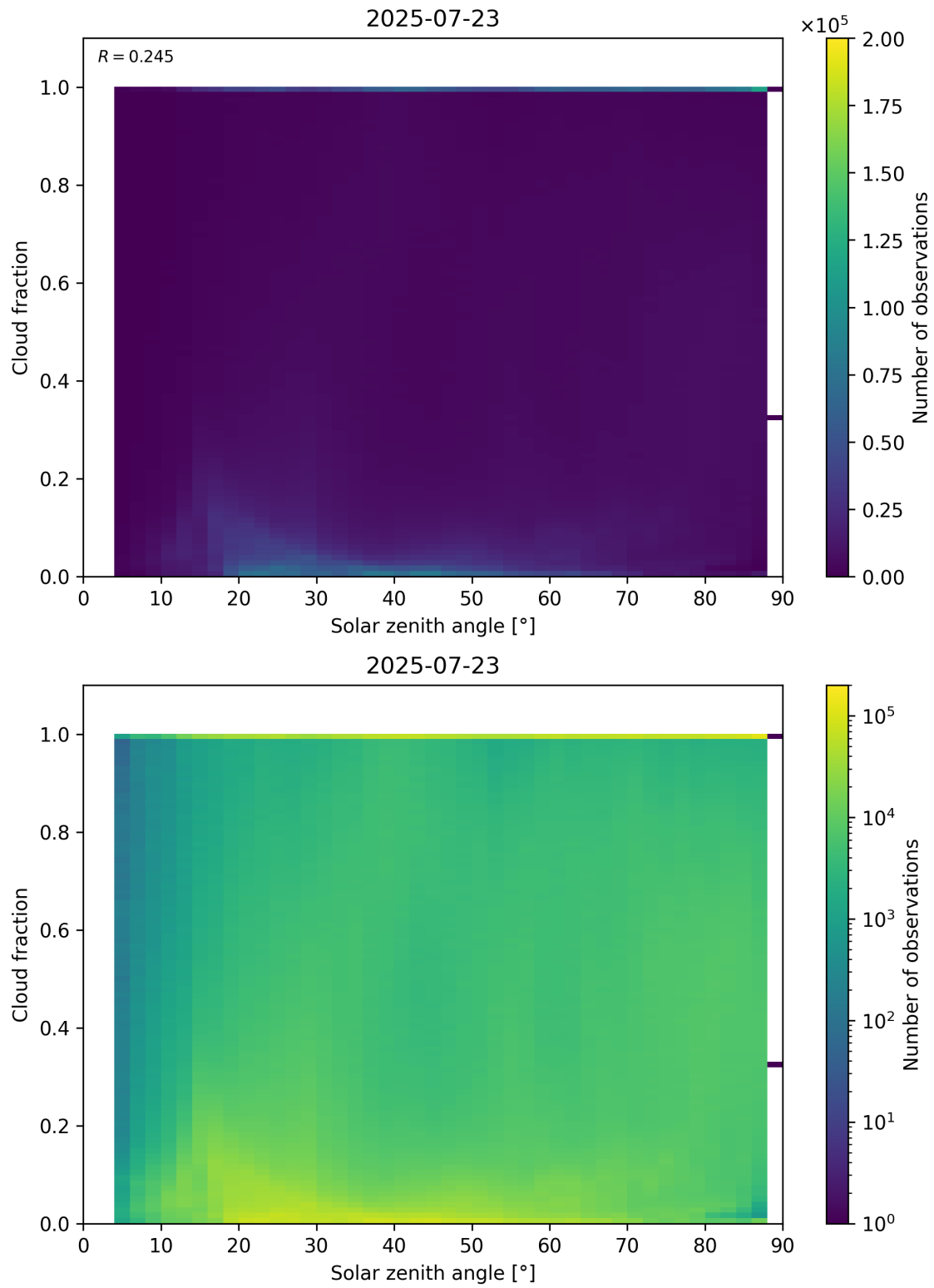
Figure 110: Scatter density plot of “Solar zenith angle” against “Cloud fraction” for 2025-07-22 to 2025-07-24.
