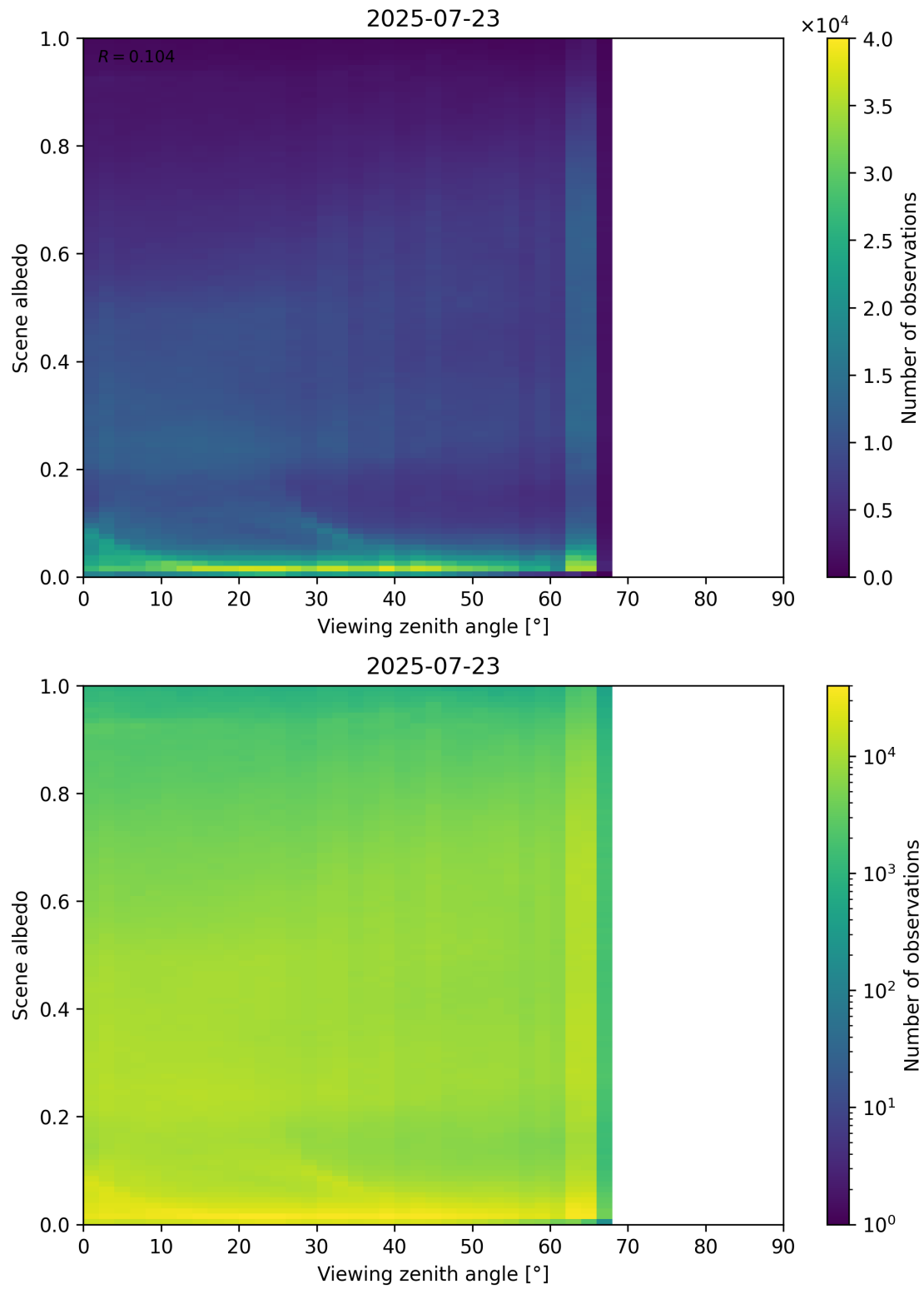
Figure 126: Scatter density plot of “Viewing zenith angle” against “Scene albedo” for 2025-07-22 to 2025-07-24.
