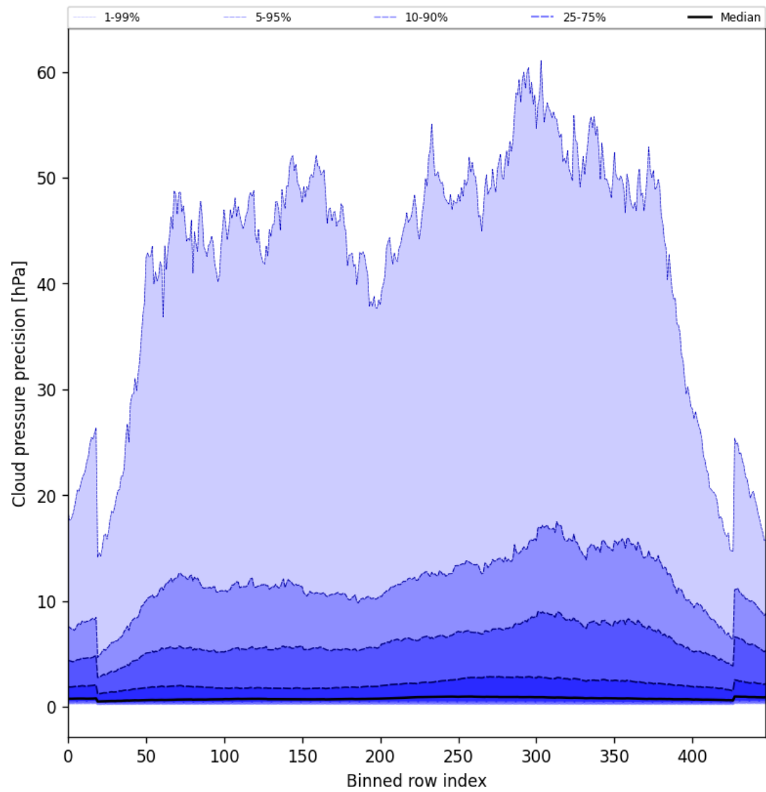
Figure 48: Along track statistics of “Cloud pressure precision” for 2025-07-22 to 2025-07-24
