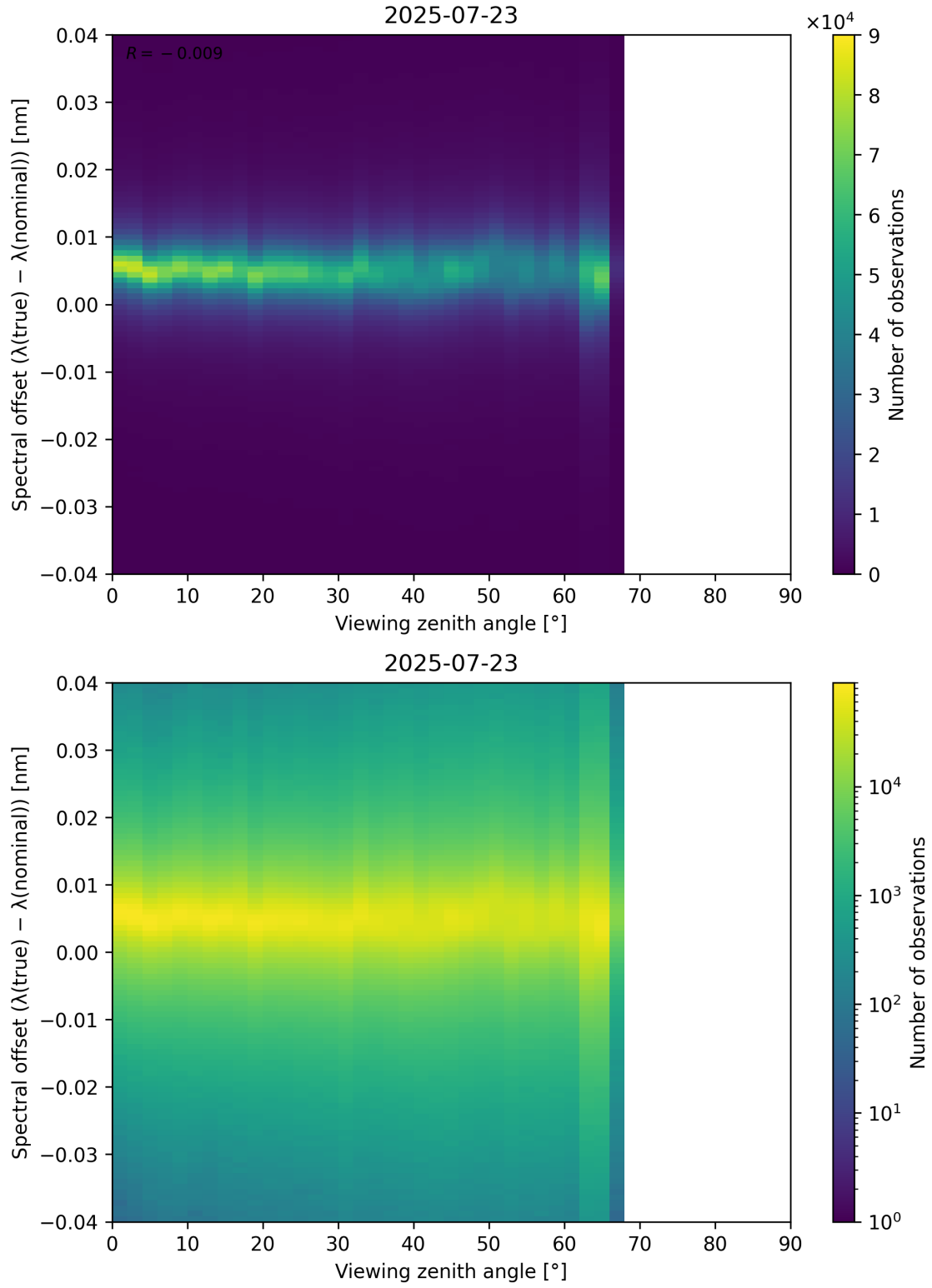
Figure 128: Scatter density plot of “Viewing zenith angle” against “Spectral offset ( \lambda_{\text{true}} - \lambda_{\text{nominal}} )” for 2025-07-22 to 2025-07-24.
