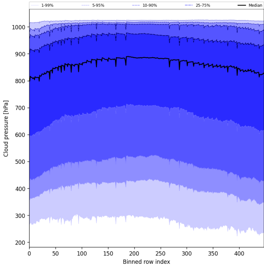
Figure 47: Along track statistics of “Cloud pressure” for 2025-07-22 to 2025-07-24
