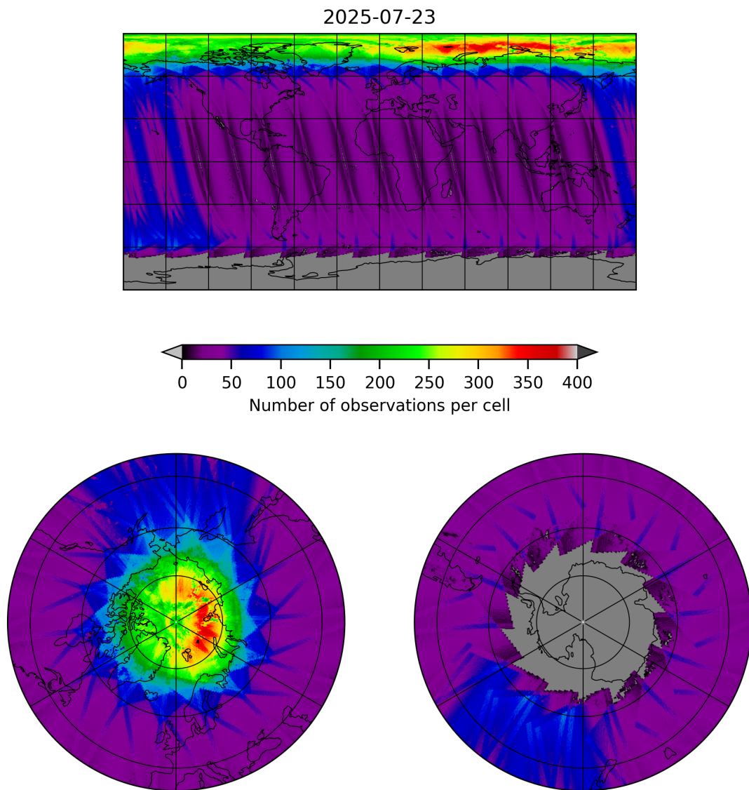
Figure 11: Map of the number of observations for 2025-07-22 to 2025-07-24
