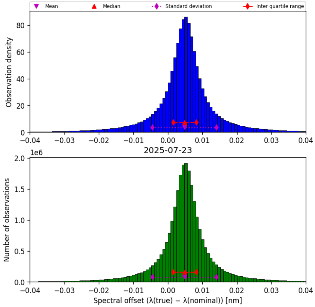
Figure 45: Histogram of “Spectral offset ( \lambda_{\text{true}} - \lambda_{\text{nominal}} )” for 2025-07-22 to 2025-07-24
