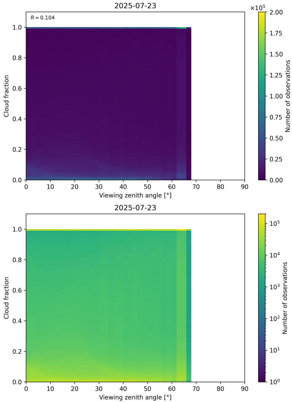
Figure 120: Scatter density plot of “Viewing zenith angle” against “Cloud fraction” for 2025-07-22 to 2025-07-24.
