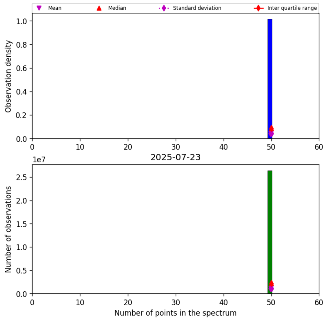
Figure 44: Histogram of “Number of points in the spectrum” for 2025-07-22 to 2025-07-24
