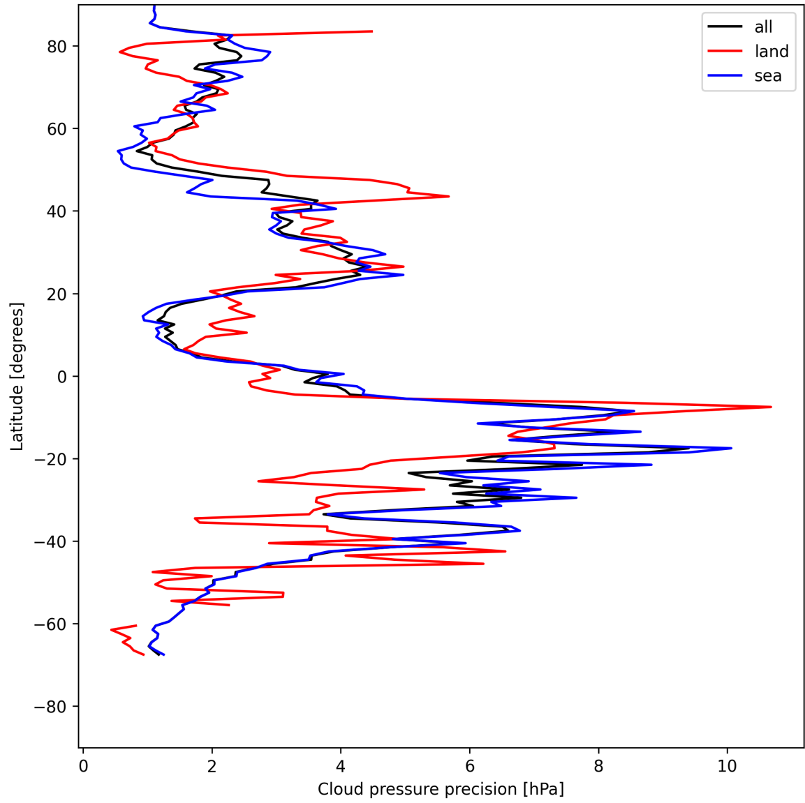
Figure 14: Zonal average of “Cloud pressure precision” for 2025-07-22 to 2025-07-24.
