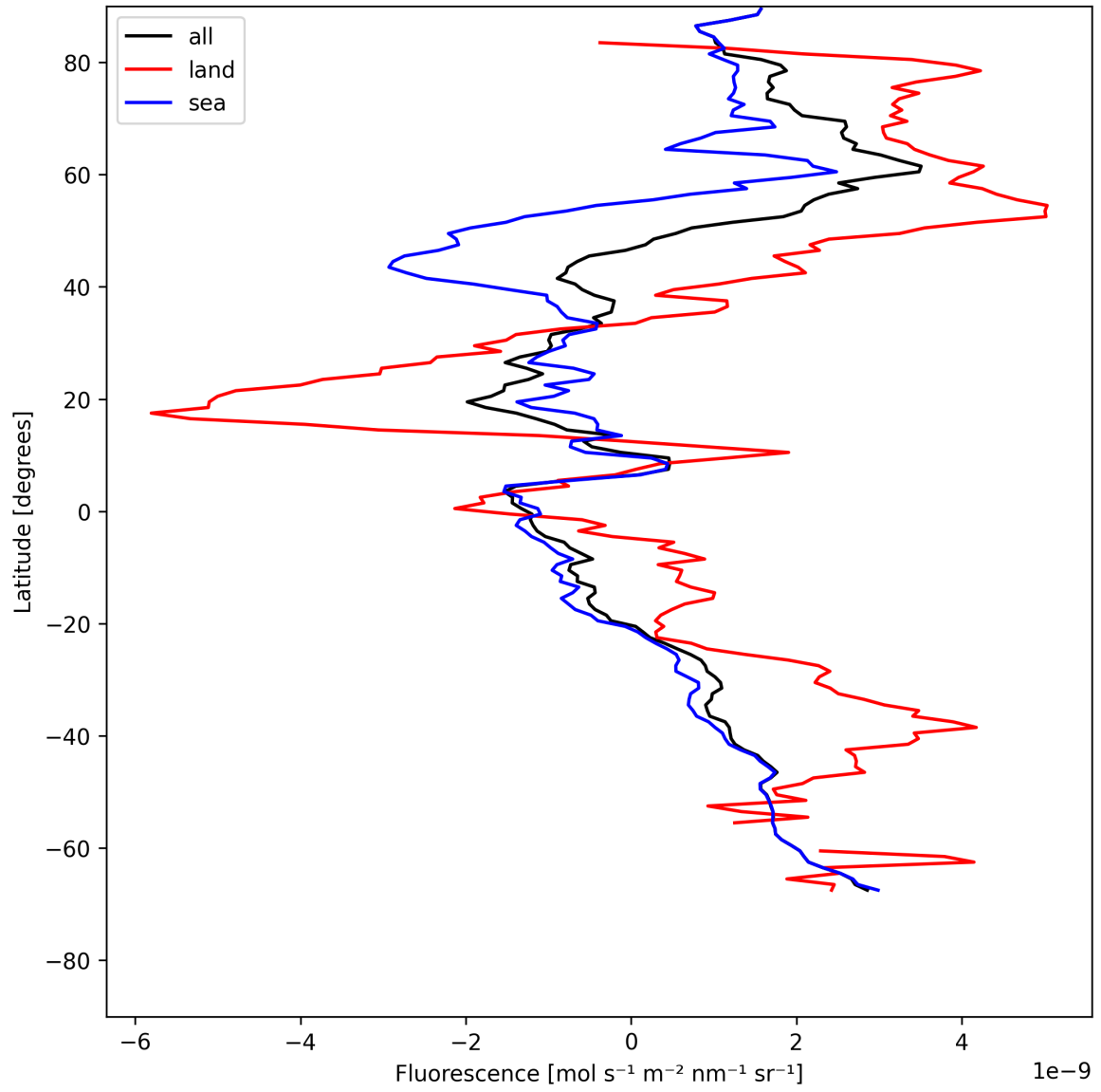
Figure 23: Zonal average of “Fluorescence” for 2025-07-22 to 2025-07-24.
