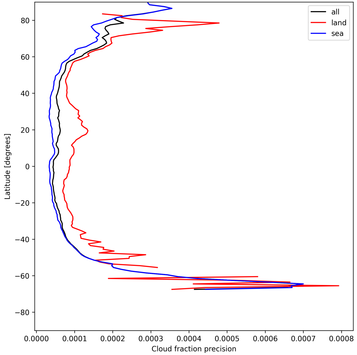
Figure 16: Zonal average of “Cloud fraction precision” for 2025-07-22 to 2025-07-24.
