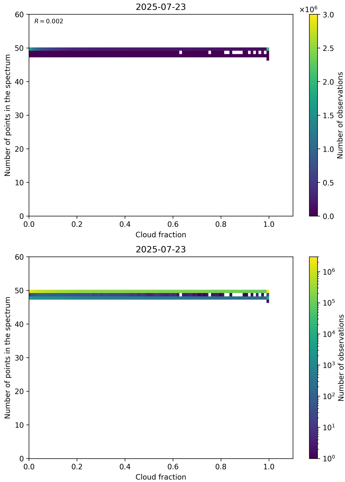
Figure 74: Scatter density plot of “Cloud fraction” against “Number of points in the spectrum” for 2025-07-22 to 2025-07-24.
