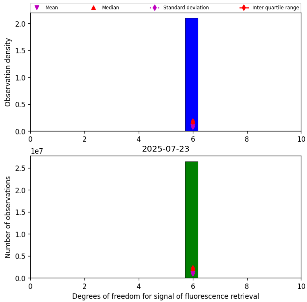
Figure 43: Histogram of “Degrees of freedom for signal of fluorescence retrieval” for 2025-07-22 to 2025-07-24
