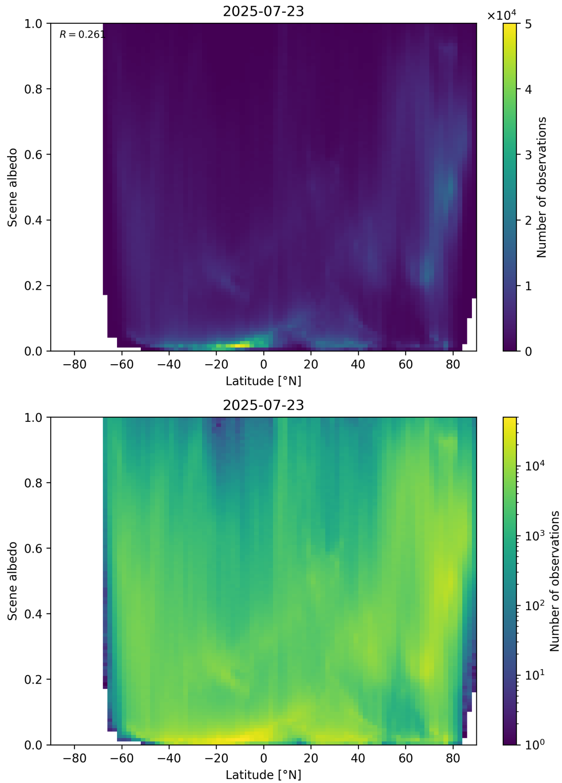
Figure 95: Scatter density plot of “Latitude” against “Scene albedo” for 2025-07-22 to 2025-07-24.
