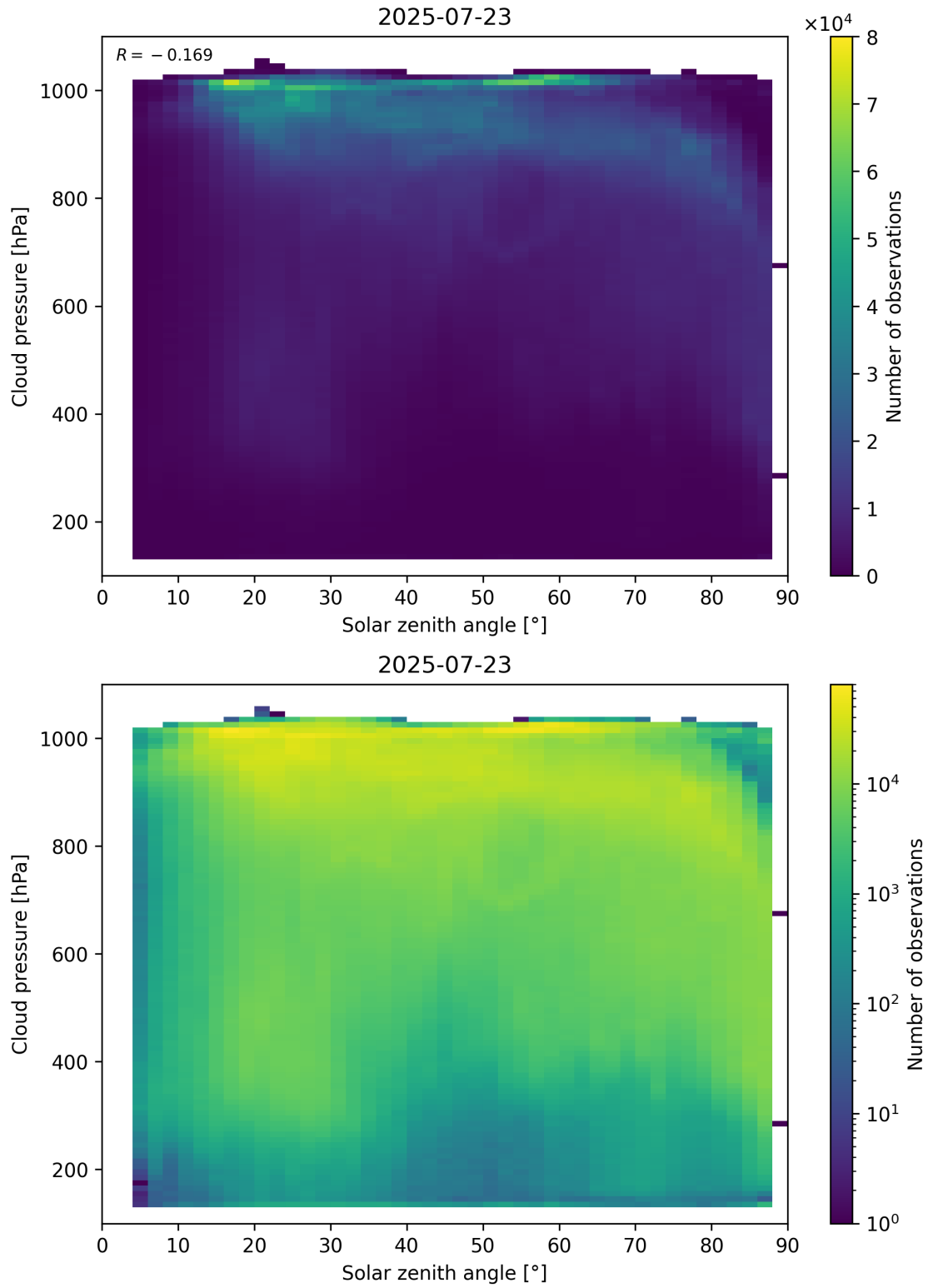
Figure 111: Scatter density plot of “Solar zenith angle” against “Cloud pressure” for 2025-07-22 to 2025-07-24.
