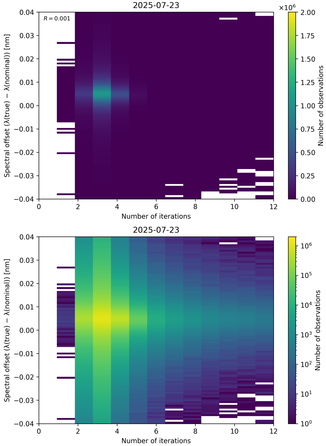
Figure 100: Scatter density plot of “Number of iterations” against “Spectral offset ( \lambda_{\text{true}} - \lambda_{\text{nominal}} )” for 2025-07-22 to 2025-07-24.
