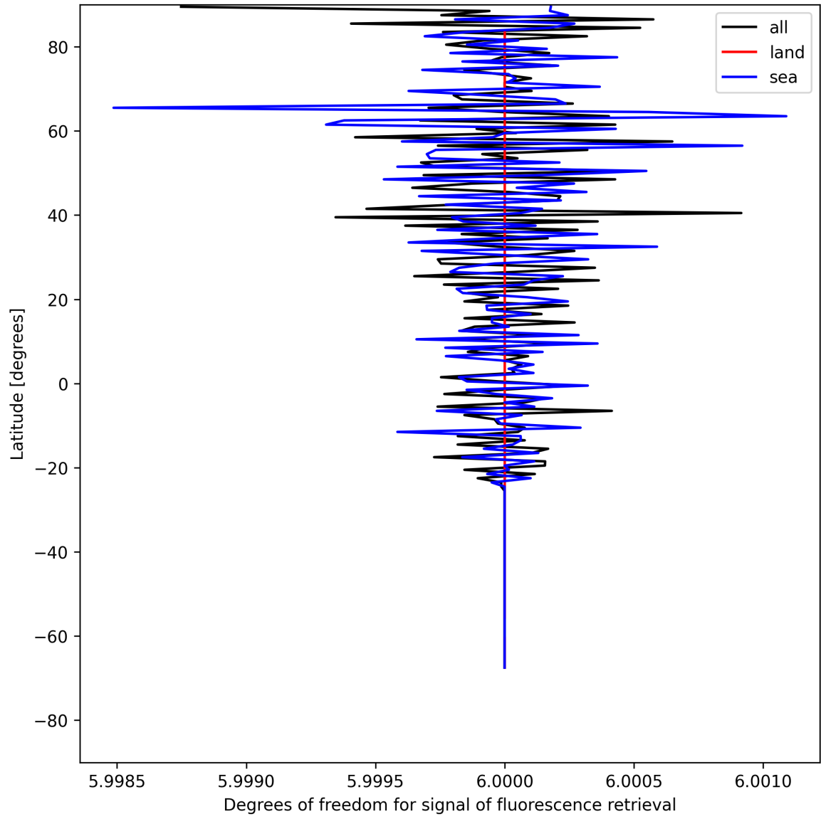
Figure 26: Zonal average of “Degrees of freedom for signal of fluorescence retrieval” for 2025-07-22 to 2025-07-24.
