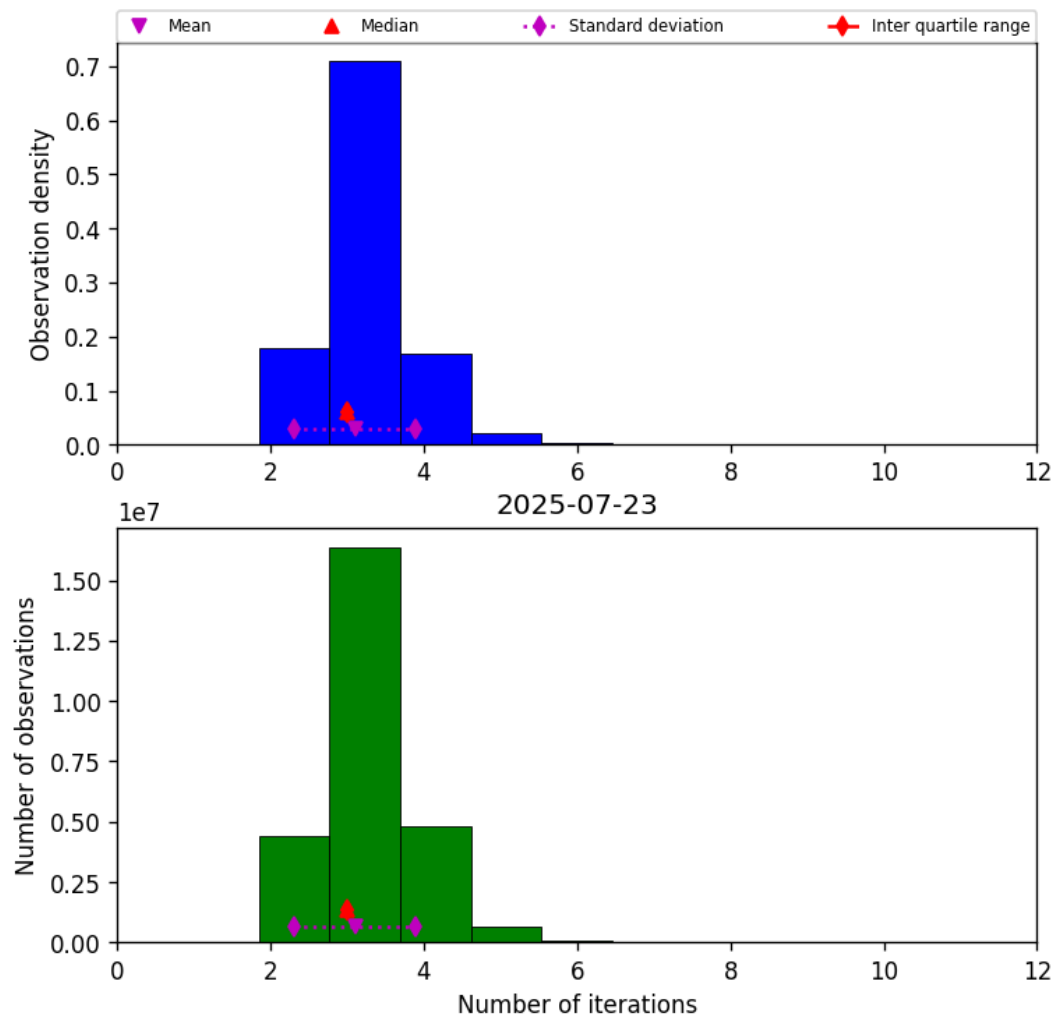
Figure 39: Histogram of “Number of iterations” for 2025-07-22 to 2025-07-24
