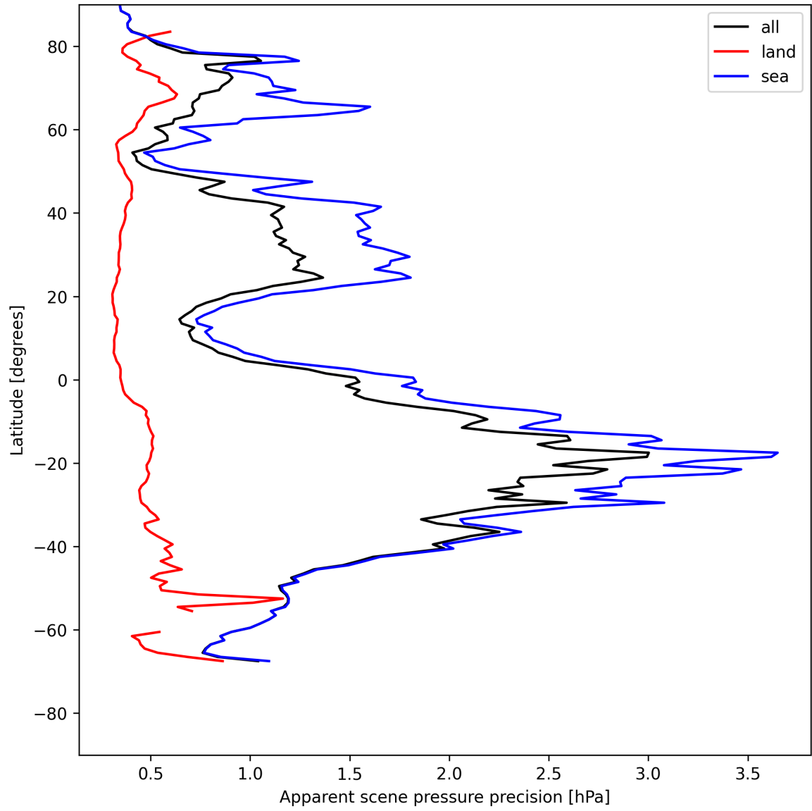
Figure 20: Zonal average of “Apparent scene pressure precision” for 2025-07-22 to 2025-07-24.
