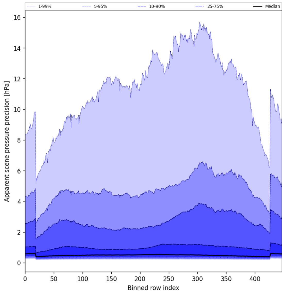
Figure 54: Along track statistics of “Apparent scene pressure precision” for 2025-07-22 to 2025-07-24
