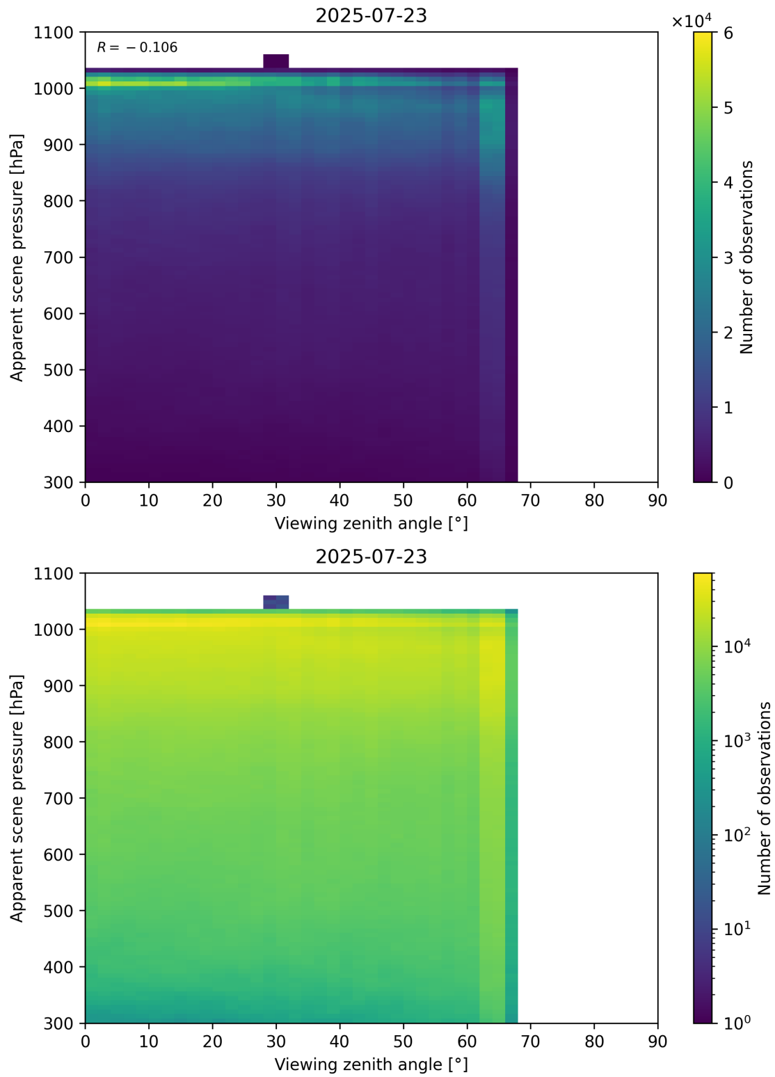
Figure 118: Scatter density plot of “Viewing zenith angle” against “Apparent scene pressure” for 2025-07-22 to 2025-07-24.
