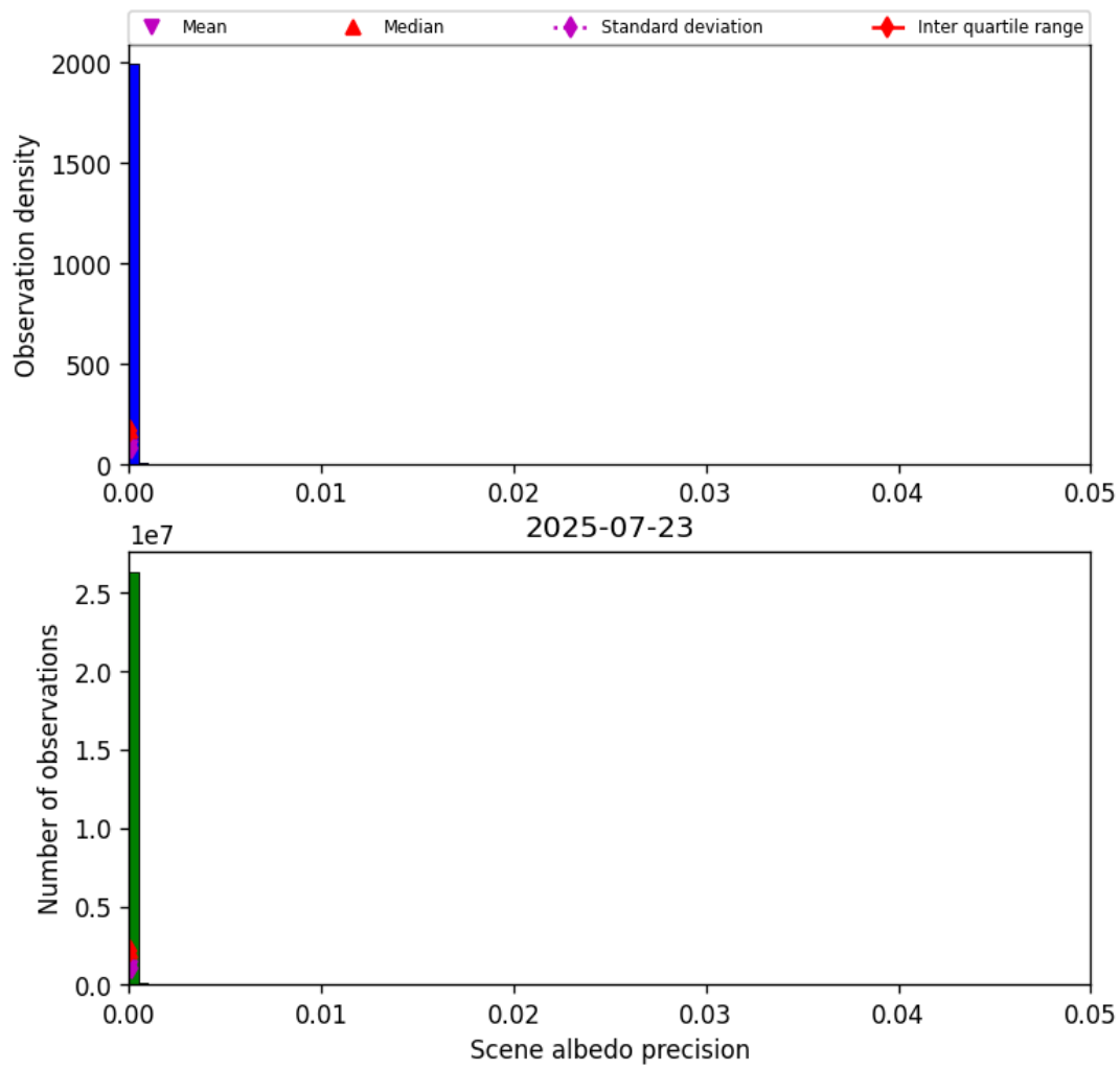
Figure 35: Histogram of “Scene albedo precision” for 2025-07-22 to 2025-07-24
