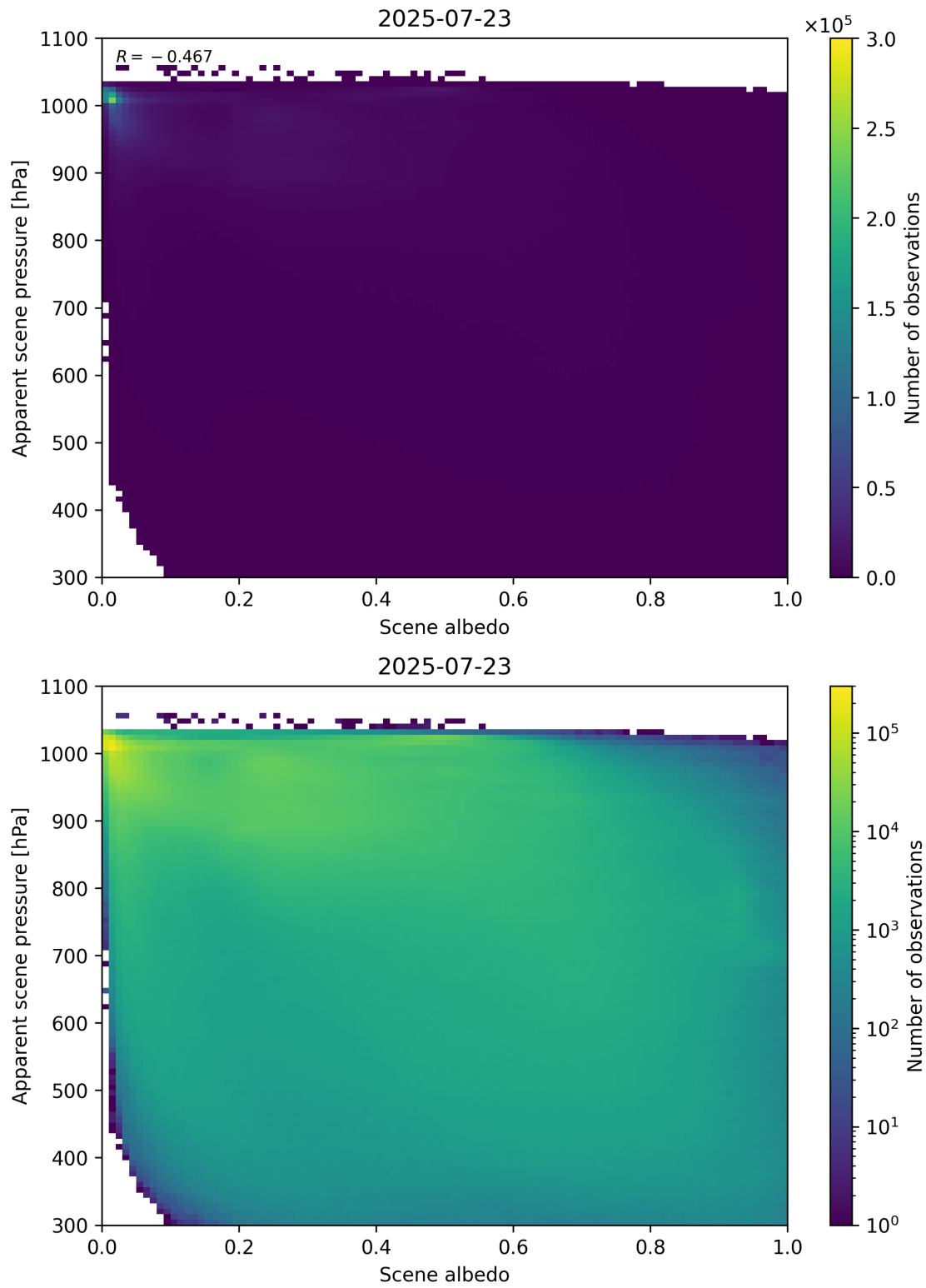
Figure 102: Scatter density plot of “Scene albedo” against “Apparent scene pressure” for 2025-07-22 to 2025-07-24.
