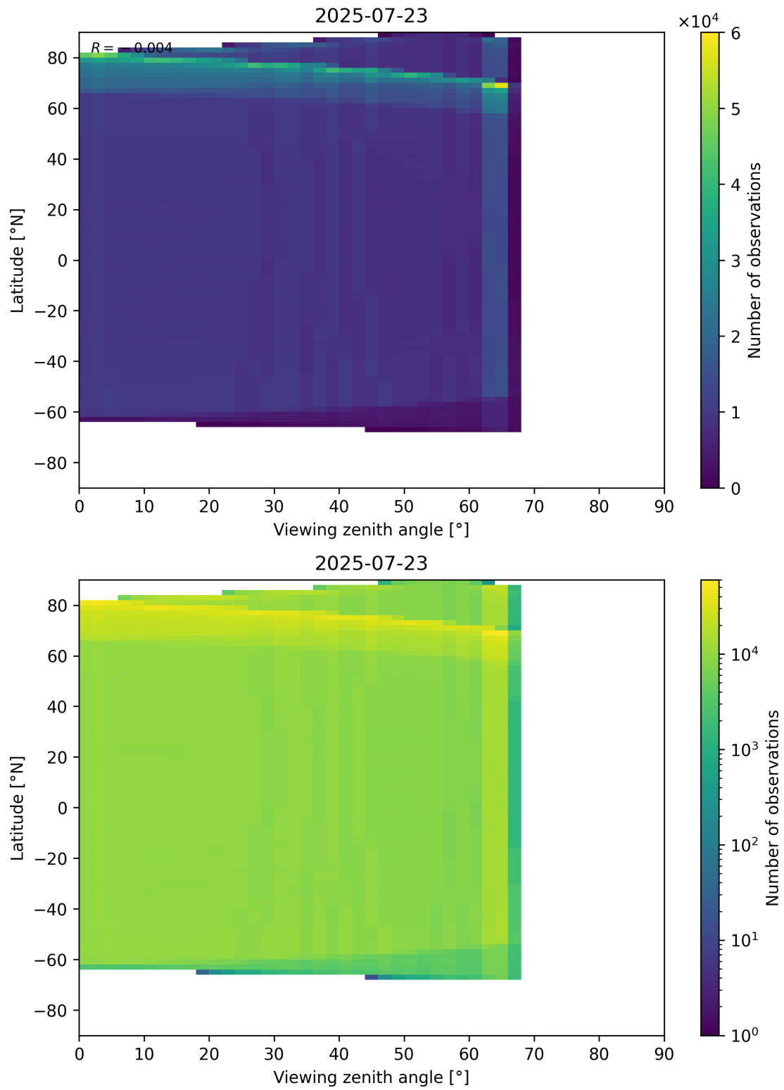
Figure 123: Scatter density plot of “Viewing zenith angle” against “Latitude” for 2025-07-22 to 2025-07-24.
