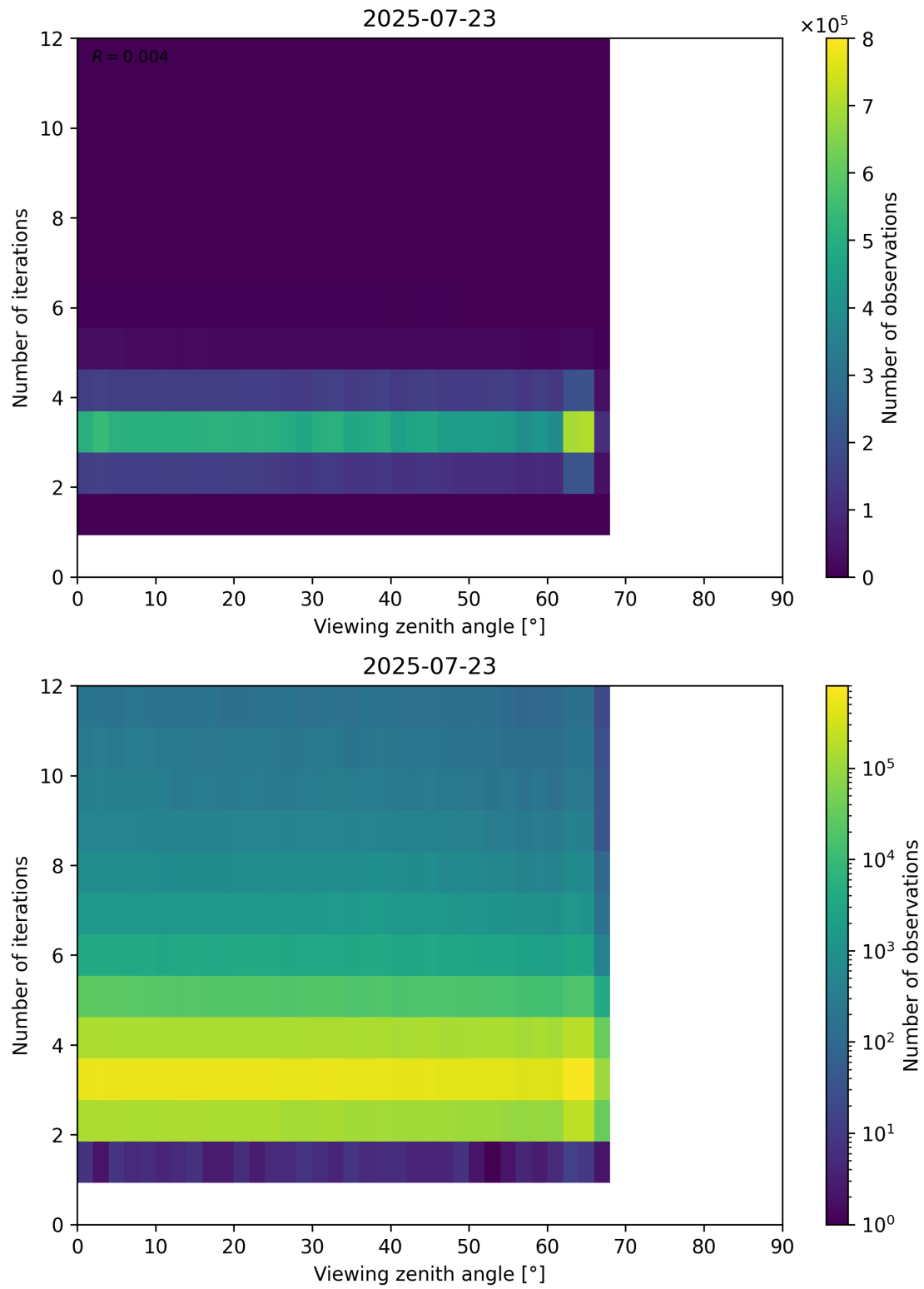
Figure 124: Scatter density plot of “Viewing zenith angle” against “Number of iterations” for 2025-07-22 to 2025-07-24.
