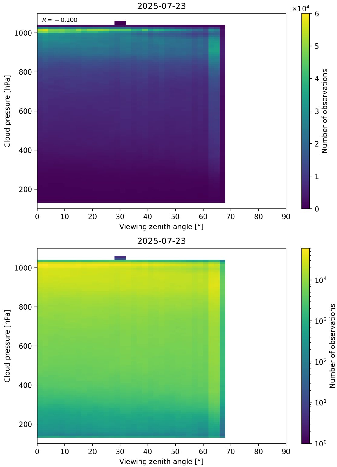
Figure 121: Scatter density plot of “Viewing zenith angle” against “Cloud pressure” for 2025-07-22 to 2025-07-24.
