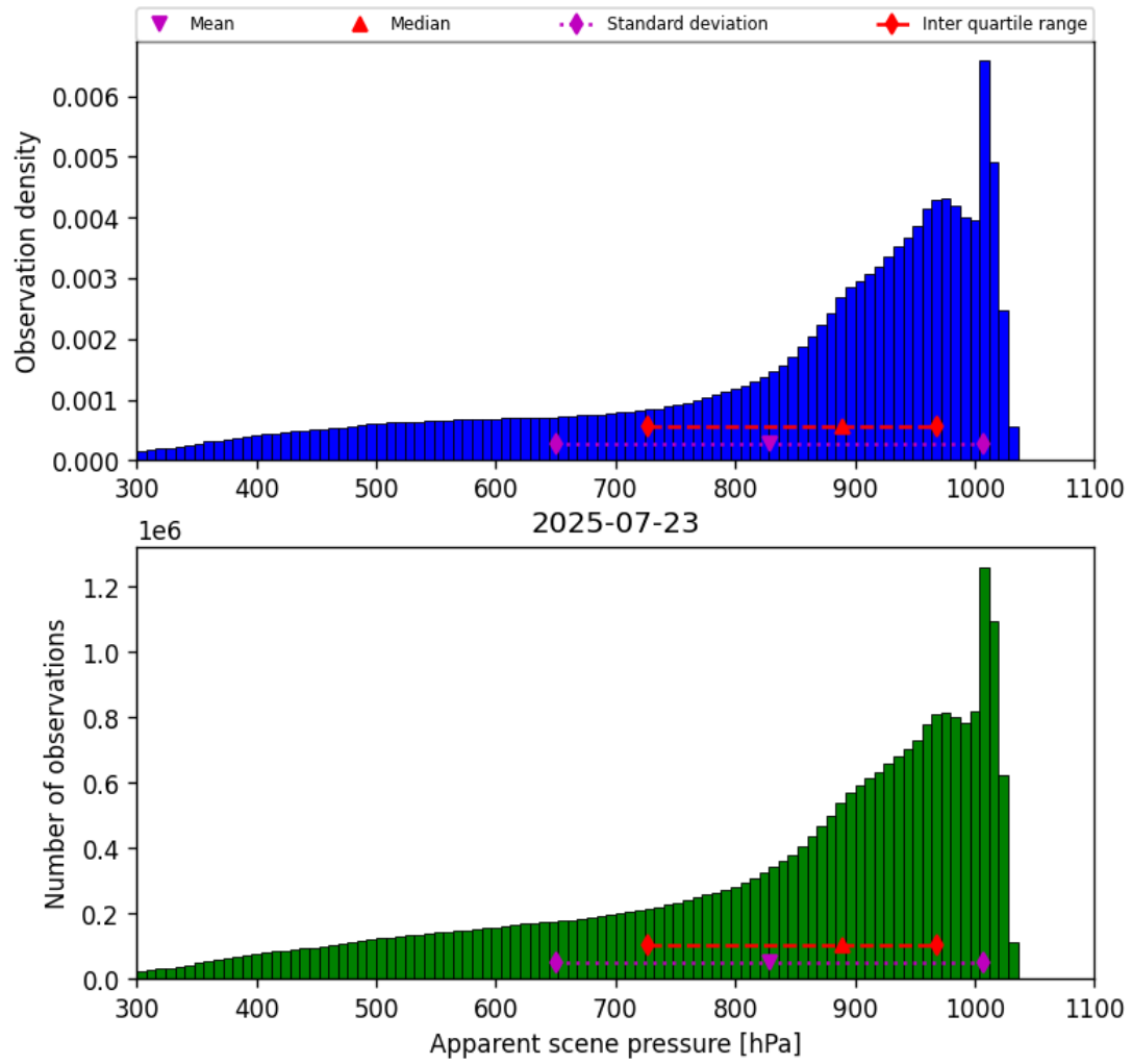
Figure 36: Histogram of “Apparent scene pressure” for 2025-07-22 to 2025-07-24
