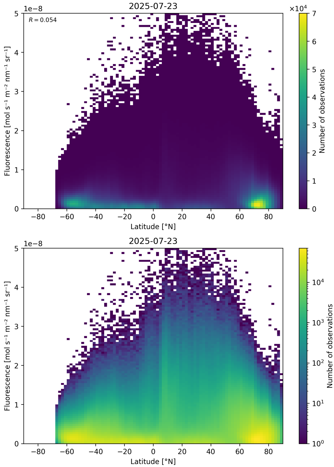
Figure 92: Scatter density plot of “Latitude” against “Fluorescence” for 2025-07-22 to 2025-07-24.
