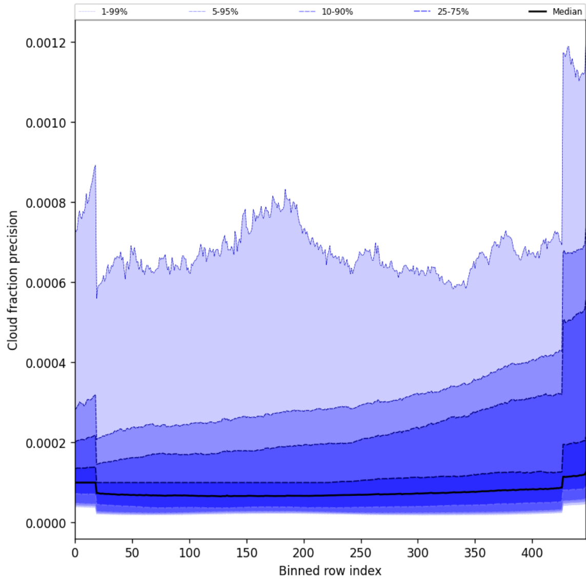
Figure 50: Along track statistics of “Cloud fraction precision” for 2025-07-22 to 2025-07-24
