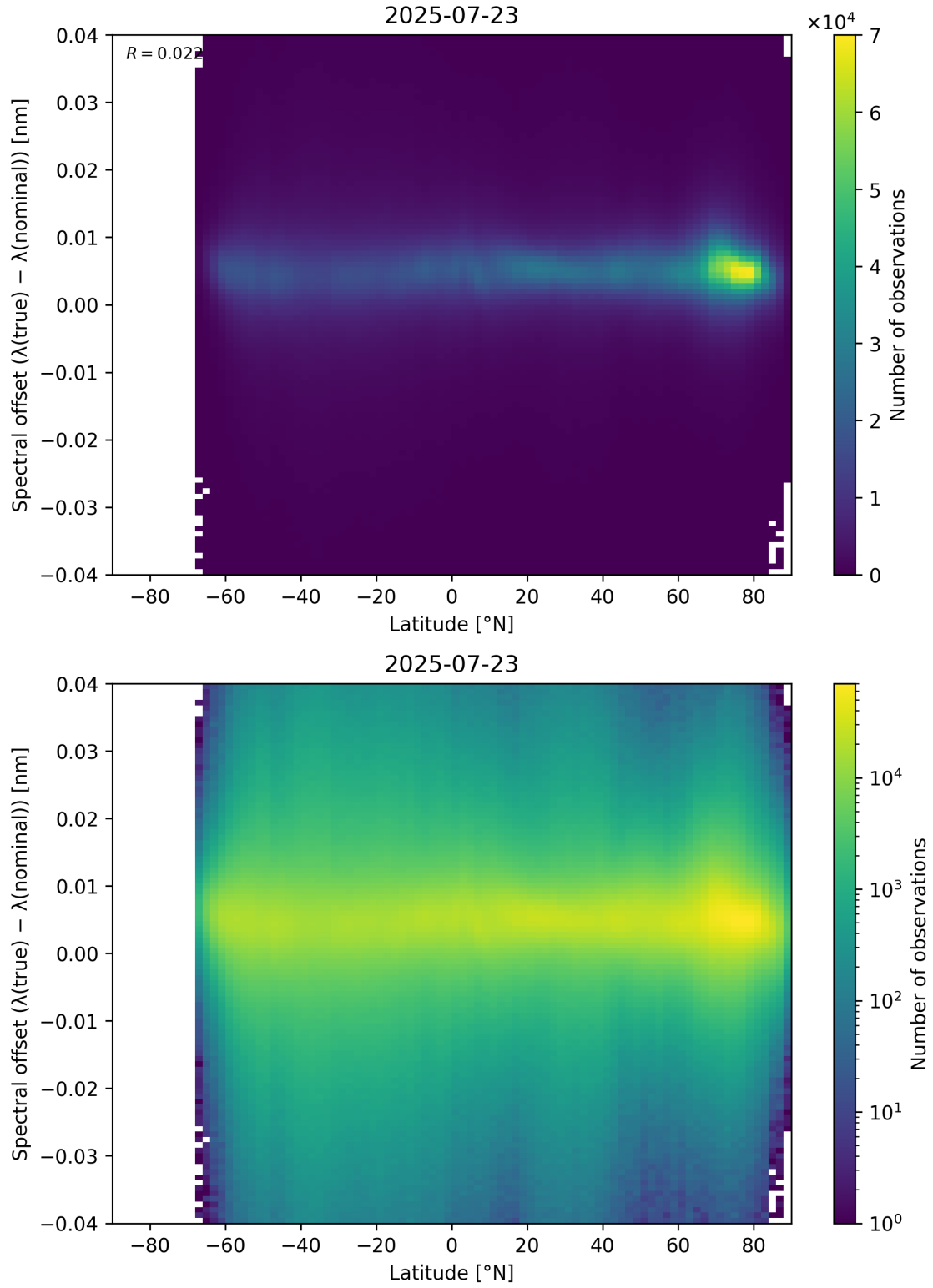
Figure 96: Scatter density plot of “Latitude” against “Spectral offset ( \lambda_{\text{true}} - \lambda_{\text{nominal}} )” for 2025-07-22 to 2025-07-24.
