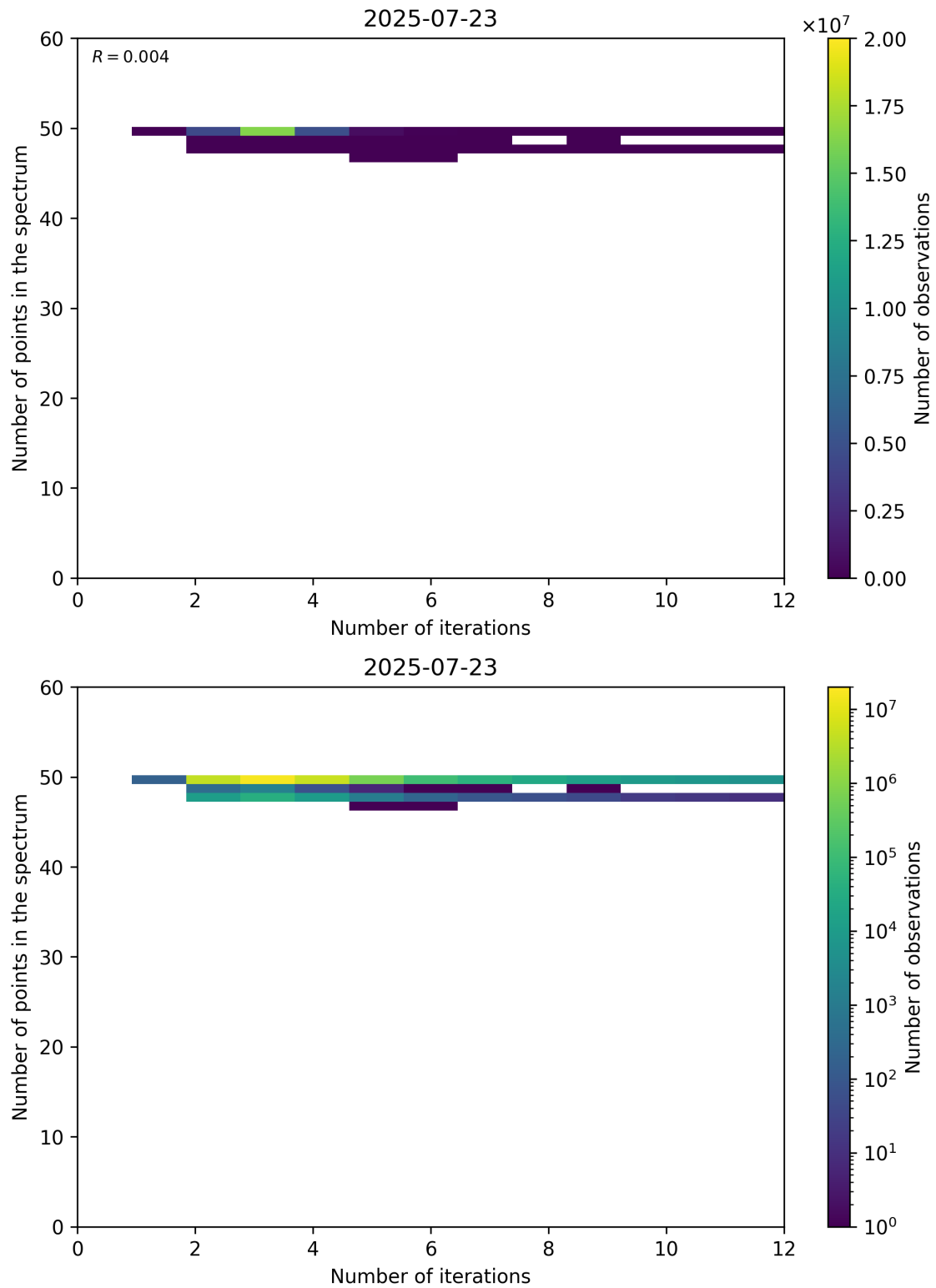
Figure 99: Scatter density plot of “Number of iterations” against “Number of points in the spectrum” for 2025-07-22 to 2025-07-24.
