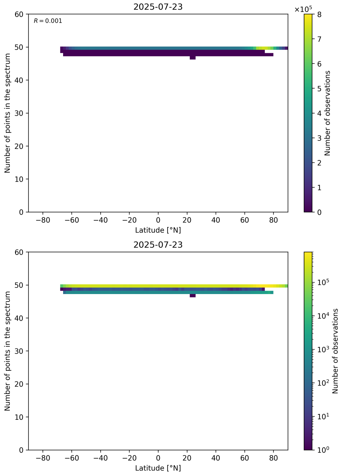
Figure 94: Scatter density plot of “Latitude” against “Number of points in the spectrum” for 2025-07-22 to 2025-07-24.
