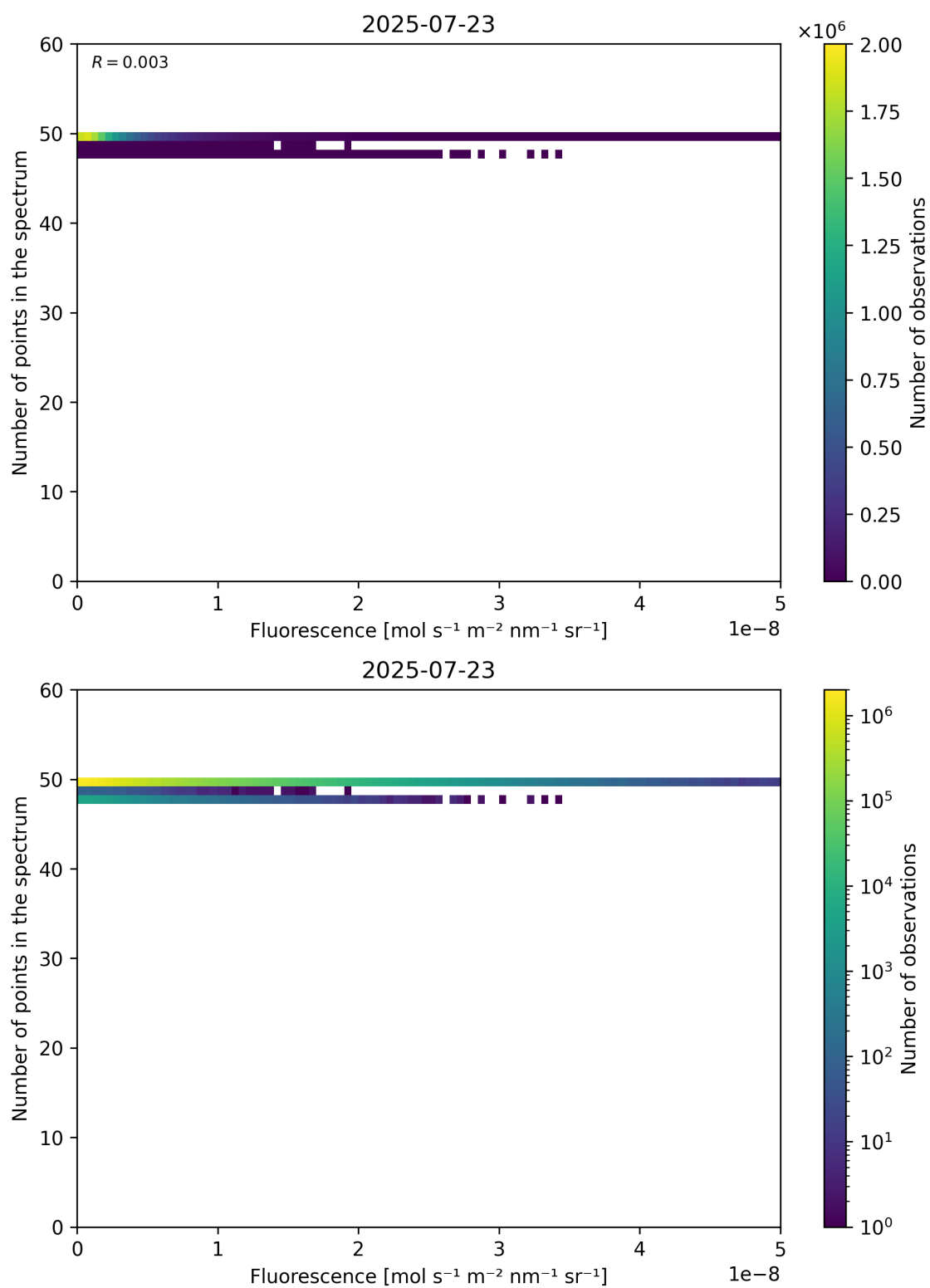
Figure 86: Scatter density plot of “Fluorescence” against “Number of points in the spectrum” for 2025-07-22 to 2025-07-24.
