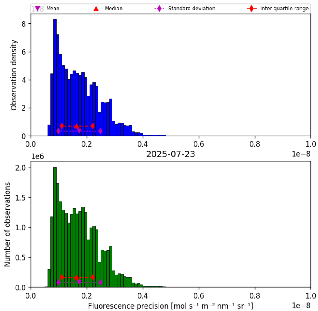
Figure 41: Histogram of “Fluorescence precision” for 2025-07-22 to 2025-07-24
