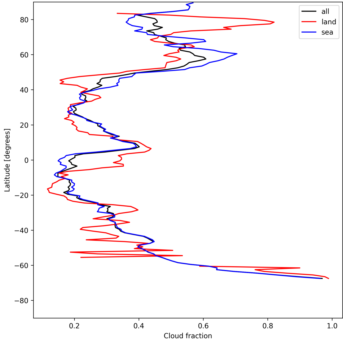
Figure 15: Zonal average of “Cloud fraction” for 2025-07-22 to 2025-07-24.
