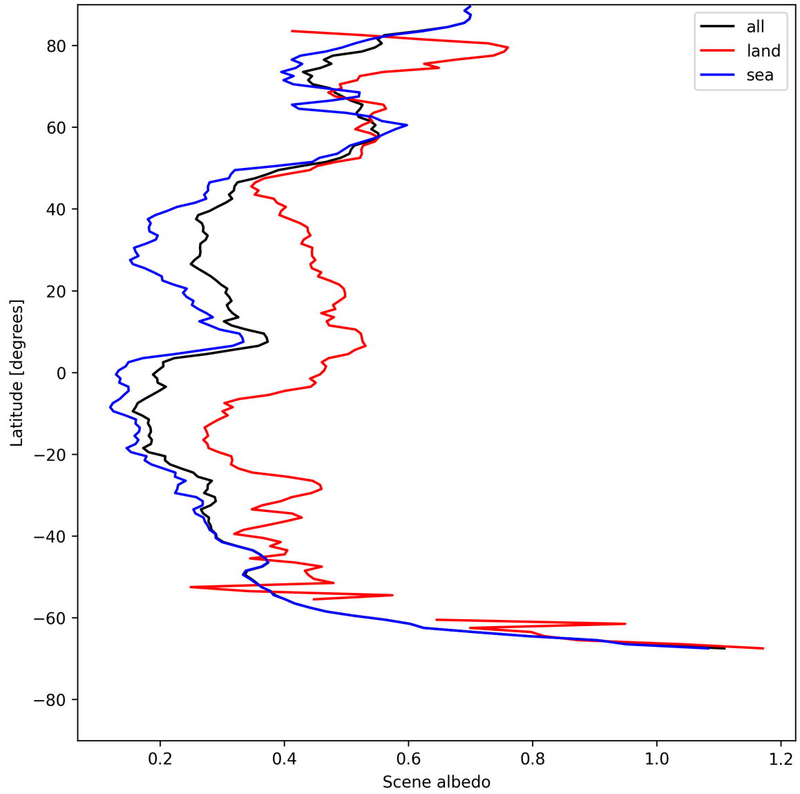
Figure 17: Zonal average of “Scene albedo” for 2025-07-22 to 2025-07-24.
