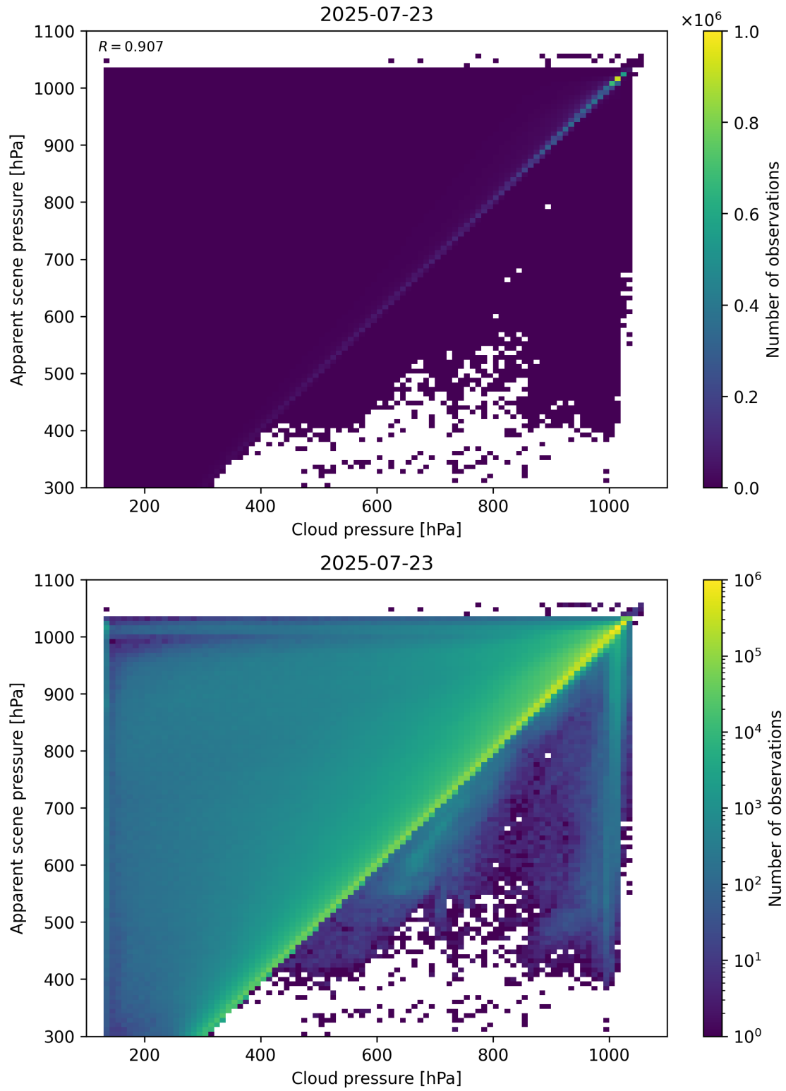
Figure 77: Scatter density plot of “Cloud pressure” against “Apparent scene pressure” for 2025-07-22 to 2025-07-24.
