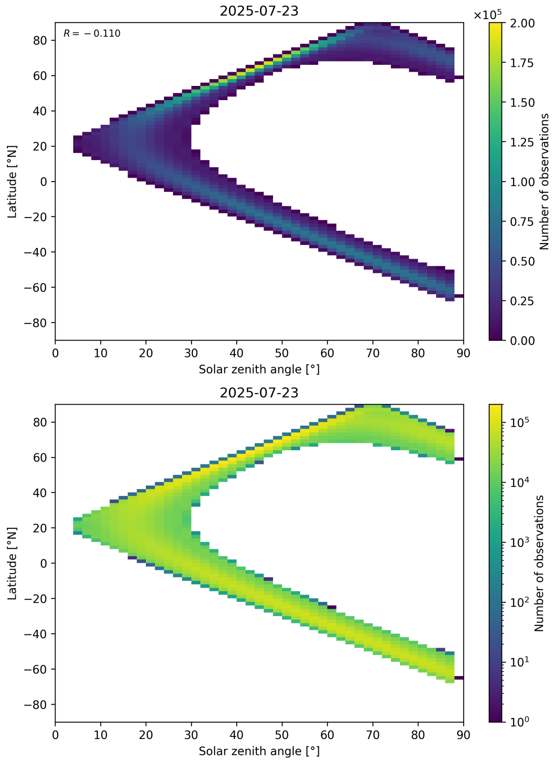
Figure 113: Scatter density plot of “Solar zenith angle” against “Latitude” for 2025-07-22 to 2025-07-24.
