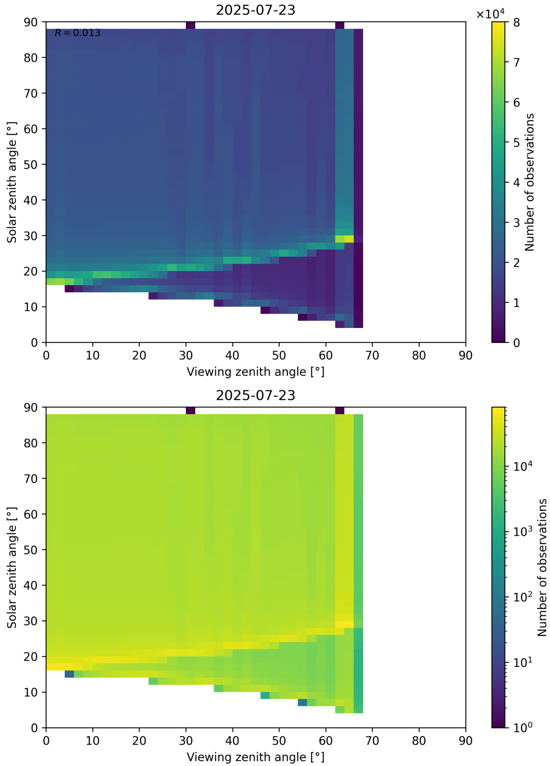
Figure 127: Scatter density plot of “Viewing zenith angle” against “Solar zenith angle” for 2025-07-22 to 2025-07-24.
