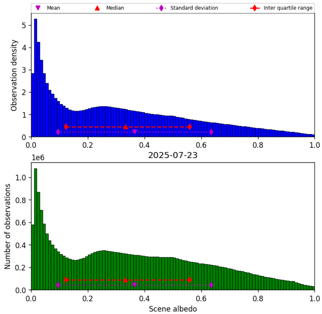
Figure 34: Histogram of “Scene albedo” for 2025-07-22 to 2025-07-24
