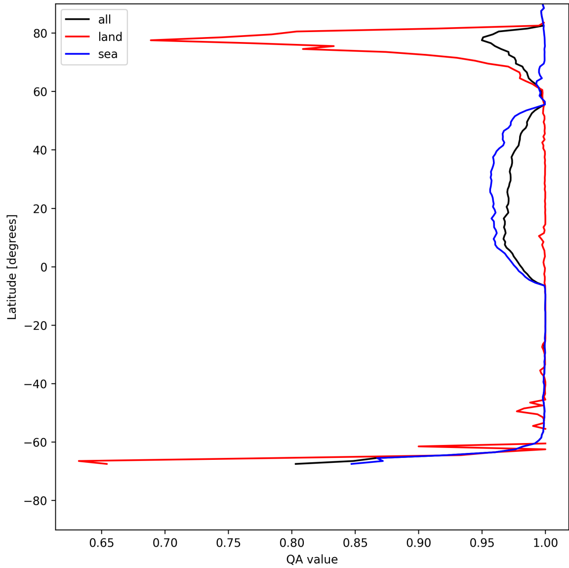
Figure 12: Zonal average of “QA value” for 2025-07-22 to 2025-07-24.
