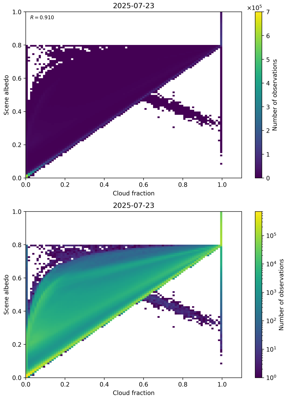
Figure 75: Scatter density plot of “Cloud fraction” against “Scene albedo” for 2025-07-22 to 2025-07-24.
