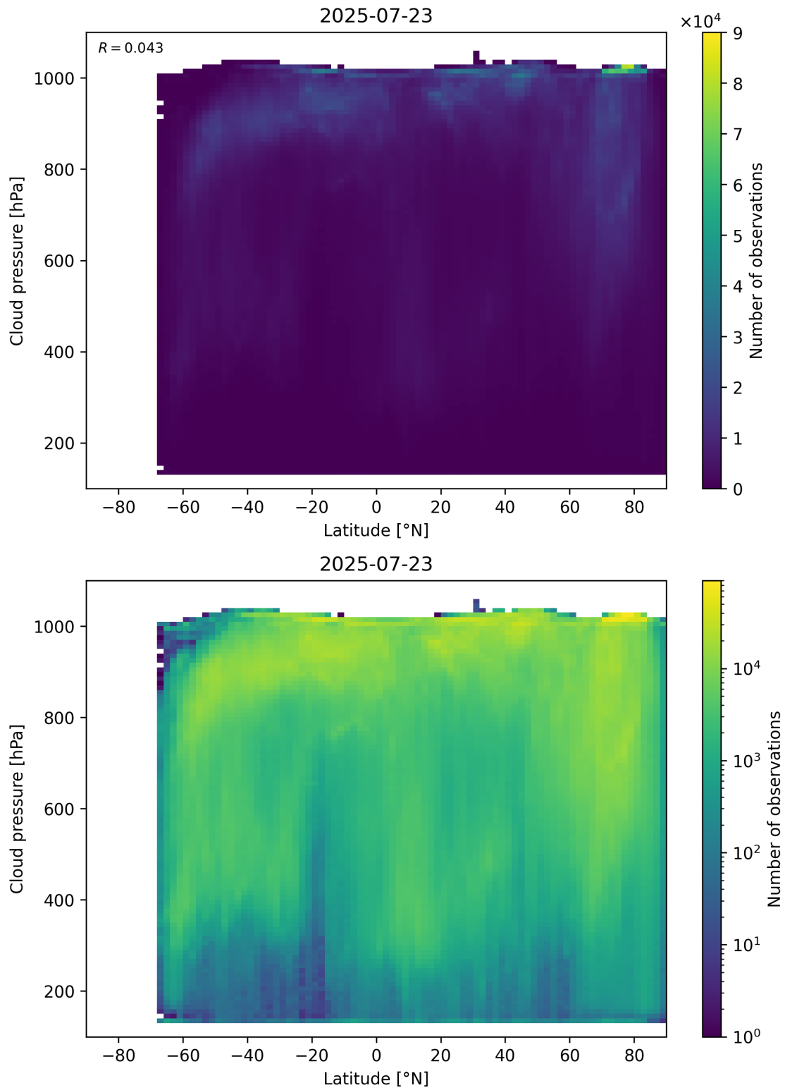
Figure 91: Scatter density plot of “Latitude” against “Cloud pressure” for 2025-07-22 to 2025-07-24.
