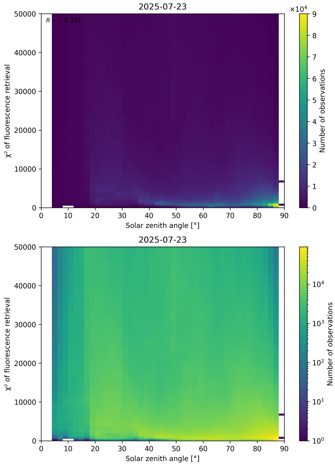
Figure 109: Scatter density plot of “Solar zenith angle” against “ \chi^2 of fluorescence retrieval” for 2025-07-22 to 2025-07-24.
