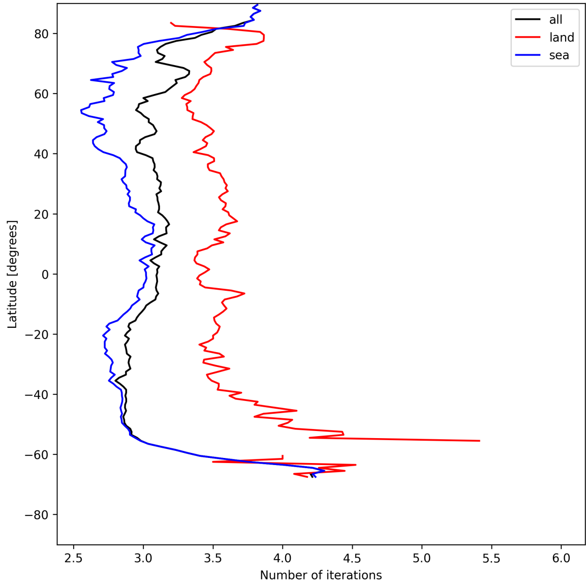
Figure 22: Zonal average of “Number of iterations” for 2025-07-22 to 2025-07-24.
