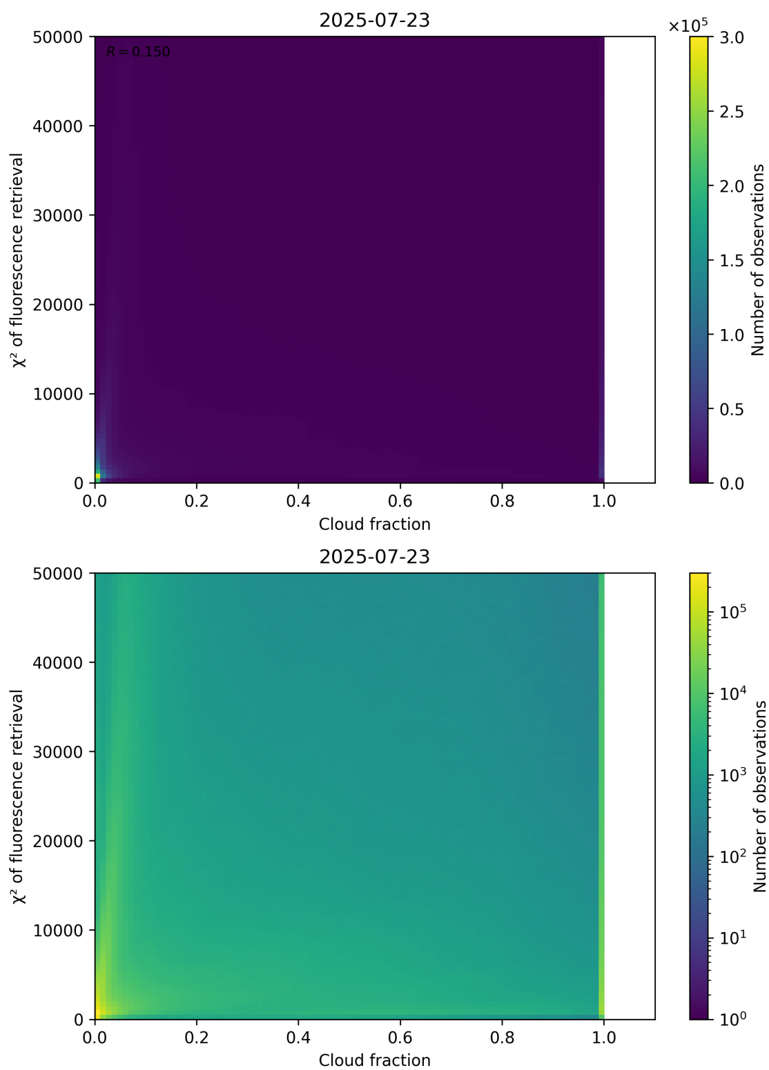
Figure 71: Scatter density plot of “Cloud fraction” against “ \chi^2 of fluorescence retrieval” for 2025-07-22 to 2025-07-24.
