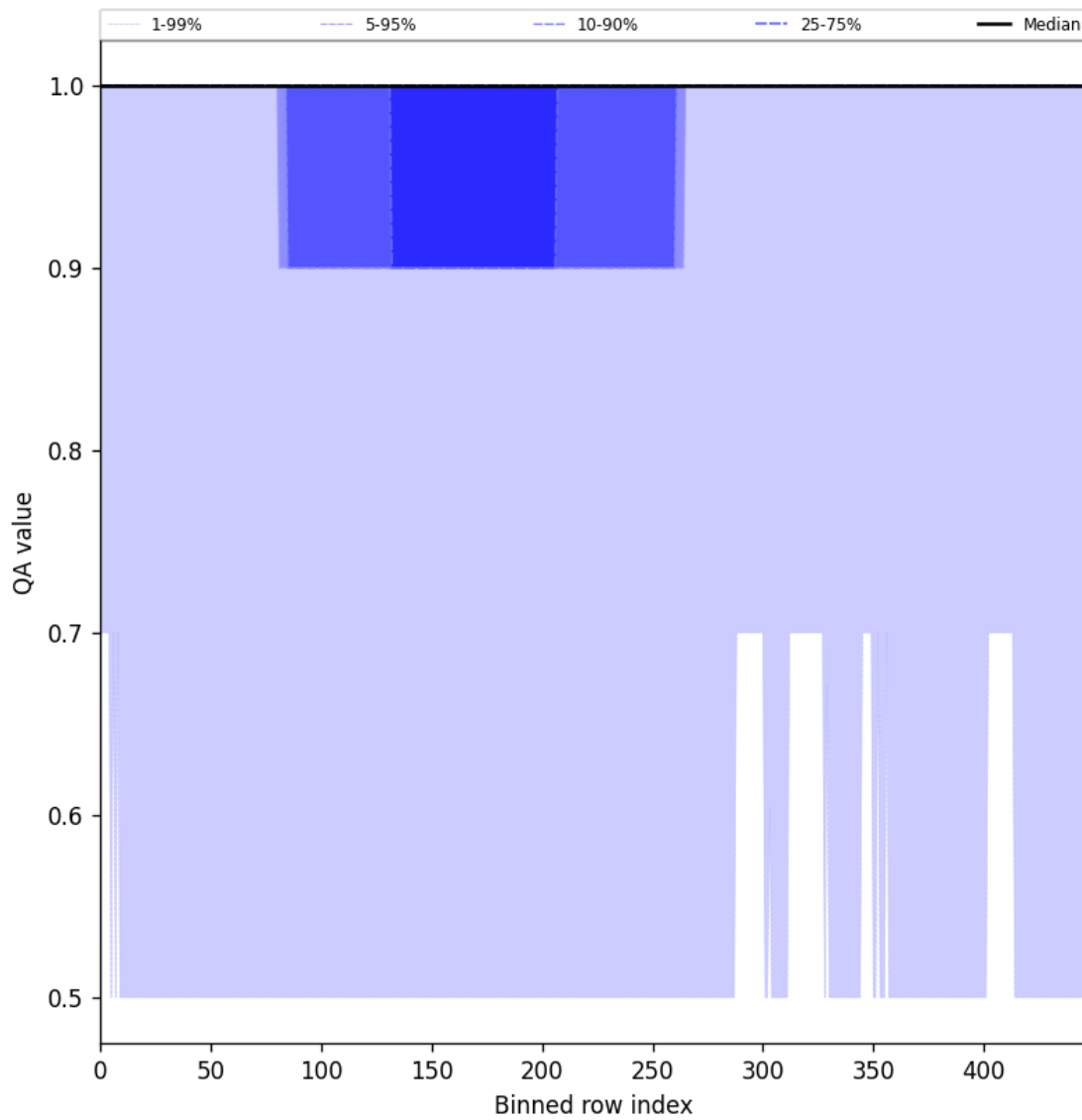
Figure 46: Along track statistics of “QA value” for 2025-07-22 to 2025-07-24
