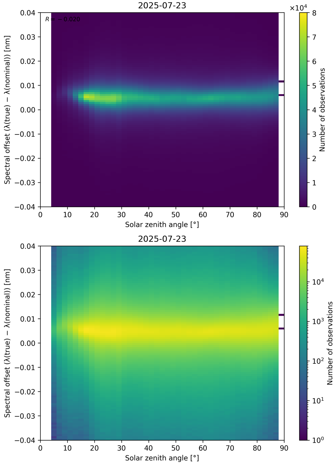
Figure 117: Scatter density plot of “Solar zenith angle” against “Spectral offset ( \lambda_{\text{true}} - \lambda_{\text{nominal}} )” for 2025-07-22 to 2025-07-24.
