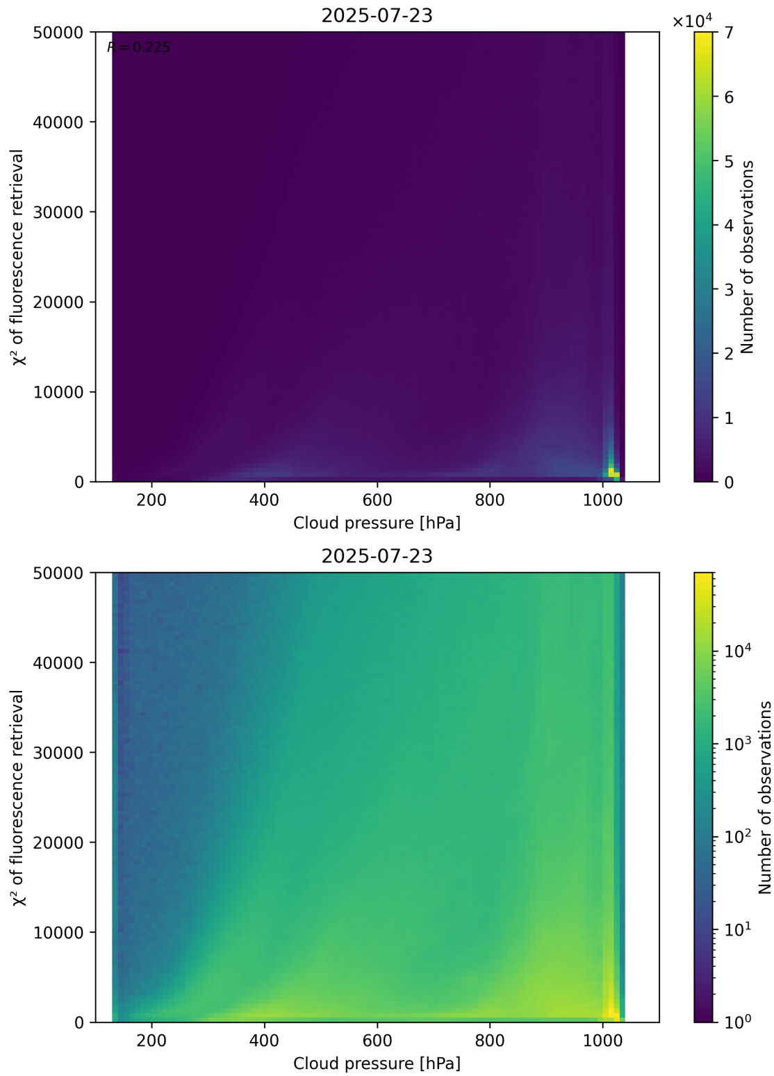
Figure 78: Scatter density plot of “Cloud pressure” against “ \chi^2 of fluorescence retrieval” for 2025-07-22 to 2025-07-24.
