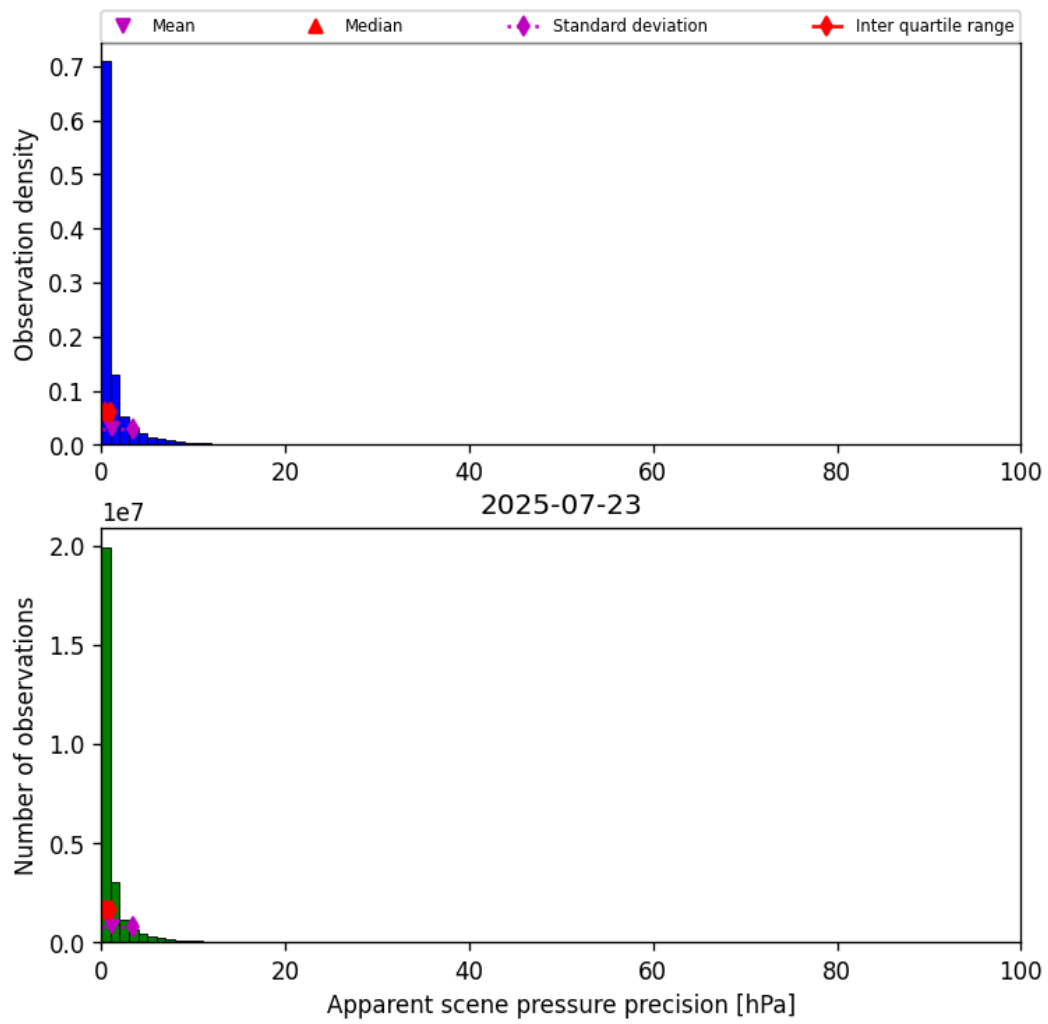
Figure 37: Histogram of “Apparent scene pressure precision” for 2025-07-22 to 2025-07-24
