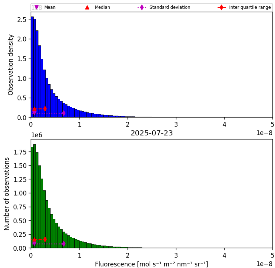
Figure 40: Histogram of “Fluorescence” for 2025-07-22 to 2025-07-24
