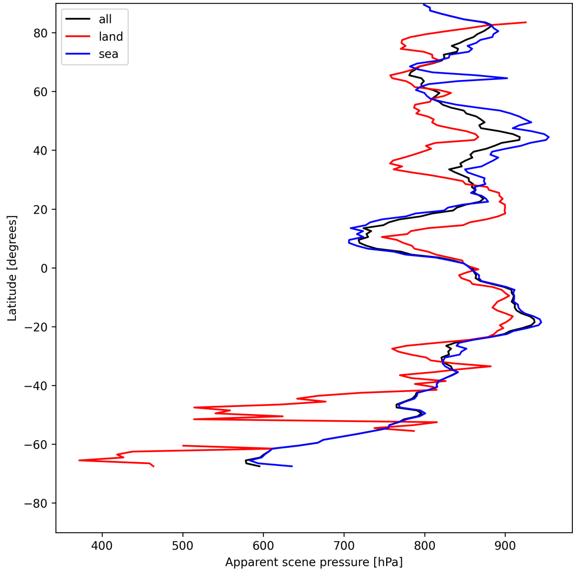
Figure 19: Zonal average of “Apparent scene pressure” for 2025-07-22 to 2025-07-24.
