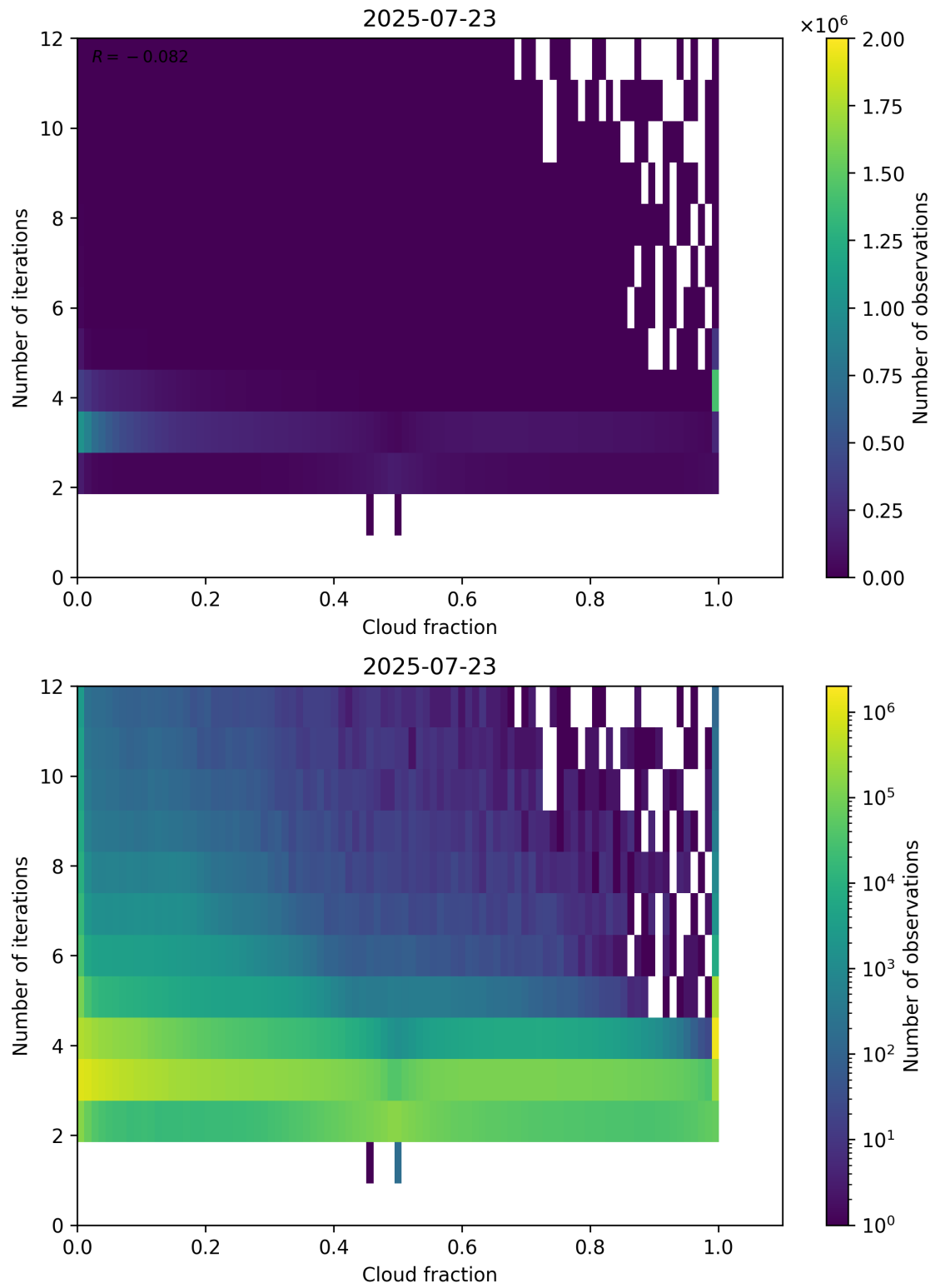
Figure 73: Scatter density plot of “Cloud fraction” against “Number of iterations” for 2025-07-22 to 2025-07-24.
