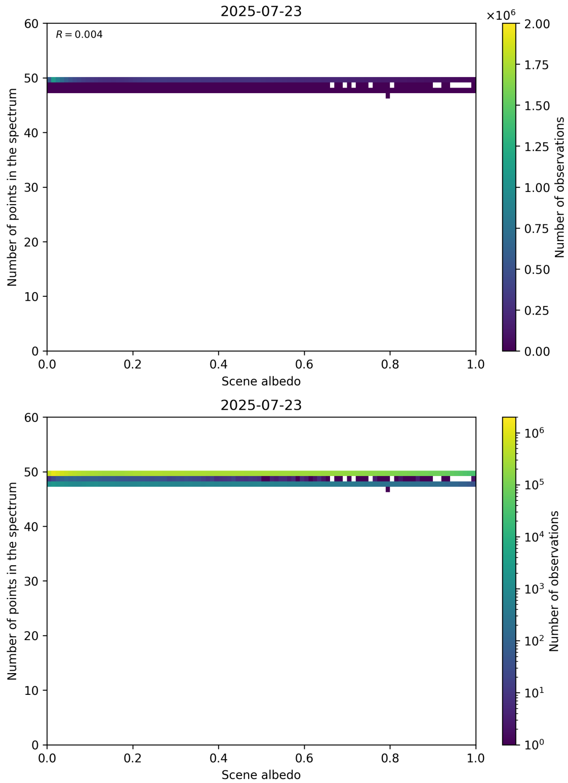
Figure 106: Scatter density plot of “Scene albedo” against “Number of points in the spectrum” for 2025-07-22 to 2025-07-24.
