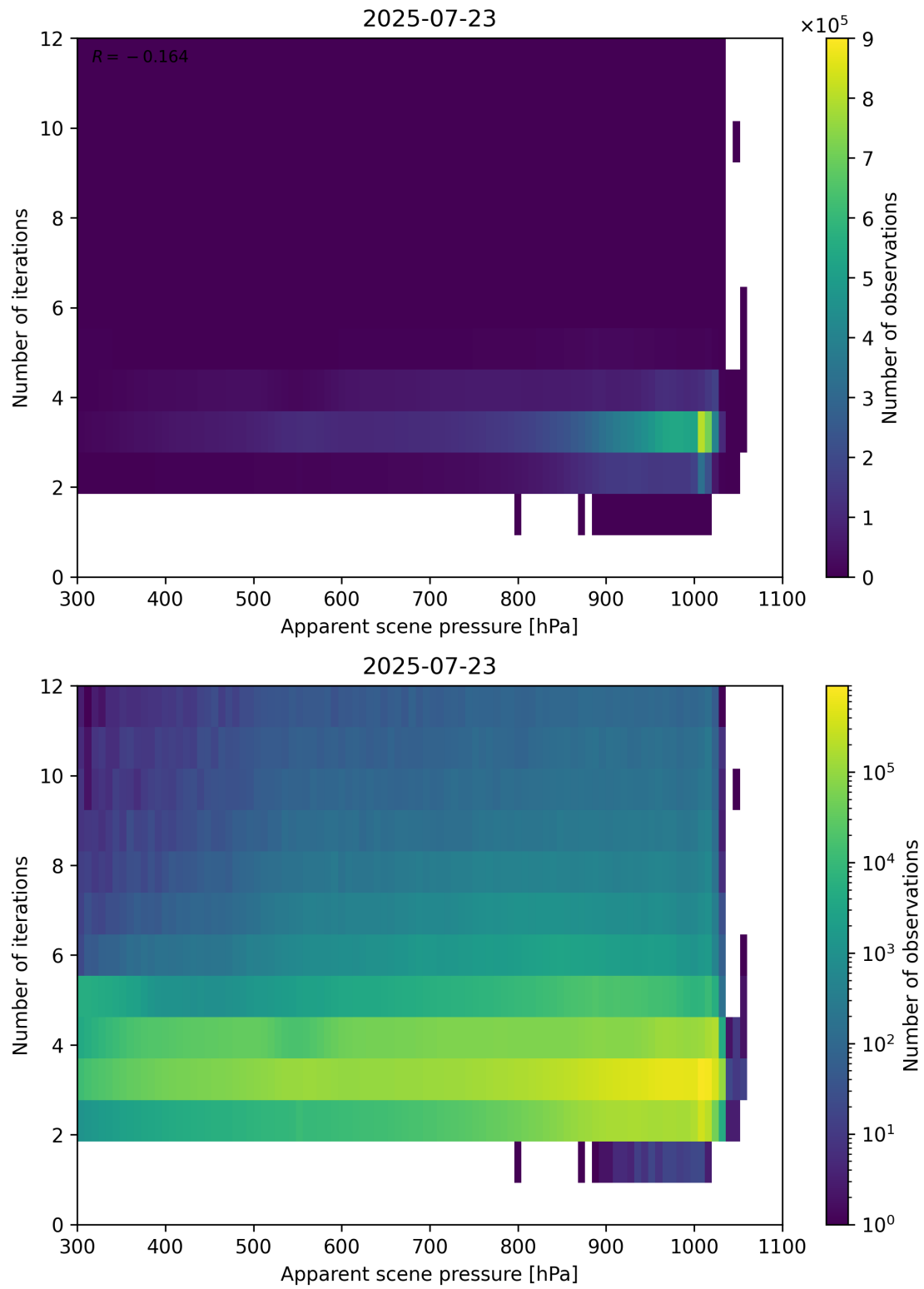
Figure 65: Scatter density plot of “Apparent scene pressure” against “Number of iterations” for 2025-07-22 to 2025-07-24.
