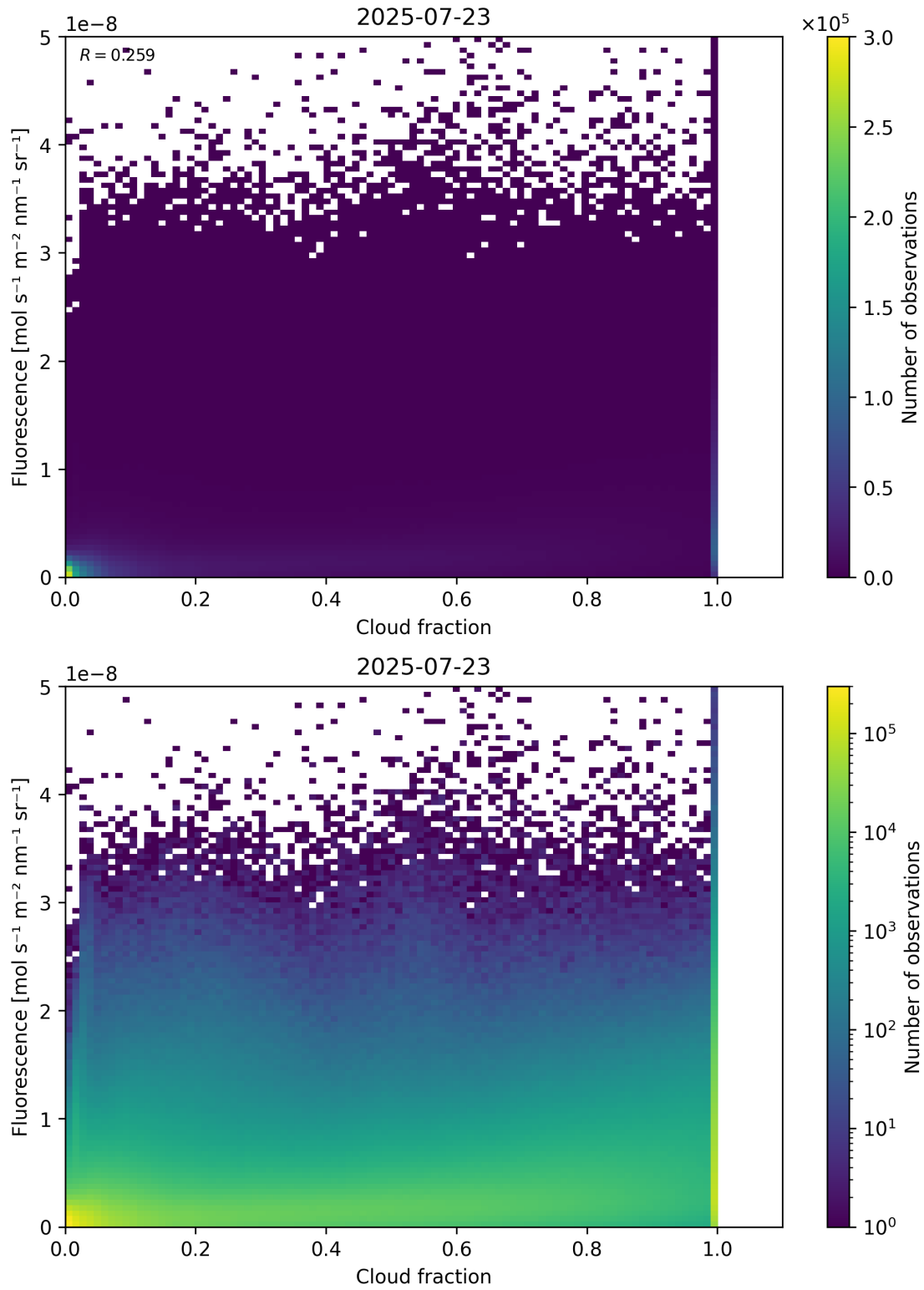
Figure 72: Scatter density plot of “Cloud fraction” against “Fluorescence” for 2025-07-22 to 2025-07-24.
