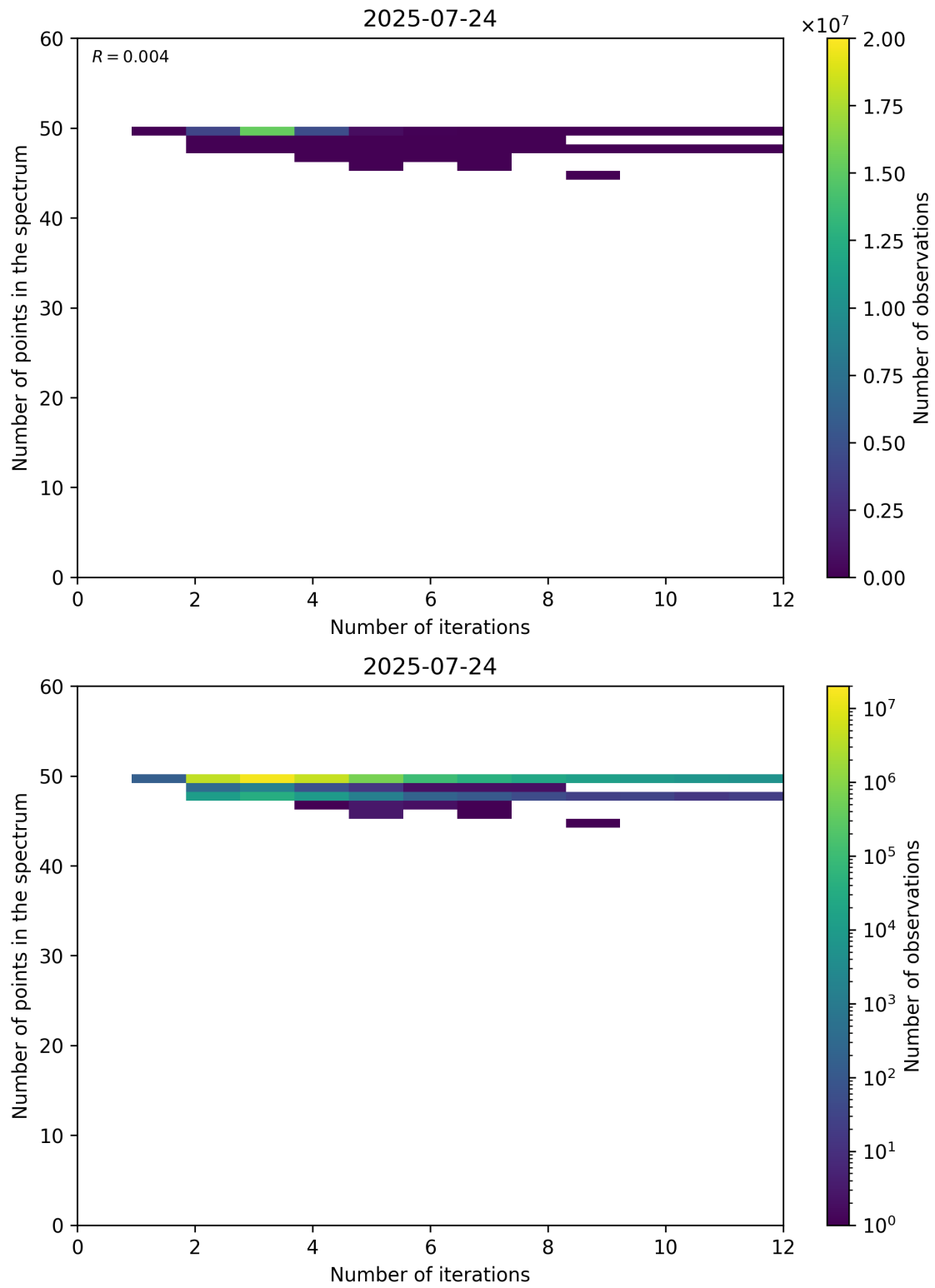
Figure 99: Scatter density plot of “Number of iterations” against “Number of points in the spectrum” for 2025-07-24 to 2025-07-25.
