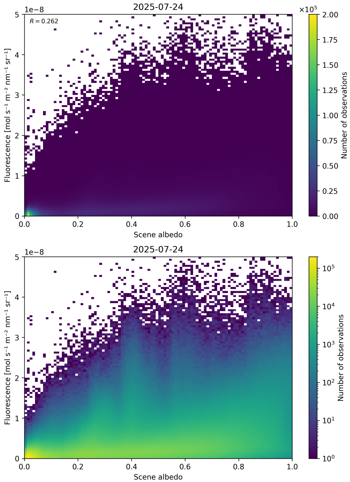
Figure 104: Scatter density plot of “Scene albedo” against “Fluorescence” for 2025-07-24 to 2025-07-25.
