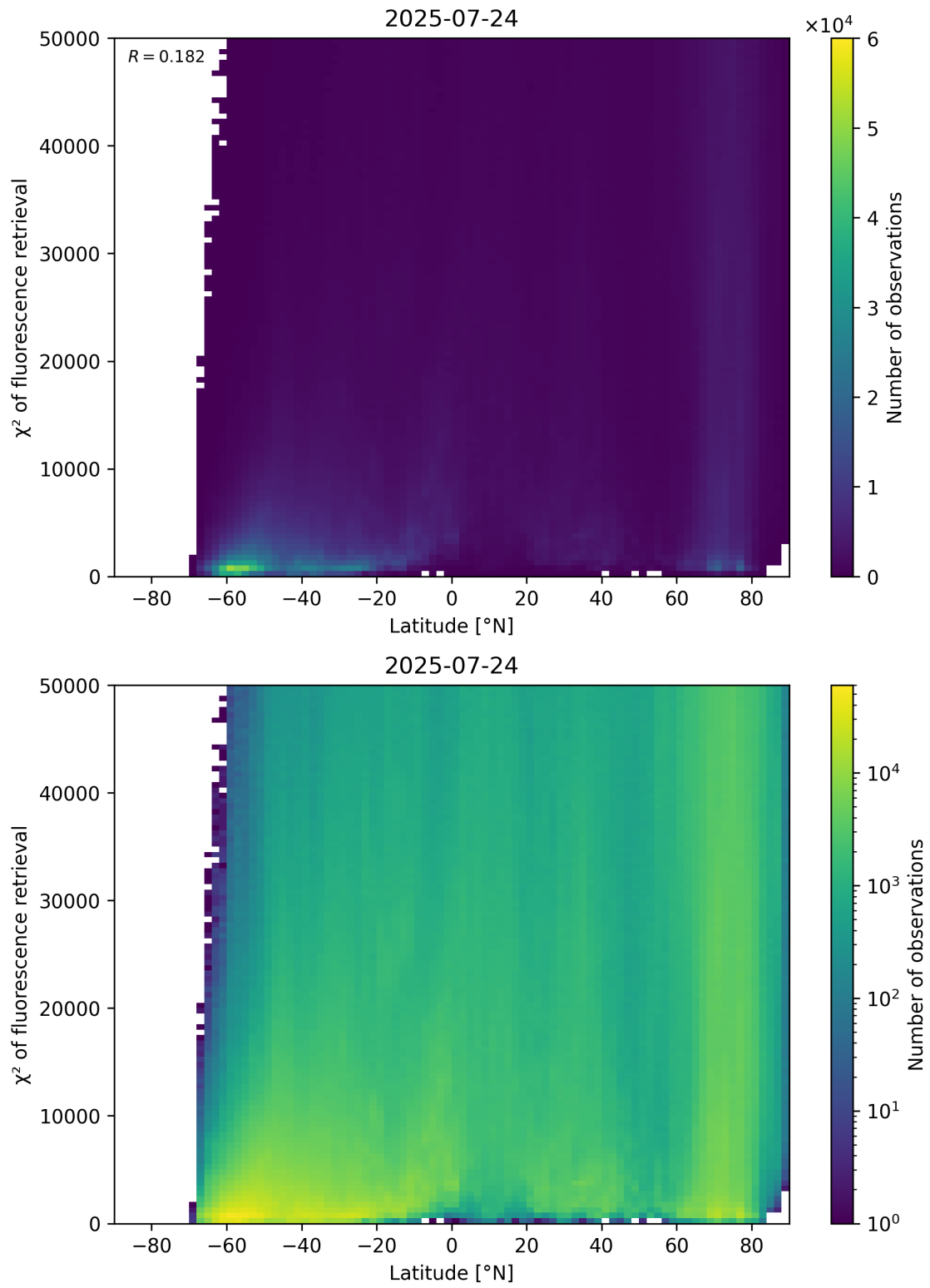
Figure 89: Scatter density plot of “Latitude” against “ \chi^2 of fluorescence retrieval” for 2025-07-24 to 2025-07-25.
