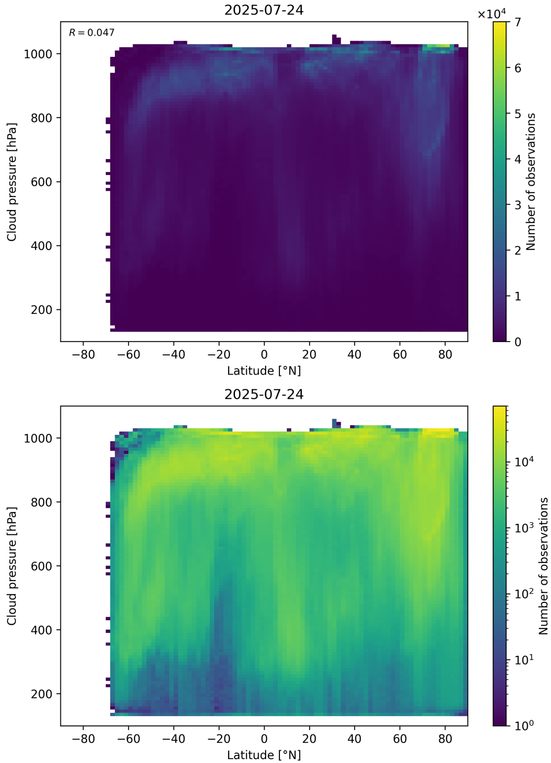
Figure 91: Scatter density plot of “Latitude” against “Cloud pressure” for 2025-07-24 to 2025-07-25.
