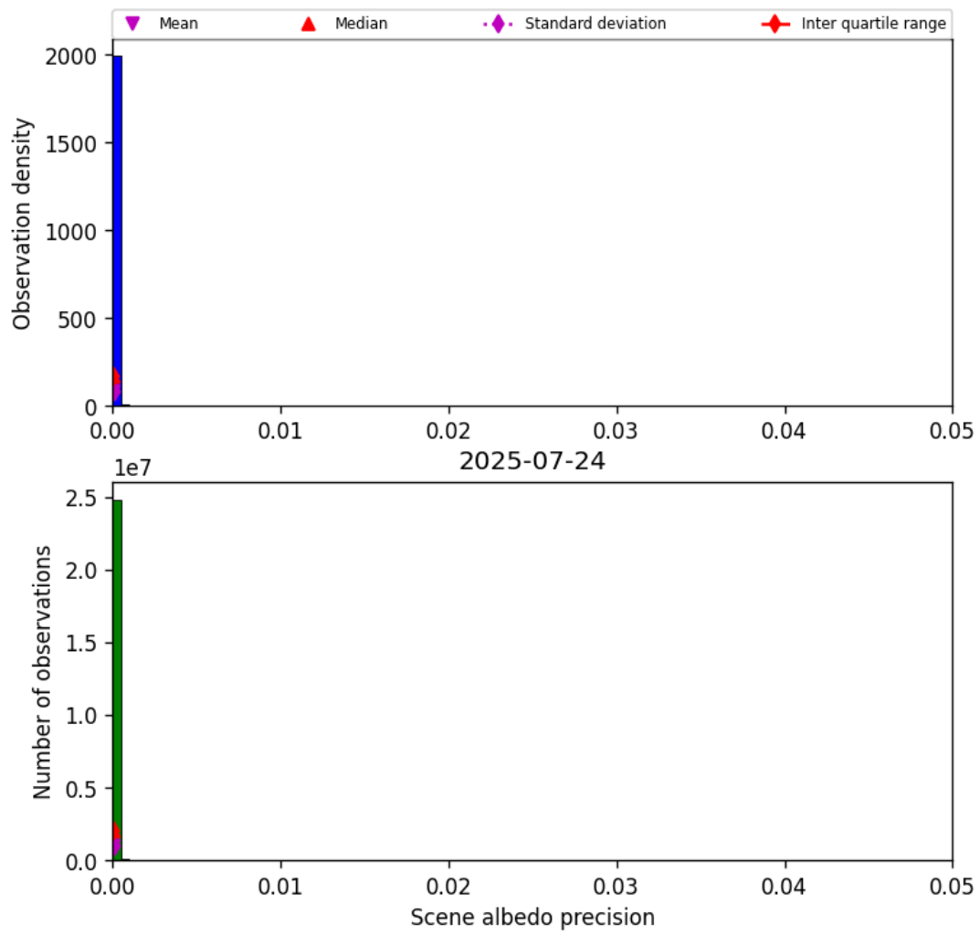
Figure 35: Histogram of “Scene albedo precision” for 2025-07-24 to 2025-07-25
