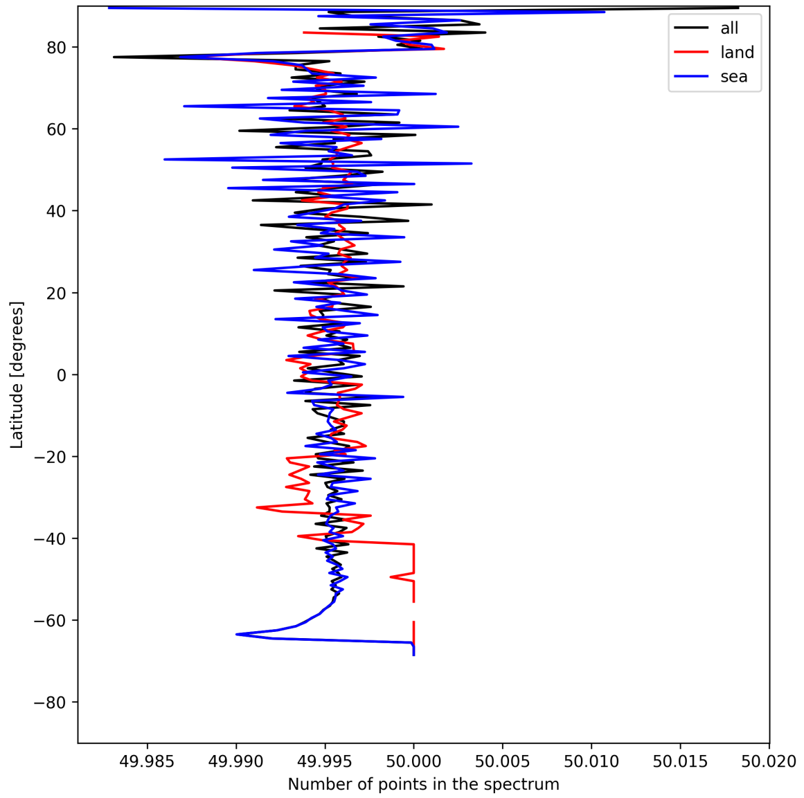
Figure 27: Zonal average of “Number of points in the spectrum” for 2025-07-24 to 2025-07-25.
