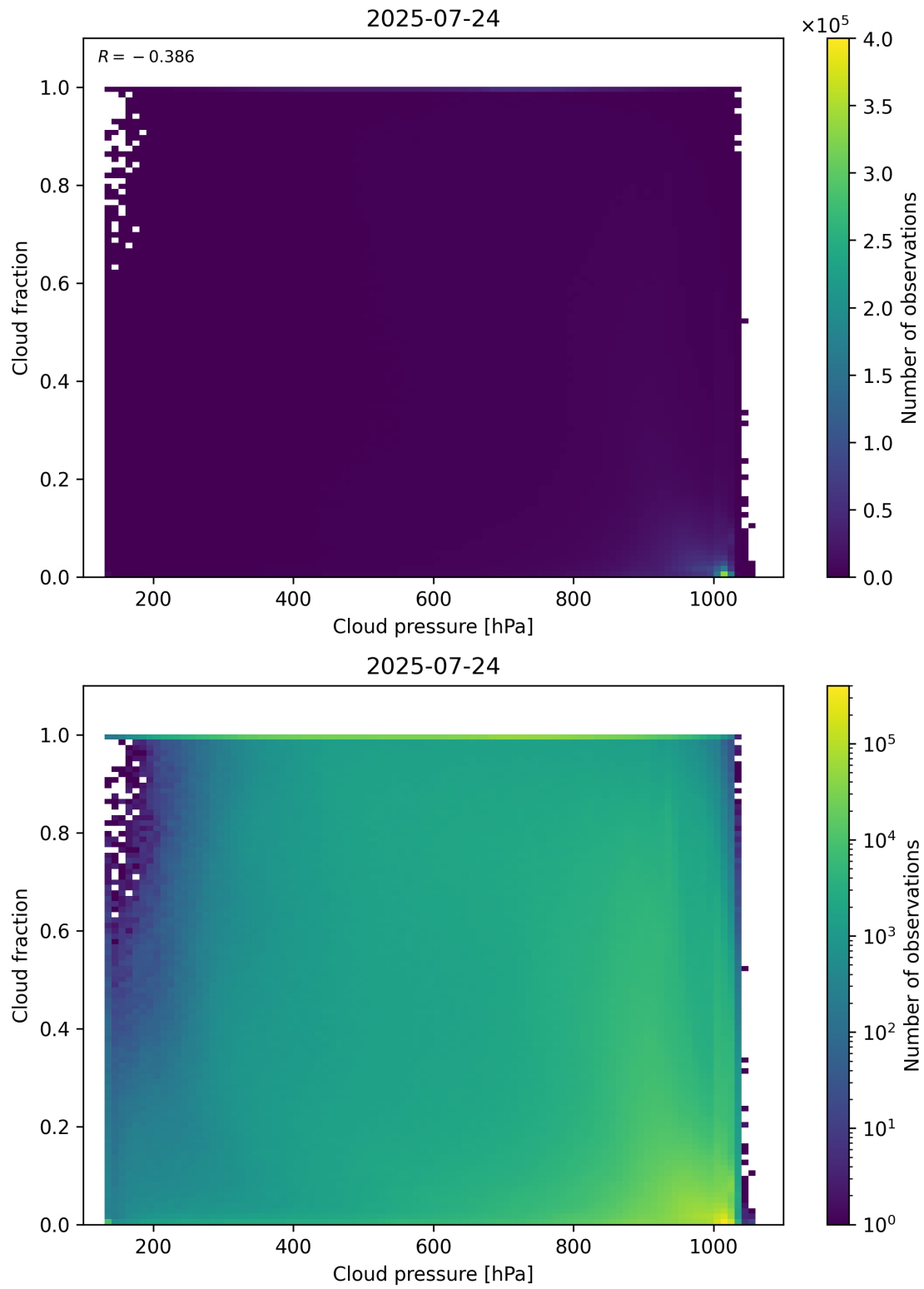
Figure 79: Scatter density plot of “Cloud pressure” against “Cloud fraction” for 2025-07-24 to 2025-07-25.
