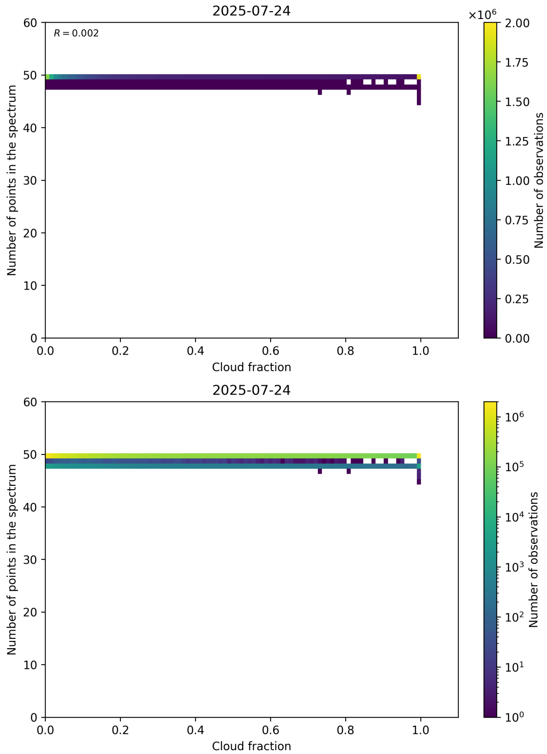
Figure 74: Scatter density plot of “Cloud fraction” against “Number of points in the spectrum” for 2025-07-24 to 2025-07-25.
