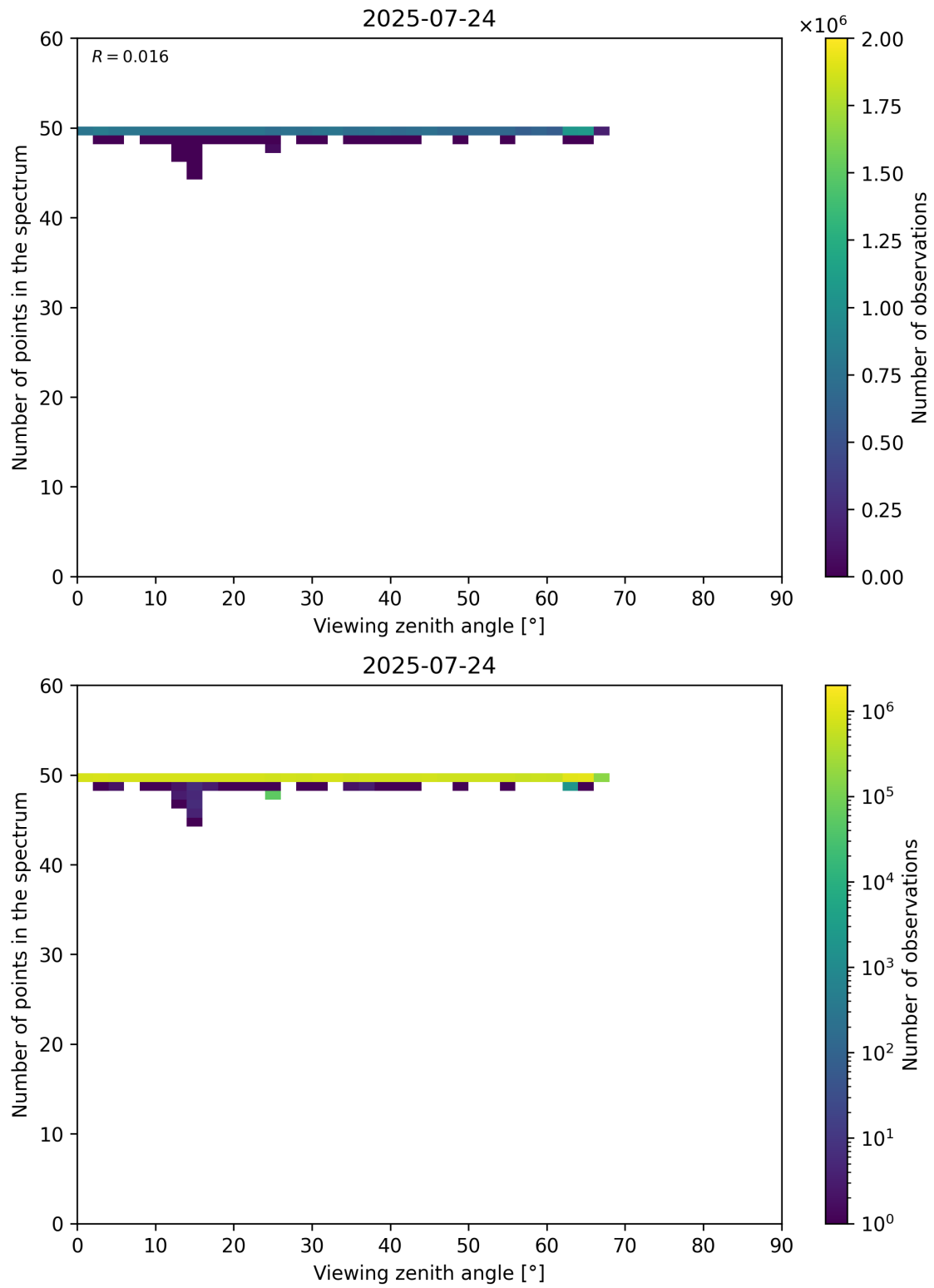
Figure 125: Scatter density plot of “Viewing zenith angle” against “Number of points in the spectrum” for 2025-07-24 to 2025-07-25.
