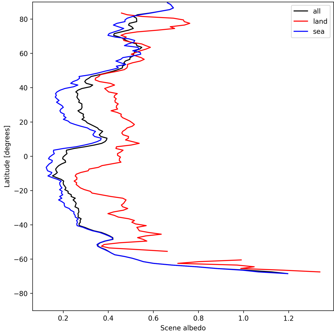
Figure 17: Zonal average of “Scene albedo” for 2025-07-24 to 2025-07-25.
