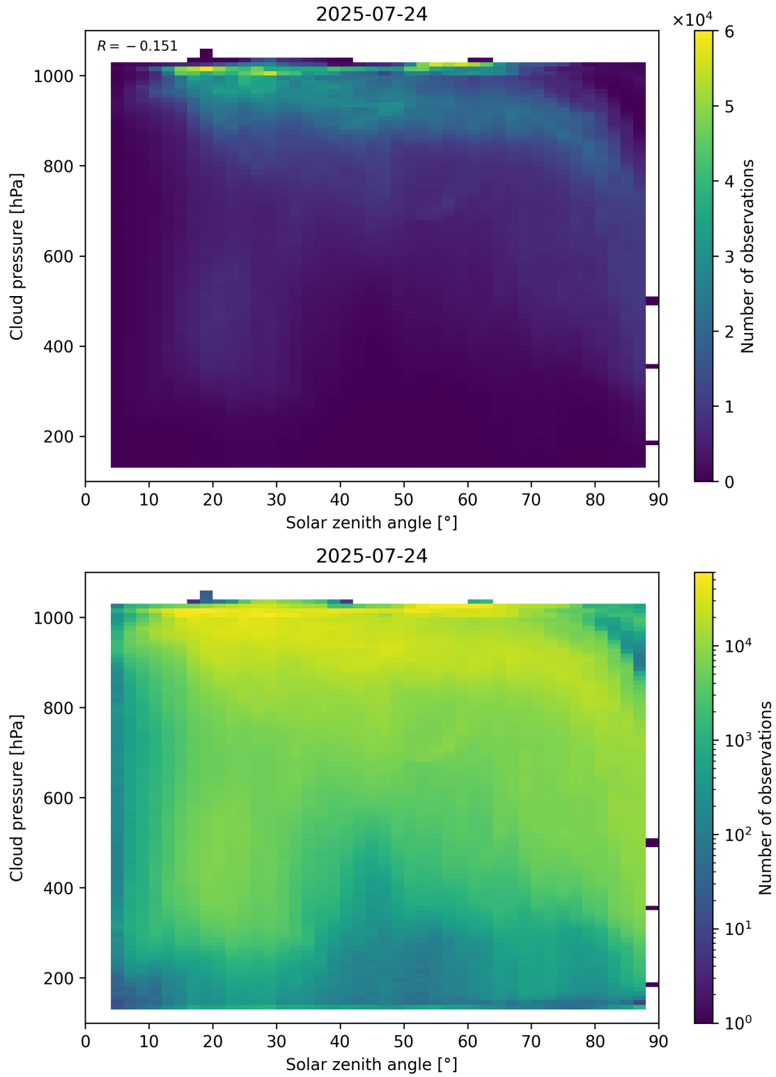
Figure 111: Scatter density plot of “Solar zenith angle” against “Cloud pressure” for 2025-07-24 to 2025-07-25.
