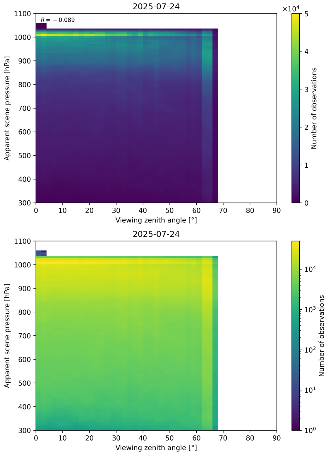
Figure 118: Scatter density plot of “Viewing zenith angle” against “Apparent scene pressure” for 2025-07-24 to 2025-07-25.
