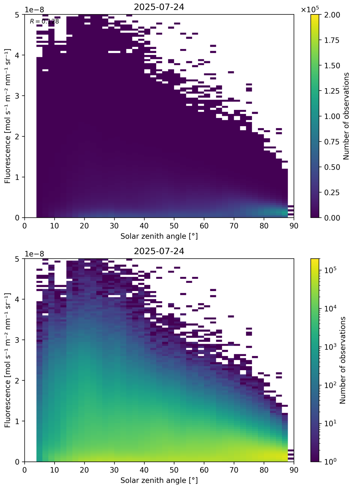
Figure 112: Scatter density plot of “Solar zenith angle” against “Fluorescence” for 2025-07-24 to 2025-07-25.
