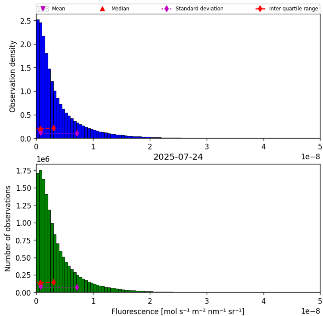
Figure 40: Histogram of “Fluorescence” for 2025-07-24 to 2025-07-25
