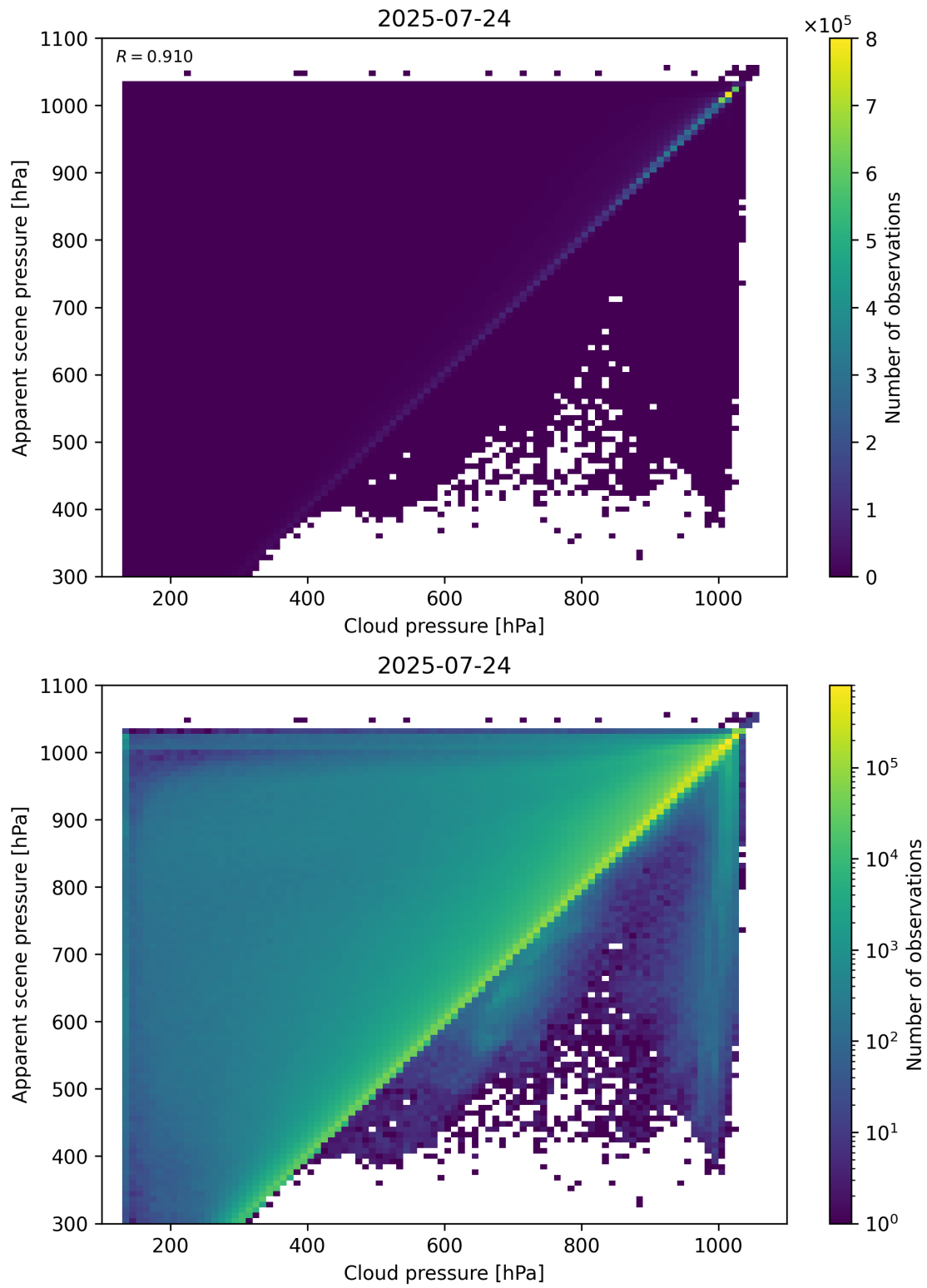
Figure 77: Scatter density plot of “Cloud pressure” against “Apparent scene pressure” for 2025-07-24 to 2025-07-25.
