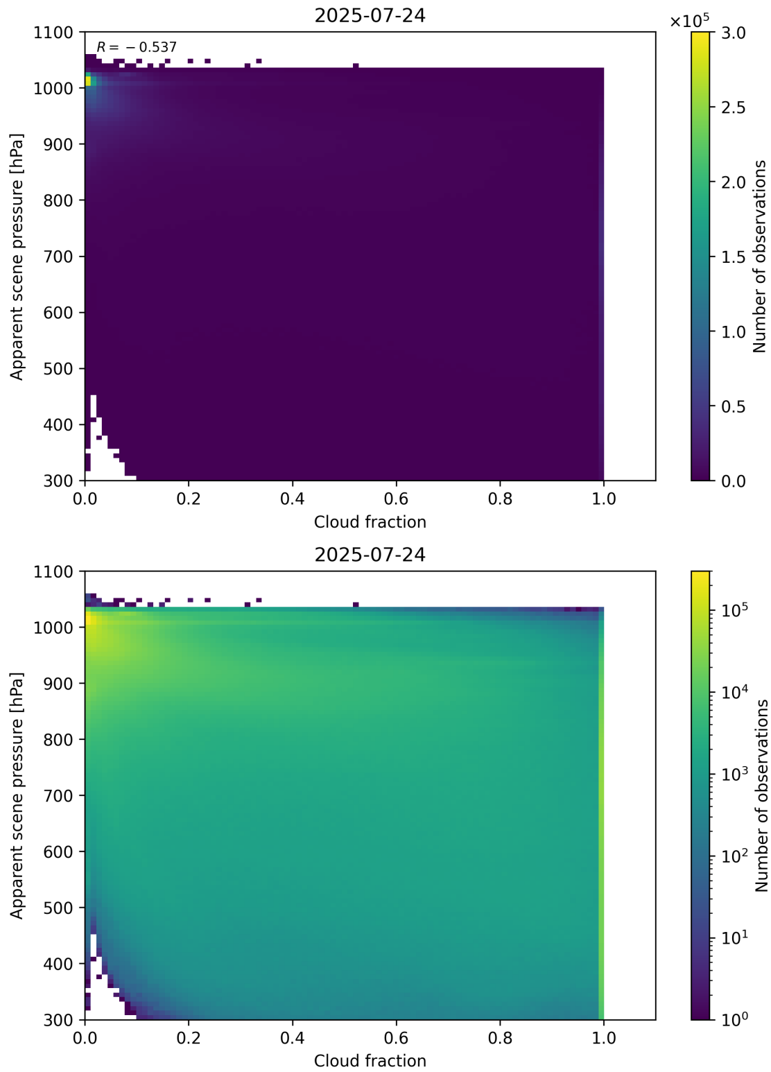
Figure 70: Scatter density plot of “Cloud fraction” against “Apparent scene pressure” for 2025-07-24 to 2025-07-25.
