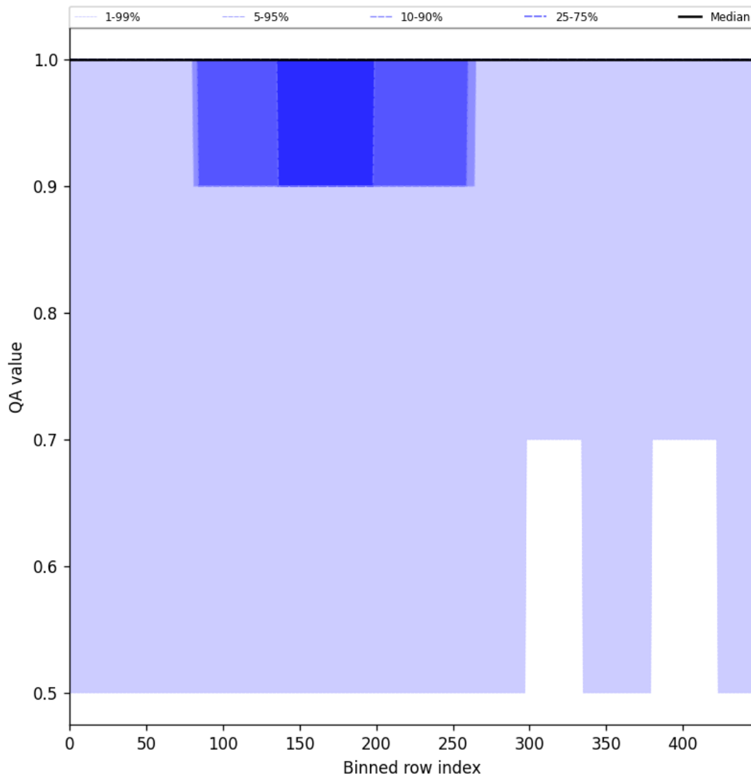
Figure 46: Along track statistics of “QA value” for 2025-07-24 to 2025-07-25
