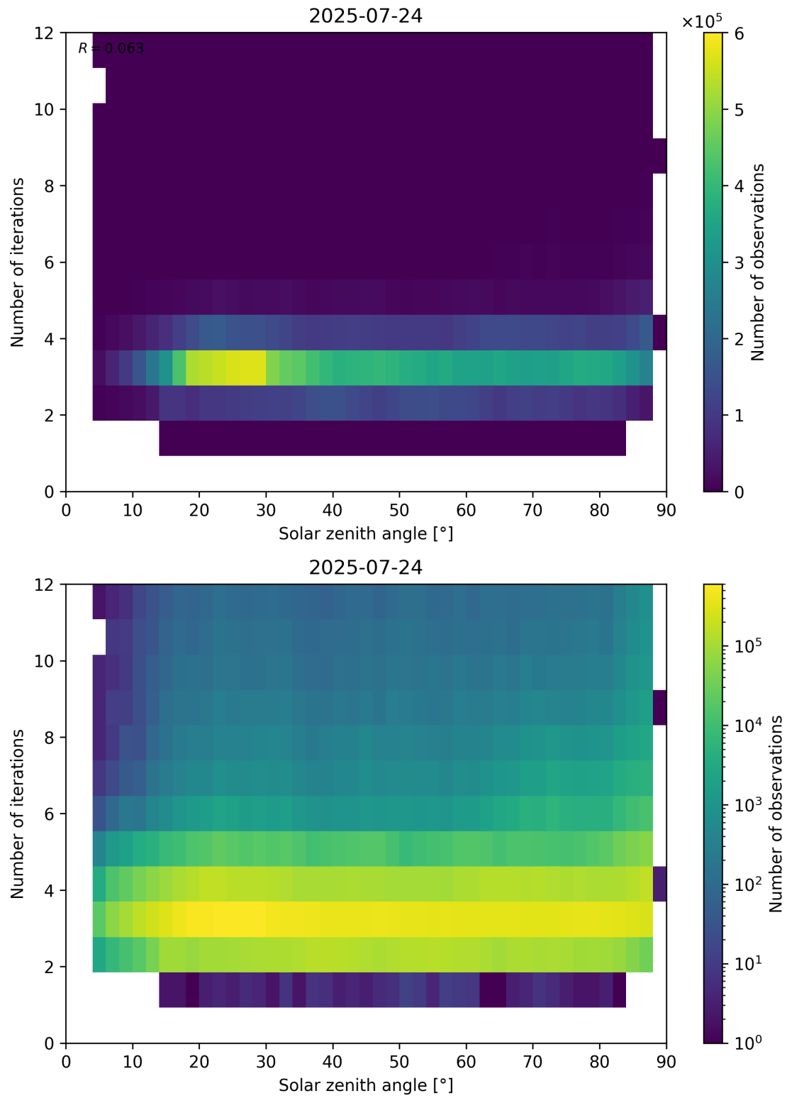
Figure 114: Scatter density plot of “Solar zenith angle” against “Number of iterations” for 2025-07-24 to 2025-07-25.
