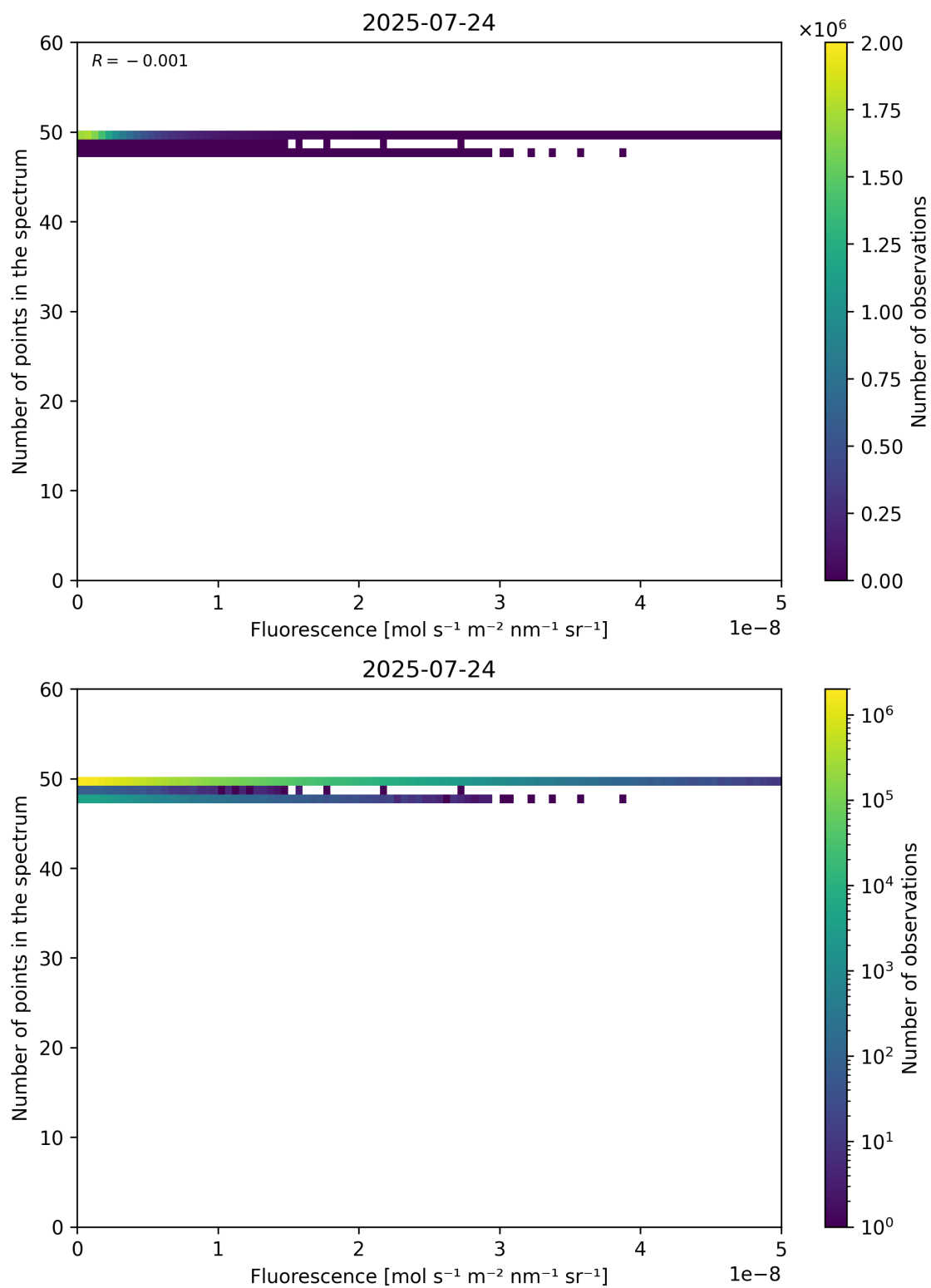
Figure 86: Scatter density plot of “Fluorescence” against “Number of points in the spectrum” for 2025-07-24 to 2025-07-25.
