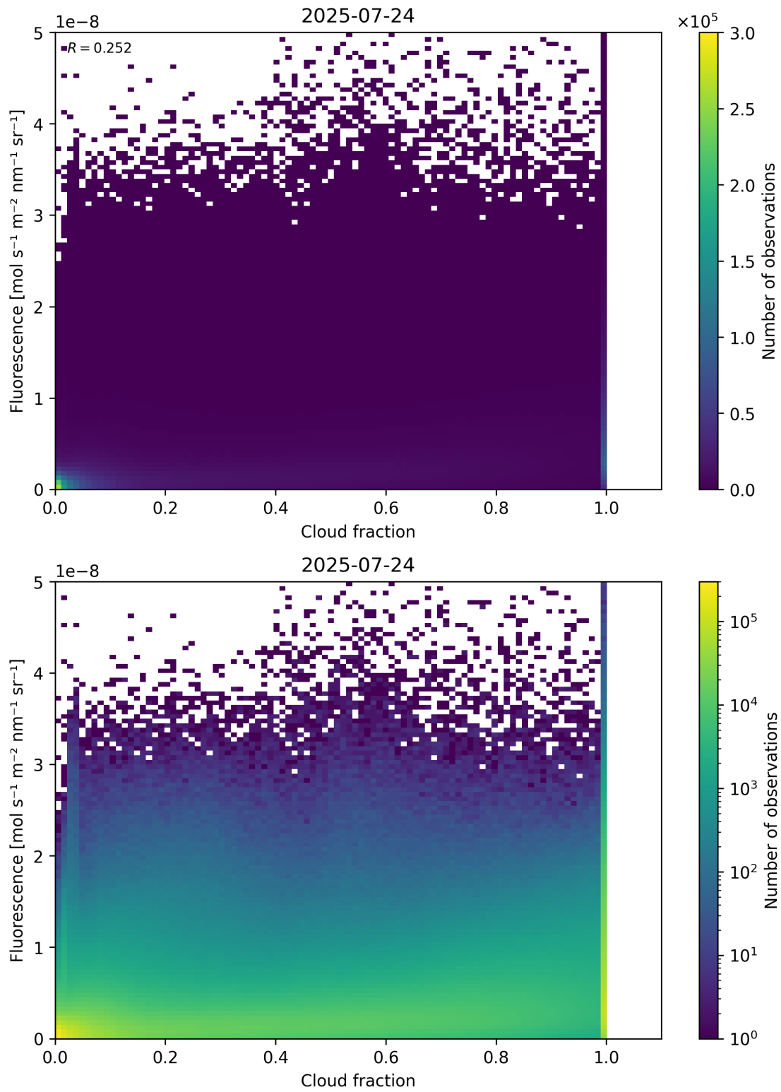
Figure 72: Scatter density plot of “Cloud fraction” against “Fluorescence” for 2025-07-24 to 2025-07-25.
