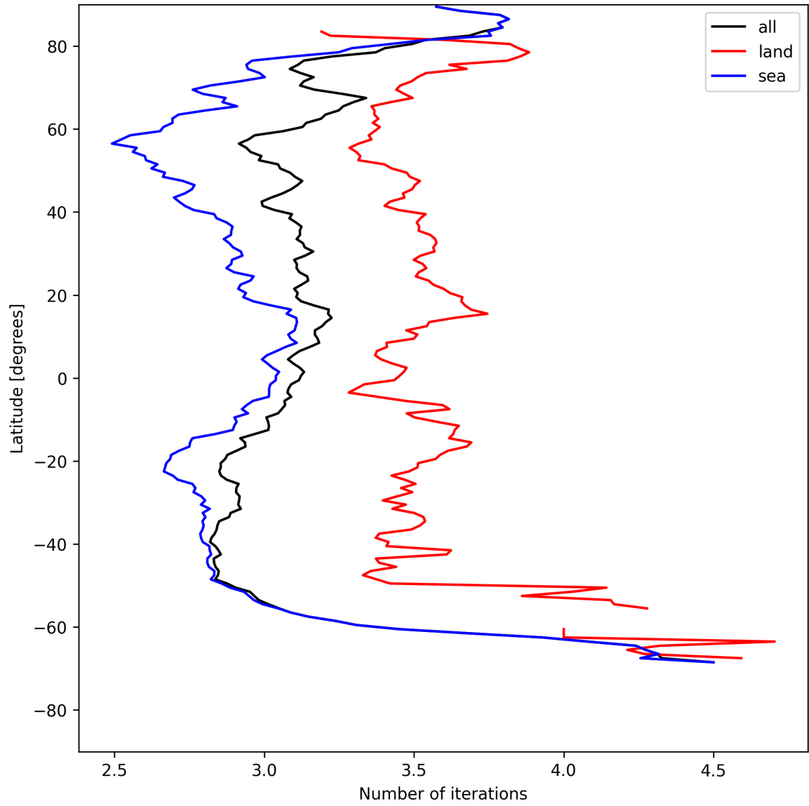
Figure 22: Zonal average of “Number of iterations” for 2025-07-24 to 2025-07-25.
