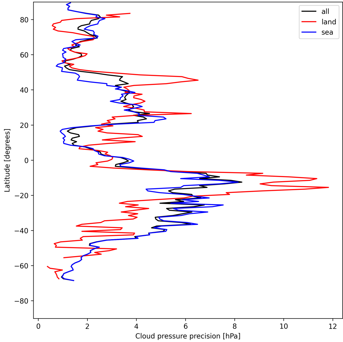
Figure 14: Zonal average of “Cloud pressure precision” for 2025-07-24 to 2025-07-25.
