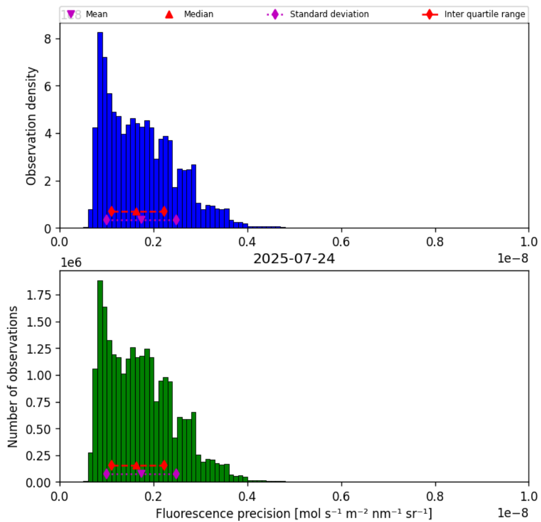
Figure 41: Histogram of “Fluorescence precision” for 2025-07-24 to 2025-07-25
