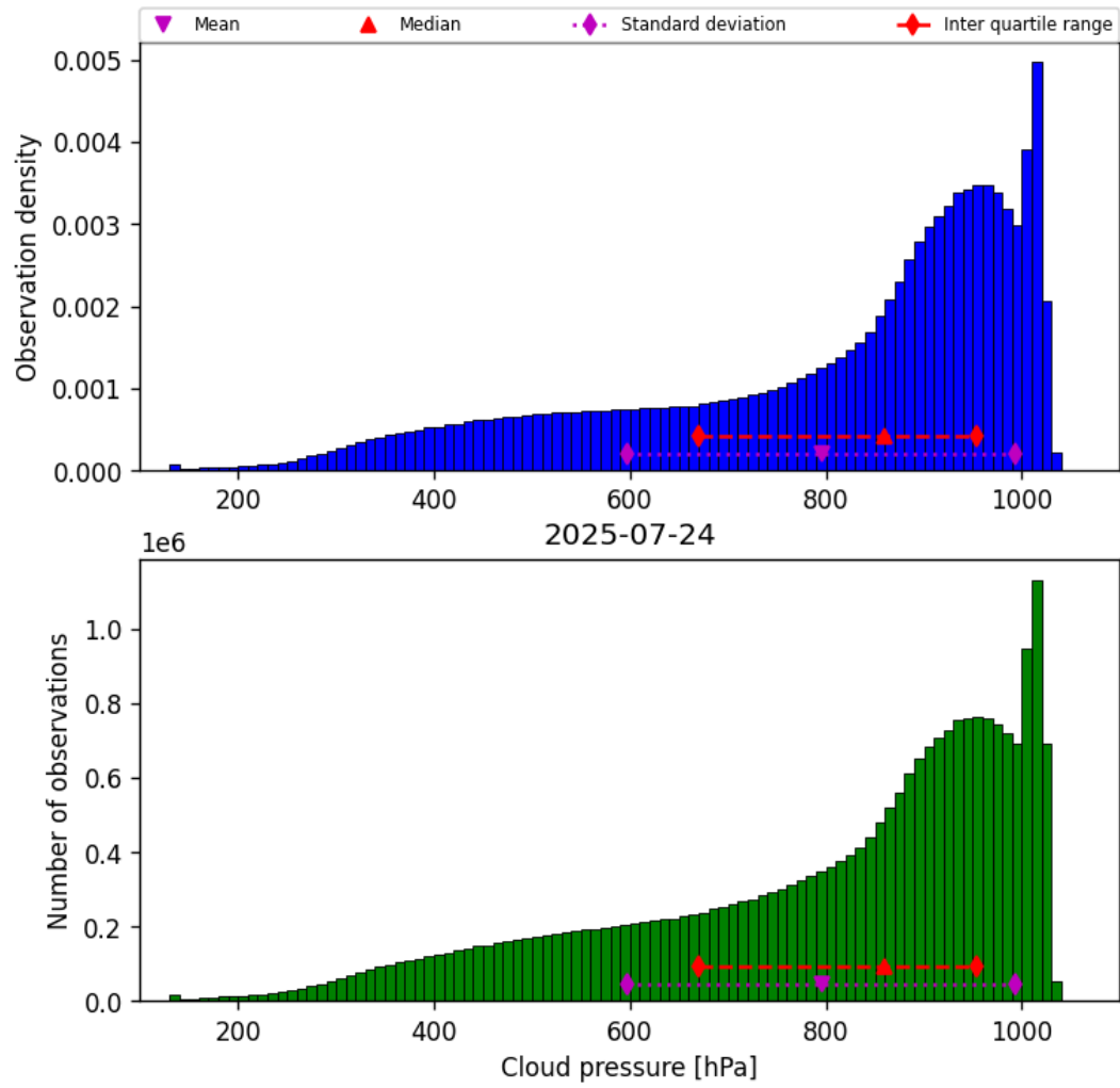
Figure 30: Histogram of “Cloud pressure” for 2025-07-24 to 2025-07-25
