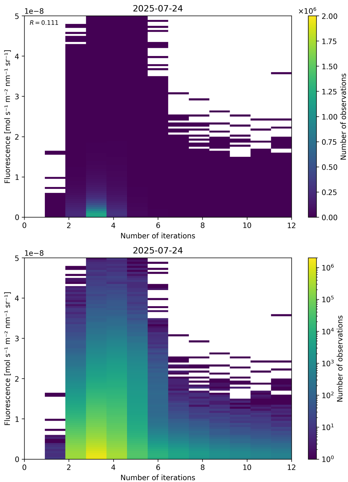
Figure 98: Scatter density plot of “Number of iterations” against “Fluorescence” for 2025-07-24 to 2025-07-25.
