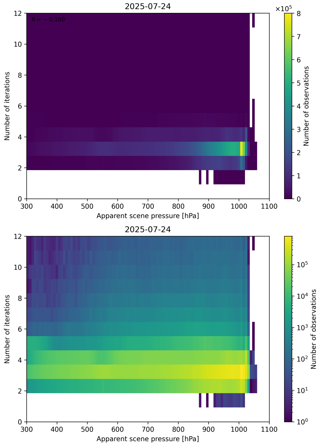
Figure 65: Scatter density plot of “Apparent scene pressure” against “Number of iterations” for 2025-07-24 to 2025-07-25.
