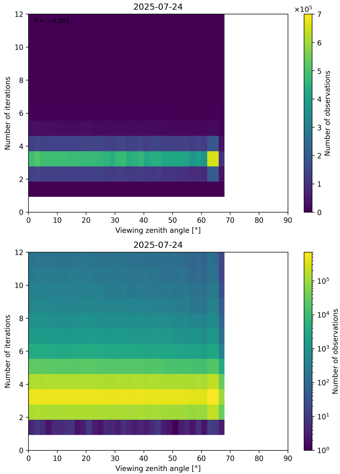
Figure 124: Scatter density plot of “Viewing zenith angle” against “Number of iterations” for 2025-07-24 to 2025-07-25.
