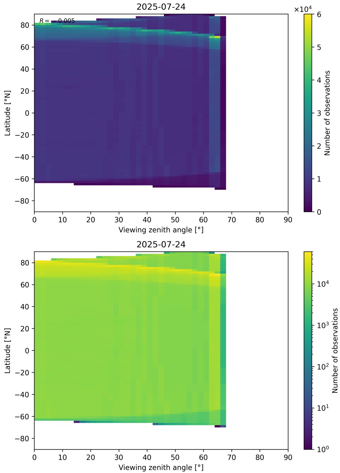
Figure 123: Scatter density plot of “Viewing zenith angle” against “Latitude” for 2025-07-24 to 2025-07-25.
