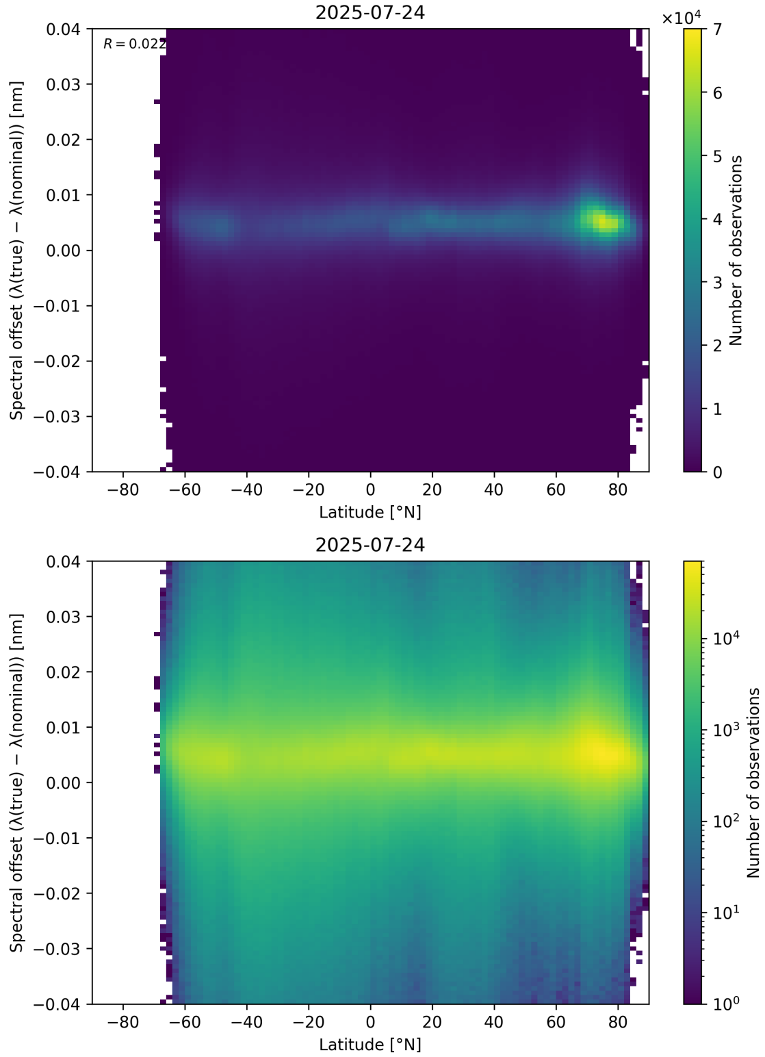
Figure 96: Scatter density plot of “Latitude” against “Spectral offset ( \lambda_{\text{true}} - \lambda_{\text{nominal}} )” for 2025-07-24 to 2025-07-25.
