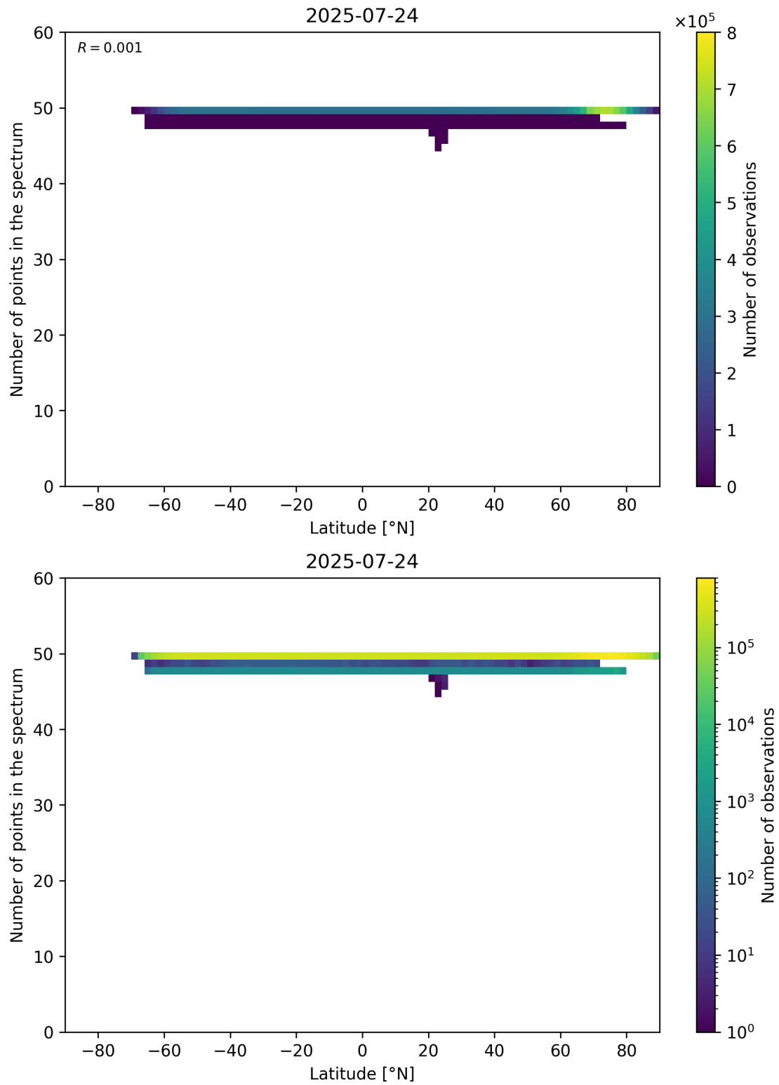
Figure 94: Scatter density plot of “Latitude” against “Number of points in the spectrum” for 2025-07-24 to 2025-07-25.
