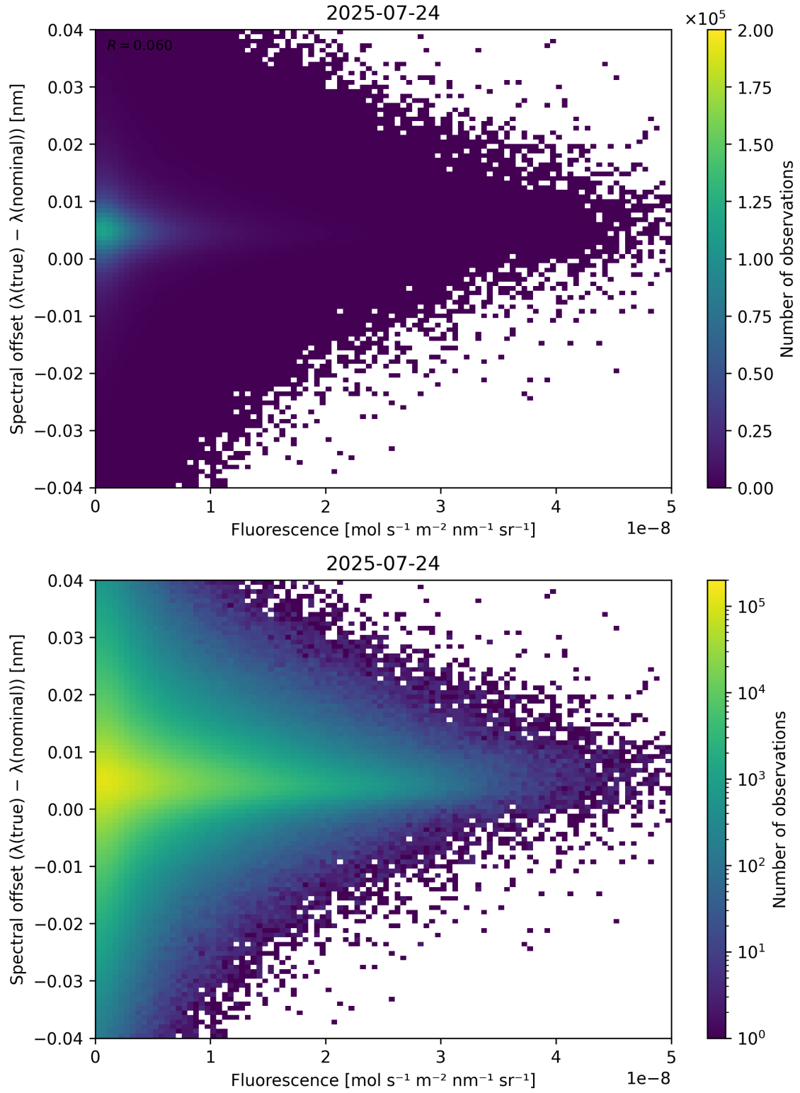
Figure 87: Scatter density plot of “Fluorescence” against “Spectral offset ( \lambda_{\text{true}} - \lambda_{\text{nominal}} )” for 2025-07-24 to 2025-07-25.
