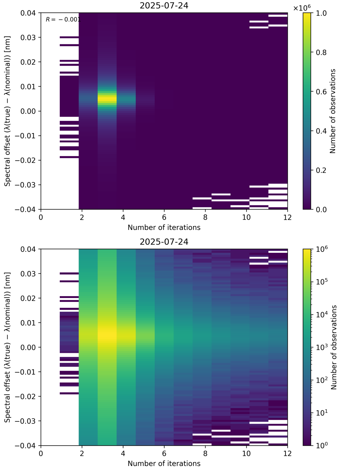
Figure 100: Scatter density plot of “Number of iterations” against “Spectral offset ( \lambda_{\text{true}} - \lambda_{\text{nominal}} )” for 2025-07-24 to 2025-07-25.
