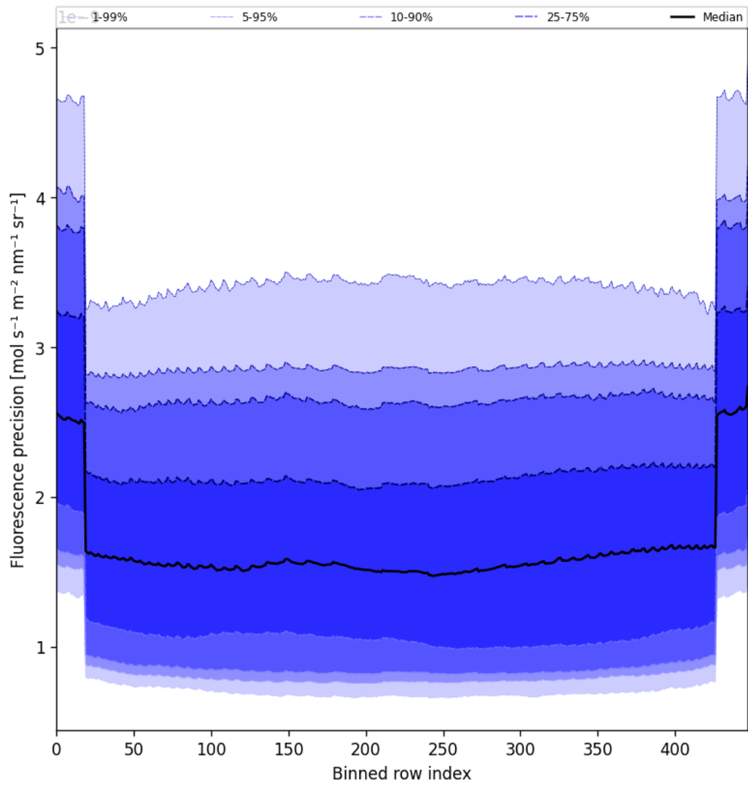
Figure 58: Along track statistics of “Fluorescence precision” for 2025-07-24 to 2025-07-25
