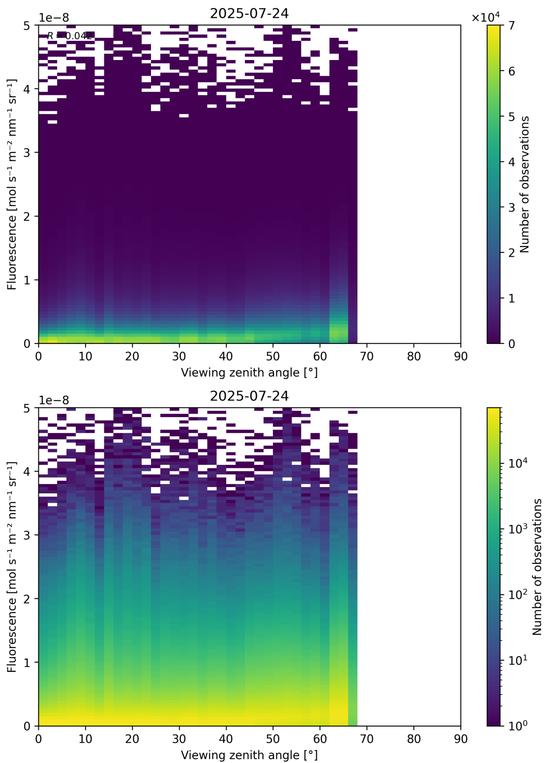
Figure 122: Scatter density plot of “Viewing zenith angle” against “Fluorescence” for 2025-07-24 to 2025-07-25.
