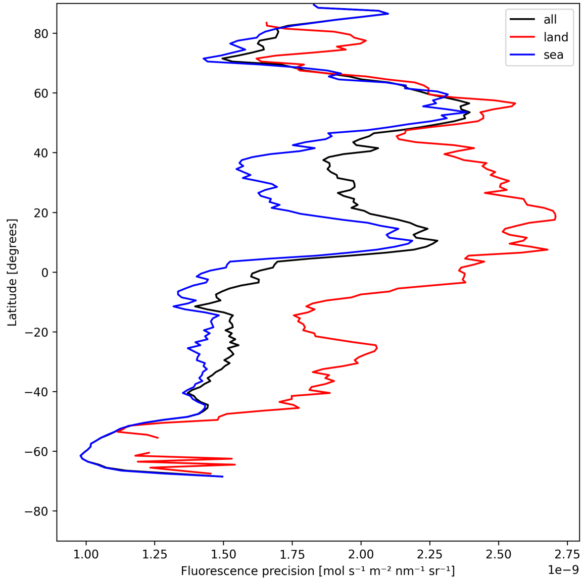
Figure 24: Zonal average of “Fluorescence precision” for 2025-07-24 to 2025-07-25.
