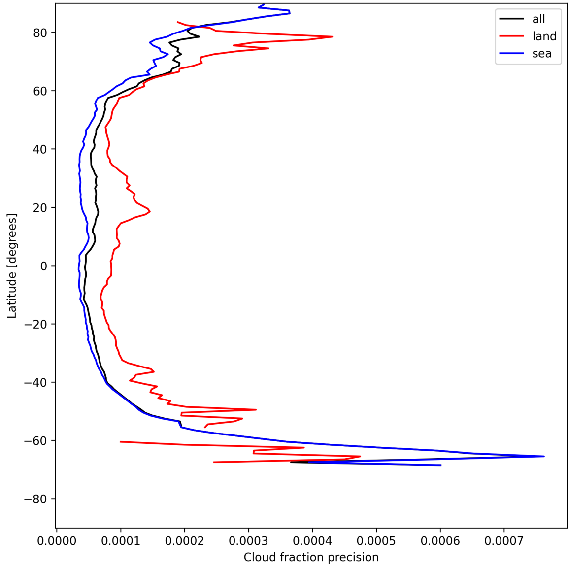
Figure 16: Zonal average of “Cloud fraction precision” for 2025-07-24 to 2025-07-25.
