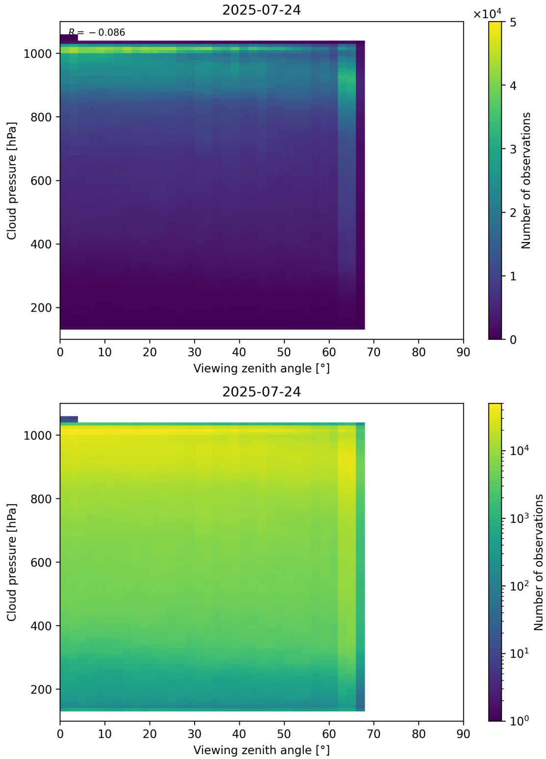
Figure 121: Scatter density plot of “Viewing zenith angle” against “Cloud pressure” for 2025-07-24 to 2025-07-25.
