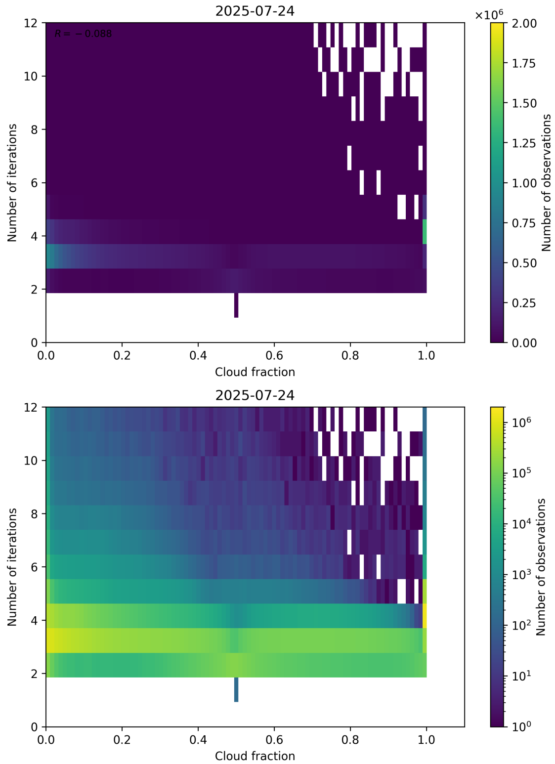
Figure 73: Scatter density plot of “Cloud fraction” against “Number of iterations” for 2025-07-24 to 2025-07-25.
