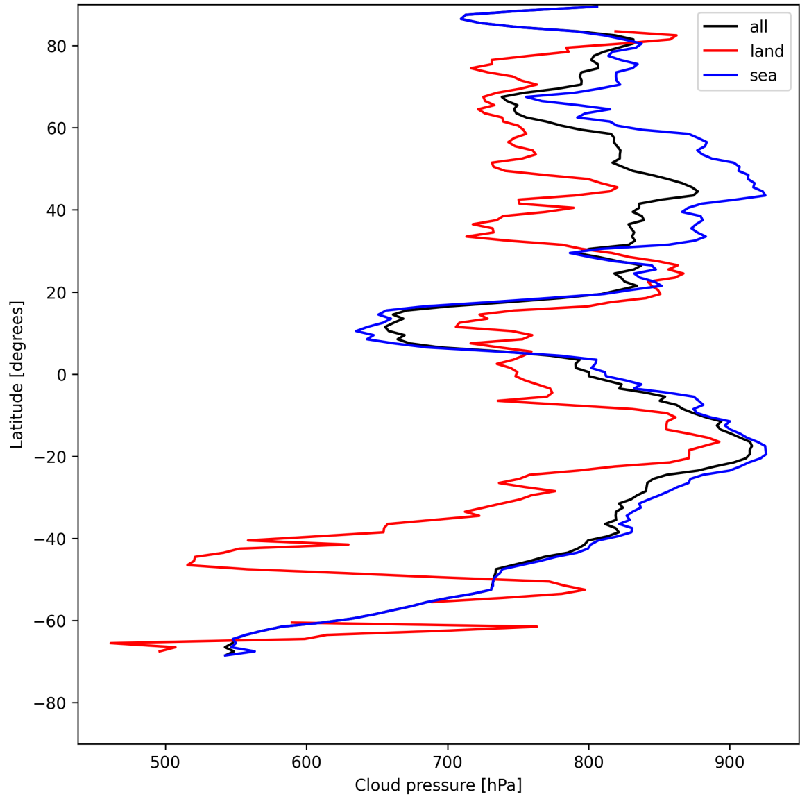
Figure 13: Zonal average of “Cloud pressure” for 2025-07-24 to 2025-07-25.
