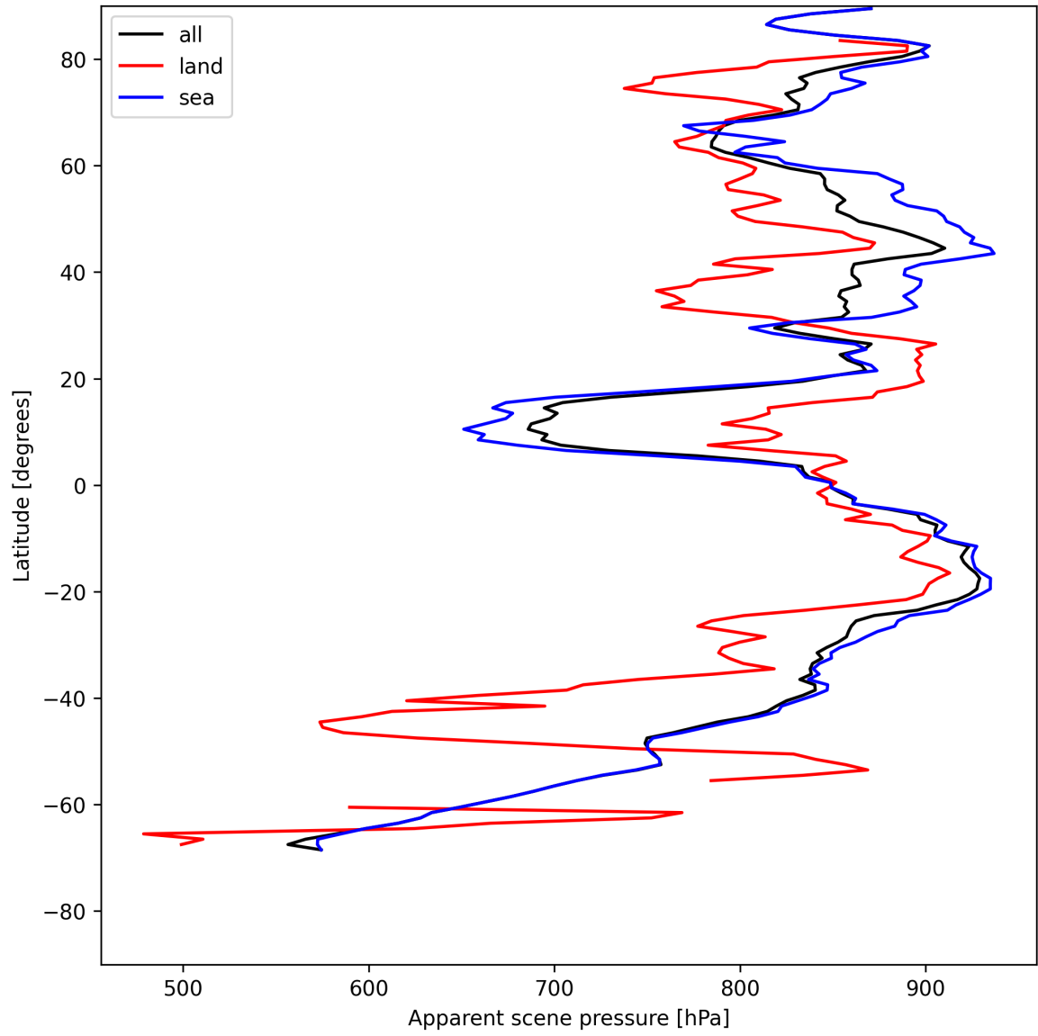
Figure 19: Zonal average of “Apparent scene pressure” for 2025-07-24 to 2025-07-25.
