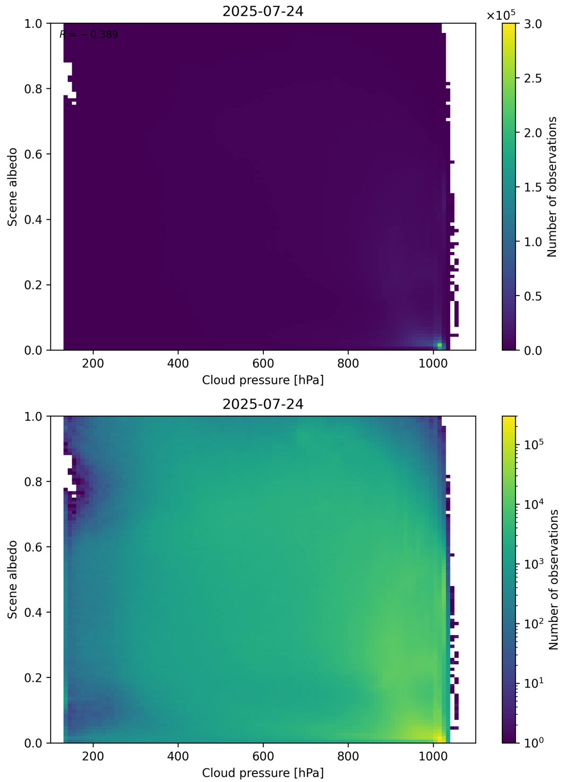
Figure 83: Scatter density plot of “Cloud pressure” against “Scene albedo” for 2025-07-24 to 2025-07-25.
