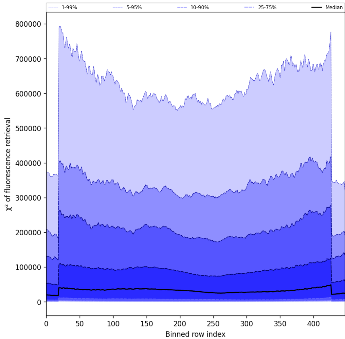
Figure 59: Along track statistics of “ \chi^2 of fluorescence retrieval” for 2025-07-24 to 2025-07-25
