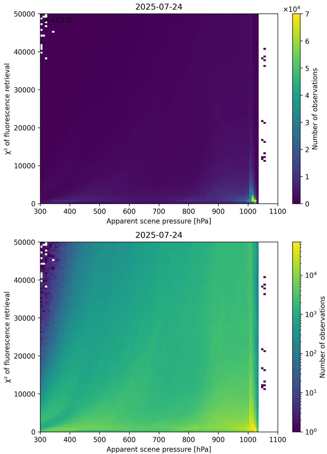
Figure 63: Scatter density plot of “Apparent scene pressure” against “ \chi^2 of fluorescence retrieval” for 2025-07-24 to 2025-07-25.
