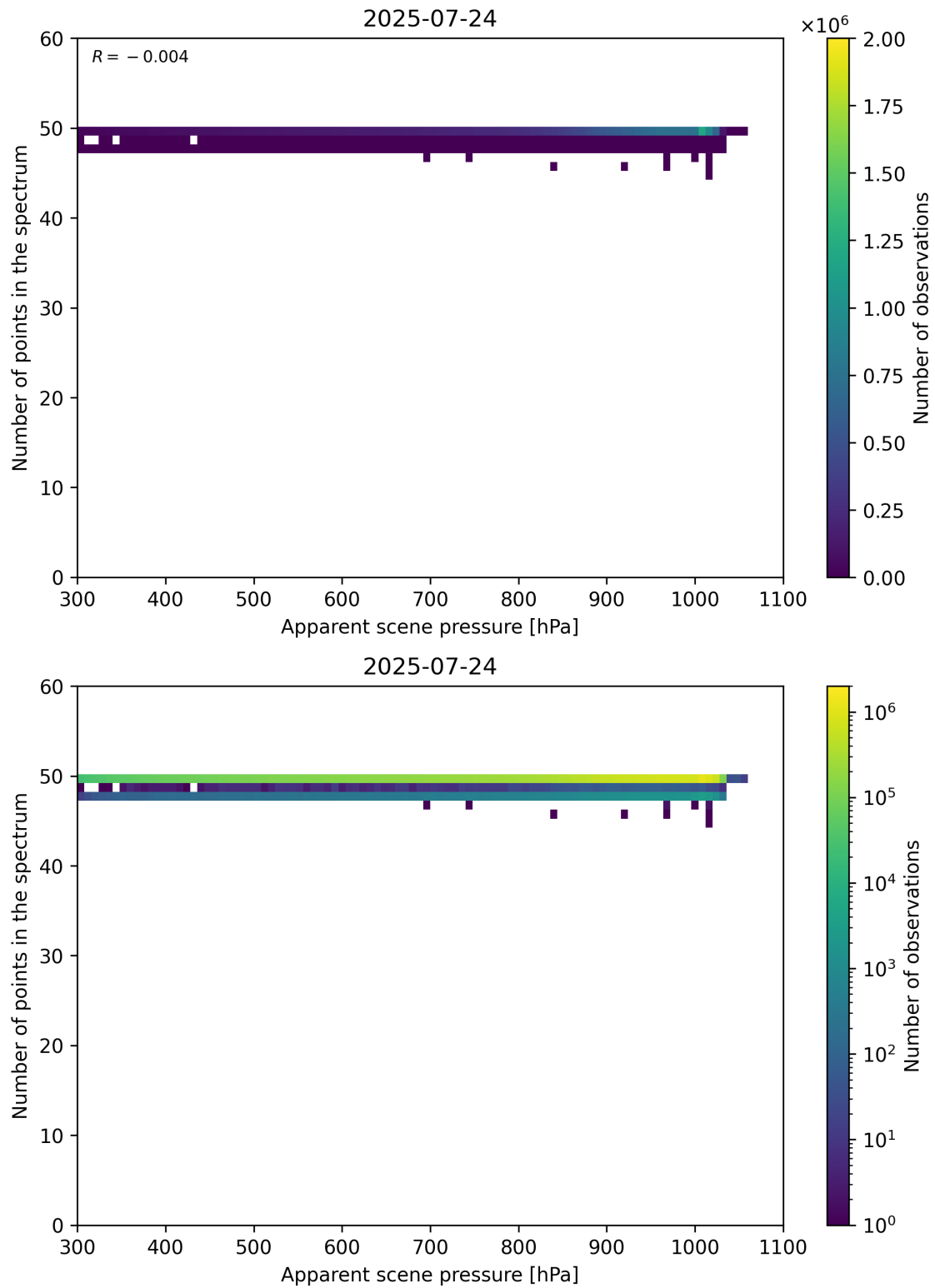
Figure 66: Scatter density plot of “Apparent scene pressure” against “Number of points in the spectrum” for 2025-07-24 to 2025-07-25.
