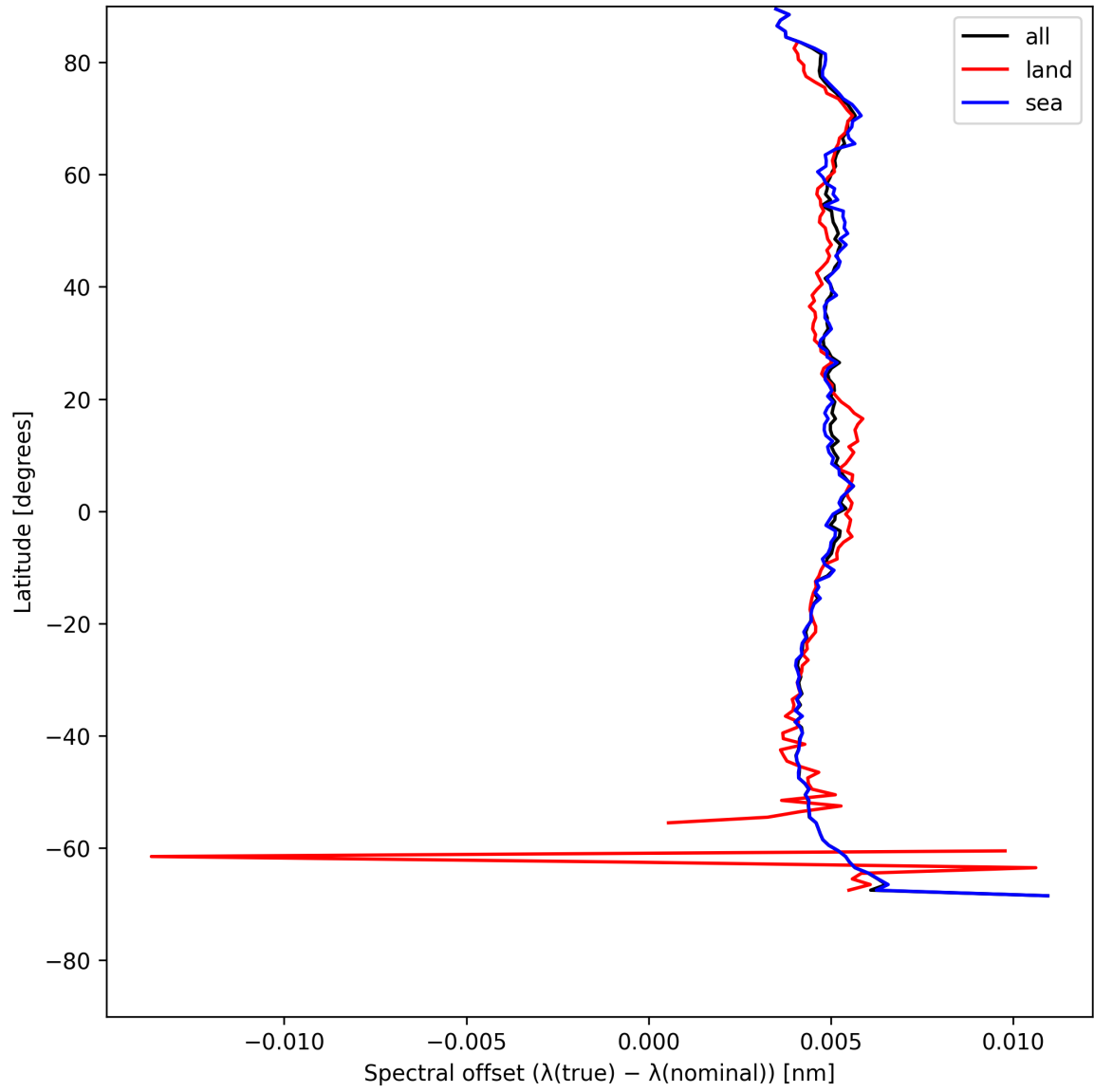
Figure 28: Zonal average of “Spectral offset ( \lambda_{\text{true}} - \lambda_{\text{nominal}} )” for 2025-07-24 to 2025-07-25.
