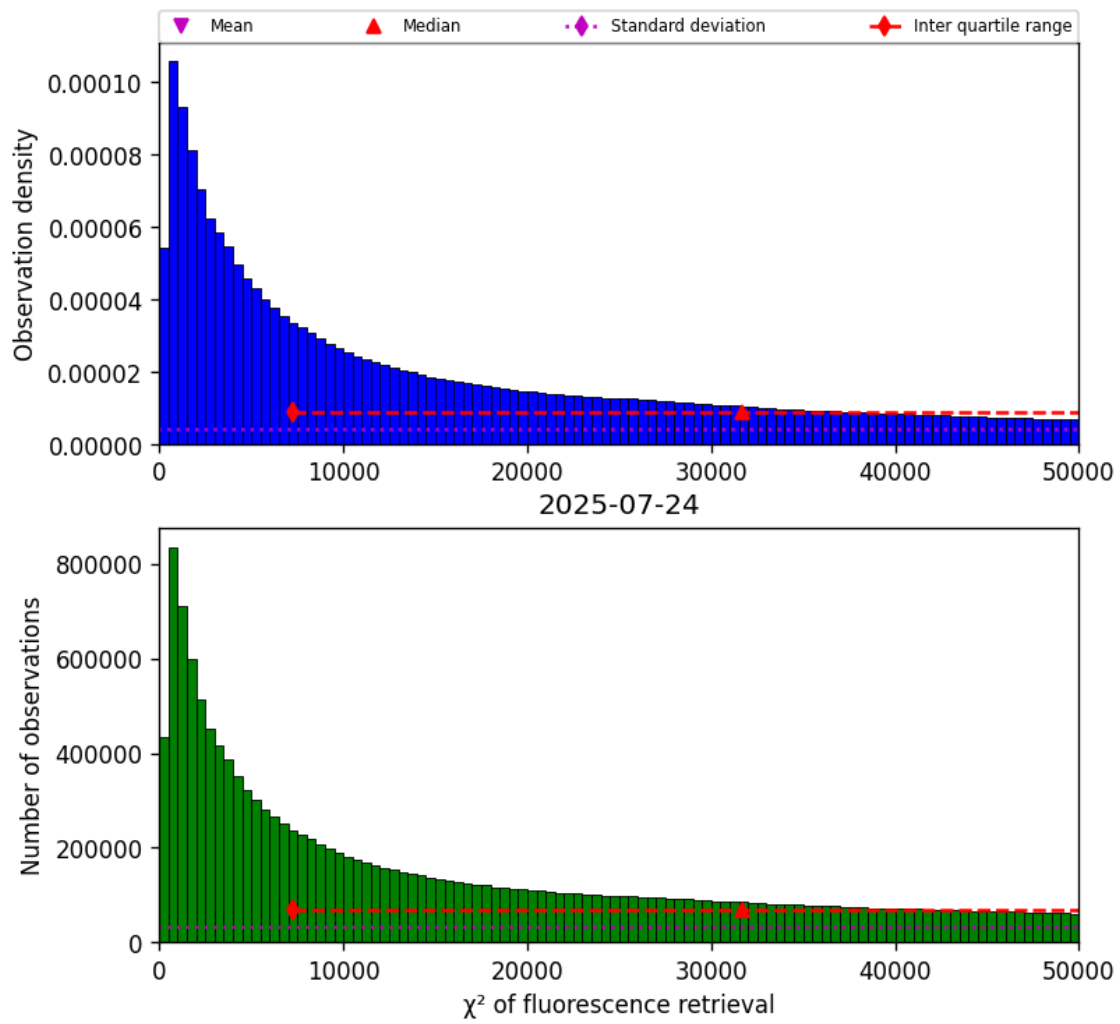
Figure 42: Histogram of “ \chi^2 of fluorescence retrieval” for 2025-07-24 to 2025-07-25
