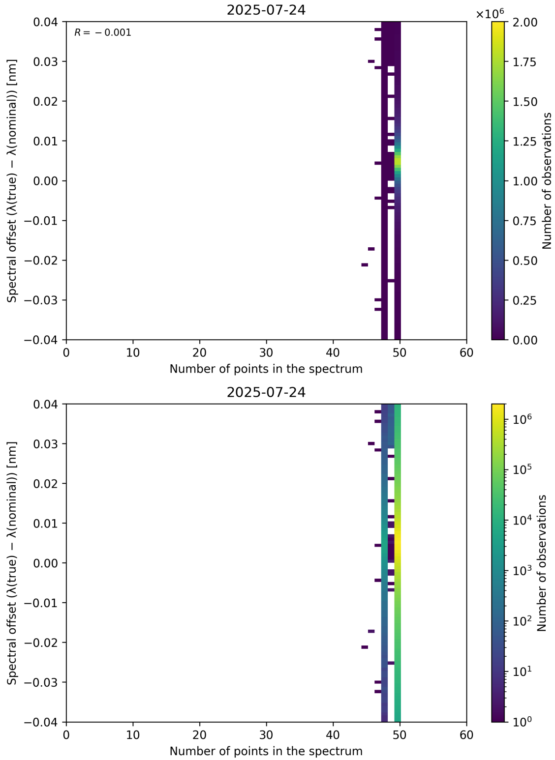
Figure 101: Scatter density plot of “Number of points in the spectrum” against “Spectral offset ( \lambda_{\text{true}} - \lambda_{\text{nominal}} )” for 2025-07-24 to 2025-07-25.
