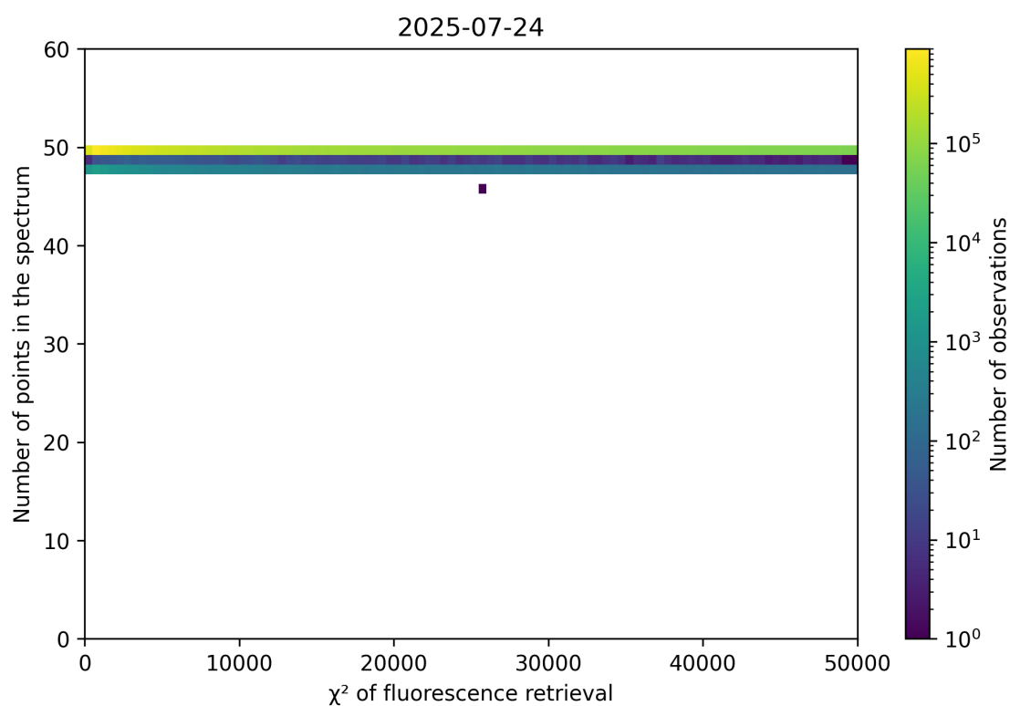
Figure 68: Scatter density plot of “ \chi^2 of fluorescence retrieval” against “Number of points in the spectrum” for 2025-07-24 to 2025-07-25.
