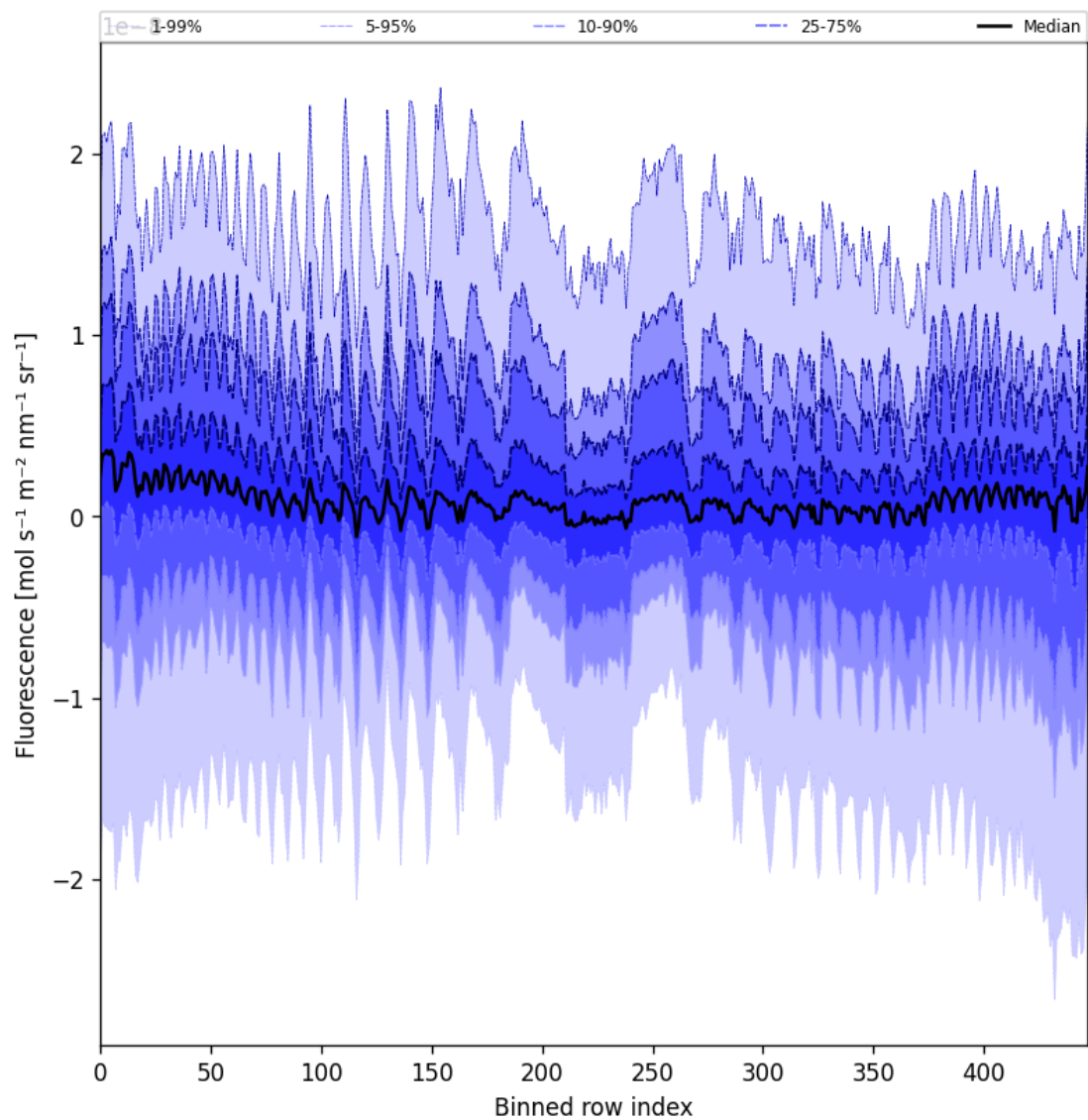
Figure 57: Along track statistics of "Fluorescence" for 2025-07-24 to 2025-07-25
