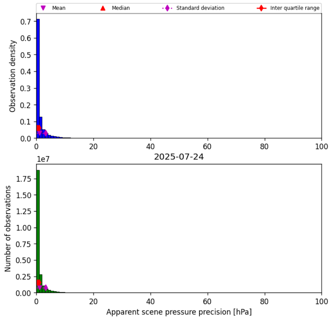
Figure 37: Histogram of “Apparent scene pressure precision” for 2025-07-24 to 2025-07-25
