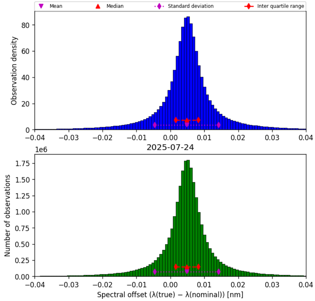
Figure 45: Histogram of “Spectral offset ( \lambda_{\text{true}} - \lambda_{\text{nominal}} )” for 2025-07-24 to 2025-07-25
