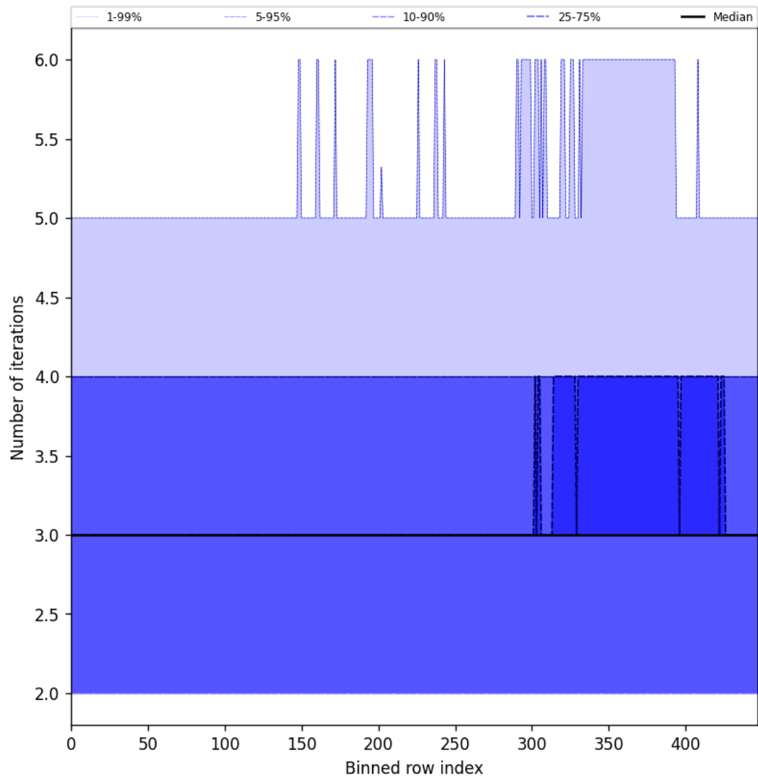
Figure 56: Along track statistics of “Number of iterations” for 2025-07-24 to 2025-07-25
