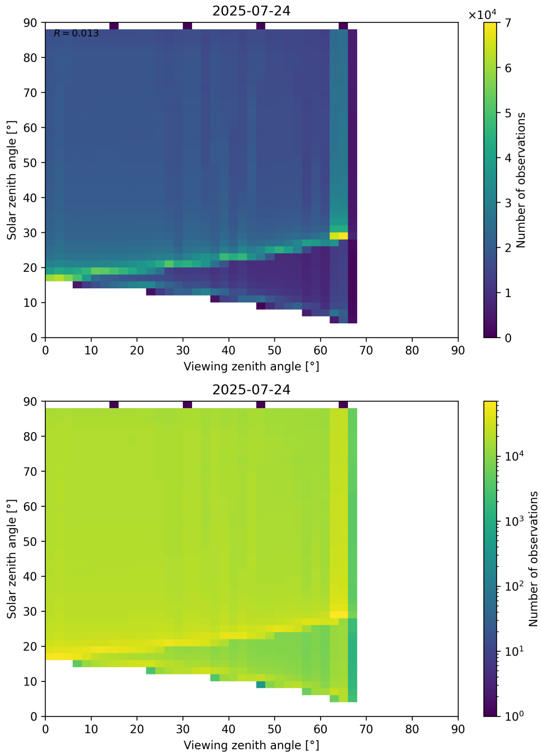
Figure 127: Scatter density plot of “Viewing zenith angle” against “Solar zenith angle” for 2025-07-24 to 2025-07-25.
