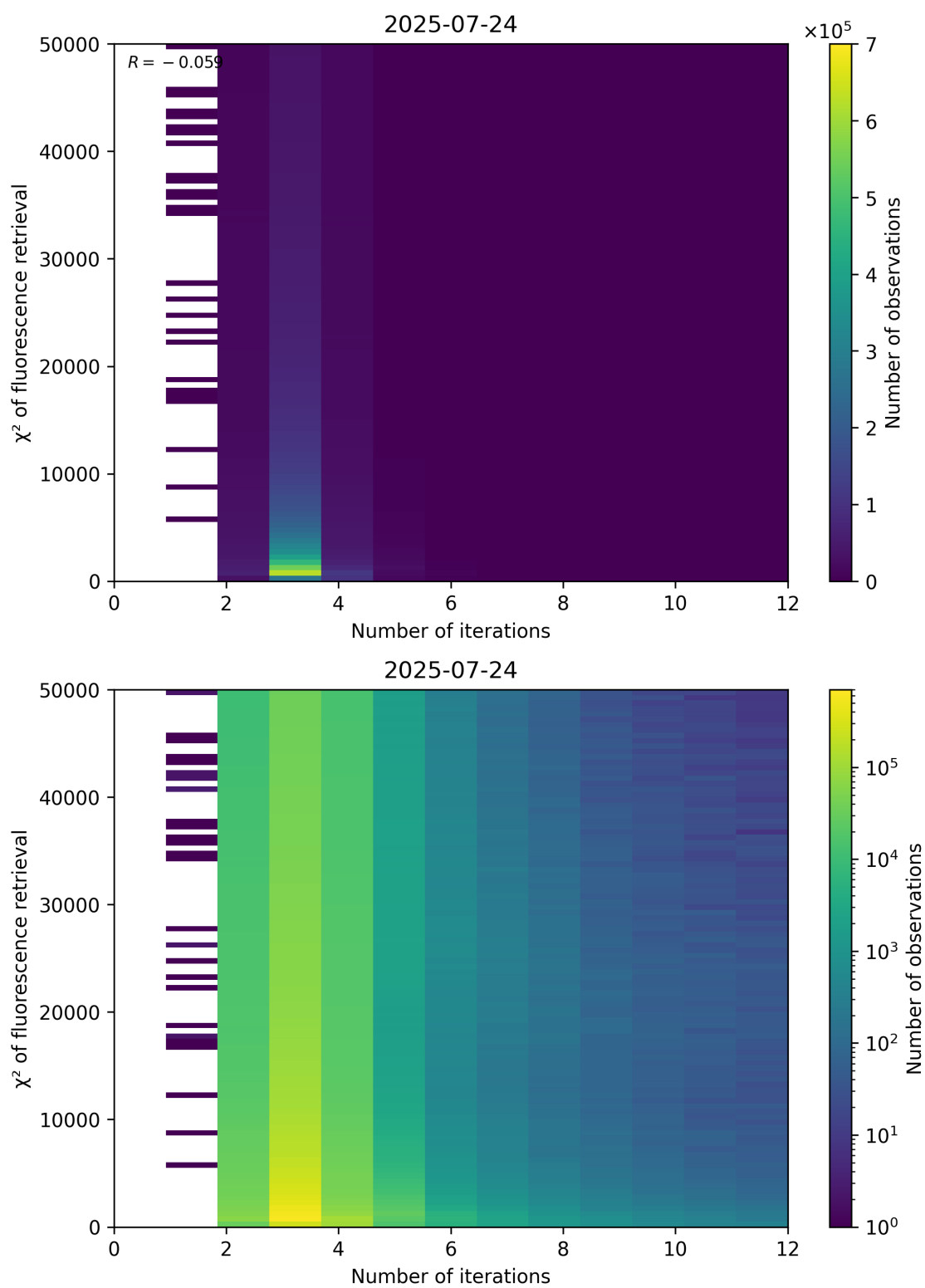
Figure 97: Scatter density plot of “Number of iterations” against “ \chi^2 of fluorescence retrieval” for 2025-07-24 to 2025-07-25.
