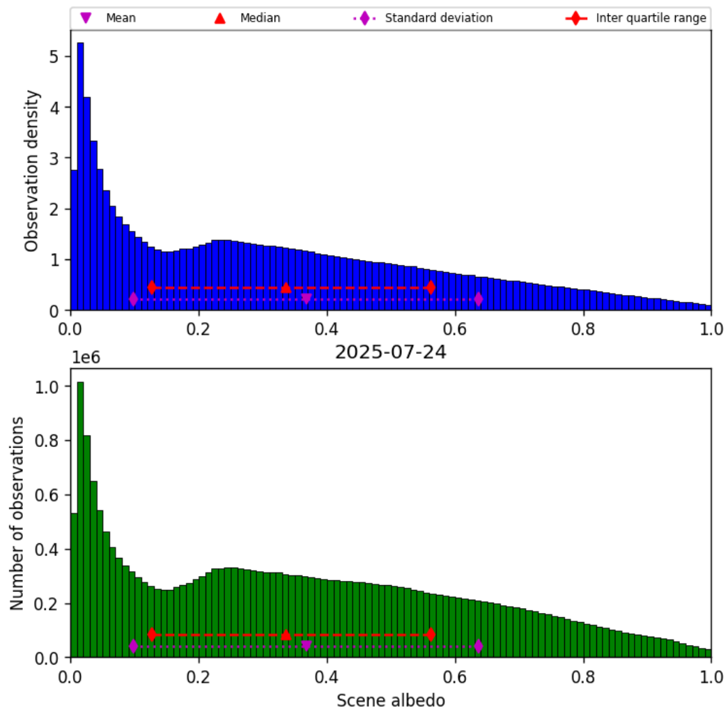
Figure 34: Histogram of “Scene albedo” for 2025-07-24 to 2025-07-25
