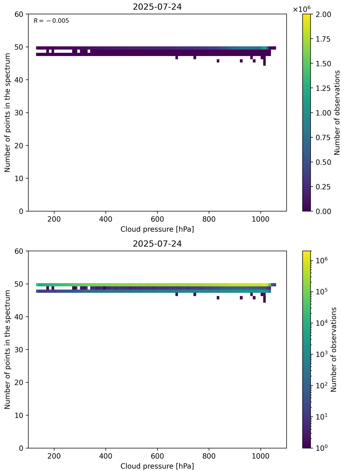
Figure 82: Scatter density plot of “Cloud pressure” against “Number of points in the spectrum” for 2025-07-24 to 2025-07-25.
