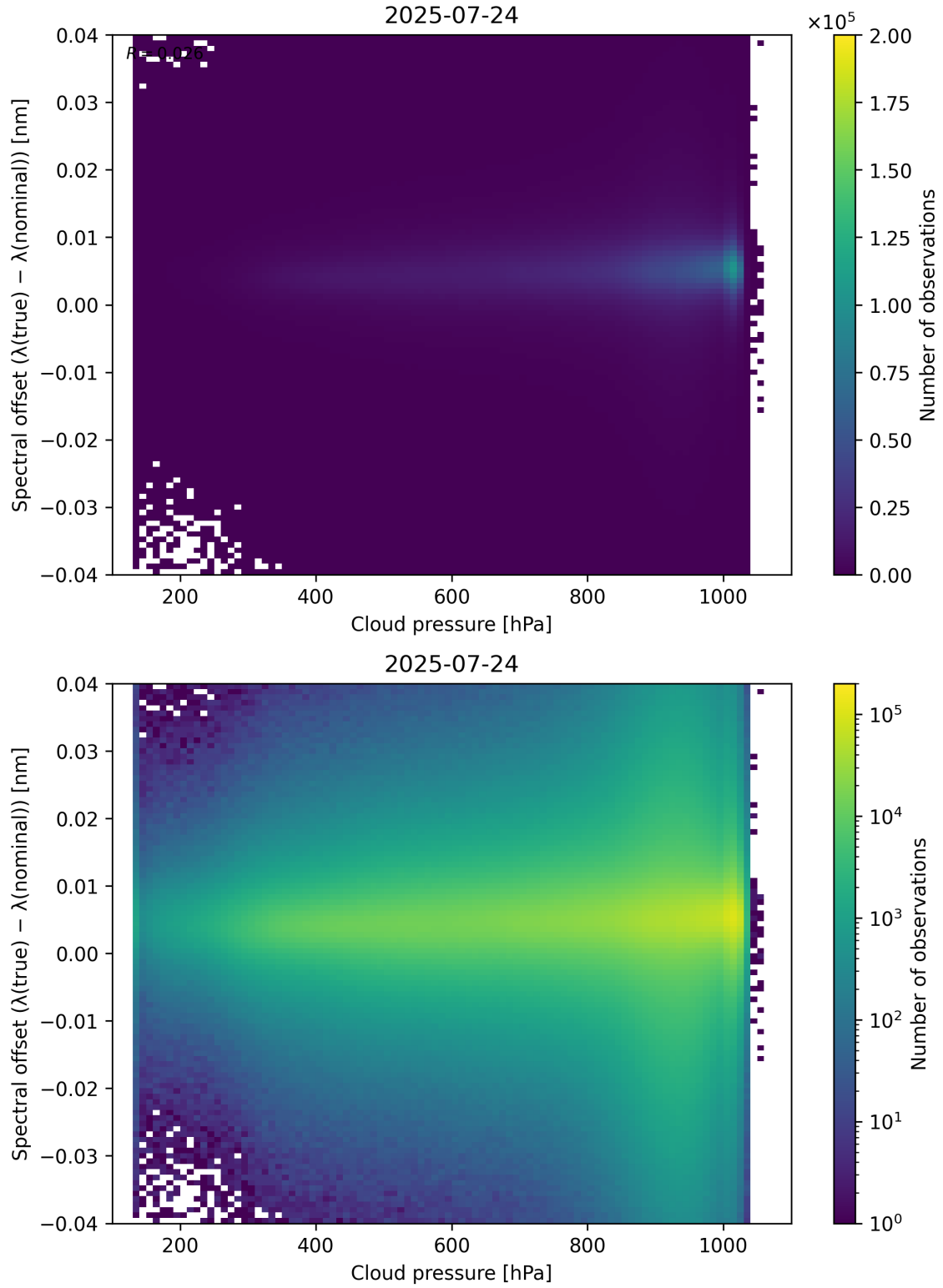
Figure 84: Scatter density plot of “Cloud pressure” against “Spectral offset ( \lambda_{\text{true}} - \lambda_{\text{nominal}} )” for 2025-07-24 to 2025-07-25.
