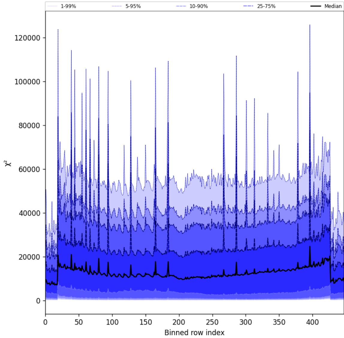
Figure 55: Along track statistics of “ \chi^2 ” for 2025-07-24 to 2025-07-25
