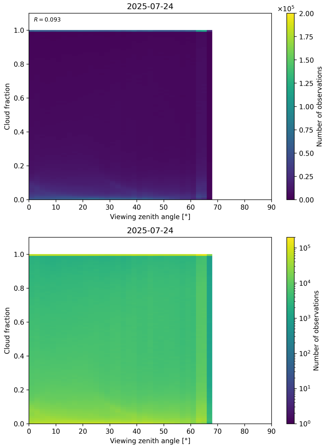
Figure 120: Scatter density plot of “Viewing zenith angle” against “Cloud fraction” for 2025-07-24 to 2025-07-25.
