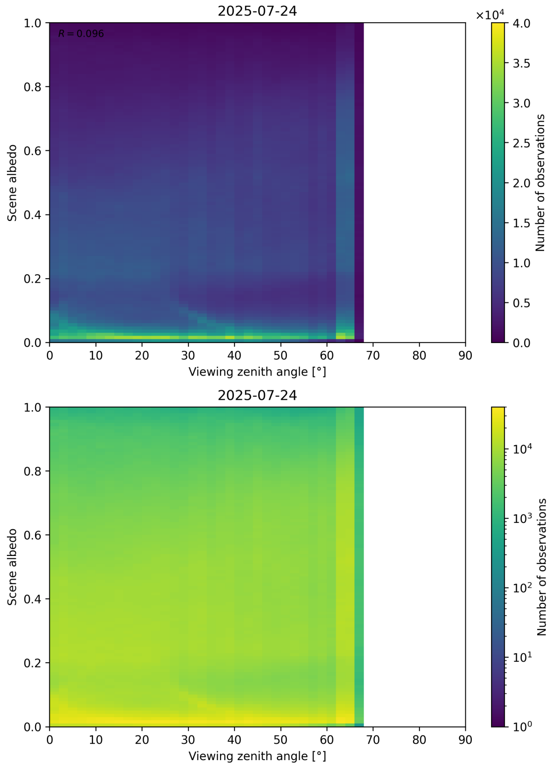
Figure 126: Scatter density plot of “Viewing zenith angle” against “Scene albedo” for 2025-07-24 to 2025-07-25.
