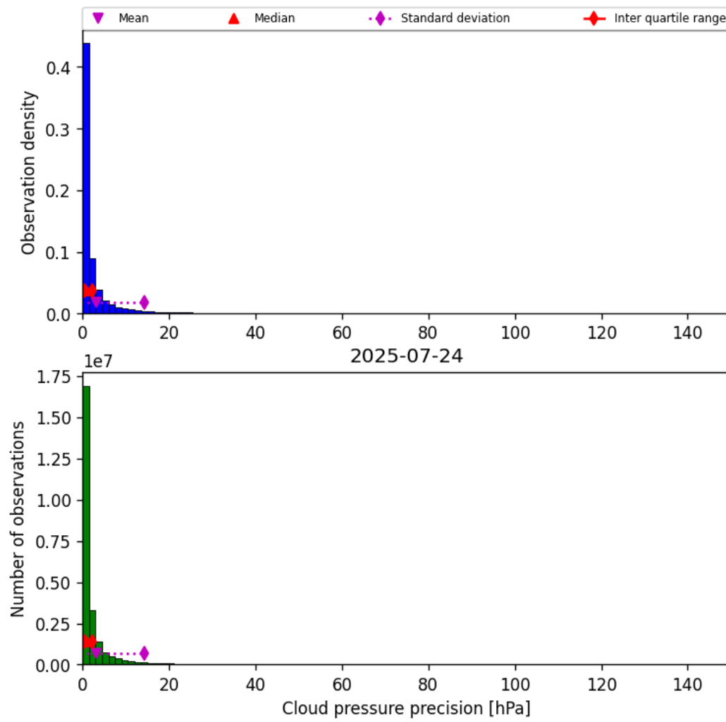
Figure 31: Histogram of “Cloud pressure precision” for 2025-07-24 to 2025-07-25
