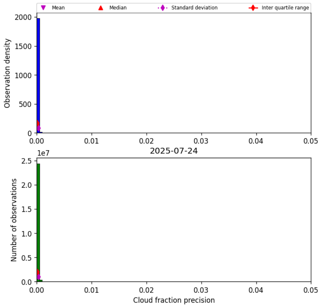
Figure 33: Histogram of “Cloud fraction precision” for 2025-07-24 to 2025-07-25
