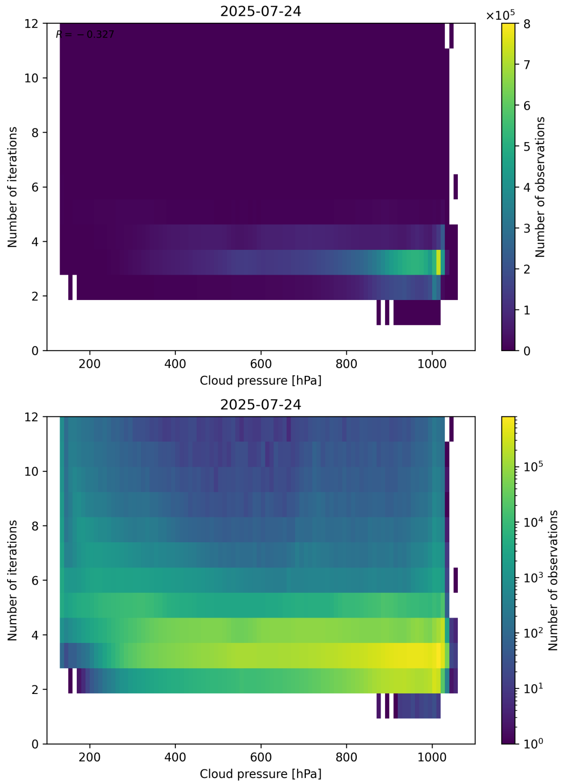
Figure 81: Scatter density plot of “Cloud pressure” against “Number of iterations” for 2025-07-24 to 2025-07-25.
