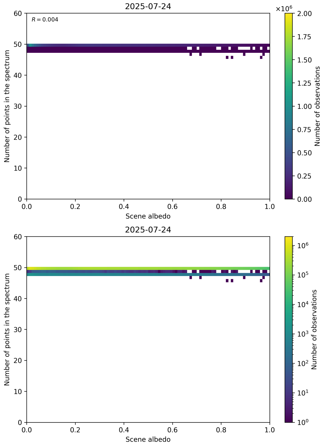
Figure 106: Scatter density plot of “Scene albedo” against “Number of points in the spectrum” for 2025-07-24 to 2025-07-25.
