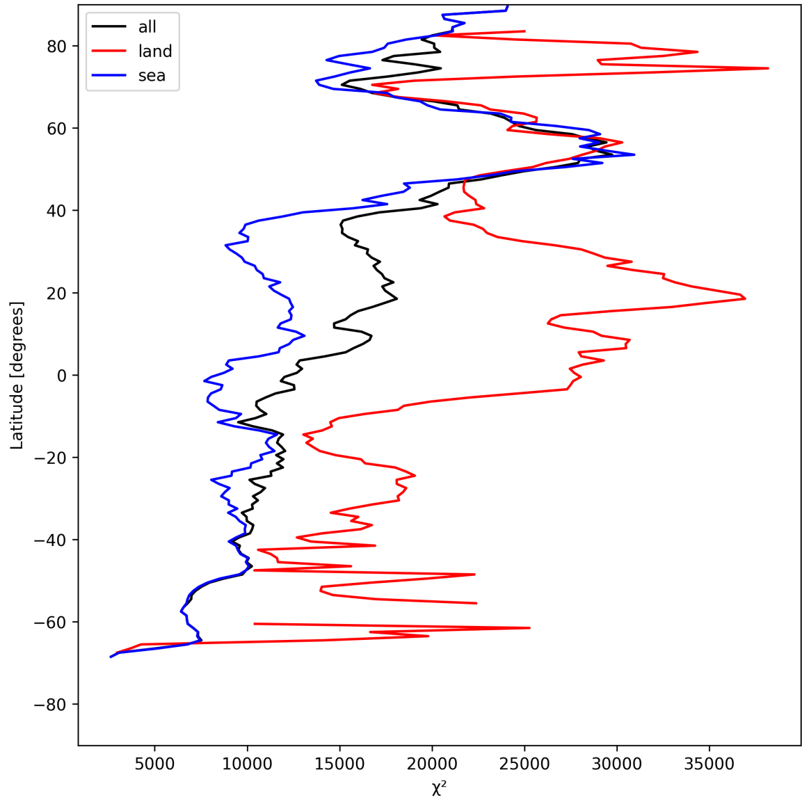
Figure 21: Zonal average of “ \chi^2 ” for 2025-07-24 to 2025-07-25.
