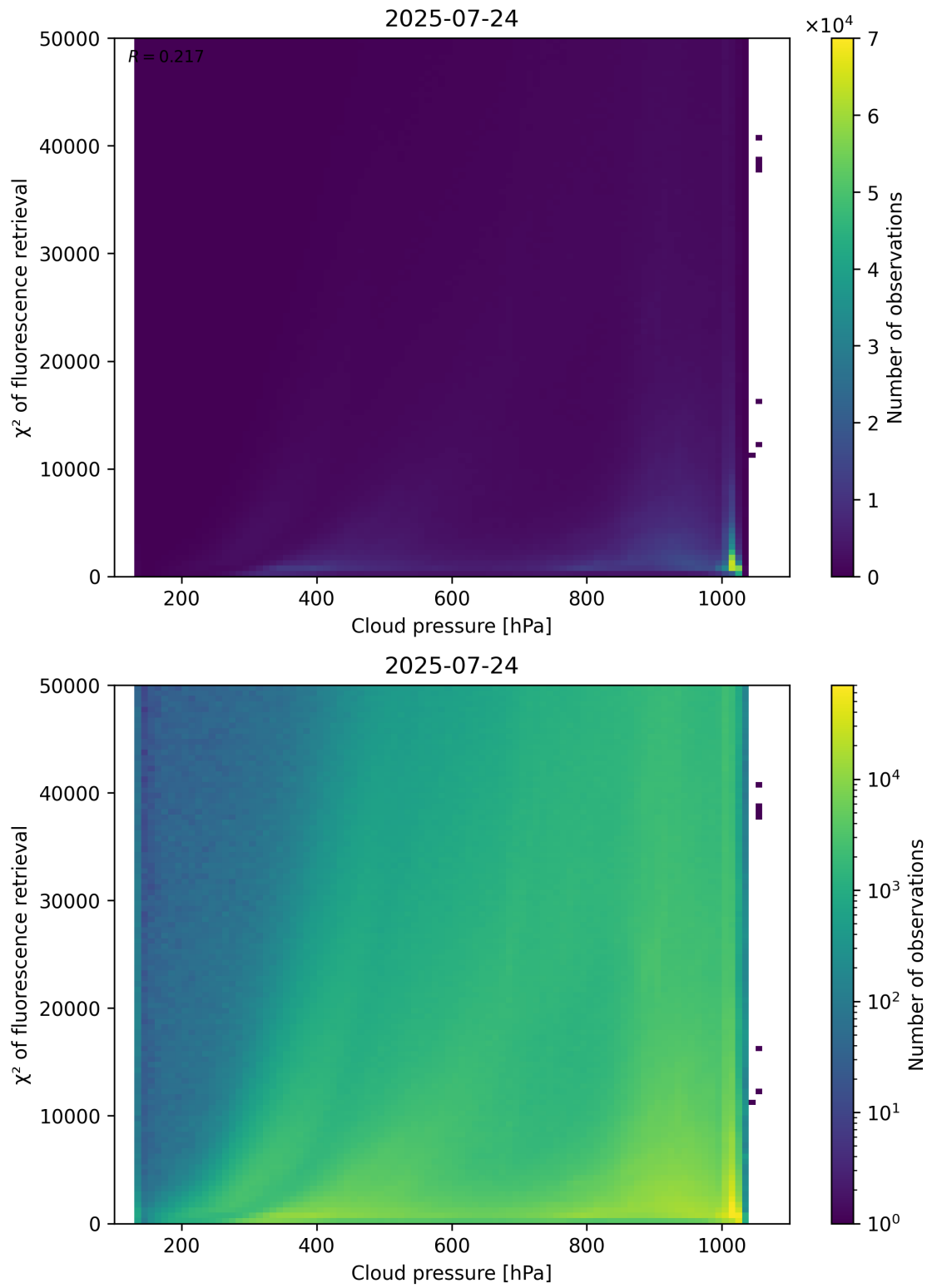
Figure 78: Scatter density plot of “Cloud pressure” against “ \chi^2 of fluorescence retrieval” for 2025-07-24 to 2025-07-25.
