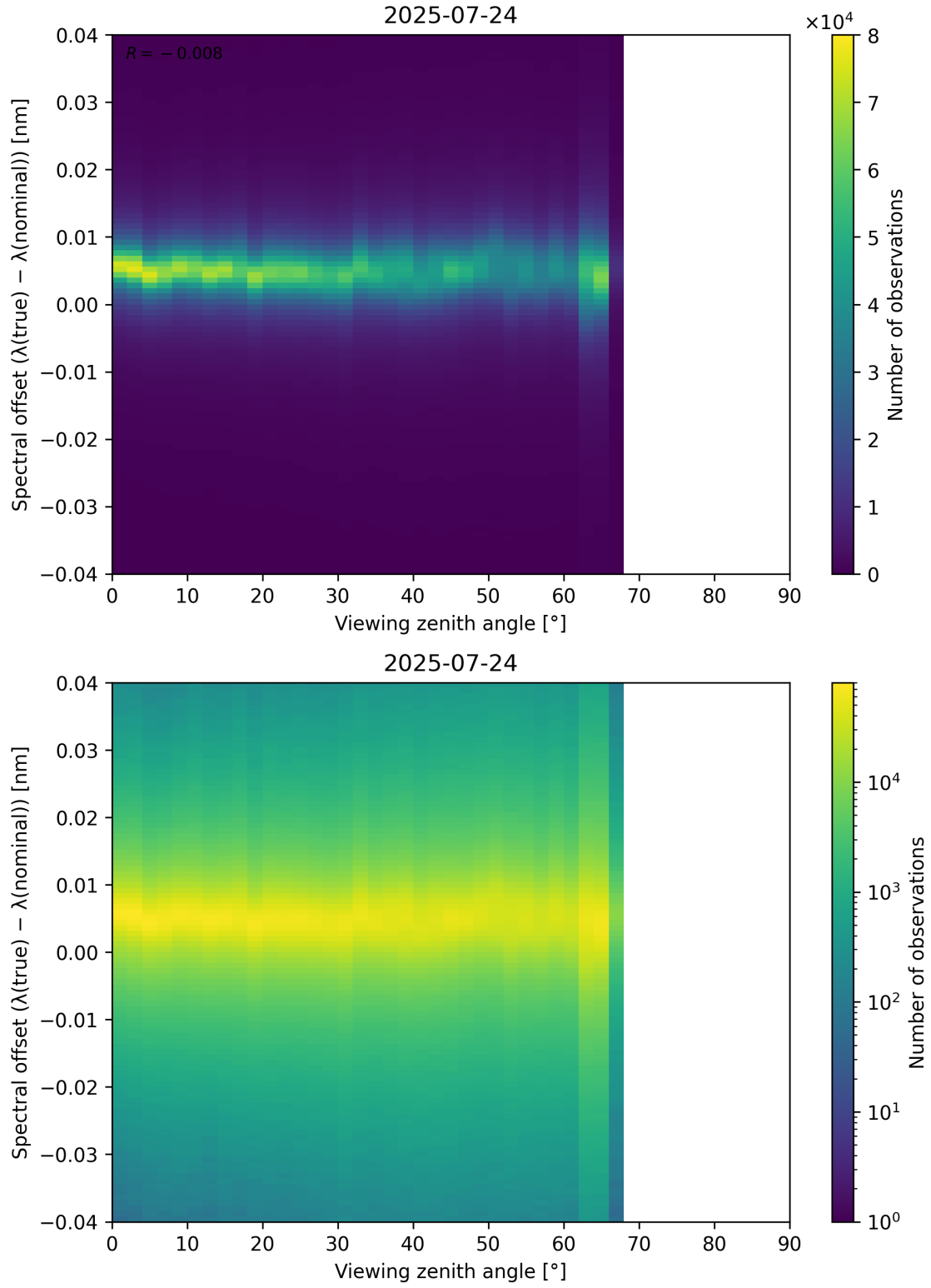
Figure 128: Scatter density plot of “Viewing zenith angle” against “Spectral offset ( \lambda_{\text{true}} - \lambda_{\text{nominal}} )” for 2025-07-24 to 2025-07-25.
