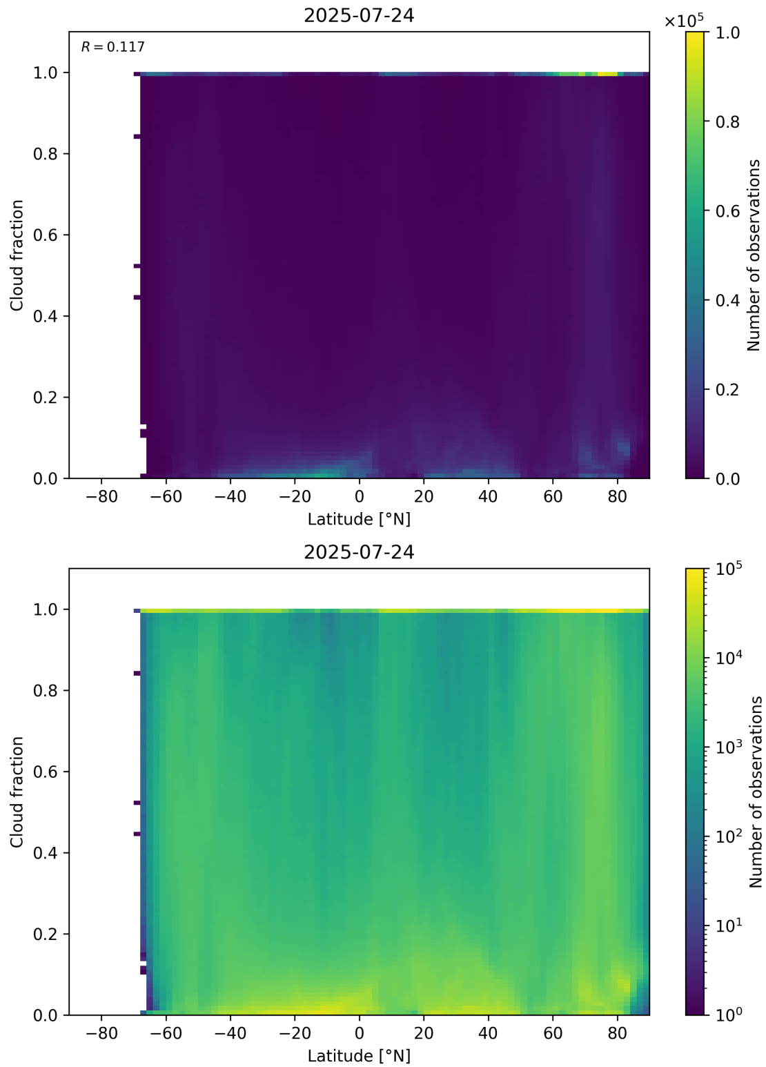
Figure 90: Scatter density plot of “Latitude” against “Cloud fraction” for 2025-07-24 to 2025-07-25.
