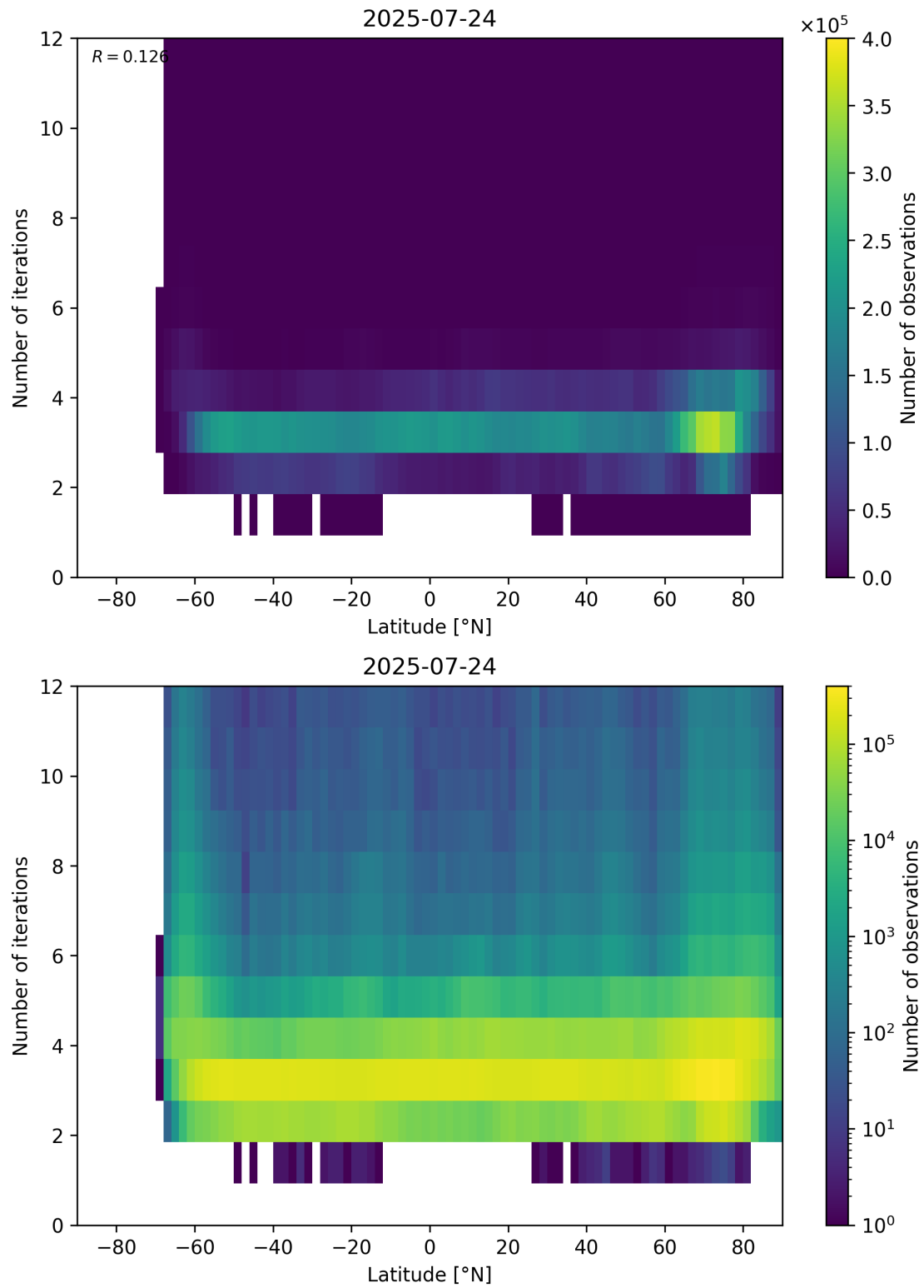
Figure 93: Scatter density plot of “Latitude” against “Number of iterations” for 2025-07-24 to 2025-07-25.
