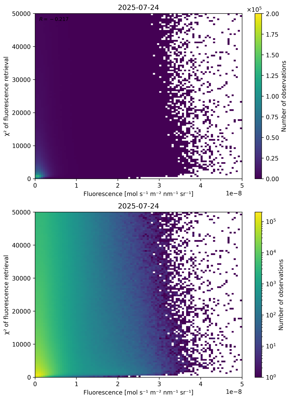
Figure 85: Scatter density plot of “Fluorescence” against “ \chi^2 of fluorescence retrieval” for 2025-07-24 to 2025-07-25.
