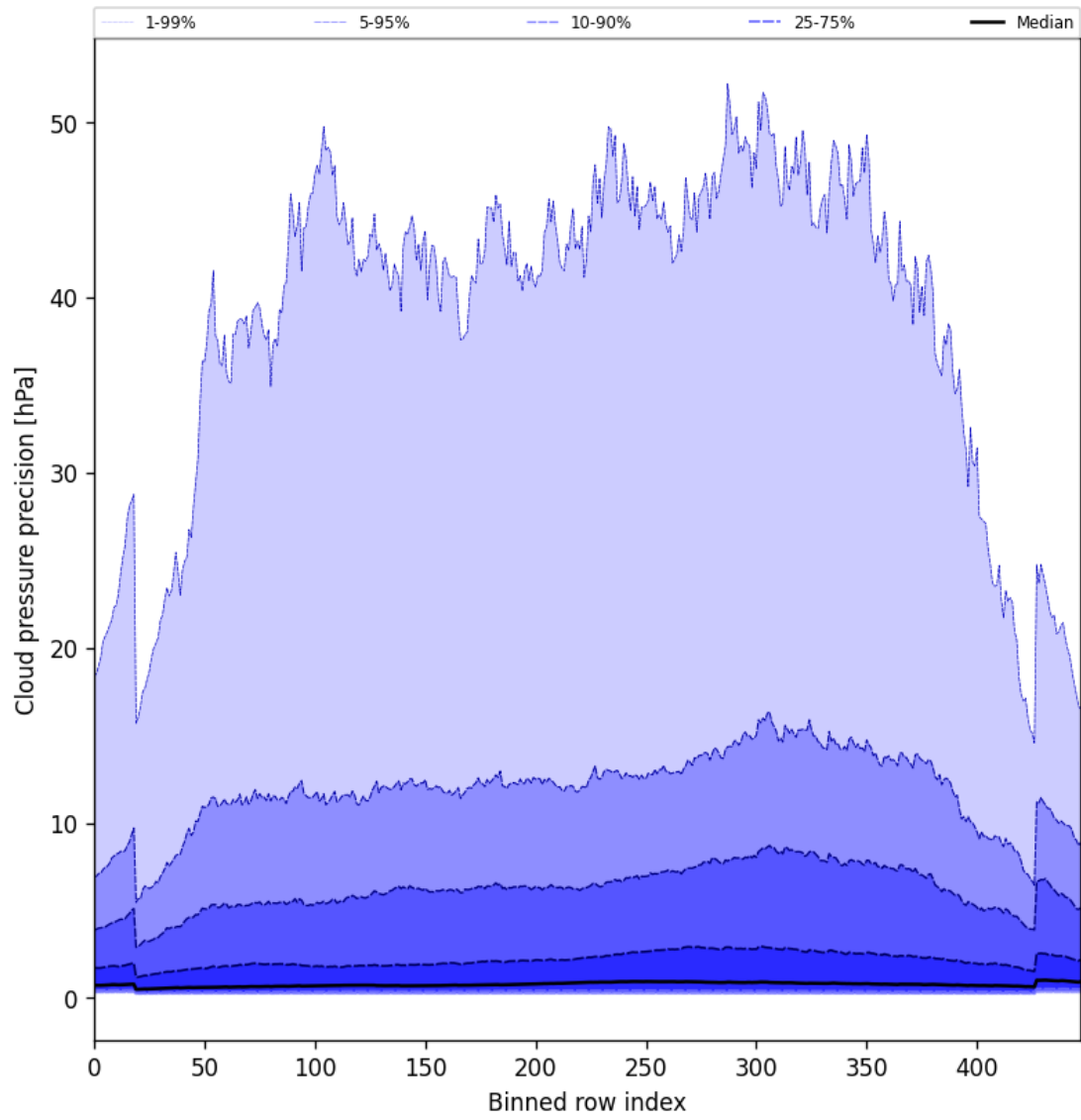
Figure 48: Along track statistics of “Cloud pressure precision” for 2025-07-24 to 2025-07-25
