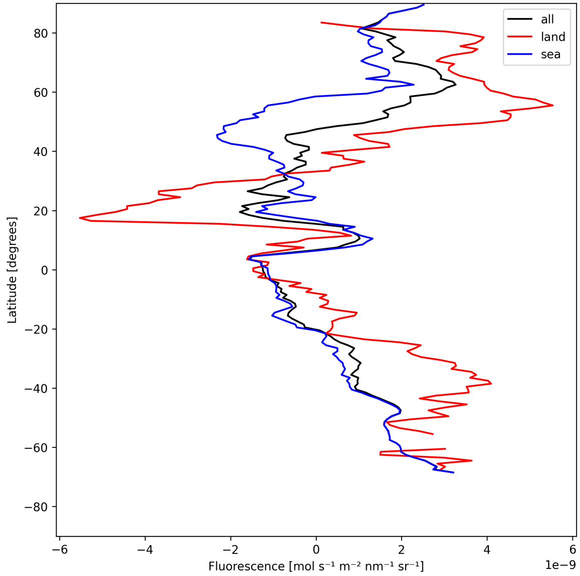
Figure 23: Zonal average of “Fluorescence” for 2025-07-24 to 2025-07-25.
