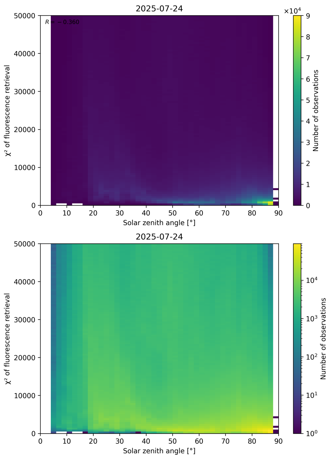
Figure 109: Scatter density plot of “Solar zenith angle” against “ \chi^2 of fluorescence retrieval” for 2025-07-24 to 2025-07-25.
