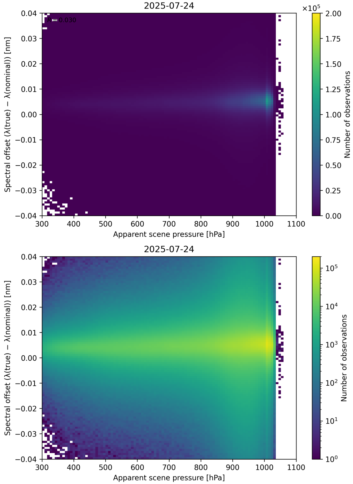
Figure 67: Scatter density plot of “Apparent scene pressure” against “Spectral offset ( \lambda_{\text{true}} - \lambda_{\text{nominal}} )” for 2025-07-24 to 2025-07-25.
