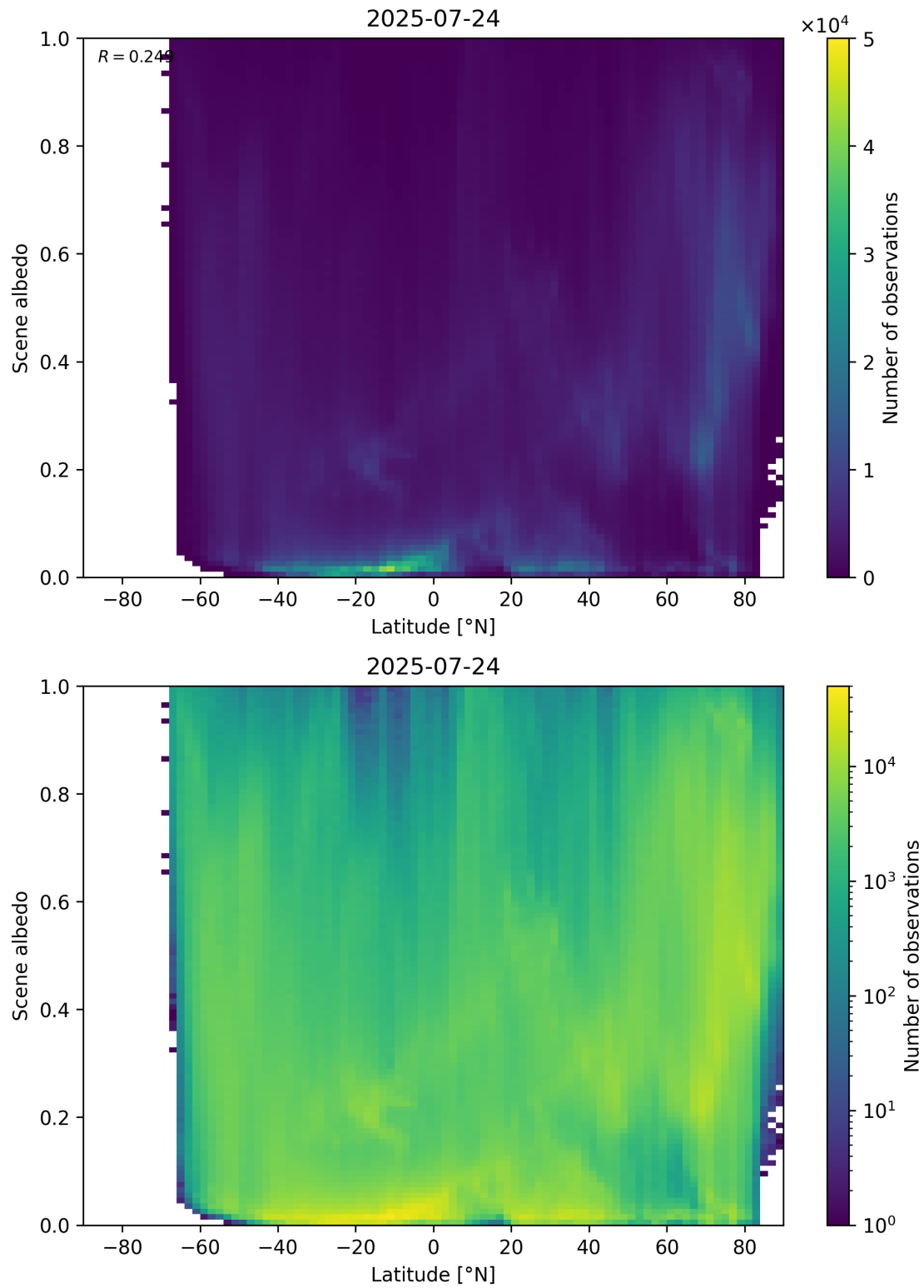
Figure 95: Scatter density plot of “Latitude” against “Scene albedo” for 2025-07-24 to 2025-07-25.
