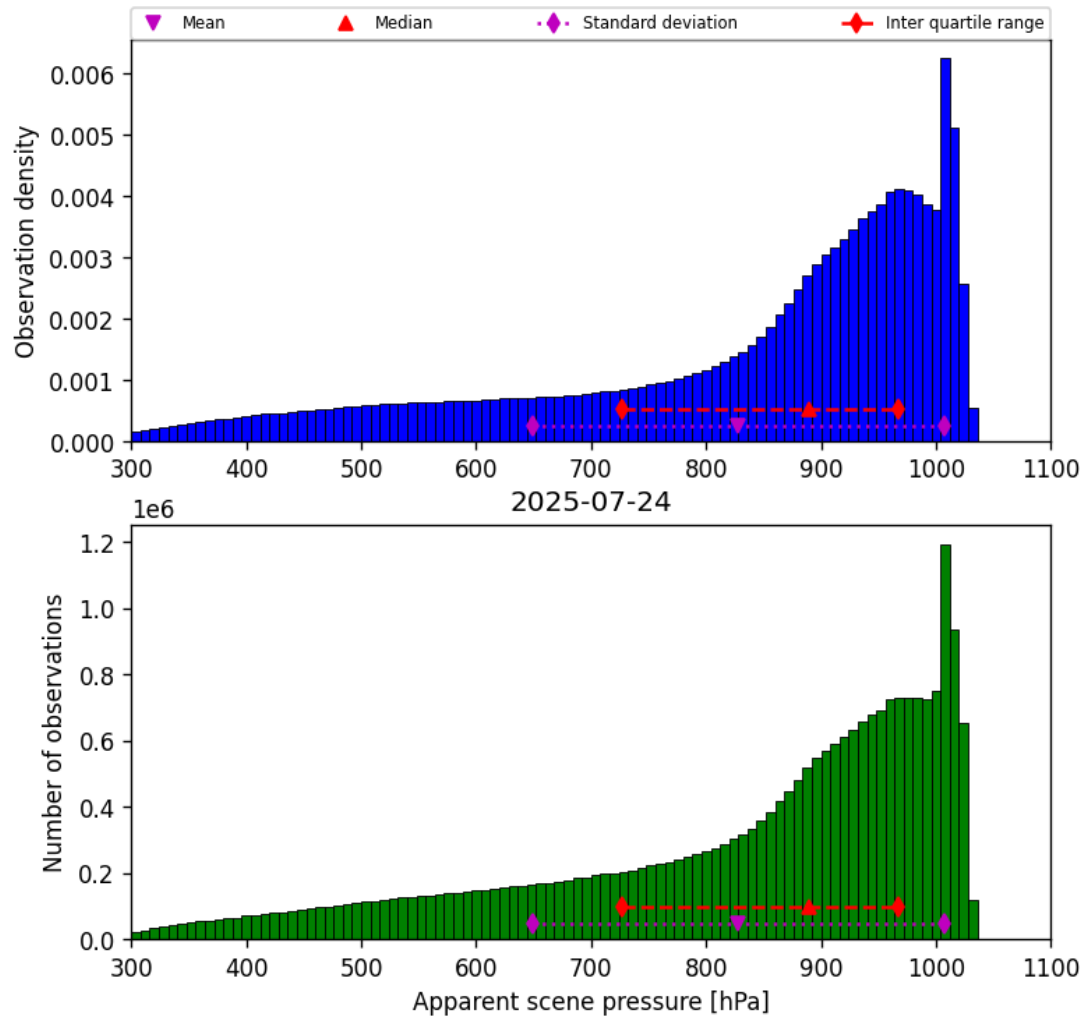
Figure 36: Histogram of “Apparent scene pressure” for 2025-07-24 to 2025-07-25
