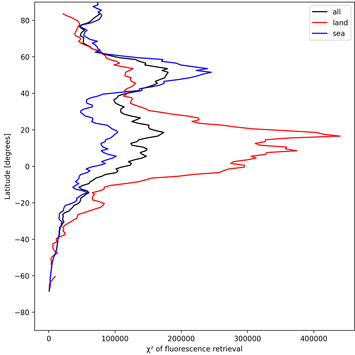
Figure 25: Zonal average of “ \chi^2 of fluorescence retrieval” for 2025-07-24 to 2025-07-25.
