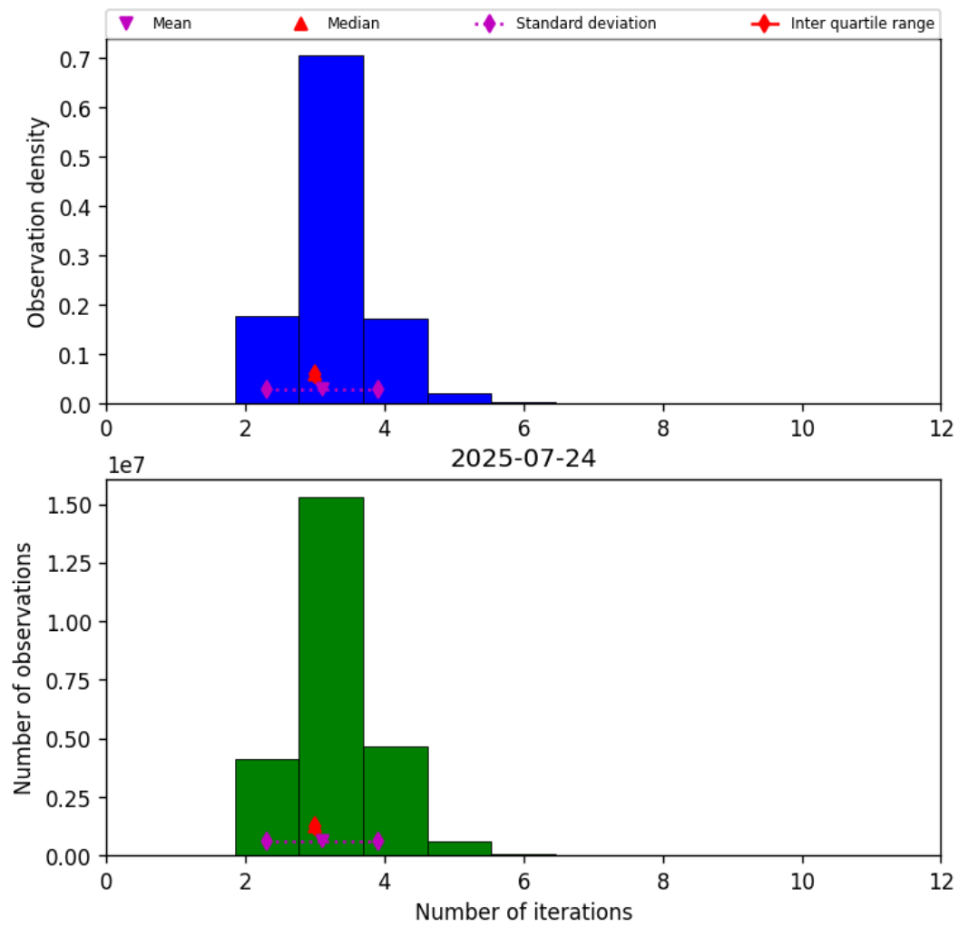
Figure 39: Histogram of “Number of iterations” for 2025-07-24 to 2025-07-25
