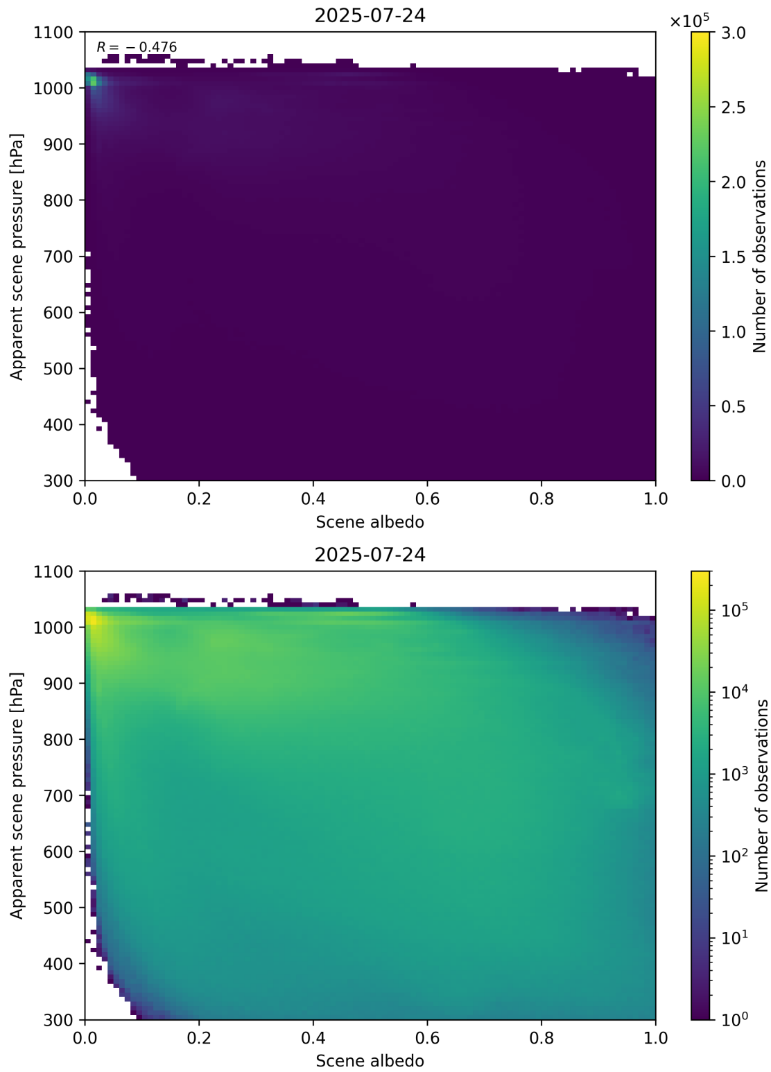
Figure 102: Scatter density plot of “Scene albedo” against “Apparent scene pressure” for 2025-07-24 to 2025-07-25.
