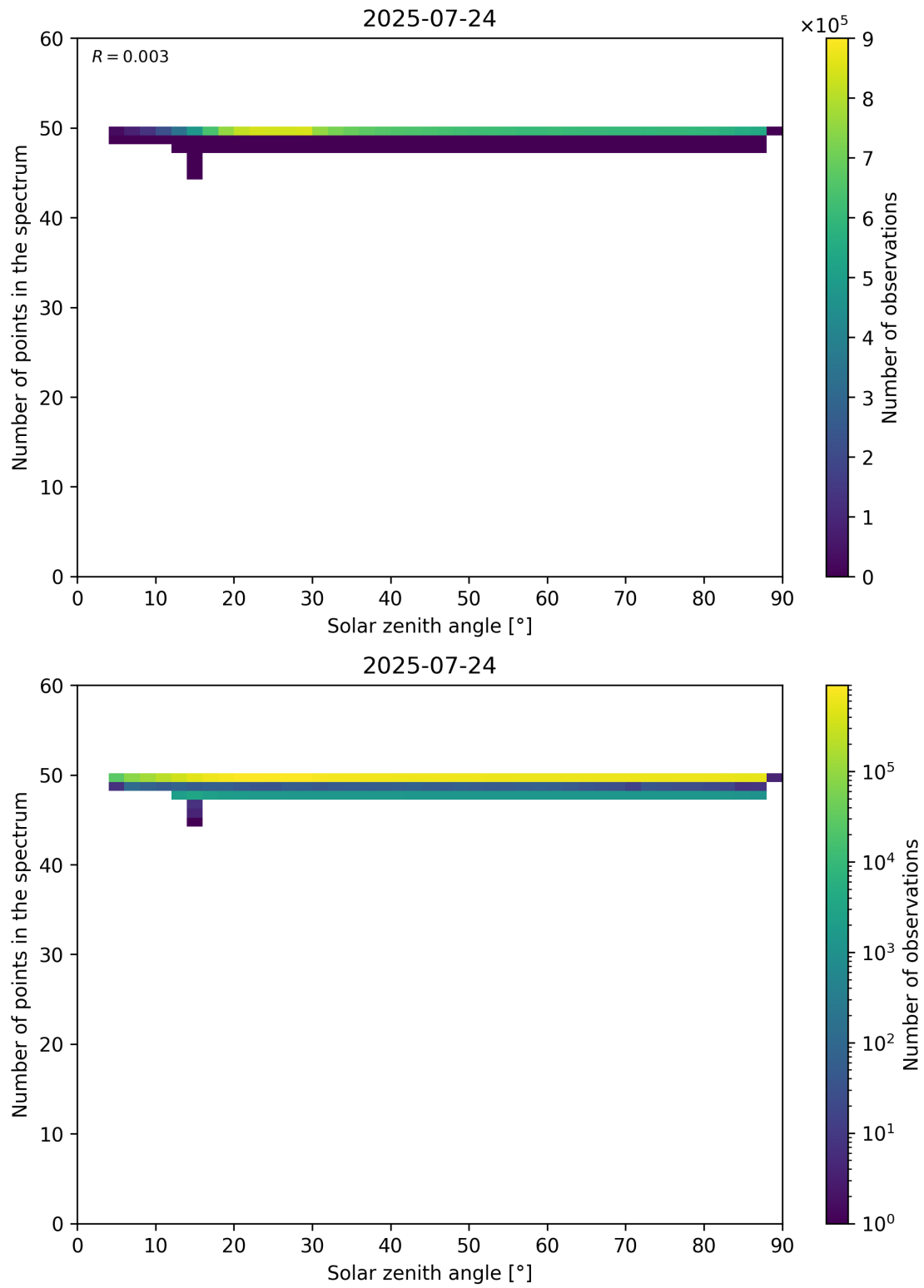
Figure 115: Scatter density plot of “Solar zenith angle” against “Number of points in the spectrum” for 2025-07-24 to 2025-07-25.
