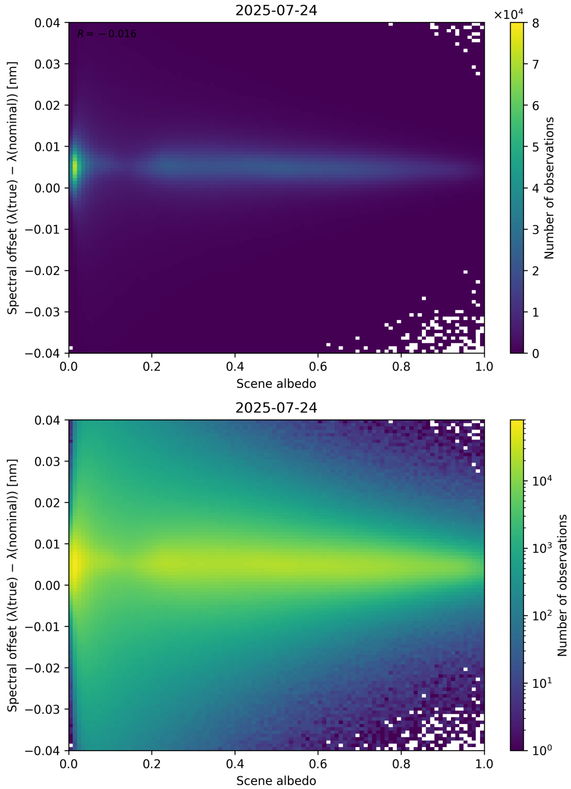
Figure 107: Scatter density plot of “Scene albedo” against “Spectral offset ( \lambda_{\text{true}} - \lambda_{\text{nominal}} )” for 2025-07-24 to 2025-07-25.
