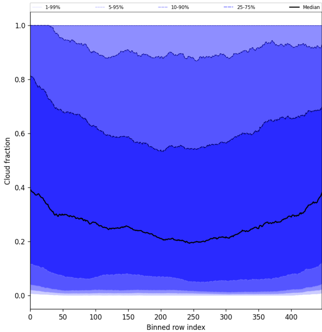
Figure 49: Along track statistics of “Cloud fraction” for 2025-07-24 to 2025-07-25
