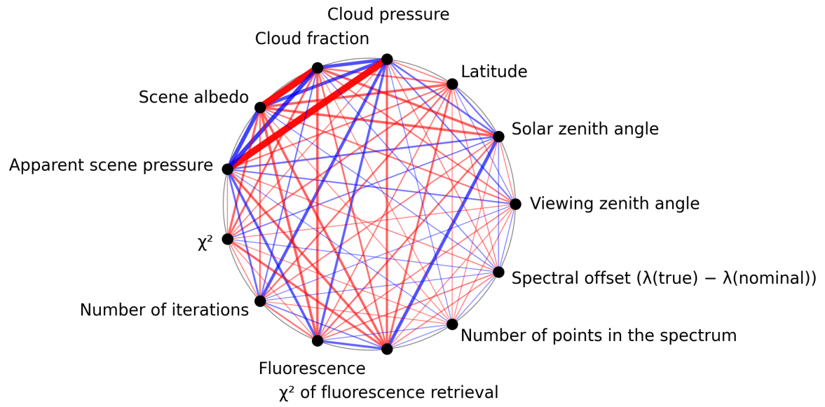
Figure 1: Map of correlation graph for 2025-07-24 to 2025-07-25.
