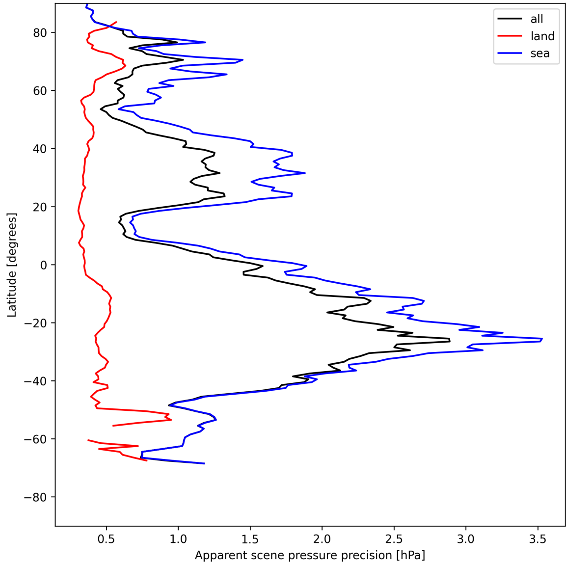
Figure 20: Zonal average of “Apparent scene pressure precision” for 2025-07-24 to 2025-07-25.
