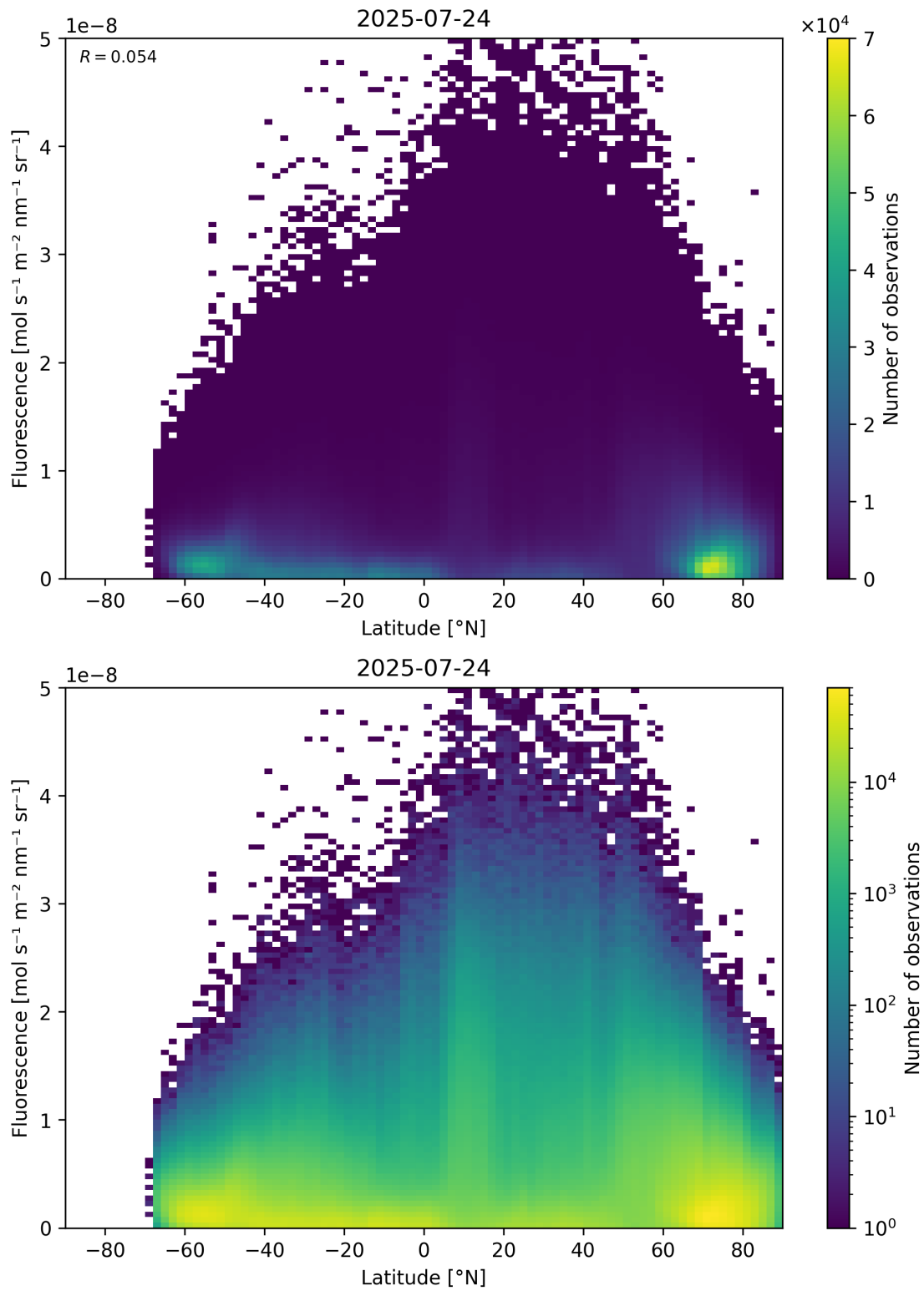
Figure 92: Scatter density plot of “Latitude” against “Fluorescence” for 2025-07-24 to 2025-07-25.
