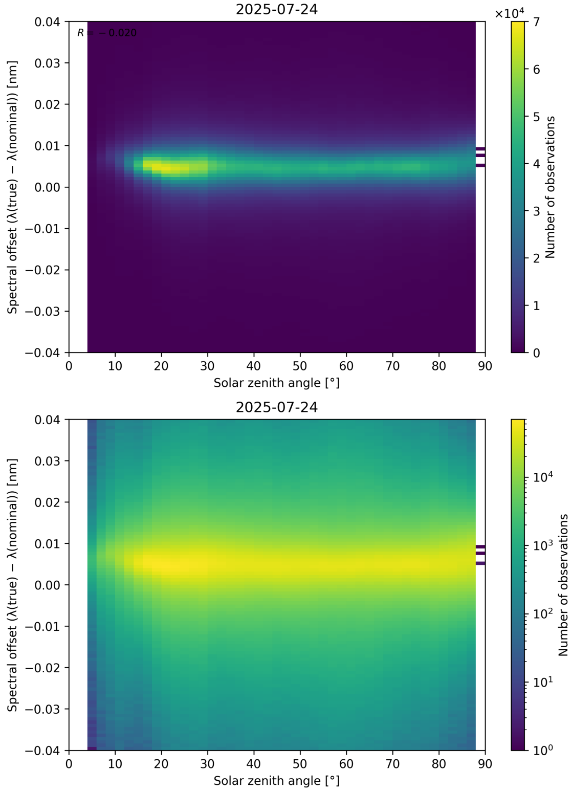
Figure 117: Scatter density plot of “Solar zenith angle” against “Spectral offset ( \lambda_{\text{true}} - \lambda_{\text{nominal}} )” for 2025-07-24 to 2025-07-25.
