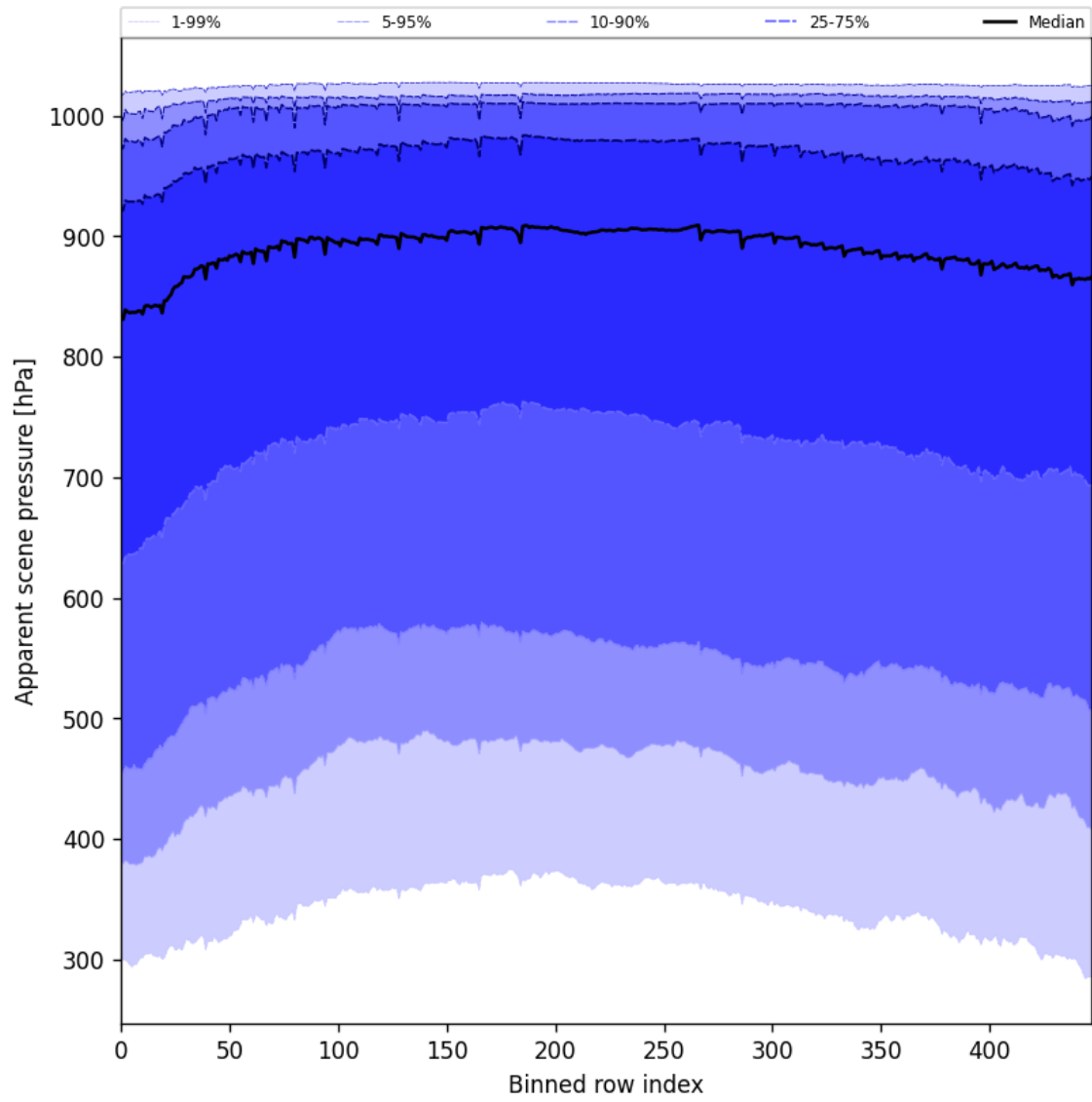
Figure 53: Along track statistics of “Apparent scene pressure” for 2025-07-24 to 2025-07-25
