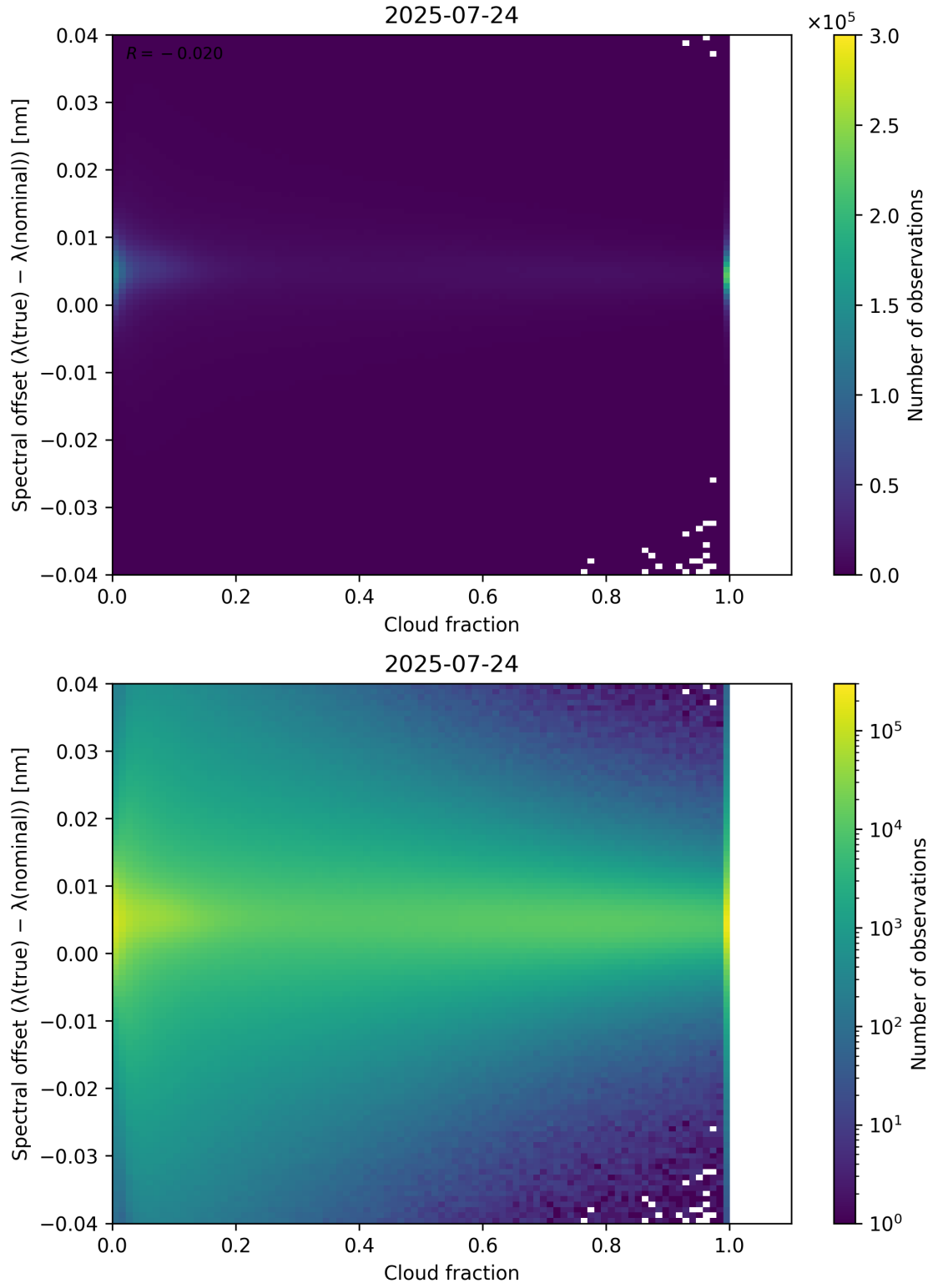
Figure 76: Scatter density plot of “Cloud fraction” against “Spectral offset ( \lambda_{\text{true}} - \lambda_{\text{nominal}} )” for 2025-07-24 to 2025-07-25.
