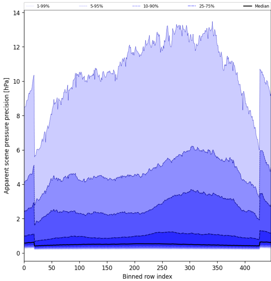
Figure 54: Along track statistics of “Apparent scene pressure precision” for 2025-07-24 to 2025-07-25
