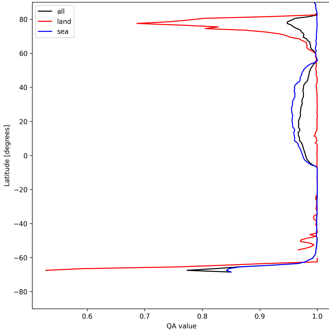
Figure 12: Zonal average of "QA value" for 2025-07-24 to 2025-07-25.
