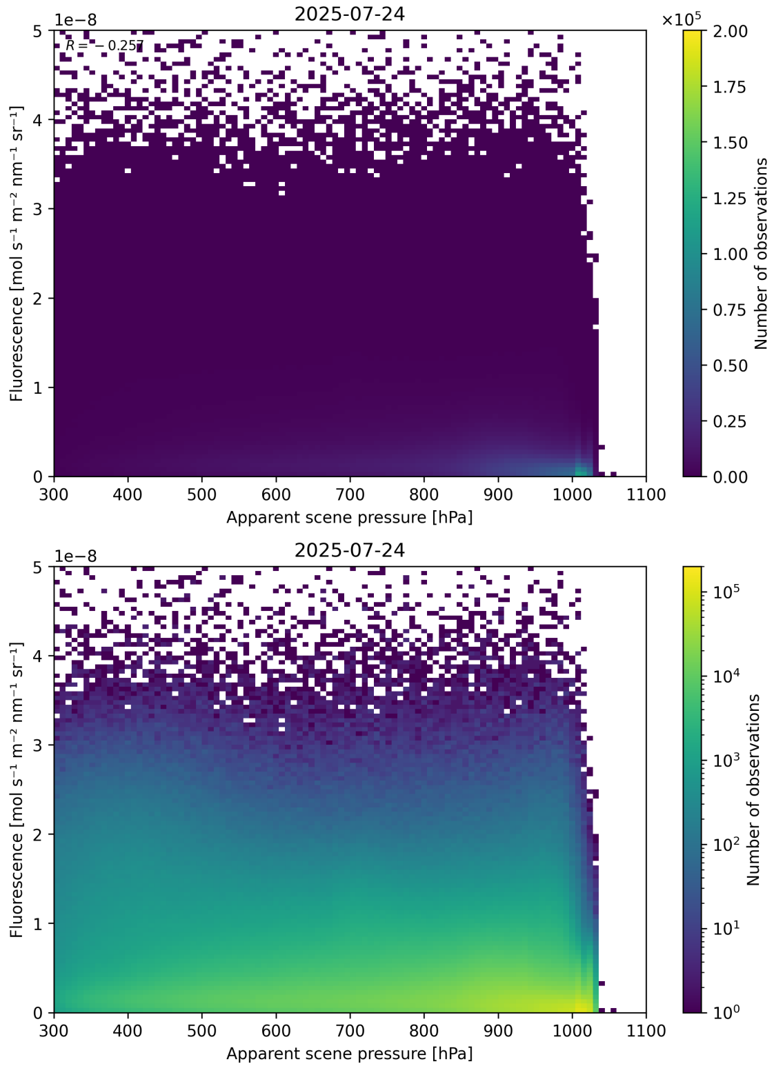
Figure 64: Scatter density plot of “Apparent scene pressure” against “Fluorescence” for 2025-07-24 to 2025-07-25.
