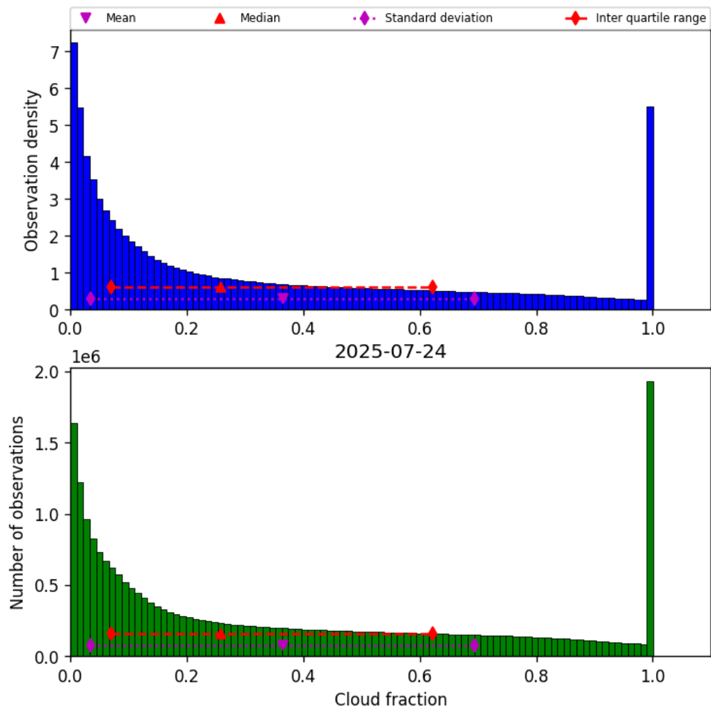
Figure 32: Histogram of “Cloud fraction” for 2025-07-24 to 2025-07-25
