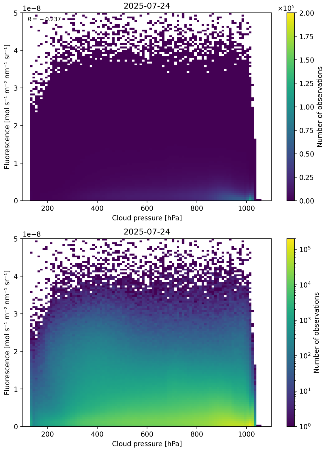
Figure 80: Scatter density plot of “Cloud pressure” against “Fluorescence” for 2025-07-24 to 2025-07-25.
