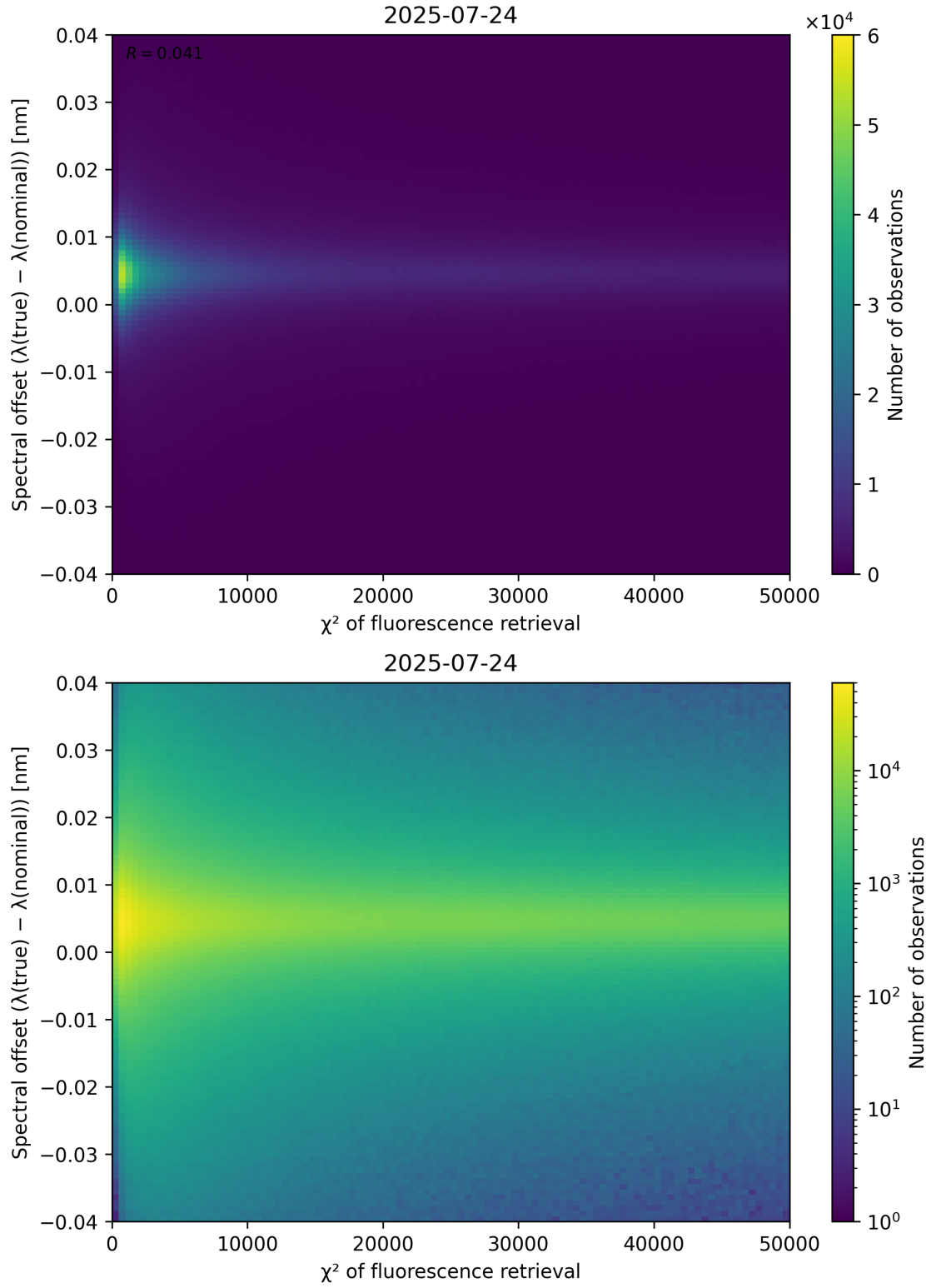
Figure 69: Scatter density plot of “ \chi^2 of fluorescence retrieval” against “Spectral offset ( \lambda_{\text{true}} - \lambda_{\text{nominal}} )” for 2025-07-24 to 2025-07-25.
