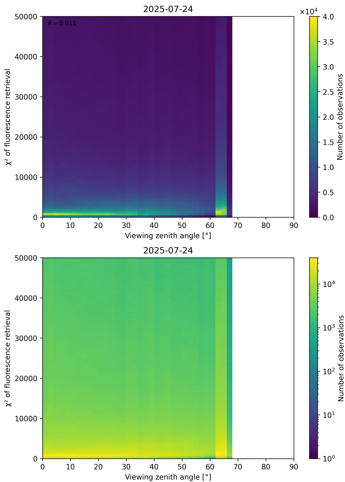
Figure 119: Scatter density plot of “Viewing zenith angle” against “ \chi^2 of fluorescence retrieval” for 2025-07-24 to 2025-07-25.
