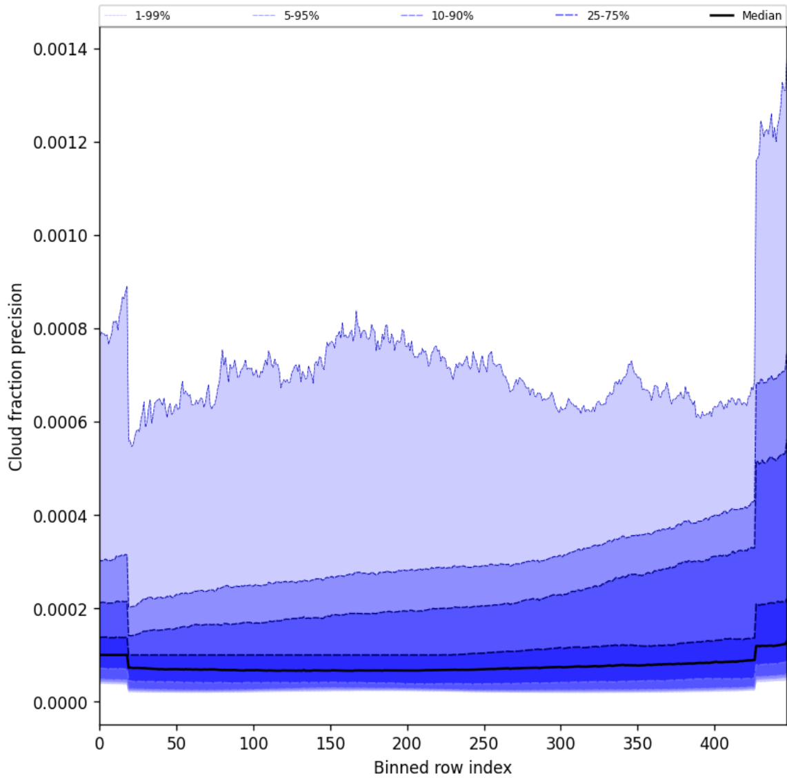
Figure 50: Along track statistics of “Cloud fraction precision” for 2025-07-24 to 2025-07-25
