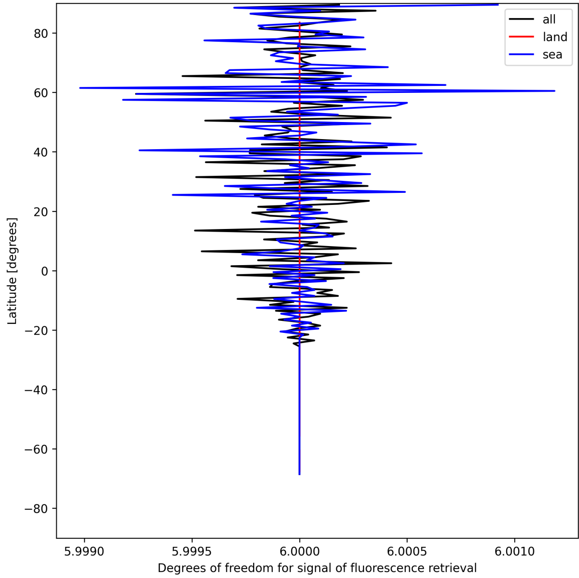
Figure 26: Zonal average of “Degrees of freedom for signal of fluorescence retrieval” for 2025-07-24 to 2025-07-25.
