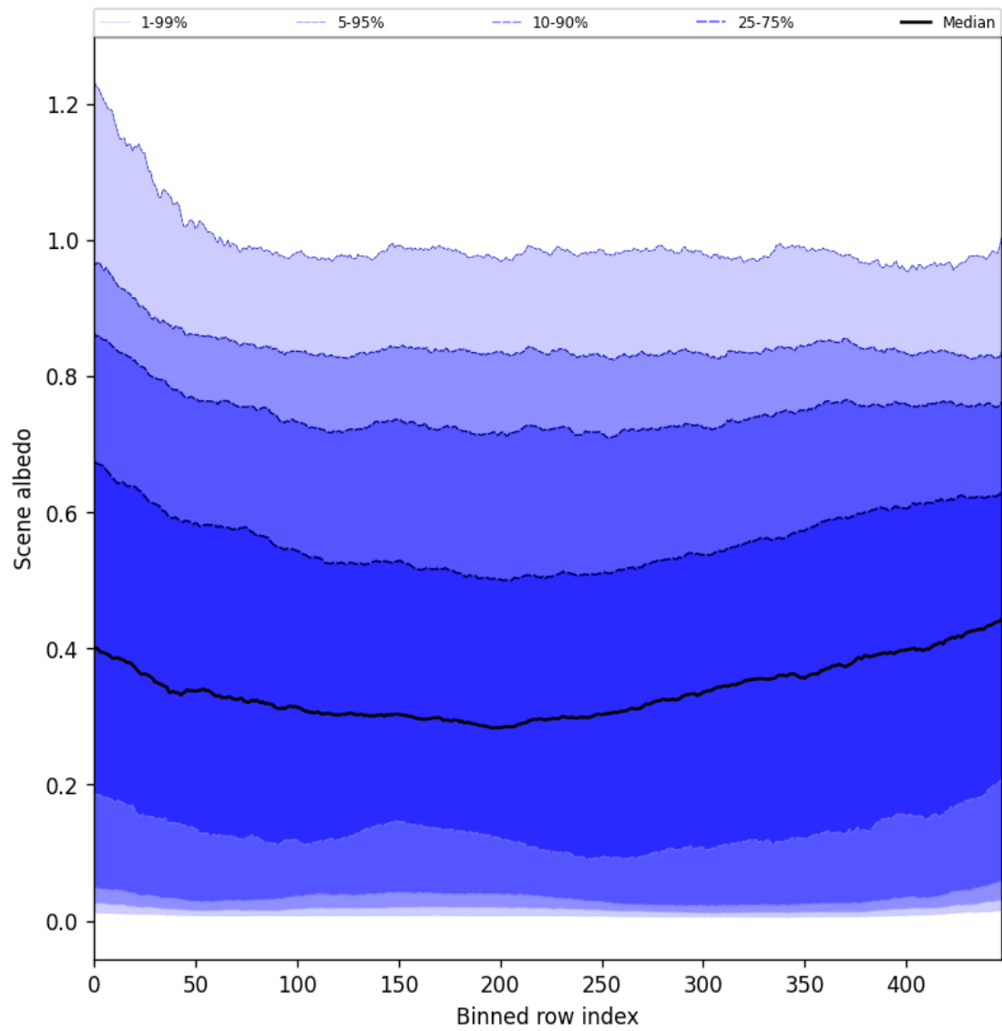
Figure 51: Along track statistics of “Scene albedo” for 2025-07-24 to 2025-07-25
