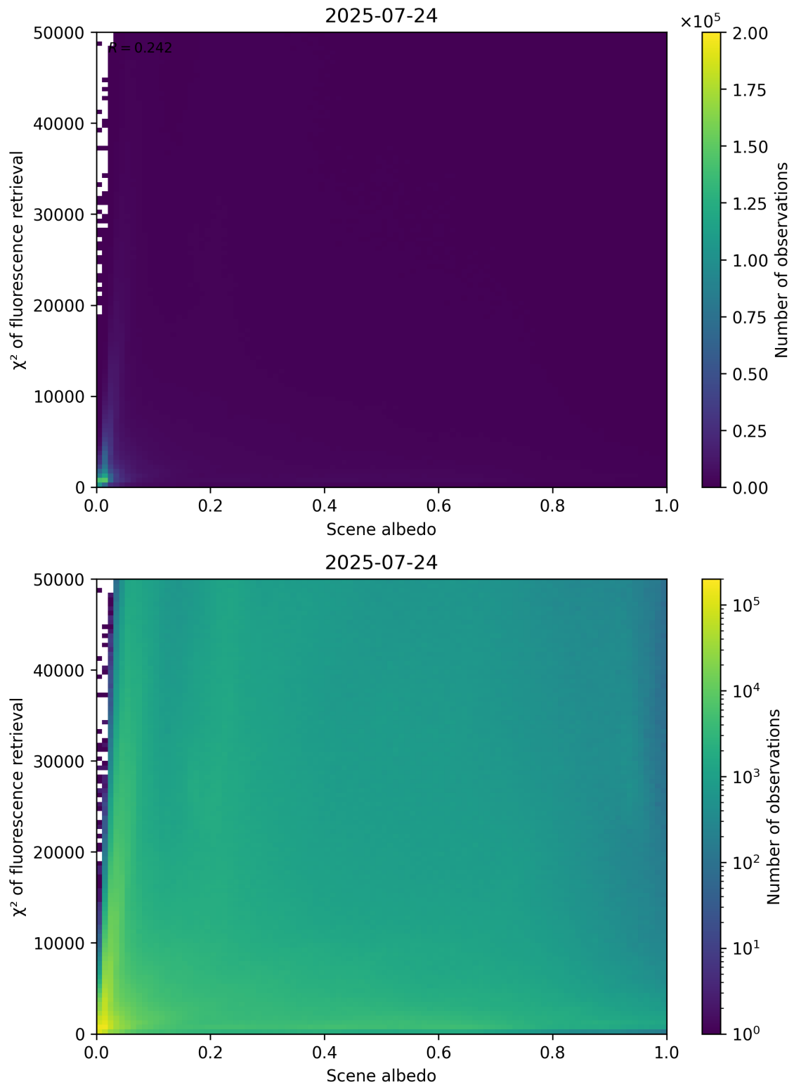
Figure 103: Scatter density plot of “Scene albedo” against “ \chi^2 of fluorescence retrieval” for 2025-07-24 to 2025-07-25.
