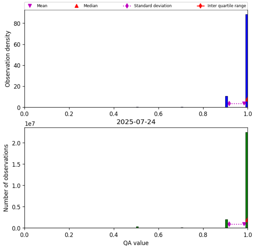
Figure 29: Histogram of “QA value” for 2025-07-24 to 2025-07-25
