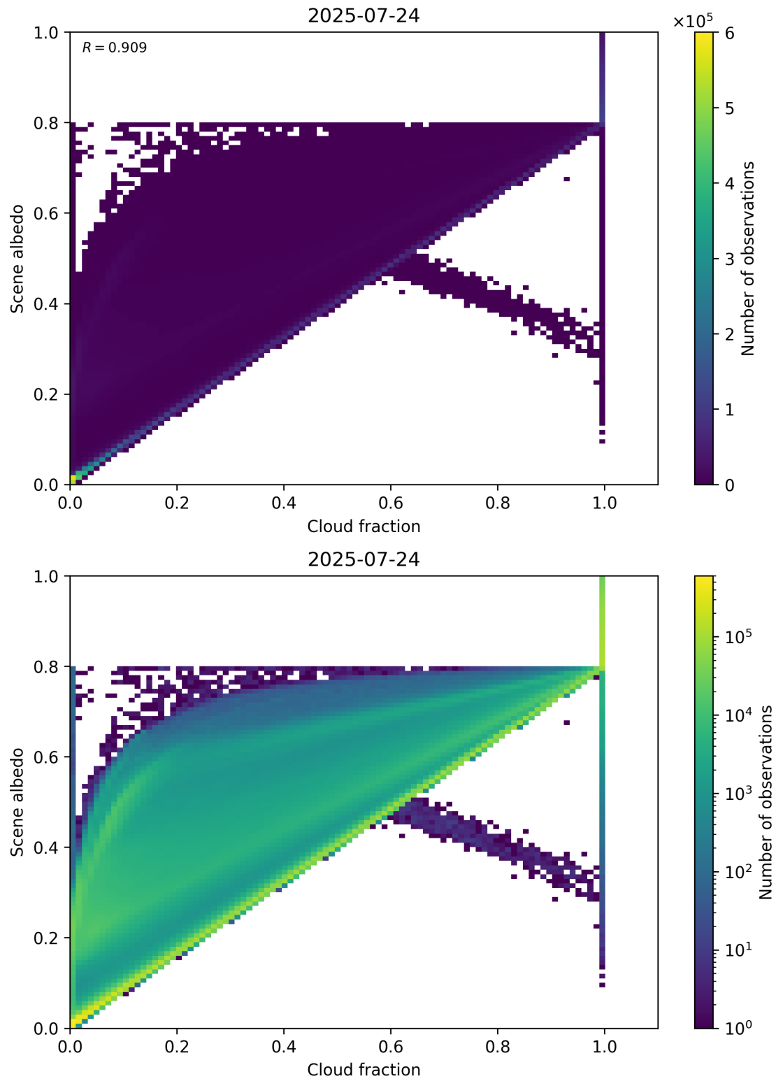
Figure 75: Scatter density plot of “Cloud fraction” against “Scene albedo” for 2025-07-24 to 2025-07-25.
