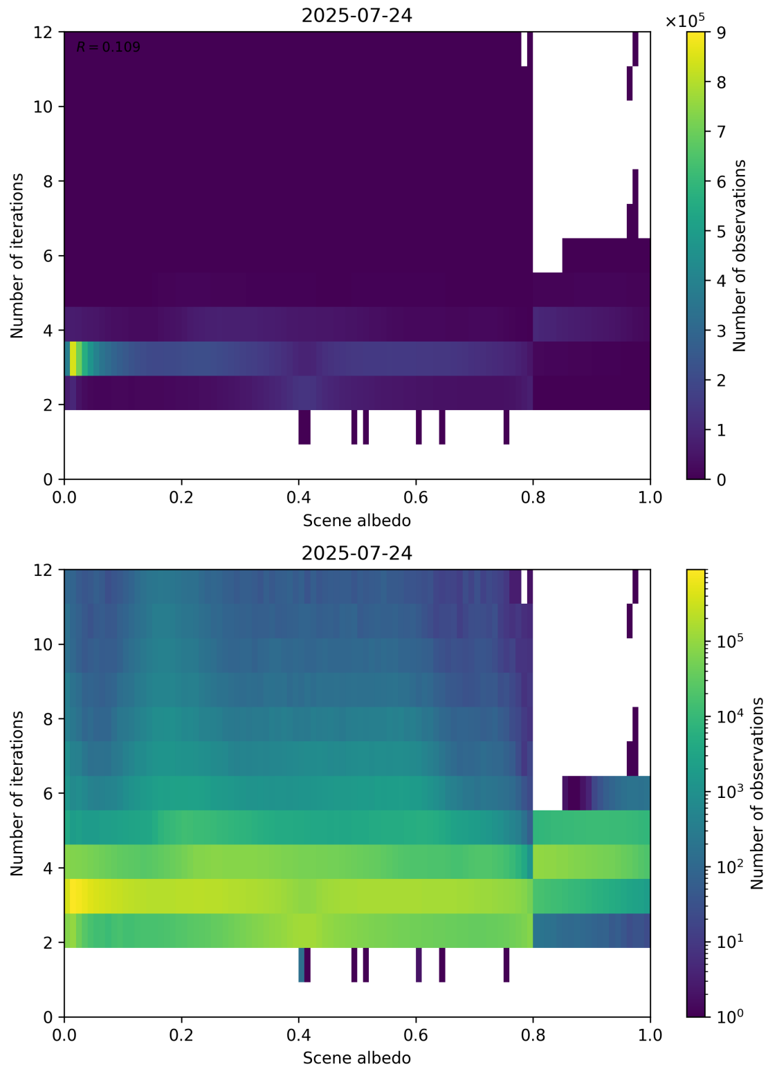
Figure 105: Scatter density plot of “Scene albedo” against “Number of iterations” for 2025-07-24 to 2025-07-25.
