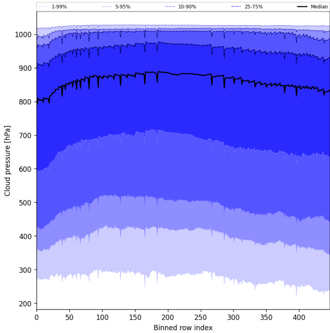
Figure 47: Along track statistics of “Cloud pressure” for 2025-07-24 to 2025-07-25
