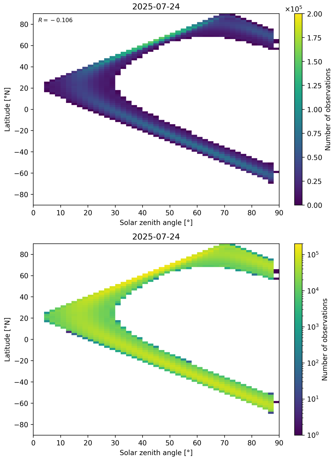
Figure 113: Scatter density plot of “Solar zenith angle” against “Latitude” for 2025-07-24 to 2025-07-25.
