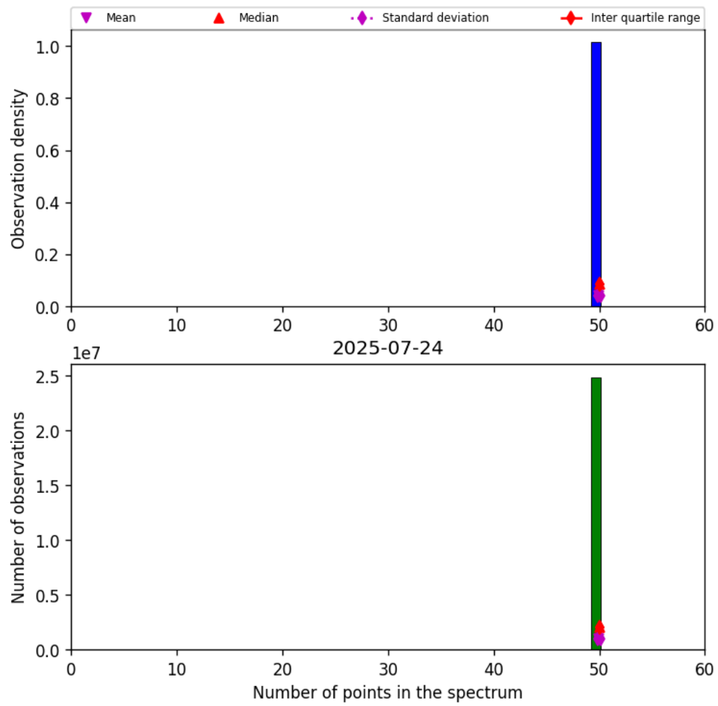
Figure 44: Histogram of “Number of points in the spectrum” for 2025-07-24 to 2025-07-25
