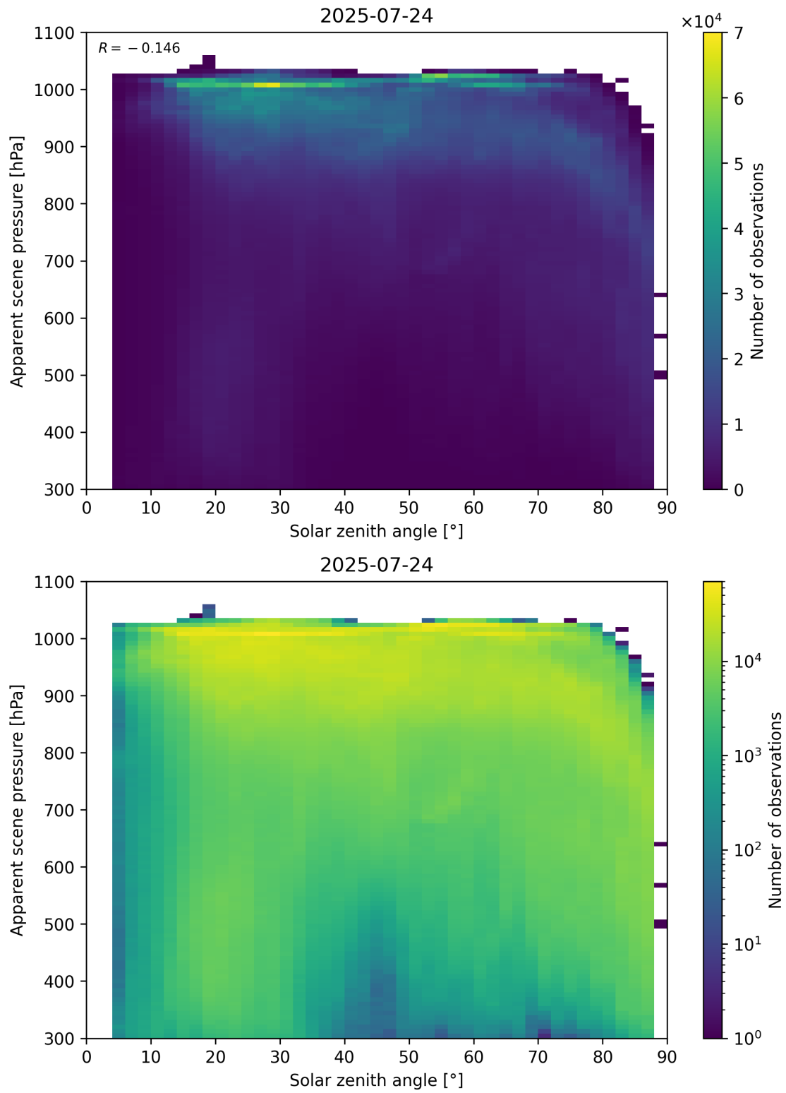
Figure 108: Scatter density plot of “Solar zenith angle” against “Apparent scene pressure” for 2025-07-24 to 2025-07-25.
