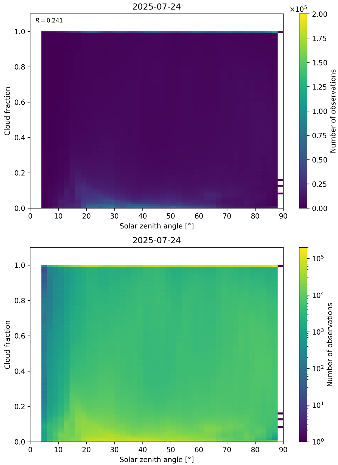
Figure 110: Scatter density plot of “Solar zenith angle” against “Cloud fraction” for 2025-07-24 to 2025-07-25.
