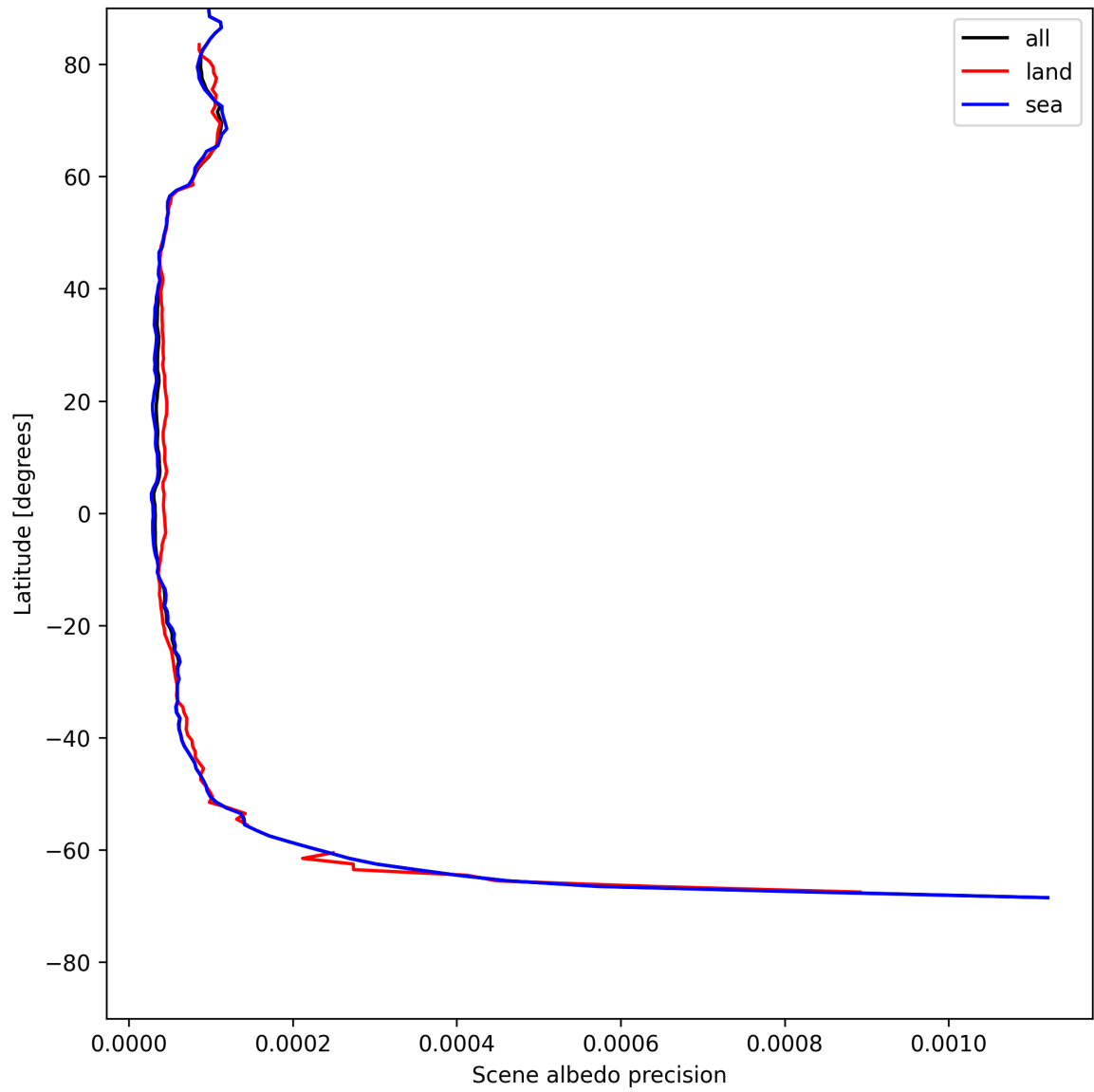
Figure 18: Zonal average of “Scene albedo precision” for 2025-07-24 to 2025-07-25.
