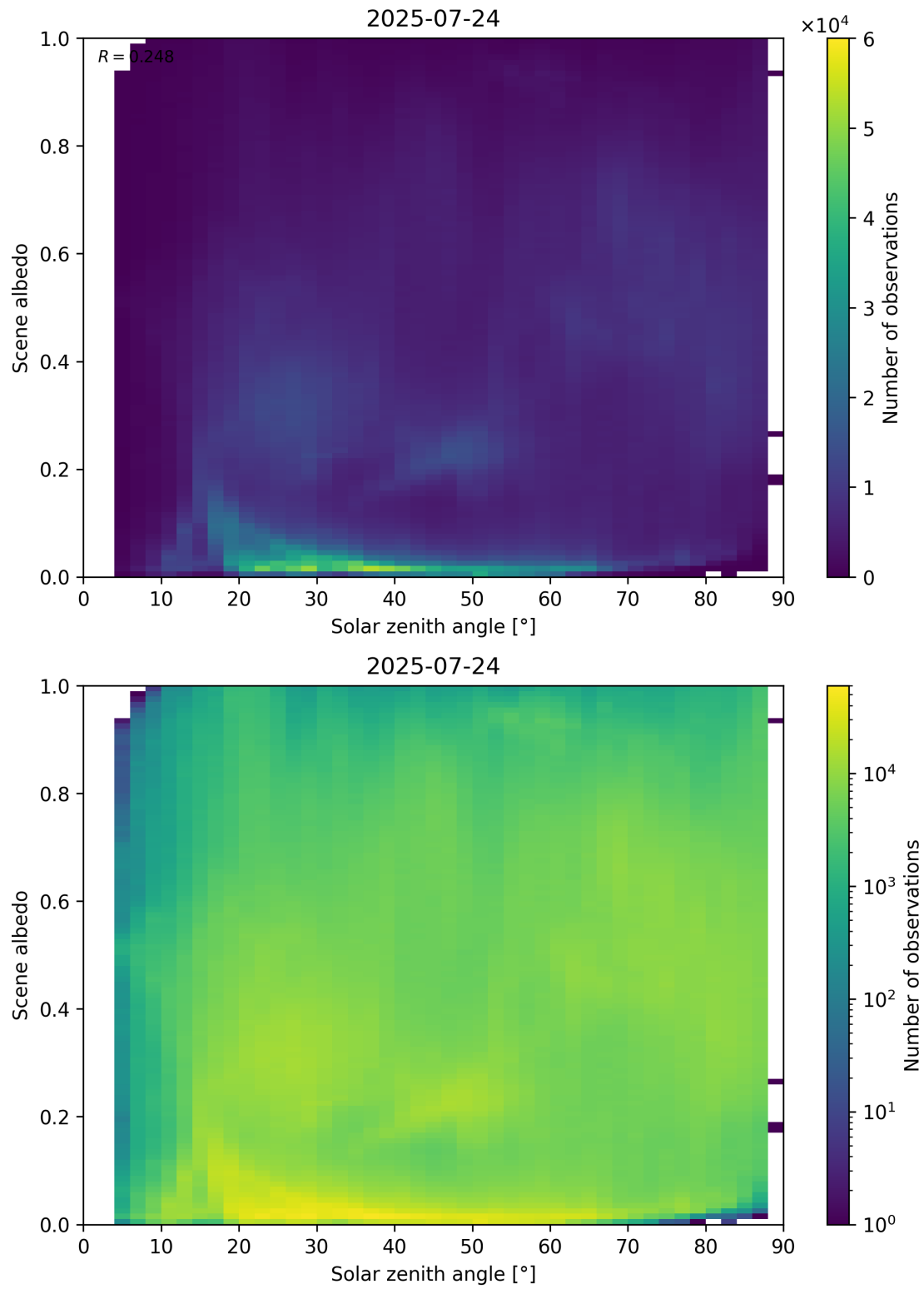
Figure 116: Scatter density plot of “Solar zenith angle” against “Scene albedo” for 2025-07-24 to 2025-07-25.
