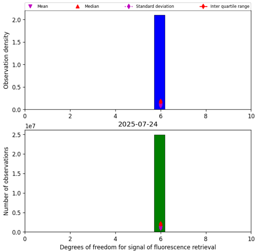
Figure 43: Histogram of “Degrees of freedom for signal of fluorescence retrieval” for 2025-07-24 to 2025-07-25
