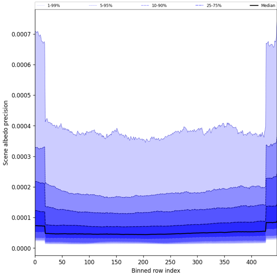
Figure 52: Along track statistics of “Scene albedo precision” for 2025-07-24 to 2025-07-25
