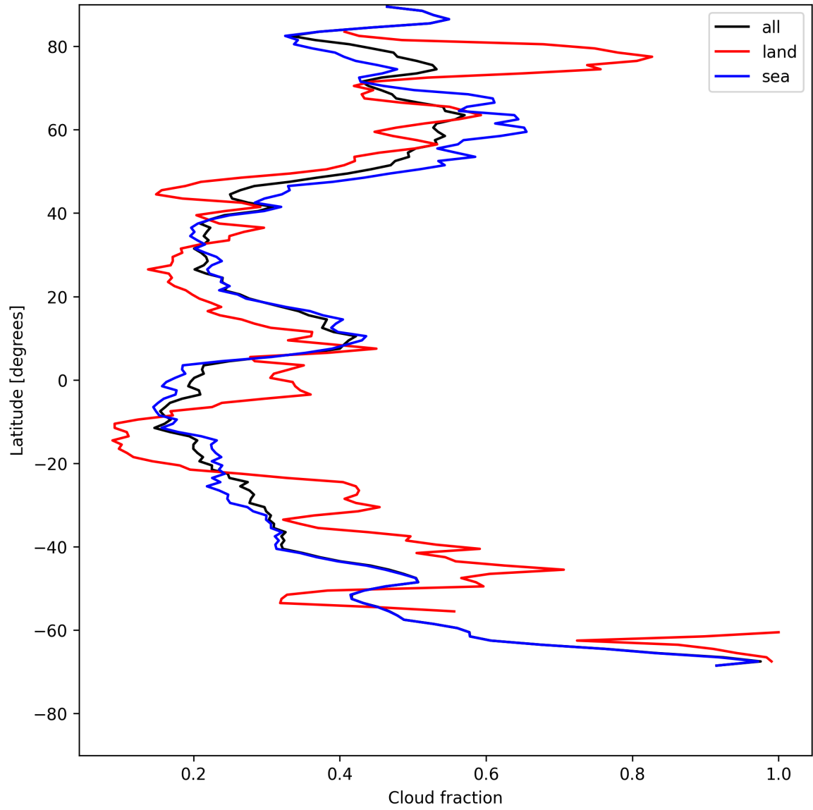
Figure 15: Zonal average of “Cloud fraction” for 2025-07-24 to 2025-07-25.
