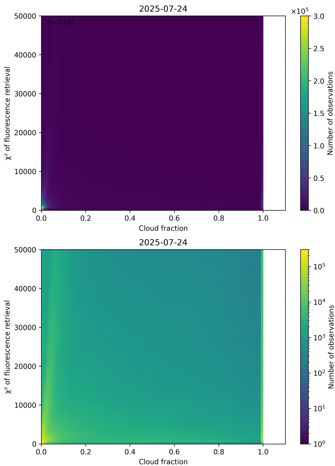
Figure 71: Scatter density plot of “Cloud fraction” against “ \chi^2 of fluorescence retrieval” for 2025-07-24 to 2025-07-25.
