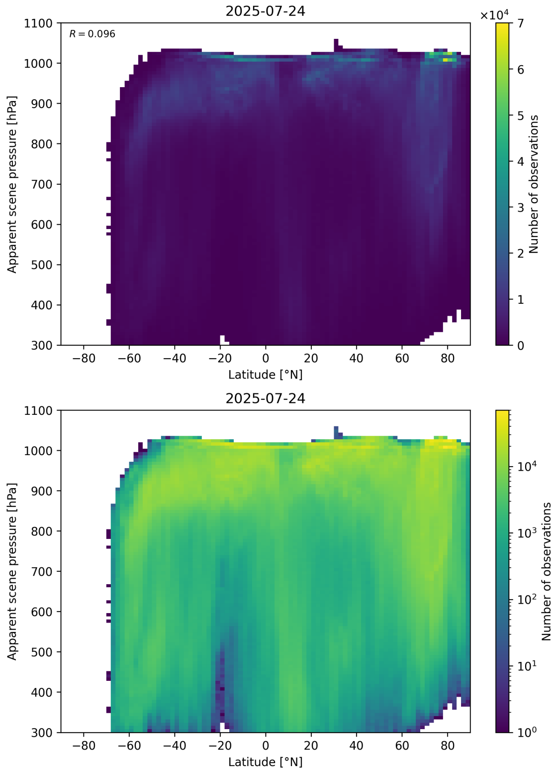
Figure 88: Scatter density plot of “Latitude” against “Apparent scene pressure” for 2025-07-24 to 2025-07-25.
