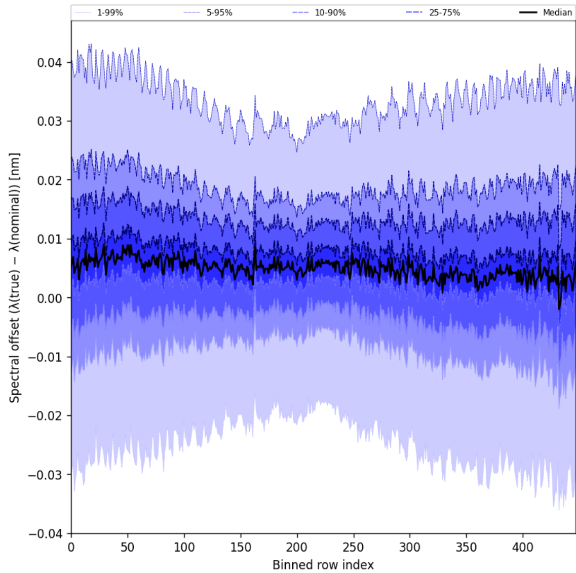
Figure 62: Along track statistics of “Spectral offset ( \lambda_{\text{true}} - \lambda_{\text{nominal}} )” for 2025-07-24 to 2025-07-25
