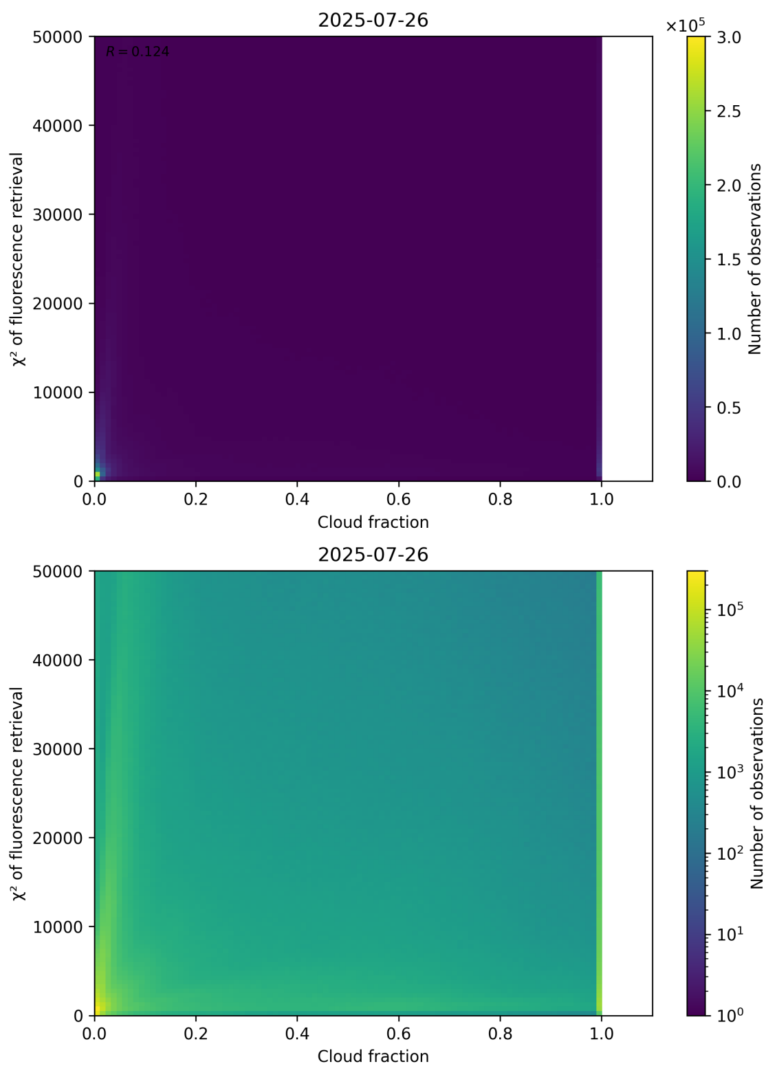
Figure 71: Scatter density plot of “Cloud fraction” against “ \chi^2 of fluorescence retrieval” for 2025-07-25 to 2025-07-27.
