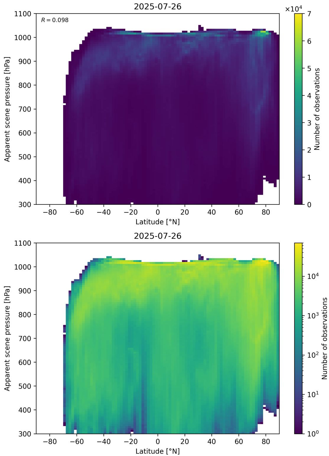
Figure 88: Scatter density plot of “Latitude” against “Apparent scene pressure” for 2025-07-25 to 2025-07-27.
