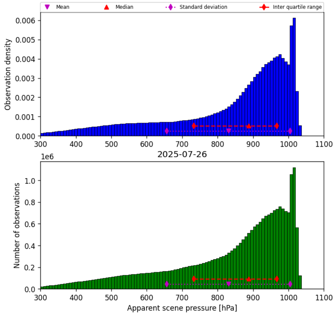
Figure 36: Histogram of “Apparent scene pressure” for 2025-07-25 to 2025-07-27
