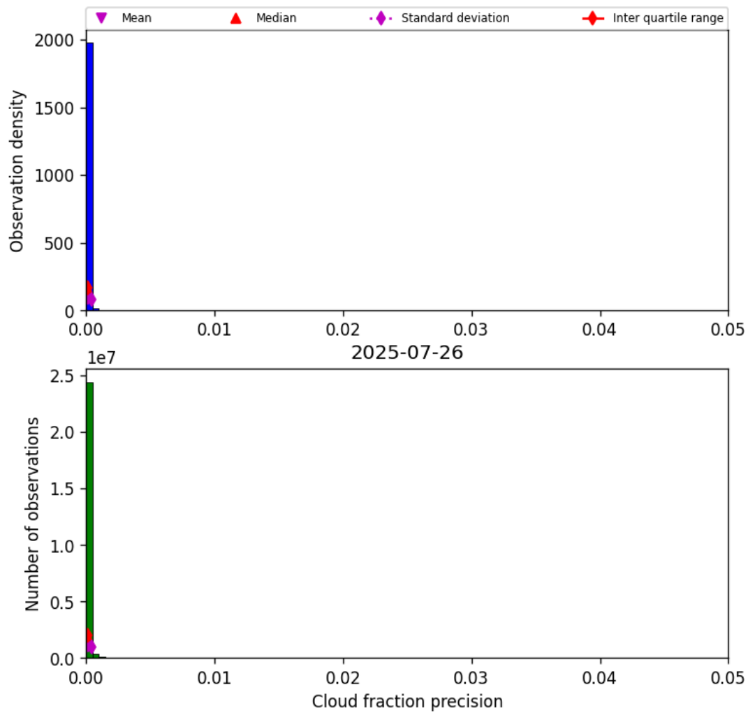
Figure 33: Histogram of “Cloud fraction precision” for 2025-07-25 to 2025-07-27
