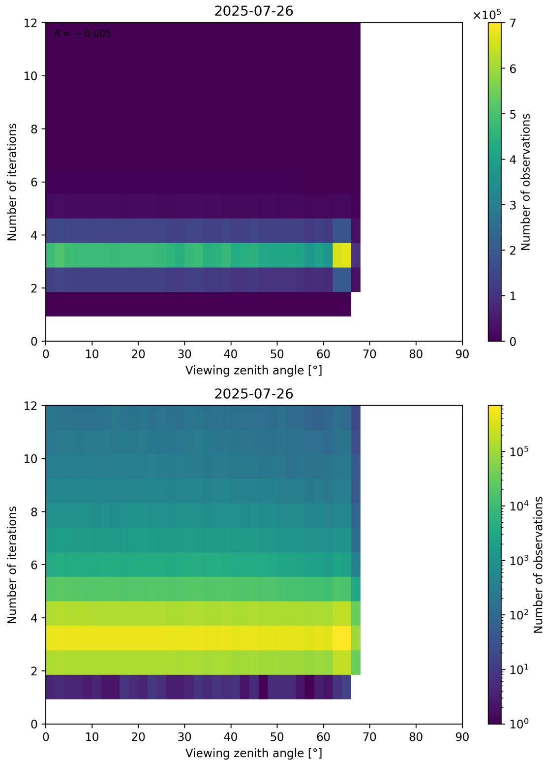
Figure 124: Scatter density plot of “Viewing zenith angle” against “Number of iterations” for 2025-07-25 to 2025-07-27.
