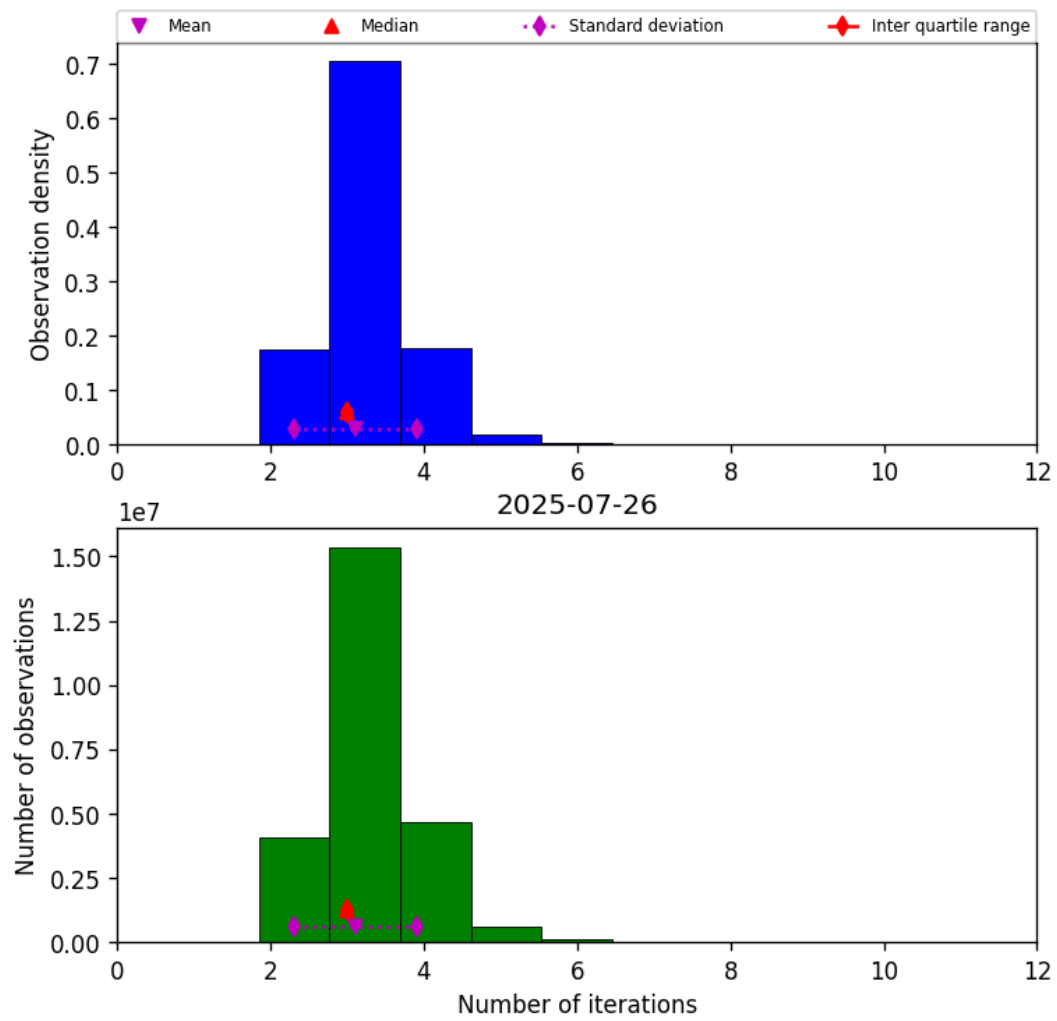
Figure 39: Histogram of “Number of iterations” for 2025-07-25 to 2025-07-27
