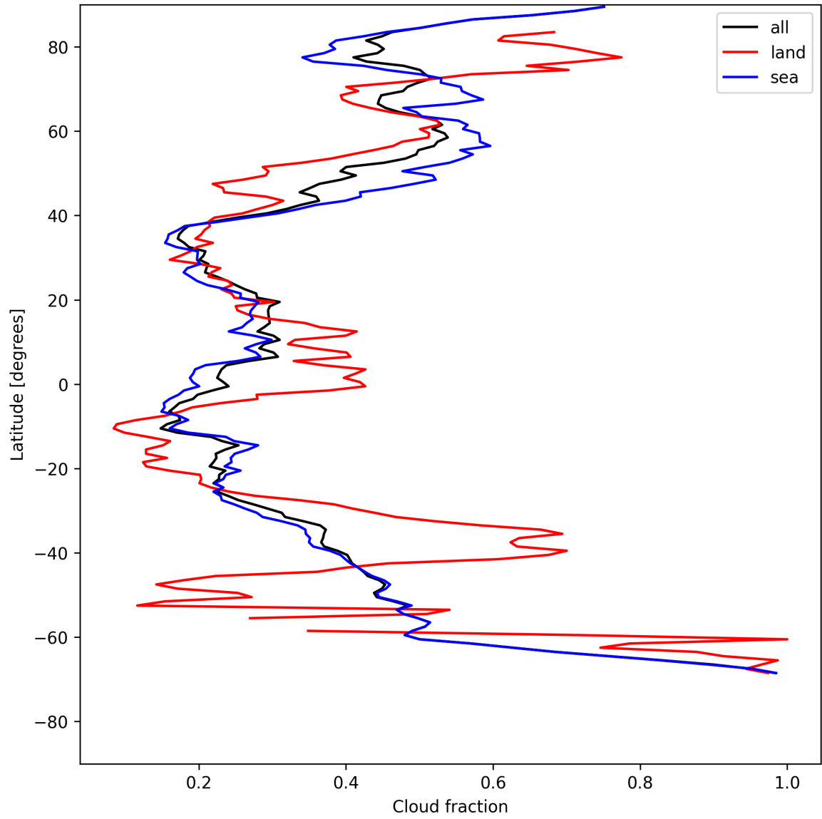
Figure 15: Zonal average of “Cloud fraction” for 2025-07-25 to 2025-07-27.
