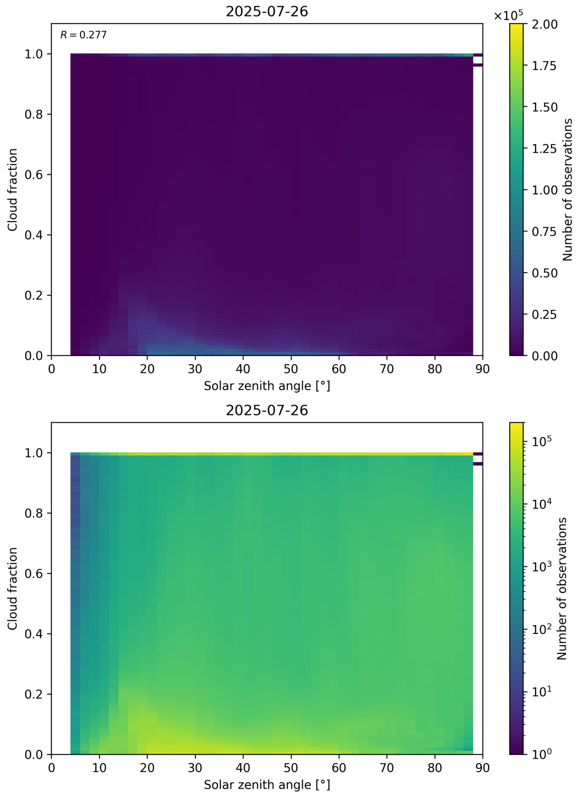
Figure 110: Scatter density plot of “Solar zenith angle” against “Cloud fraction” for 2025-07-25 to 2025-07-27.
