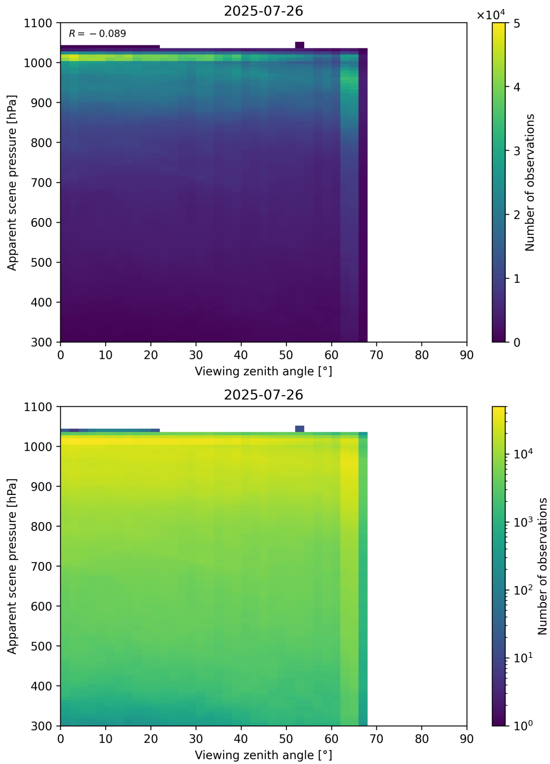
Figure 118: Scatter density plot of “Viewing zenith angle” against “Apparent scene pressure” for 2025-07-25 to 2025-07-27.
