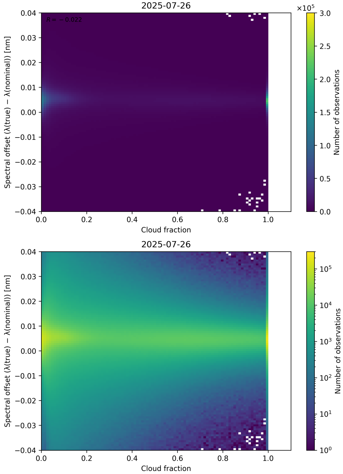
Figure 76: Scatter density plot of “Cloud fraction” against “Spectral offset ( \lambda_{\text{true}} - \lambda_{\text{nominal}} )” for 2025-07-25 to 2025-07-27.
