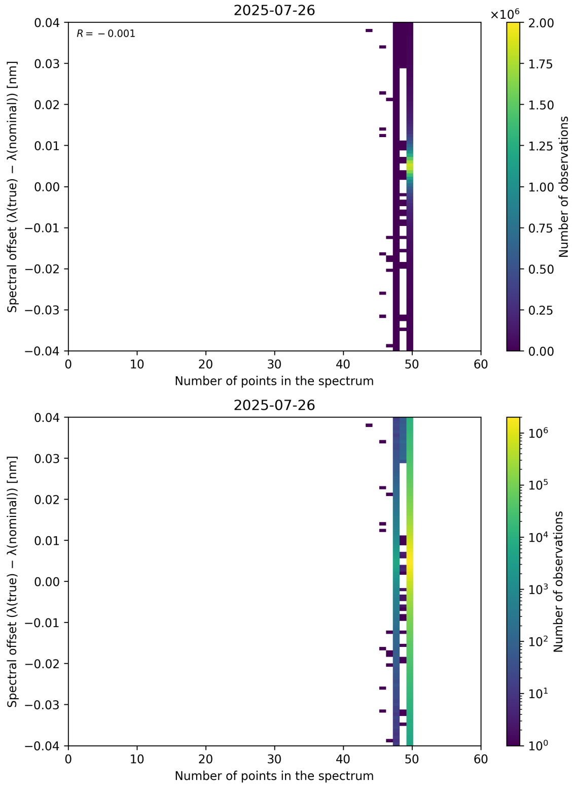
Figure 101: Scatter density plot of “Number of points in the spectrum” against “Spectral offset ( \lambda_{\text{true}} - \lambda_{\text{nominal}} )” for 2025-07-25 to 2025-07-27.
