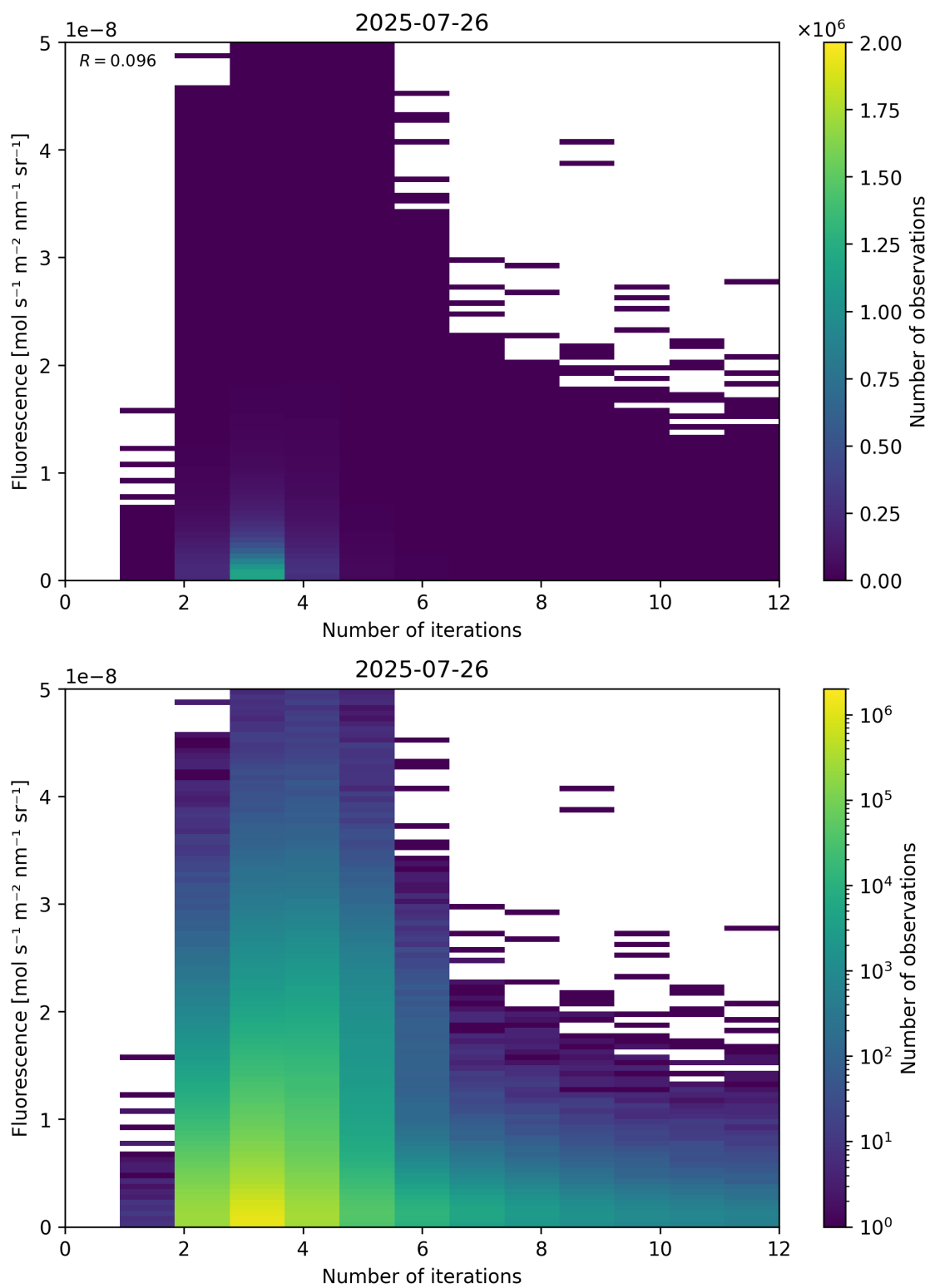
Figure 98: Scatter density plot of “Number of iterations” against “Fluorescence” for 2025-07-25 to 2025-07-27.
