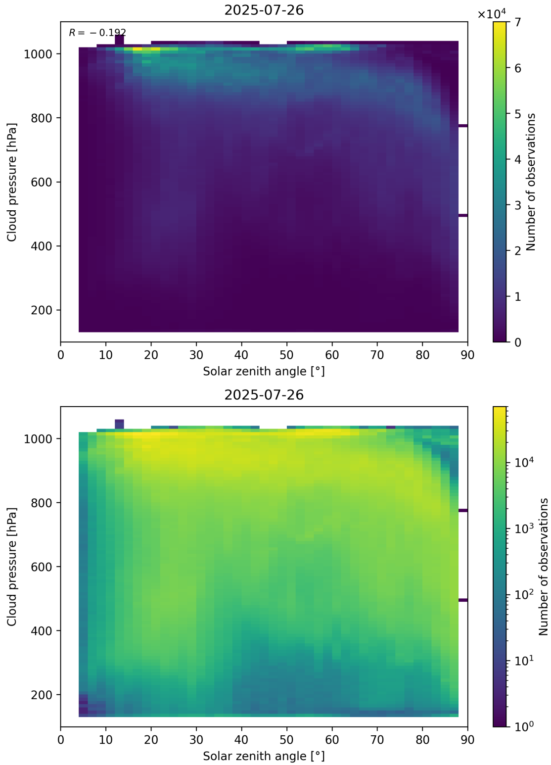
Figure 111: Scatter density plot of “Solar zenith angle” against “Cloud pressure” for 2025-07-25 to 2025-07-27.
