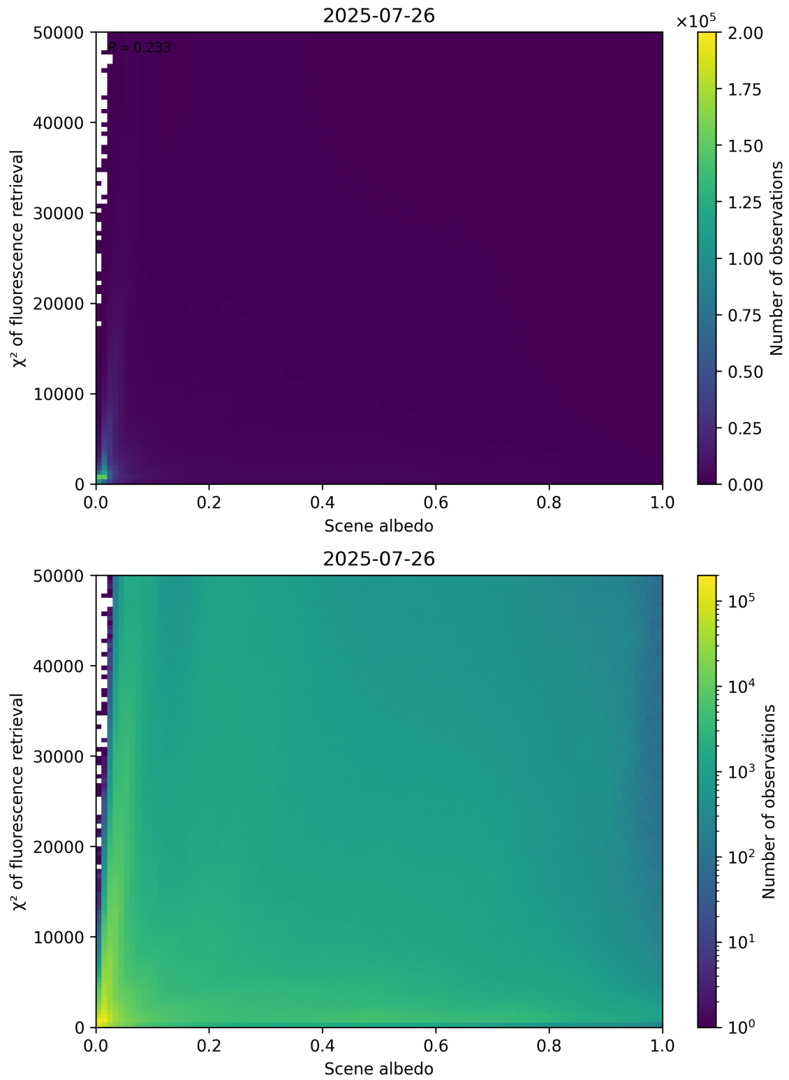
Figure 103: Scatter density plot of “Scene albedo” against “ \chi^2 of fluorescence retrieval” for 2025-07-25 to 2025-07-27.
