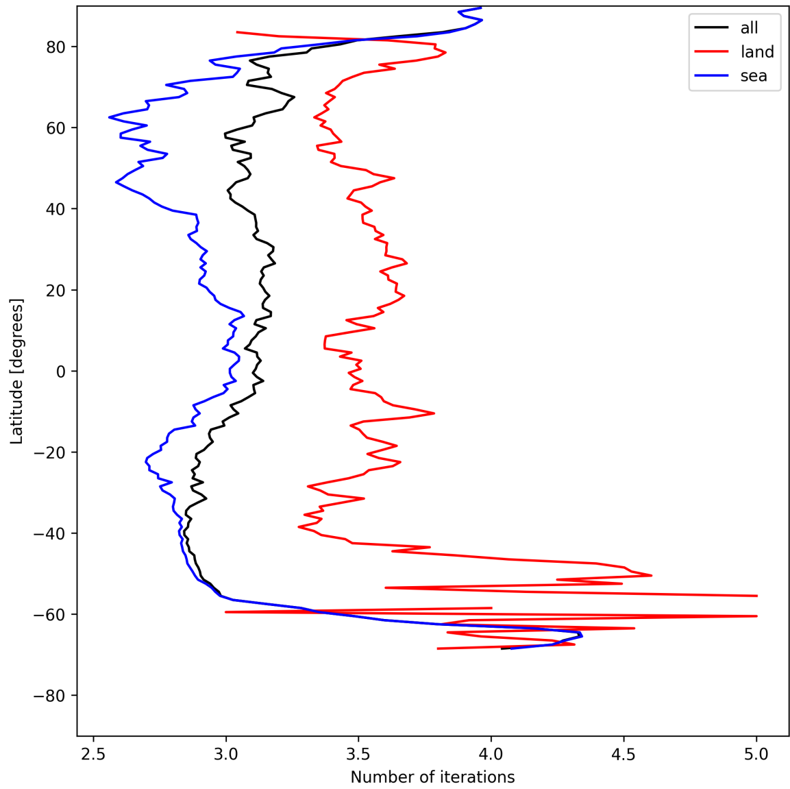
Figure 22: Zonal average of “Number of iterations” for 2025-07-25 to 2025-07-27.
