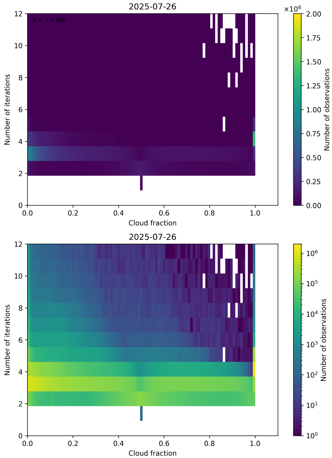
Figure 73: Scatter density plot of “Cloud fraction” against “Number of iterations” for 2025-07-25 to 2025-07-27.
