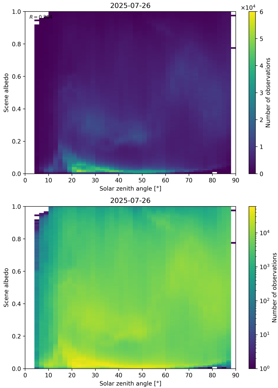
Figure 116: Scatter density plot of “Solar zenith angle” against “Scene albedo” for 2025-07-25 to 2025-07-27.
