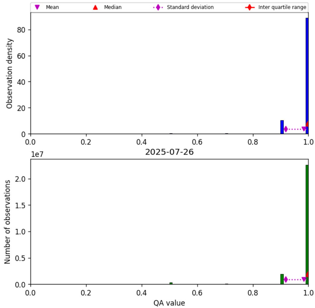
Figure 29: Histogram of “QA value” for 2025-07-25 to 2025-07-27
