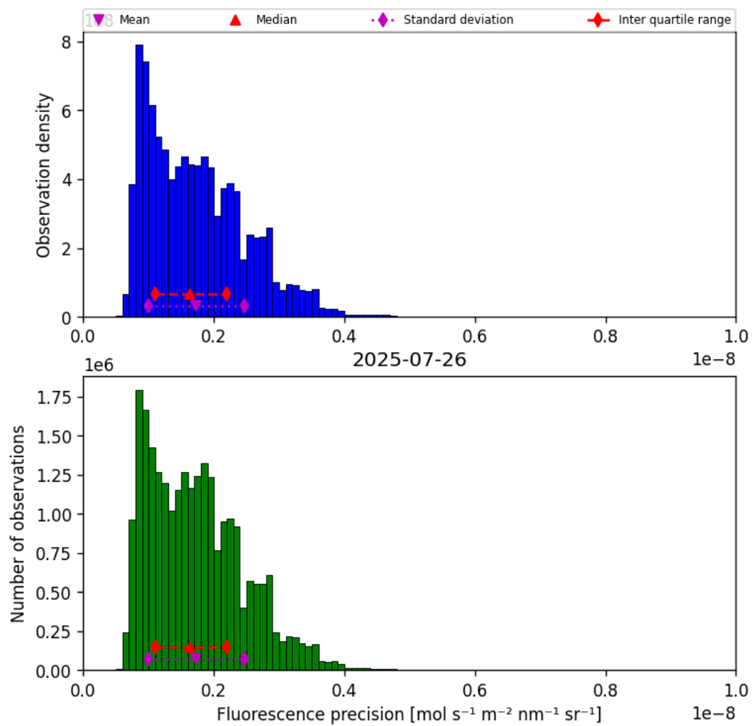
Figure 41: Histogram of “Fluorescence precision” for 2025-07-25 to 2025-07-27
