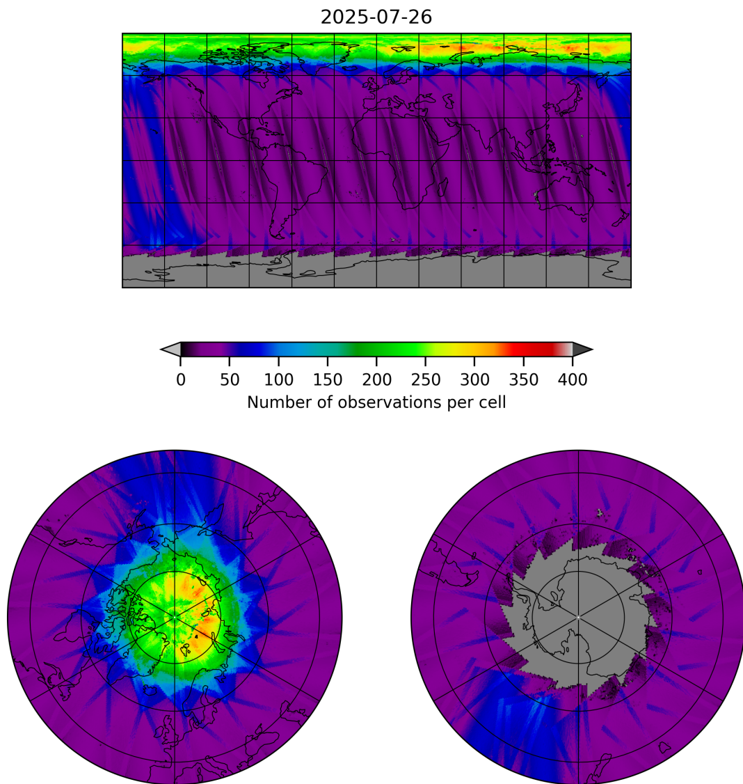
Figure 11: Map of the number of observations for 2025-07-25 to 2025-07-27
