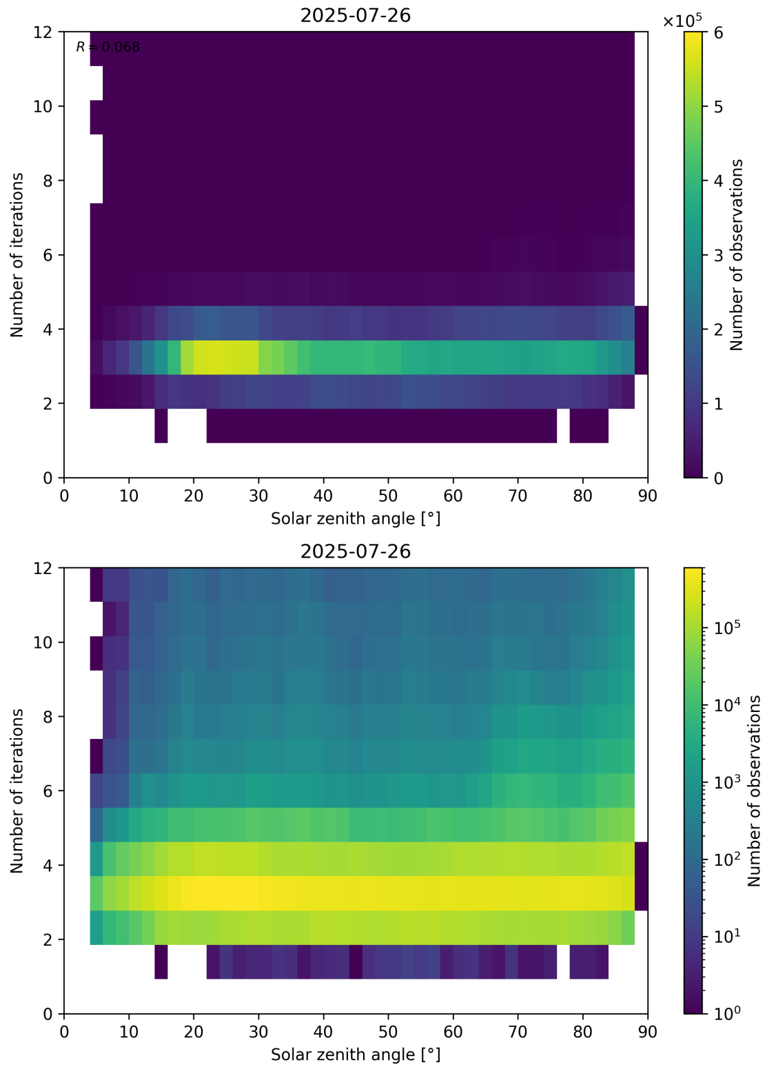
Figure 114: Scatter density plot of “Solar zenith angle” against “Number of iterations” for 2025-07-25 to 2025-07-27.
