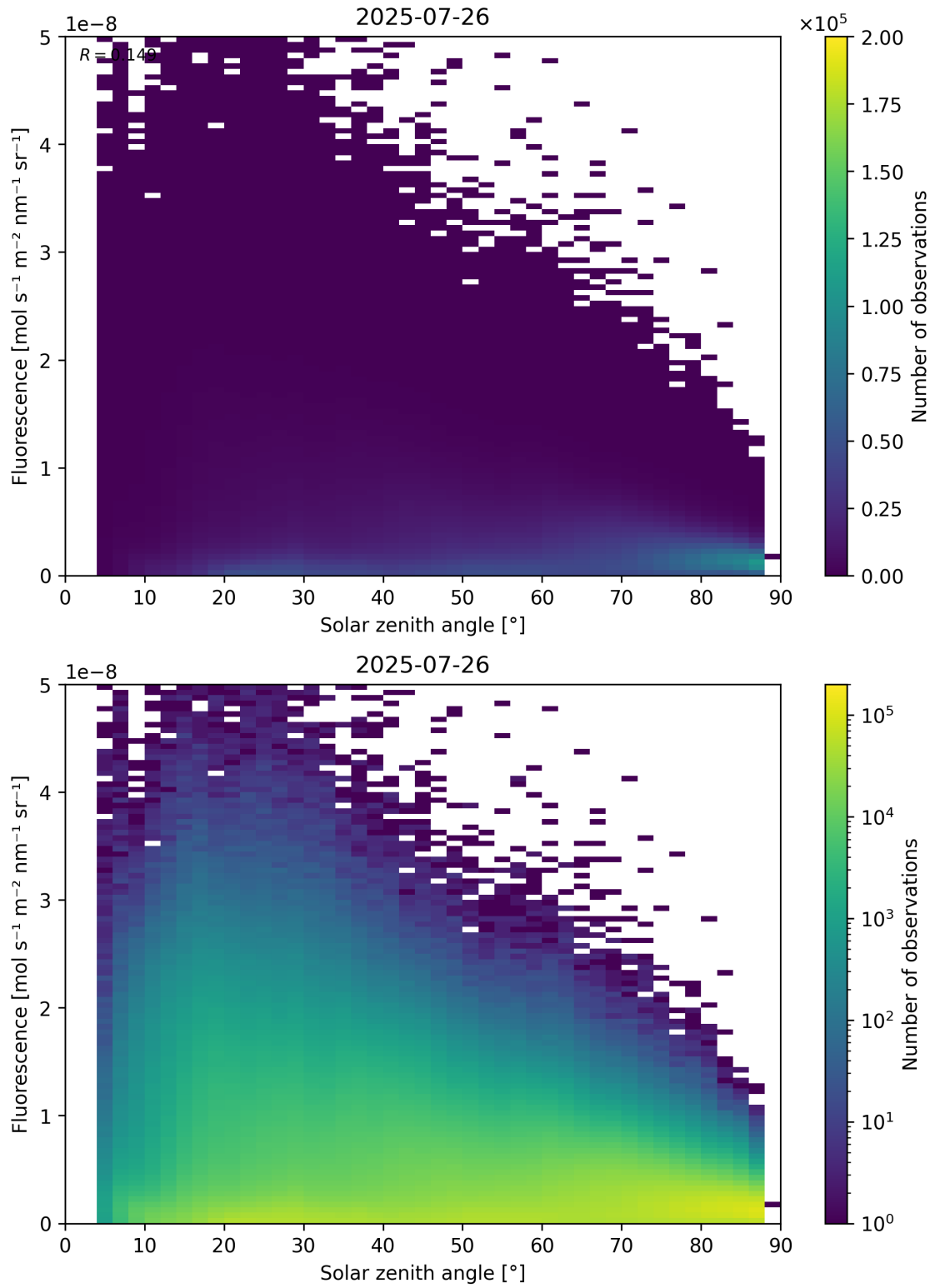
Figure 112: Scatter density plot of “Solar zenith angle” against “Fluorescence” for 2025-07-25 to 2025-07-27.
