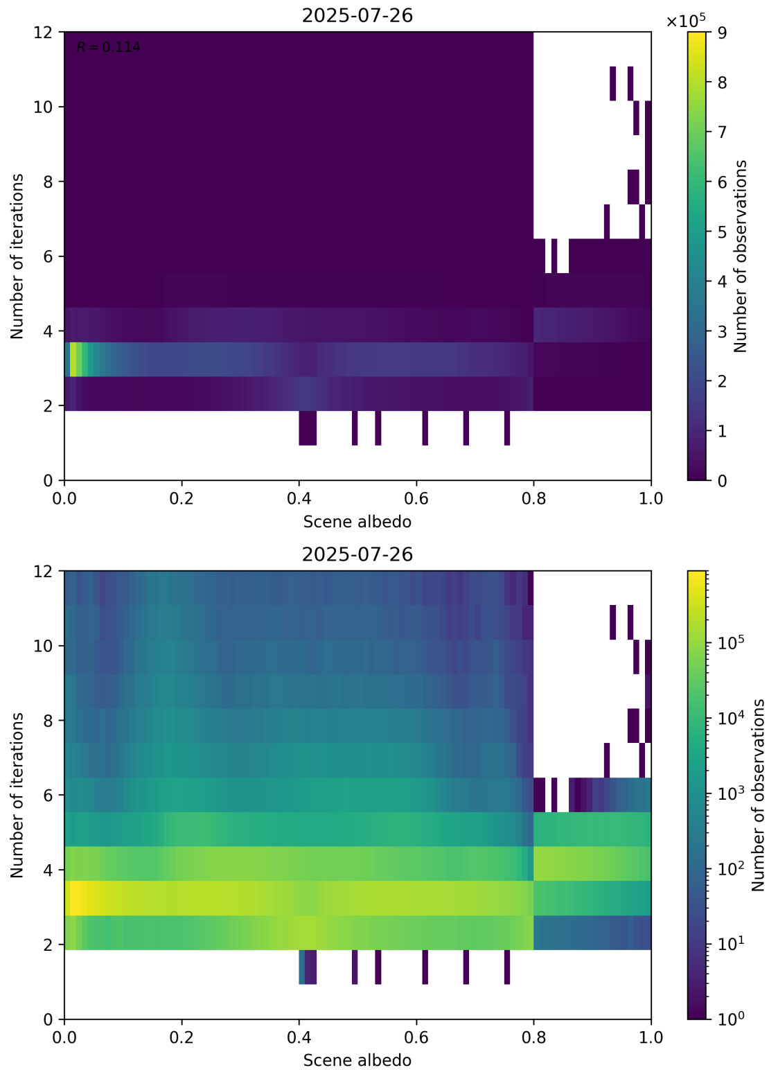
Figure 105: Scatter density plot of “Scene albedo” against “Number of iterations” for 2025-07-25 to 2025-07-27.
