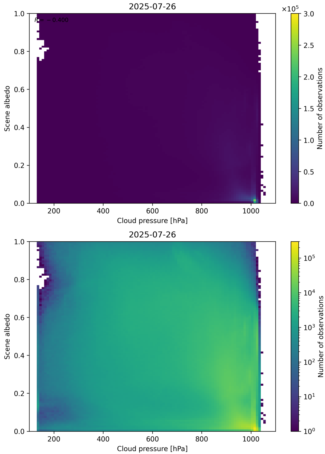
Figure 83: Scatter density plot of “Cloud pressure” against “Scene albedo” for 2025-07-25 to 2025-07-27.
