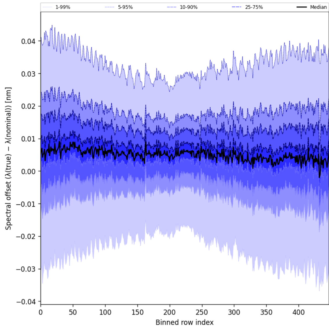
Figure 62: Along track statistics of “Spectral offset ( \lambda_{\text{true}} - \lambda_{\text{nominal}} )” for 2025-07-25 to 2025-07-27
