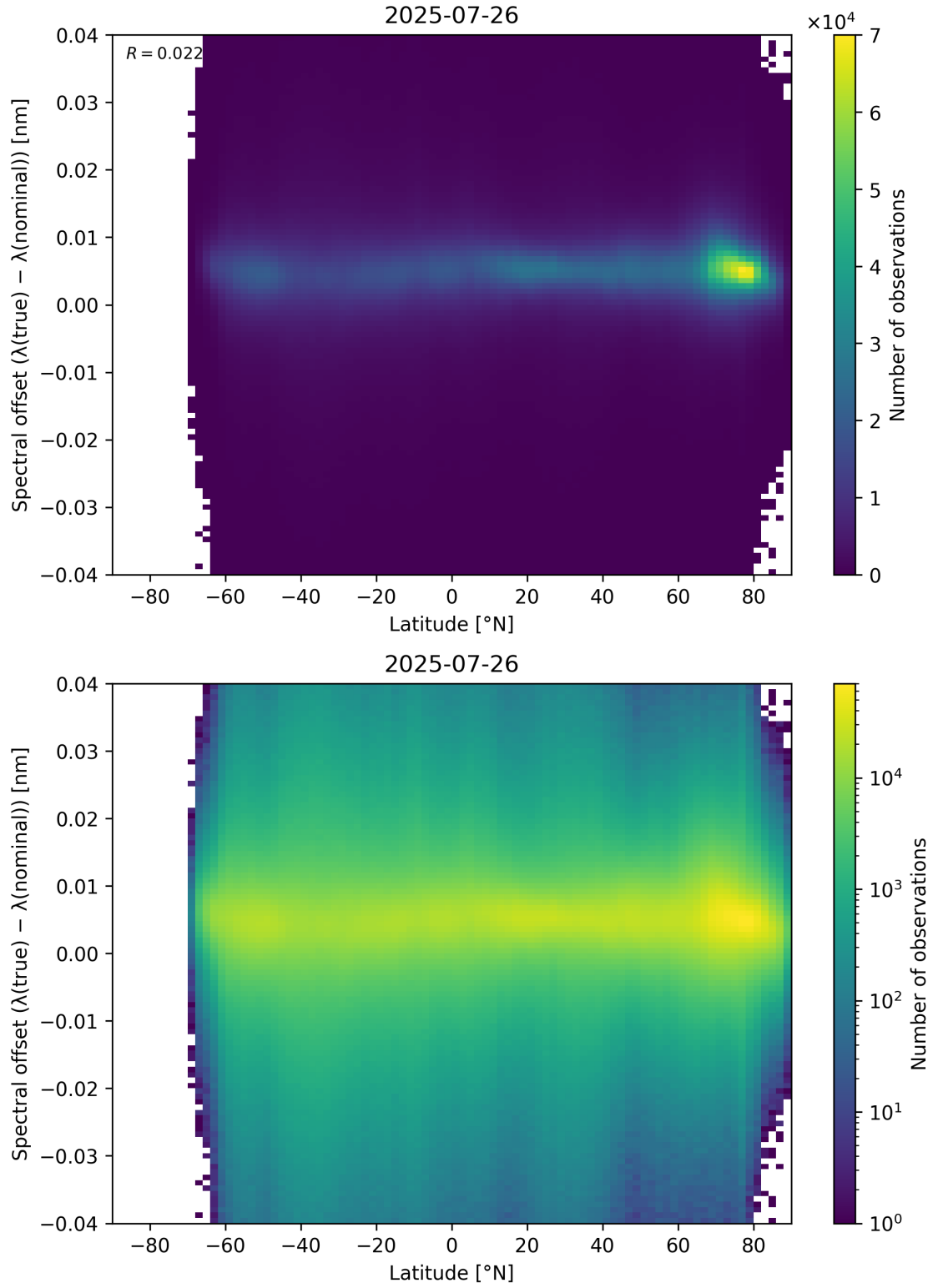
Figure 96: Scatter density plot of “Latitude” against “Spectral offset ( \lambda_{\text{true}} - \lambda_{\text{nominal}} )” for 2025-07-25 to 2025-07-27.
