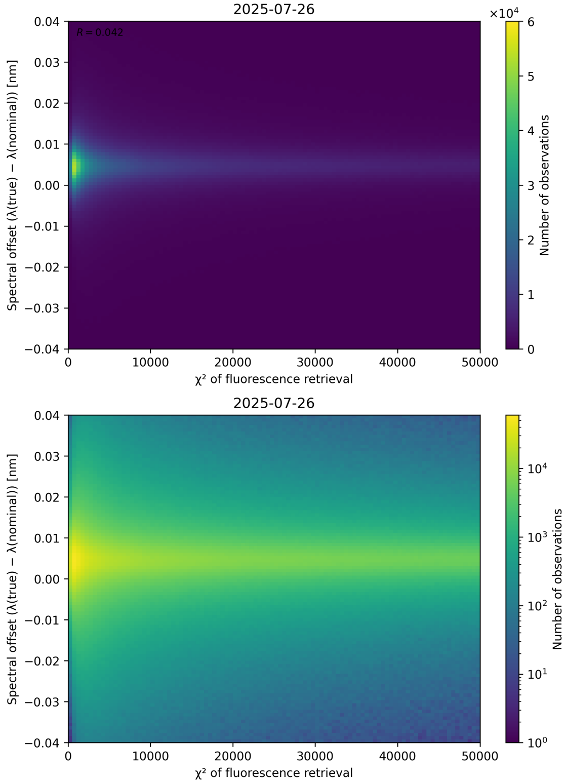
Figure 69: Scatter density plot of “ \chi^2 of fluorescence retrieval” against “Spectral offset ( \lambda_{\text{true}} - \lambda_{\text{nominal}} )” for 2025-07-25 to 2025-07-27.
