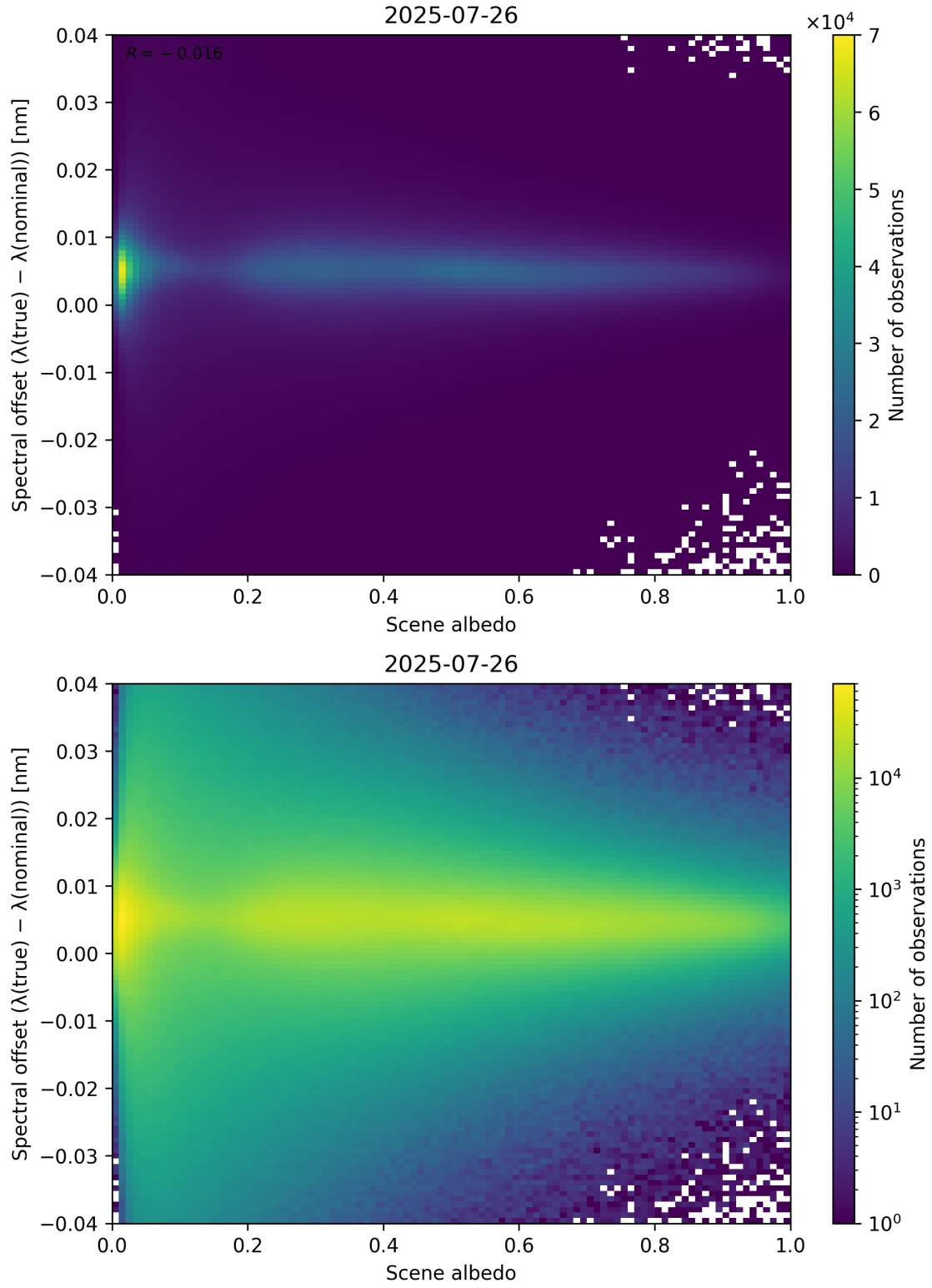
Figure 107: Scatter density plot of “Scene albedo” against “Spectral offset ( \lambda_{\text{true}} - \lambda_{\text{nominal}} )” for 2025-07-25 to 2025-07-27.
