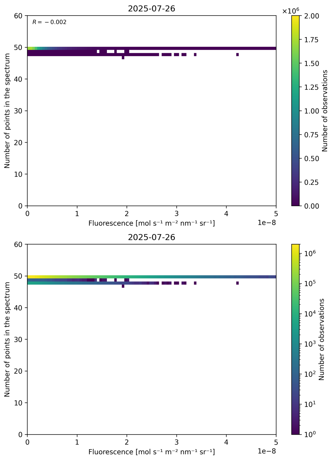
Figure 86: Scatter density plot of “Fluorescence” against “Number of points in the spectrum” for 2025-07-25 to 2025-07-27.
