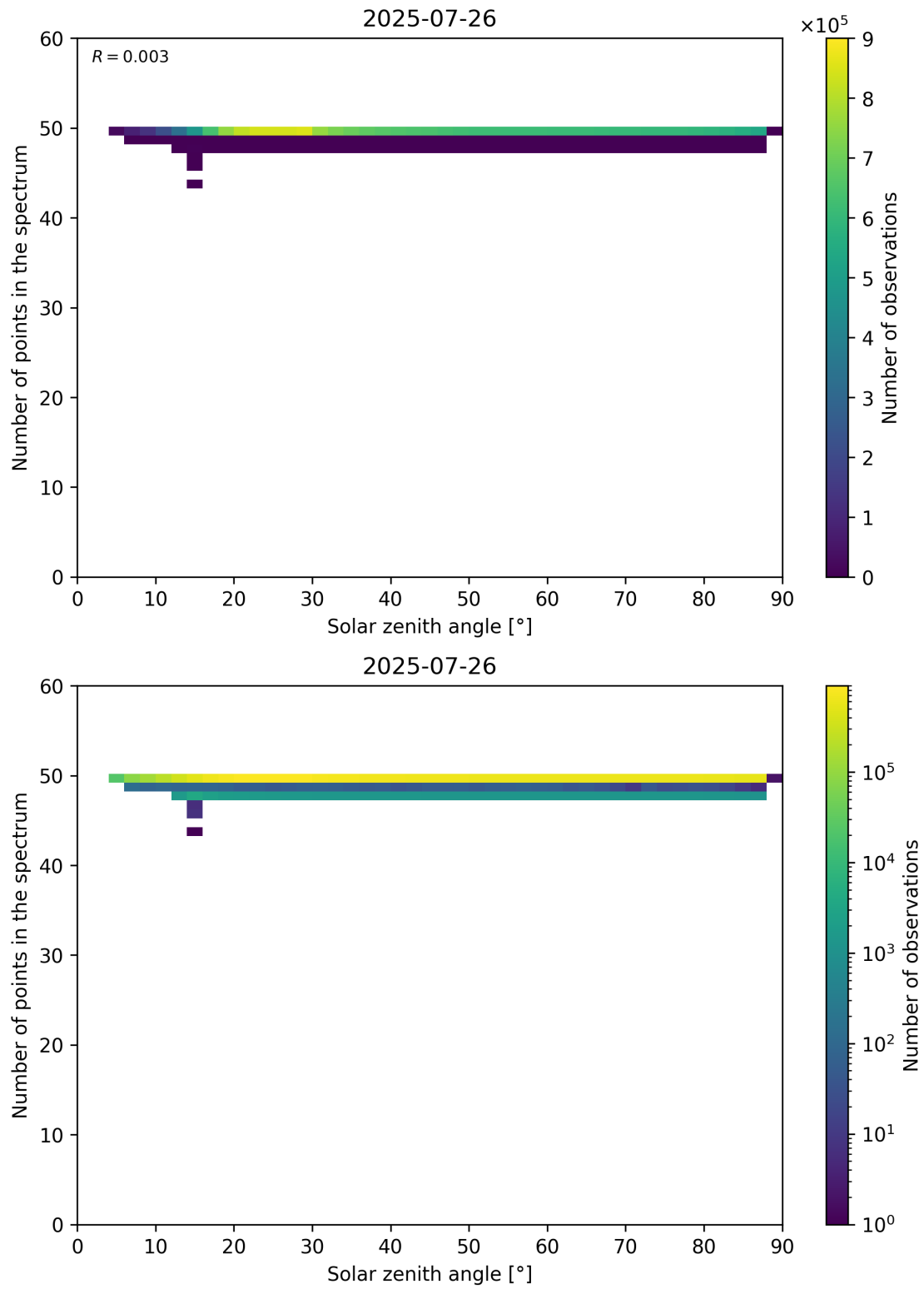
Figure 115: Scatter density plot of “Solar zenith angle” against “Number of points in the spectrum” for 2025-07-25 to 2025-07-27.
