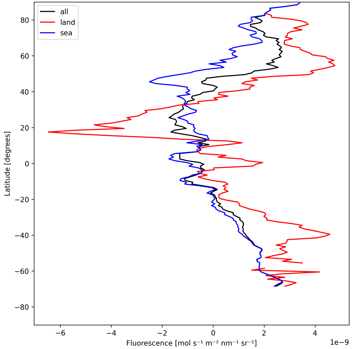
Figure 23: Zonal average of “Fluorescence” for 2025-07-25 to 2025-07-27.
