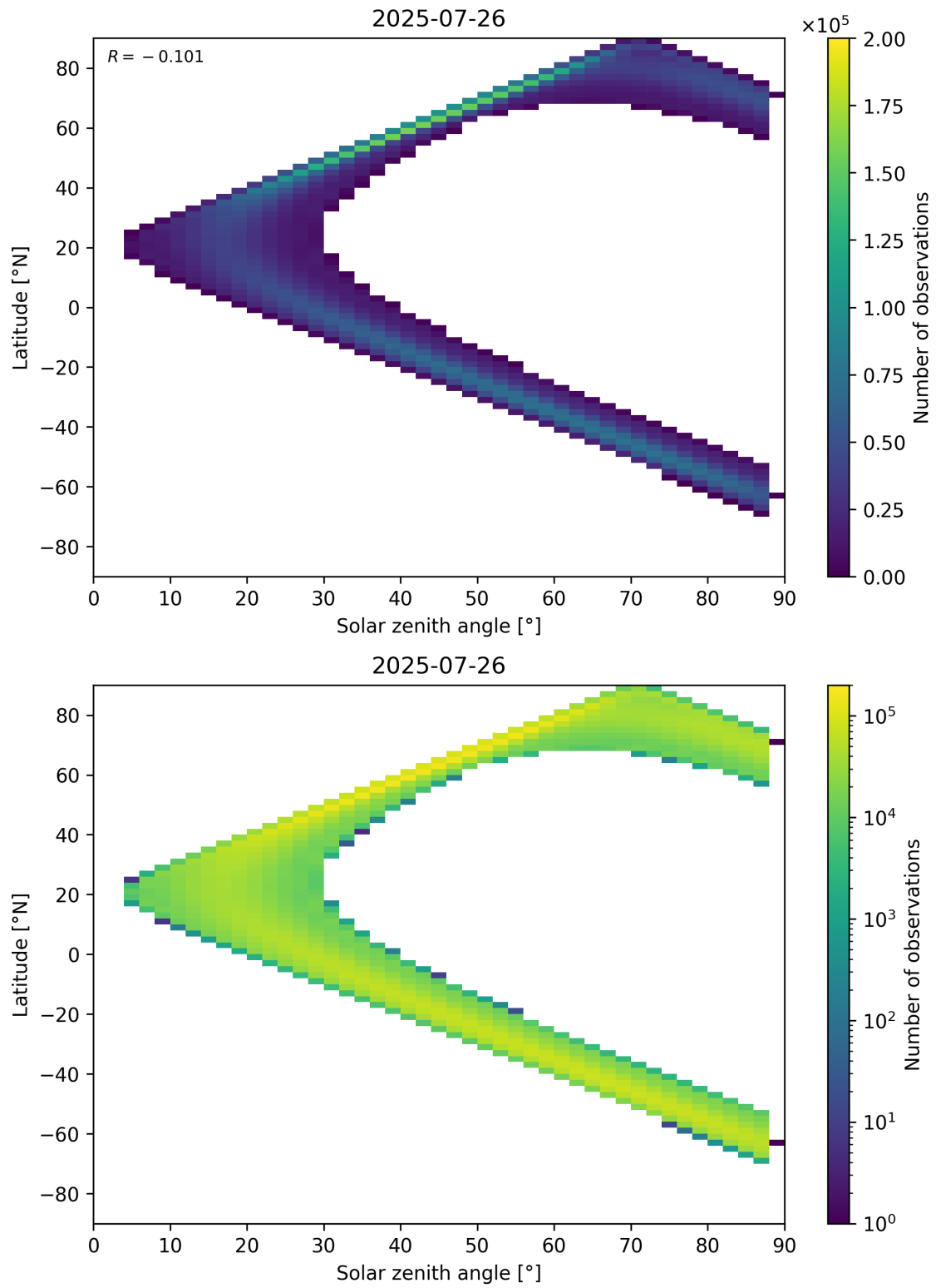
Figure 113: Scatter density plot of “Solar zenith angle” against “Latitude” for 2025-07-25 to 2025-07-27.
