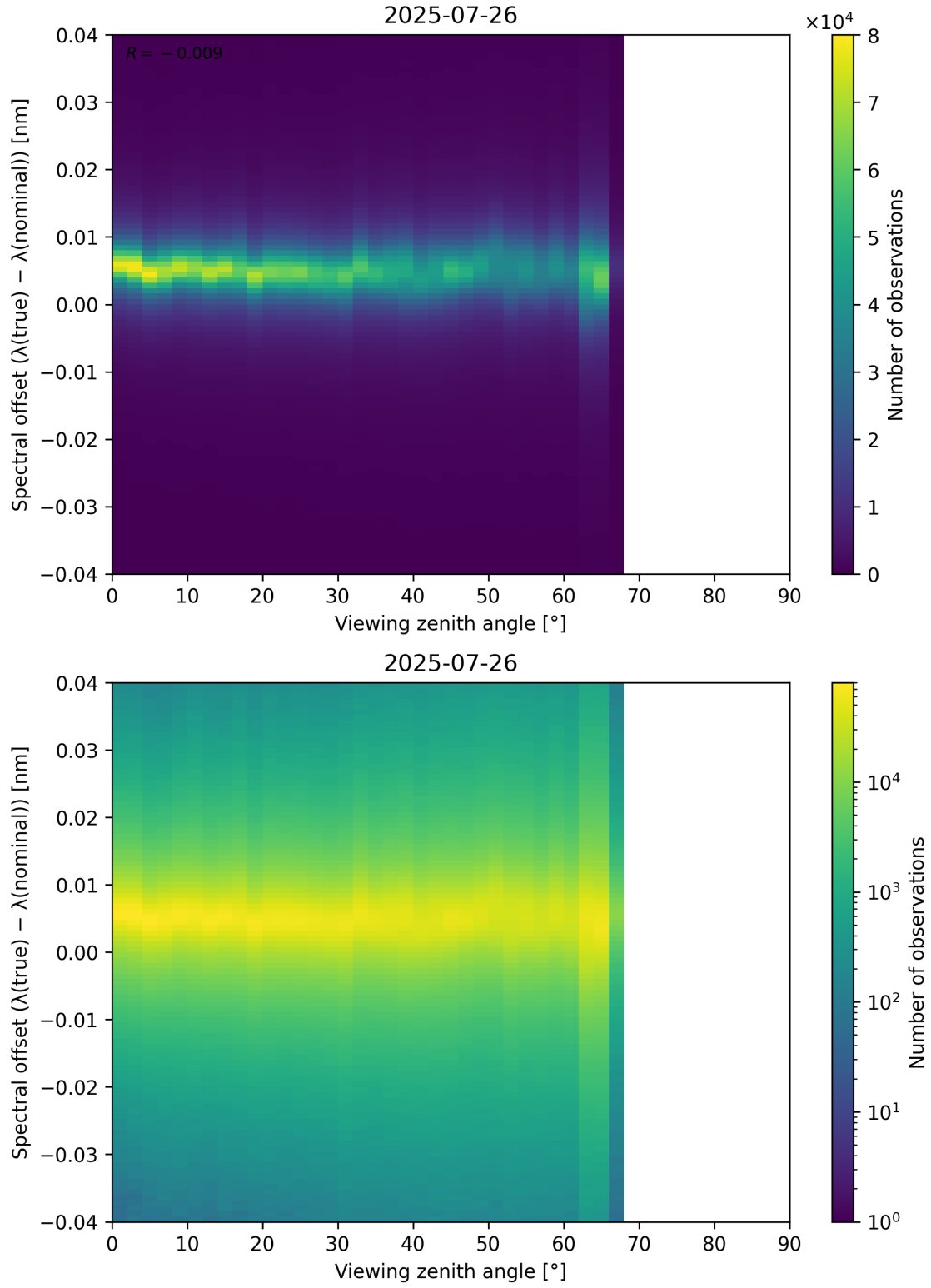
Figure 128: Scatter density plot of “Viewing zenith angle” against “Spectral offset ( \lambda_{\text{true}} - \lambda_{\text{nominal}} )” for 2025-07-25 to 2025-07-27.
