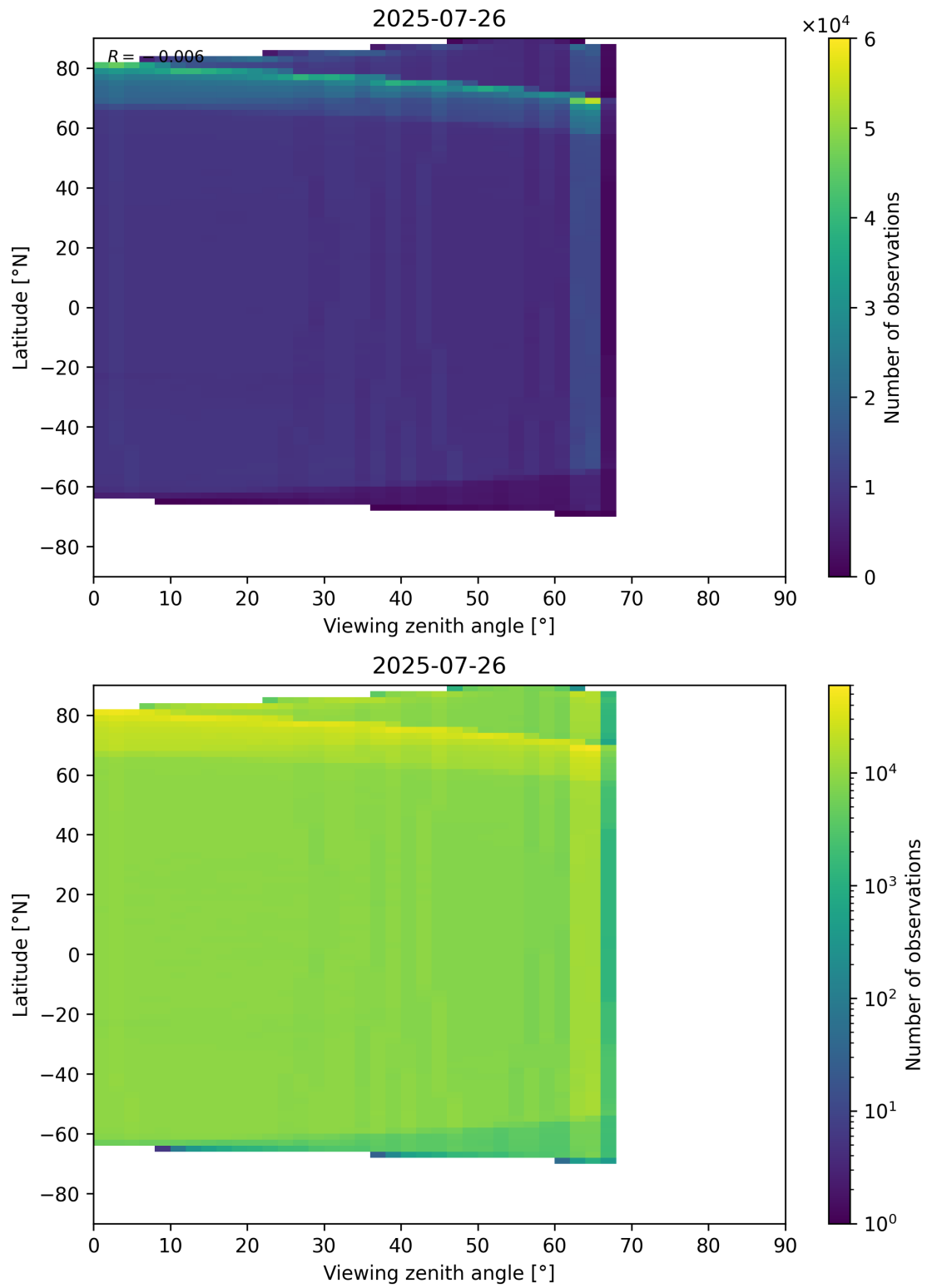
Figure 123: Scatter density plot of “Viewing zenith angle” against “Latitude” for 2025-07-25 to 2025-07-27.
