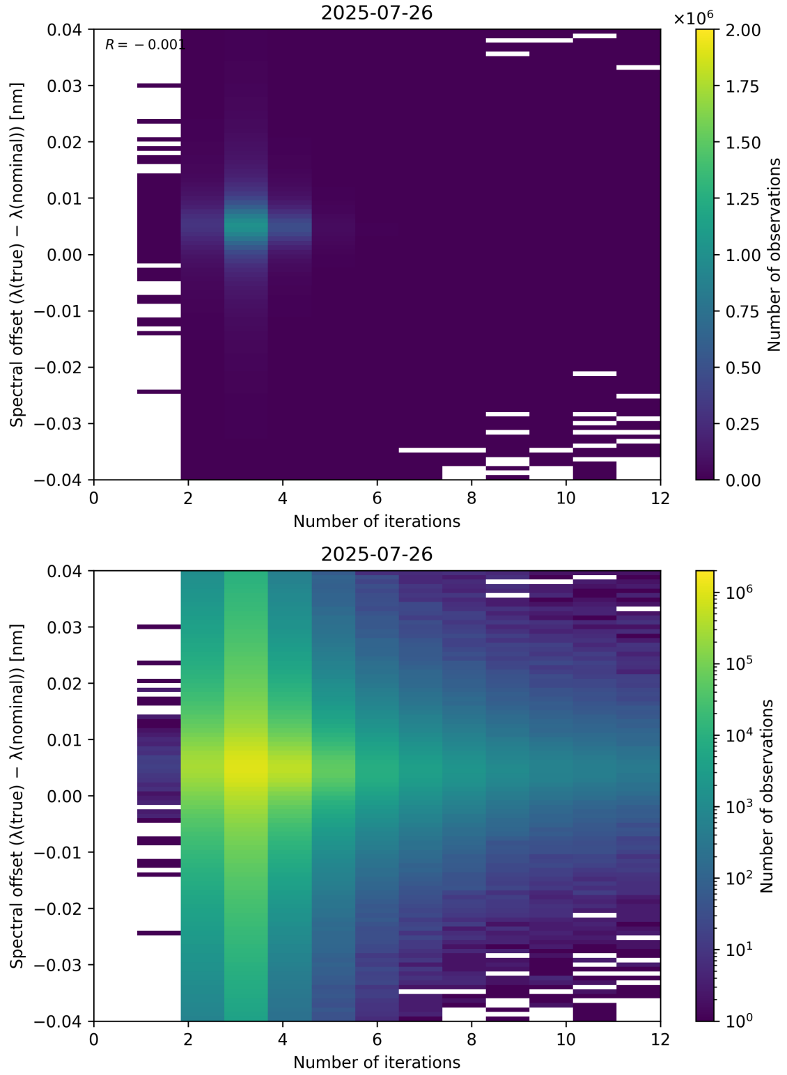
Figure 100: Scatter density plot of “Number of iterations” against “Spectral offset ( \lambda_{\text{true}} - \lambda_{\text{nominal}} )” for 2025-07-25 to 2025-07-27.
