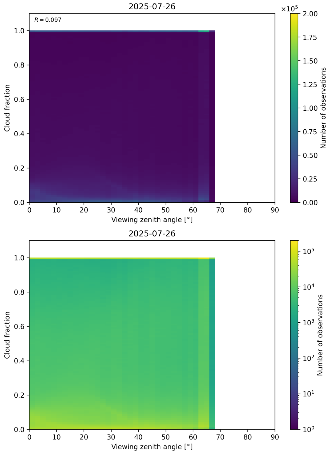
Figure 120: Scatter density plot of “Viewing zenith angle” against “Cloud fraction” for 2025-07-25 to 2025-07-27.
