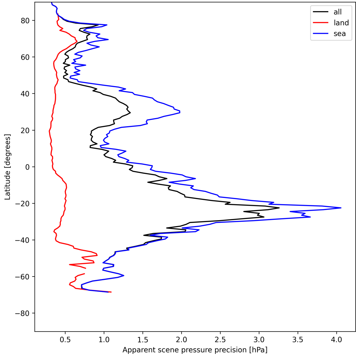
Figure 20: Zonal average of “Apparent scene pressure precision” for 2025-07-25 to 2025-07-27.
