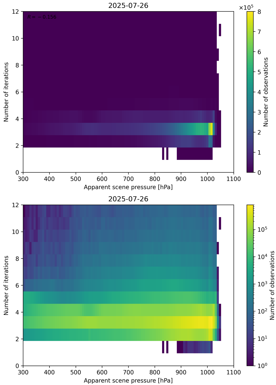
Figure 65: Scatter density plot of “Apparent scene pressure” against “Number of iterations” for 2025-07-25 to 2025-07-27.
