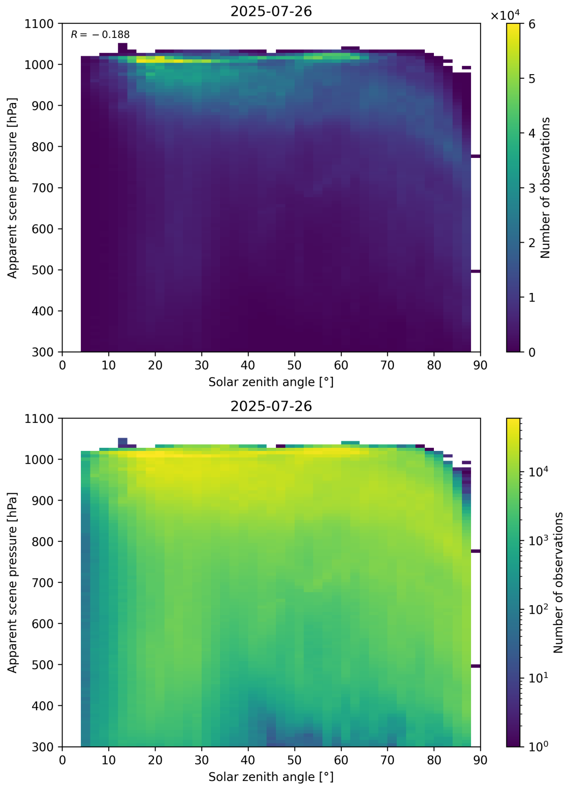
Figure 108: Scatter density plot of “Solar zenith angle” against “Apparent scene pressure” for 2025-07-25 to 2025-07-27.
