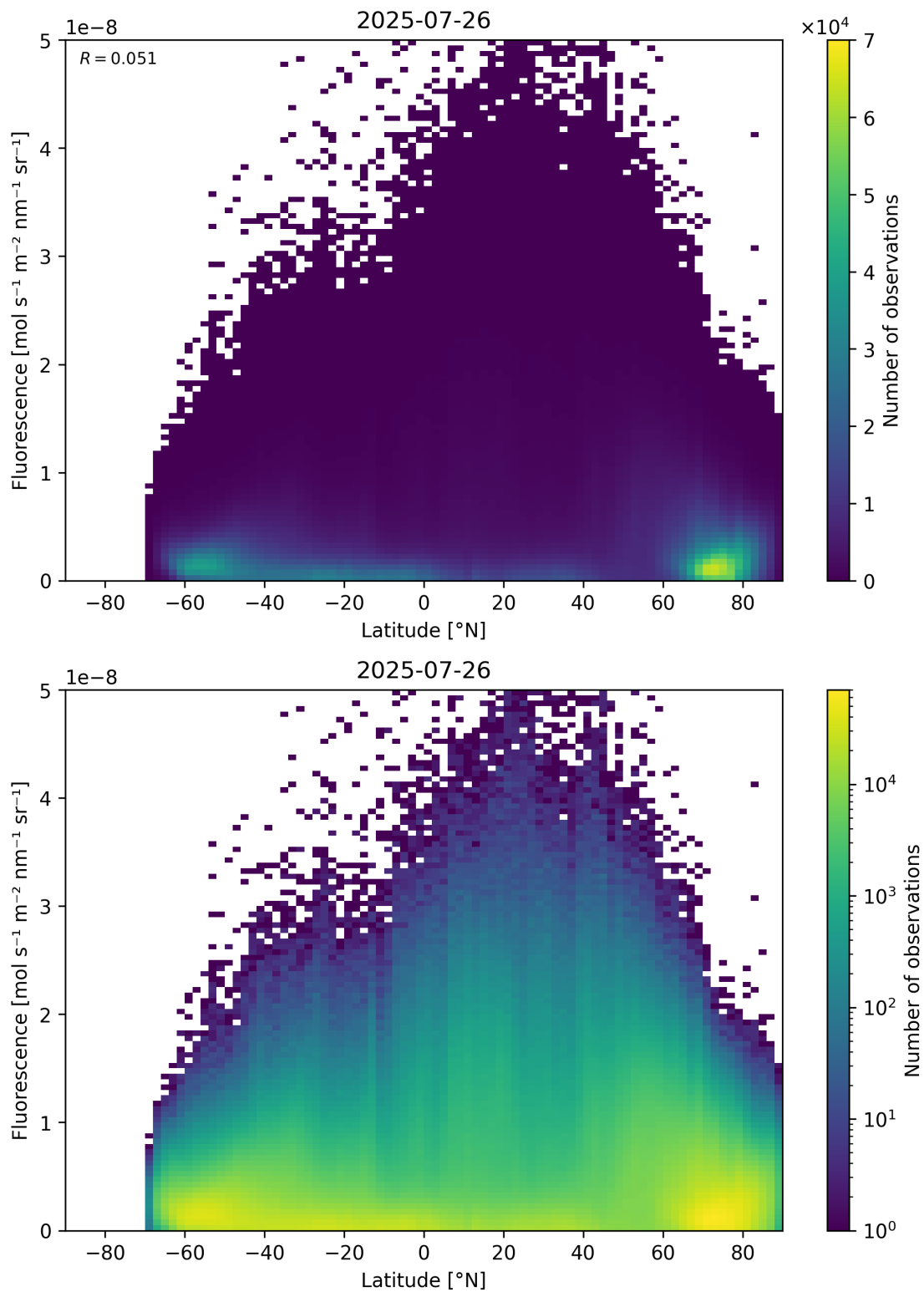
Figure 92: Scatter density plot of “Latitude” against “Fluorescence” for 2025-07-25 to 2025-07-27.
