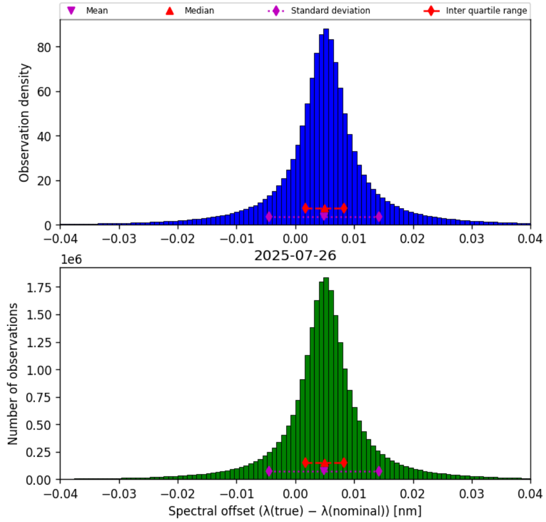
Figure 45: Histogram of “Spectral offset ( \lambda_{\text{true}} - \lambda_{\text{nominal}} )” for 2025-07-25 to 2025-07-27
