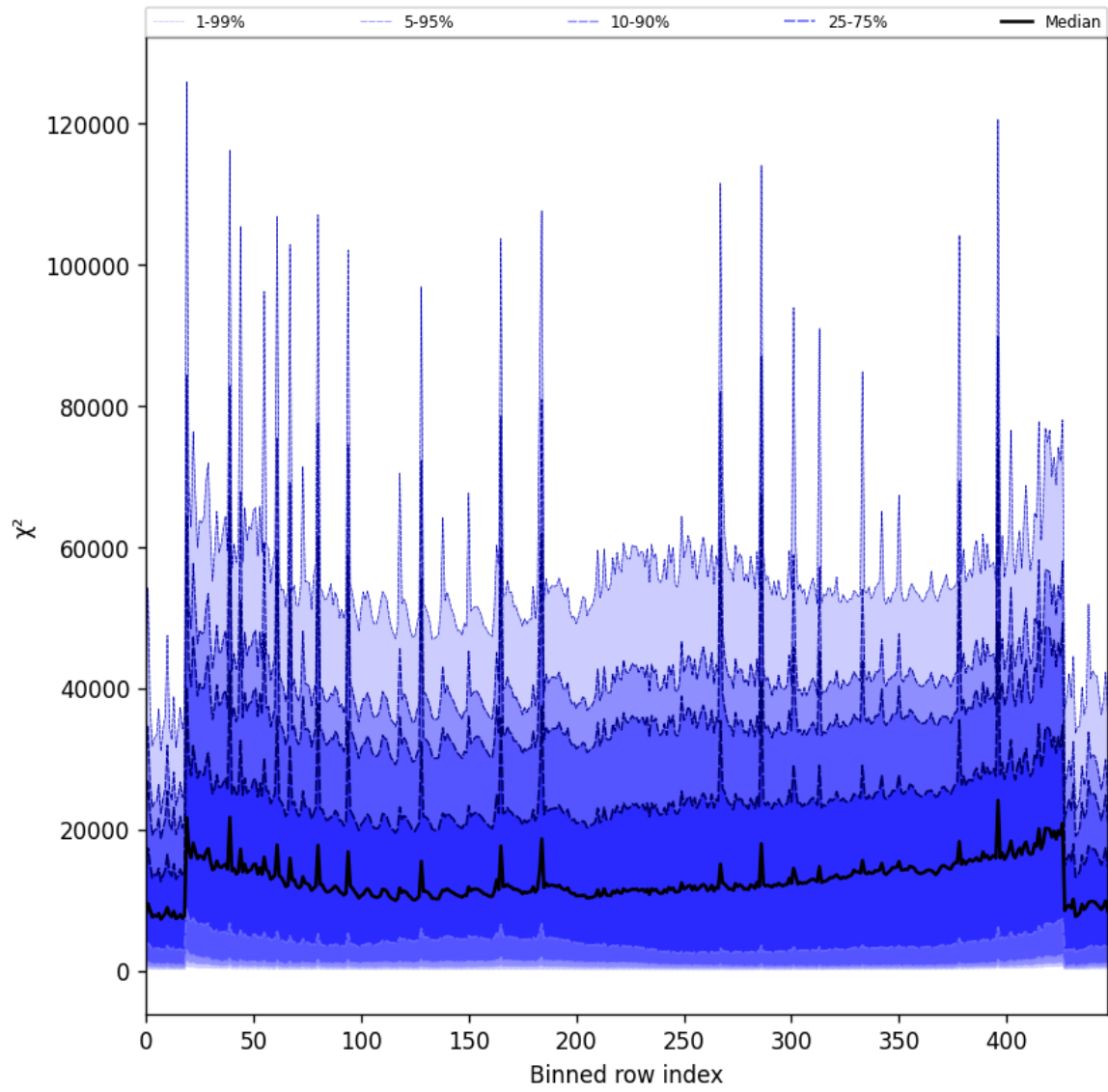
Figure 55: Along track statistics of “ \chi^2 ” for 2025-07-25 to 2025-07-27
