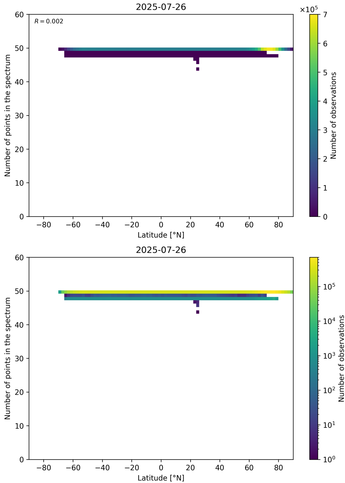
Figure 94: Scatter density plot of “Latitude” against “Number of points in the spectrum” for 2025-07-25 to 2025-07-27.
