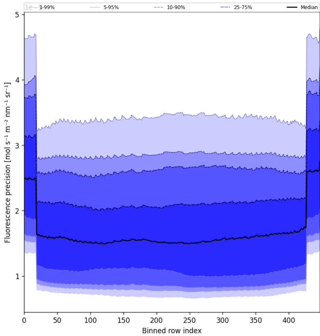
Figure 58: Along track statistics of “Fluorescence precision” for 2025-07-25 to 2025-07-27
