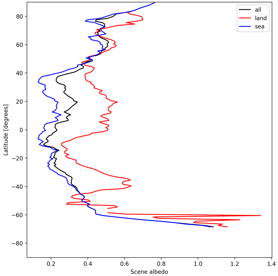
Figure 17: Zonal average of "Scene albedo" for 2025-07-25 to 2025-07-27.
