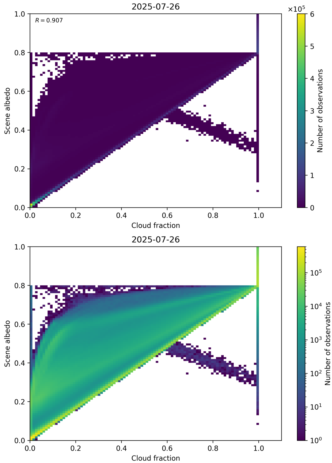
Figure 75: Scatter density plot of “Cloud fraction” against “Scene albedo” for 2025-07-25 to 2025-07-27.
