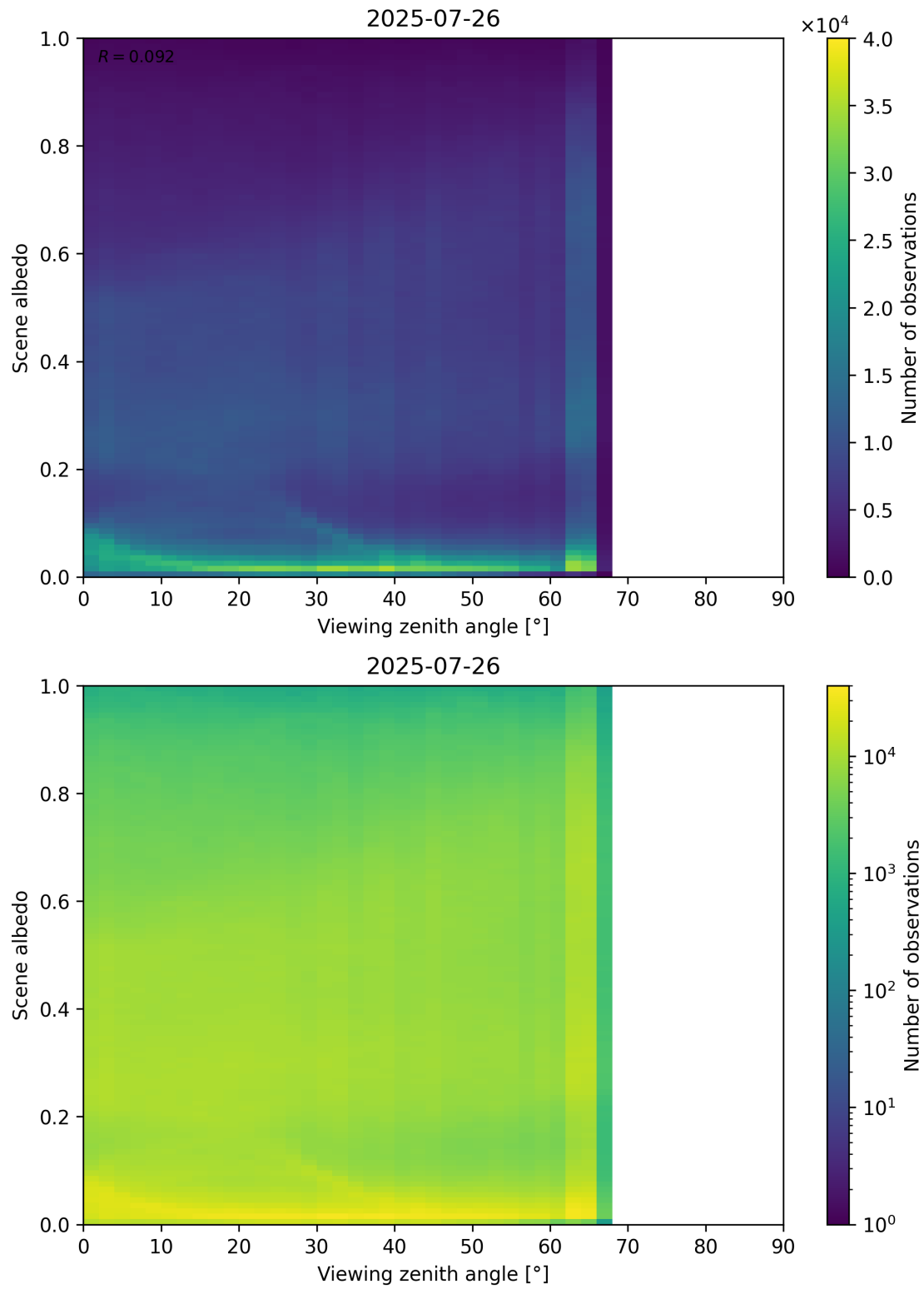
Figure 126: Scatter density plot of “Viewing zenith angle” against “Scene albedo” for 2025-07-25 to 2025-07-27.
