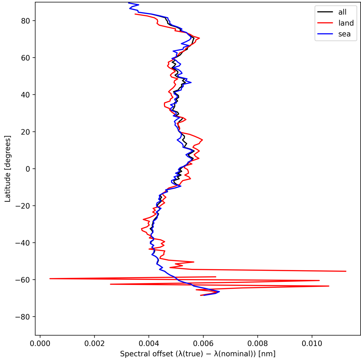
Figure 28: Zonal average of “Spectral offset ( \lambda_{\text{true}} - \lambda_{\text{nominal}} )” for 2025-07-25 to 2025-07-27.
