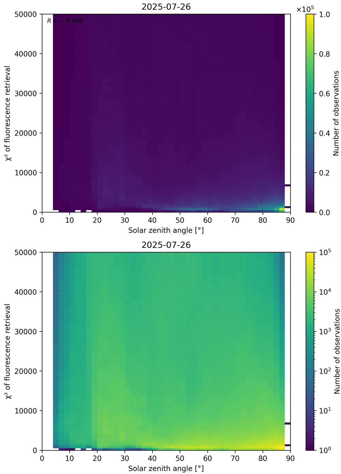
Figure 109: Scatter density plot of “Solar zenith angle” against “ \chi^2 of fluorescence retrieval” for 2025-07-25 to 2025-07-27.
