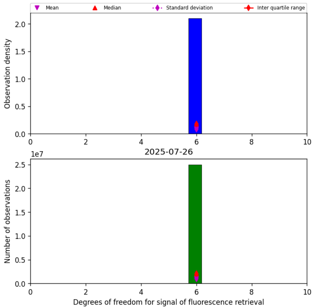
Figure 43: Histogram of “Degrees of freedom for signal of fluorescence retrieval” for 2025-07-25 to 2025-07-27
