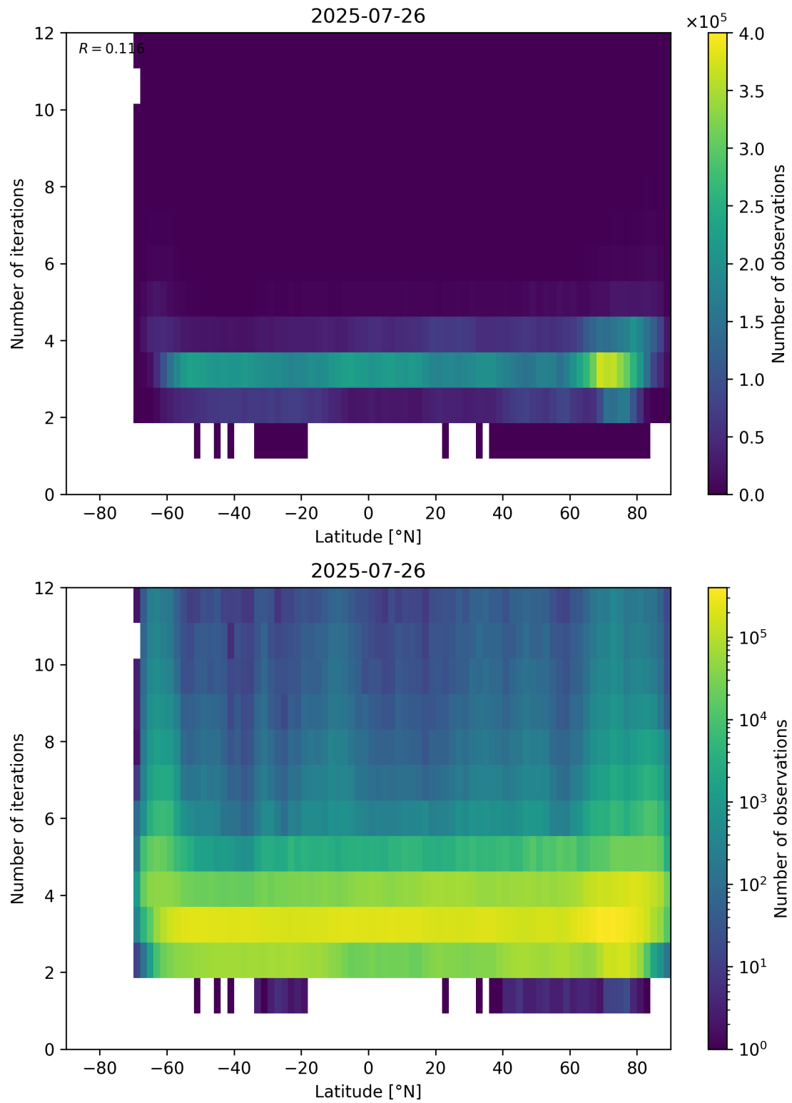
Figure 93: Scatter density plot of “Latitude” against “Number of iterations” for 2025-07-25 to 2025-07-27.
