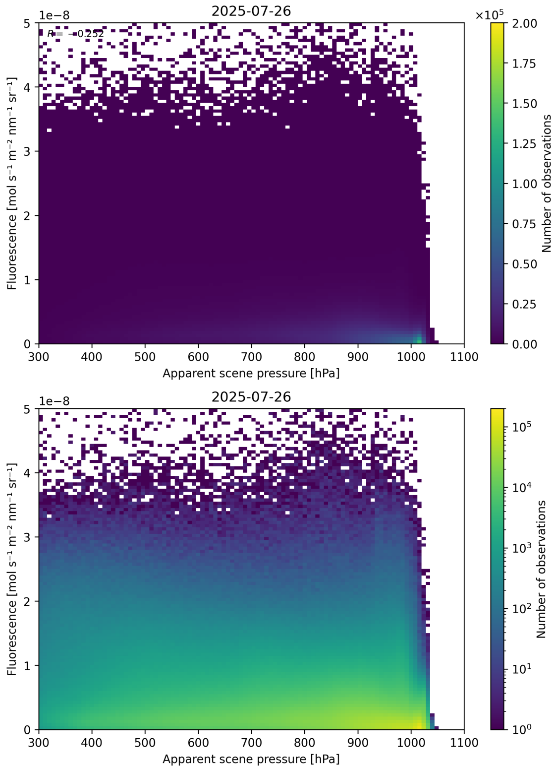
Figure 64: Scatter density plot of “Apparent scene pressure” against “Fluorescence” for 2025-07-25 to 2025-07-27.
