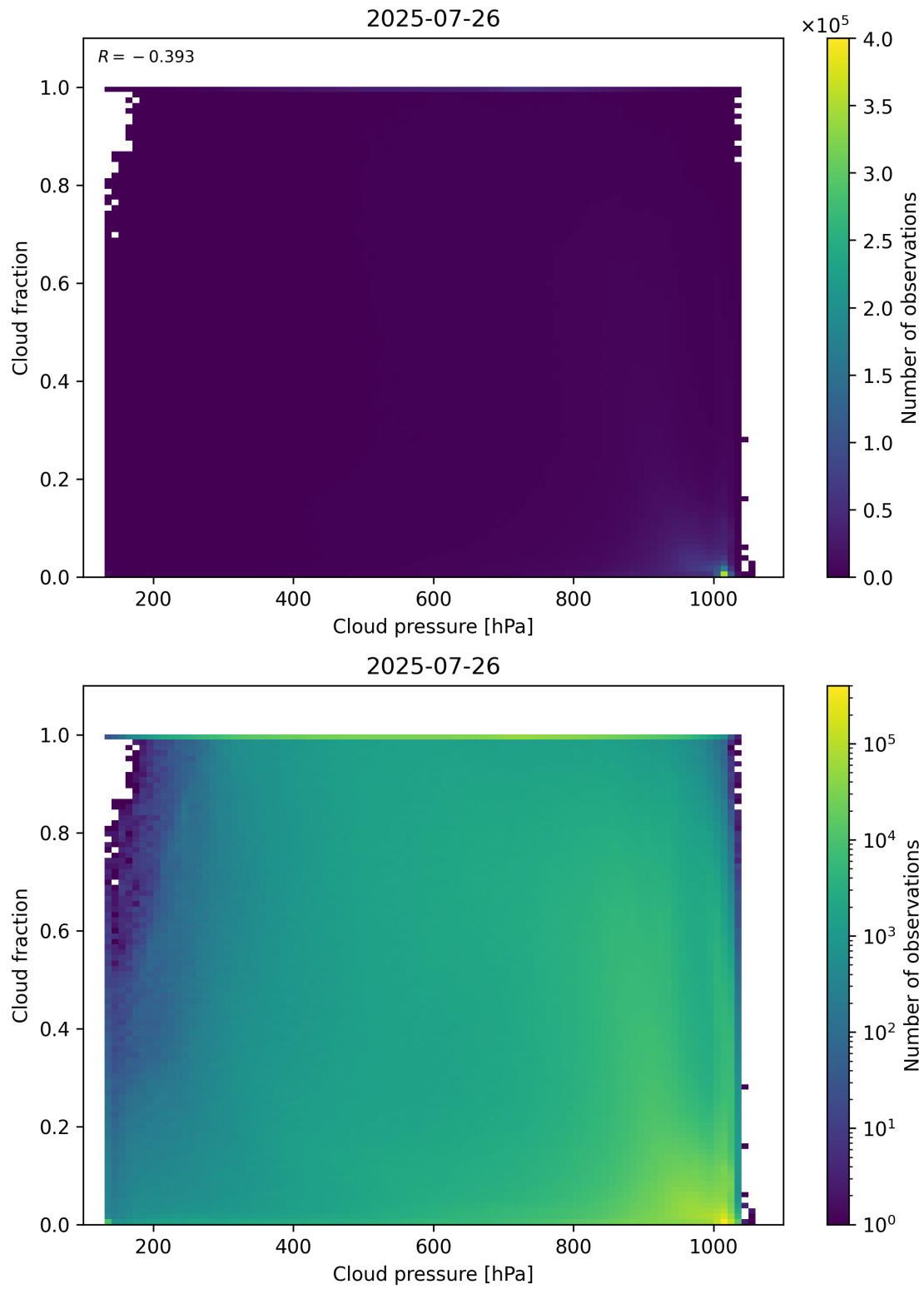
Figure 79: Scatter density plot of “Cloud pressure” against “Cloud fraction” for 2025-07-25 to 2025-07-27.
