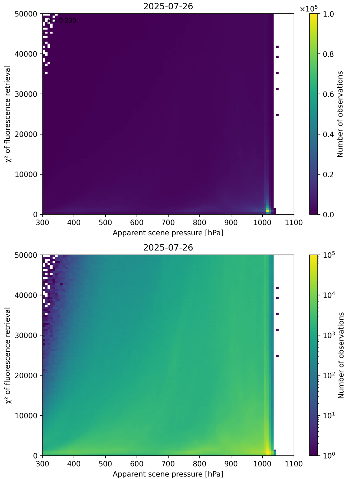
Figure 63: Scatter density plot of “Apparent scene pressure” against “ \chi^2 of fluorescence retrieval” for 2025-07-25 to 2025-07-27.
