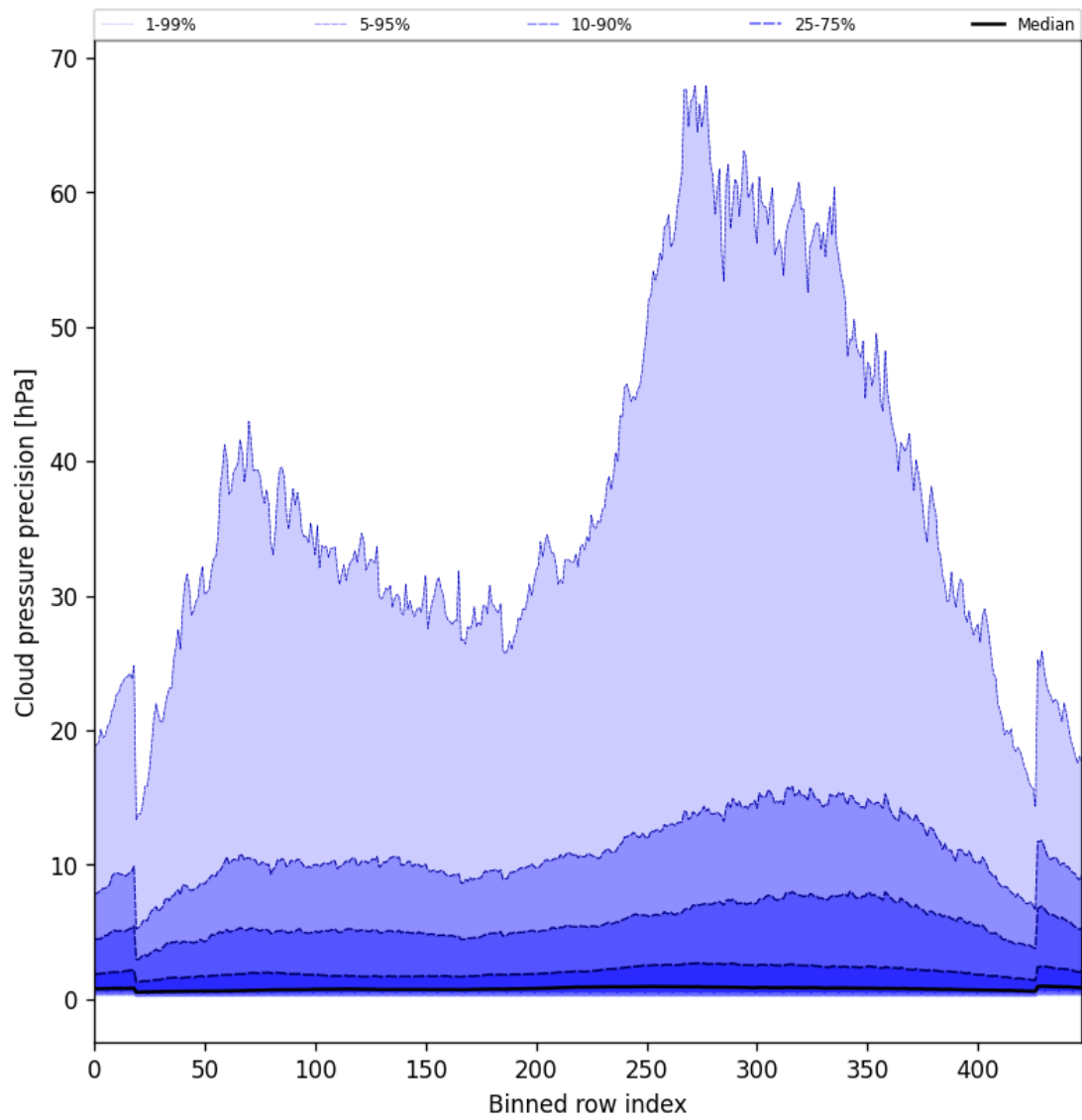
Figure 48: Along track statistics of “Cloud pressure precision” for 2025-07-25 to 2025-07-27
