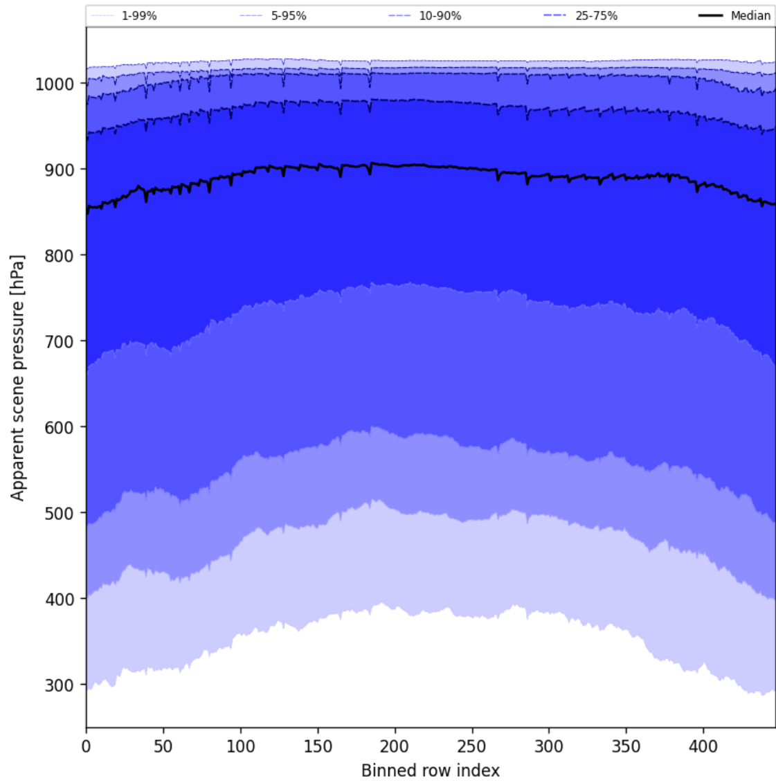
Figure 53: Along track statistics of “Apparent scene pressure” for 2025-07-25 to 2025-07-27
