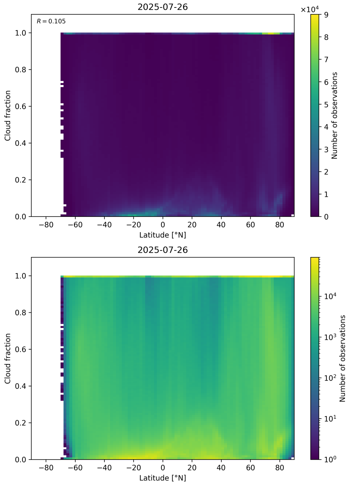
Figure 90: Scatter density plot of “Latitude” against “Cloud fraction” for 2025-07-25 to 2025-07-27.
