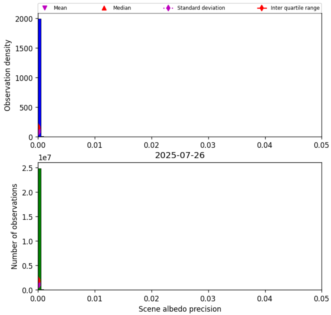
Figure 35: Histogram of “Scene albedo precision” for 2025-07-25 to 2025-07-27
