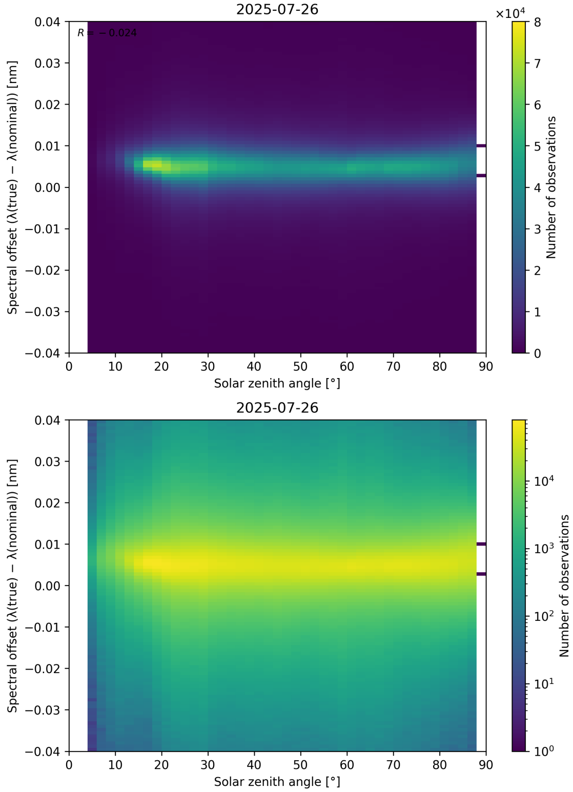
Figure 117: Scatter density plot of “Solar zenith angle” against “Spectral offset ( \lambda_{\text{true}} - \lambda_{\text{nominal}} )” for 2025-07-25 to 2025-07-27.
