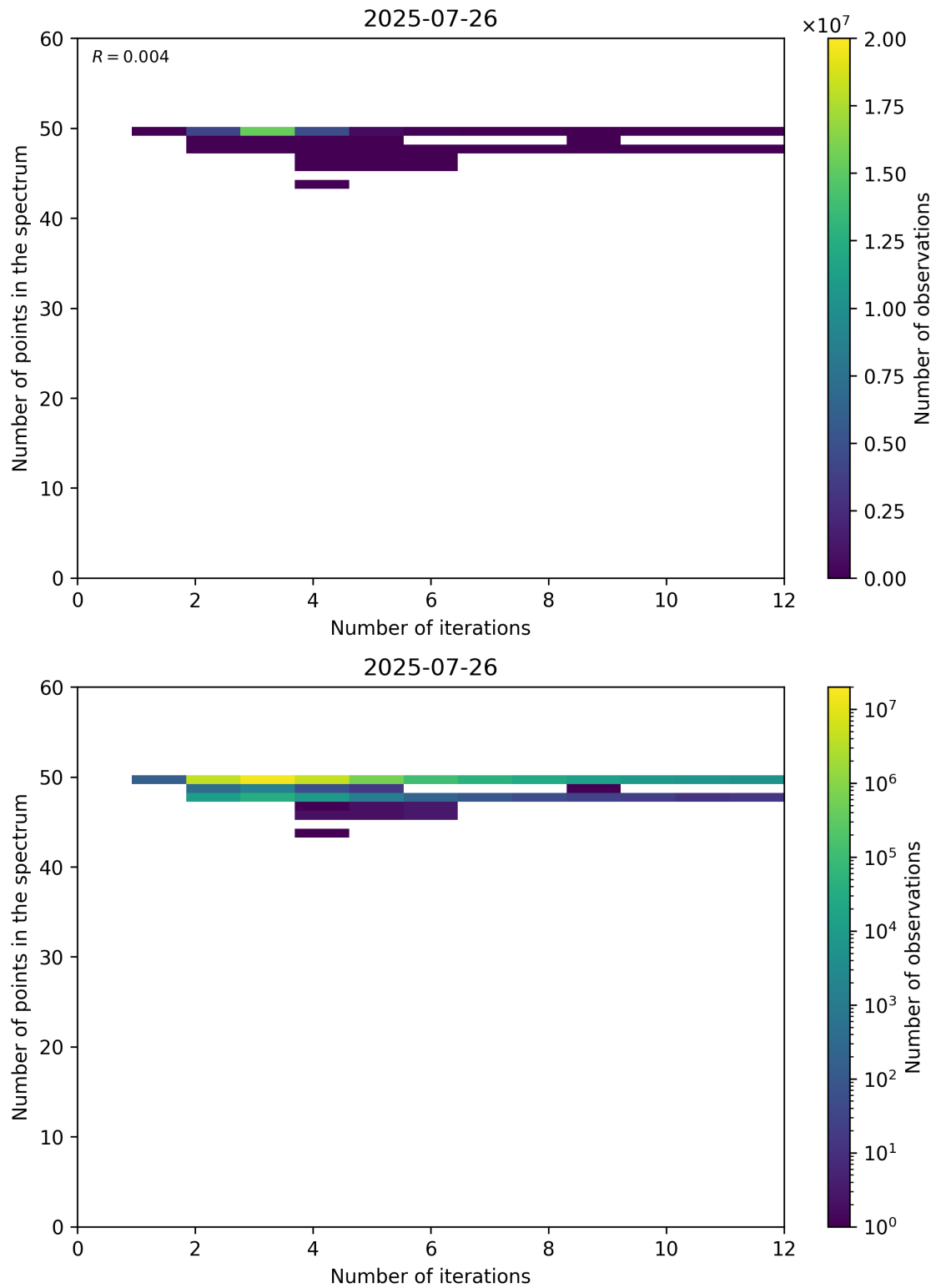
Figure 99: Scatter density plot of “Number of iterations” against “Number of points in the spectrum” for 2025-07-25 to 2025-07-27.
