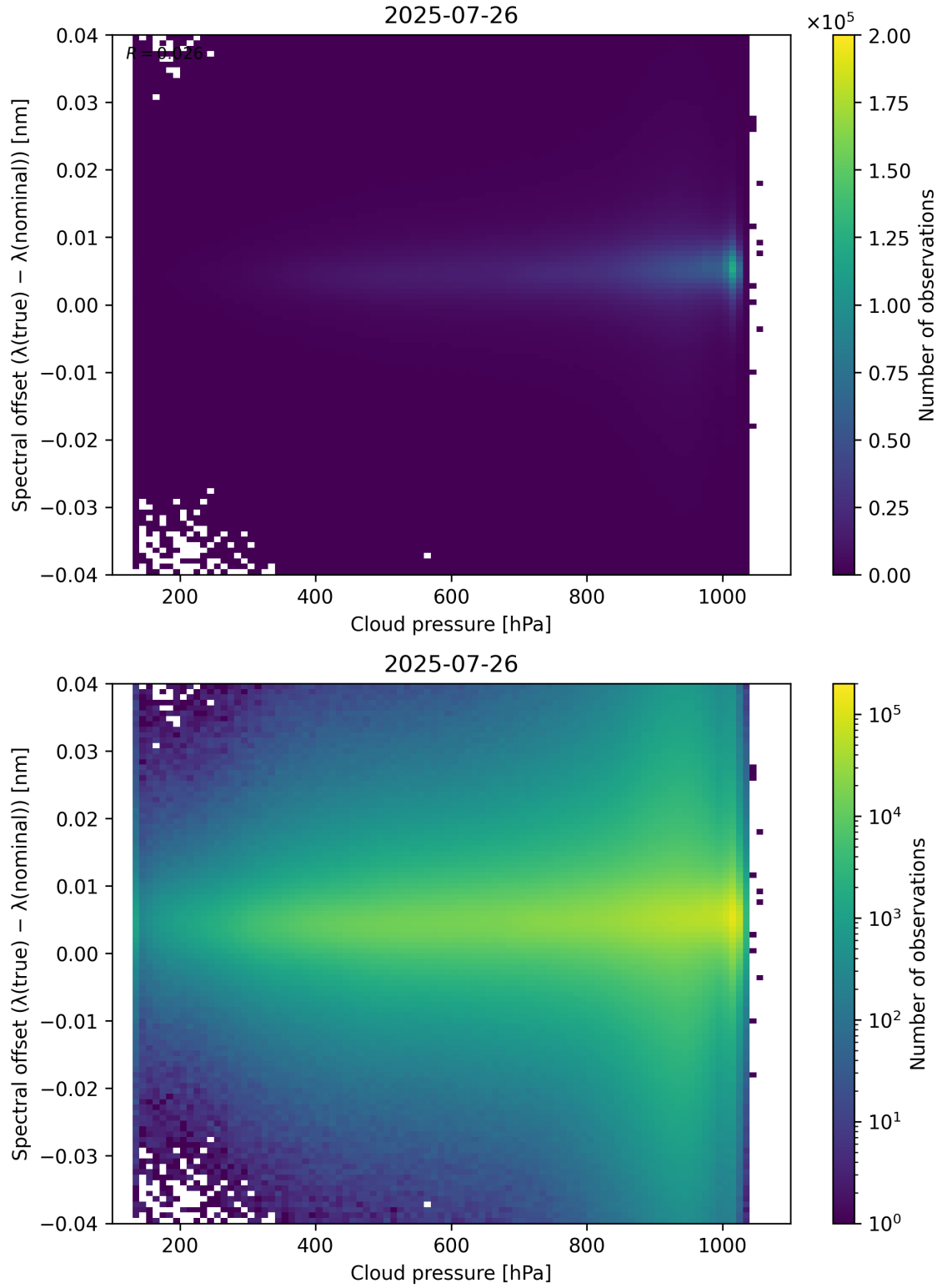
Figure 84: Scatter density plot of “Cloud pressure” against “Spectral offset ( \lambda_{\text{true}} - \lambda_{\text{nominal}} )” for 2025-07-25 to 2025-07-27.
