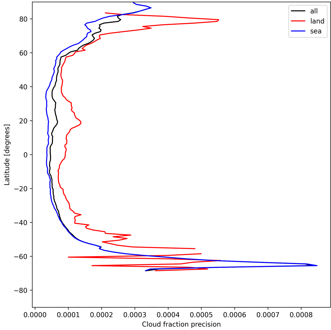
Figure 16: Zonal average of “Cloud fraction precision” for 2025-07-25 to 2025-07-27.
