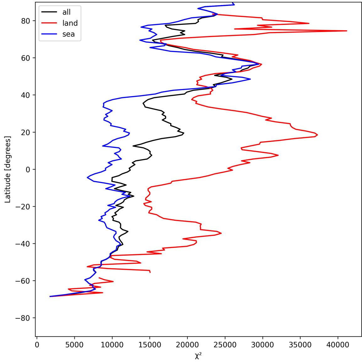
Figure 21: Zonal average of “ \chi^2 ” for 2025-07-25 to 2025-07-27.
