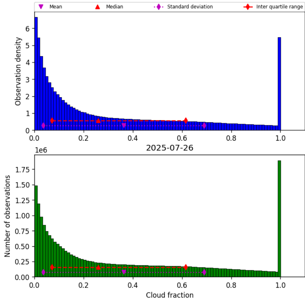
Figure 32: Histogram of “Cloud fraction” for 2025-07-25 to 2025-07-27
