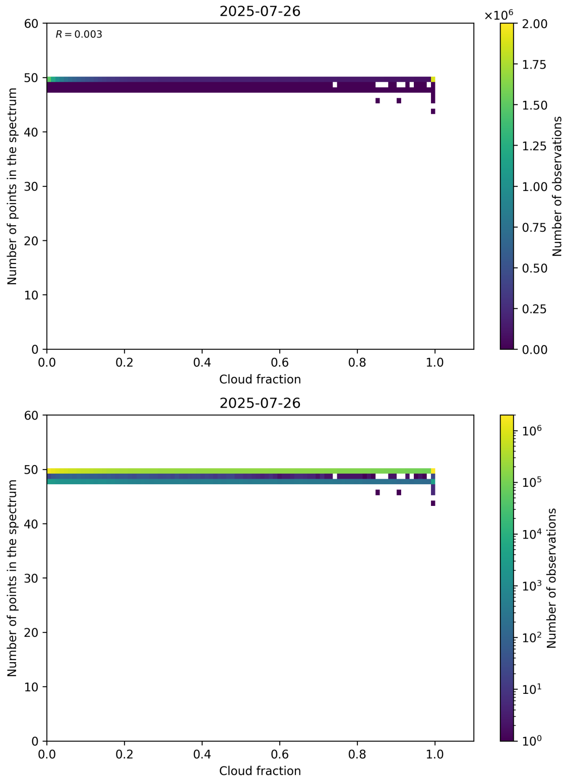
Figure 74: Scatter density plot of “Cloud fraction” against “Number of points in the spectrum” for 2025-07-25 to 2025-07-27.
