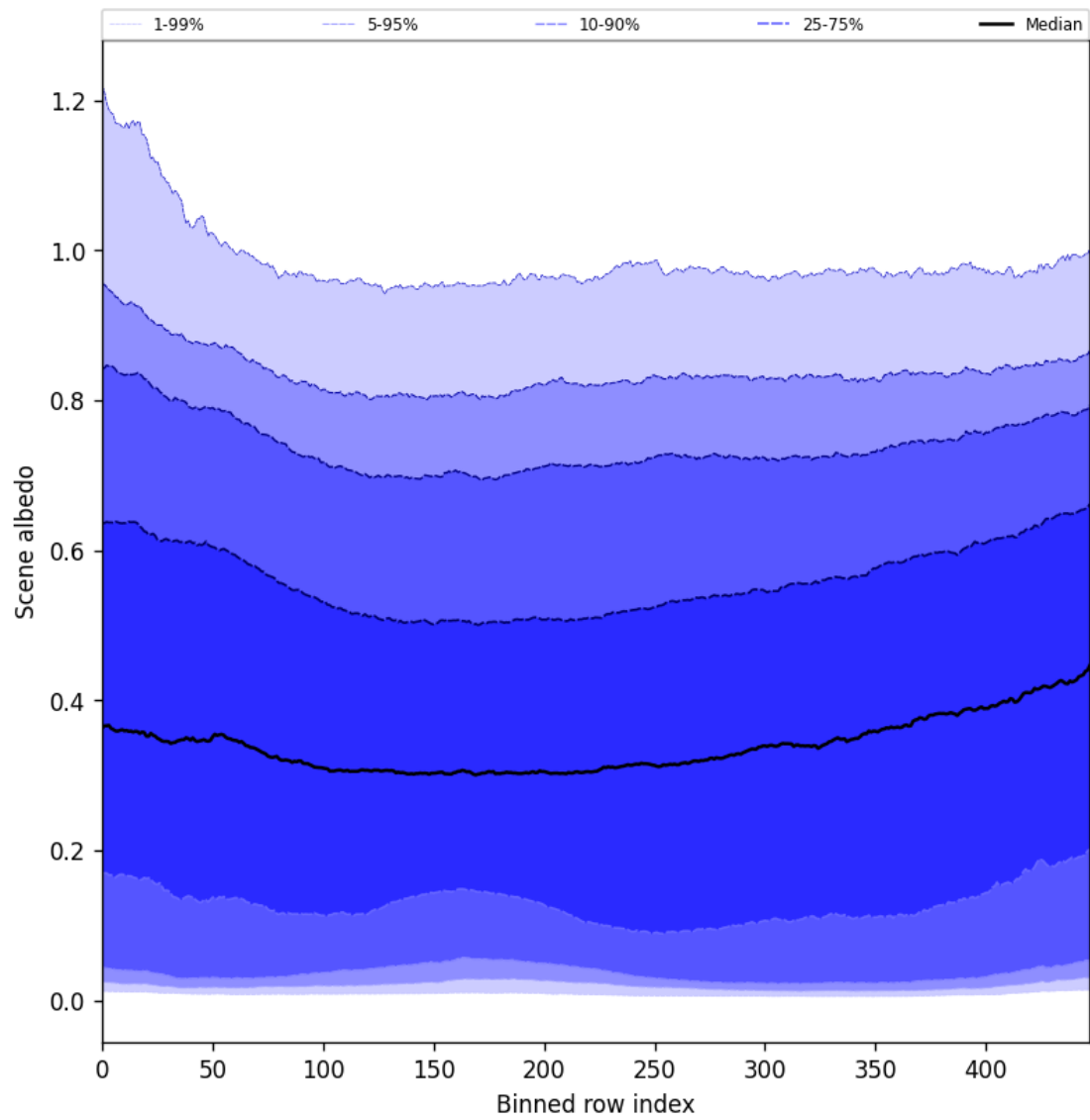
Figure 51: Along track statistics of “Scene albedo” for 2025-07-25 to 2025-07-27
