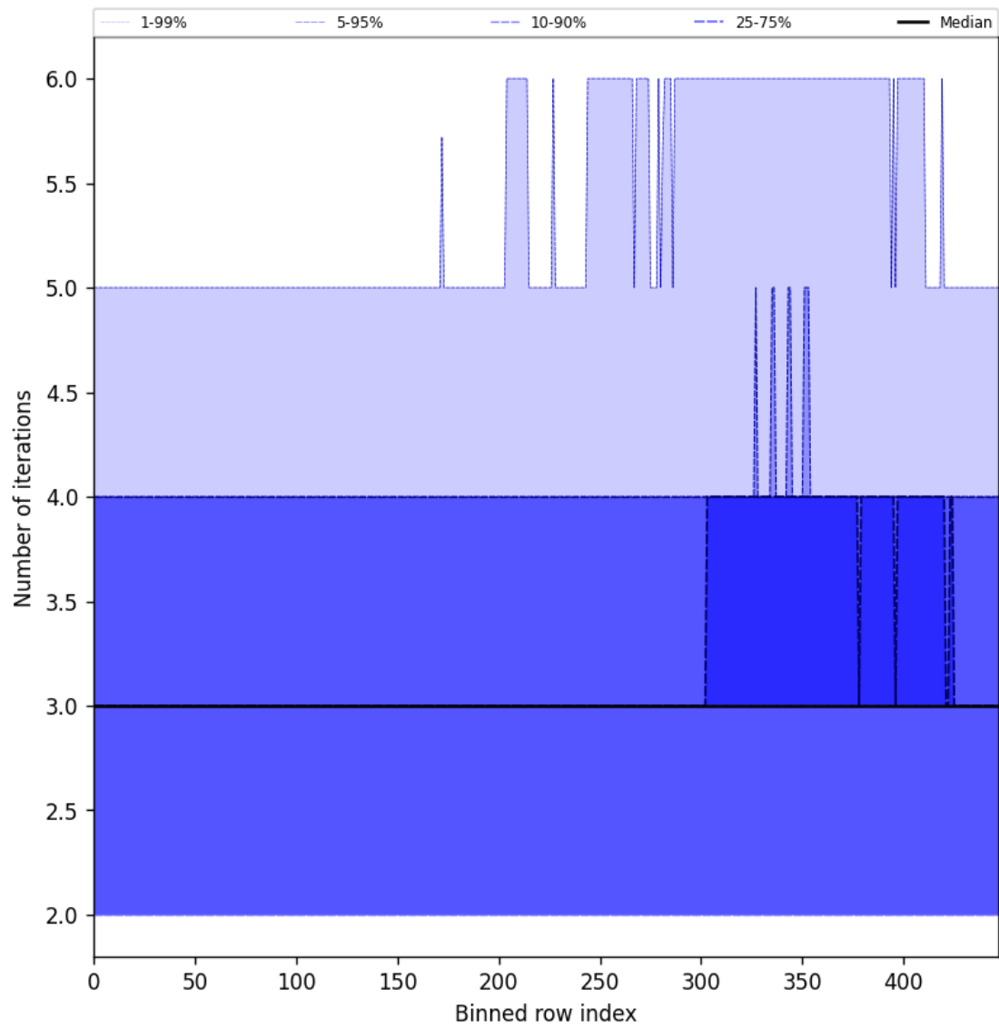
Figure 56: Along track statistics of “Number of iterations” for 2025-07-25 to 2025-07-27
