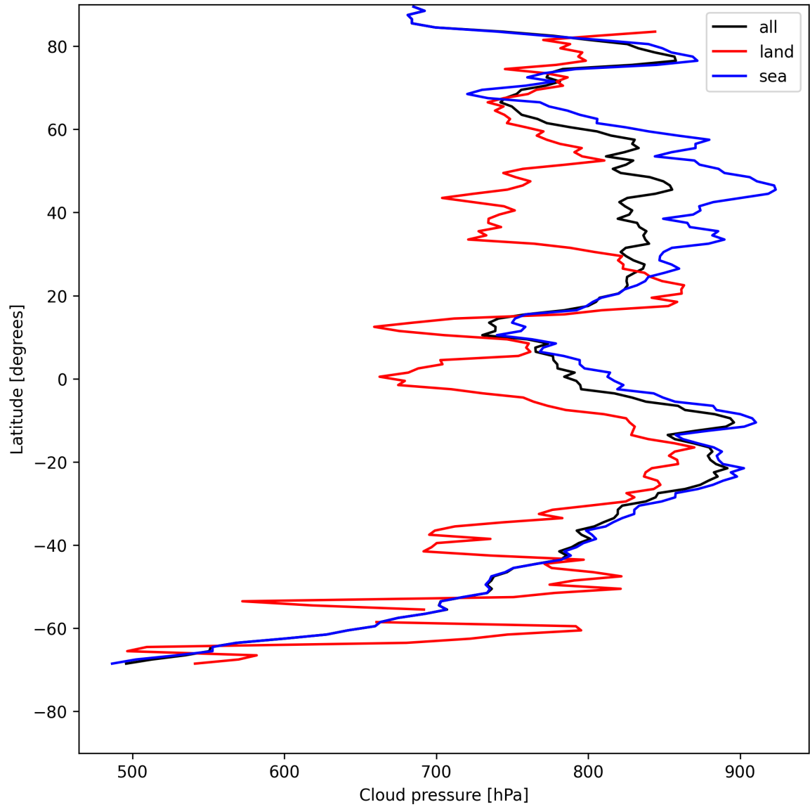
Figure 13: Zonal average of “Cloud pressure” for 2025-07-25 to 2025-07-27.
