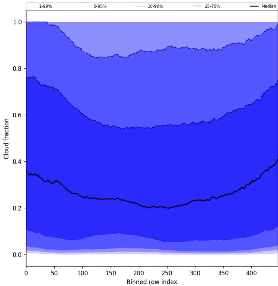
Figure 49: Along track statistics of “Cloud fraction” for 2025-07-25 to 2025-07-27
