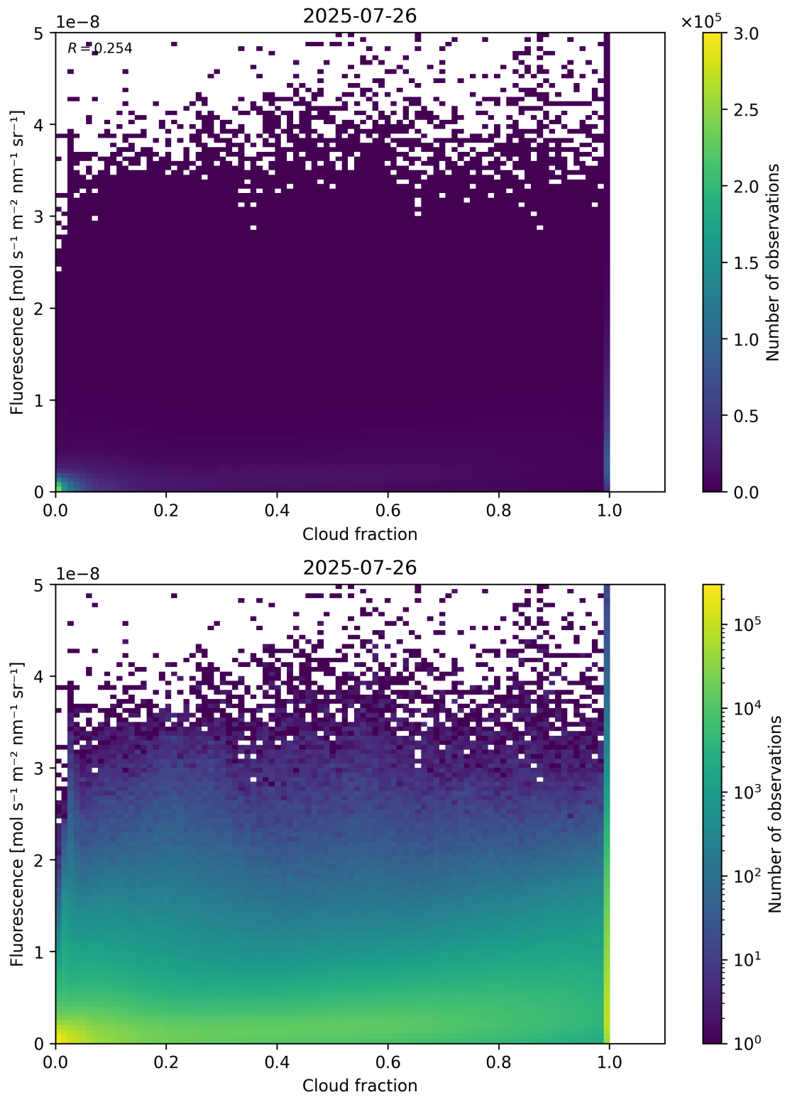
Figure 72: Scatter density plot of “Cloud fraction” against “Fluorescence” for 2025-07-25 to 2025-07-27.
