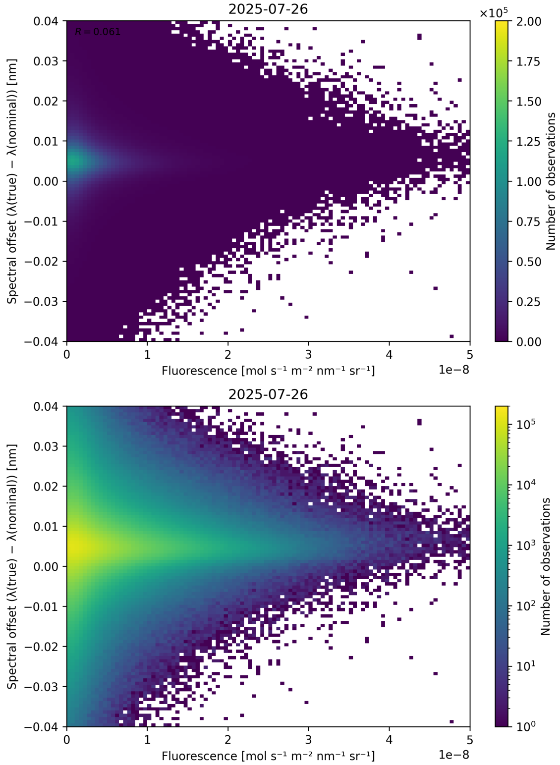
Figure 87: Scatter density plot of “Fluorescence” against “Spectral offset ( \lambda_{\text{true}} - \lambda_{\text{nominal}} )” for 2025-07-25 to 2025-07-27.
