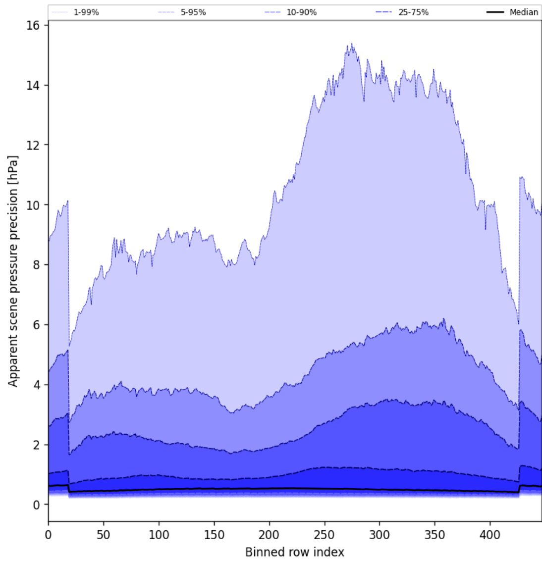
Figure 54: Along track statistics of “Apparent scene pressure precision” for 2025-07-25 to 2025-07-27
