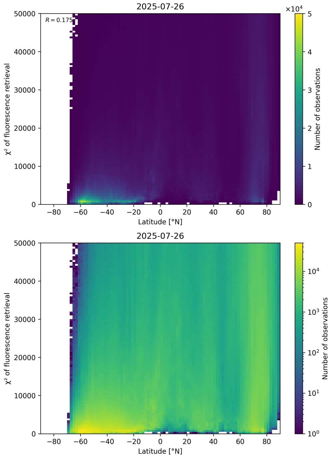
Figure 89: Scatter density plot of “Latitude” against “ \chi^2 of fluorescence retrieval” for 2025-07-25 to 2025-07-27.
