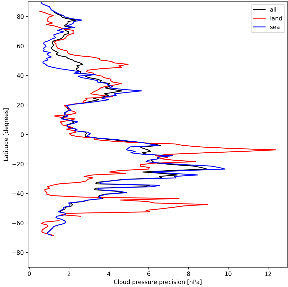
Figure 14: Zonal average of "Cloud pressure precision" for 2025-07-25 to 2025-07-27.
