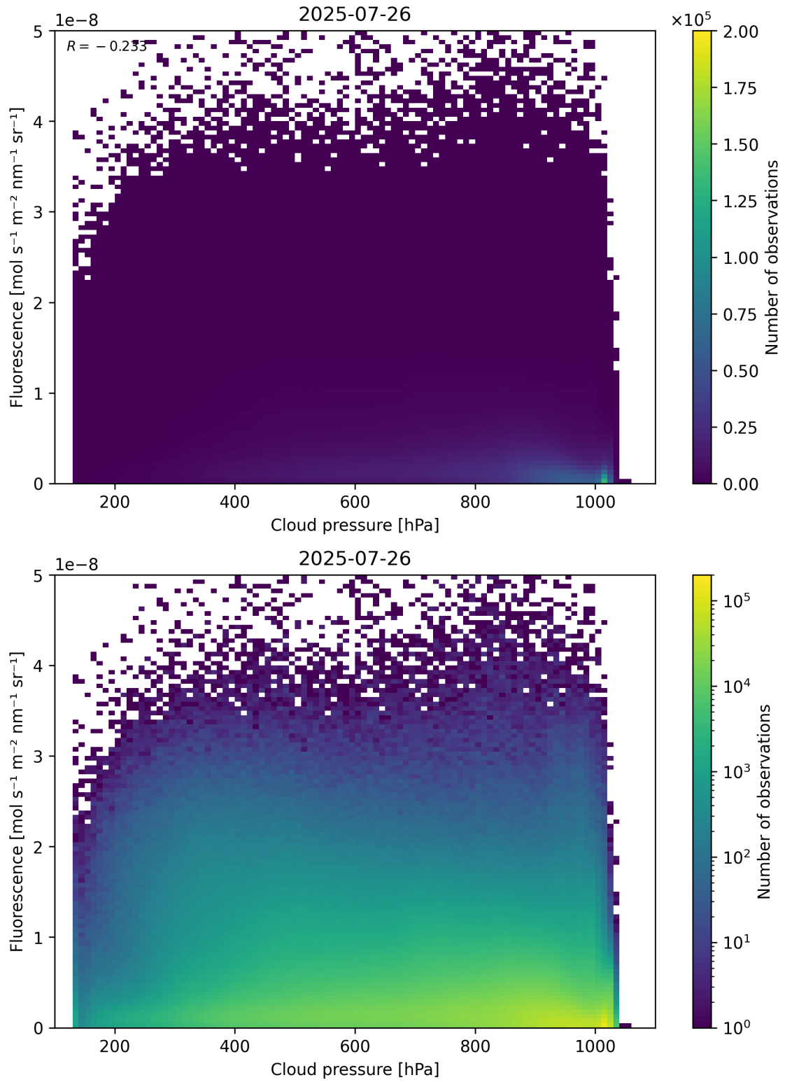
Figure 80: Scatter density plot of “Cloud pressure” against “Fluorescence” for 2025-07-25 to 2025-07-27.
