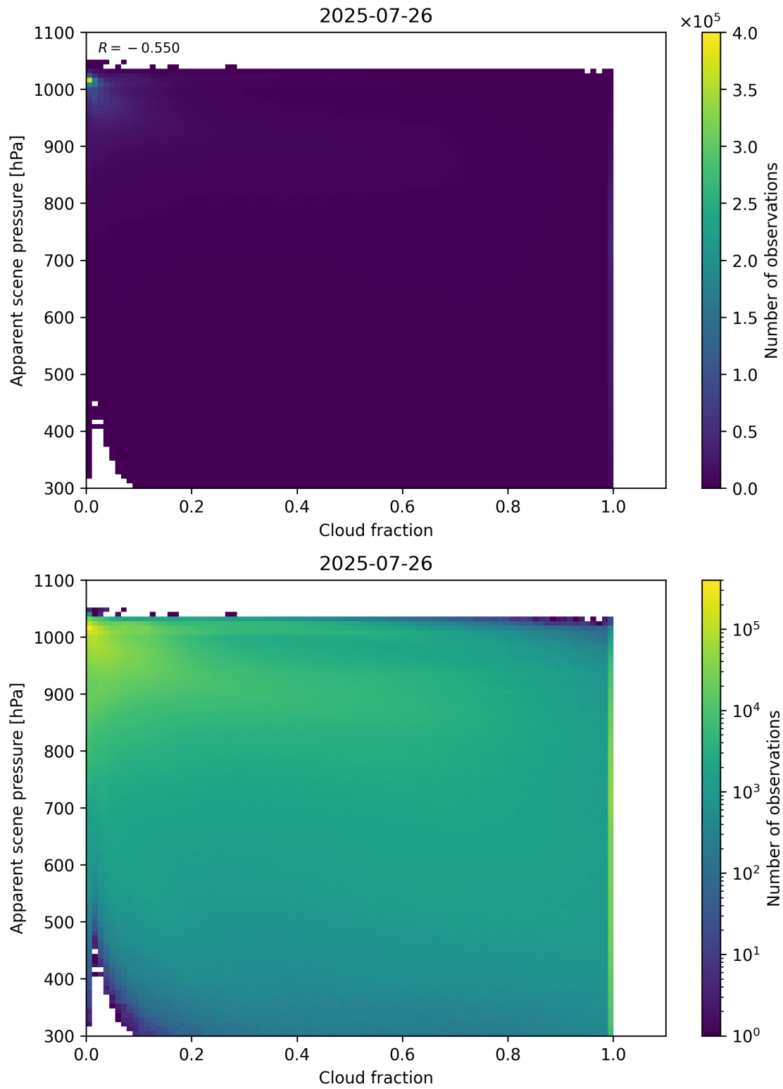
Figure 70: Scatter density plot of “Cloud fraction” against “Apparent scene pressure” for 2025-07-25 to 2025-07-27.
