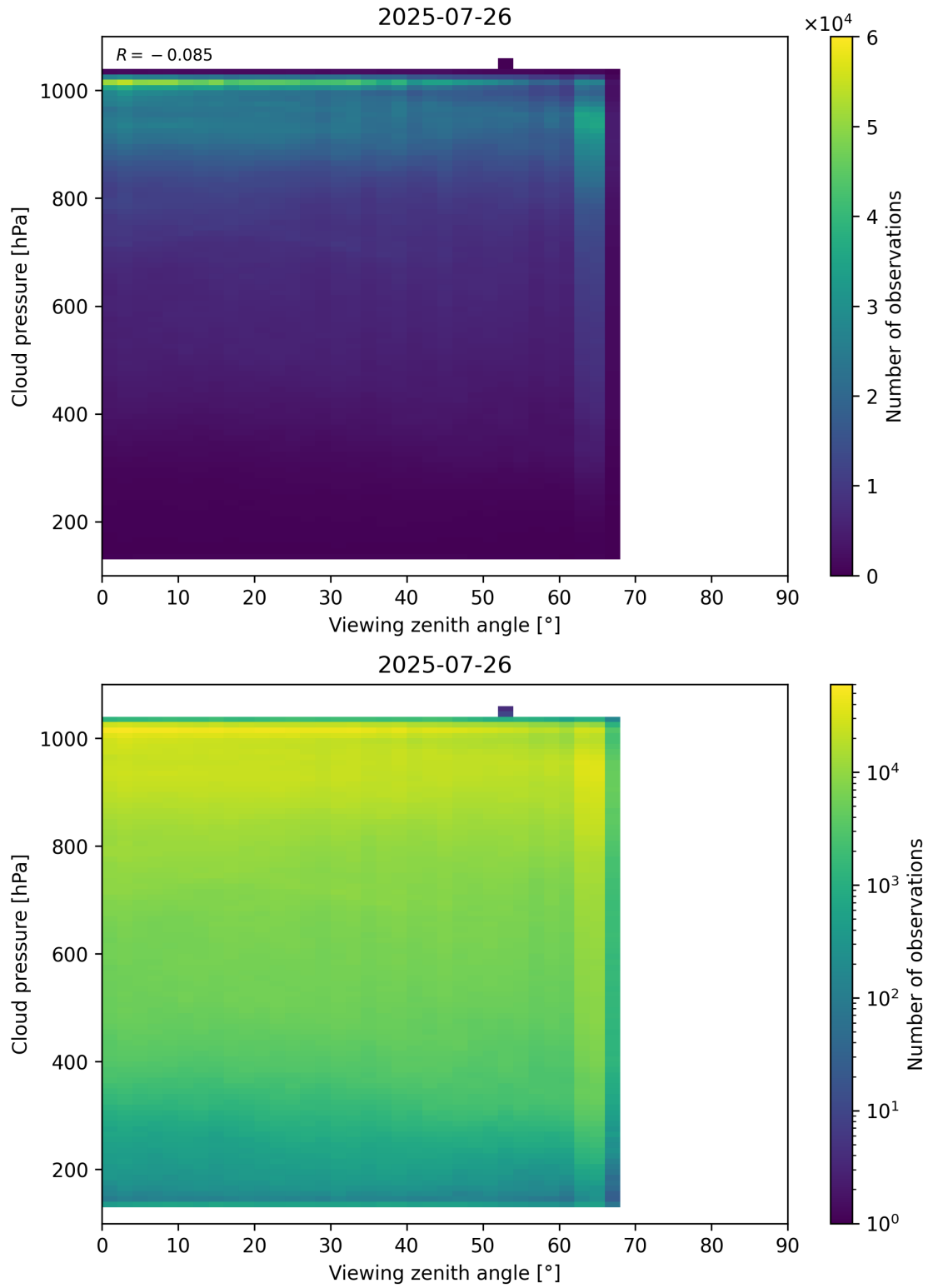
Figure 121: Scatter density plot of “Viewing zenith angle” against “Cloud pressure” for 2025-07-25 to 2025-07-27.
