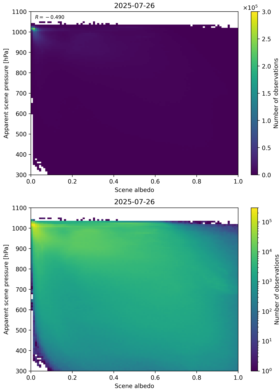
Figure 102: Scatter density plot of “Scene albedo” against “Apparent scene pressure” for 2025-07-25 to 2025-07-27.
