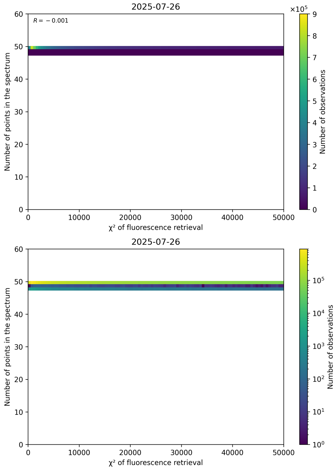
Figure 68: Scatter density plot of “ \chi^2 of fluorescence retrieval” against “Number of points in the spectrum” for 2025-07-25 to 2025-07-27.
