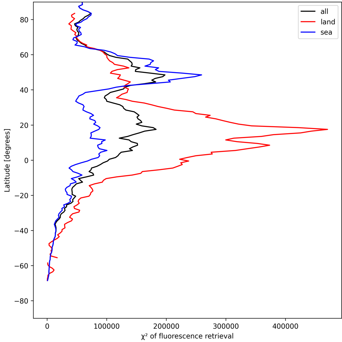
Figure 25: Zonal average of “ \chi^2 of fluorescence retrieval” for 2025-07-25 to 2025-07-27.
