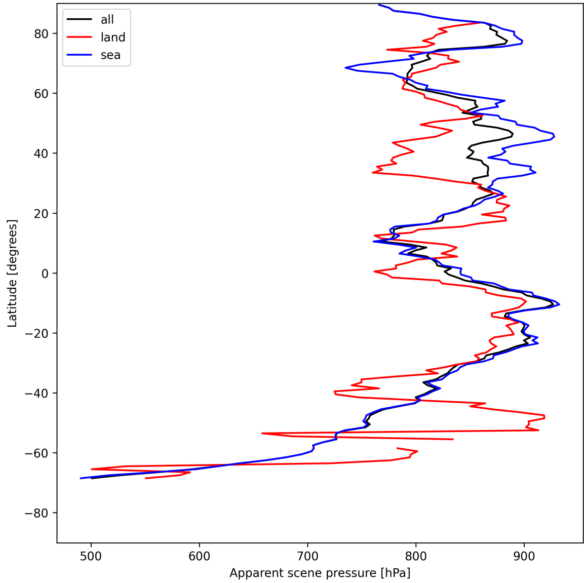
Figure 19: Zonal average of “Apparent scene pressure” for 2025-07-25 to 2025-07-27.
