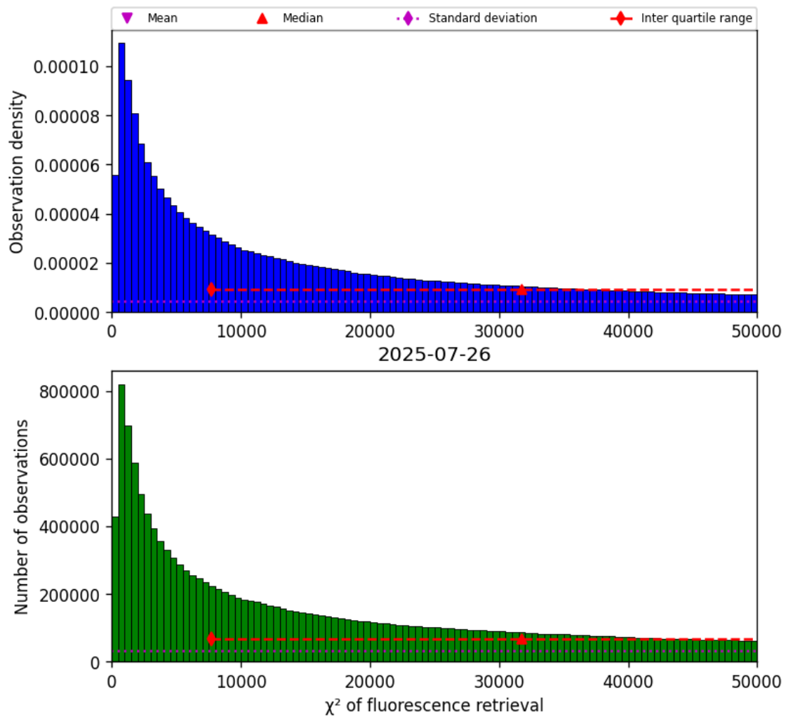
Figure 42: Histogram of “ \chi^2 of fluorescence retrieval” for 2025-07-25 to 2025-07-27
