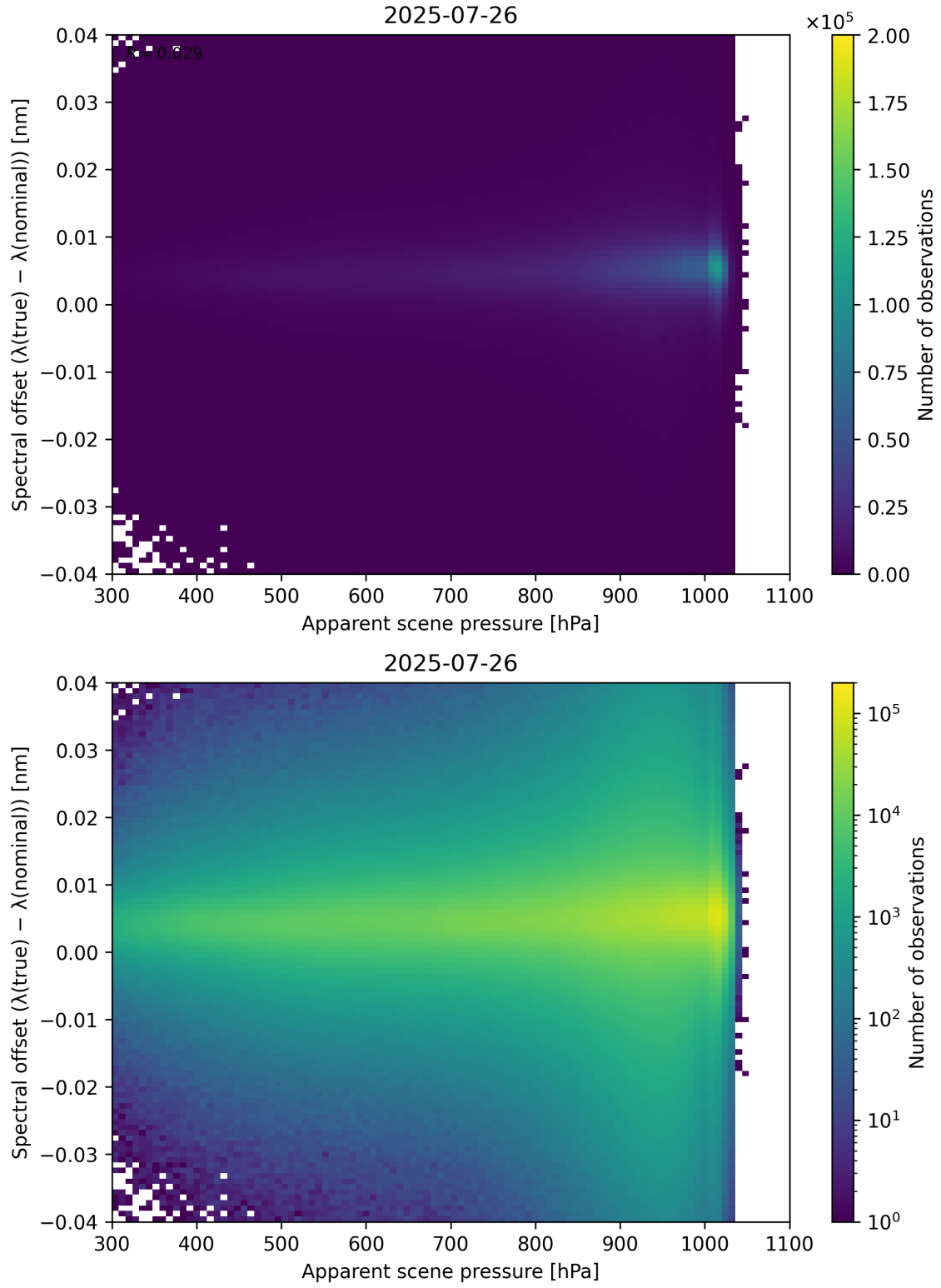
Figure 67: Scatter density plot of “Apparent scene pressure” against “Spectral offset ( \lambda_{\text{true}} - \lambda_{\text{nominal}} )” for 2025-07-25 to 2025-07-27.
