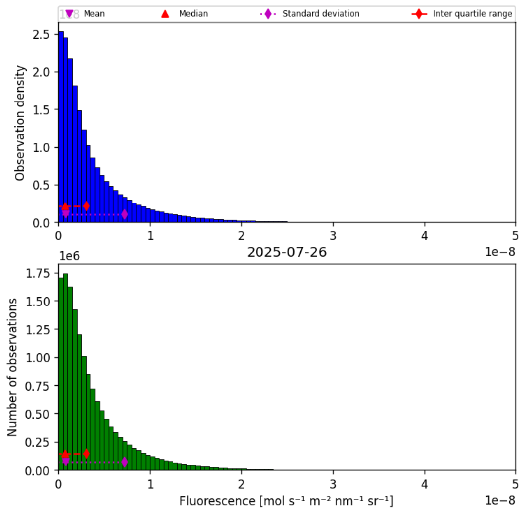
Figure 40: Histogram of “Fluorescence” for 2025-07-25 to 2025-07-27
