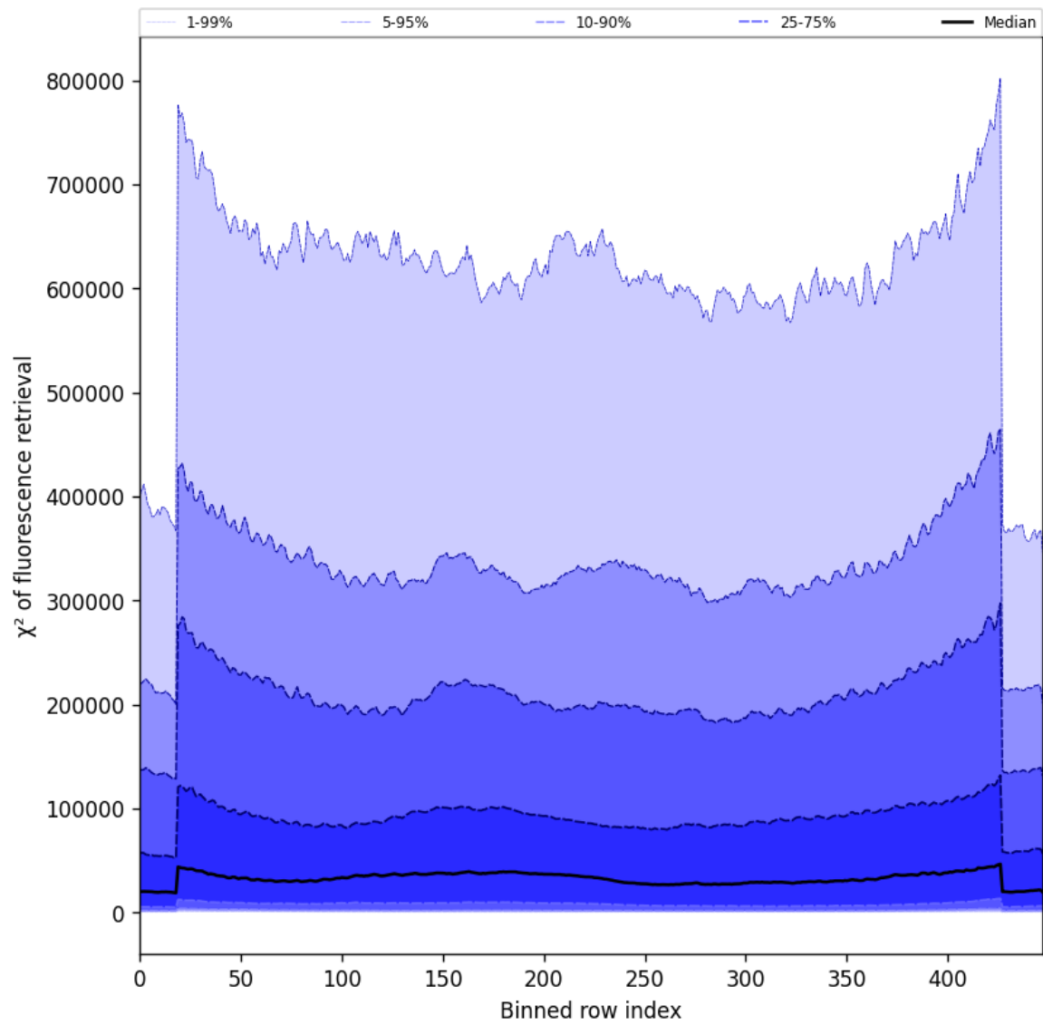
Figure 59: Along track statistics of “ \chi^2 of fluorescence retrieval” for 2025-07-25 to 2025-07-27
