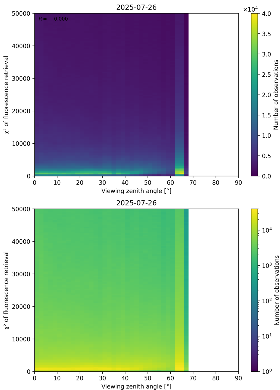
Figure 119: Scatter density plot of “Viewing zenith angle” against “ \chi^2 of fluorescence retrieval” for 2025-07-25 to 2025-07-27.
