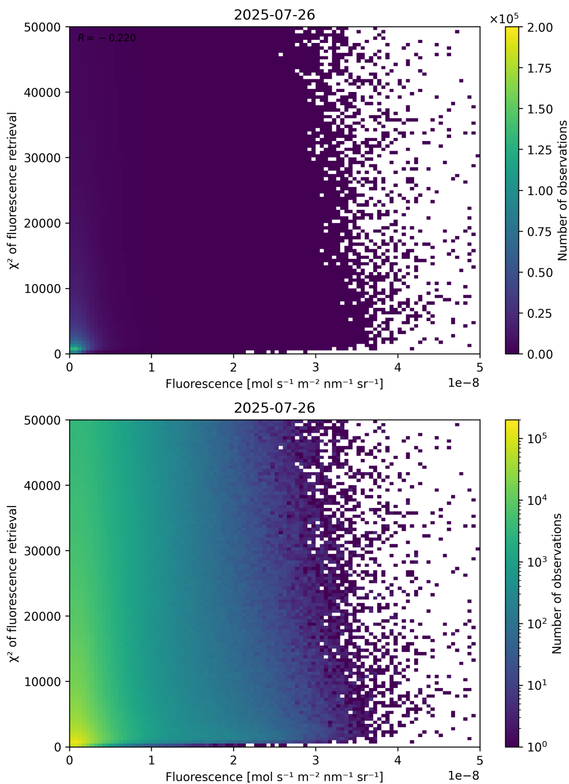
Figure 85: Scatter density plot of “Fluorescence” against “ \chi^2 of fluorescence retrieval” for 2025-07-25 to 2025-07-27.
