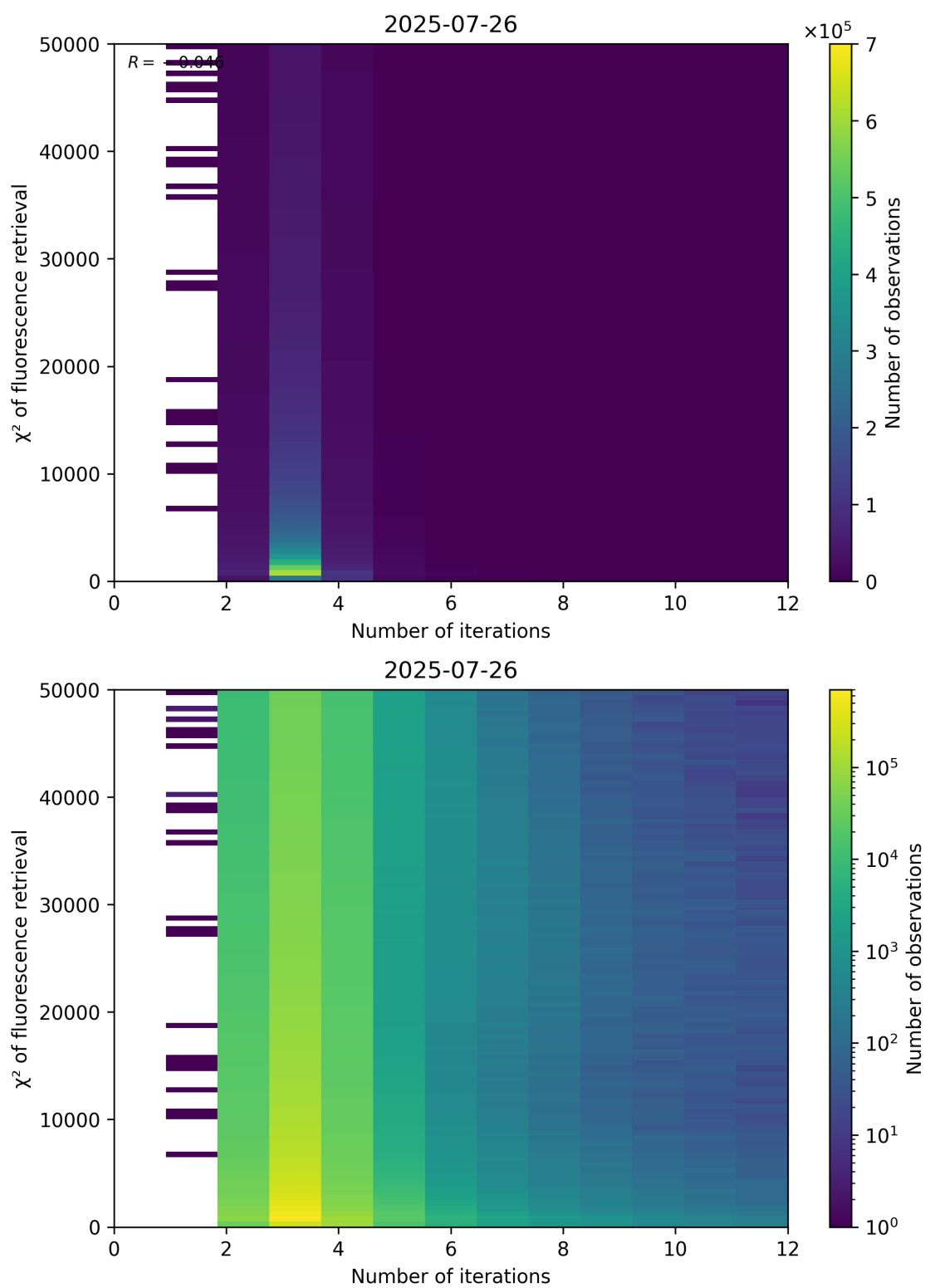
Figure 97: Scatter density plot of “Number of iterations” against “ \chi^2 of fluorescence retrieval” for 2025-07-25 to 2025-07-27.
