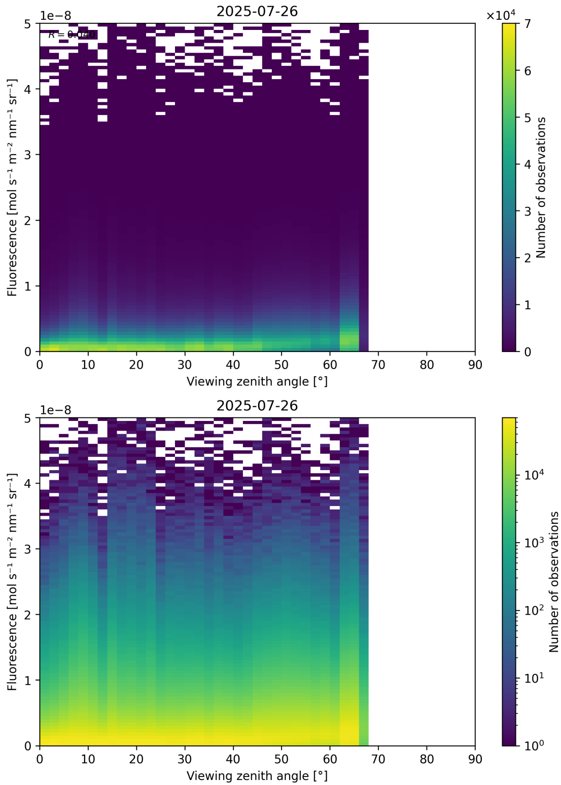
Figure 122: Scatter density plot of “Viewing zenith angle” against “Fluorescence” for 2025-07-25 to 2025-07-27.
