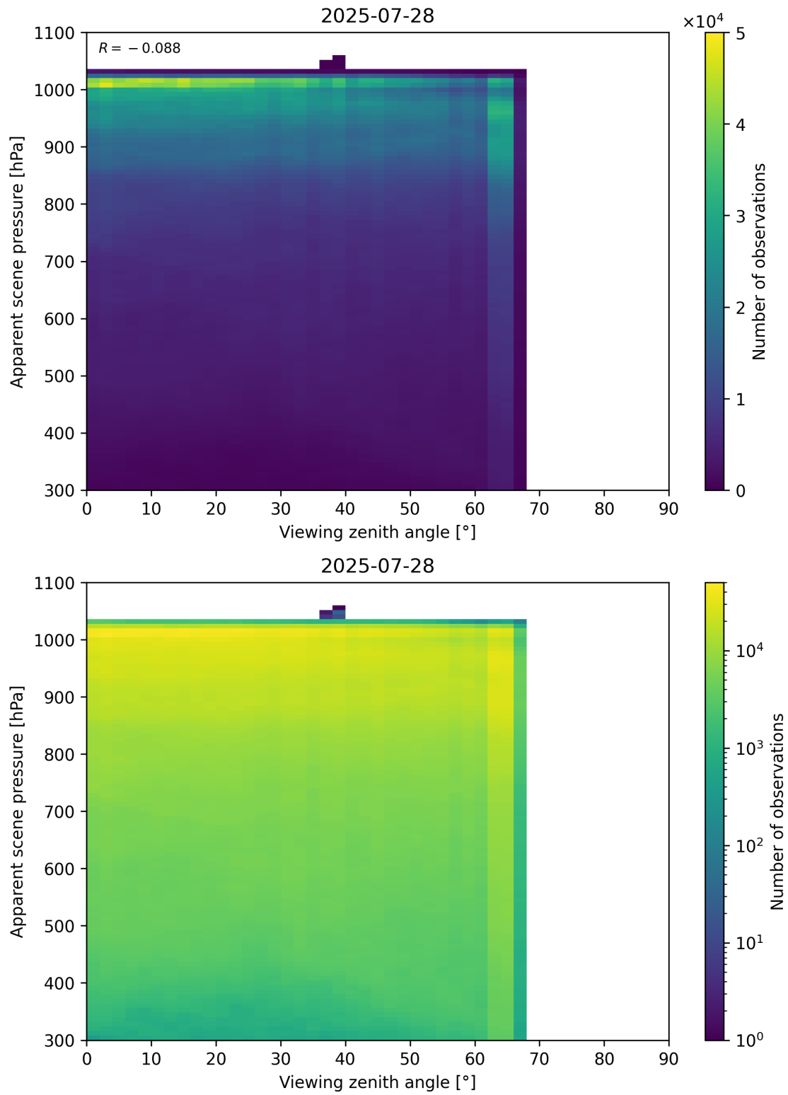
Figure 118: Scatter density plot of “Viewing zenith angle” against “Apparent scene pressure” for 2025-07-27 to 2025-07-29.
