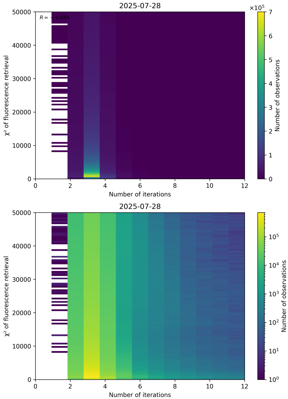
Figure 97: Scatter density plot of “Number of iterations” against “ \chi^2 of fluorescence retrieval” for 2025-07-27 to 2025-07-29.
