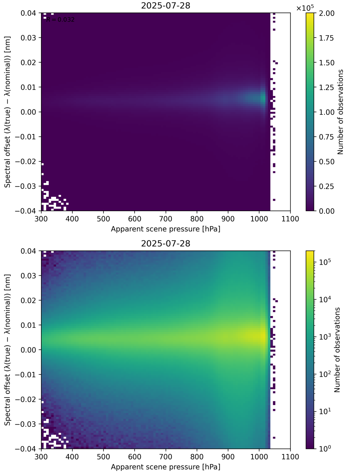
Figure 67: Scatter density plot of “Apparent scene pressure” against “Spectral offset ( \lambda_{\text{true}} - \lambda_{\text{nominal}} )” for 2025-07-27 to 2025-07-29.
