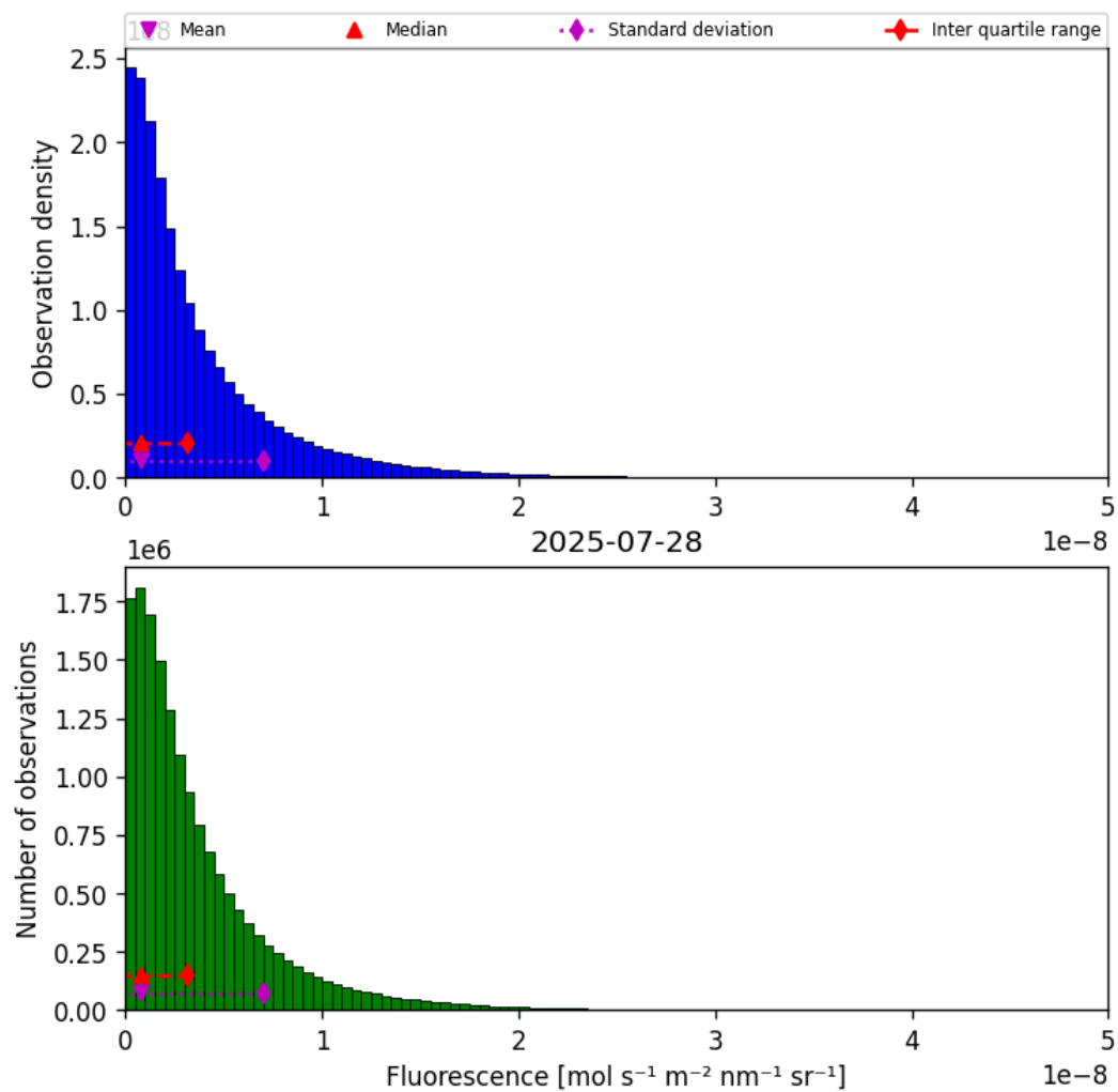
Figure 40: Histogram of “Fluorescence” for 2025-07-27 to 2025-07-29
