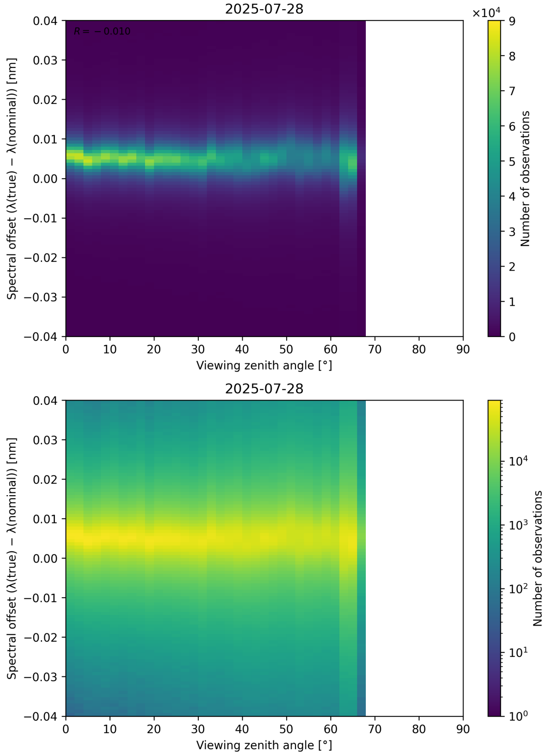
Figure 128: Scatter density plot of “Viewing zenith angle” against “Spectral offset ( \lambda_{\text{true}} - \lambda_{\text{nominal}} )” for 2025-07-27 to 2025-07-29.
