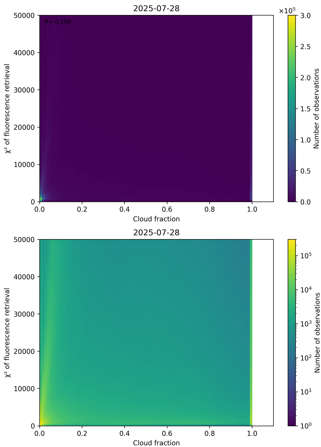
Figure 71: Scatter density plot of “Cloud fraction” against “ \chi^2 of fluorescence retrieval” for 2025-07-27 to 2025-07-29.
