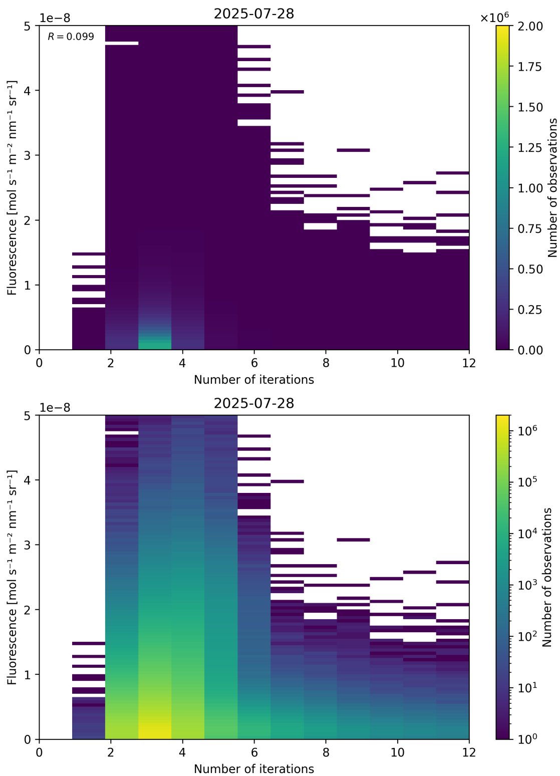
Figure 98: Scatter density plot of “Number of iterations” against “Fluorescence” for 2025-07-27 to 2025-07-29.
