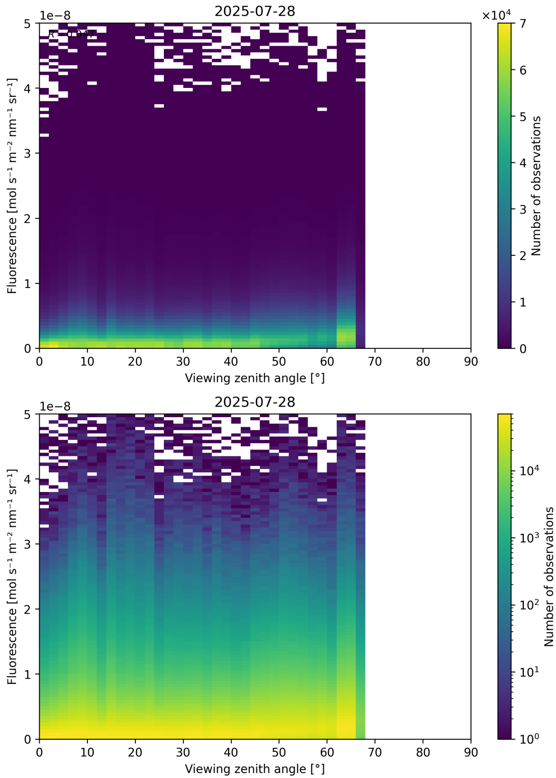
Figure 122: Scatter density plot of "Viewing zenith angle" against "Fluorescence" for 2025-07-27 to 2025-07-29.
