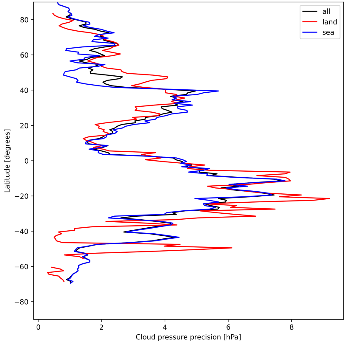
Figure 14: Zonal average of “Cloud pressure precision” for 2025-07-27 to 2025-07-29.
