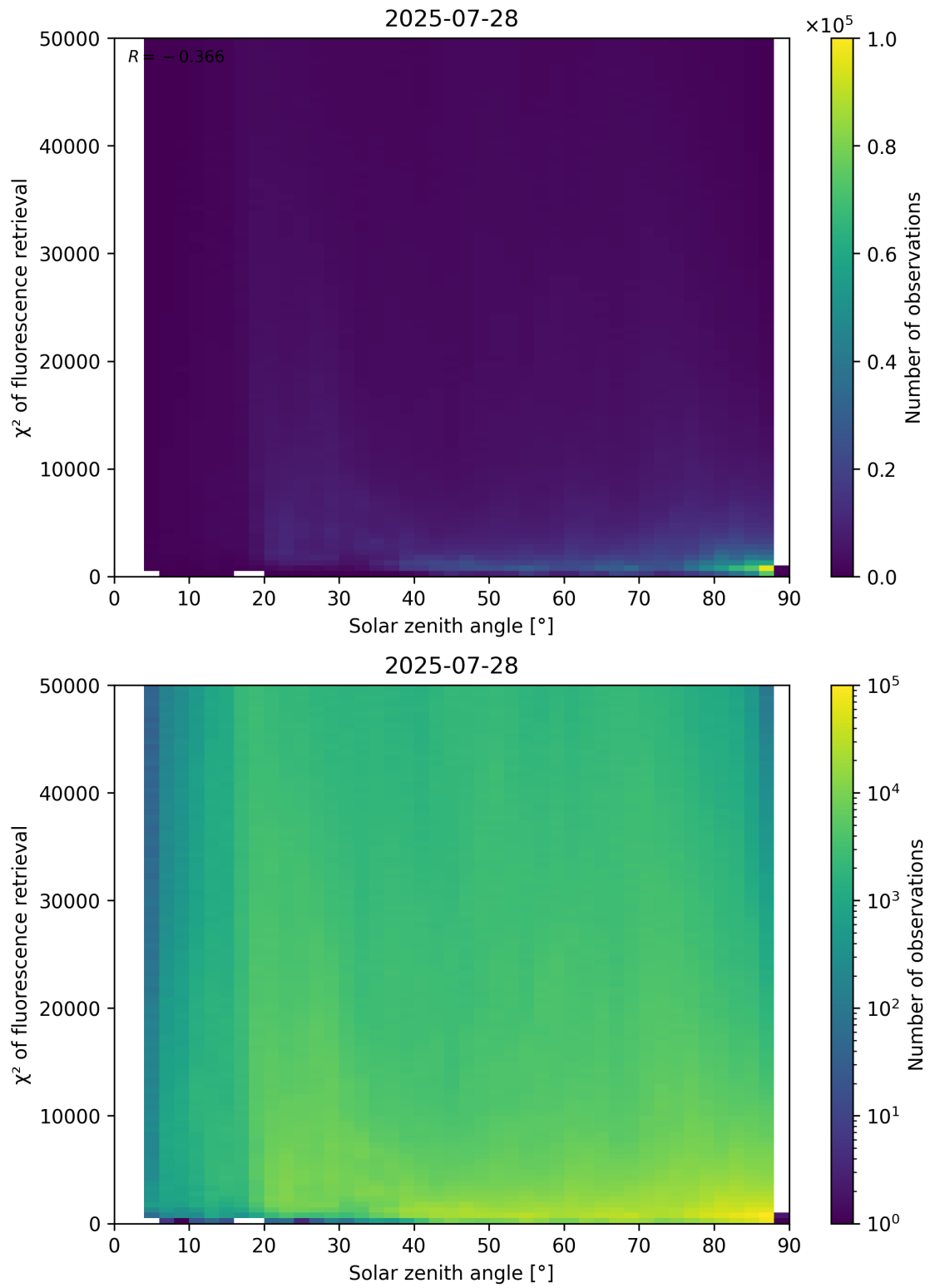
Figure 109: Scatter density plot of “Solar zenith angle” against “ \chi^2 of fluorescence retrieval” for 2025-07-27 to 2025-07-29.
