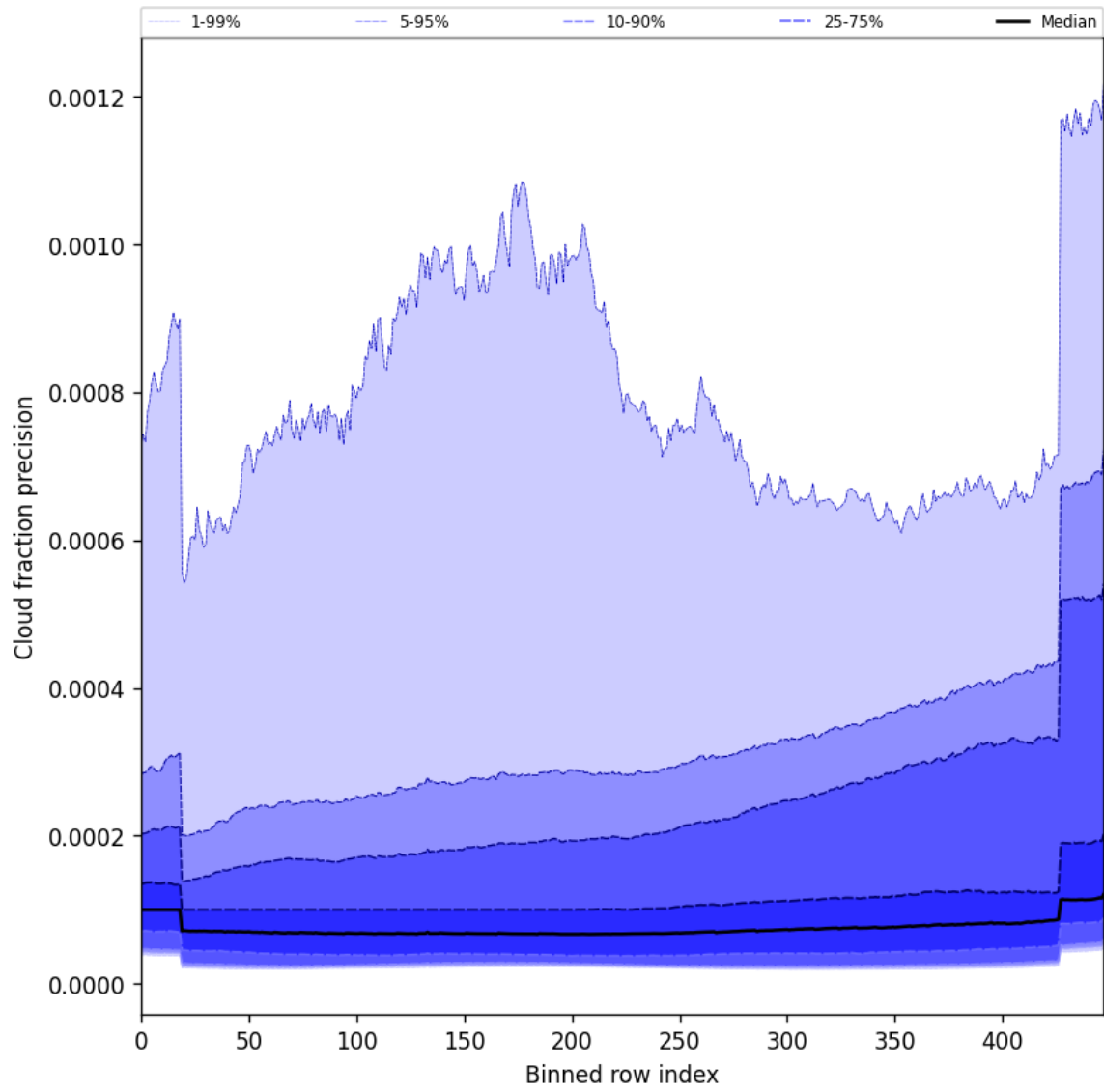
Figure 50: Along track statistics of “Cloud fraction precision” for 2025-07-27 to 2025-07-29
