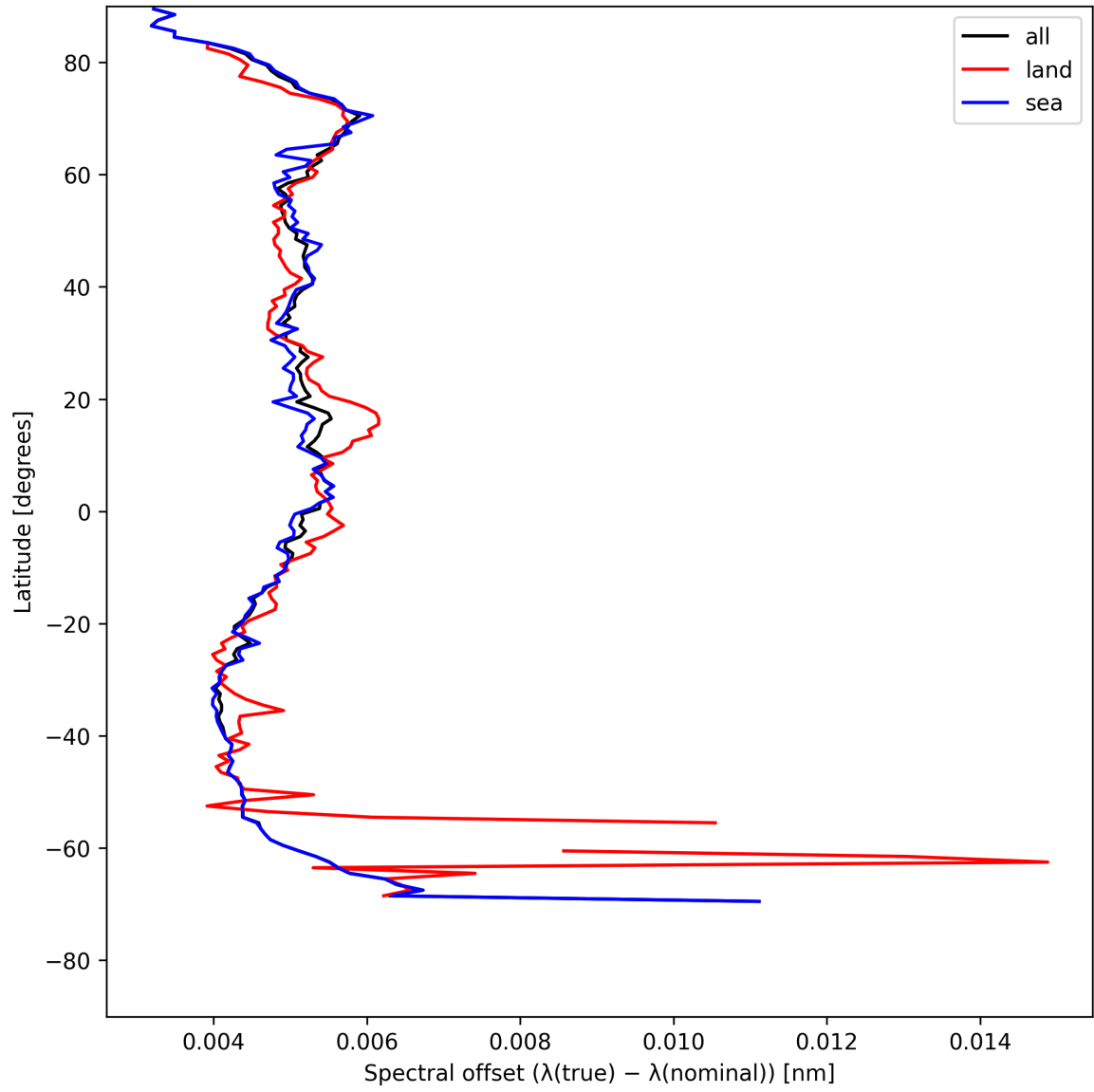
Figure 28: Zonal average of “Spectral offset ( \lambda_{\text{true}} - \lambda_{\text{nominal}} )” for 2025-07-27 to 2025-07-29.
