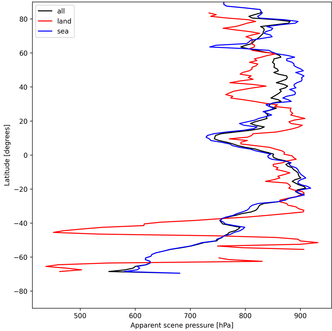
Figure 19: Zonal average of “Apparent scene pressure” for 2025-07-27 to 2025-07-29.
