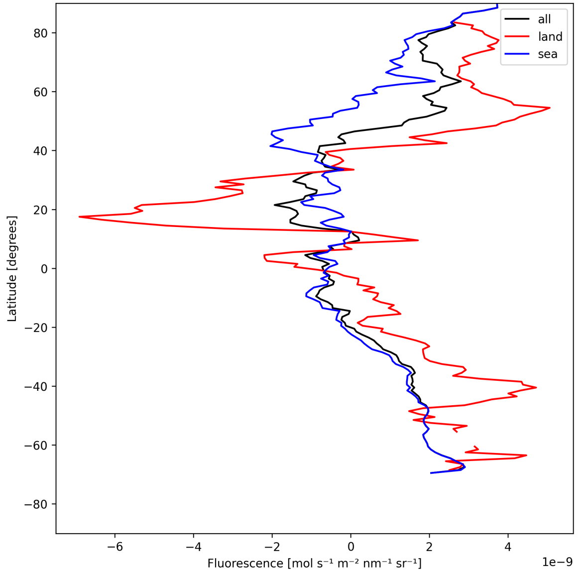
Figure 23: Zonal average of “Fluorescence” for 2025-07-27 to 2025-07-29.
