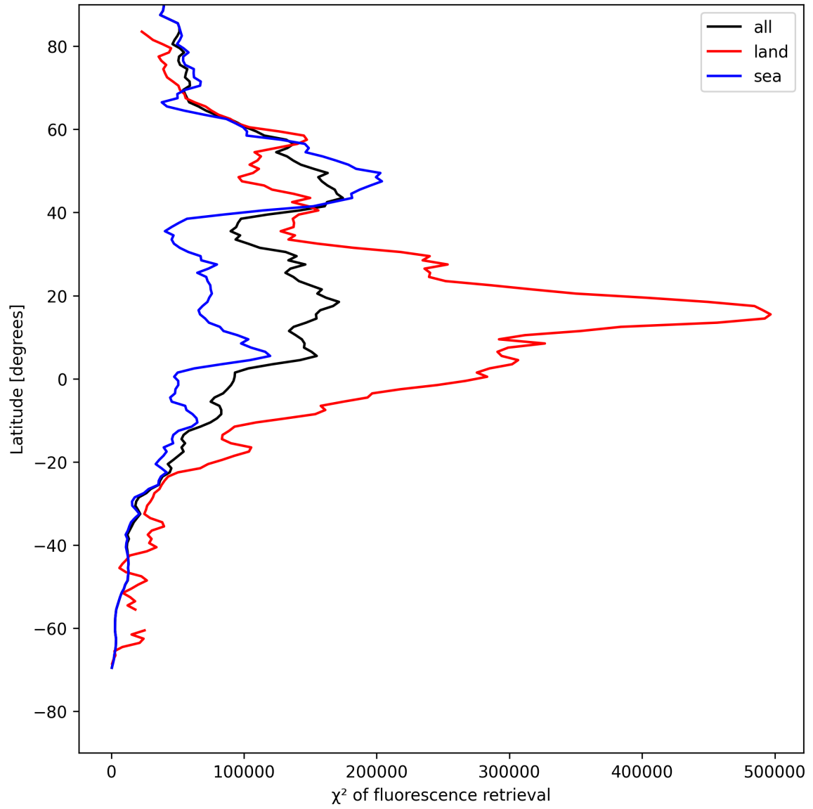
Figure 25: Zonal average of “ \chi^2 of fluorescence retrieval” for 2025-07-27 to 2025-07-29.
