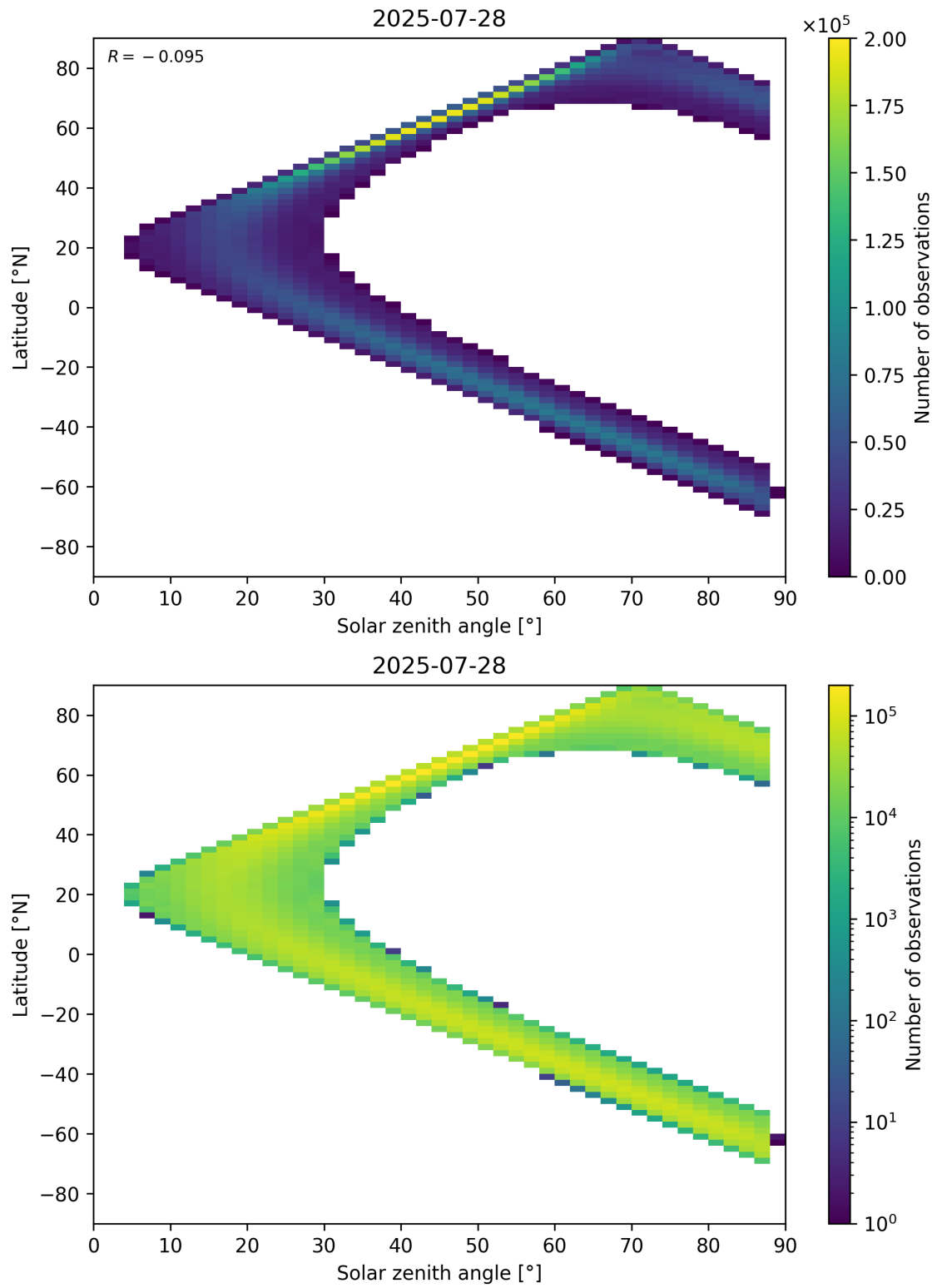
Figure 113: Scatter density plot of “Solar zenith angle” against “Latitude” for 2025-07-27 to 2025-07-29.
