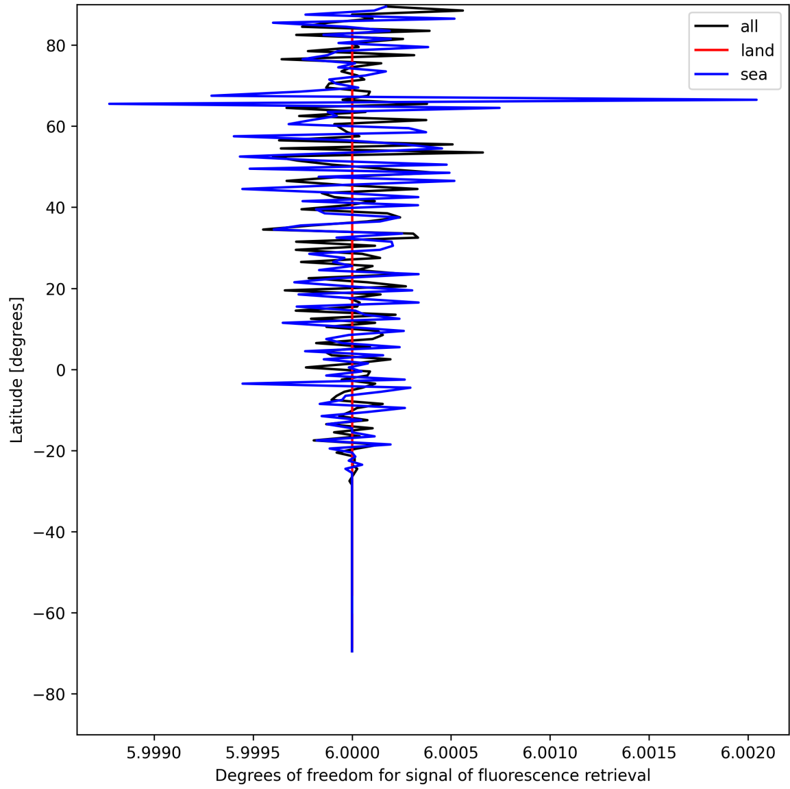
Figure 26: Zonal average of “Degrees of freedom for signal of fluorescence retrieval” for 2025-07-27 to 2025-07-29.
