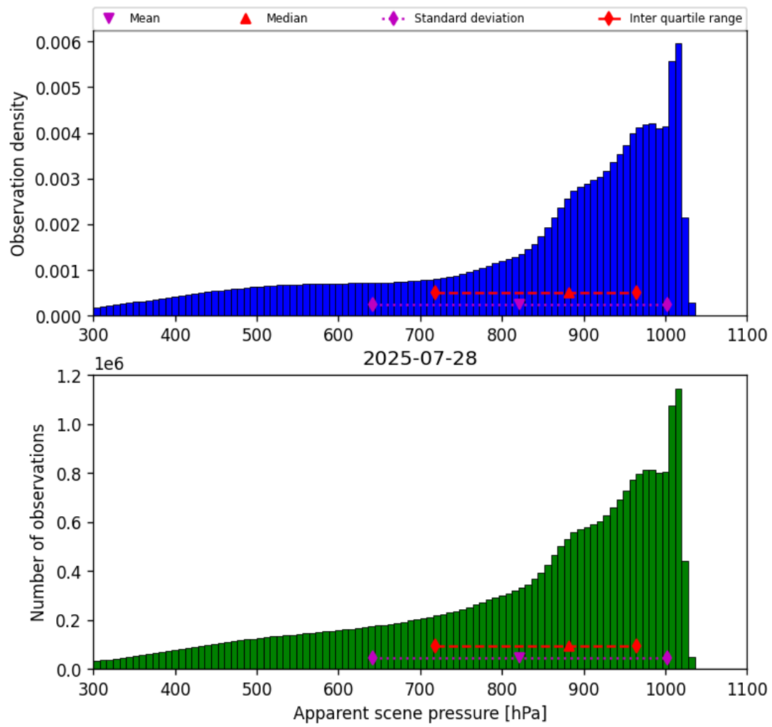
Figure 36: Histogram of “Apparent scene pressure” for 2025-07-27 to 2025-07-29
