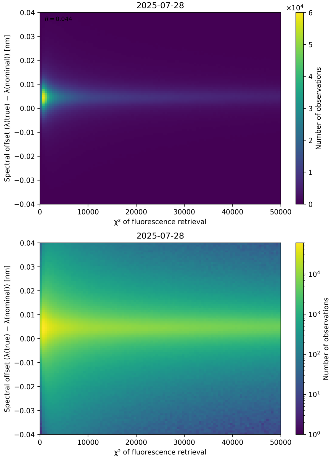
Figure 69: Scatter density plot of “ \chi^2 of fluorescence retrieval” against “Spectral offset ( \lambda_{\text{true}} - \lambda_{\text{nominal}} )” for 2025-07-27 to 2025-07-29.
