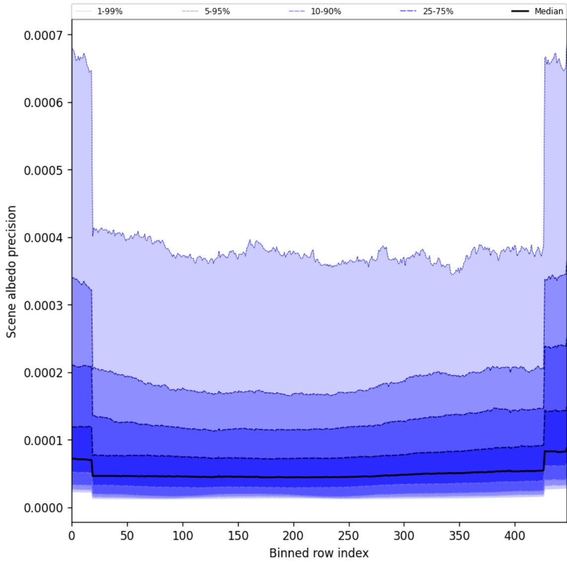
Figure 52: Along track statistics of “Scene albedo precision” for 2025-07-27 to 2025-07-29
