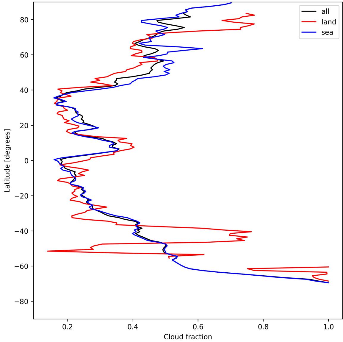
Figure 15: Zonal average of “Cloud fraction” for 2025-07-27 to 2025-07-29.
