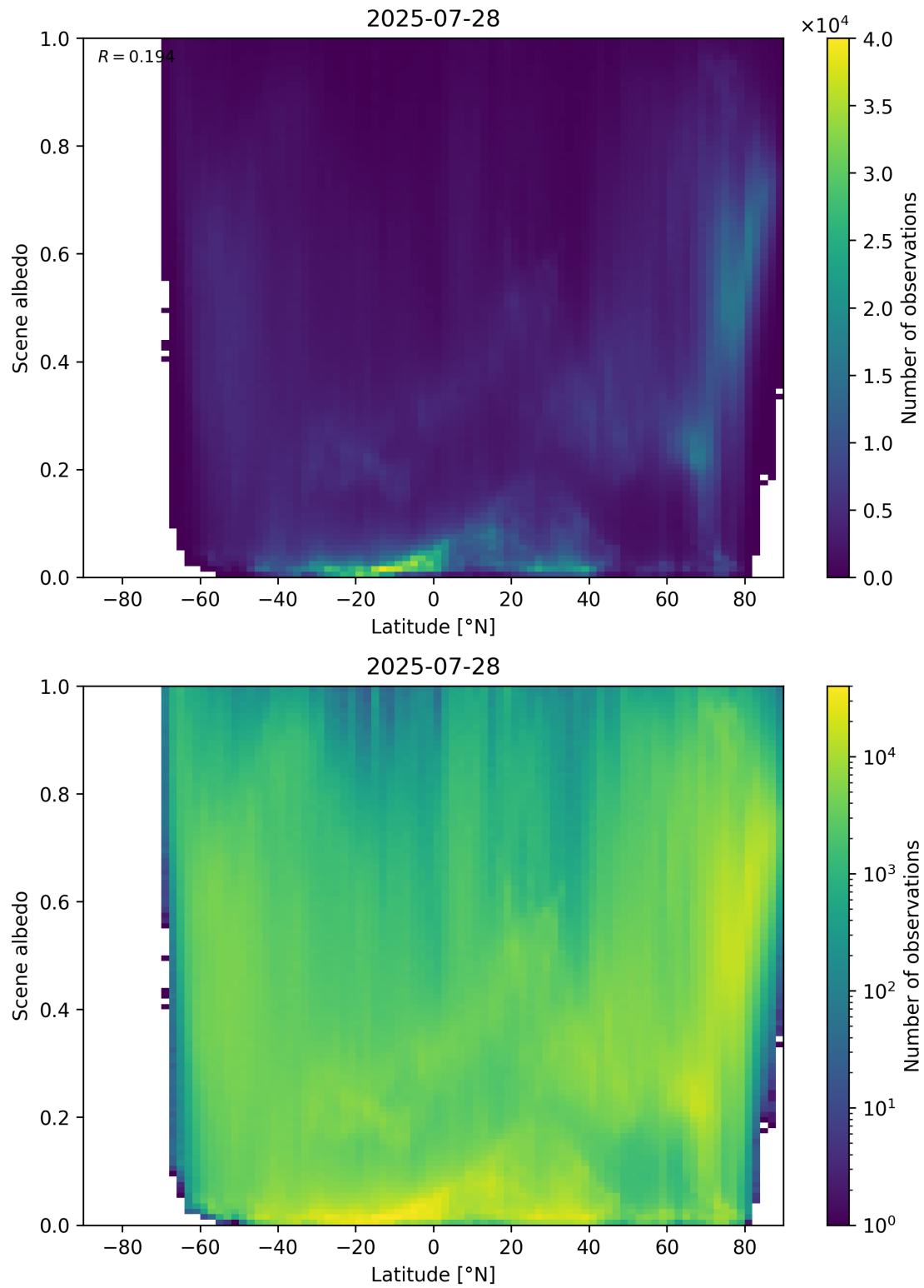
Figure 95: Scatter density plot of “Latitude” against “Scene albedo” for 2025-07-27 to 2025-07-29.
