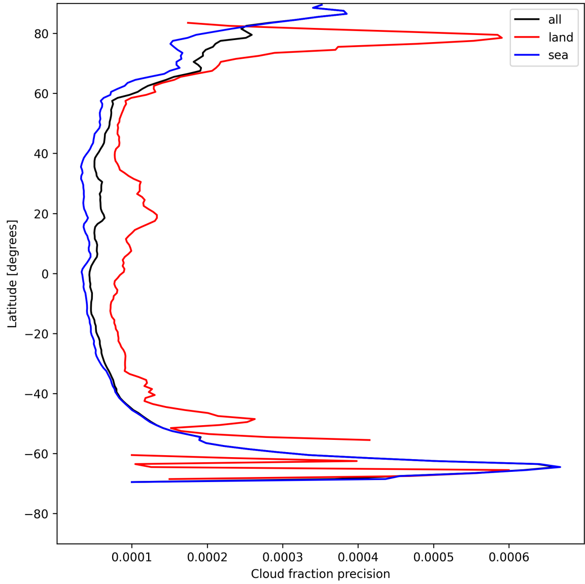
Figure 16: Zonal average of “Cloud fraction precision” for 2025-07-27 to 2025-07-29.
