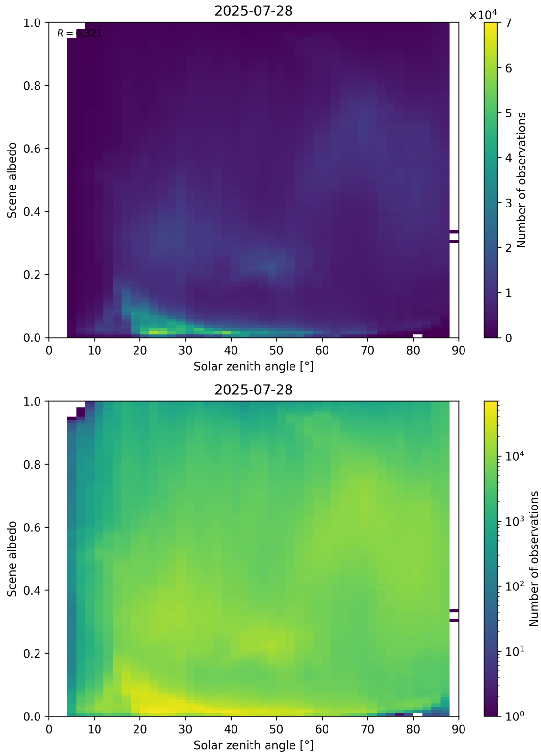
Figure 116: Scatter density plot of “Solar zenith angle” against “Scene albedo” for 2025-07-27 to 2025-07-29.
