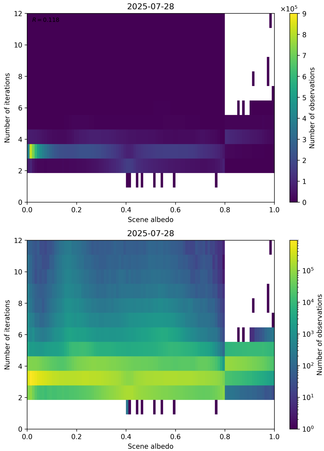
Figure 105: Scatter density plot of “Scene albedo” against “Number of iterations” for 2025-07-27 to 2025-07-29.
