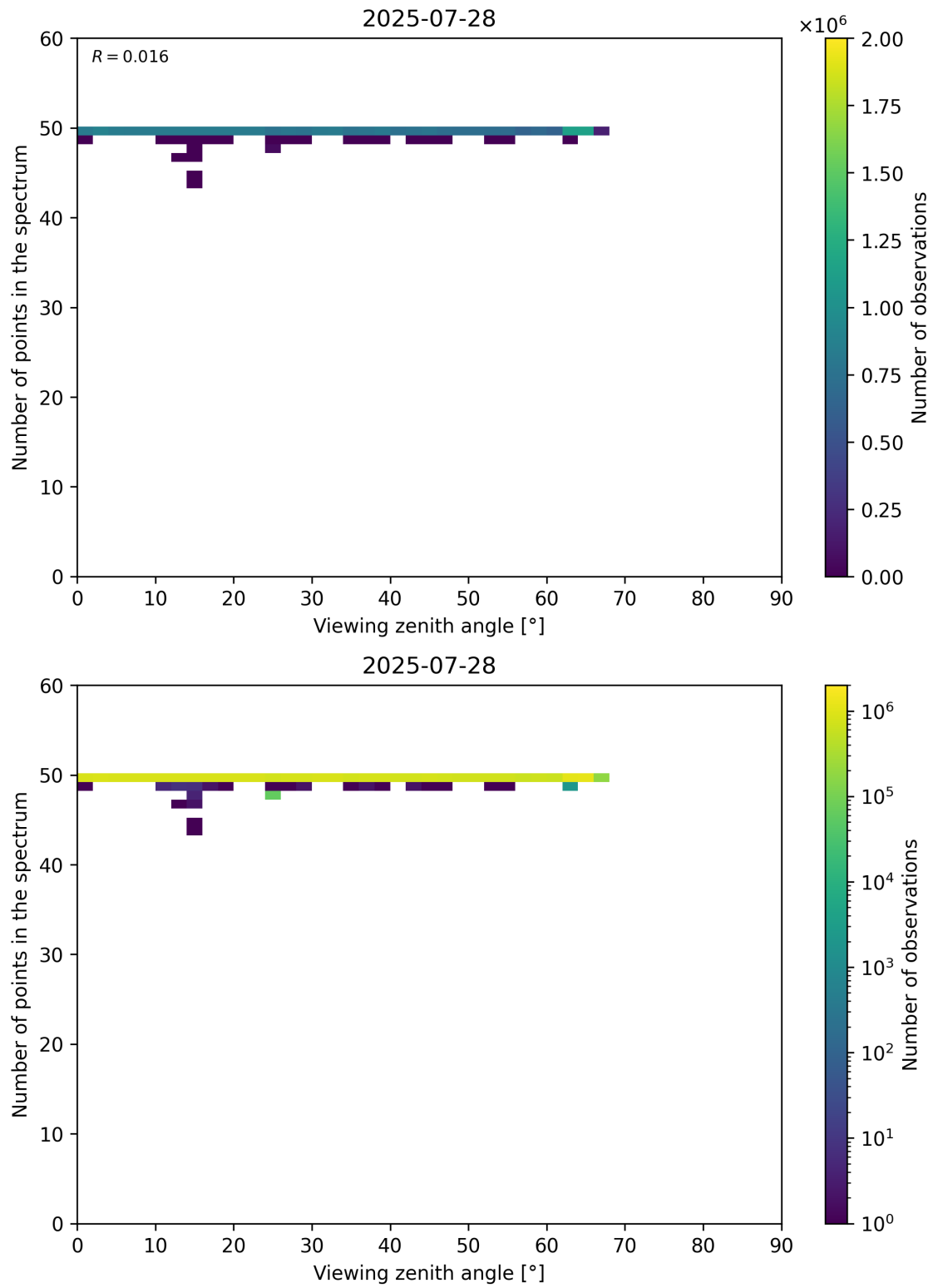
Figure 125: Scatter density plot of “Viewing zenith angle” against “Number of points in the spectrum” for 2025-07-27 to 2025-07-29.
