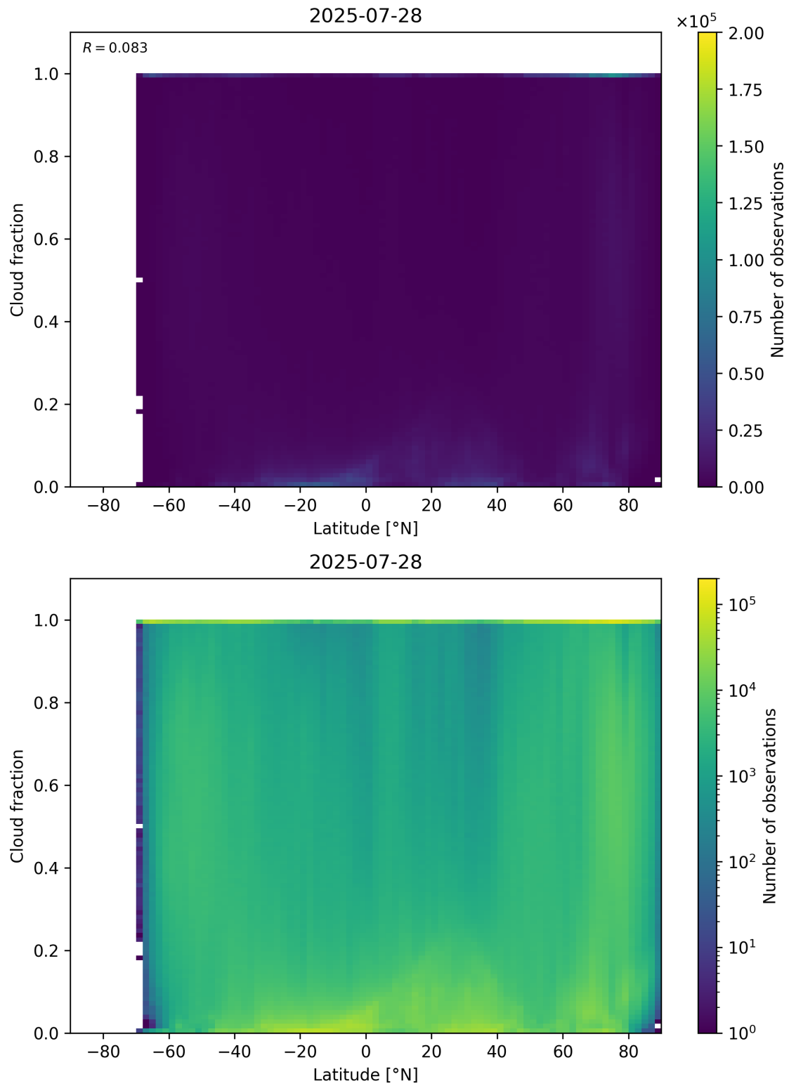
Figure 90: Scatter density plot of “Latitude” against “Cloud fraction” for 2025-07-27 to 2025-07-29.
