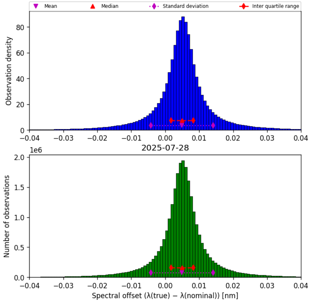
Figure 45: Histogram of “Spectral offset ( \lambda_{\text{true}} - \lambda_{\text{nominal}} )” for 2025-07-27 to 2025-07-29
