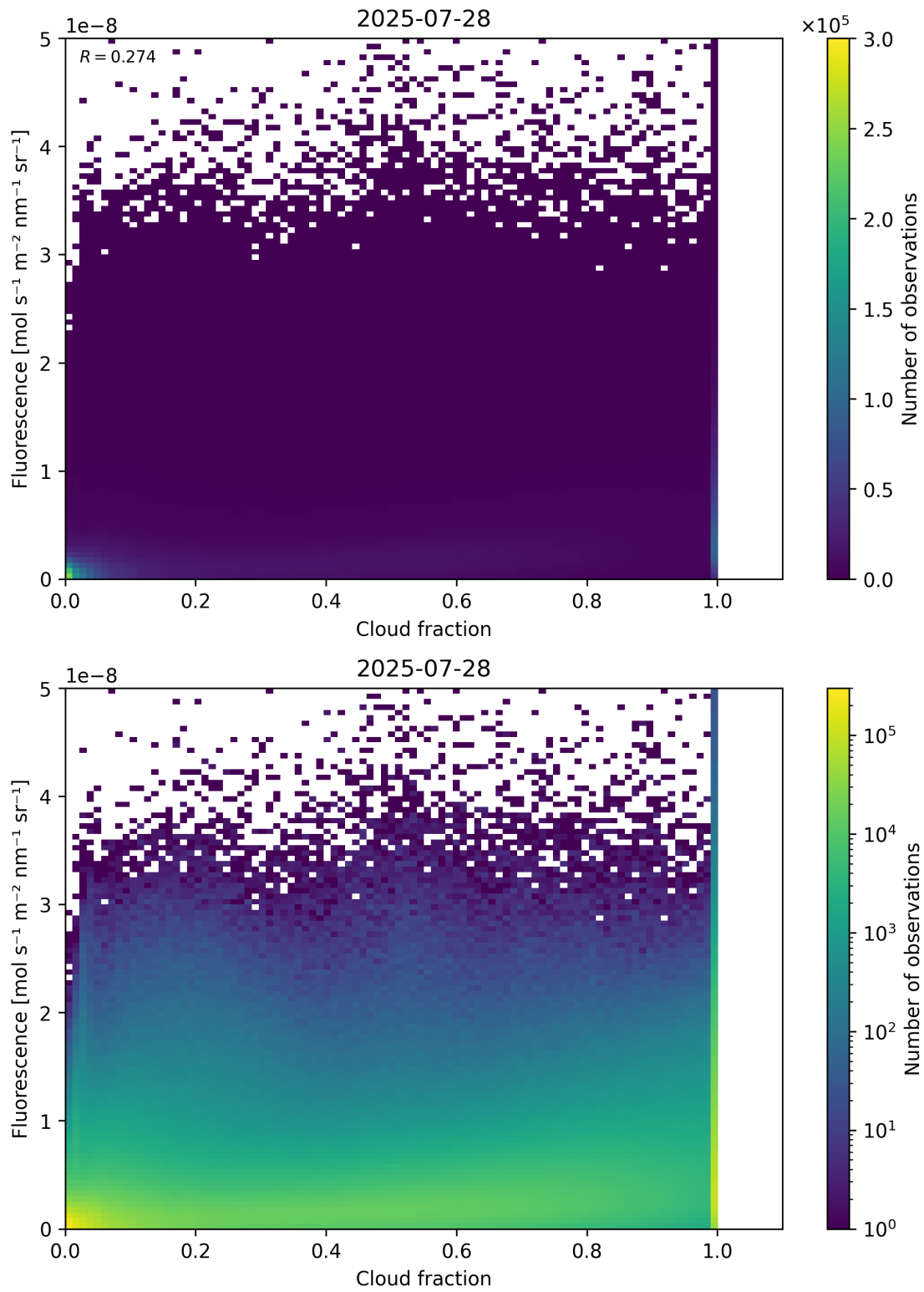
Figure 72: Scatter density plot of “Cloud fraction” against “Fluorescence” for 2025-07-27 to 2025-07-29.
