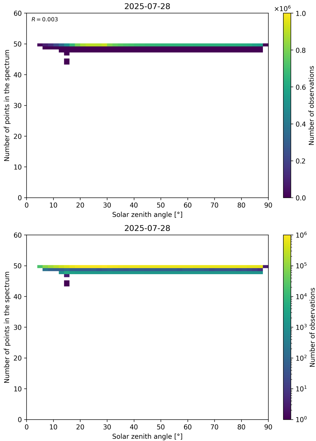
Figure 115: Scatter density plot of “Solar zenith angle” against “Number of points in the spectrum” for 2025-07-27 to 2025-07-29.
