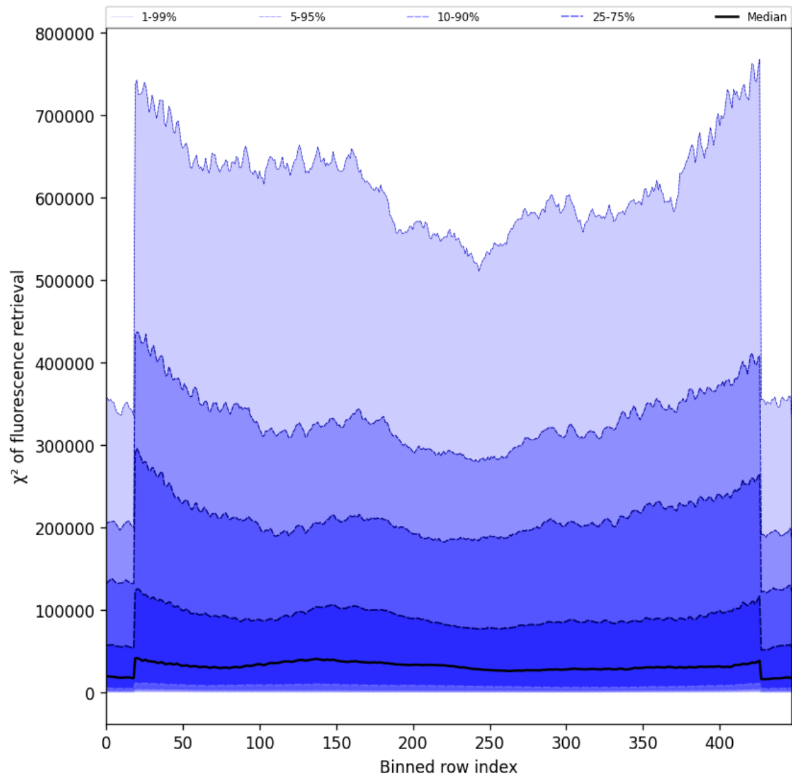
Figure 59: Along track statistics of “ \chi^2 of fluorescence retrieval” for 2025-07-27 to 2025-07-29
