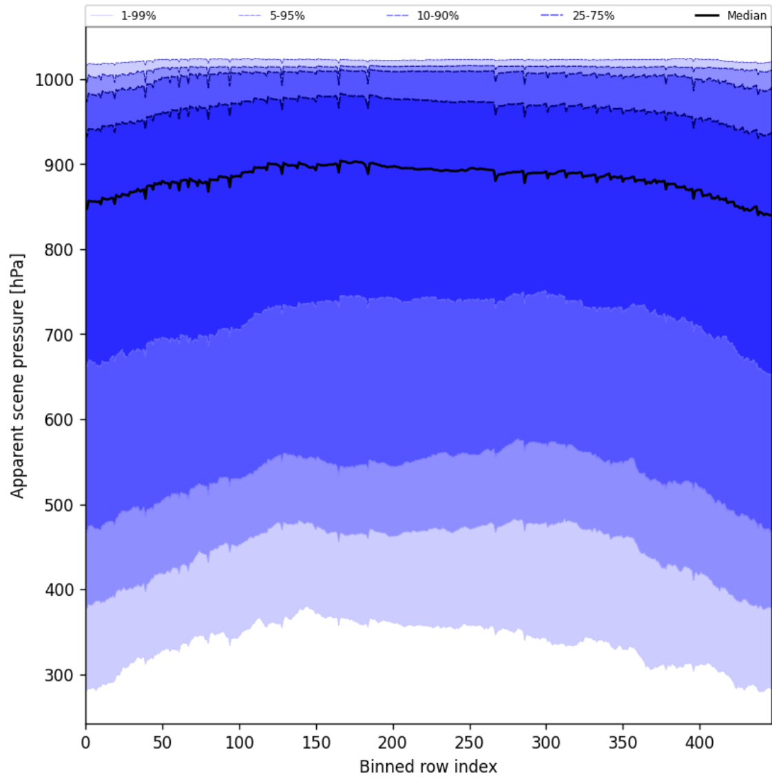
Figure 53: Along track statistics of “Apparent scene pressure” for 2025-07-27 to 2025-07-29
