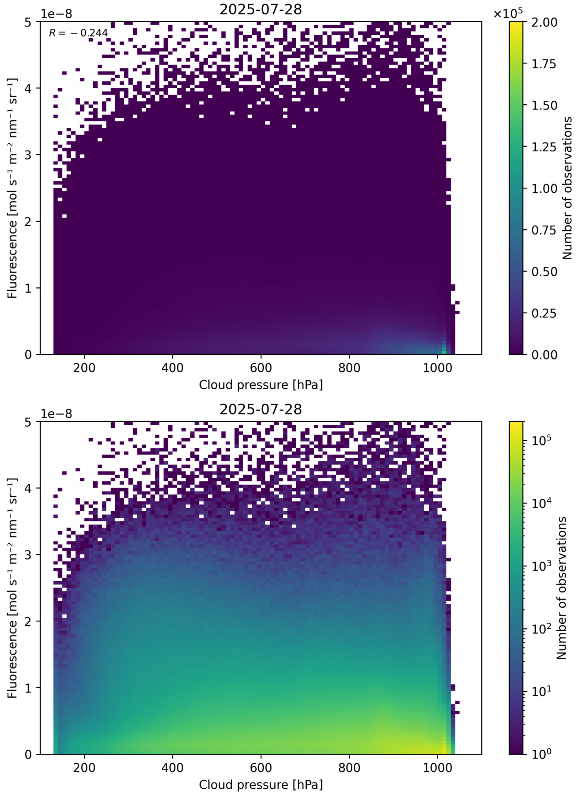
Figure 80: Scatter density plot of “Cloud pressure” against “Fluorescence” for 2025-07-27 to 2025-07-29.
