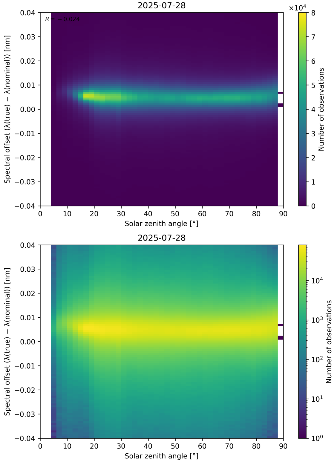
Figure 117: Scatter density plot of “Solar zenith angle” against “Spectral offset ( \lambda_{\text{true}} - \lambda_{\text{nominal}} )” for 2025-07-27 to 2025-07-29.
