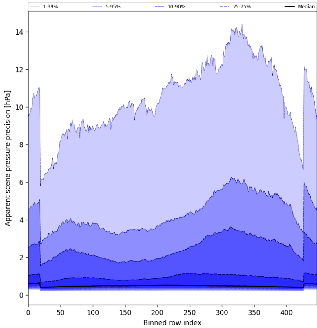
Figure 54: Along track statistics of “Apparent scene pressure precision” for 2025-07-27 to 2025-07-29
