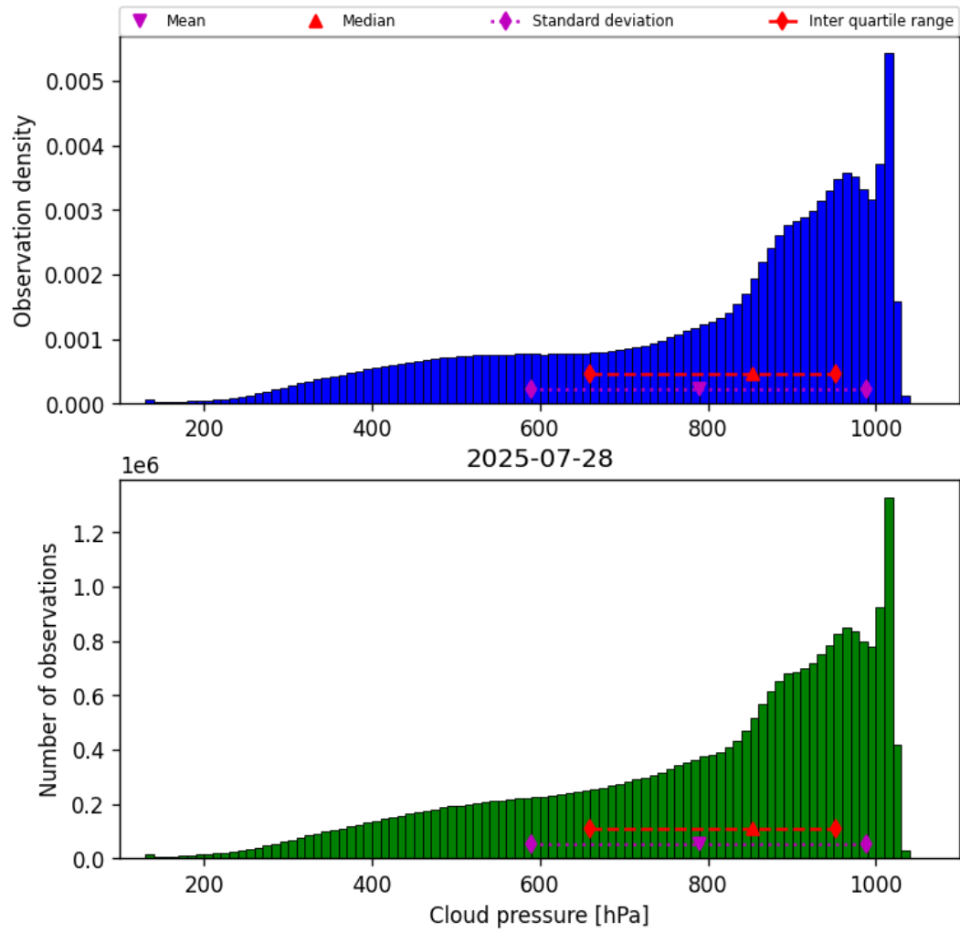
Figure 30: Histogram of “Cloud pressure” for 2025-07-27 to 2025-07-29
