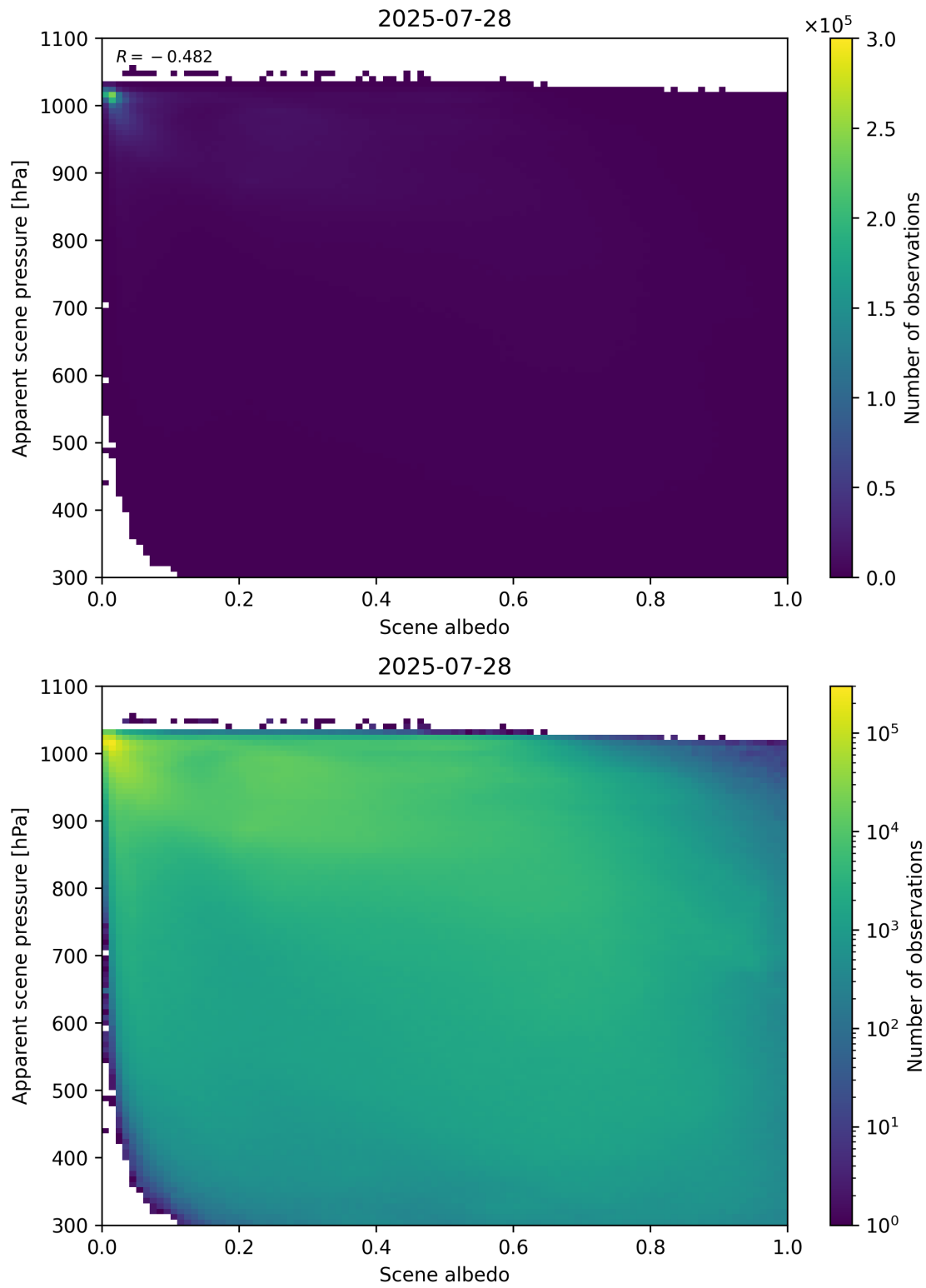
Figure 102: Scatter density plot of “Scene albedo” against “Apparent scene pressure” for 2025-07-27 to 2025-07-29.
