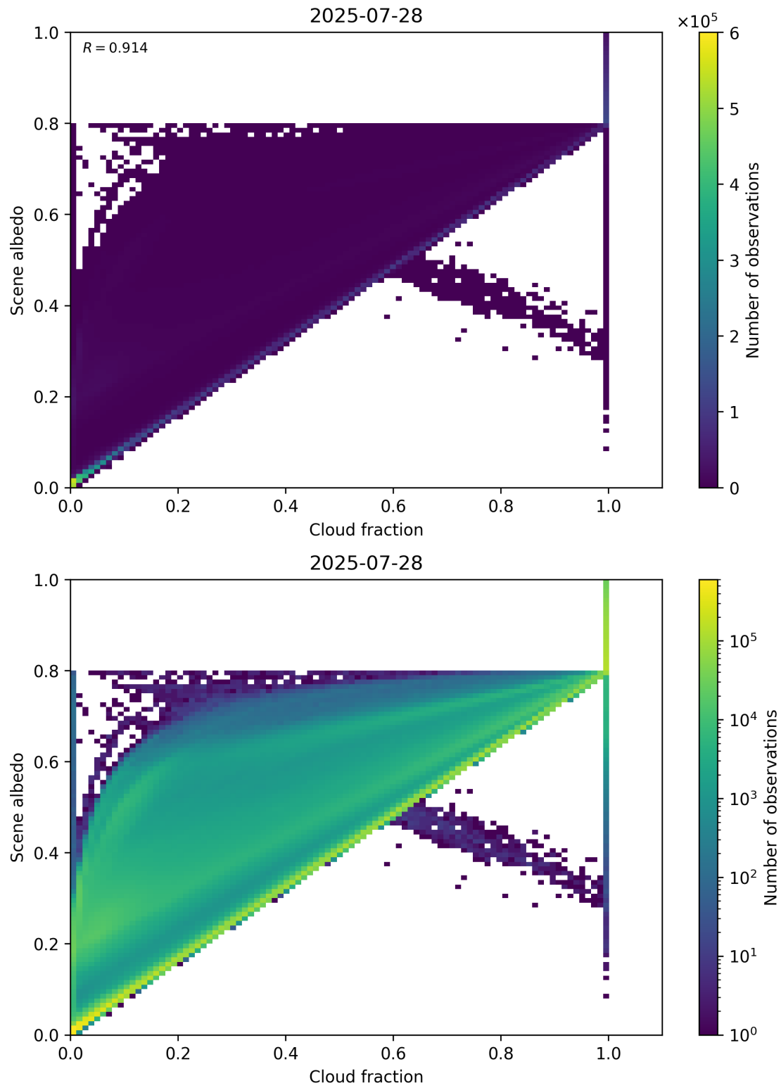
Figure 75: Scatter density plot of “Cloud fraction” against “Scene albedo” for 2025-07-27 to 2025-07-29.
