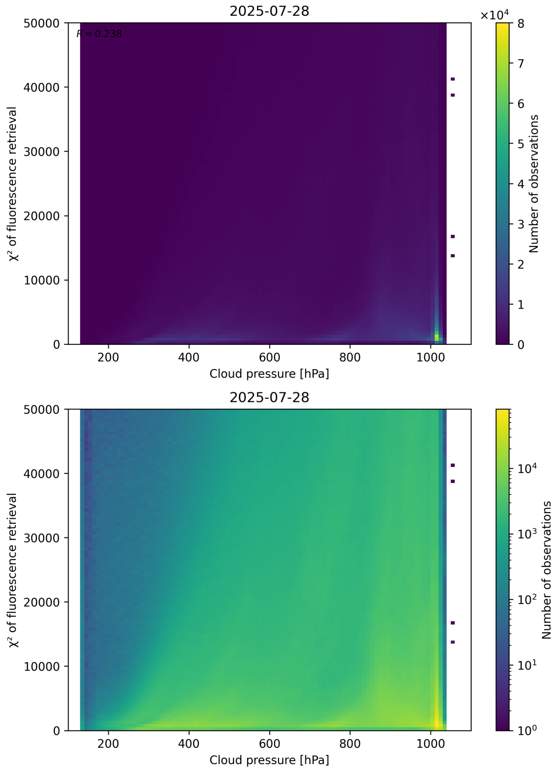
Figure 78: Scatter density plot of “Cloud pressure” against “ \chi^2 of fluorescence retrieval” for 2025-07-27 to 2025-07-29.
