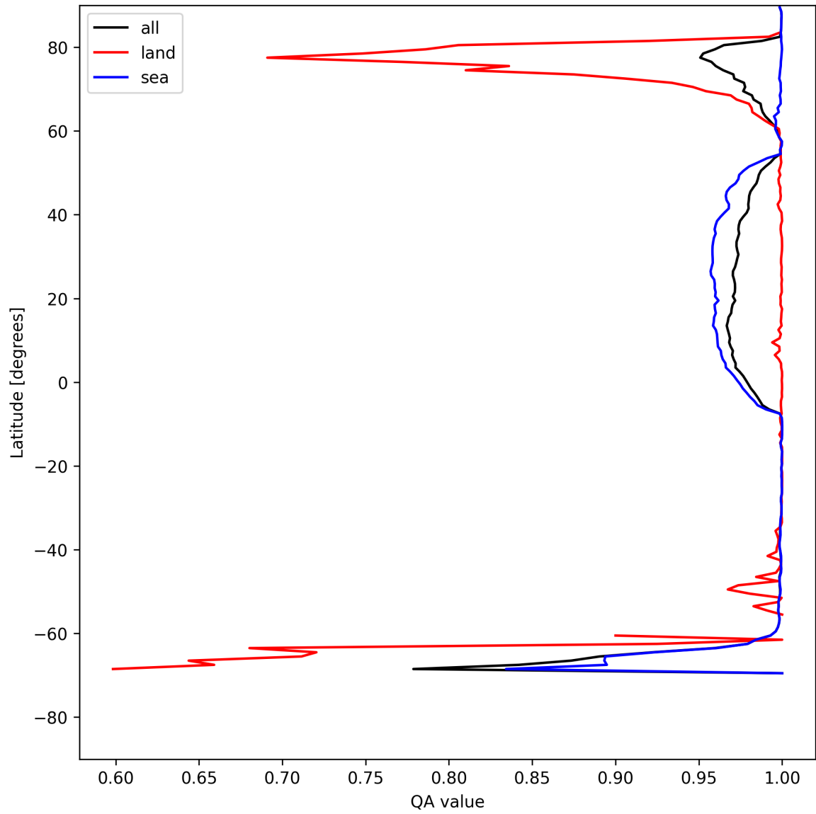
Figure 12: Zonal average of “QA value” for 2025-07-27 to 2025-07-29.
