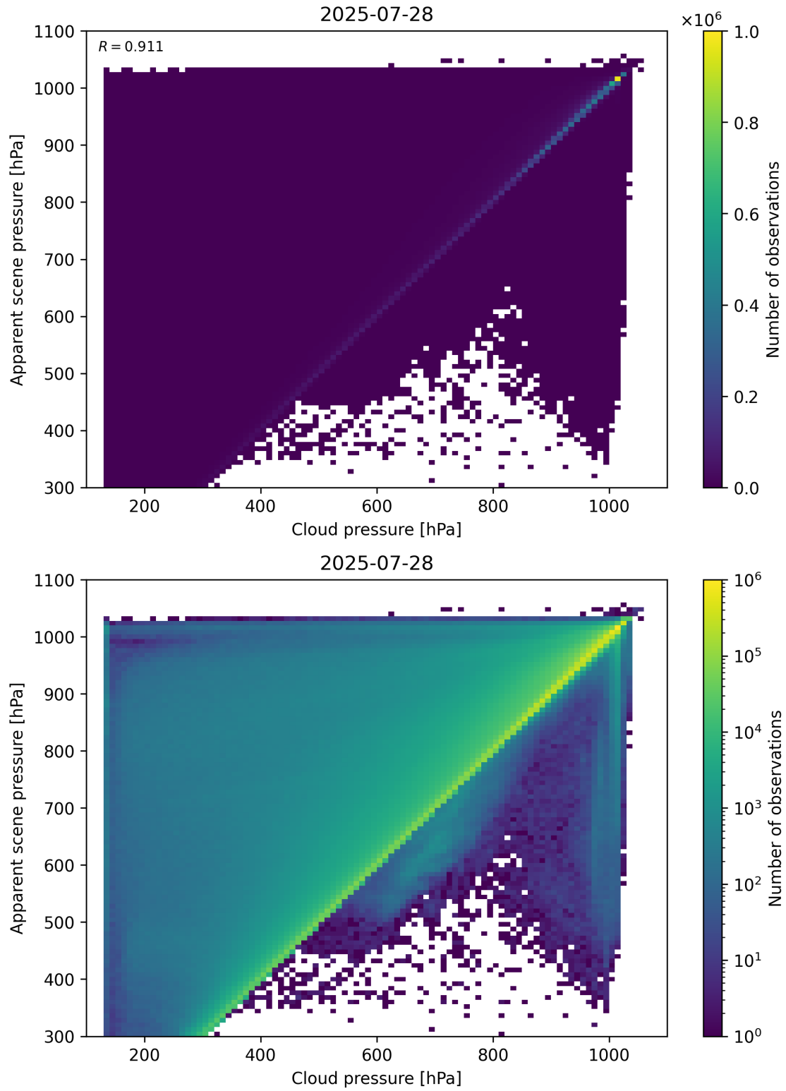
Figure 77: Scatter density plot of “Cloud pressure” against “Apparent scene pressure” for 2025-07-27 to 2025-07-29.
