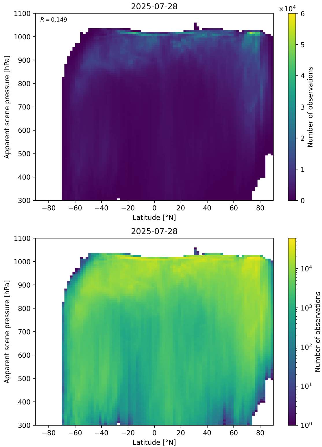
Figure 88: Scatter density plot of “Latitude” against “Apparent scene pressure” for 2025-07-27 to 2025-07-29.
