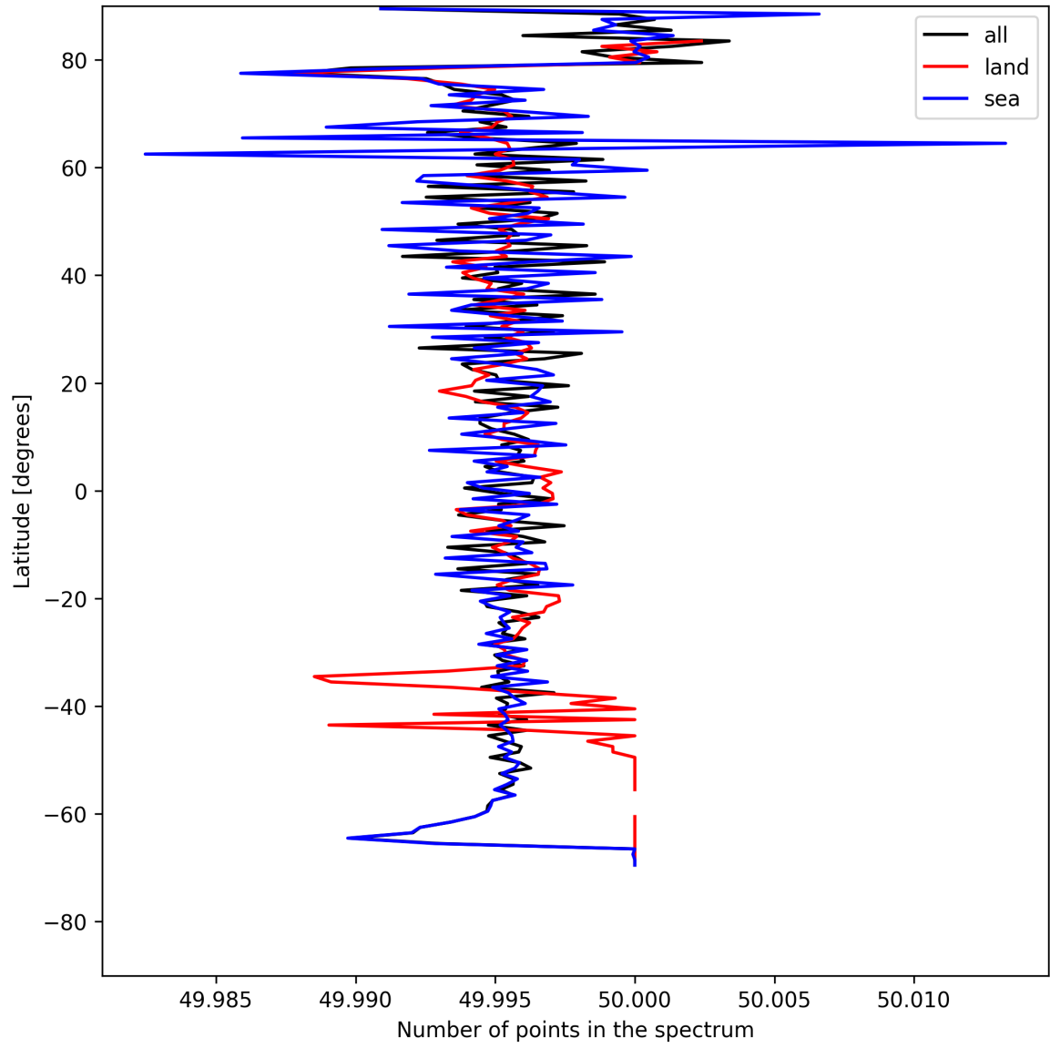
Figure 27: Zonal average of “Number of points in the spectrum” for 2025-07-27 to 2025-07-29.
