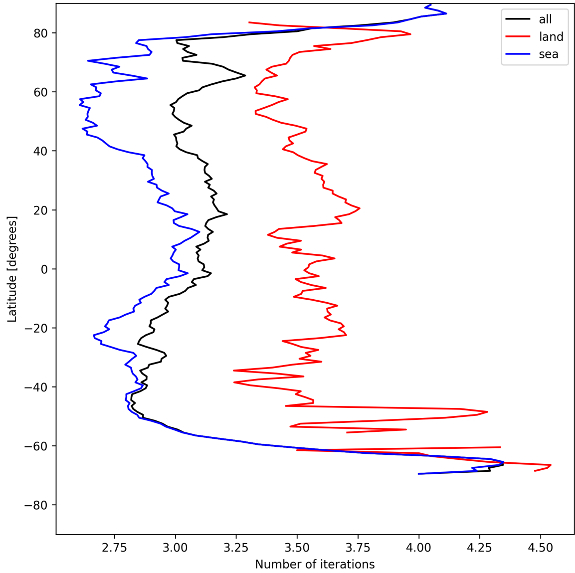
Figure 22: Zonal average of “Number of iterations” for 2025-07-27 to 2025-07-29.
