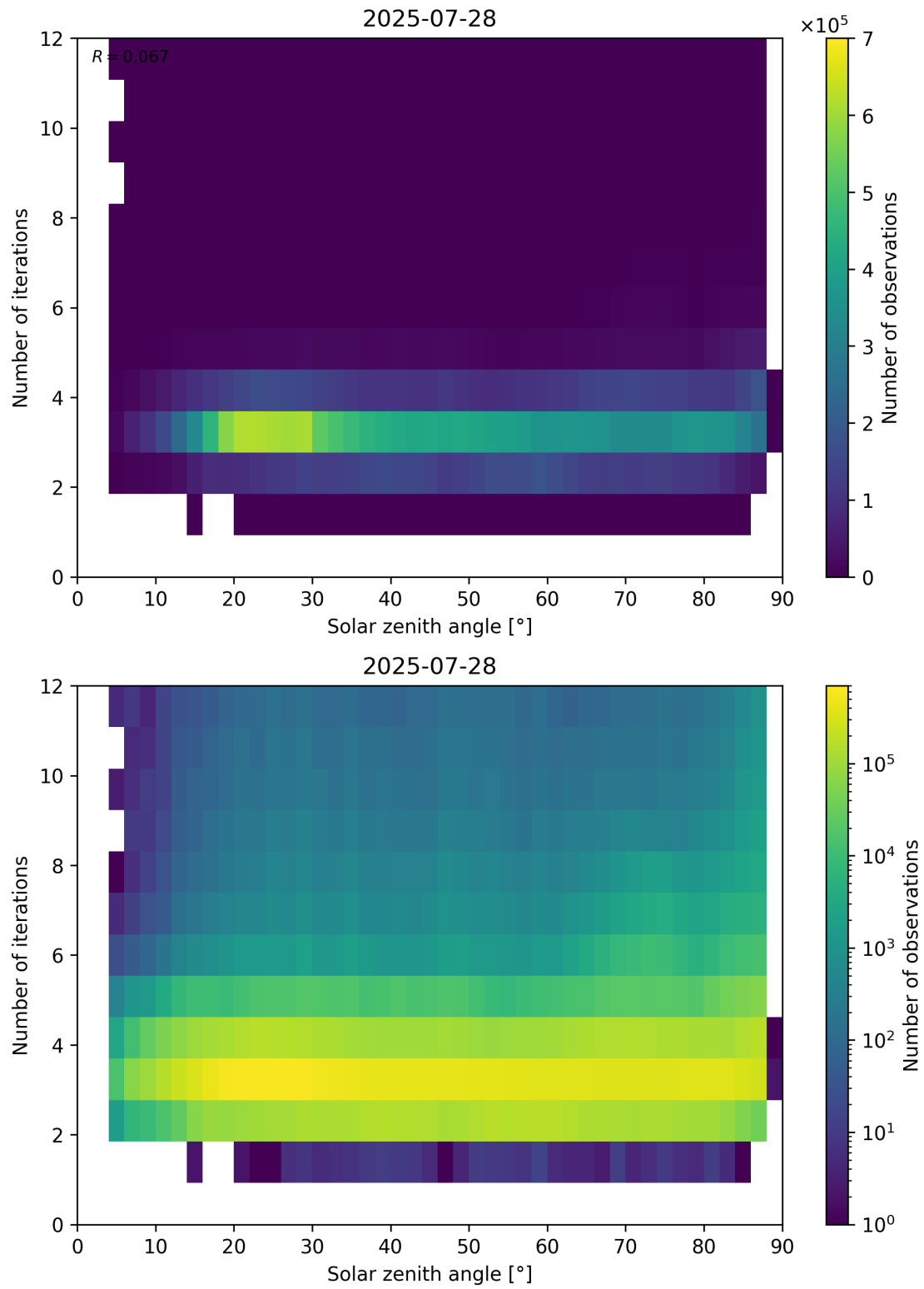
Figure 114: Scatter density plot of “Solar zenith angle” against “Number of iterations” for 2025-07-27 to 2025-07-29.
