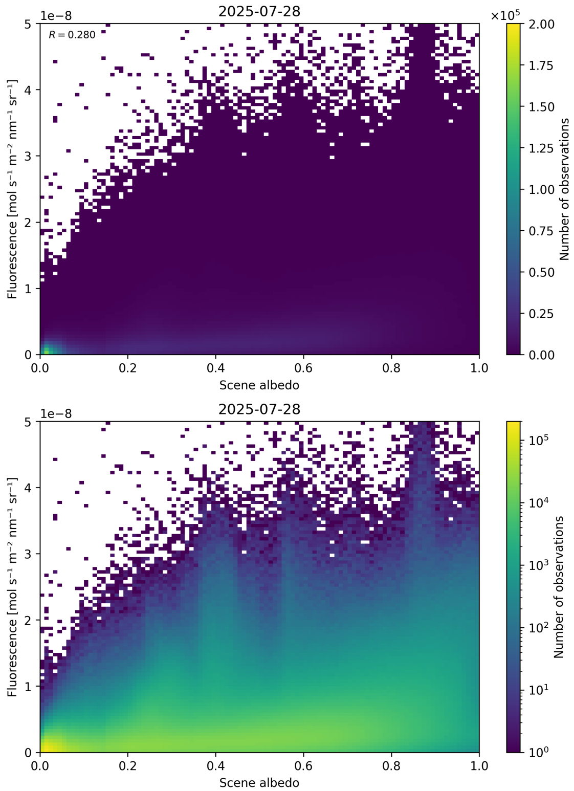
Figure 104: Scatter density plot of “Scene albedo” against “Fluorescence” for 2025-07-27 to 2025-07-29.
