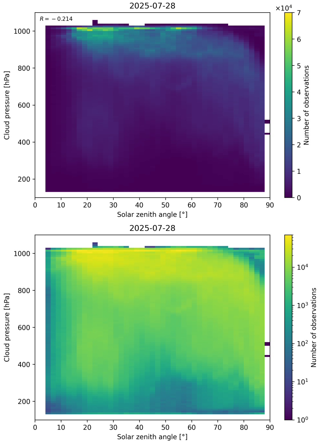
Figure 111: Scatter density plot of “Solar zenith angle” against “Cloud pressure” for 2025-07-27 to 2025-07-29.
