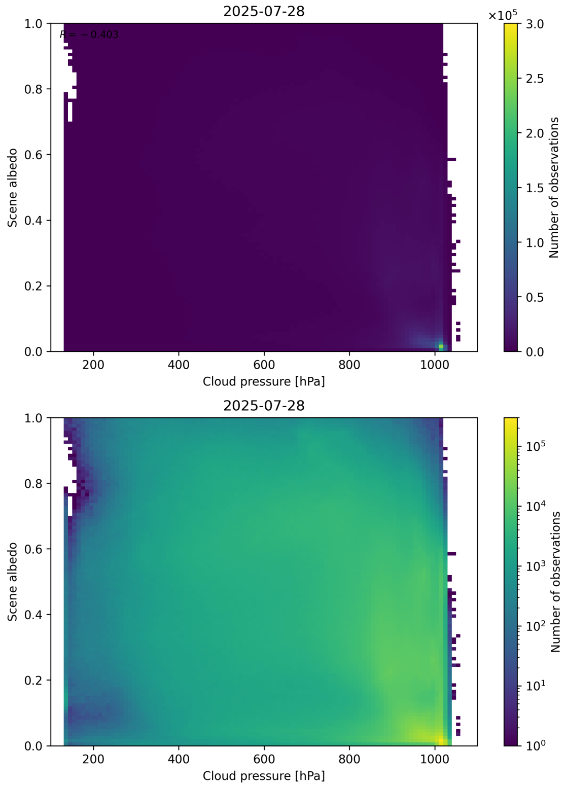
Figure 83: Scatter density plot of “Cloud pressure” against “Scene albedo” for 2025-07-27 to 2025-07-29.
