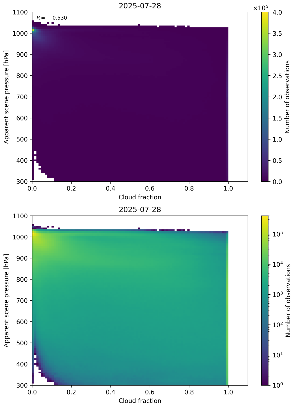
Figure 70: Scatter density plot of “Cloud fraction” against “Apparent scene pressure” for 2025-07-27 to 2025-07-29.
