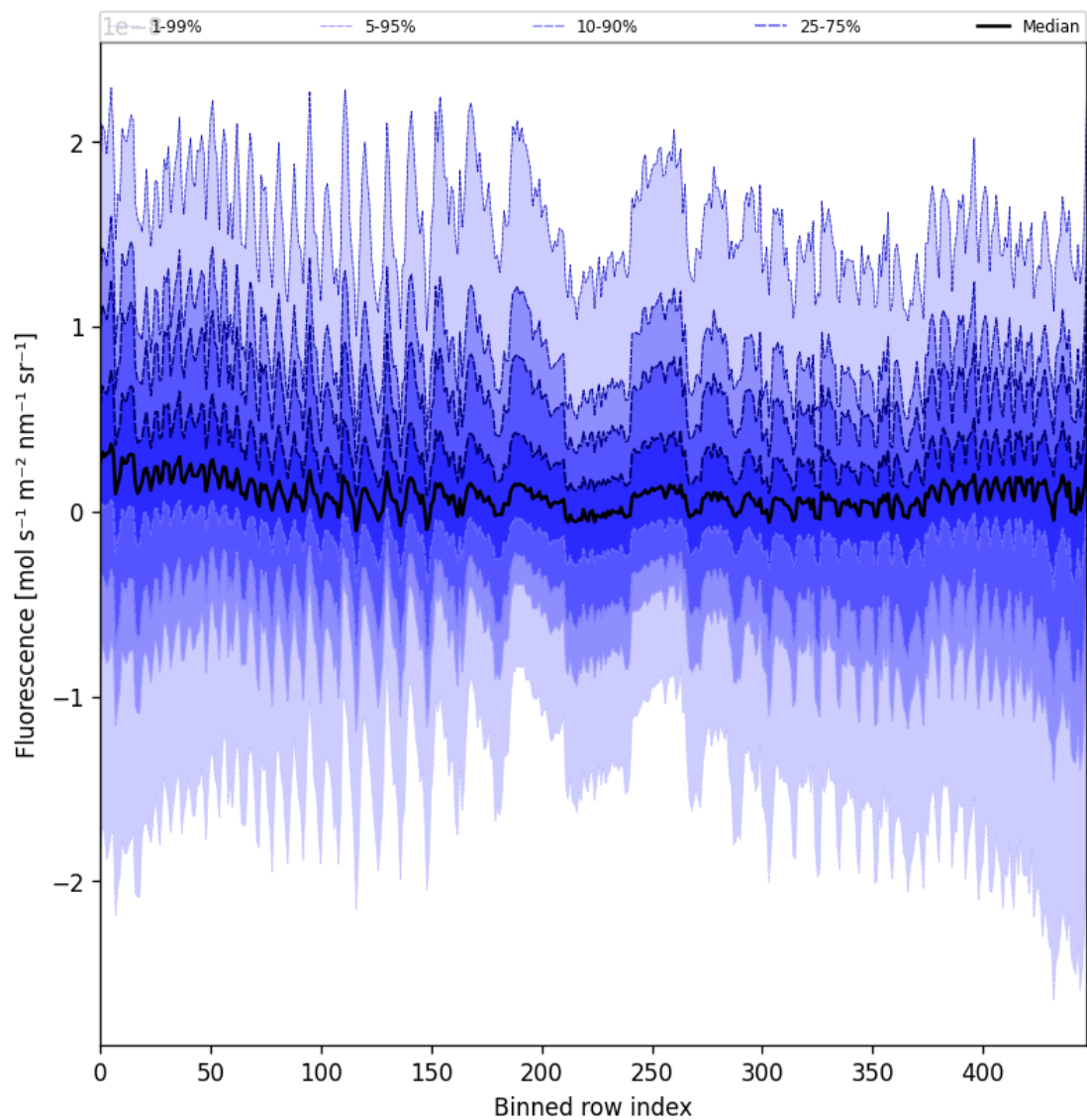
Figure 57: Along track statistics of “Fluorescence” for 2025-07-27 to 2025-07-29
