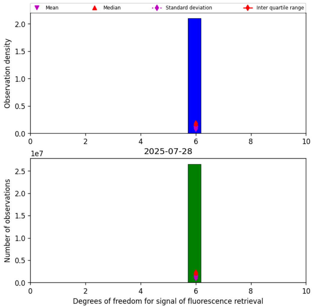
Figure 43: Histogram of "Degrees of freedom for signal of fluorescence retrieval" for 2025-07-27 to 2025-07-29
