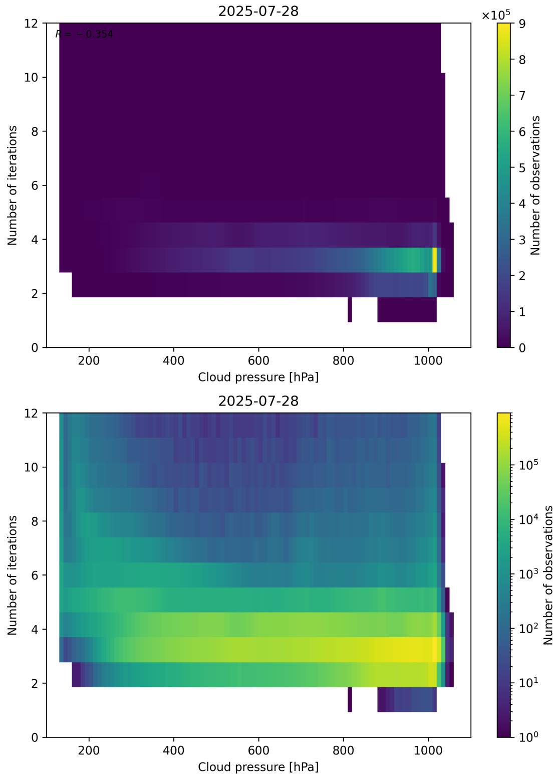
Figure 81: Scatter density plot of “Cloud pressure” against “Number of iterations” for 2025-07-27 to 2025-07-29.
