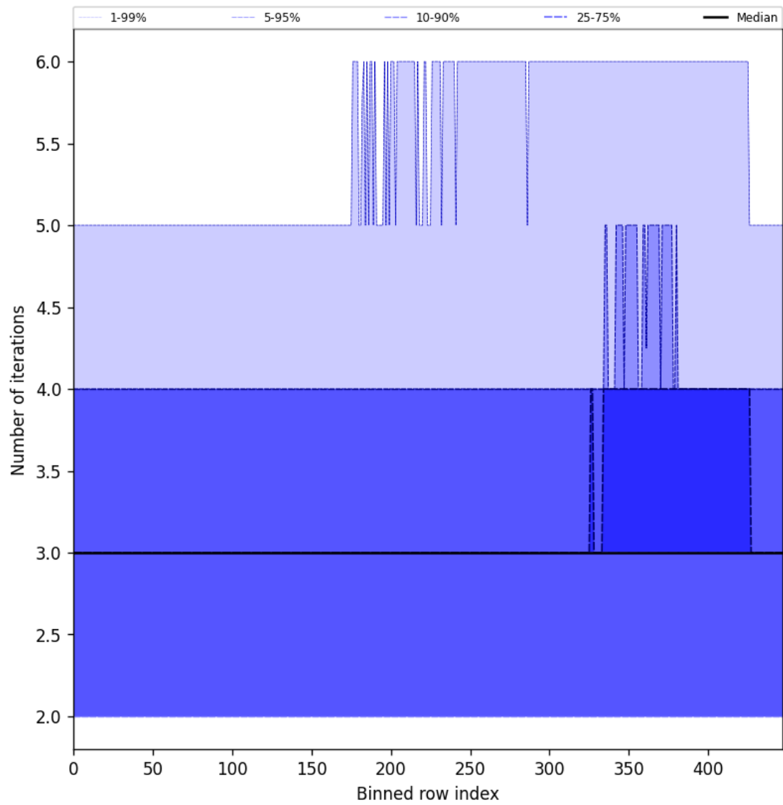
Figure 56: Along track statistics of “Number of iterations” for 2025-07-27 to 2025-07-29
