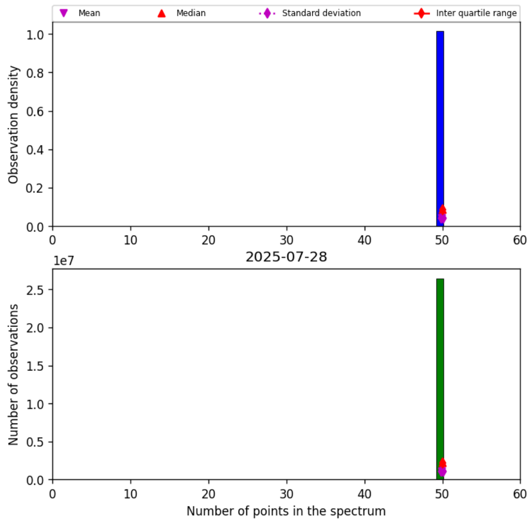
Figure 44: Histogram of "Number of points in the spectrum" for 2025-07-27 to 2025-07-29
