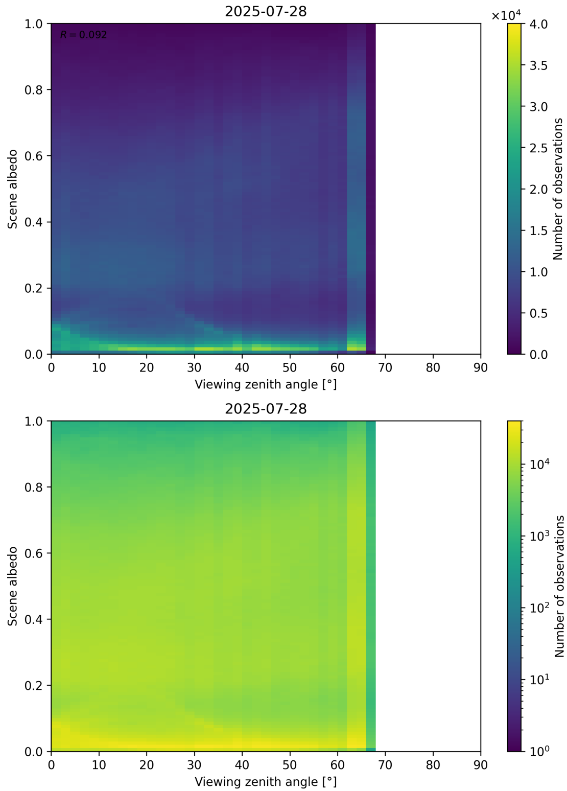
Figure 126: Scatter density plot of “Viewing zenith angle” against “Scene albedo” for 2025-07-27 to 2025-07-29.
