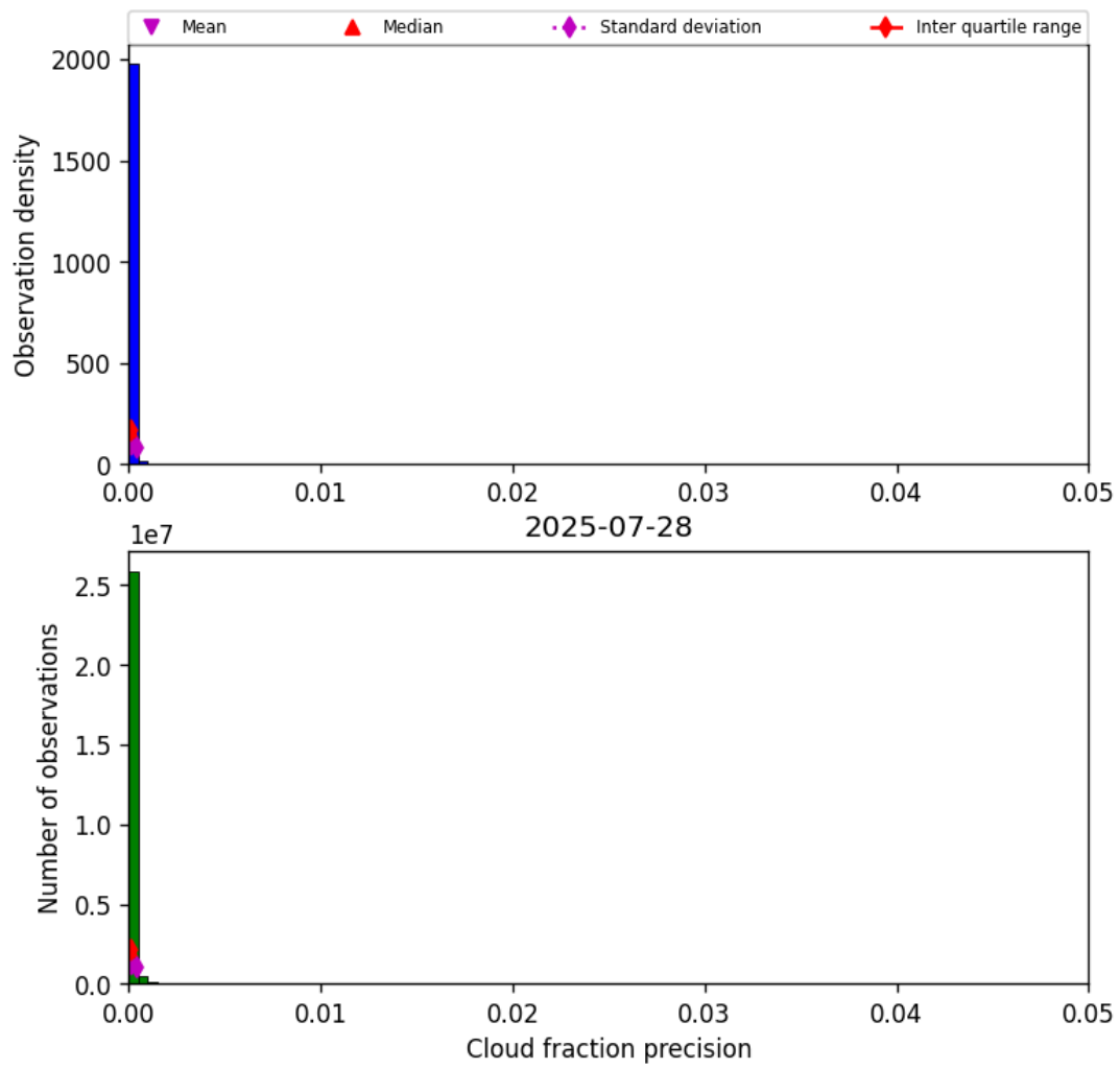
Figure 33: Histogram of “Cloud fraction precision” for 2025-07-27 to 2025-07-29
