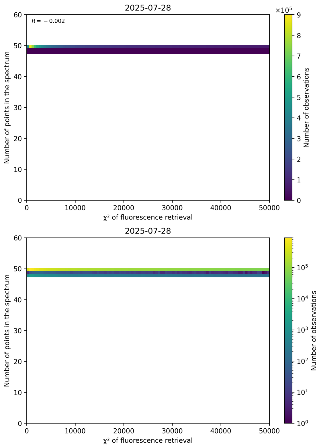
Figure 68: Scatter density plot of “ \chi^2 of fluorescence retrieval” against “Number of points in the spectrum” for 2025-07-27 to 2025-07-29.
