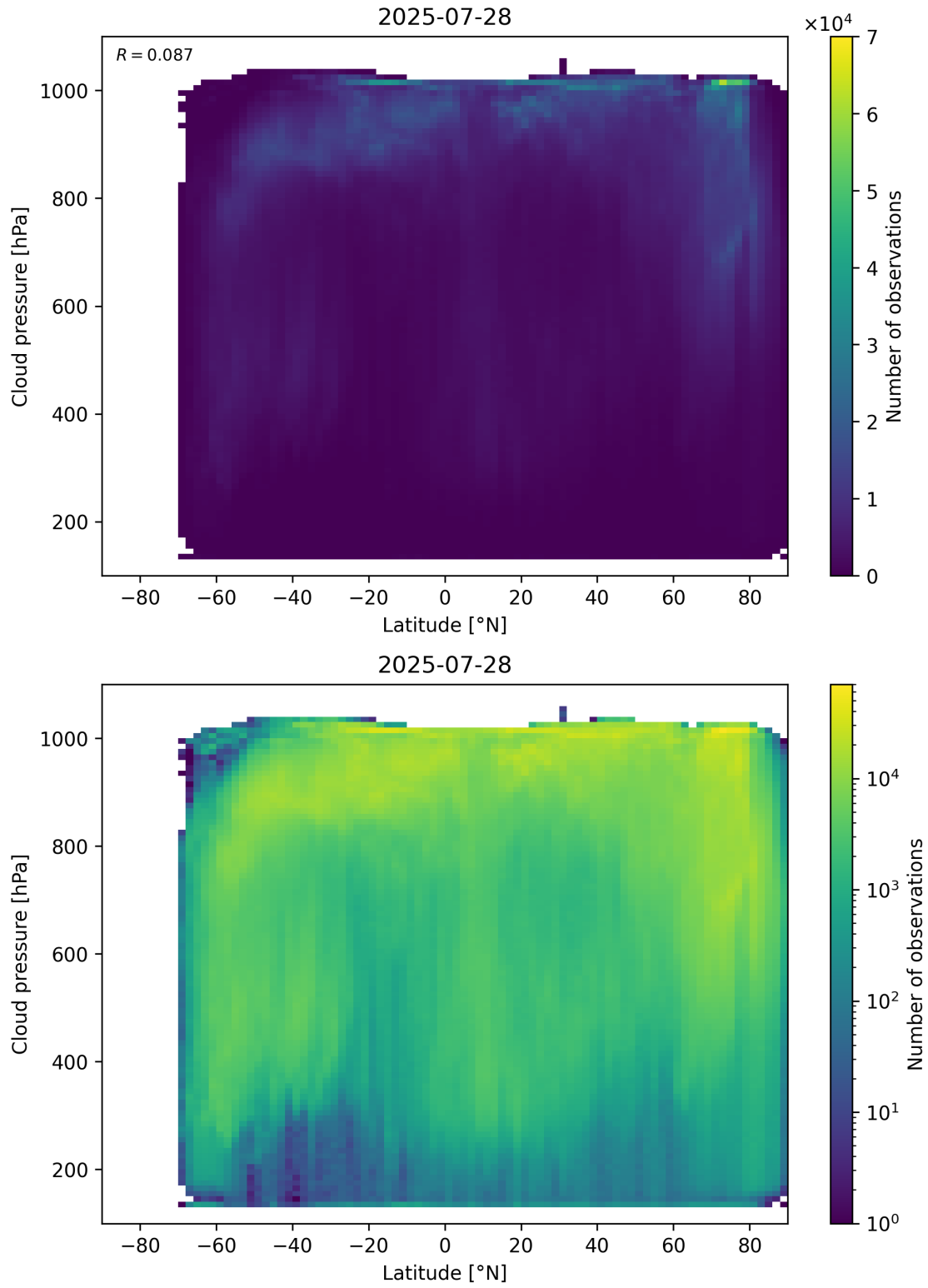
Figure 91: Scatter density plot of “Latitude” against “Cloud pressure” for 2025-07-27 to 2025-07-29.
