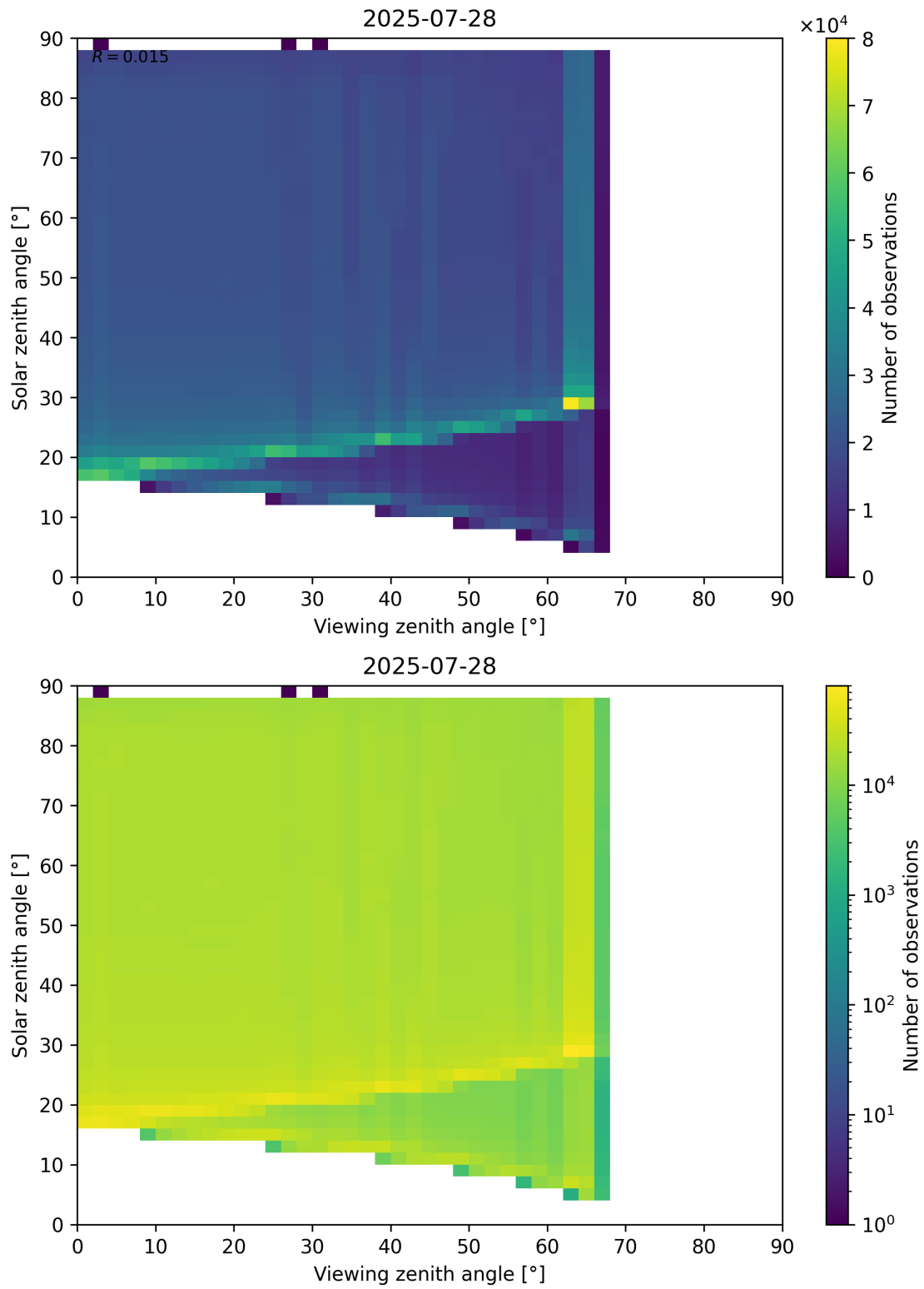
Figure 127: Scatter density plot of “Viewing zenith angle” against “Solar zenith angle” for 2025-07-27 to 2025-07-29.
