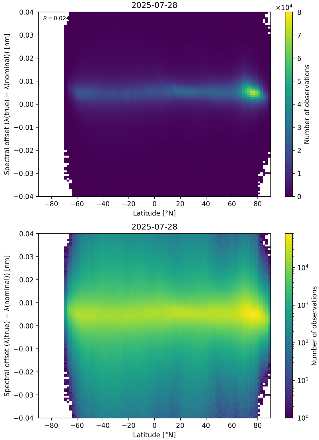
Figure 96: Scatter density plot of “Latitude” against “Spectral offset ( \lambda_{\text{true}} - \lambda_{\text{nominal}} )” for 2025-07-27 to 2025-07-29.
