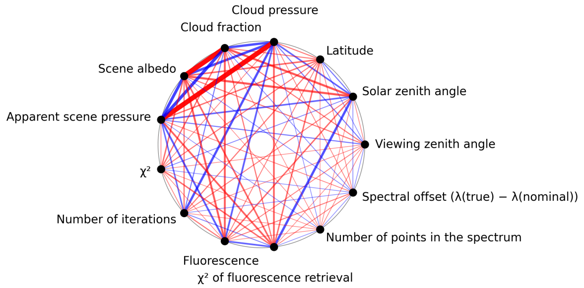
Figure 1: Map of correlation graph for 2025-07-27 to 2025-07-29.
