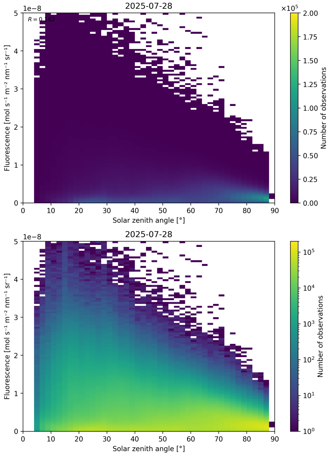
Figure 112: Scatter density plot of “Solar zenith angle” against “Fluorescence” for 2025-07-27 to 2025-07-29.
