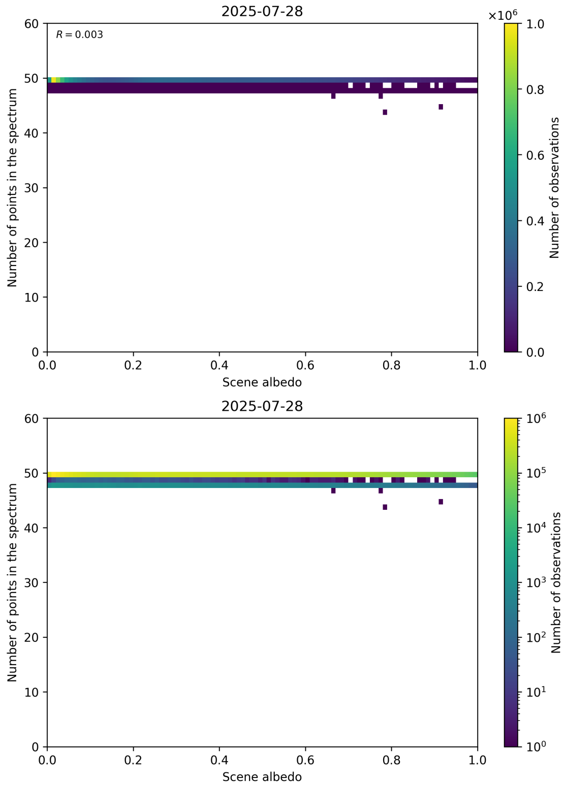
Figure 106: Scatter density plot of “Scene albedo” against “Number of points in the spectrum” for 2025-07-27 to 2025-07-29.
