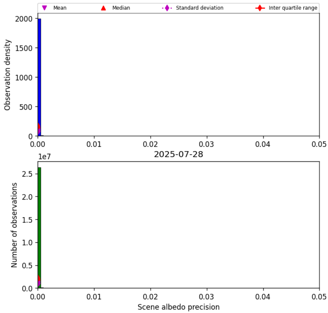
Figure 35: Histogram of “Scene albedo precision” for 2025-07-27 to 2025-07-29
