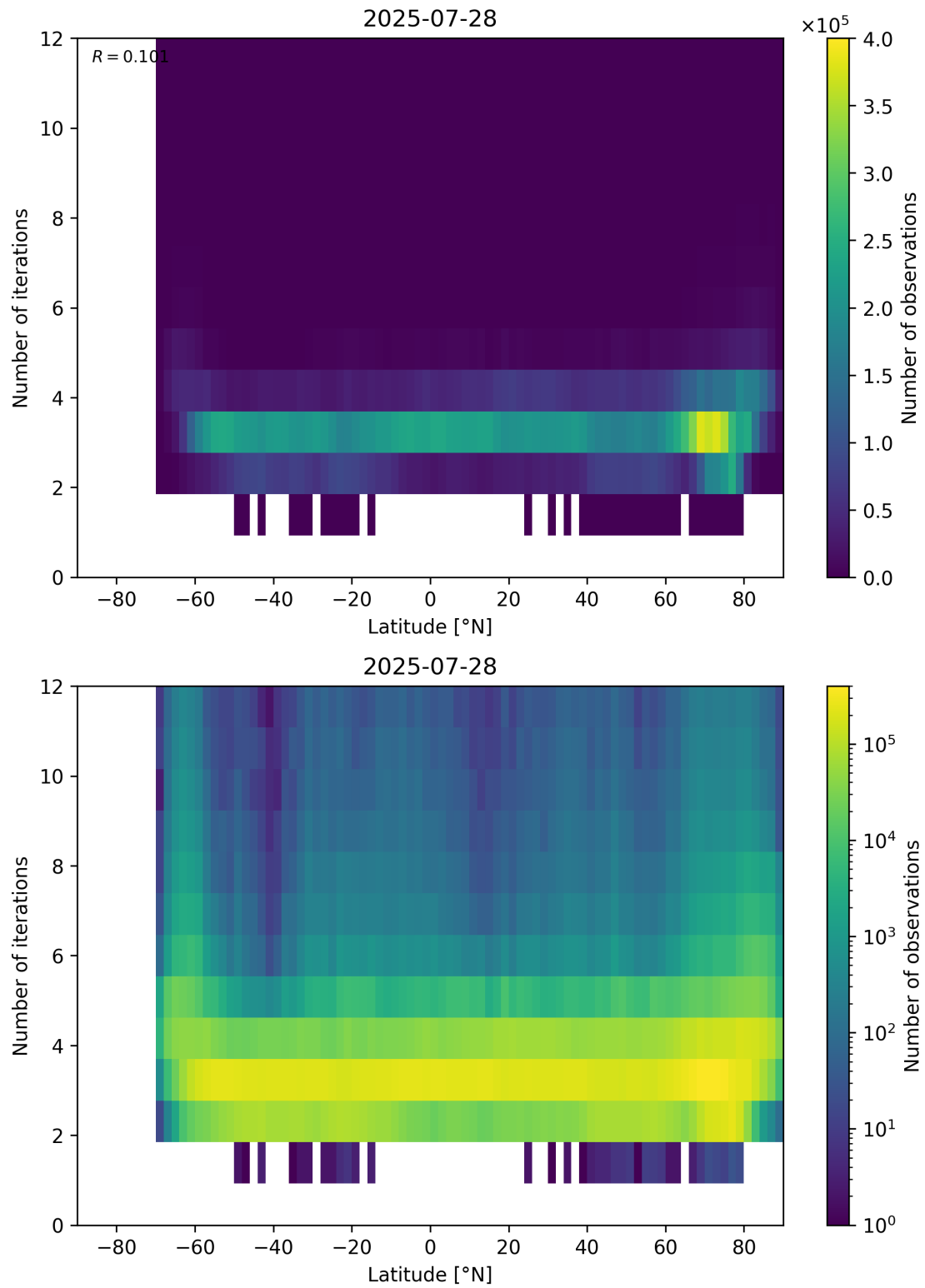
Figure 93: Scatter density plot of “Latitude” against “Number of iterations” for 2025-07-27 to 2025-07-29.
