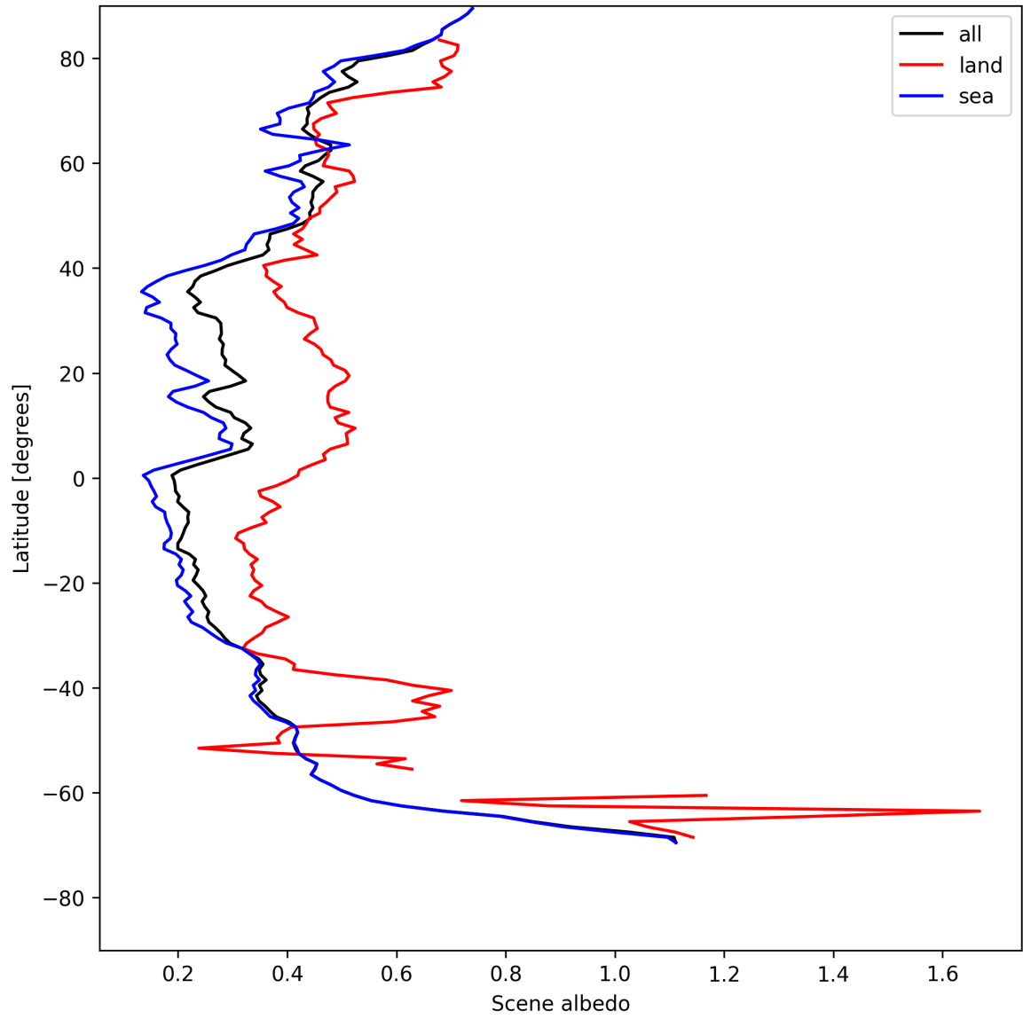
Figure 17: Zonal average of “Scene albedo” for 2025-07-27 to 2025-07-29.
