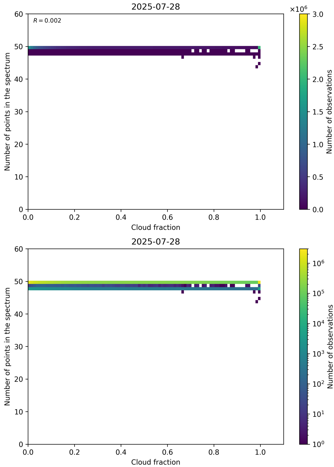
Figure 74: Scatter density plot of “Cloud fraction” against “Number of points in the spectrum” for 2025-07-27 to 2025-07-29.
