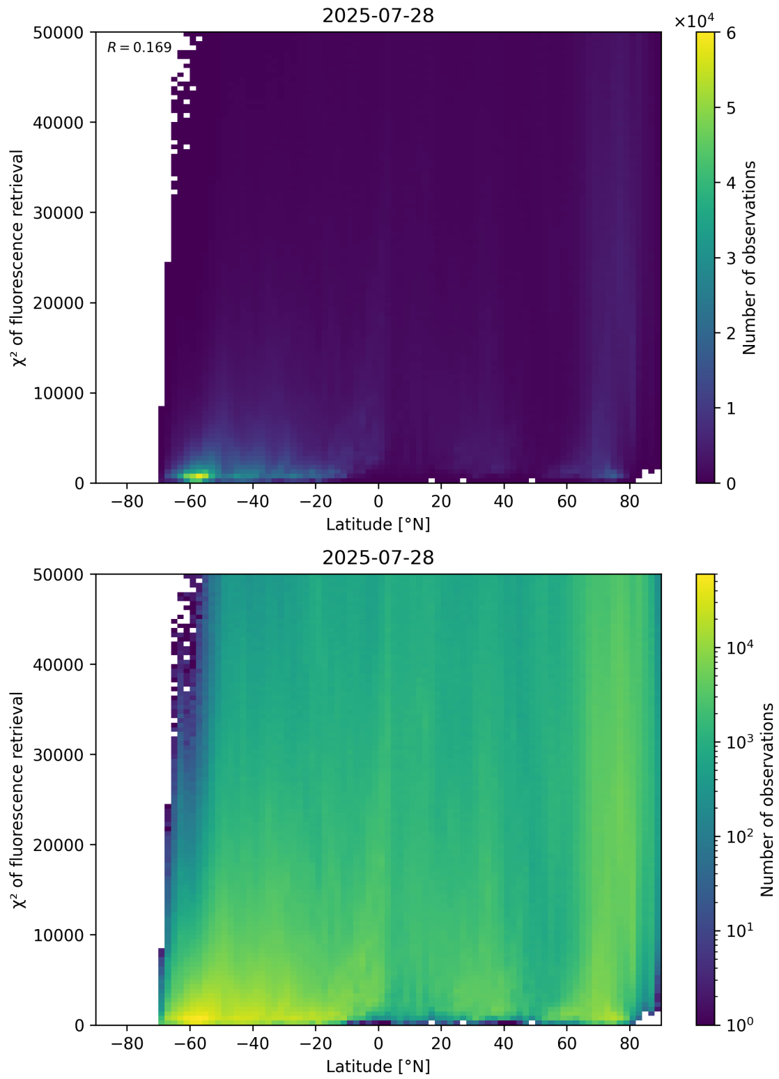
Figure 89: Scatter density plot of “Latitude” against “ \chi^2 of fluorescence retrieval” for 2025-07-27 to 2025-07-29.
