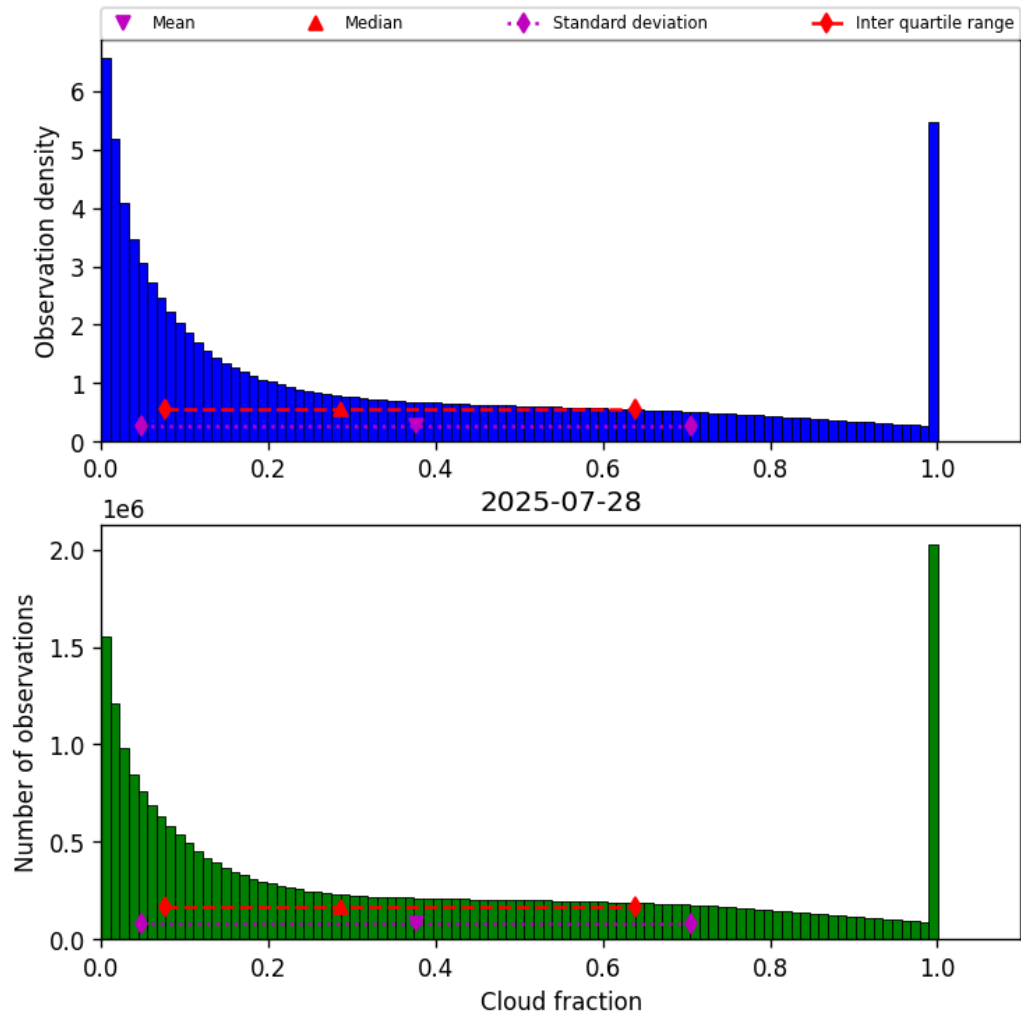
Figure 32: Histogram of “Cloud fraction” for 2025-07-27 to 2025-07-29
