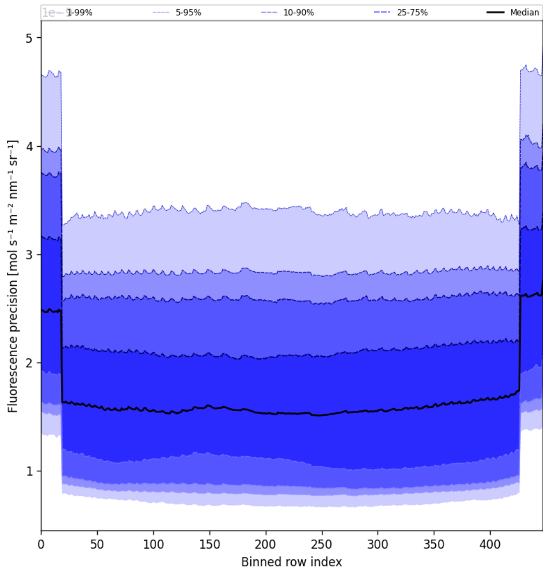
Figure 58: Along track statistics of “Fluorescence precision” for 2025-07-27 to 2025-07-29
