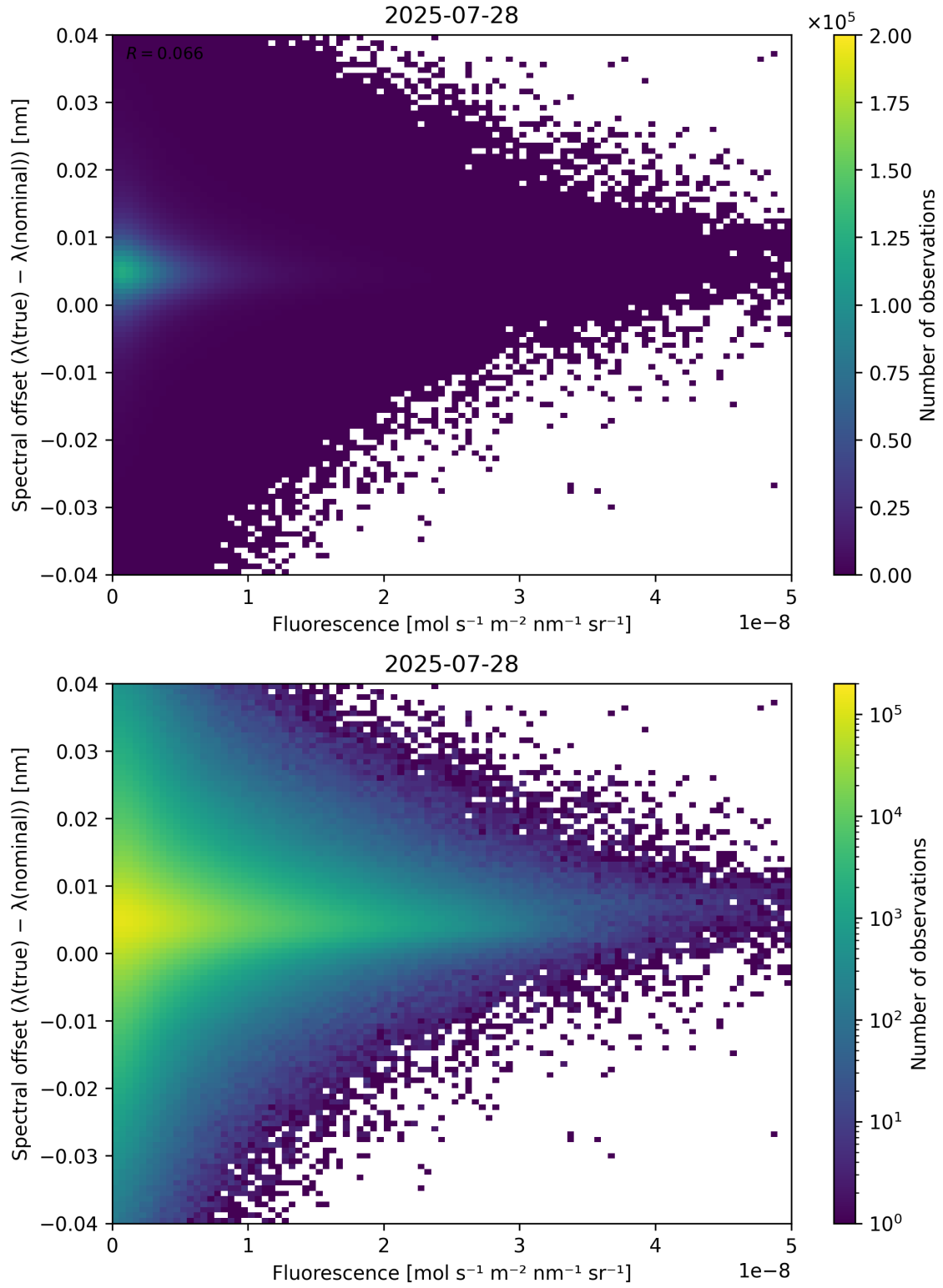
Figure 87: Scatter density plot of “Fluorescence” against “Spectral offset ( \lambda_{\text{true}} - \lambda_{\text{nominal}} )” for 2025-07-27 to 2025-07-29.
