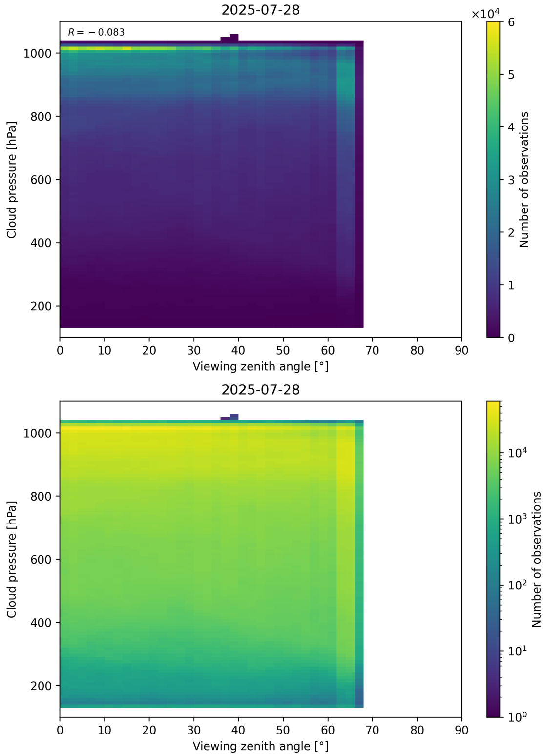
Figure 121: Scatter density plot of “Viewing zenith angle” against “Cloud pressure” for 2025-07-27 to 2025-07-29.
