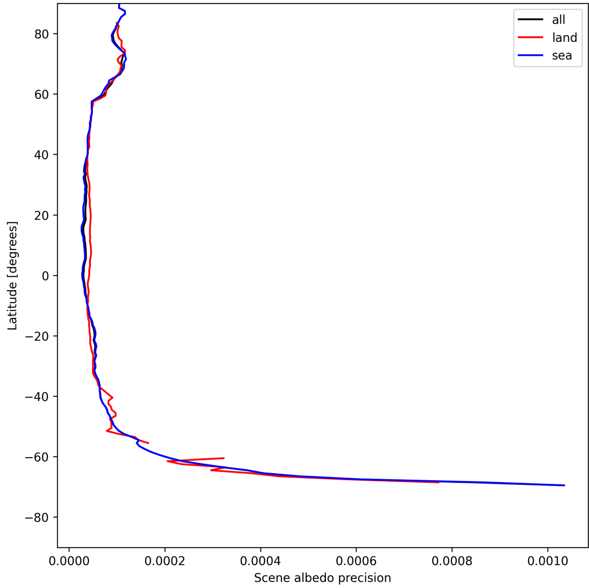
Figure 18: Zonal average of “Scene albedo precision” for 2025-07-27 to 2025-07-29.
