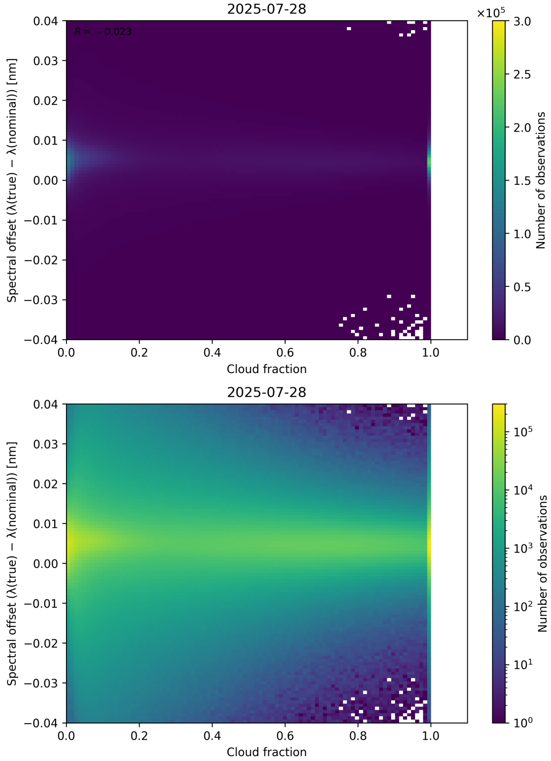
Figure 76: Scatter density plot of “Cloud fraction” against “Spectral offset ( \lambda_{\text{true}} - \lambda_{\text{nominal}} )” for 2025-07-27 to 2025-07-29.
