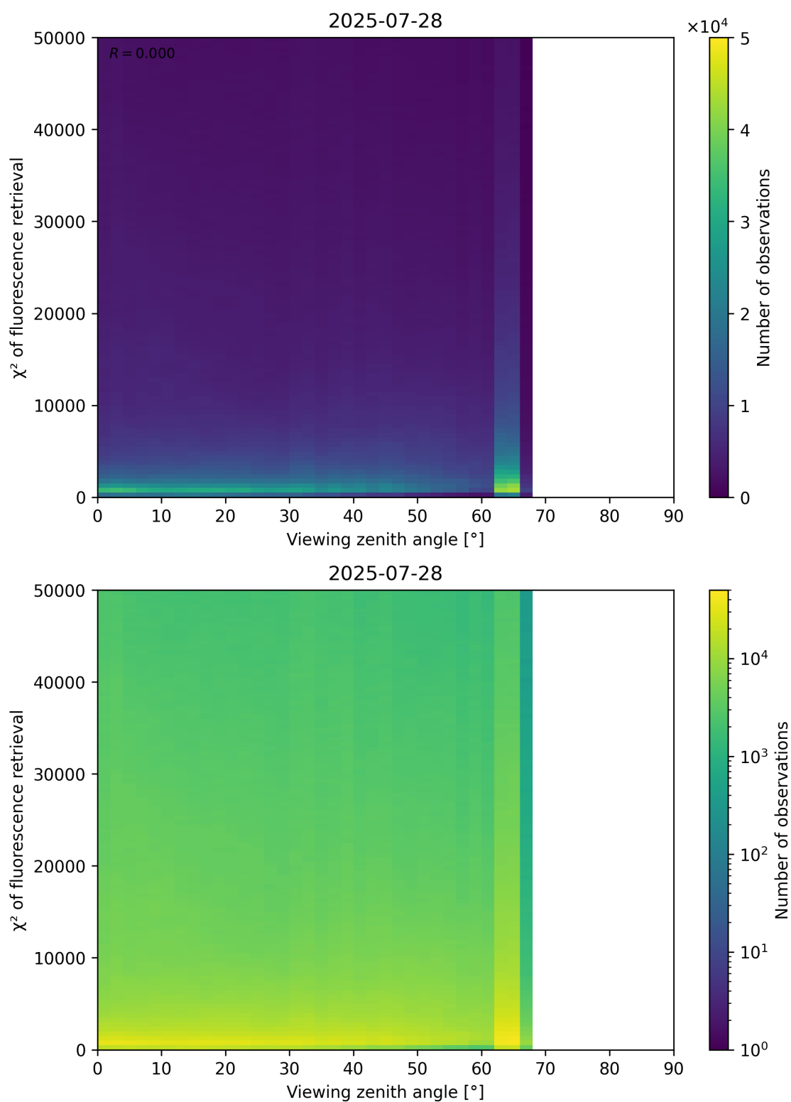
Figure 119: Scatter density plot of “Viewing zenith angle” against “ \chi^2 of fluorescence retrieval” for 2025-07-27 to 2025-07-29.
