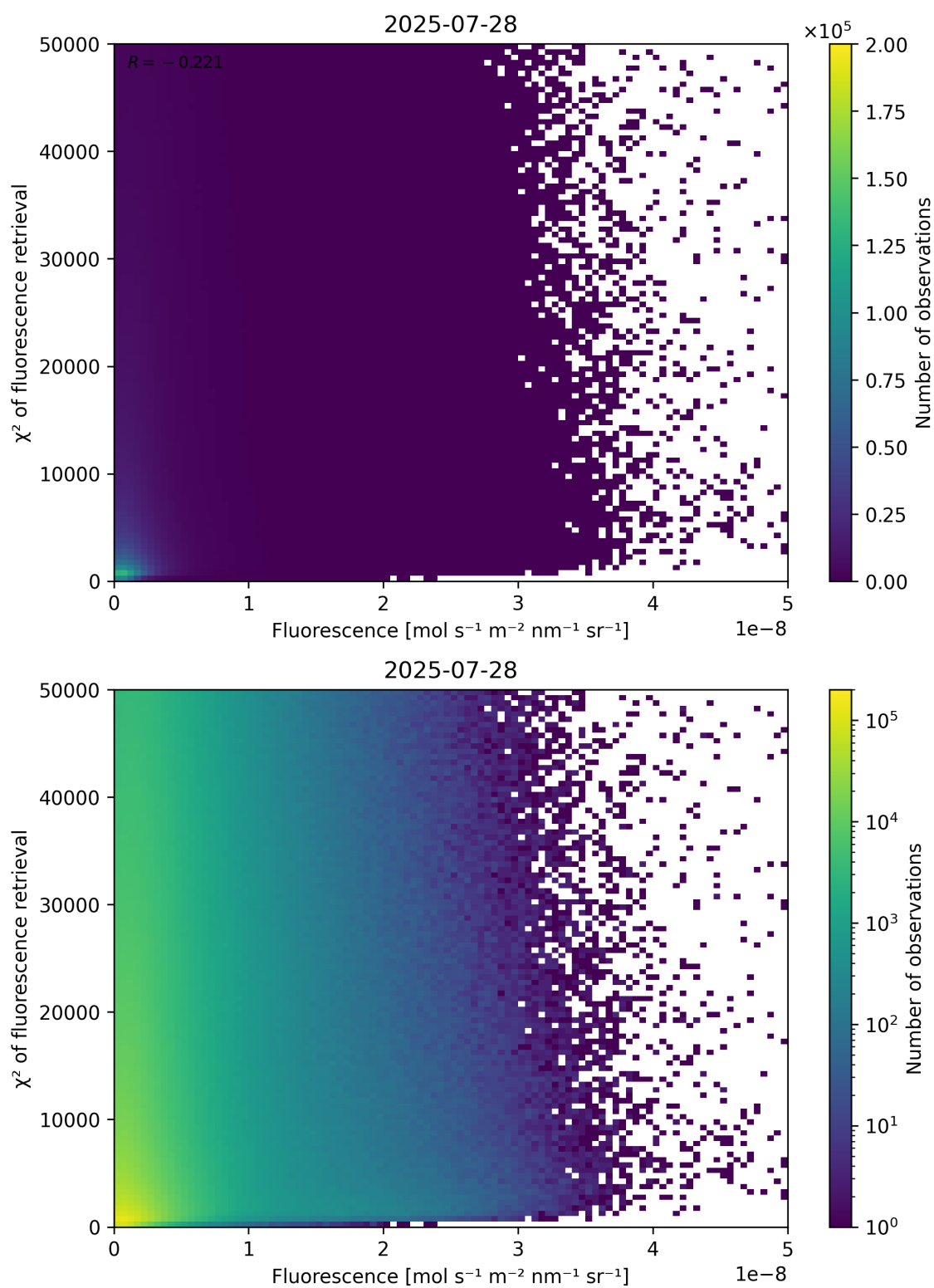
Figure 85: Scatter density plot of “Fluorescence” against “ \chi^2 of fluorescence retrieval” for 2025-07-27 to 2025-07-29.
