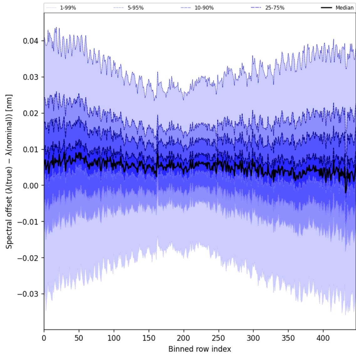
Figure 62: Along track statistics of “Spectral offset ( \lambda_{\text{true}} - \lambda_{\text{nominal}} )” for 2025-07-27 to 2025-07-29
