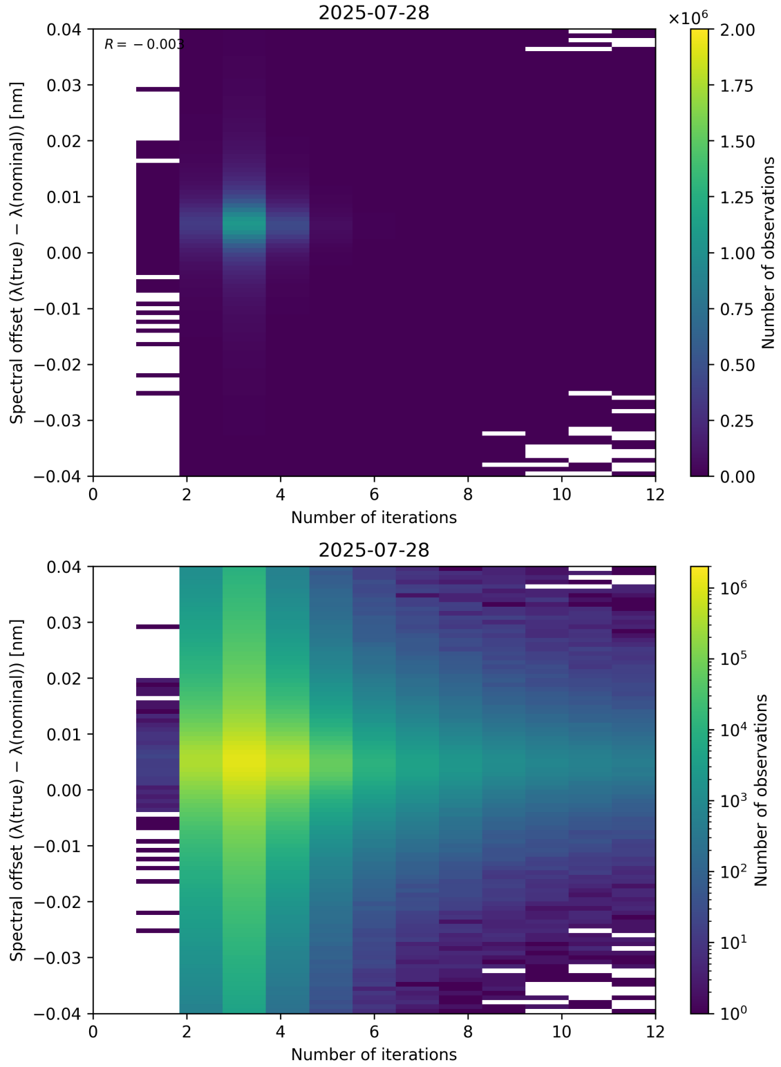
Figure 100: Scatter density plot of “Number of iterations” against “Spectral offset ( \lambda_{\text{true}} - \lambda_{\text{nominal}} )” for 2025-07-27 to 2025-07-29.
