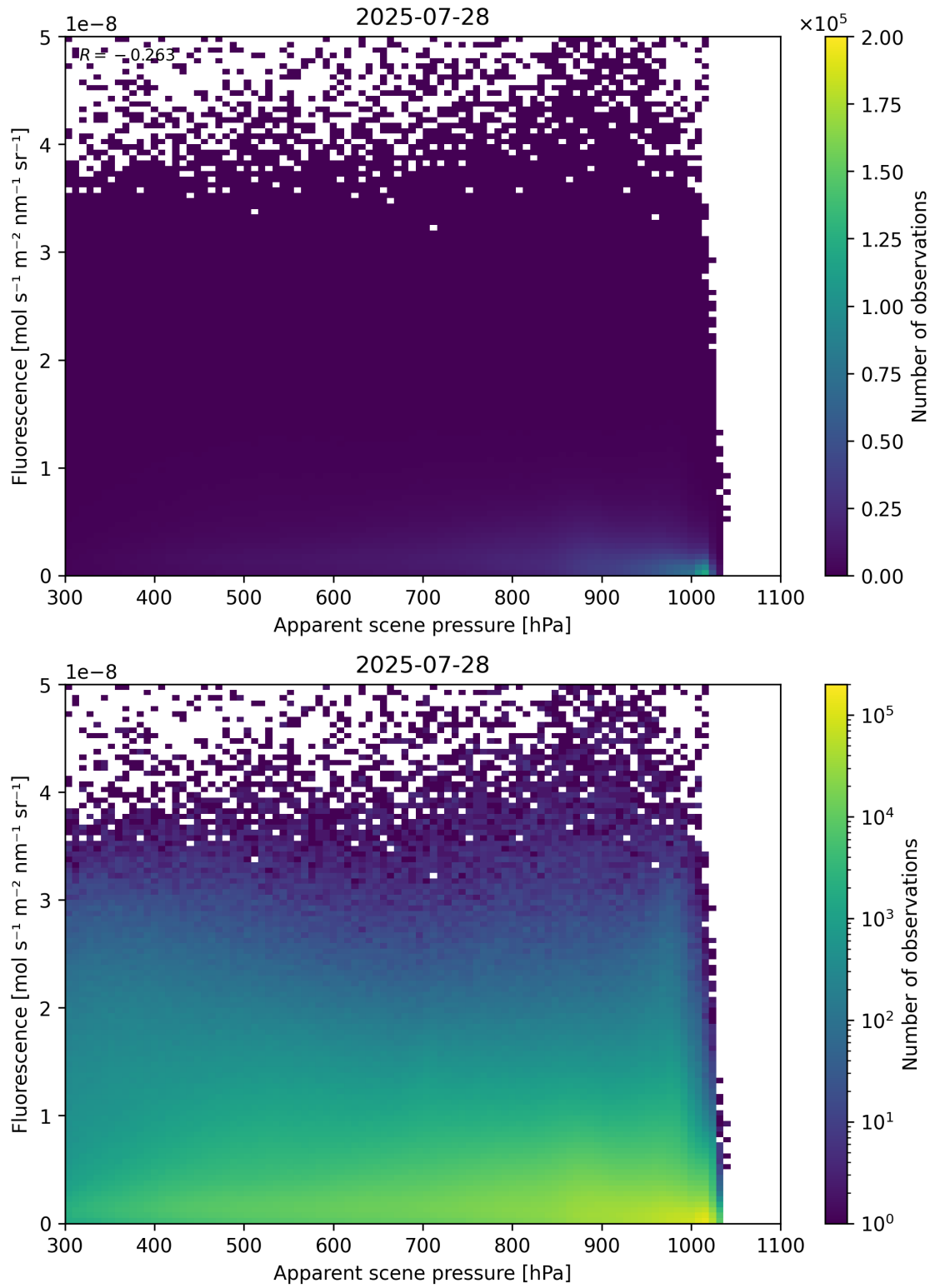
Figure 64: Scatter density plot of “Apparent scene pressure” against “Fluorescence” for 2025-07-27 to 2025-07-29.
