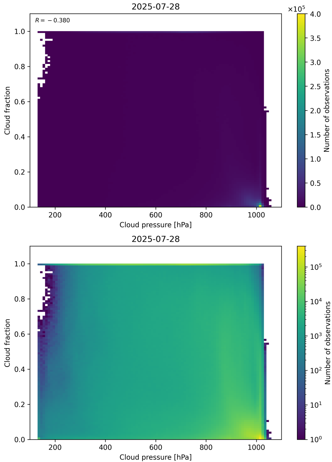
Figure 79: Scatter density plot of “Cloud pressure” against “Cloud fraction” for 2025-07-27 to 2025-07-29.
