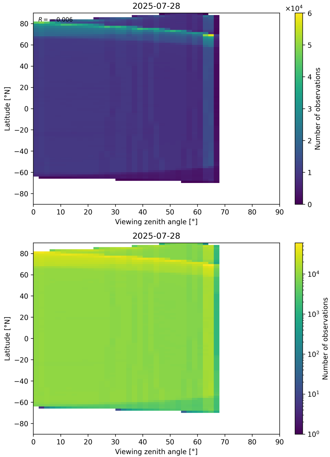
Figure 123: Scatter density plot of “Viewing zenith angle” against “Latitude” for 2025-07-27 to 2025-07-29.
