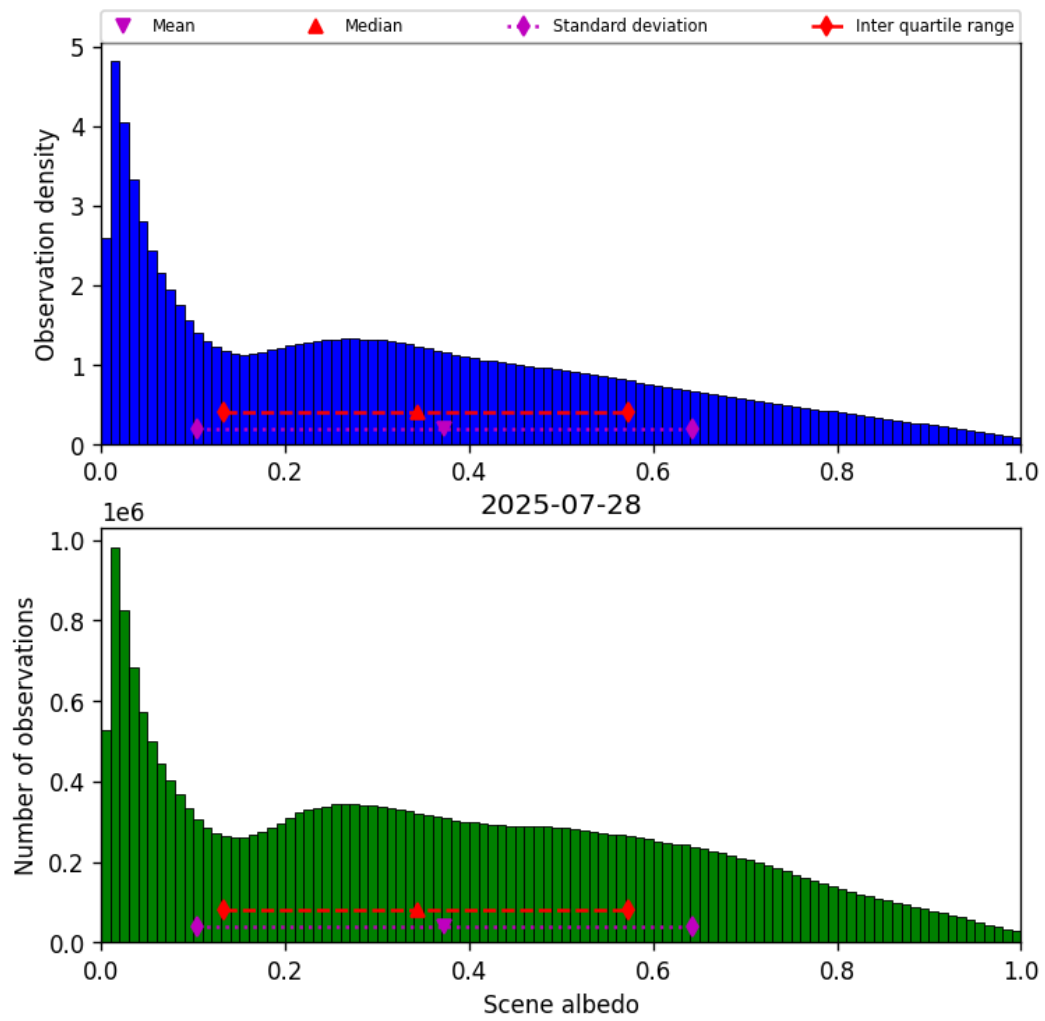
Figure 34: Histogram of “Scene albedo” for 2025-07-27 to 2025-07-29
