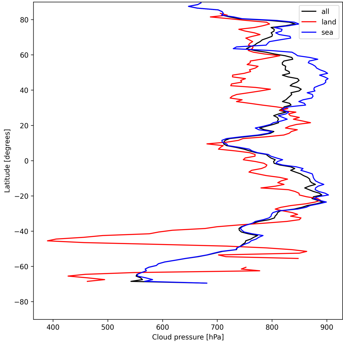
Figure 13: Zonal average of “Cloud pressure” for 2025-07-27 to 2025-07-29.
