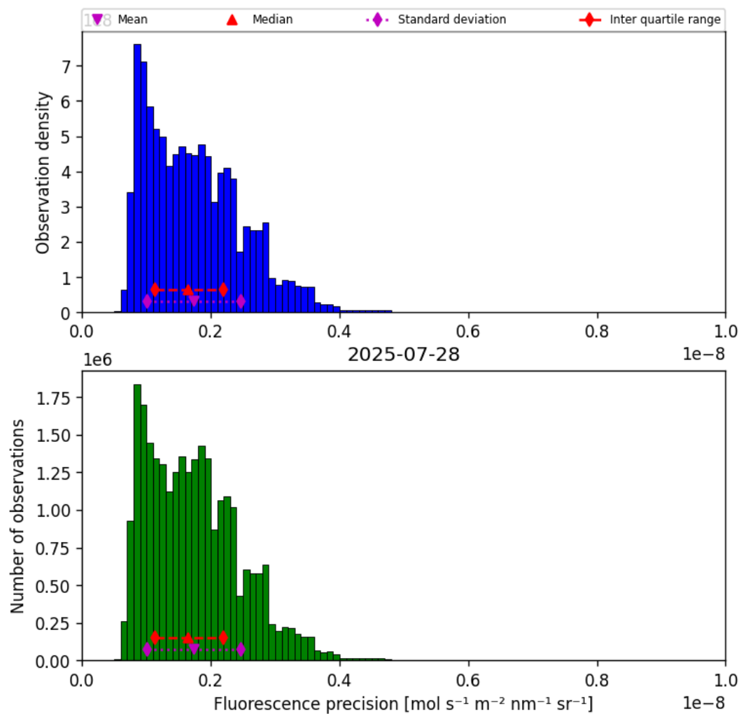
Figure 41: Histogram of “Fluorescence precision” for 2025-07-27 to 2025-07-29
