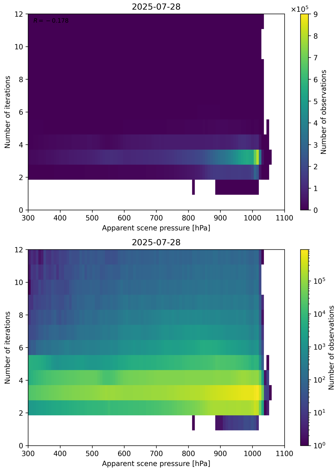
Figure 65: Scatter density plot of “Apparent scene pressure” against “Number of iterations” for 2025-07-27 to 2025-07-29.
