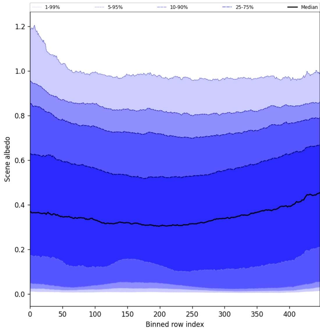
Figure 51: Along track statistics of “Scene albedo” for 2025-07-27 to 2025-07-29
