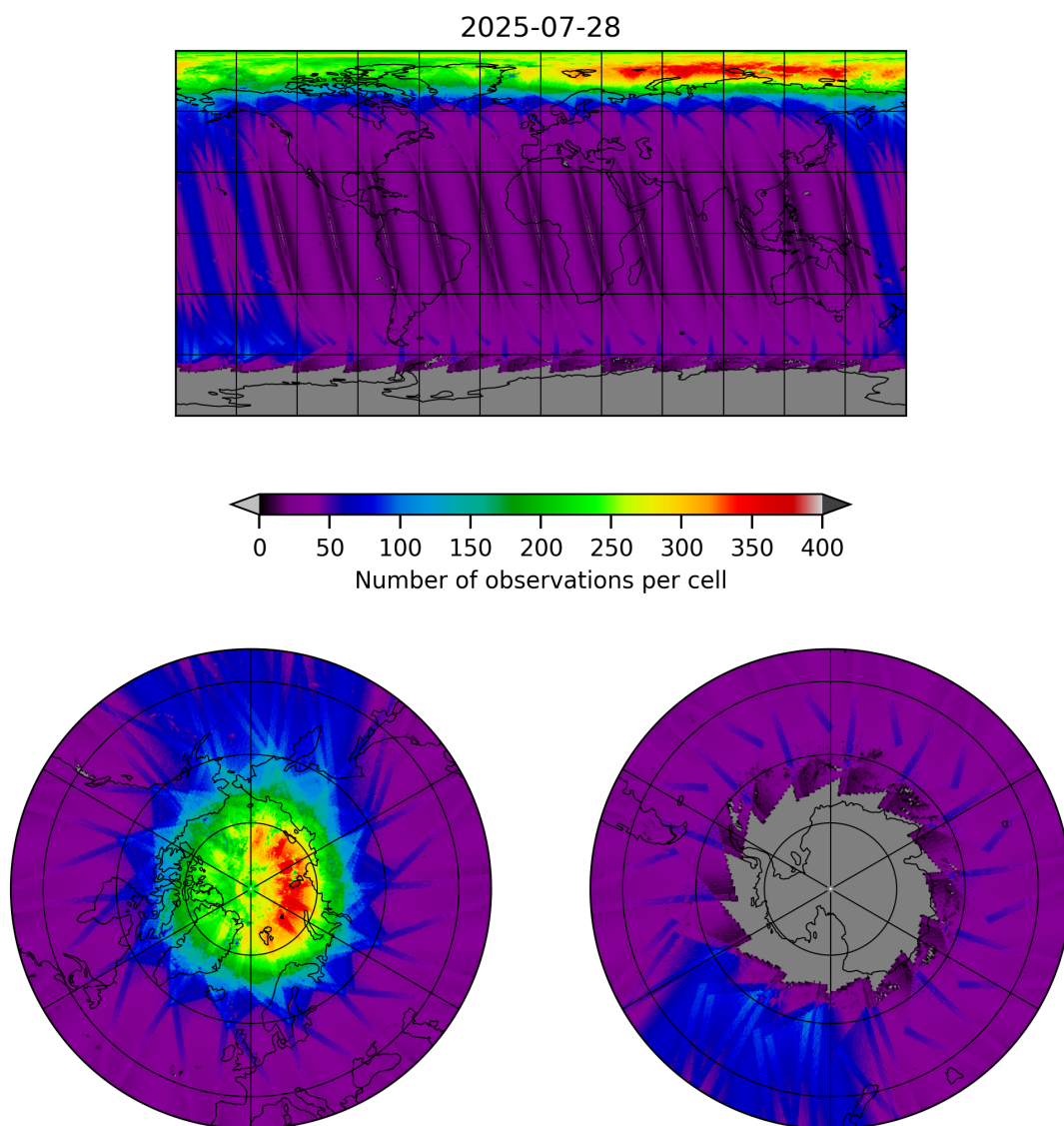
Figure 11: Map of the number of observations for 2025-07-27 to 2025-07-29
