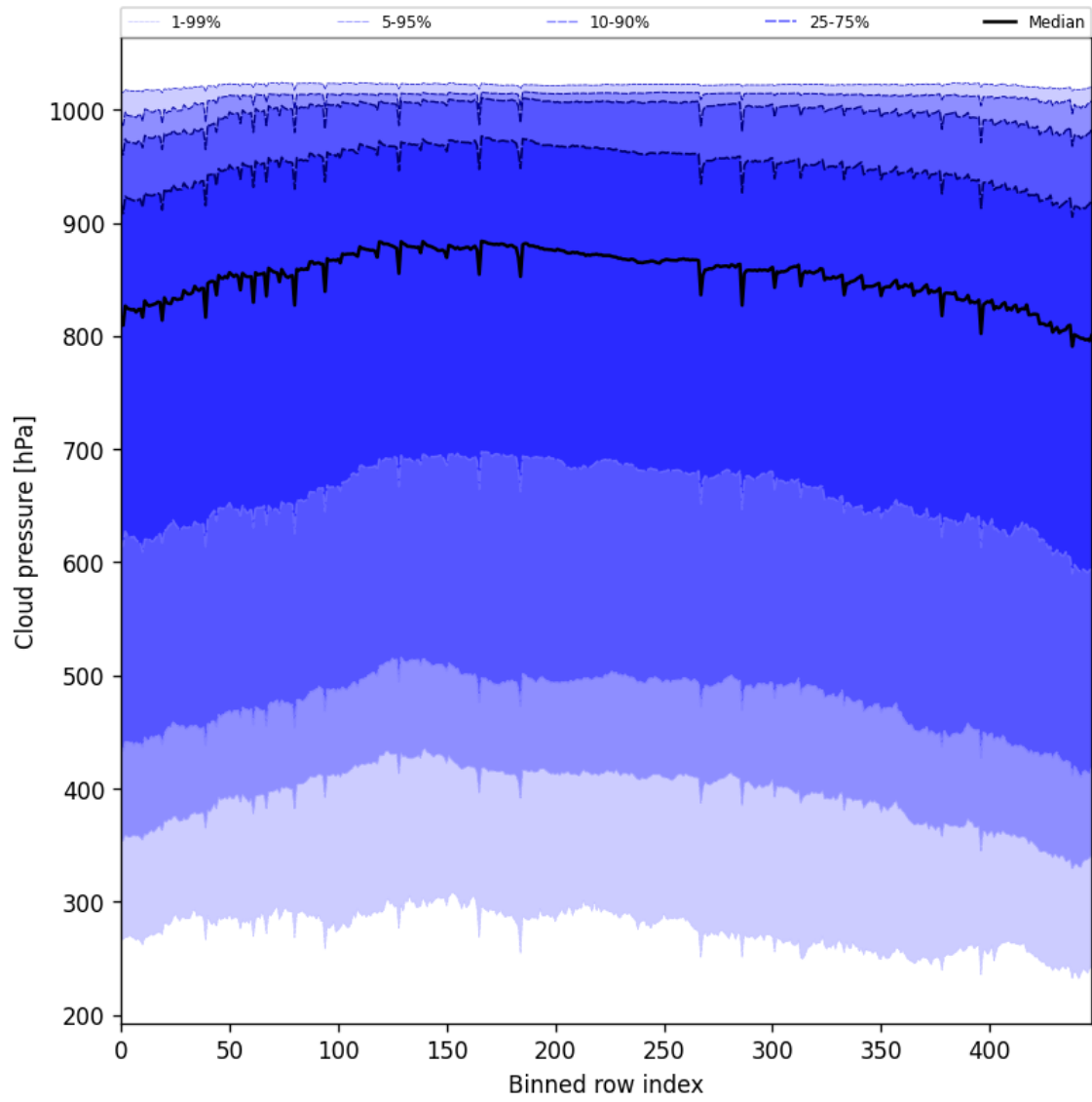
Figure 47: Along track statistics of “Cloud pressure” for 2025-07-27 to 2025-07-29
