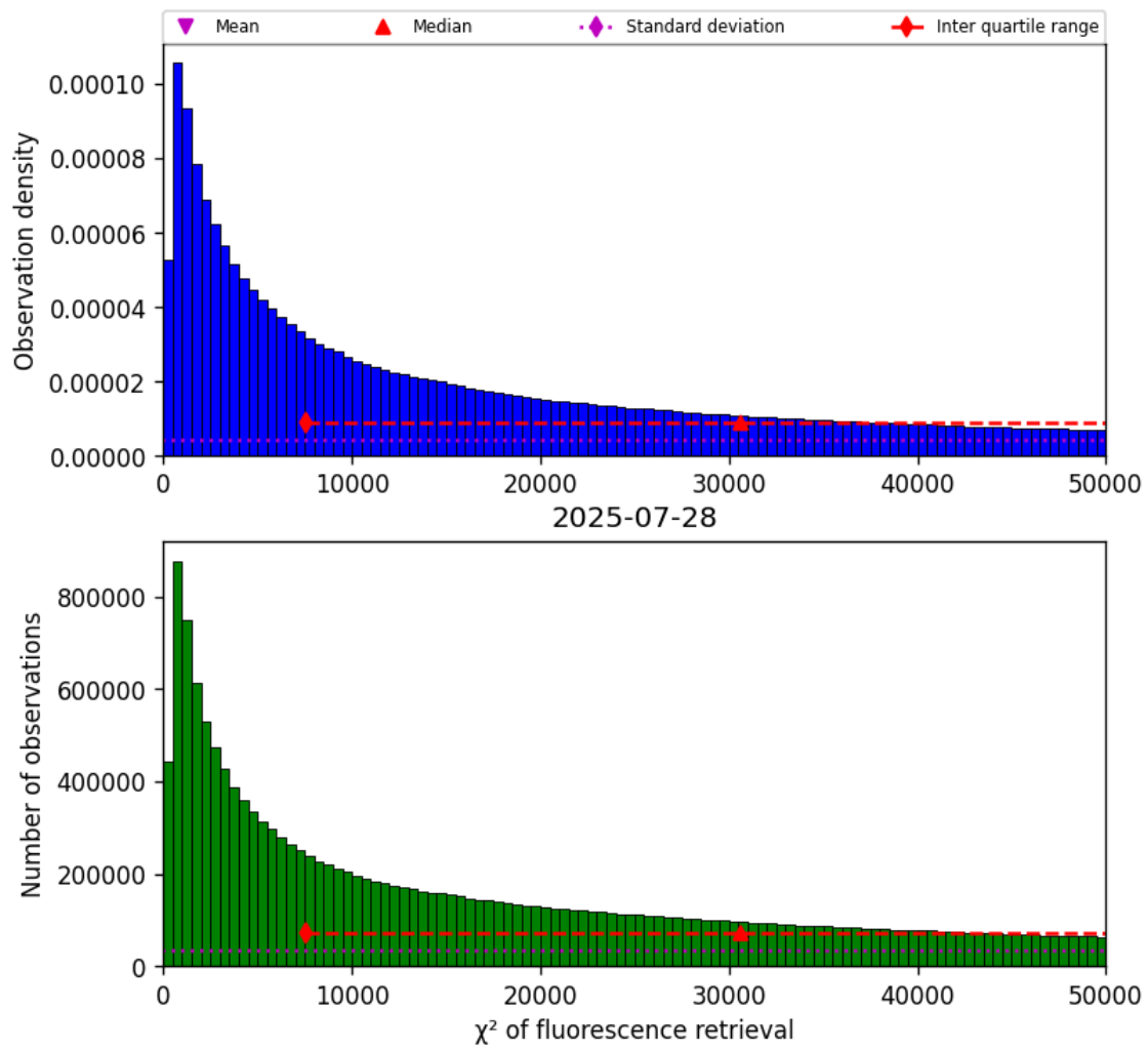
Figure 42: Histogram of “ \chi^2 of fluorescence retrieval” for 2025-07-27 to 2025-07-29
