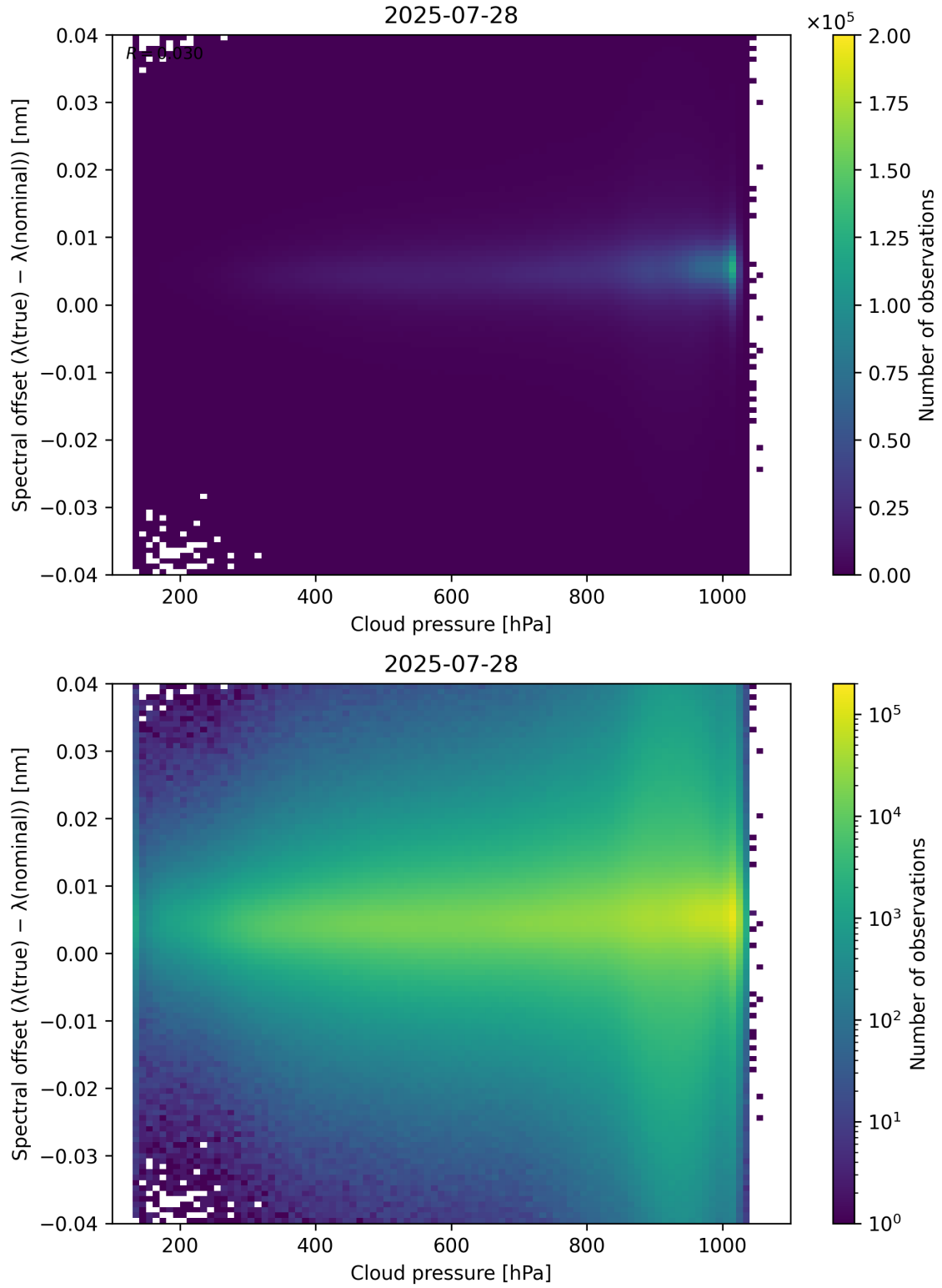
Figure 84: Scatter density plot of “Cloud pressure” against “Spectral offset ( \lambda_{\text{true}} - \lambda_{\text{nominal}} )” for 2025-07-27 to 2025-07-29.
