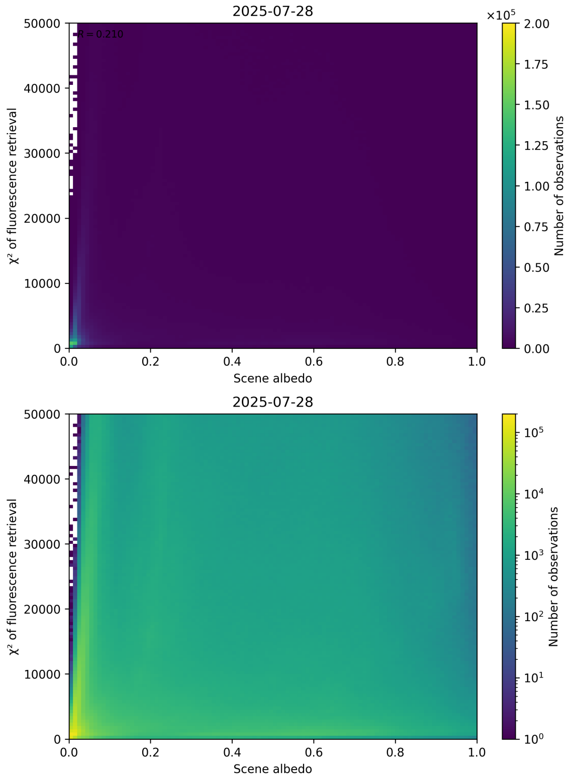
Figure 103: Scatter density plot of “Scene albedo” against “ \chi^2 of fluorescence retrieval” for 2025-07-27 to 2025-07-29.
