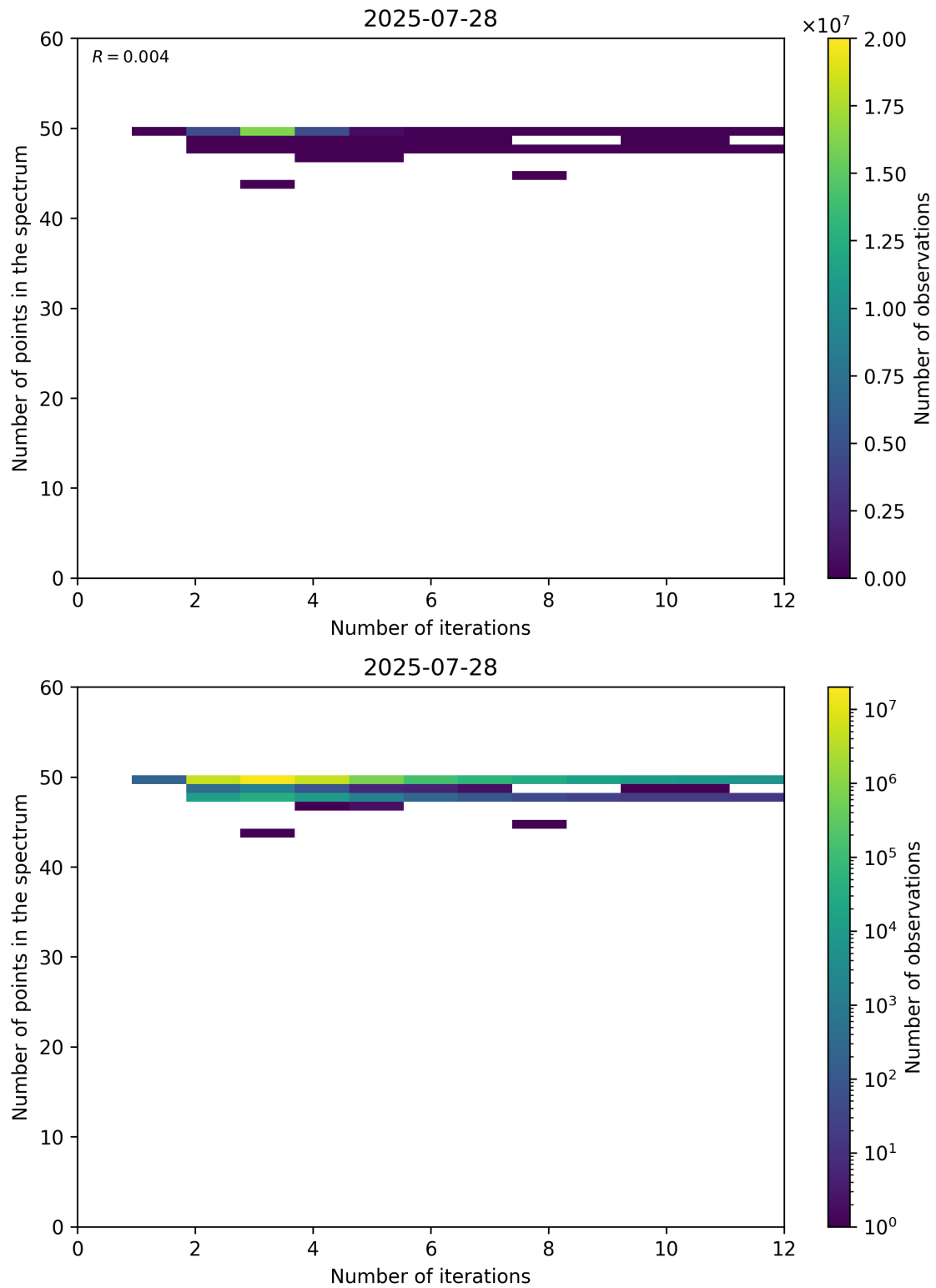
Figure 99: Scatter density plot of “Number of iterations” against “Number of points in the spectrum” for 2025-07-27 to 2025-07-29.
