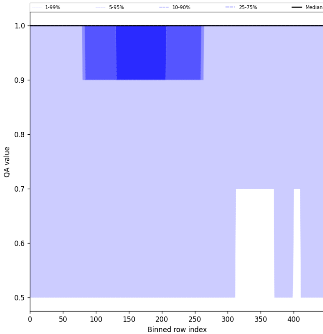
Figure 46: Along track statistics of “QA value” for 2025-07-27 to 2025-07-29
