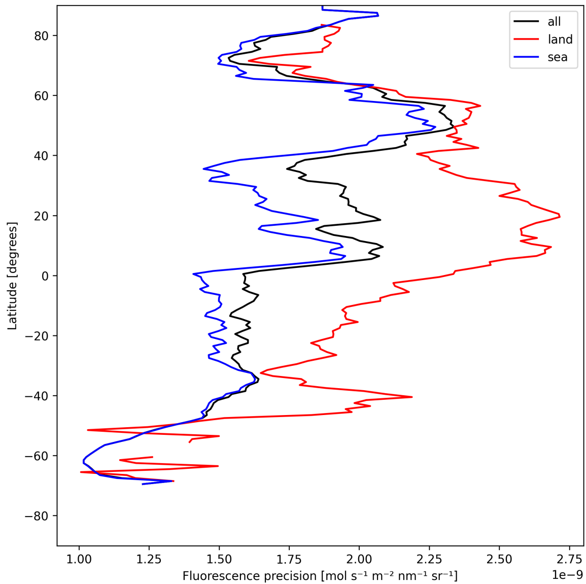
Figure 24: Zonal average of “Fluorescence precision” for 2025-07-27 to 2025-07-29.
