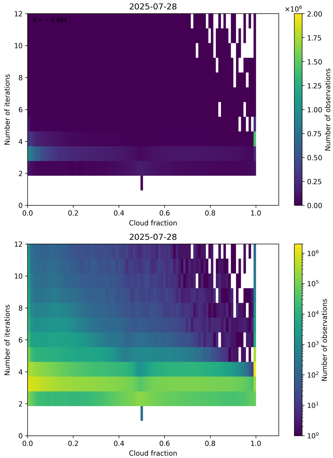
Figure 73: Scatter density plot of “Cloud fraction” against “Number of iterations” for 2025-07-27 to 2025-07-29.
