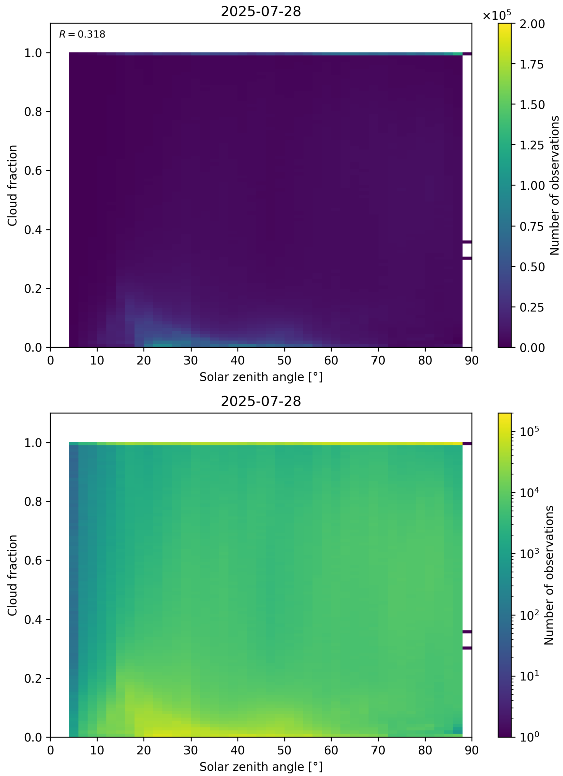
Figure 110: Scatter density plot of “Solar zenith angle” against “Cloud fraction” for 2025-07-27 to 2025-07-29.
