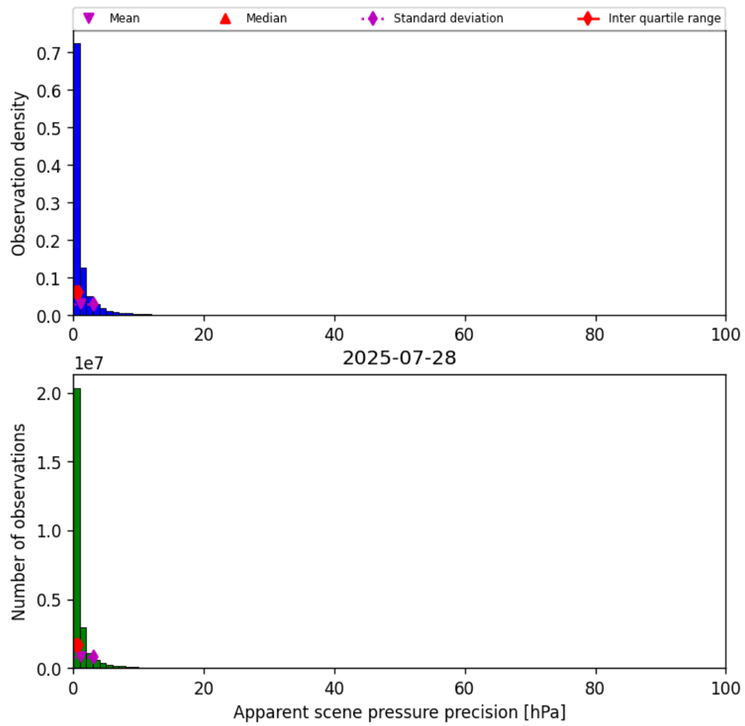
Figure 37: Histogram of “Apparent scene pressure precision” for 2025-07-27 to 2025-07-29
