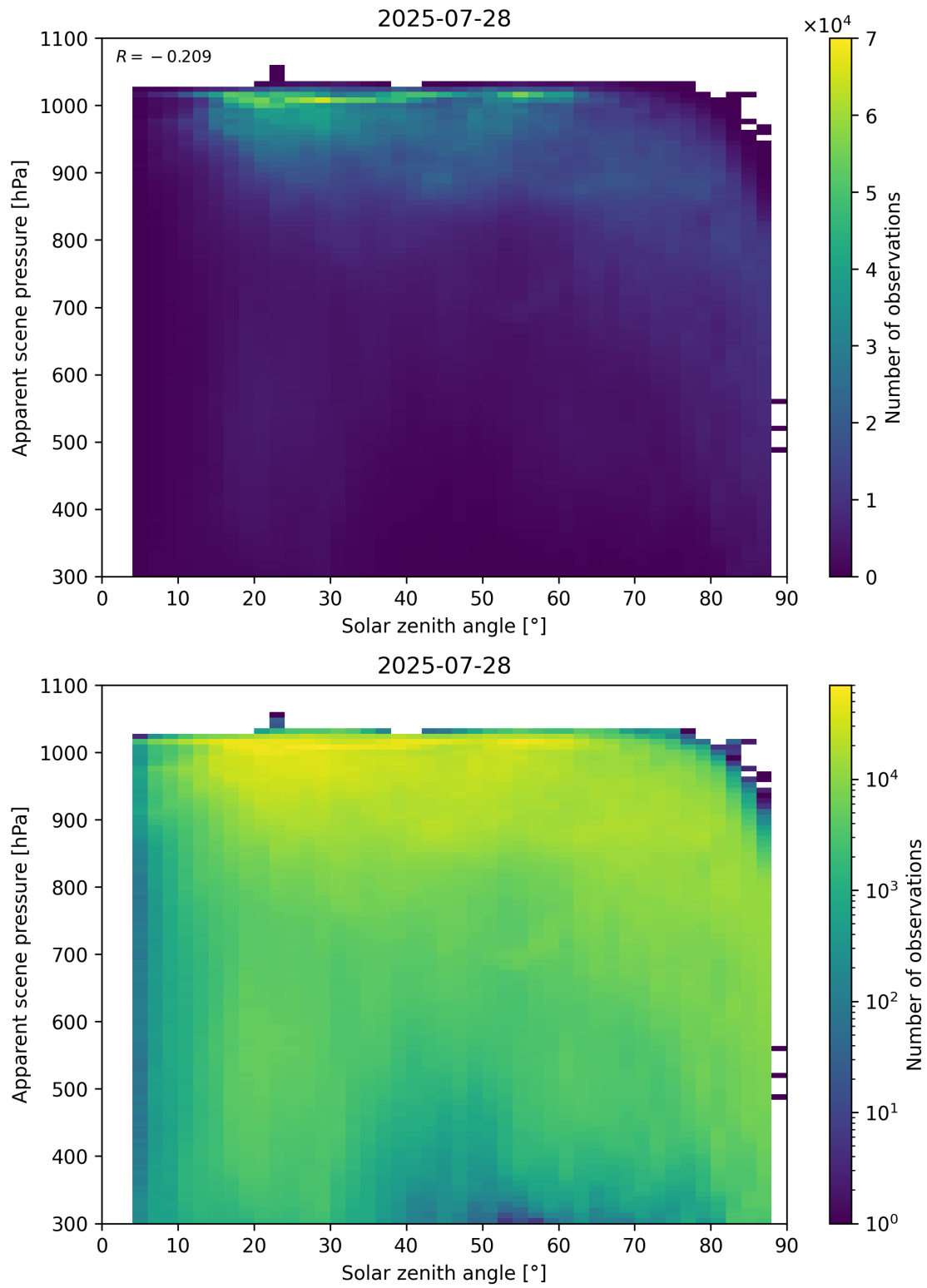
Figure 108: Scatter density plot of “Solar zenith angle” against “Apparent scene pressure” for 2025-07-27 to 2025-07-29.
