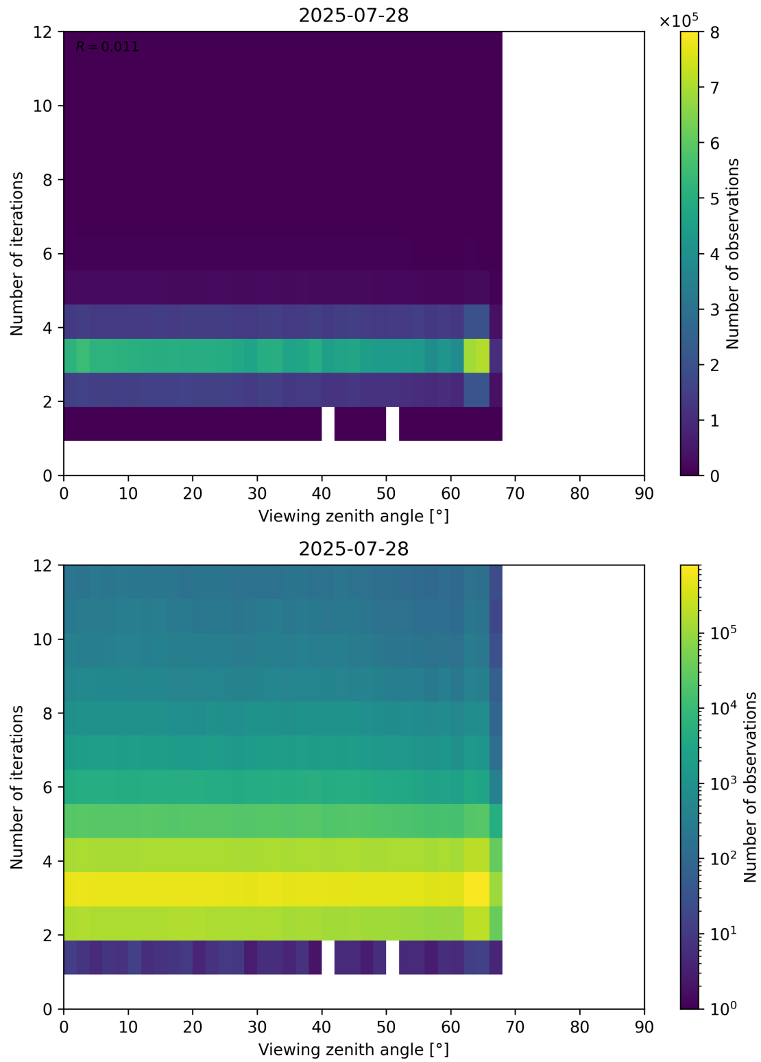
Figure 124: Scatter density plot of “Viewing zenith angle” against “Number of iterations” for 2025-07-27 to 2025-07-29.
