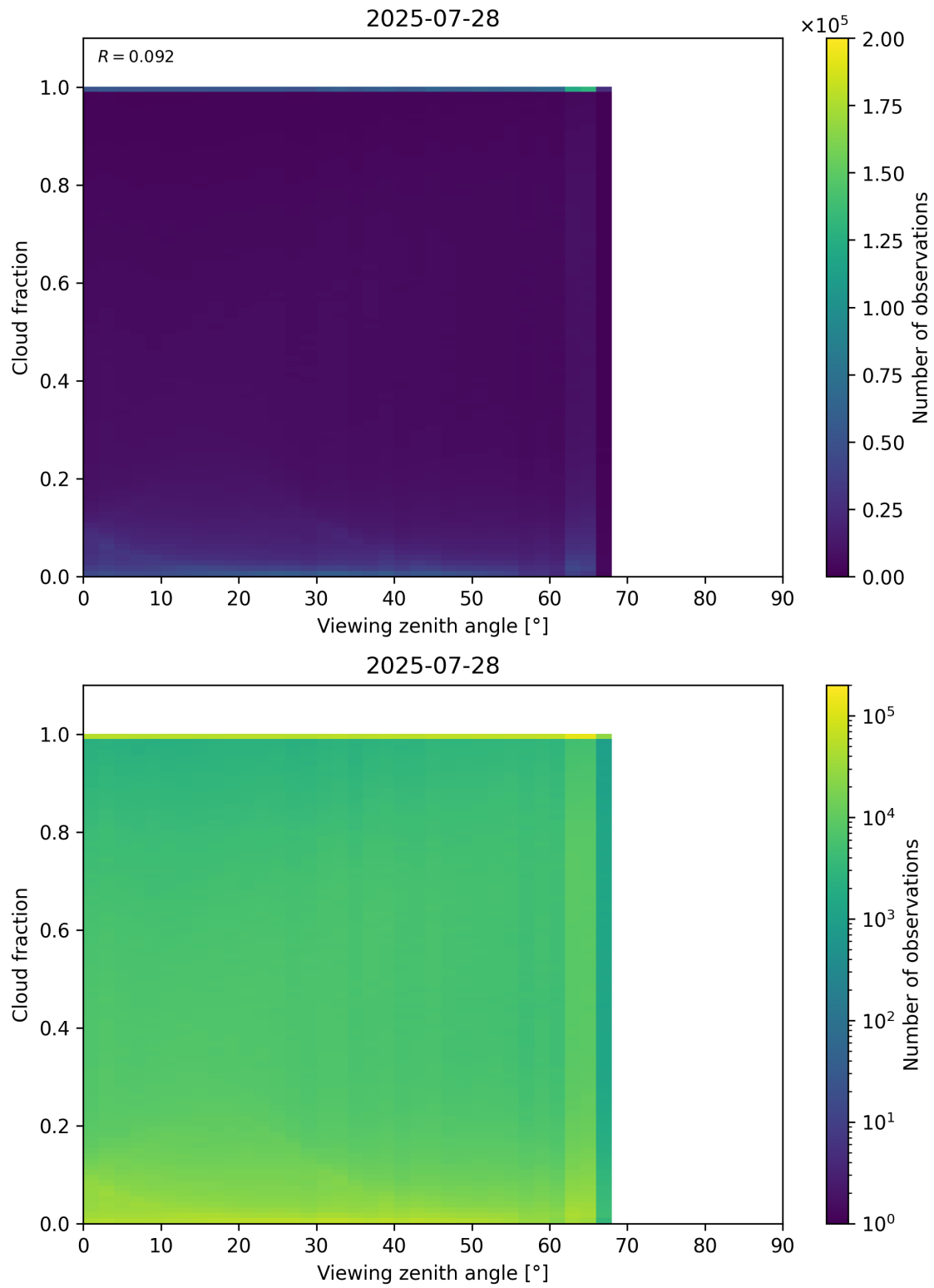
Figure 120: Scatter density plot of “Viewing zenith angle” against “Cloud fraction” for 2025-07-27 to 2025-07-29.
