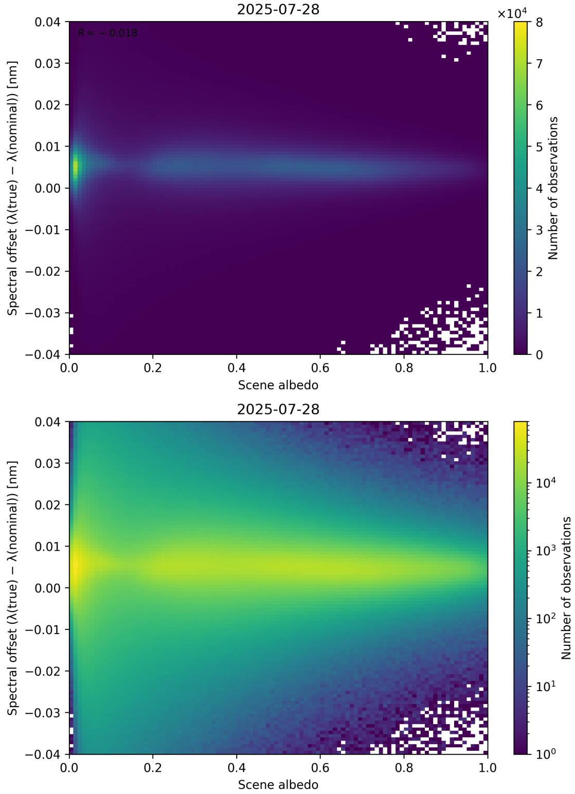
Figure 107: Scatter density plot of “Scene albedo” against “Spectral offset ( \lambda_{\text{true}} - \lambda_{\text{nominal}} )” for 2025-07-27 to 2025-07-29.
