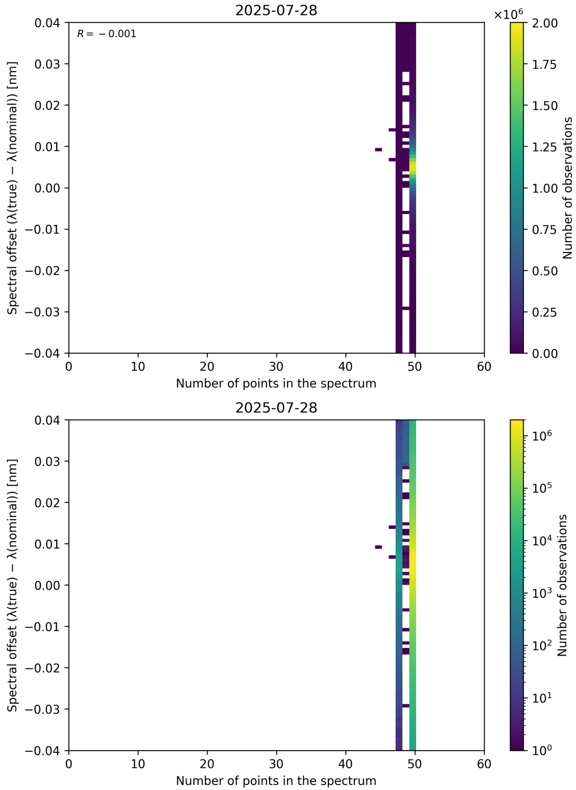
Figure 101: Scatter density plot of “Number of points in the spectrum” against “Spectral offset ( \lambda_{\text{true}} - \lambda_{\text{nominal}} )” for 2025-07-27 to 2025-07-29.
