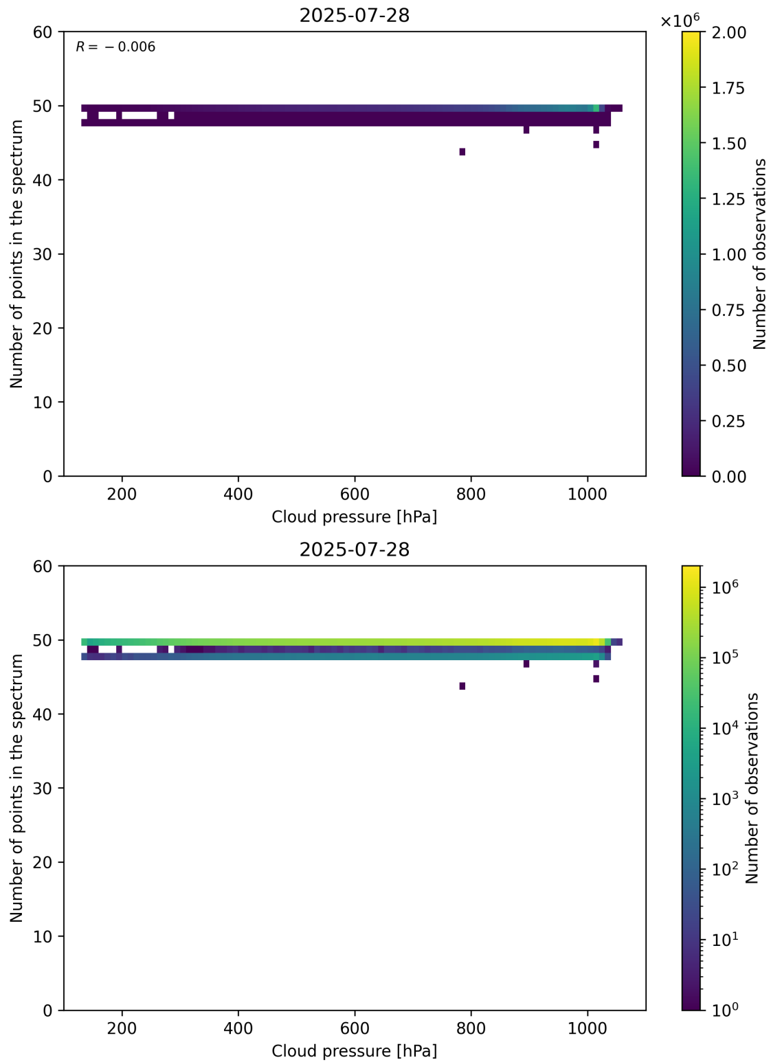
Figure 82: Scatter density plot of “Cloud pressure” against “Number of points in the spectrum” for 2025-07-27 to 2025-07-29.
