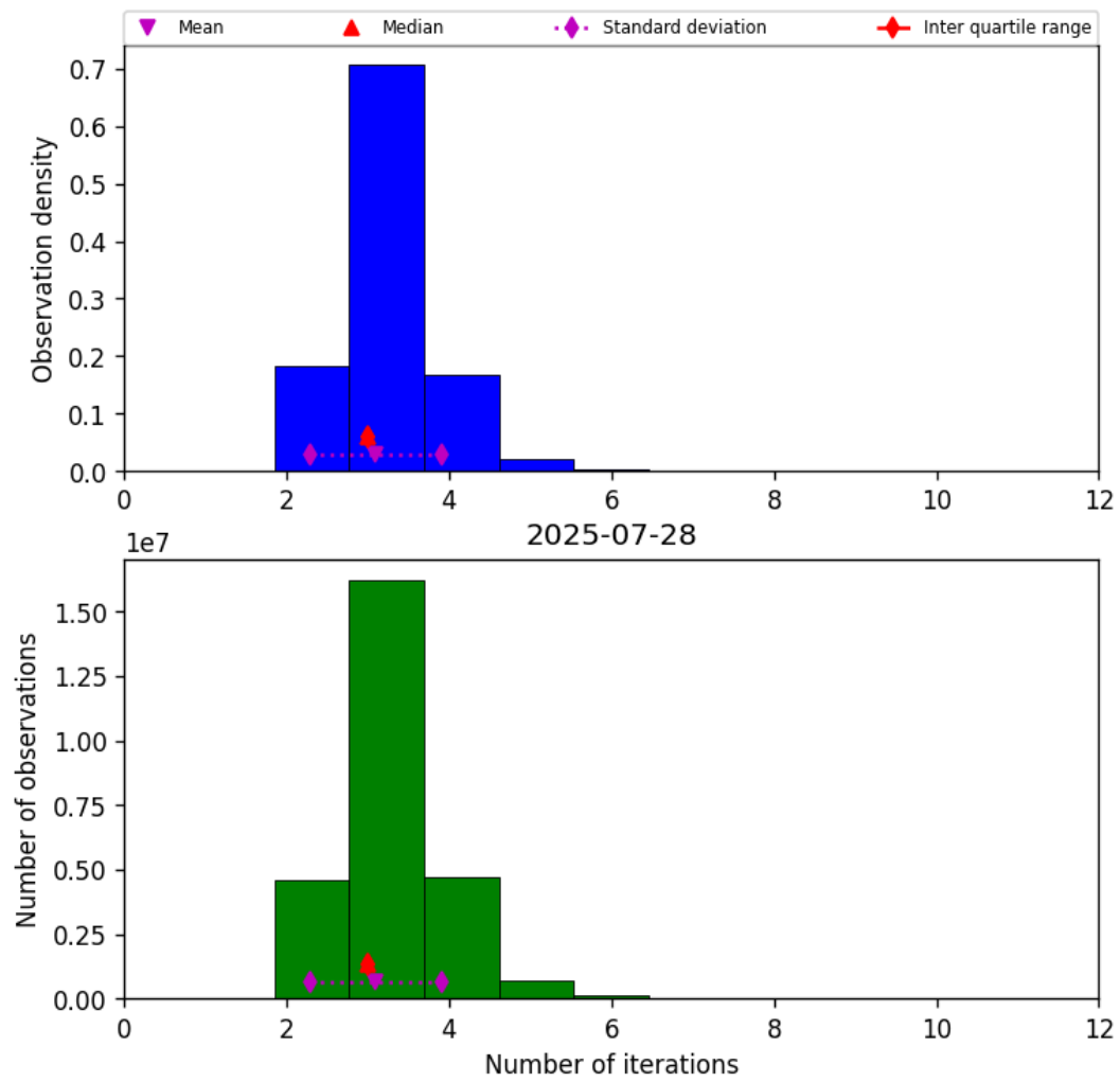
Figure 39: Histogram of “Number of iterations” for 2025-07-27 to 2025-07-29
