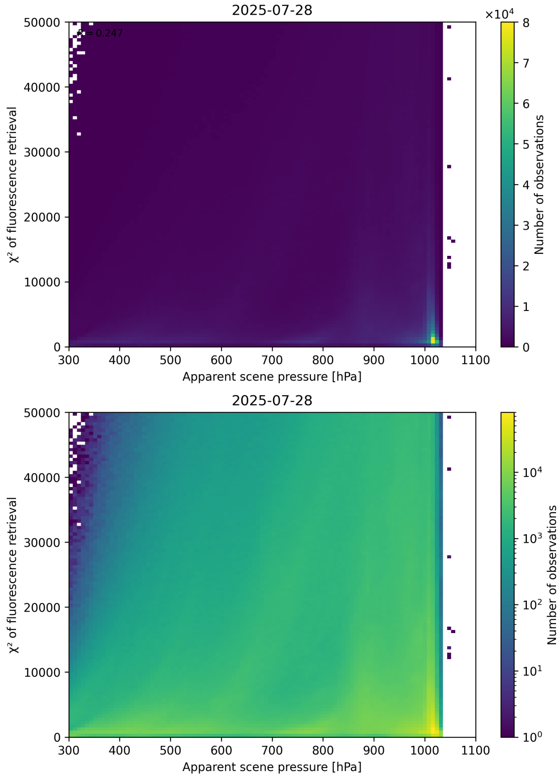
Figure 63: Scatter density plot of “Apparent scene pressure” against “ \chi^2 of fluorescence retrieval” for 2025-07-27 to 2025-07-29.
