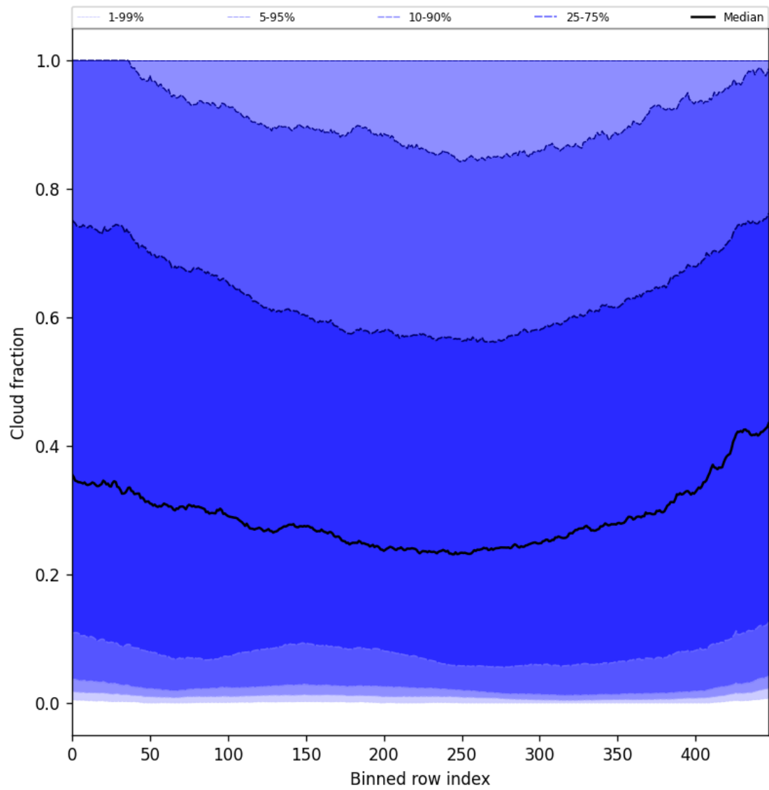
Figure 49: Along track statistics of “Cloud fraction” for 2025-07-27 to 2025-07-29
