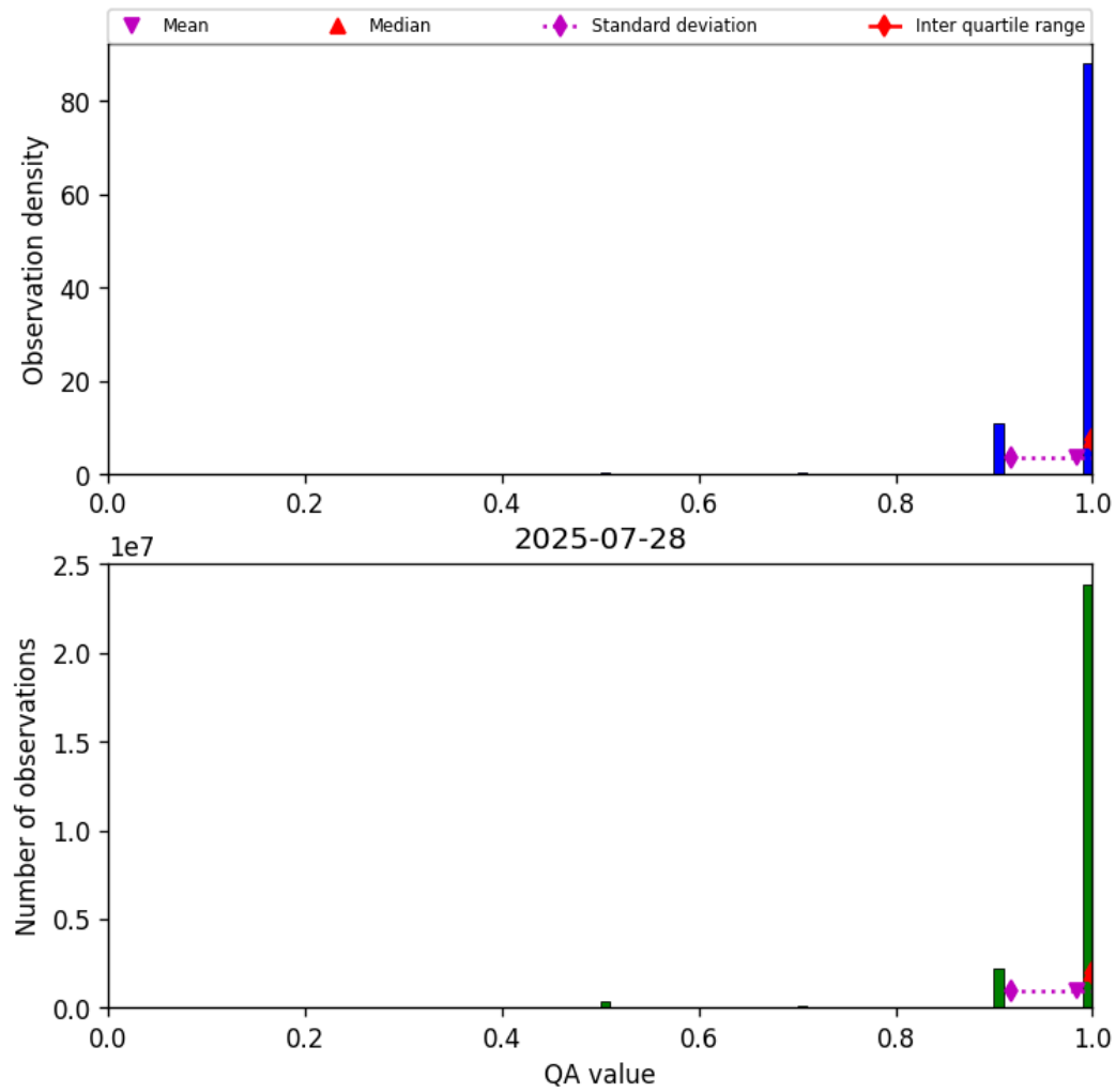
Figure 29: Histogram of “QA value” for 2025-07-27 to 2025-07-29
