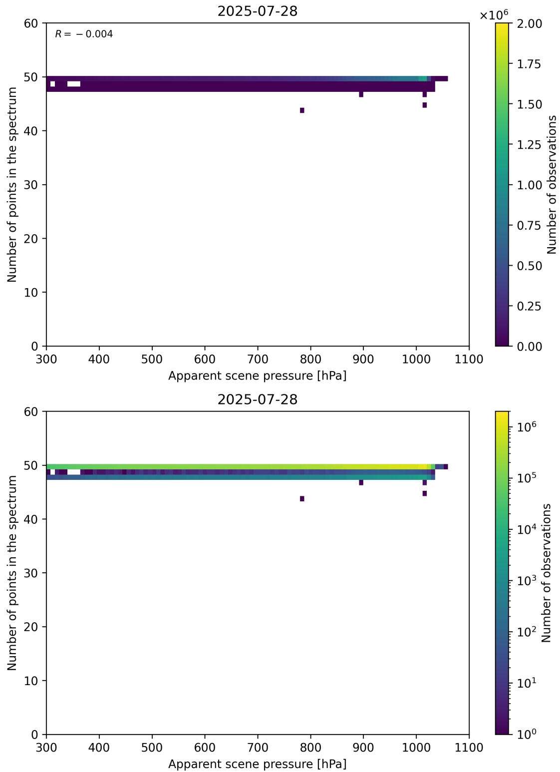
Figure 66: Scatter density plot of “Apparent scene pressure” against “Number of points in the spectrum” for 2025-07-27 to 2025-07-29.
