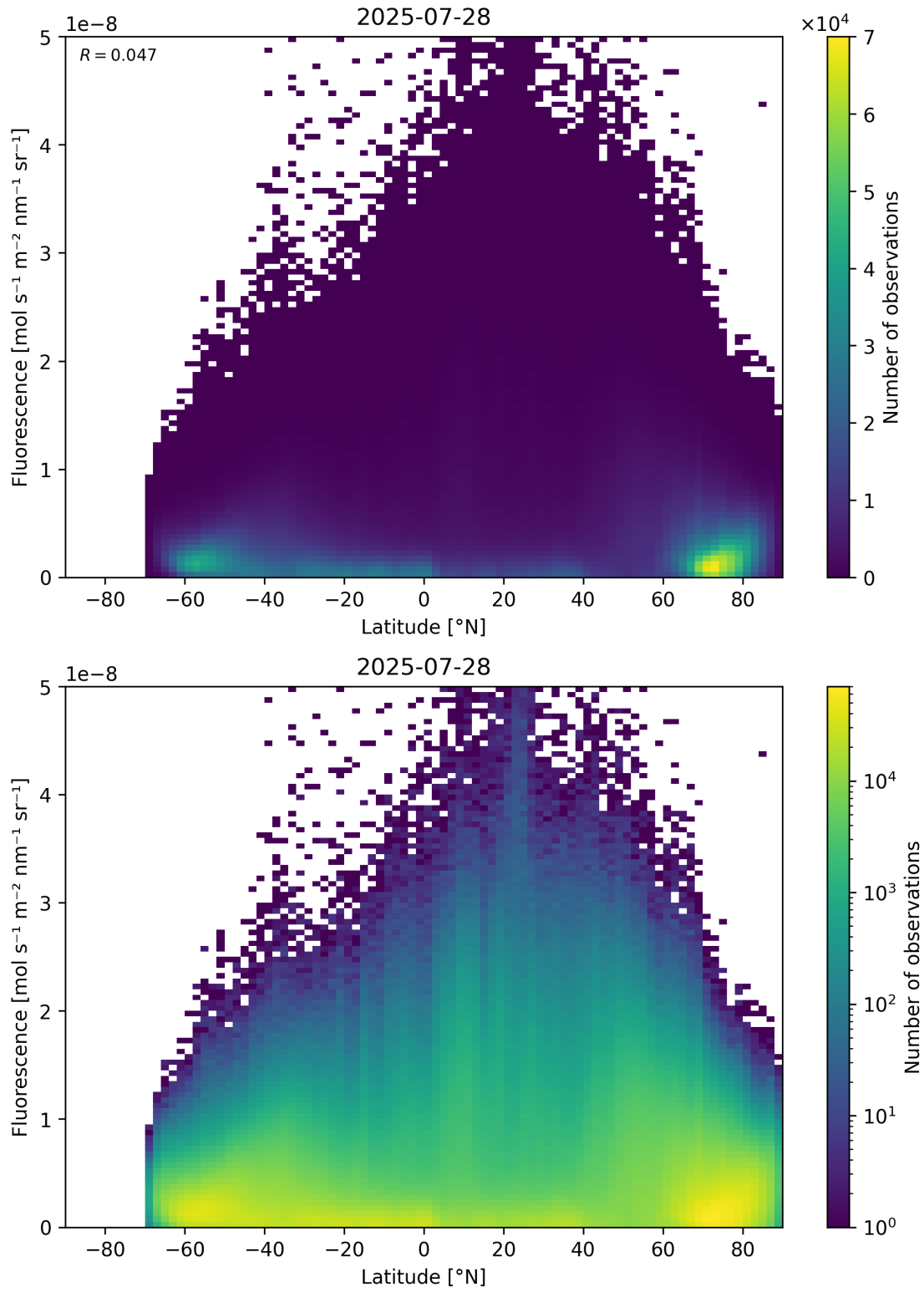
Figure 92: Scatter density plot of “Latitude” against “Fluorescence” for 2025-07-27 to 2025-07-29.
