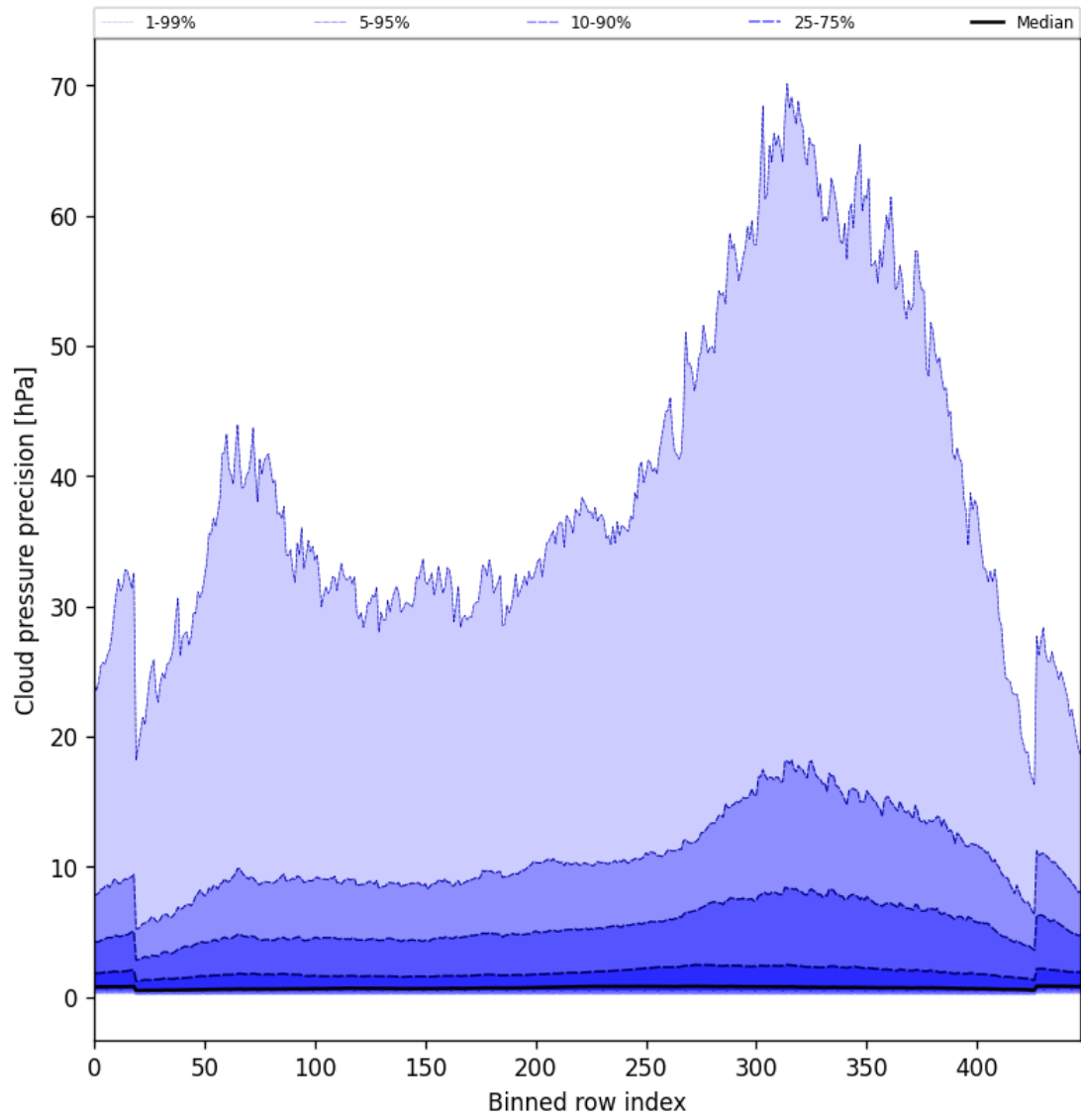
Figure 48: Along track statistics of “Cloud pressure precision” for 2025-07-27 to 2025-07-29
