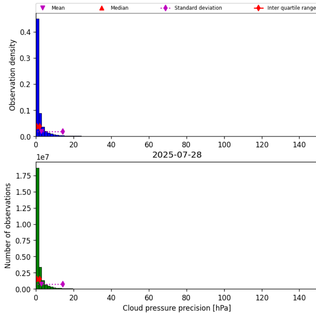
Figure 31: Histogram of “Cloud pressure precision” for 2025-07-27 to 2025-07-29
