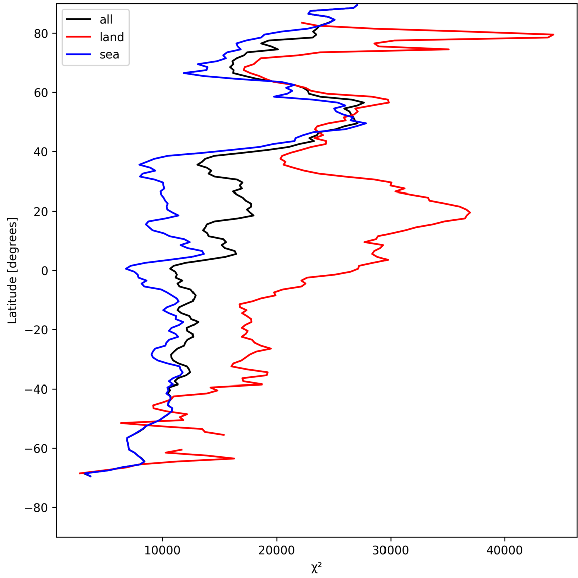
Figure 21: Zonal average of “ \chi^2 ” for 2025-07-27 to 2025-07-29.
