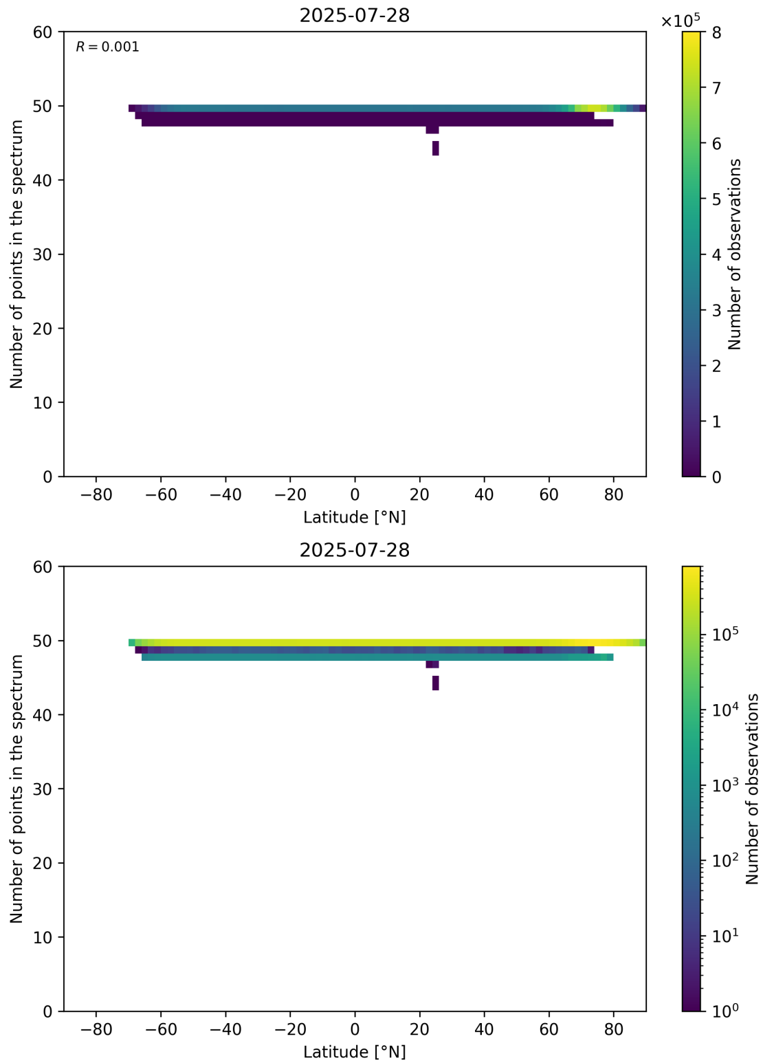
Figure 94: Scatter density plot of “Latitude” against “Number of points in the spectrum” for 2025-07-27 to 2025-07-29.
