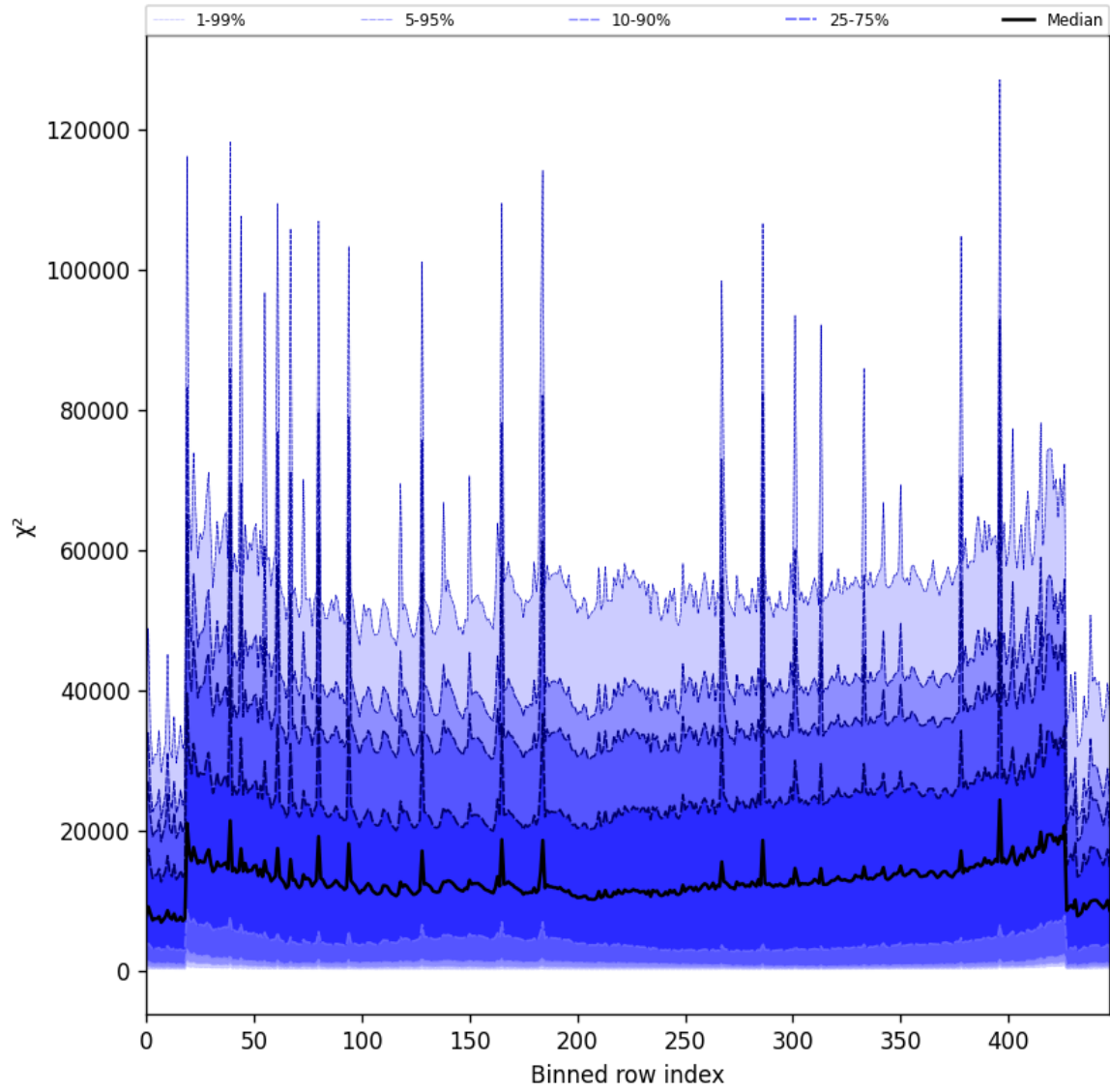
Figure 55: Along track statistics of “ \chi^2 ” for 2025-07-27 to 2025-07-29
