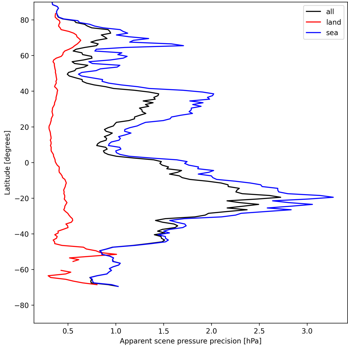
Figure 20: Zonal average of “Apparent scene pressure precision” for 2025-07-27 to 2025-07-29.
