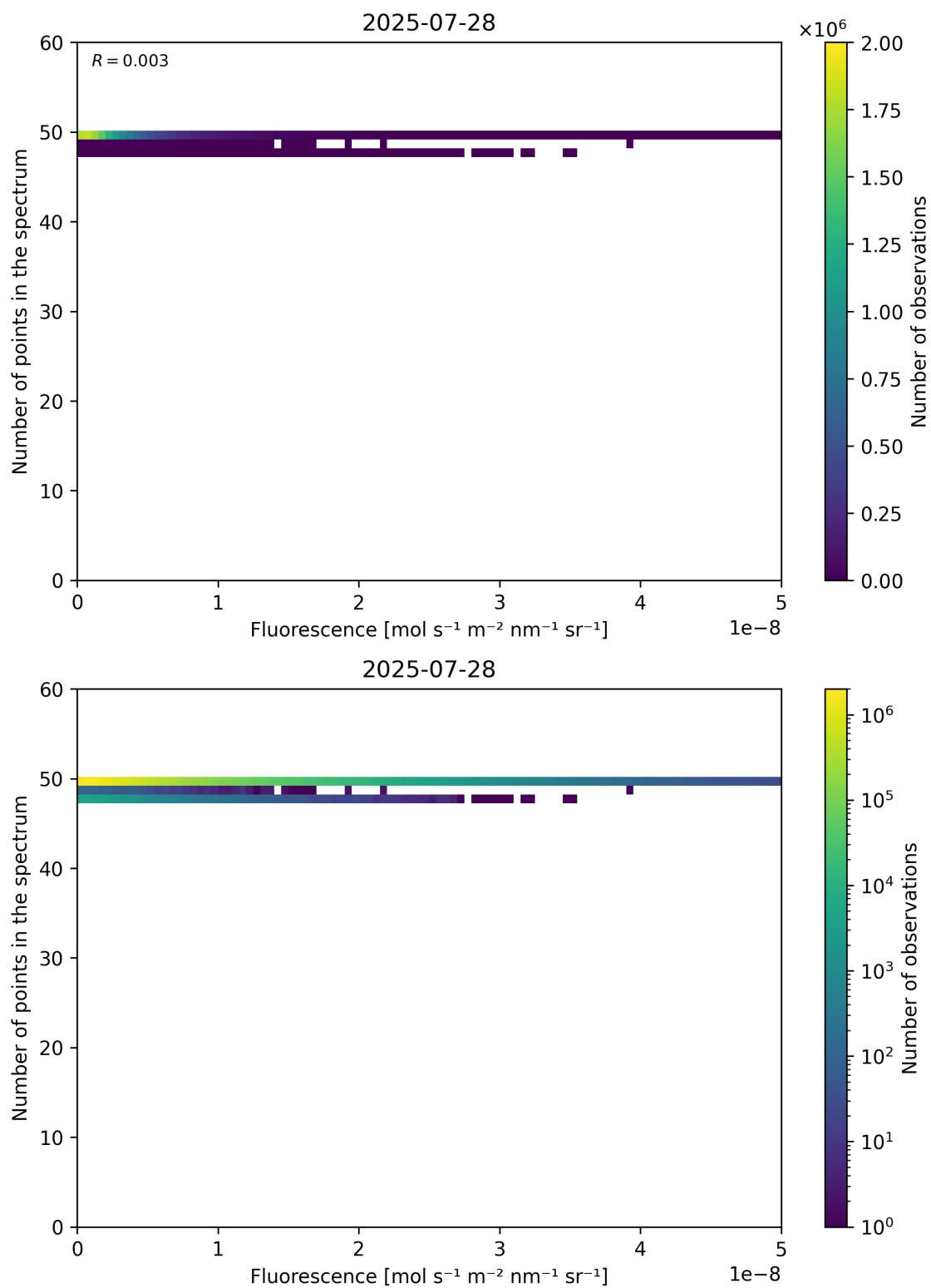
Figure 86: Scatter density plot of “Fluorescence” against “Number of points in the spectrum” for 2025-07-27 to 2025-07-29.
