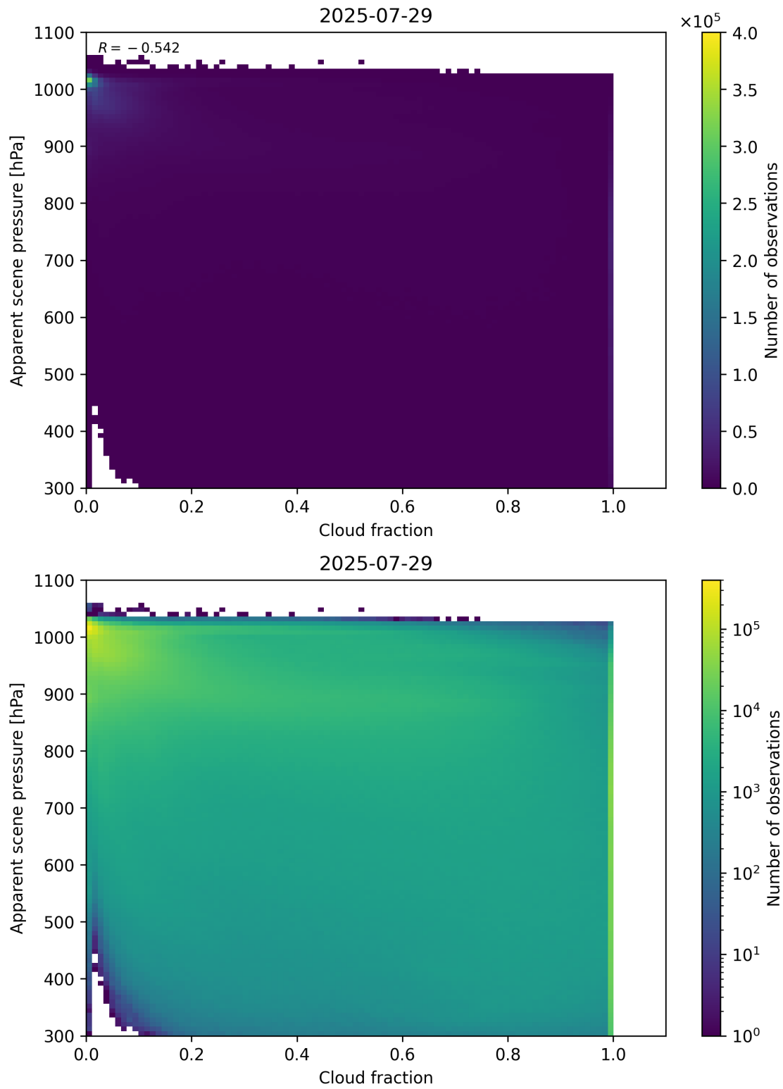
Figure 70: Scatter density plot of “Cloud fraction” against “Apparent scene pressure” for 2025-07-29 to 2025-07-30.
