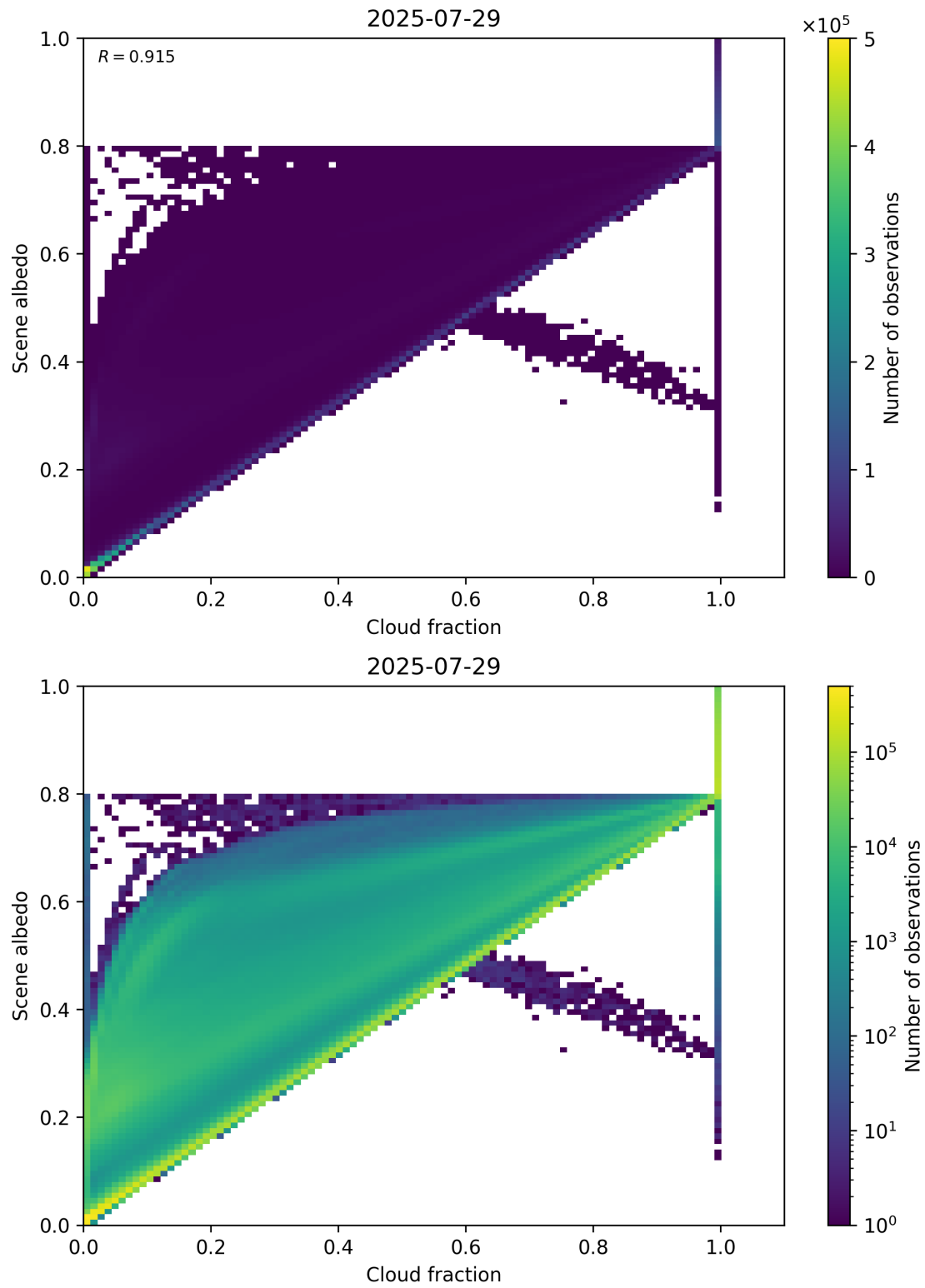
Figure 75: Scatter density plot of “Cloud fraction” against “Scene albedo” for 2025-07-29 to 2025-07-30.
