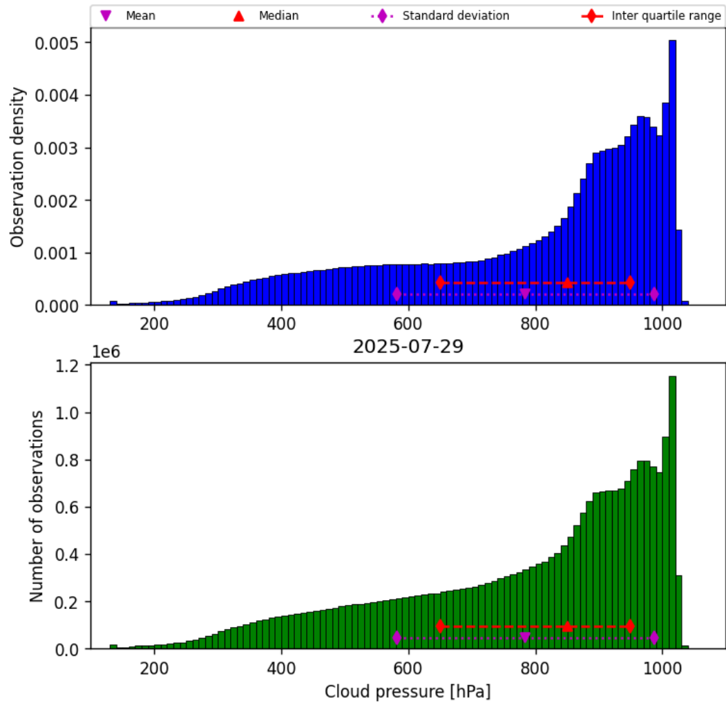
Figure 30: Histogram of “Cloud pressure” for 2025-07-29 to 2025-07-30
