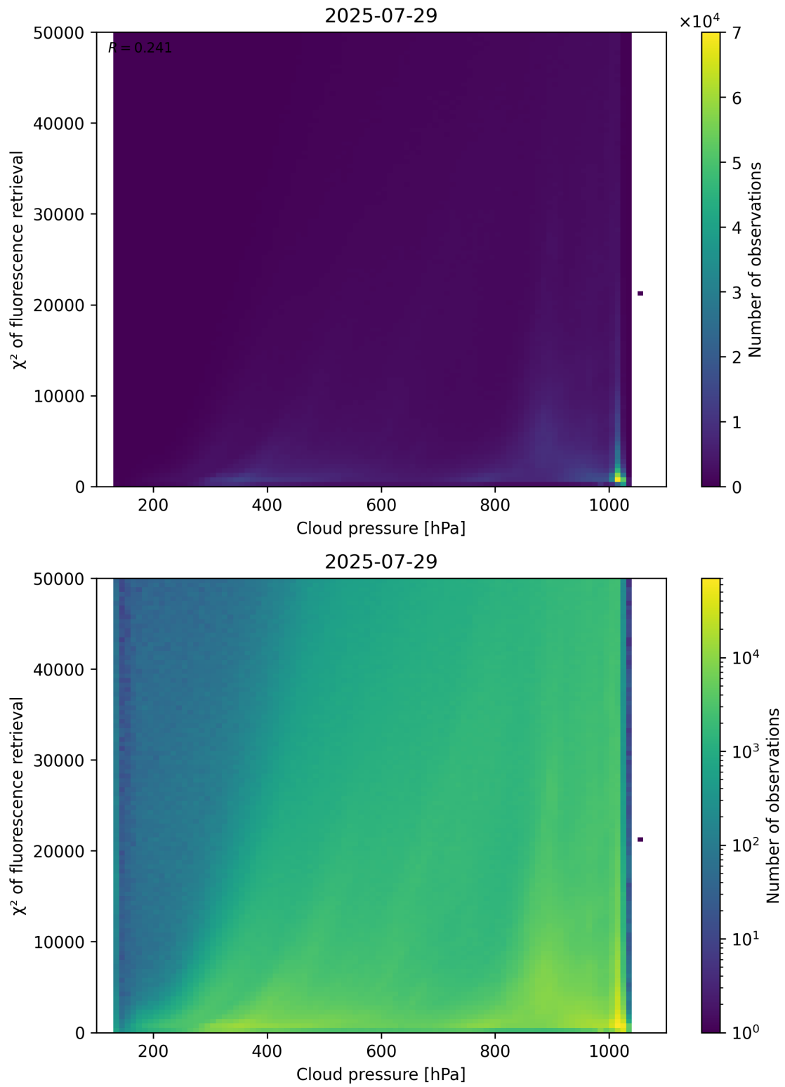
Figure 78: Scatter density plot of “Cloud pressure” against “ \chi^2 of fluorescence retrieval” for 2025-07-29 to 2025-07-30.
