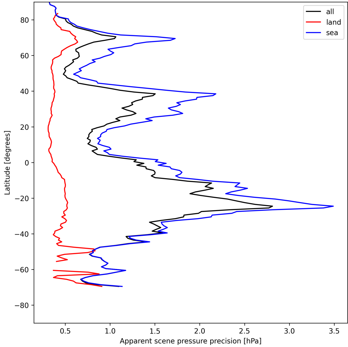
Figure 20: Zonal average of “Apparent scene pressure precision” for 2025-07-29 to 2025-07-30.
