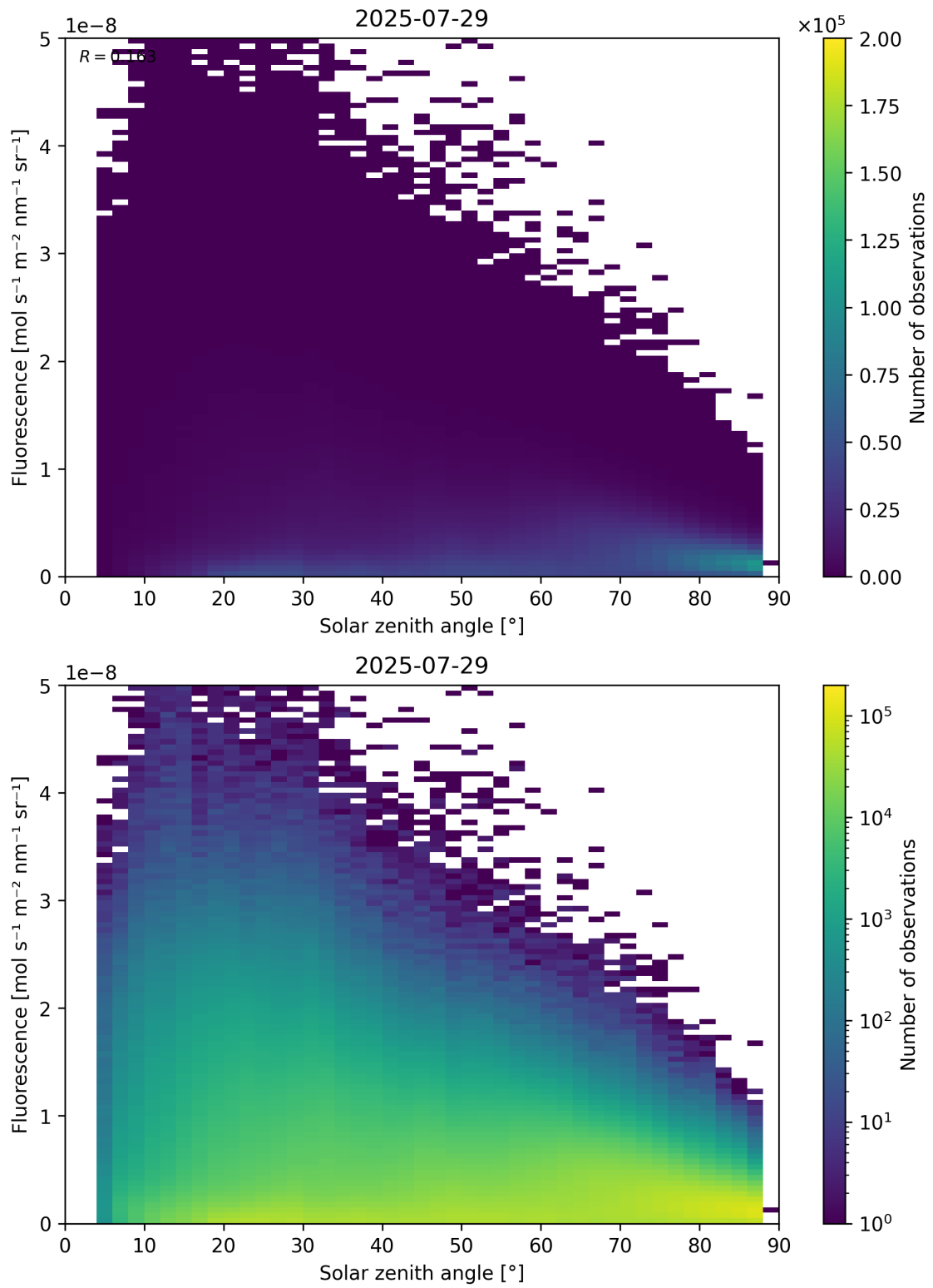
Figure 112: Scatter density plot of “Solar zenith angle” against “Fluorescence” for 2025-07-29 to 2025-07-30.
