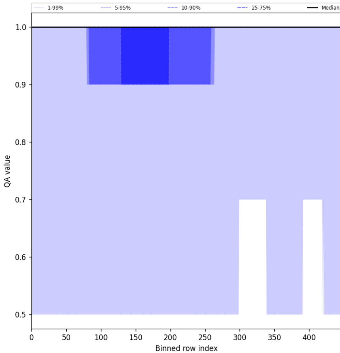
Figure 46: Along track statistics of “QA value” for 2025-07-29 to 2025-07-30
