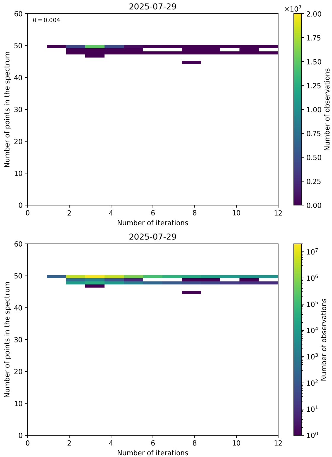
Figure 99: Scatter density plot of “Number of iterations” against “Number of points in the spectrum” for 2025-07-29 to 2025-07-30.
