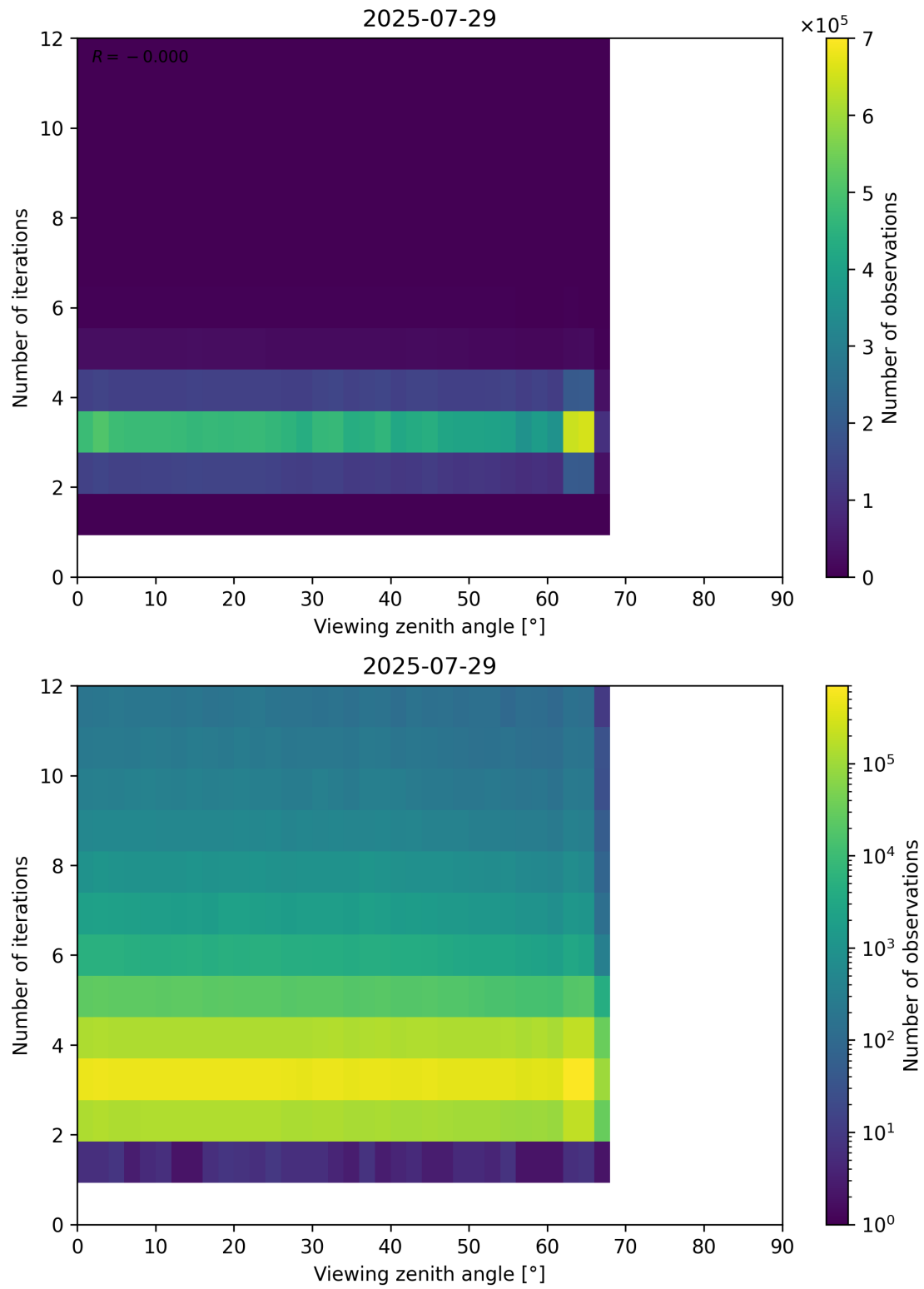
Figure 124: Scatter density plot of “Viewing zenith angle” against “Number of iterations” for 2025-07-29 to 2025-07-30.
