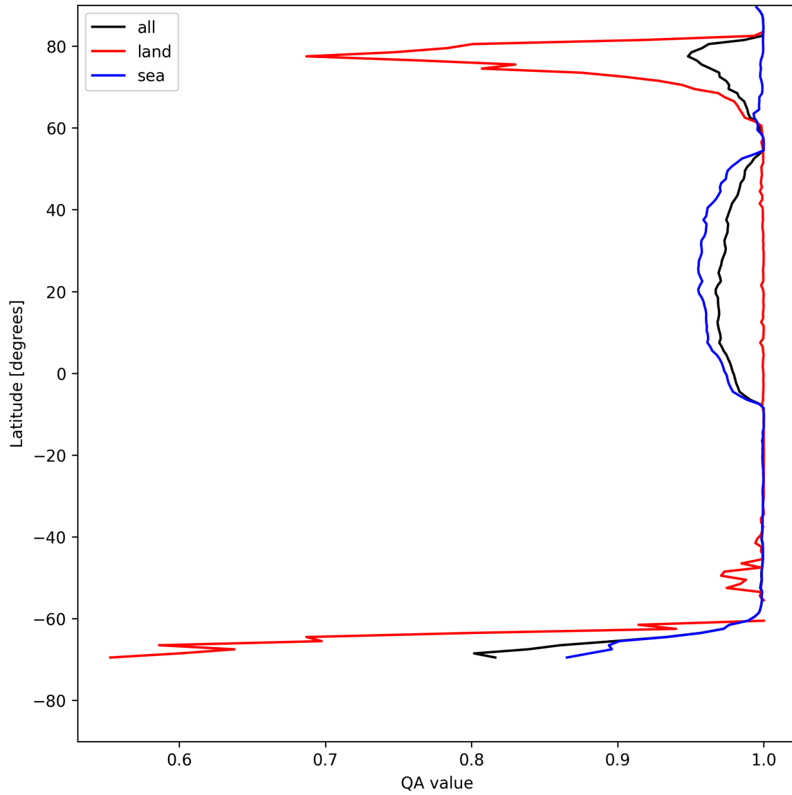
Figure 12: Zonal average of “QA value” for 2025-07-29 to 2025-07-30.
