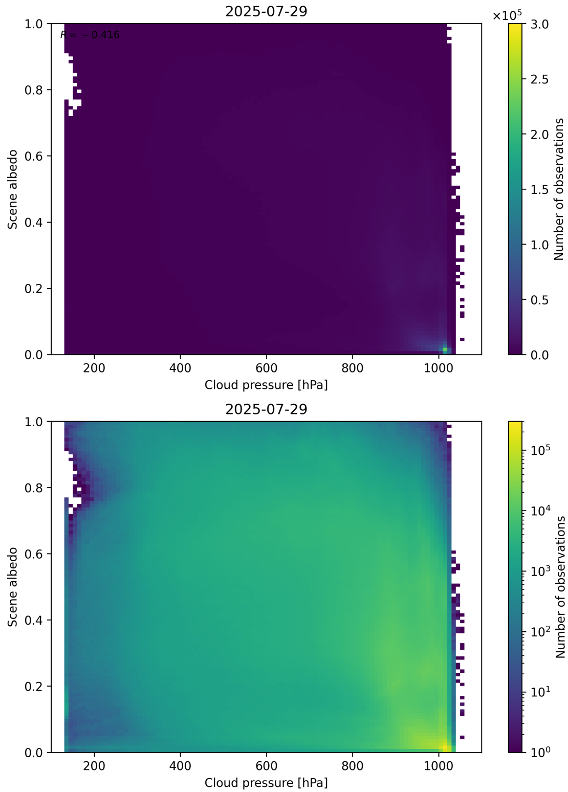
Figure 83: Scatter density plot of “Cloud pressure” against “Scene albedo” for 2025-07-29 to 2025-07-30.
