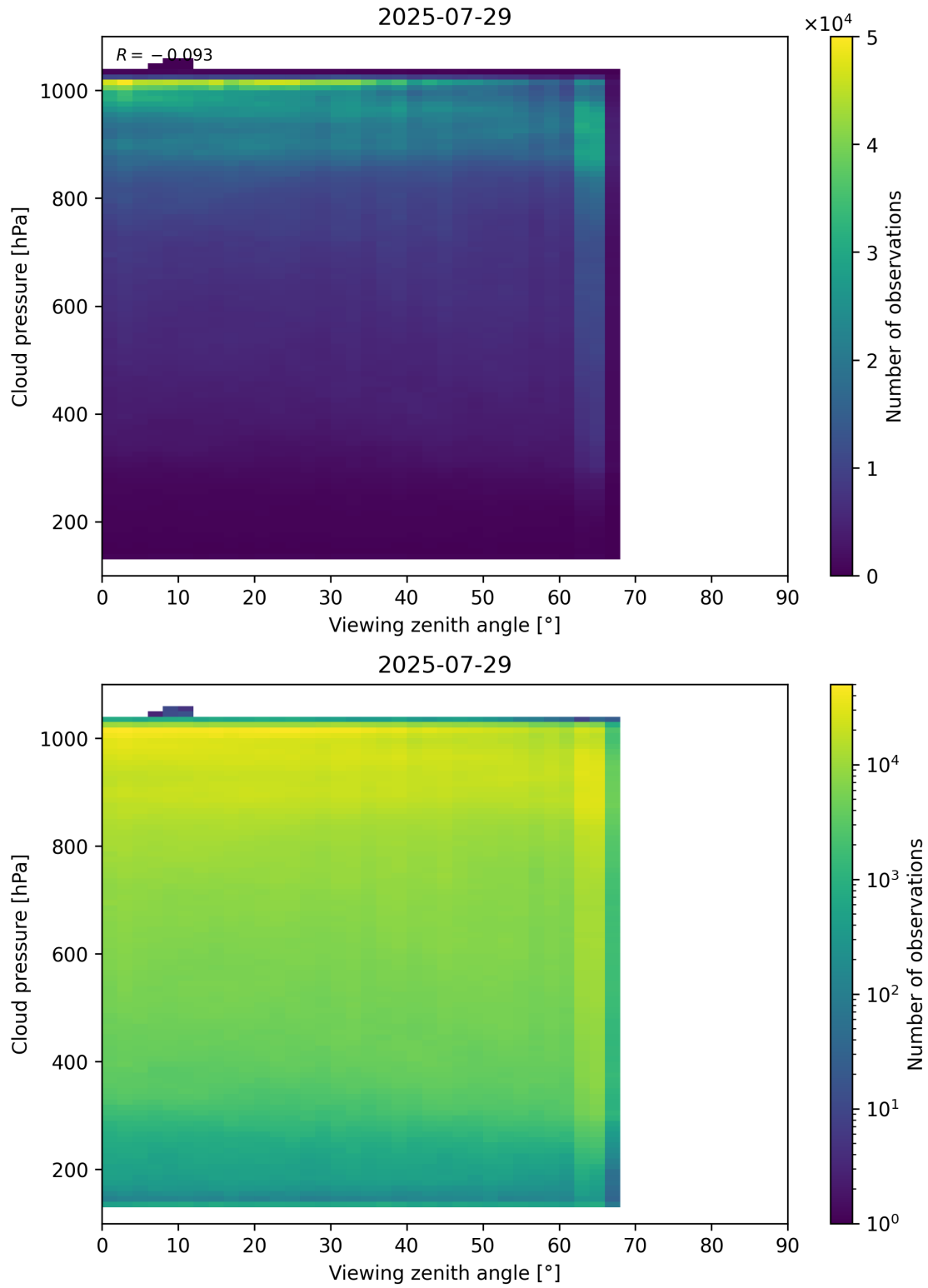
Figure 121: Scatter density plot of “Viewing zenith angle” against “Cloud pressure” for 2025-07-29 to 2025-07-30.
