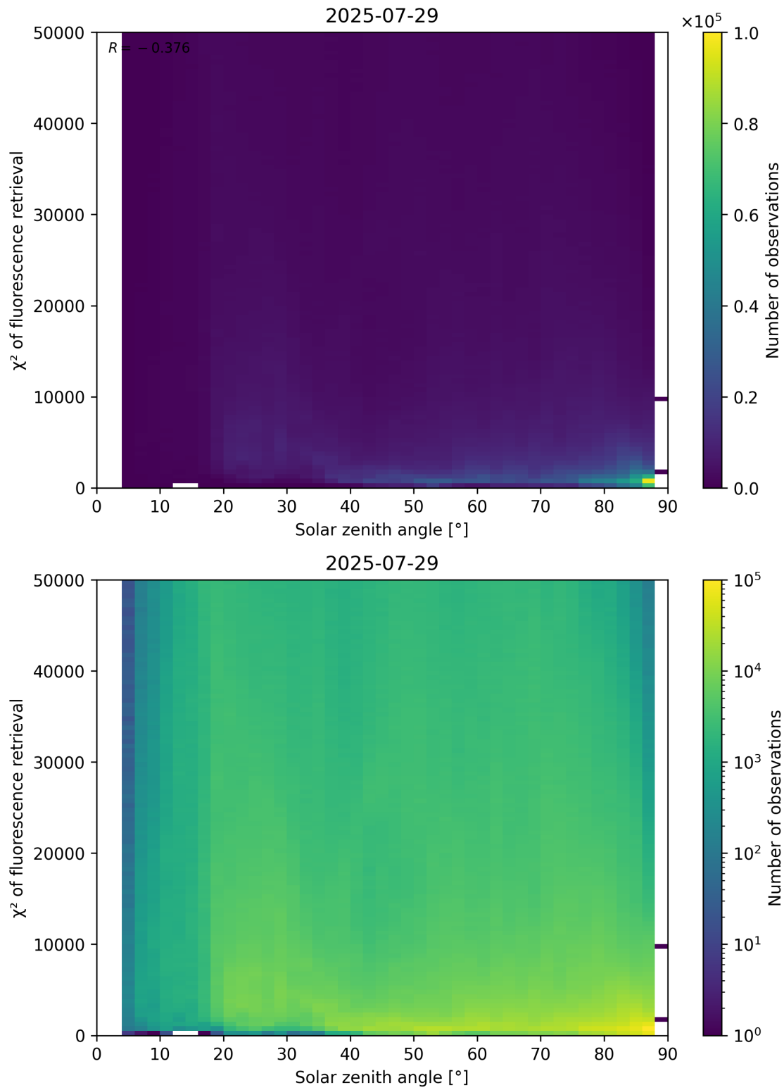
Figure 109: Scatter density plot of “Solar zenith angle” against “ \chi^2 of fluorescence retrieval” for 2025-07-29 to 2025-07-30.
