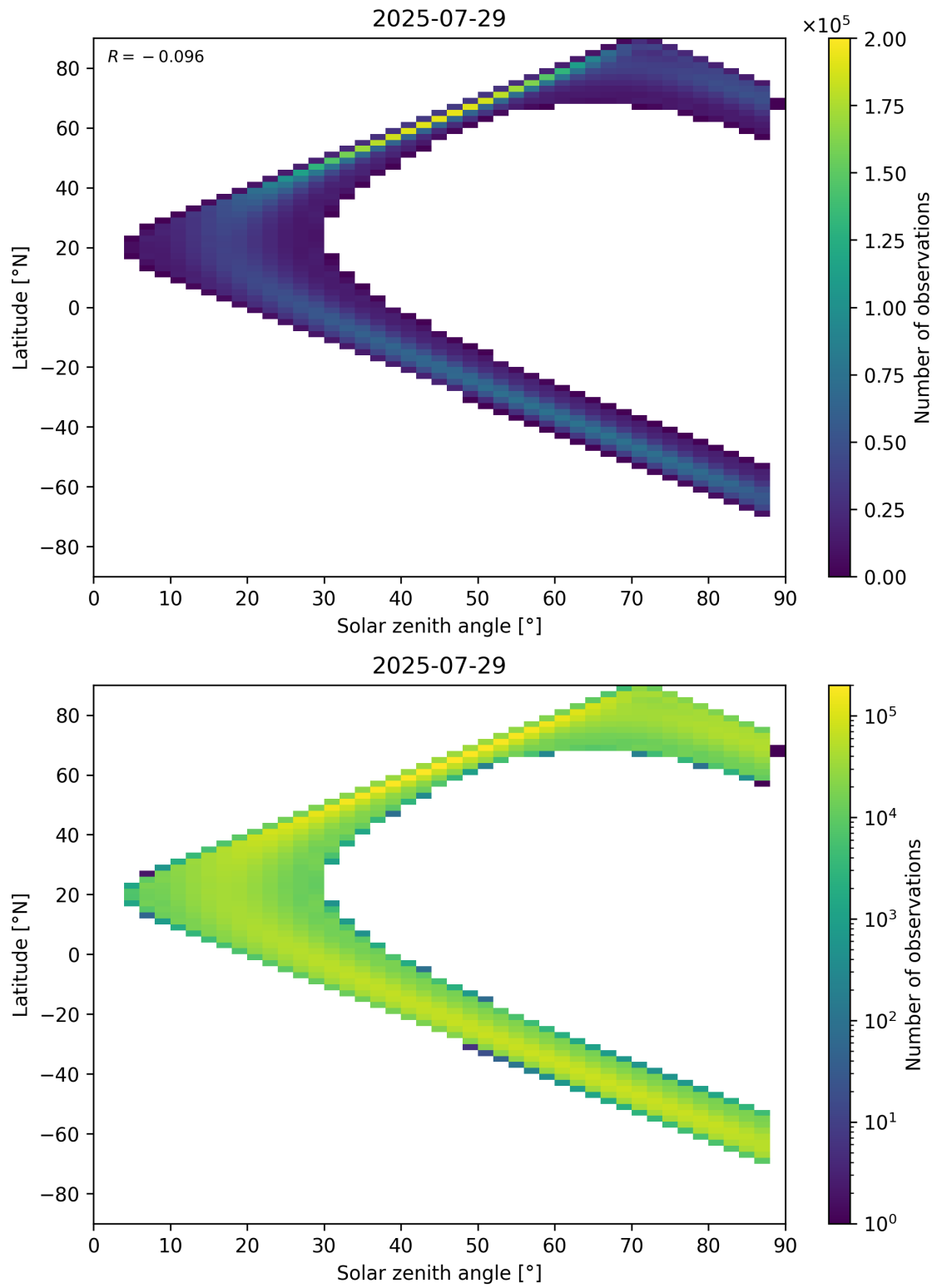
Figure 113: Scatter density plot of “Solar zenith angle” against “Latitude” for 2025-07-29 to 2025-07-30.
