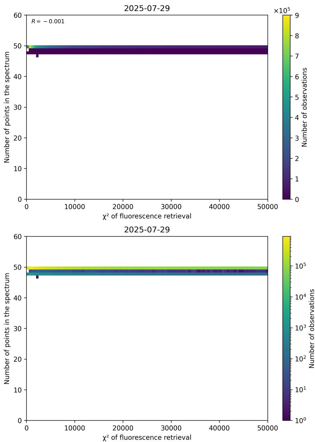
Figure 68: Scatter density plot of " \chi^2 of fluorescence retrieval" against "Number of points in the spectrum" for 2025-07-29 to 2025-07-30.
