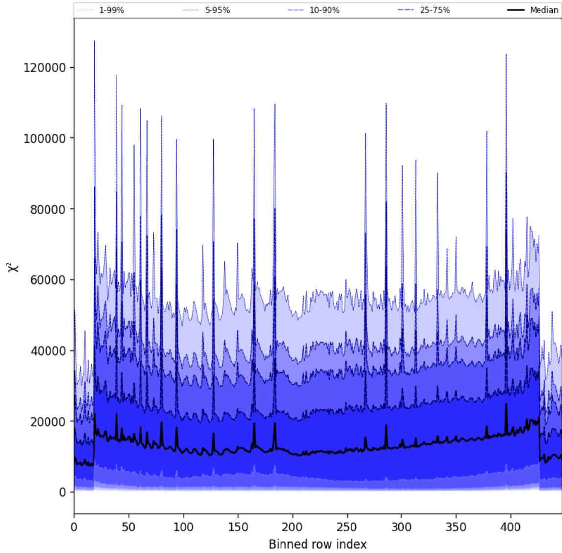
Figure 55: Along track statistics of “ \chi^2 ” for 2025-07-29 to 2025-07-30
