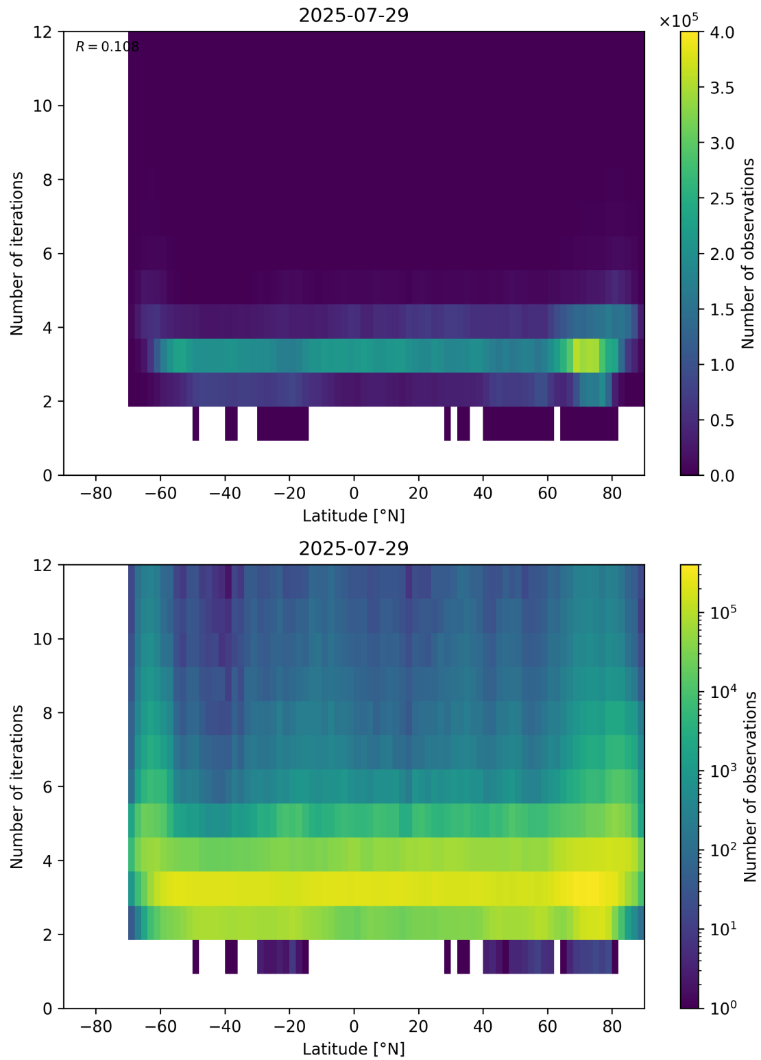
Figure 93: Scatter density plot of “Latitude” against “Number of iterations” for 2025-07-29 to 2025-07-30.
