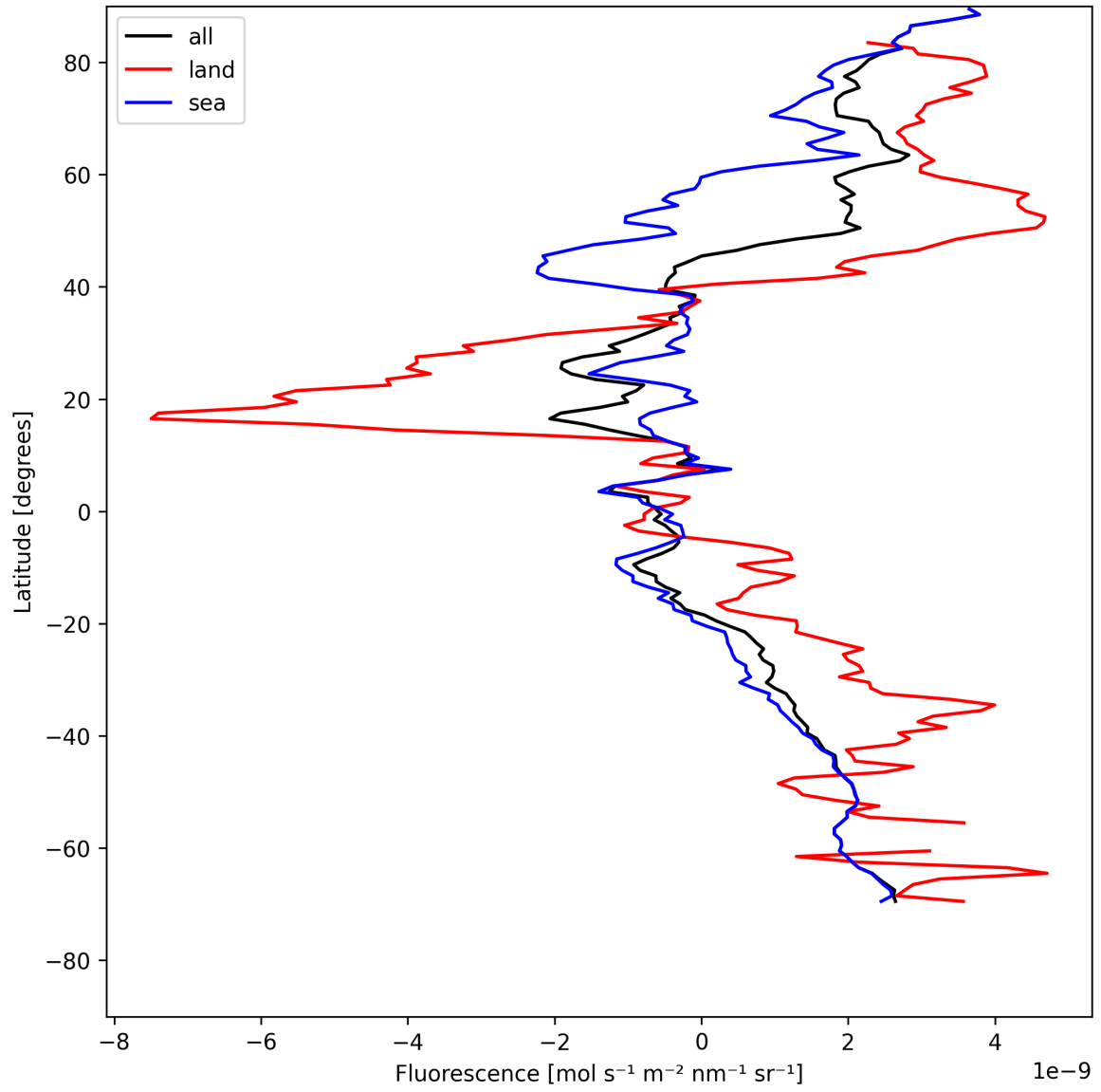
Figure 23: Zonal average of “Fluorescence” for 2025-07-29 to 2025-07-30.
