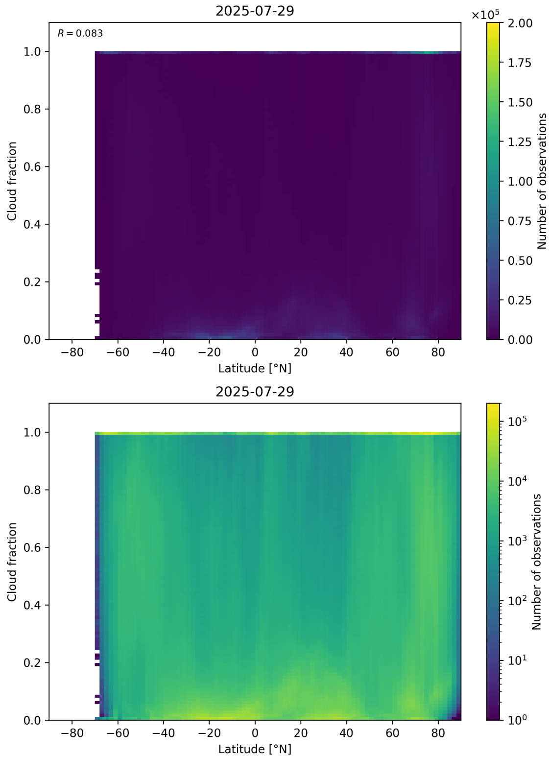
Figure 90: Scatter density plot of “Latitude” against “Cloud fraction” for 2025-07-29 to 2025-07-30.
