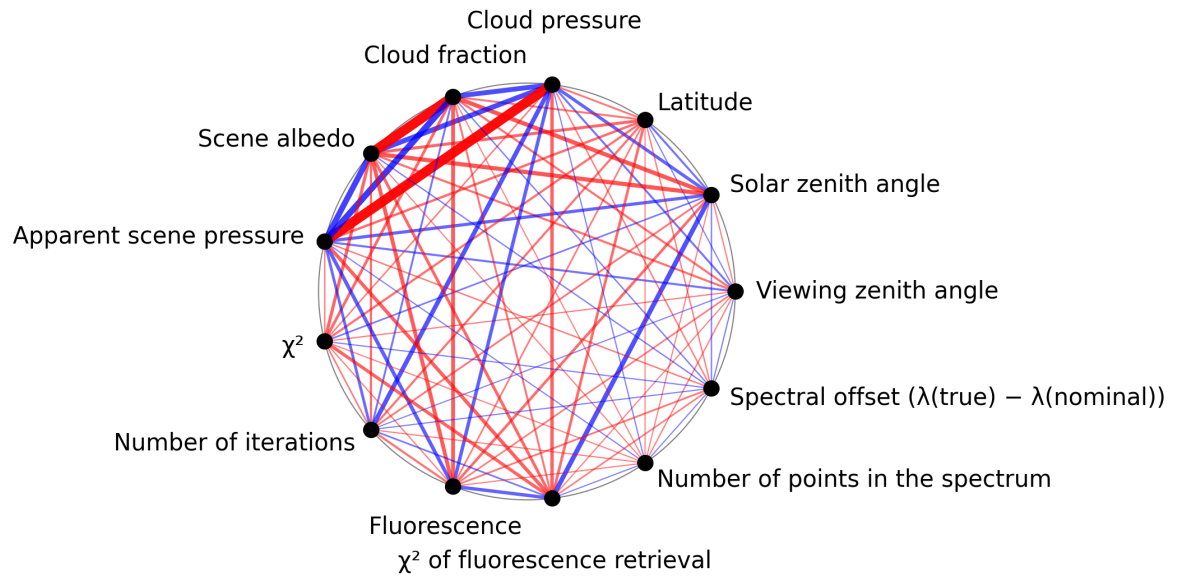
Figure 1: Map of correlation graph for 2025-07-29 to 2025-07-30.
