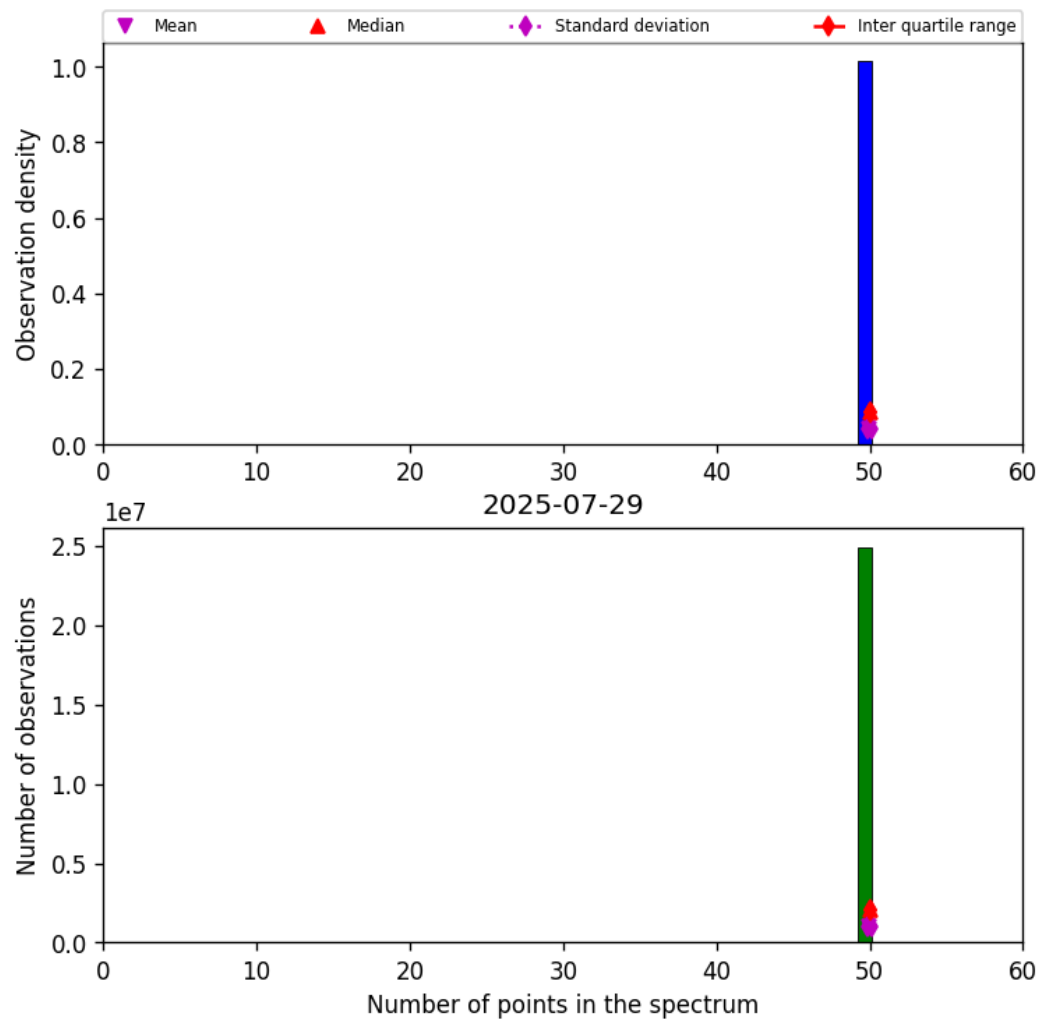
Figure 44: Histogram of “Number of points in the spectrum” for 2025-07-29 to 2025-07-30
