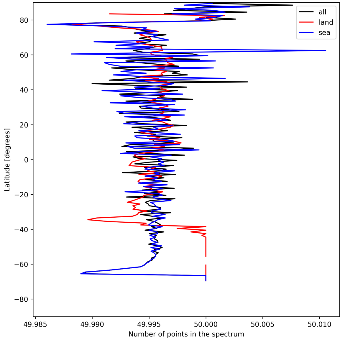
Figure 27: Zonal average of “Number of points in the spectrum” for 2025-07-29 to 2025-07-30.
