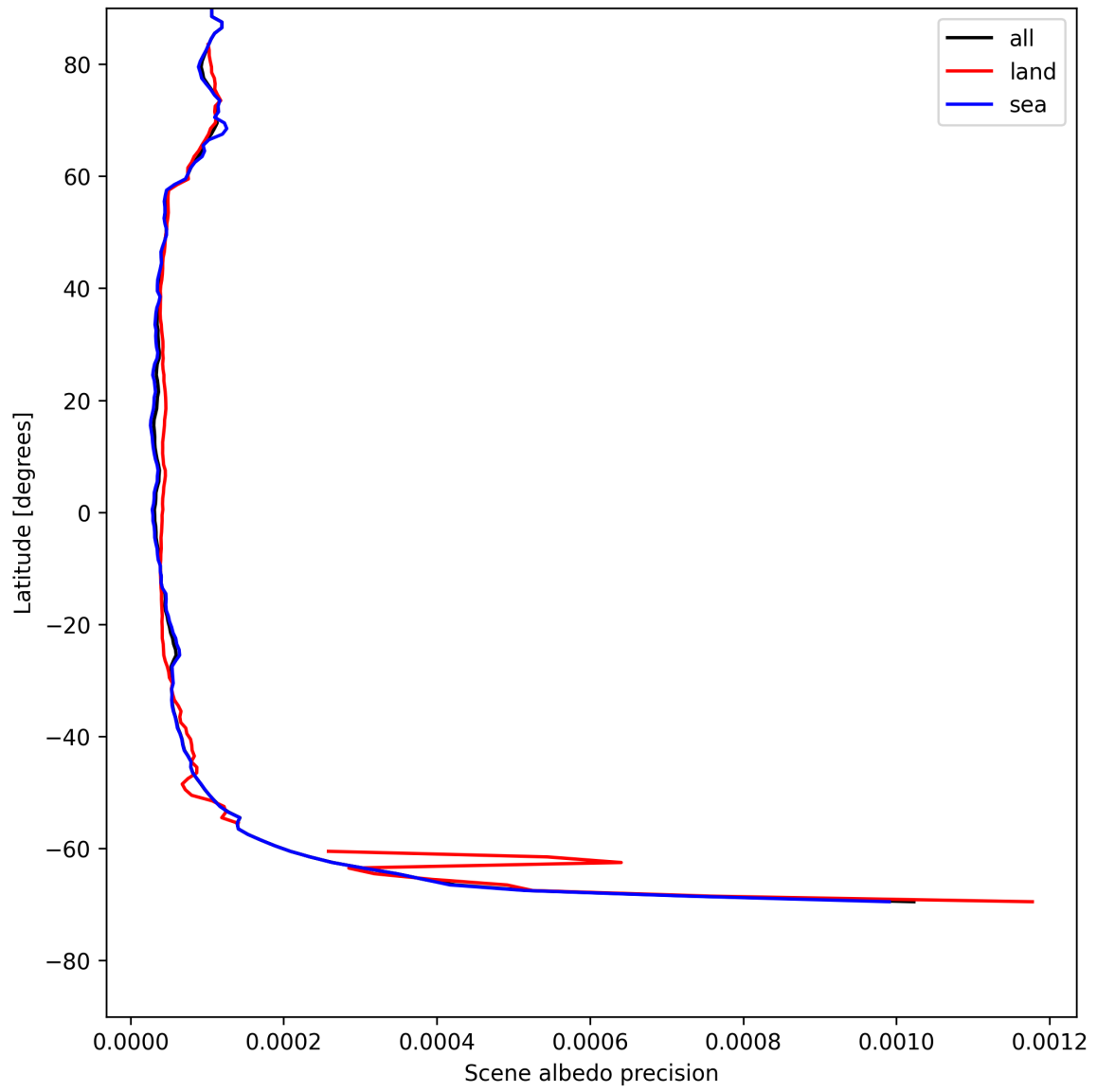
Figure 18: Zonal average of “Scene albedo precision” for 2025-07-29 to 2025-07-30.
