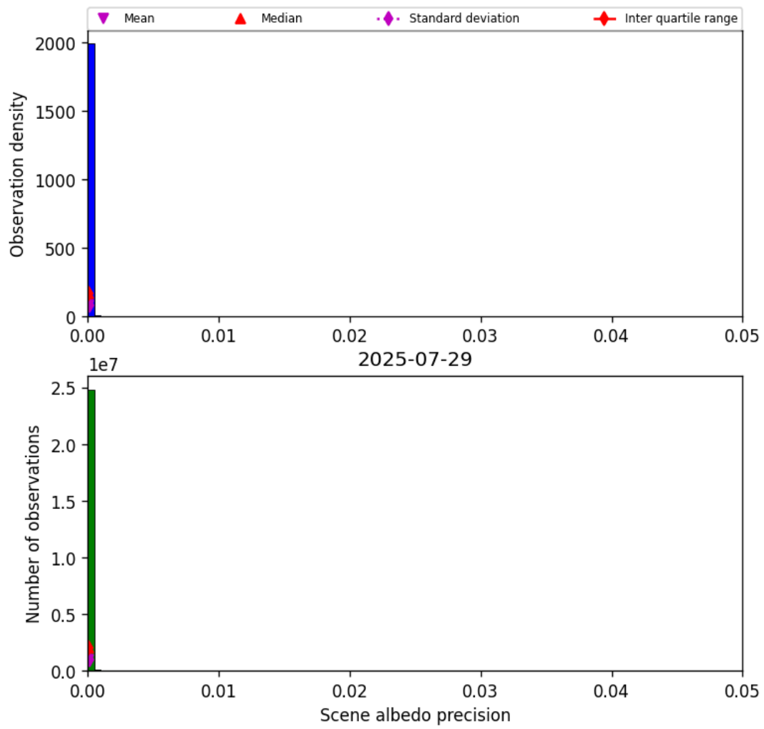
Figure 35: Histogram of “Scene albedo precision” for 2025-07-29 to 2025-07-30
