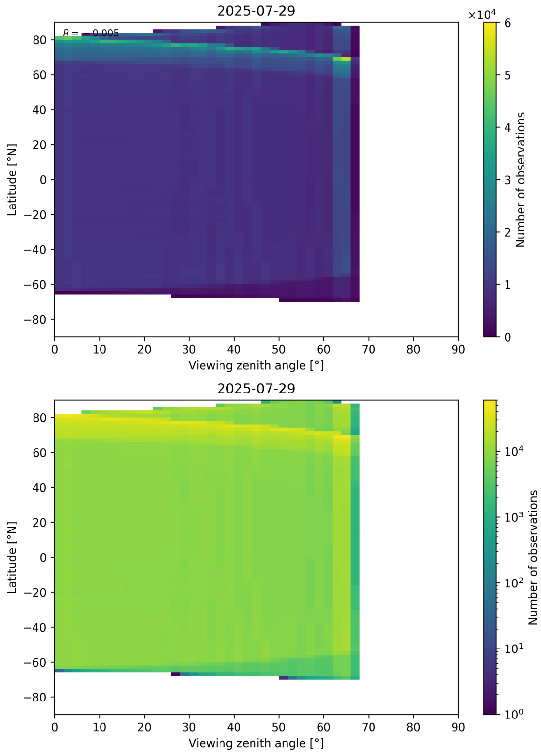
Figure 123: Scatter density plot of “Viewing zenith angle” against “Latitude” for 2025-07-29 to 2025-07-30.
