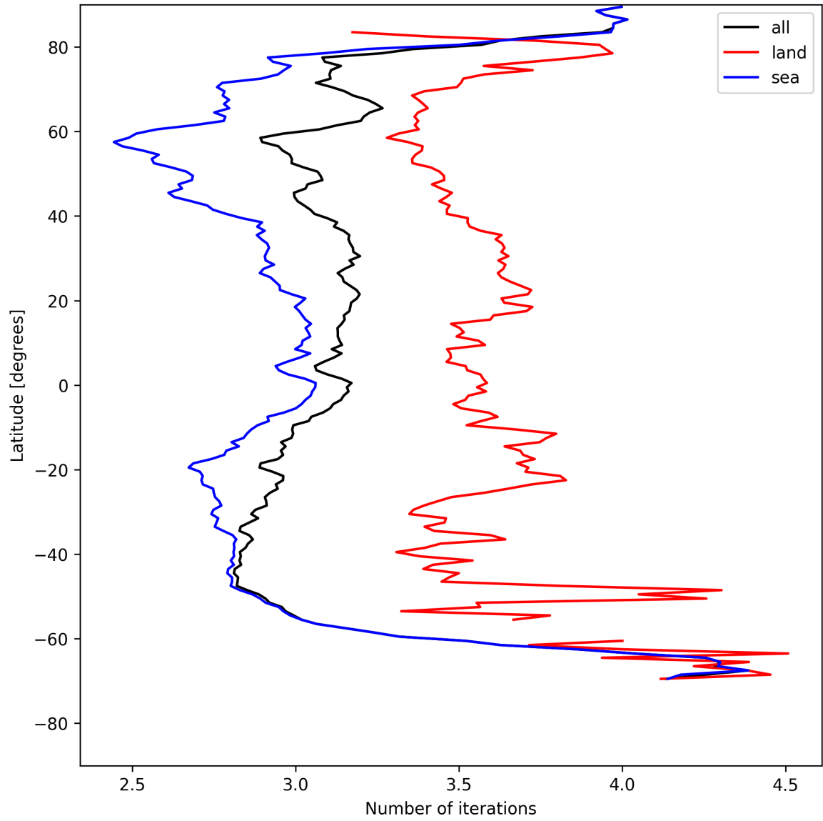
Figure 22: Zonal average of “Number of iterations” for 2025-07-29 to 2025-07-30.
