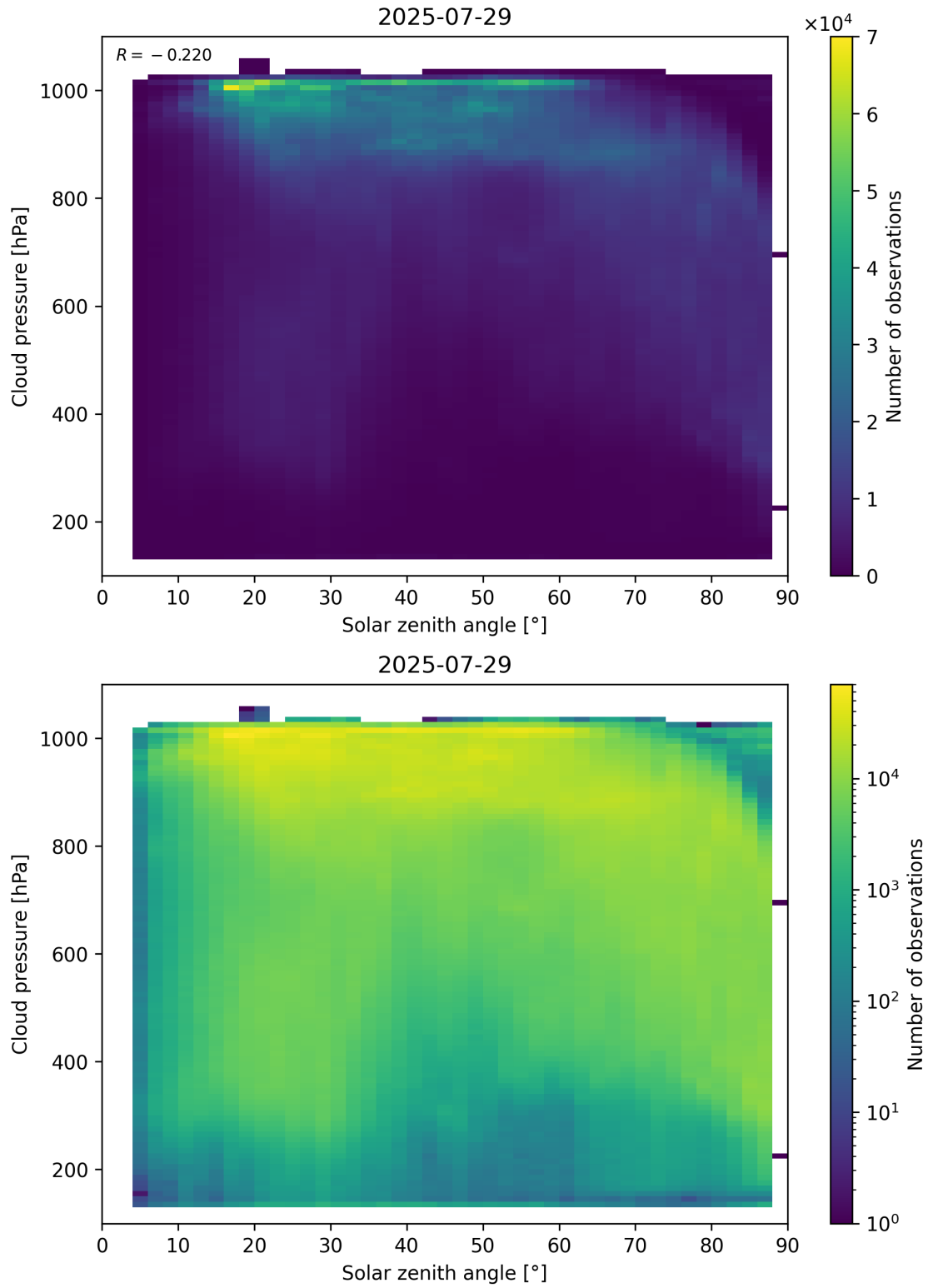
Figure 111: Scatter density plot of “Solar zenith angle” against “Cloud pressure” for 2025-07-29 to 2025-07-30.
