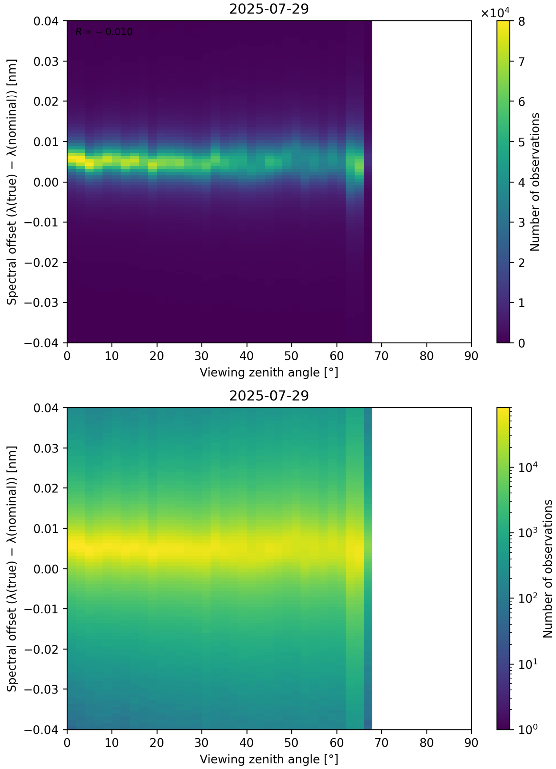
Figure 128: Scatter density plot of “Viewing zenith angle” against “Spectral offset ( \lambda_{\text{true}} - \lambda_{\text{nominal}} )” for 2025-07-29 to 2025-07-30.
