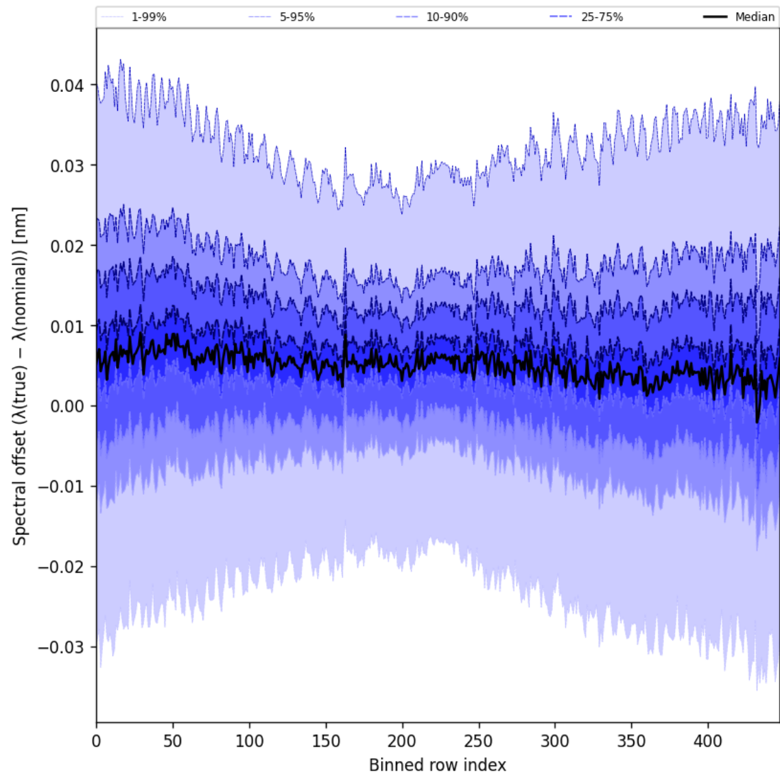
Figure 62: Along track statistics of “Spectral offset ( \lambda_{\text{true}} - \lambda_{\text{nominal}} )” for 2025-07-29 to 2025-07-30
