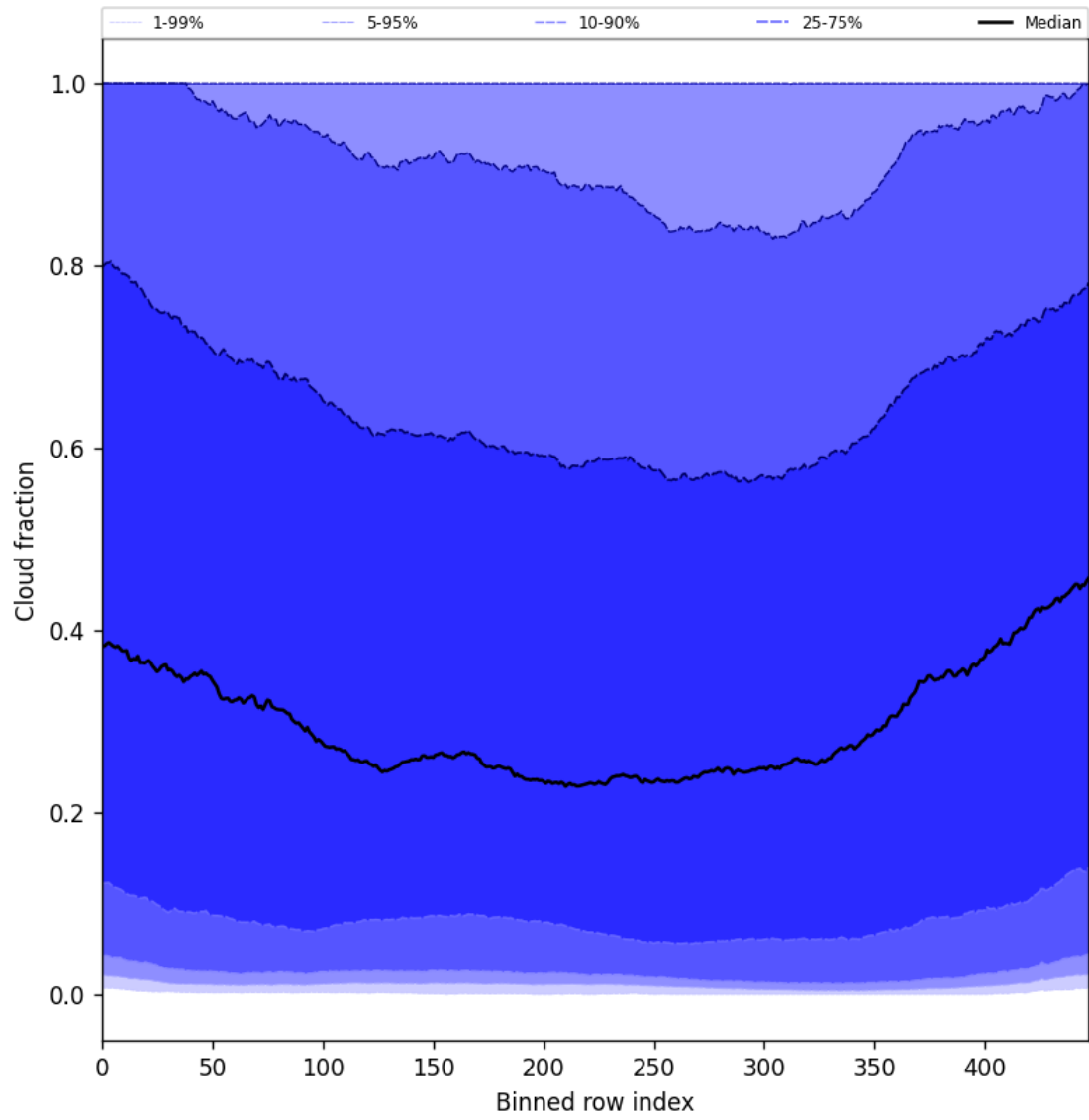
Figure 49: Along track statistics of “Cloud fraction” for 2025-07-29 to 2025-07-30
