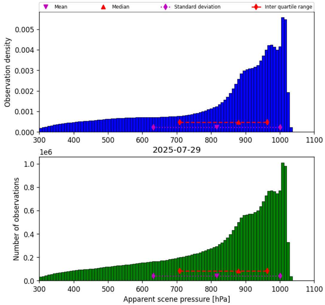
Figure 36: Histogram of “Apparent scene pressure” for 2025-07-29 to 2025-07-30
