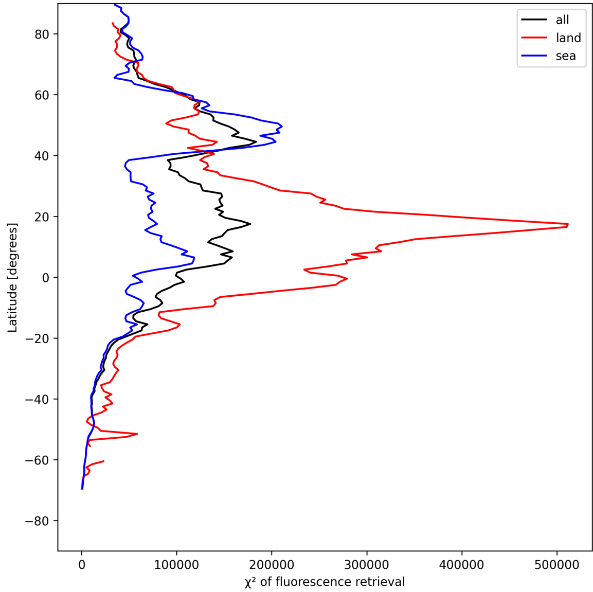
Figure 25: Zonal average of “ \chi^2 of fluorescence retrieval” for 2025-07-29 to 2025-07-30.
