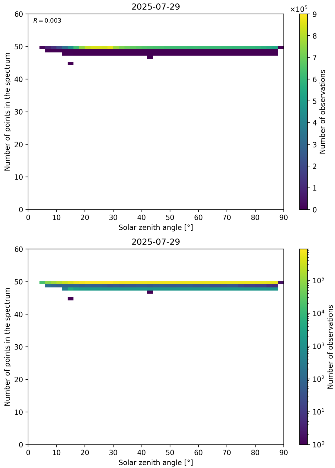
Figure 115: Scatter density plot of “Solar zenith angle” against “Number of points in the spectrum” for 2025-07-29 to 2025-07-30.
