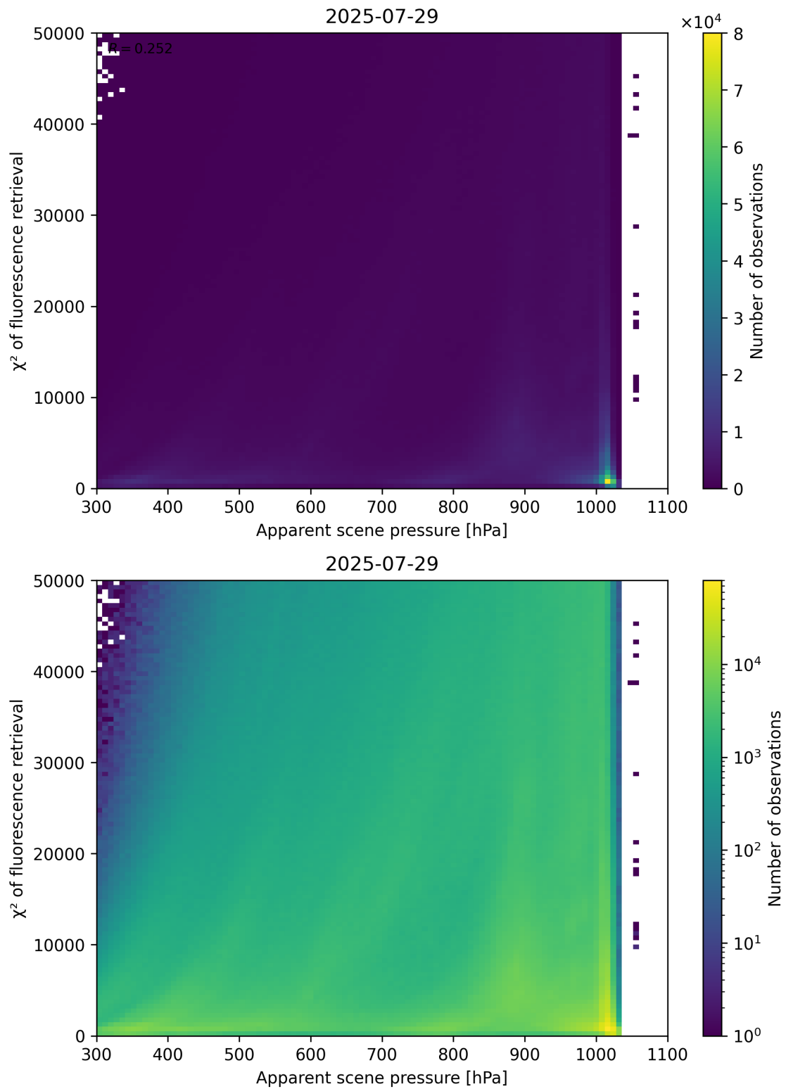
Figure 63: Scatter density plot of “Apparent scene pressure” against “ \chi^2 of fluorescence retrieval” for 2025-07-29 to 2025-07-30.
