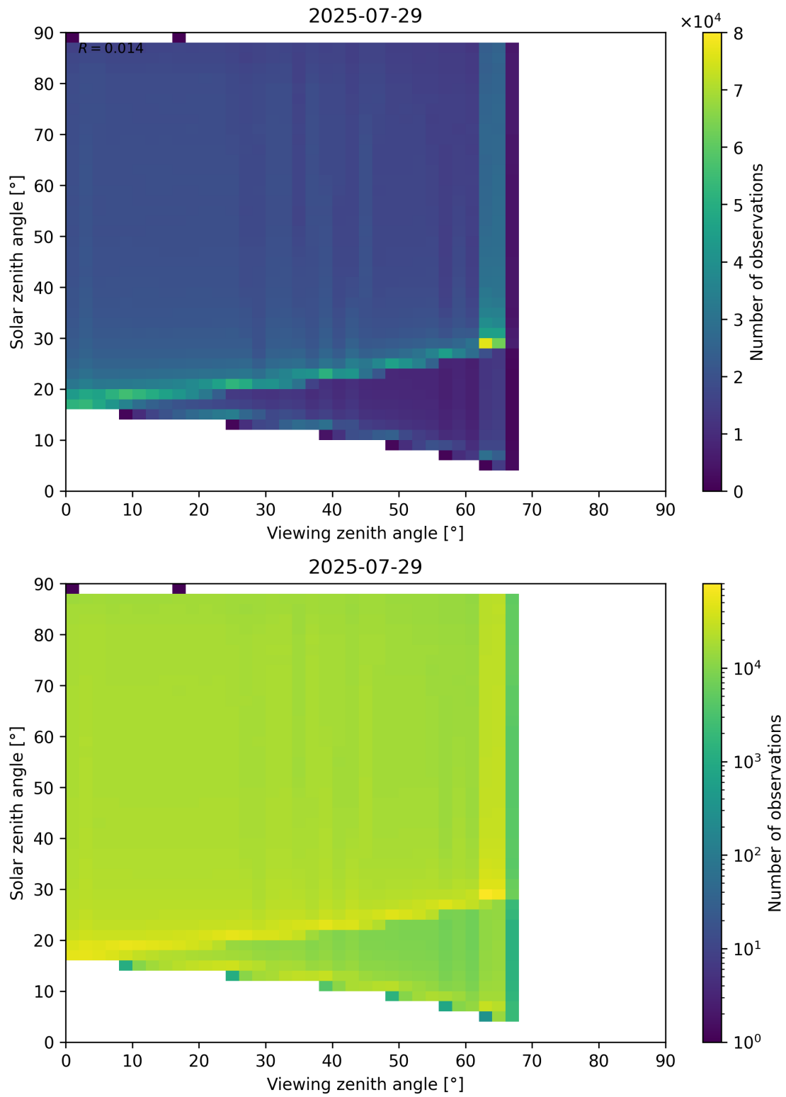
Figure 127: Scatter density plot of “Viewing zenith angle” against “Solar zenith angle” for 2025-07-29 to 2025-07-30.
