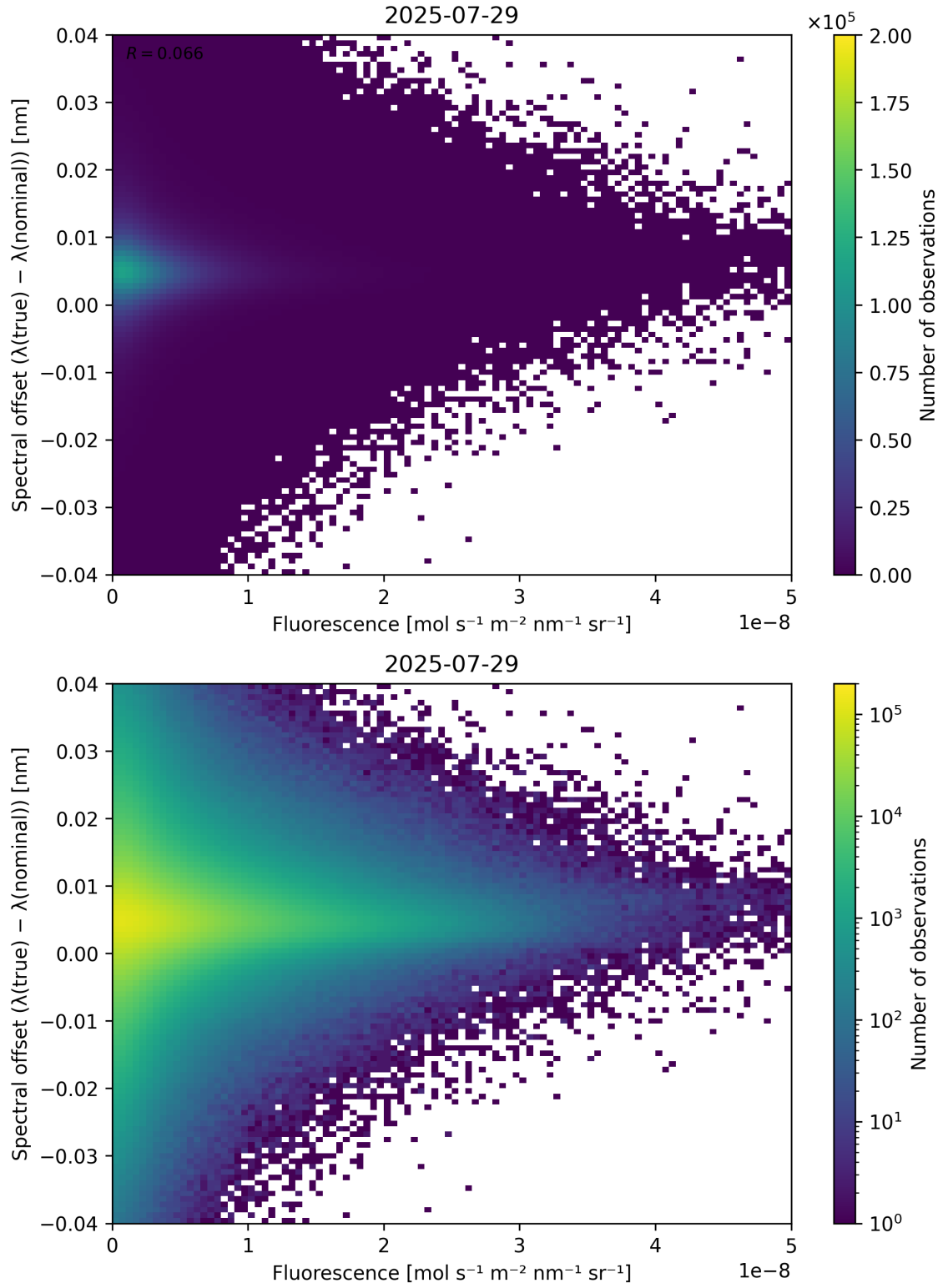
Figure 87: Scatter density plot of “Fluorescence” against “Spectral offset ( \lambda_{\text{true}} - \lambda_{\text{nominal}} )” for 2025-07-29 to 2025-07-30.
