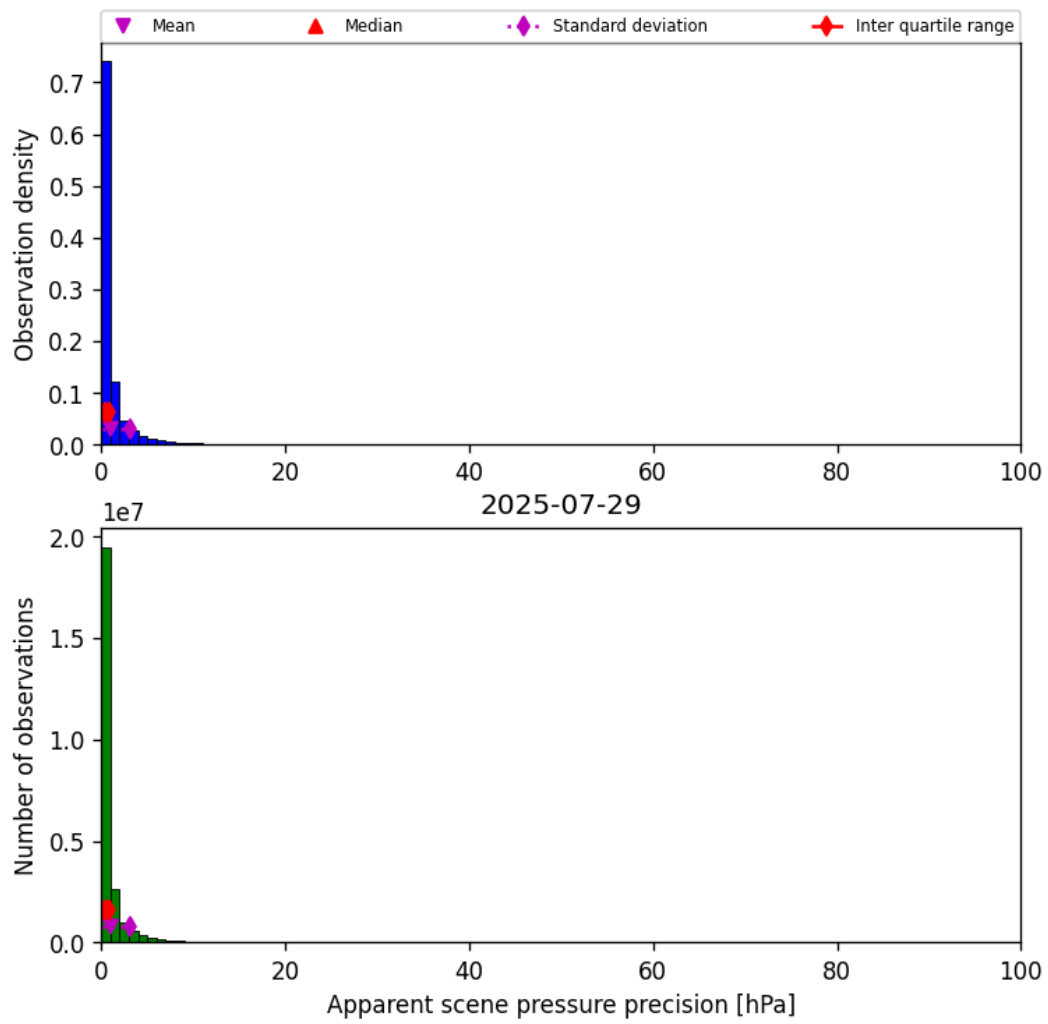
Figure 37: Histogram of “Apparent scene pressure precision” for 2025-07-29 to 2025-07-30
