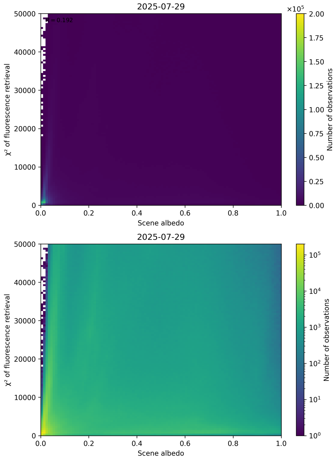
Figure 103: Scatter density plot of “Scene albedo” against “ \chi^2 of fluorescence retrieval” for 2025-07-29 to 2025-07-30.
