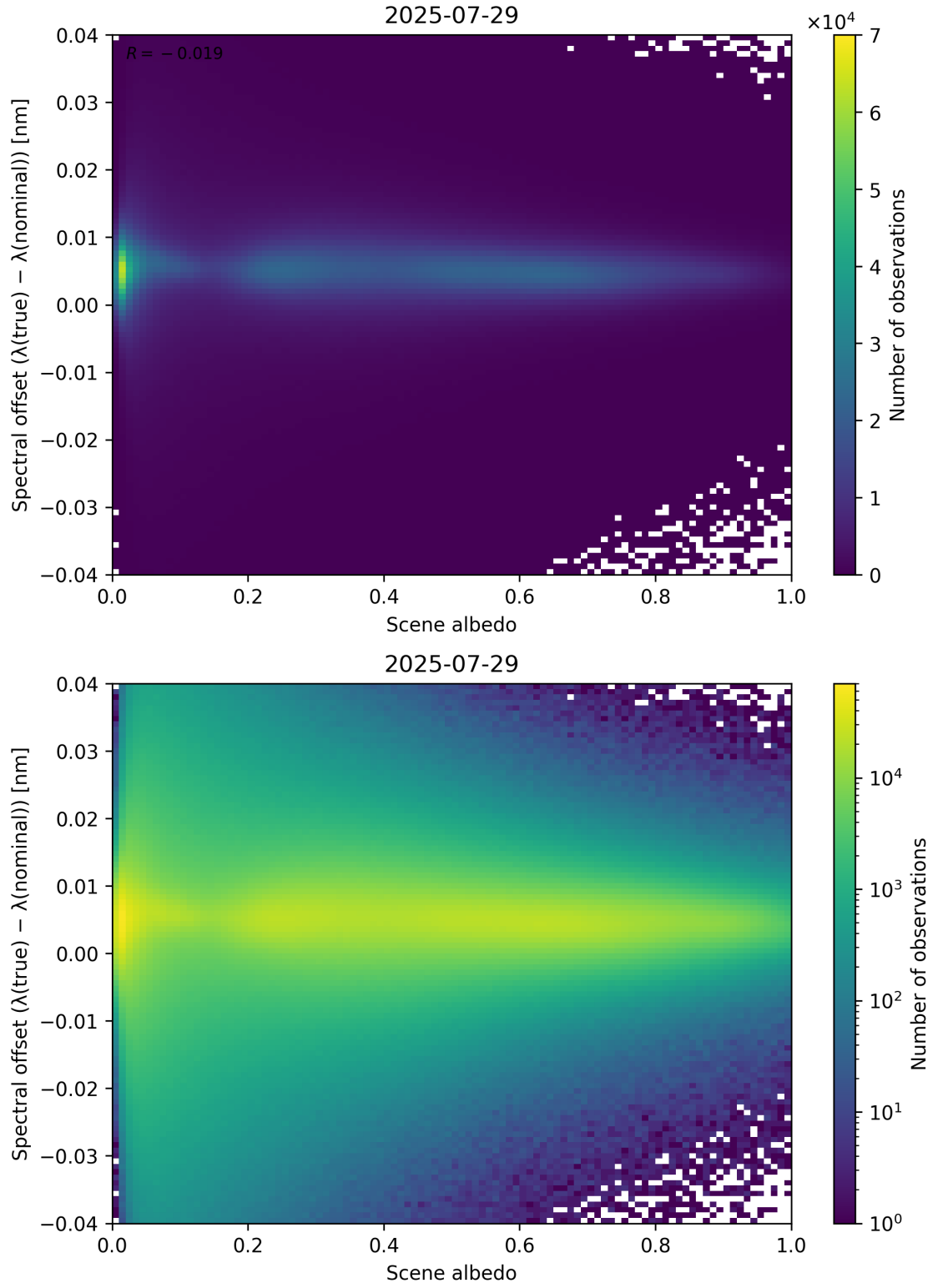
Figure 107: Scatter density plot of “Scene albedo” against “Spectral offset ( \lambda_{\text{true}} - \lambda_{\text{nominal}} )” for 2025-07-29 to 2025-07-30.
