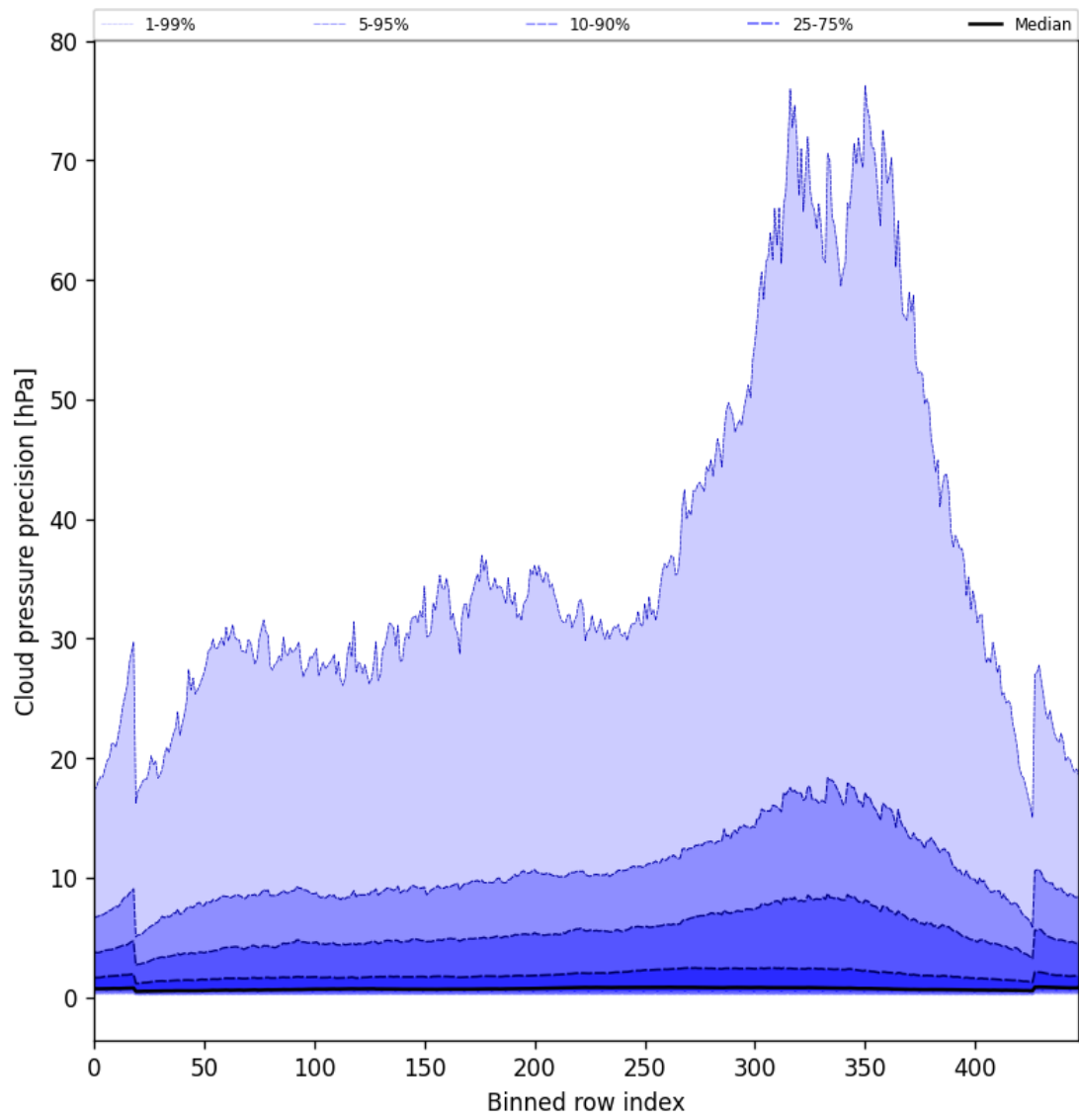
Figure 48: Along track statistics of “Cloud pressure precision” for 2025-07-29 to 2025-07-30
