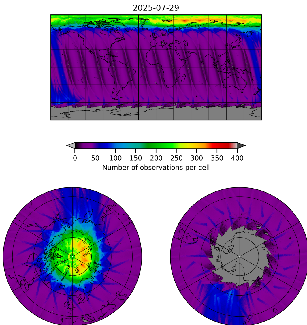
Figure 11: Map of the number of observations for 2025-07-29 to 2025-07-30
