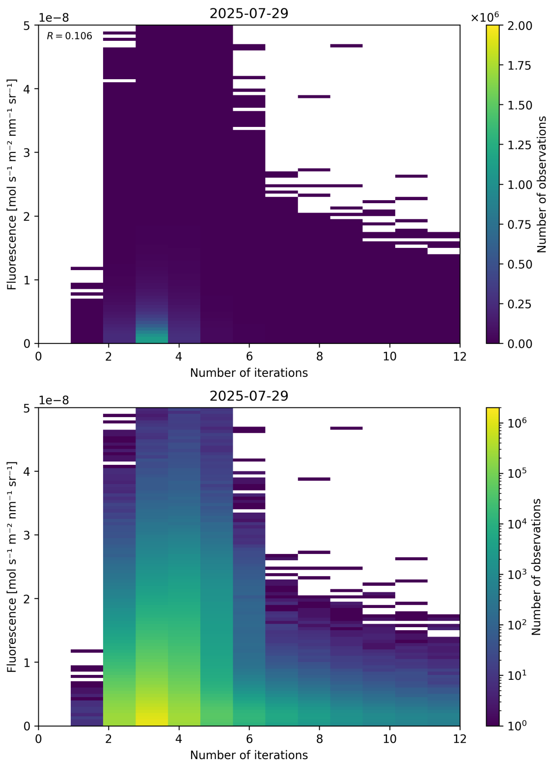
Figure 98: Scatter density plot of “Number of iterations” against “Fluorescence” for 2025-07-29 to 2025-07-30.
