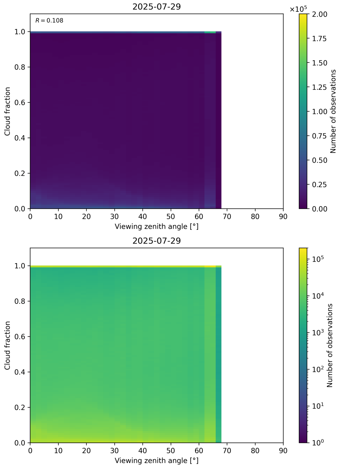
Figure 120: Scatter density plot of “Viewing zenith angle” against “Cloud fraction” for 2025-07-29 to 2025-07-30.
