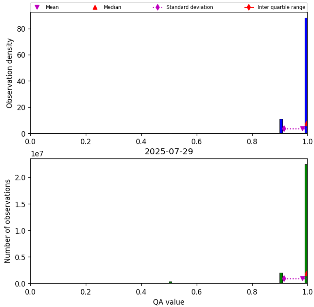
Figure 29: Histogram of “QA value” for 2025-07-29 to 2025-07-30
