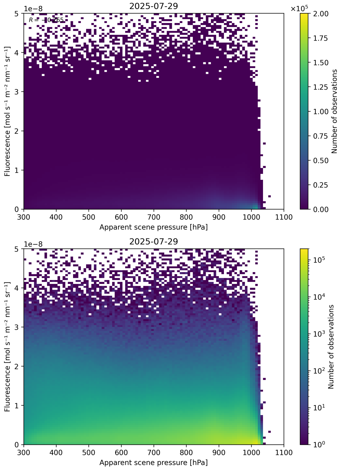
Figure 64: Scatter density plot of “Apparent scene pressure” against “Fluorescence” for 2025-07-29 to 2025-07-30.
