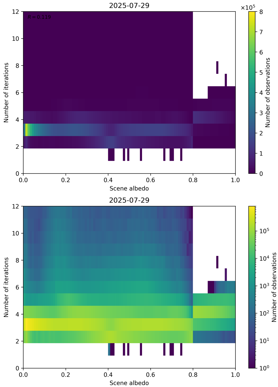
Figure 105: Scatter density plot of “Scene albedo” against “Number of iterations” for 2025-07-29 to 2025-07-30.
