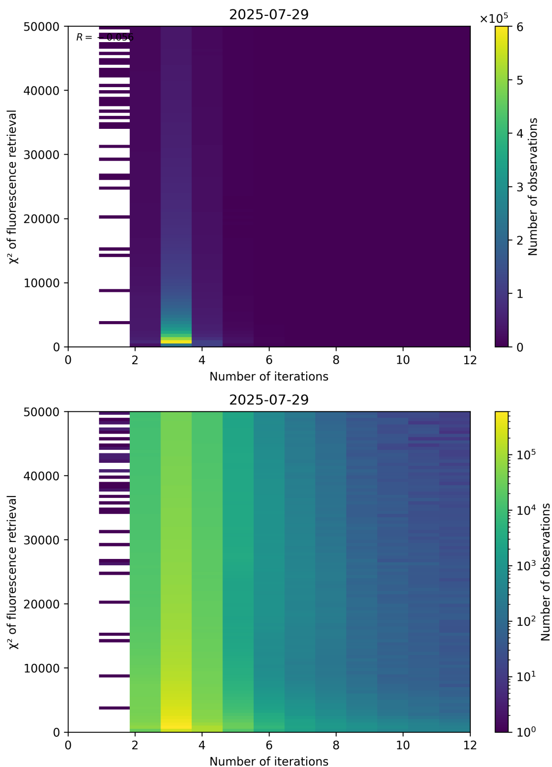
Figure 97: Scatter density plot of “Number of iterations” against “ \chi^2 of fluorescence retrieval” for 2025-07-29 to 2025-07-30.
