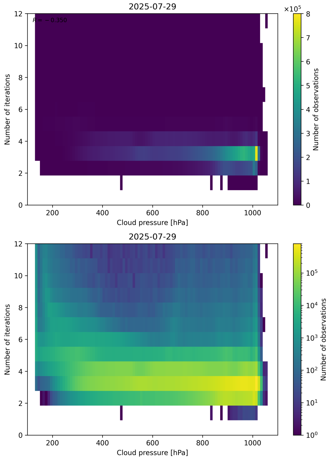
Figure 81: Scatter density plot of “Cloud pressure” against “Number of iterations” for 2025-07-29 to 2025-07-30.
