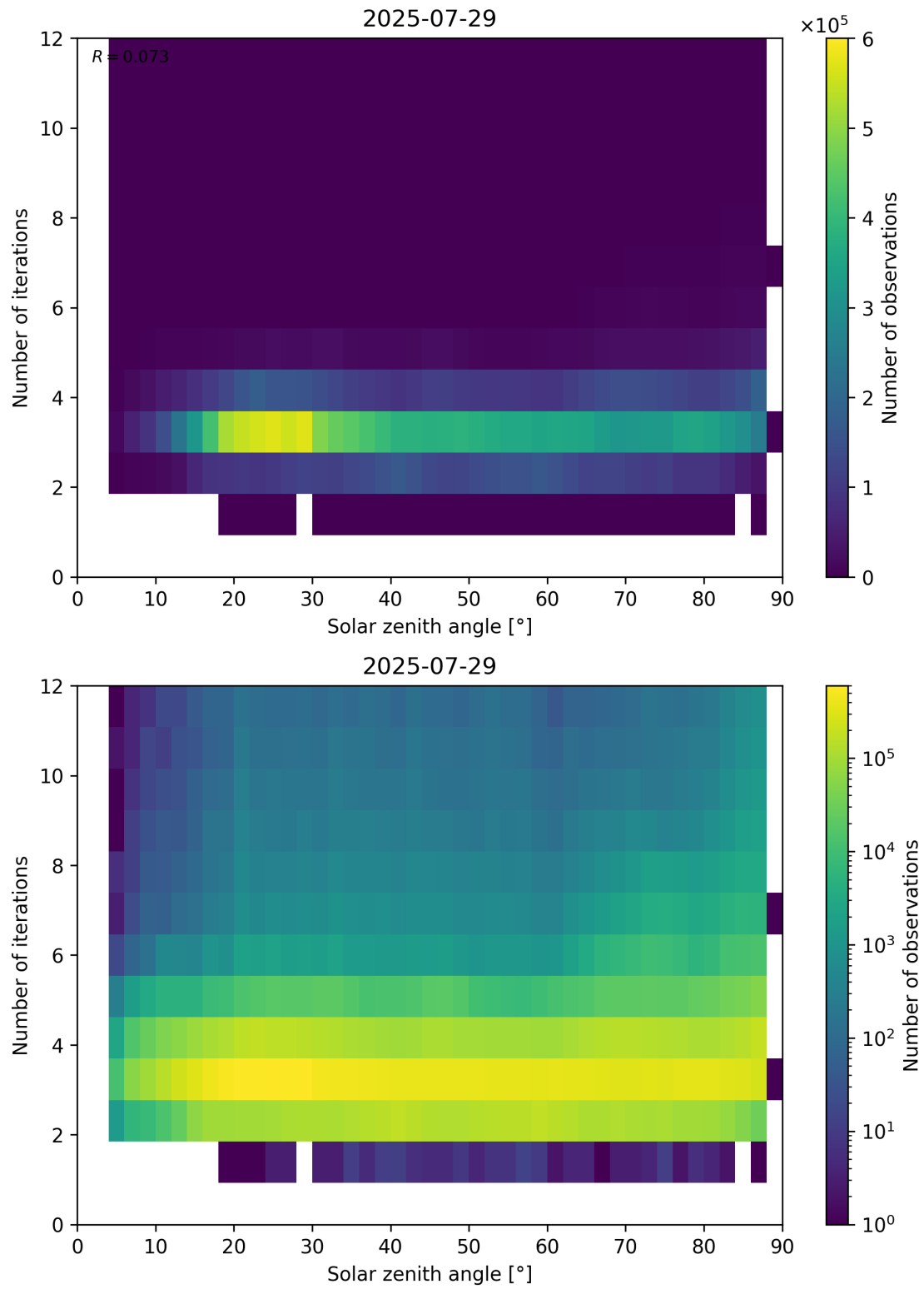
Figure 114: Scatter density plot of “Solar zenith angle” against “Number of iterations” for 2025-07-29 to 2025-07-30.
