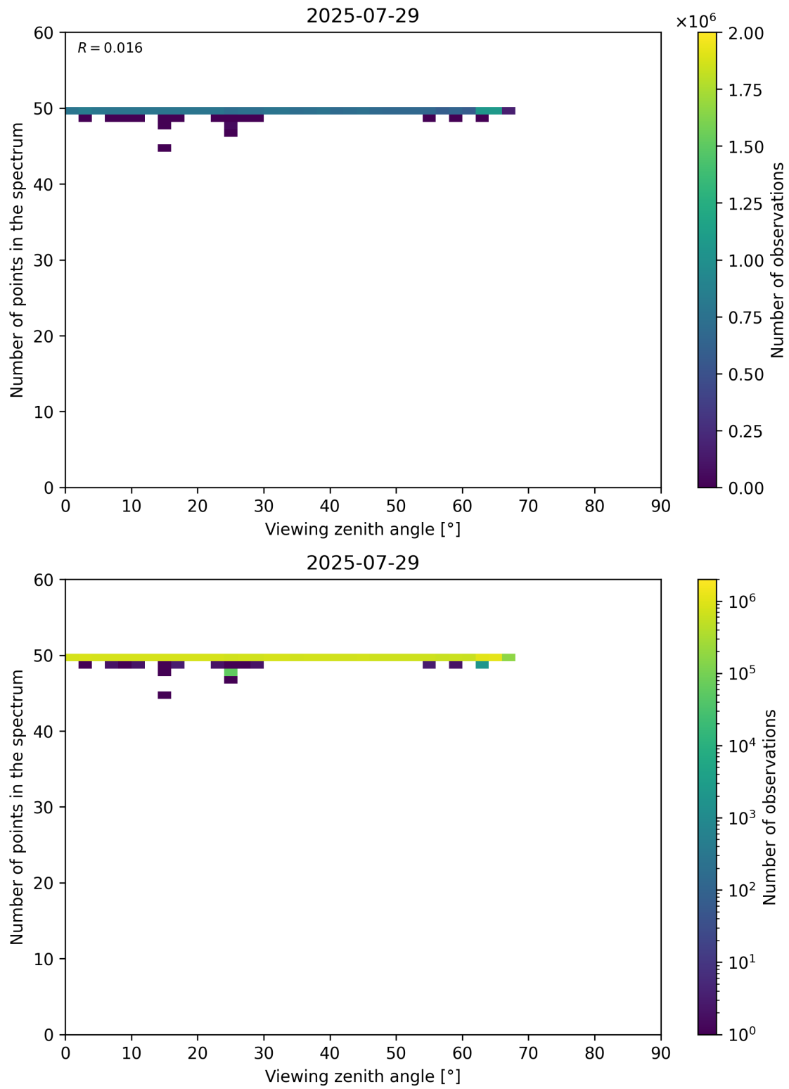
Figure 125: Scatter density plot of “Viewing zenith angle” against “Number of points in the spectrum” for 2025-07-29 to 2025-07-30.
