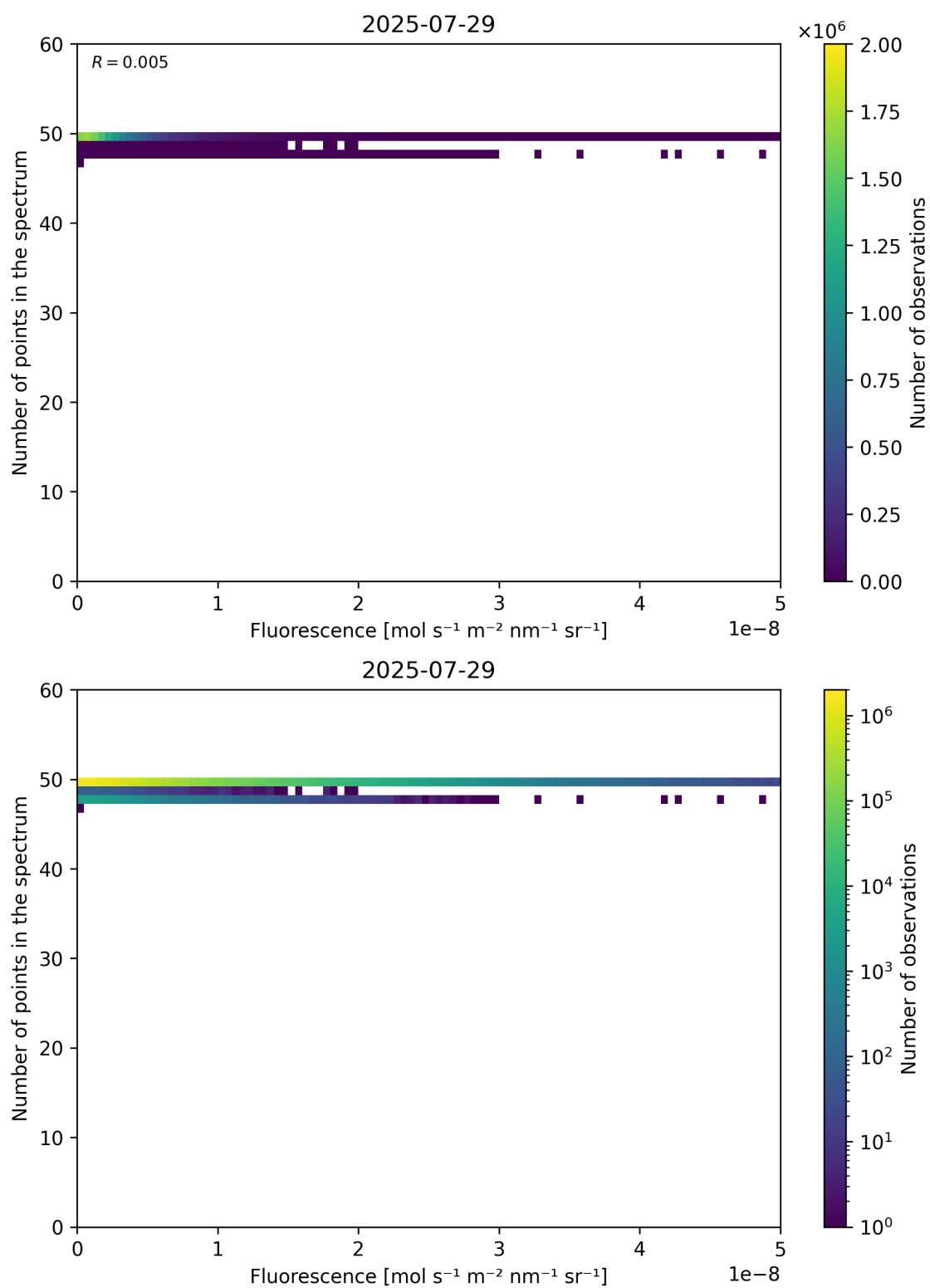
Figure 86: Scatter density plot of “Fluorescence” against “Number of points in the spectrum” for 2025-07-29 to 2025-07-30.
