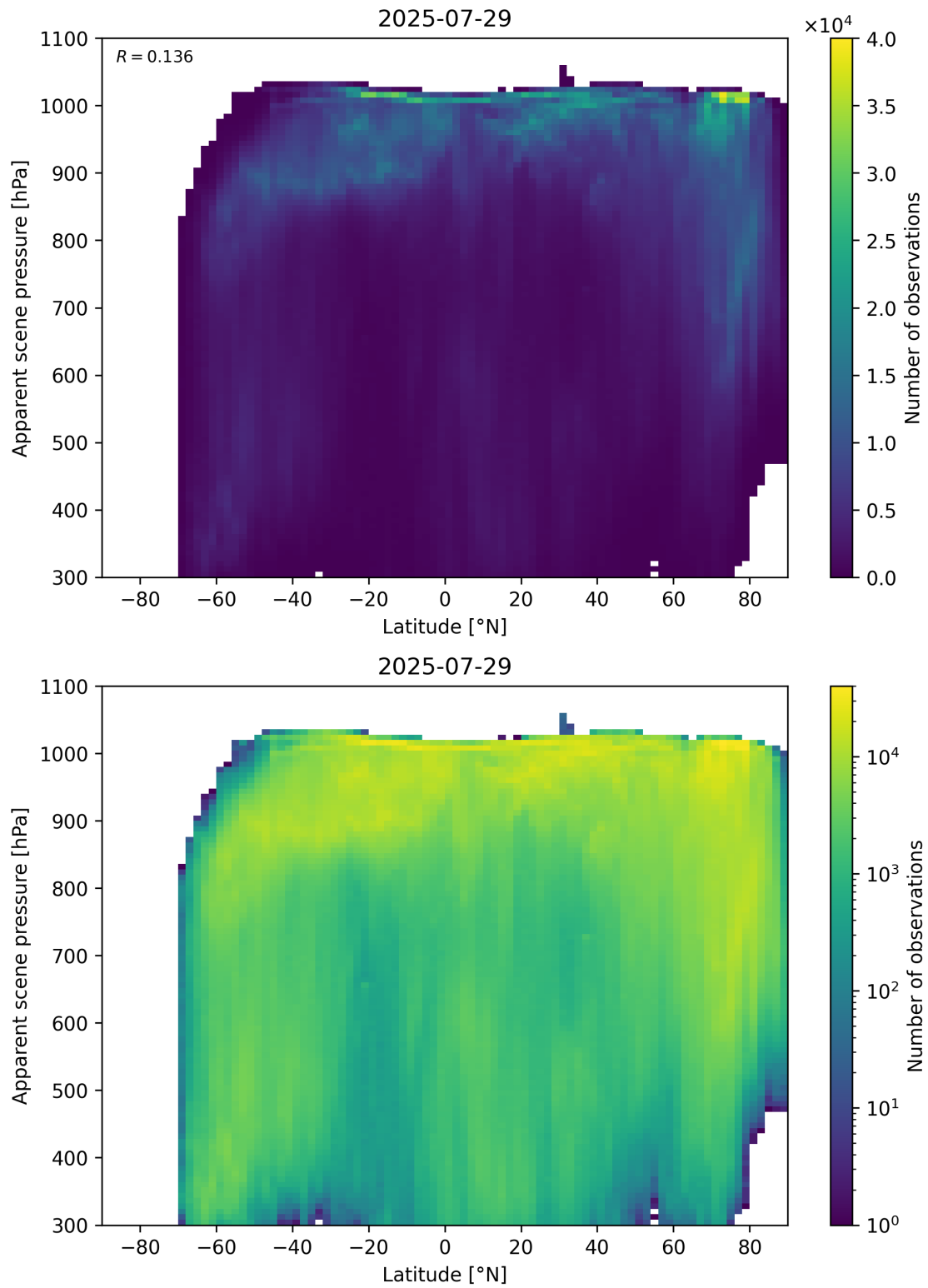
Figure 88: Scatter density plot of “Latitude” against “Apparent scene pressure” for 2025-07-29 to 2025-07-30.
