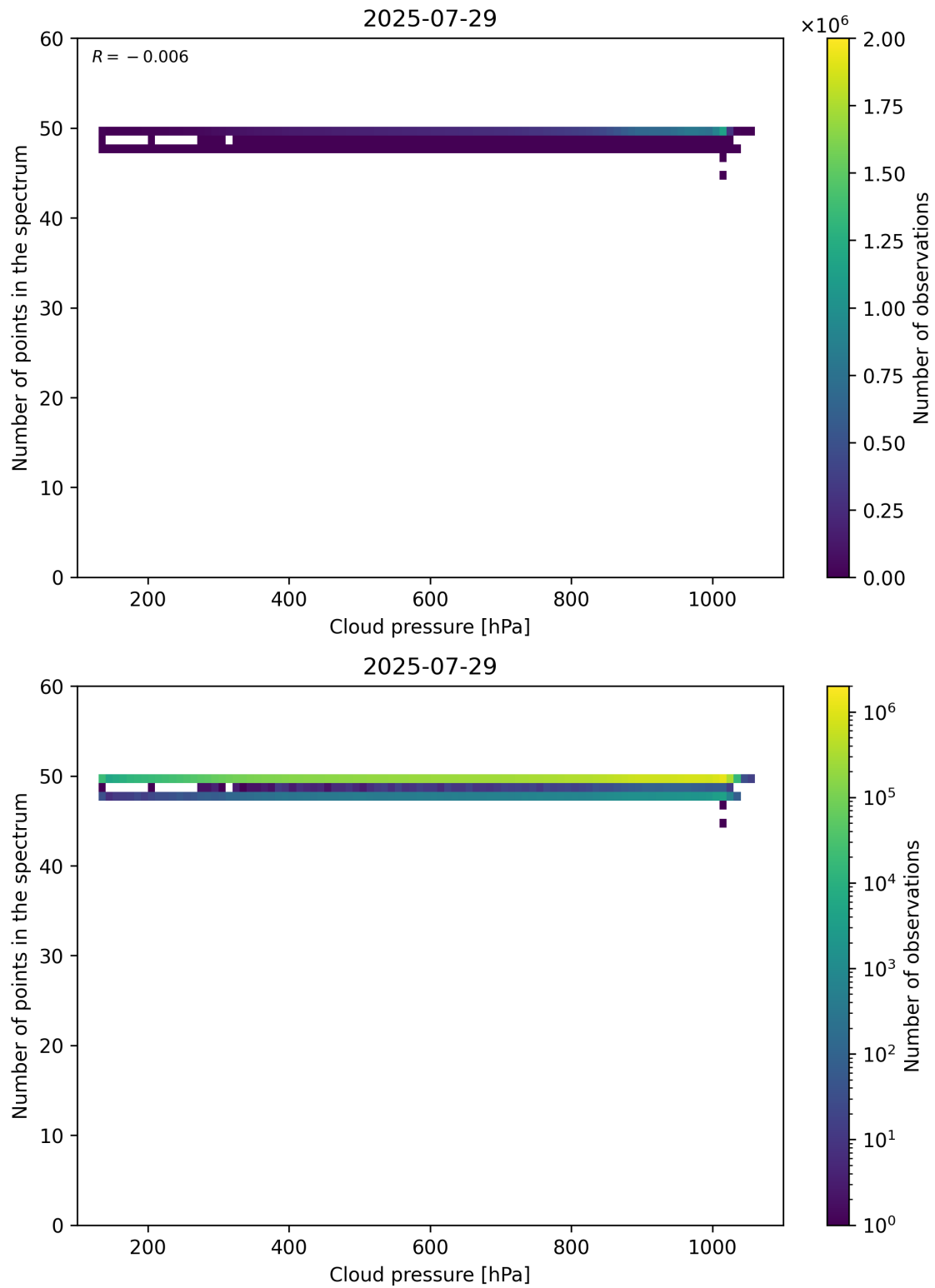
Figure 82: Scatter density plot of “Cloud pressure” against “Number of points in the spectrum” for 2025-07-29 to 2025-07-30.
