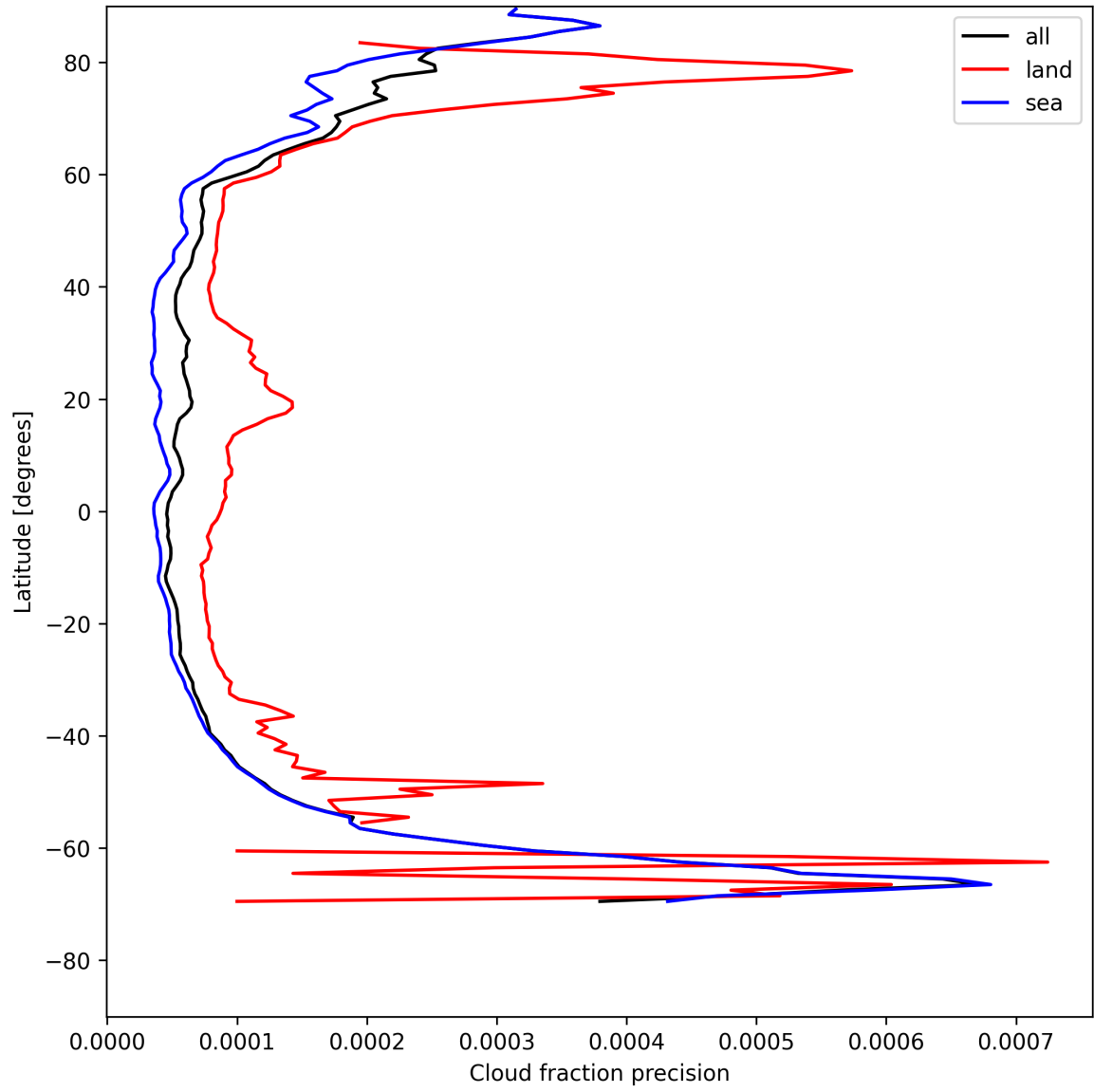
Figure 16: Zonal average of “Cloud fraction precision” for 2025-07-29 to 2025-07-30.
