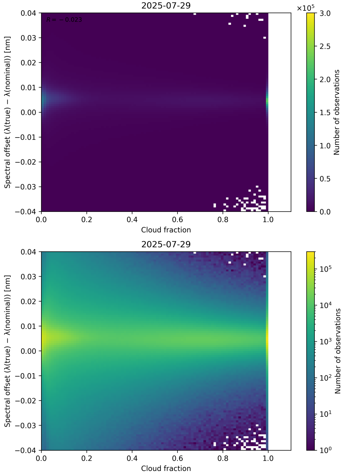
Figure 76: Scatter density plot of “Cloud fraction” against “Spectral offset ( \lambda_{\text{true}} - \lambda_{\text{nominal}} )” for 2025-07-29 to 2025-07-30.
