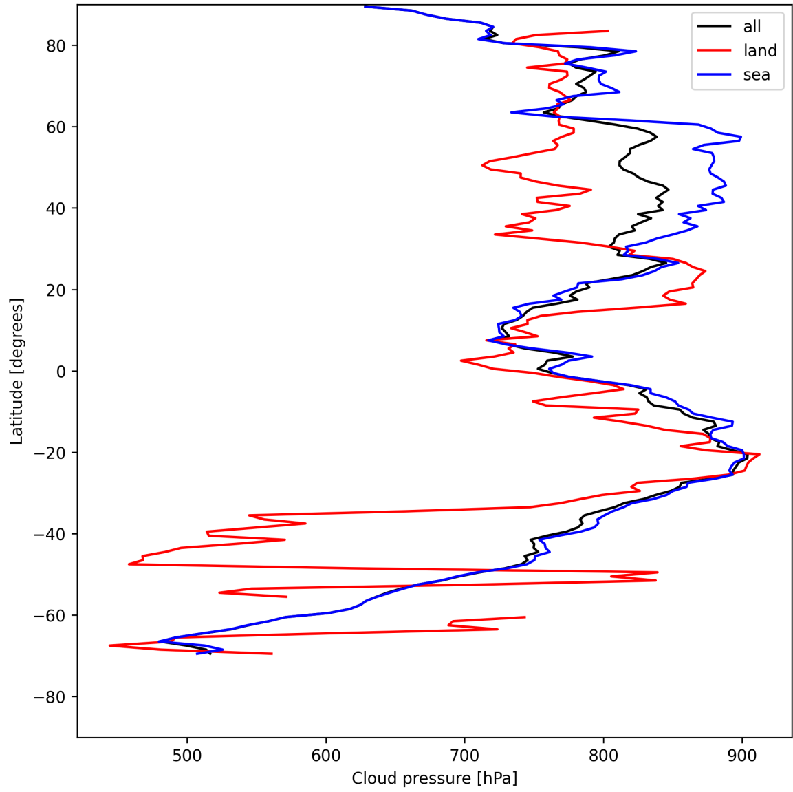
Figure 13: Zonal average of “Cloud pressure” for 2025-07-29 to 2025-07-30.
