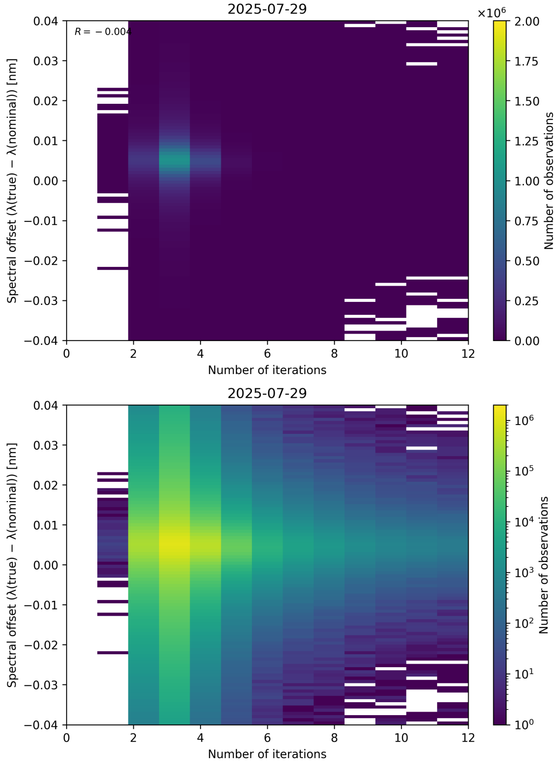
Figure 100: Scatter density plot of “Number of iterations” against “Spectral offset ( \lambda_{\text{true}} - \lambda_{\text{nominal}} )” for 2025-07-29 to 2025-07-30.
