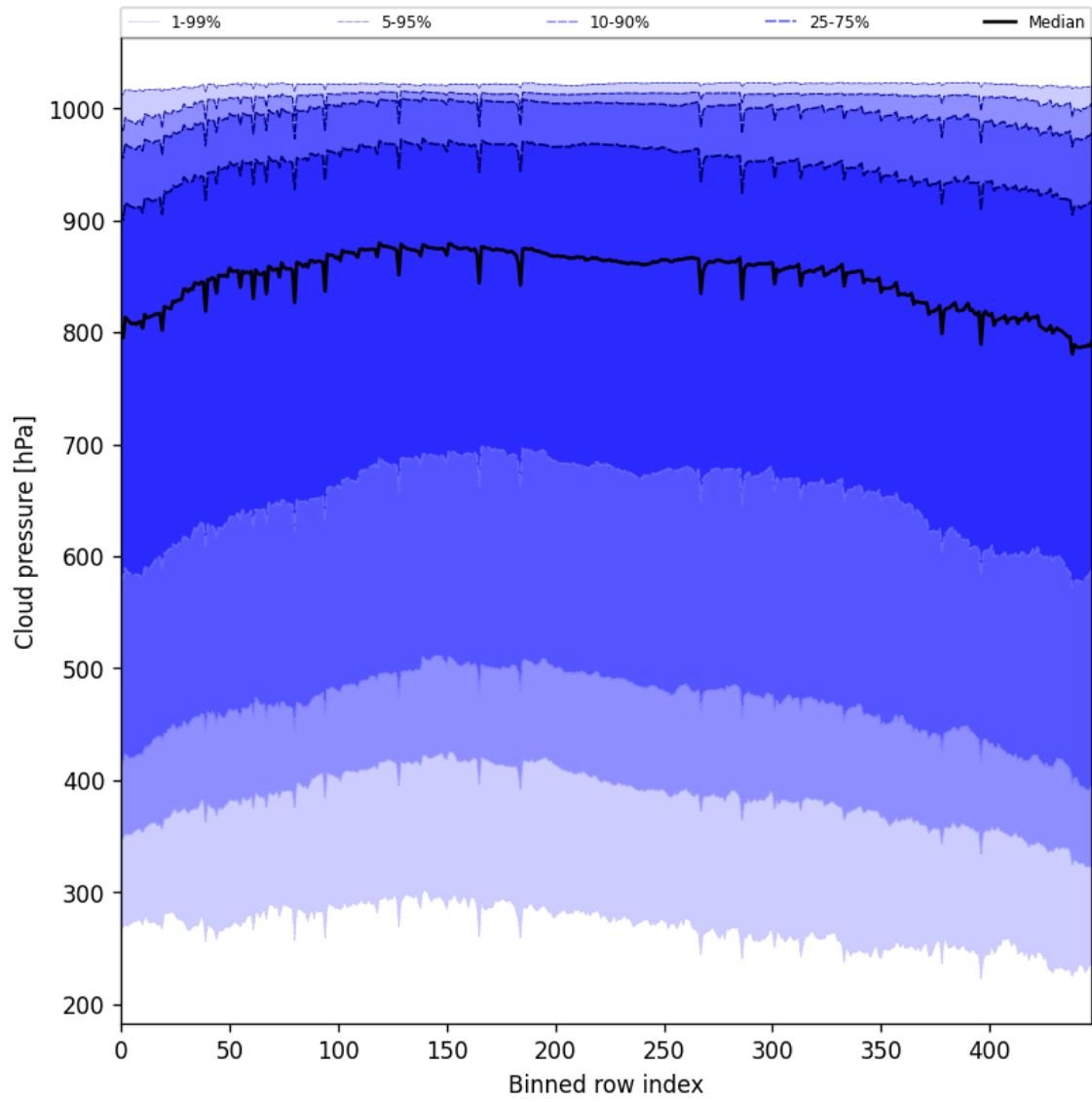
Figure 47: Along track statistics of “Cloud pressure” for 2025-07-29 to 2025-07-30
