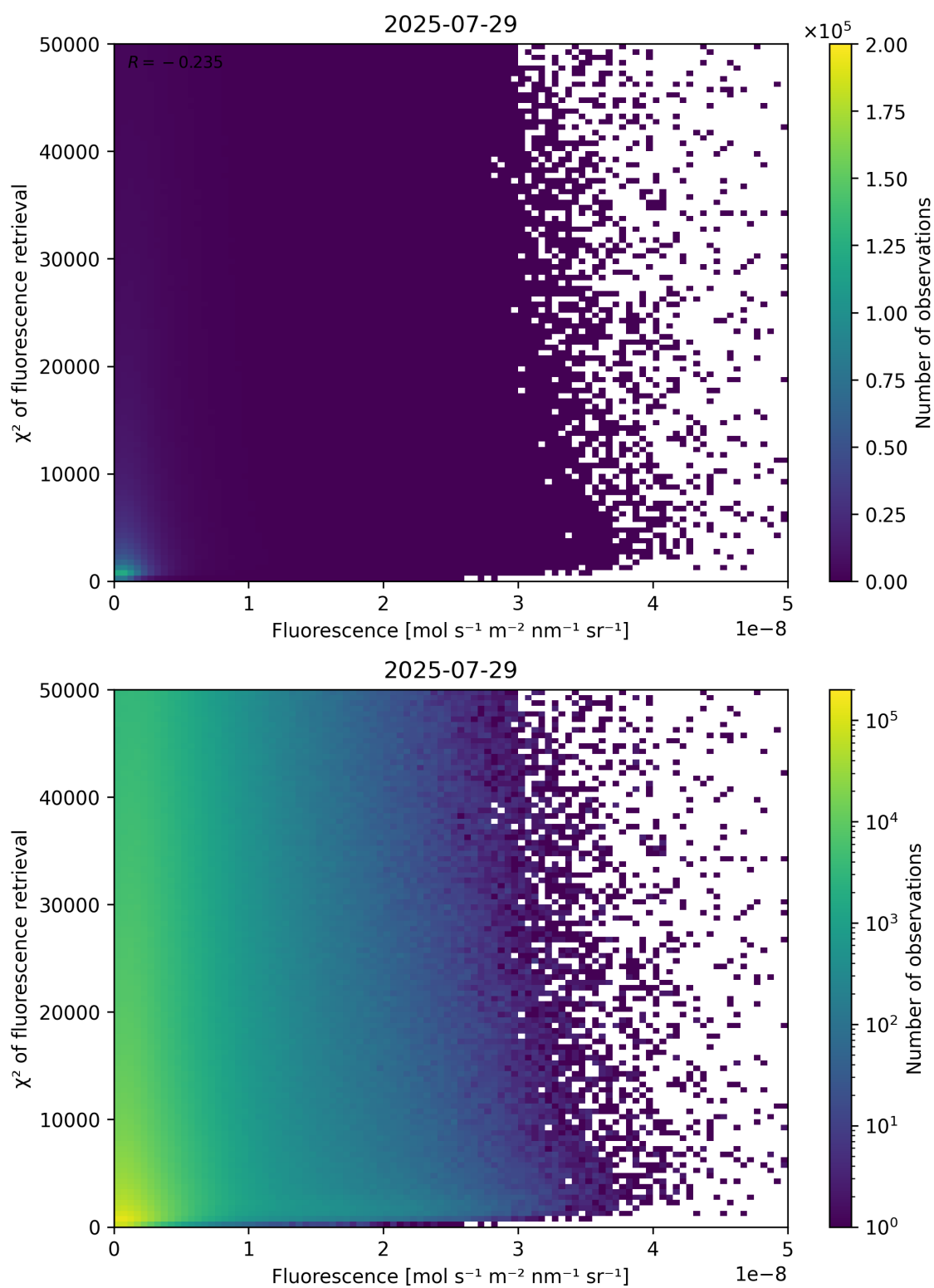
Figure 85: Scatter density plot of “Fluorescence” against “ \chi^2 of fluorescence retrieval” for 2025-07-29 to 2025-07-30.
