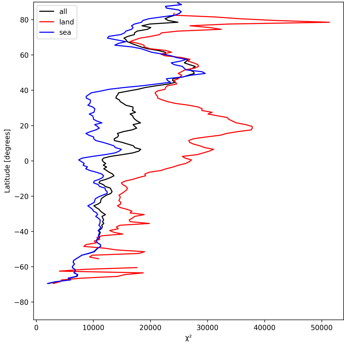
Figure 21: Zonal average of “ \chi^2 ” for 2025-07-29 to 2025-07-30.
