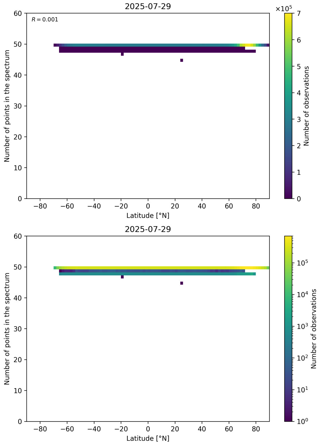
Figure 94: Scatter density plot of “Latitude” against “Number of points in the spectrum” for 2025-07-29 to 2025-07-30.
