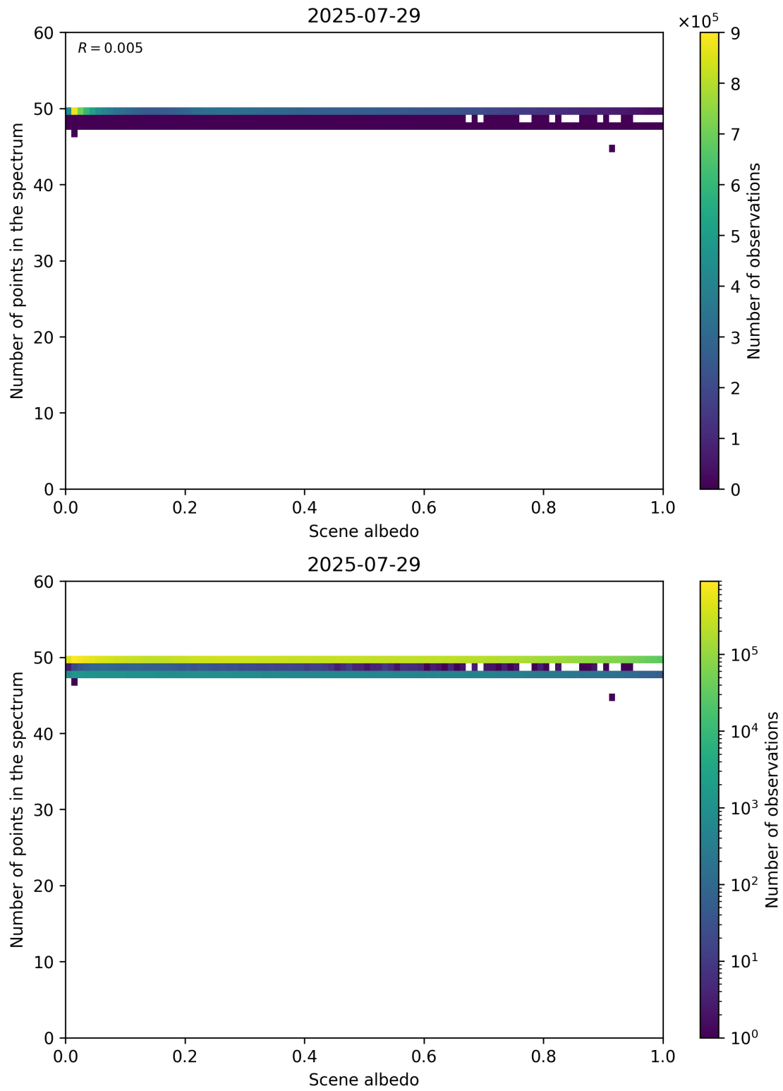
Figure 106: Scatter density plot of “Scene albedo” against “Number of points in the spectrum” for 2025-07-29 to 2025-07-30.
