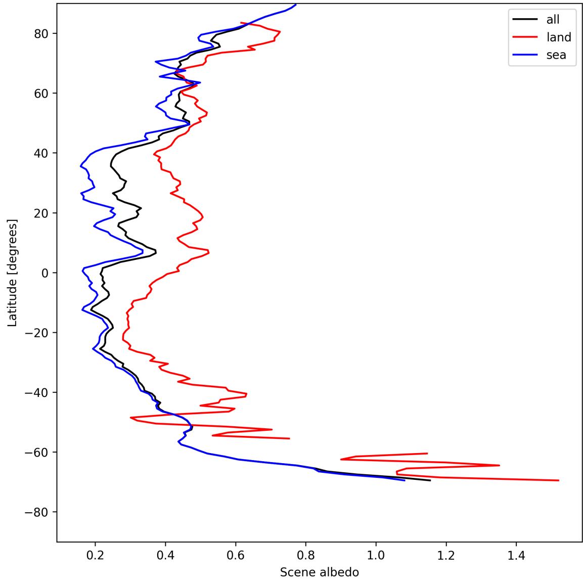
Figure 17: Zonal average of “Scene albedo” for 2025-07-29 to 2025-07-30.
