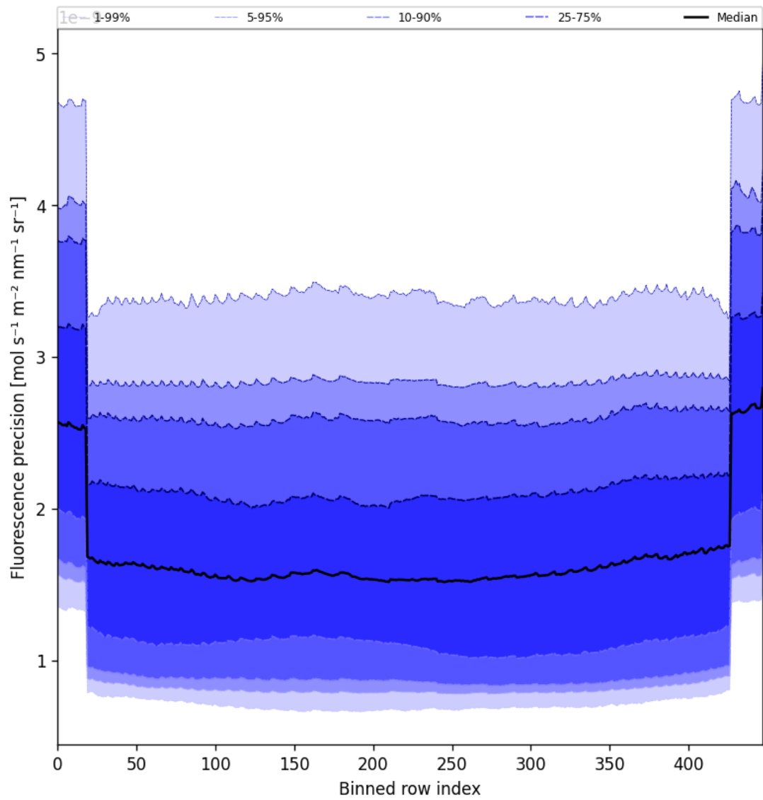
Figure 58: Along track statistics of “Fluorescence precision” for 2025-07-29 to 2025-07-30
