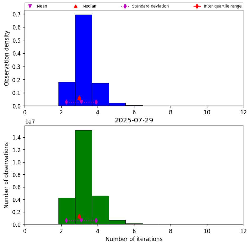
Figure 39: Histogram of “Number of iterations” for 2025-07-29 to 2025-07-30
