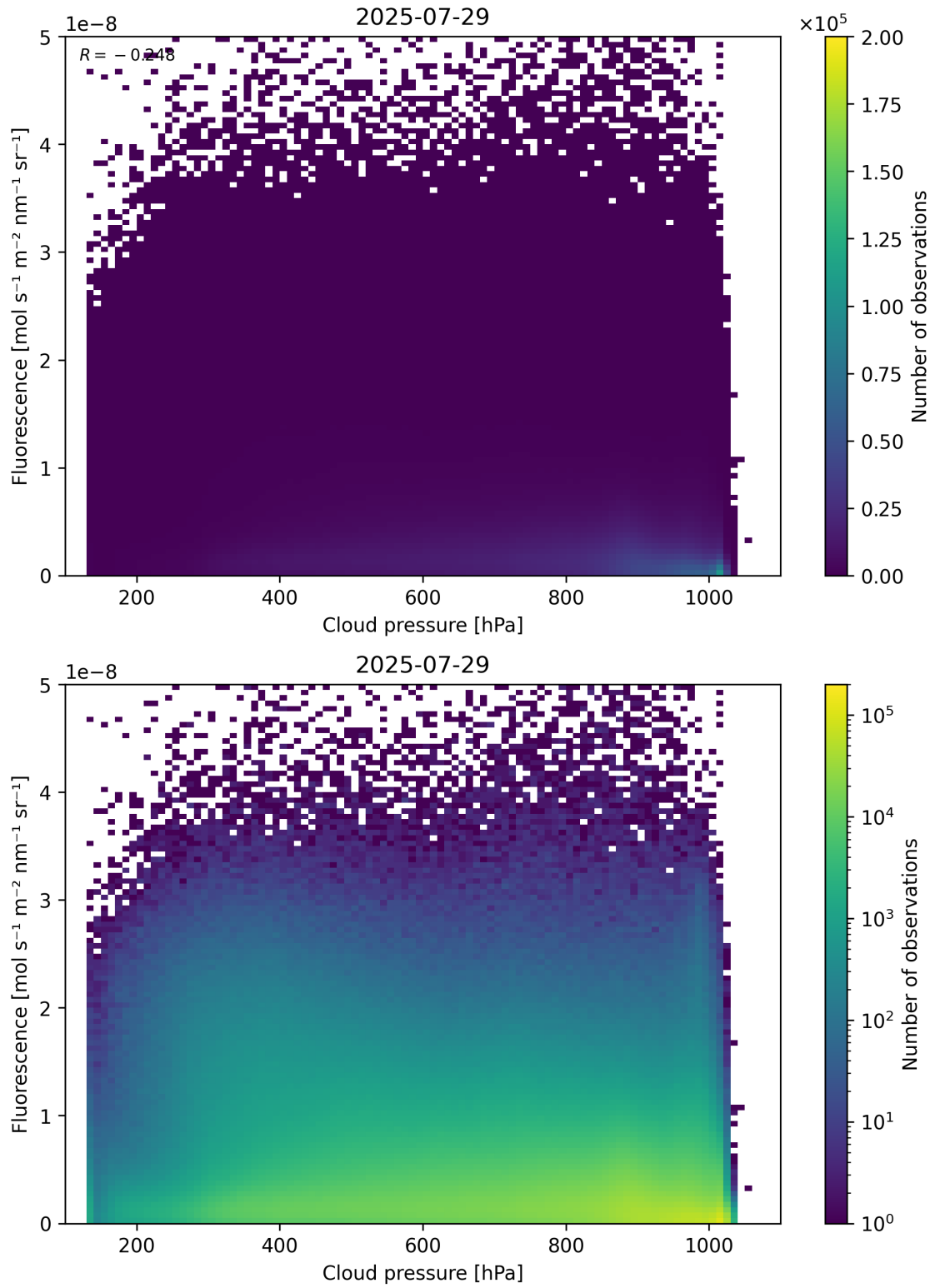
Figure 80: Scatter density plot of “Cloud pressure” against “Fluorescence” for 2025-07-29 to 2025-07-30.
