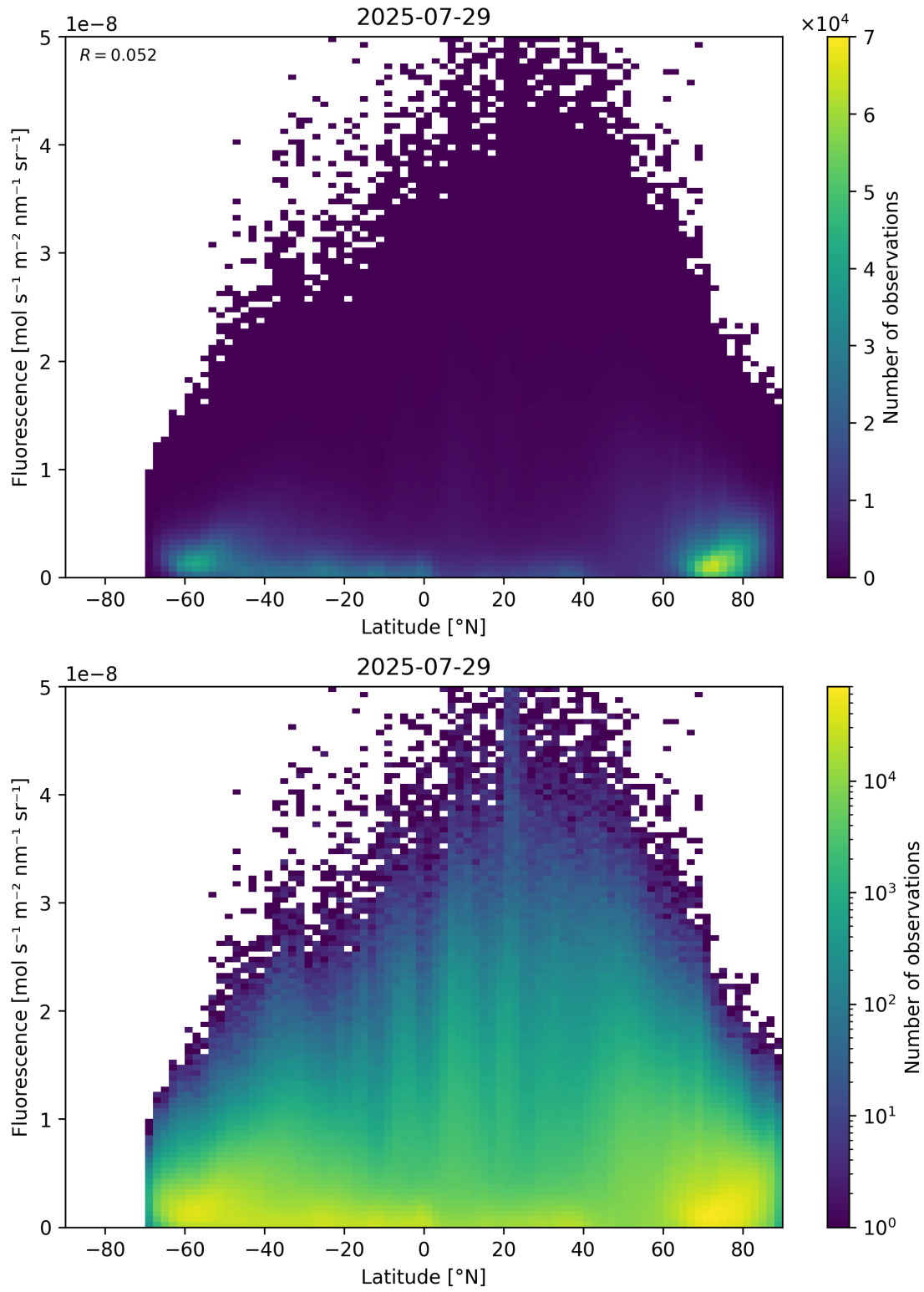
Figure 92: Scatter density plot of “Latitude” against “Fluorescence” for 2025-07-29 to 2025-07-30.
