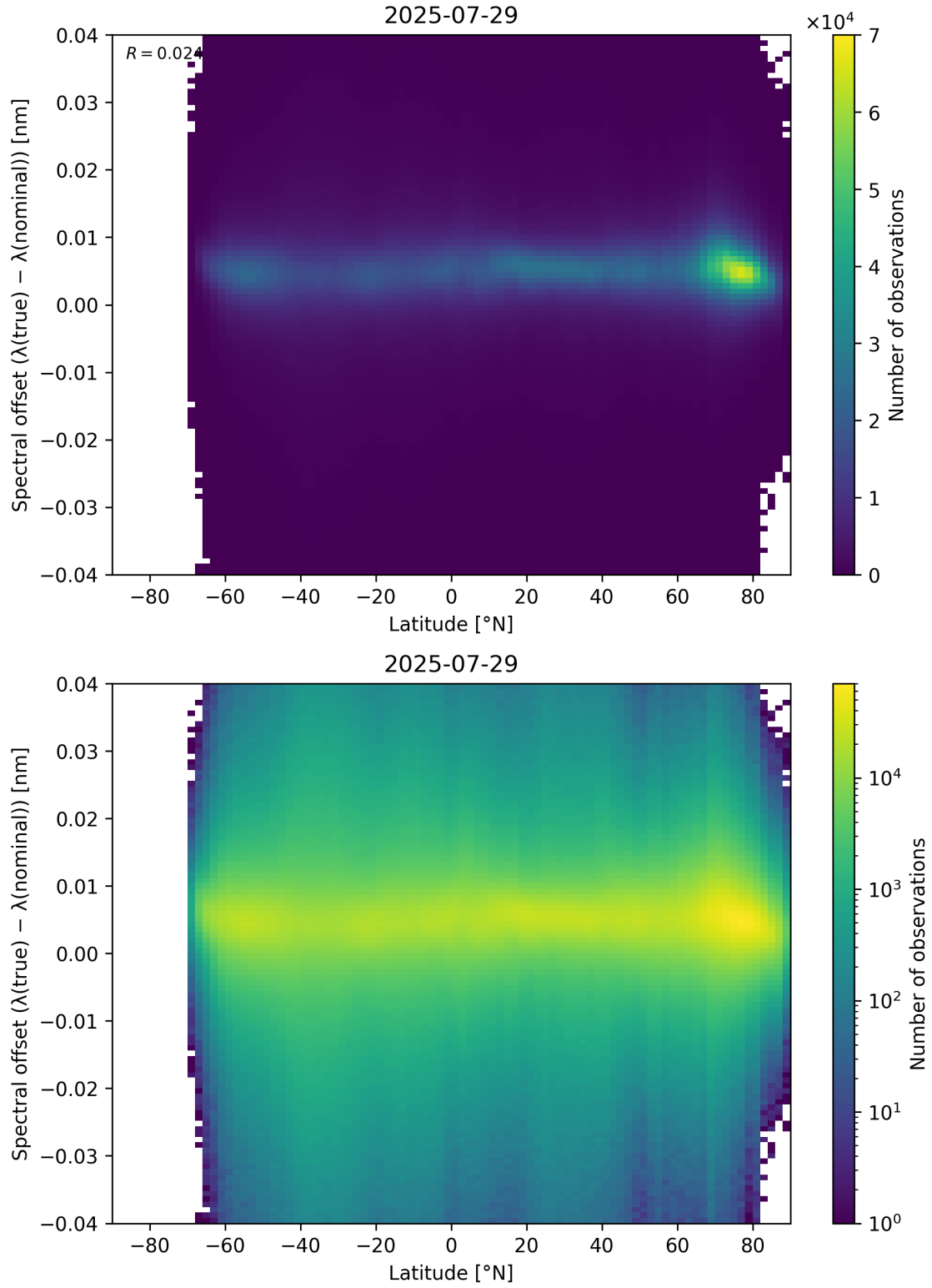
Figure 96: Scatter density plot of “Latitude” against “Spectral offset ( \lambda_{\text{true}} - \lambda_{\text{nominal}} )” for 2025-07-29 to 2025-07-30.
