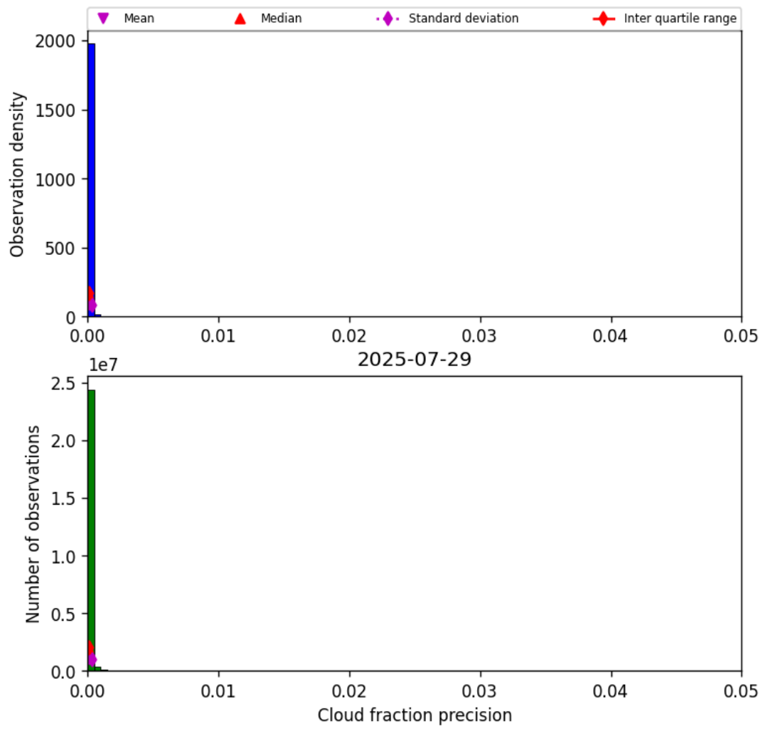
Figure 33: Histogram of “Cloud fraction precision” for 2025-07-29 to 2025-07-30
