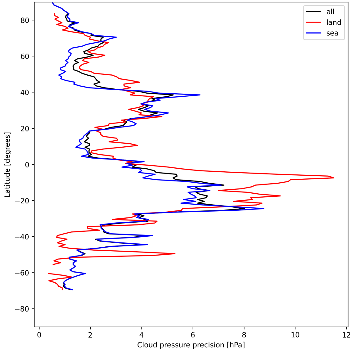
Figure 14: Zonal average of "Cloud pressure precision" for 2025-07-29 to 2025-07-30.
