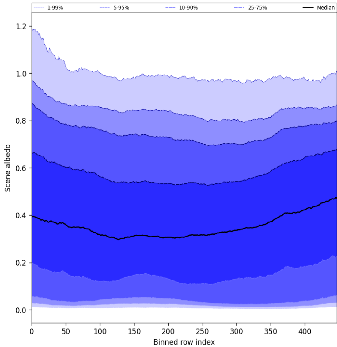
Figure 51: Along track statistics of “Scene albedo” for 2025-07-29 to 2025-07-30
