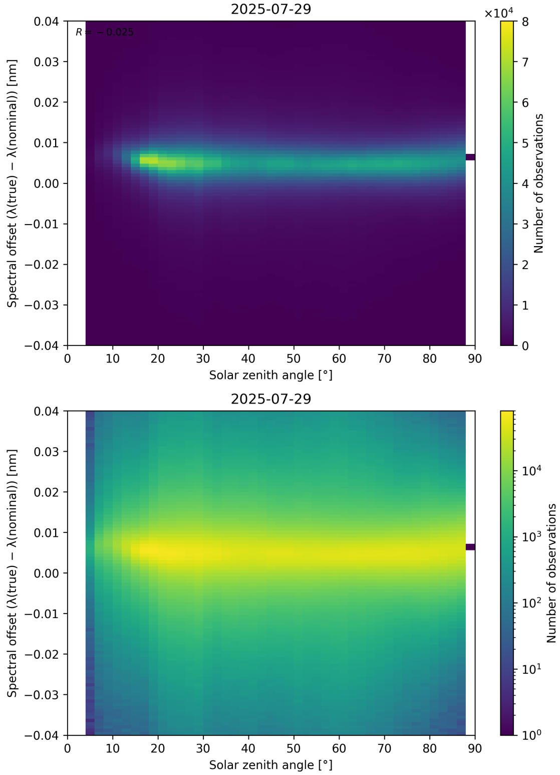
Figure 117: Scatter density plot of “Solar zenith angle” against “Spectral offset ( \lambda_{\text{true}} - \lambda_{\text{nominal}} )” for 2025-07-29 to 2025-07-30.
