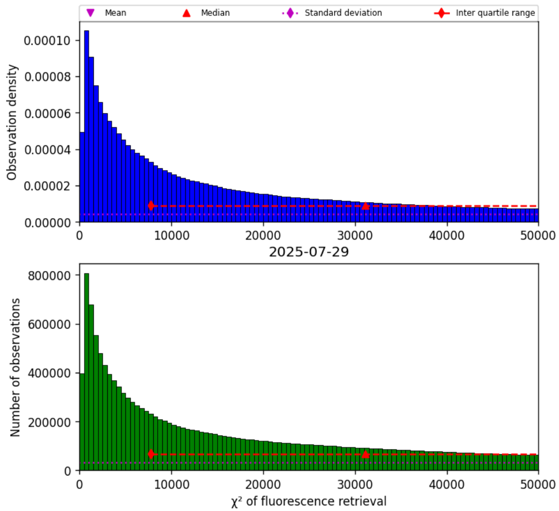
Figure 42: Histogram of “ \chi^2 of fluorescence retrieval” for 2025-07-29 to 2025-07-30
