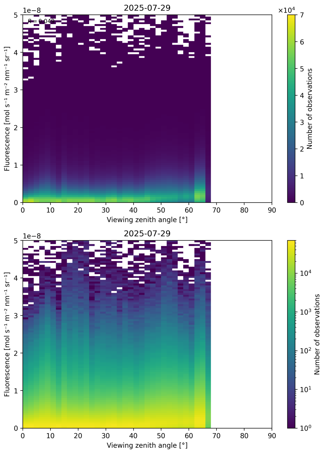
Figure 122: Scatter density plot of “Viewing zenith angle” against “Fluorescence” for 2025-07-29 to 2025-07-30.
