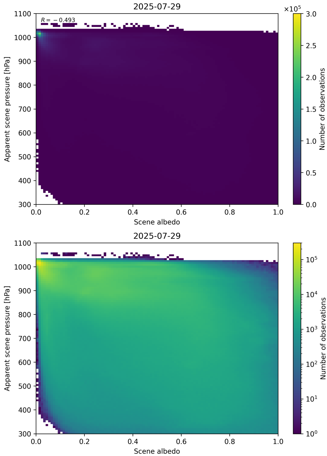
Figure 102: Scatter density plot of “Scene albedo” against “Apparent scene pressure” for 2025-07-29 to 2025-07-30.
