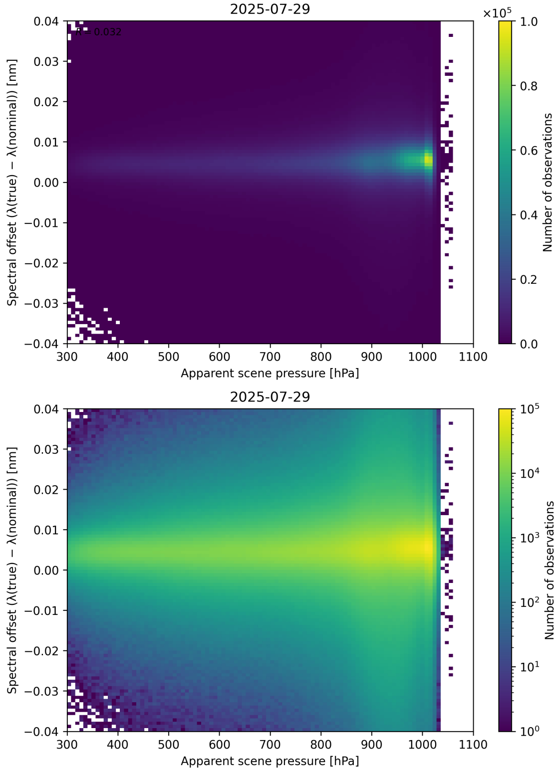
Figure 67: Scatter density plot of “Apparent scene pressure” against “Spectral offset ( \lambda_{\text{true}} - \lambda_{\text{nominal}} )” for 2025-07-29 to 2025-07-30.
