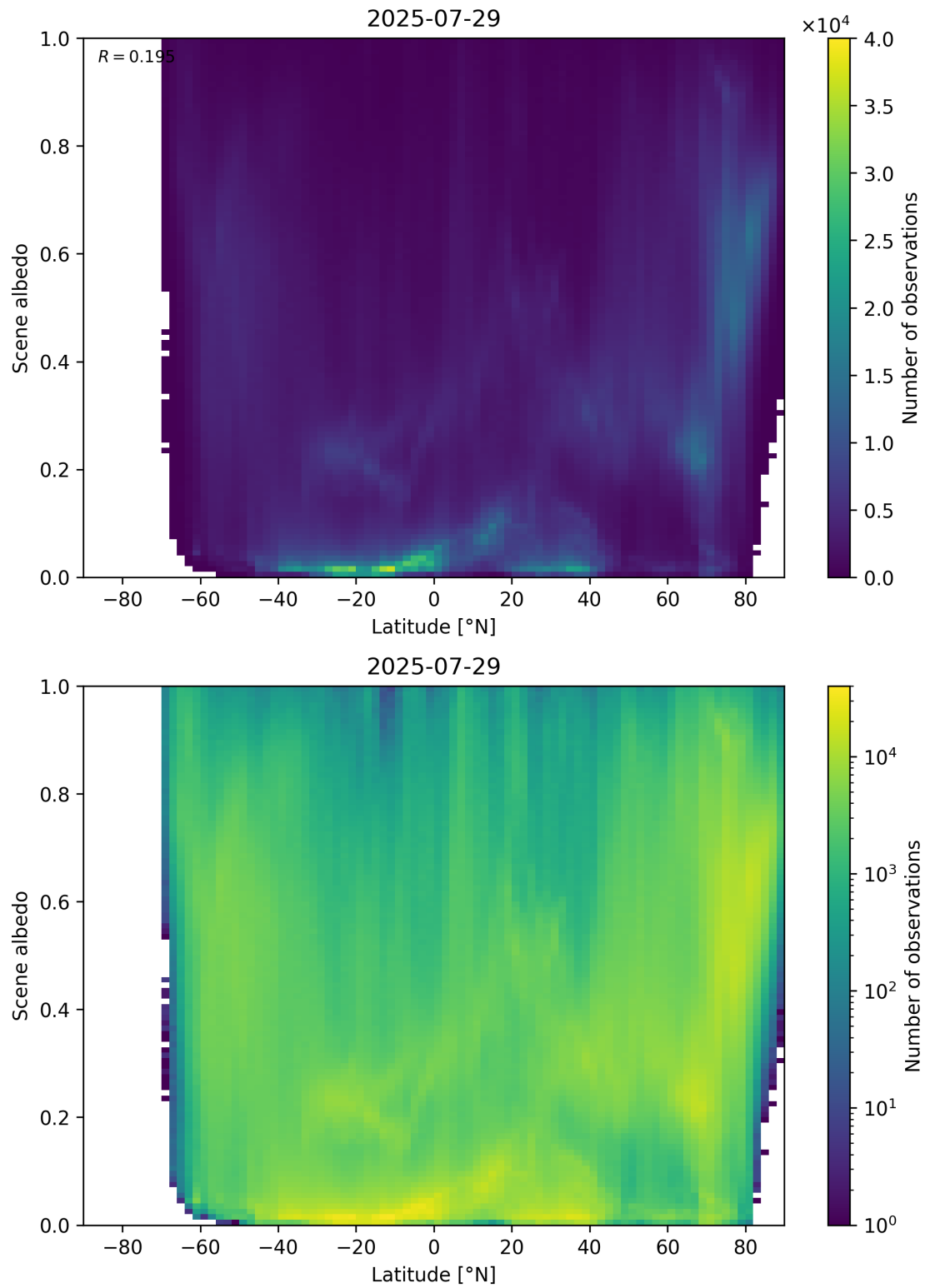
Figure 95: Scatter density plot of “Latitude” against “Scene albedo” for 2025-07-29 to 2025-07-30.
