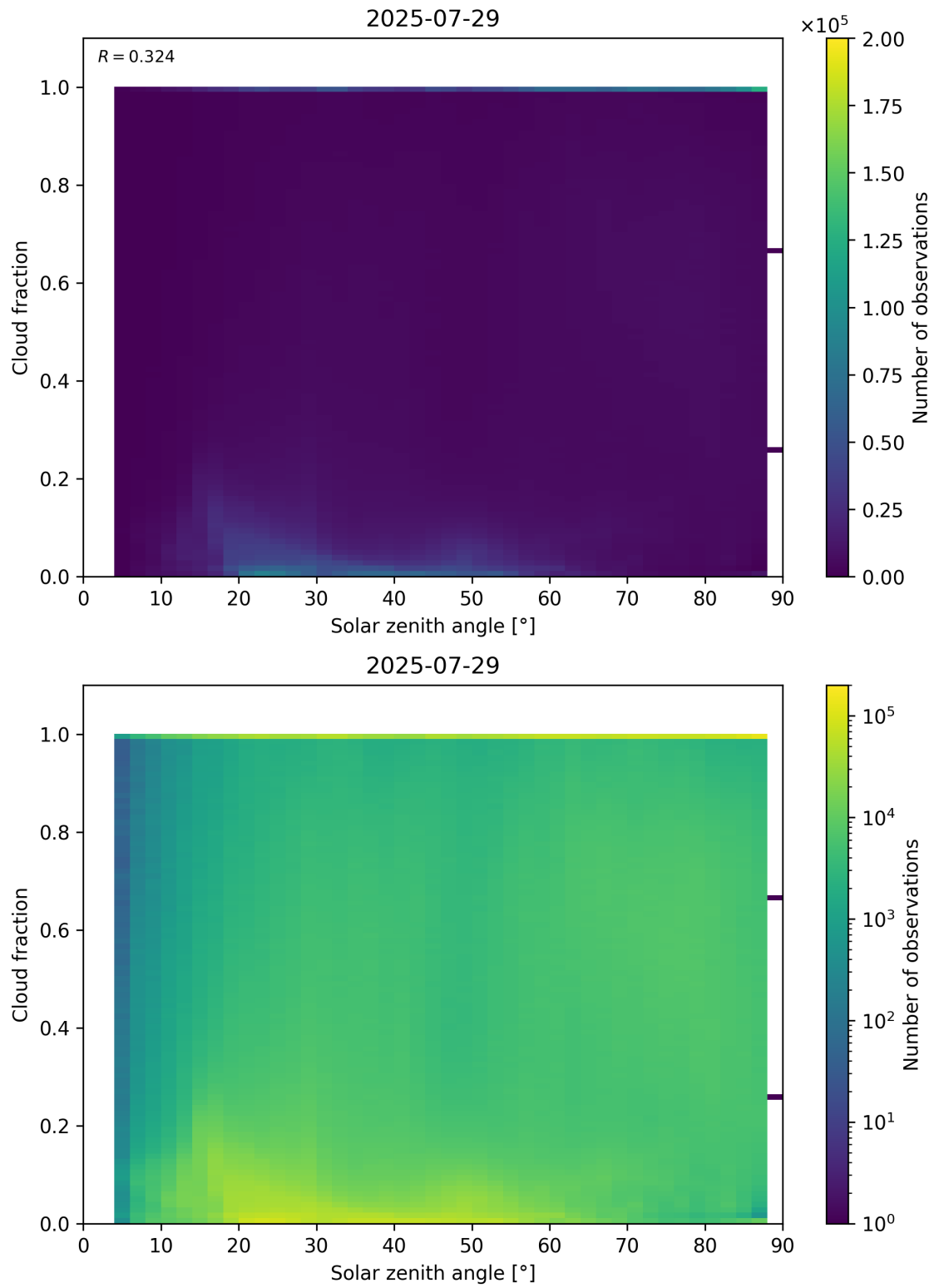
Figure 110: Scatter density plot of “Solar zenith angle” against “Cloud fraction” for 2025-07-29 to 2025-07-30.
