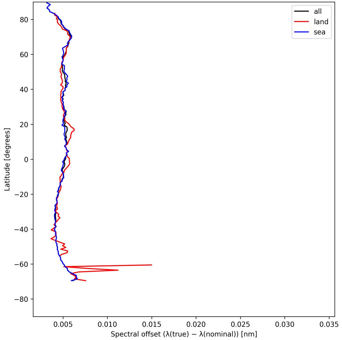
Figure 28: Zonal average of “Spectral offset ( \lambda_{\text{true}} - \lambda_{\text{nominal}} )” for 2025-07-29 to 2025-07-30.
