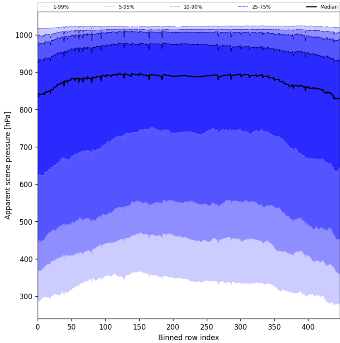
Figure 53: Along track statistics of “Apparent scene pressure” for 2025-07-29 to 2025-07-30
