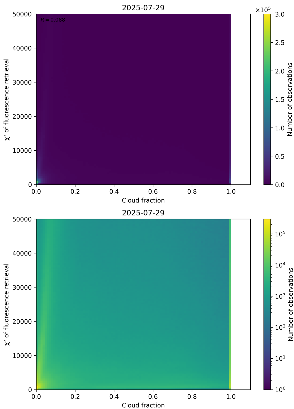
Figure 71: Scatter density plot of “Cloud fraction” against “ \chi^2 of fluorescence retrieval” for 2025-07-29 to 2025-07-30.
