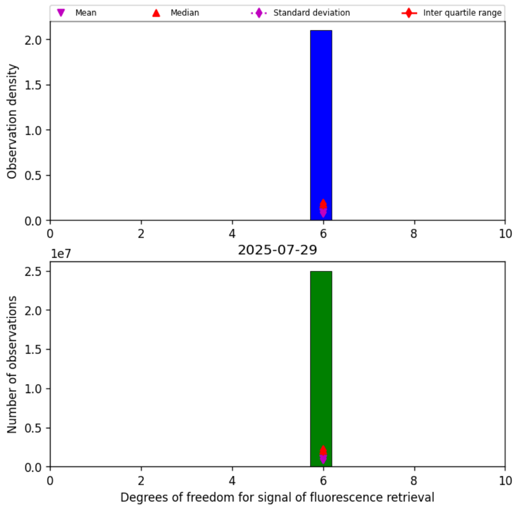
Figure 43: Histogram of “Degrees of freedom for signal of fluorescence retrieval” for 2025-07-29 to 2025-07-30
