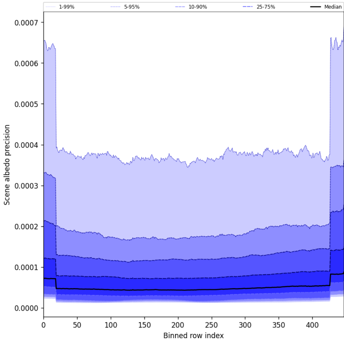
Figure 52: Along track statistics of “Scene albedo precision” for 2025-07-29 to 2025-07-30
