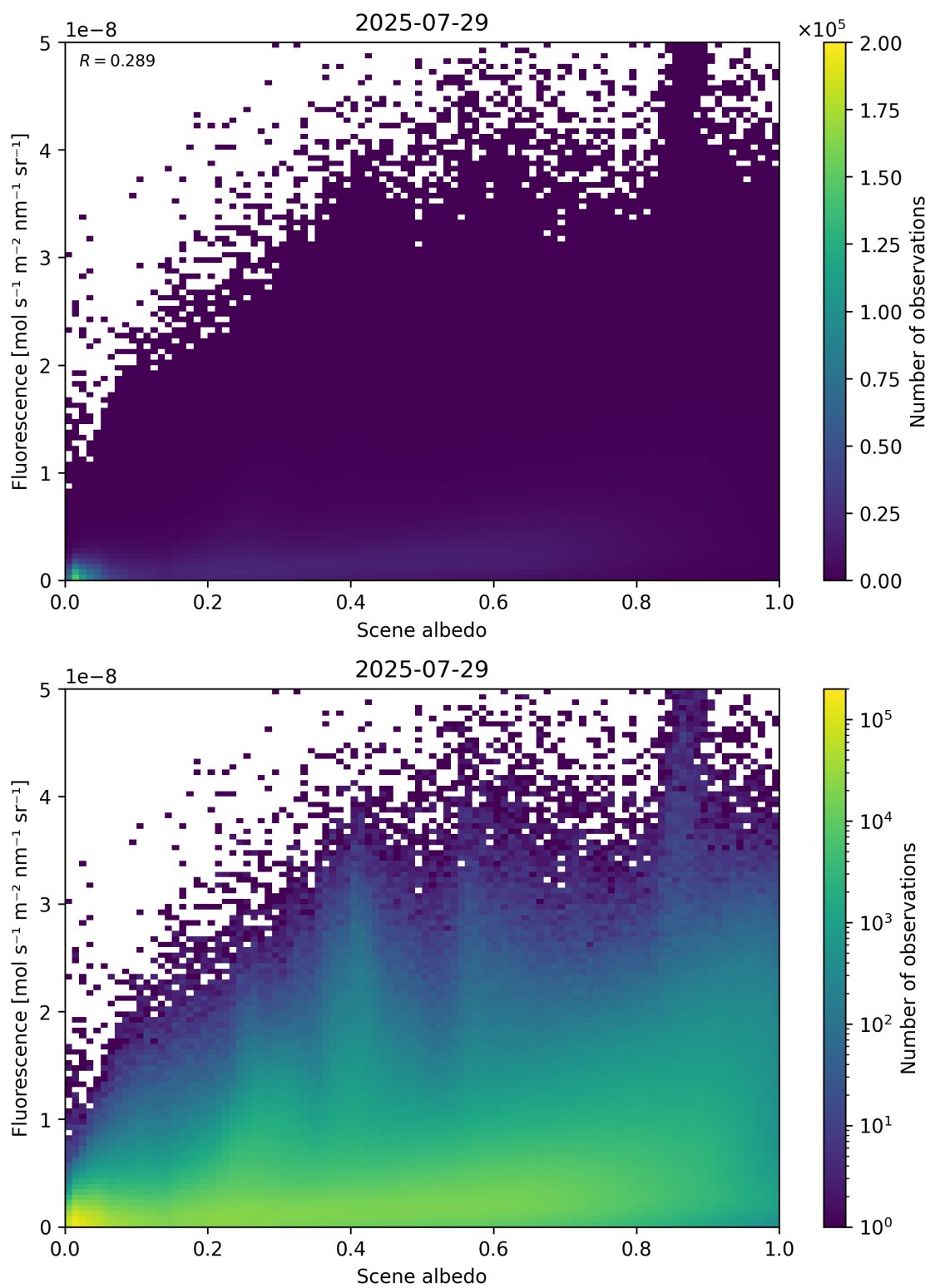
Figure 104: Scatter density plot of “Scene albedo” against “Fluorescence” for 2025-07-29 to 2025-07-30.
