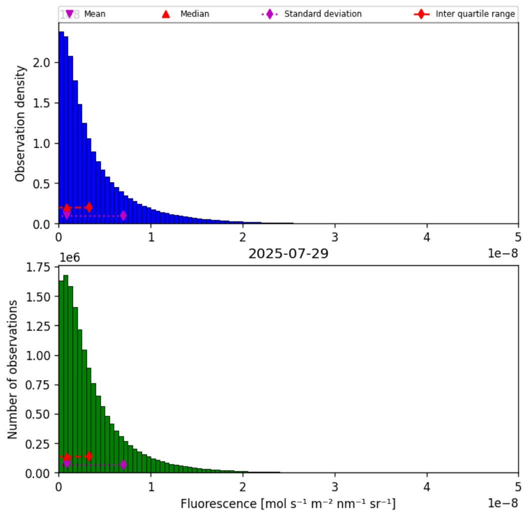
Figure 40: Histogram of “Fluorescence” for 2025-07-29 to 2025-07-30
