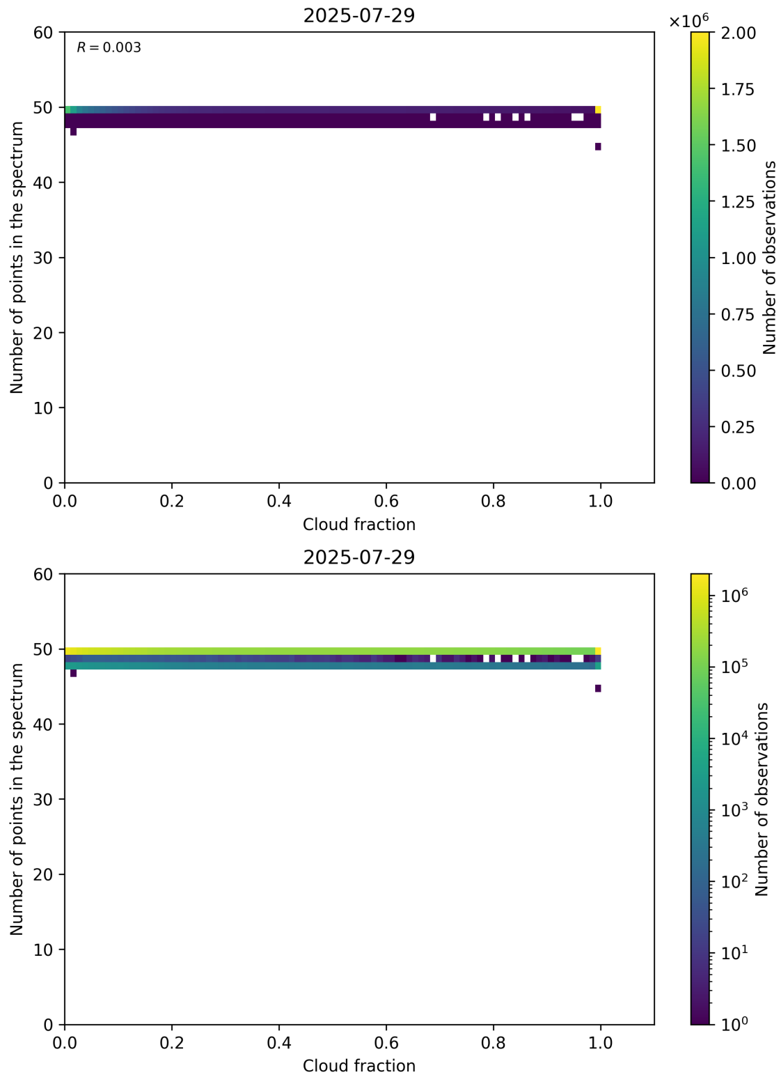
Figure 74: Scatter density plot of “Cloud fraction” against “Number of points in the spectrum” for 2025-07-29 to 2025-07-30.
