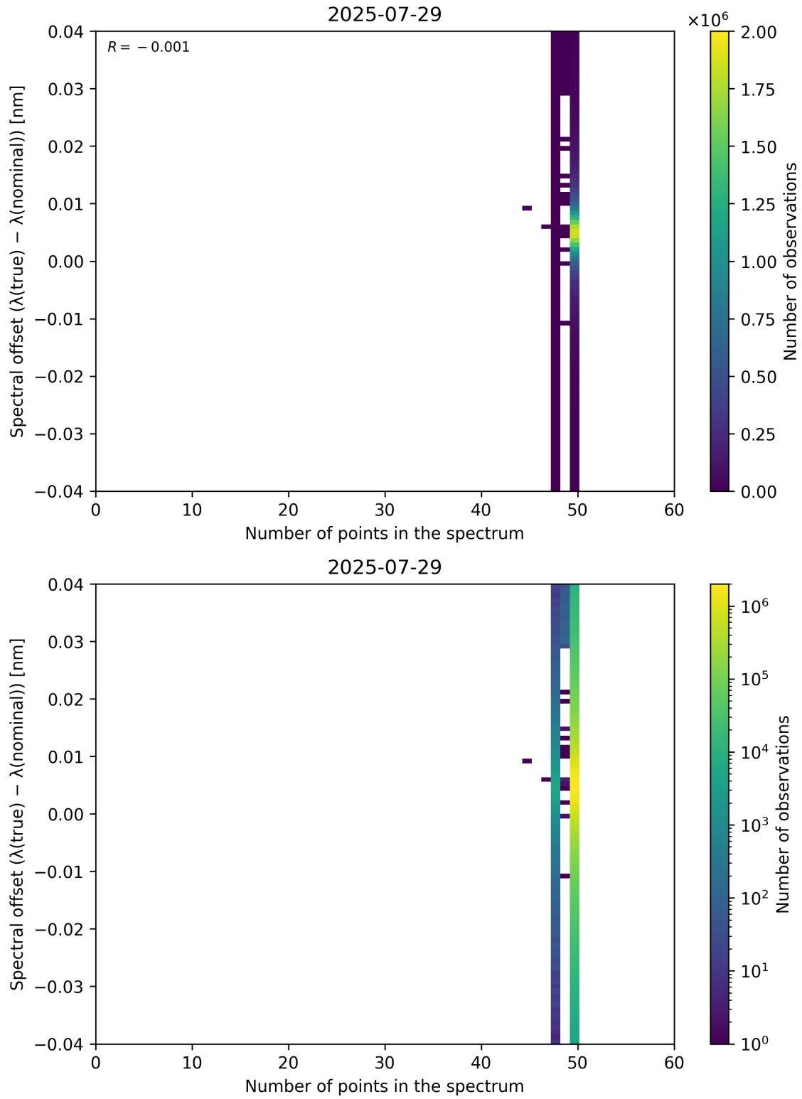
Figure 101: Scatter density plot of “Number of points in the spectrum” against “Spectral offset ( \lambda_{\text{true}} - \lambda_{\text{nominal}} )” for 2025-07-29 to 2025-07-30.
