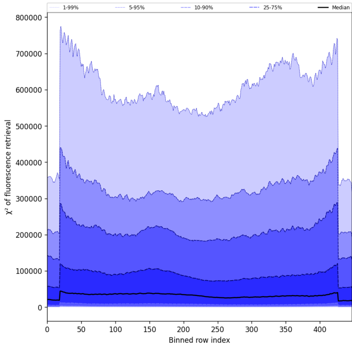
Figure 59: Along track statistics of “ \chi^2 of fluorescence retrieval” for 2025-07-29 to 2025-07-30
