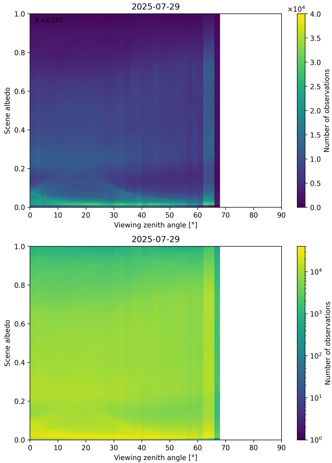
Figure 126: Scatter density plot of “Viewing zenith angle” against “Scene albedo” for 2025-07-29 to 2025-07-30.
