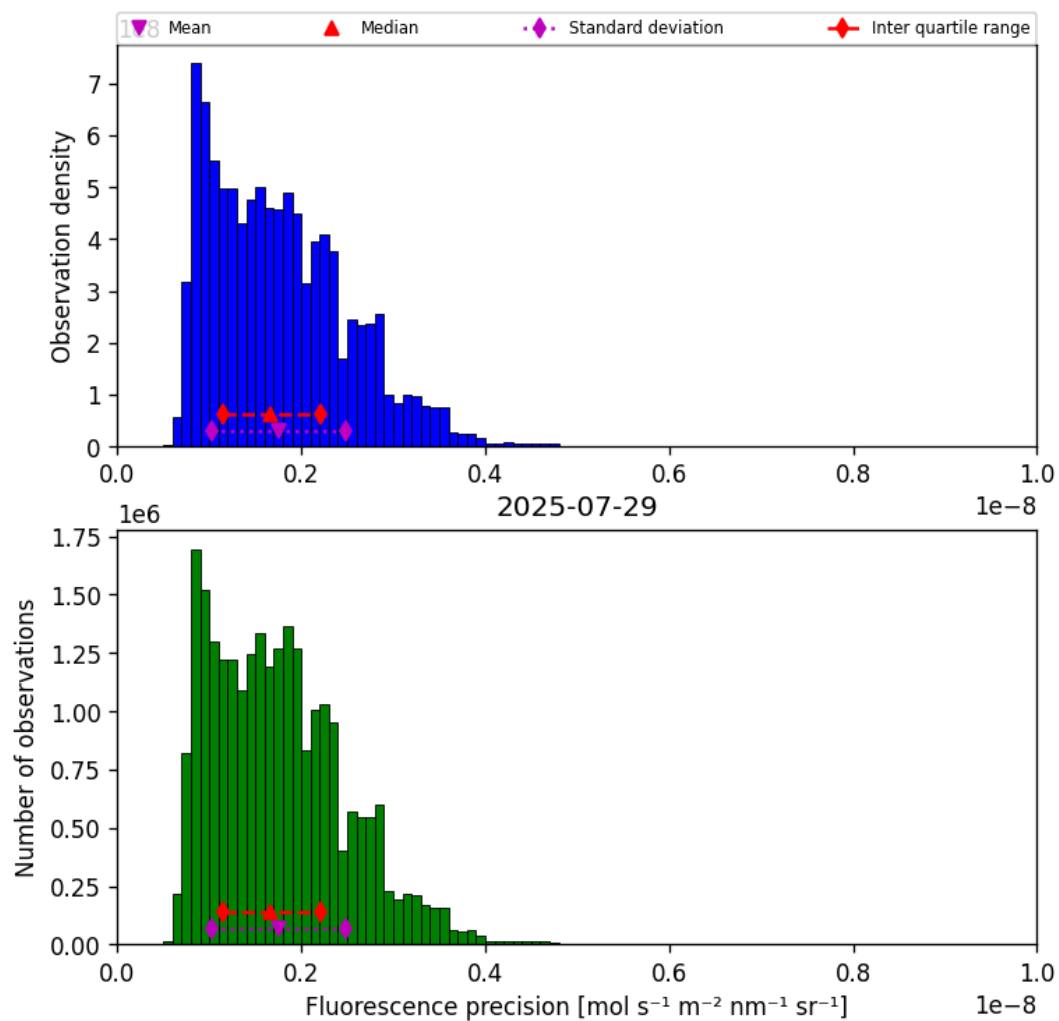
Figure 41: Histogram of “Fluorescence precision” for 2025-07-29 to 2025-07-30
