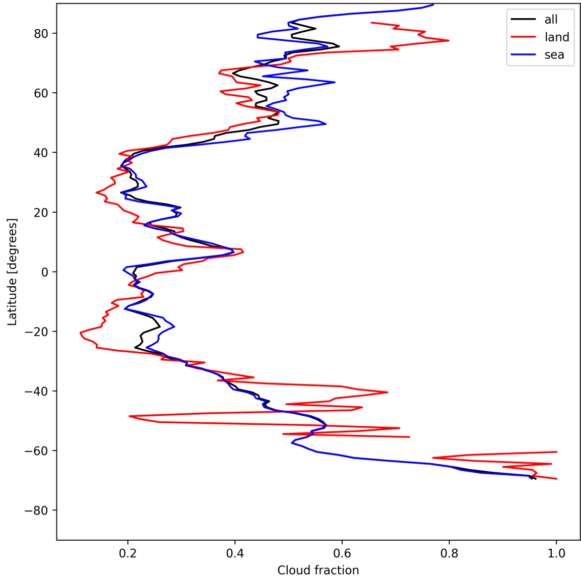
Figure 15: Zonal average of “Cloud fraction” for 2025-07-29 to 2025-07-30.
