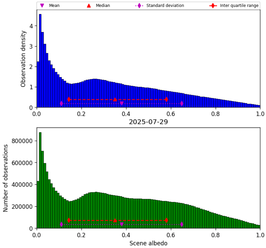
Figure 34: Histogram of “Scene albedo” for 2025-07-29 to 2025-07-30
