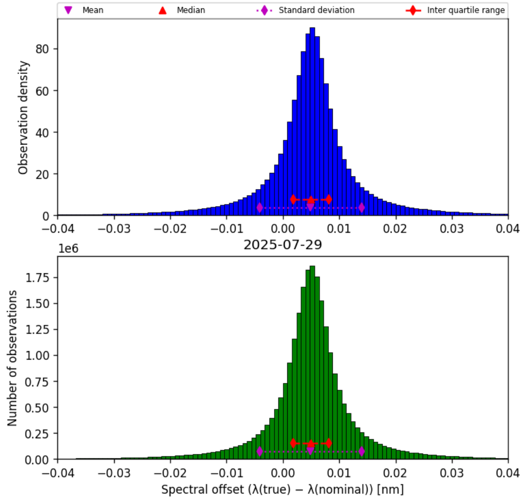
Figure 45: Histogram of “Spectral offset ( \lambda_{\text{true}} - \lambda_{\text{nominal}} )” for 2025-07-29 to 2025-07-30
