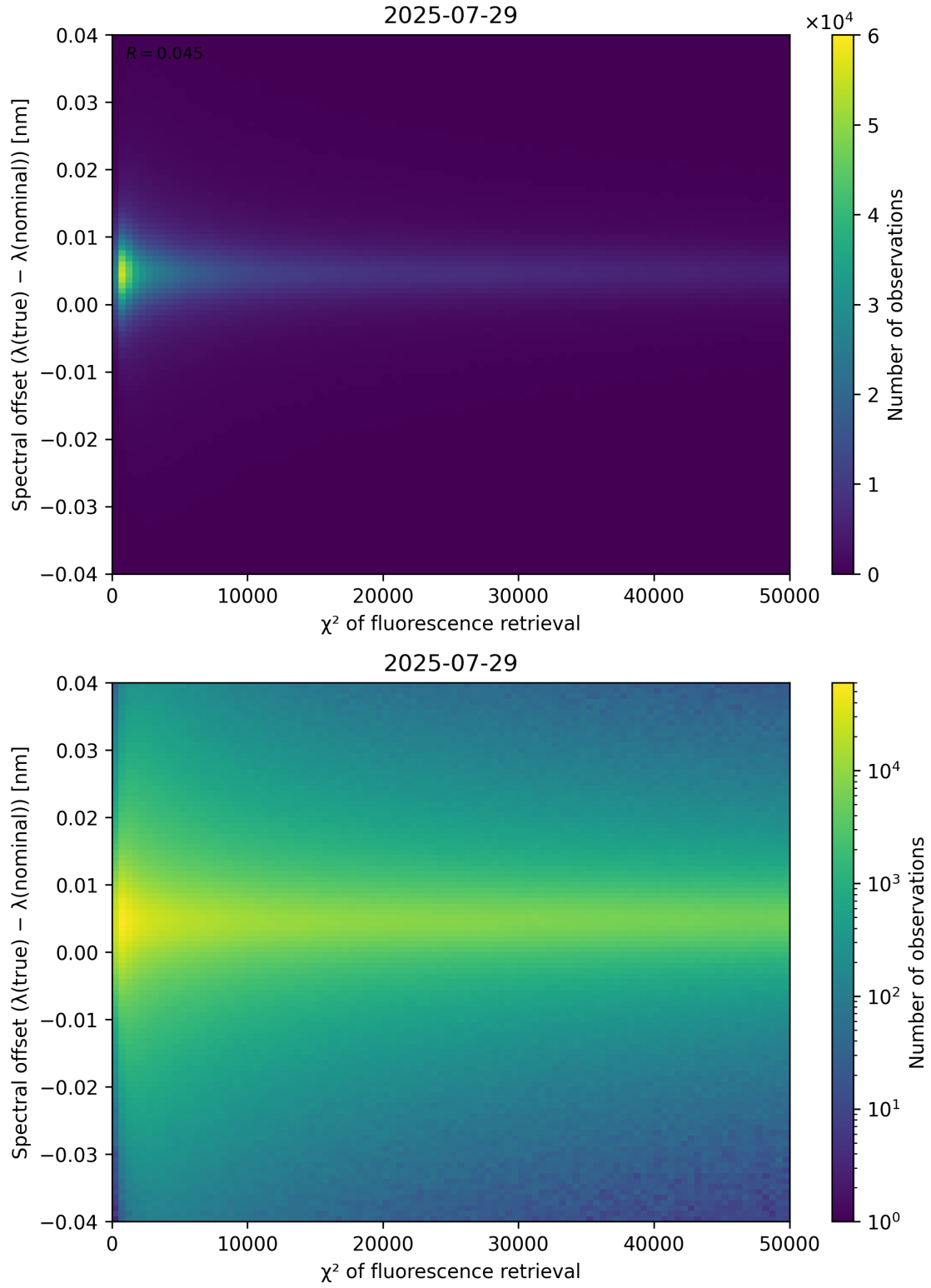
Figure 69: Scatter density plot of “ \chi^2 of fluorescence retrieval” against “Spectral offset ( \lambda_{\text{true}} - \lambda_{\text{nominal}} )” for 2025-07-29 to 2025-07-30.
