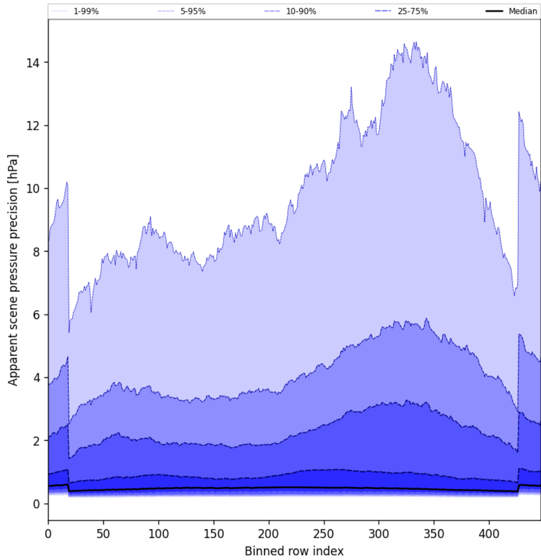
Figure 54: Along track statistics of “Apparent scene pressure precision” for 2025-07-29 to 2025-07-30
