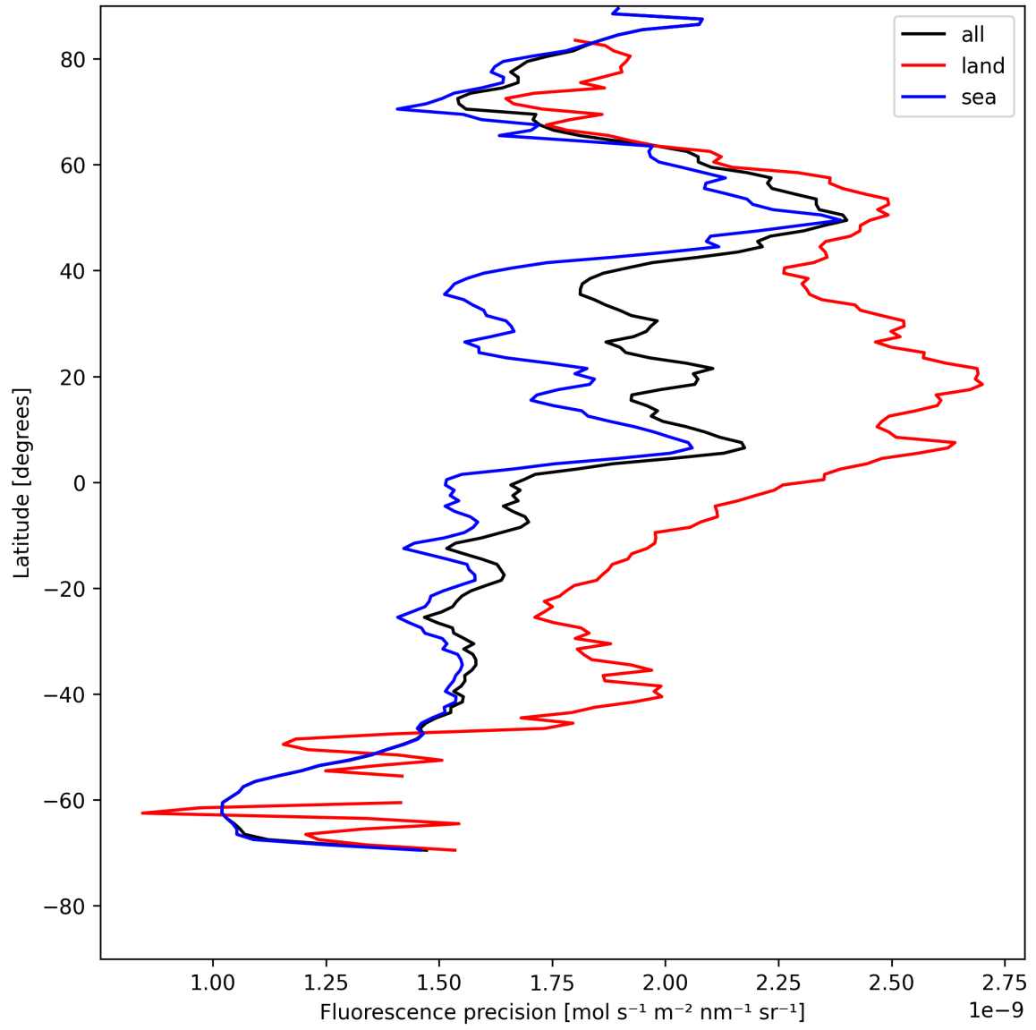
Figure 24: Zonal average of “Fluorescence precision” for 2025-07-29 to 2025-07-30.
