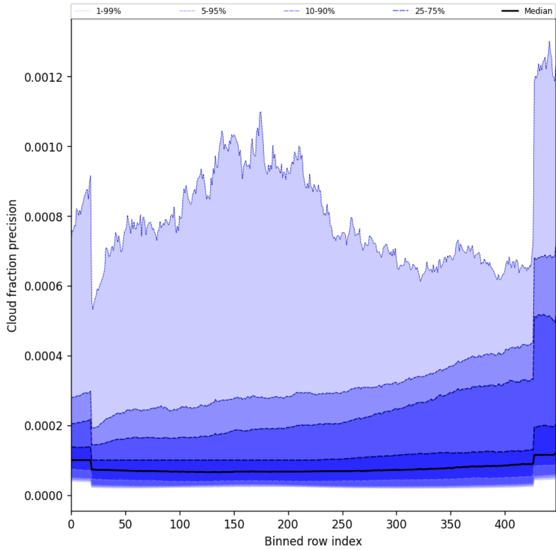
Figure 50: Along track statistics of “Cloud fraction precision” for 2025-07-29 to 2025-07-30
