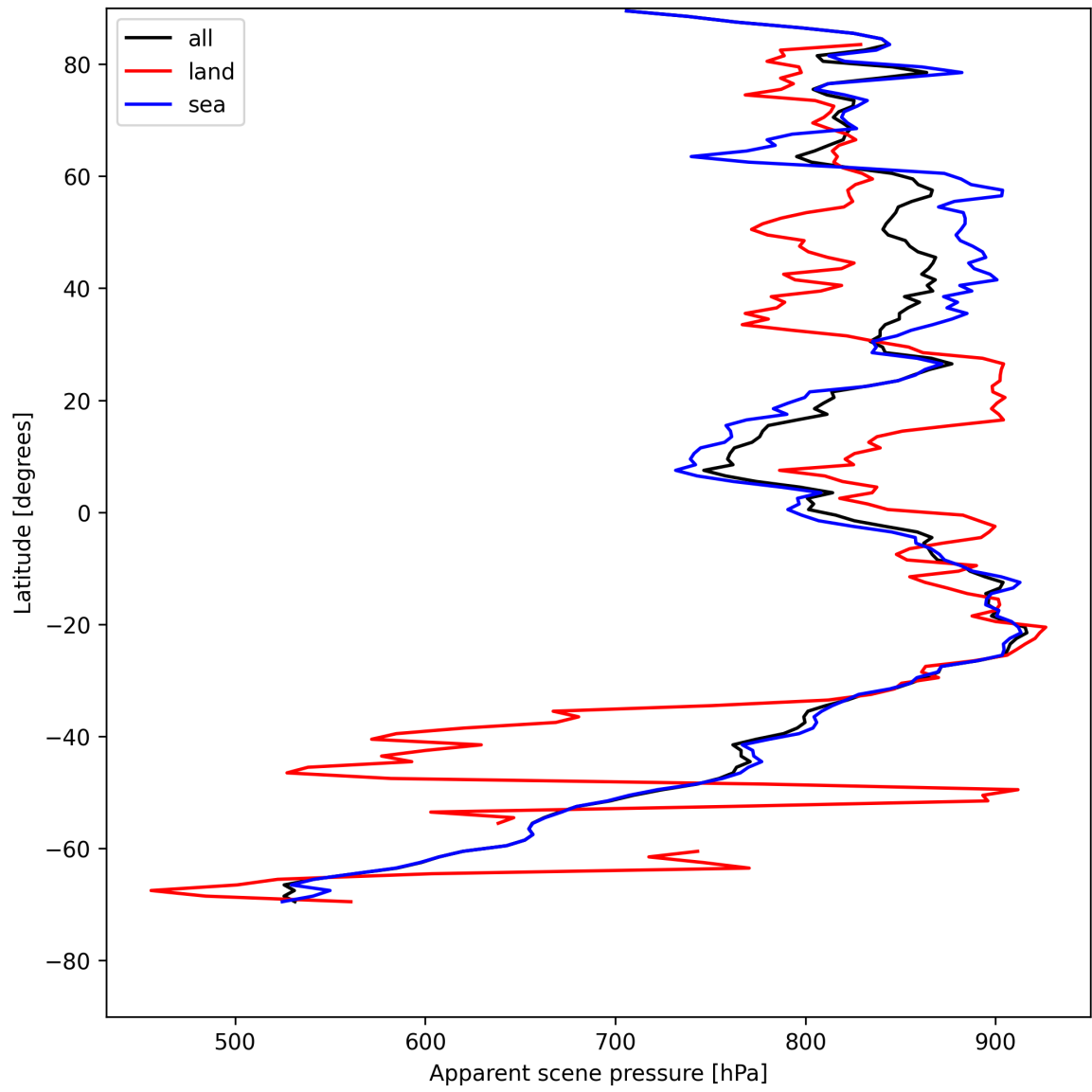
Figure 19: Zonal average of “Apparent scene pressure” for 2025-07-29 to 2025-07-30.
