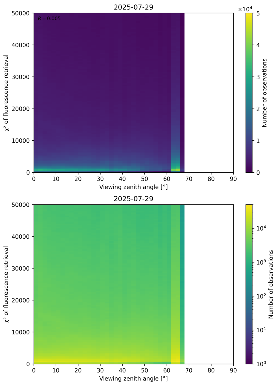
Figure 119: Scatter density plot of “Viewing zenith angle” against “ \chi^2 of fluorescence retrieval” for 2025-07-29 to 2025-07-30.
