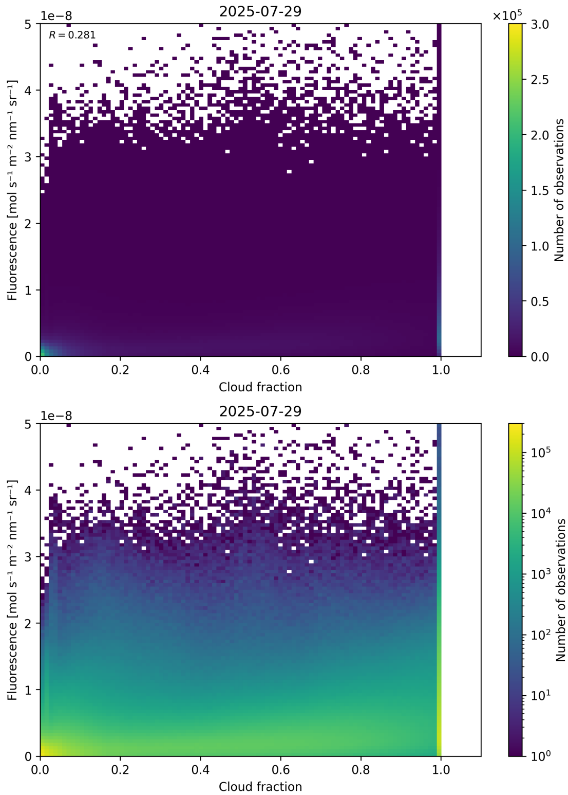
Figure 72: Scatter density plot of “Cloud fraction” against “Fluorescence” for 2025-07-29 to 2025-07-30.
