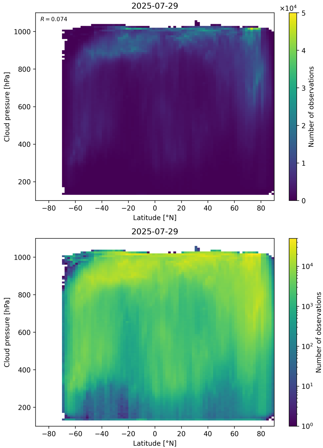
Figure 91: Scatter density plot of “Latitude” against “Cloud pressure” for 2025-07-29 to 2025-07-30.
