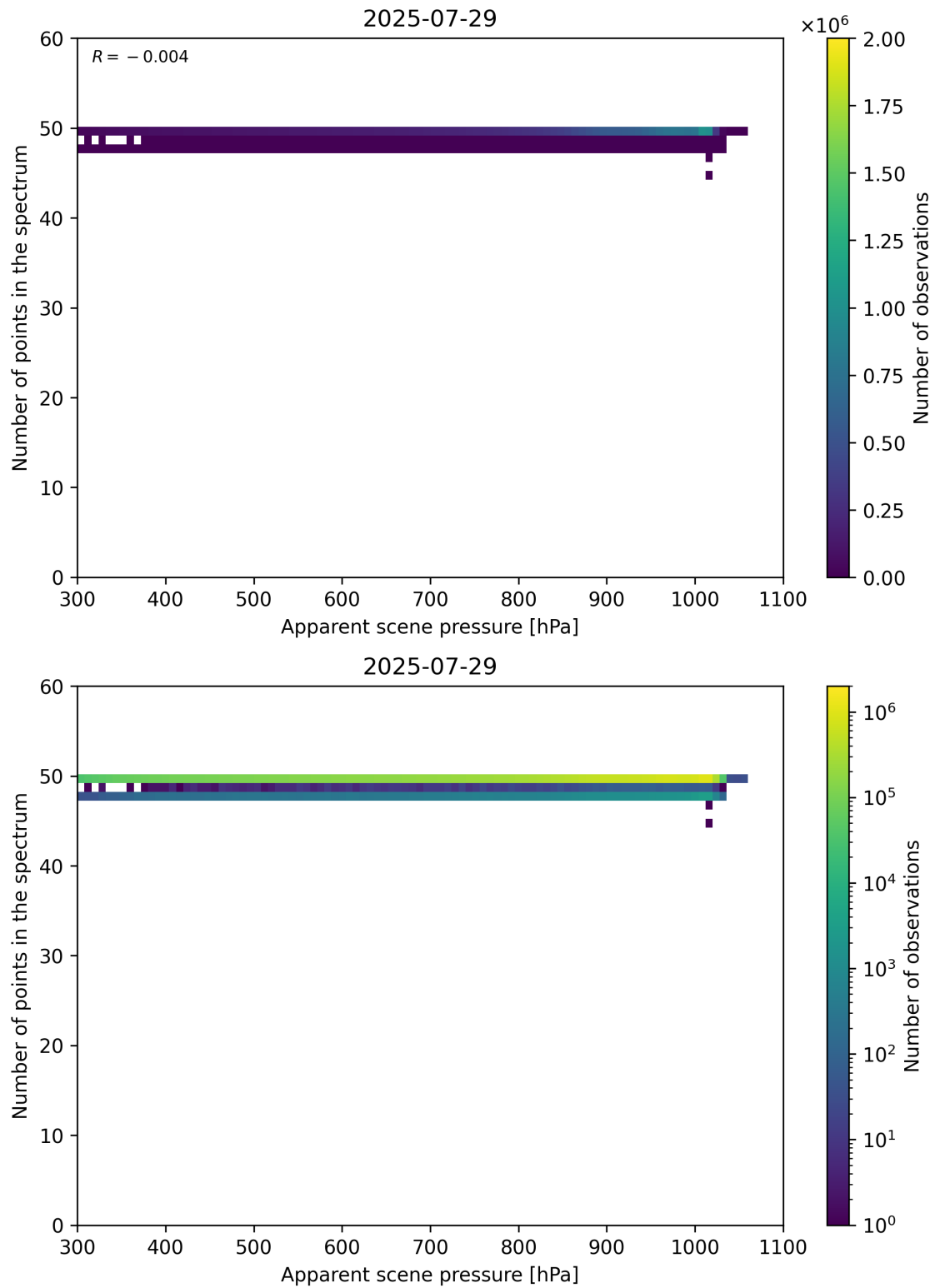
Figure 66: Scatter density plot of “Apparent scene pressure” against “Number of points in the spectrum” for 2025-07-29 to 2025-07-30.
