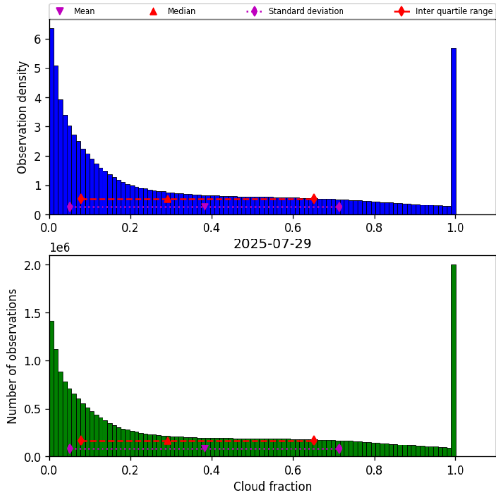
Figure 32: Histogram of “Cloud fraction” for 2025-07-29 to 2025-07-30
