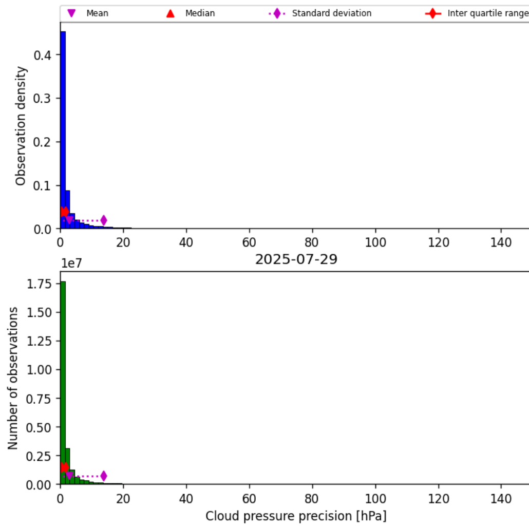
Figure 31: Histogram of “Cloud pressure precision” for 2025-07-29 to 2025-07-30
