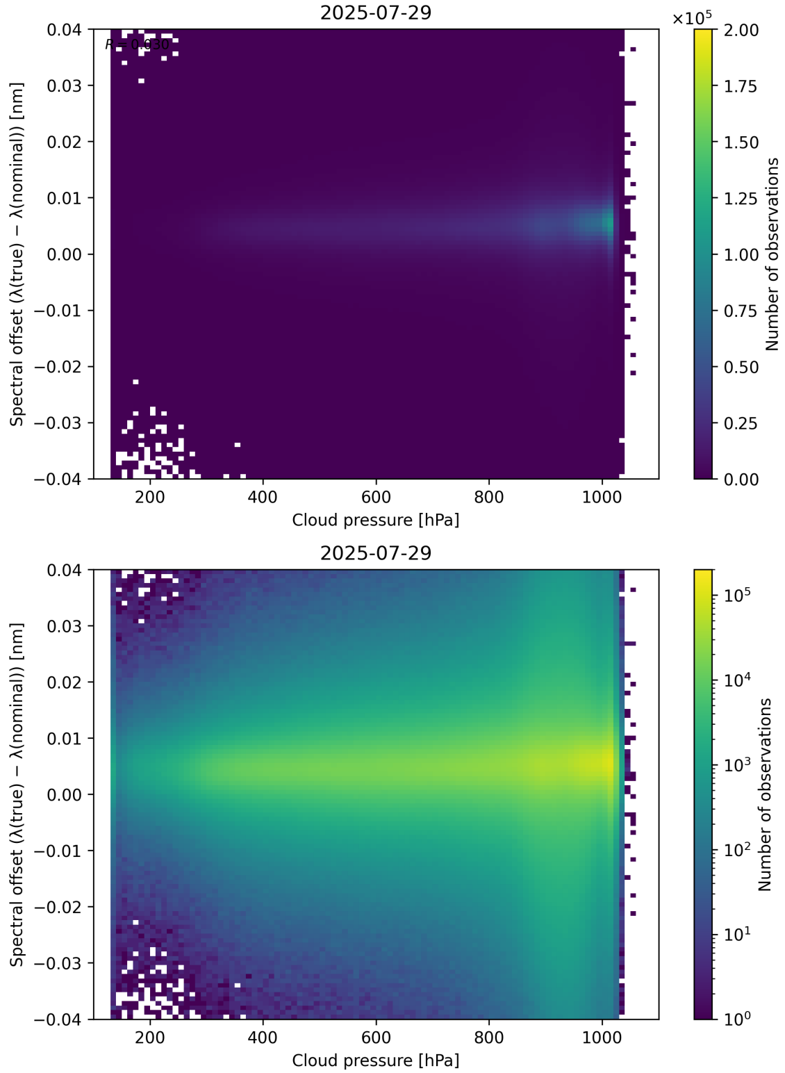
Figure 84: Scatter density plot of “Cloud pressure” against “Spectral offset ( \lambda_{\text{true}} - \lambda_{\text{nominal}} )” for 2025-07-29 to 2025-07-30.
