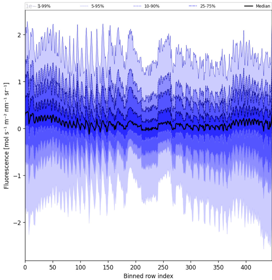
Figure 57: Along track statistics of “Fluorescence” for 2025-07-29 to 2025-07-30
