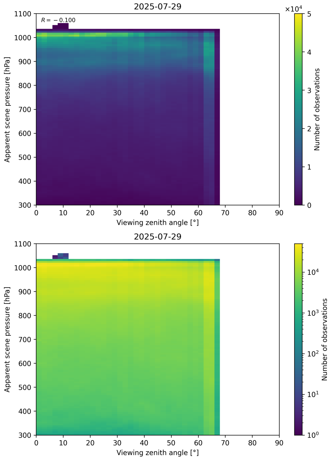
Figure 118: Scatter density plot of “Viewing zenith angle” against “Apparent scene pressure” for 2025-07-29 to 2025-07-30.
