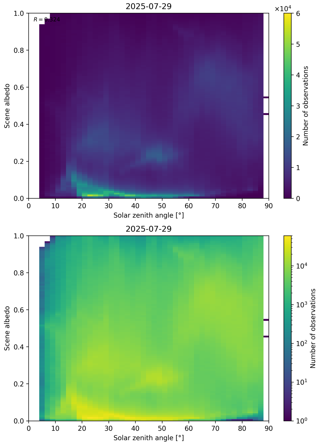
Figure 116: Scatter density plot of “Solar zenith angle” against “Scene albedo” for 2025-07-29 to 2025-07-30.
