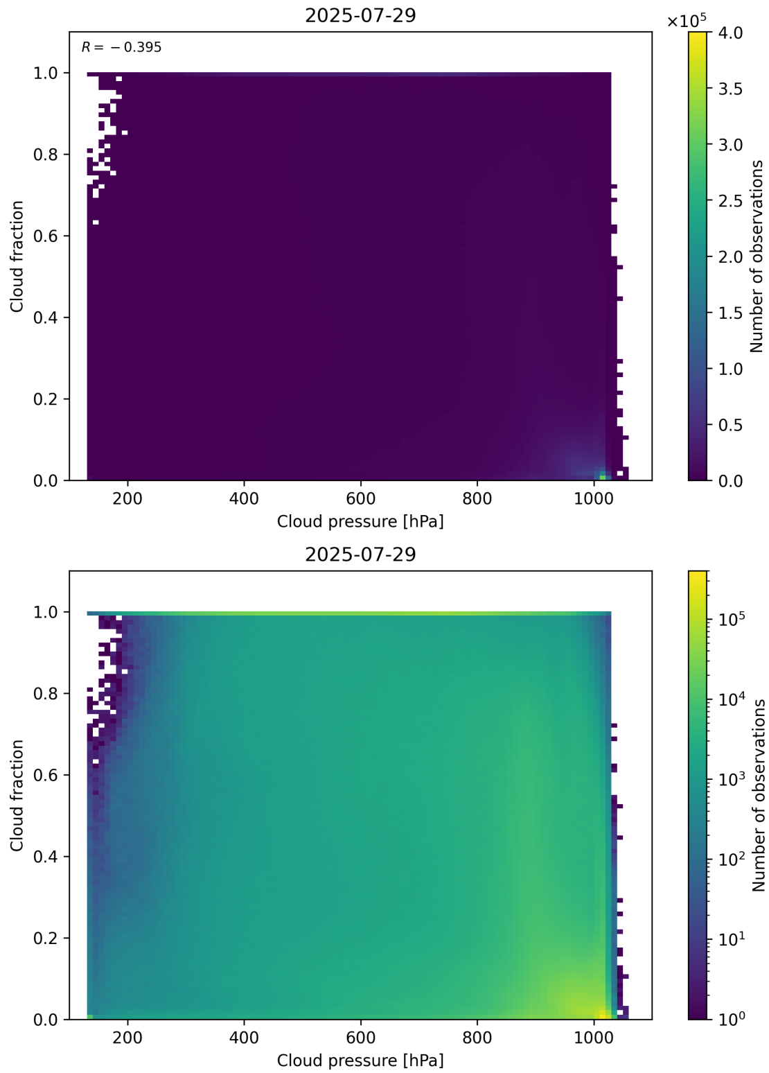
Figure 79: Scatter density plot of “Cloud pressure” against “Cloud fraction” for 2025-07-29 to 2025-07-30.
