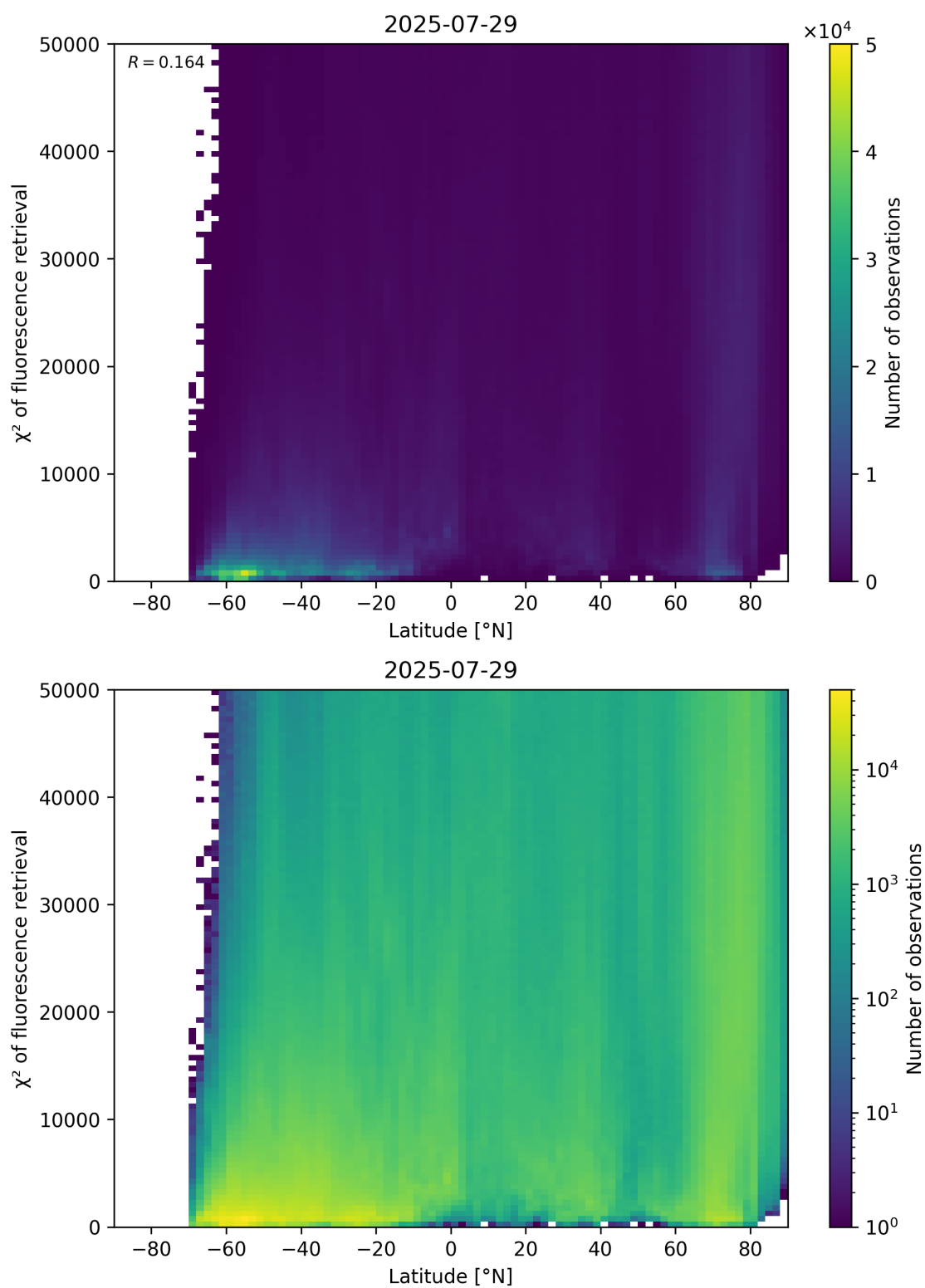
Figure 89: Scatter density plot of “Latitude” against “ \chi^2 of fluorescence retrieval” for 2025-07-29 to 2025-07-30.
