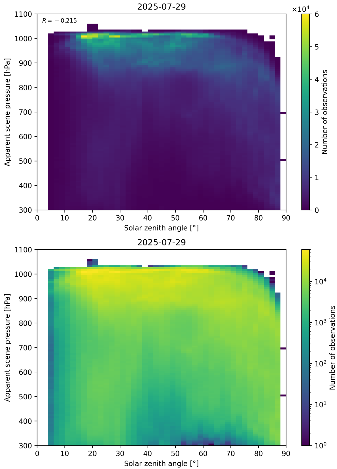
Figure 108: Scatter density plot of “Solar zenith angle” against “Apparent scene pressure” for 2025-07-29 to 2025-07-30.
