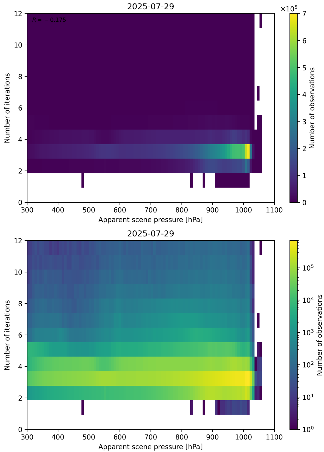
Figure 65: Scatter density plot of “Apparent scene pressure” against “Number of iterations” for 2025-07-29 to 2025-07-30.
