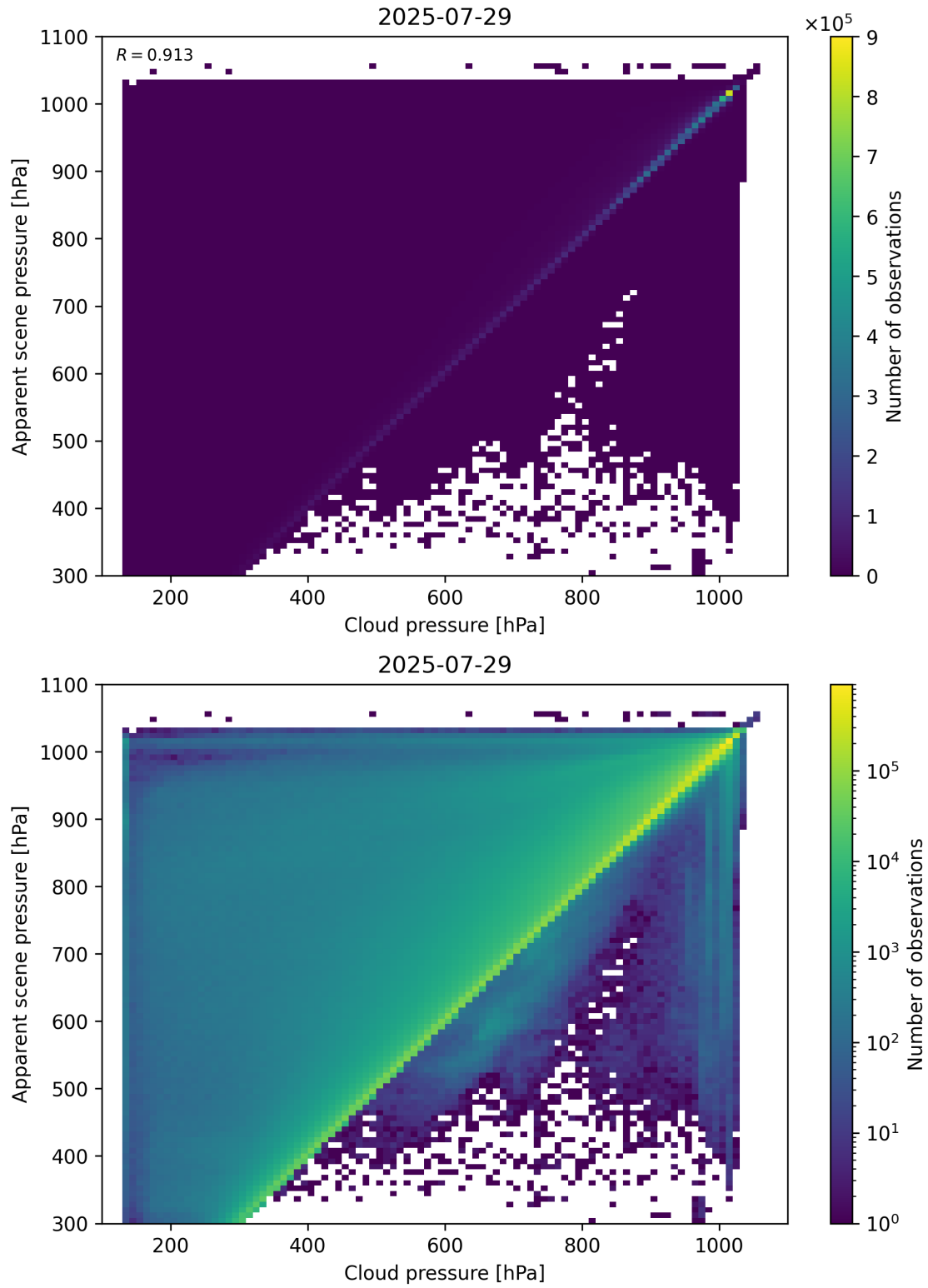
Figure 77: Scatter density plot of “Cloud pressure” against “Apparent scene pressure” for 2025-07-29 to 2025-07-30.
