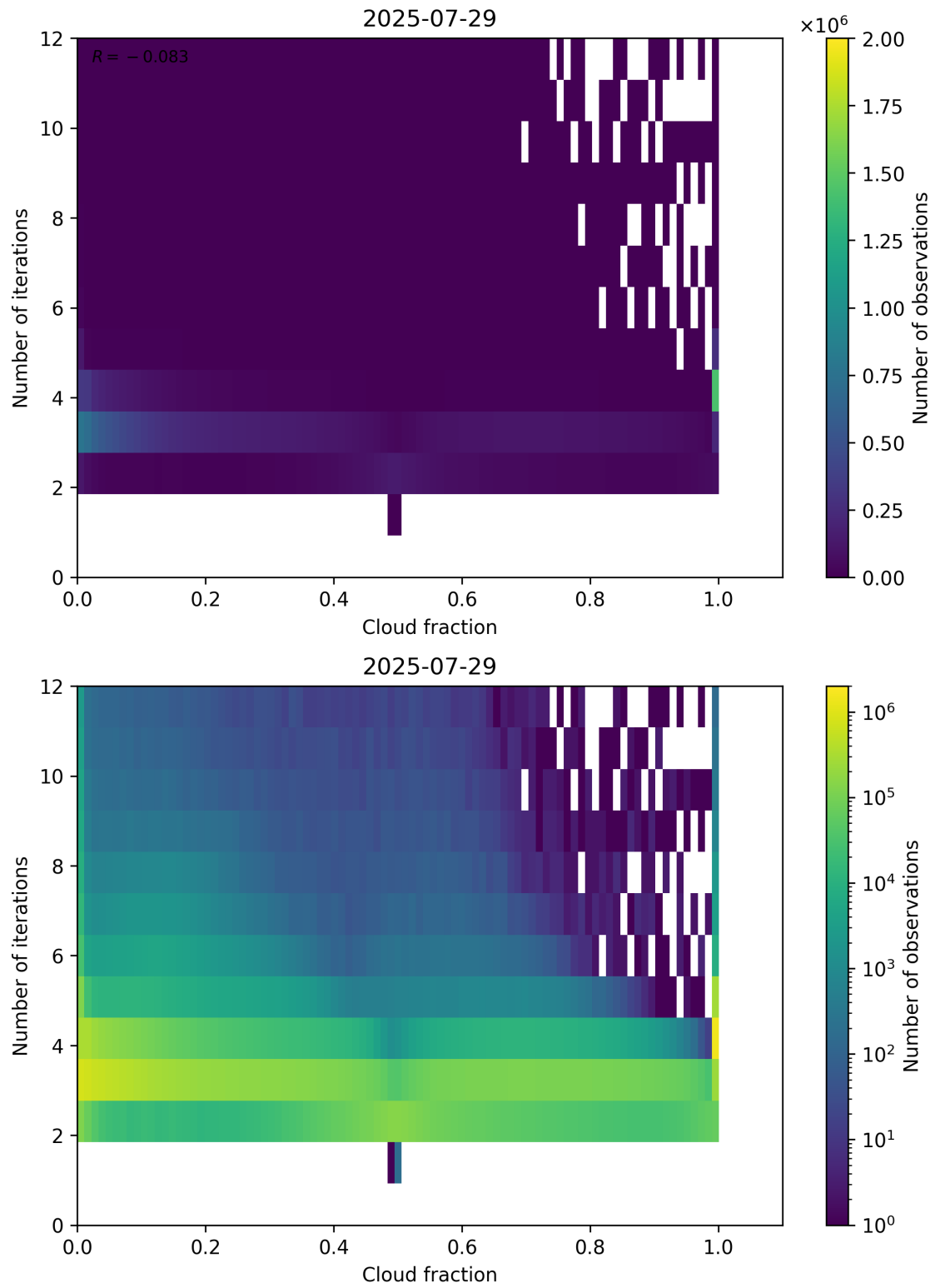
Figure 73: Scatter density plot of “Cloud fraction” against “Number of iterations” for 2025-07-29 to 2025-07-30.
