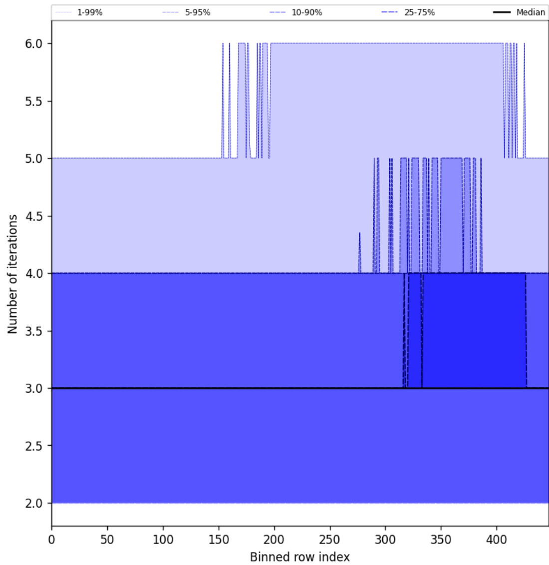
Figure 56: Along track statistics of “Number of iterations” for 2025-07-29 to 2025-07-30
