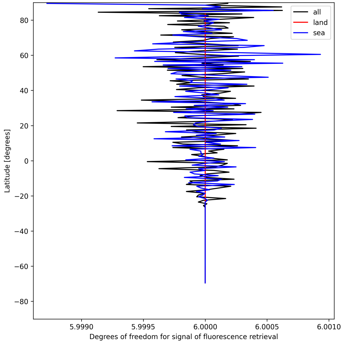
Figure 26: Zonal average of “Degrees of freedom for signal of fluorescence retrieval” for 2025-07-29 to 2025-07-30.
