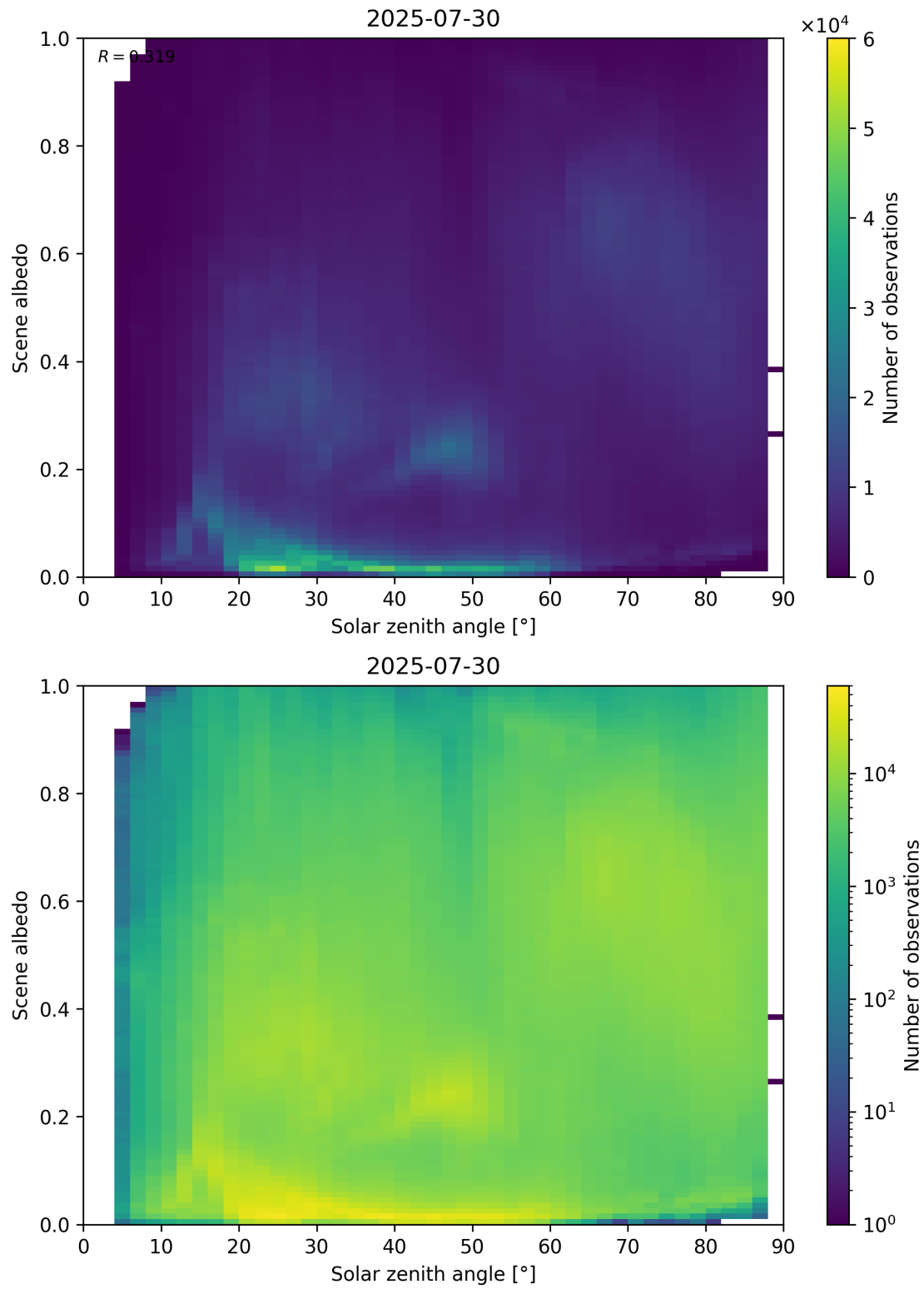
Figure 116: Scatter density plot of “Solar zenith angle” against “Scene albedo” for 2025-07-29 to 2025-07-31.
