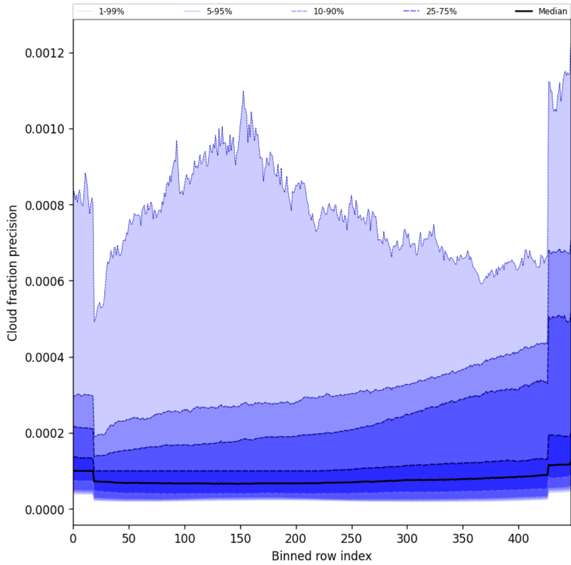
Figure 50: Along track statistics of “Cloud fraction precision” for 2025-07-29 to 2025-07-31
