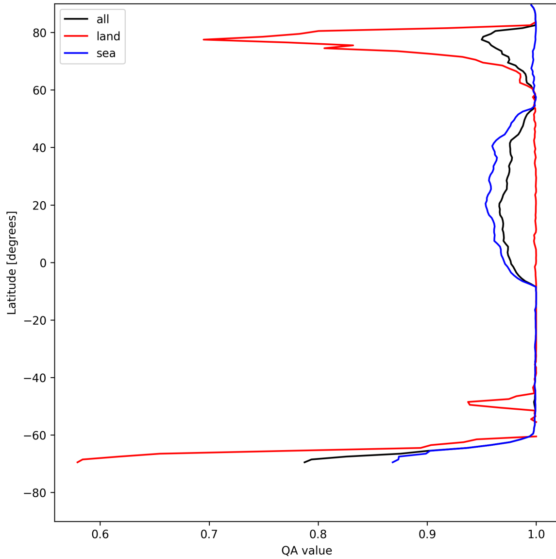
Figure 12: Zonal average of "QA value" for 2025-07-29 to 2025-07-31.
