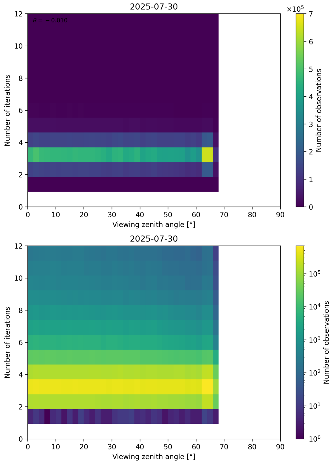
Figure 124: Scatter density plot of “Viewing zenith angle” against “Number of iterations” for 2025-07-29 to 2025-07-31.
