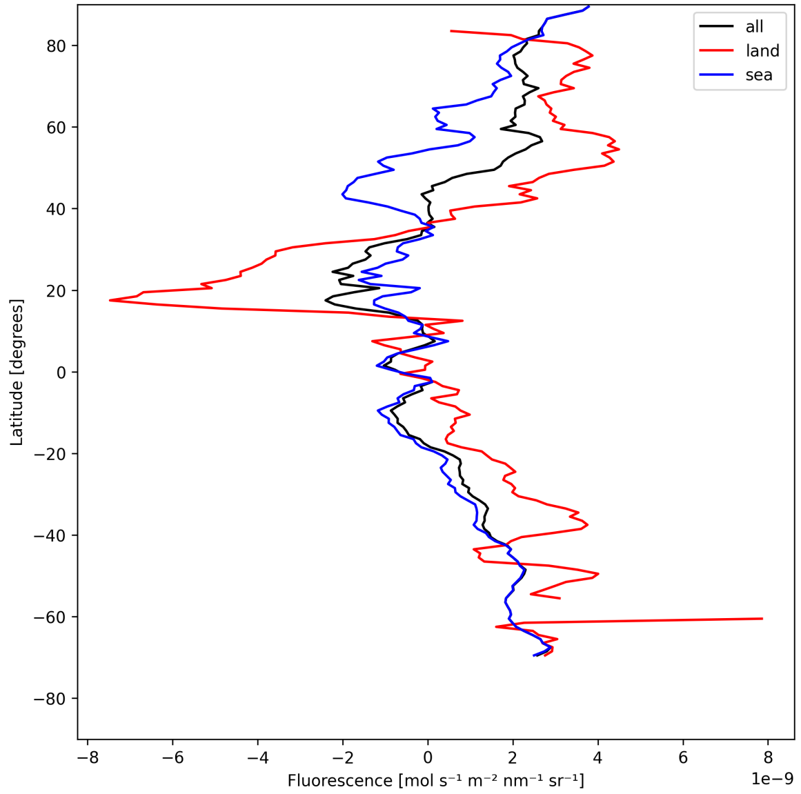
Figure 23: Zonal average of “Fluorescence” for 2025-07-29 to 2025-07-31.
