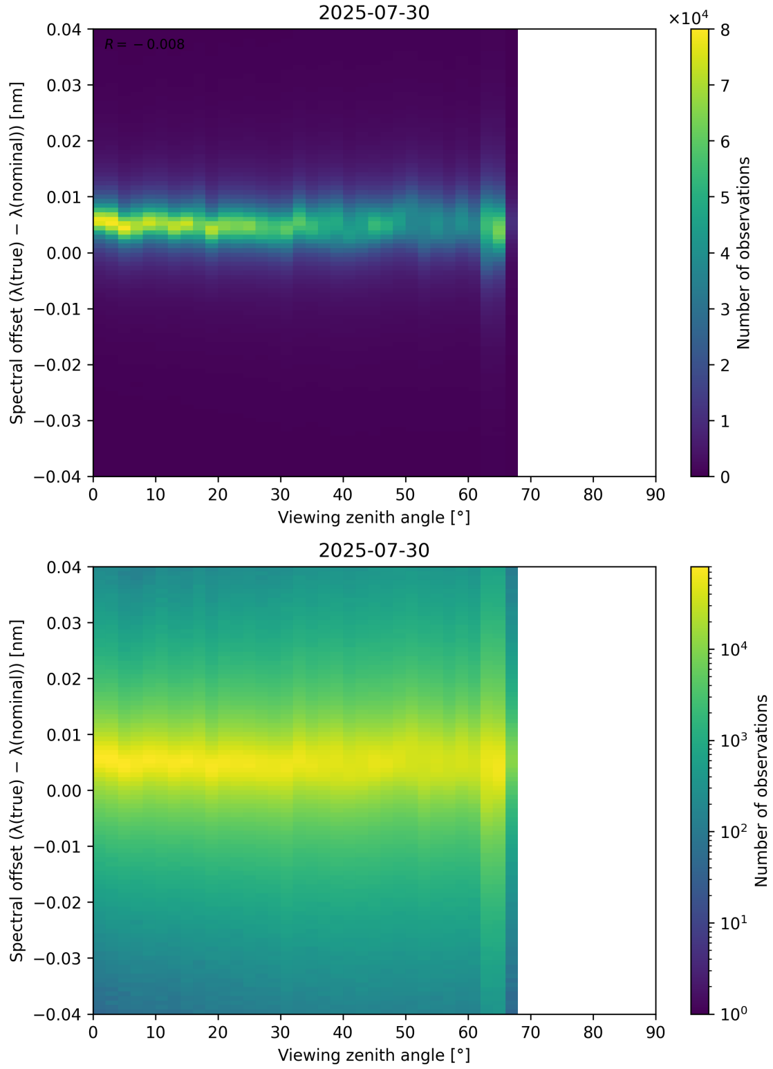
Figure 128: Scatter density plot of “Viewing zenith angle” against “Spectral offset ( \lambda_{\text{true}} - \lambda_{\text{nominal}} )” for 2025-07-29 to 2025-07-31.
