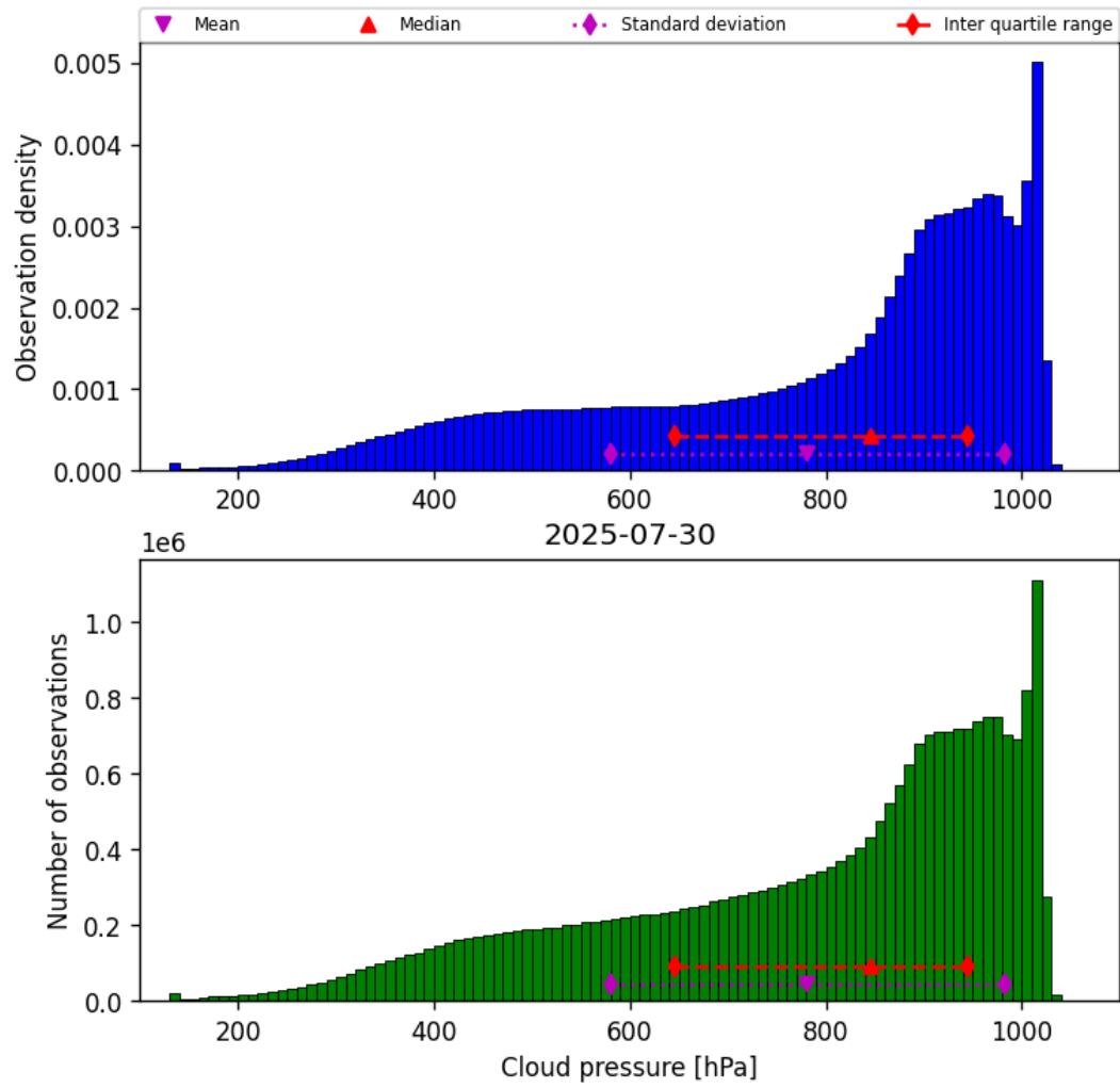
Figure 30: Histogram of “Cloud pressure” for 2025-07-29 to 2025-07-31
