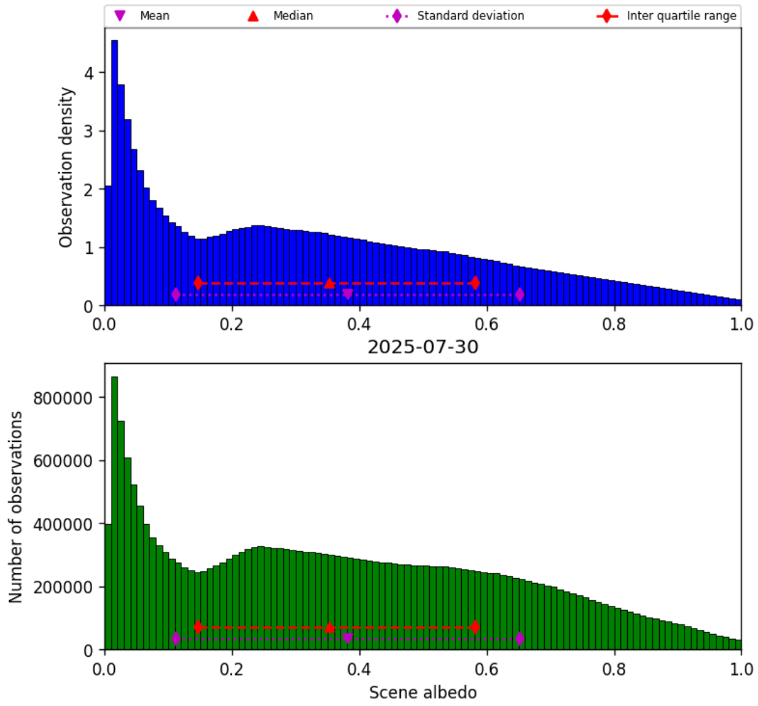
Figure 34: Histogram of “Scene albedo” for 2025-07-29 to 2025-07-31
