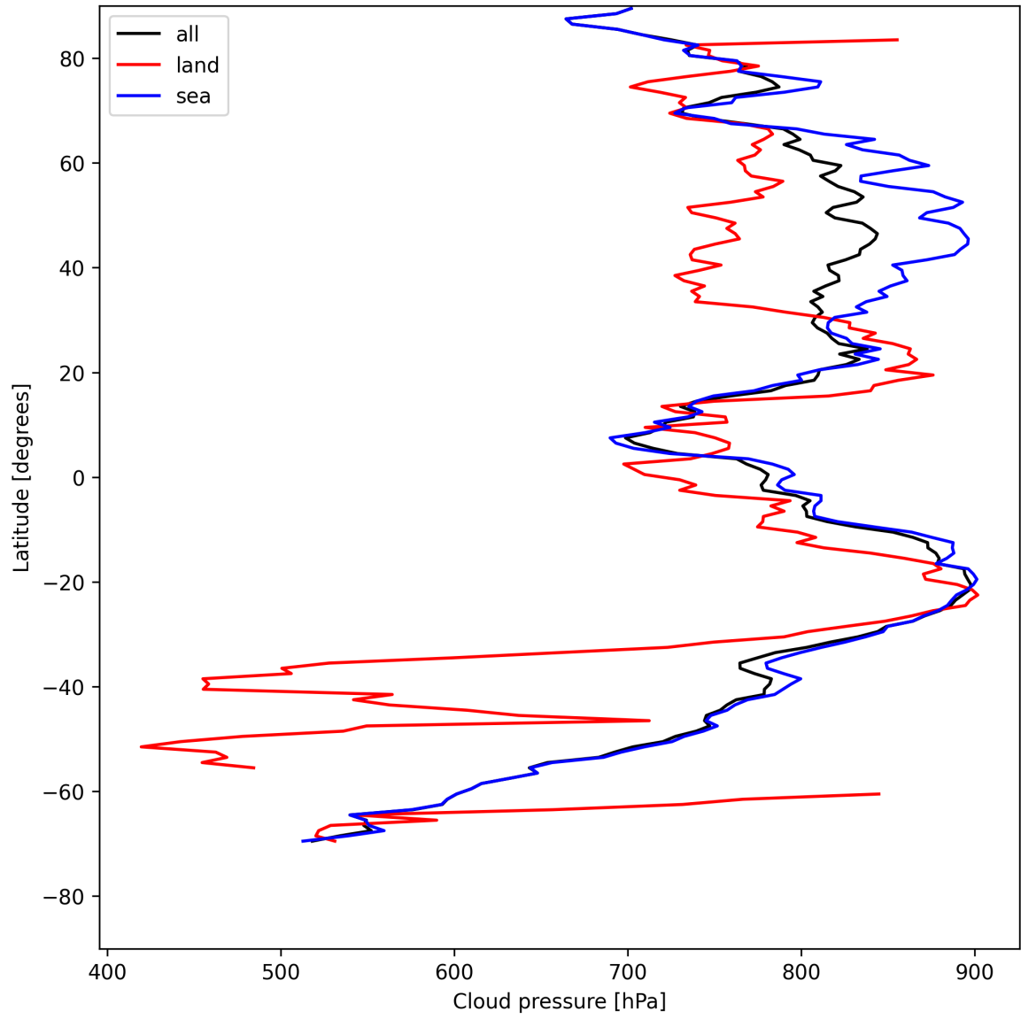
Figure 13: Zonal average of “Cloud pressure” for 2025-07-29 to 2025-07-31.
