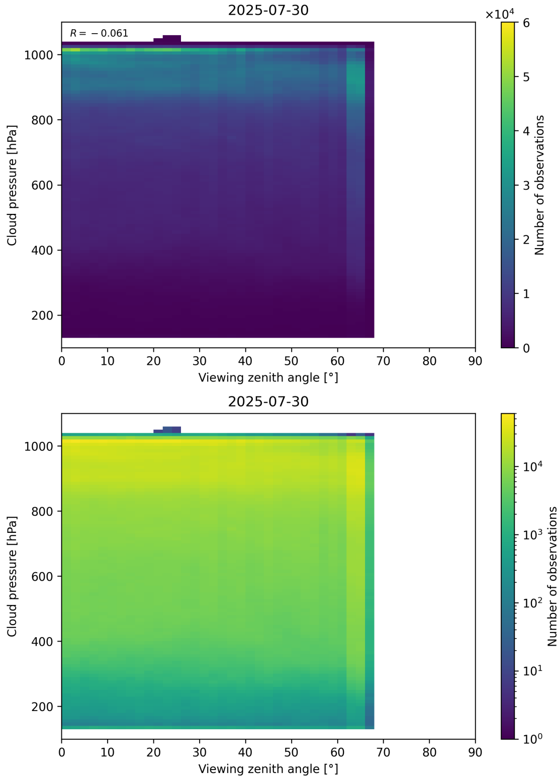
Figure 121: Scatter density plot of “Viewing zenith angle” against “Cloud pressure” for 2025-07-29 to 2025-07-31.
