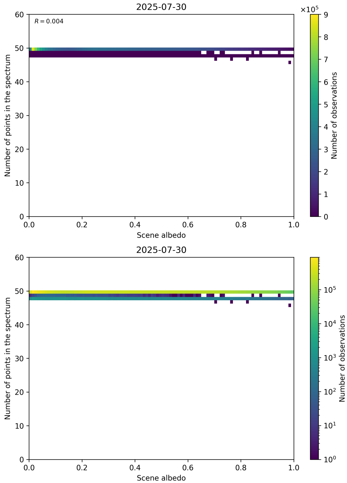
Figure 106: Scatter density plot of “Scene albedo” against “Number of points in the spectrum” for 2025-07-29 to 2025-07-31.
