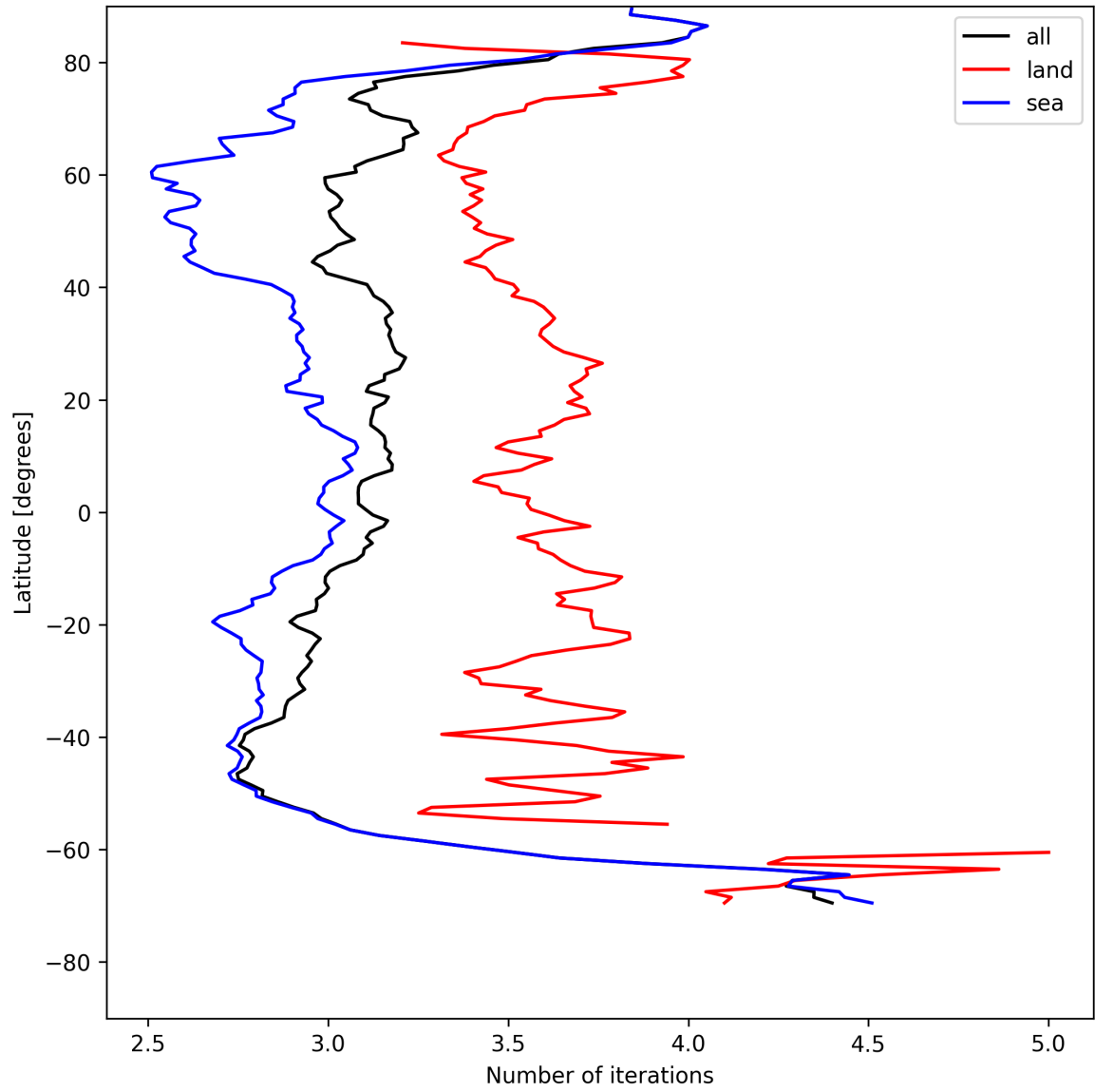
Figure 22: Zonal average of “Number of iterations” for 2025-07-29 to 2025-07-31.
