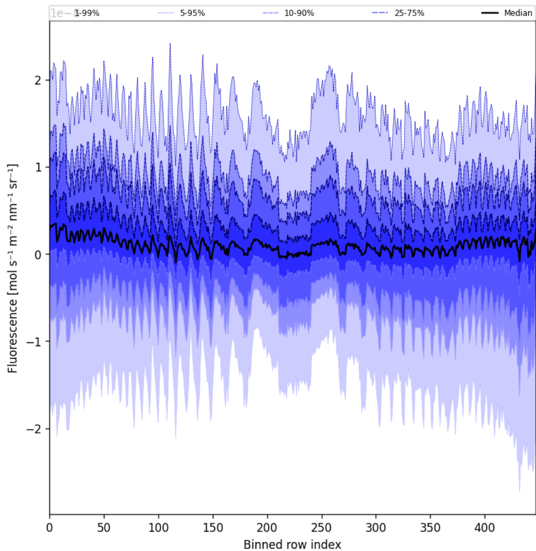
Figure 57: Along track statistics of "Fluorescence" for 2025-07-29 to 2025-07-31
