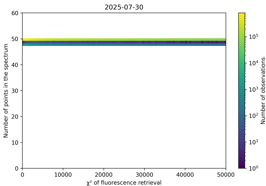
Figure 68: Scatter density plot of “ \chi^2 of fluorescence retrieval” against “Number of points in the spectrum” for 2025-07-29 to 2025-07-31.
