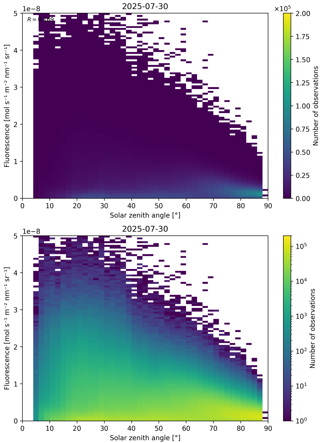
Figure 112: Scatter density plot of “Solar zenith angle” against “Fluorescence” for 2025-07-29 to 2025-07-31.
