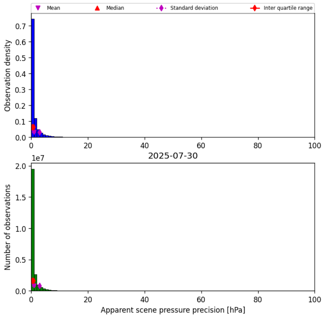
Figure 37: Histogram of “Apparent scene pressure precision” for 2025-07-29 to 2025-07-31
