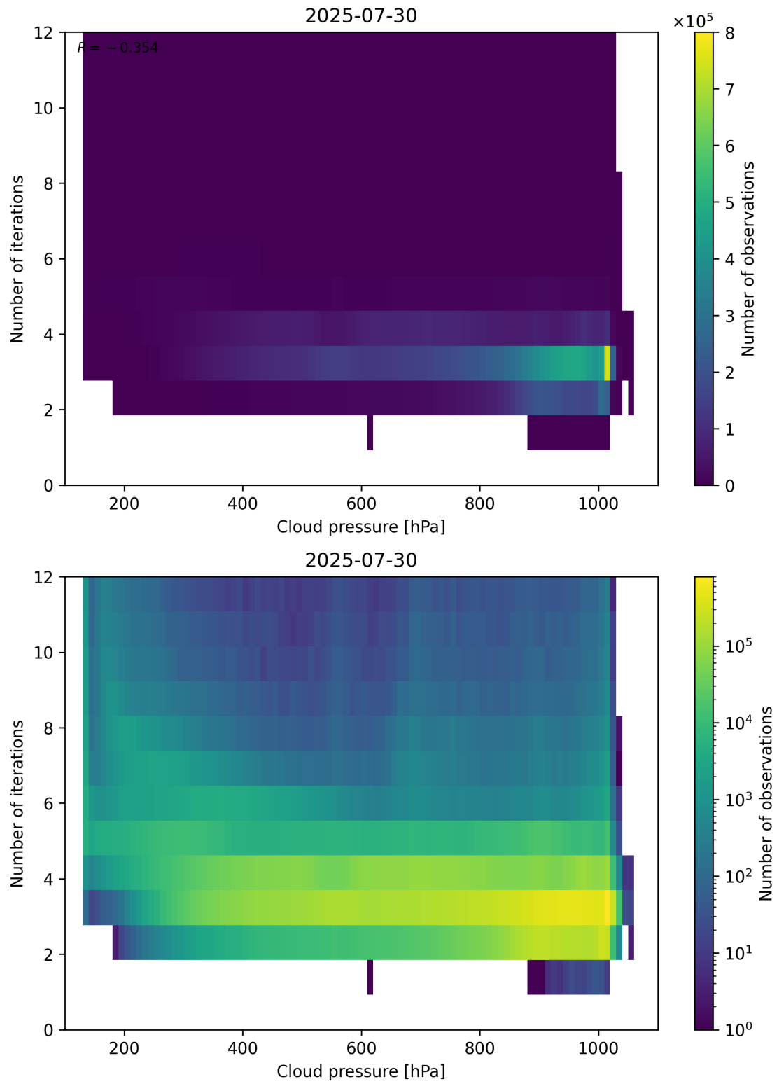
Figure 81: Scatter density plot of “Cloud pressure” against “Number of iterations” for 2025-07-29 to 2025-07-31.
