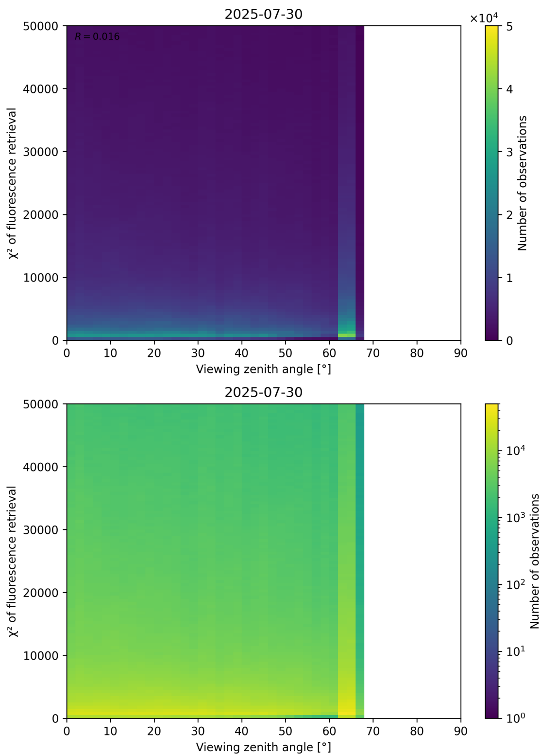
Figure 119: Scatter density plot of “Viewing zenith angle” against “ \chi^2 of fluorescence retrieval” for 2025-07-29 to 2025-07-31.
