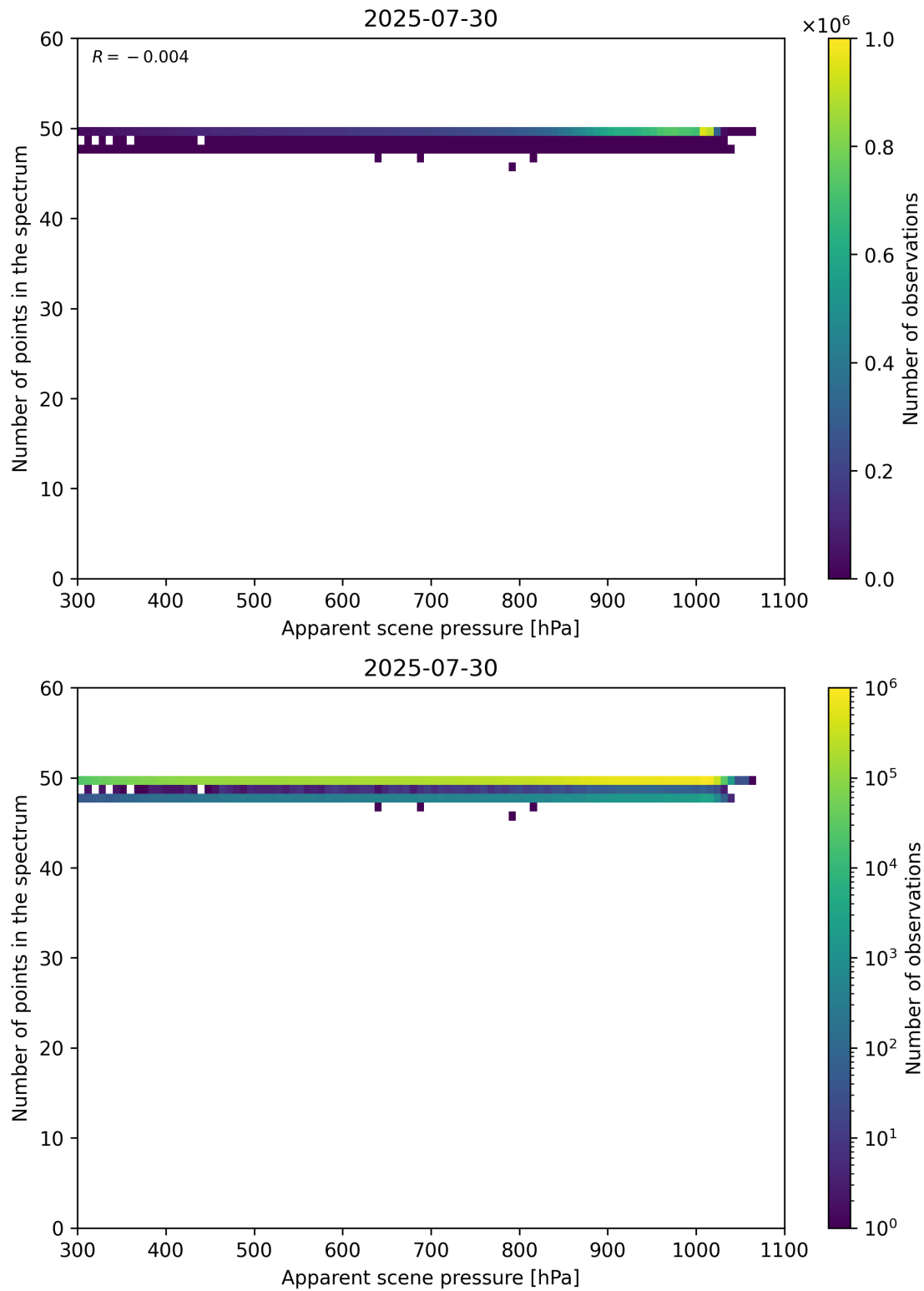
Figure 66: Scatter density plot of “Apparent scene pressure” against “Number of points in the spectrum” for 2025-07-29 to 2025-07-31.
