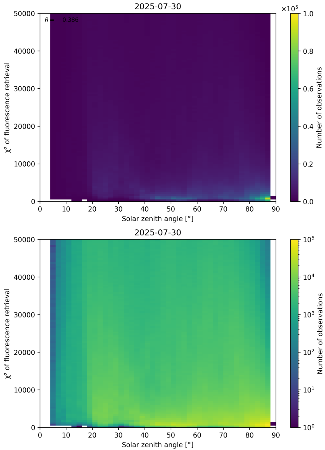
Figure 109: Scatter density plot of “Solar zenith angle” against “ \chi^2 of fluorescence retrieval” for 2025-07-29 to 2025-07-31.
