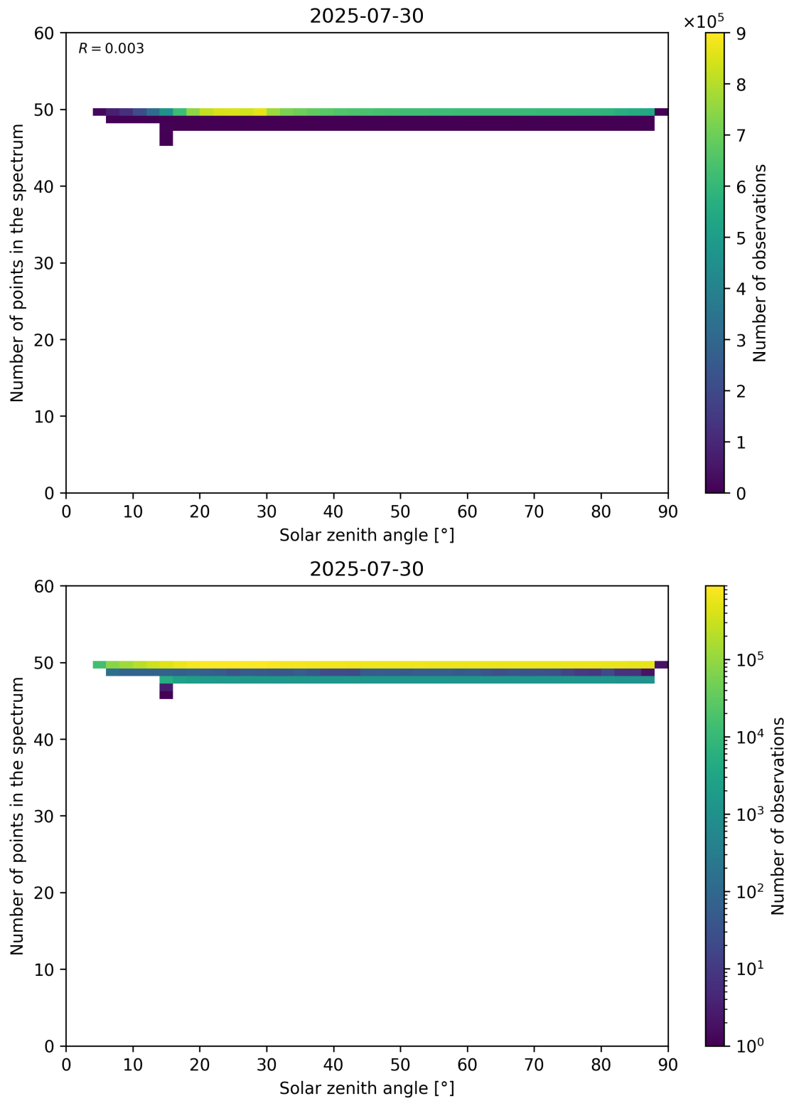
Figure 115: Scatter density plot of “Solar zenith angle” against “Number of points in the spectrum” for 2025-07-29 to 2025-07-31.
