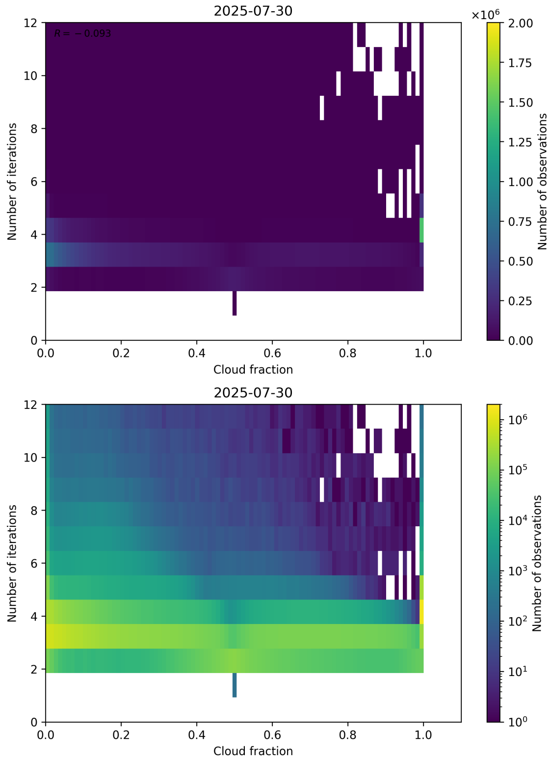
Figure 73: Scatter density plot of “Cloud fraction” against “Number of iterations” for 2025-07-29 to 2025-07-31.
