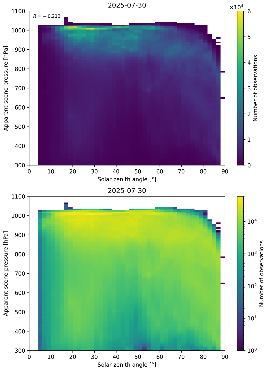
Figure 108: Scatter density plot of “Solar zenith angle” against “Apparent scene pressure” for 2025-07-29 to 2025-07-31.
