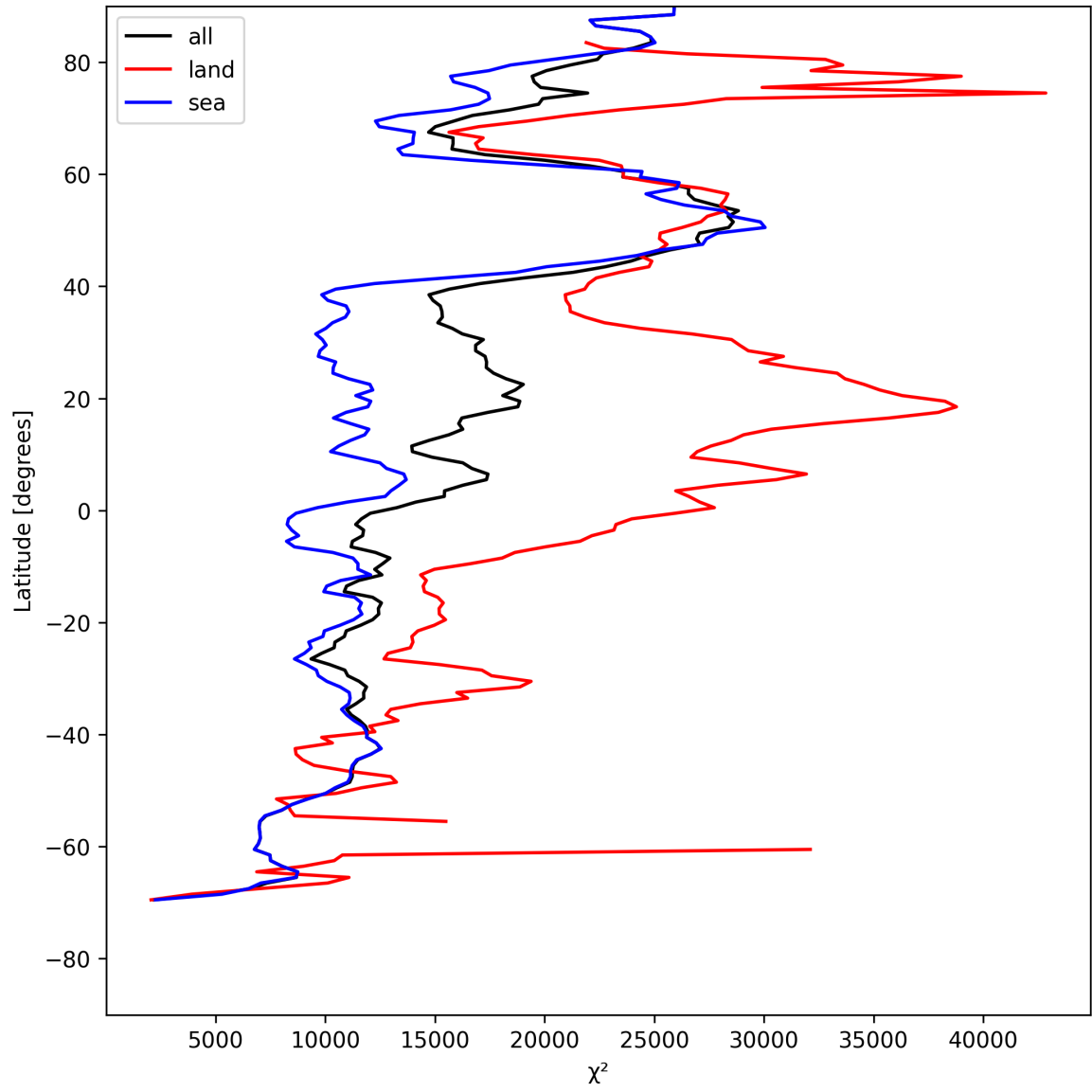
Figure 21: Zonal average of “ \chi^2 ” for 2025-07-29 to 2025-07-31.
