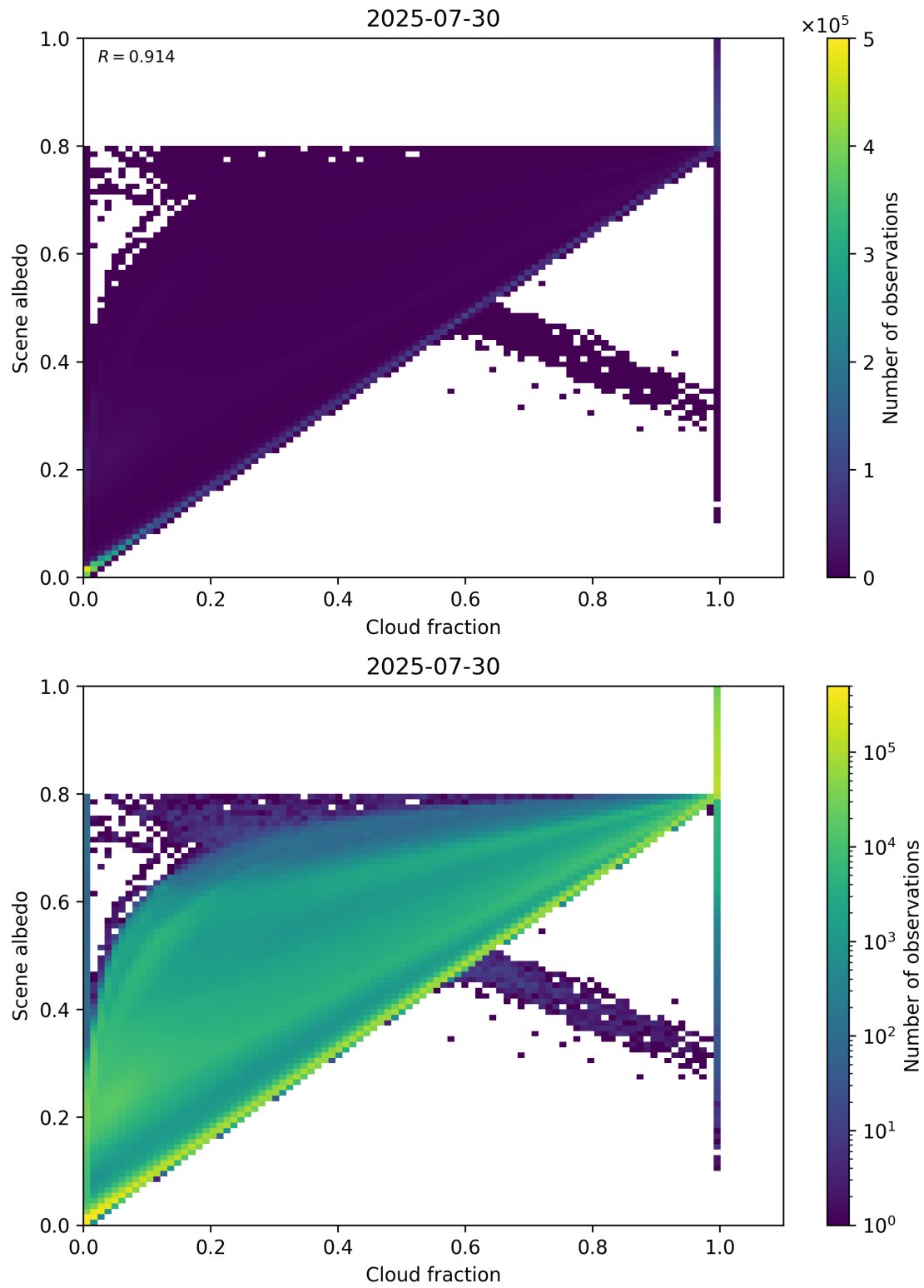
Figure 75: Scatter density plot of “Cloud fraction” against “Scene albedo” for 2025-07-29 to 2025-07-31.
