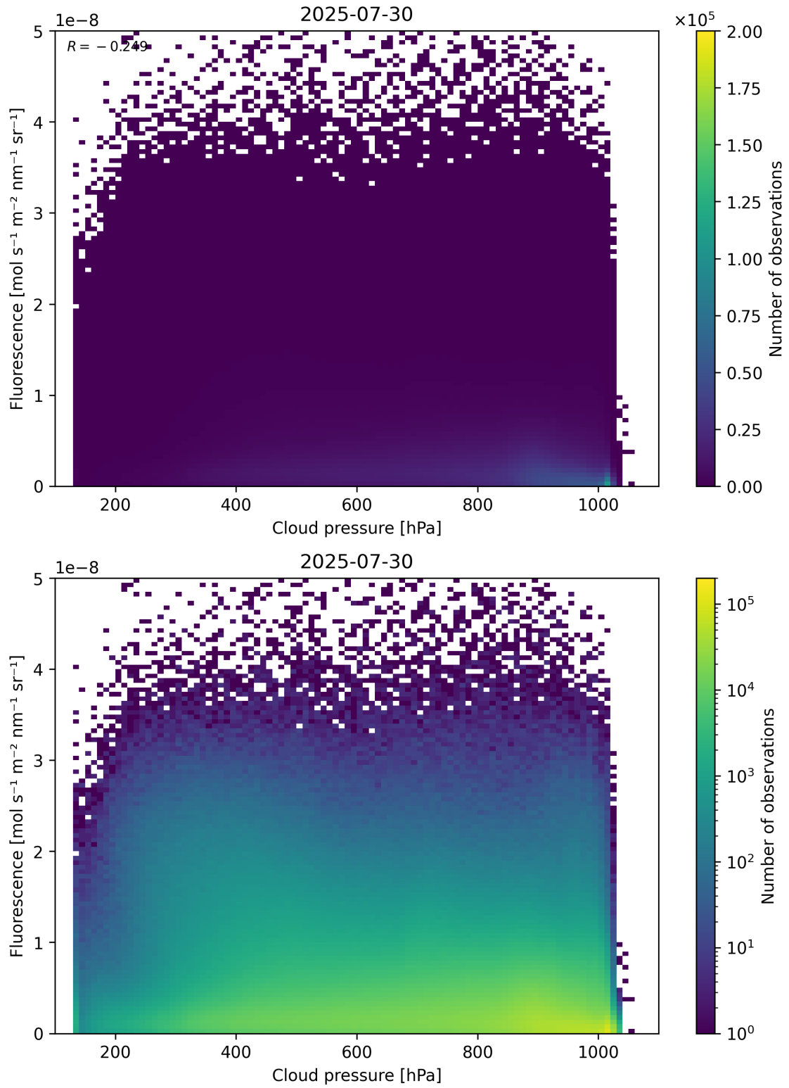
Figure 80: Scatter density plot of “Cloud pressure” against “Fluorescence” for 2025-07-29 to 2025-07-31.
