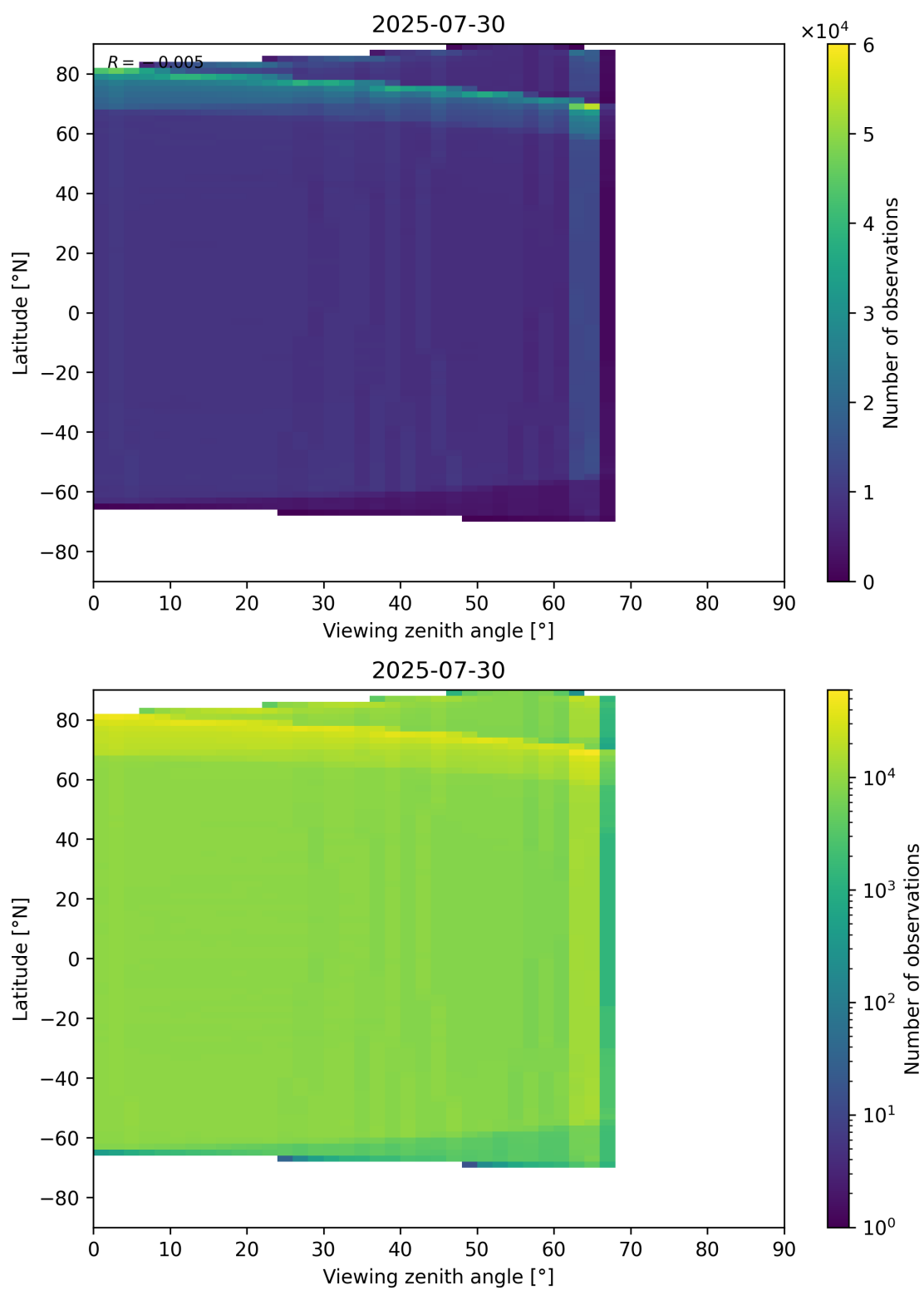
Figure 123: Scatter density plot of “Viewing zenith angle” against “Latitude” for 2025-07-29 to 2025-07-31.
