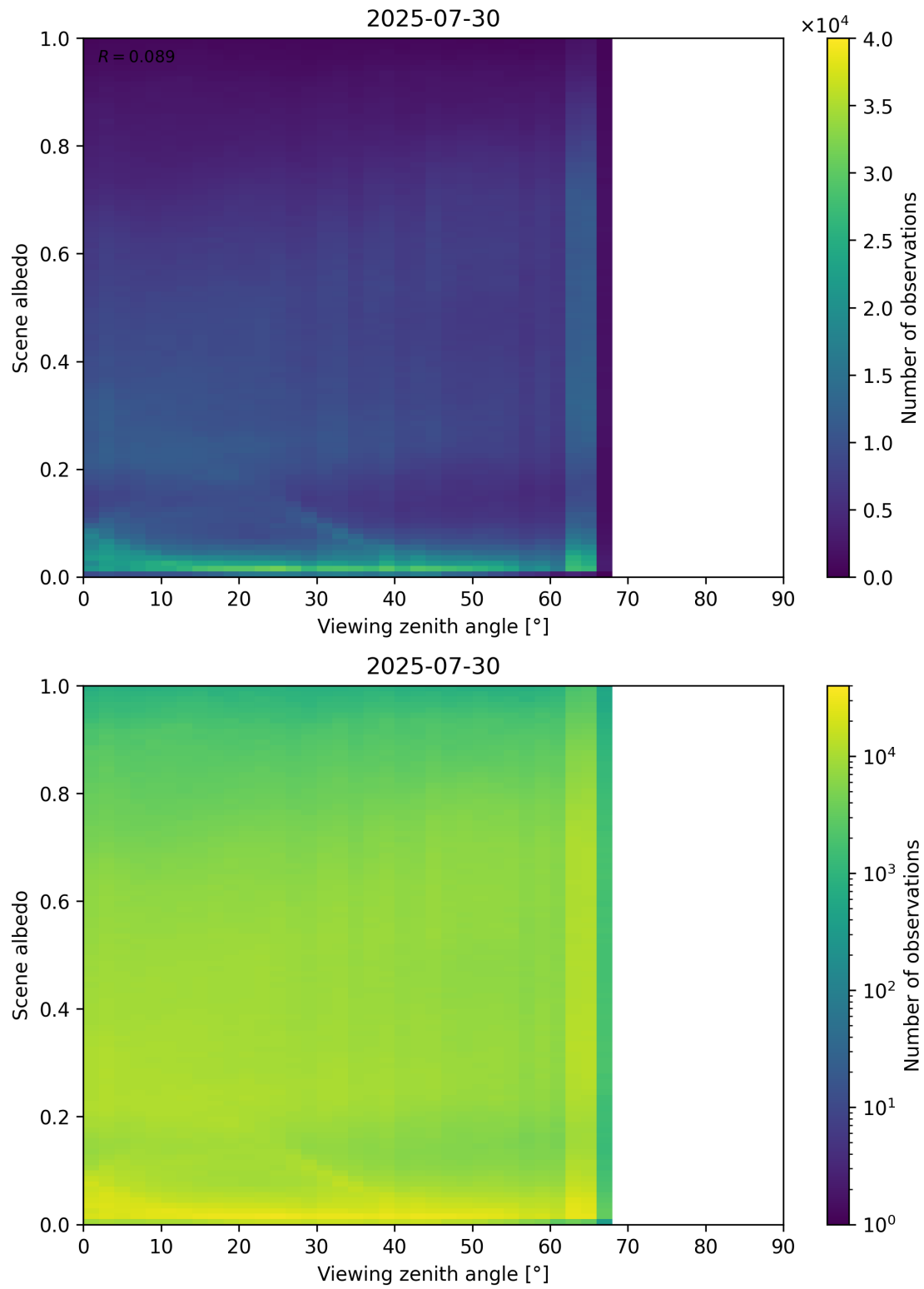
Figure 126: Scatter density plot of “Viewing zenith angle” against “Scene albedo” for 2025-07-29 to 2025-07-31.
