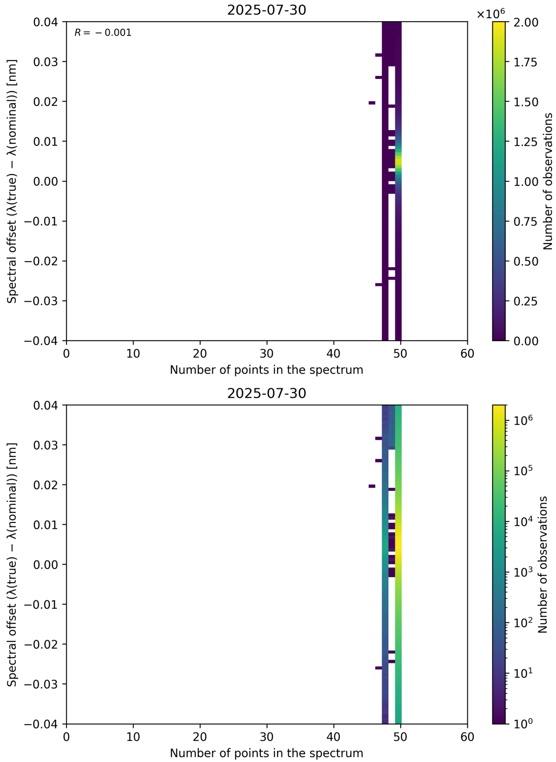
Figure 101: Scatter density plot of “Number of points in the spectrum” against “Spectral offset ( \lambda_{\text{true}} - \lambda_{\text{nominal}} )” for 2025-07-29 to 2025-07-31.
