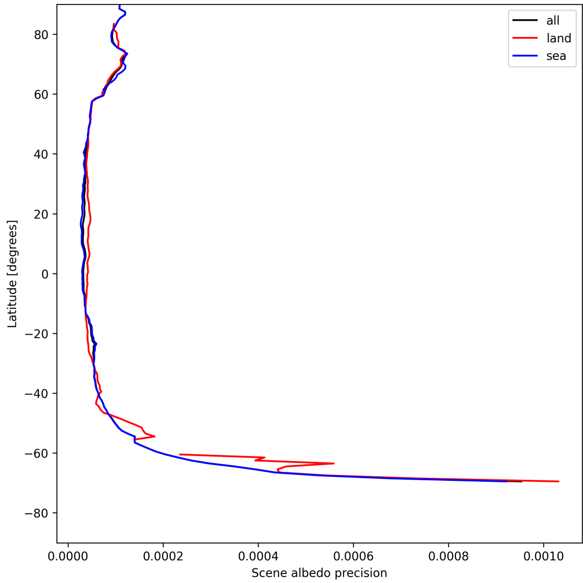
Figure 18: Zonal average of “Scene albedo precision” for 2025-07-29 to 2025-07-31.
