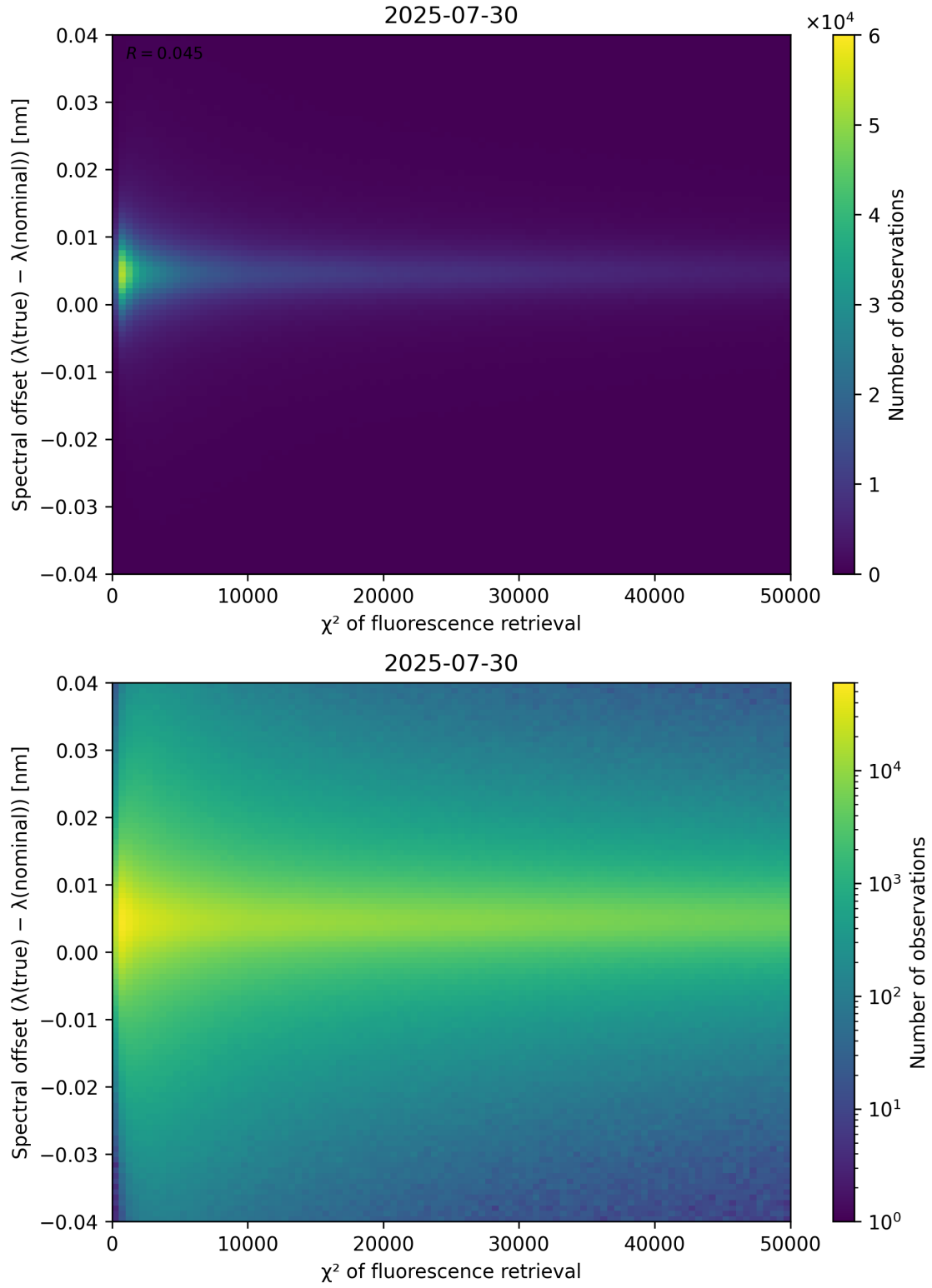
Figure 69: Scatter density plot of “ \chi^2 of fluorescence retrieval” against “Spectral offset ( \lambda_{\text{true}} - \lambda_{\text{nominal}} )” for 2025-07-29 to 2025-07-31.
