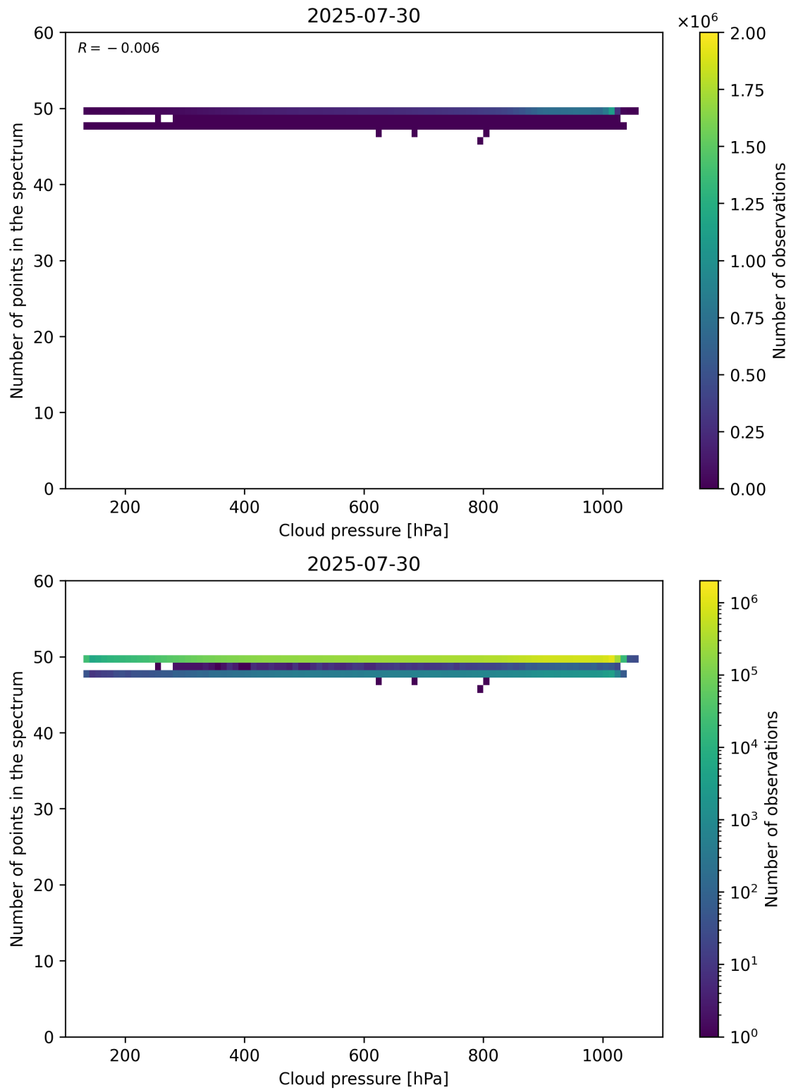
Figure 82: Scatter density plot of “Cloud pressure” against “Number of points in the spectrum” for 2025-07-29 to 2025-07-31.
