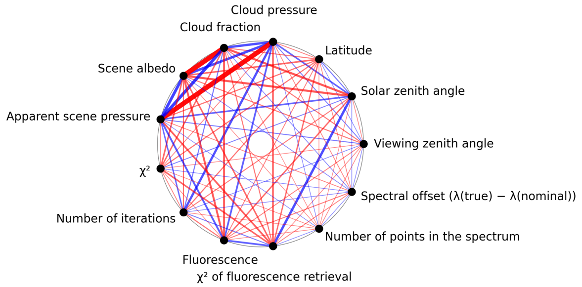
Figure 1: Map of correlation graph for 2025-07-29 to 2025-07-31.
