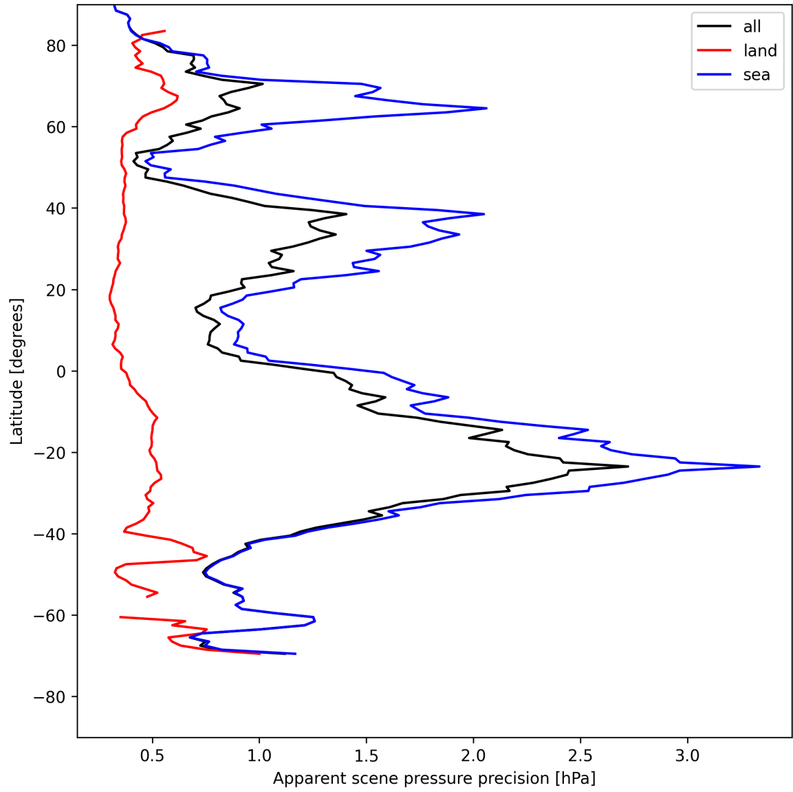
Figure 20: Zonal average of “Apparent scene pressure precision” for 2025-07-29 to 2025-07-31.
