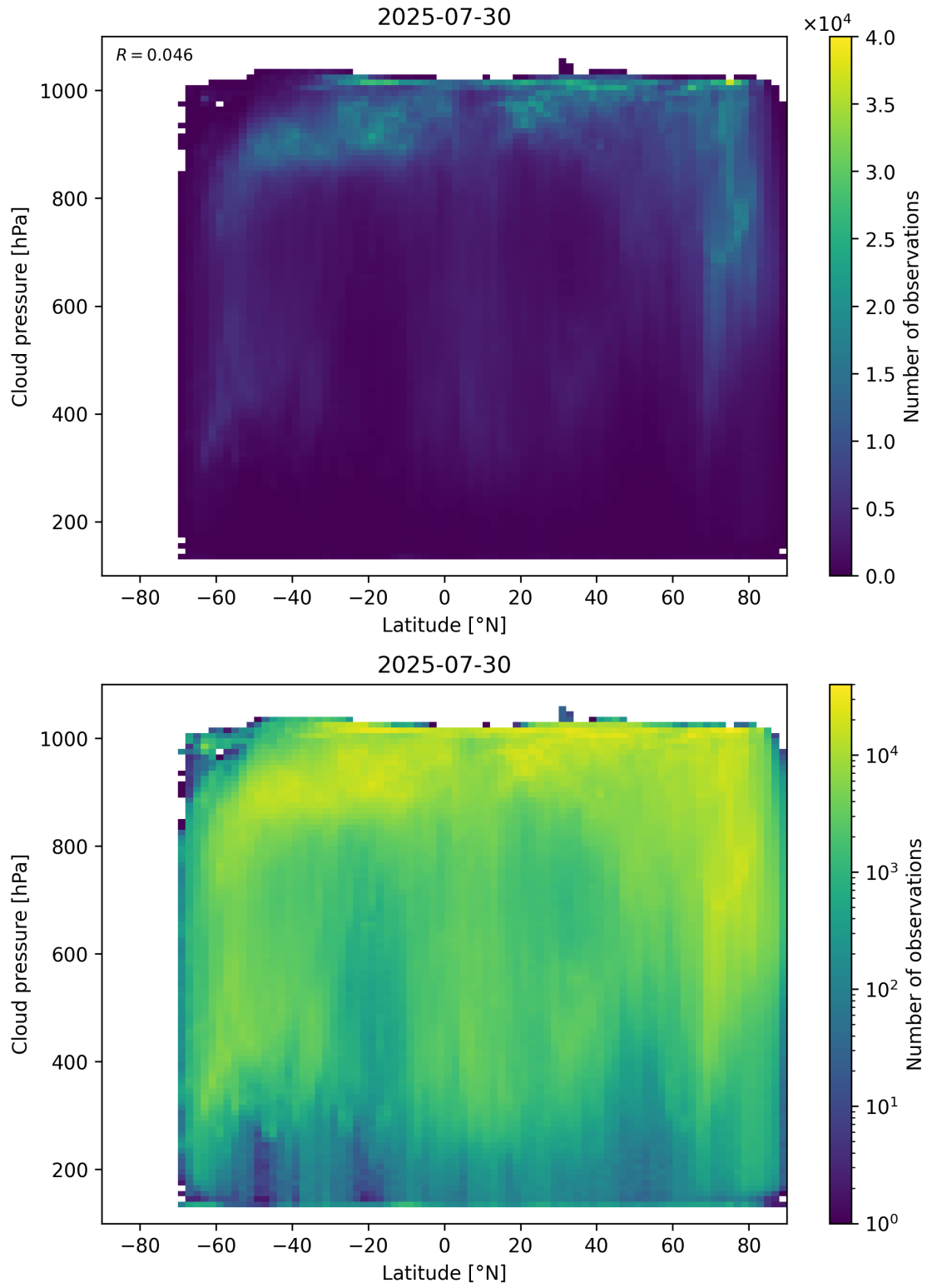
Figure 91: Scatter density plot of “Latitude” against “Cloud pressure” for 2025-07-29 to 2025-07-31.
