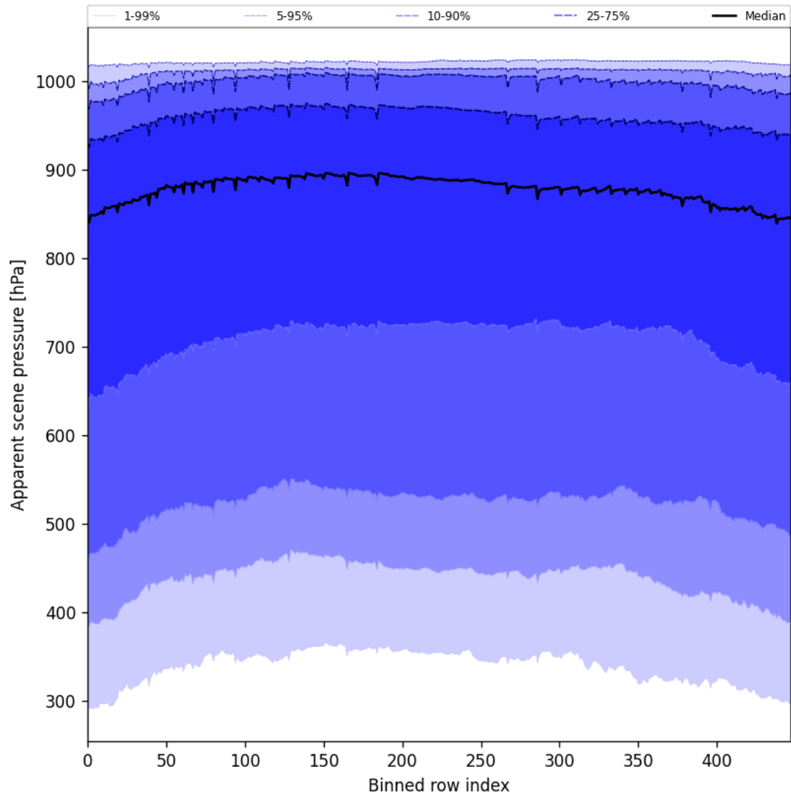
Figure 53: Along track statistics of “Apparent scene pressure” for 2025-07-29 to 2025-07-31
