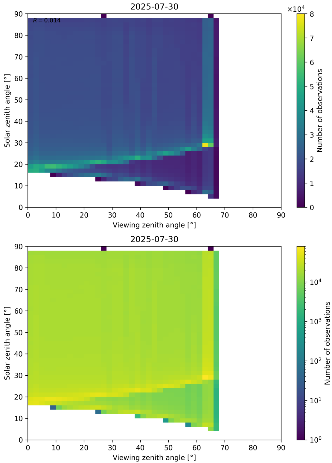
Figure 127: Scatter density plot of “Viewing zenith angle” against “Solar zenith angle” for 2025-07-29 to 2025-07-31.
