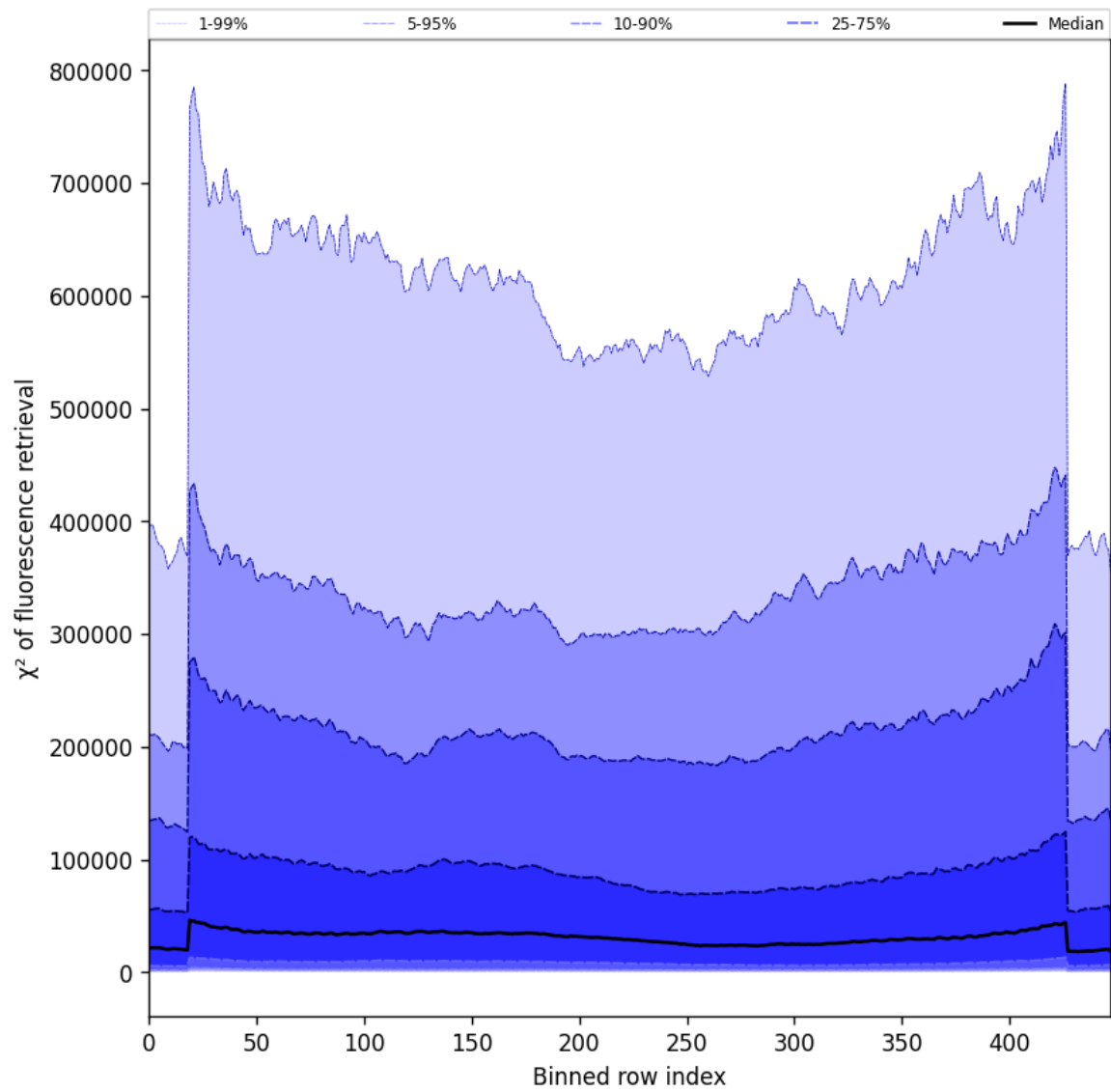
Figure 59: Along track statistics of “ \chi^2 of fluorescence retrieval” for 2025-07-29 to 2025-07-31
