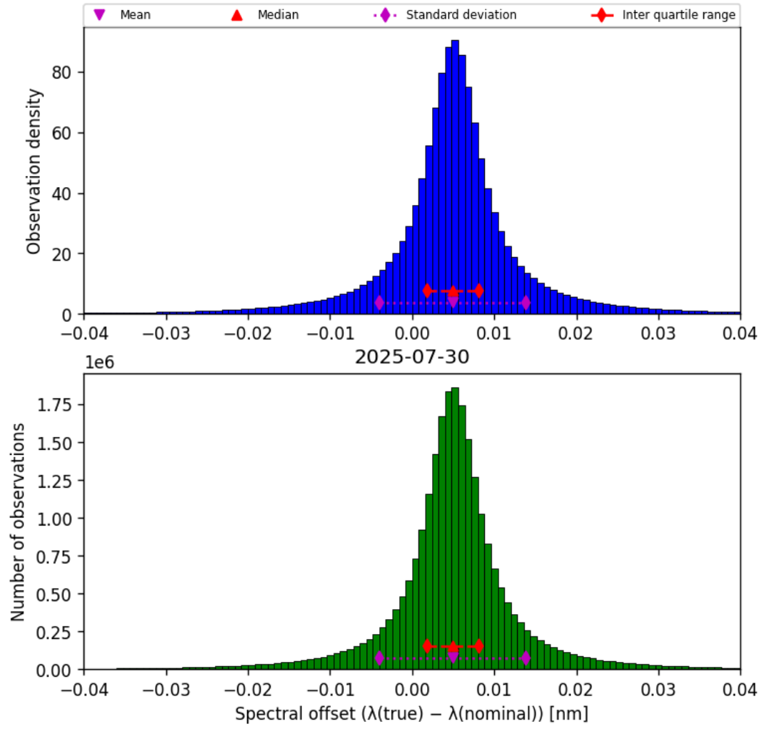
Figure 45: Histogram of “Spectral offset ( \lambda_{\text{true}} - \lambda_{\text{nominal}} )” for 2025-07-29 to 2025-07-31
