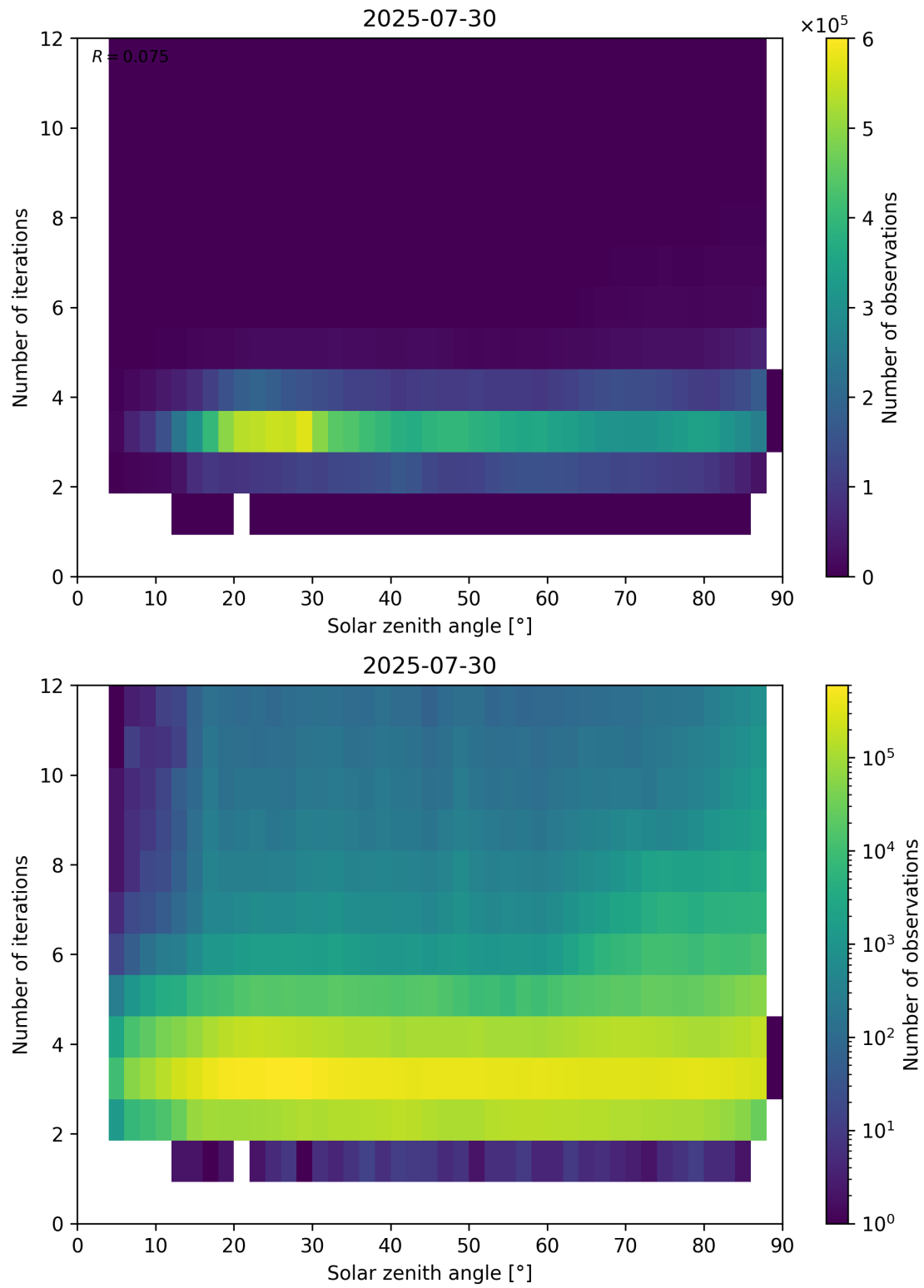
Figure 114: Scatter density plot of “Solar zenith angle” against “Number of iterations” for 2025-07-29 to 2025-07-31.
