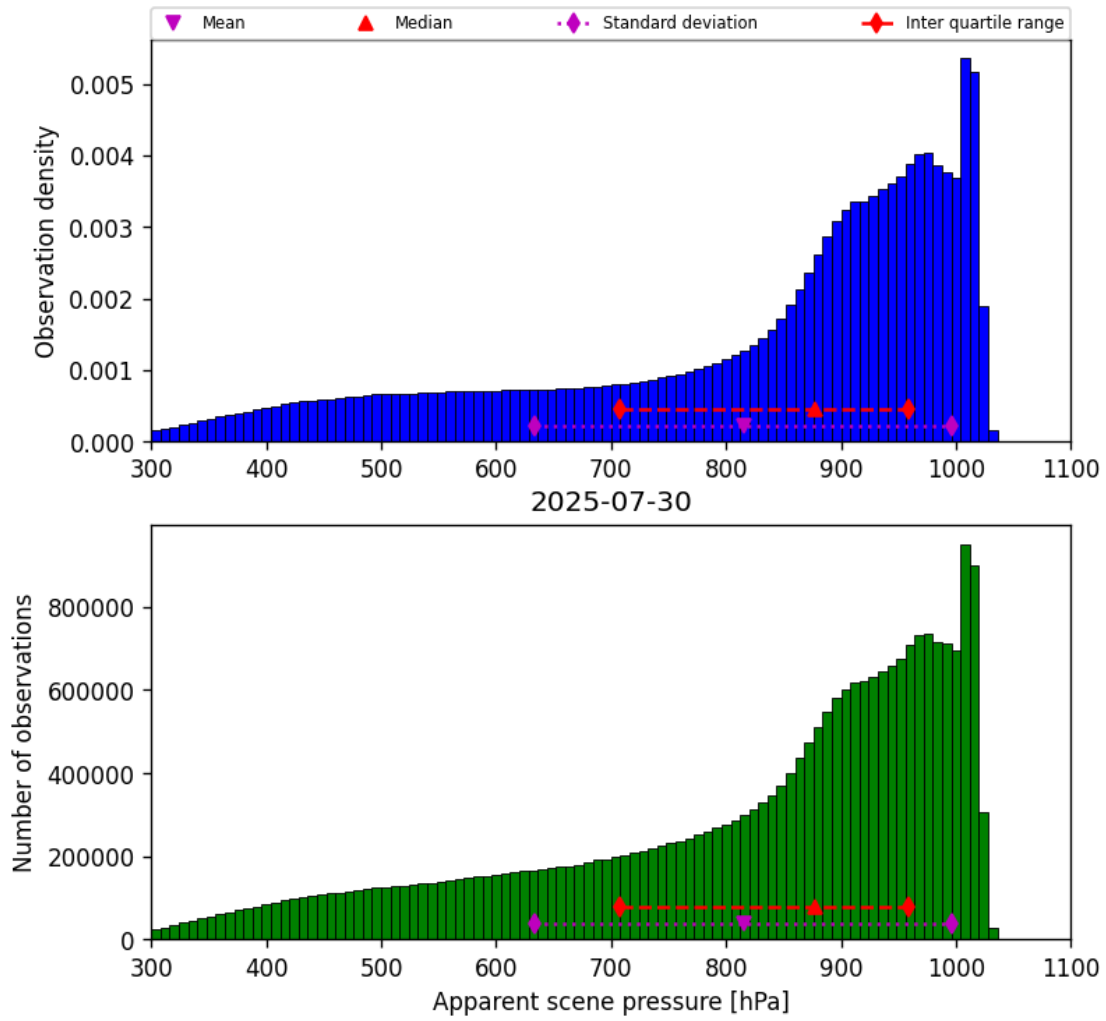
Figure 36: Histogram of “Apparent scene pressure” for 2025-07-29 to 2025-07-31
