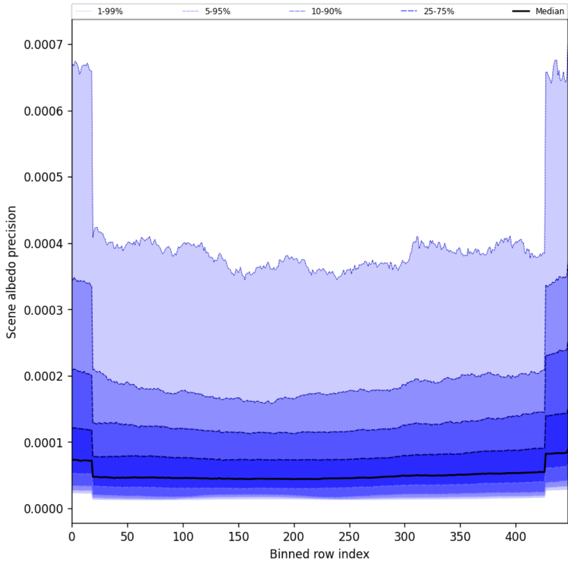
Figure 52: Along track statistics of “Scene albedo precision” for 2025-07-29 to 2025-07-31
