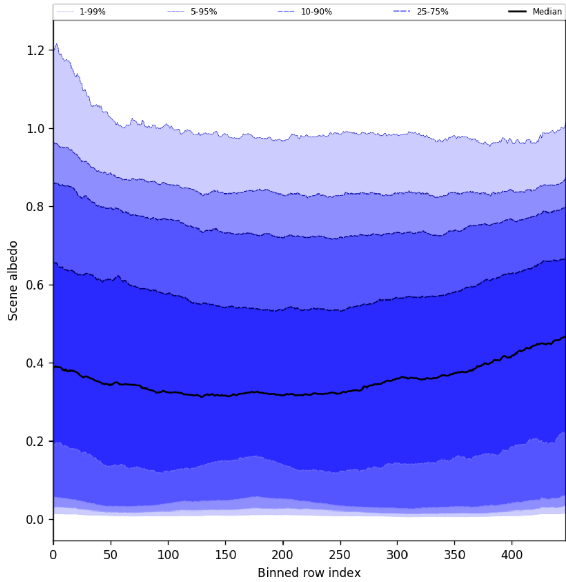
Figure 51: Along track statistics of “Scene albedo” for 2025-07-29 to 2025-07-31
