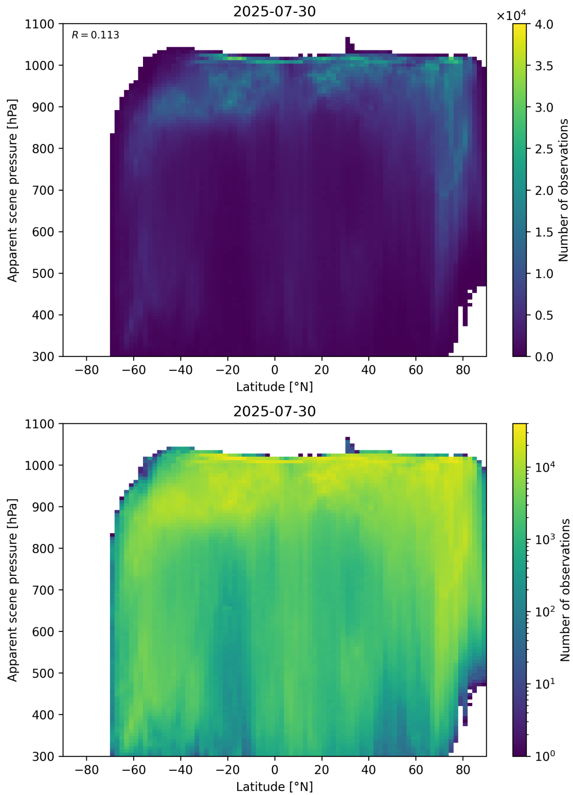
Figure 88: Scatter density plot of “Latitude” against “Apparent scene pressure” for 2025-07-29 to 2025-07-31.
