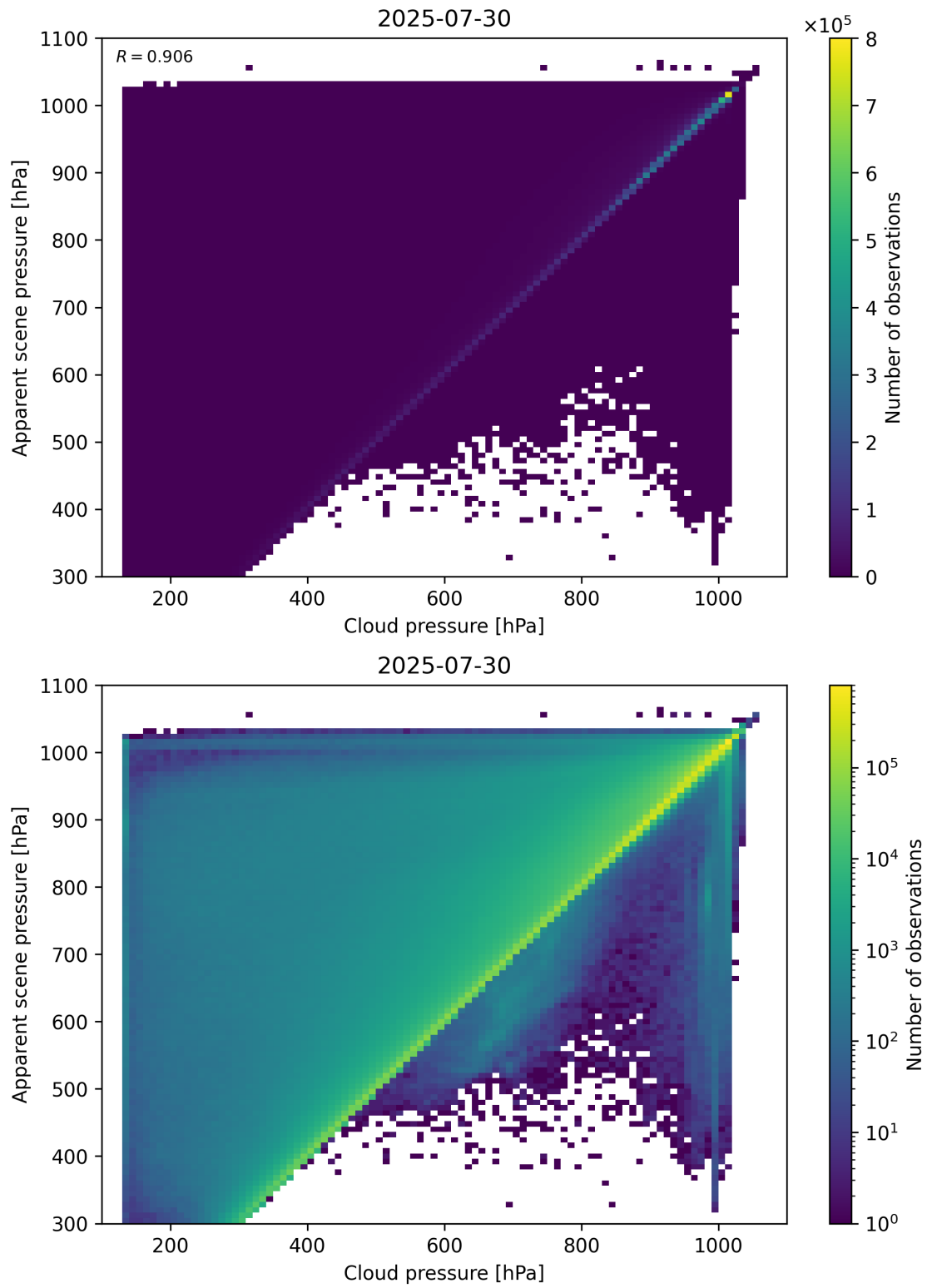
Figure 77: Scatter density plot of “Cloud pressure” against “Apparent scene pressure” for 2025-07-29 to 2025-07-31.
