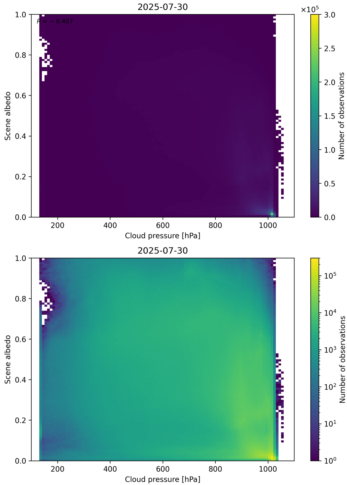
Figure 83: Scatter density plot of “Cloud pressure” against “Scene albedo” for 2025-07-29 to 2025-07-31.
