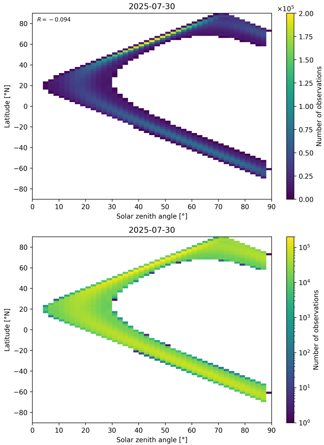
Figure 113: Scatter density plot of “Solar zenith angle” against “Latitude” for 2025-07-29 to 2025-07-31.
