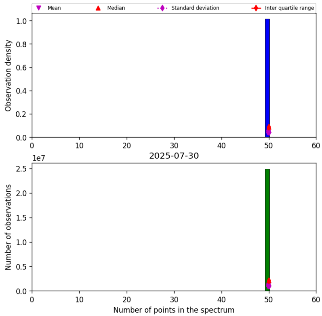
Figure 44: Histogram of “Number of points in the spectrum” for 2025-07-29 to 2025-07-31
