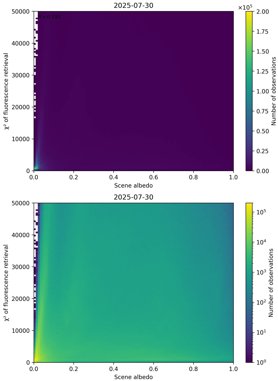
Figure 103: Scatter density plot of “Scene albedo” against “ \chi^2 of fluorescence retrieval” for 2025-07-29 to 2025-07-31.
