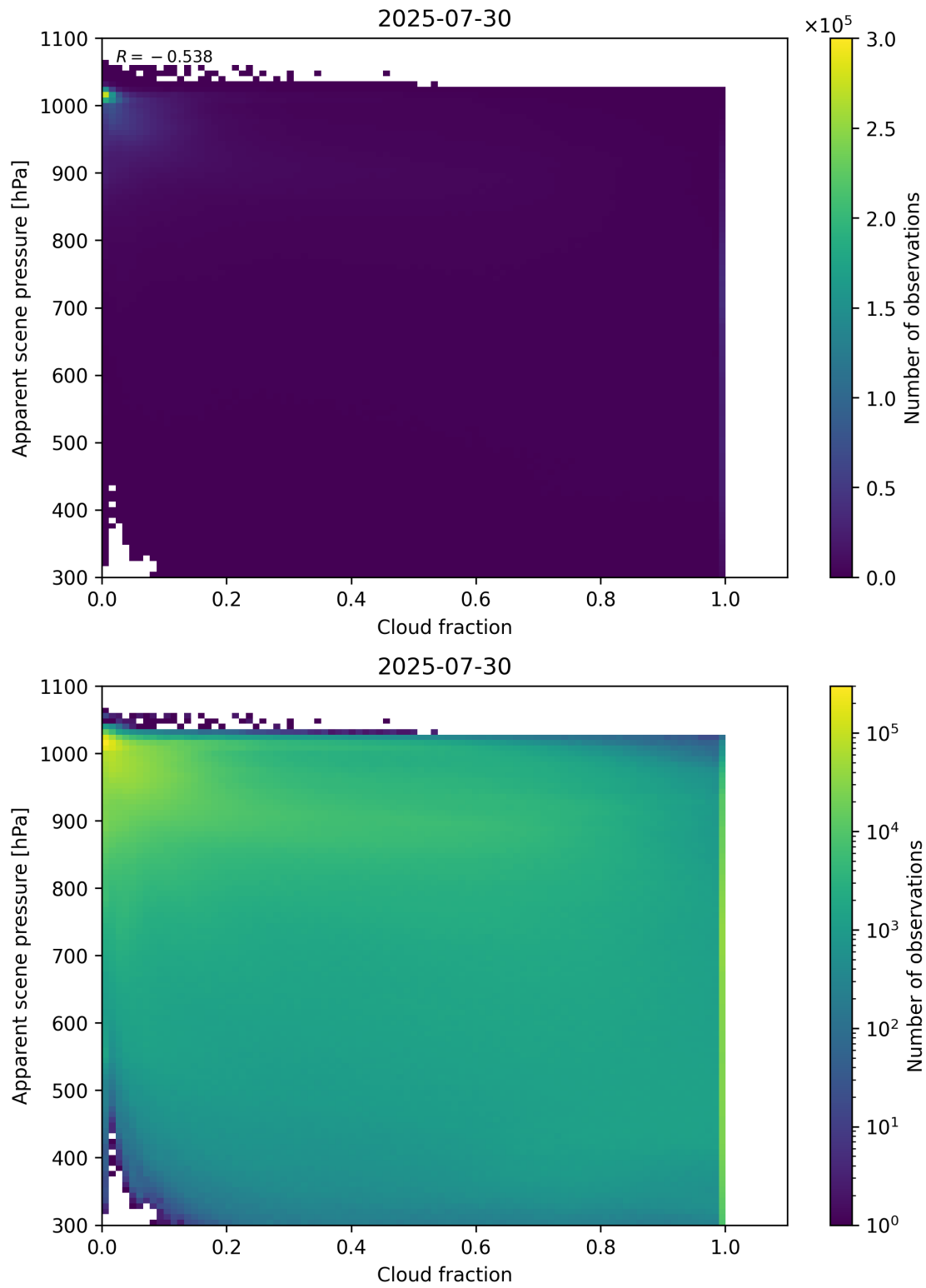
Figure 70: Scatter density plot of “Cloud fraction” against “Apparent scene pressure” for 2025-07-29 to 2025-07-31.
