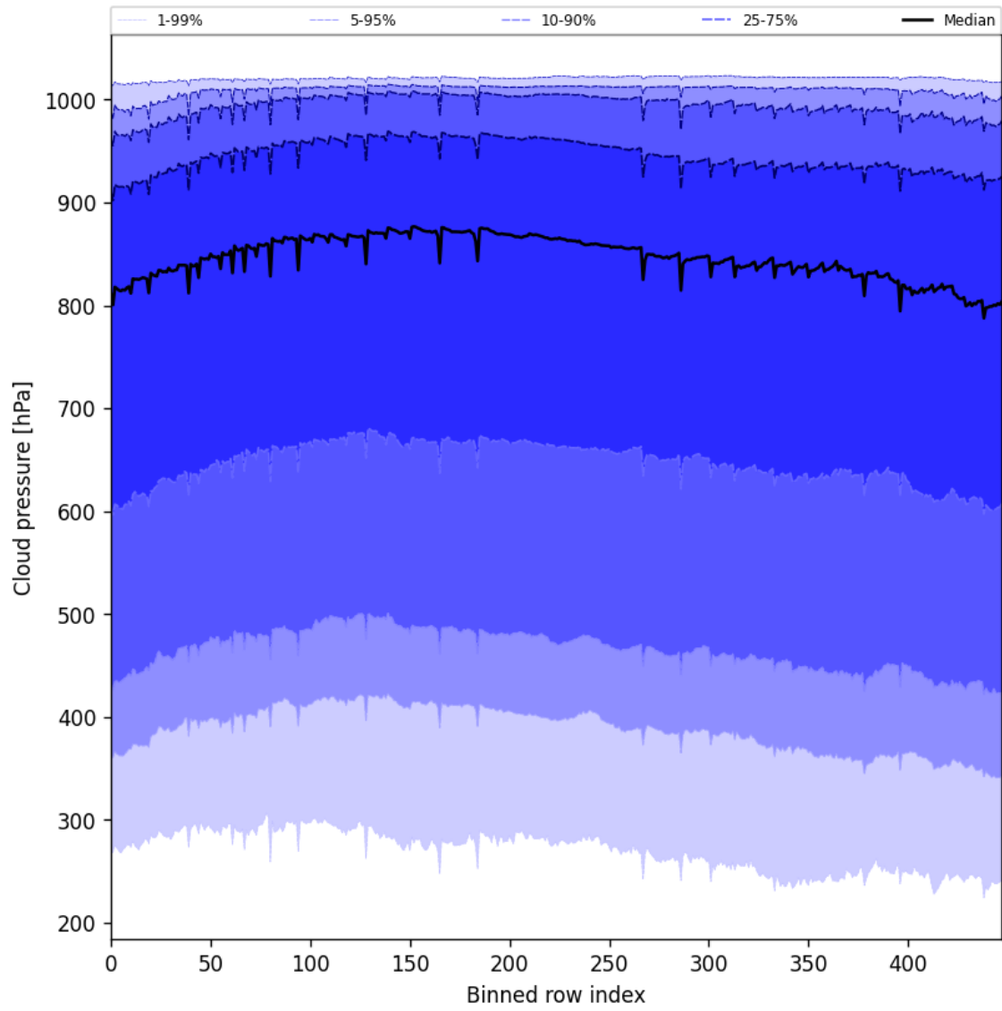
Figure 47: Along track statistics of “Cloud pressure” for 2025-07-29 to 2025-07-31
