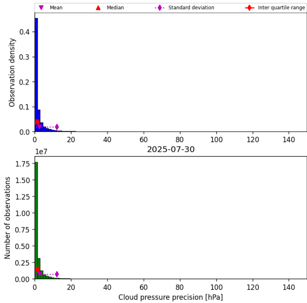
Figure 31: Histogram of “Cloud pressure precision” for 2025-07-29 to 2025-07-31
