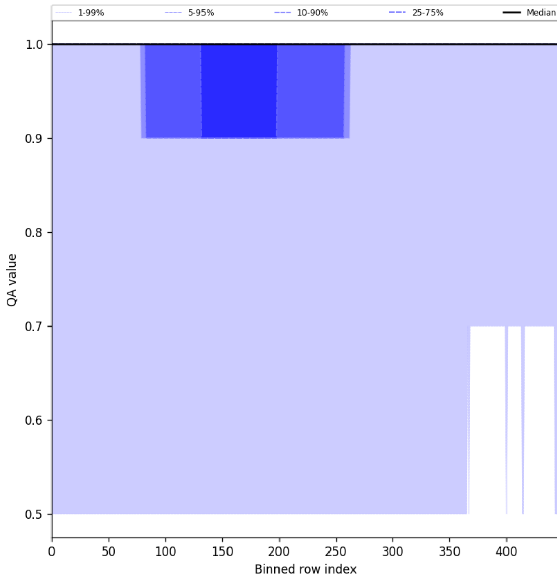
Figure 46: Along track statistics of “QA value” for 2025-07-29 to 2025-07-31
