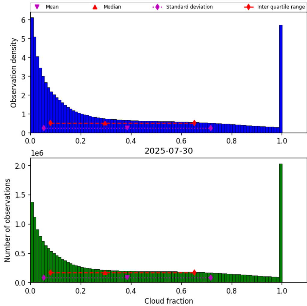
Figure 32: Histogram of “Cloud fraction” for 2025-07-29 to 2025-07-31
