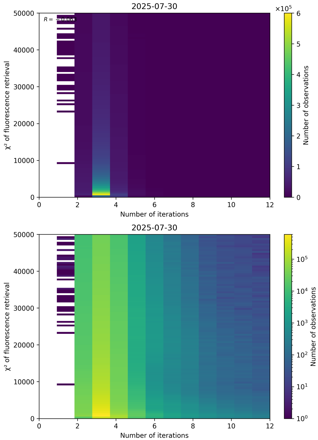
Figure 97: Scatter density plot of “Number of iterations” against “ \chi^2 of fluorescence retrieval” for 2025-07-29 to 2025-07-31.
