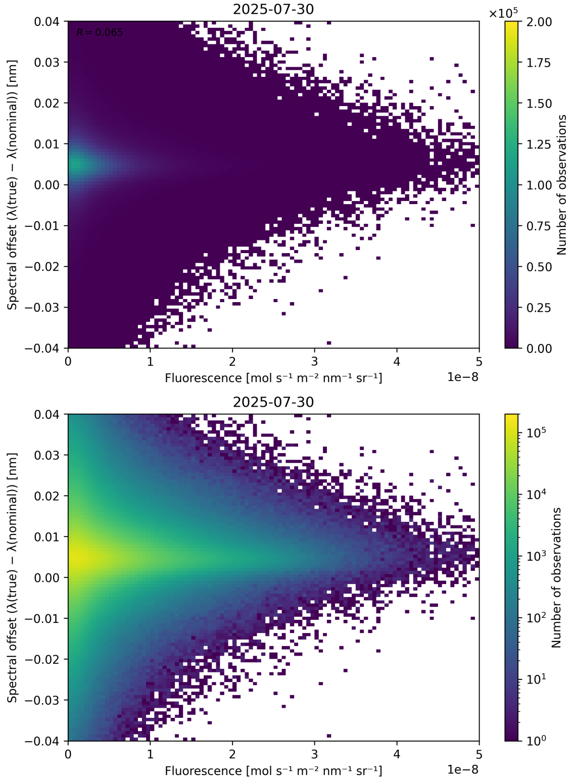
Figure 87: Scatter density plot of “Fluorescence” against “Spectral offset ( \lambda_{\text{true}} - \lambda_{\text{nominal}} )” for 2025-07-29 to 2025-07-31.
