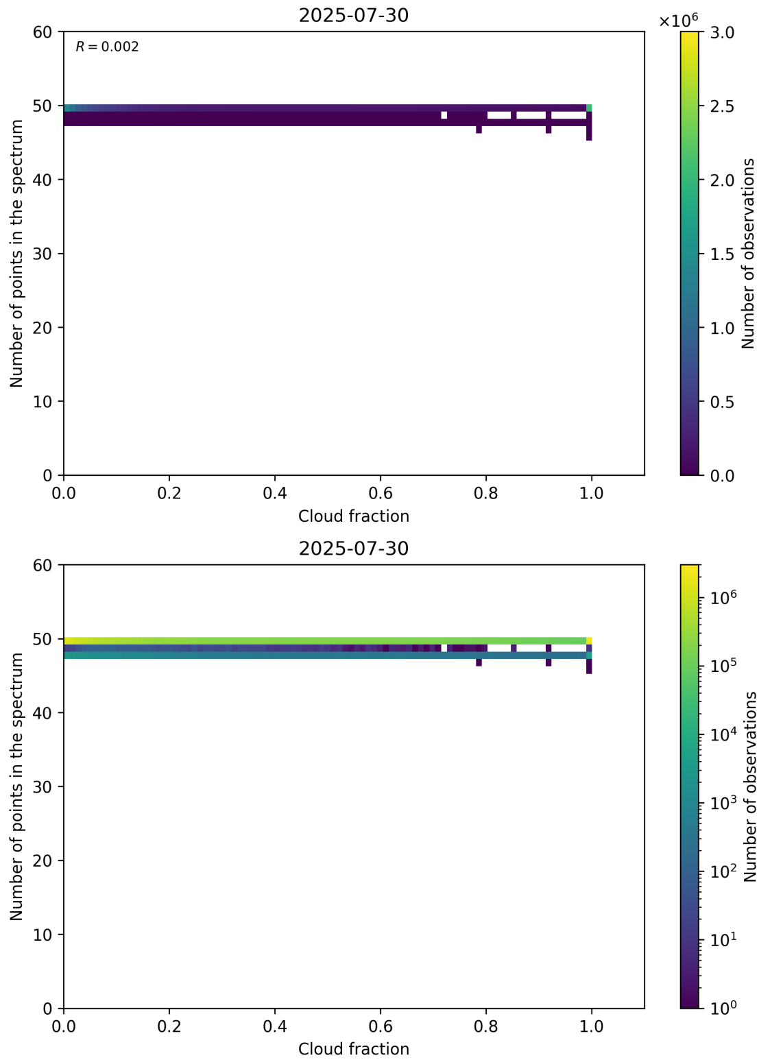
Figure 74: Scatter density plot of “Cloud fraction” against “Number of points in the spectrum” for 2025-07-29 to 2025-07-31.
