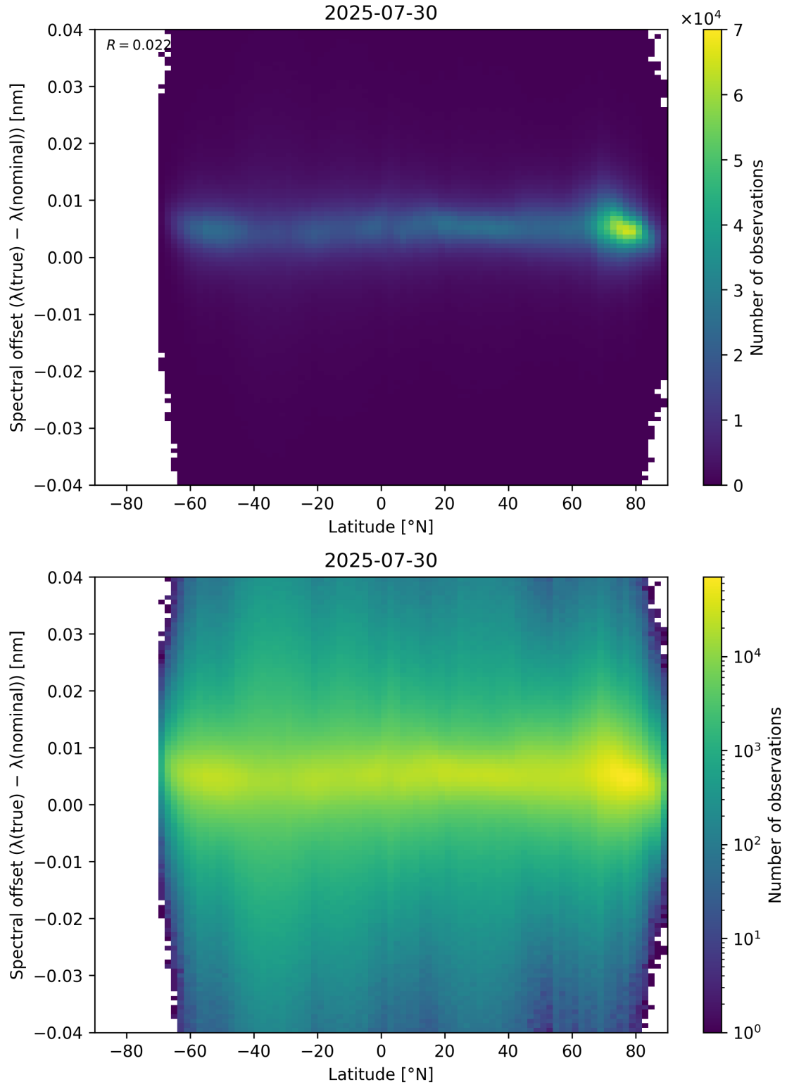
Figure 96: Scatter density plot of “Latitude” against “Spectral offset ( \lambda_{\text{true}} - \lambda_{\text{nominal}} )” for 2025-07-29 to 2025-07-31.
