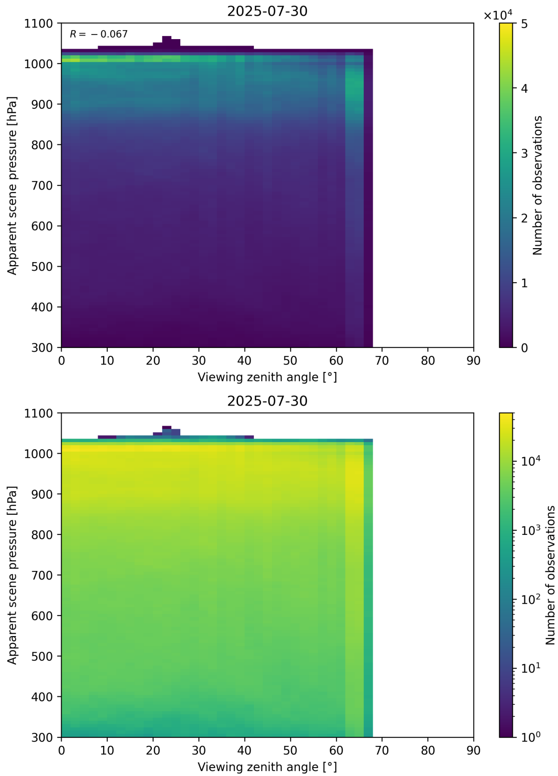
Figure 118: Scatter density plot of “Viewing zenith angle” against “Apparent scene pressure” for 2025-07-29 to 2025-07-31.
