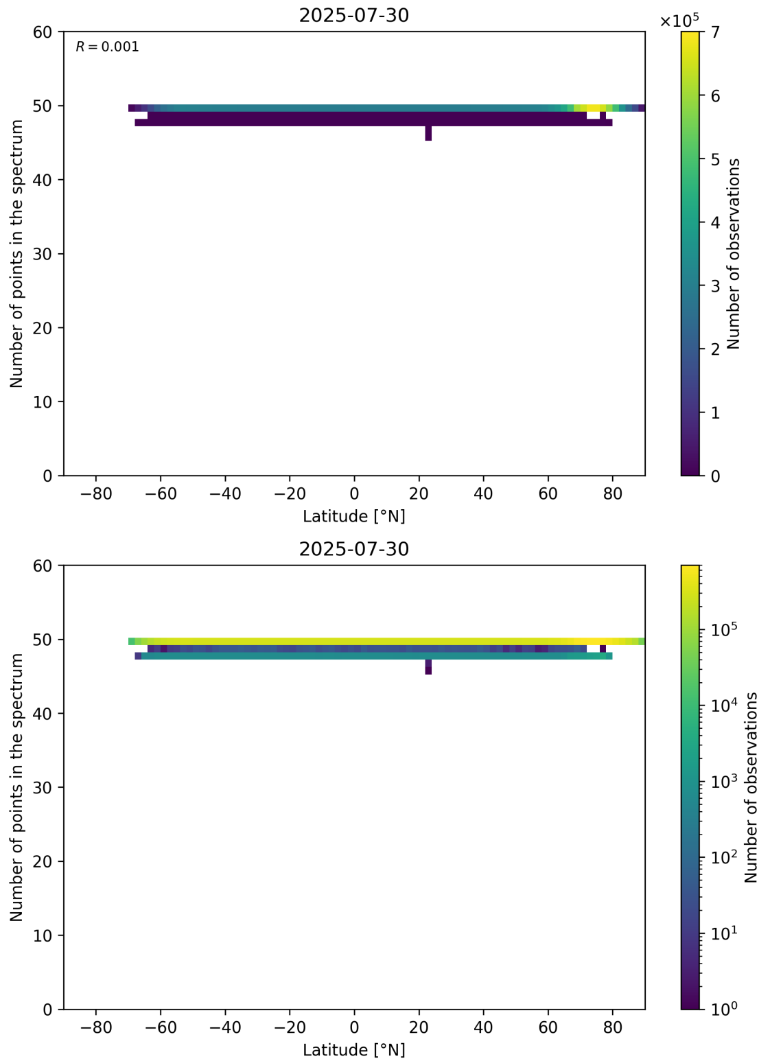
Figure 94: Scatter density plot of “Latitude” against “Number of points in the spectrum” for 2025-07-29 to 2025-07-31.
