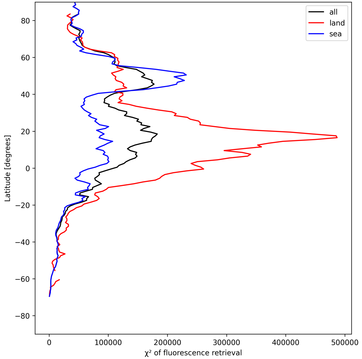
Figure 25: Zonal average of “ \chi^2 of fluorescence retrieval” for 2025-07-29 to 2025-07-31.
