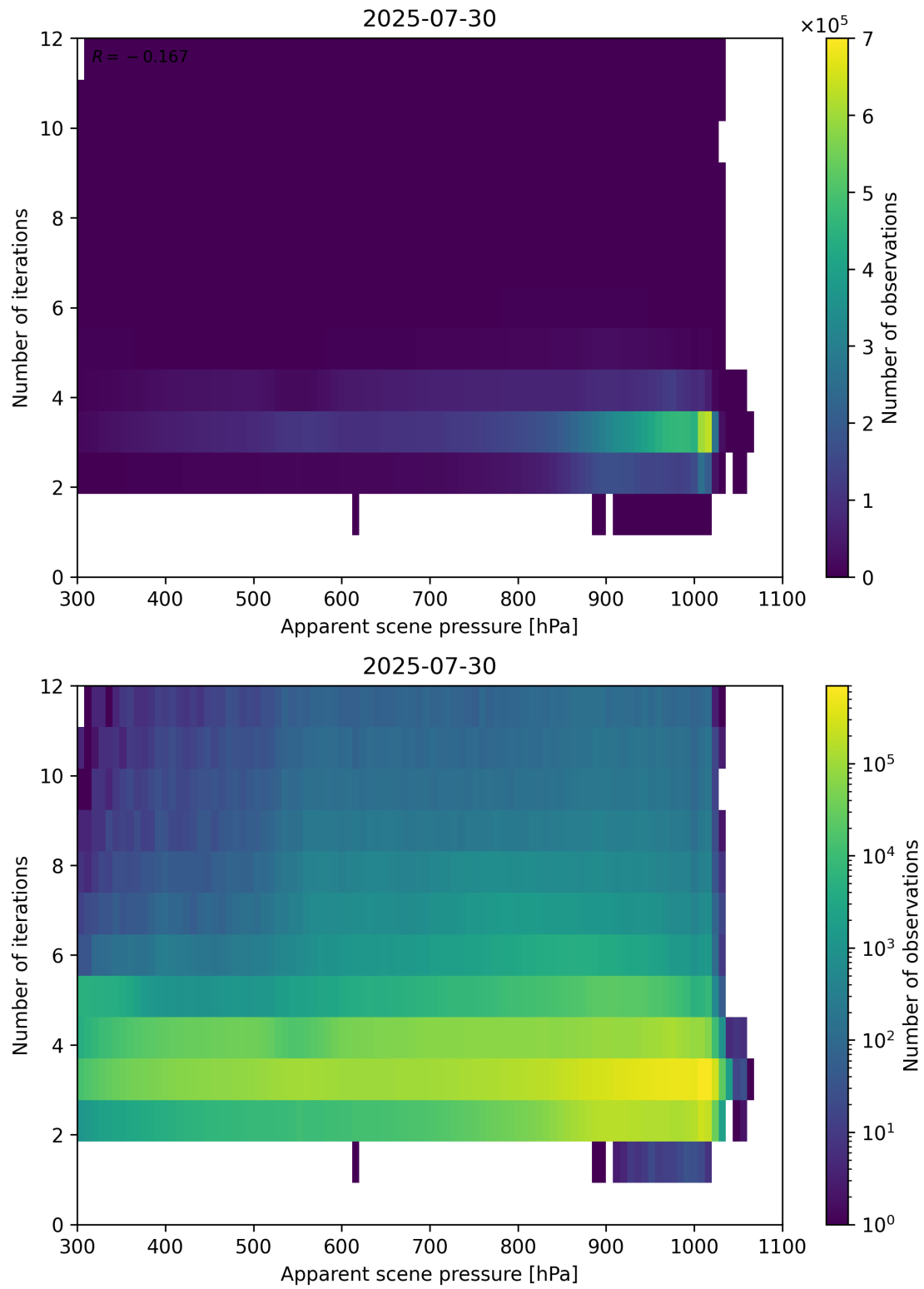
Figure 65: Scatter density plot of “Apparent scene pressure” against “Number of iterations” for 2025-07-29 to 2025-07-31.
