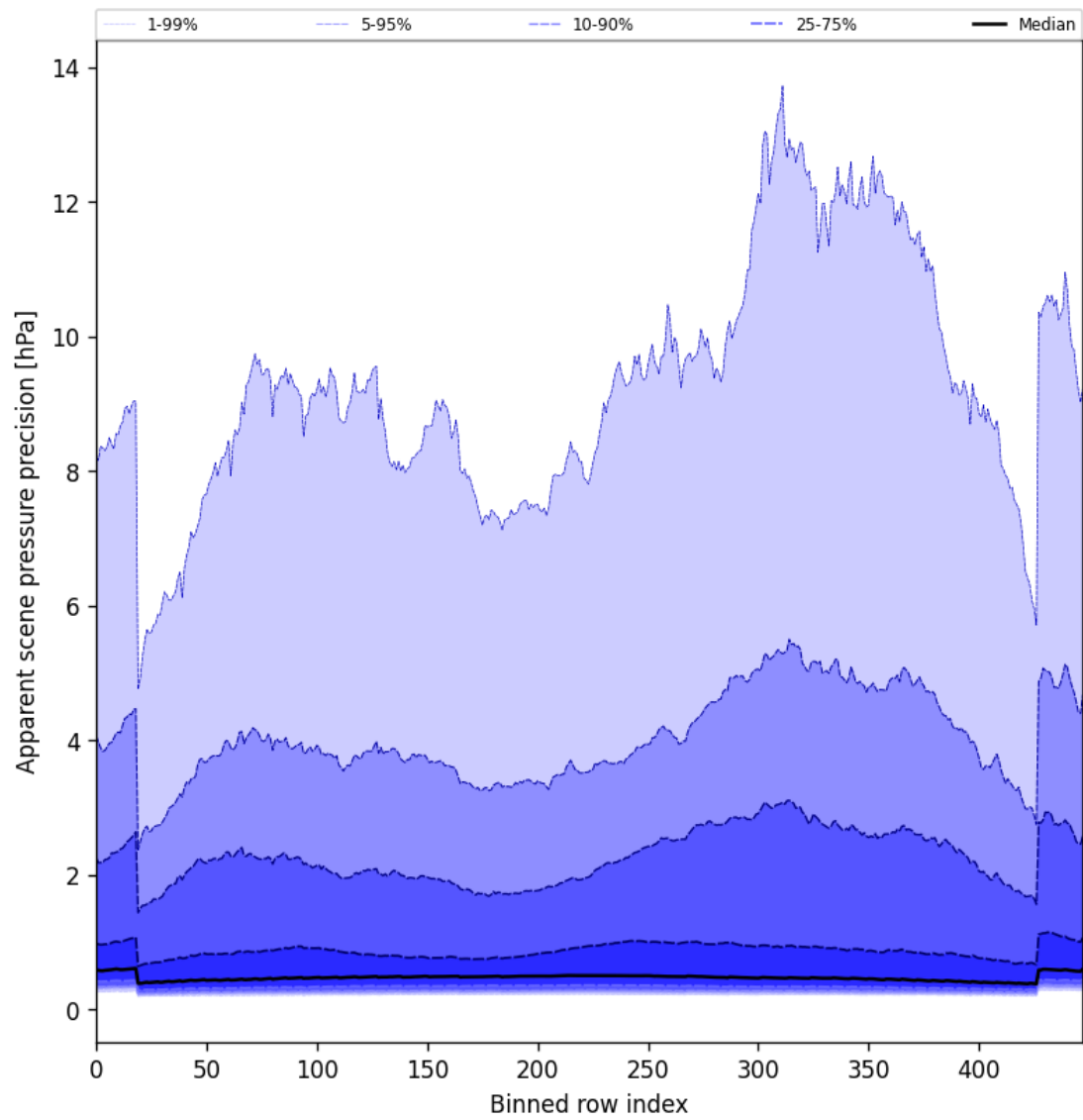
Figure 54: Along track statistics of “Apparent scene pressure precision” for 2025-07-29 to 2025-07-31
