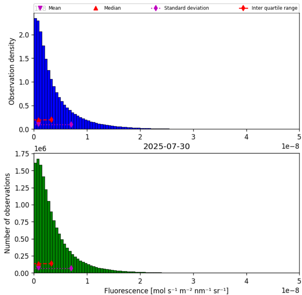
Figure 40: Histogram of “Fluorescence” for 2025-07-29 to 2025-07-31
