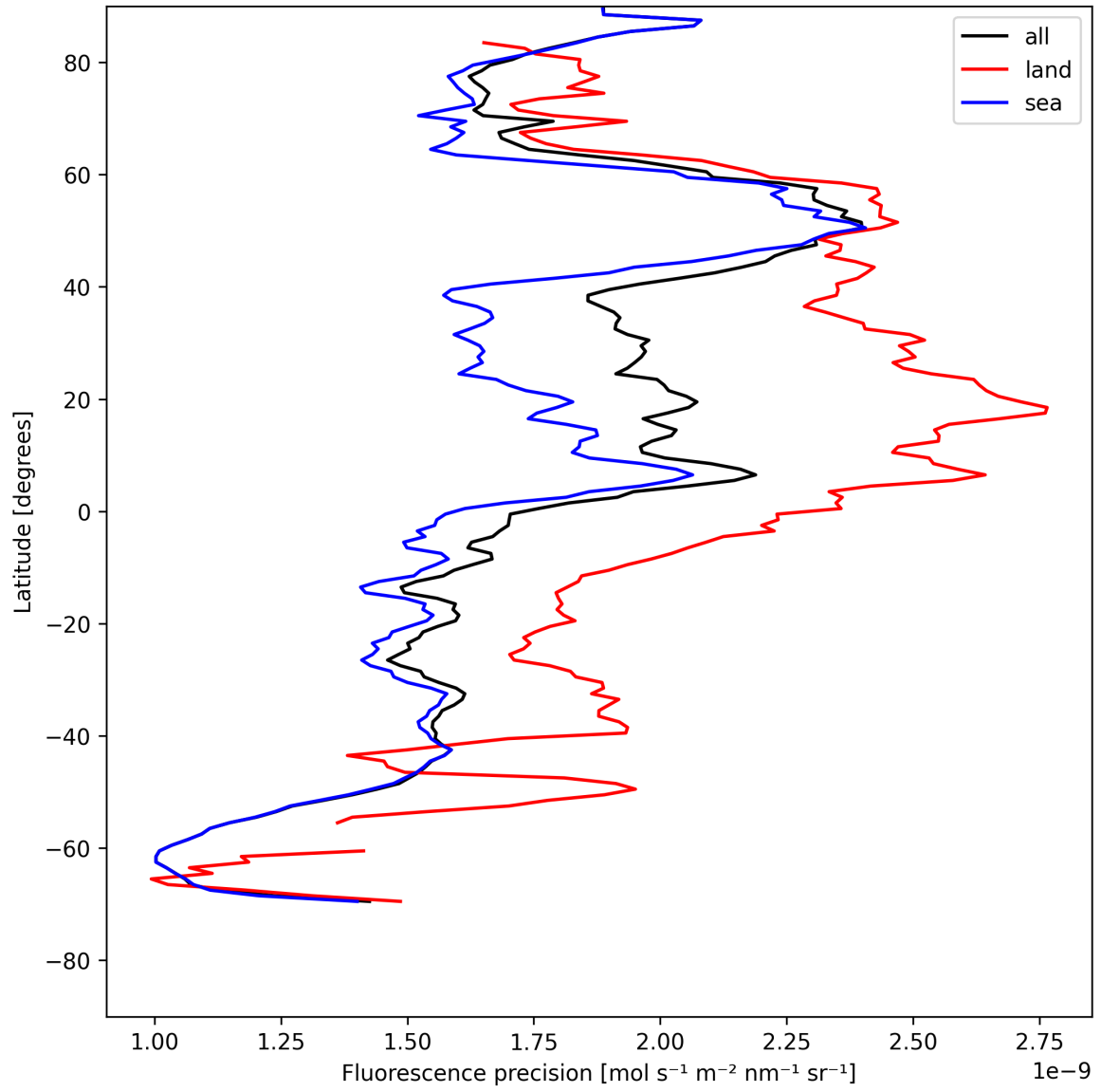
Figure 24: Zonal average of “Fluorescence precision” for 2025-07-29 to 2025-07-31.
