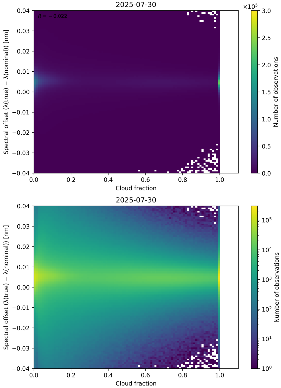
Figure 76: Scatter density plot of “Cloud fraction” against “Spectral offset ( \lambda_{\text{true}} - \lambda_{\text{nominal}} )” for 2025-07-29 to 2025-07-31.
