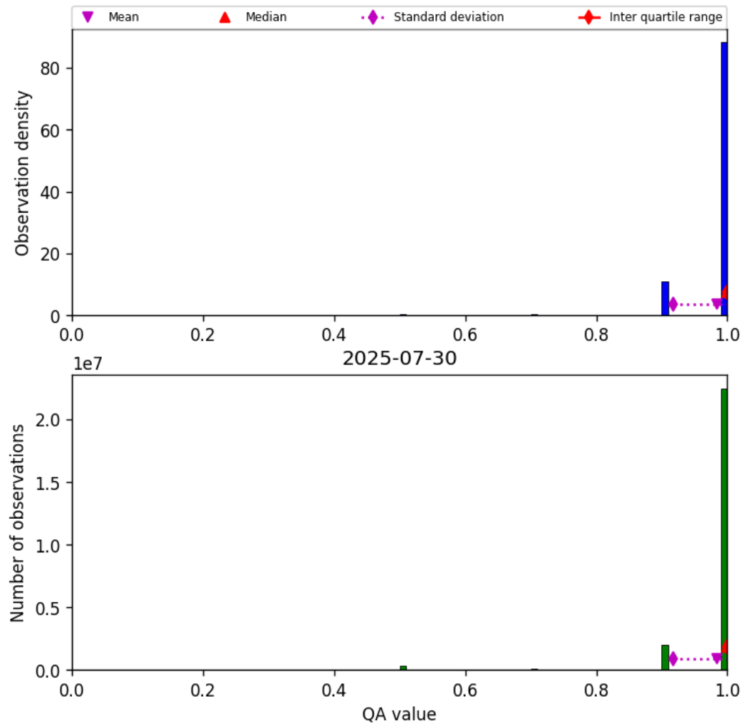
Figure 29: Histogram of “QA value” for 2025-07-29 to 2025-07-31
