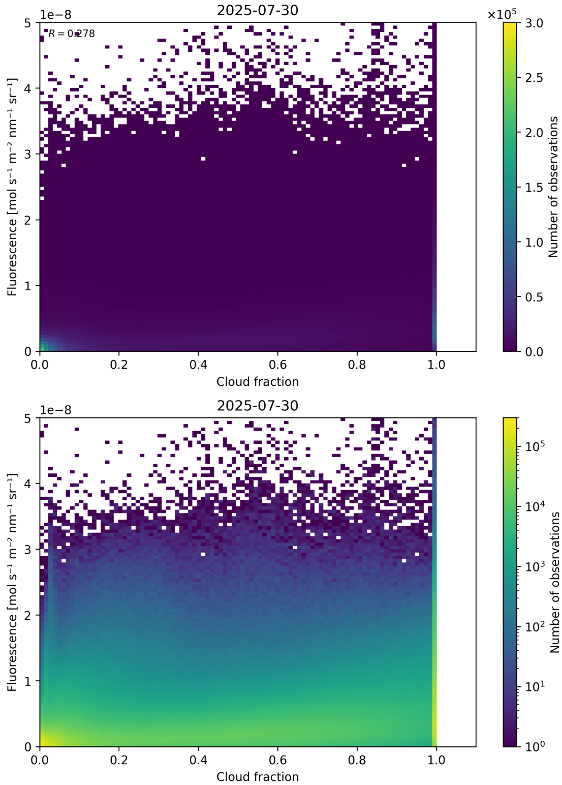
Figure 72: Scatter density plot of “Cloud fraction” against “Fluorescence” for 2025-07-29 to 2025-07-31.
