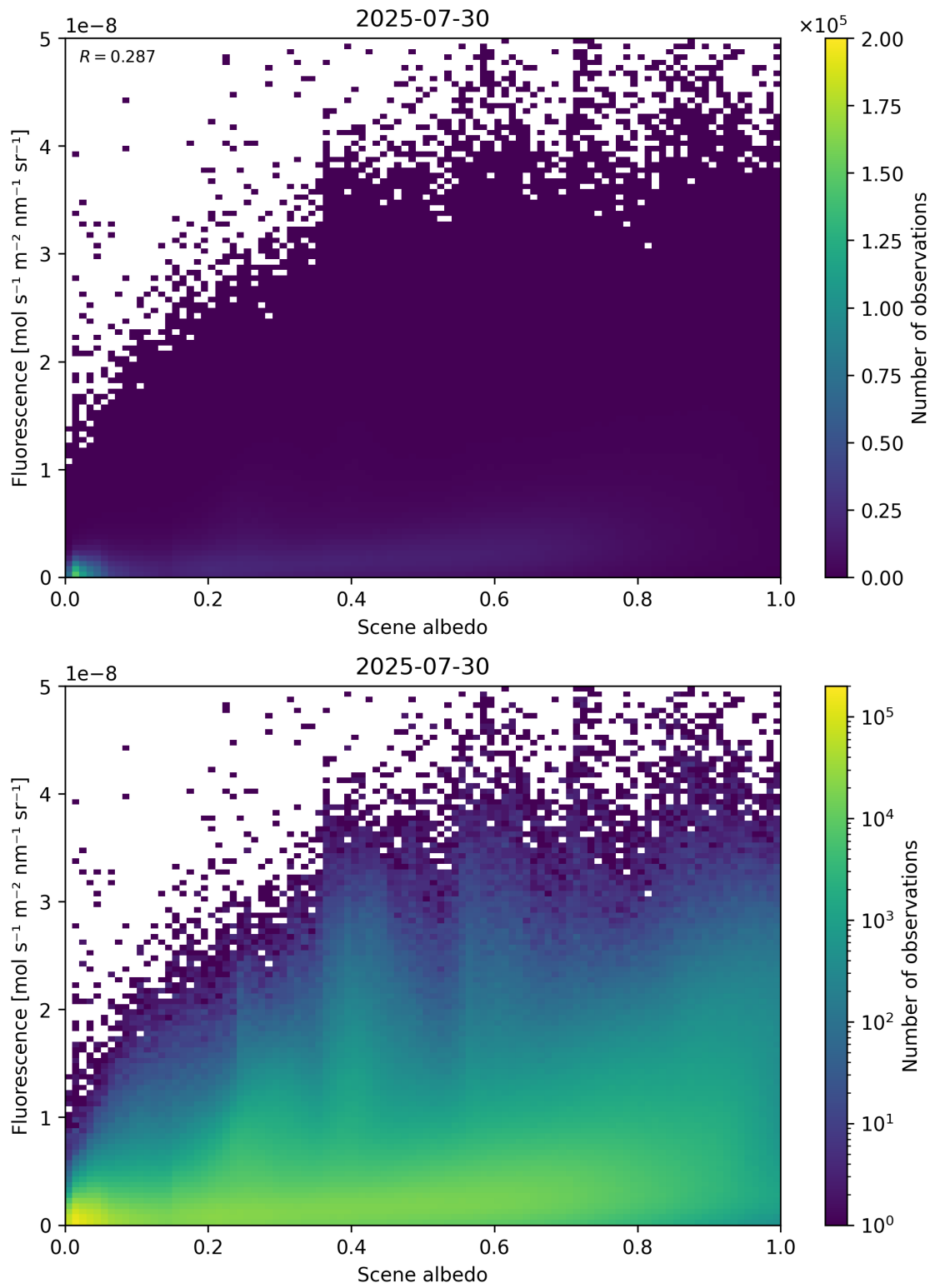
Figure 104: Scatter density plot of “Scene albedo” against “Fluorescence” for 2025-07-29 to 2025-07-31.
