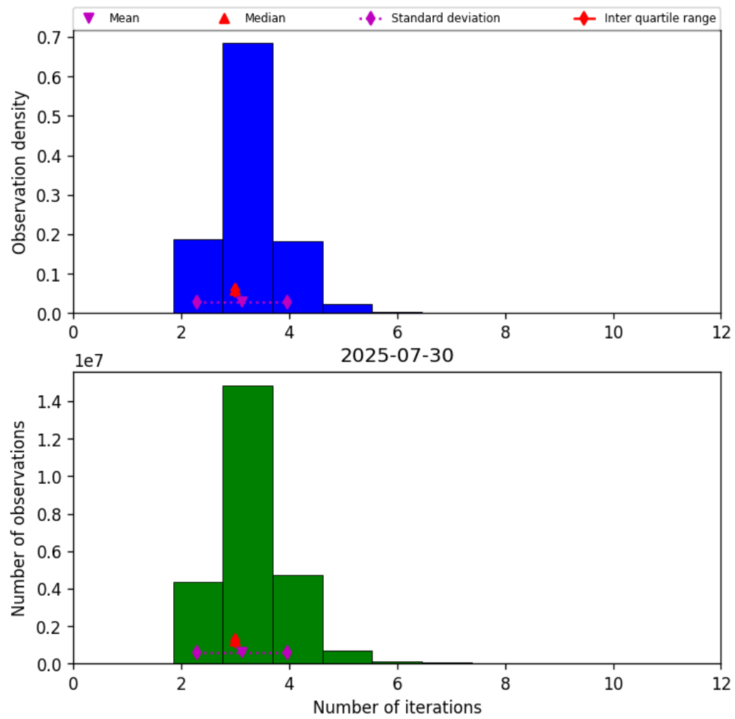
Figure 39: Histogram of “Number of iterations” for 2025-07-29 to 2025-07-31
