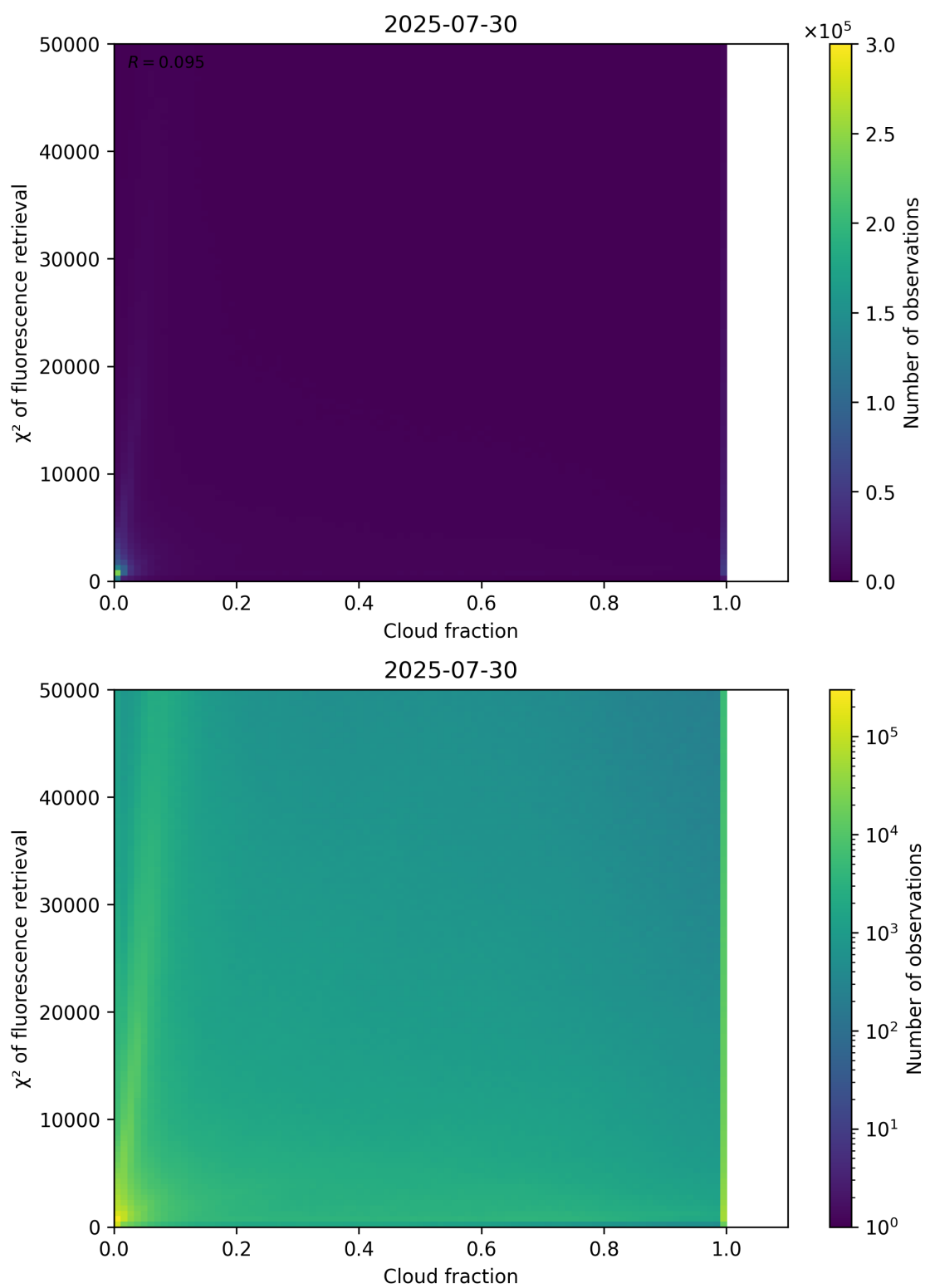
Figure 71: Scatter density plot of “Cloud fraction” against “ \chi^2 of fluorescence retrieval” for 2025-07-29 to 2025-07-31.
