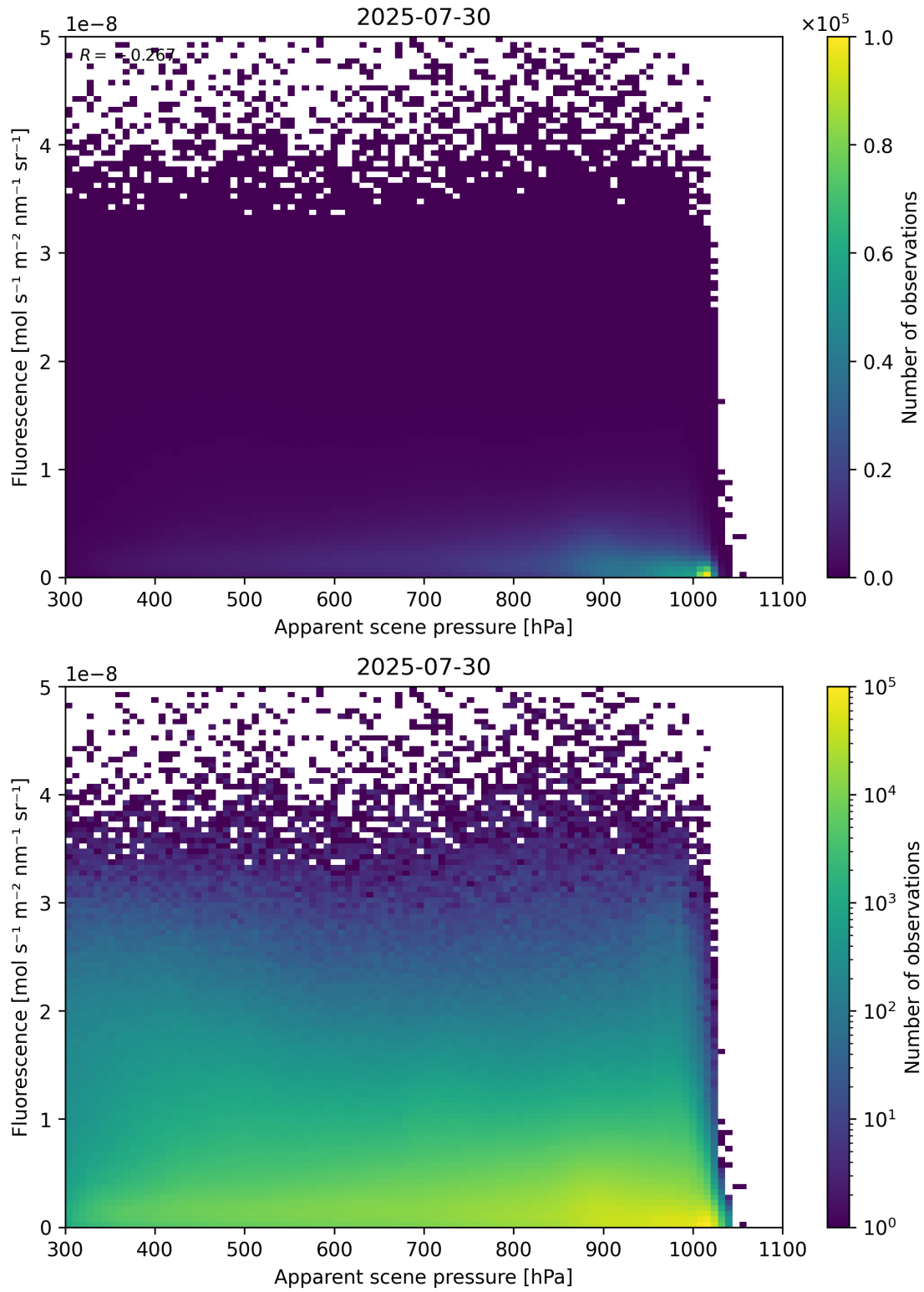
Figure 64: Scatter density plot of “Apparent scene pressure” against “Fluorescence” for 2025-07-29 to 2025-07-31.
