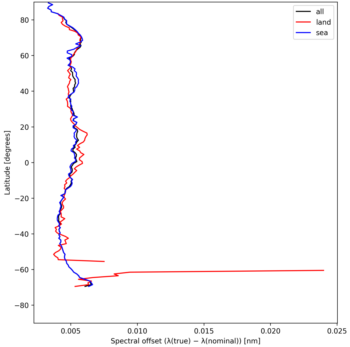
Figure 28: Zonal average of “Spectral offset ( \lambda_{\text{true}} - \lambda_{\text{nominal}} )” for 2025-07-29 to 2025-07-31.
