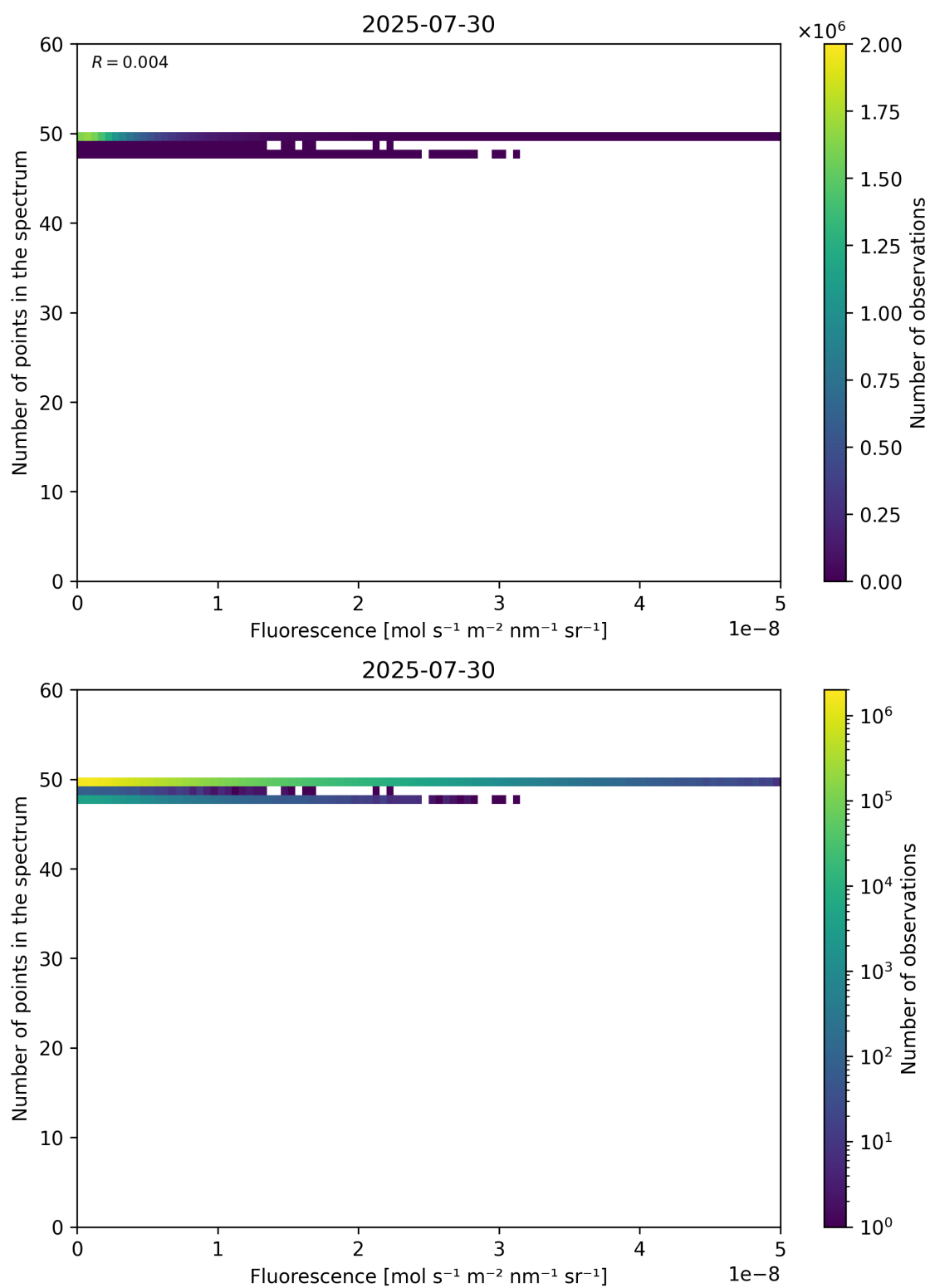
Figure 86: Scatter density plot of “Fluorescence” against “Number of points in the spectrum” for 2025-07-29 to 2025-07-31.
