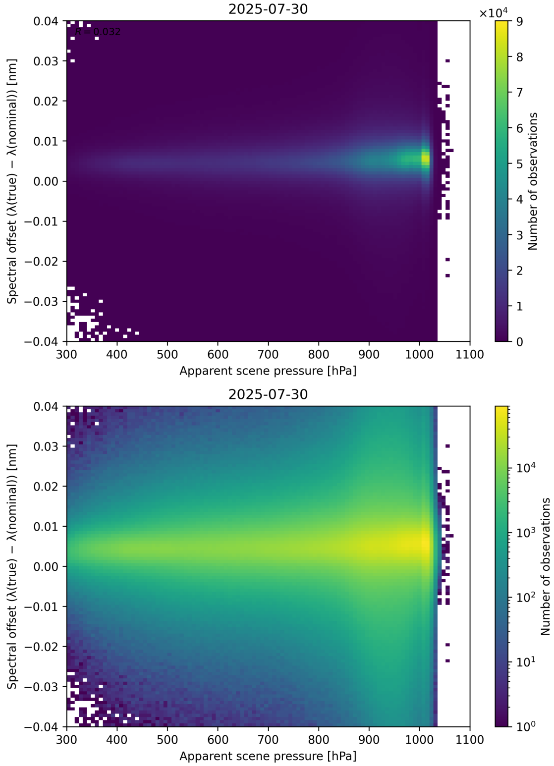
Figure 67: Scatter density plot of “Apparent scene pressure” against “Spectral offset ( \lambda_{\text{true}} - \lambda_{\text{nominal}} )” for 2025-07-29 to 2025-07-31.
