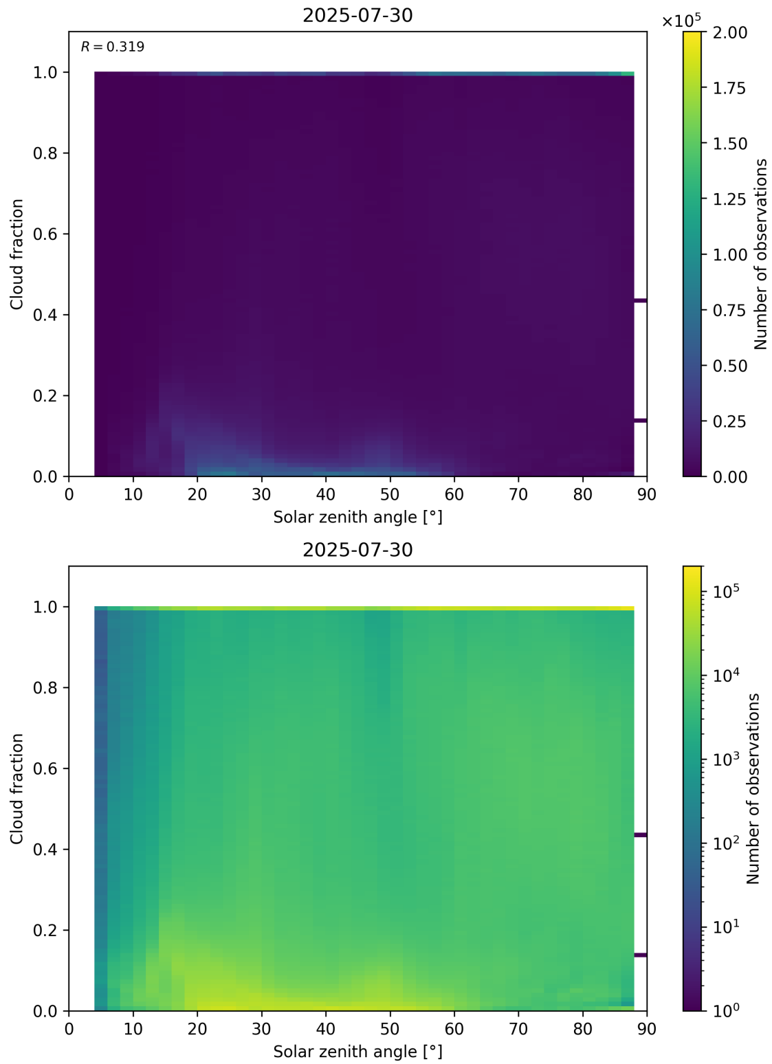
Figure 110: Scatter density plot of “Solar zenith angle” against “Cloud fraction” for 2025-07-29 to 2025-07-31.
