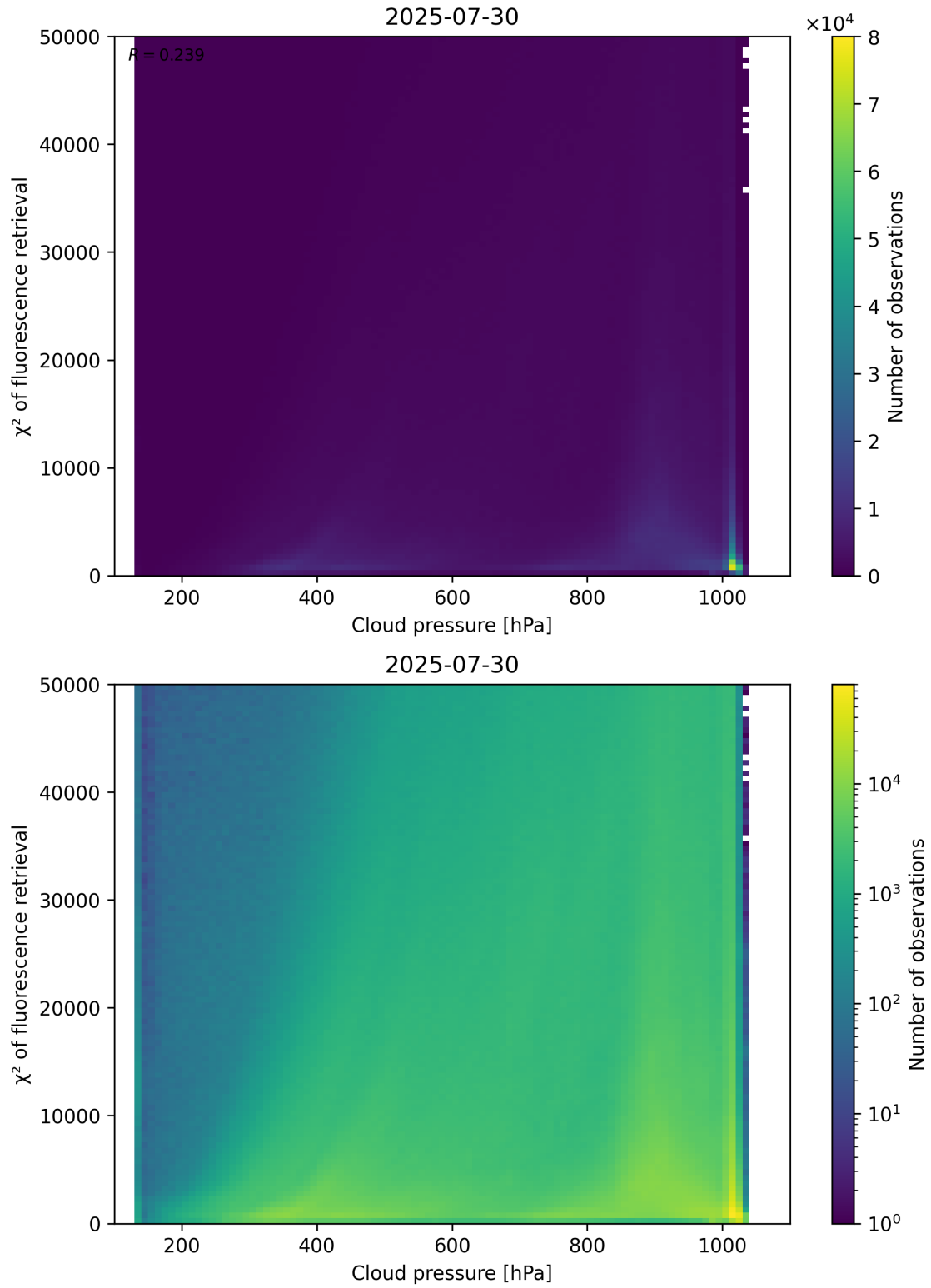
Figure 78: Scatter density plot of “Cloud pressure” against “ \chi^2 of fluorescence retrieval” for 2025-07-29 to 2025-07-31.
