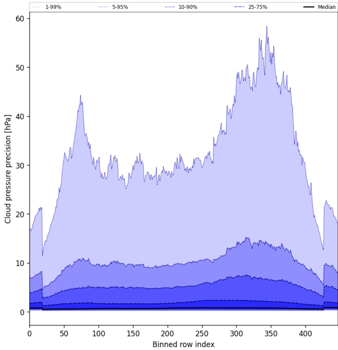
Figure 48: Along track statistics of “Cloud pressure precision” for 2025-07-29 to 2025-07-31
