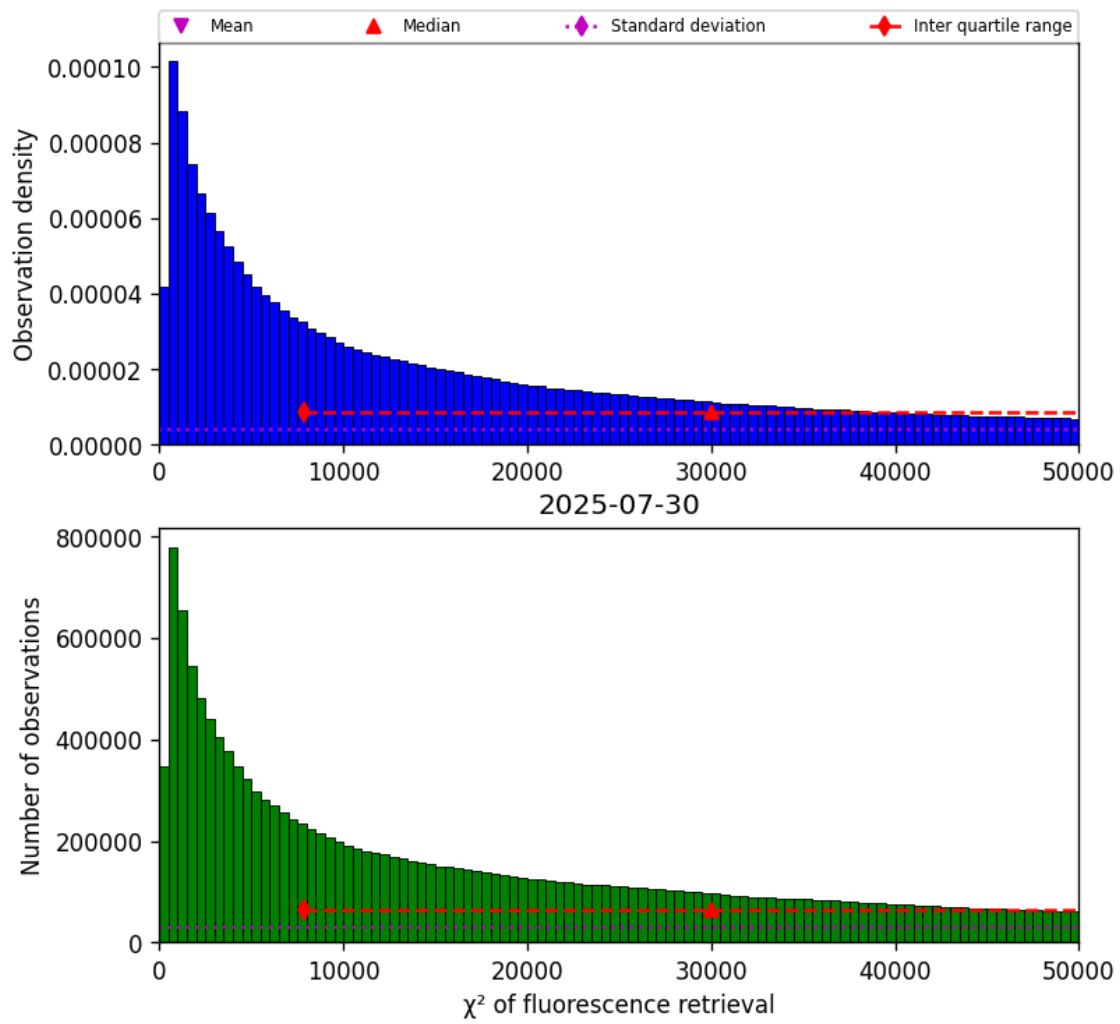
Figure 42: Histogram of “ \chi^2 of fluorescence retrieval” for 2025-07-29 to 2025-07-31
