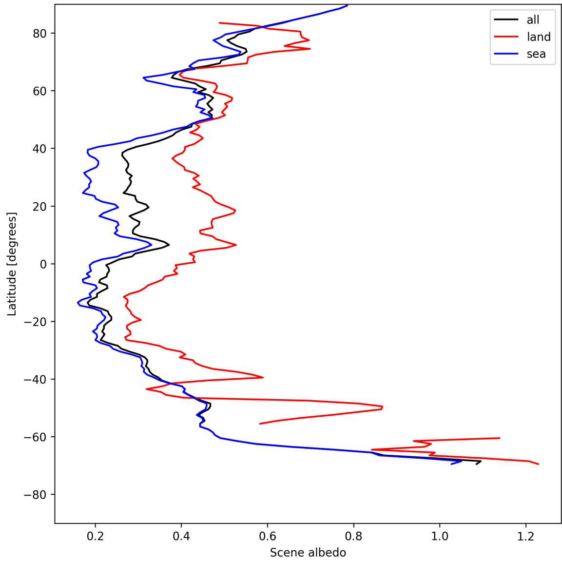
Figure 17: Zonal average of “Scene albedo” for 2025-07-29 to 2025-07-31.
