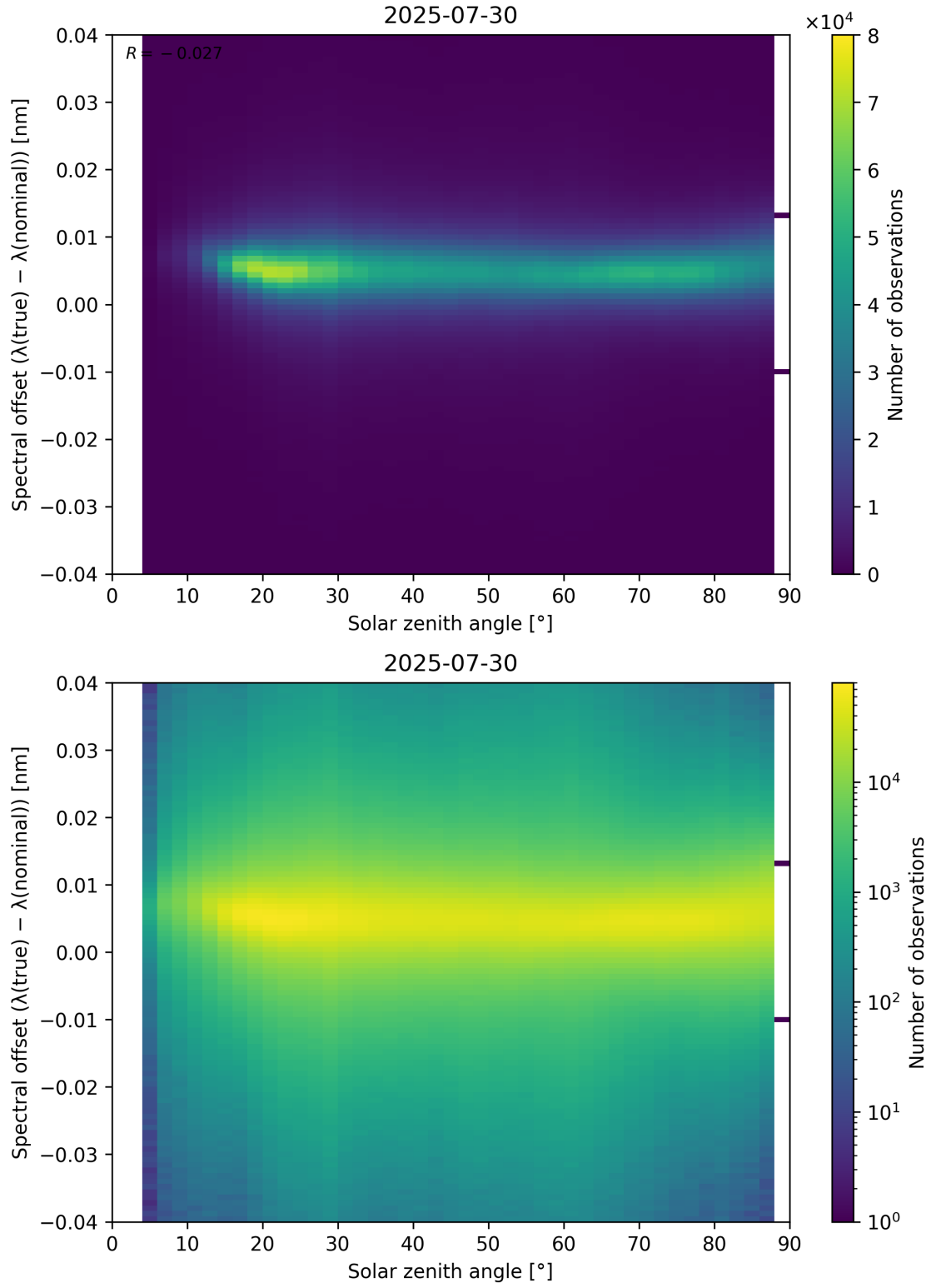
Figure 117: Scatter density plot of “Solar zenith angle” against “Spectral offset ( \lambda_{\text{true}} - \lambda_{\text{nominal}} )” for 2025-07-29 to 2025-07-31.
