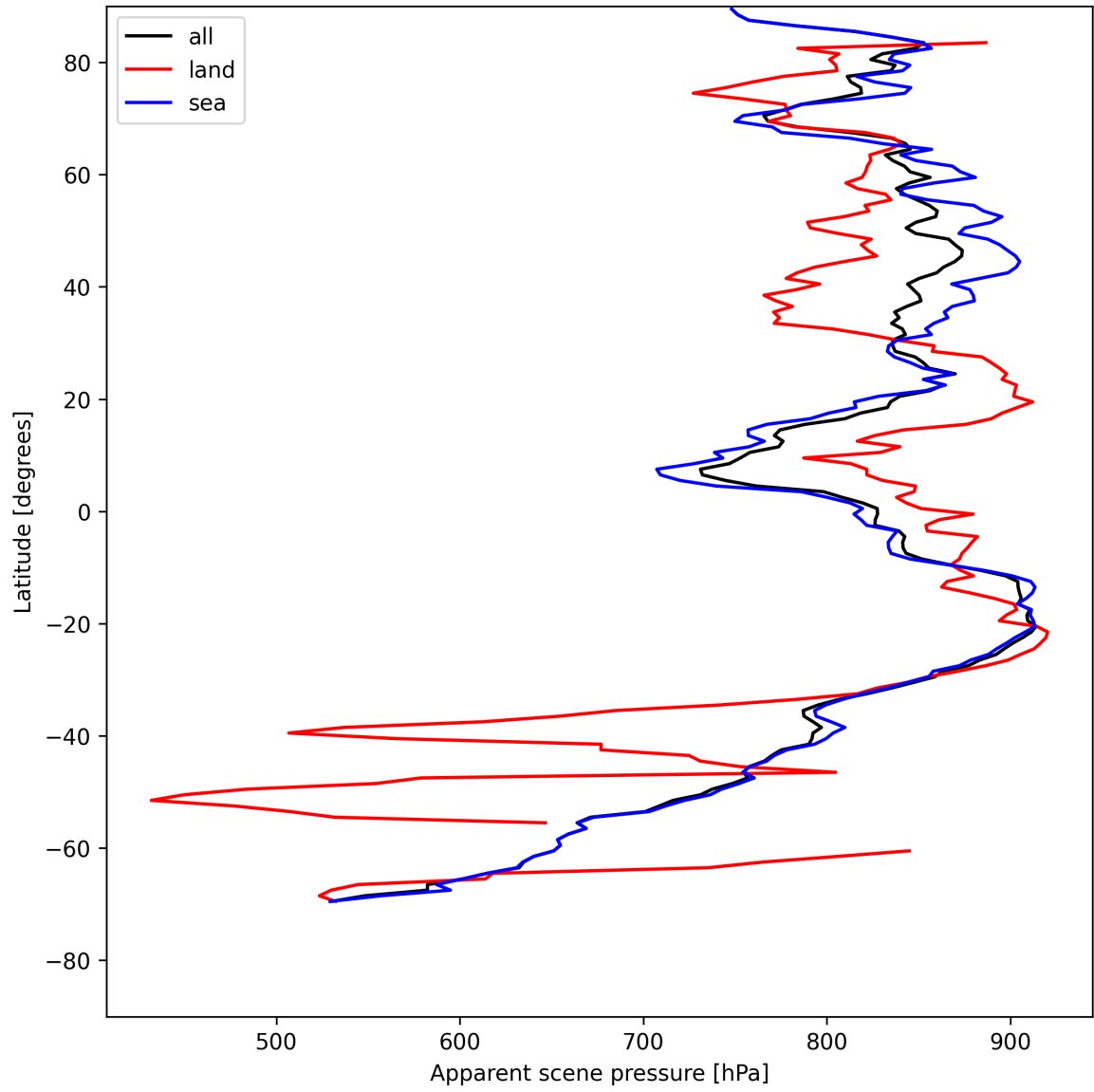
Figure 19: Zonal average of “Apparent scene pressure” for 2025-07-29 to 2025-07-31.
