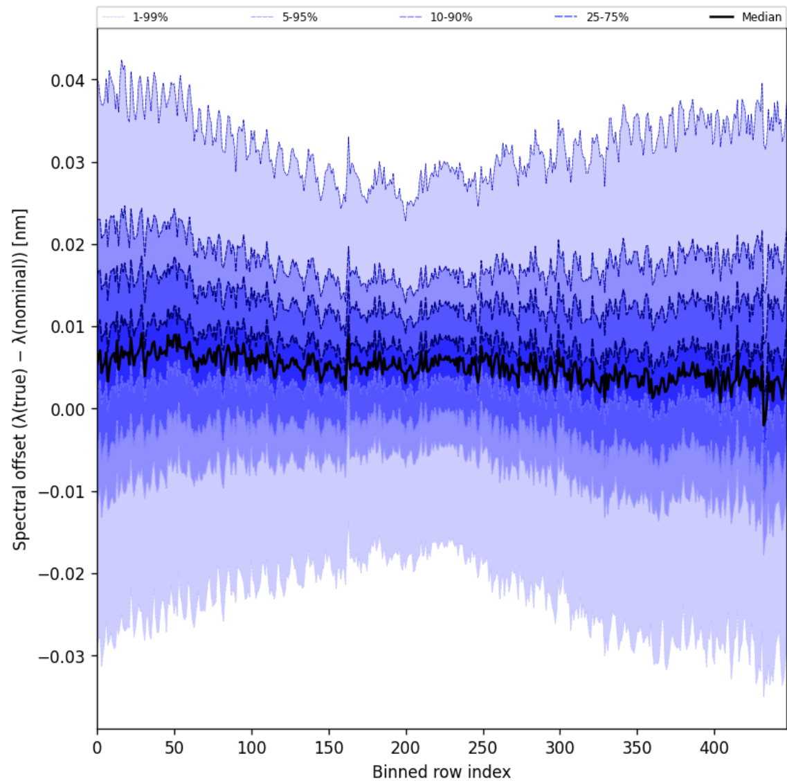
Figure 62: Along track statistics of “Spectral offset ( \lambda_{\text{true}} - \lambda_{\text{nominal}} )” for 2025-07-29 to 2025-07-31
