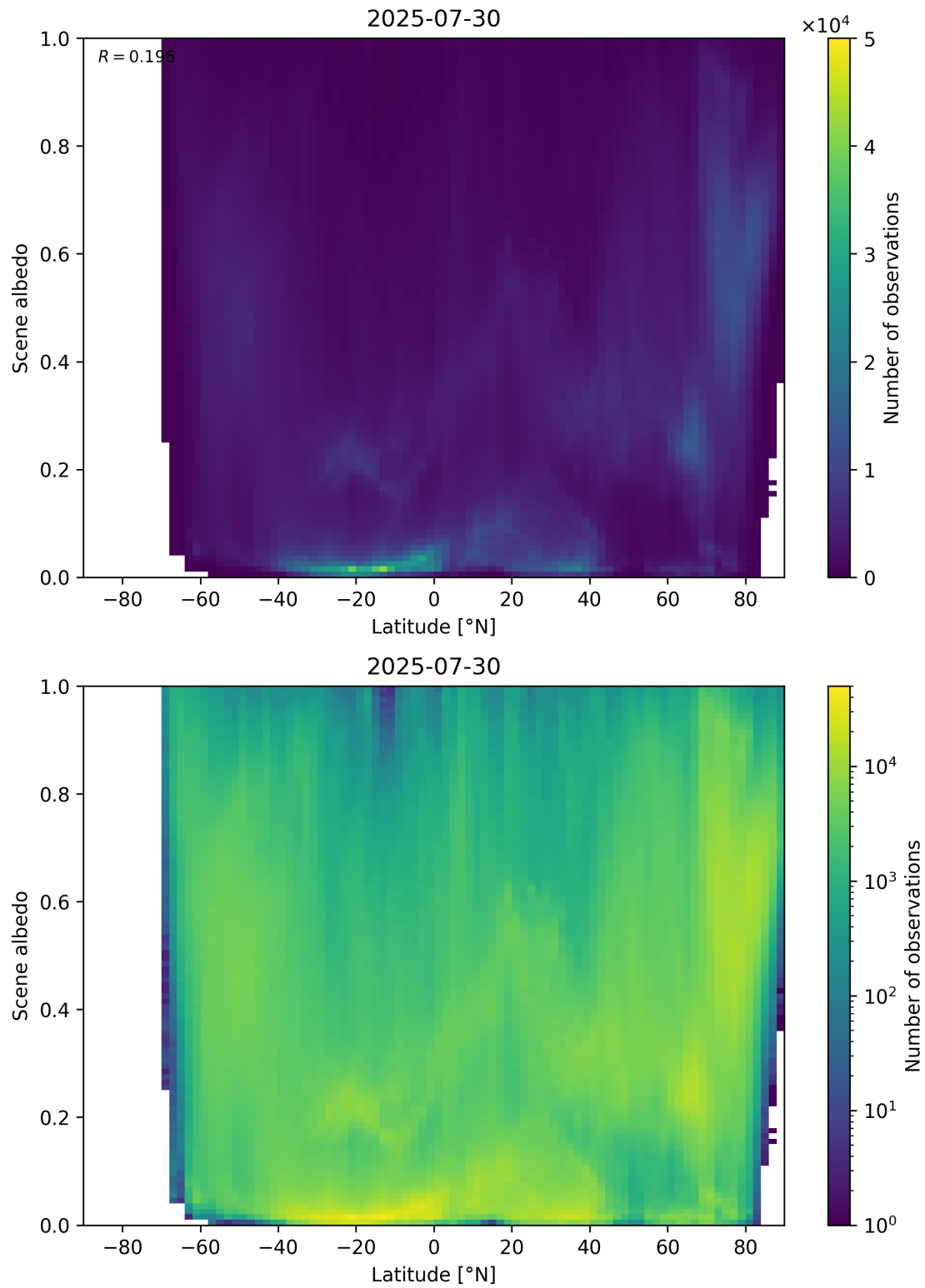
Figure 95: Scatter density plot of “Latitude” against “Scene albedo” for 2025-07-29 to 2025-07-31.
