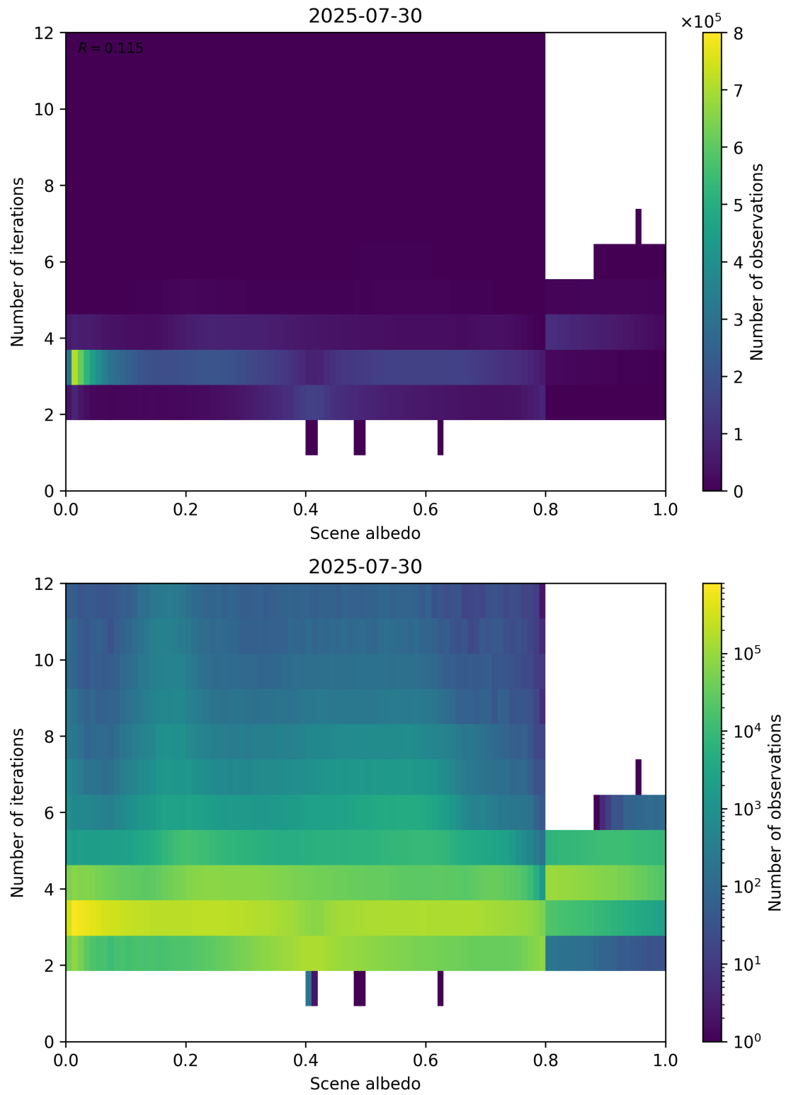
Figure 105: Scatter density plot of “Scene albedo” against “Number of iterations” for 2025-07-29 to 2025-07-31.
