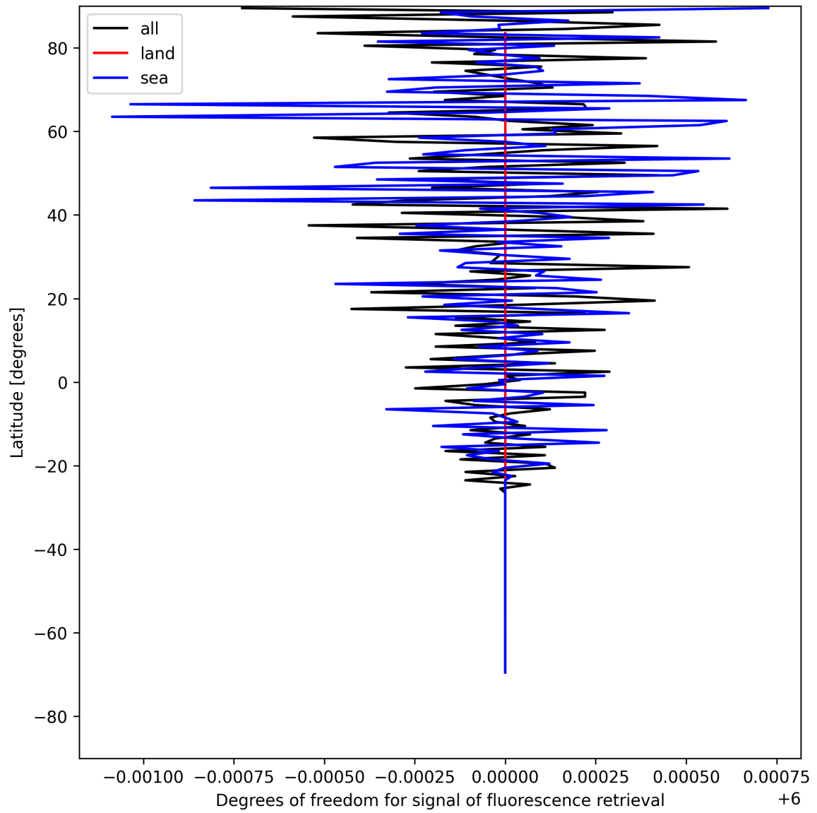
Figure 26: Zonal average of “Degrees of freedom for signal of fluorescence retrieval” for 2025-07-29 to 2025-07-31.
