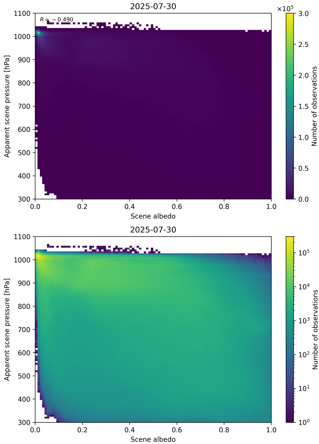
Figure 102: Scatter density plot of “Scene albedo” against “Apparent scene pressure” for 2025-07-29 to 2025-07-31.
