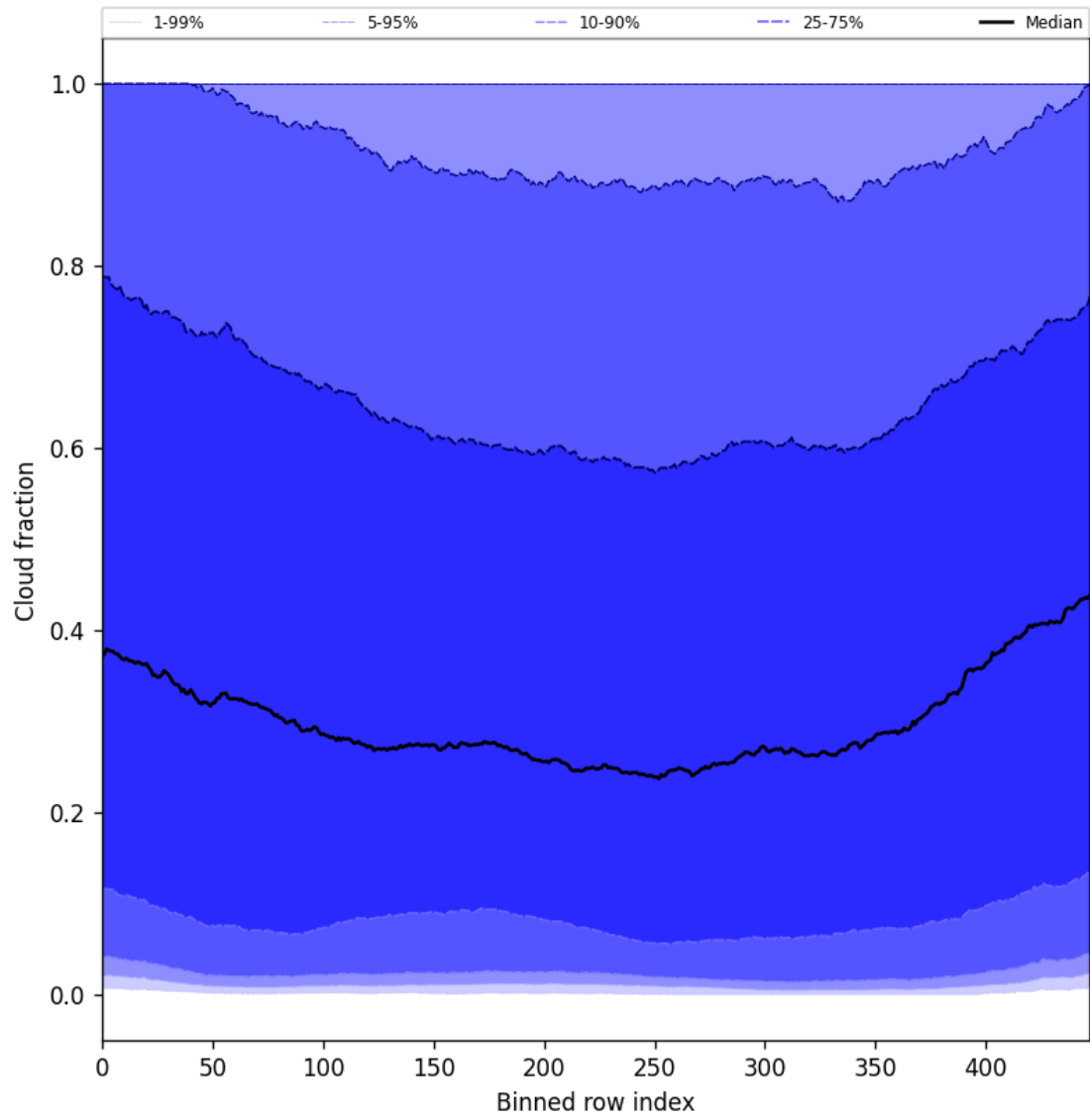
Figure 49: Along track statistics of “Cloud fraction” for 2025-07-29 to 2025-07-31
