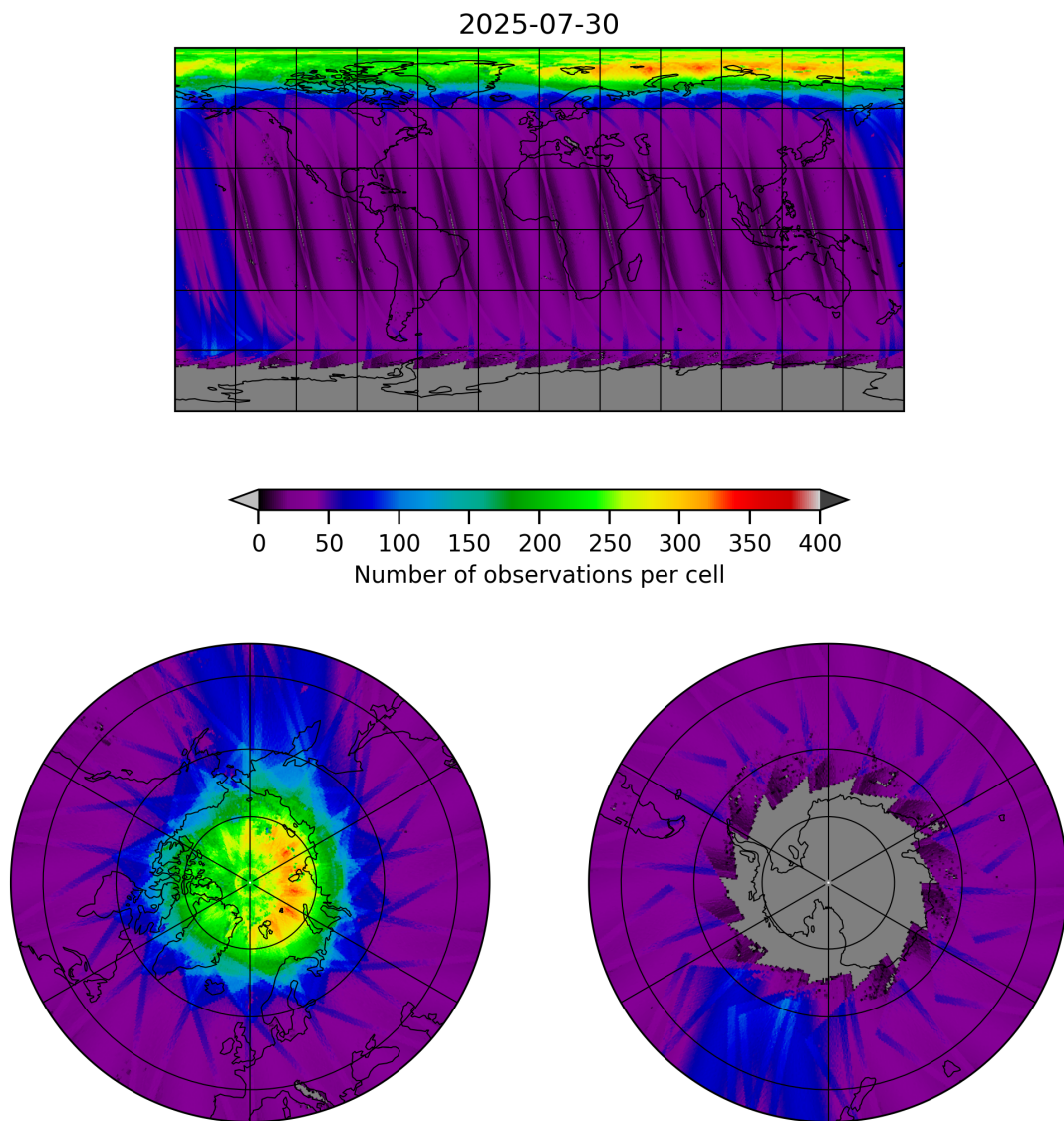
Figure 11: Map of the number of observations for 2025-07-29 to 2025-07-31
