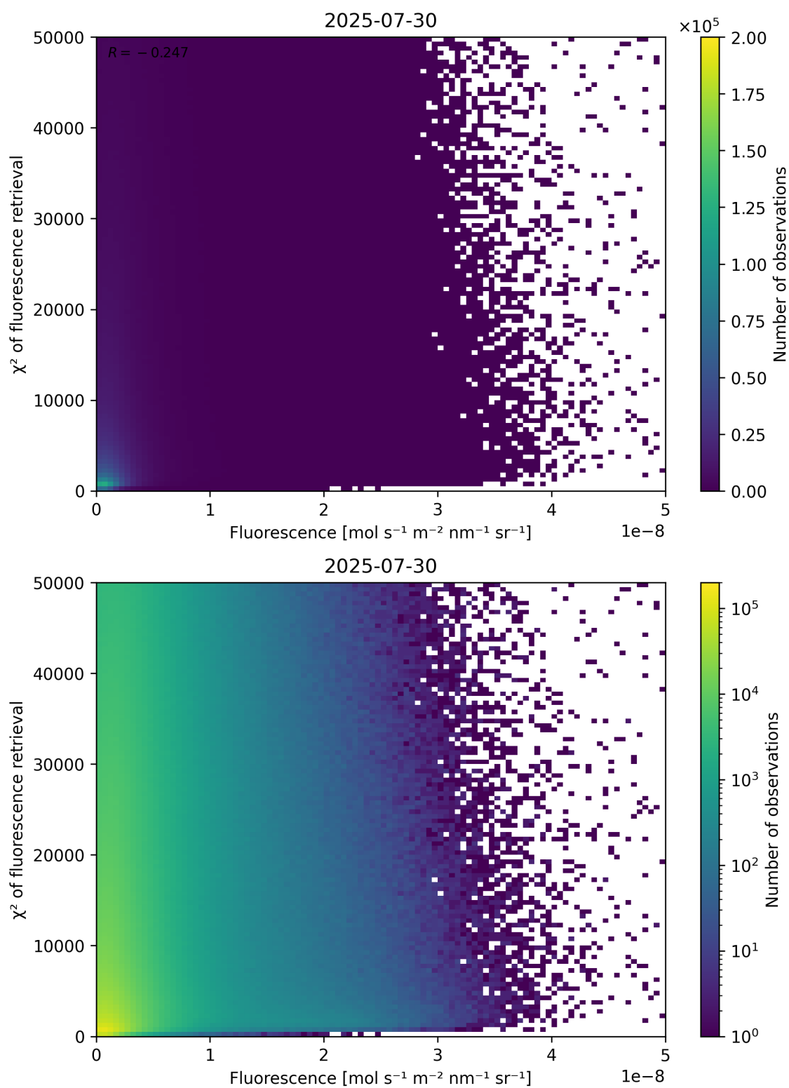
Figure 85: Scatter density plot of “Fluorescence” against “ \chi^2 of fluorescence retrieval” for 2025-07-29 to 2025-07-31.
