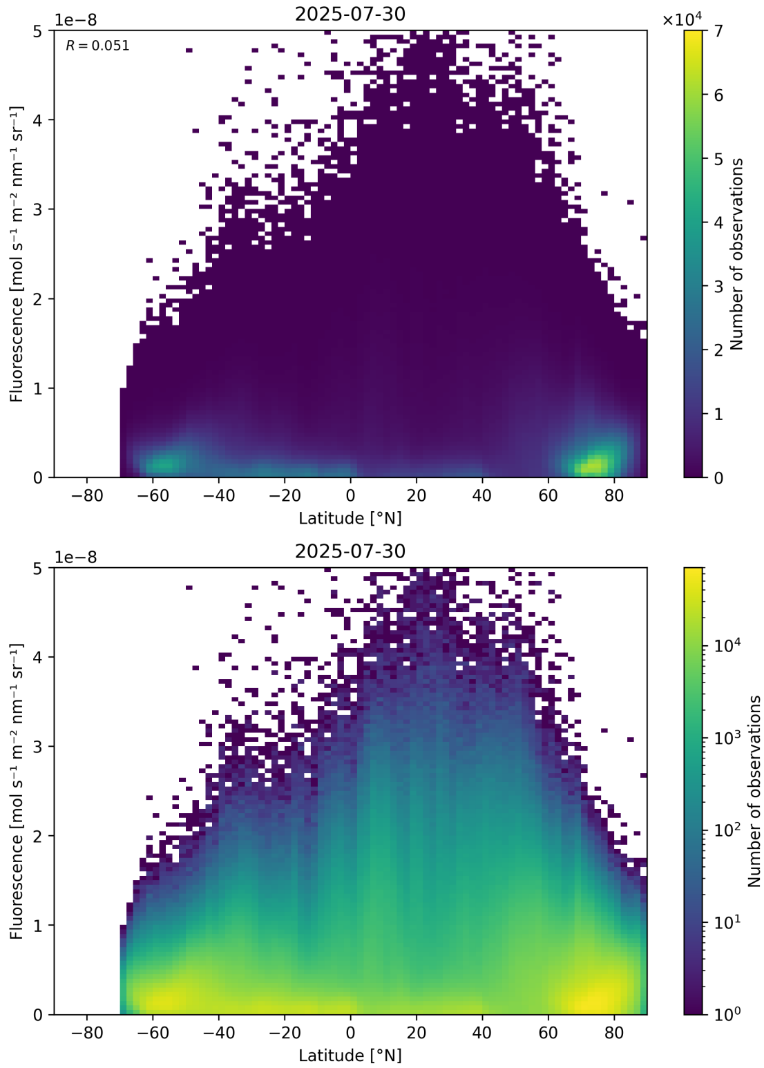
Figure 92: Scatter density plot of “Latitude” against “Fluorescence” for 2025-07-29 to 2025-07-31.
