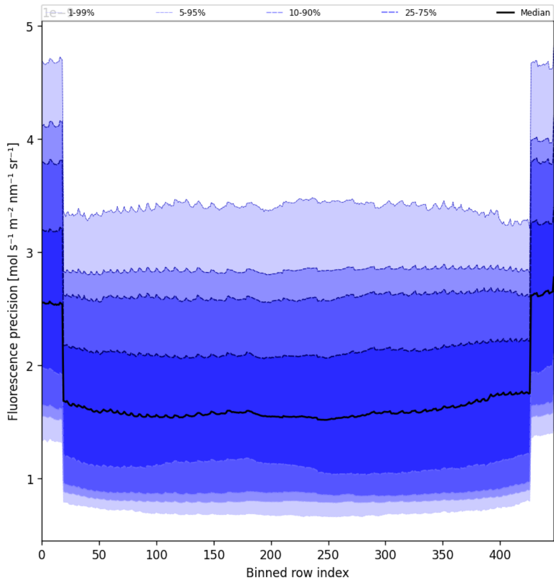
Figure 58: Along track statistics of “Fluorescence precision” for 2025-07-29 to 2025-07-31
