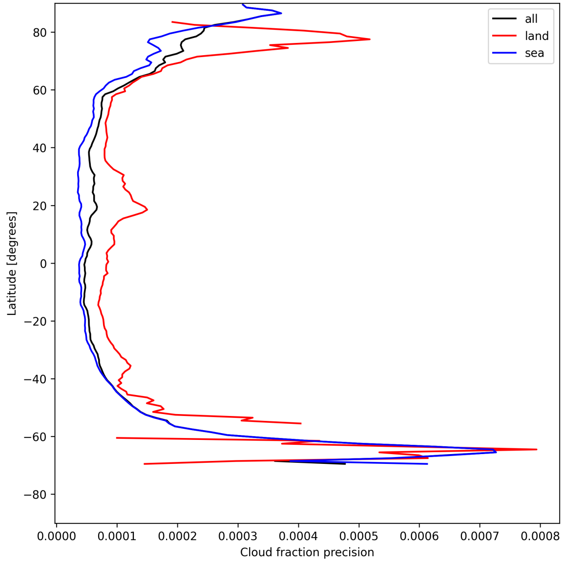
Figure 16: Zonal average of “Cloud fraction precision” for 2025-07-29 to 2025-07-31.
