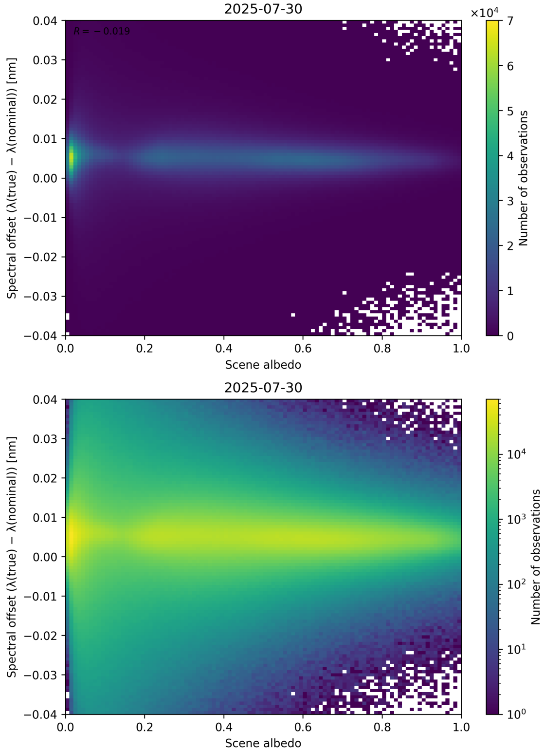
Figure 107: Scatter density plot of “Scene albedo” against “Spectral offset ( \lambda_{\text{true}} - \lambda_{\text{nominal}} )” for 2025-07-29 to 2025-07-31.
