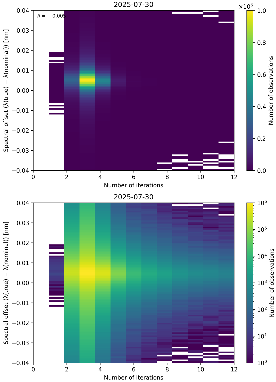
Figure 100: Scatter density plot of “Number of iterations” against “Spectral offset ( \lambda_{\text{true}} - \lambda_{\text{nominal}} )” for 2025-07-29 to 2025-07-31.
