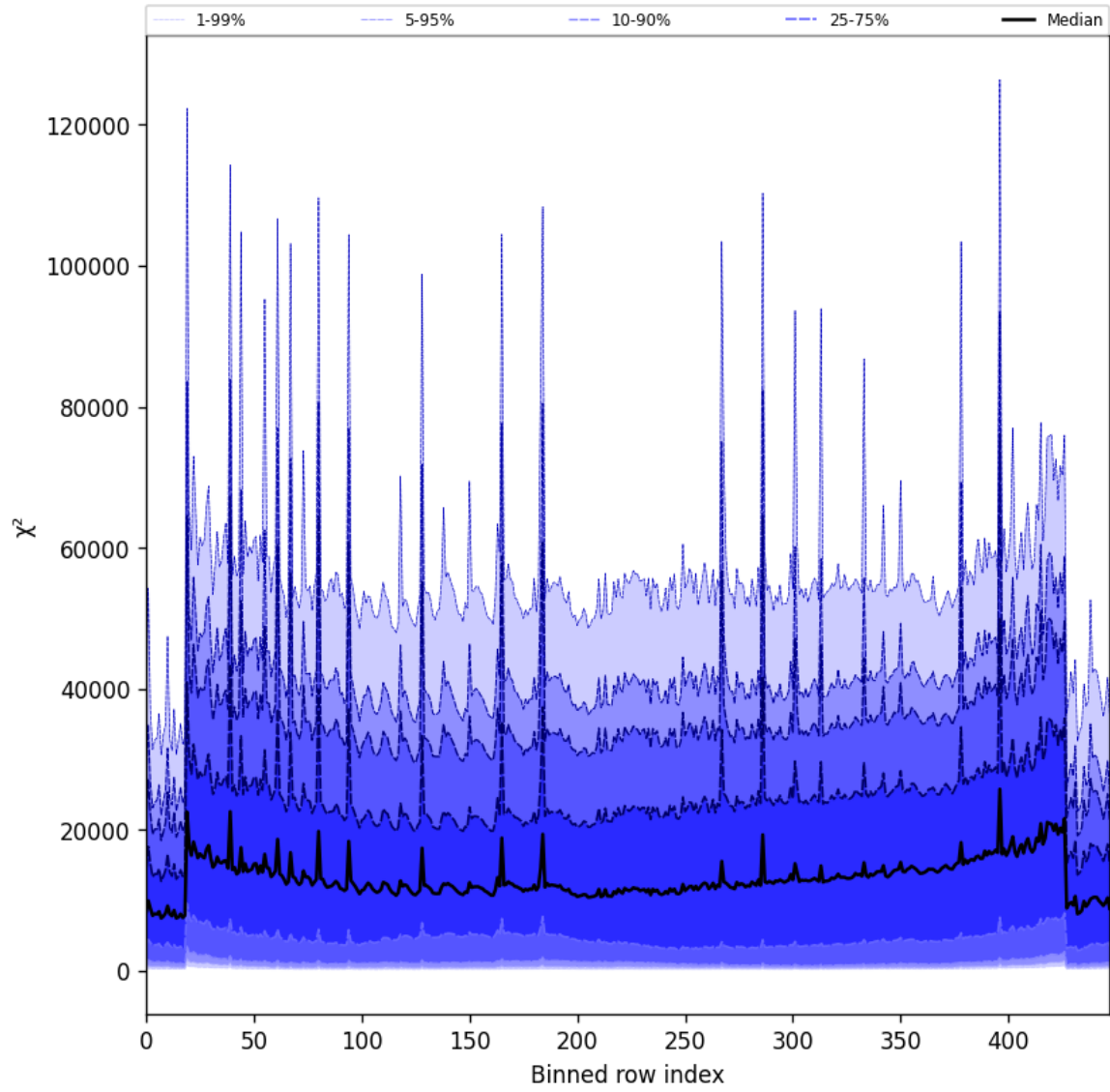
Figure 55: Along track statistics of “ \chi^2 ” for 2025-07-29 to 2025-07-31
