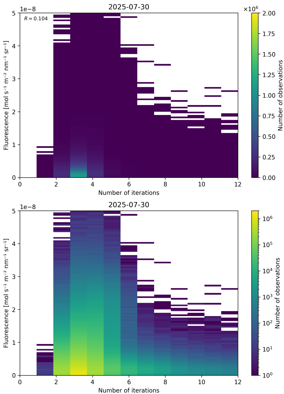
Figure 98: Scatter density plot of “Number of iterations” against “Fluorescence” for 2025-07-29 to 2025-07-31.
