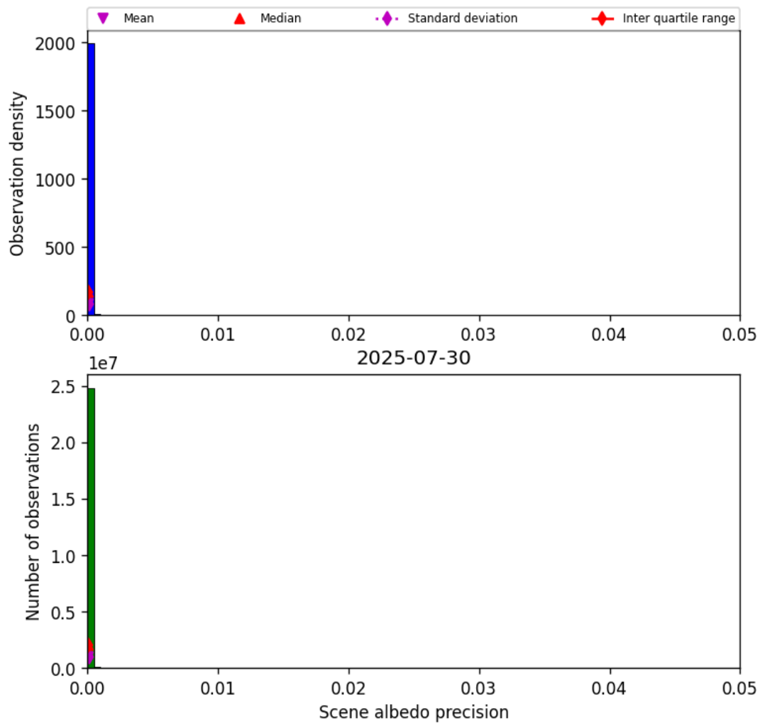
Figure 35: Histogram of “Scene albedo precision” for 2025-07-29 to 2025-07-31
