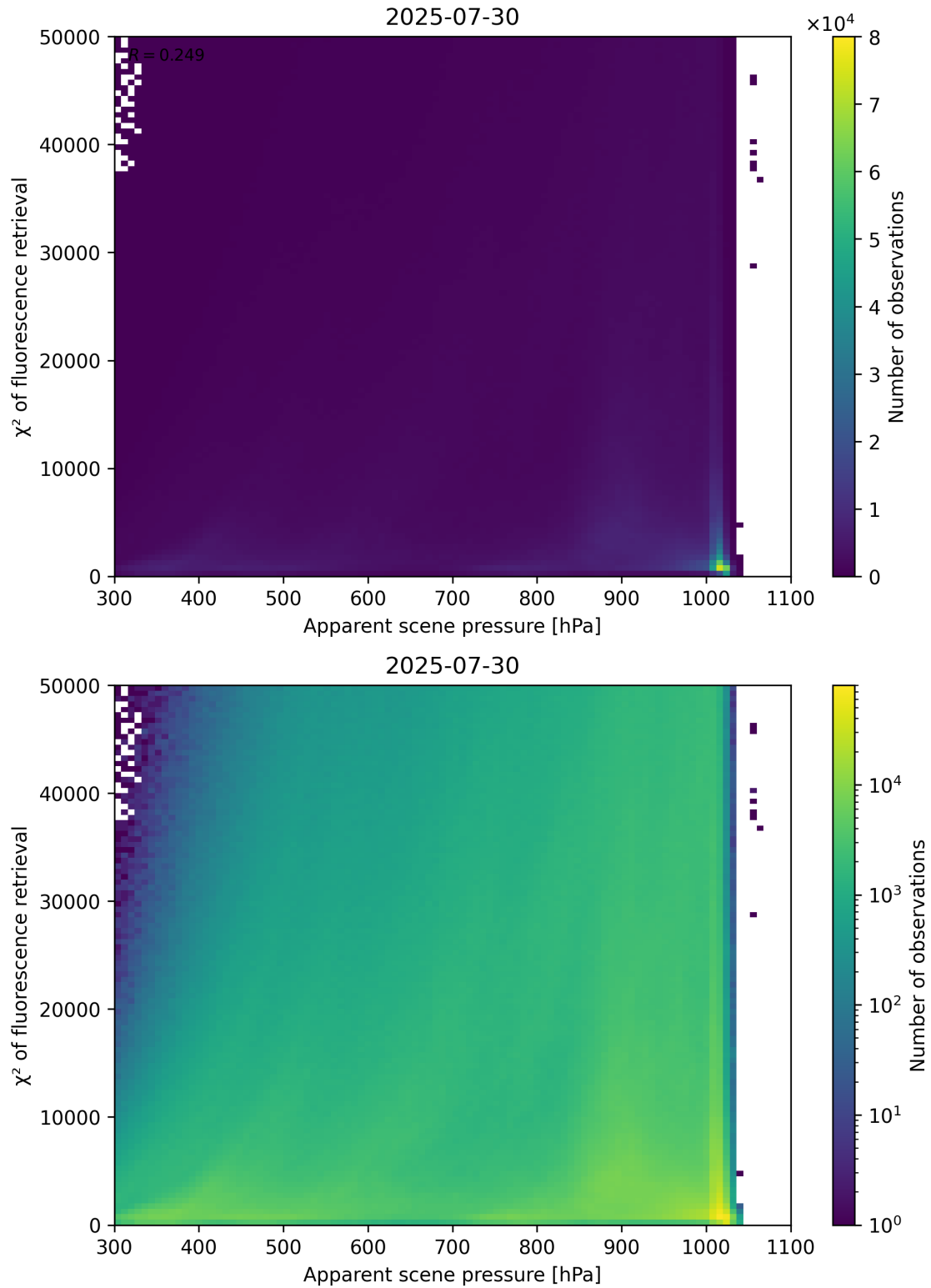
Figure 63: Scatter density plot of “Apparent scene pressure” against “ \chi^2 of fluorescence retrieval” for 2025-07-29 to 2025-07-31.
