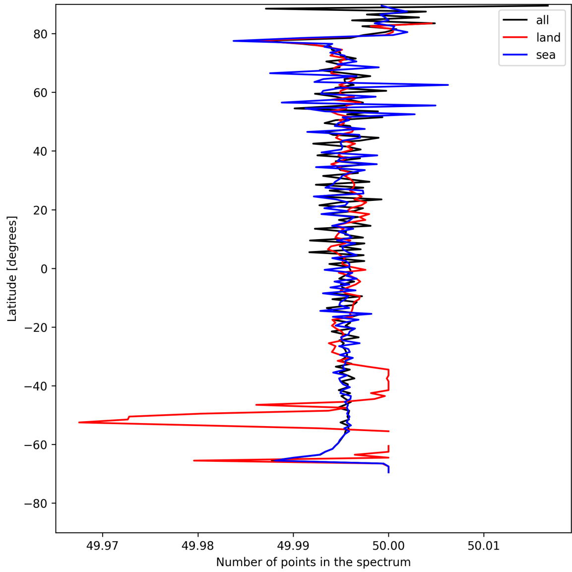
Figure 27: Zonal average of “Number of points in the spectrum” for 2025-07-29 to 2025-07-31.
