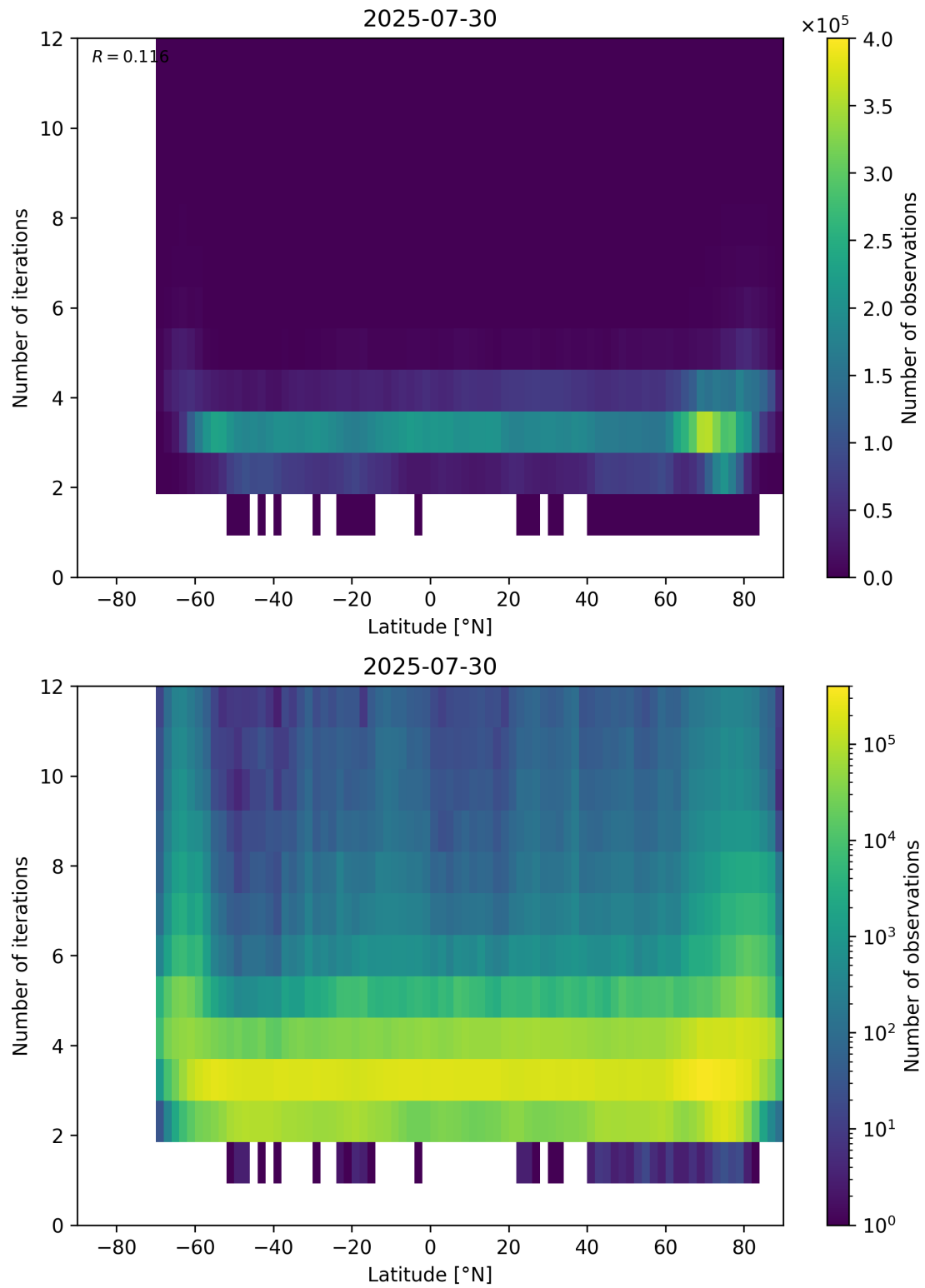
Figure 93: Scatter density plot of “Latitude” against “Number of iterations” for 2025-07-29 to 2025-07-31.
