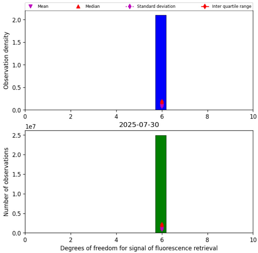
Figure 43: Histogram of "Degrees of freedom for signal of fluorescence retrieval" for 2025-07-29 to 2025-07-31
