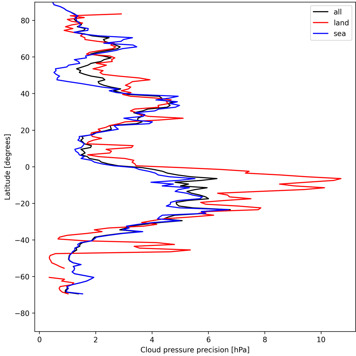
Figure 14: Zonal average of “Cloud pressure precision” for 2025-07-29 to 2025-07-31.
