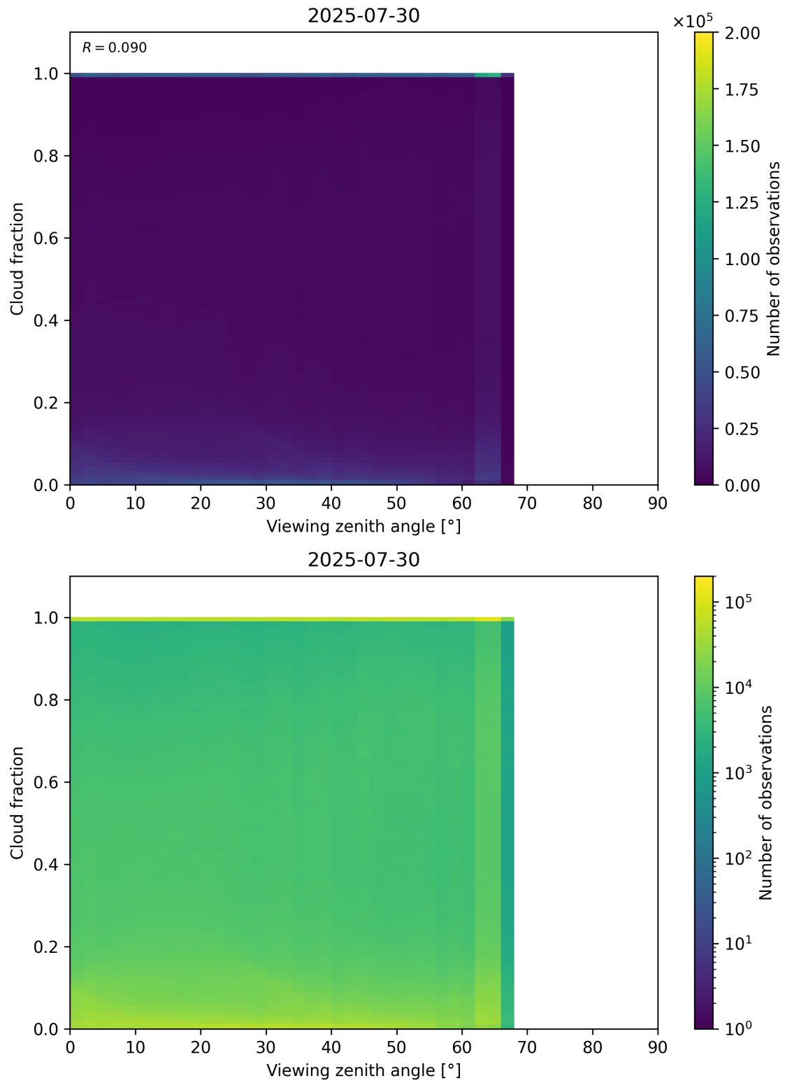
Figure 120: Scatter density plot of “Viewing zenith angle” against “Cloud fraction” for 2025-07-29 to 2025-07-31.
