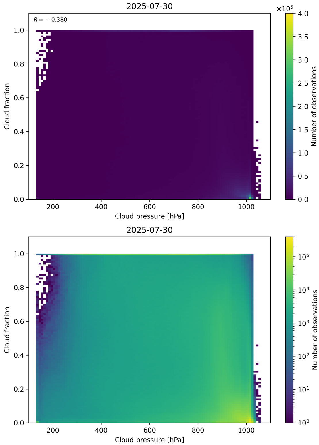
Figure 79: Scatter density plot of “Cloud pressure” against “Cloud fraction” for 2025-07-29 to 2025-07-31.
