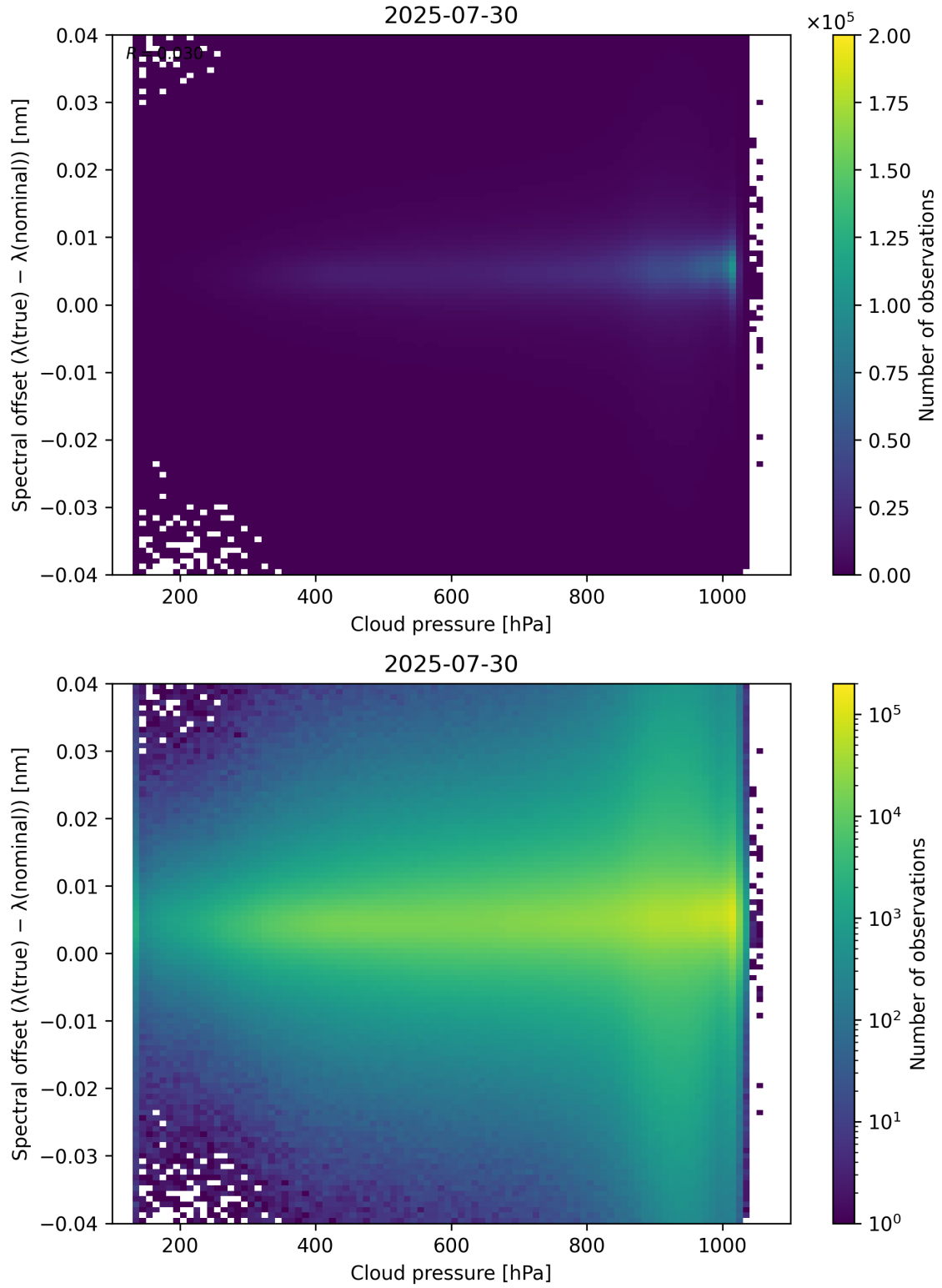
Figure 84: Scatter density plot of “Cloud pressure” against “Spectral offset ( \lambda_{\text{true}} - \lambda_{\text{nominal}} )” for 2025-07-29 to 2025-07-31.
