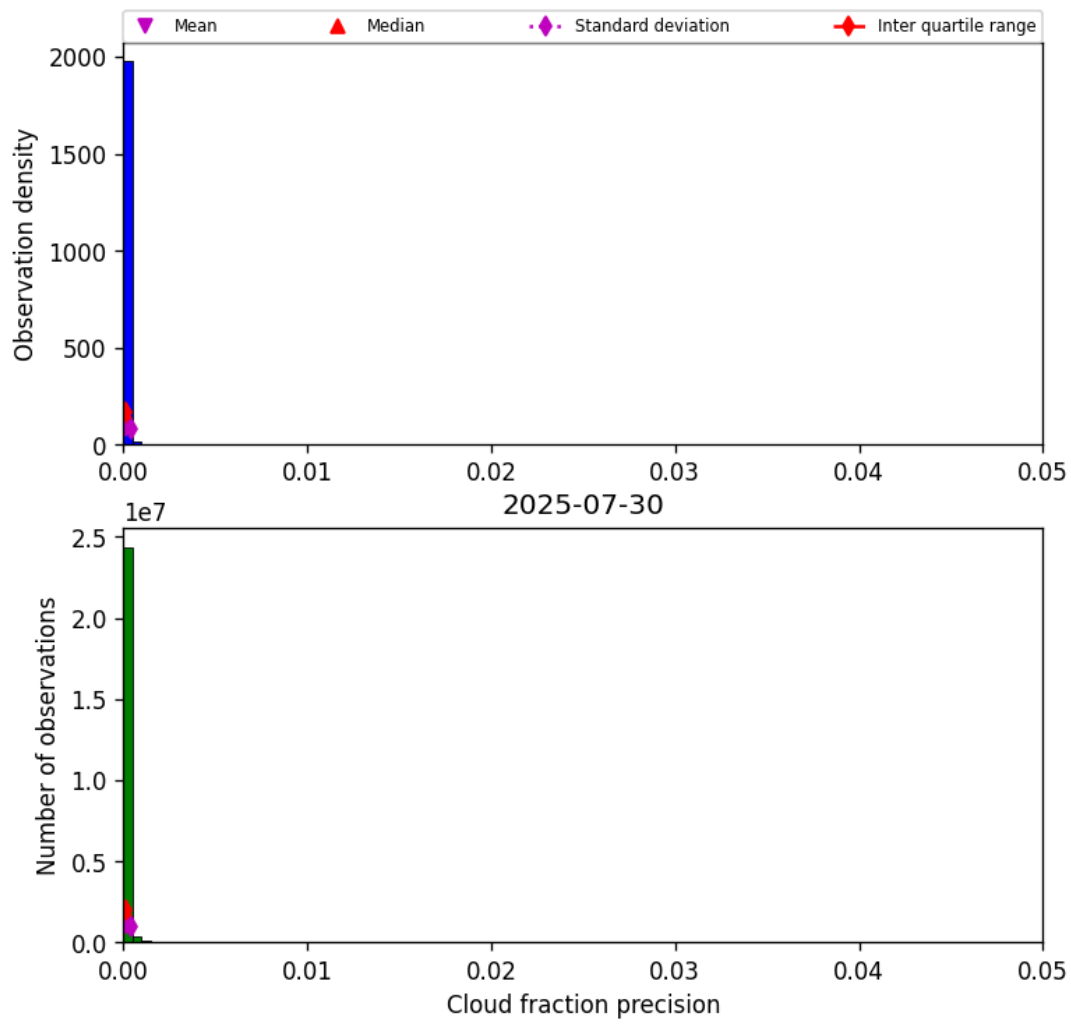
Figure 33: Histogram of “Cloud fraction precision” for 2025-07-29 to 2025-07-31
