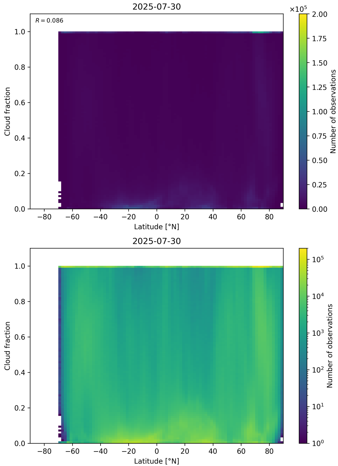
Figure 90: Scatter density plot of “Latitude” against “Cloud fraction” for 2025-07-29 to 2025-07-31.
