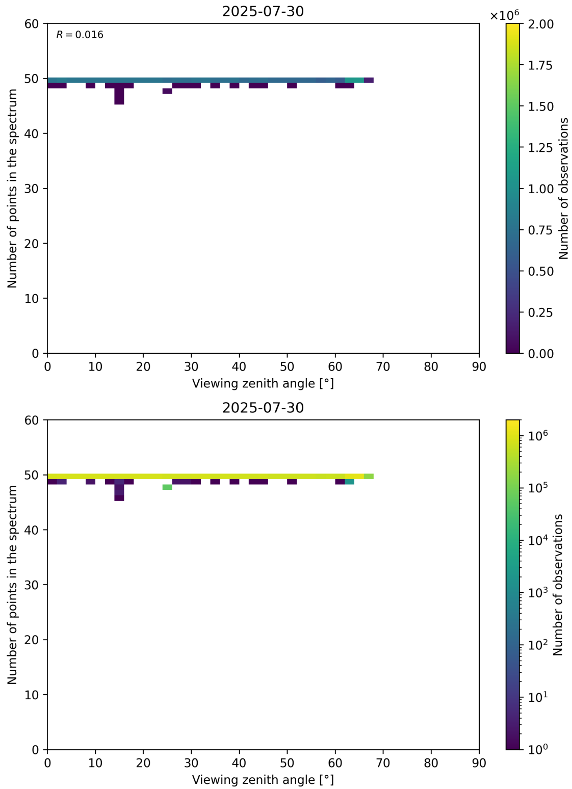
Figure 125: Scatter density plot of “Viewing zenith angle” against “Number of points in the spectrum” for 2025-07-29 to 2025-07-31.
