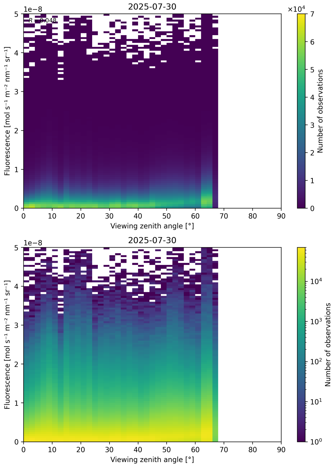
Figure 122: Scatter density plot of “Viewing zenith angle” against “Fluorescence” for 2025-07-29 to 2025-07-31.
