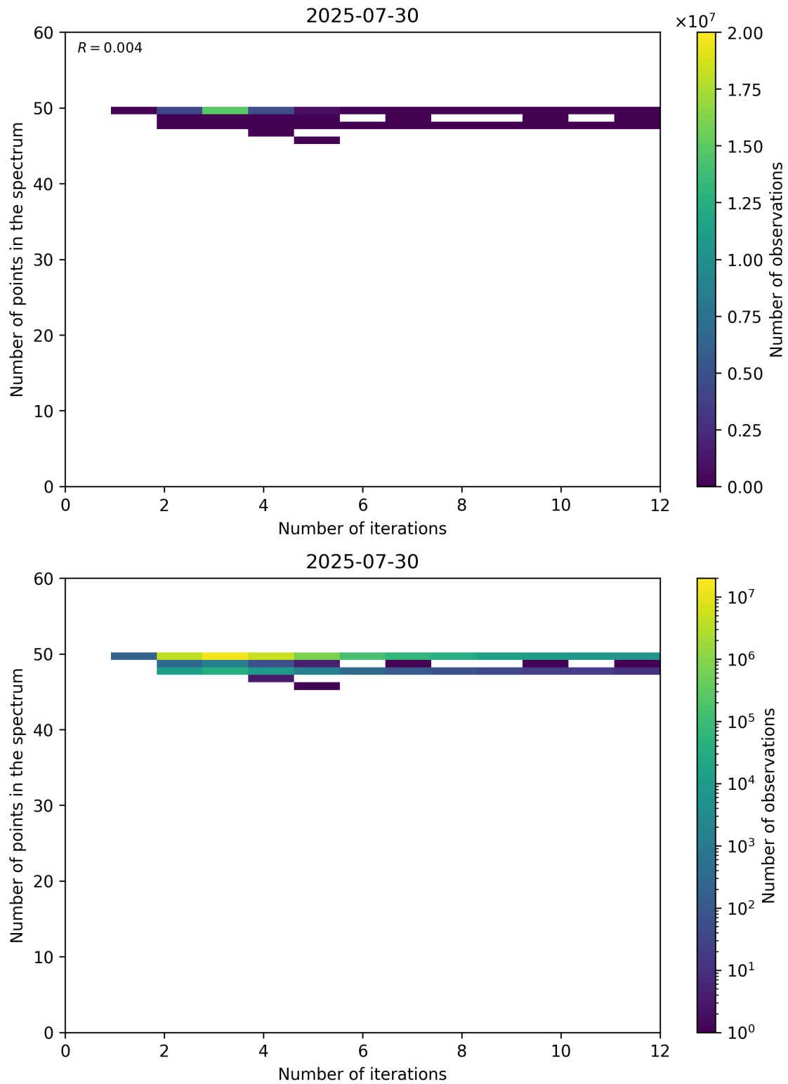
Figure 99: Scatter density plot of “Number of iterations” against “Number of points in the spectrum” for 2025-07-29 to 2025-07-31.
