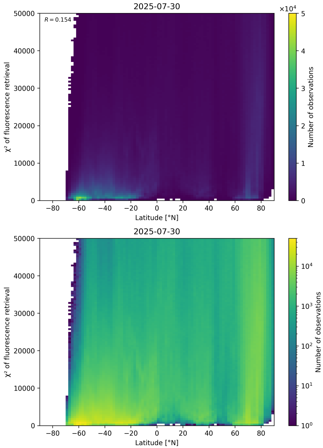
Figure 89: Scatter density plot of “Latitude” against “ \chi^2 of fluorescence retrieval” for 2025-07-29 to 2025-07-31.
