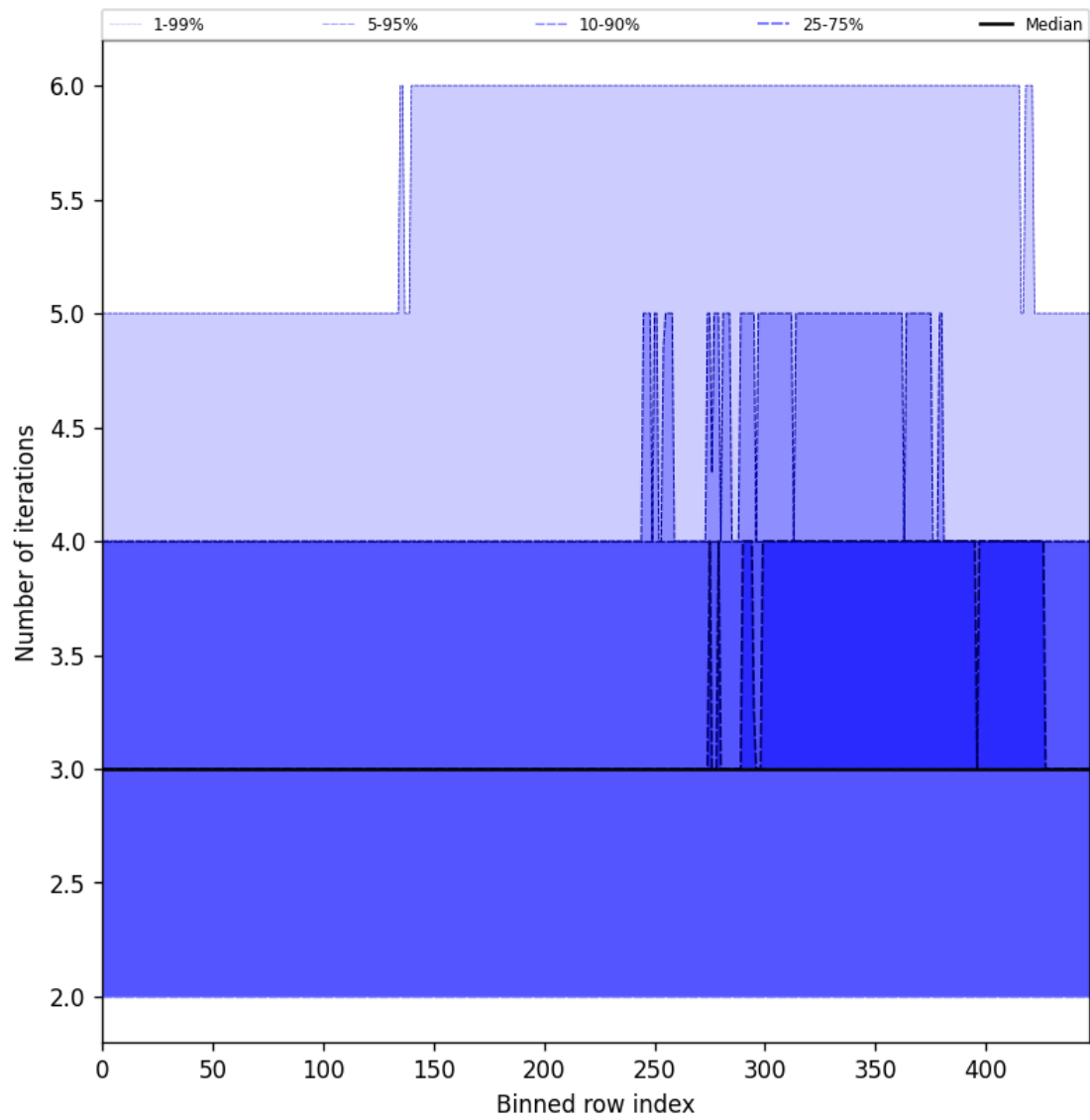
Figure 56: Along track statistics of “Number of iterations” for 2025-07-29 to 2025-07-31
