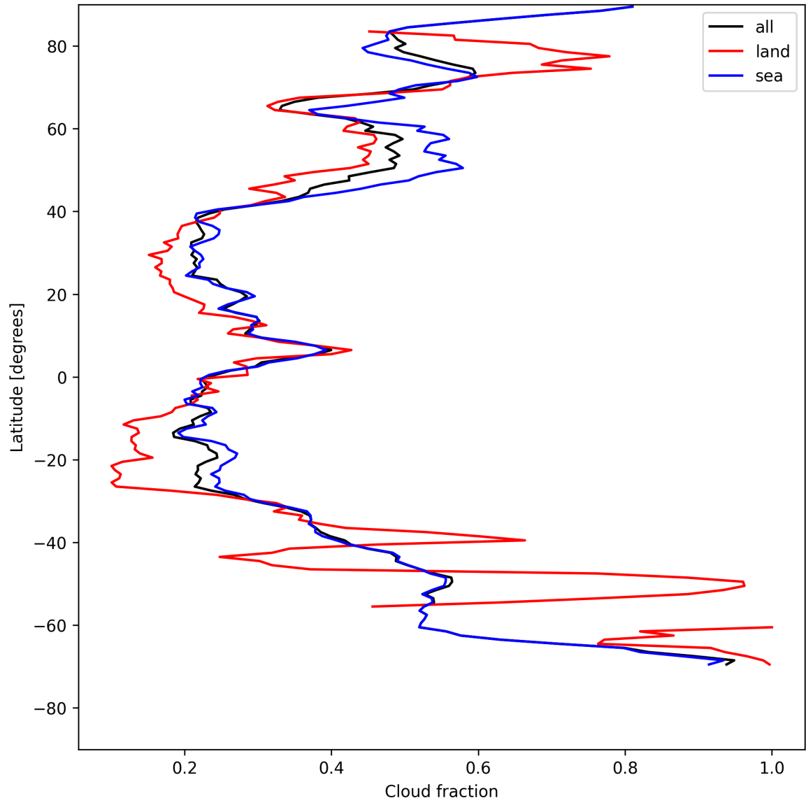
Figure 15: Zonal average of “Cloud fraction” for 2025-07-29 to 2025-07-31.
