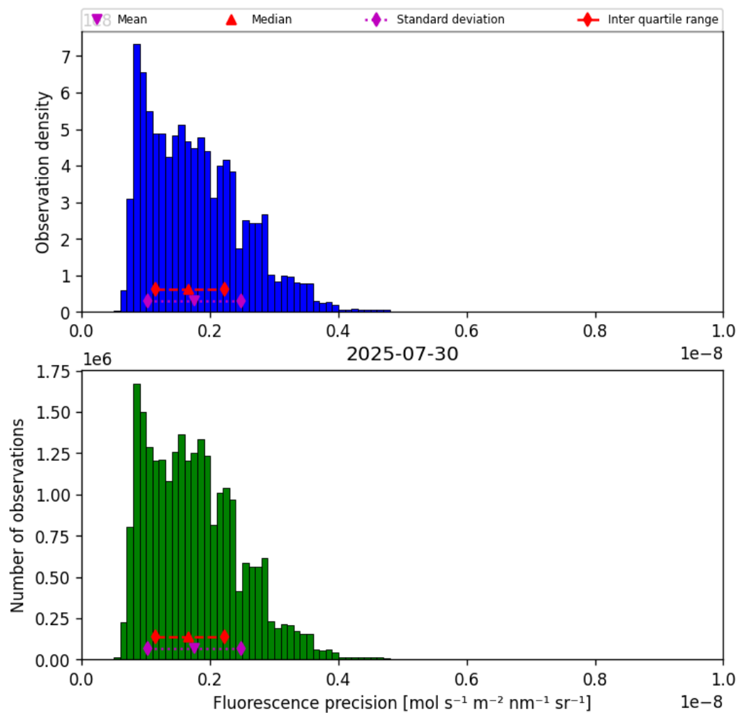
Figure 41: Histogram of “Fluorescence precision” for 2025-07-29 to 2025-07-31
