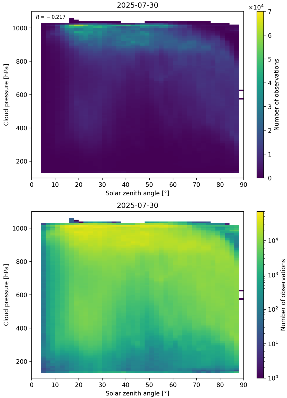
Figure 111: Scatter density plot of “Solar zenith angle” against “Cloud pressure” for 2025-07-29 to 2025-07-31.
