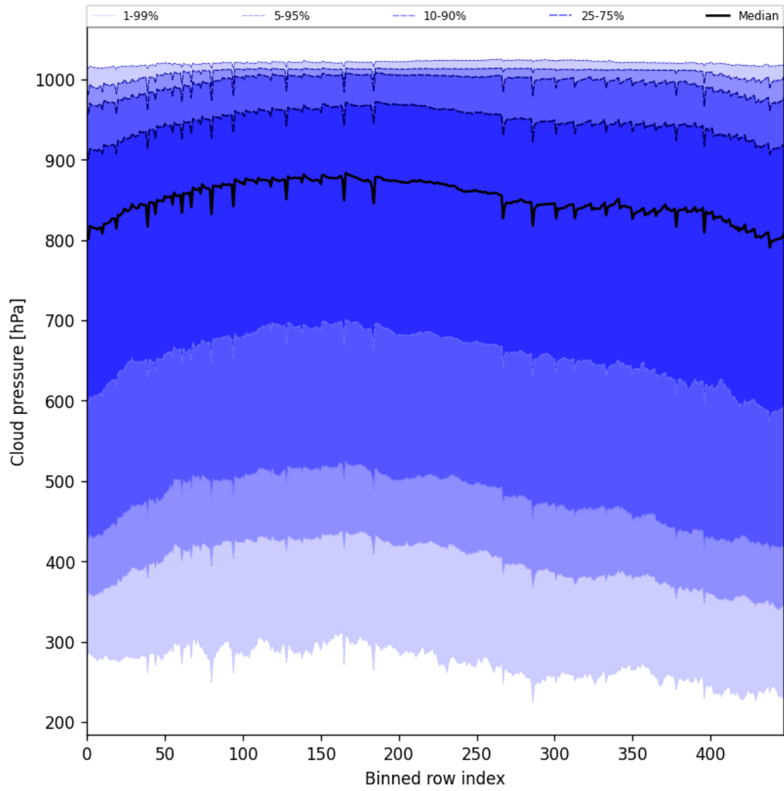
Figure 47: Along track statistics of “Cloud pressure” for 2025-07-31 to 2025-08-02
