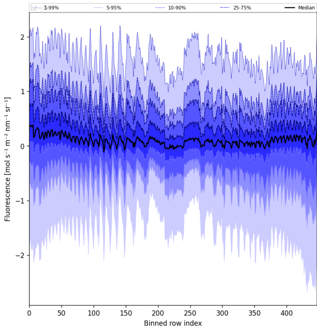
Figure 57: Along track statistics of “Fluorescence” for 2025-07-31 to 2025-08-02
