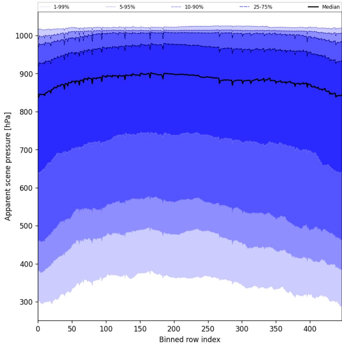
Figure 53: Along track statistics of “Apparent scene pressure” for 2025-07-31 to 2025-08-02
