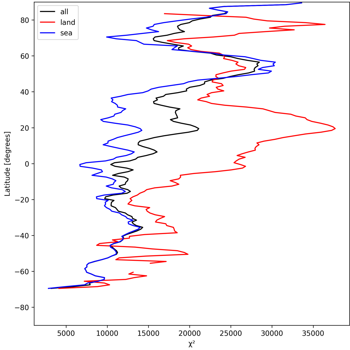
Figure 21: Zonal average of “ \chi^2 ” for 2025-07-31 to 2025-08-02.
