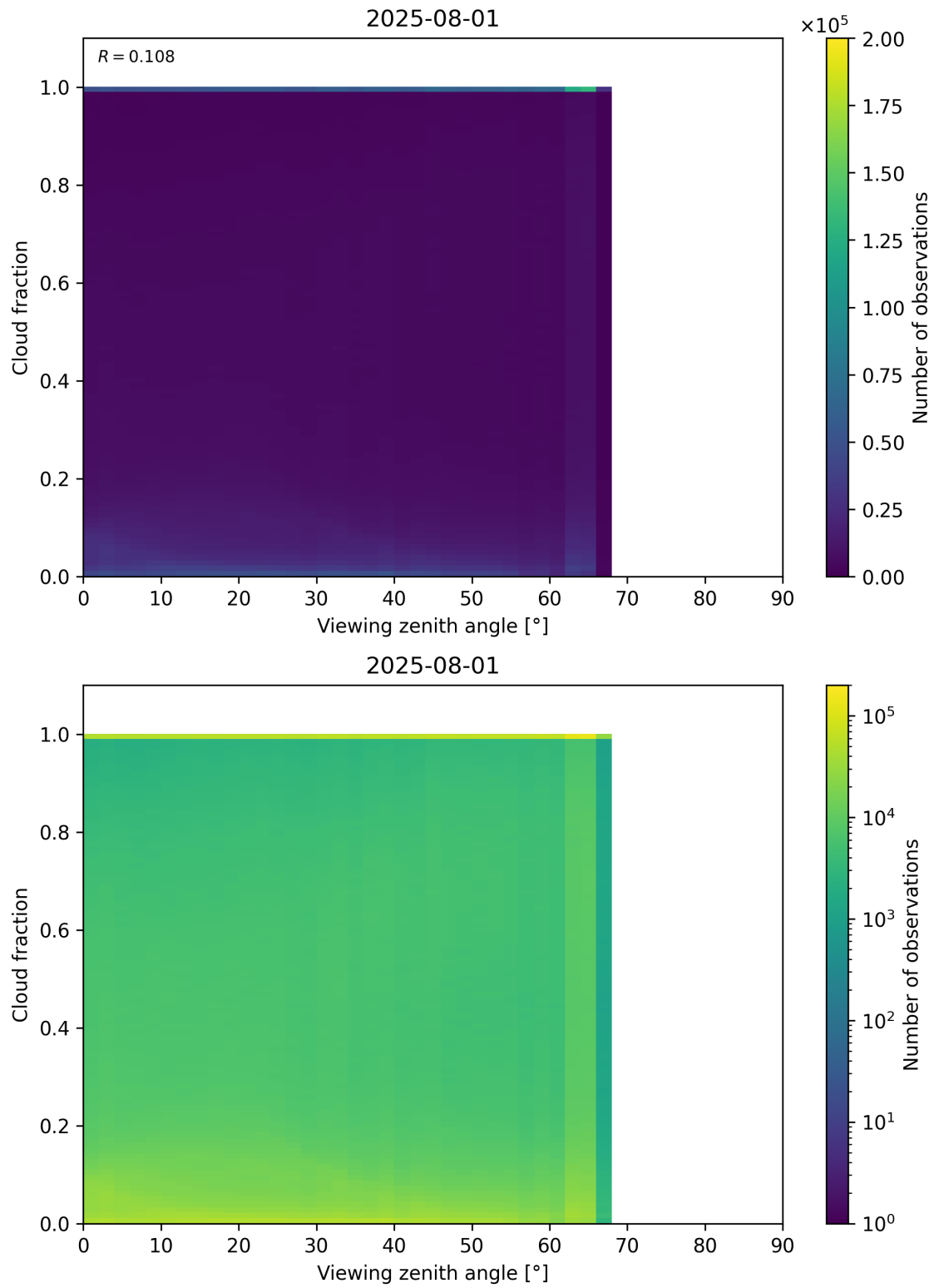
Figure 120: Scatter density plot of “Viewing zenith angle” against “Cloud fraction” for 2025-07-31 to 2025-08-02.
