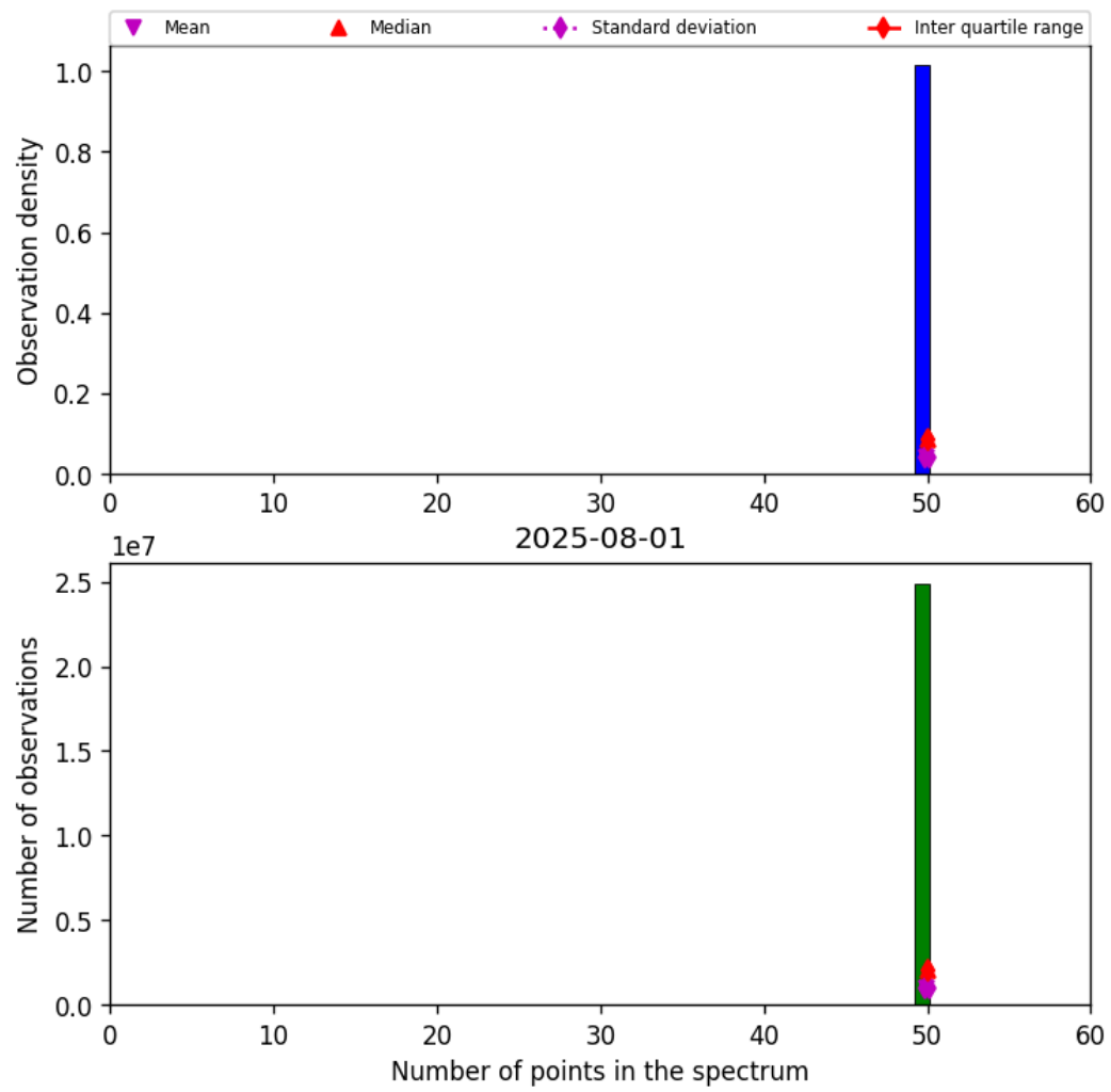
Figure 44: Histogram of "Number of points in the spectrum" for 2025-07-31 to 2025-08-02
