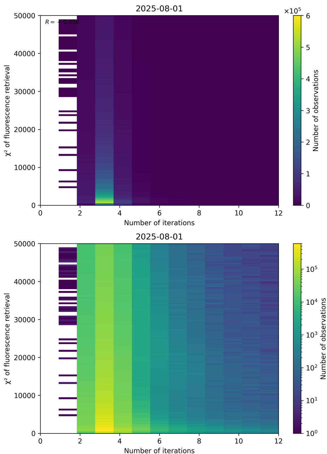
Figure 97: Scatter density plot of “Number of iterations” against “ \chi^2 of fluorescence retrieval” for 2025-07-31 to 2025-08-02.
