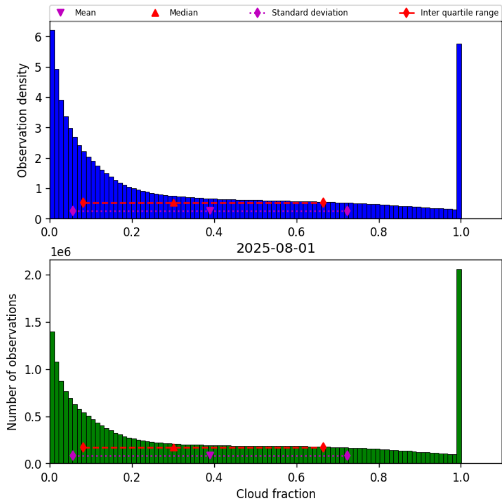
Figure 32: Histogram of “Cloud fraction” for 2025-07-31 to 2025-08-02
