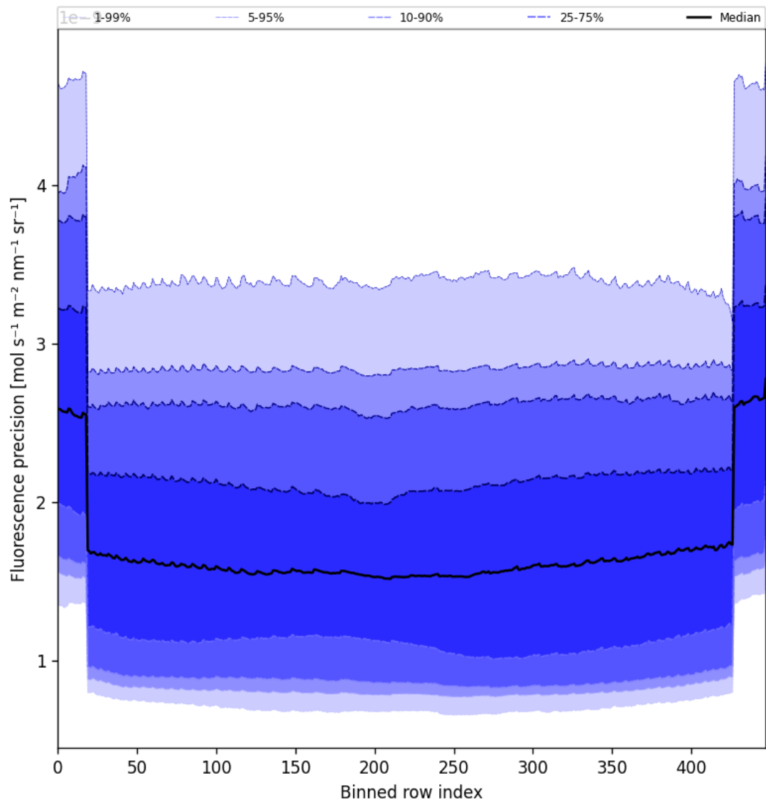
Figure 58: Along track statistics of “Fluorescence precision” for 2025-07-31 to 2025-08-02
