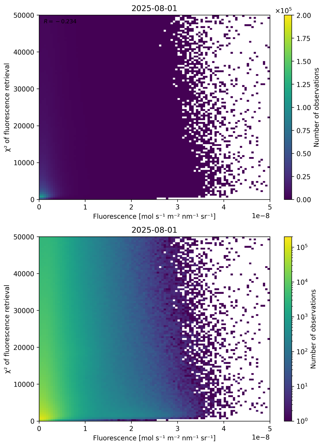
Figure 85: Scatter density plot of “Fluorescence” against “ \chi^2 of fluorescence retrieval” for 2025-07-31 to 2025-08-02.
