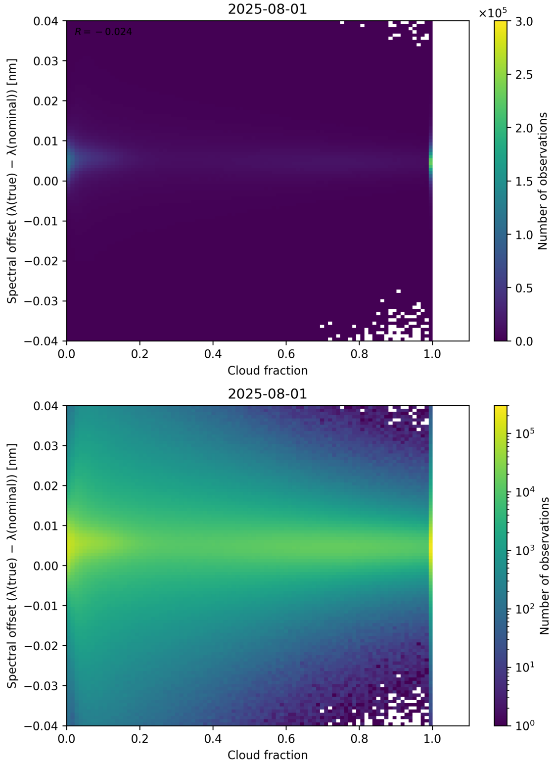
Figure 76: Scatter density plot of “Cloud fraction” against “Spectral offset ( \lambda_{\text{true}} - \lambda_{\text{nominal}} )” for 2025-07-31 to 2025-08-02.
