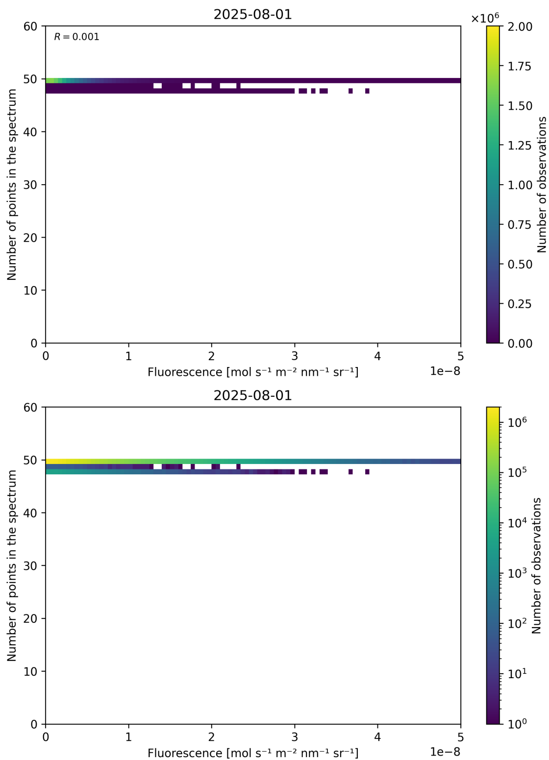
Figure 86: Scatter density plot of “Fluorescence” against “Number of points in the spectrum” for 2025-07-31 to 2025-08-02.
