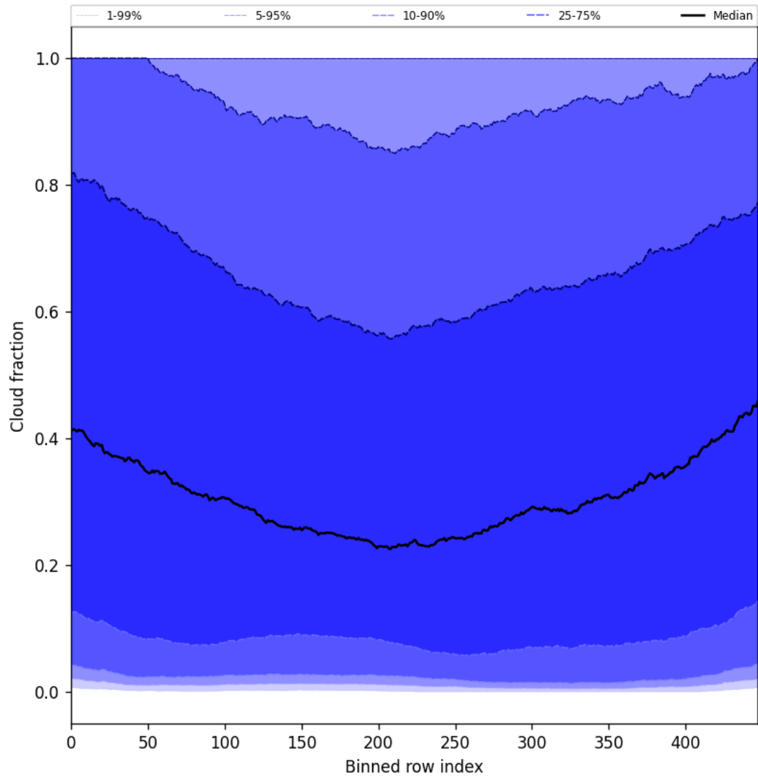
Figure 49: Along track statistics of “Cloud fraction” for 2025-07-31 to 2025-08-02
