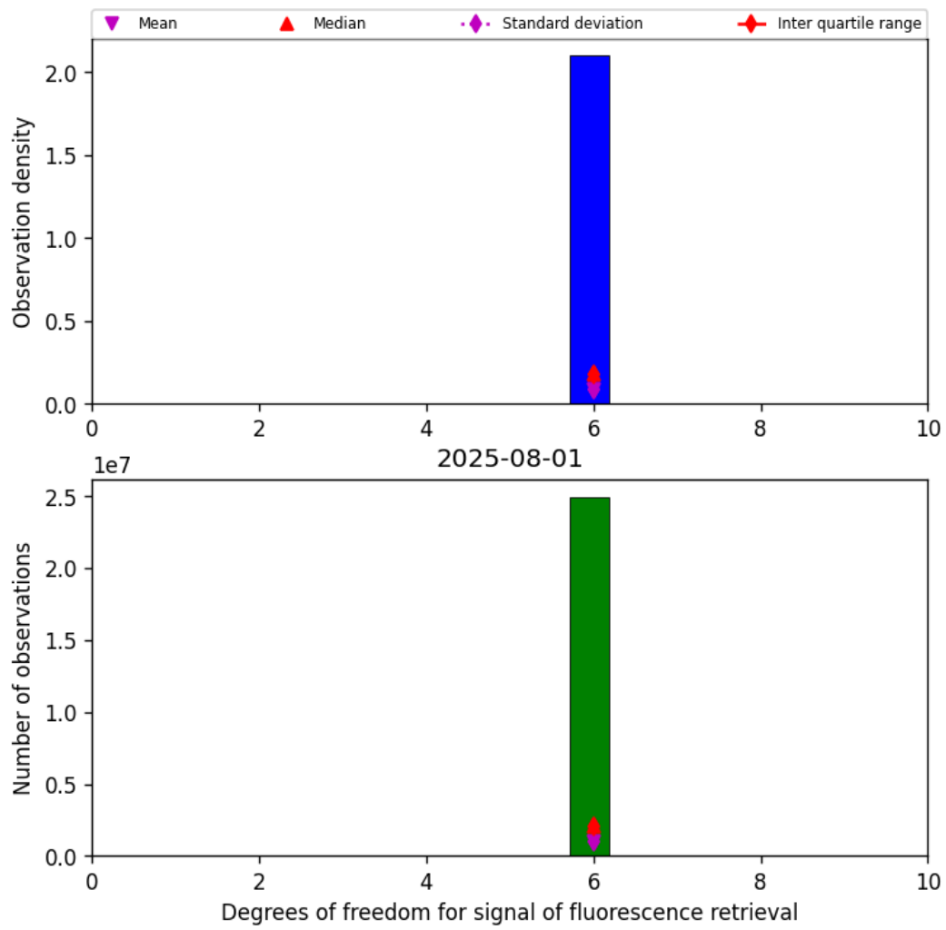
Figure 43: Histogram of "Degrees of freedom for signal of fluorescence retrieval" for 2025-07-31 to 2025-08-02
