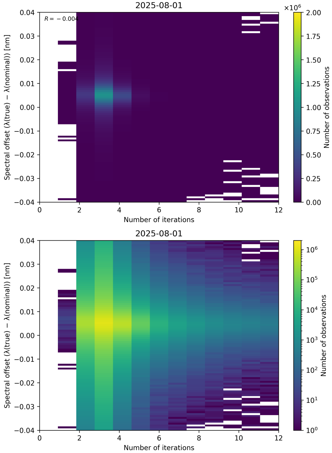
Figure 100: Scatter density plot of “Number of iterations” against “Spectral offset ( \lambda_{\text{true}} - \lambda_{\text{nominal}} )” for 2025-07-31 to 2025-08-02.
