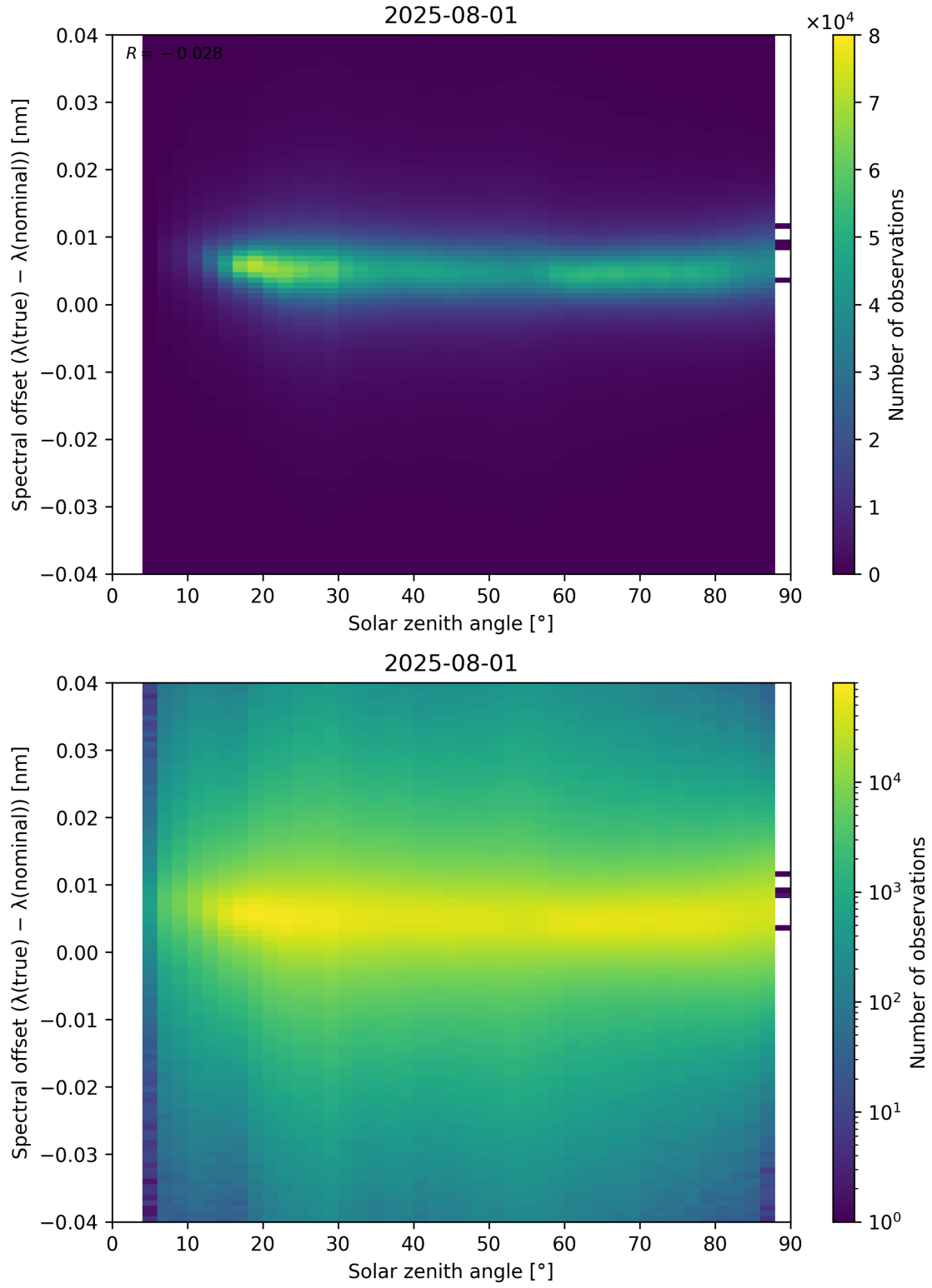
Figure 117: Scatter density plot of “Solar zenith angle” against “Spectral offset ( \lambda_{\text{true}} - \lambda_{\text{nominal}} )” for 2025-07-31 to 2025-08-02.
