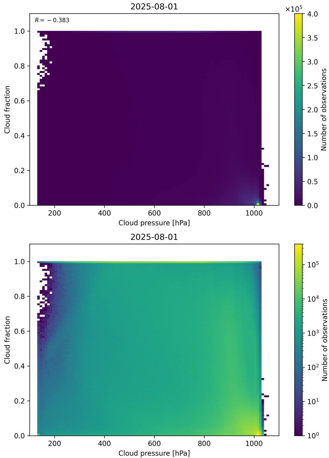
Figure 79: Scatter density plot of “Cloud pressure” against “Cloud fraction” for 2025-07-31 to 2025-08-02.
