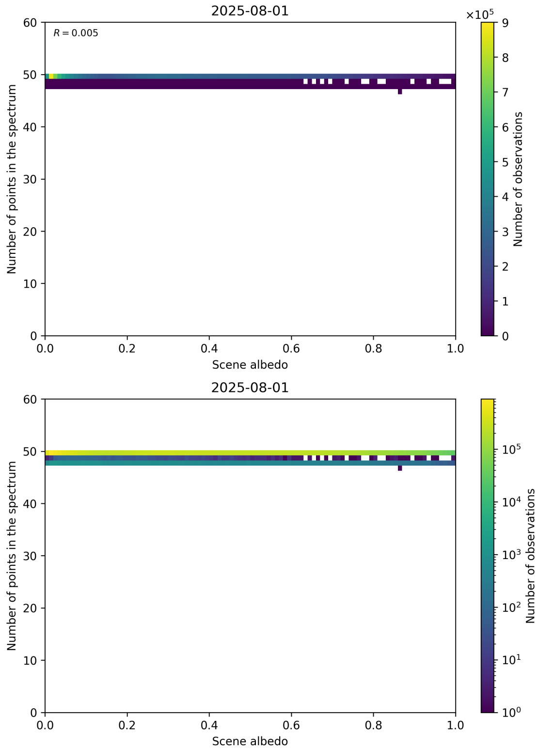
Figure 106: Scatter density plot of “Scene albedo” against “Number of points in the spectrum” for 2025-07-31 to 2025-08-02.
