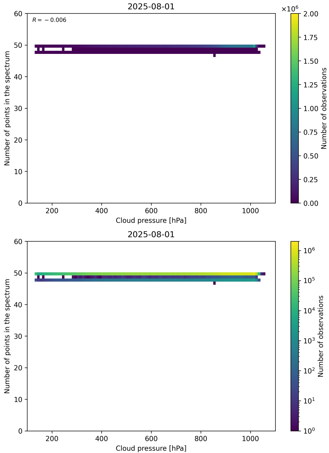
Figure 82: Scatter density plot of “Cloud pressure” against “Number of points in the spectrum” for 2025-07-31 to 2025-08-02.
