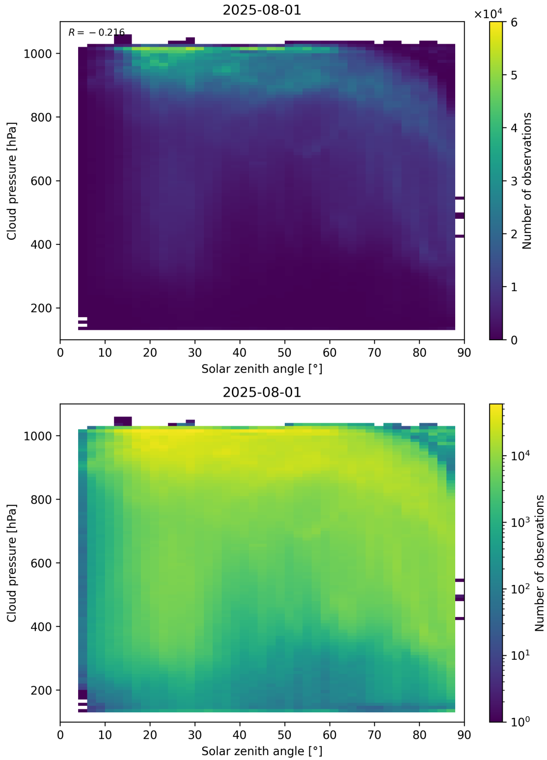
Figure 111: Scatter density plot of “Solar zenith angle” against “Cloud pressure” for 2025-07-31 to 2025-08-02.
