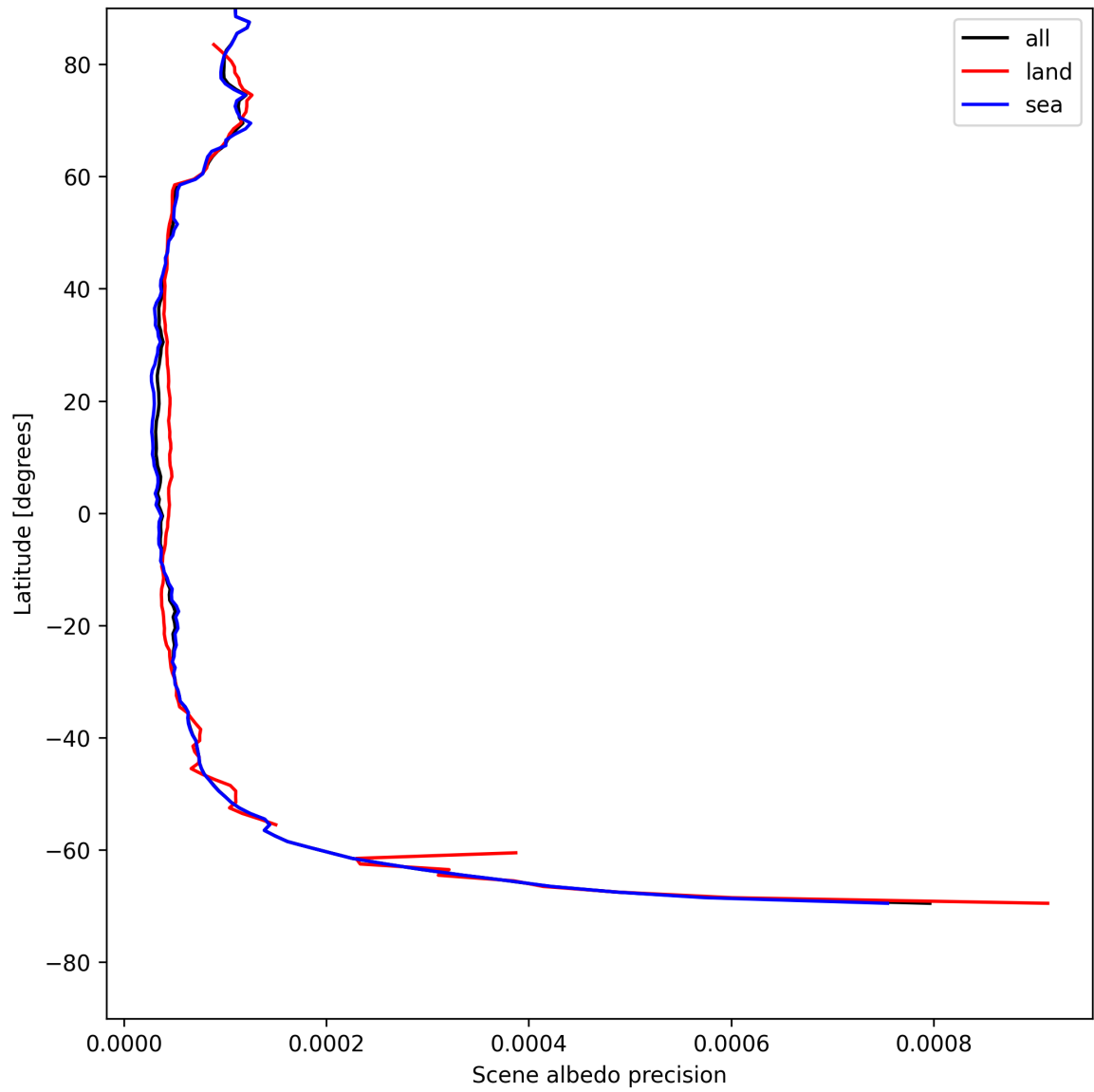
Figure 18: Zonal average of “Scene albedo precision” for 2025-07-31 to 2025-08-02.
