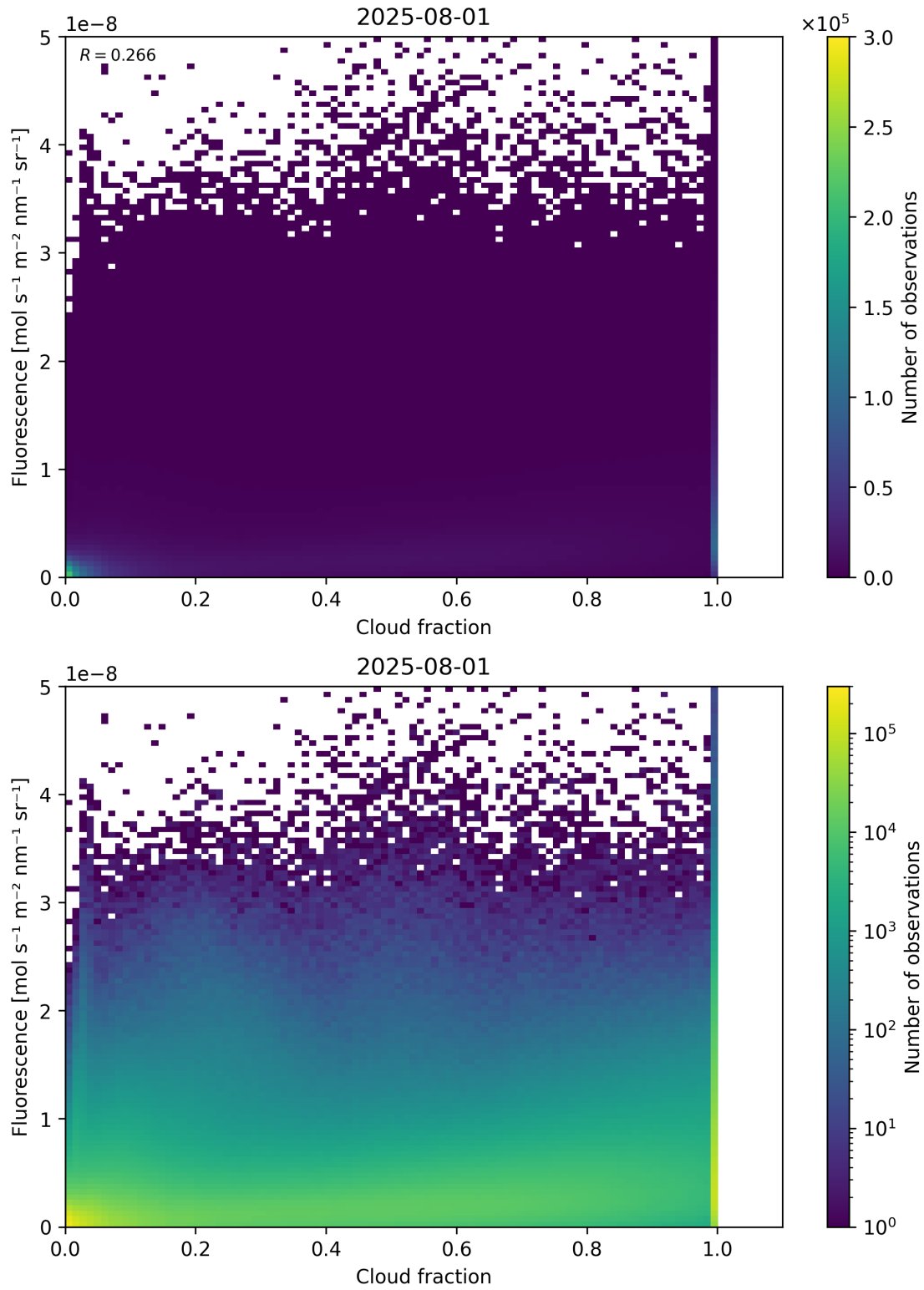
Figure 72: Scatter density plot of “Cloud fraction” against “Fluorescence” for 2025-07-31 to 2025-08-02.
