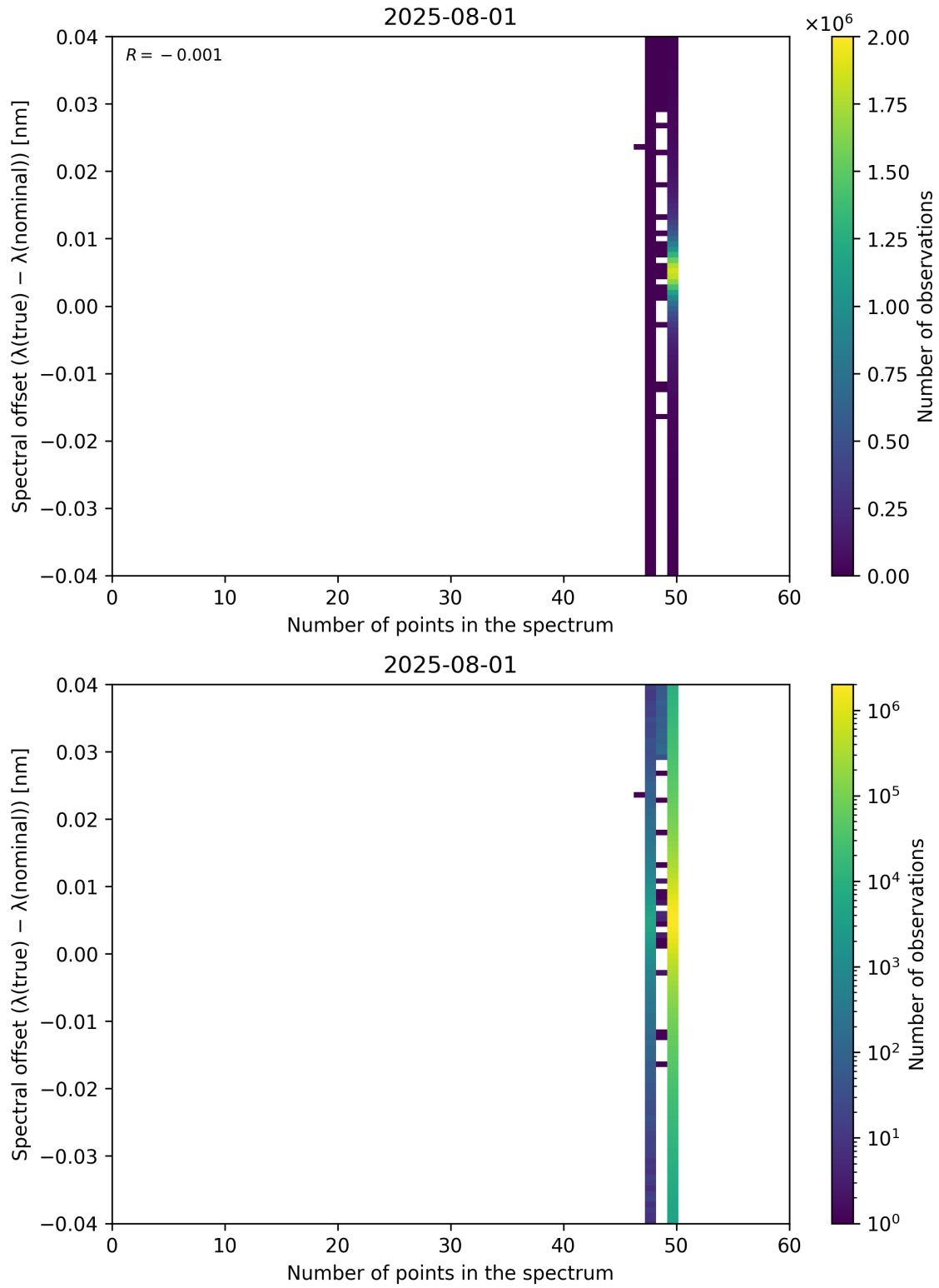
Figure 101: Scatter density plot of “Number of points in the spectrum” against “Spectral offset ( \lambda_{\text{true}} - \lambda_{\text{nominal}} )” for 2025-07-31 to 2025-08-02.
