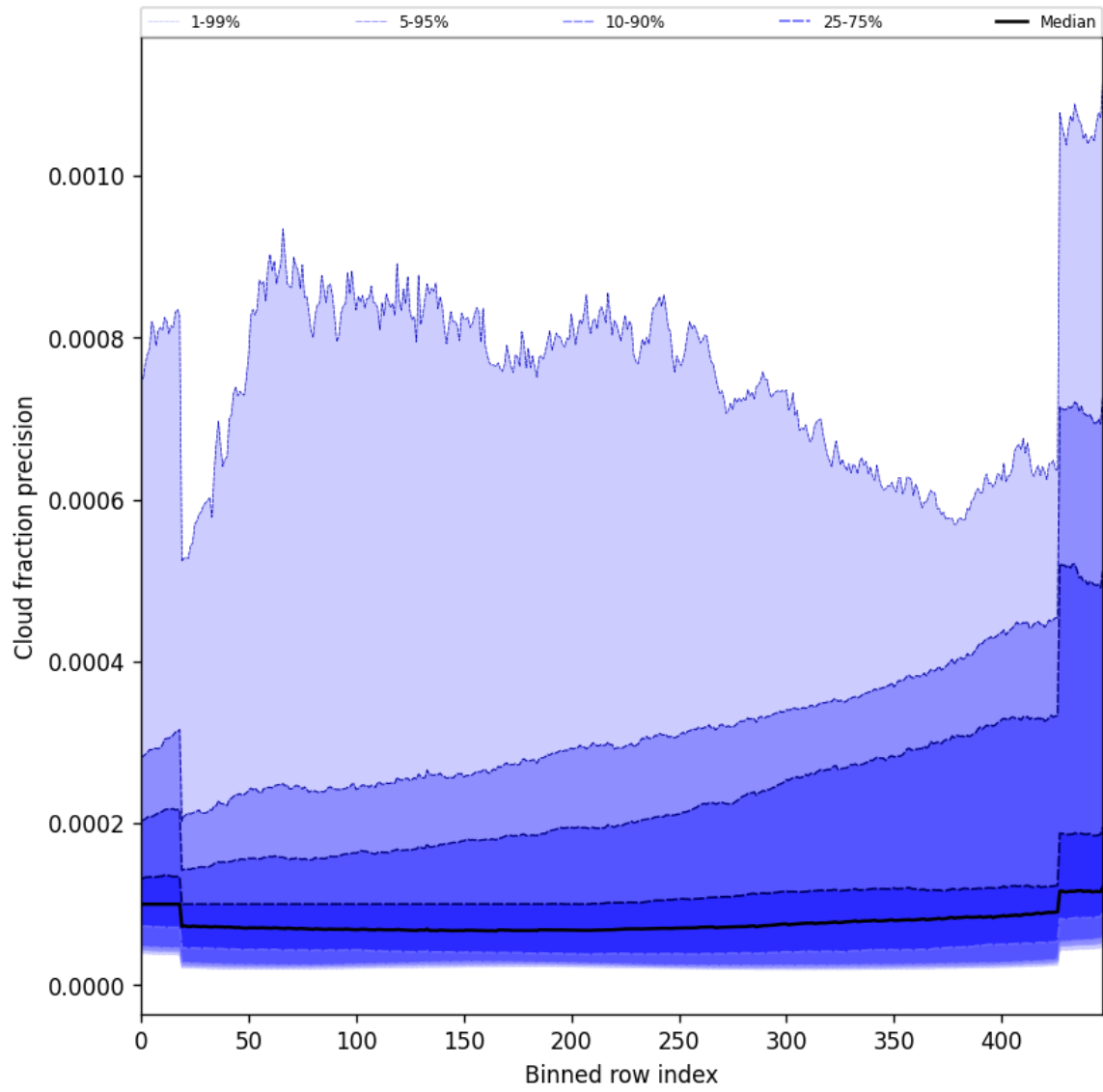
Figure 50: Along track statistics of “Cloud fraction precision” for 2025-07-31 to 2025-08-02
