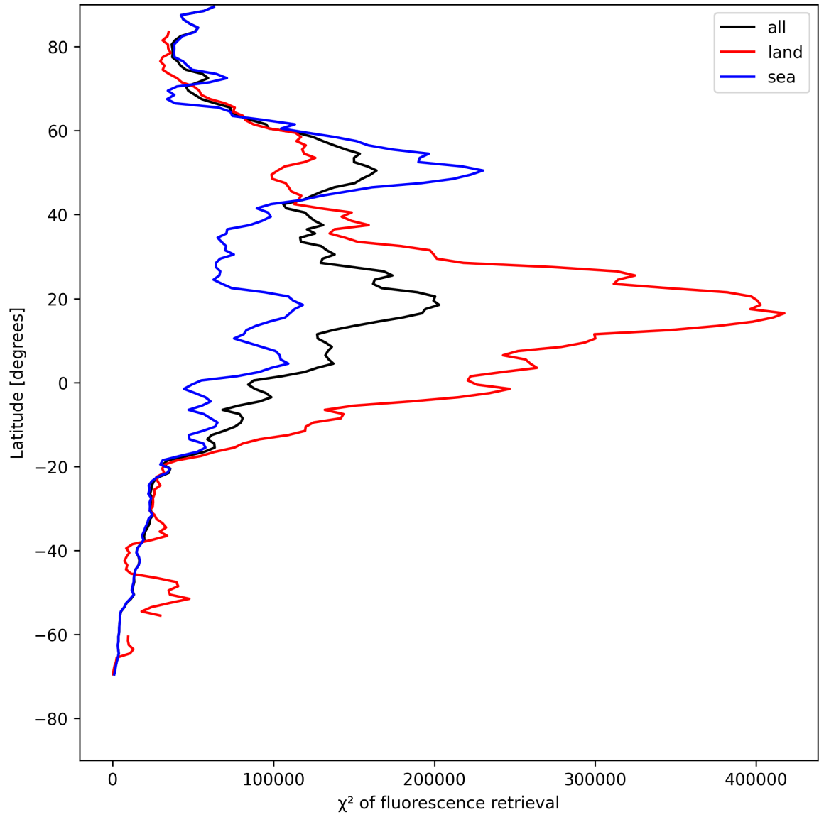
Figure 25: Zonal average of “ \chi^2 of fluorescence retrieval” for 2025-07-31 to 2025-08-02.
