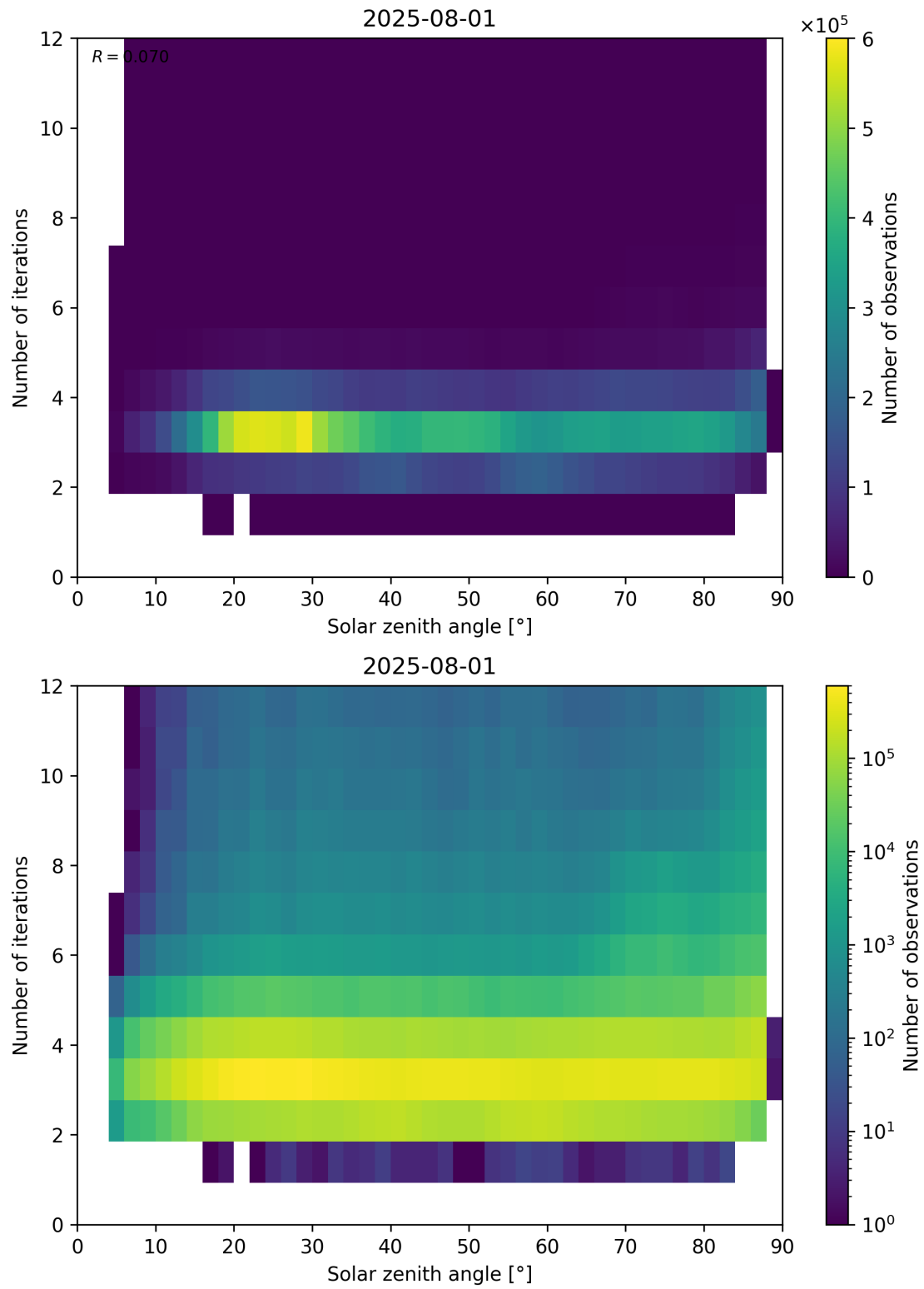
Figure 114: Scatter density plot of “Solar zenith angle” against “Number of iterations” for 2025-07-31 to 2025-08-02.
