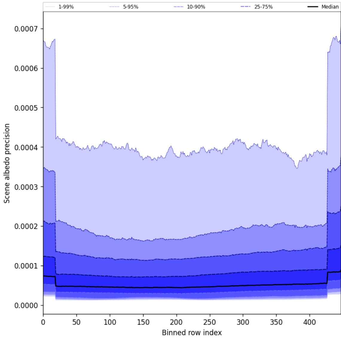
Figure 52: Along track statistics of “Scene albedo precision” for 2025-07-31 to 2025-08-02
