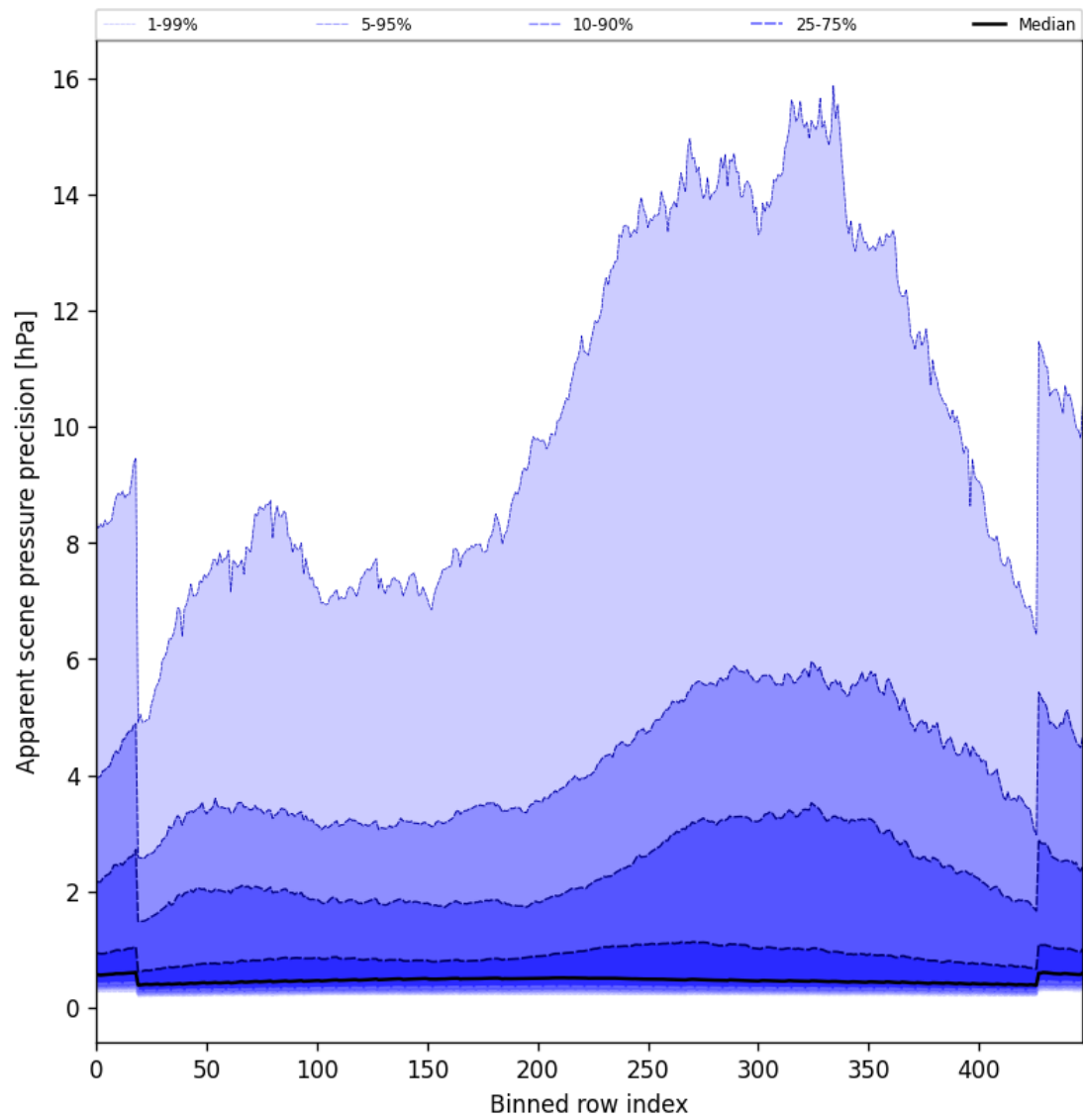
Figure 54: Along track statistics of “Apparent scene pressure precision” for 2025-07-31 to 2025-08-02
