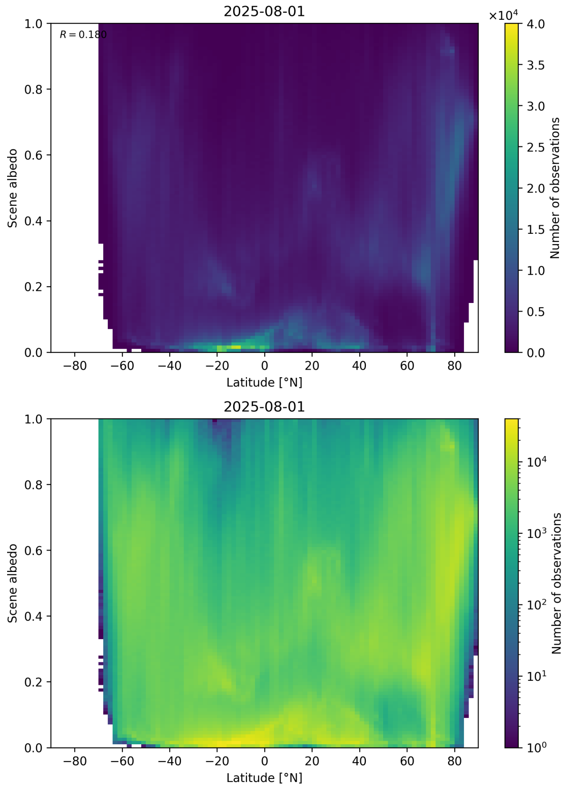
Figure 95: Scatter density plot of “Latitude” against “Scene albedo” for 2025-07-31 to 2025-08-02.
