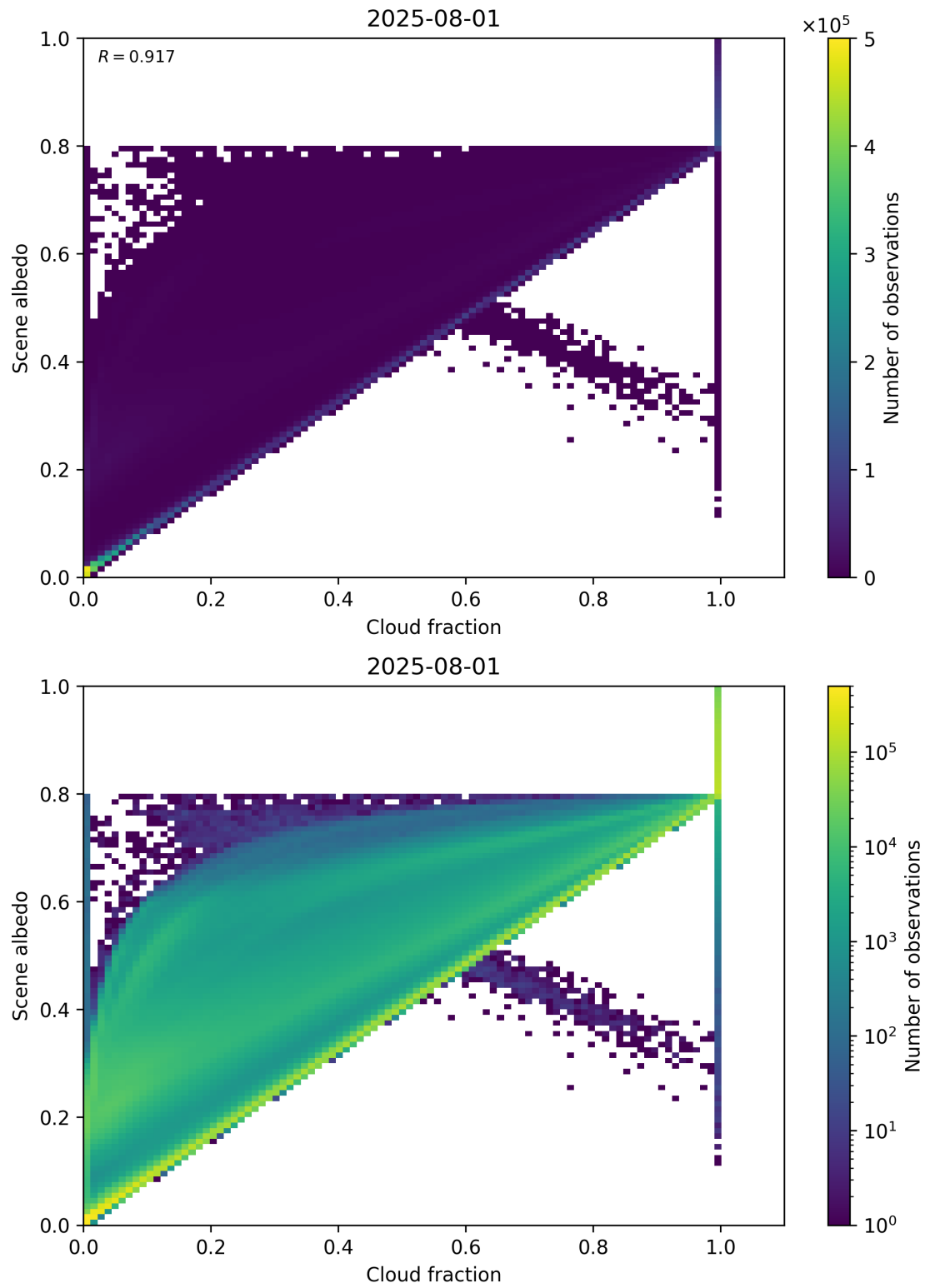
Figure 75: Scatter density plot of “Cloud fraction” against “Scene albedo” for 2025-07-31 to 2025-08-02.
