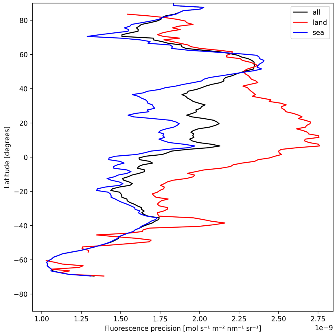
Figure 24: Zonal average of “Fluorescence precision” for 2025-07-31 to 2025-08-02.
