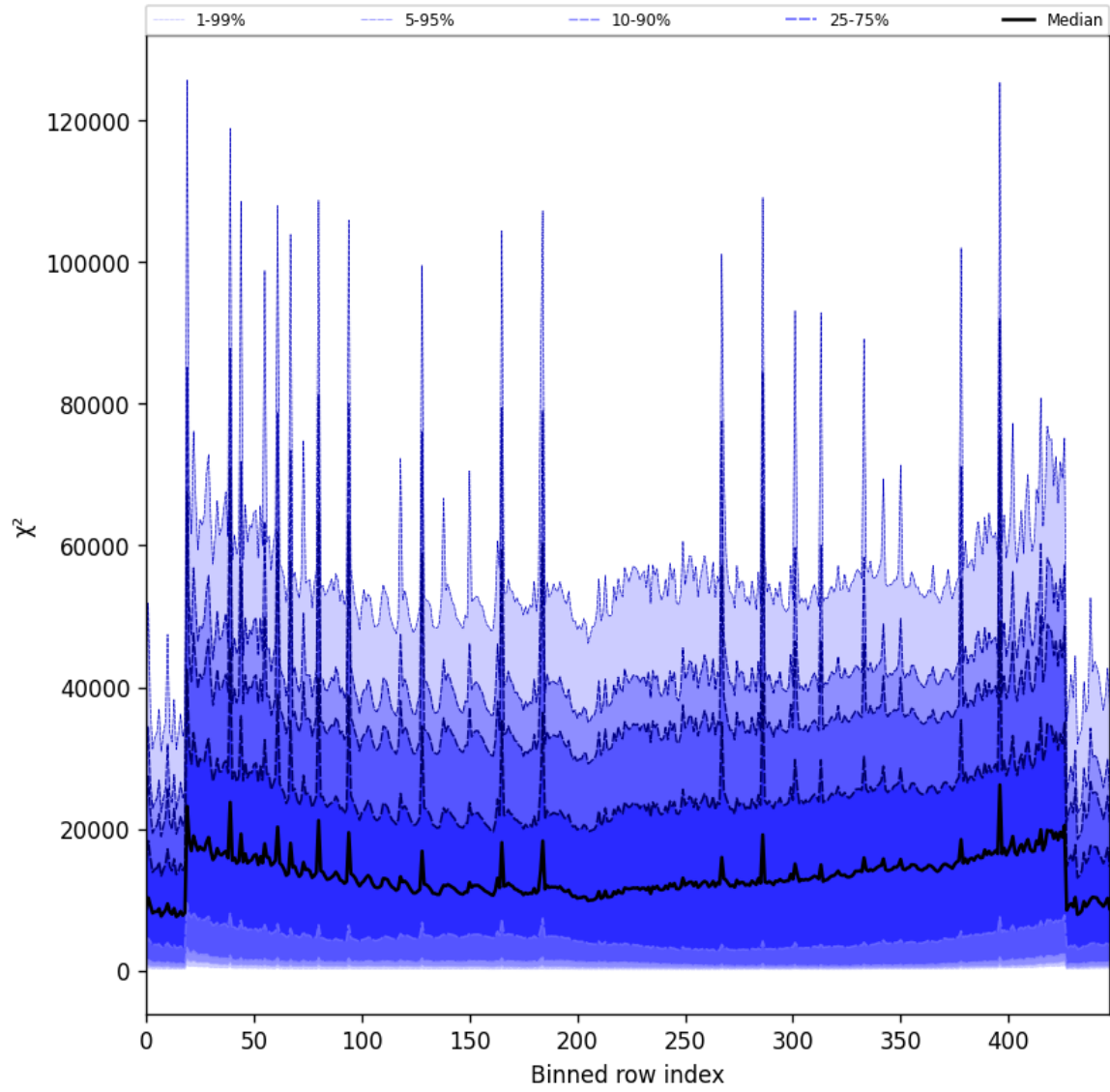
Figure 55: Along track statistics of “ \chi^2 ” for 2025-07-31 to 2025-08-02
