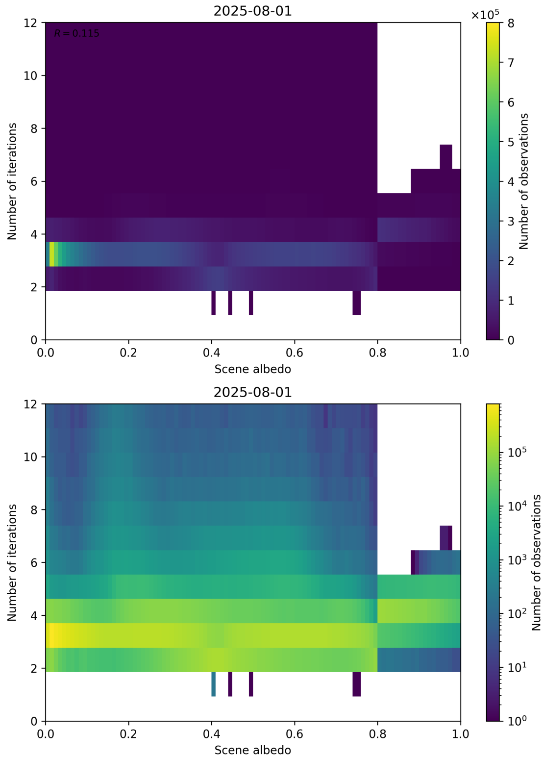
Figure 105: Scatter density plot of “Scene albedo” against “Number of iterations” for 2025-07-31 to 2025-08-02.
