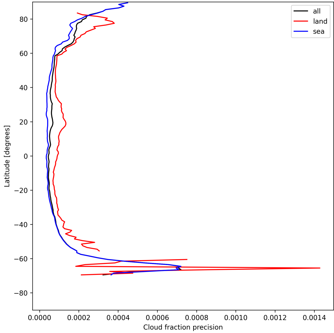
Figure 16: Zonal average of “Cloud fraction precision” for 2025-07-31 to 2025-08-02.
