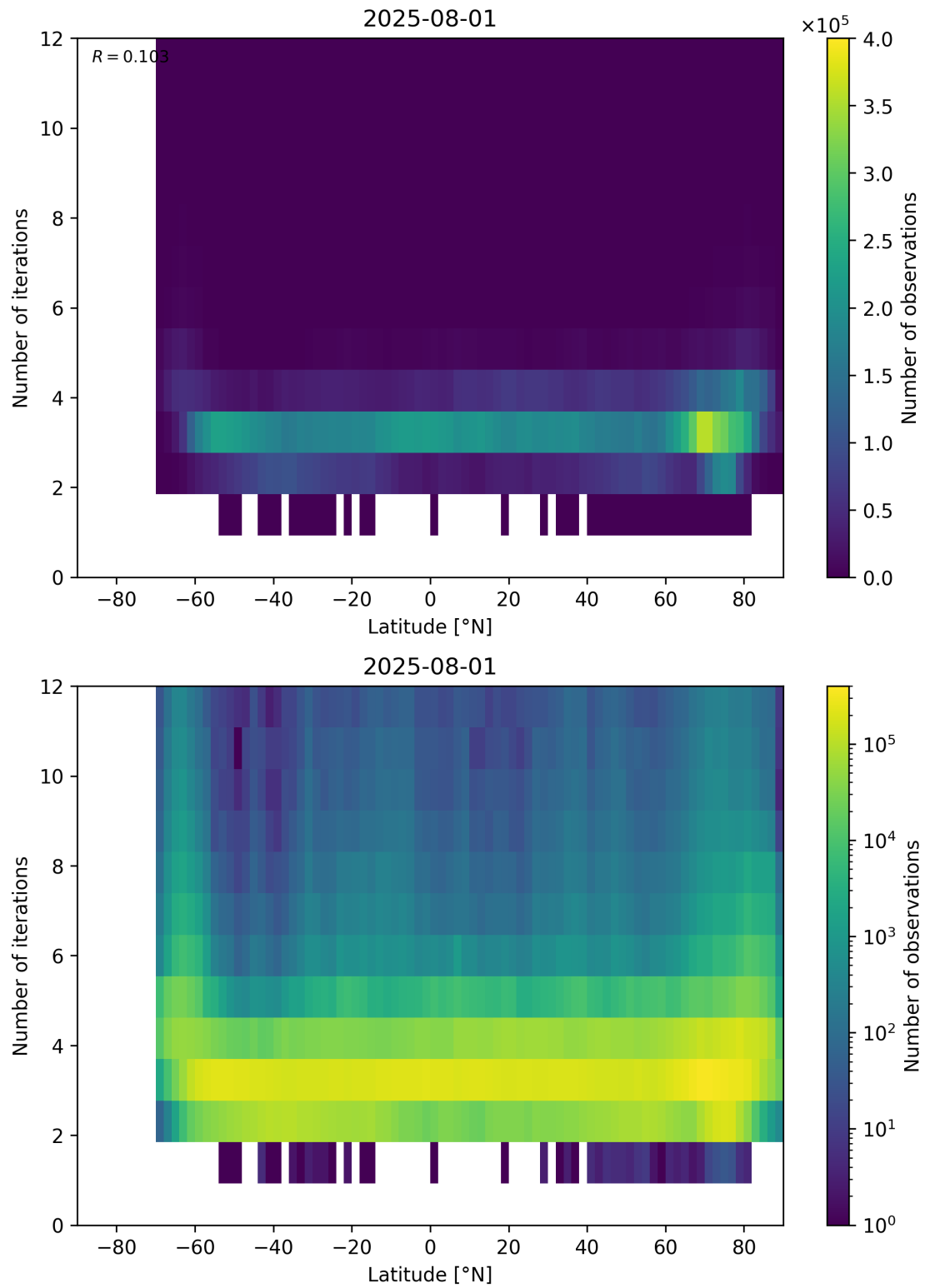
Figure 93: Scatter density plot of “Latitude” against “Number of iterations” for 2025-07-31 to 2025-08-02.
