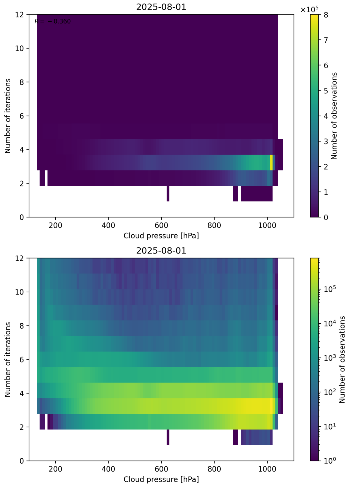
Figure 81: Scatter density plot of “Cloud pressure” against “Number of iterations” for 2025-07-31 to 2025-08-02.
