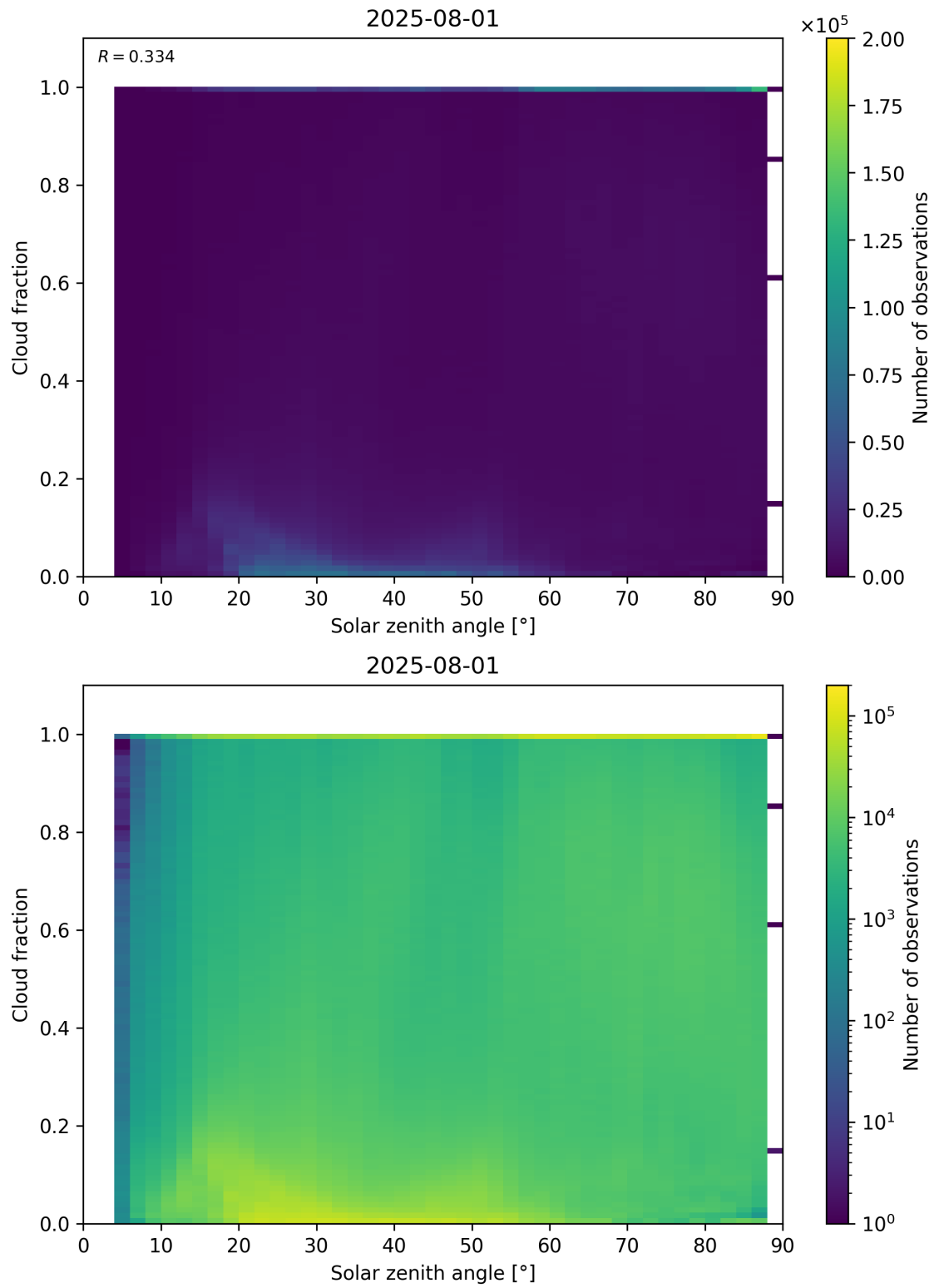
Figure 110: Scatter density plot of “Solar zenith angle” against “Cloud fraction” for 2025-07-31 to 2025-08-02.
