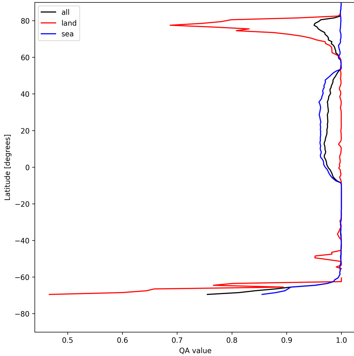
Figure 12: Zonal average of “QA value” for 2025-07-31 to 2025-08-02.
