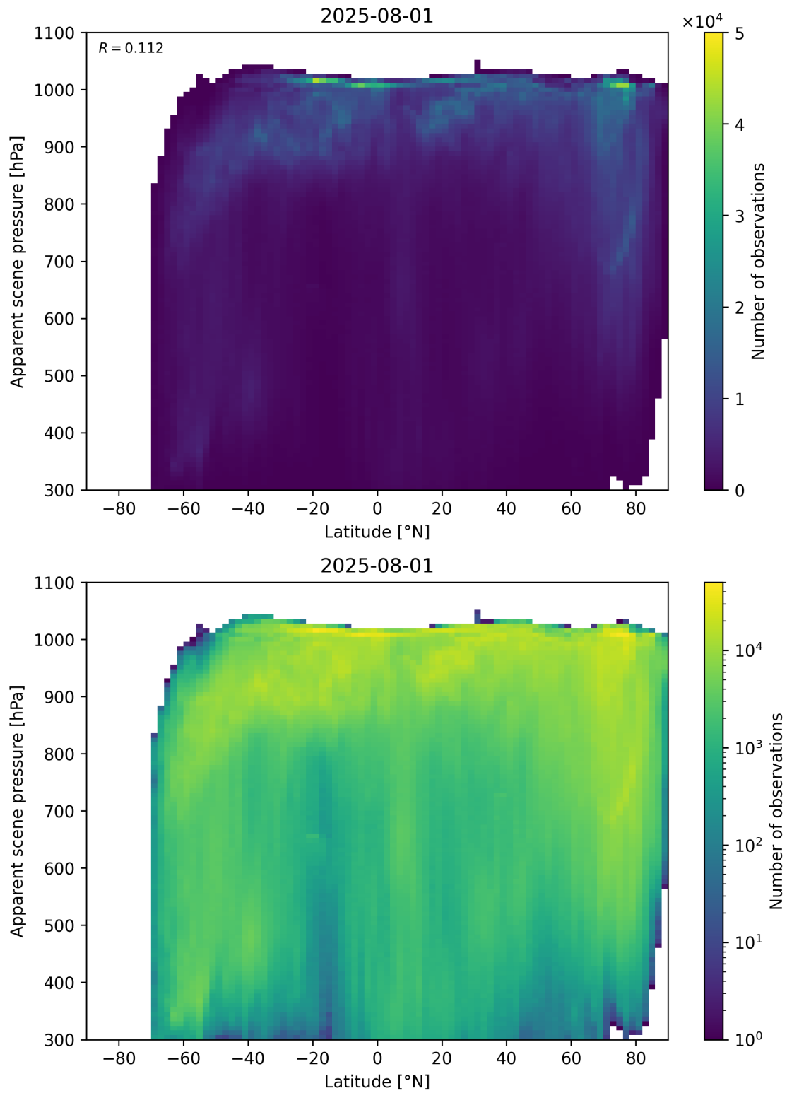
Figure 88: Scatter density plot of “Latitude” against “Apparent scene pressure” for 2025-07-31 to 2025-08-02.
