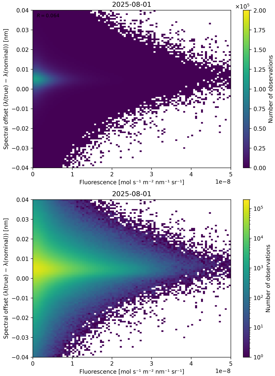
Figure 87: Scatter density plot of “Fluorescence” against “Spectral offset ( \lambda_{\text{true}} - \lambda_{\text{nominal}} )” for 2025-07-31 to 2025-08-02.
