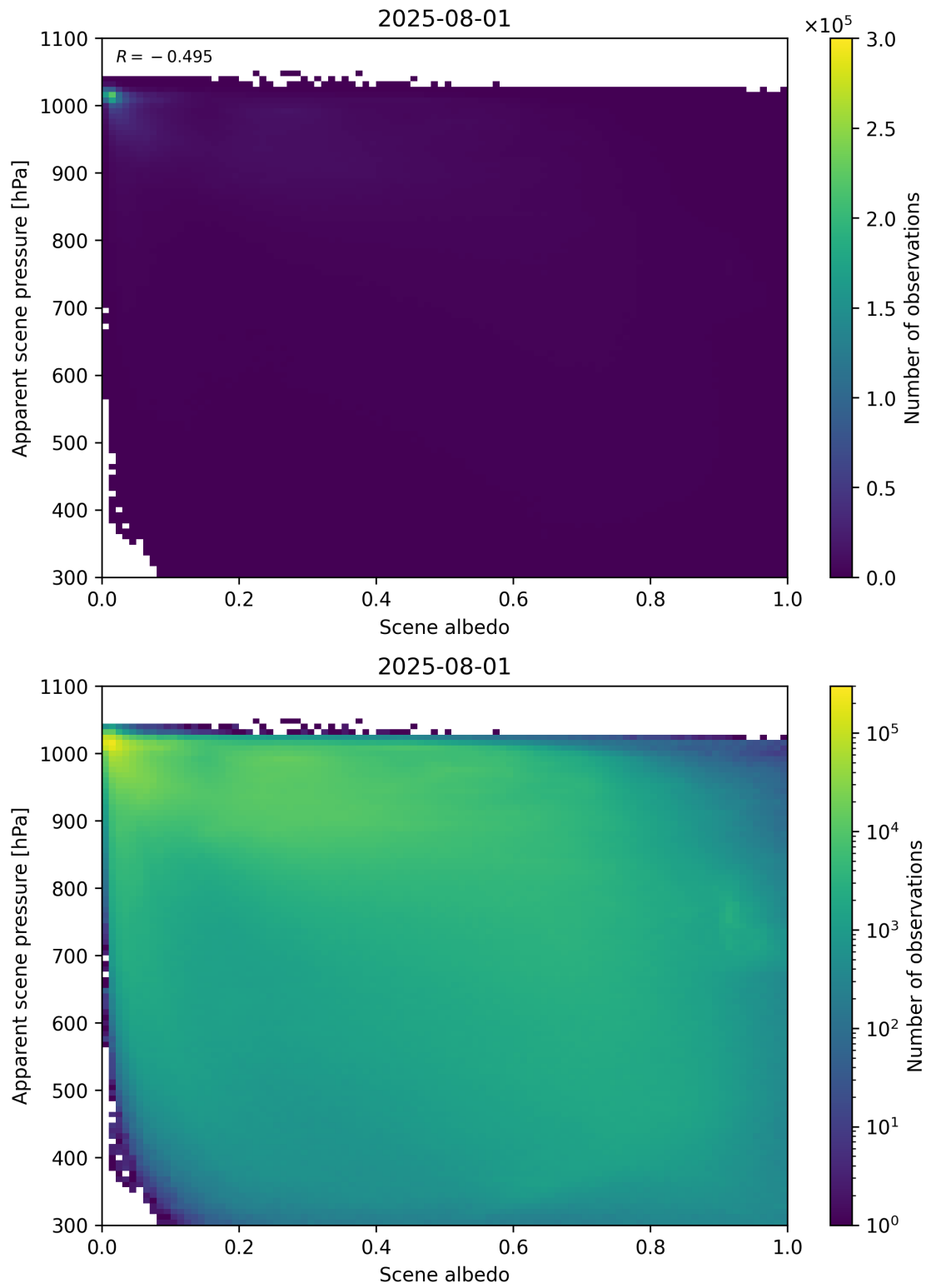
Figure 102: Scatter density plot of “Scene albedo” against “Apparent scene pressure” for 2025-07-31 to 2025-08-02.
