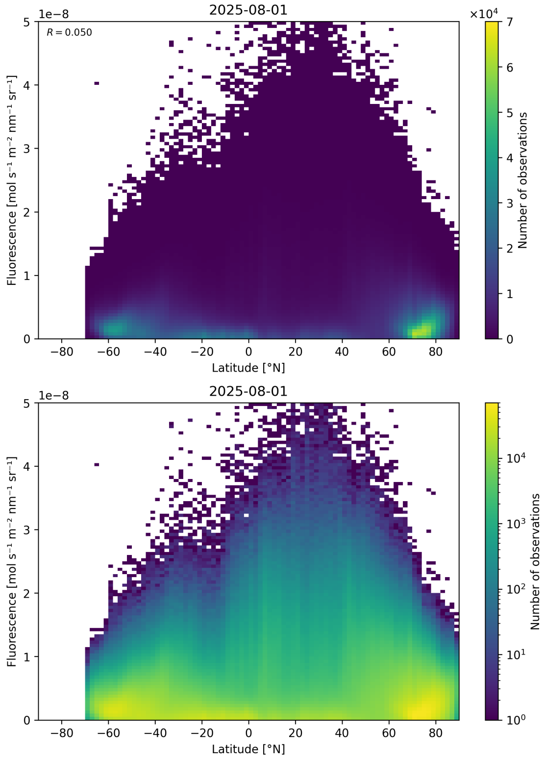
Figure 92: Scatter density plot of “Latitude” against “Fluorescence” for 2025-07-31 to 2025-08-02.
