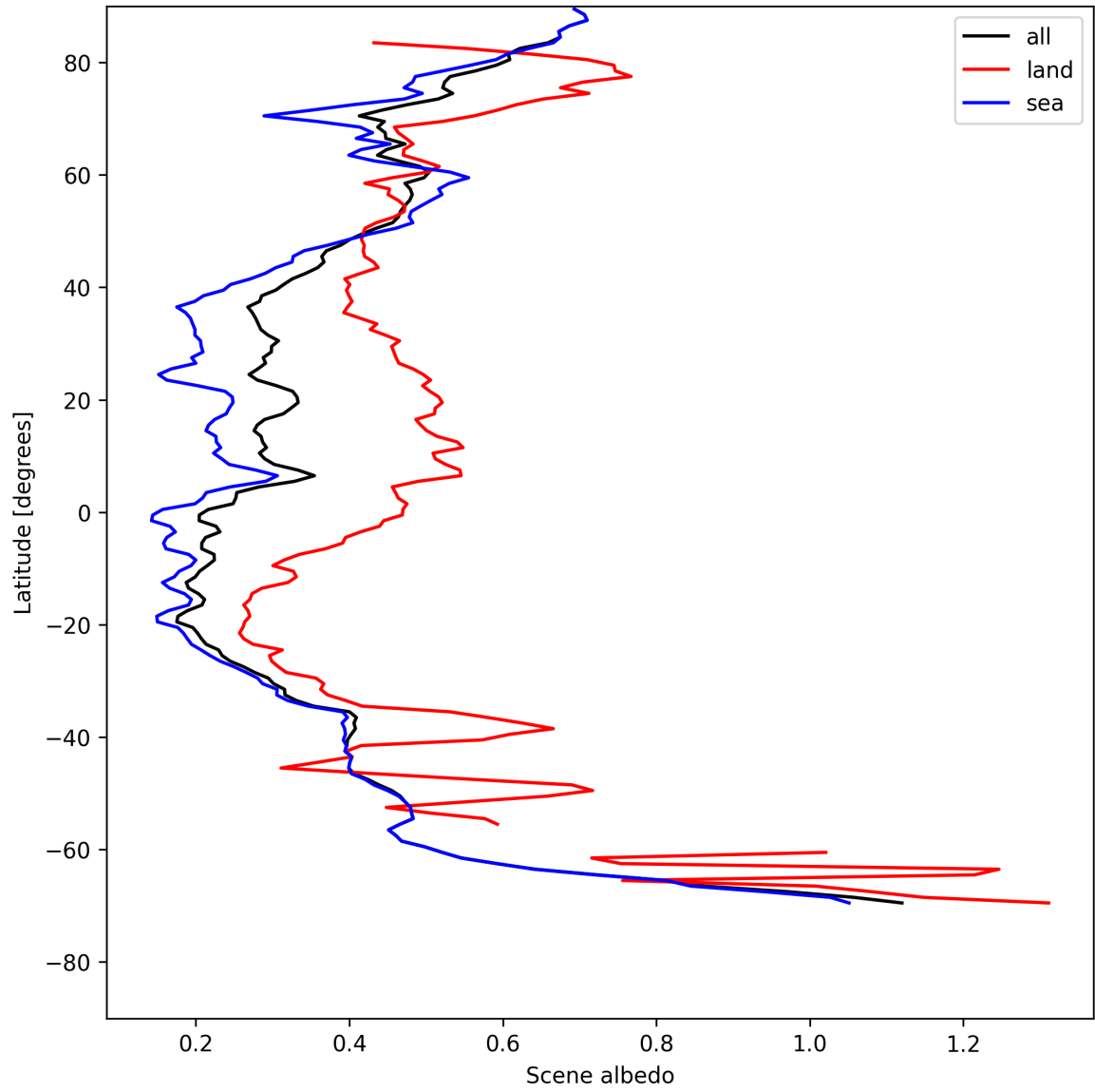
Figure 17: Zonal average of “Scene albedo” for 2025-07-31 to 2025-08-02.
