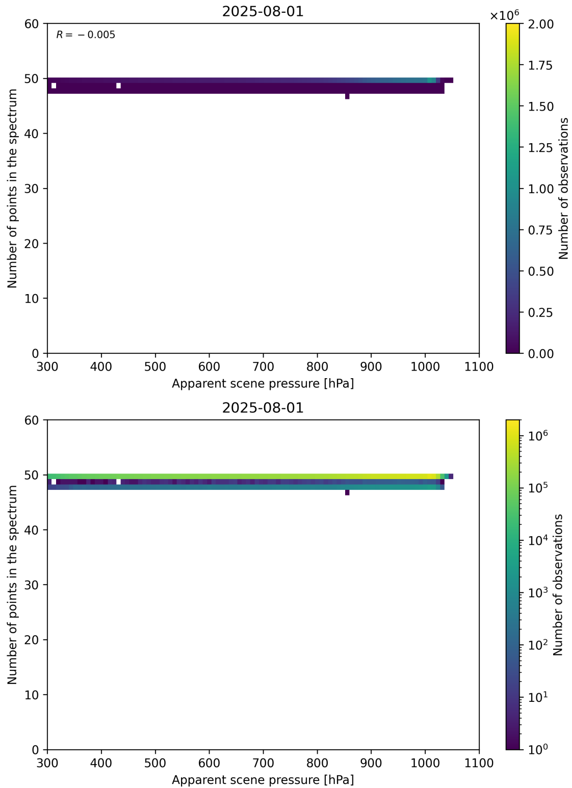
Figure 66: Scatter density plot of “Apparent scene pressure” against “Number of points in the spectrum” for 2025-07-31 to 2025-08-02.
