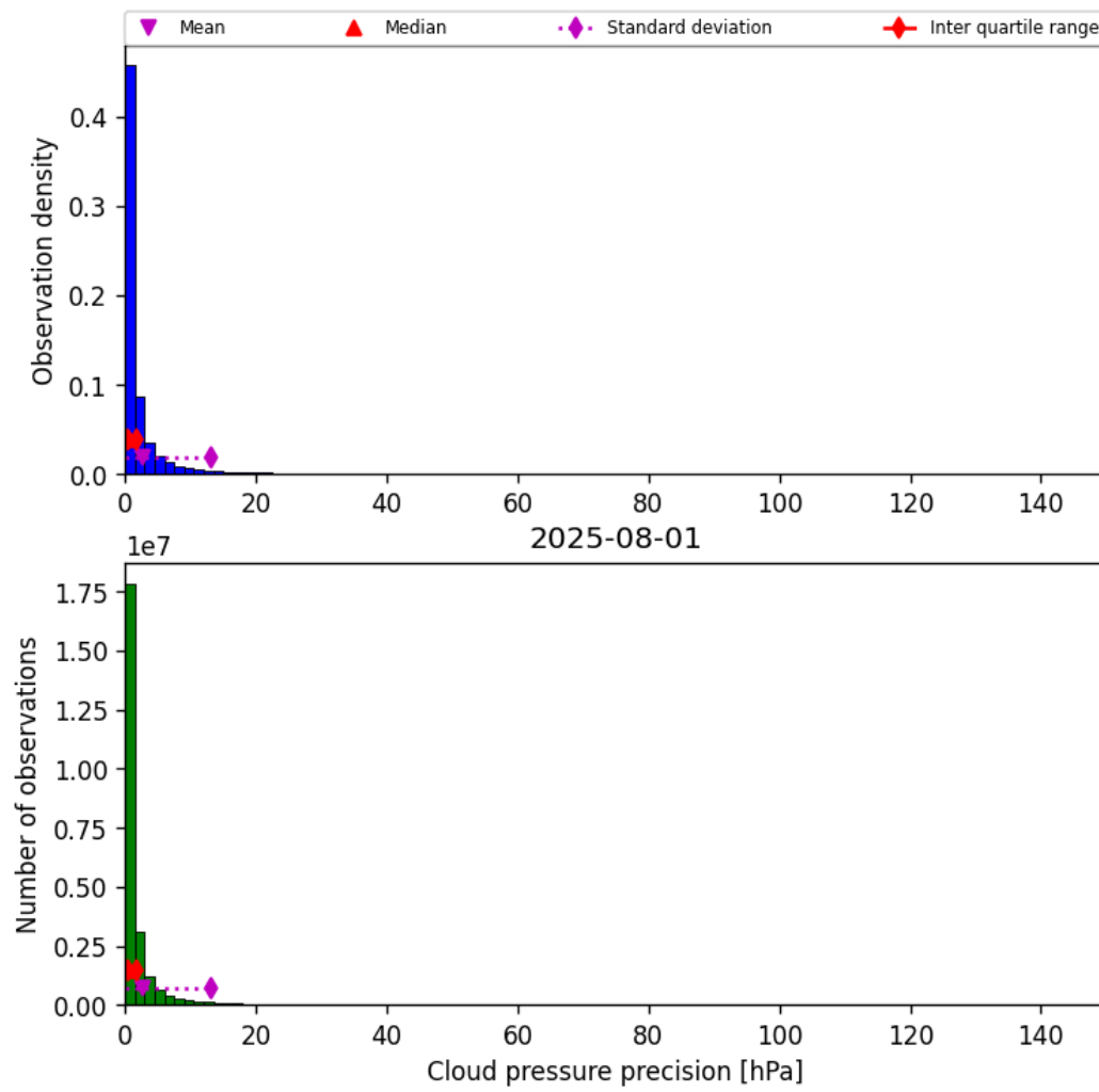
Figure 31: Histogram of “Cloud pressure precision” for 2025-07-31 to 2025-08-02
