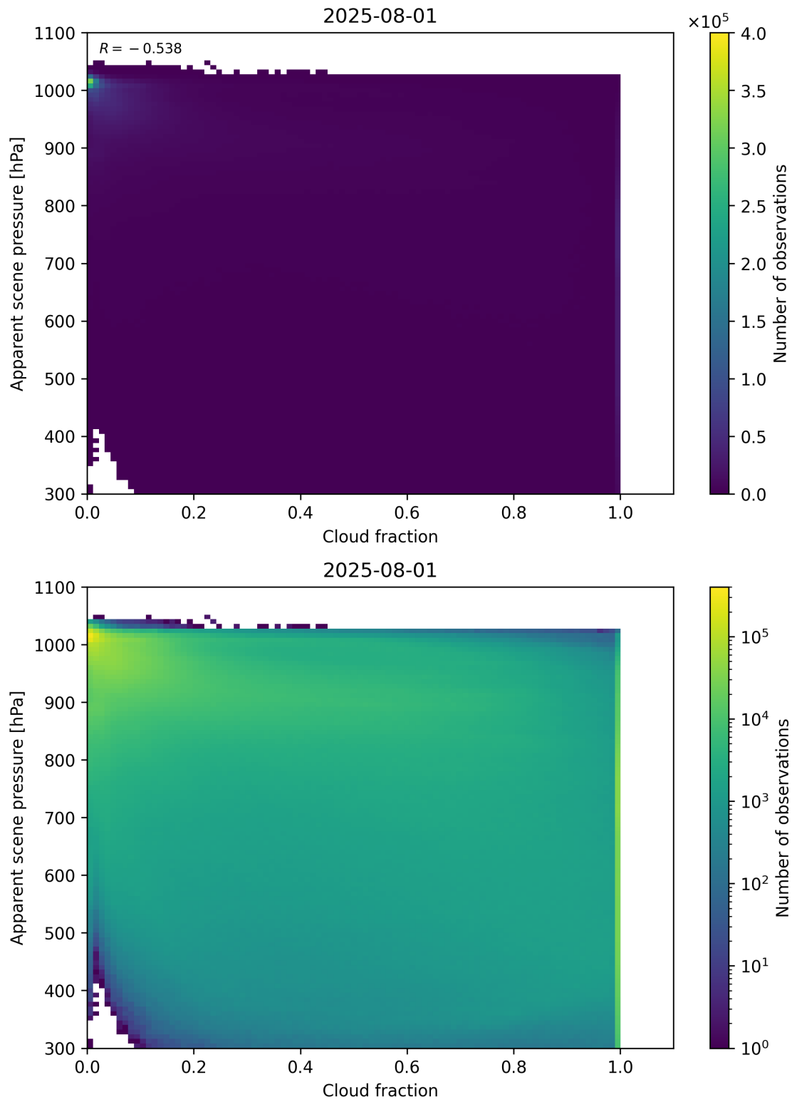
Figure 70: Scatter density plot of “Cloud fraction” against “Apparent scene pressure” for 2025-07-31 to 2025-08-02.
