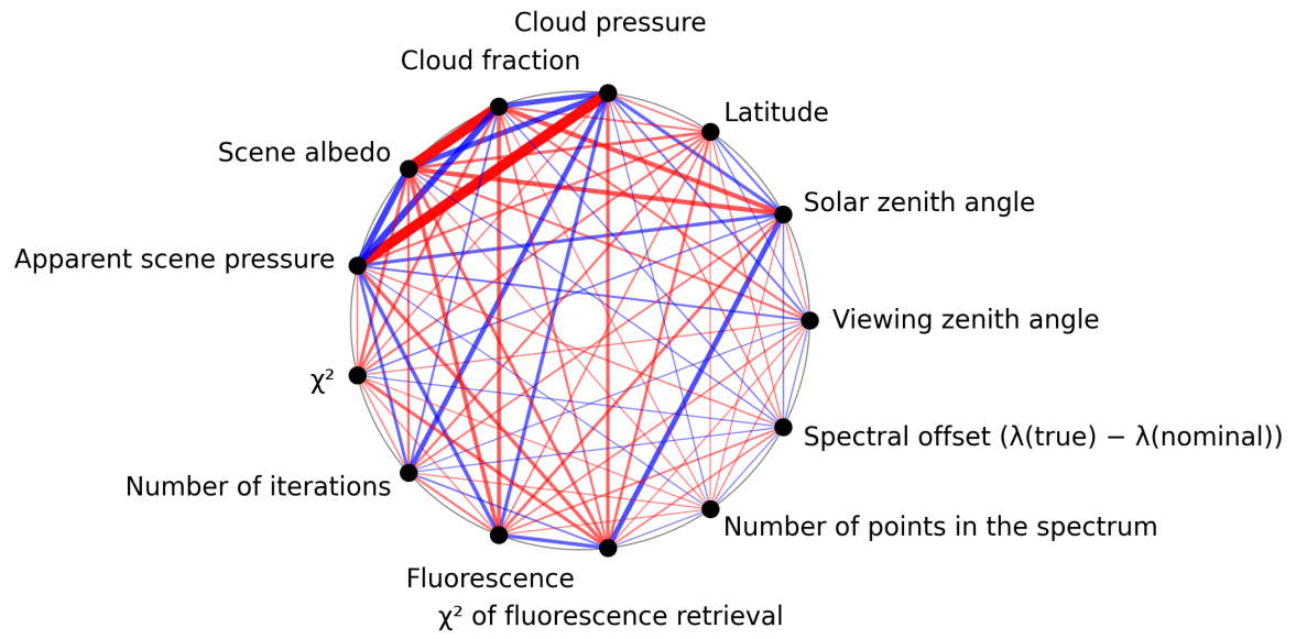
Figure 1: Map of correlation graph for 2025-07-31 to 2025-08-02.
