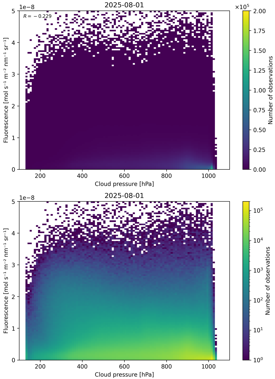
Figure 80: Scatter density plot of “Cloud pressure” against “Fluorescence” for 2025-07-31 to 2025-08-02.
