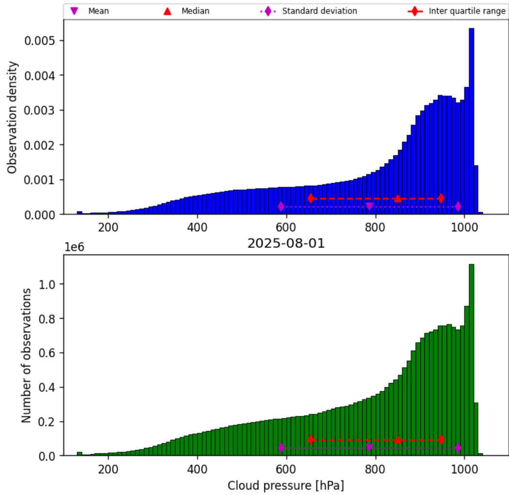
Figure 30: Histogram of “Cloud pressure” for 2025-07-31 to 2025-08-02
