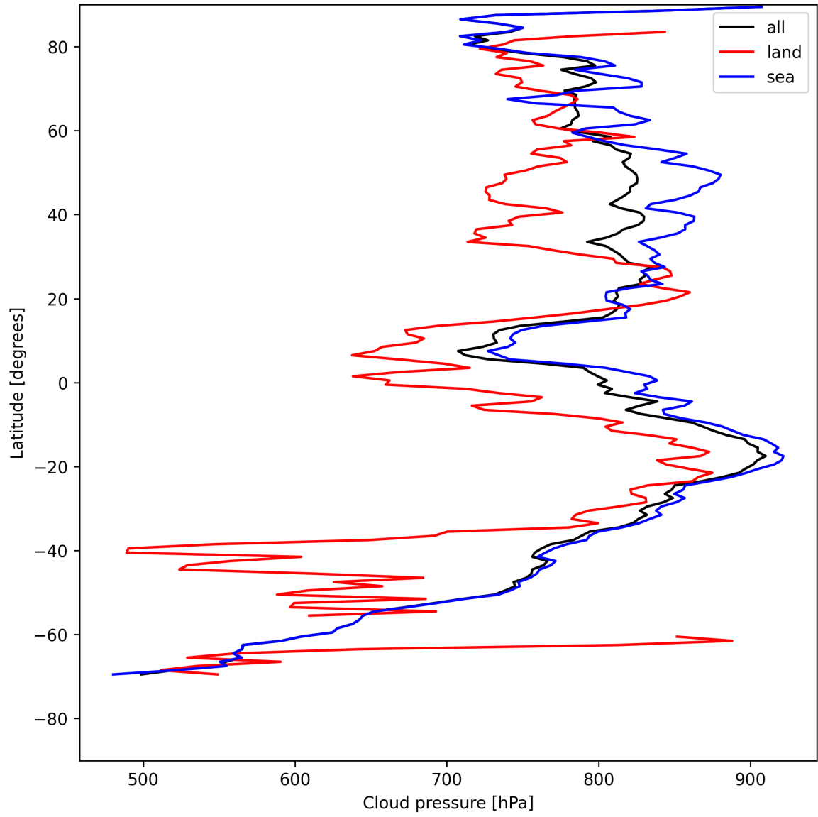
Figure 13: Zonal average of “Cloud pressure” for 2025-07-31 to 2025-08-02.
