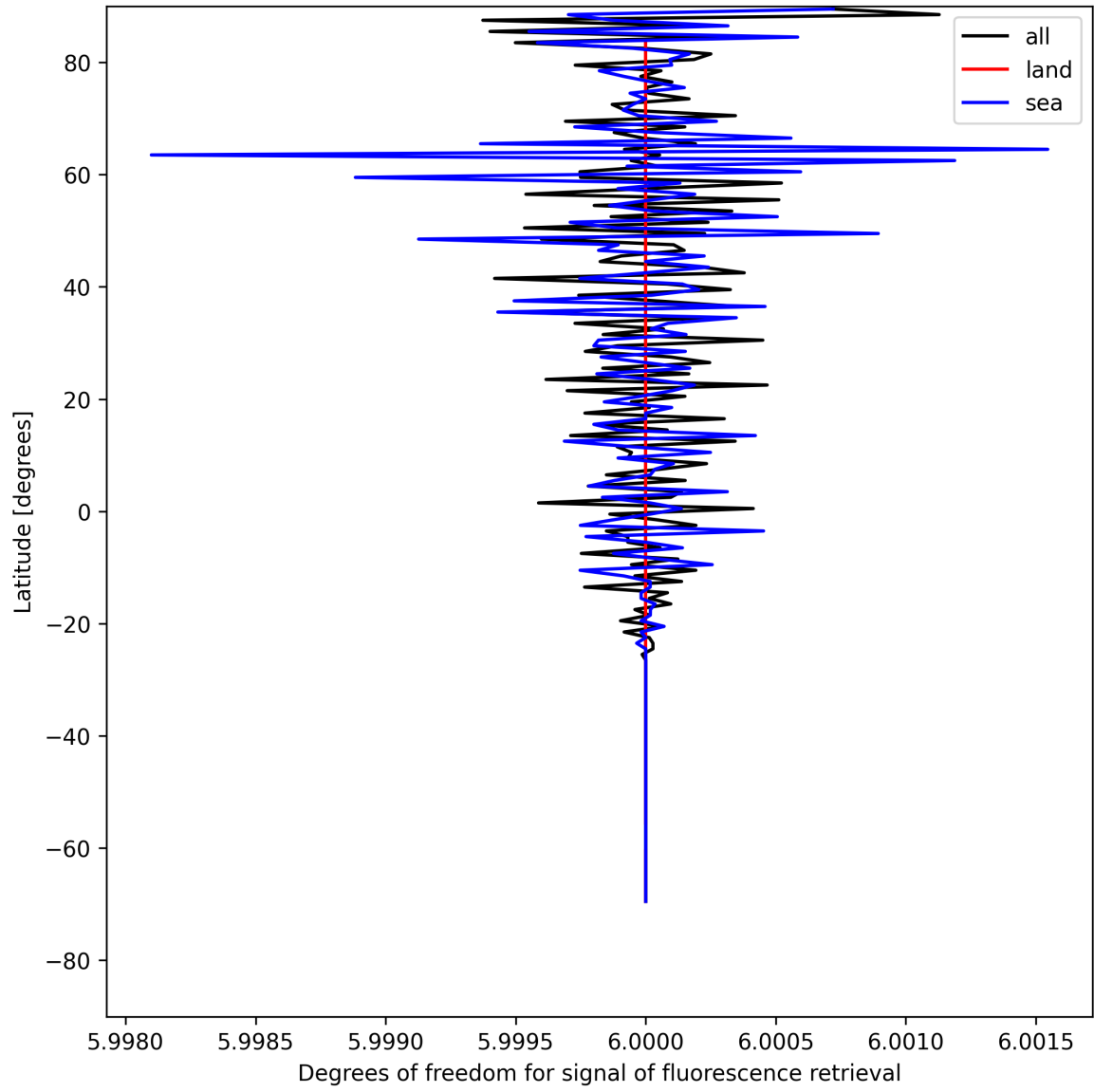
Figure 26: Zonal average of “Degrees of freedom for signal of fluorescence retrieval” for 2025-07-31 to 2025-08-02.
