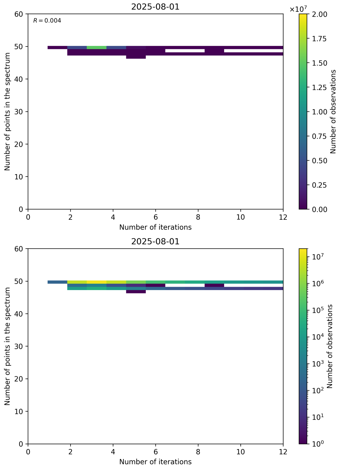
Figure 99: Scatter density plot of “Number of iterations” against “Number of points in the spectrum” for 2025-07-31 to 2025-08-02.
