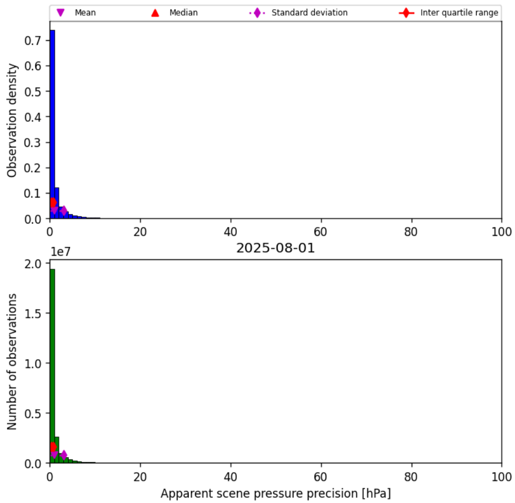
Figure 37: Histogram of “Apparent scene pressure precision” for 2025-07-31 to 2025-08-02
