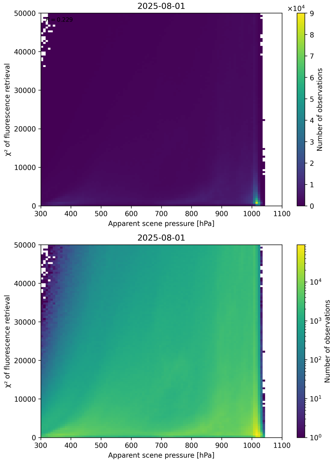
Figure 63: Scatter density plot of “Apparent scene pressure” against “ \chi^2 of fluorescence retrieval” for 2025-07-31 to 2025-08-02.
