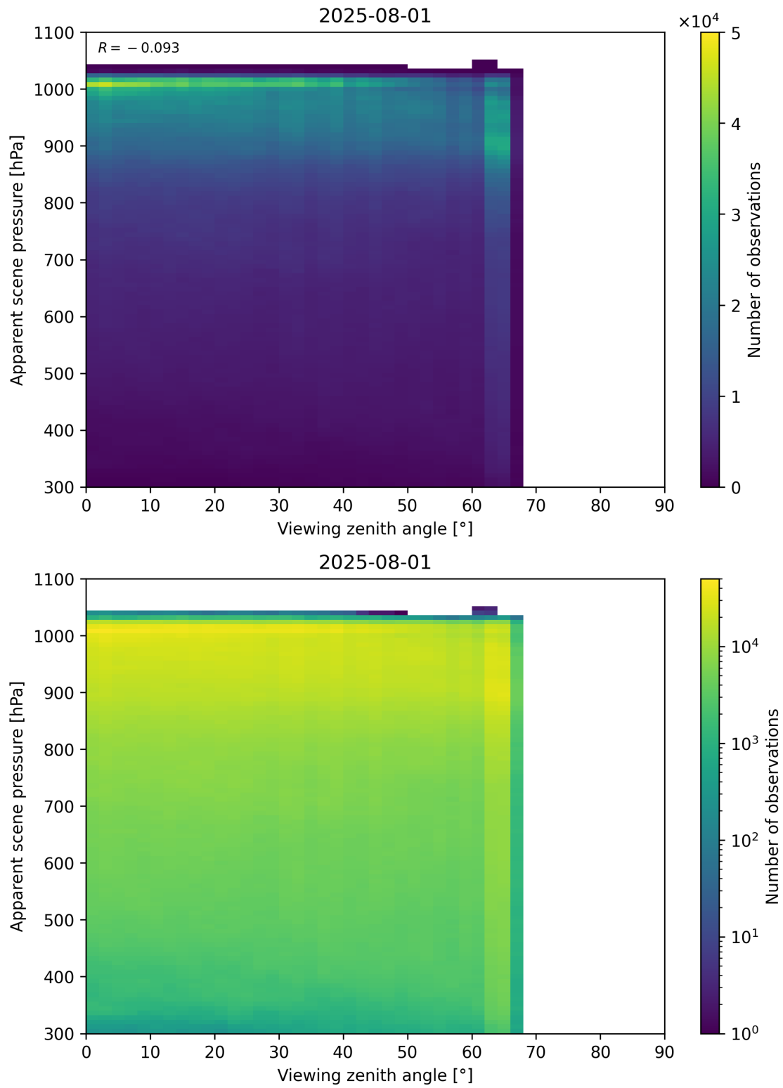
Figure 118: Scatter density plot of “Viewing zenith angle” against “Apparent scene pressure” for 2025-07-31 to 2025-08-02.
