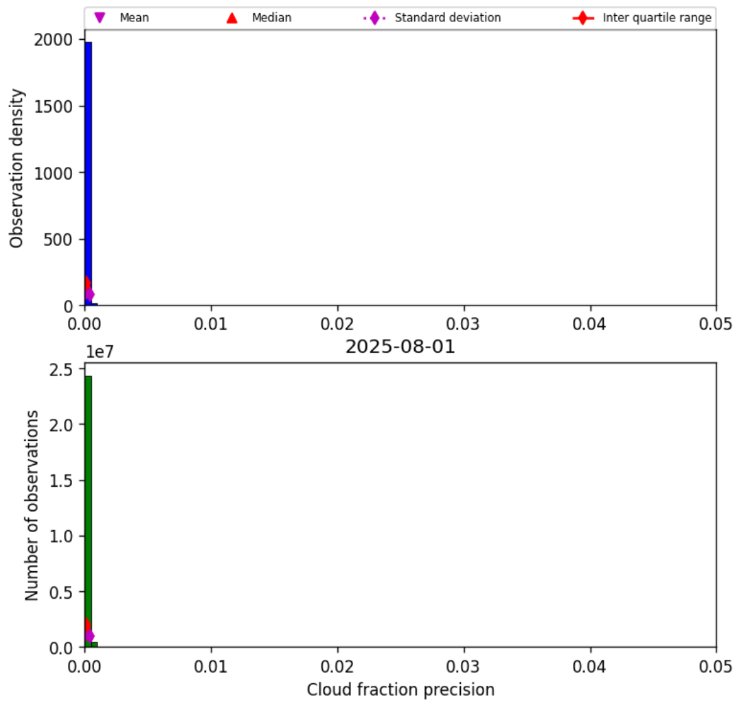
Figure 33: Histogram of “Cloud fraction precision” for 2025-07-31 to 2025-08-02
