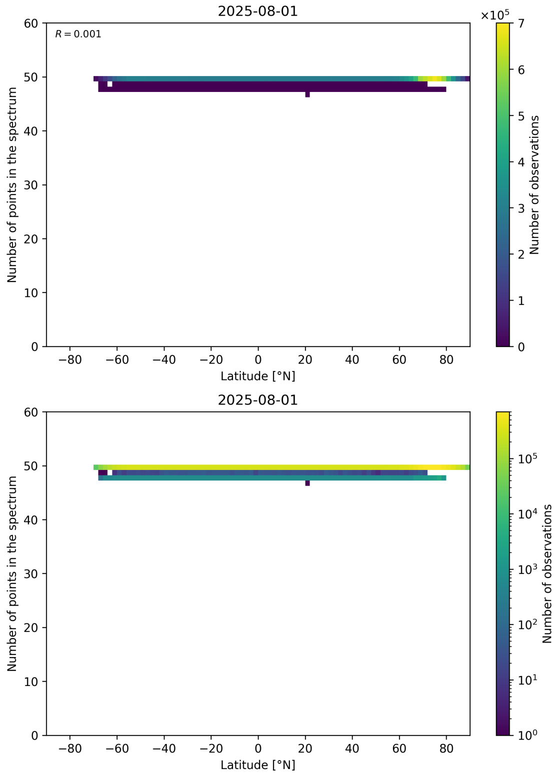
Figure 94: Scatter density plot of “Latitude” against “Number of points in the spectrum” for 2025-07-31 to 2025-08-02.
