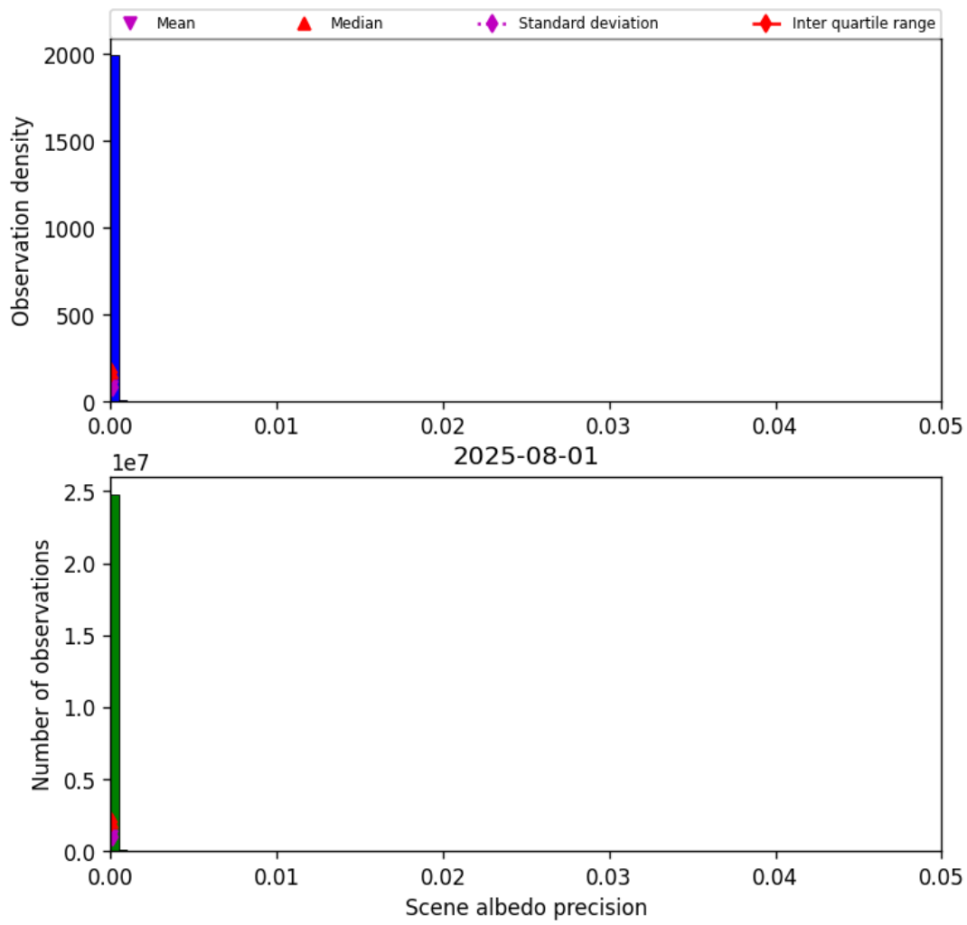
Figure 35: Histogram of “Scene albedo precision” for 2025-07-31 to 2025-08-02
