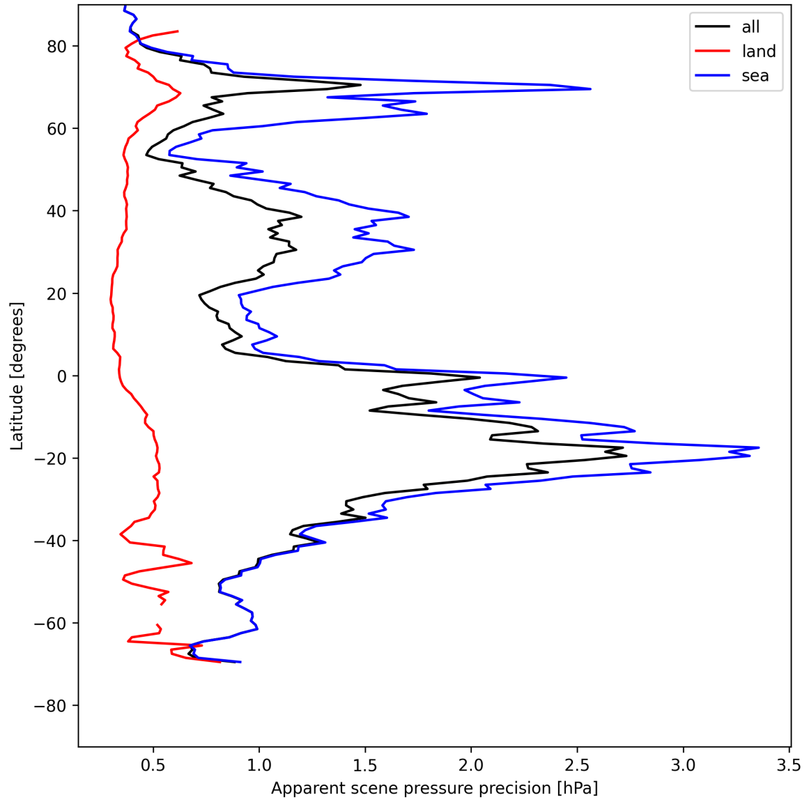
Figure 20: Zonal average of “Apparent scene pressure precision” for 2025-07-31 to 2025-08-02.
