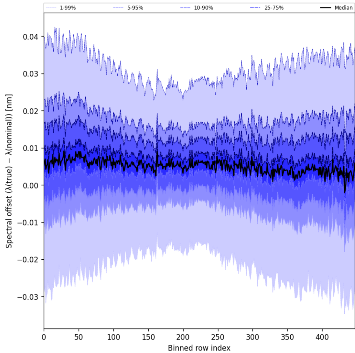
Figure 62: Along track statistics of “Spectral offset ( \lambda_{\text{true}} - \lambda_{\text{nominal}} )” for 2025-07-31 to 2025-08-02
