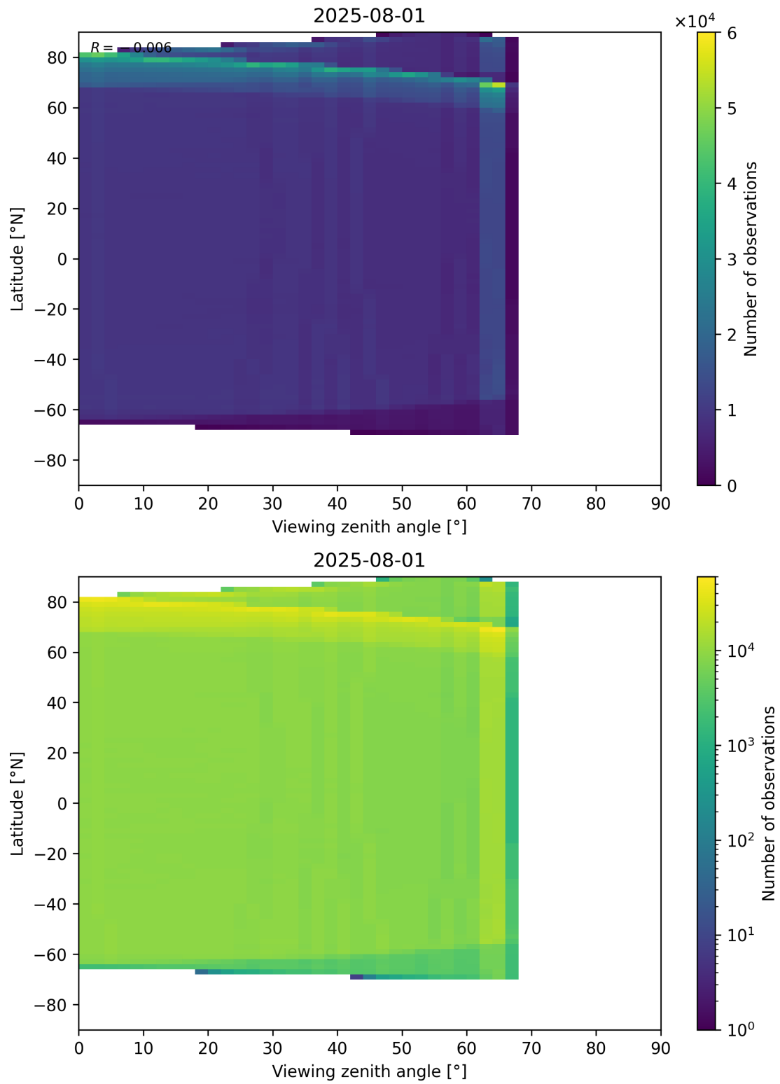
Figure 123: Scatter density plot of “Viewing zenith angle” against “Latitude” for 2025-07-31 to 2025-08-02.
