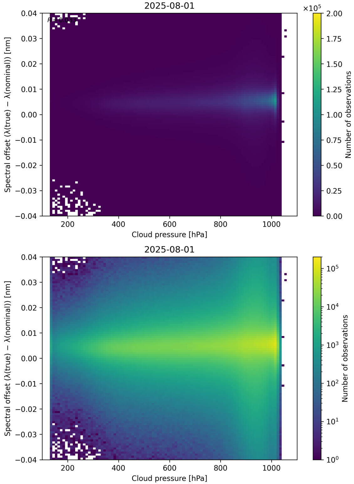
Figure 84: Scatter density plot of “Cloud pressure” against “Spectral offset ( \lambda_{\text{true}} - \lambda_{\text{nominal}} )” for 2025-07-31 to 2025-08-02.
