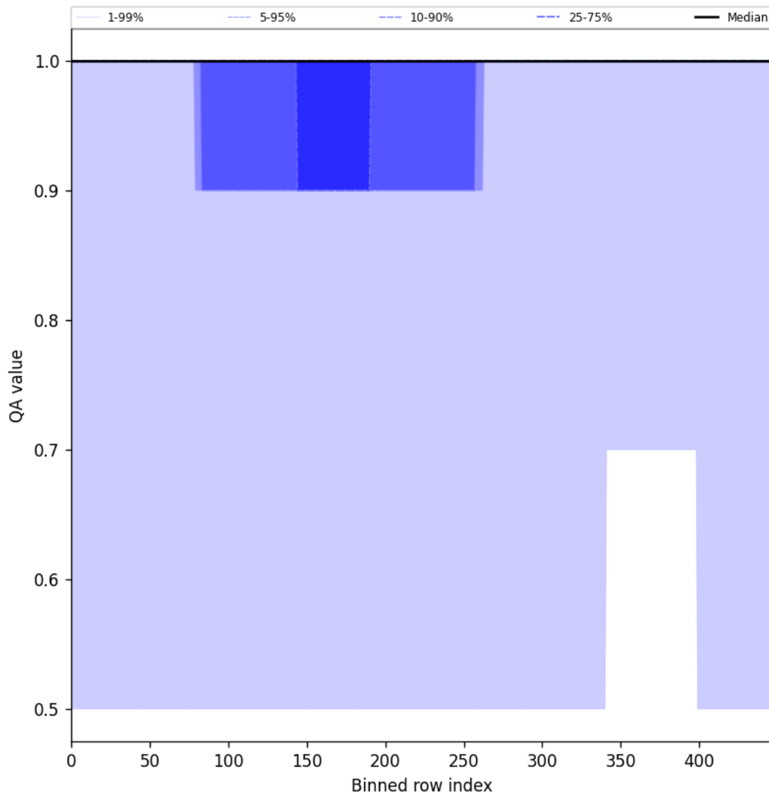
Figure 46: Along track statistics of “QA value” for 2025-07-31 to 2025-08-02
