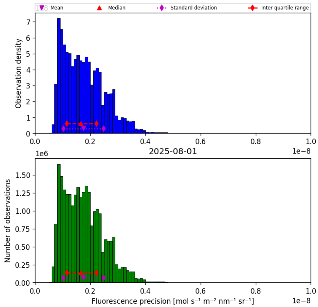
Figure 41: Histogram of “Fluorescence precision” for 2025-07-31 to 2025-08-02
