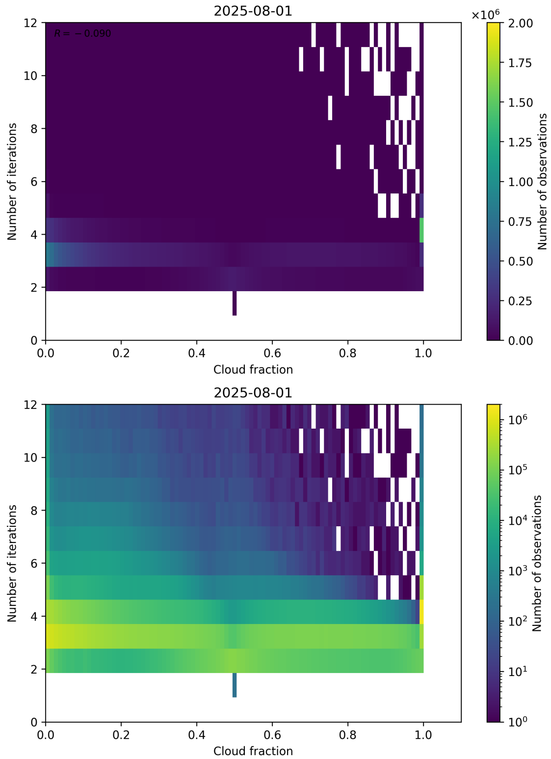
Figure 73: Scatter density plot of “Cloud fraction” against “Number of iterations” for 2025-07-31 to 2025-08-02.
