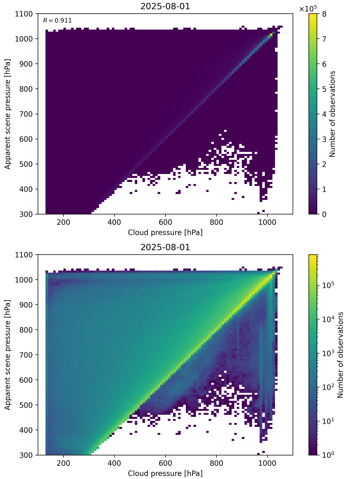
Figure 77: Scatter density plot of “Cloud pressure” against “Apparent scene pressure” for 2025-07-31 to 2025-08-02.
