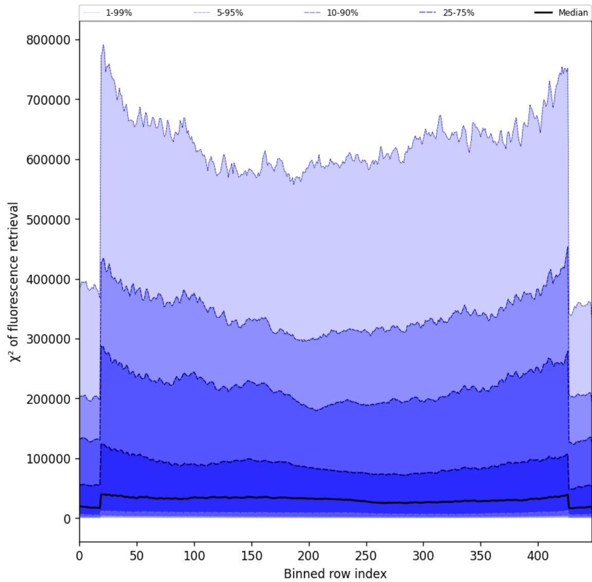
Figure 59: Along track statistics of “ \chi^2 of fluorescence retrieval” for 2025-07-31 to 2025-08-02
