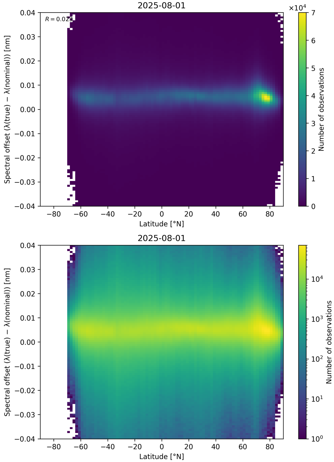
Figure 96: Scatter density plot of “Latitude” against “Spectral offset ( \lambda_{\text{true}} - \lambda_{\text{nominal}} )” for 2025-07-31 to 2025-08-02.
