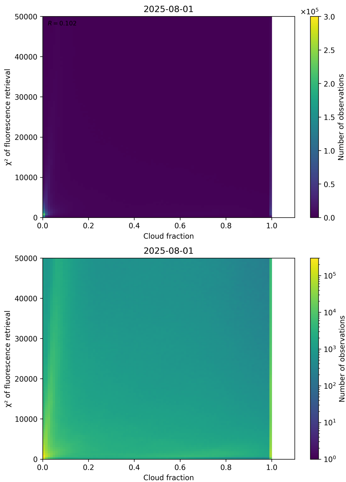
Figure 71: Scatter density plot of “Cloud fraction” against “ \chi^2 of fluorescence retrieval” for 2025-07-31 to 2025-08-02.
