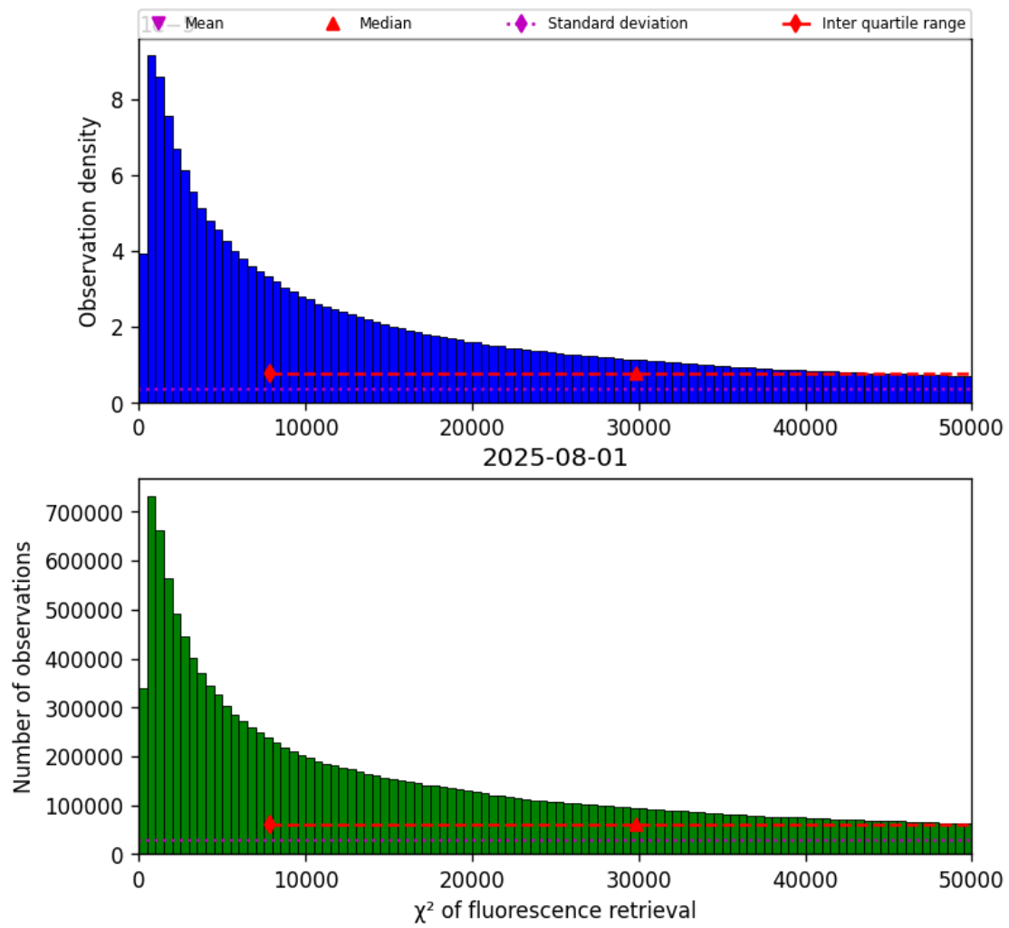
Figure 42: Histogram of “ \chi^2 of fluorescence retrieval” for 2025-07-31 to 2025-08-02
