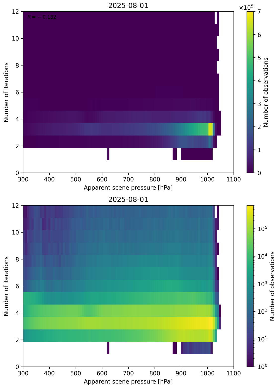
Figure 65: Scatter density plot of “Apparent scene pressure” against “Number of iterations” for 2025-07-31 to 2025-08-02.
