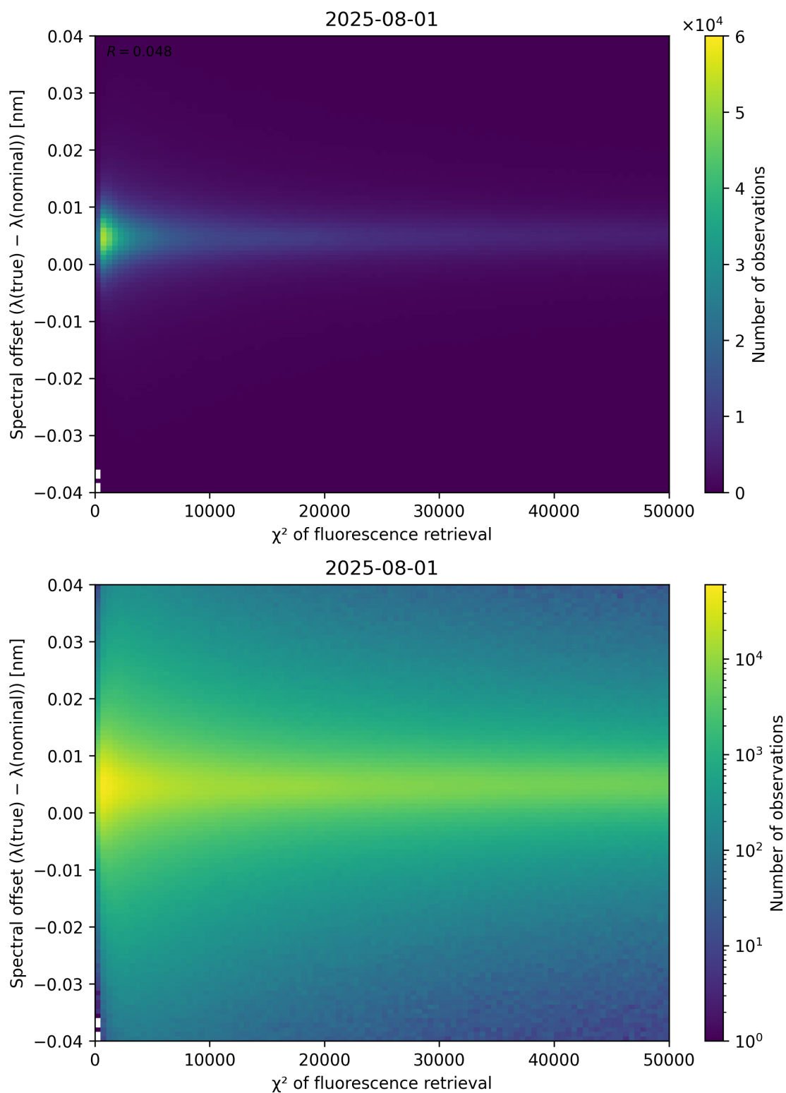
Figure 69: Scatter density plot of “ \chi^2 of fluorescence retrieval” against “Spectral offset ( \lambda_{\text{true}} - \lambda_{\text{nominal}} )” for 2025-07-31 to 2025-08-02.
