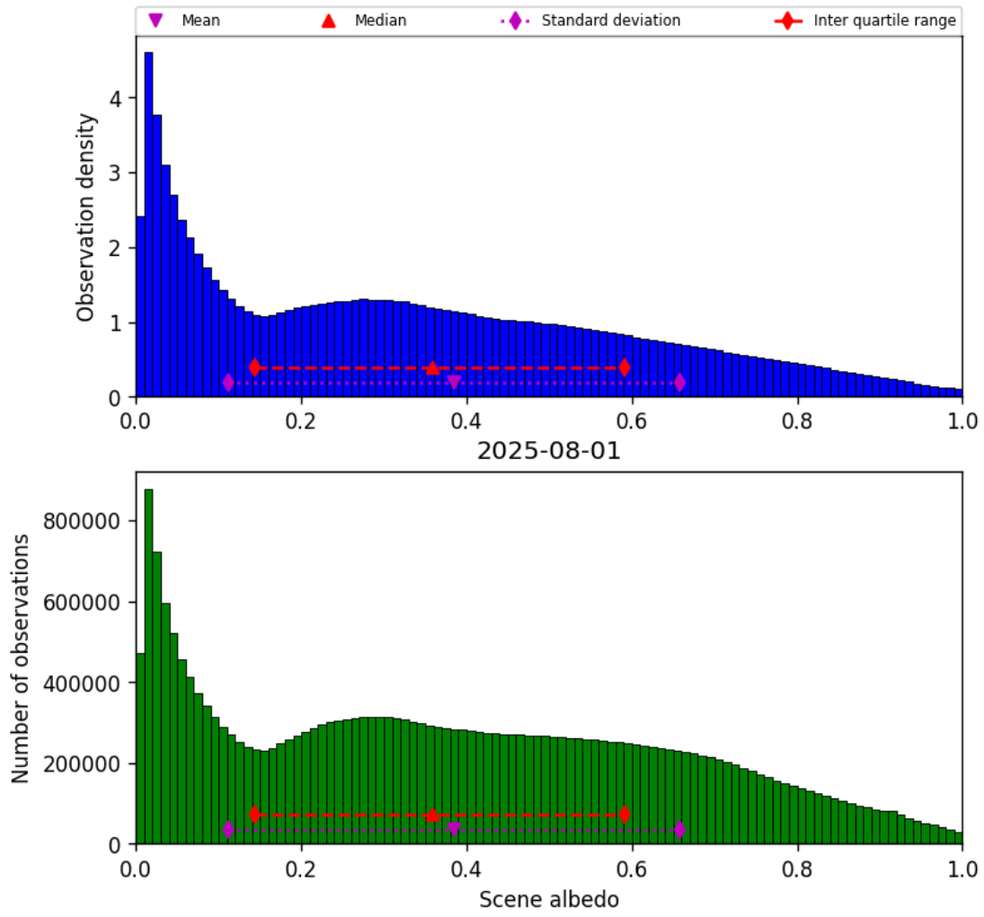
Figure 34: Histogram of “Scene albedo” for 2025-07-31 to 2025-08-02
