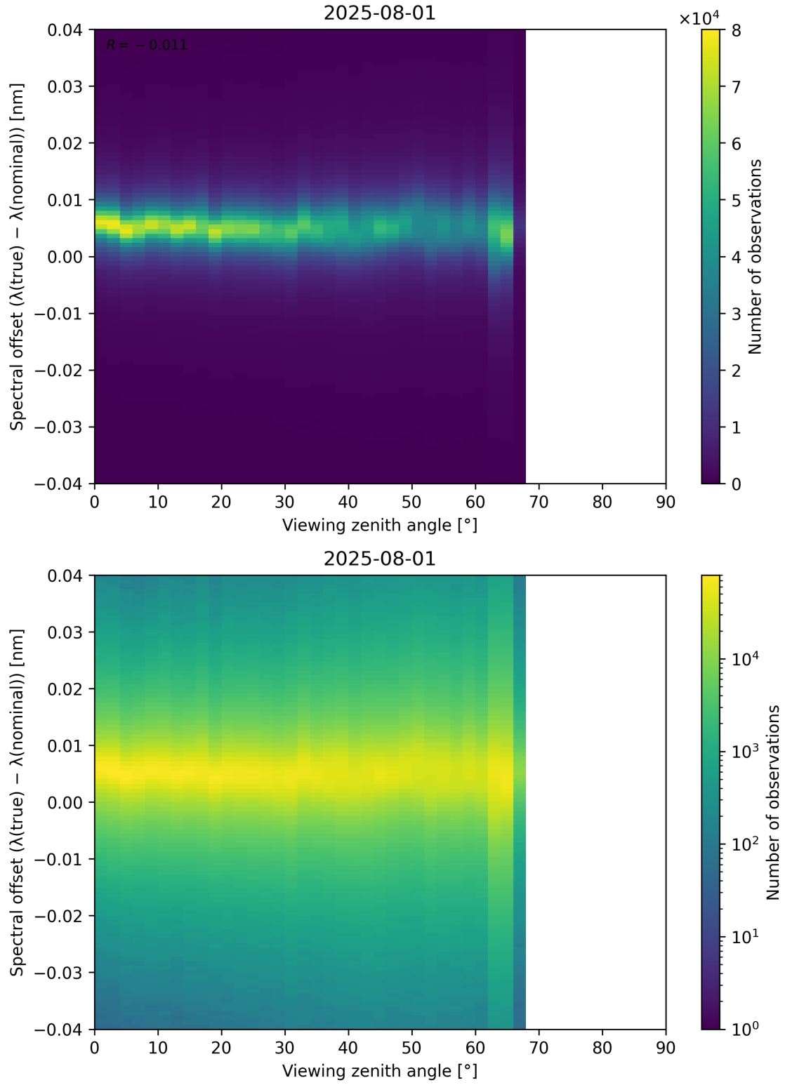
Figure 128: Scatter density plot of “Viewing zenith angle” against “Spectral offset ( \lambda_{\text{true}} - \lambda_{\text{nominal}} )” for 2025-07-31 to 2025-08-02.
