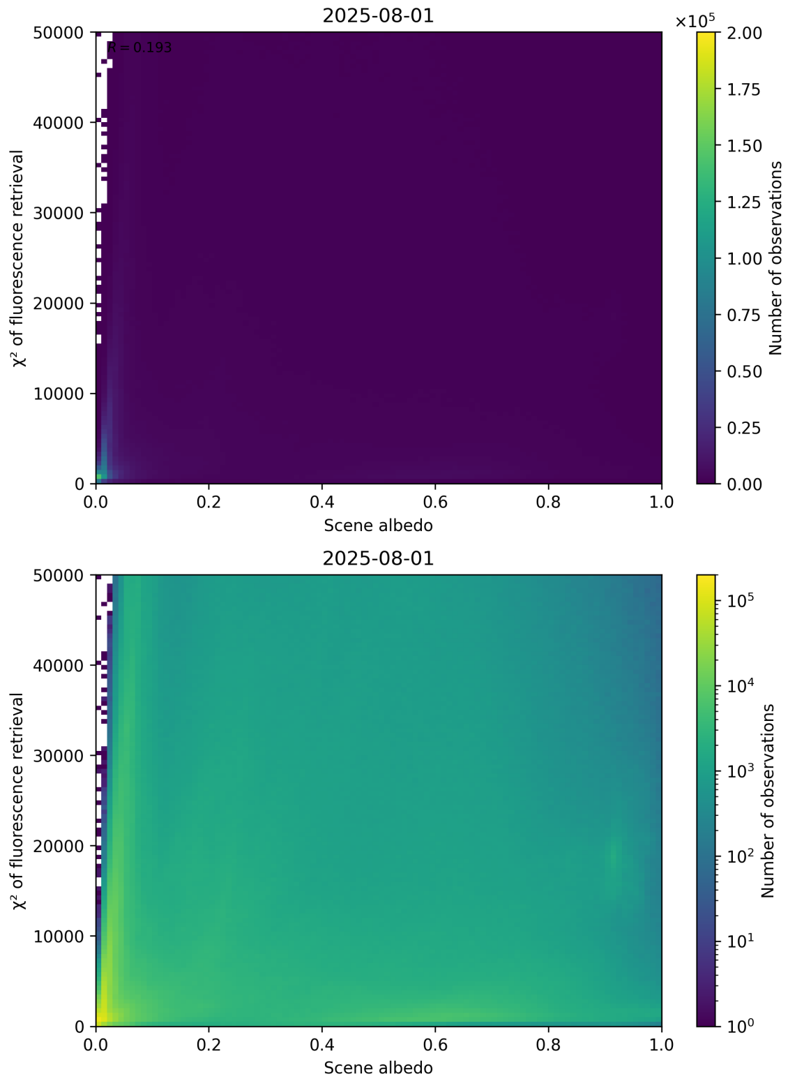
Figure 103: Scatter density plot of “Scene albedo” against “ \chi^2 of fluorescence retrieval” for 2025-07-31 to 2025-08-02.
