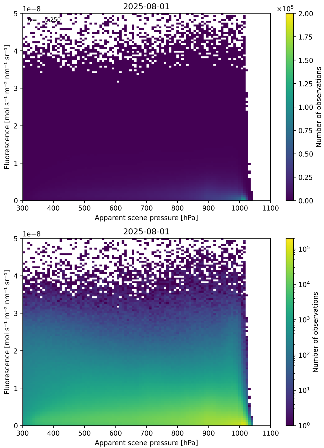
Figure 64: Scatter density plot of “Apparent scene pressure” against “Fluorescence” for 2025-07-31 to 2025-08-02.
