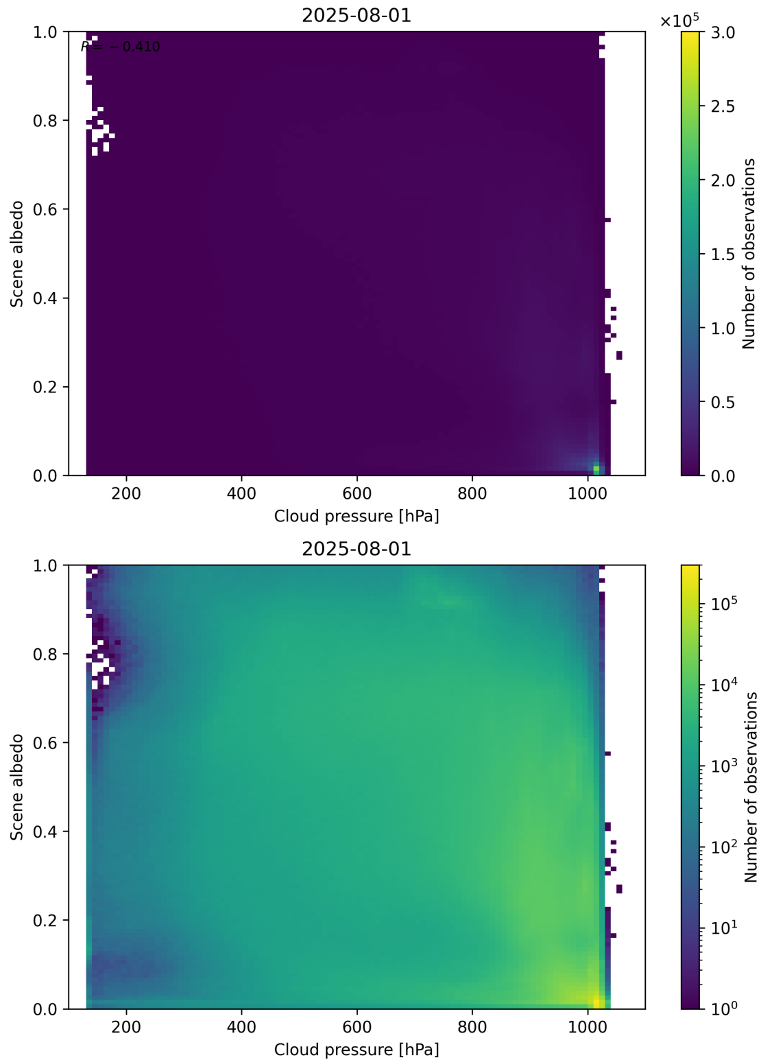
Figure 83: Scatter density plot of “Cloud pressure” against “Scene albedo” for 2025-07-31 to 2025-08-02.
