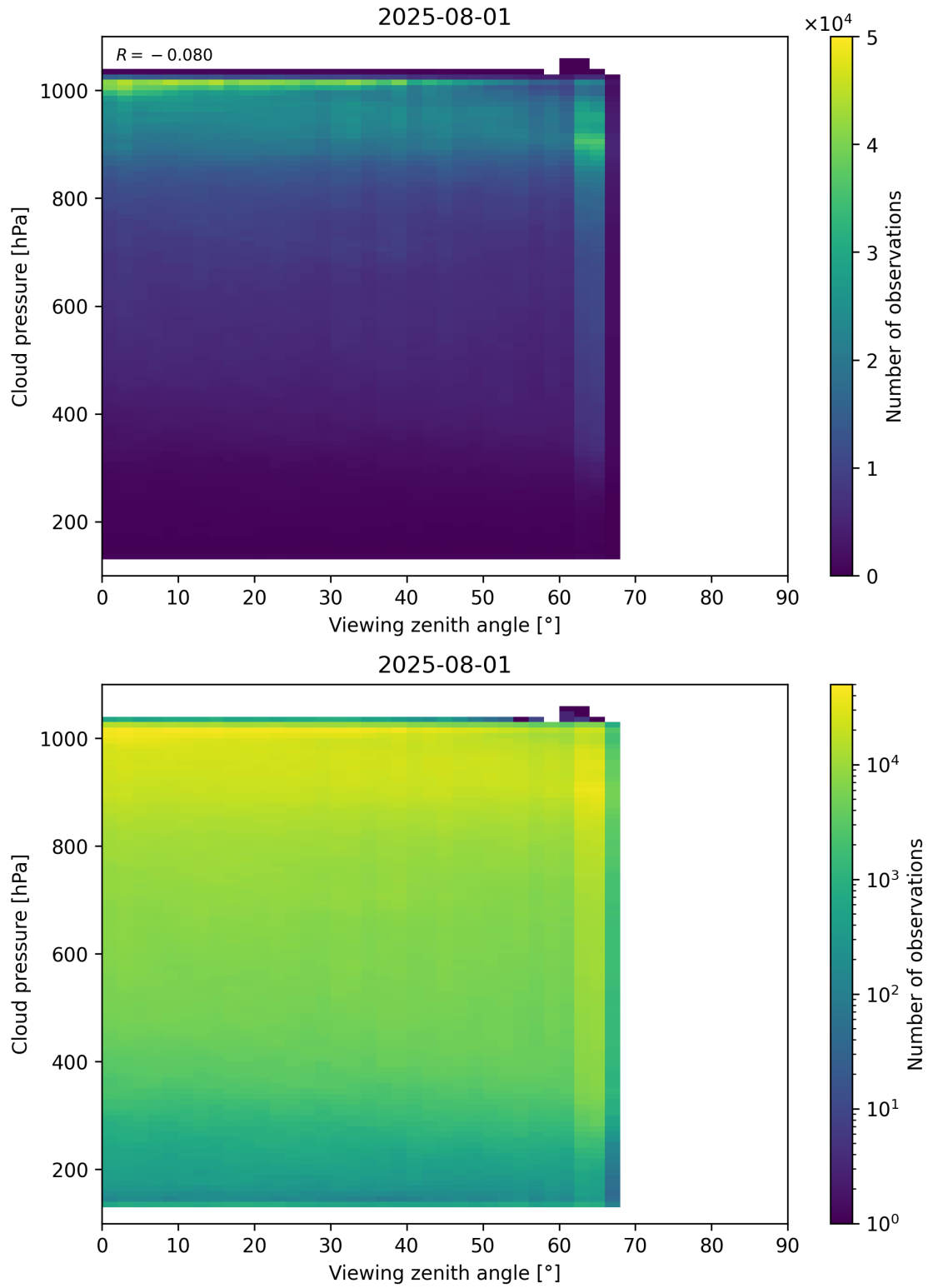
Figure 121: Scatter density plot of “Viewing zenith angle” against “Cloud pressure” for 2025-07-31 to 2025-08-02.
