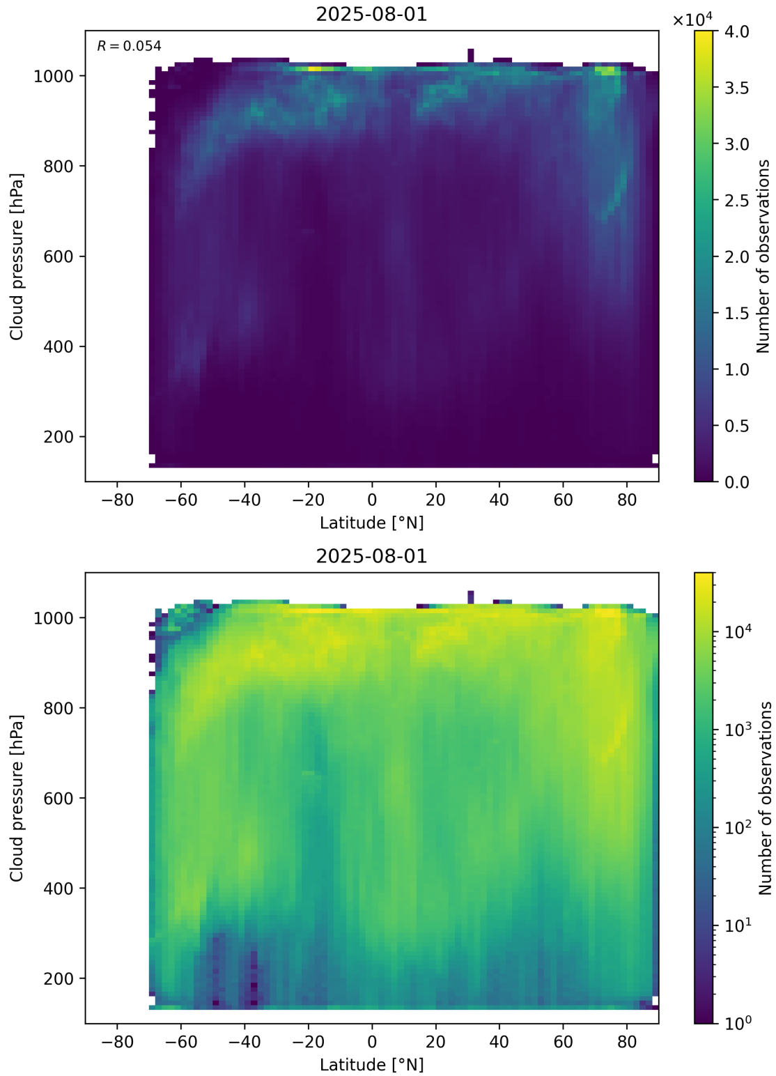
Figure 91: Scatter density plot of “Latitude” against “Cloud pressure” for 2025-07-31 to 2025-08-02.
