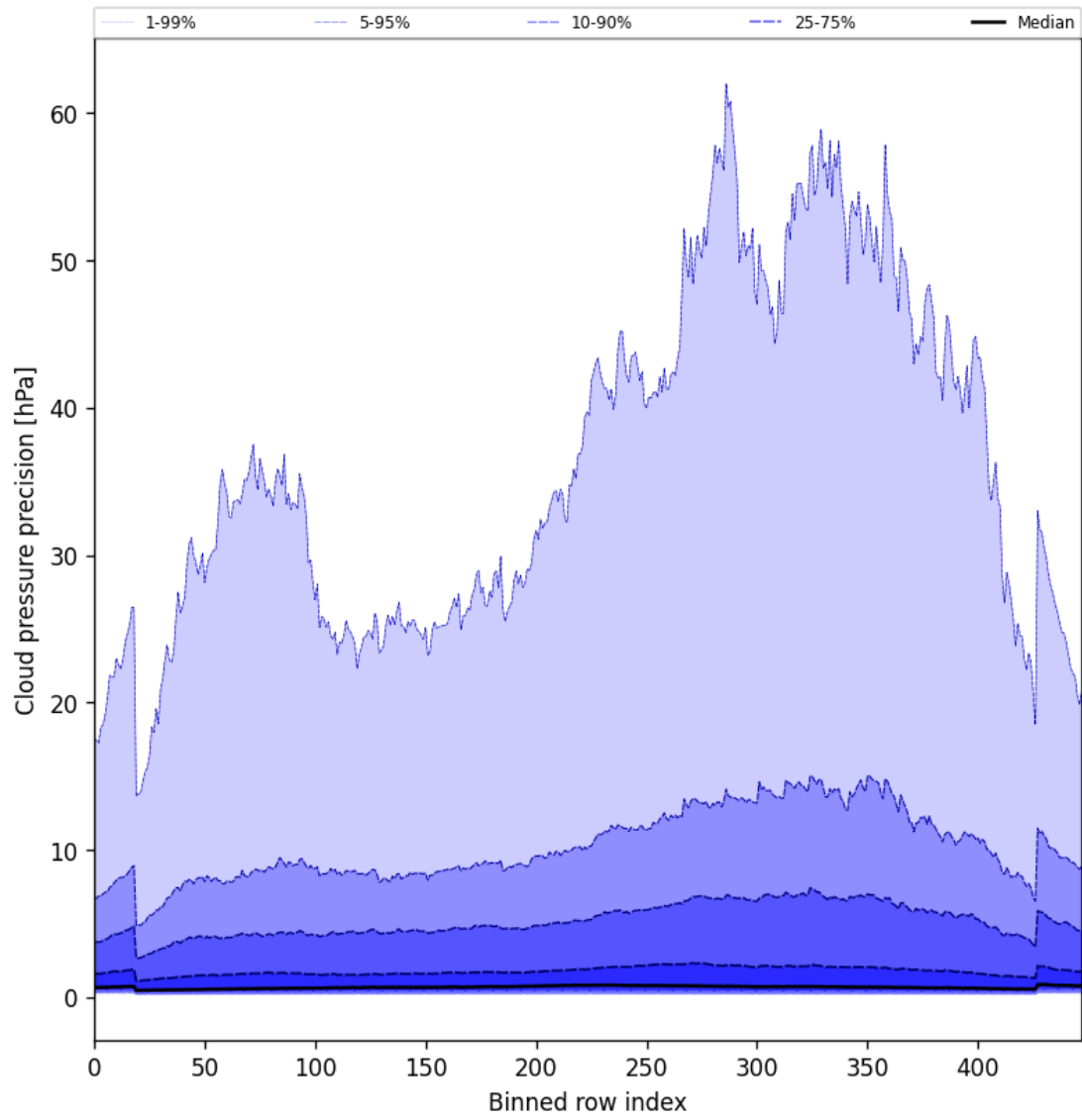
Figure 48: Along track statistics of “Cloud pressure precision” for 2025-07-31 to 2025-08-02
