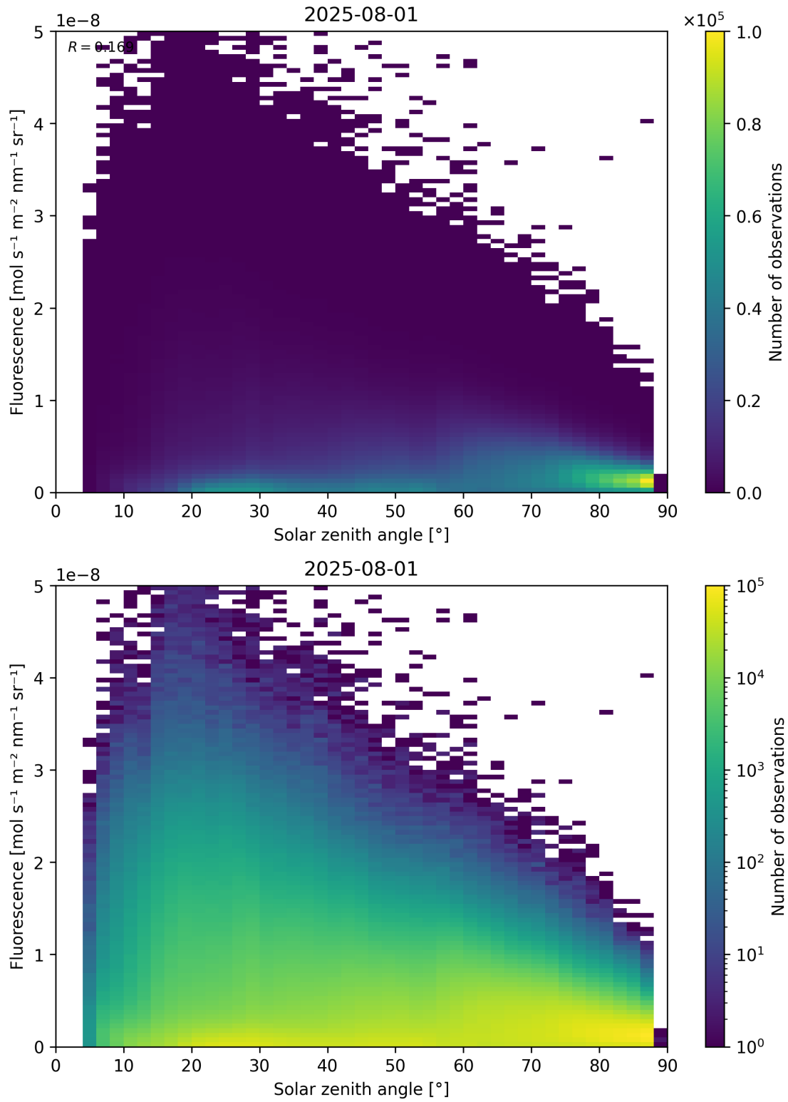
Figure 112: Scatter density plot of “Solar zenith angle” against “Fluorescence” for 2025-07-31 to 2025-08-02.
