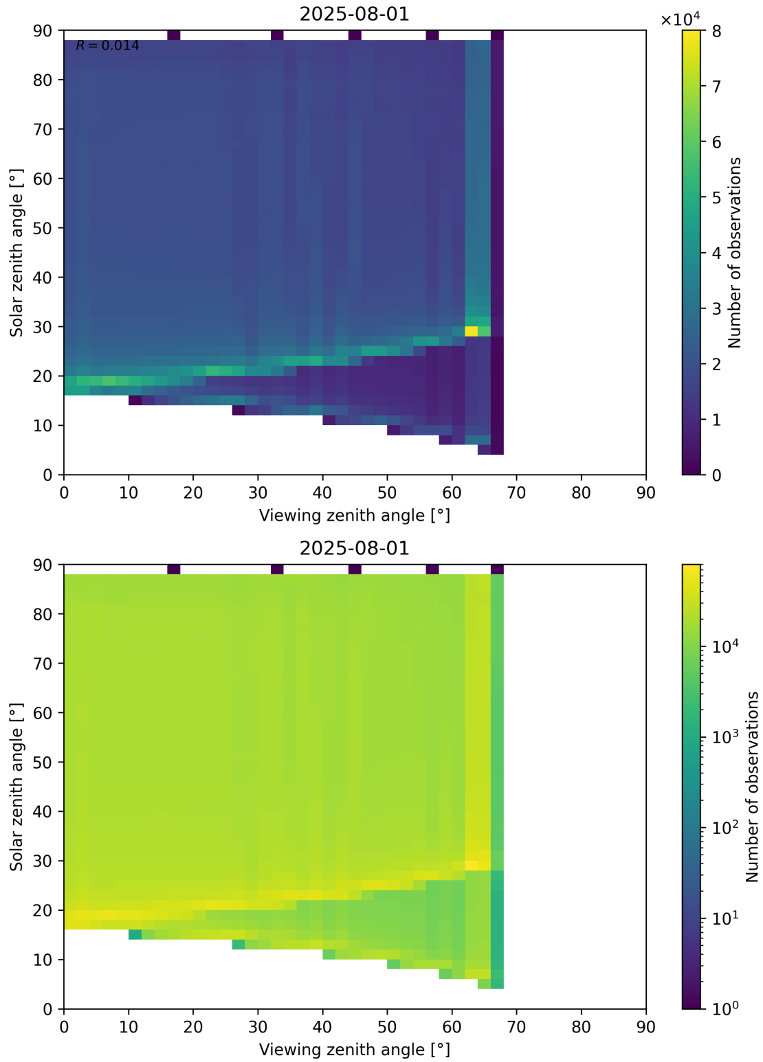
Figure 127: Scatter density plot of “Viewing zenith angle” against “Solar zenith angle” for 2025-07-31 to 2025-08-02.
