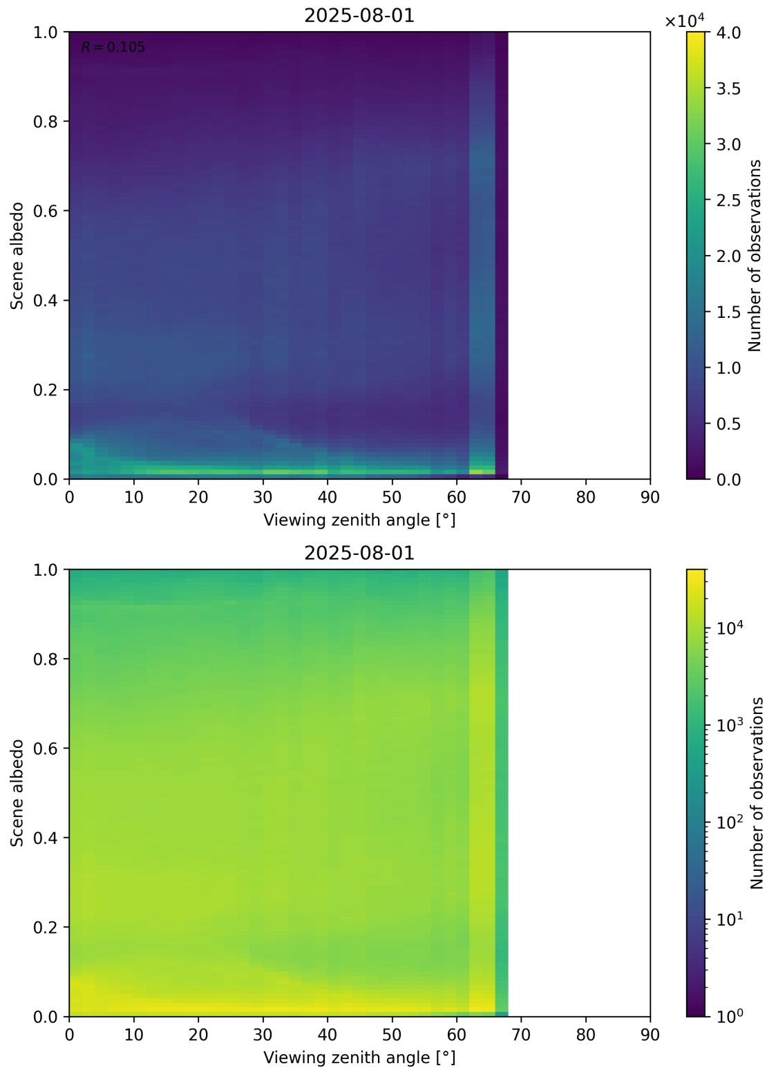
Figure 126: Scatter density plot of “Viewing zenith angle” against “Scene albedo” for 2025-07-31 to 2025-08-02.
