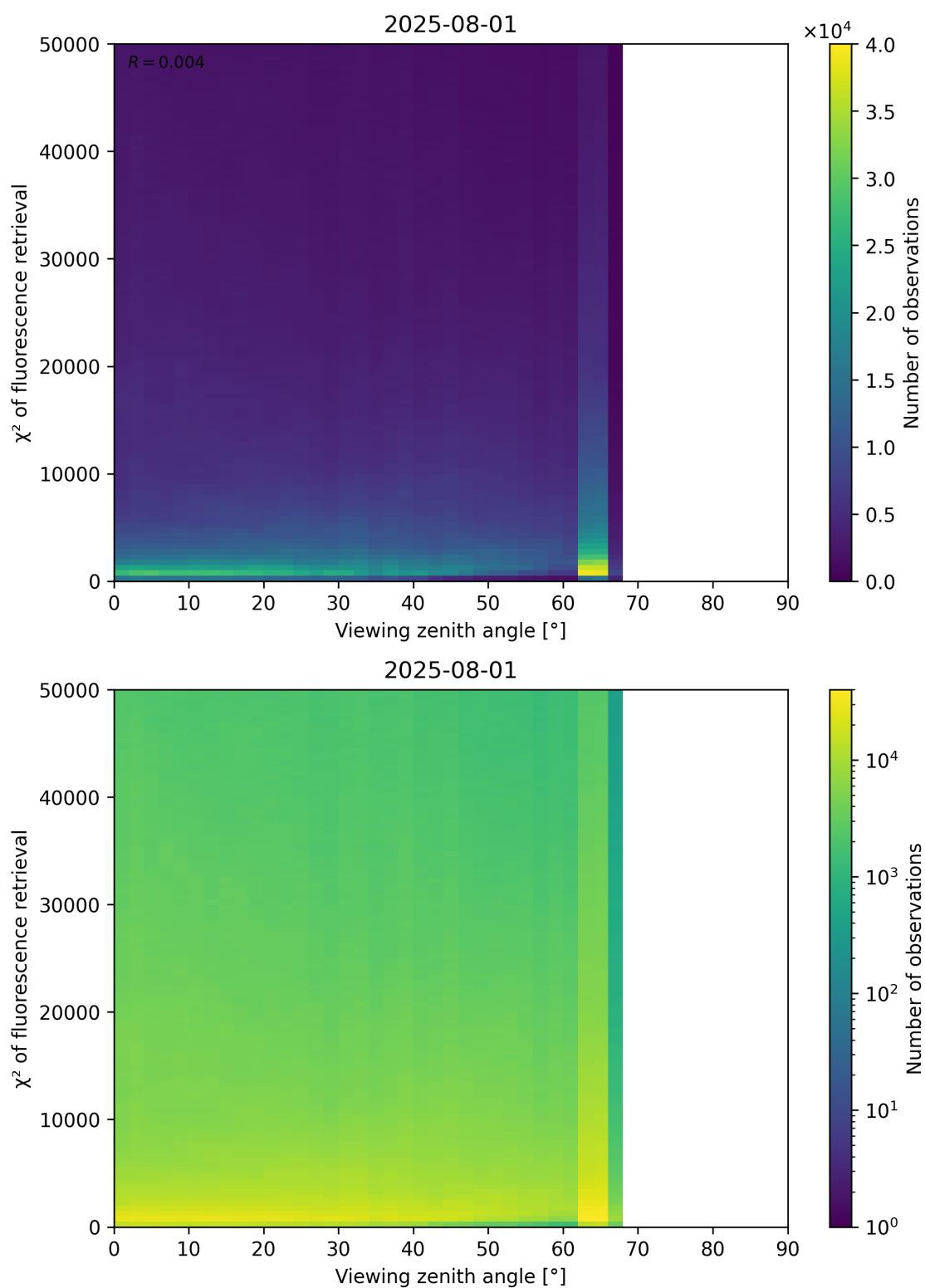
Figure 119: Scatter density plot of “Viewing zenith angle” against “ \chi^2 of fluorescence retrieval” for 2025-07-31 to 2025-08-02.
