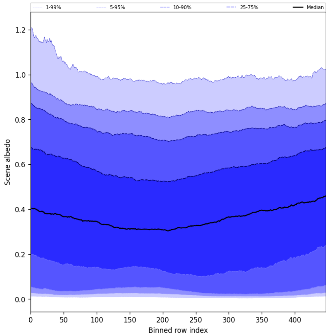
Figure 51: Along track statistics of “Scene albedo” for 2025-07-31 to 2025-08-02
