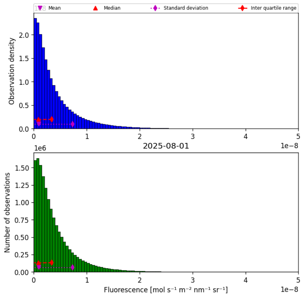
Figure 40: Histogram of “Fluorescence” for 2025-07-31 to 2025-08-02
