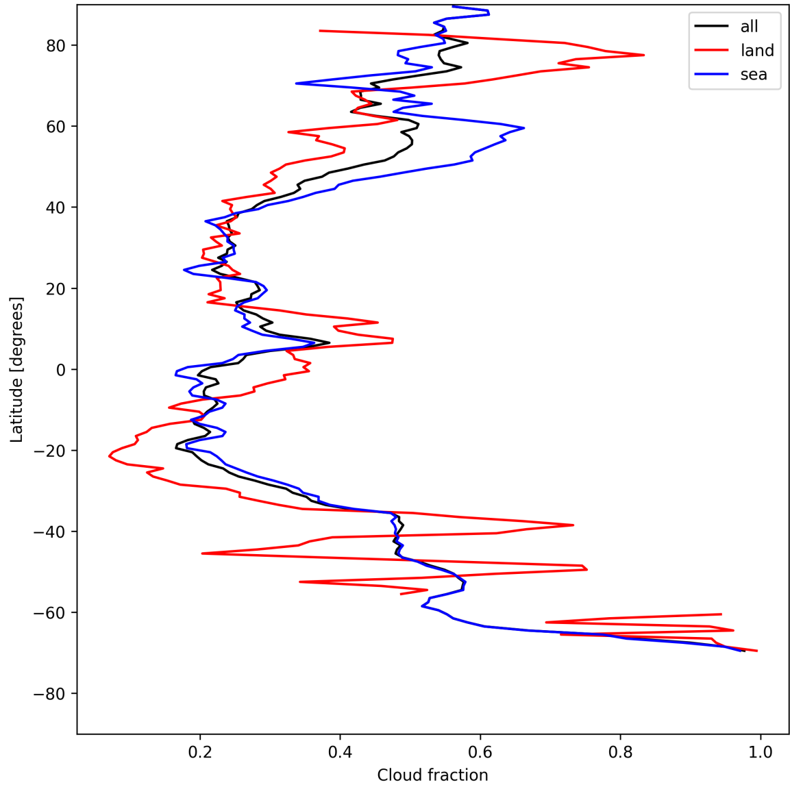
Figure 15: Zonal average of “Cloud fraction” for 2025-07-31 to 2025-08-02.
