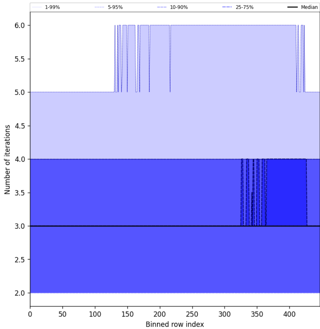
Figure 56: Along track statistics of “Number of iterations” for 2025-07-31 to 2025-08-02
