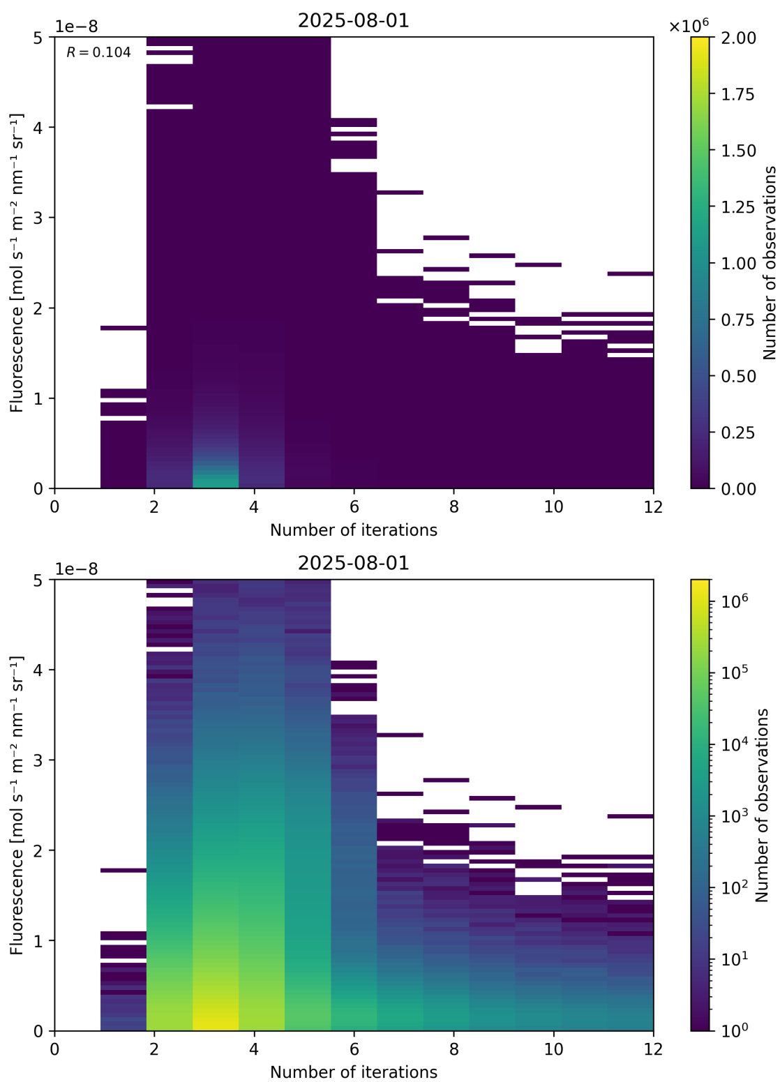
Figure 98: Scatter density plot of “Number of iterations” against “Fluorescence” for 2025-07-31 to 2025-08-02.
