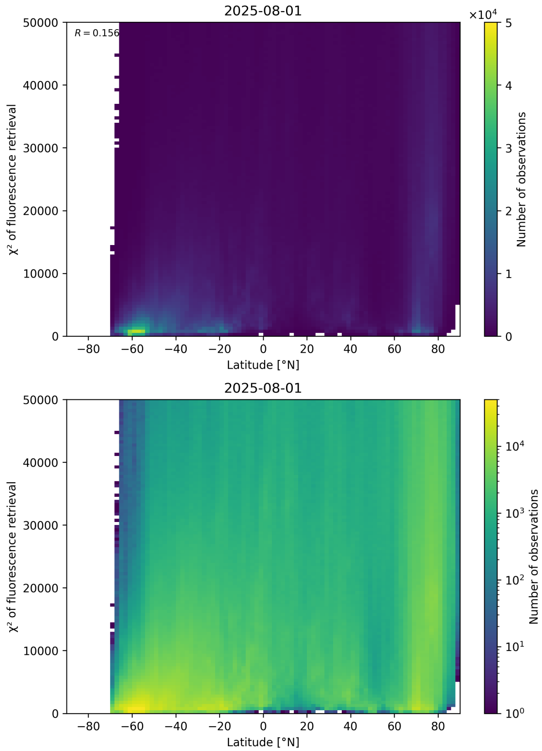
Figure 89: Scatter density plot of “Latitude” against “ \chi^2 of fluorescence retrieval” for 2025-07-31 to 2025-08-02.
