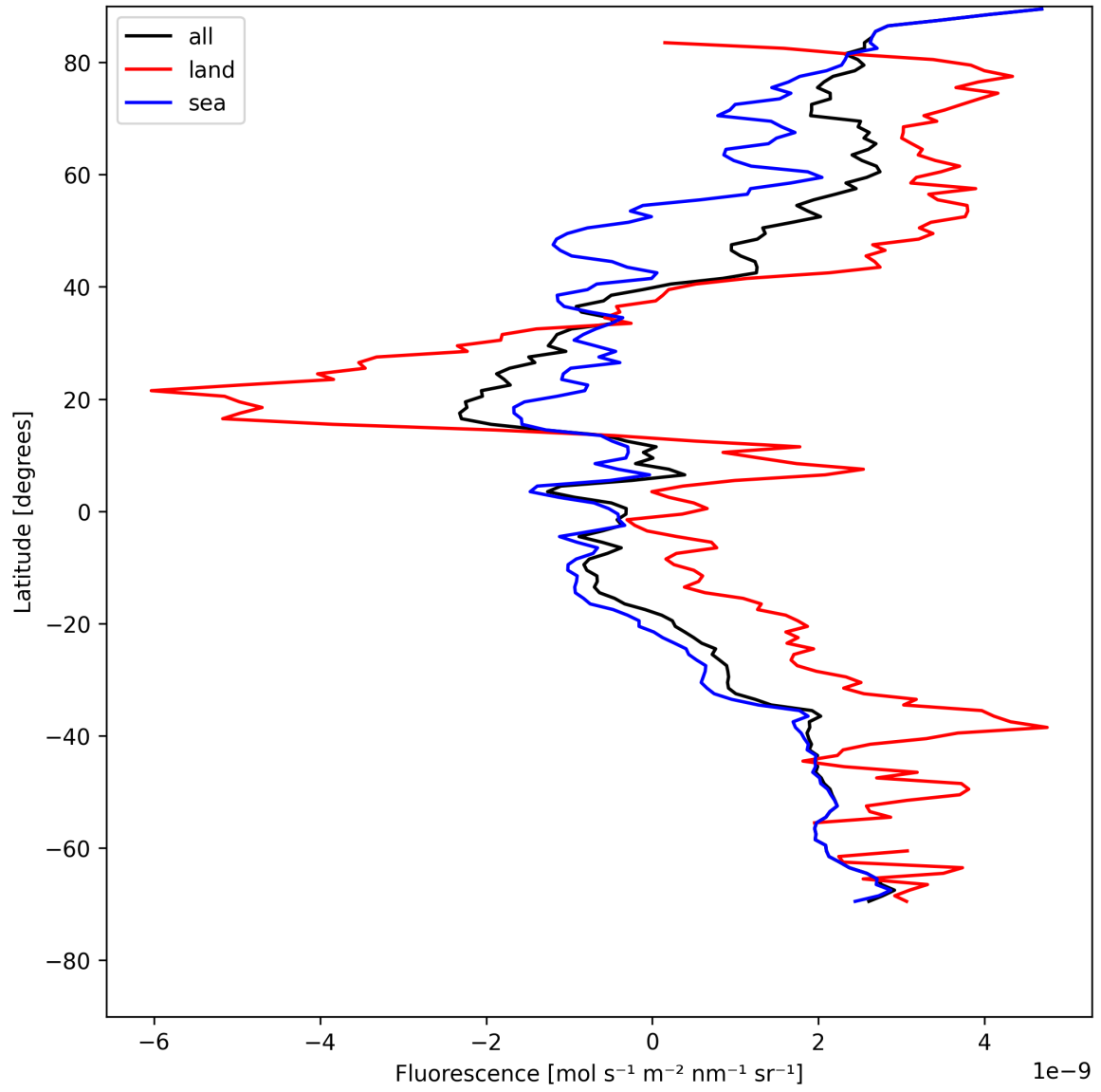
Figure 23: Zonal average of “Fluorescence” for 2025-07-31 to 2025-08-02.
