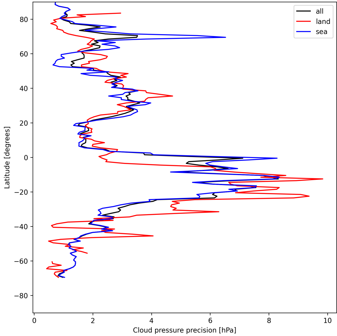
Figure 14: Zonal average of “Cloud pressure precision” for 2025-07-31 to 2025-08-02.
