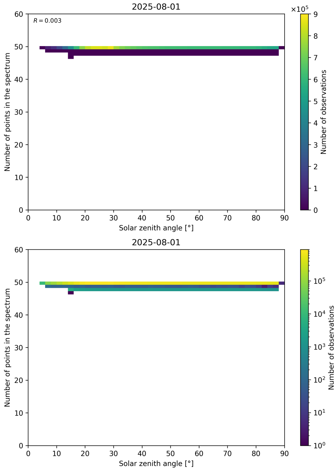
Figure 115: Scatter density plot of “Solar zenith angle” against “Number of points in the spectrum” for 2025-07-31 to 2025-08-02.
