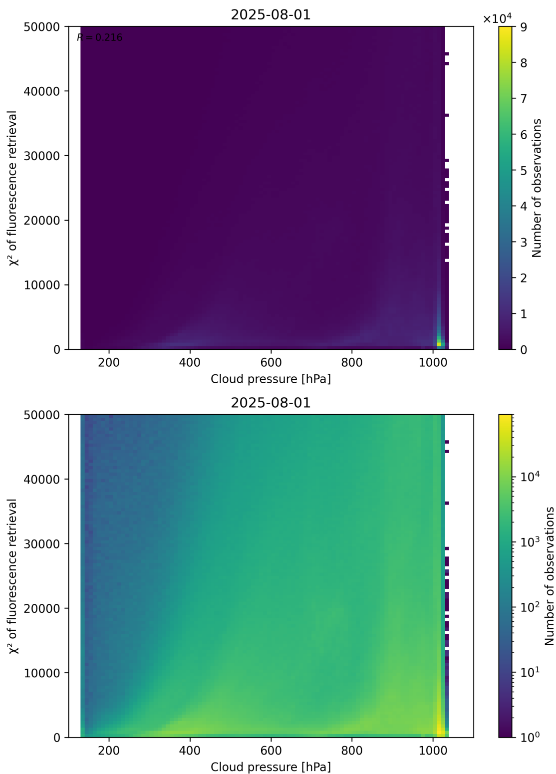
Figure 78: Scatter density plot of “Cloud pressure” against “ \chi^2 of fluorescence retrieval” for 2025-07-31 to 2025-08-02.
