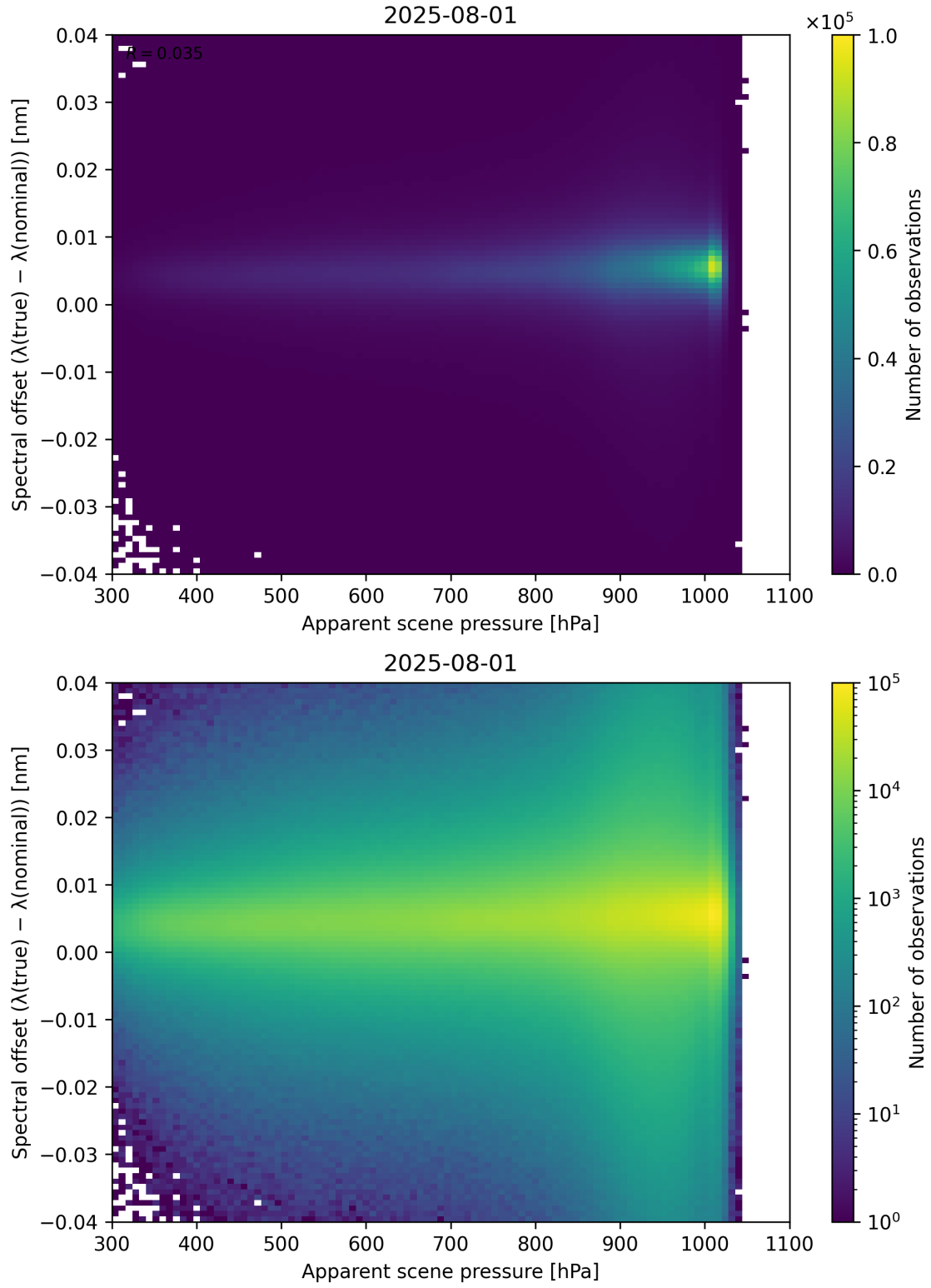
Figure 67: Scatter density plot of “Apparent scene pressure” against “Spectral offset ( \lambda_{\text{true}} - \lambda_{\text{nominal}} )” for 2025-07-31 to 2025-08-02.
