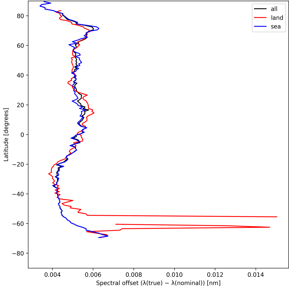
Figure 28: Zonal average of “Spectral offset ( \lambda_{\text{true}} - \lambda_{\text{nominal}} )” for 2025-07-31 to 2025-08-02.
