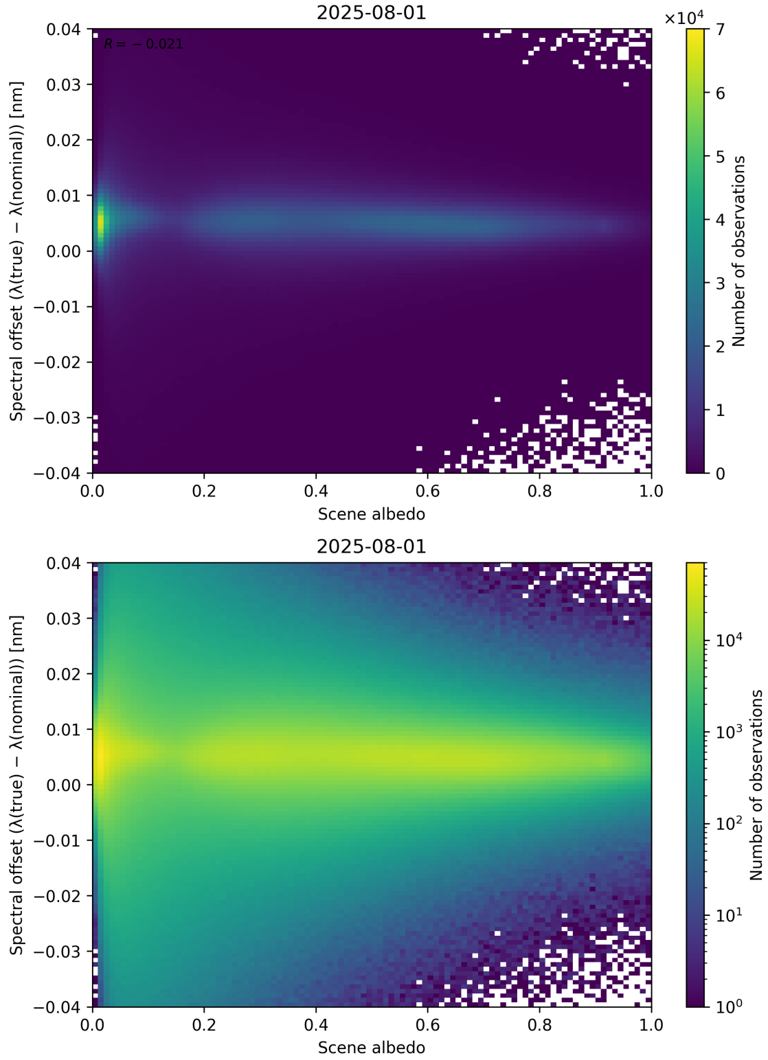
Figure 107: Scatter density plot of “Scene albedo” against “Spectral offset ( \lambda_{\text{true}} - \lambda_{\text{nominal}} )” for 2025-07-31 to 2025-08-02.
