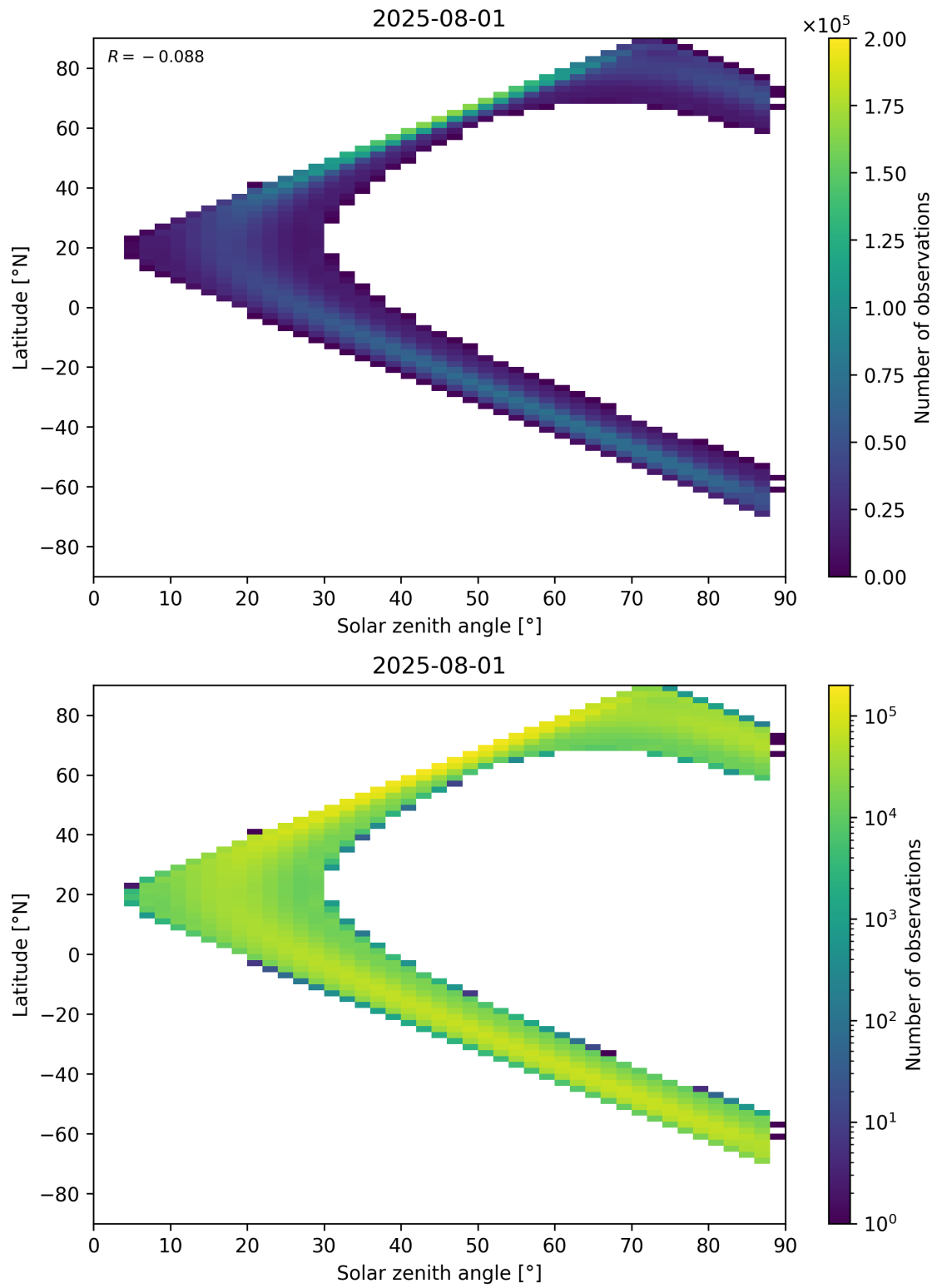
Figure 113: Scatter density plot of “Solar zenith angle” against “Latitude” for 2025-07-31 to 2025-08-02.
