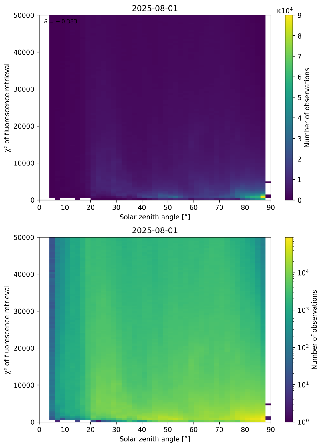
Figure 109: Scatter density plot of “Solar zenith angle” against “ \chi^2 of fluorescence retrieval” for 2025-07-31 to 2025-08-02.
