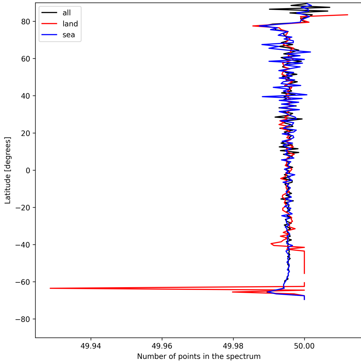
Figure 27: Zonal average of “Number of points in the spectrum” for 2025-07-31 to 2025-08-02.
