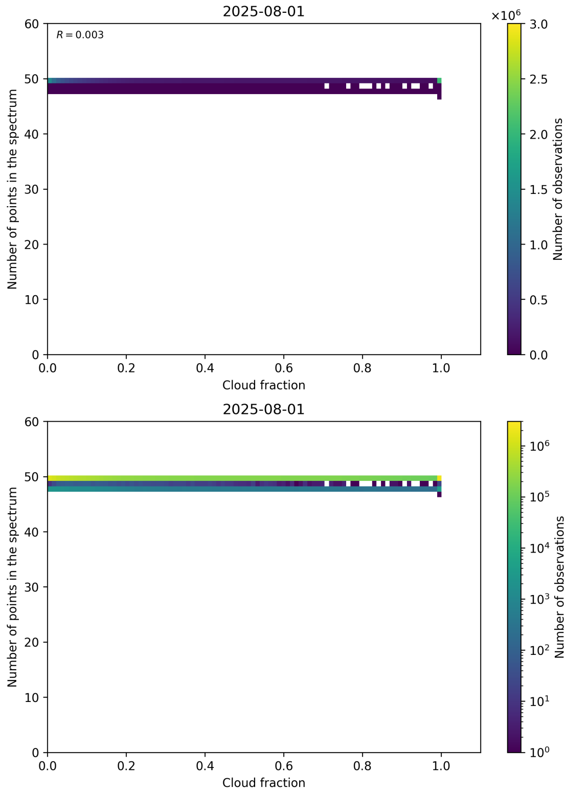
Figure 74: Scatter density plot of “Cloud fraction” against “Number of points in the spectrum” for 2025-07-31 to 2025-08-02.
