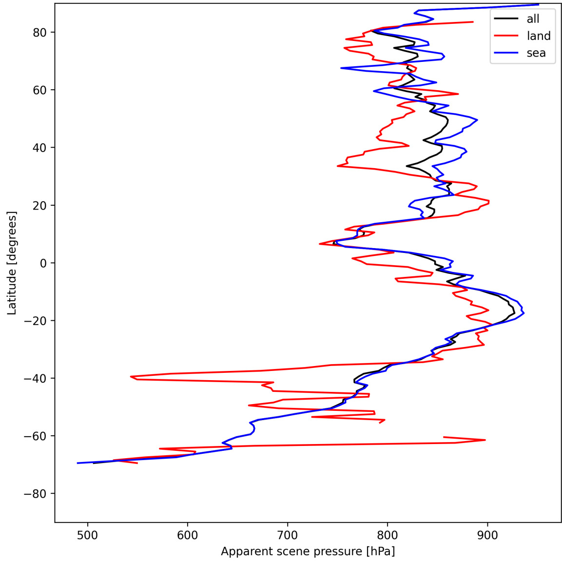
Figure 19: Zonal average of “Apparent scene pressure” for 2025-07-31 to 2025-08-02.
