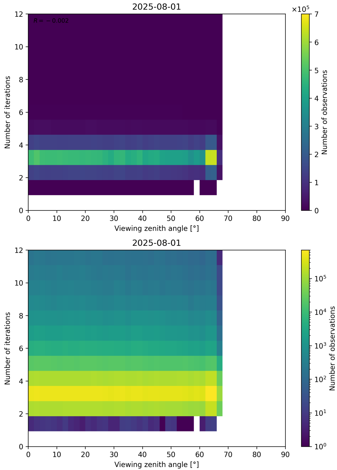
Figure 124: Scatter density plot of “Viewing zenith angle” against “Number of iterations” for 2025-07-31 to 2025-08-02.
