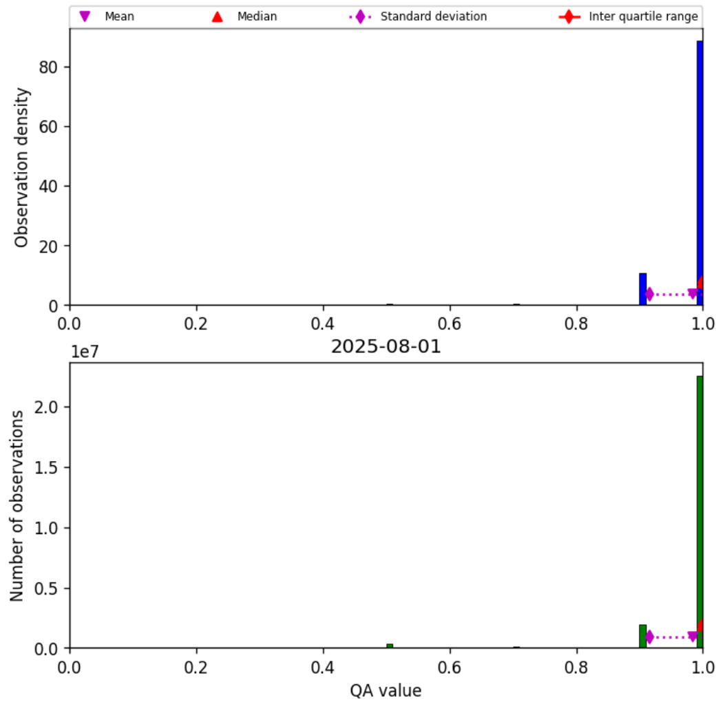
Figure 29: Histogram of “QA value” for 2025-07-31 to 2025-08-02
