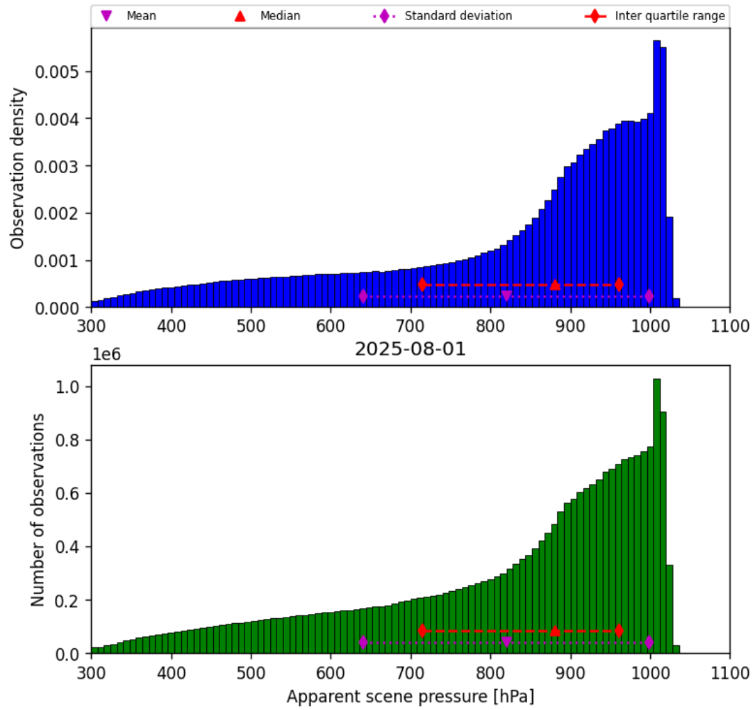
Figure 36: Histogram of “Apparent scene pressure” for 2025-07-31 to 2025-08-02
