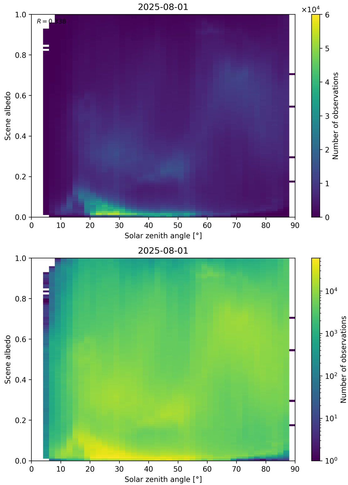
Figure 116: Scatter density plot of “Solar zenith angle” against “Scene albedo” for 2025-07-31 to 2025-08-02.
