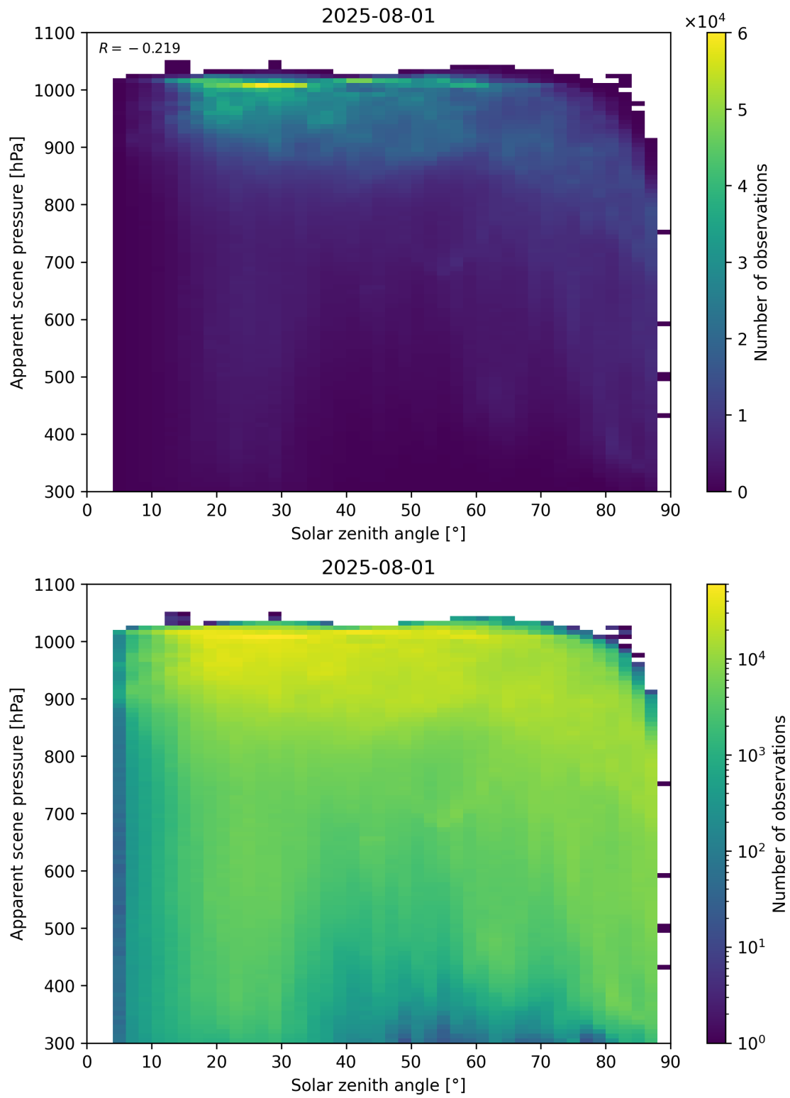
Figure 108: Scatter density plot of “Solar zenith angle” against “Apparent scene pressure” for 2025-07-31 to 2025-08-02.
