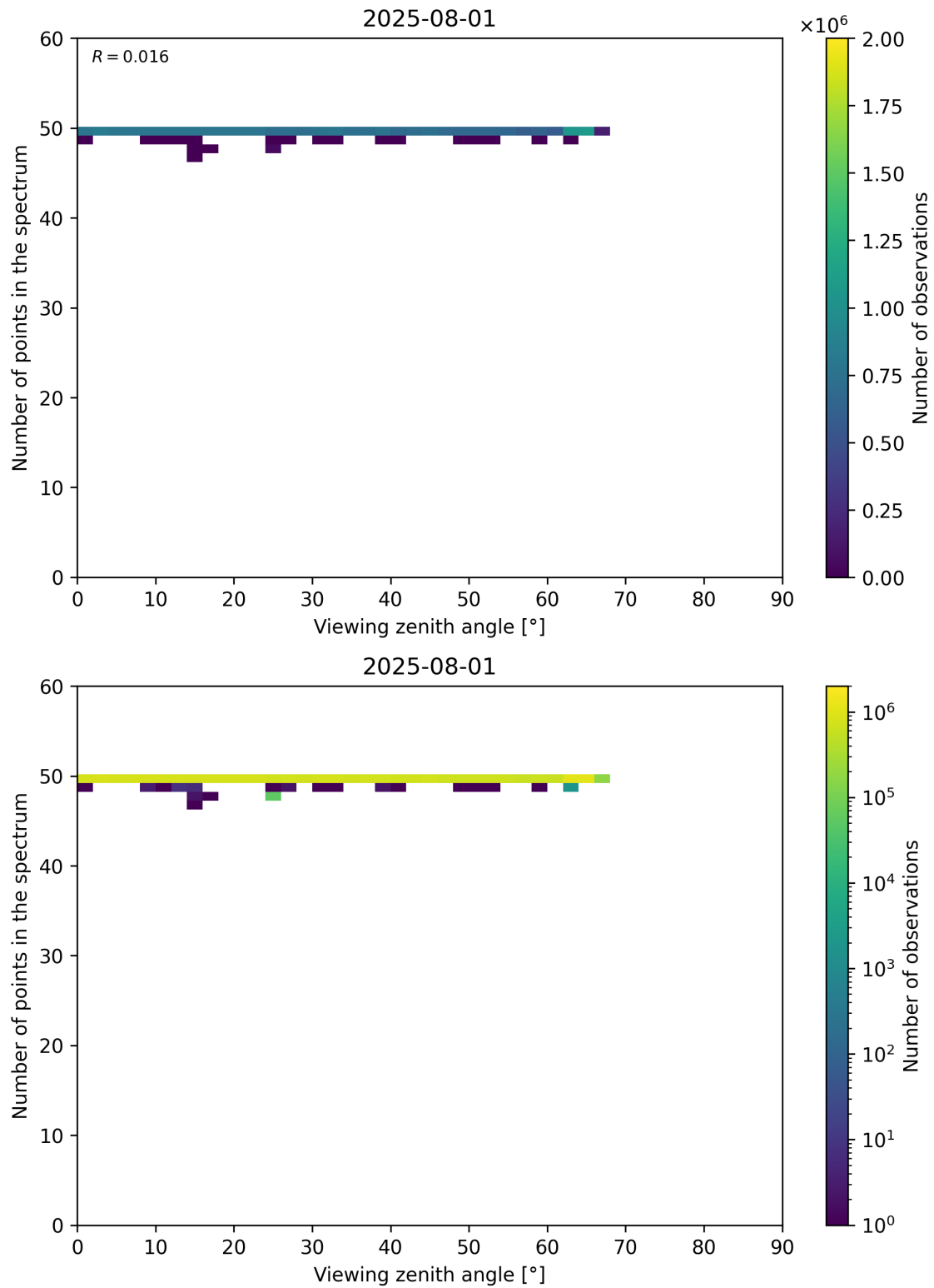
Figure 125: Scatter density plot of “Viewing zenith angle” against “Number of points in the spectrum” for 2025-07-31 to 2025-08-02.
