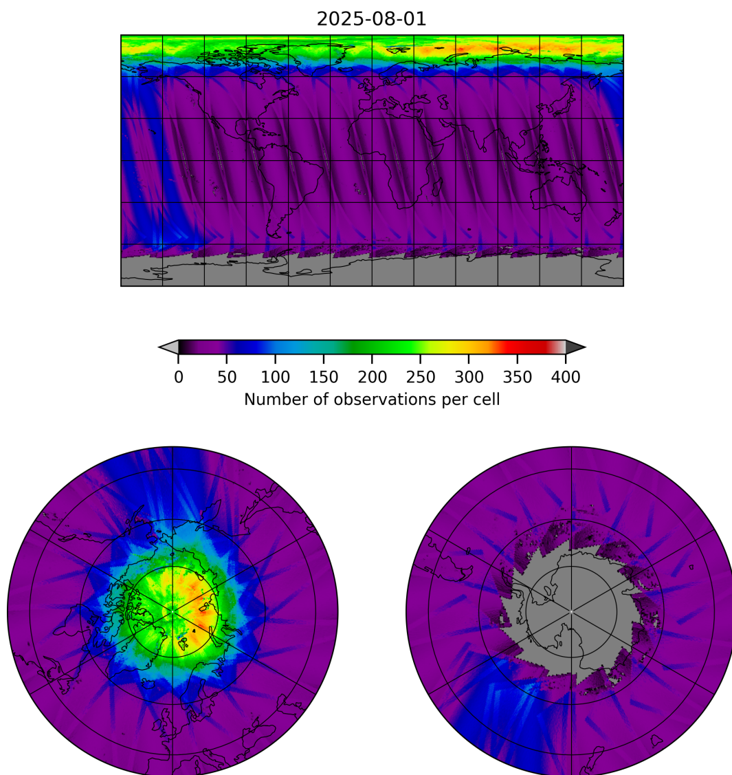
Figure 11: Map of the number of observations for 2025-07-31 to 2025-08-02
