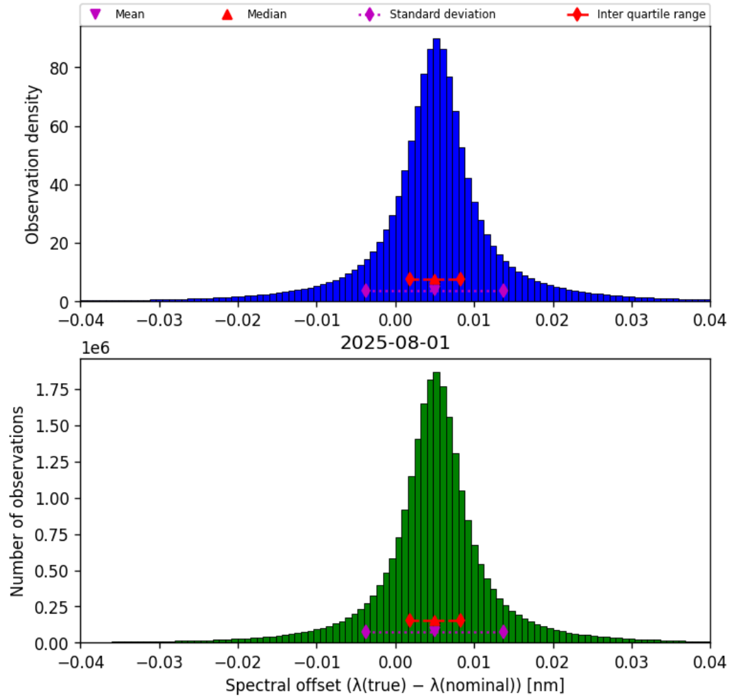
Figure 45: Histogram of “Spectral offset ( \lambda_{\text{true}} - \lambda_{\text{nominal}} )” for 2025-07-31 to 2025-08-02
