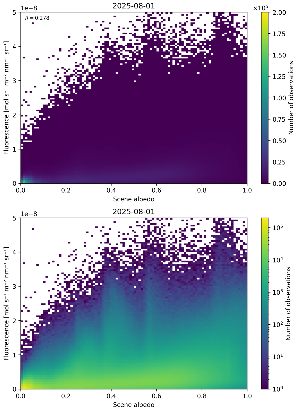
Figure 104: Scatter density plot of “Scene albedo” against “Fluorescence” for 2025-07-31 to 2025-08-02.
