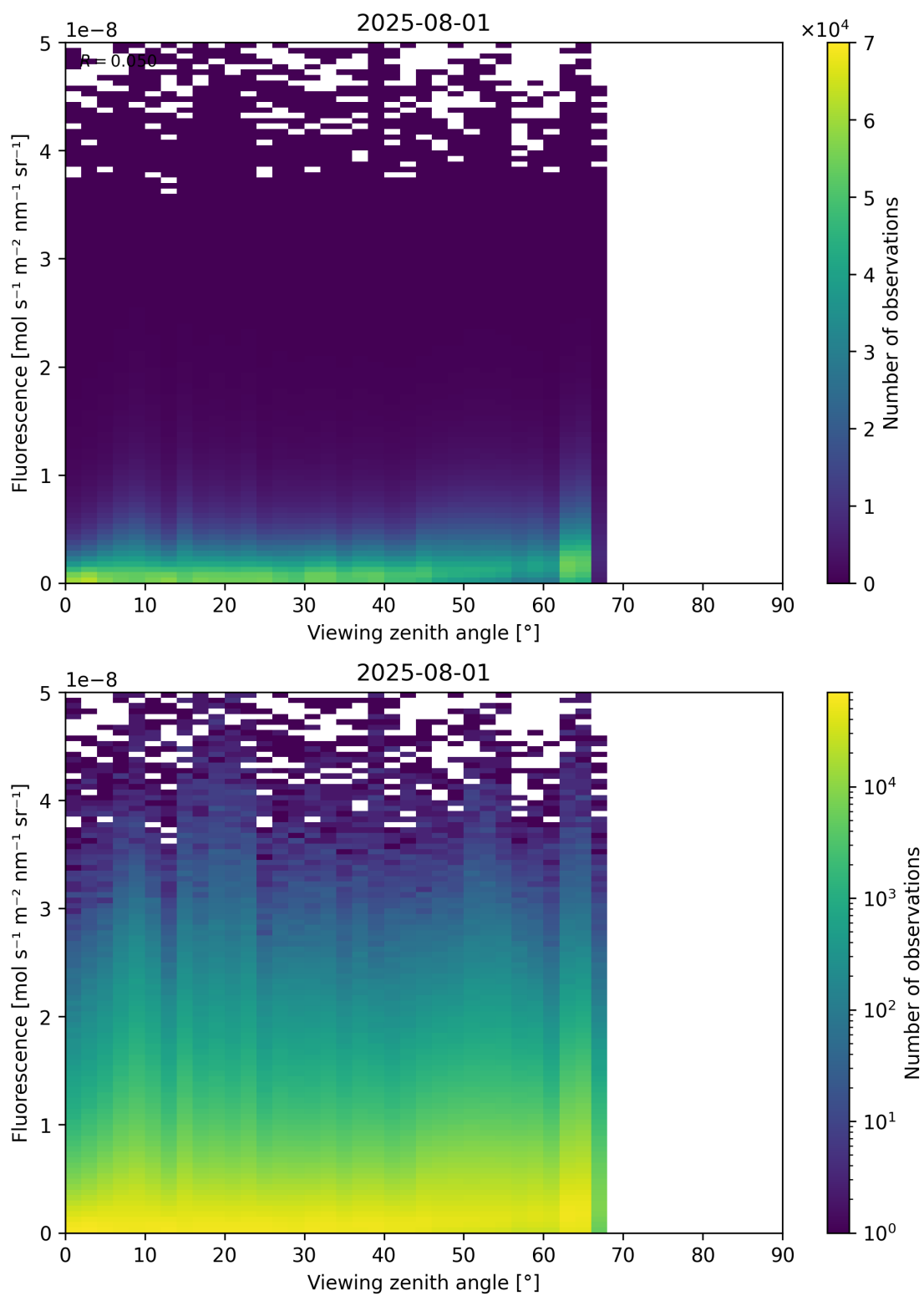
Figure 122: Scatter density plot of “Viewing zenith angle” against “Fluorescence” for 2025-07-31 to 2025-08-02.
