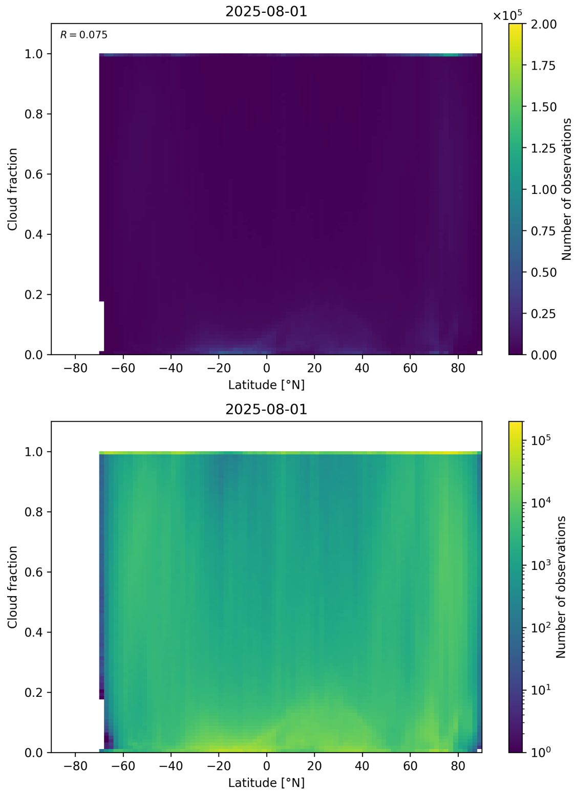
Figure 90: Scatter density plot of “Latitude” against “Cloud fraction” for 2025-07-31 to 2025-08-02.
