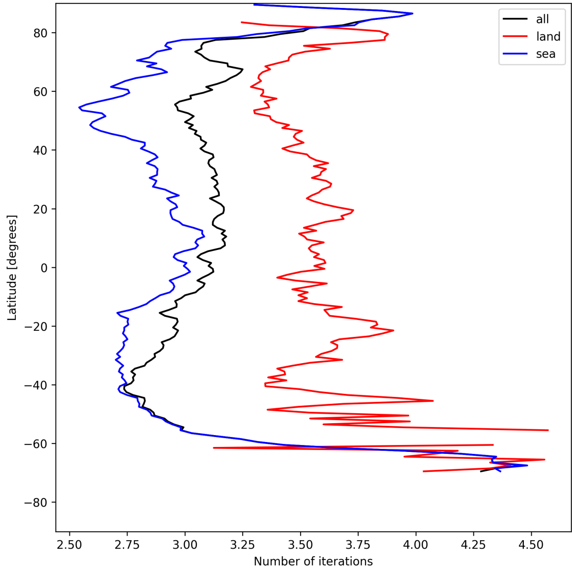
Figure 22: Zonal average of “Number of iterations” for 2025-07-31 to 2025-08-02.
