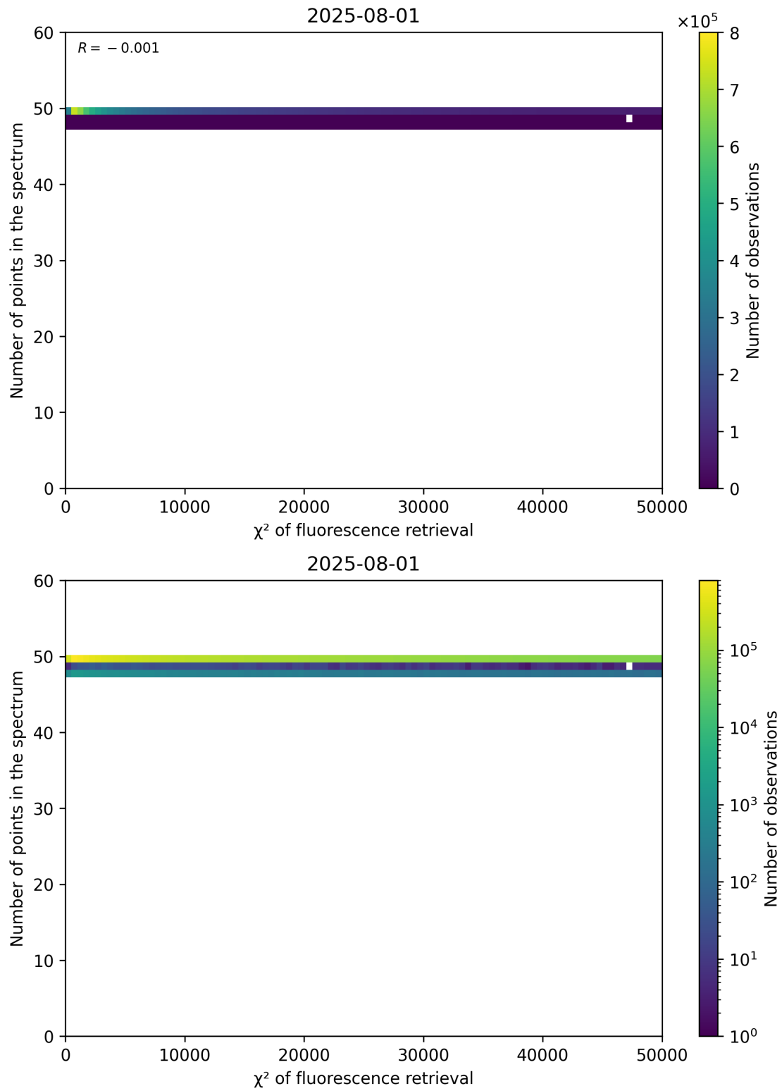
Figure 68: Scatter density plot of “ \chi^2 of fluorescence retrieval” against “Number of points in the spectrum” for 2025-07-31 to 2025-08-02.
