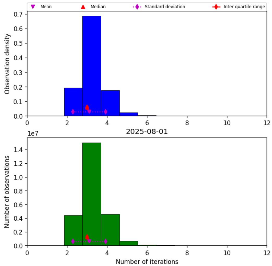
Figure 39: Histogram of “Number of iterations” for 2025-07-31 to 2025-08-02
