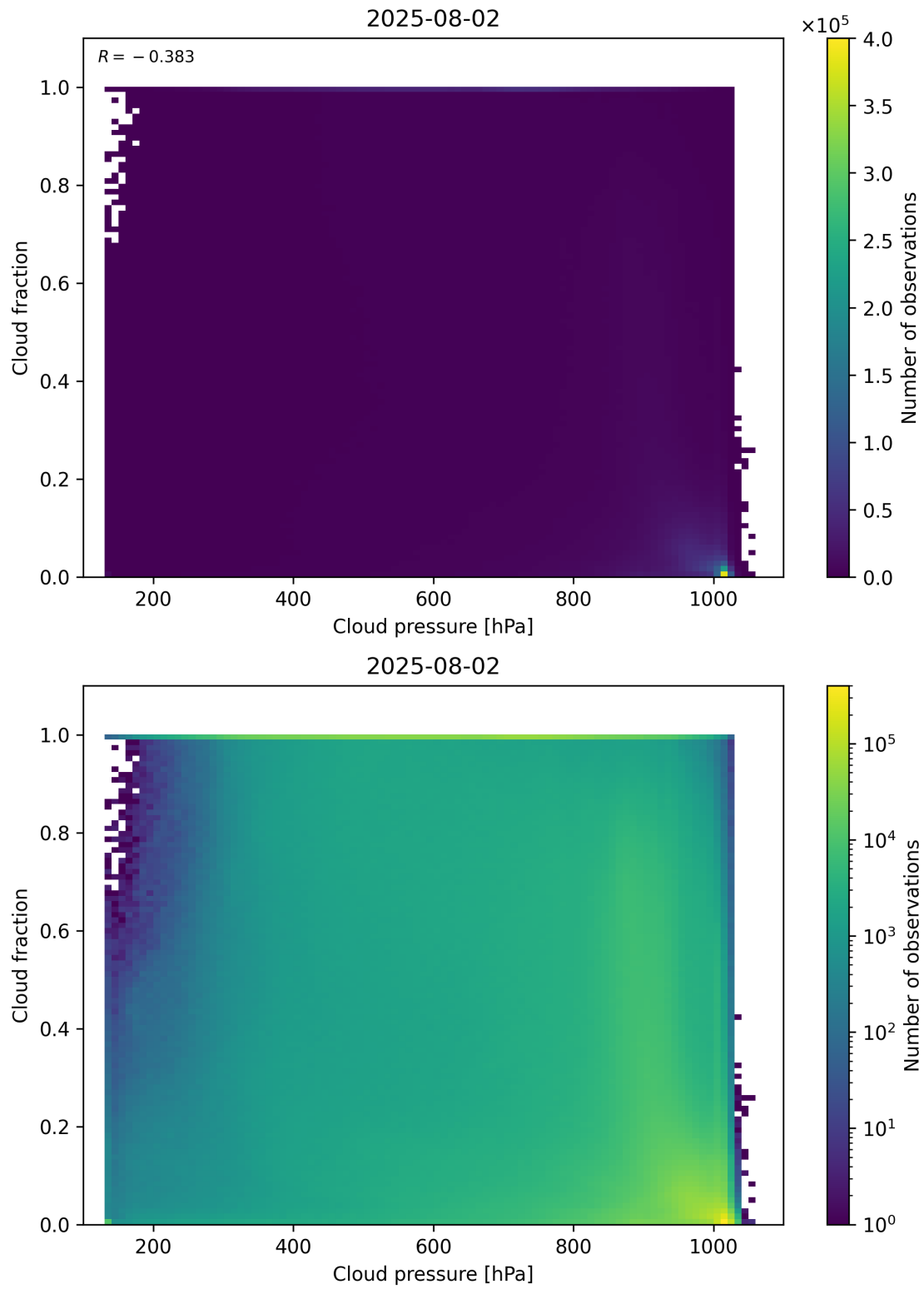
Figure 79: Scatter density plot of “Cloud pressure” against “Cloud fraction” for 2025-08-01 to 2025-08-03.
