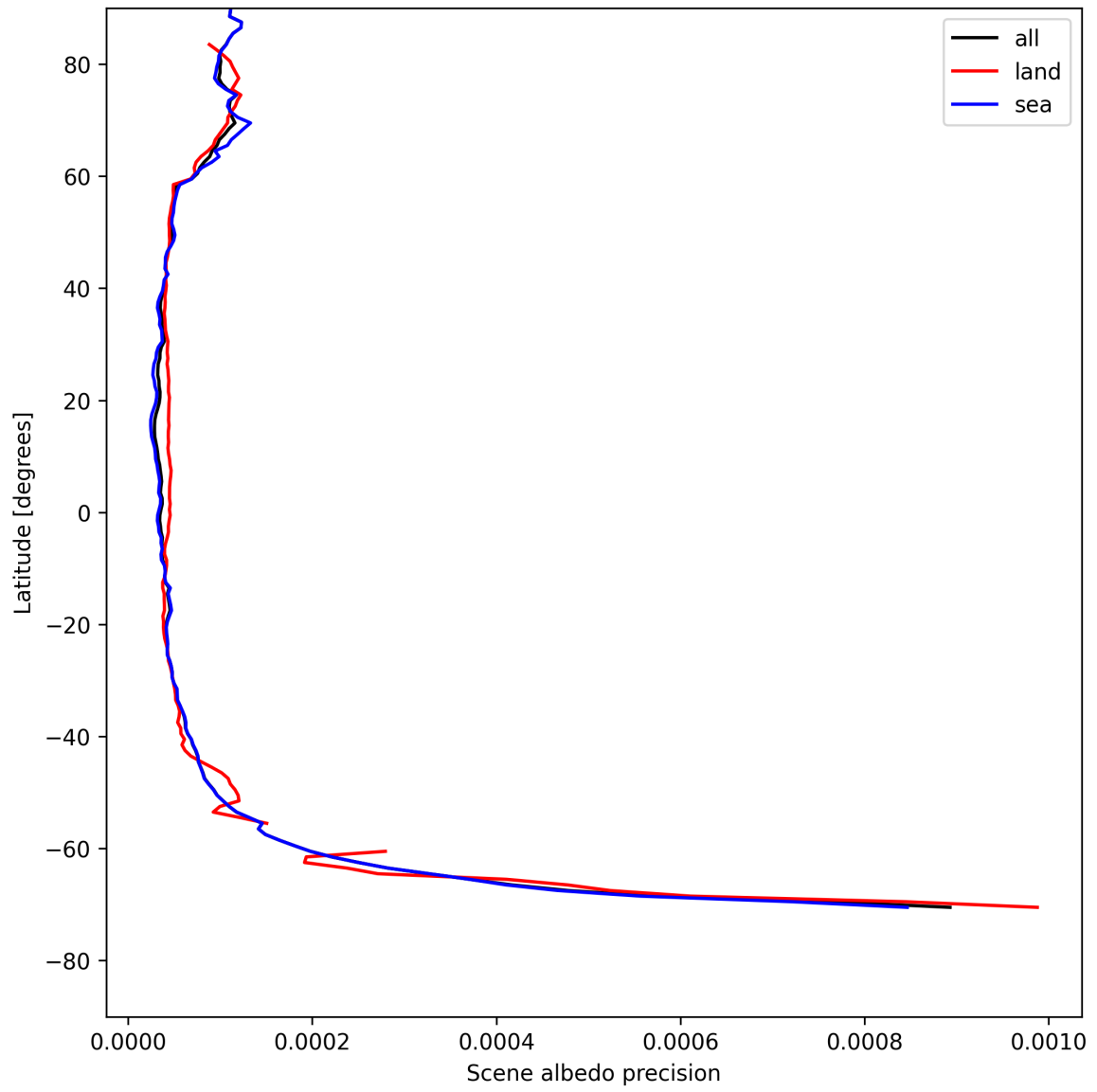
Figure 18: Zonal average of “Scene albedo precision” for 2025-08-01 to 2025-08-03.
