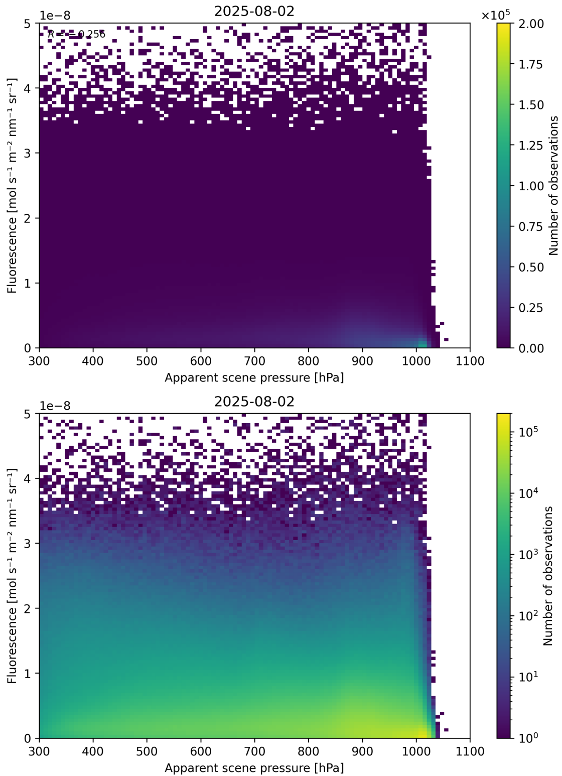
Figure 64: Scatter density plot of “Apparent scene pressure” against “Fluorescence” for 2025-08-01 to 2025-08-03.
