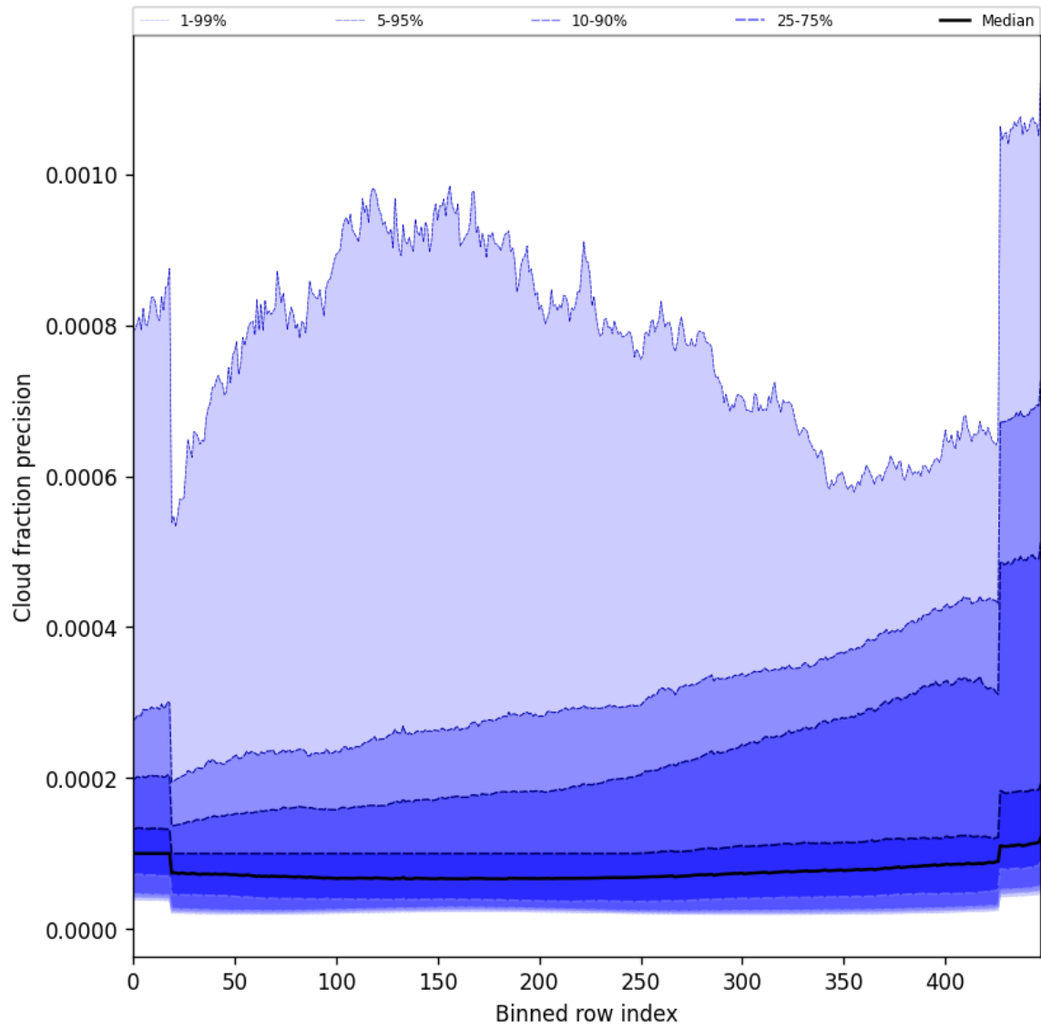
Figure 50: Along track statistics of “Cloud fraction precision” for 2025-08-01 to 2025-08-03
