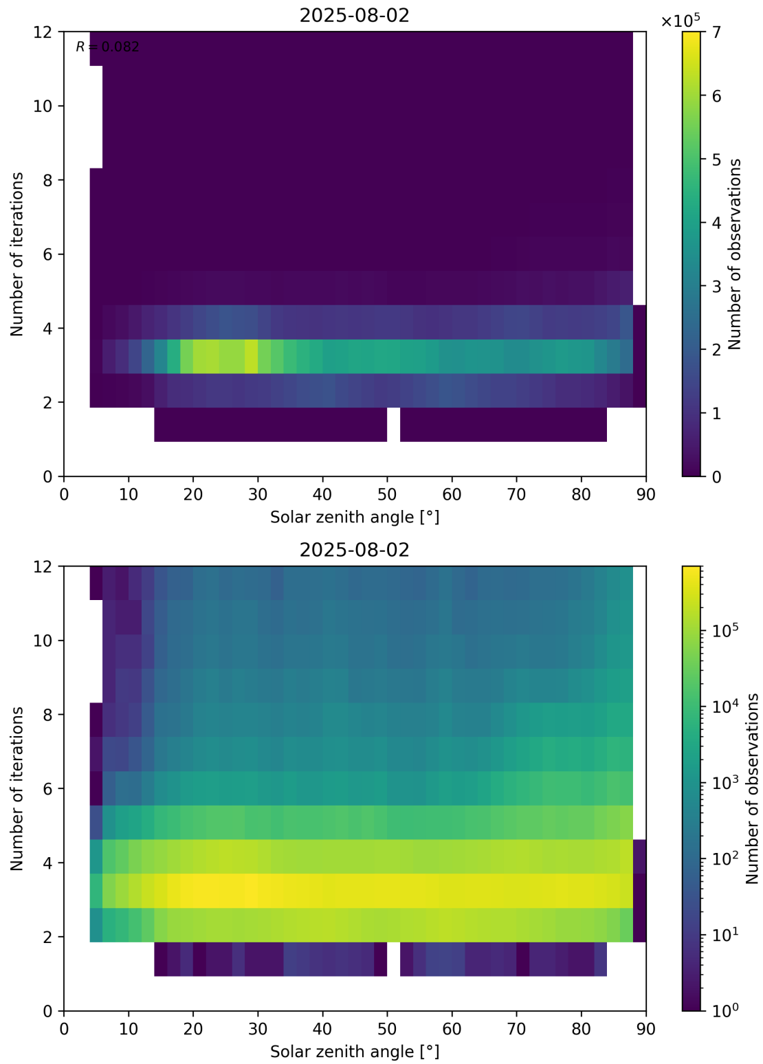
Figure 114: Scatter density plot of “Solar zenith angle” against “Number of iterations” for 2025-08-01 to 2025-08-03.
