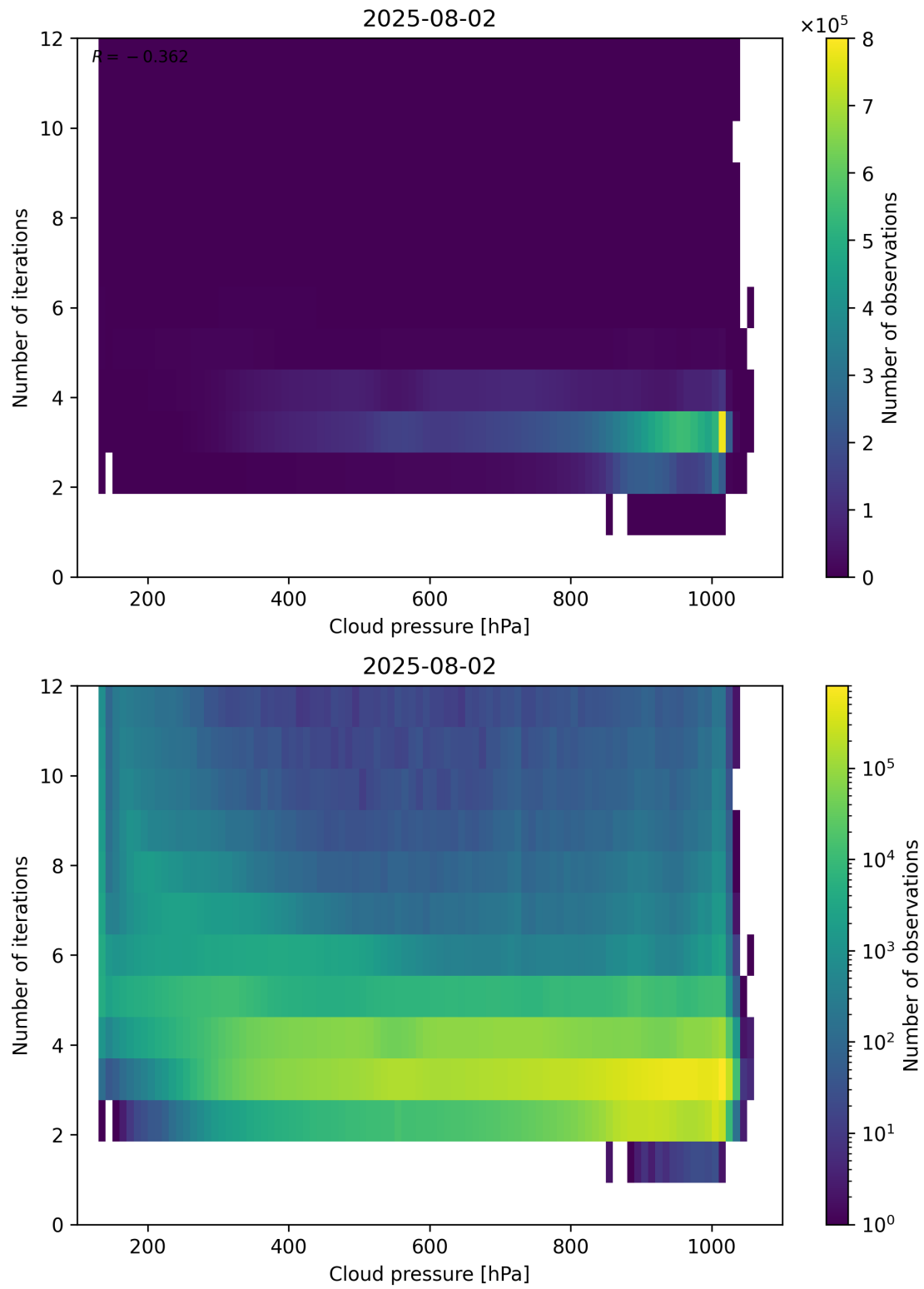
Figure 81: Scatter density plot of “Cloud pressure” against “Number of iterations” for 2025-08-01 to 2025-08-03.
