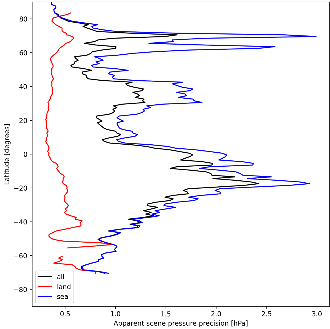
Figure 20: Zonal average of “Apparent scene pressure precision” for 2025-08-01 to 2025-08-03.
