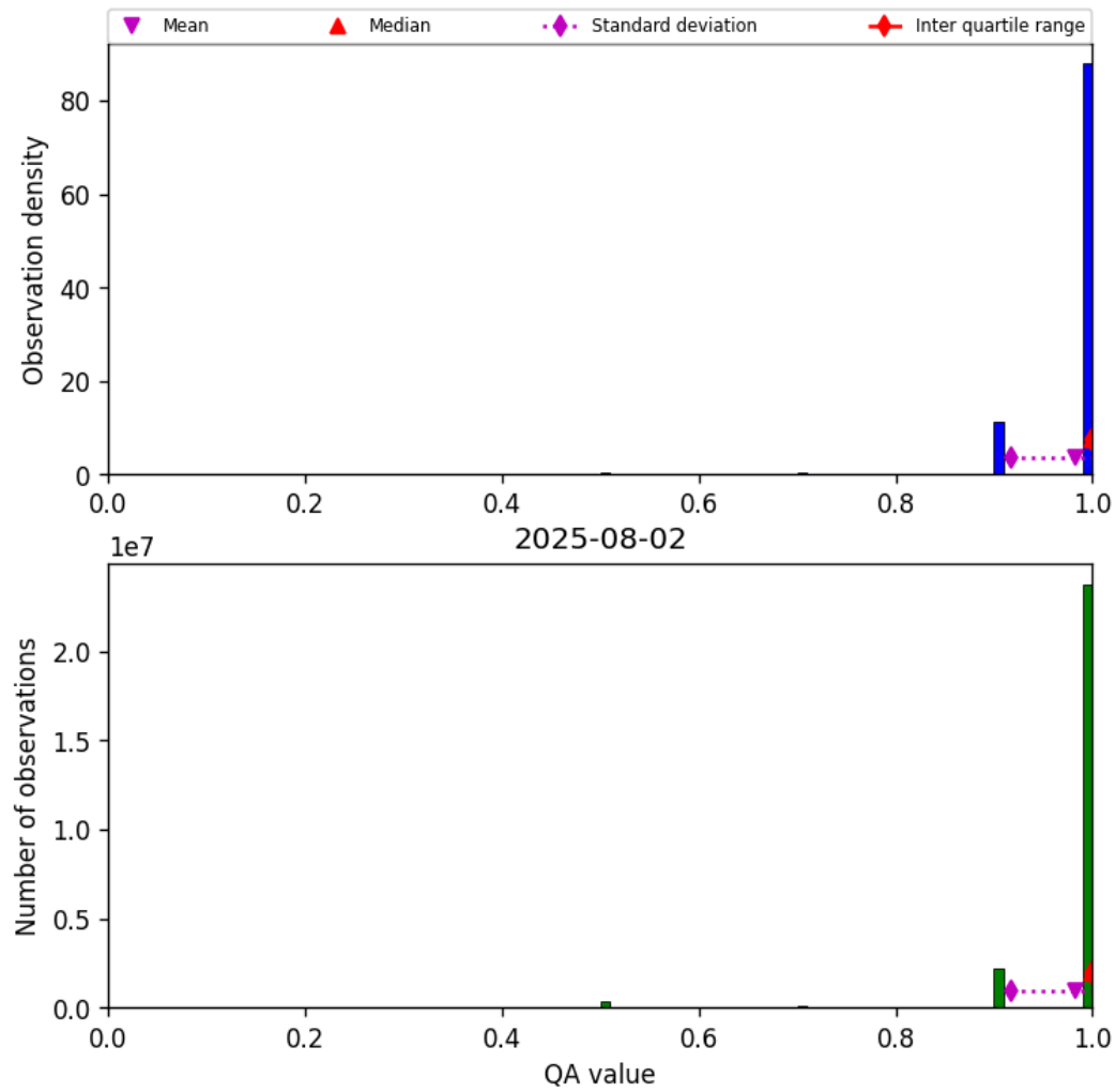
Figure 29: Histogram of “QA value” for 2025-08-01 to 2025-08-03
