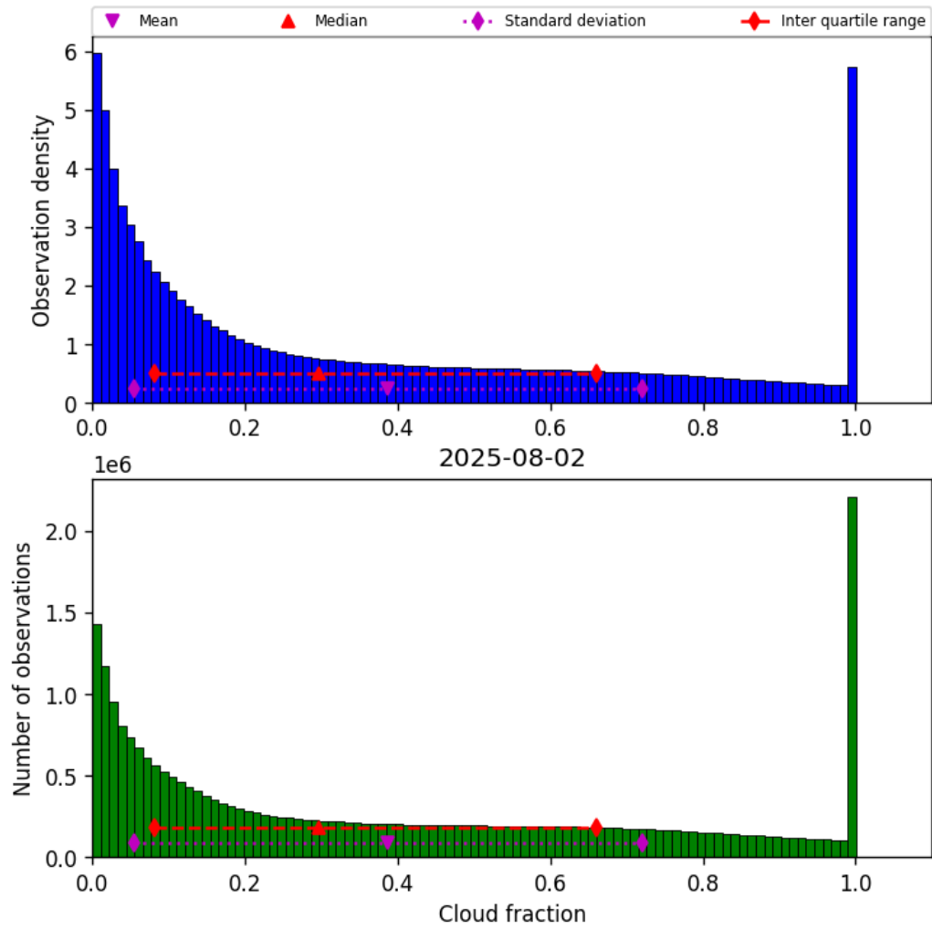
Figure 32: Histogram of “Cloud fraction” for 2025-08-01 to 2025-08-03
