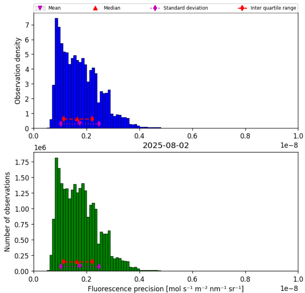
Figure 41: Histogram of “Fluorescence precision” for 2025-08-01 to 2025-08-03
