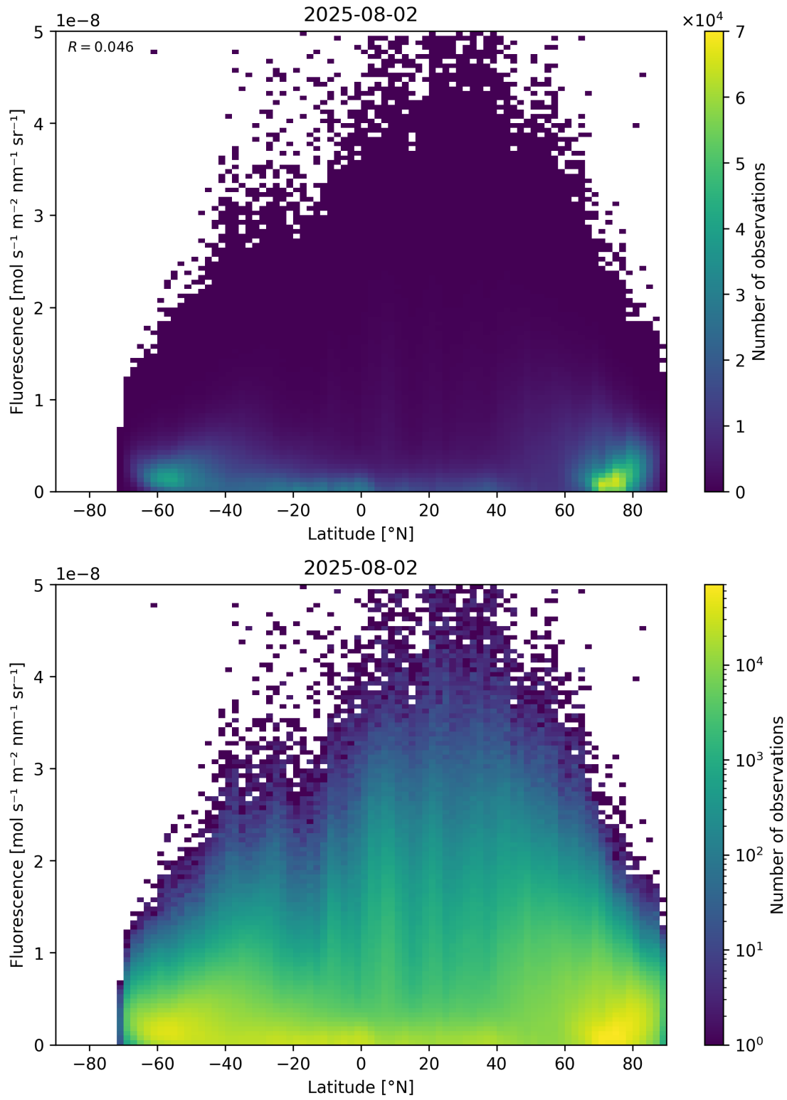
Figure 92: Scatter density plot of “Latitude” against “Fluorescence” for 2025-08-01 to 2025-08-03.
