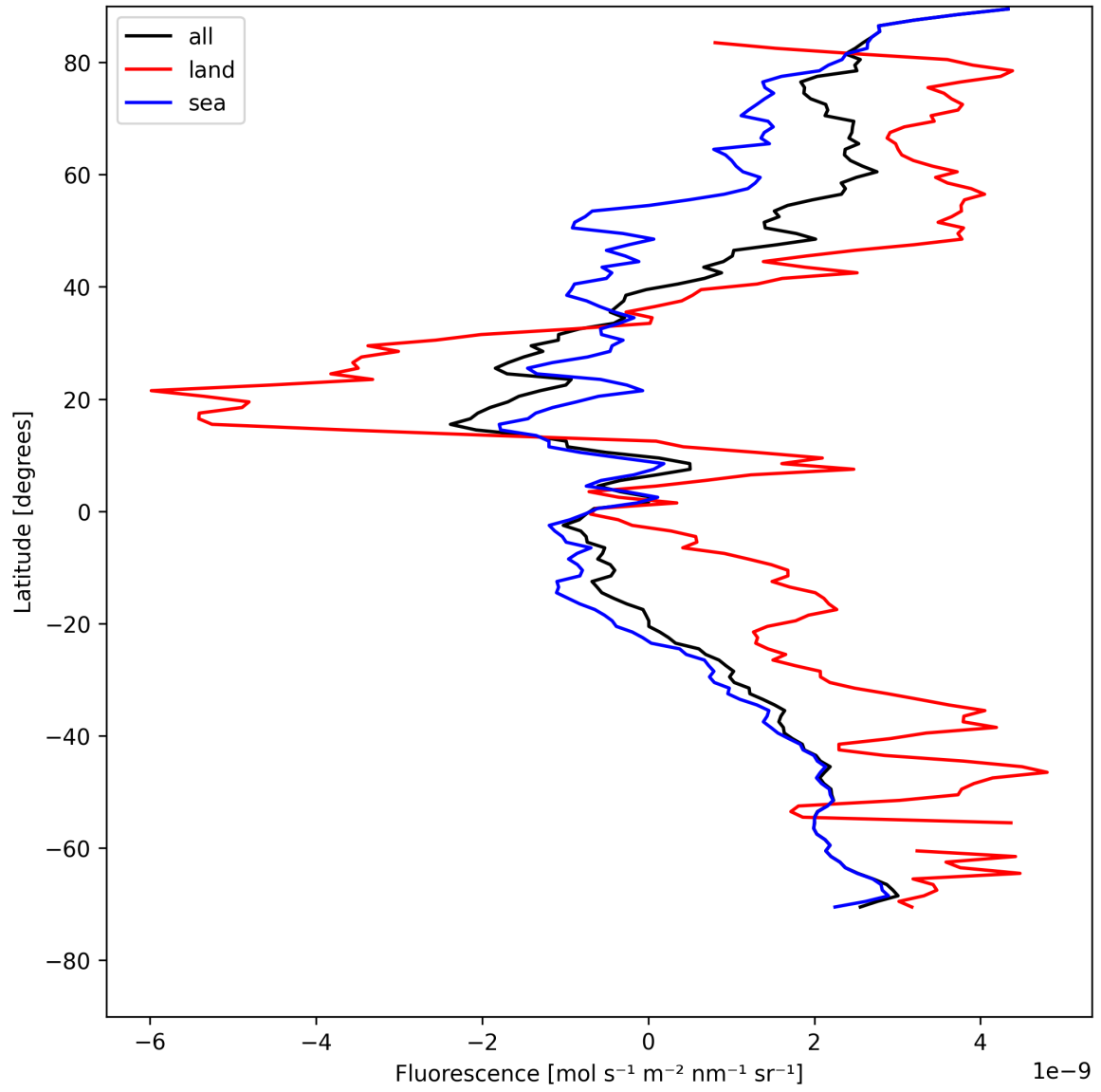
Figure 23: Zonal average of “Fluorescence” for 2025-08-01 to 2025-08-03.
