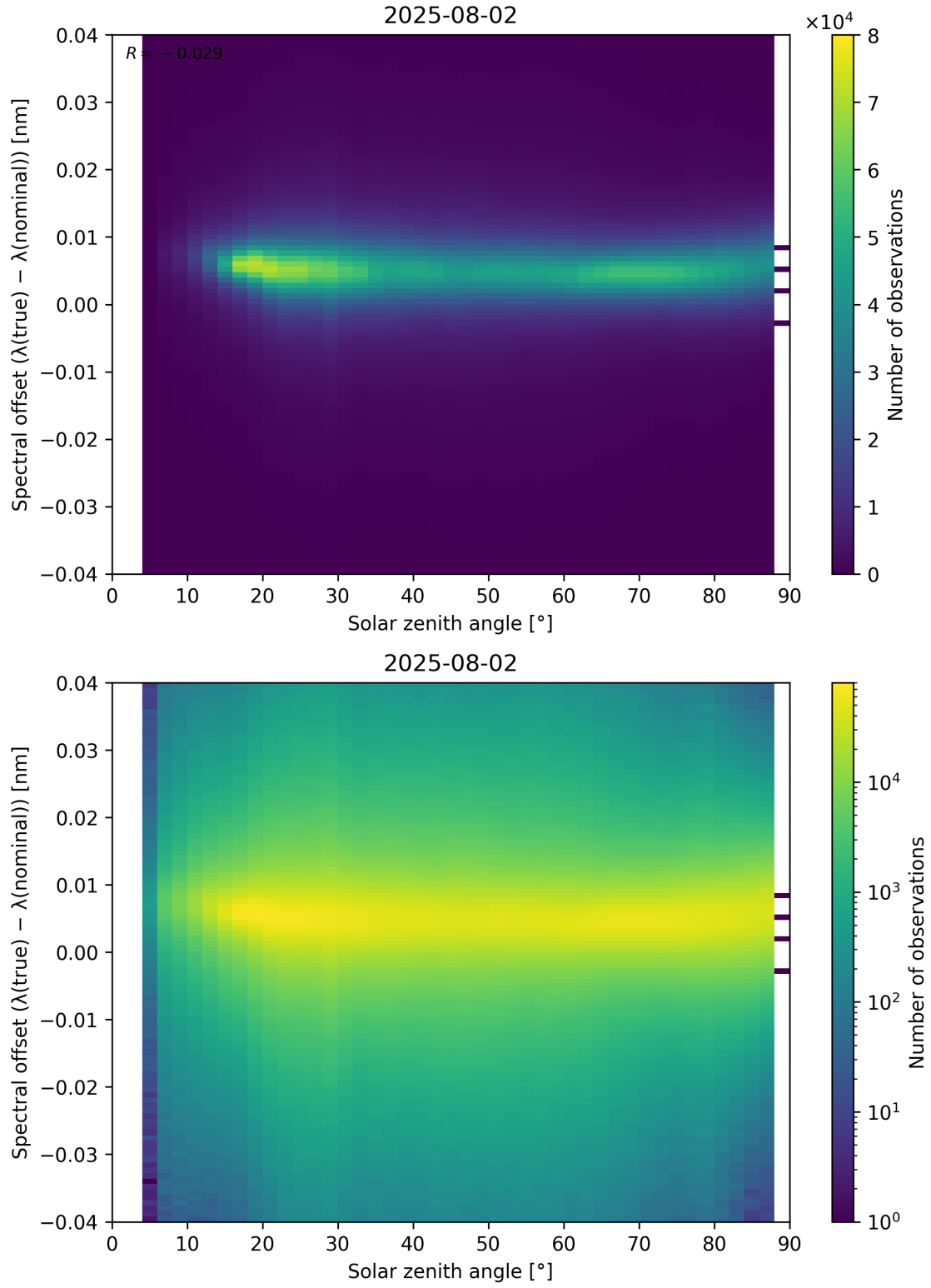
Figure 117: Scatter density plot of “Solar zenith angle” against “Spectral offset ( \lambda_{\text{true}} - \lambda_{\text{nominal}} )” for 2025-08-01 to 2025-08-03.
