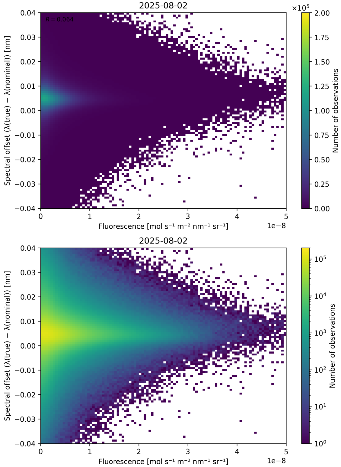
Figure 87: Scatter density plot of “Fluorescence” against “Spectral offset ( \lambda_{\text{true}} - \lambda_{\text{nominal}} )” for 2025-08-01 to 2025-08-03.
