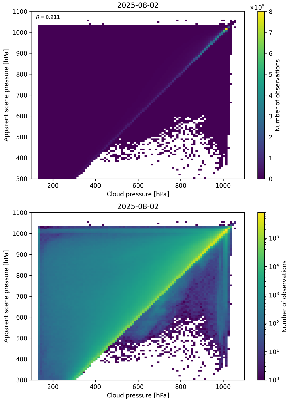
Figure 77: Scatter density plot of “Cloud pressure” against “Apparent scene pressure” for 2025-08-01 to 2025-08-03.
