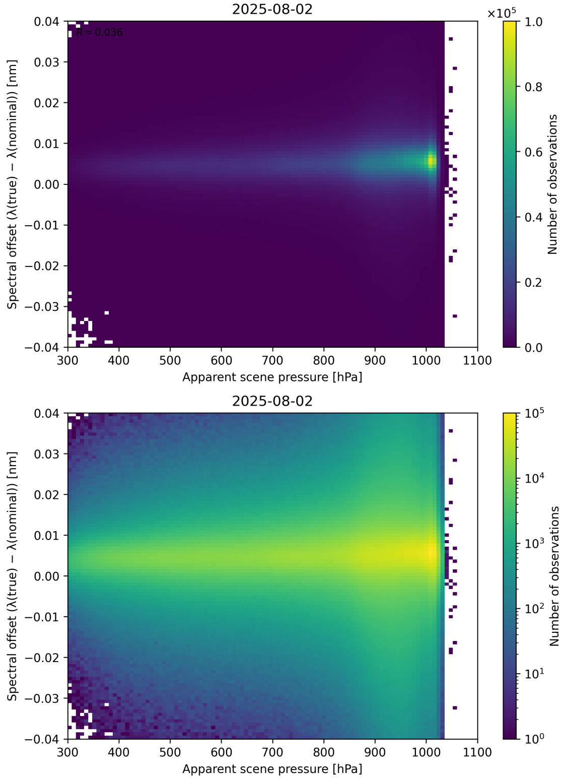
Figure 67: Scatter density plot of “Apparent scene pressure” against “Spectral offset ( \lambda_{\text{true}} - \lambda_{\text{nominal}} )” for 2025-08-01 to 2025-08-03.
