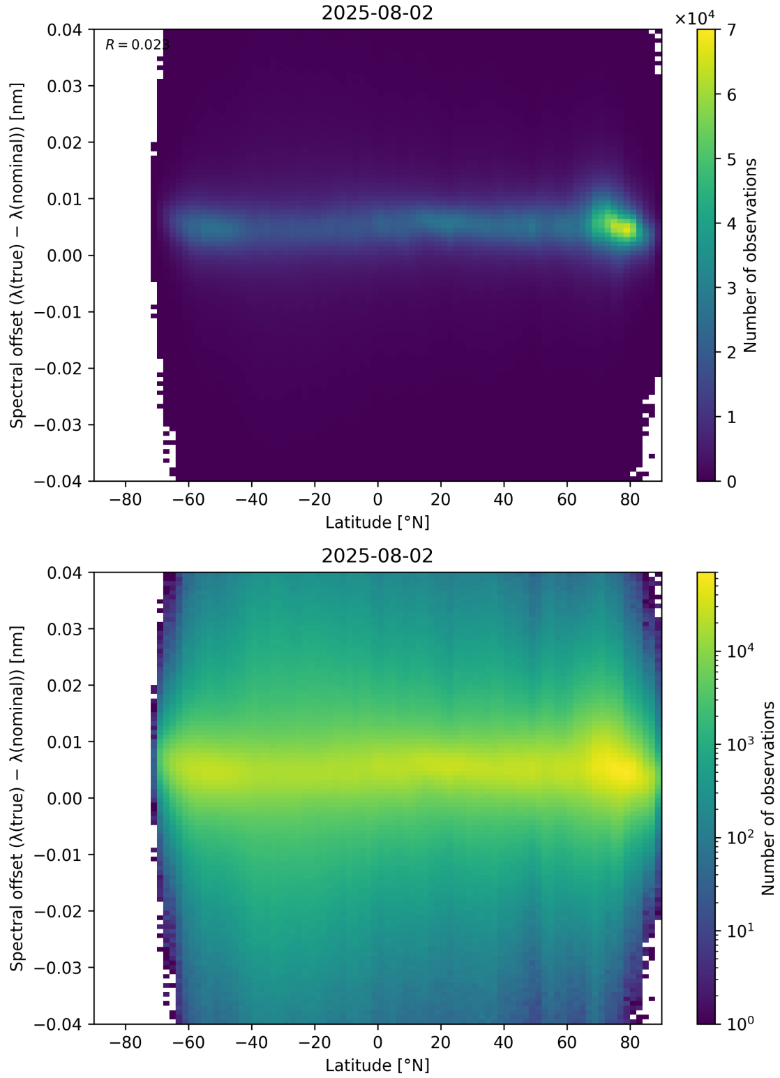
Figure 96: Scatter density plot of “Latitude” against “Spectral offset ( \lambda_{\text{true}} - \lambda_{\text{nominal}} )” for 2025-08-01 to 2025-08-03.
