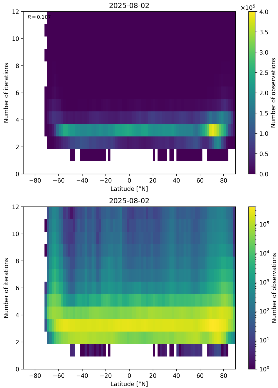
Figure 93: Scatter density plot of “Latitude” against “Number of iterations” for 2025-08-01 to 2025-08-03.
