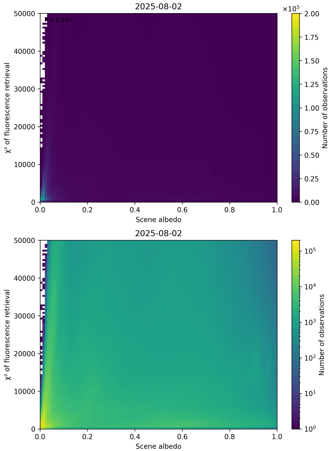
Figure 103: Scatter density plot of “Scene albedo” against “ \chi^2 of fluorescence retrieval” for 2025-08-01 to 2025-08-03.
