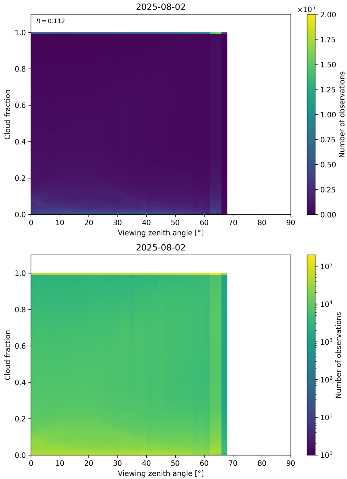
Figure 120: Scatter density plot of “Viewing zenith angle” against “Cloud fraction” for 2025-08-01 to 2025-08-03.
