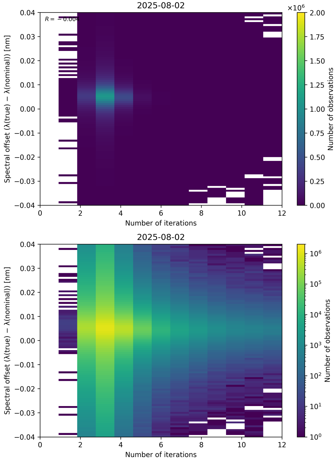
Figure 100: Scatter density plot of “Number of iterations” against “Spectral offset ( \lambda_{\text{true}} - \lambda_{\text{nominal}} )” for 2025-08-01 to 2025-08-03.
