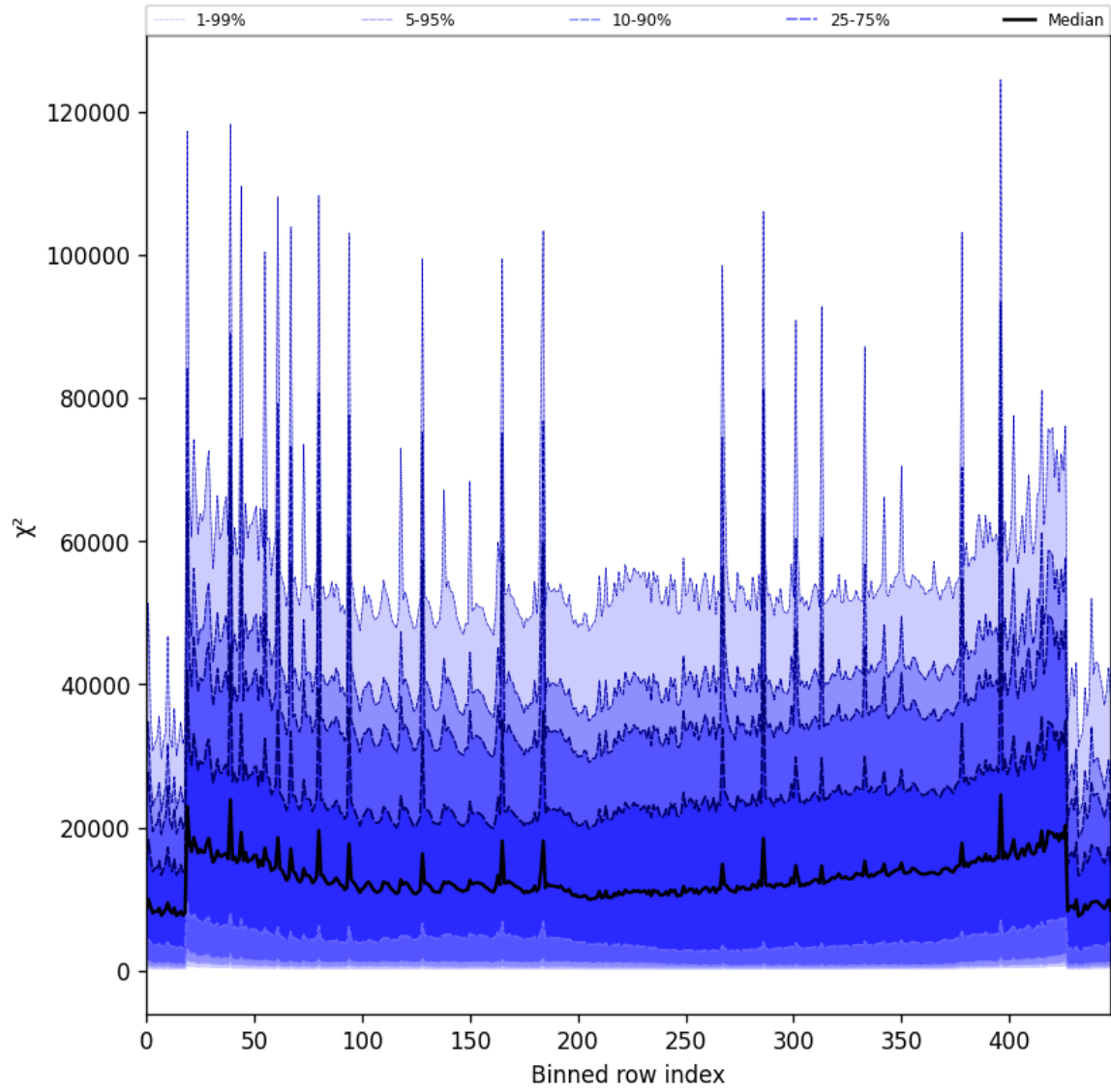
Figure 55: Along track statistics of “ \chi^2 ” for 2025-08-01 to 2025-08-03
