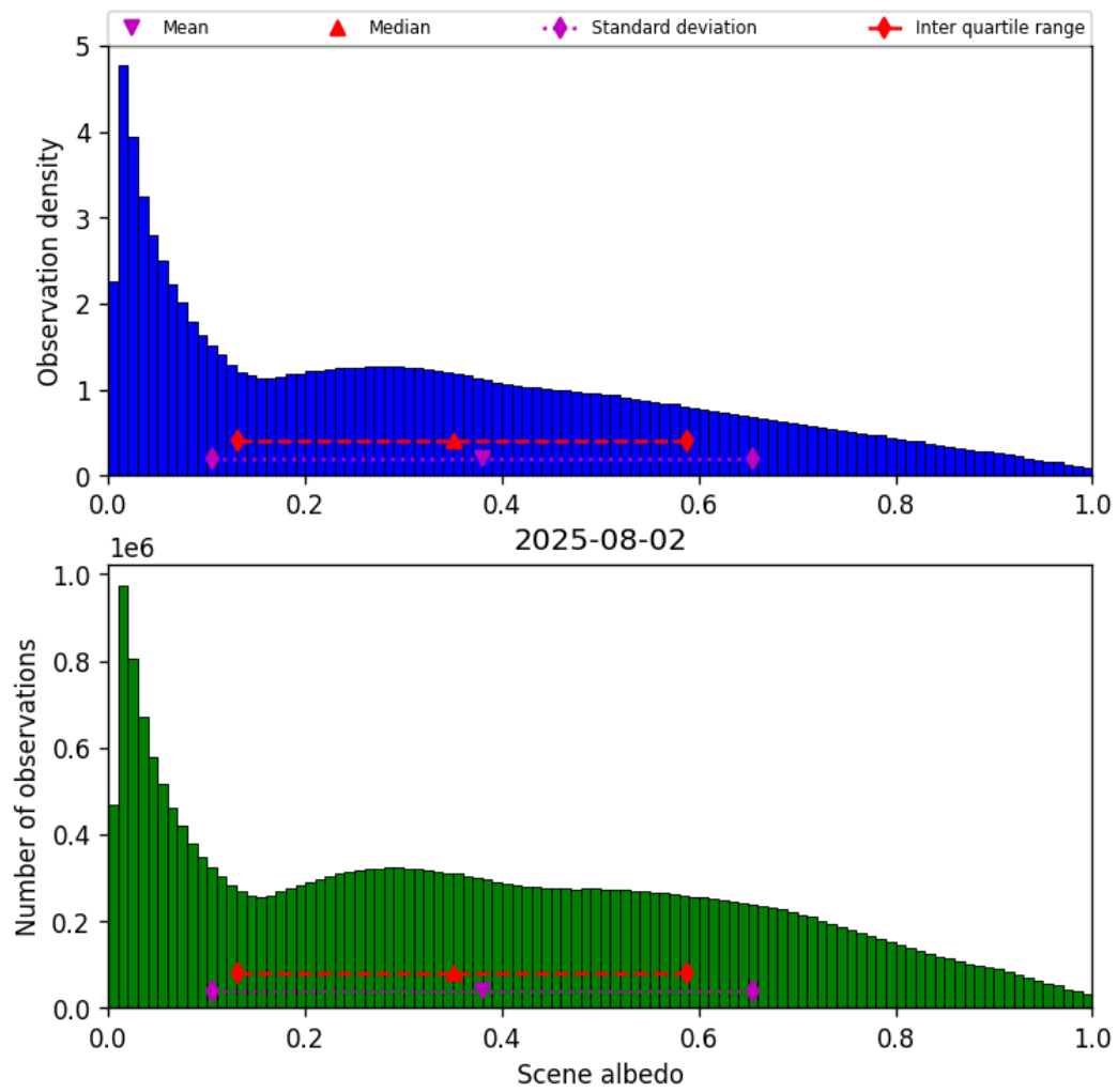
Figure 34: Histogram of “Scene albedo” for 2025-08-01 to 2025-08-03
