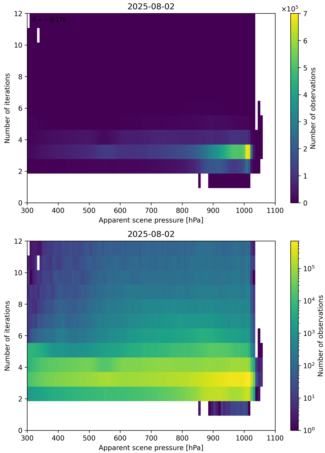
Figure 65: Scatter density plot of “Apparent scene pressure” against “Number of iterations” for 2025-08-01 to 2025-08-03.
