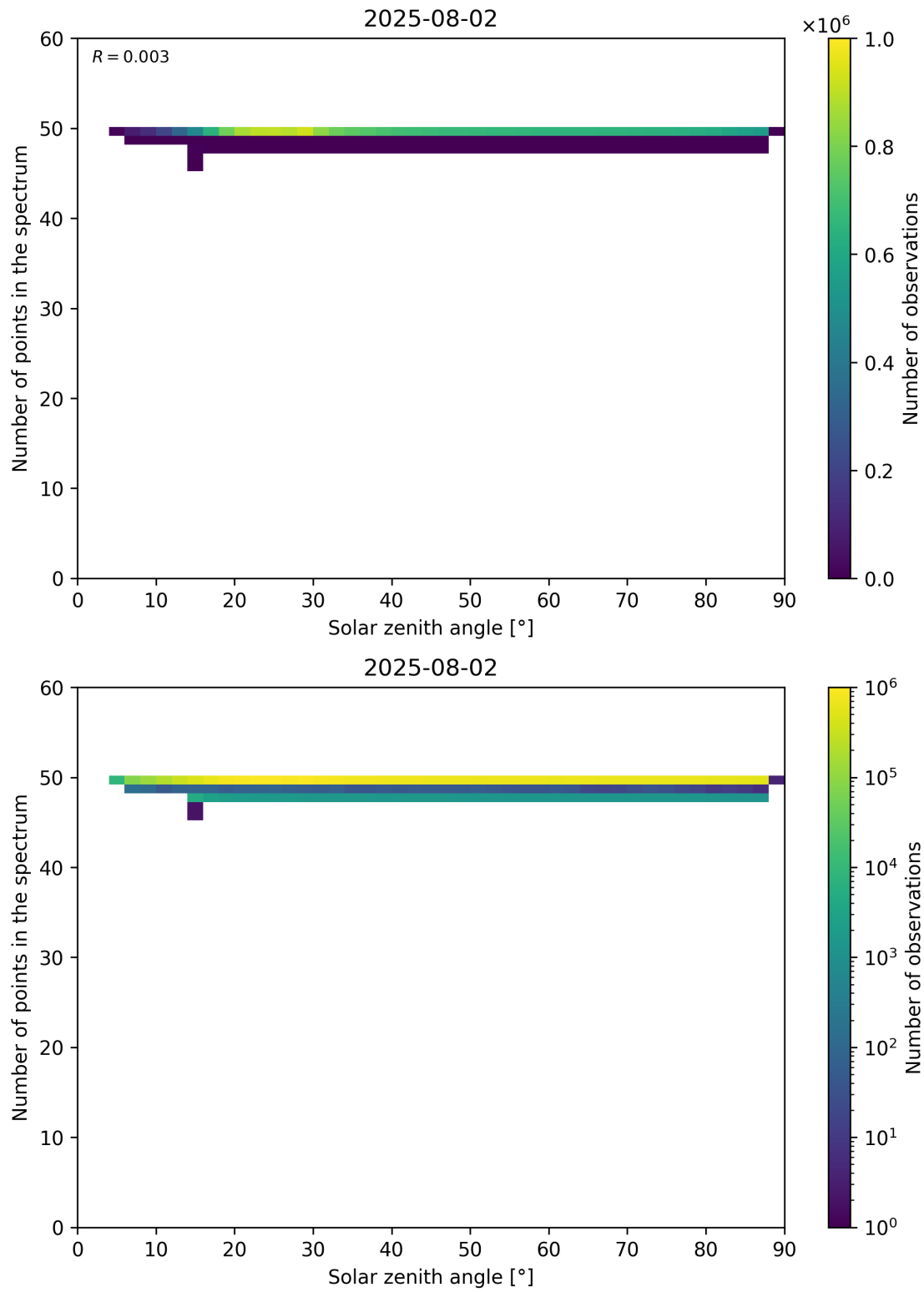
Figure 115: Scatter density plot of “Solar zenith angle” against “Number of points in the spectrum” for 2025-08-01 to 2025-08-03.
