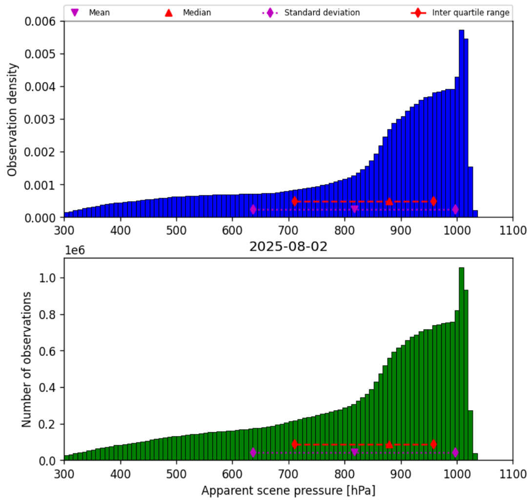
Figure 36: Histogram of “Apparent scene pressure” for 2025-08-01 to 2025-08-03
