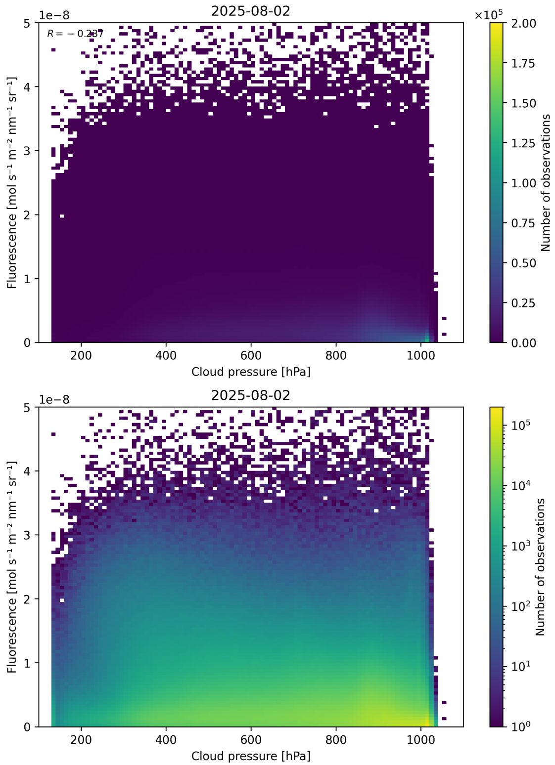
Figure 80: Scatter density plot of “Cloud pressure” against “Fluorescence” for 2025-08-01 to 2025-08-03.
