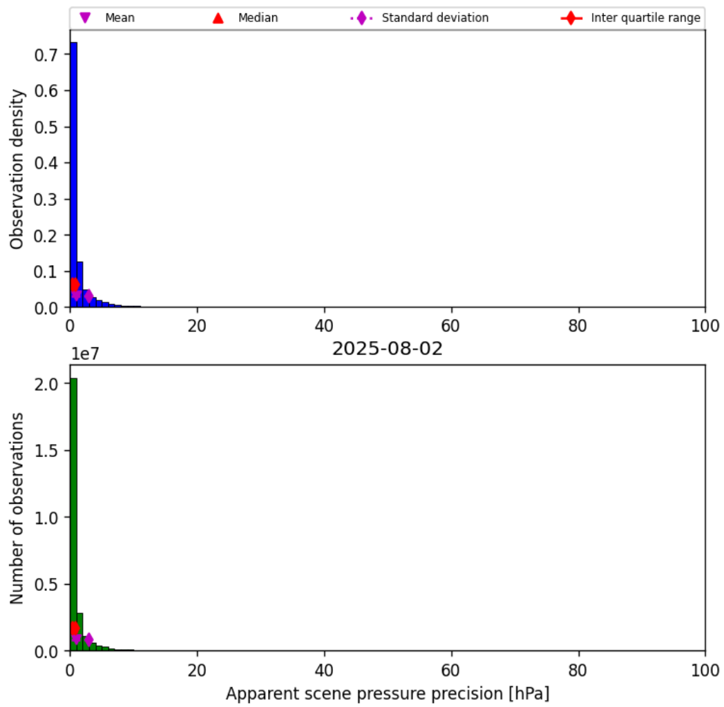
Figure 37: Histogram of “Apparent scene pressure precision” for 2025-08-01 to 2025-08-03
