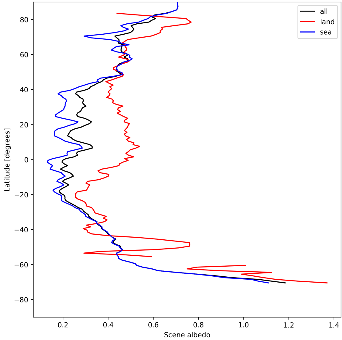
Figure 17: Zonal average of “Scene albedo” for 2025-08-01 to 2025-08-03.
