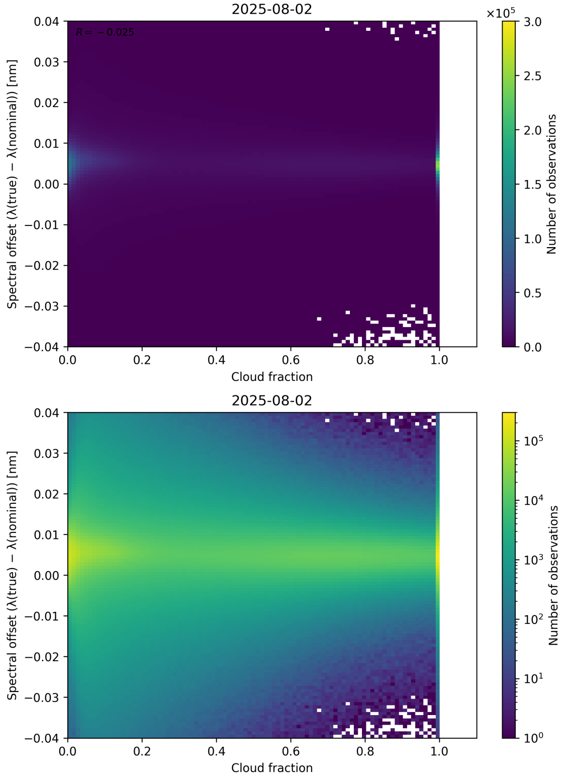
Figure 76: Scatter density plot of “Cloud fraction” against “Spectral offset ( \lambda_{\text{true}} - \lambda_{\text{nominal}} )” for 2025-08-01 to 2025-08-03.
