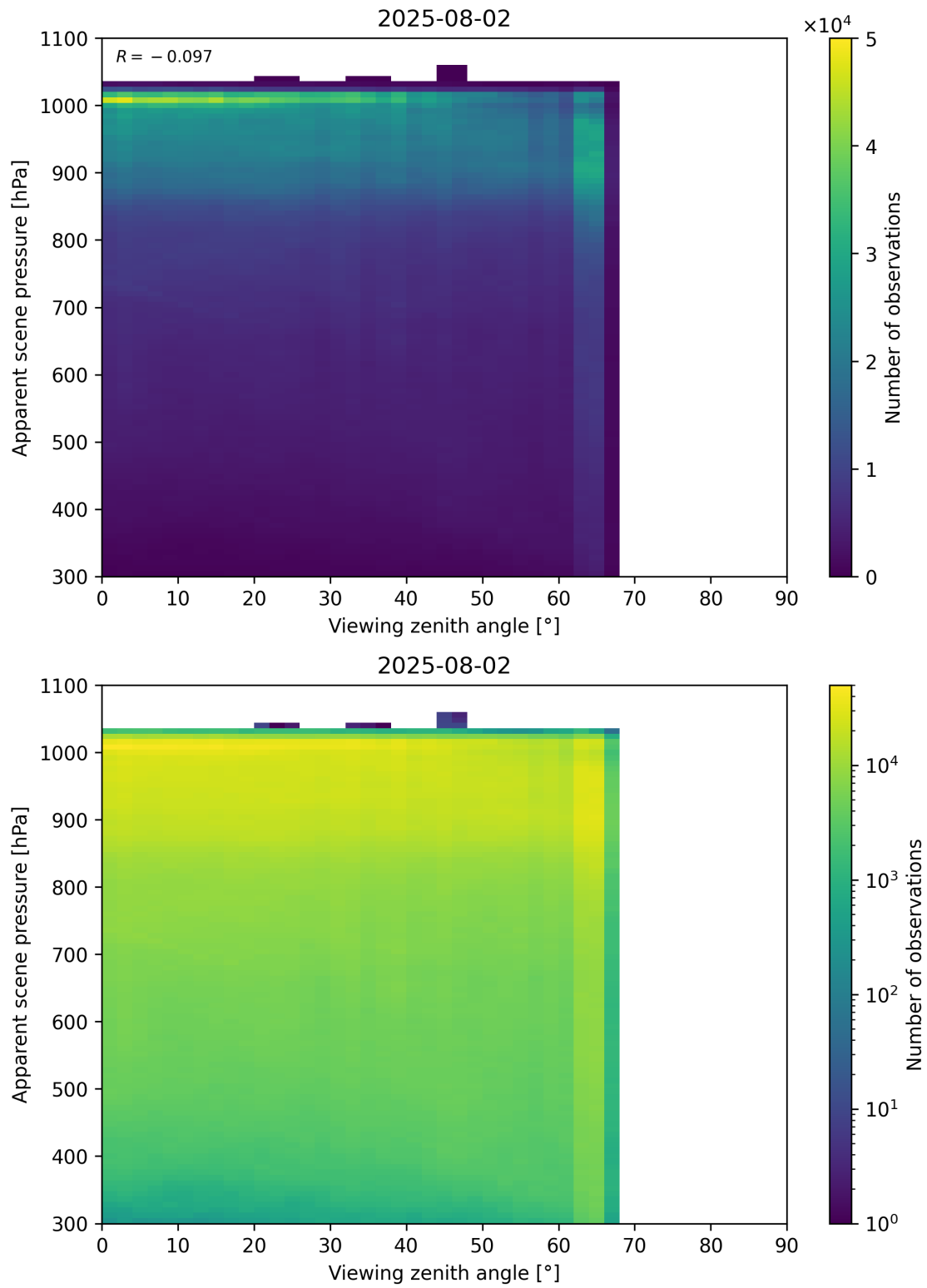
Figure 118: Scatter density plot of “Viewing zenith angle” against “Apparent scene pressure” for 2025-08-01 to 2025-08-03.
