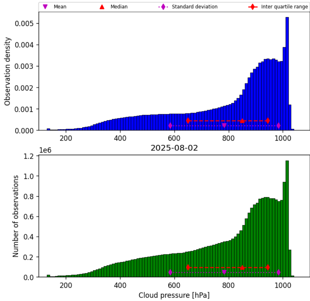
Figure 30: Histogram of “Cloud pressure” for 2025-08-01 to 2025-08-03
