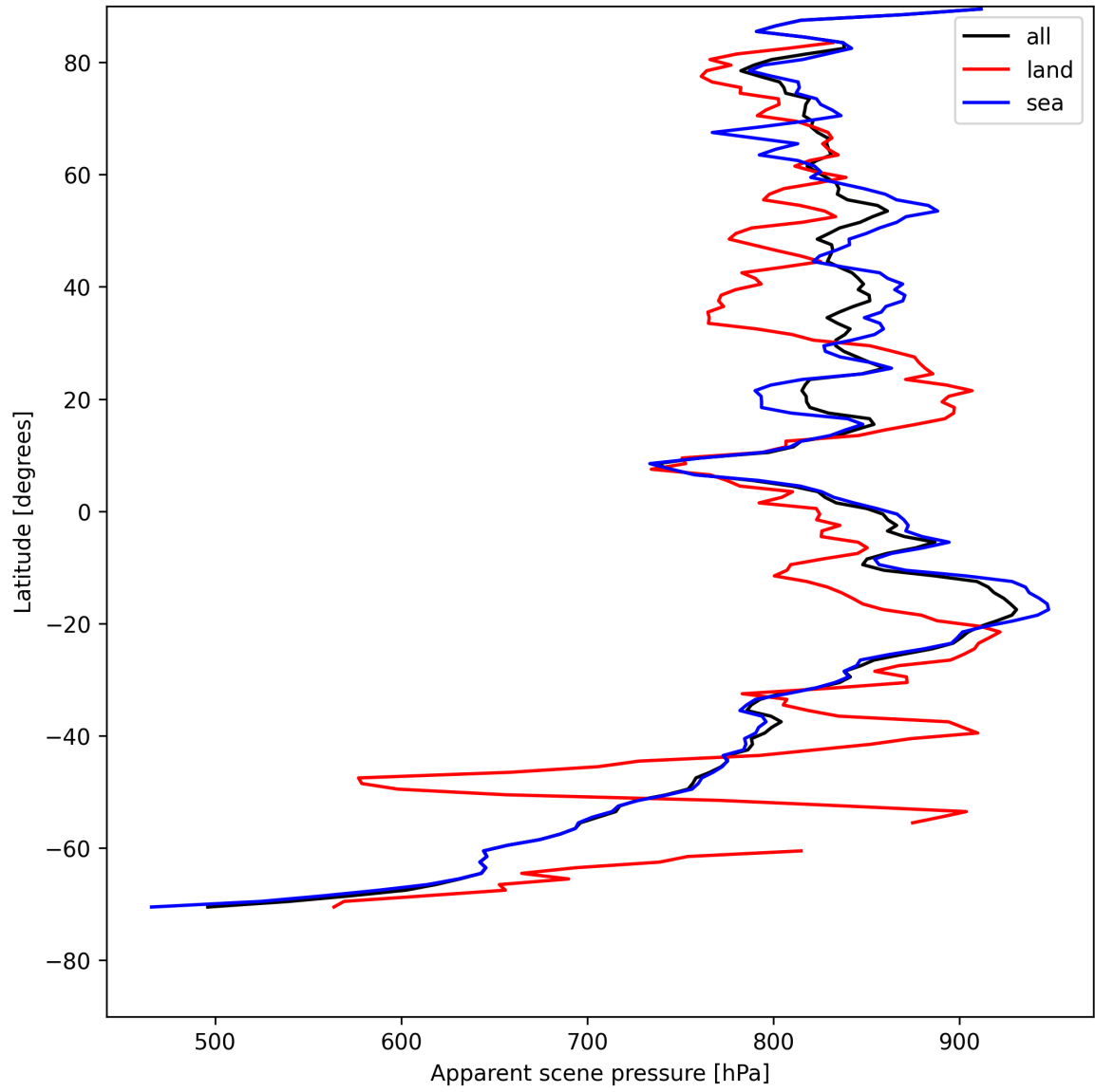
Figure 19: Zonal average of “Apparent scene pressure” for 2025-08-01 to 2025-08-03.
