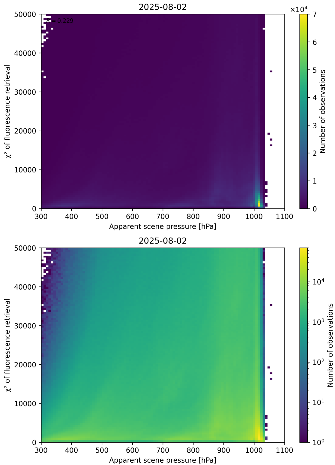
Figure 63: Scatter density plot of “Apparent scene pressure” against “ \chi^2 of fluorescence retrieval” for 2025-08-01 to 2025-08-03.
