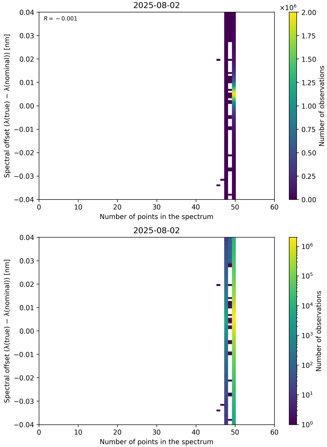
Figure 101: Scatter density plot of “Number of points in the spectrum” against “Spectral offset ( \lambda_{\text{true}} - \lambda_{\text{nominal}} )” for 2025-08-01 to 2025-08-03.
