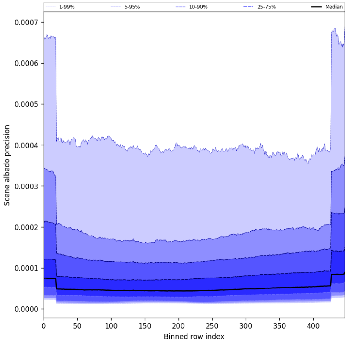
Figure 52: Along track statistics of “Scene albedo precision” for 2025-08-01 to 2025-08-03
