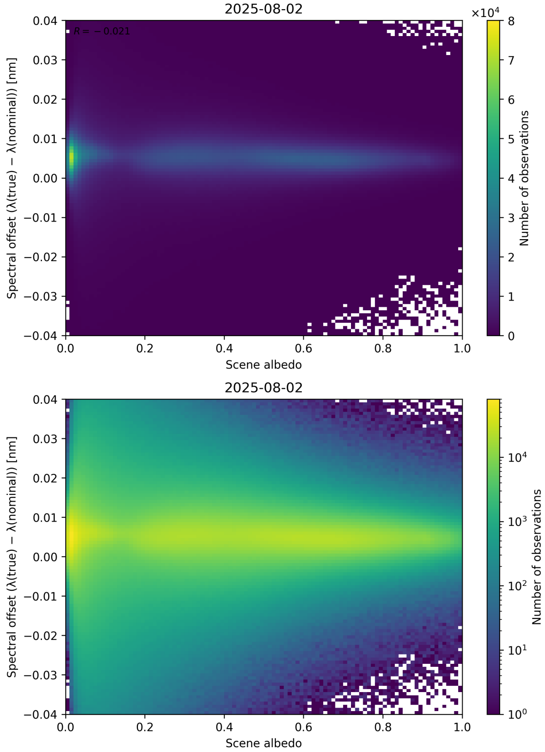
Figure 107: Scatter density plot of “Scene albedo” against “Spectral offset ( \lambda_{\text{true}} - \lambda_{\text{nominal}} )” for 2025-08-01 to 2025-08-03.
