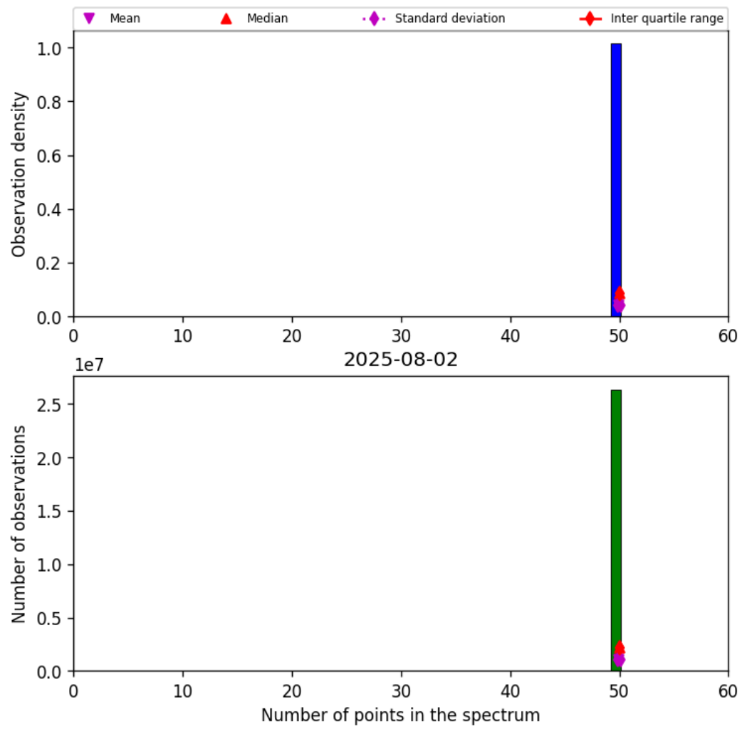
Figure 44: Histogram of “Number of points in the spectrum” for 2025-08-01 to 2025-08-03
