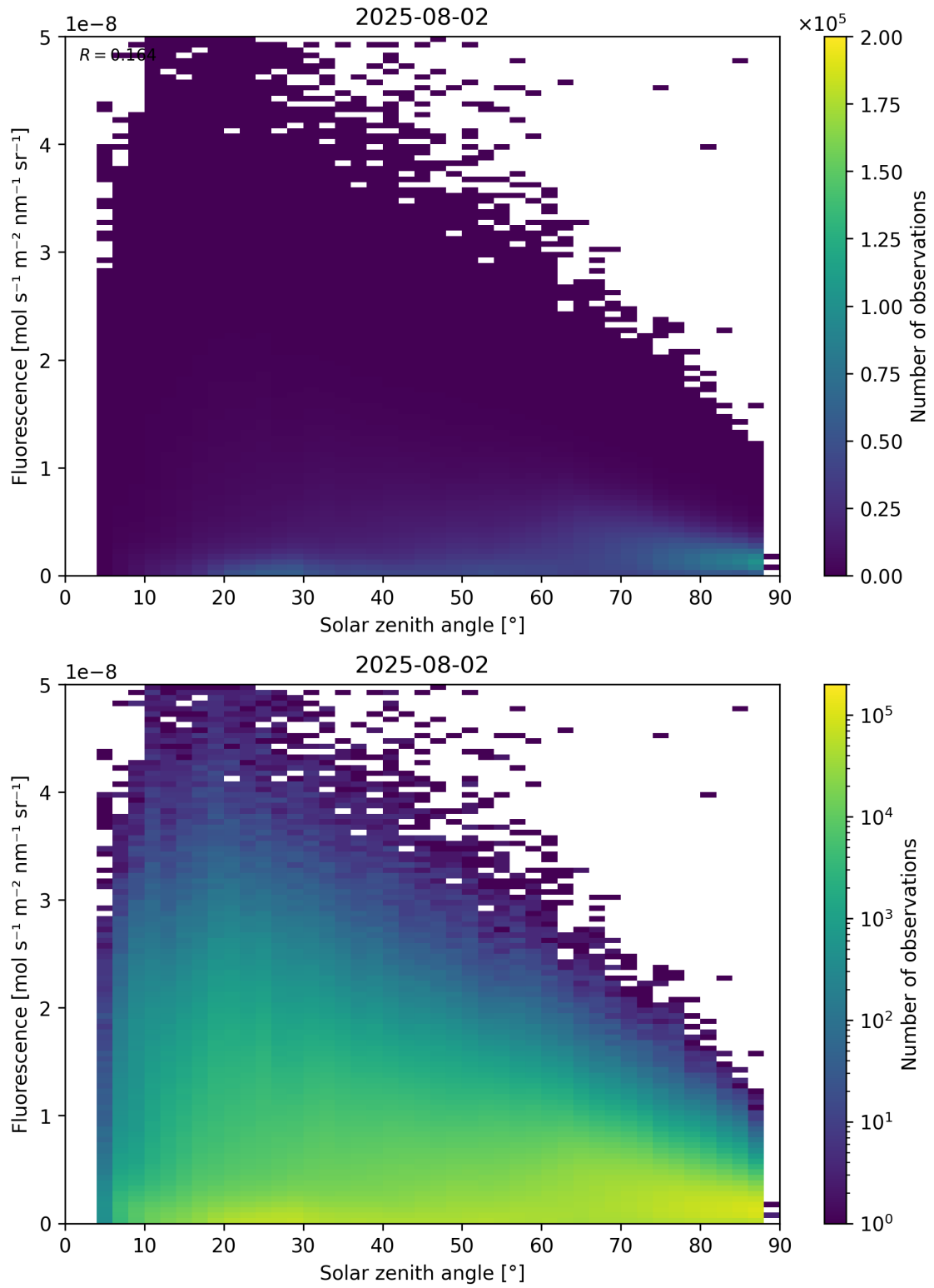
Figure 112: Scatter density plot of “Solar zenith angle” against “Fluorescence” for 2025-08-01 to 2025-08-03.
