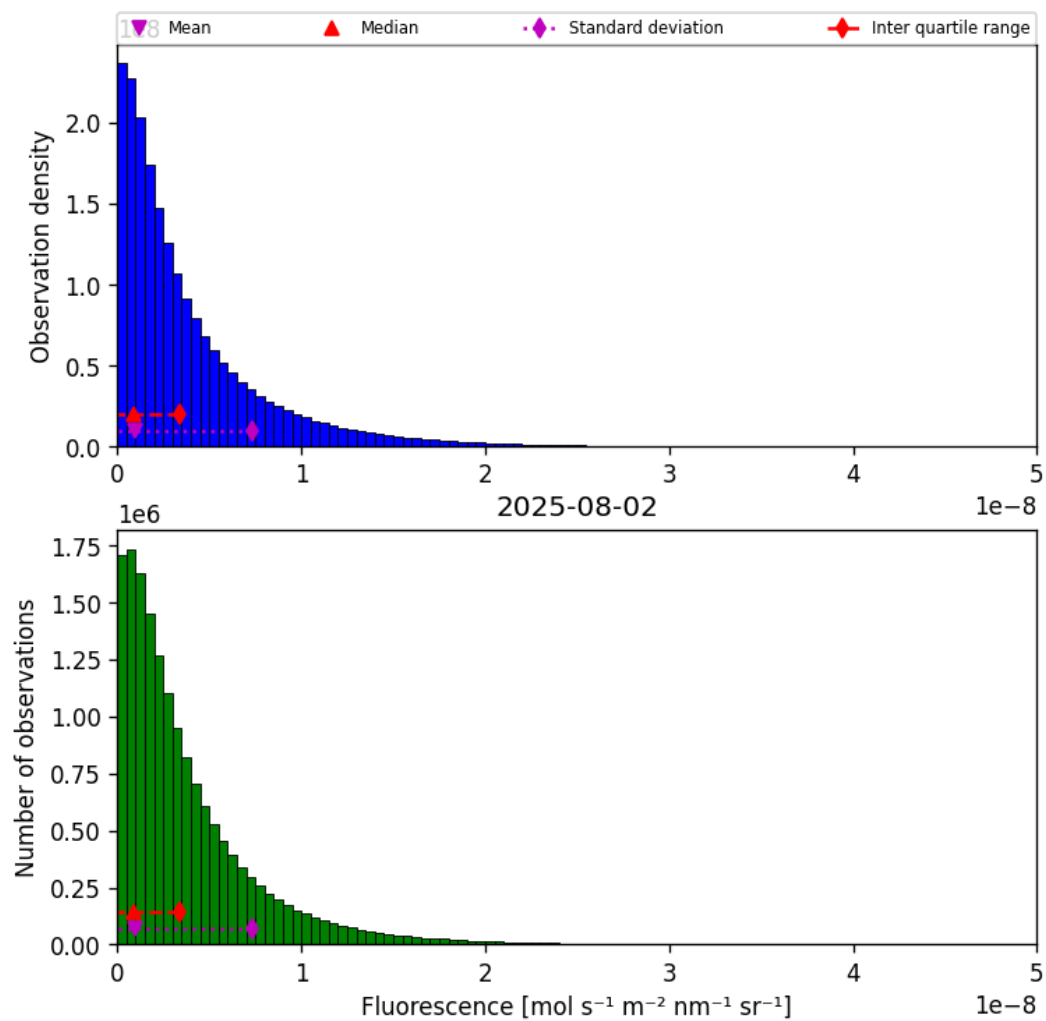
Figure 40: Histogram of “Fluorescence” for 2025-08-01 to 2025-08-03
