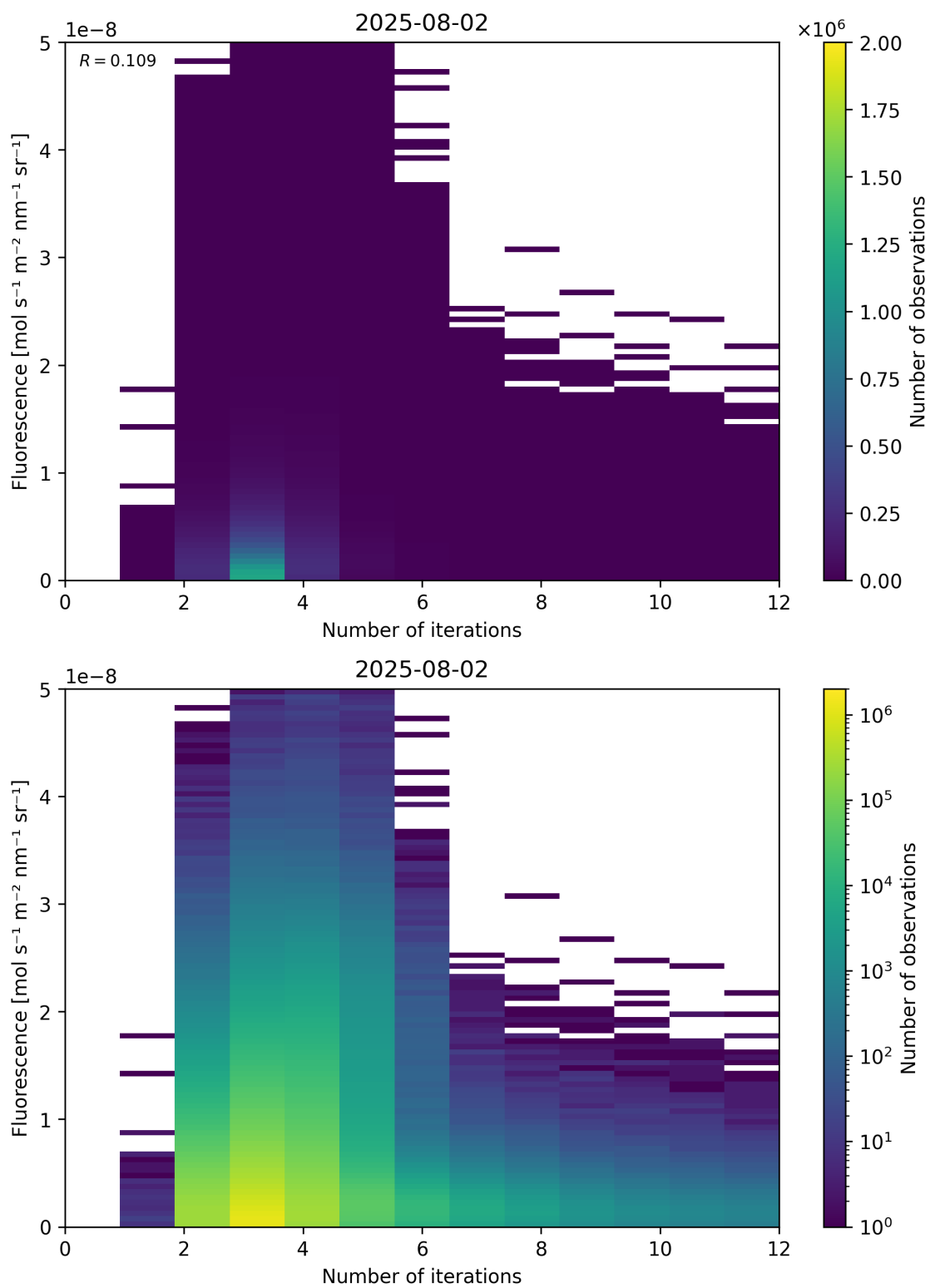
Figure 98: Scatter density plot of “Number of iterations” against “Fluorescence” for 2025-08-01 to 2025-08-03.
