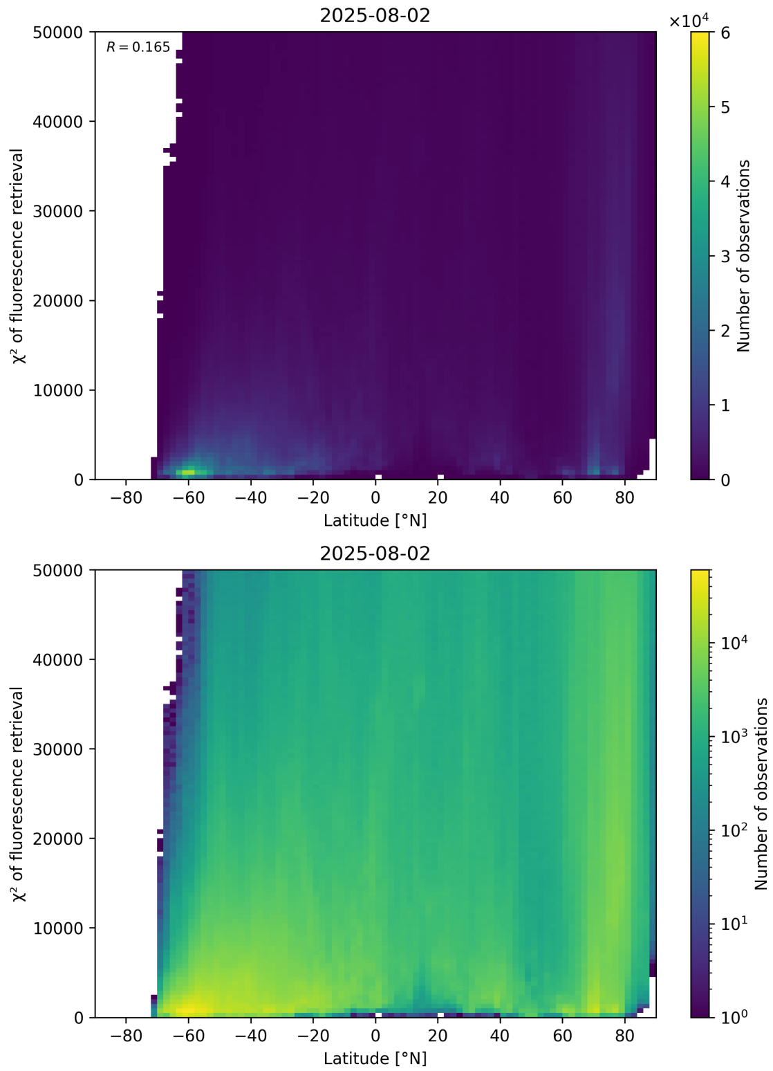
Figure 89: Scatter density plot of “Latitude” against “ \chi^2 of fluorescence retrieval” for 2025-08-01 to 2025-08-03.
