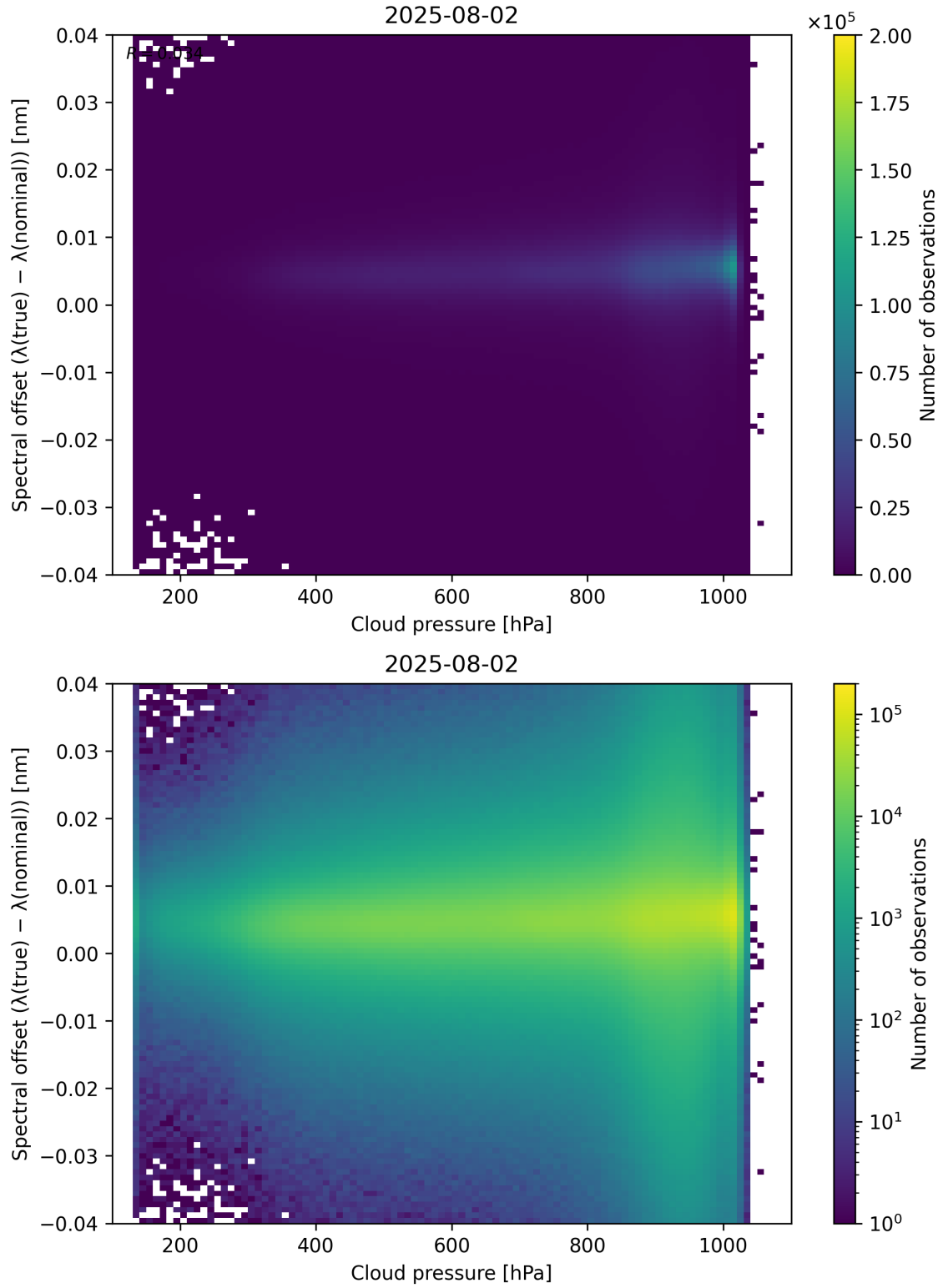
Figure 84: Scatter density plot of “Cloud pressure” against “Spectral offset ( \lambda_{\text{true}} - \lambda_{\text{nominal}} )” for 2025-08-01 to 2025-08-03.
