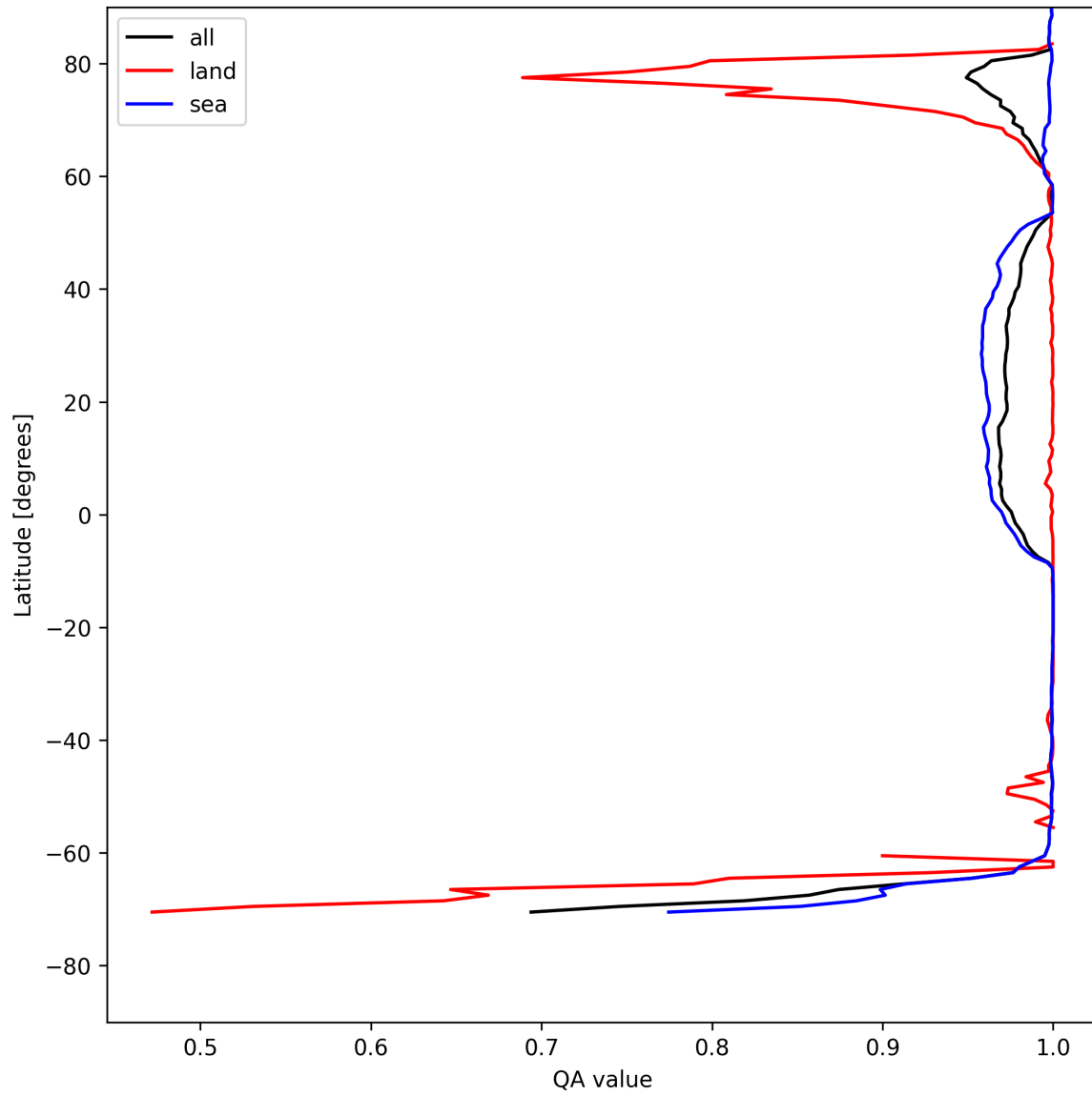
Figure 12: Zonal average of “QA value” for 2025-08-01 to 2025-08-03.
