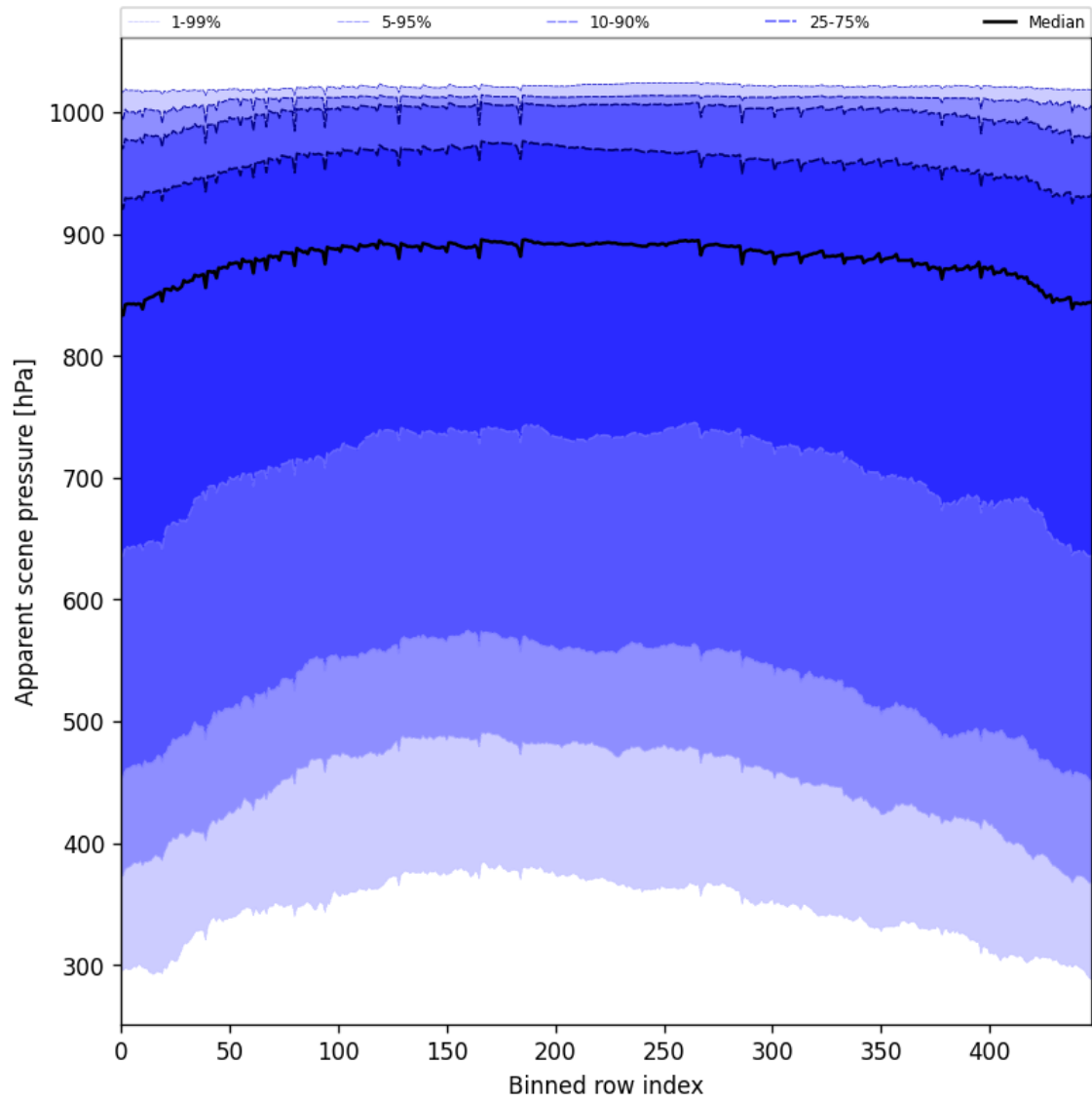
Figure 53: Along track statistics of “Apparent scene pressure” for 2025-08-01 to 2025-08-03
