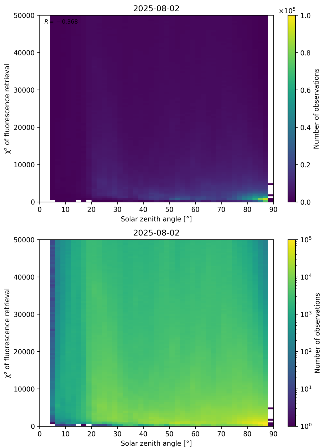
Figure 109: Scatter density plot of “Solar zenith angle” against “ \chi^2 of fluorescence retrieval” for 2025-08-01 to 2025-08-03.
