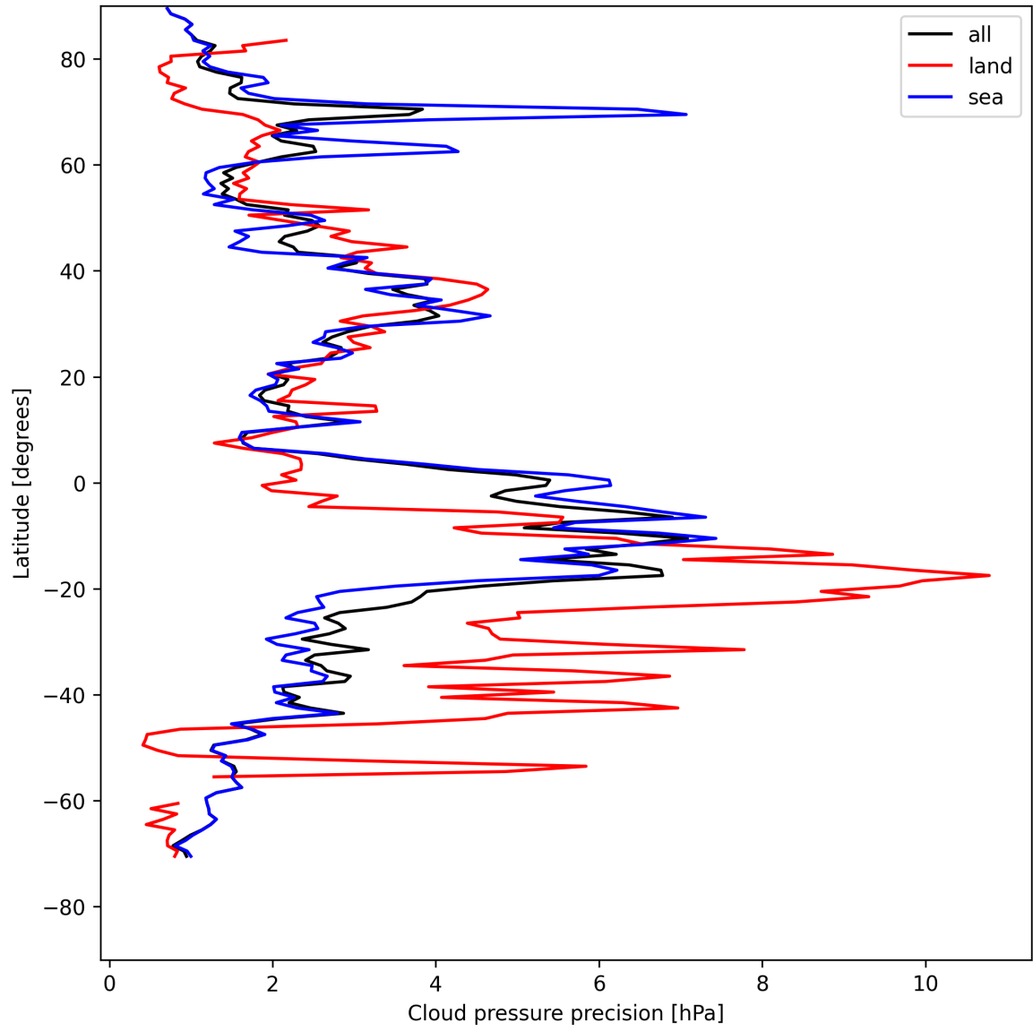
Figure 14: Zonal average of “Cloud pressure precision” for 2025-08-01 to 2025-08-03.
