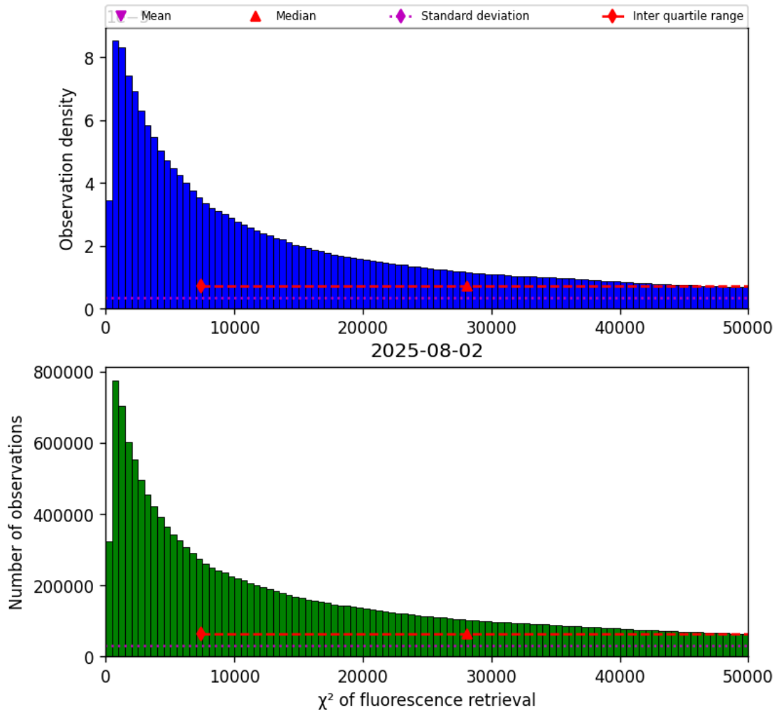
Figure 42: Histogram of “ \chi^2 of fluorescence retrieval” for 2025-08-01 to 2025-08-03
