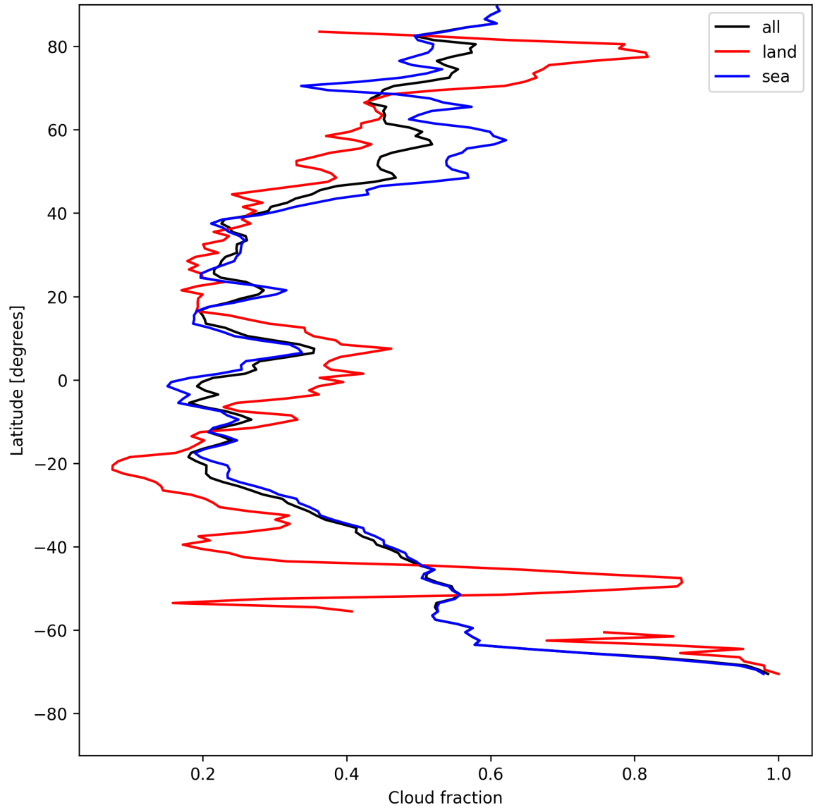
Figure 15: Zonal average of “Cloud fraction” for 2025-08-01 to 2025-08-03.
