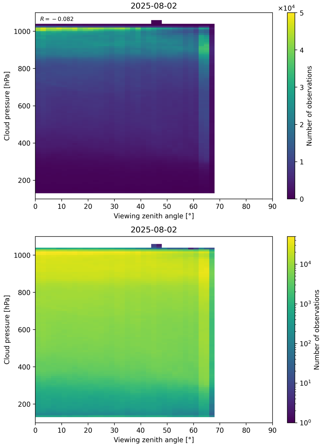
Figure 121: Scatter density plot of “Viewing zenith angle” against “Cloud pressure” for 2025-08-01 to 2025-08-03.
