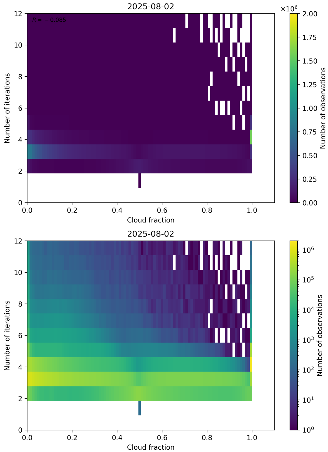
Figure 73: Scatter density plot of “Cloud fraction” against “Number of iterations” for 2025-08-01 to 2025-08-03.
