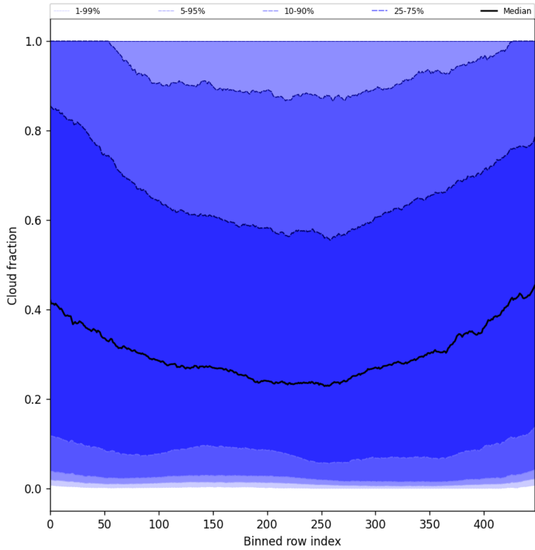
Figure 49: Along track statistics of “Cloud fraction” for 2025-08-01 to 2025-08-03
