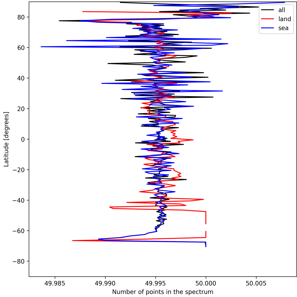
Figure 27: Zonal average of “Number of points in the spectrum” for 2025-08-01 to 2025-08-03.
