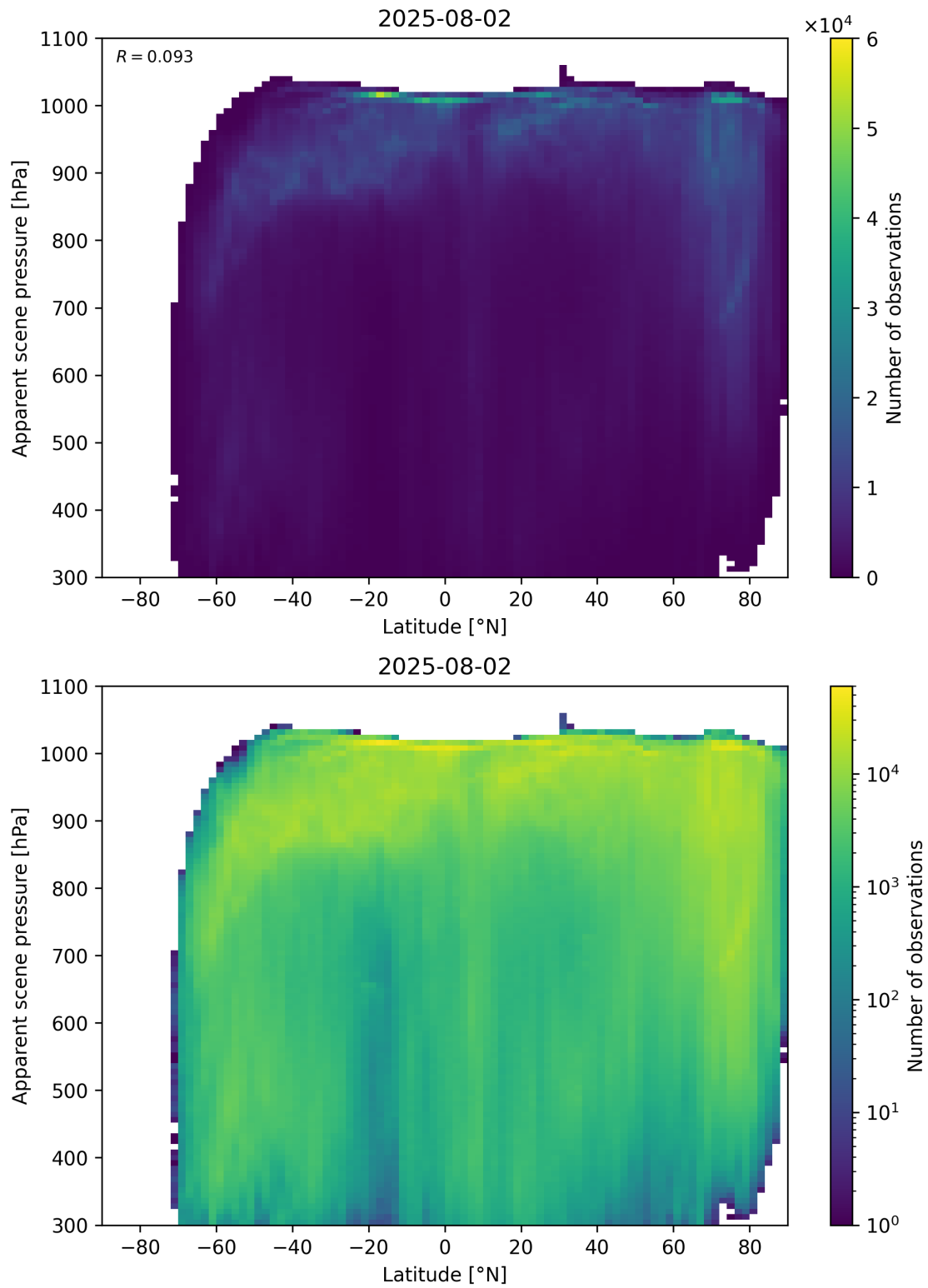
Figure 88: Scatter density plot of “Latitude” against “Apparent scene pressure” for 2025-08-01 to 2025-08-03.
