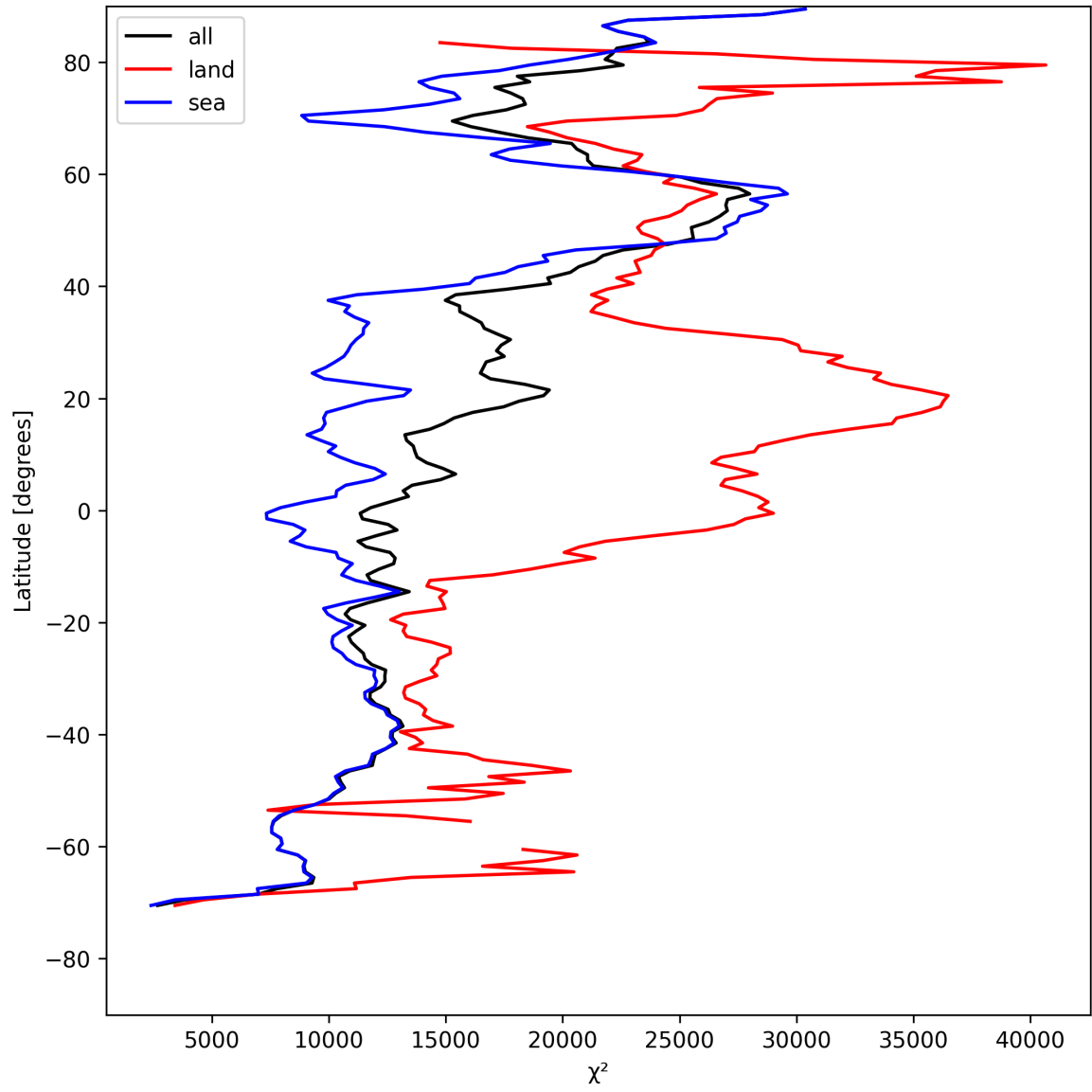
Figure 21: Zonal average of “ \chi^2 ” for 2025-08-01 to 2025-08-03.
