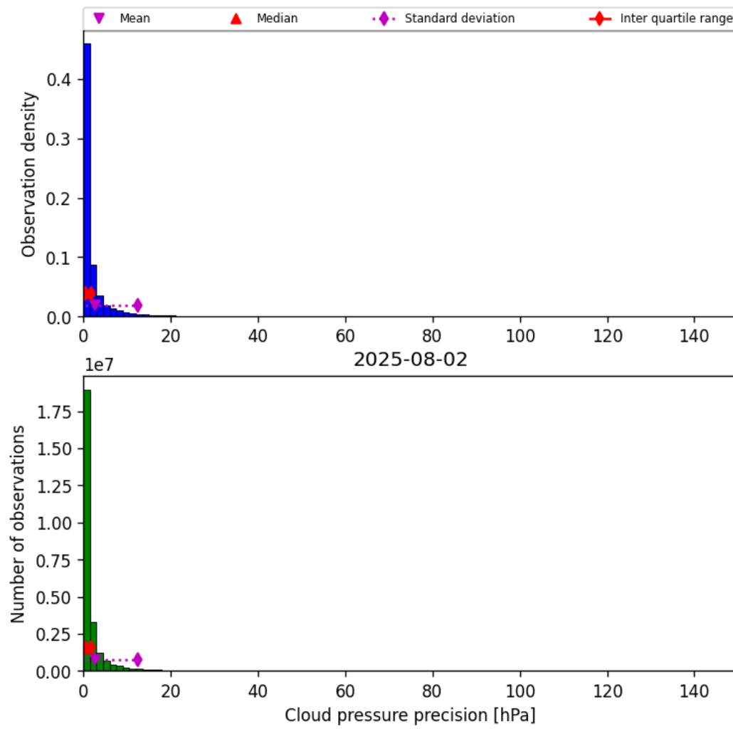
Figure 31: Histogram of “Cloud pressure precision” for 2025-08-01 to 2025-08-03
