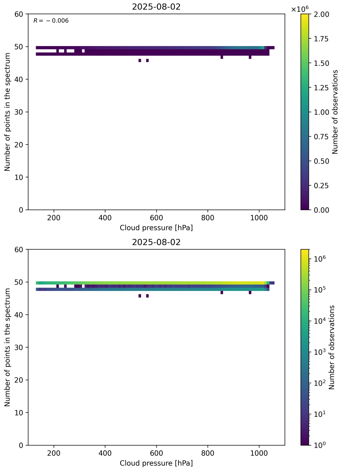
Figure 82: Scatter density plot of “Cloud pressure” against “Number of points in the spectrum” for 2025-08-01 to 2025-08-03.
