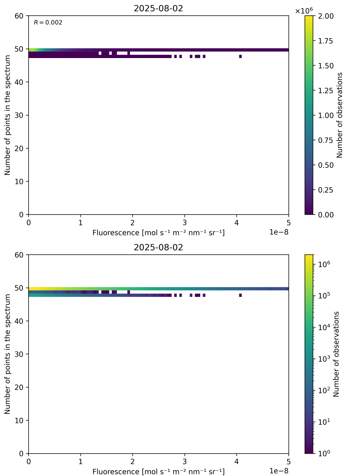
Figure 86: Scatter density plot of “Fluorescence” against “Number of points in the spectrum” for 2025-08-01 to 2025-08-03.
