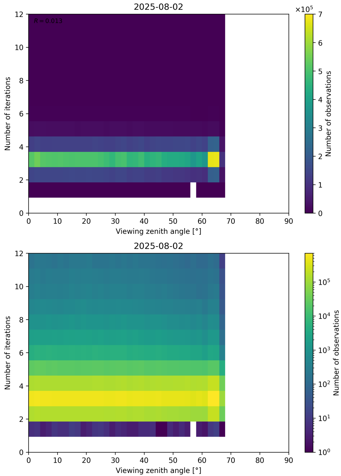
Figure 124: Scatter density plot of “Viewing zenith angle” against “Number of iterations” for 2025-08-01 to 2025-08-03.
