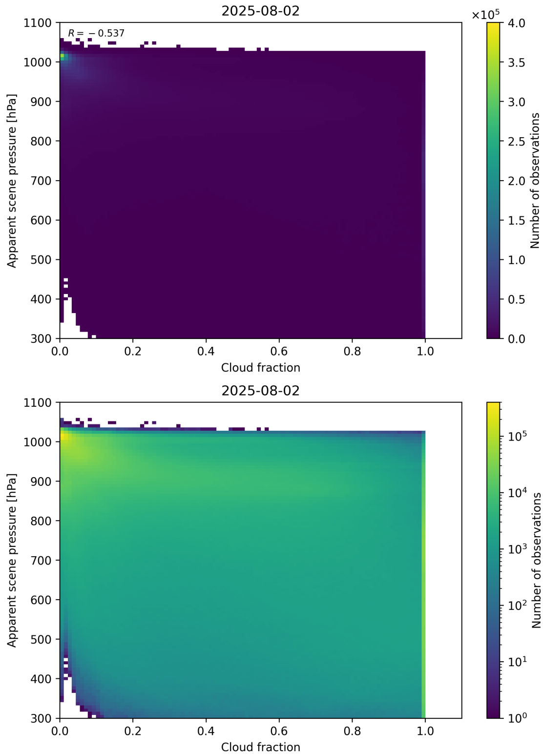
Figure 70: Scatter density plot of “Cloud fraction” against “Apparent scene pressure” for 2025-08-01 to 2025-08-03.
