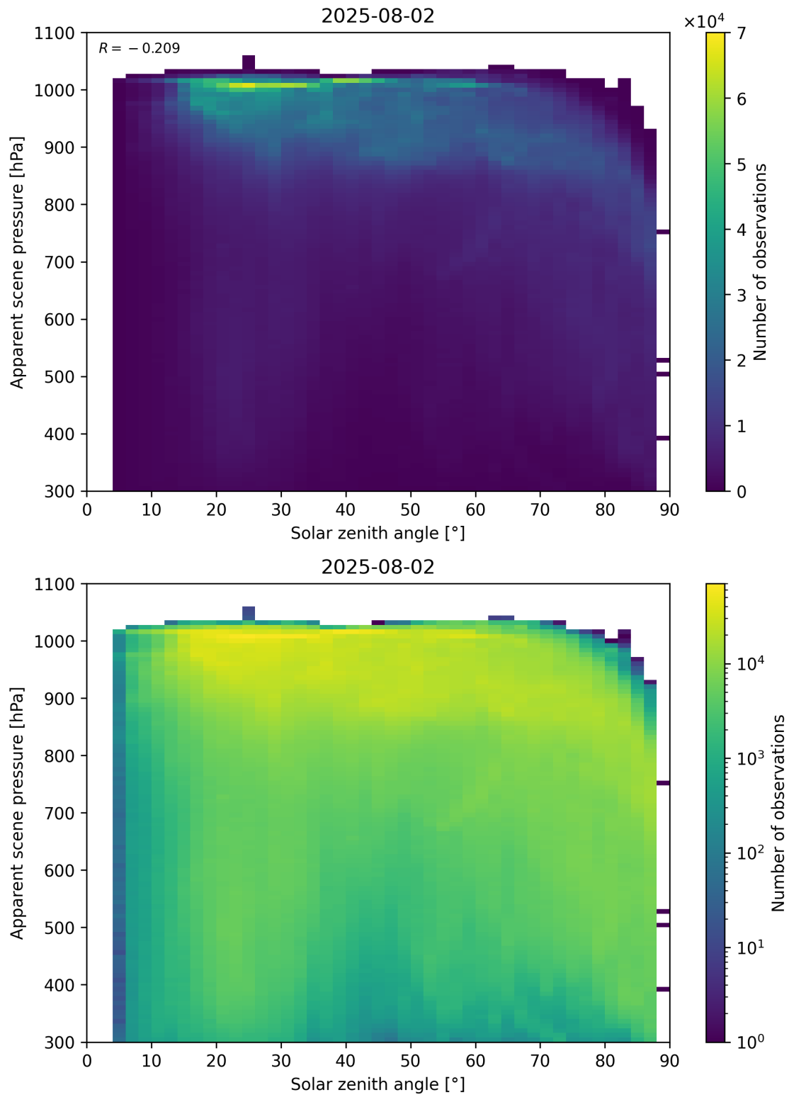
Figure 108: Scatter density plot of “Solar zenith angle” against “Apparent scene pressure” for 2025-08-01 to 2025-08-03.
