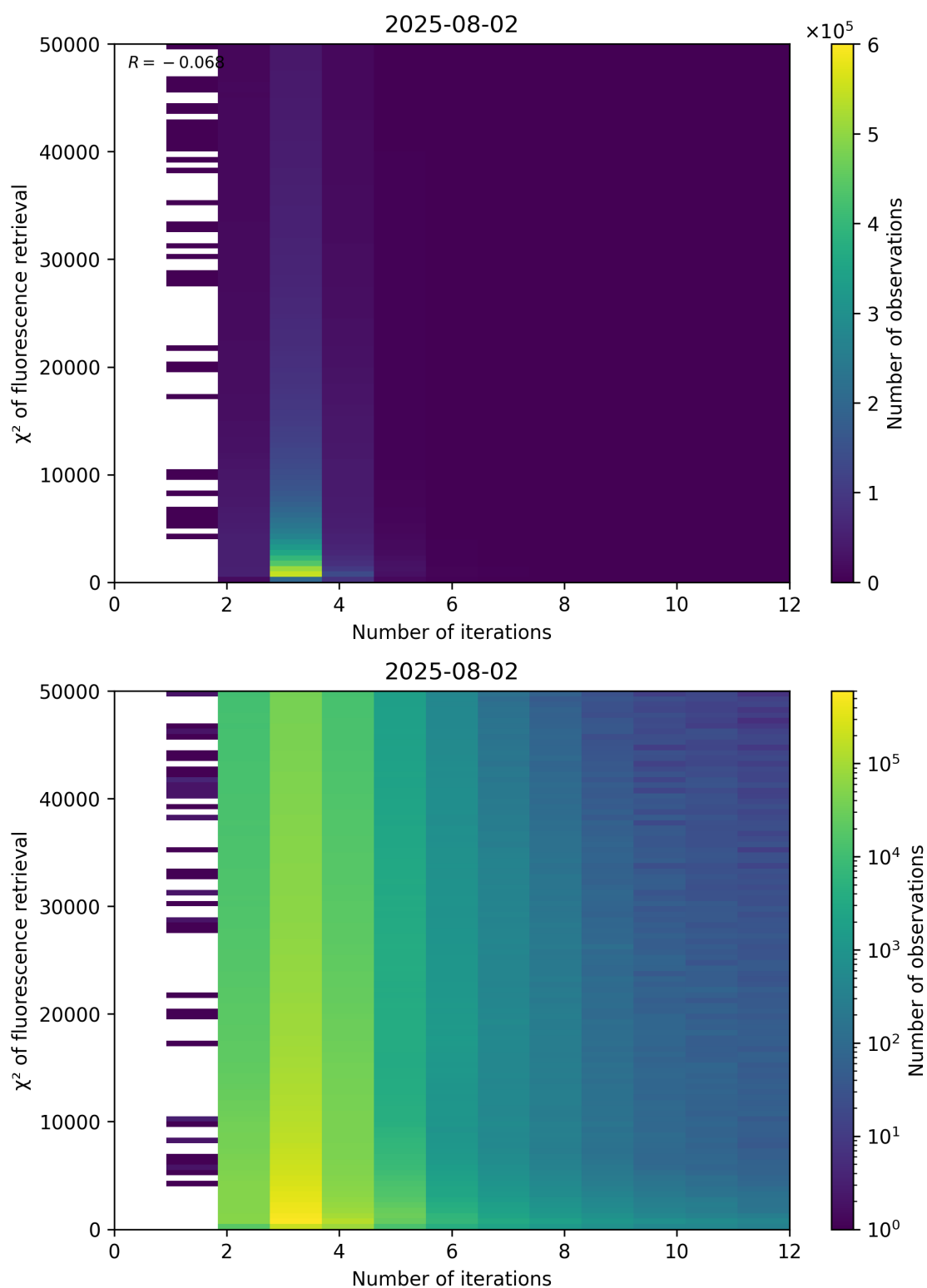
Figure 97: Scatter density plot of “Number of iterations” against “ \chi^2 of fluorescence retrieval” for 2025-08-01 to 2025-08-03.
