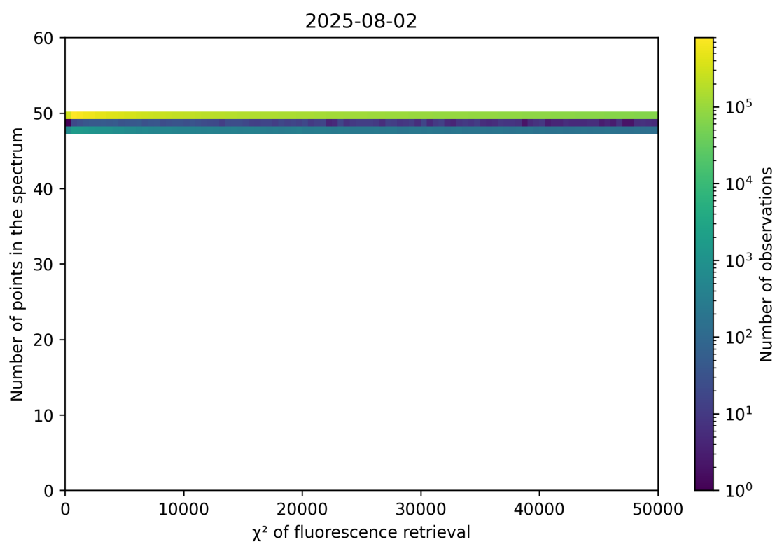
Figure 68: Scatter density plot of “ \chi^2 of fluorescence retrieval” against “Number of points in the spectrum” for 2025-08-01 to 2025-08-03.
