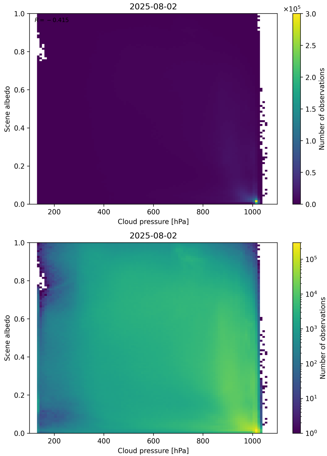
Figure 83: Scatter density plot of “Cloud pressure” against “Scene albedo” for 2025-08-01 to 2025-08-03.
