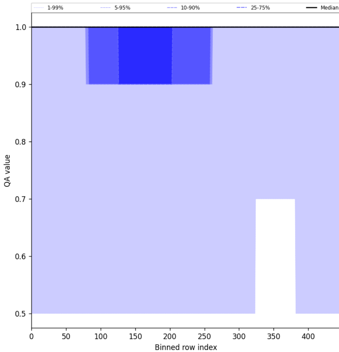
Figure 46: Along track statistics of “QA value” for 2025-08-01 to 2025-08-03
