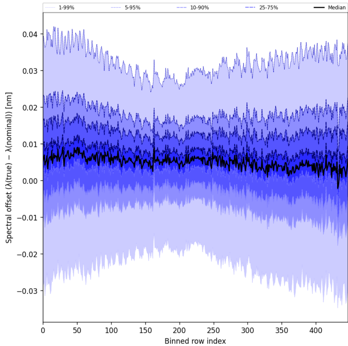
Figure 62: Along track statistics of “Spectral offset ( \lambda_{\text{true}} - \lambda_{\text{nominal}} )” for 2025-08-01 to 2025-08-03
