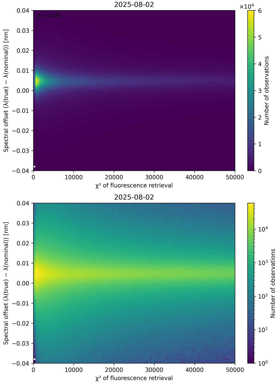
Figure 69: Scatter density plot of “ \chi^2 of fluorescence retrieval” against “Spectral offset ( \lambda_{\text{true}} - \lambda_{\text{nominal}} )” for 2025-08-01 to 2025-08-03.
