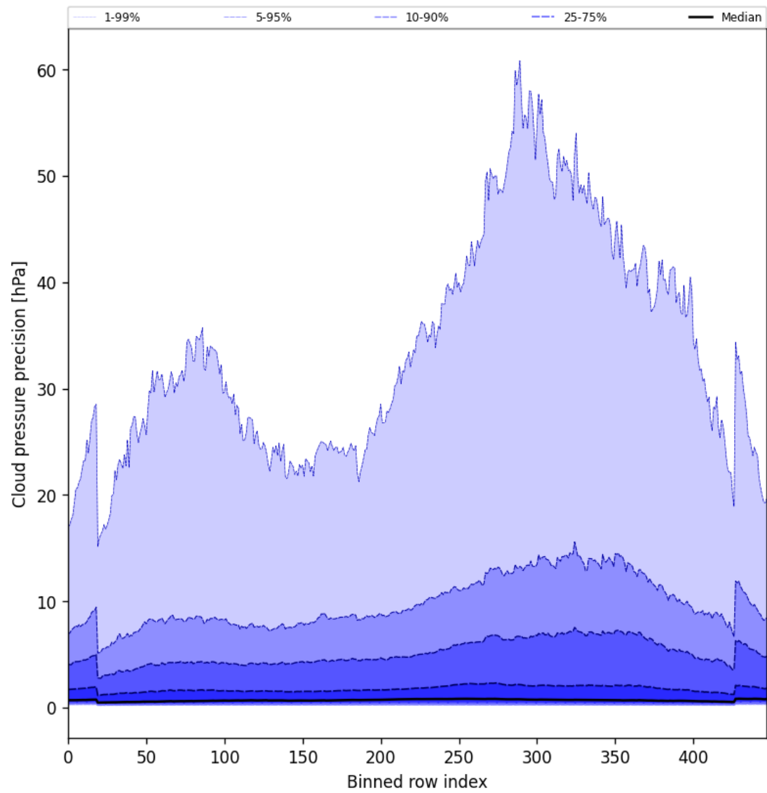
Figure 48: Along track statistics of “Cloud pressure precision” for 2025-08-01 to 2025-08-03
