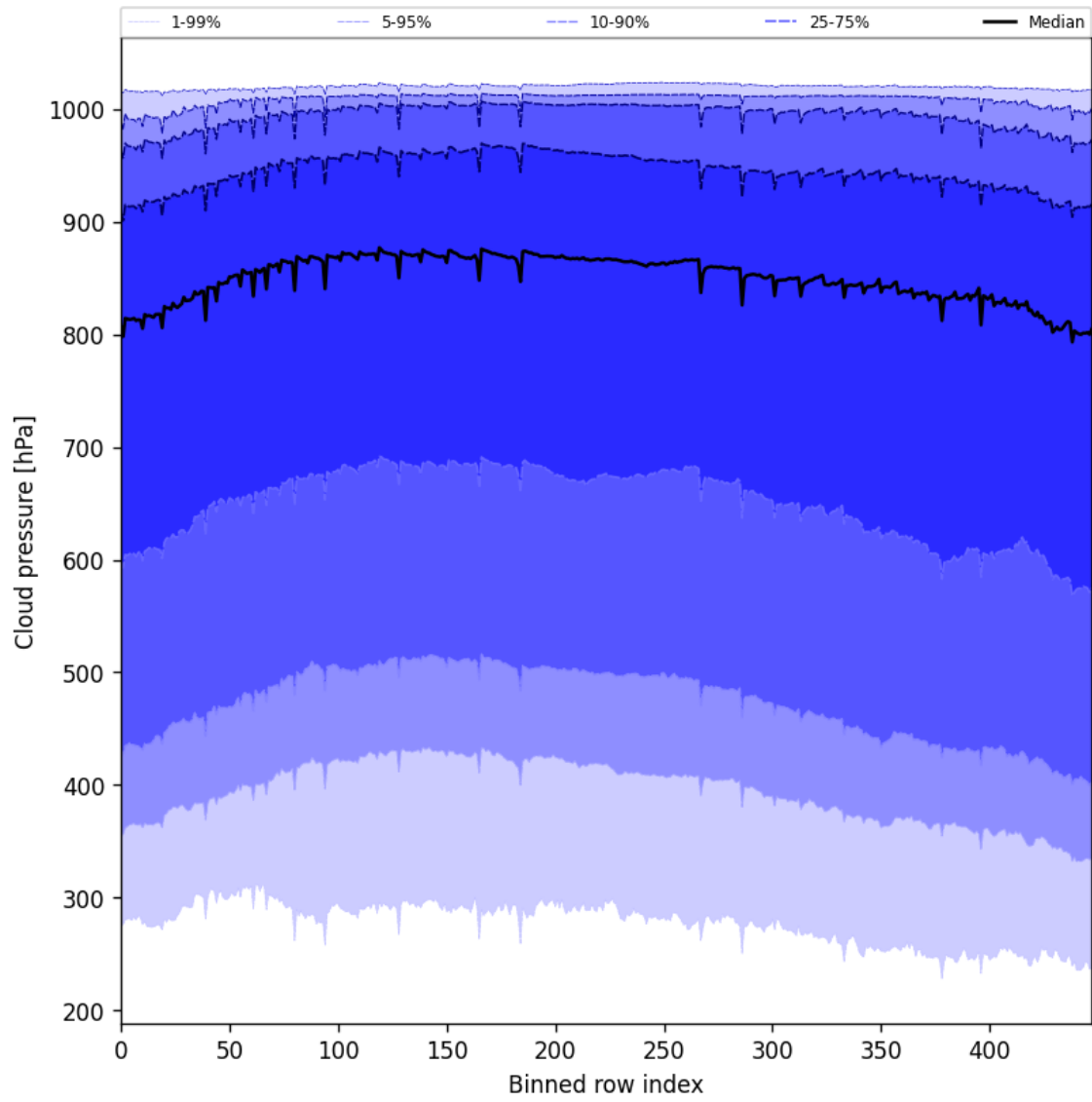
Figure 47: Along track statistics of “Cloud pressure” for 2025-08-01 to 2025-08-03
