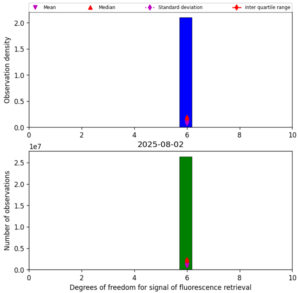
Figure 43: Histogram of "Degrees of freedom for signal of fluorescence retrieval" for 2025-08-01 to 2025-08-03
