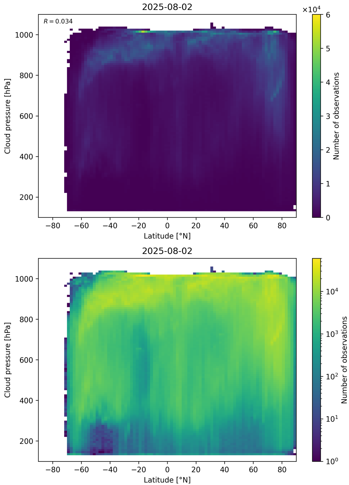
Figure 91: Scatter density plot of “Latitude” against “Cloud pressure” for 2025-08-01 to 2025-08-03.
