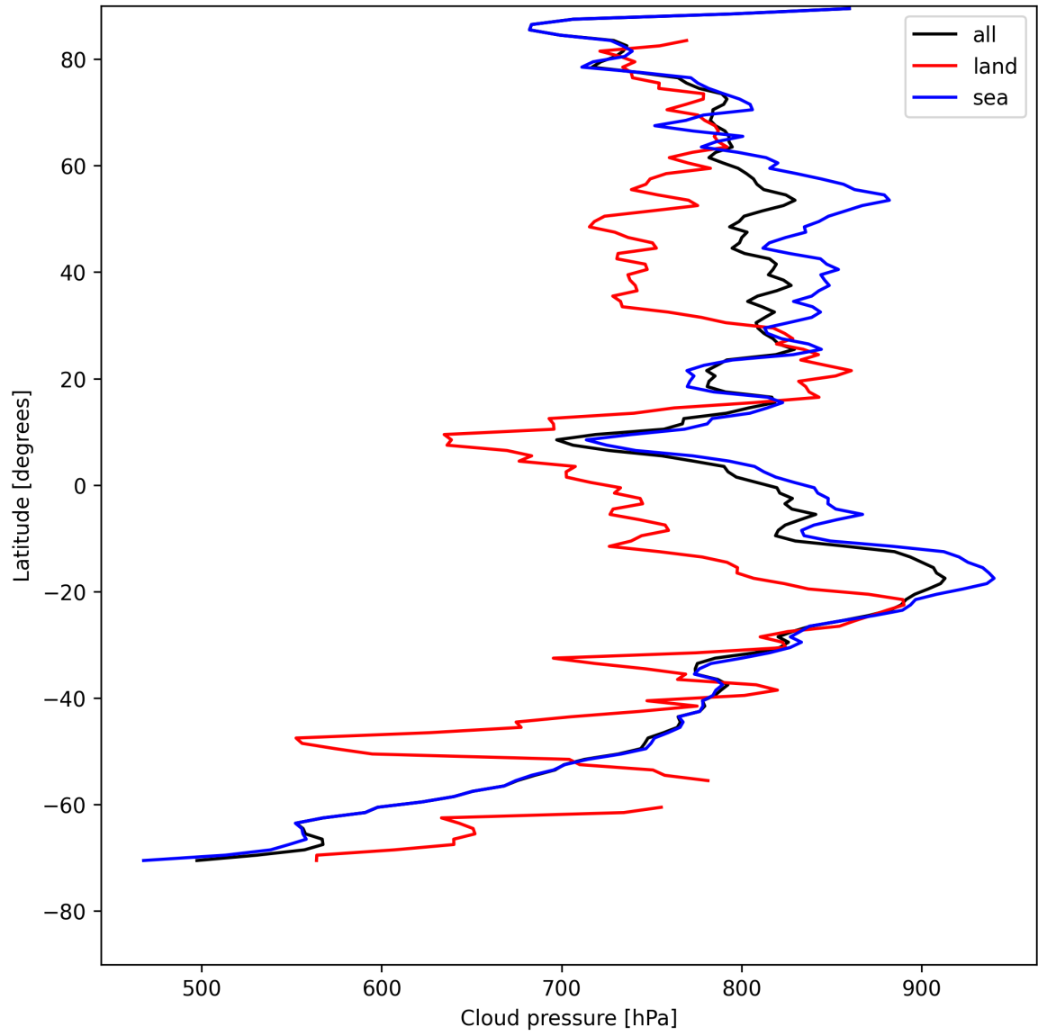
Figure 13: Zonal average of “Cloud pressure” for 2025-08-01 to 2025-08-03.
