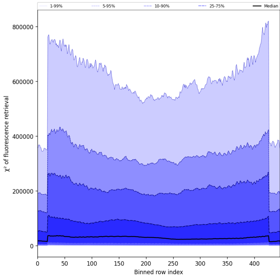
Figure 59: Along track statistics of “ \chi^2 of fluorescence retrieval” for 2025-08-01 to 2025-08-03
