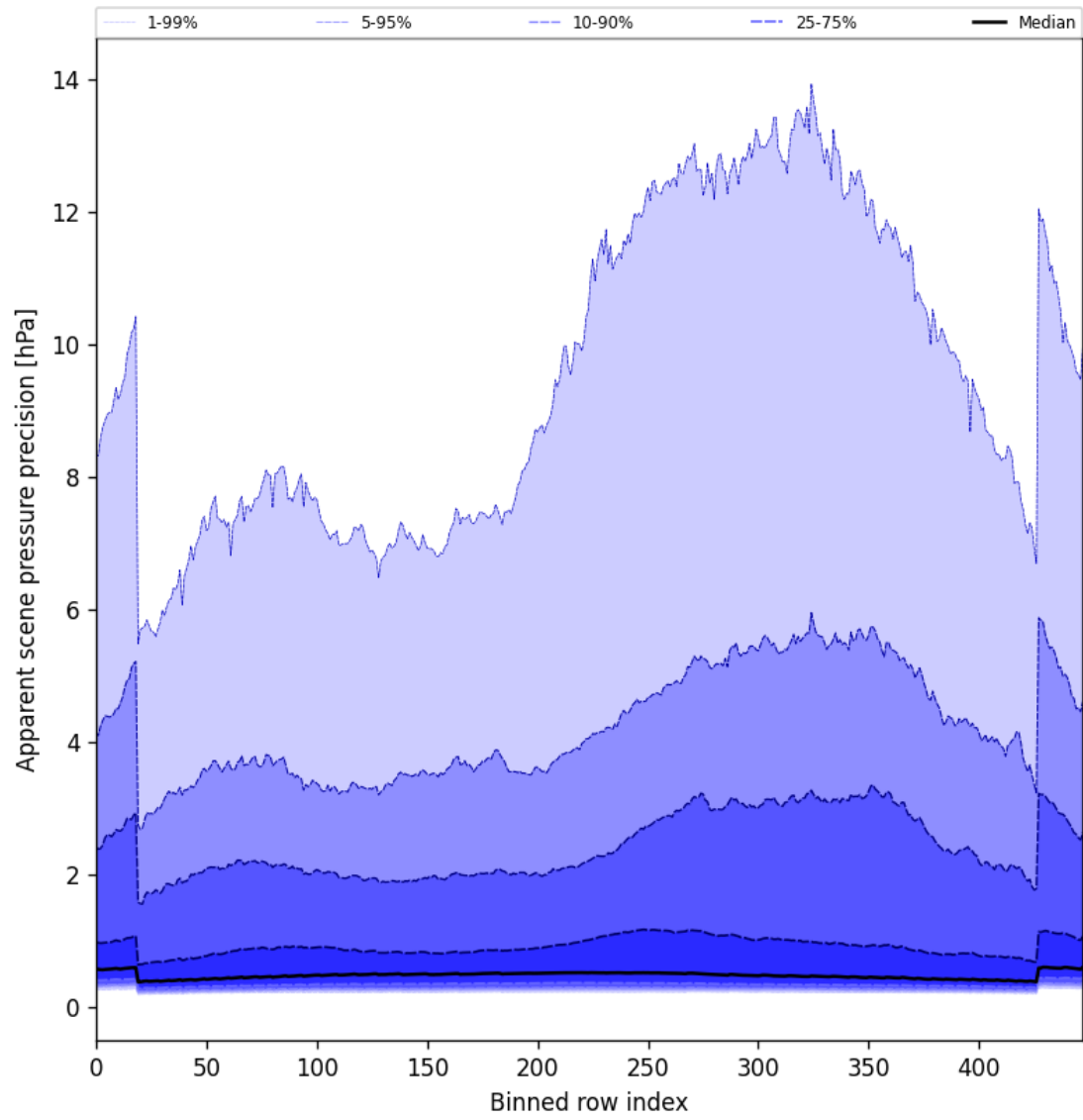
Figure 54: Along track statistics of “Apparent scene pressure precision” for 2025-08-01 to 2025-08-03
