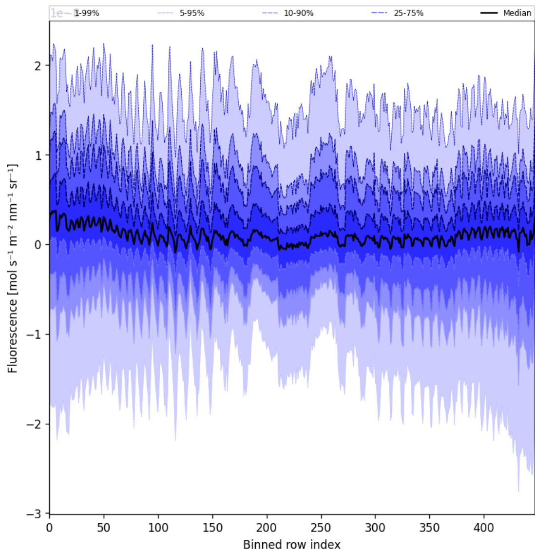
Figure 57: Along track statistics of “Fluorescence” for 2025-08-01 to 2025-08-03
