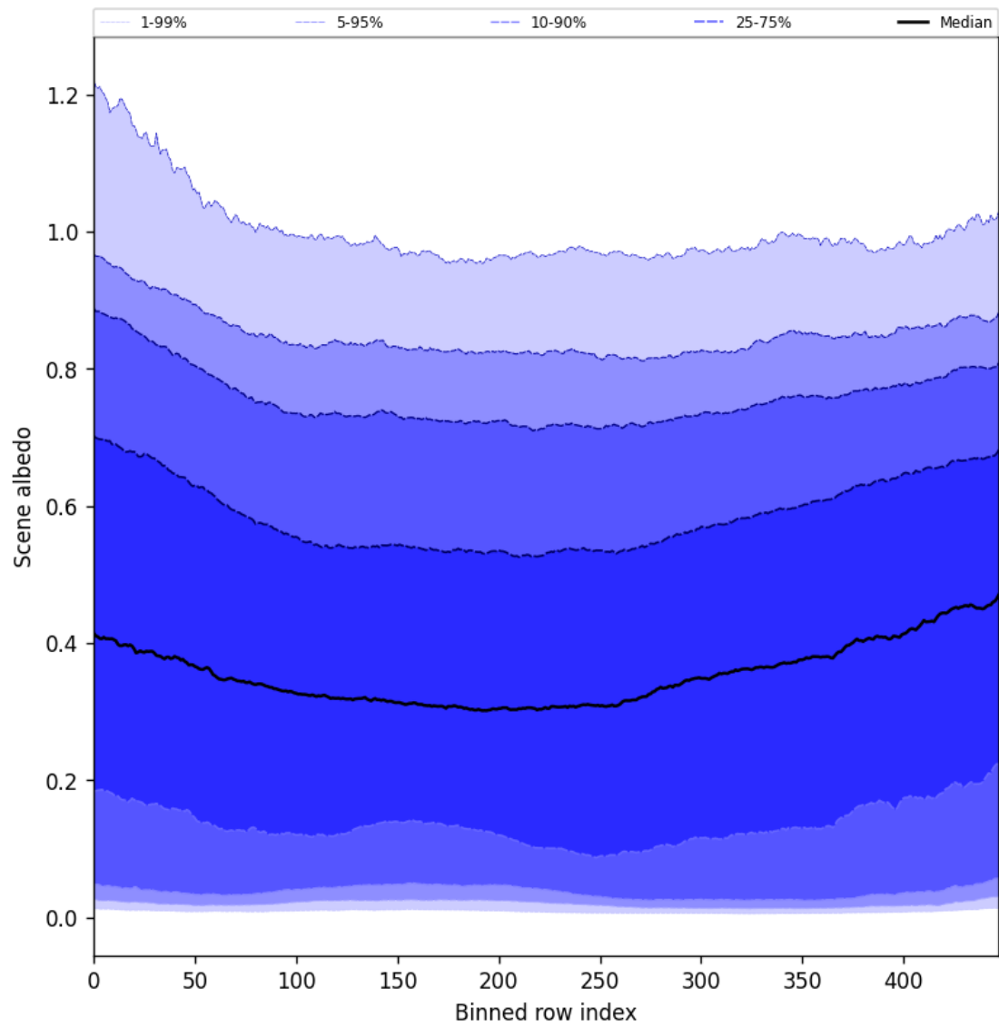
Figure 51: Along track statistics of “Scene albedo” for 2025-08-01 to 2025-08-03
