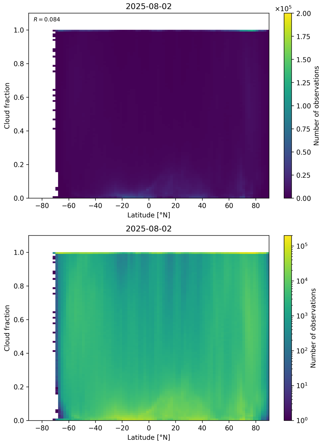
Figure 90: Scatter density plot of “Latitude” against “Cloud fraction” for 2025-08-01 to 2025-08-03.
