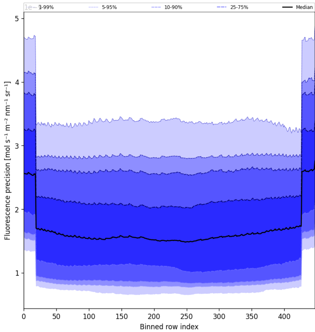
Figure 58: Along track statistics of “Fluorescence precision” for 2025-08-01 to 2025-08-03
