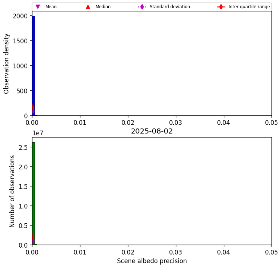
Figure 35: Histogram of “Scene albedo precision” for 2025-08-01 to 2025-08-03
