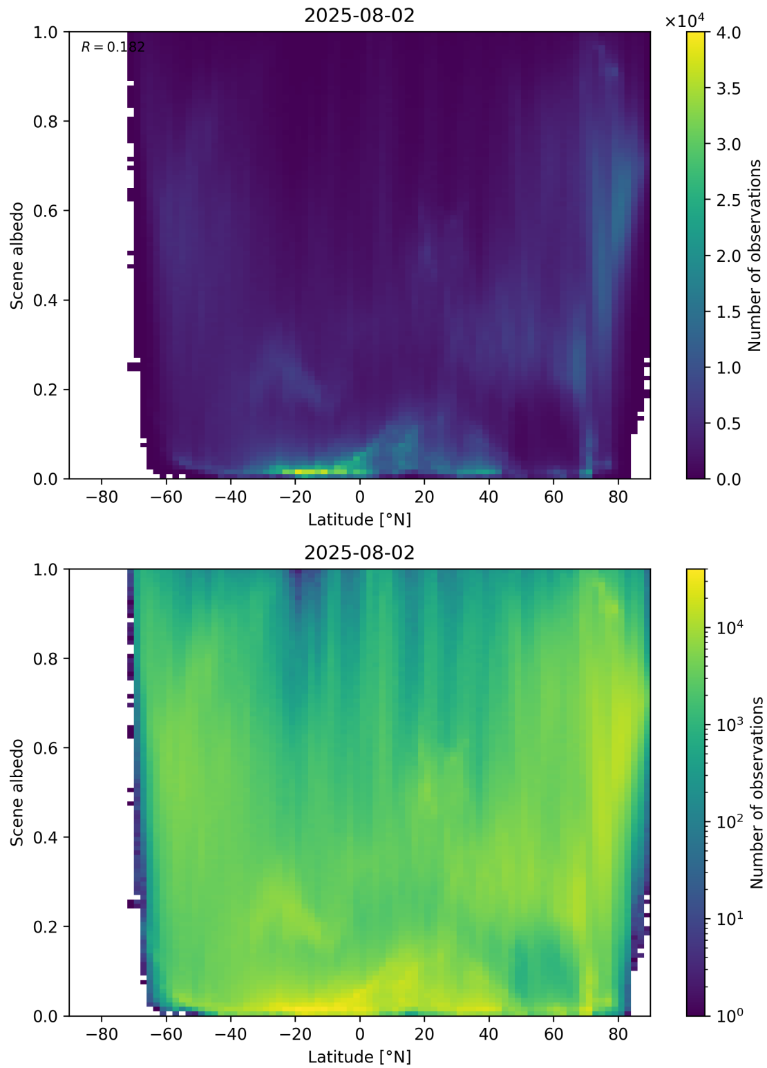
Figure 95: Scatter density plot of “Latitude” against “Scene albedo” for 2025-08-01 to 2025-08-03.
