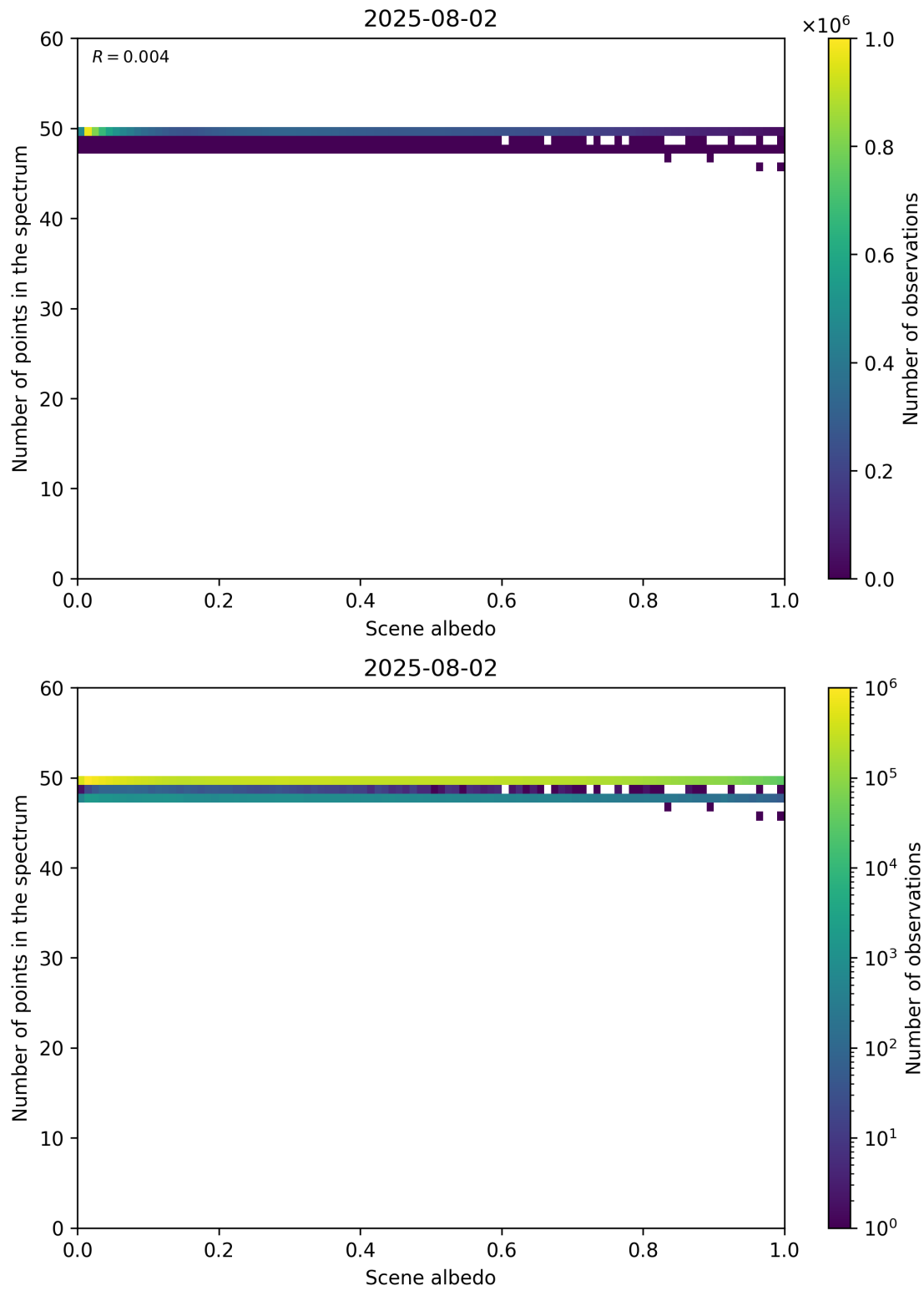
Figure 106: Scatter density plot of “Scene albedo” against “Number of points in the spectrum” for 2025-08-01 to 2025-08-03.
