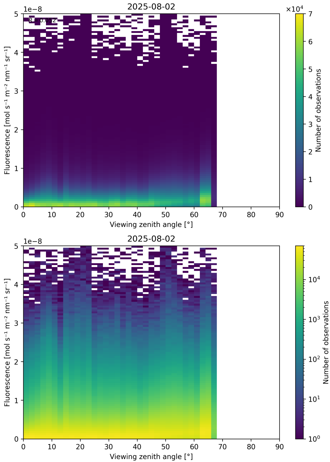
Figure 122: Scatter density plot of “Viewing zenith angle” against “Fluorescence” for 2025-08-01 to 2025-08-03.
