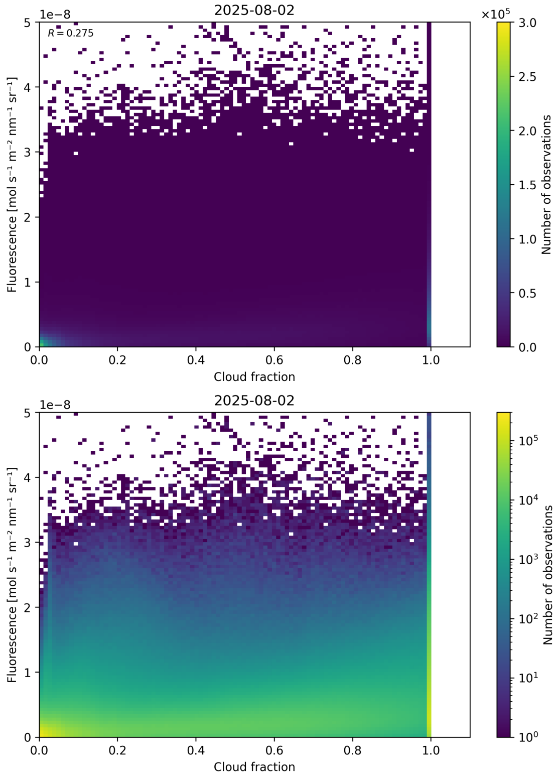
Figure 72: Scatter density plot of “Cloud fraction” against “Fluorescence” for 2025-08-01 to 2025-08-03.
