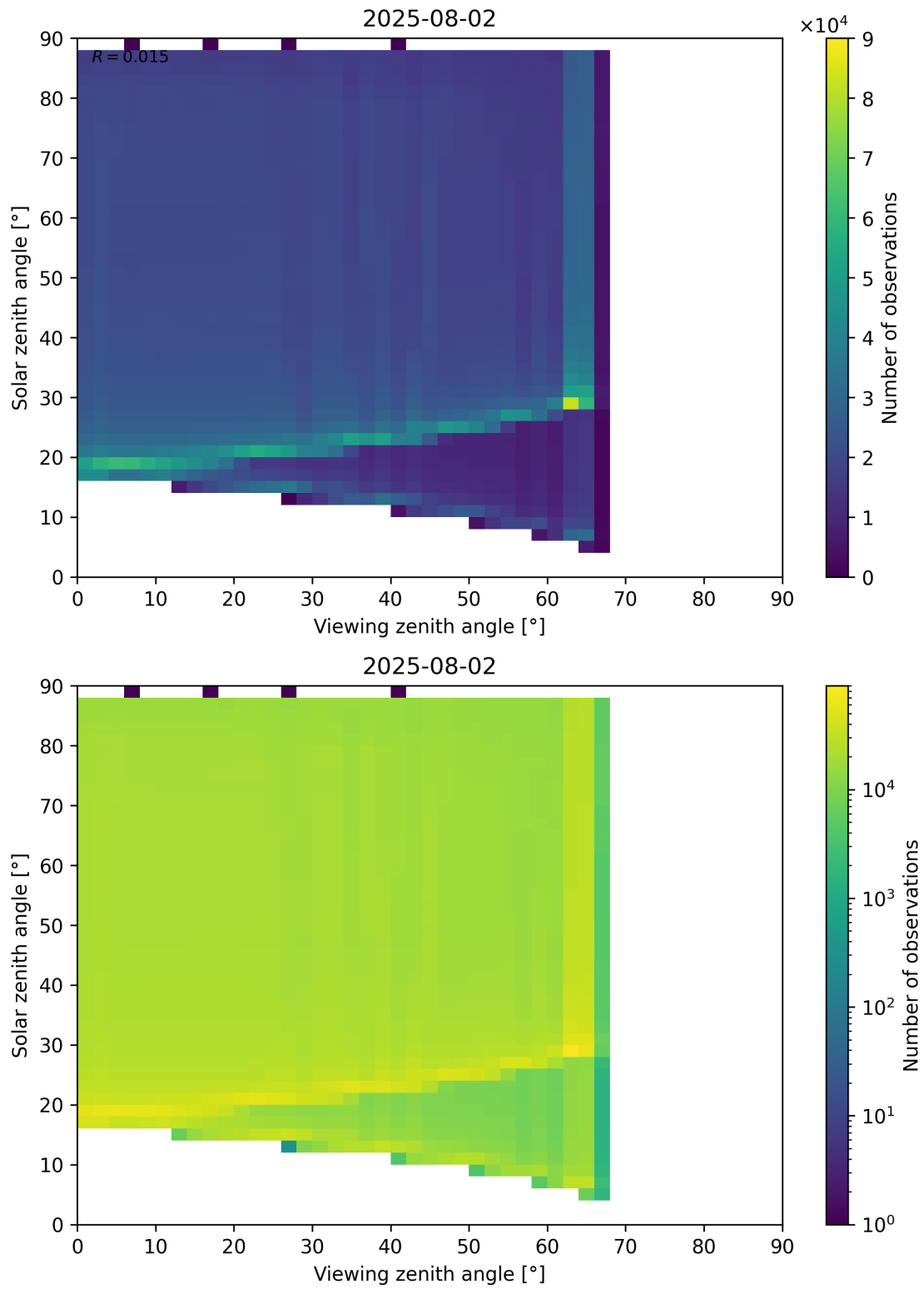
Figure 127: Scatter density plot of “Viewing zenith angle” against “Solar zenith angle” for 2025-08-01 to 2025-08-03.
