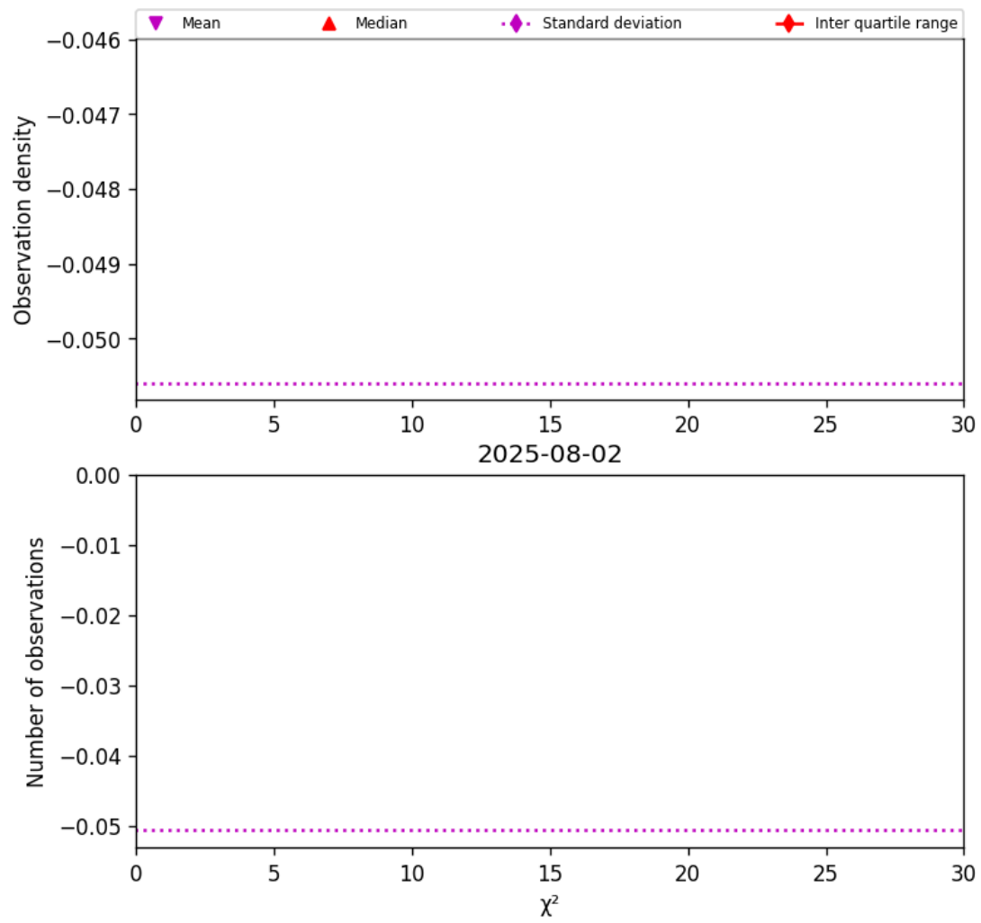
Figure 38: Histogram of “ \chi^2 ” for 2025-08-01 to 2025-08-03
