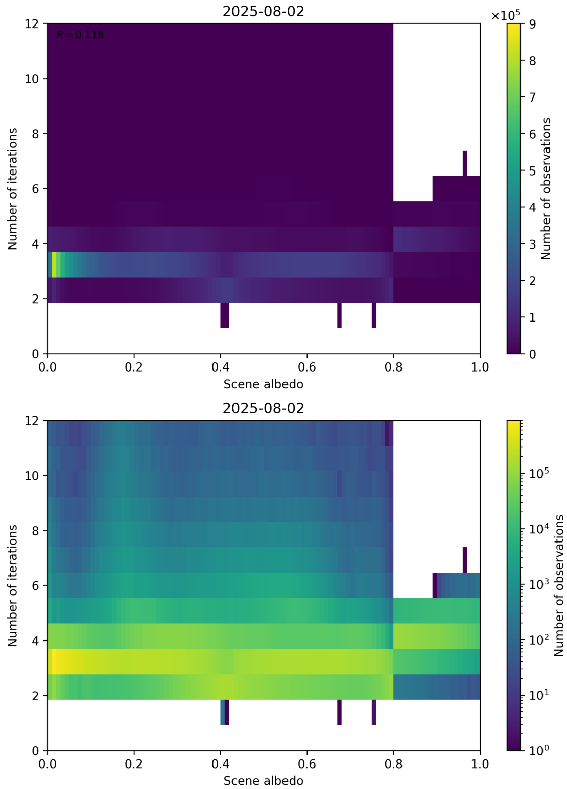
Figure 105: Scatter density plot of “Scene albedo” against “Number of iterations” for 2025-08-01 to 2025-08-03.
