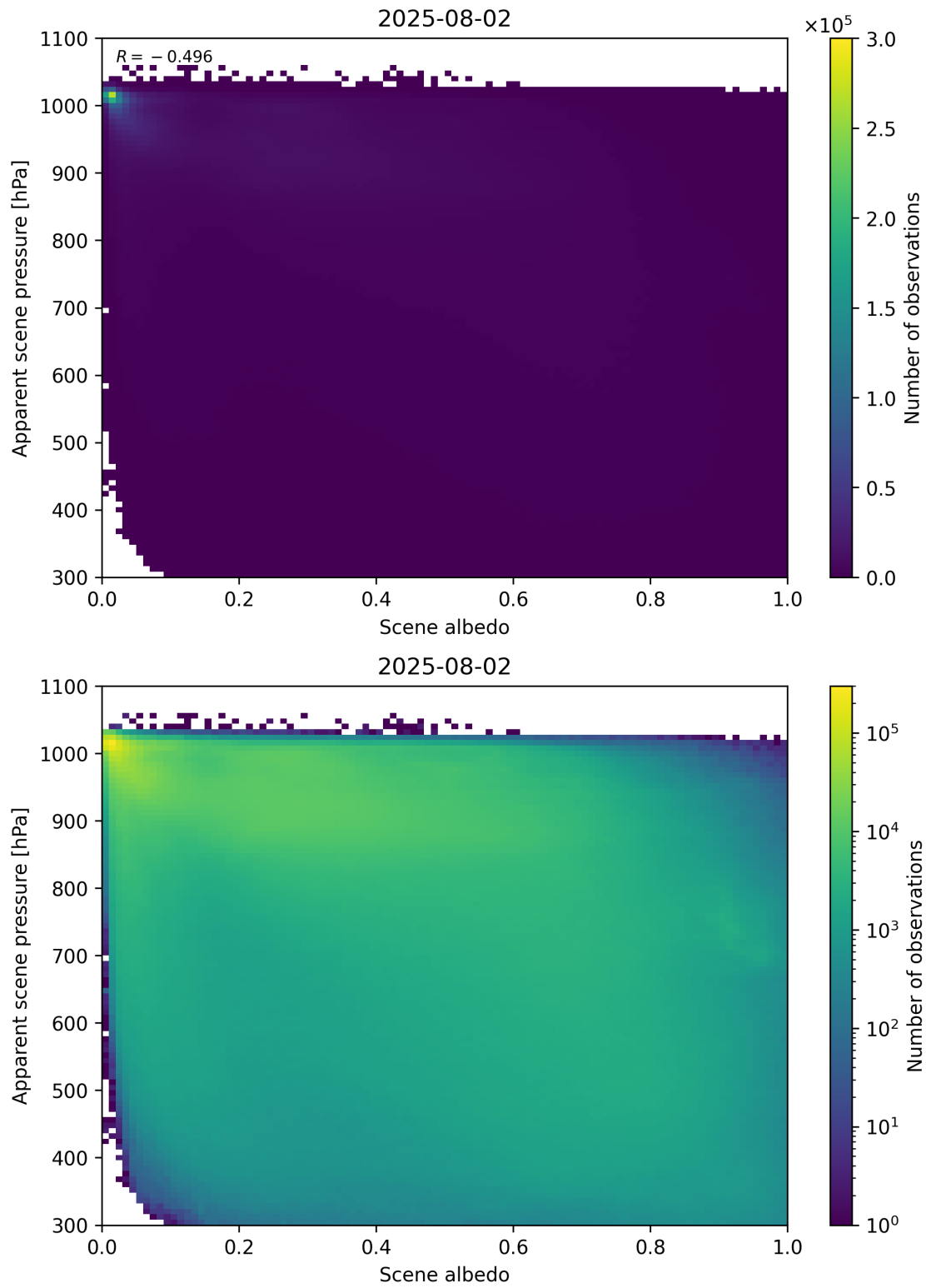
Figure 102: Scatter density plot of “Scene albedo” against “Apparent scene pressure” for 2025-08-01 to 2025-08-03.
