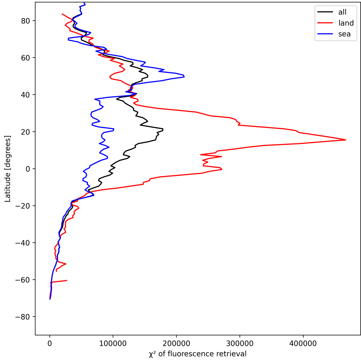
Figure 25: Zonal average of “ \chi^2 of fluorescence retrieval” for 2025-08-01 to 2025-08-03.
