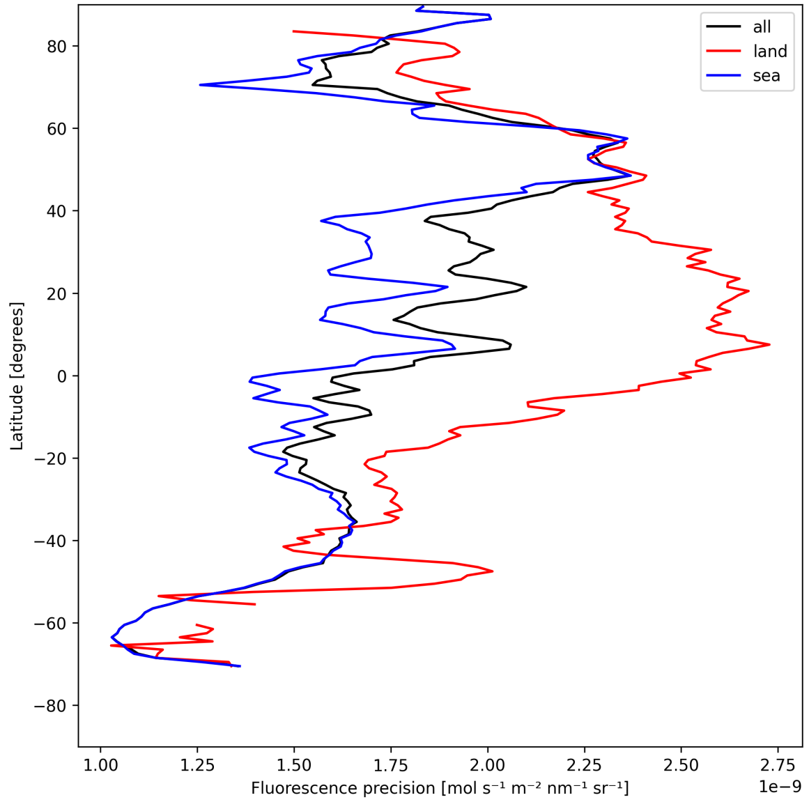
Figure 24: Zonal average of “Fluorescence precision” for 2025-08-01 to 2025-08-03.
