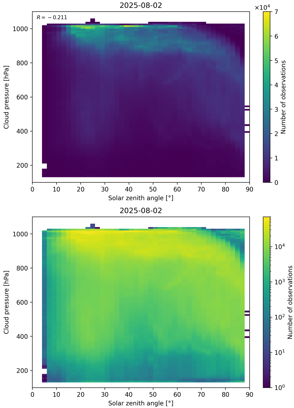
Figure 111: Scatter density plot of “Solar zenith angle” against “Cloud pressure” for 2025-08-01 to 2025-08-03.
