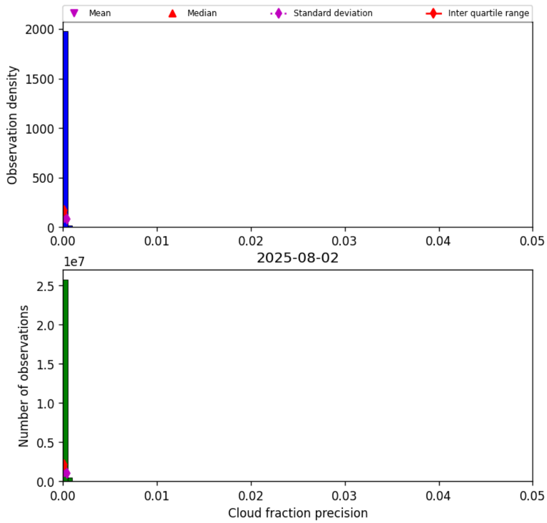
Figure 33: Histogram of “Cloud fraction precision” for 2025-08-01 to 2025-08-03
