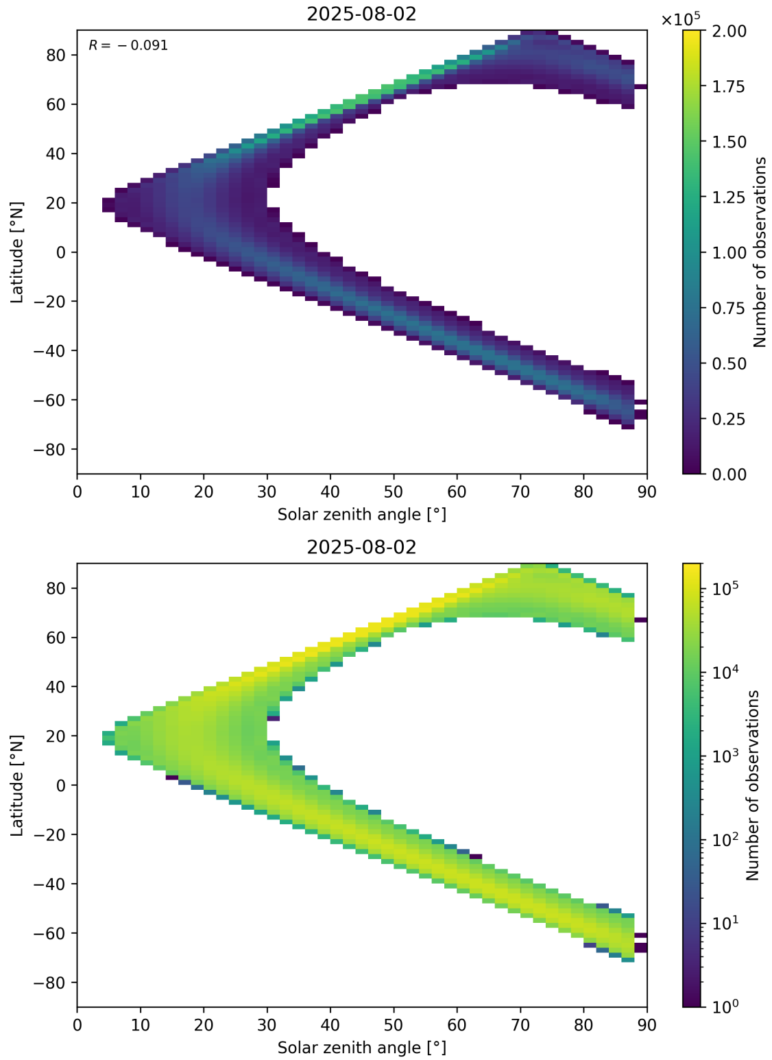
Figure 113: Scatter density plot of “Solar zenith angle” against “Latitude” for 2025-08-01 to 2025-08-03.
