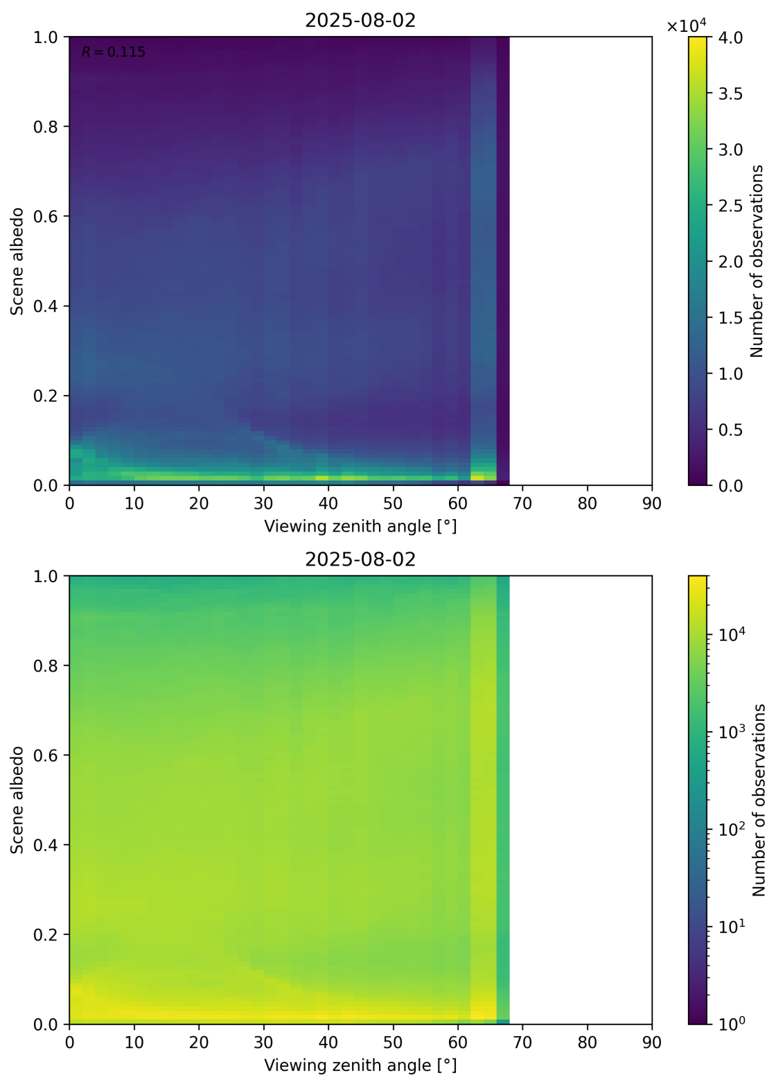
Figure 126: Scatter density plot of “Viewing zenith angle” against “Scene albedo” for 2025-08-01 to 2025-08-03.
