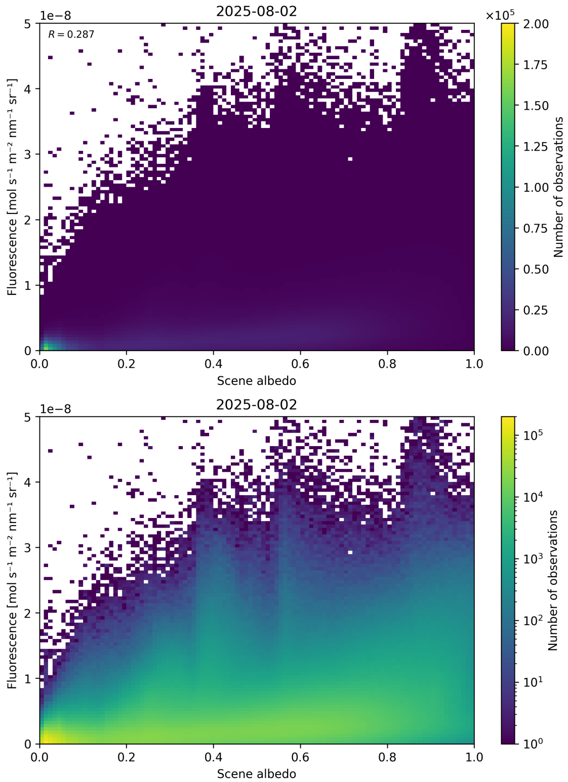
Figure 104: Scatter density plot of “Scene albedo” against “Fluorescence” for 2025-08-01 to 2025-08-03.
