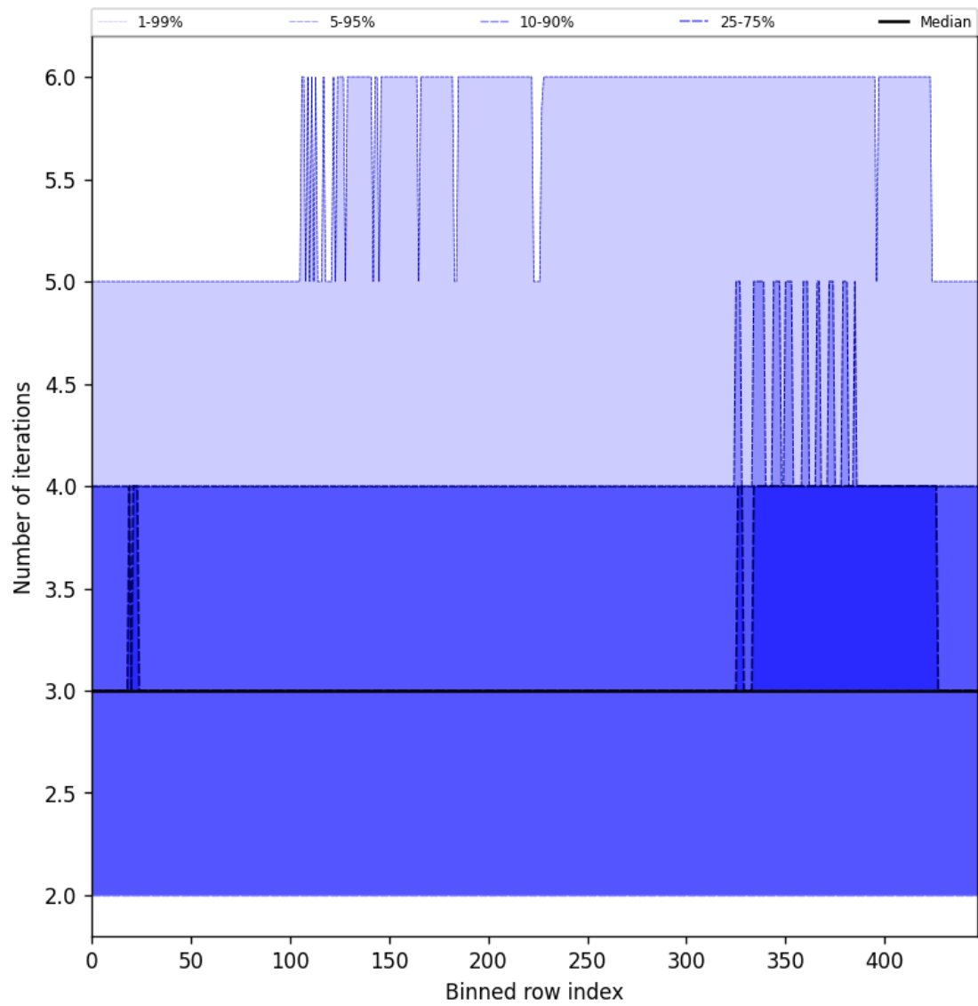
Figure 56: Along track statistics of “Number of iterations” for 2025-08-01 to 2025-08-03
