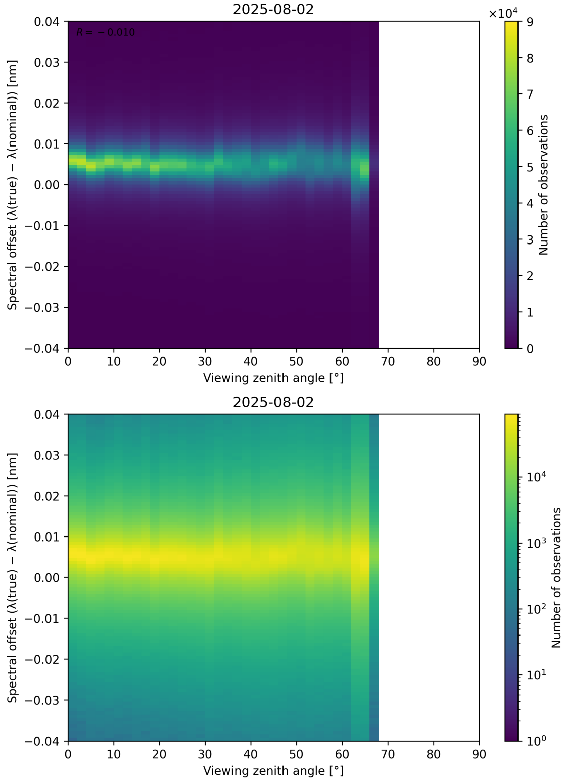
Figure 128: Scatter density plot of “Viewing zenith angle” against “Spectral offset ( \lambda_{\text{true}} - \lambda_{\text{nominal}} )” for 2025-08-01 to 2025-08-03.
