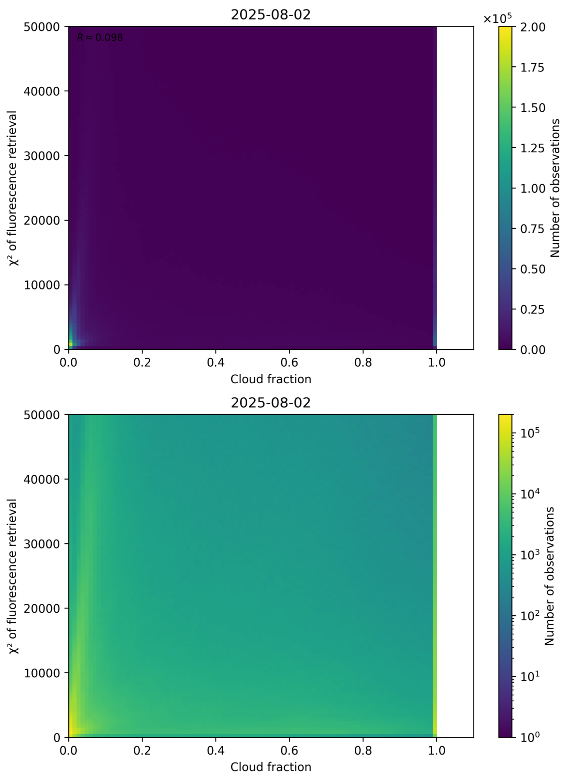
Figure 71: Scatter density plot of “Cloud fraction” against “ \chi^2 of fluorescence retrieval” for 2025-08-01 to 2025-08-03.
