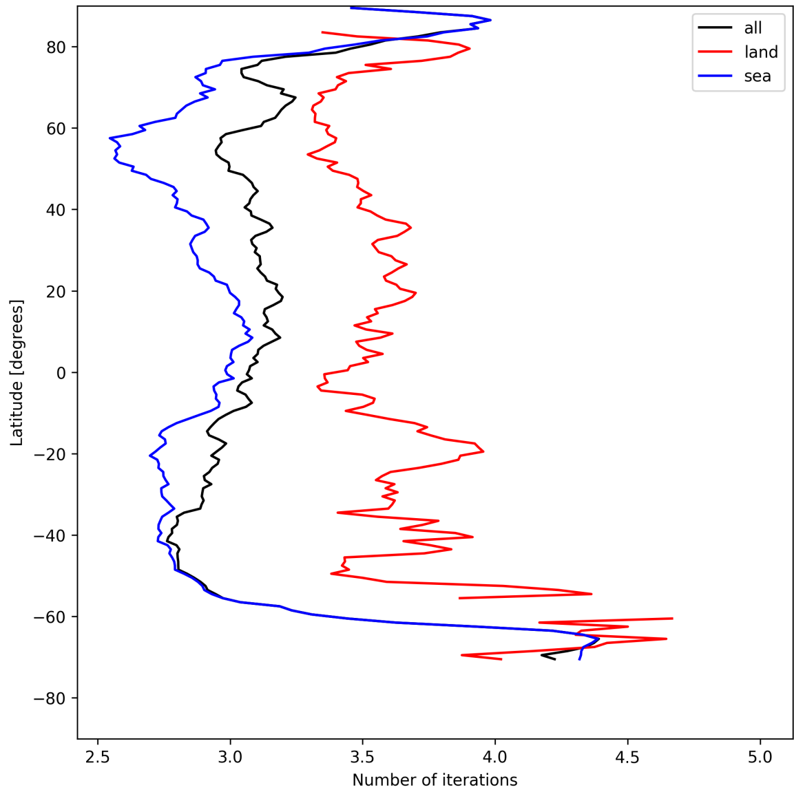
Figure 22: Zonal average of “Number of iterations” for 2025-08-01 to 2025-08-03.
