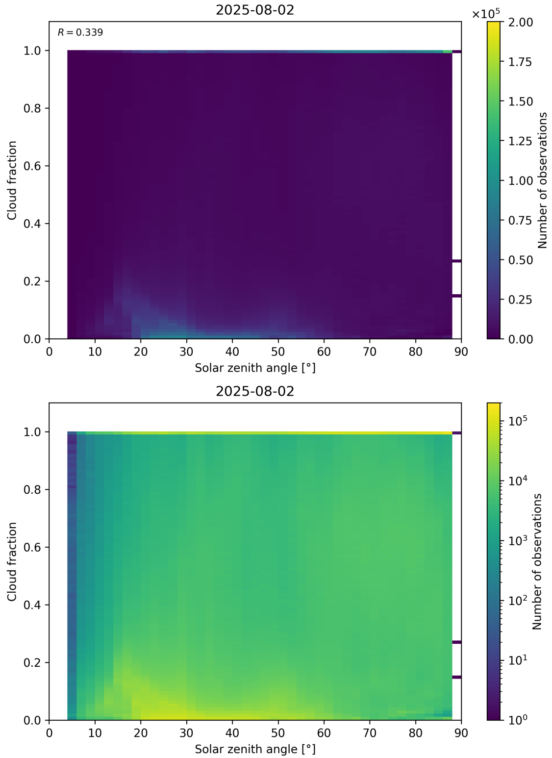
Figure 110: Scatter density plot of “Solar zenith angle” against “Cloud fraction” for 2025-08-01 to 2025-08-03.
