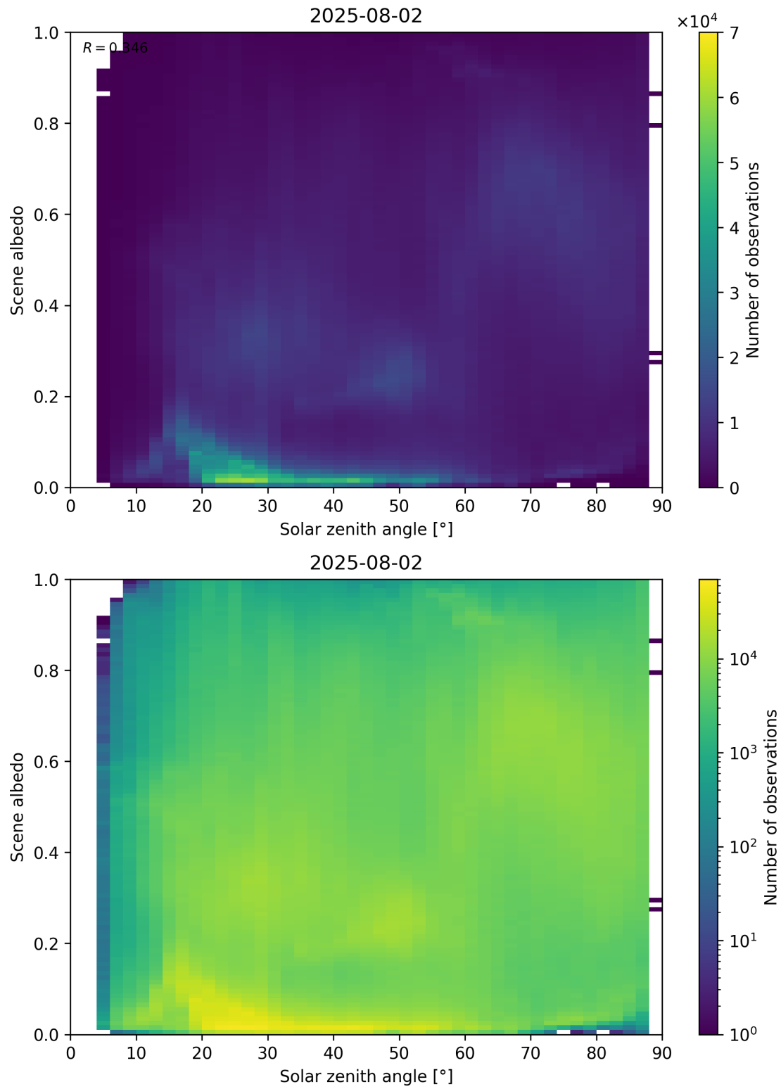
Figure 116: Scatter density plot of “Solar zenith angle” against “Scene albedo” for 2025-08-01 to 2025-08-03.
