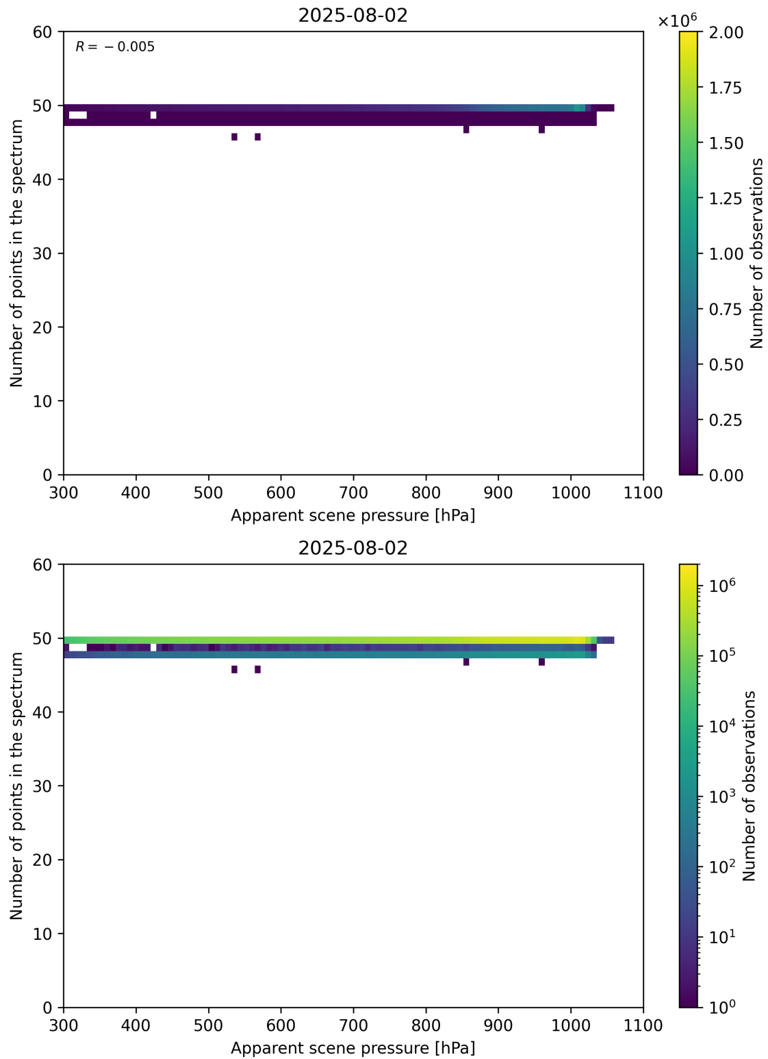
Figure 66: Scatter density plot of “Apparent scene pressure” against “Number of points in the spectrum” for 2025-08-01 to 2025-08-03.
