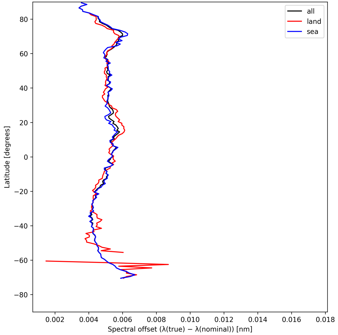
Figure 28: Zonal average of “Spectral offset ( \lambda_{\text{true}} - \lambda_{\text{nominal}} )” for 2025-08-01 to 2025-08-03.
