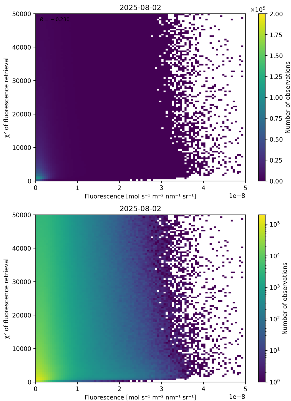
Figure 85: Scatter density plot of “Fluorescence” against “ \chi^2 of fluorescence retrieval” for 2025-08-01 to 2025-08-03.
