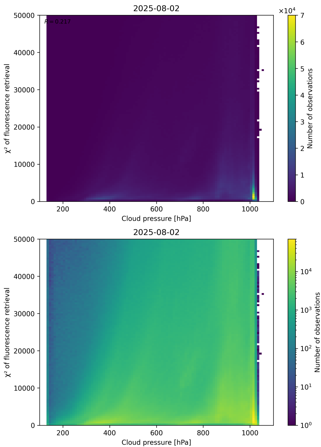
Figure 78: Scatter density plot of “Cloud pressure” against “ \chi^2 of fluorescence retrieval” for 2025-08-01 to 2025-08-03.
