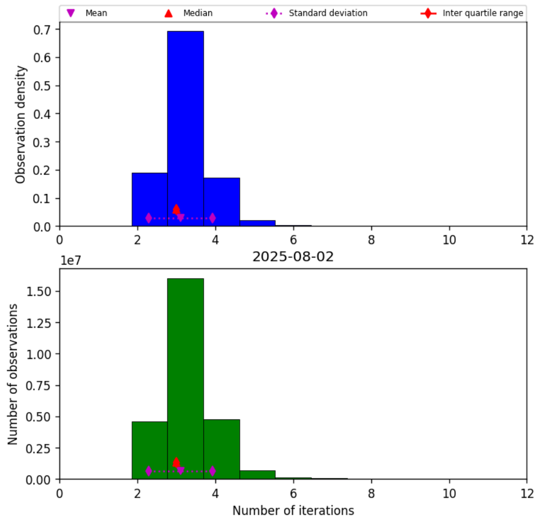
Figure 39: Histogram of “Number of iterations” for 2025-08-01 to 2025-08-03
