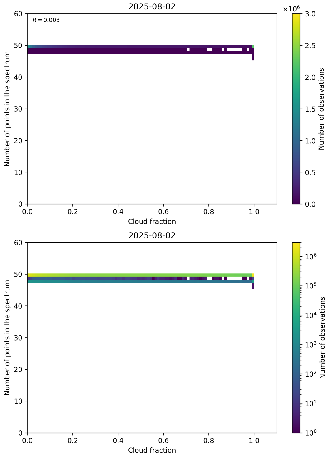
Figure 74: Scatter density plot of “Cloud fraction” against “Number of points in the spectrum” for 2025-08-01 to 2025-08-03.
