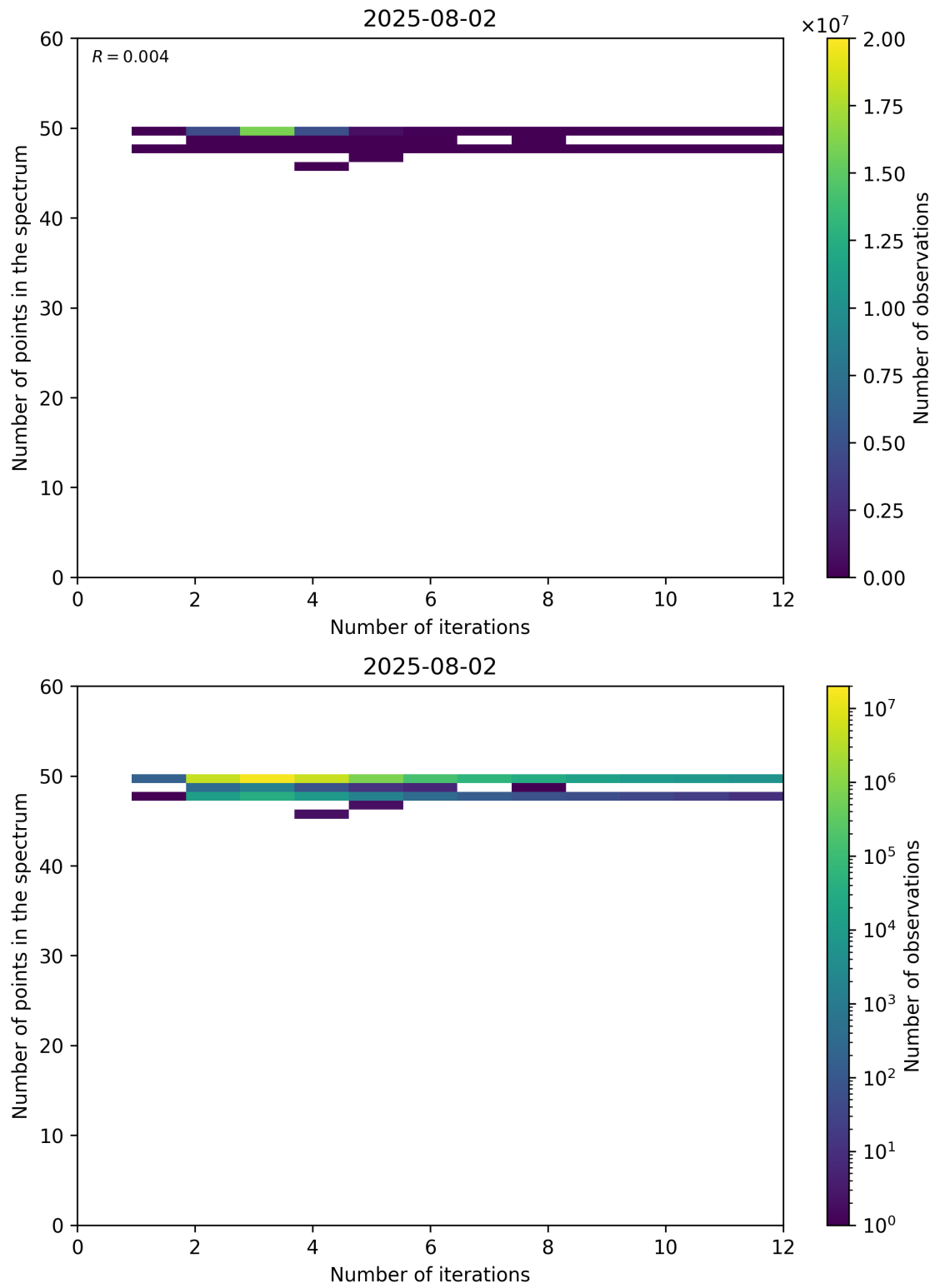
Figure 99: Scatter density plot of “Number of iterations” against “Number of points in the spectrum” for 2025-08-01 to 2025-08-03.
