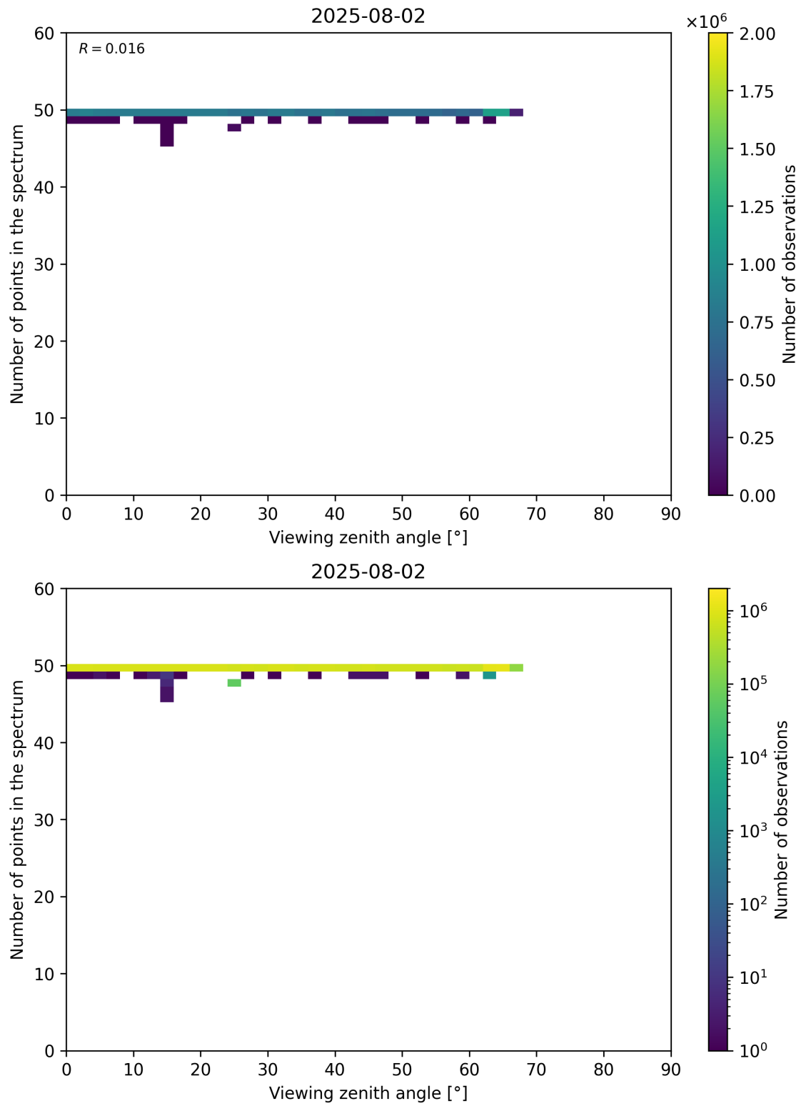
Figure 125: Scatter density plot of “Viewing zenith angle” against “Number of points in the spectrum” for 2025-08-01 to 2025-08-03.
