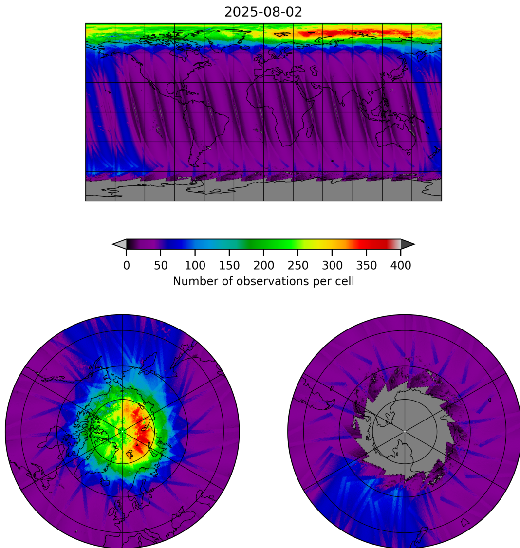
Figure 11: Map of the number of observations for 2025-08-01 to 2025-08-03
