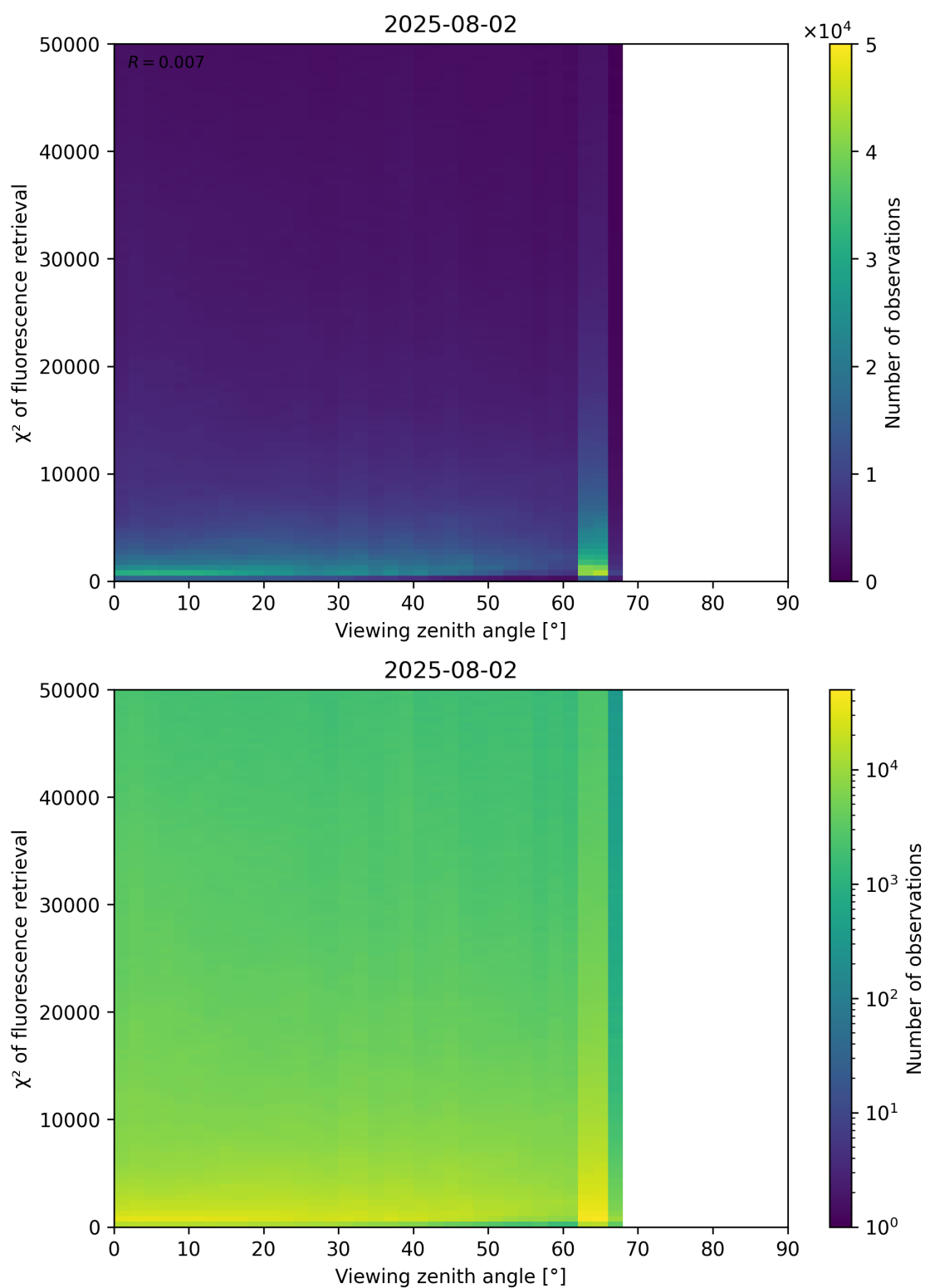
Figure 119: Scatter density plot of “Viewing zenith angle” against “ \chi^2 of fluorescence retrieval” for 2025-08-01 to 2025-08-03.
