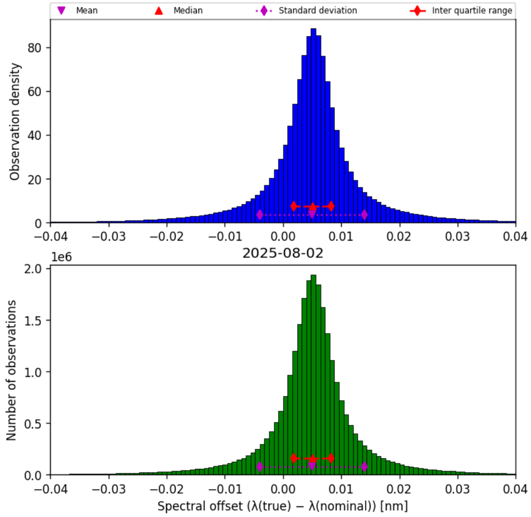
Figure 45: Histogram of “Spectral offset ( \lambda_{\text{true}} - \lambda_{\text{nominal}} )” for 2025-08-01 to 2025-08-03
