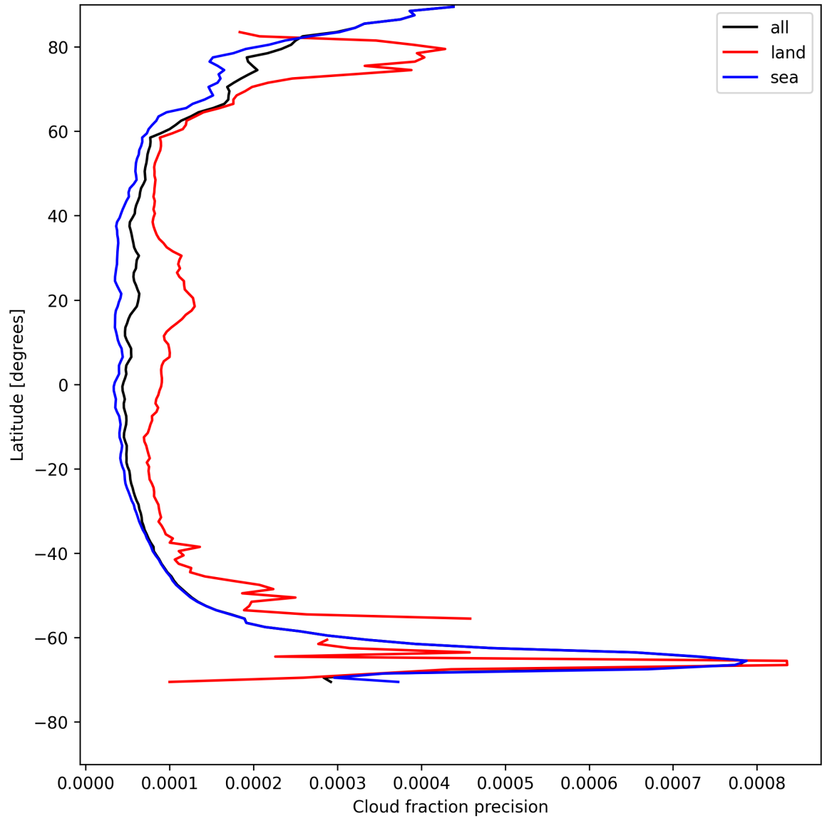
Figure 16: Zonal average of “Cloud fraction precision” for 2025-08-01 to 2025-08-03.
