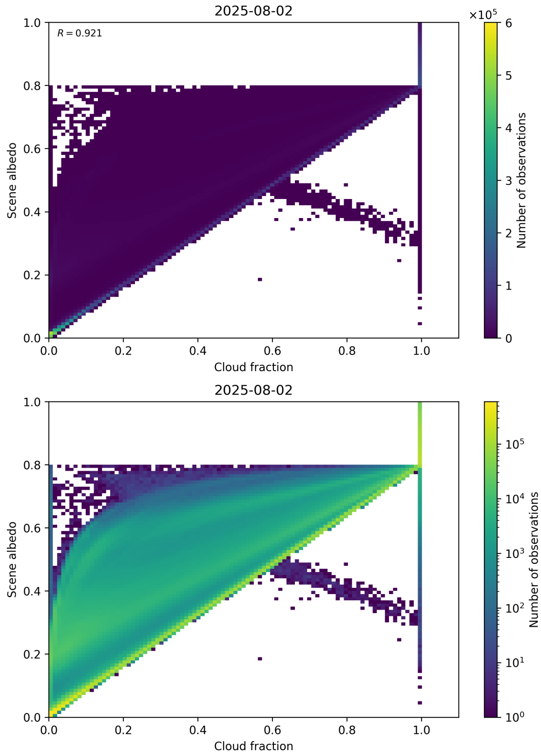
Figure 75: Scatter density plot of “Cloud fraction” against “Scene albedo” for 2025-08-01 to 2025-08-03.
