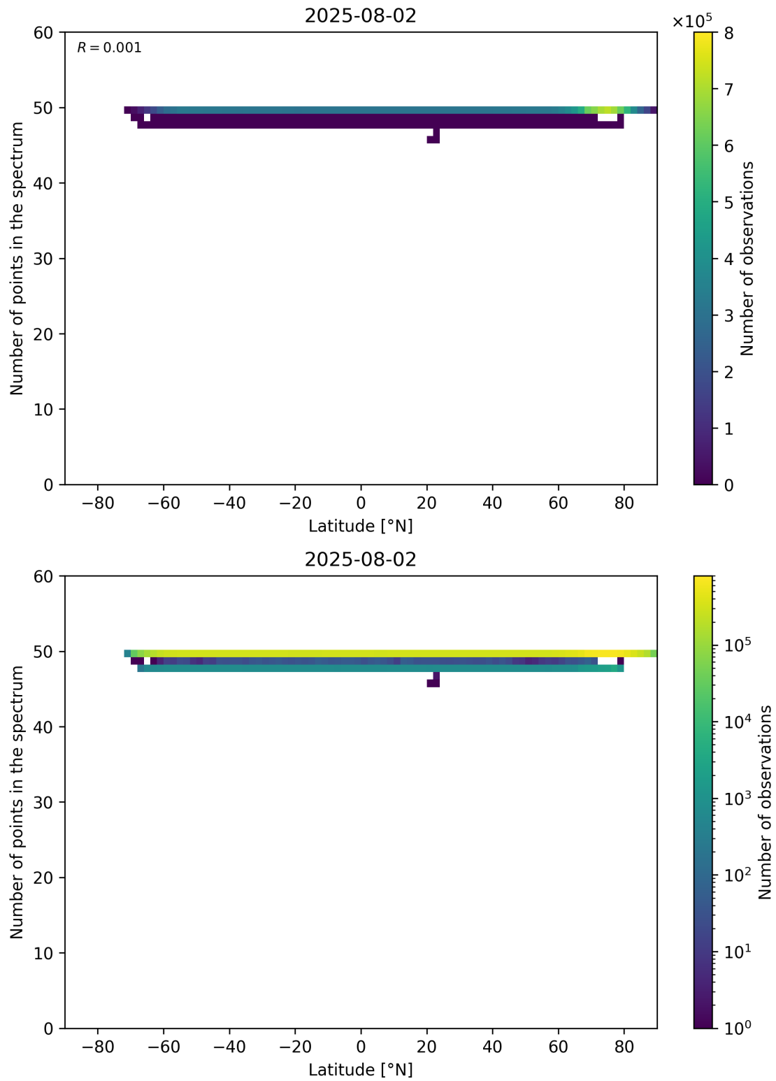
Figure 94: Scatter density plot of “Latitude” against “Number of points in the spectrum” for 2025-08-01 to 2025-08-03.
