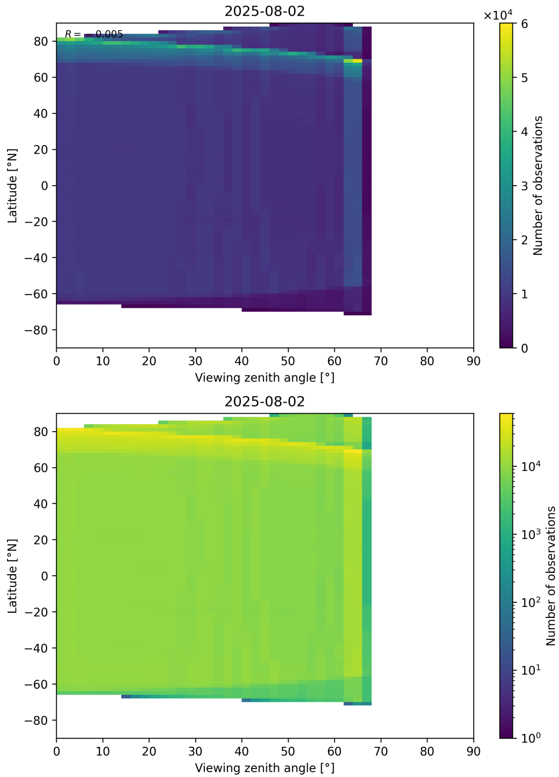
Figure 123: Scatter density plot of “Viewing zenith angle” against “Latitude” for 2025-08-01 to 2025-08-03.
