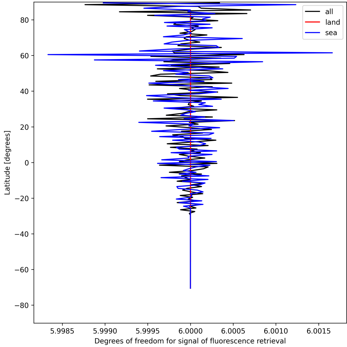
Figure 26: Zonal average of “Degrees of freedom for signal of fluorescence retrieval” for 2025-08-01 to 2025-08-03.
