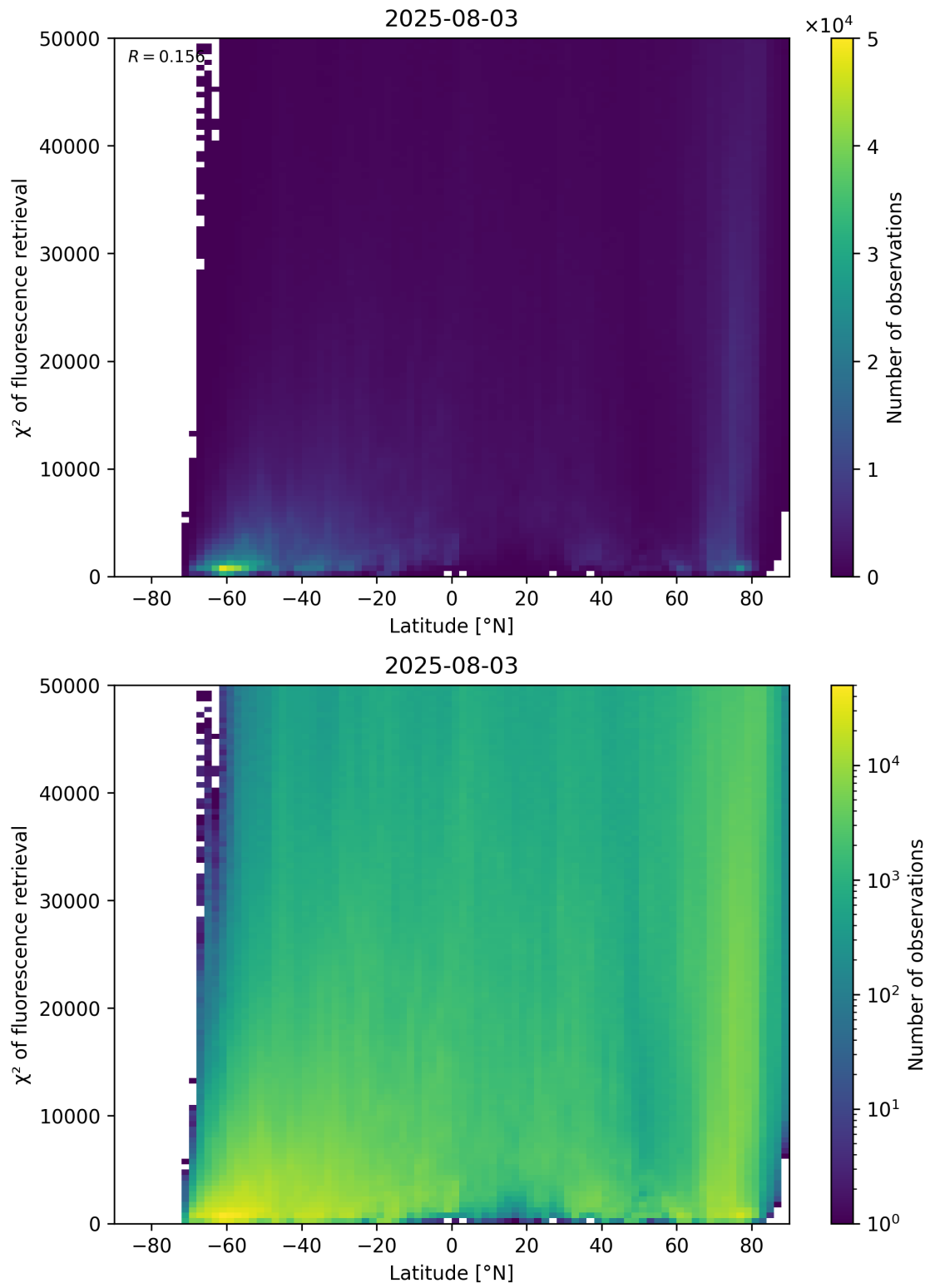
Figure 89: Scatter density plot of “Latitude” against “ \chi^2 of fluorescence retrieval” for 2025-08-03 to 2025-08-04.
