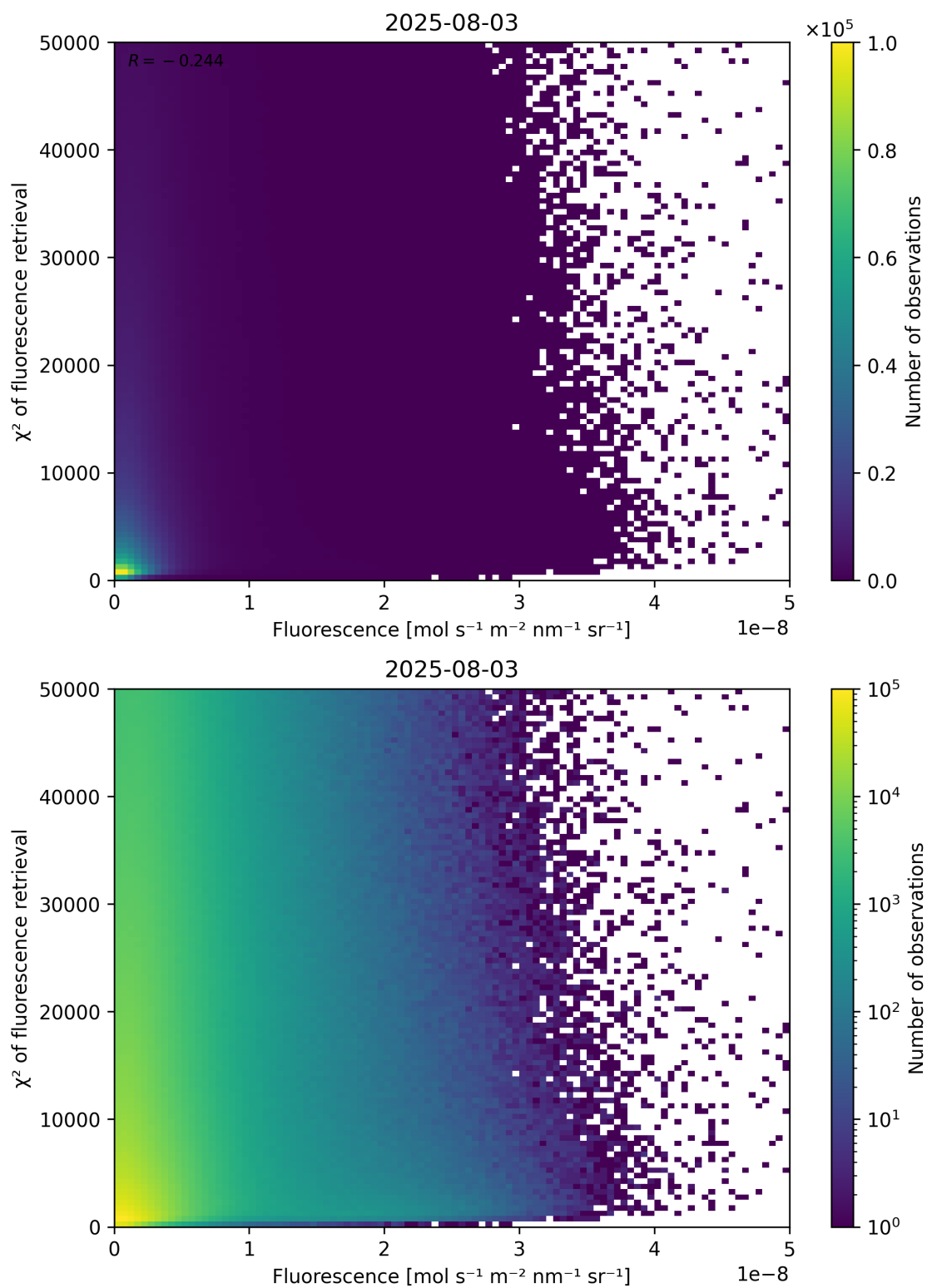
Figure 85: Scatter density plot of “Fluorescence” against “ \chi^2 of fluorescence retrieval” for 2025-08-03 to 2025-08-04.
