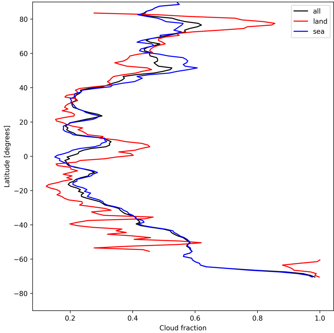
Figure 15: Zonal average of “Cloud fraction” for 2025-08-03 to 2025-08-04.
