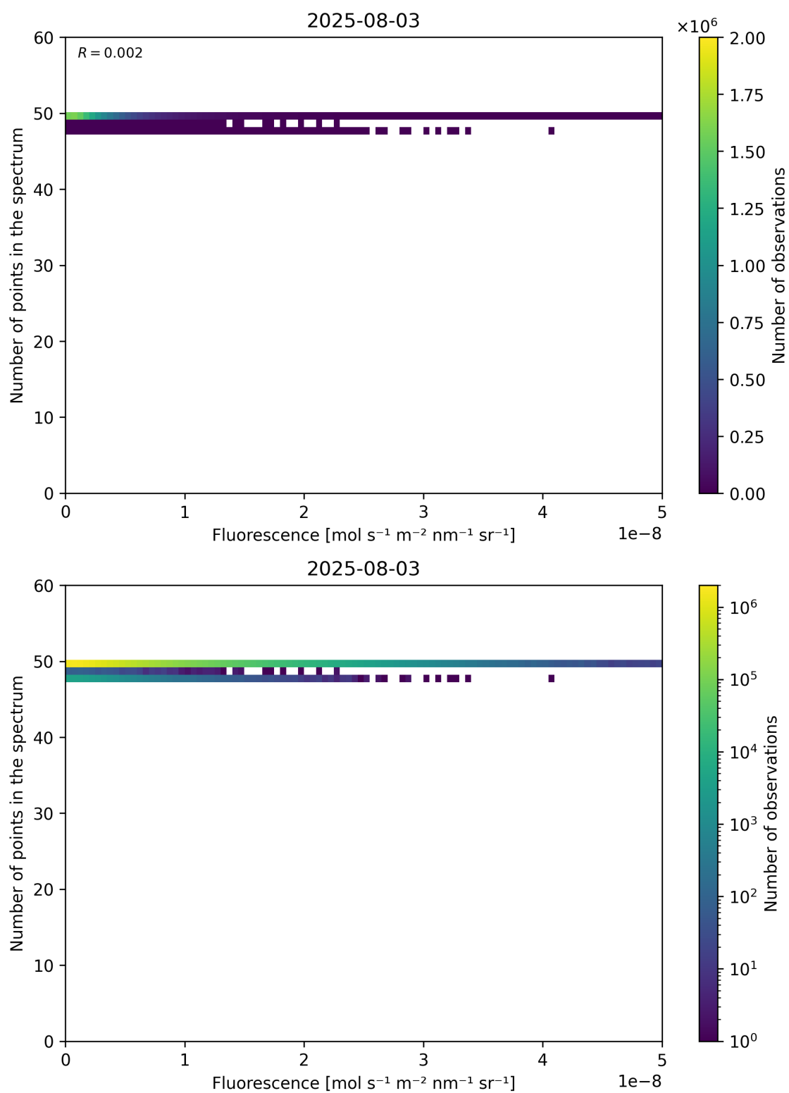
Figure 86: Scatter density plot of “Fluorescence” against “Number of points in the spectrum” for 2025-08-03 to 2025-08-04.
