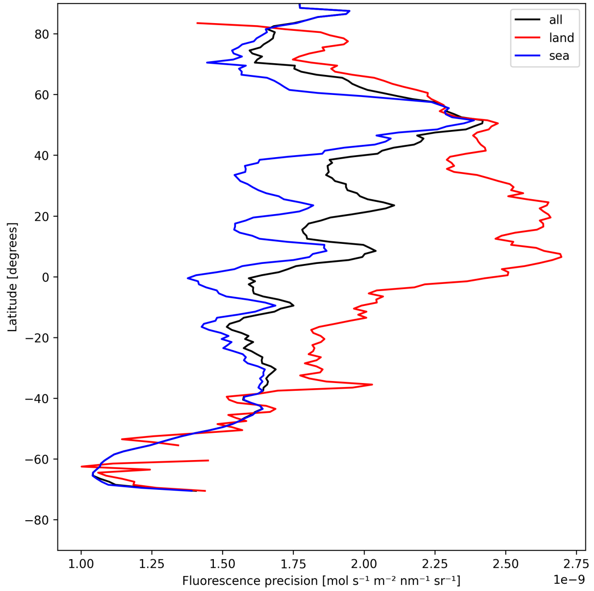
Figure 24: Zonal average of “Fluorescence precision” for 2025-08-03 to 2025-08-04.
