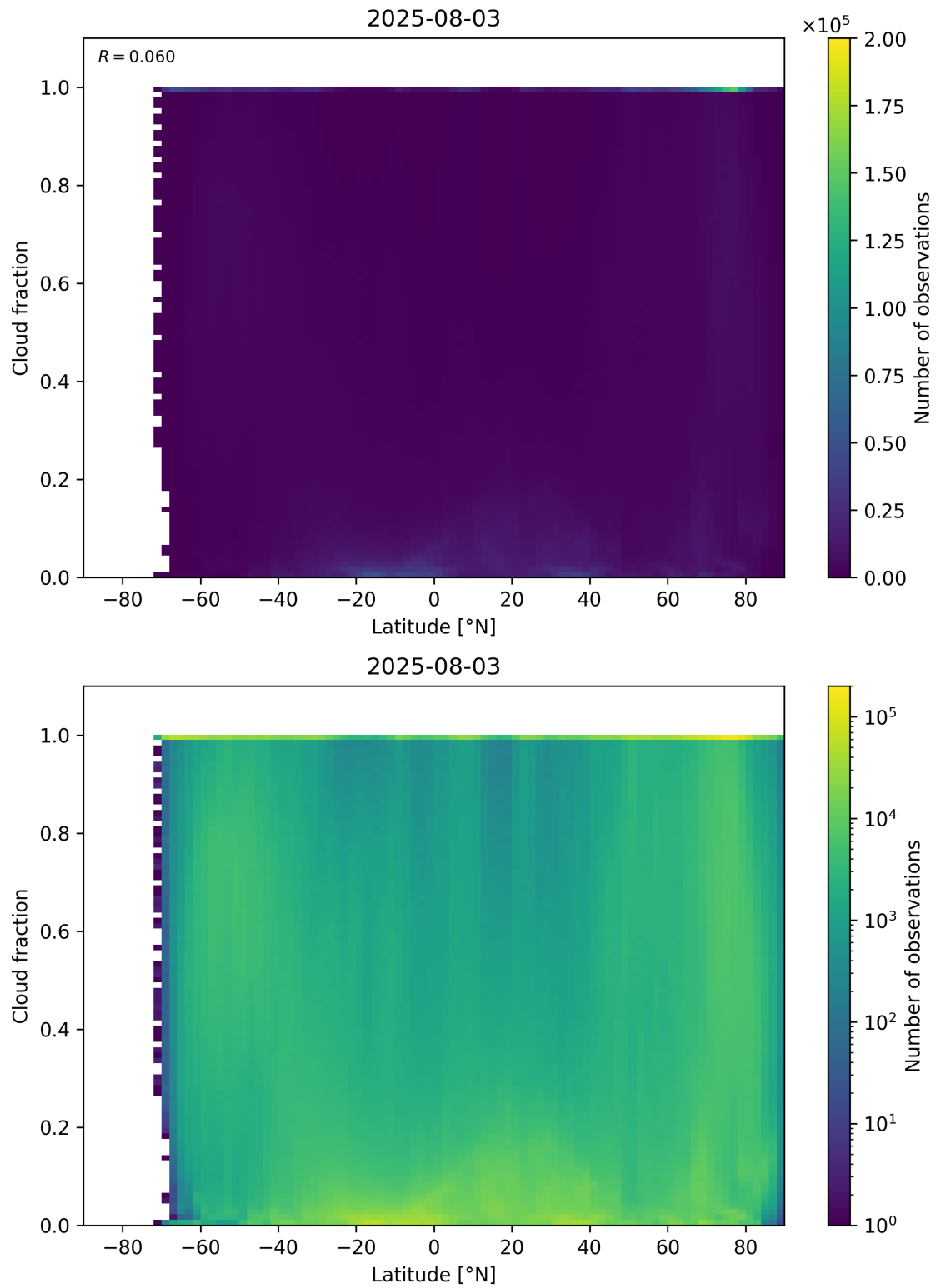
Figure 90: Scatter density plot of “Latitude” against “Cloud fraction” for 2025-08-03 to 2025-08-04.
