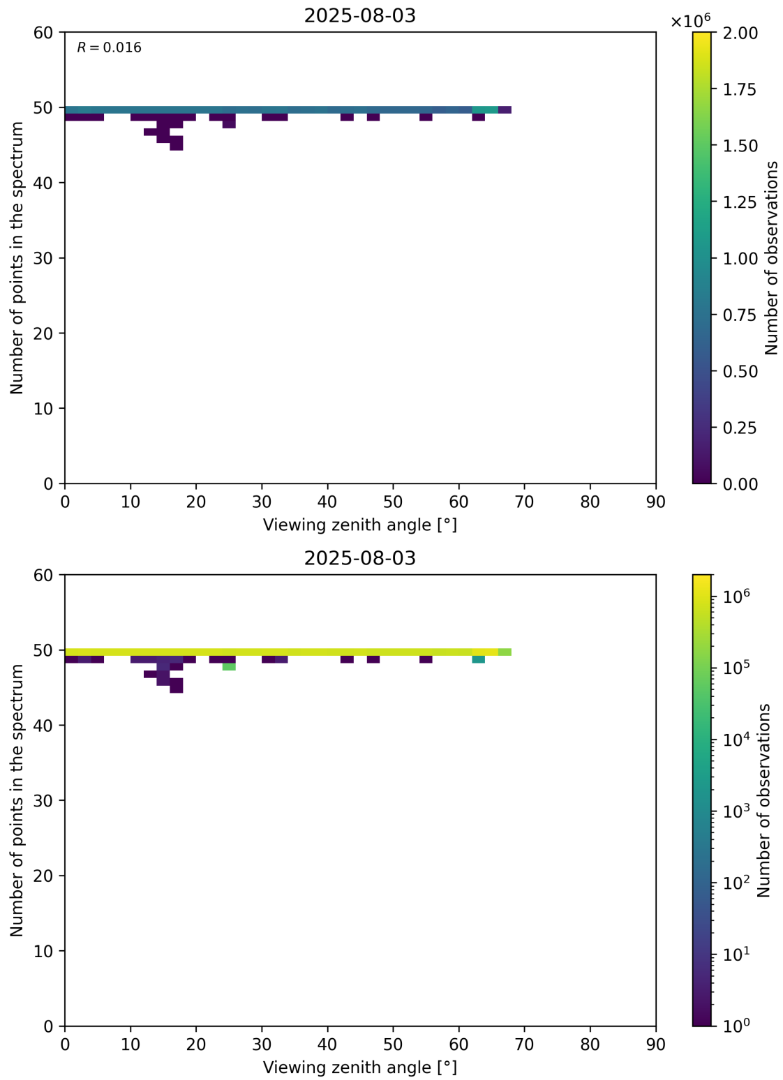
Figure 125: Scatter density plot of “Viewing zenith angle” against “Number of points in the spectrum” for 2025-08-03 to 2025-08-04.
