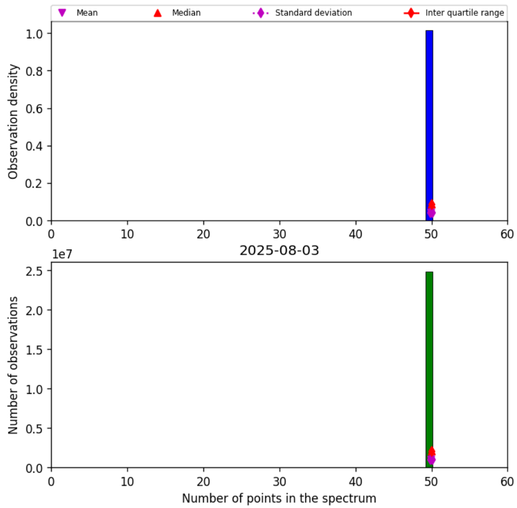
Figure 44: Histogram of “Number of points in the spectrum” for 2025-08-03 to 2025-08-04
