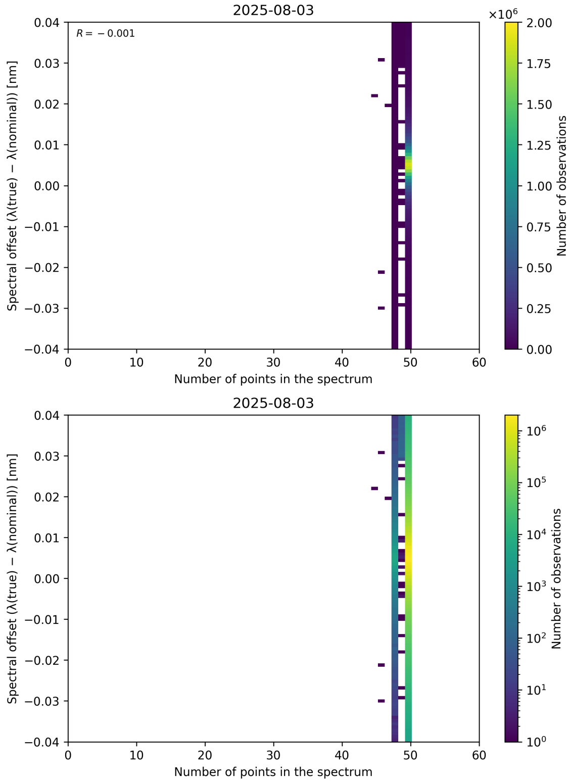
Figure 101: Scatter density plot of “Number of points in the spectrum” against “Spectral offset ( \lambda_{\text{true}} - \lambda_{\text{nominal}} )” for 2025-08-03 to 2025-08-04.
