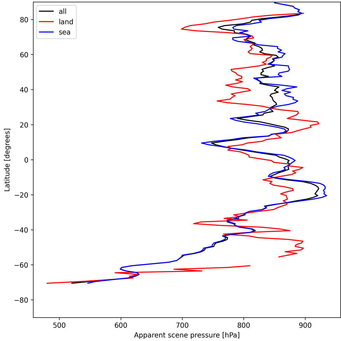
Figure 19: Zonal average of “Apparent scene pressure” for 2025-08-03 to 2025-08-04.
