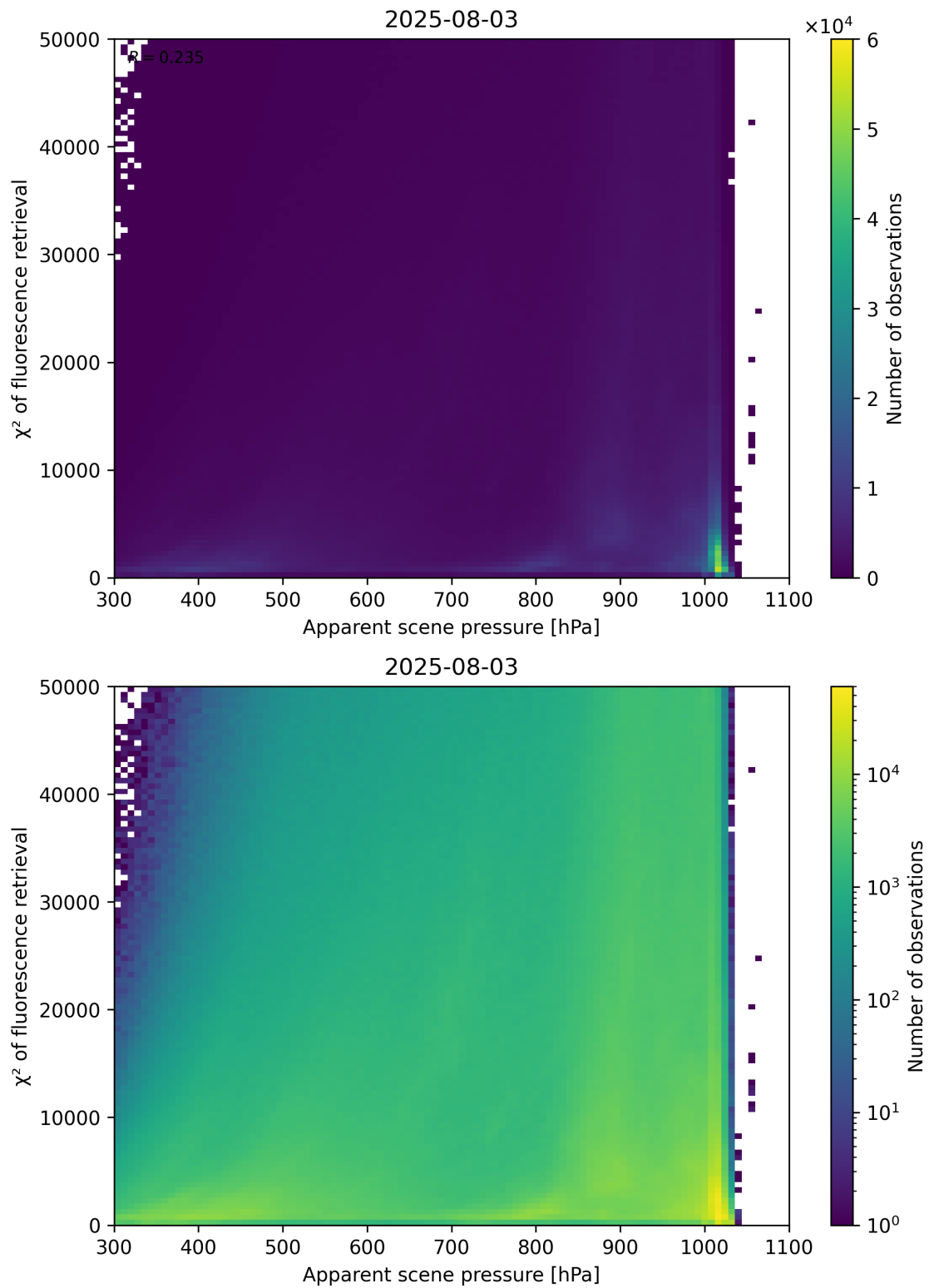
Figure 63: Scatter density plot of “Apparent scene pressure” against “ \chi^2 of fluorescence retrieval” for 2025-08-03 to 2025-08-04.
