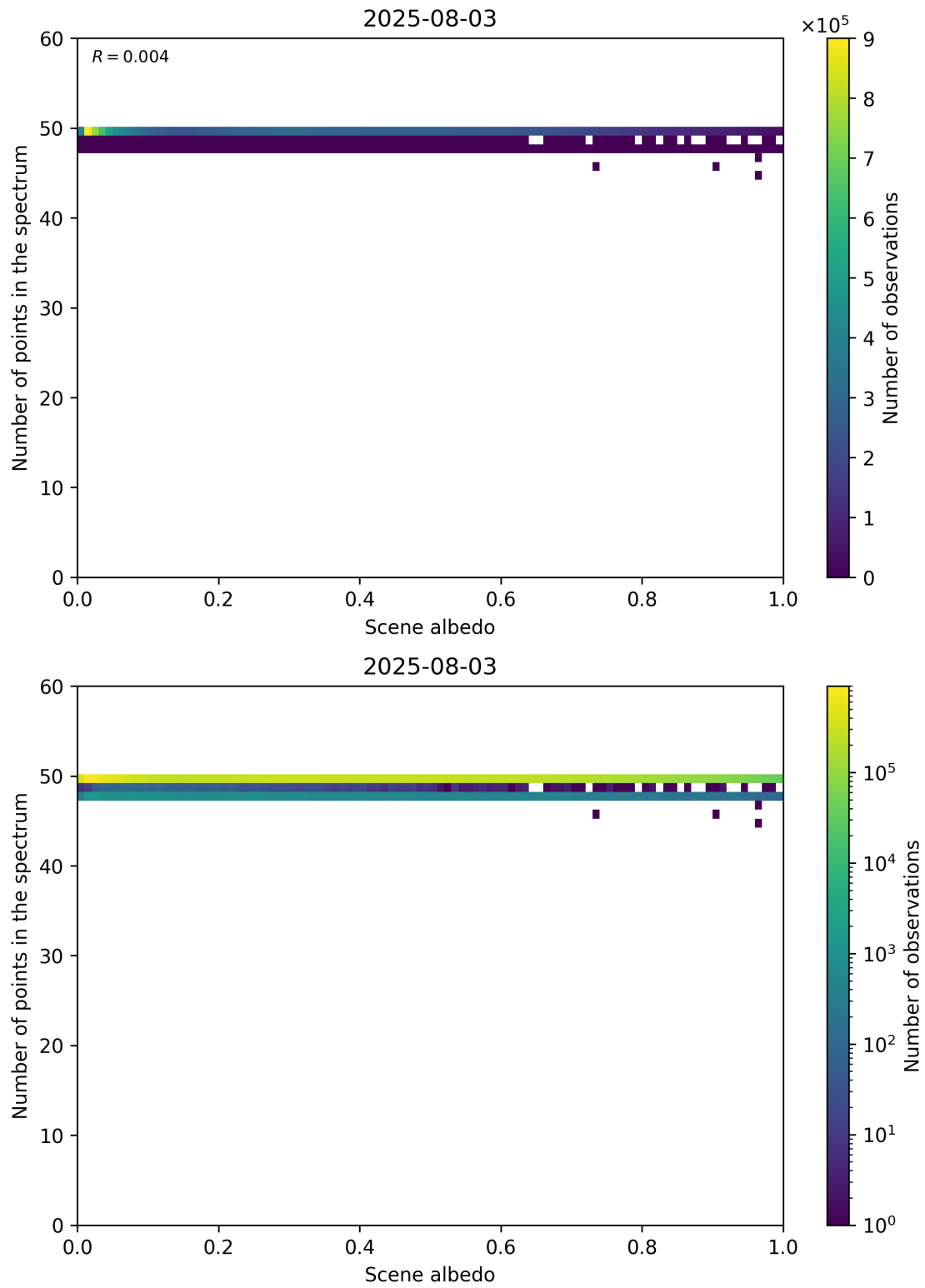
Figure 106: Scatter density plot of “Scene albedo” against “Number of points in the spectrum” for 2025-08-03 to 2025-08-04.
