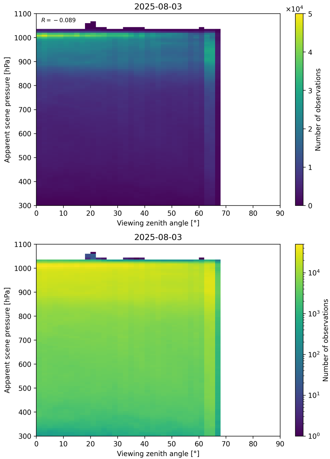
Figure 118: Scatter density plot of “Viewing zenith angle” against “Apparent scene pressure” for 2025-08-03 to 2025-08-04.
