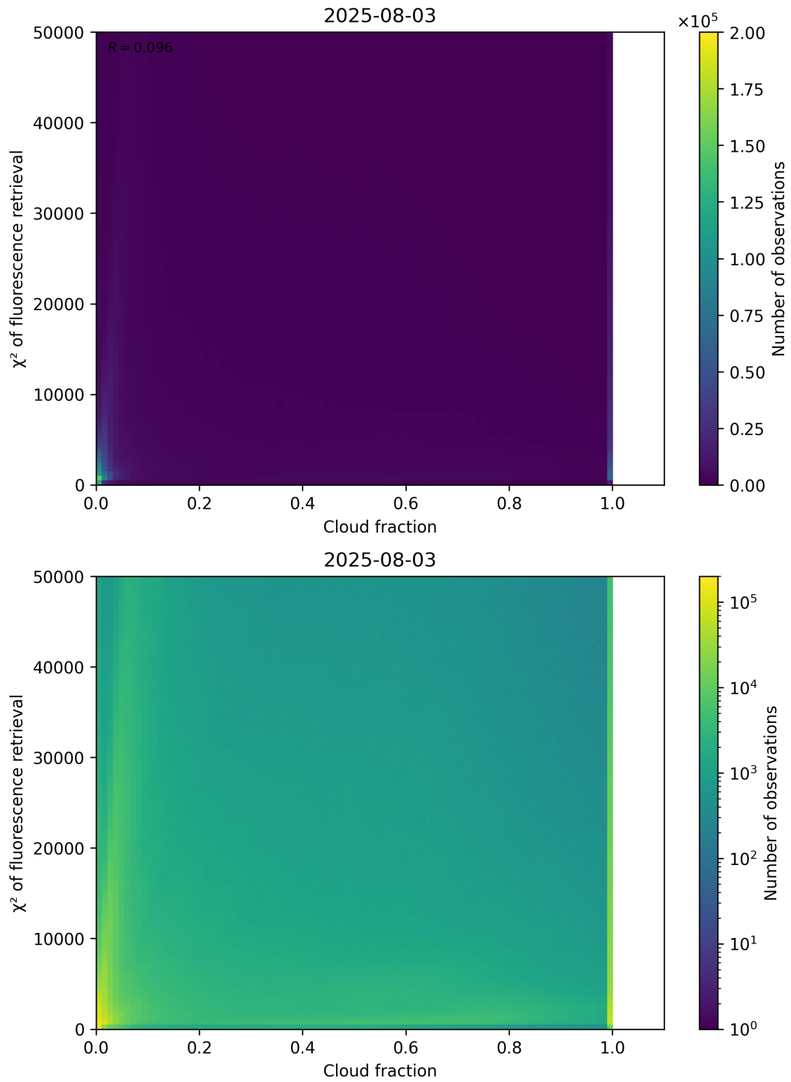
Figure 71: Scatter density plot of “Cloud fraction” against “ \chi^2 of fluorescence retrieval” for 2025-08-03 to 2025-08-04.
