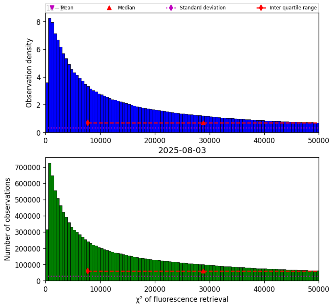
Figure 42: Histogram of “ \chi^2 of fluorescence retrieval” for 2025-08-03 to 2025-08-04
