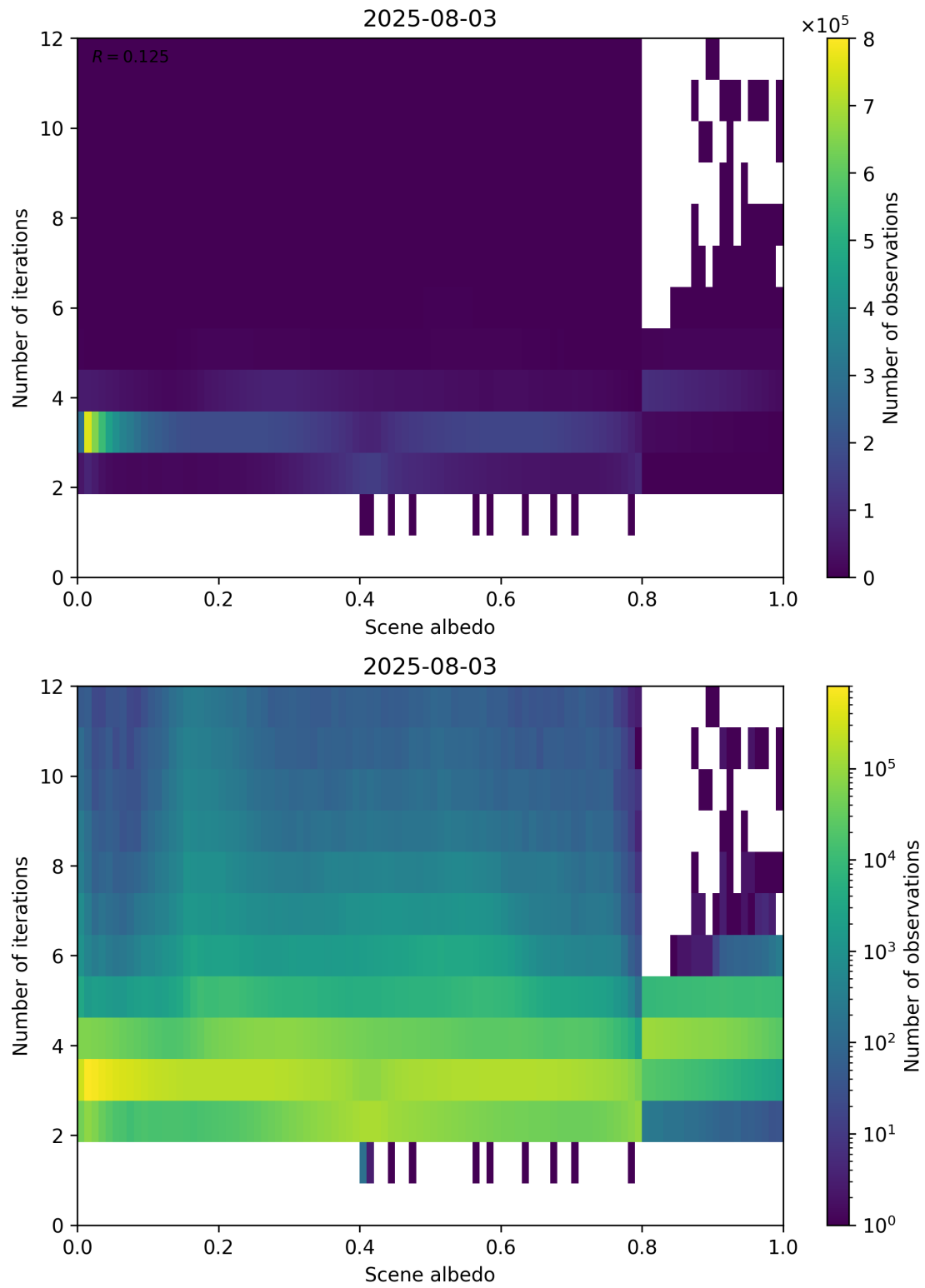
Figure 105: Scatter density plot of “Scene albedo” against “Number of iterations” for 2025-08-03 to 2025-08-04.
