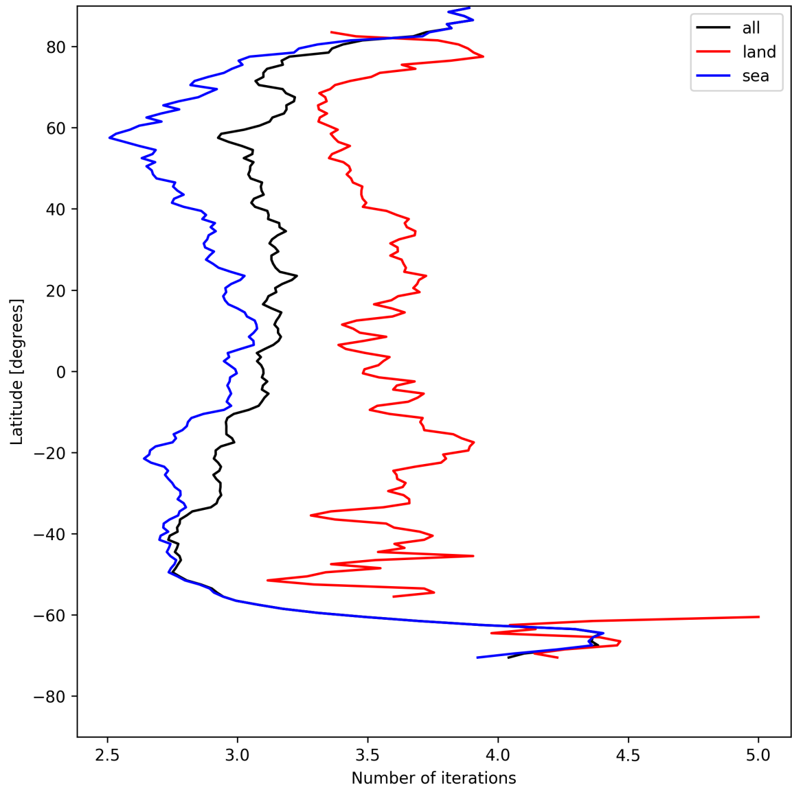
Figure 22: Zonal average of “Number of iterations” for 2025-08-03 to 2025-08-04.
