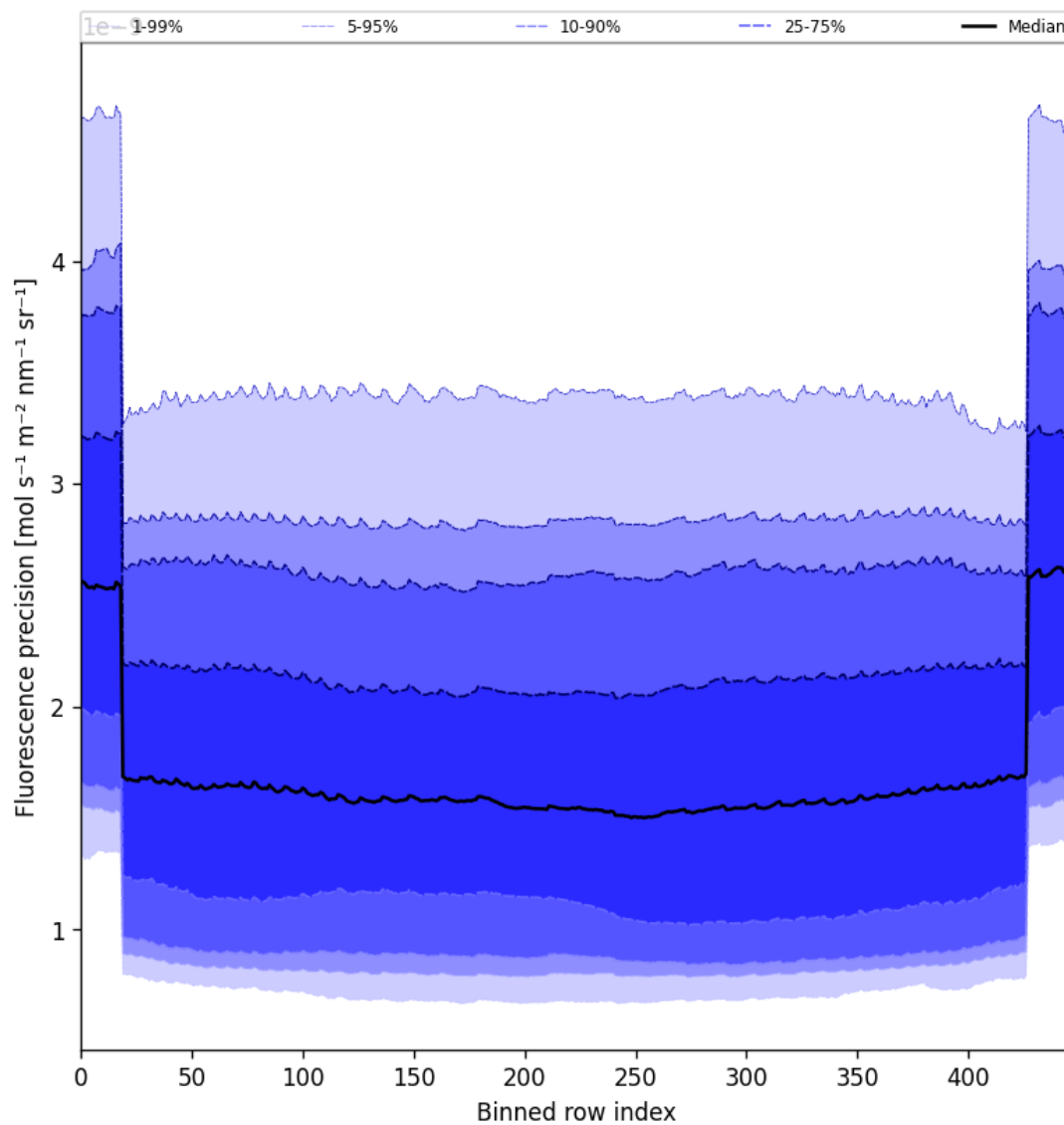
Figure 58: Along track statistics of “Fluorescence precision” for 2025-08-03 to 2025-08-04
