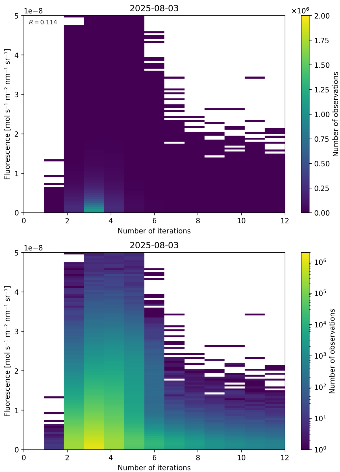
Figure 98: Scatter density plot of “Number of iterations” against “Fluorescence” for 2025-08-03 to 2025-08-04.
