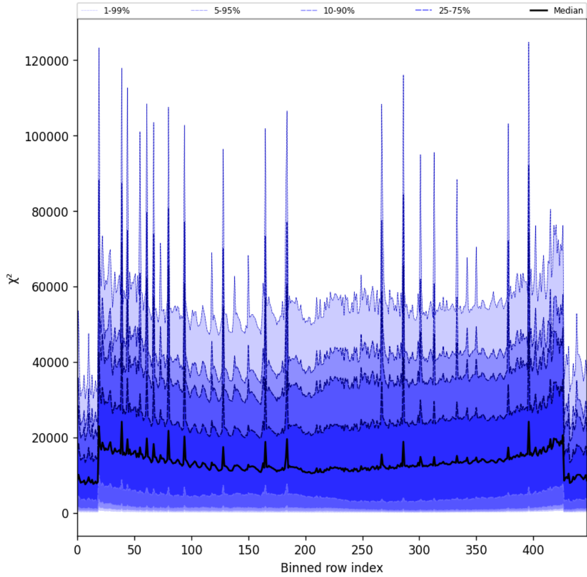
Figure 55: Along track statistics of “ \chi^2 ” for 2025-08-03 to 2025-08-04
