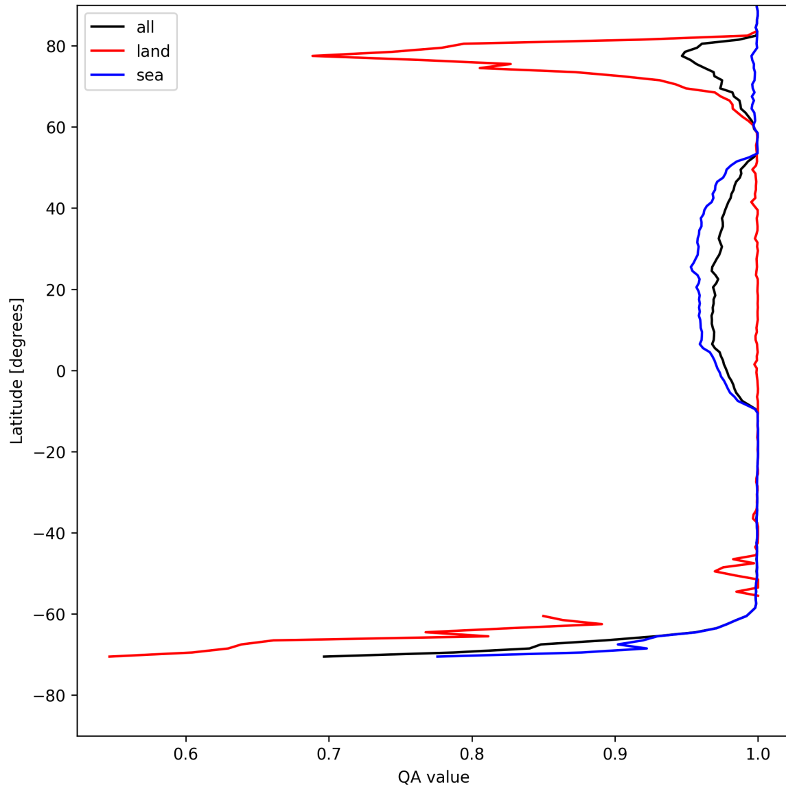
Figure 12: Zonal average of “QA value” for 2025-08-03 to 2025-08-04.
