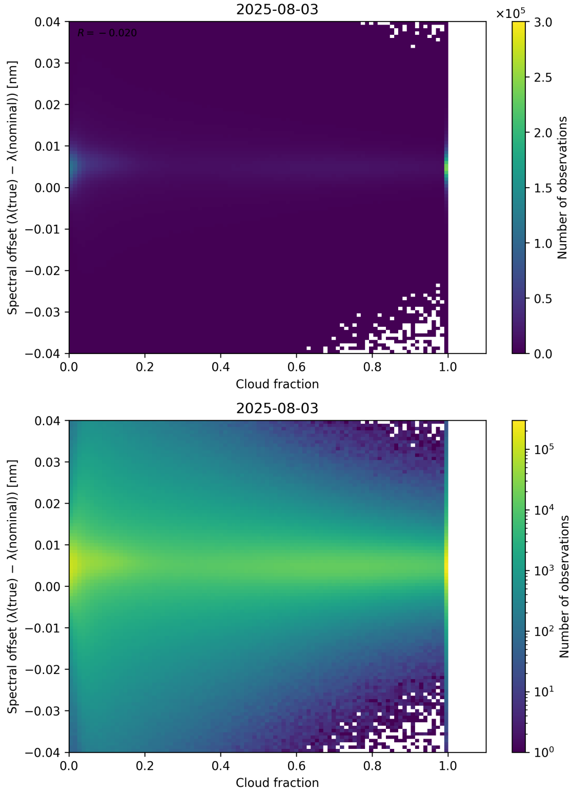
Figure 76: Scatter density plot of “Cloud fraction” against “Spectral offset ( \lambda_{\text{true}} - \lambda_{\text{nominal}} )” for 2025-08-03 to 2025-08-04.
