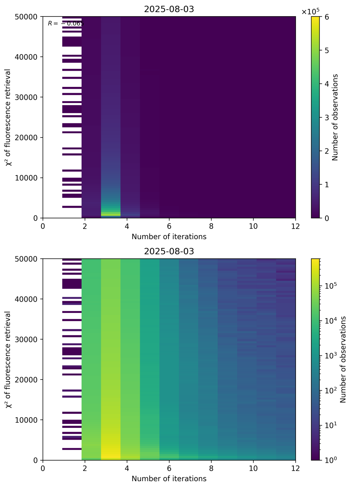
Figure 97: Scatter density plot of “Number of iterations” against “ \chi^2 of fluorescence retrieval” for 2025-08-03 to 2025-08-04.
