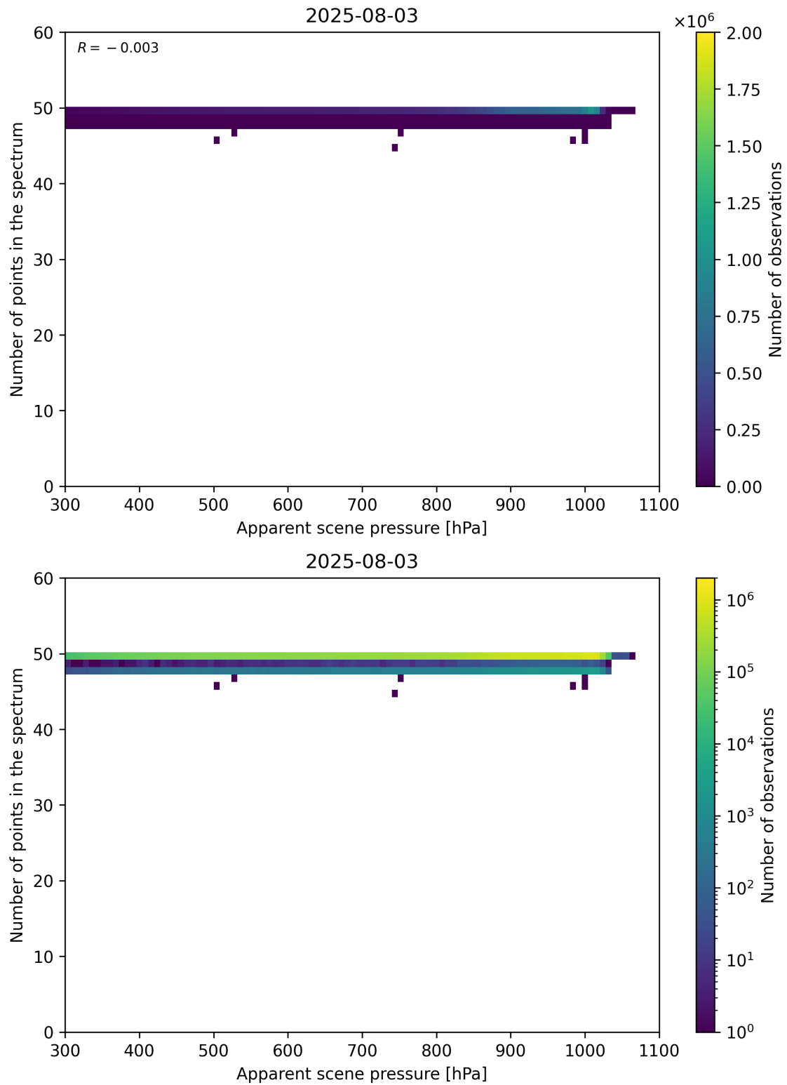
Figure 66: Scatter density plot of “Apparent scene pressure” against “Number of points in the spectrum” for 2025-08-03 to 2025-08-04.
