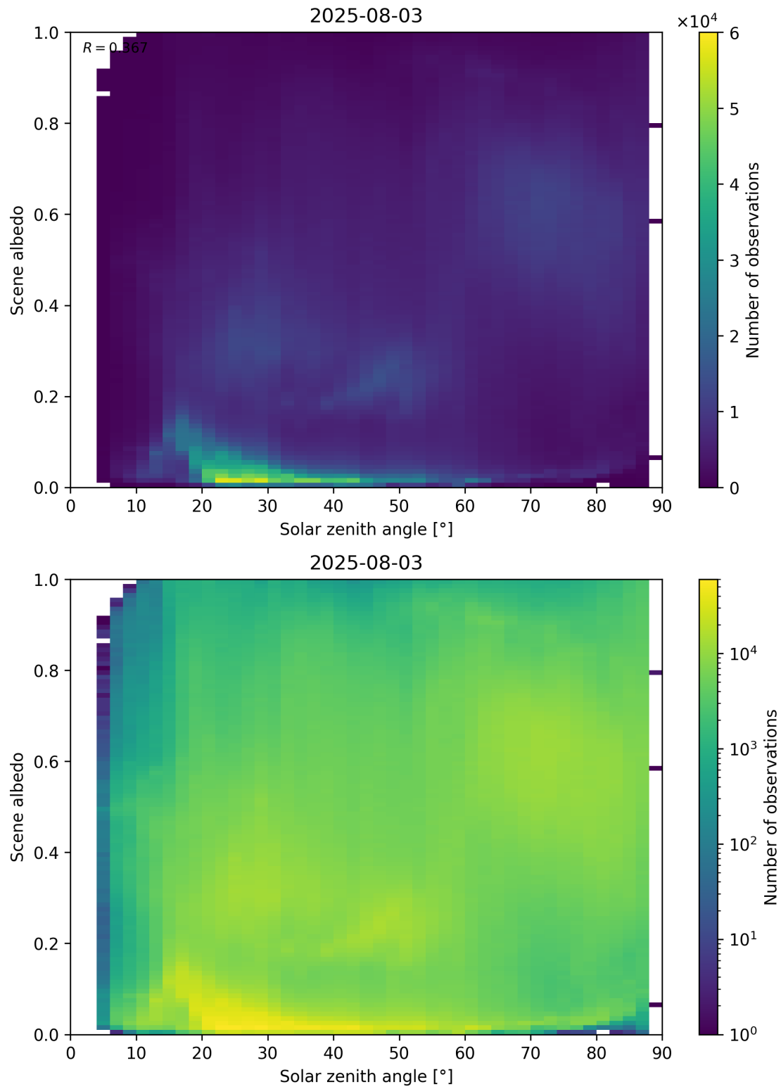
Figure 116: Scatter density plot of “Solar zenith angle” against “Scene albedo” for 2025-08-03 to 2025-08-04.
