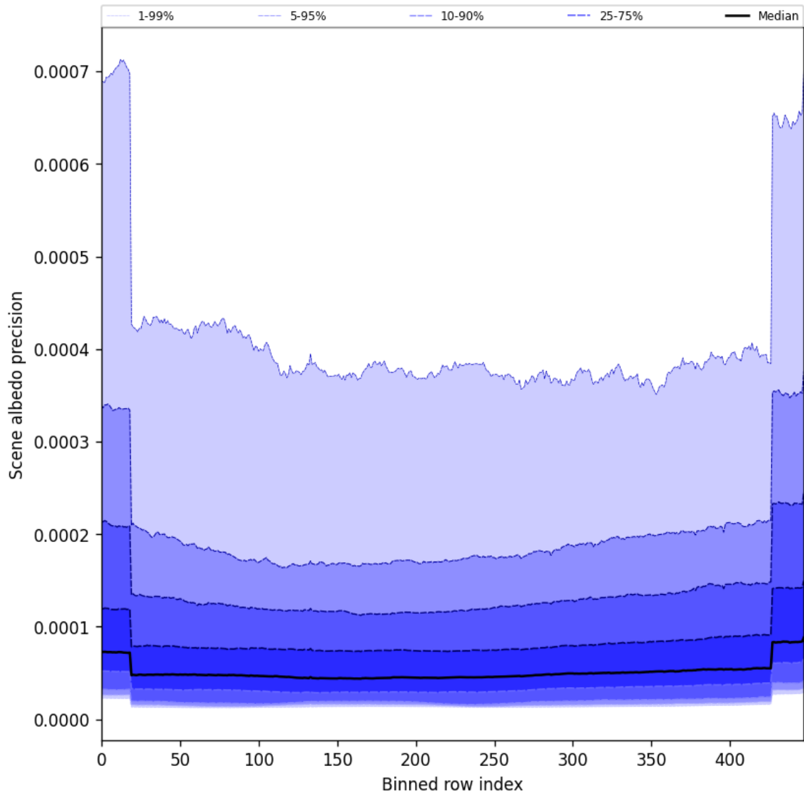
Figure 52: Along track statistics of “Scene albedo precision” for 2025-08-03 to 2025-08-04
