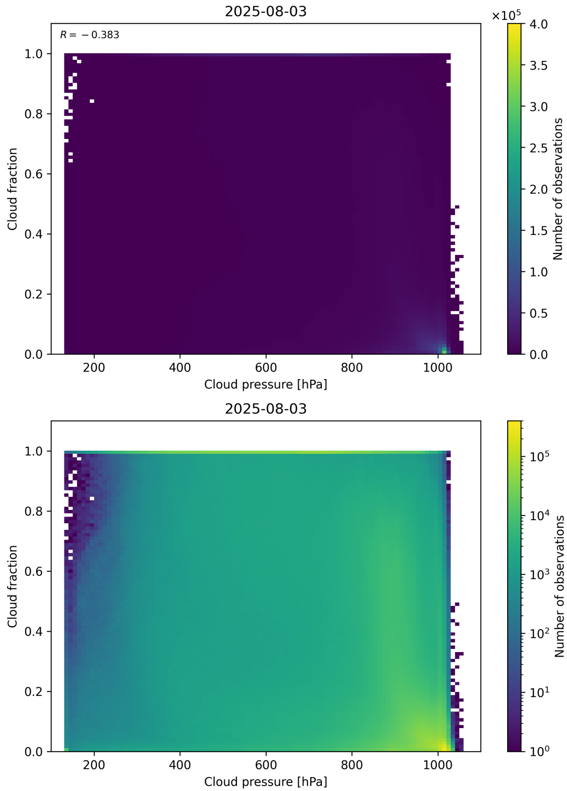
Figure 79: Scatter density plot of “Cloud pressure” against “Cloud fraction” for 2025-08-03 to 2025-08-04.
