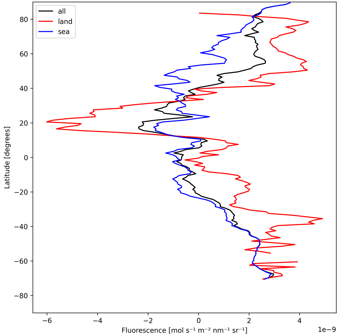
Figure 23: Zonal average of “Fluorescence” for 2025-08-03 to 2025-08-04.
