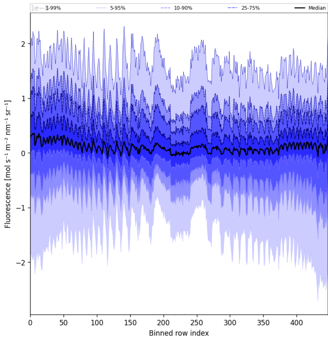
Figure 57: Along track statistics of “Fluorescence” for 2025-08-03 to 2025-08-04
