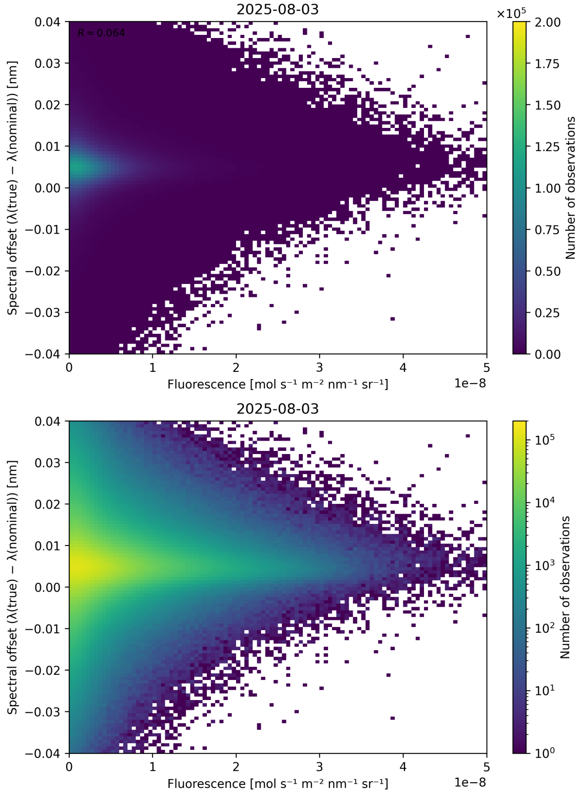
Figure 87: Scatter density plot of “Fluorescence” against “Spectral offset ( \lambda_{\text{true}} - \lambda_{\text{nominal}} )” for 2025-08-03 to 2025-08-04.
