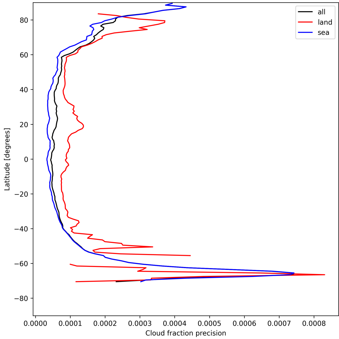
Figure 16: Zonal average of “Cloud fraction precision” for 2025-08-03 to 2025-08-04.
