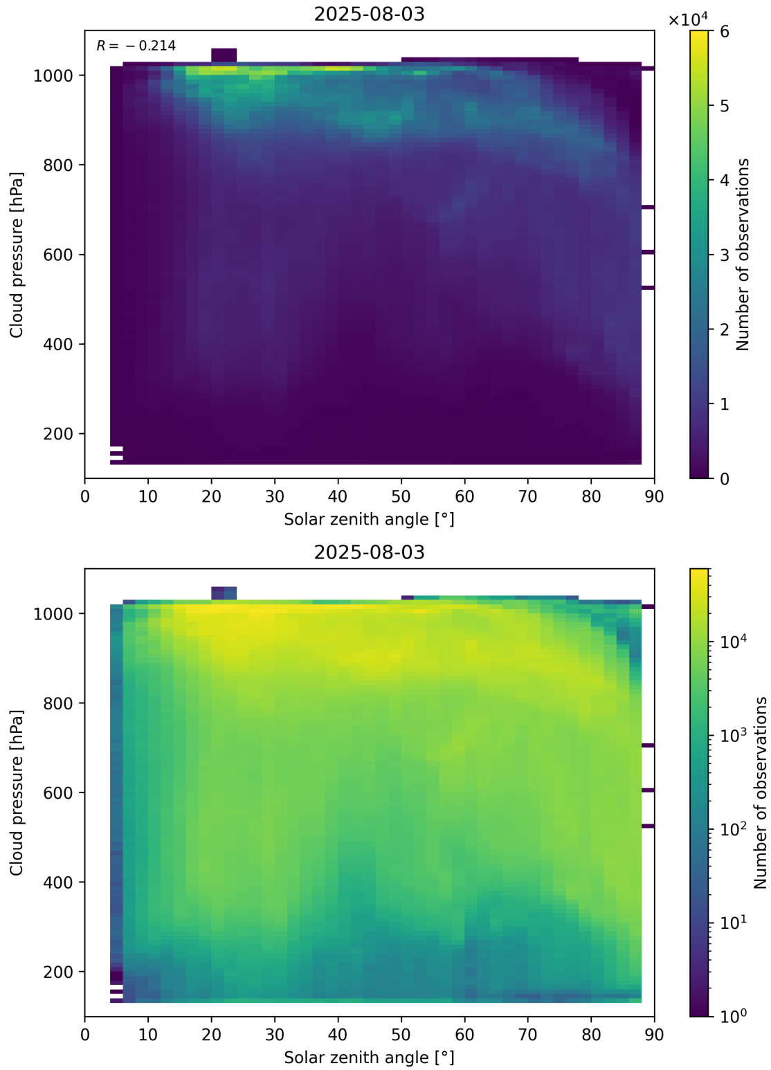
Figure 111: Scatter density plot of “Solar zenith angle” against “Cloud pressure” for 2025-08-03 to 2025-08-04.
