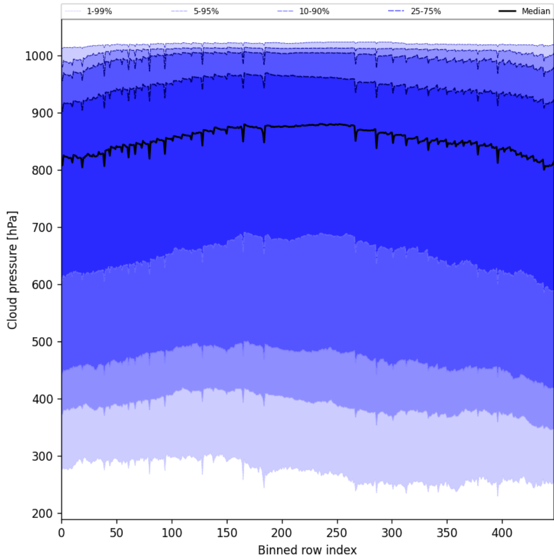
Figure 47: Along track statistics of “Cloud pressure” for 2025-08-03 to 2025-08-04
