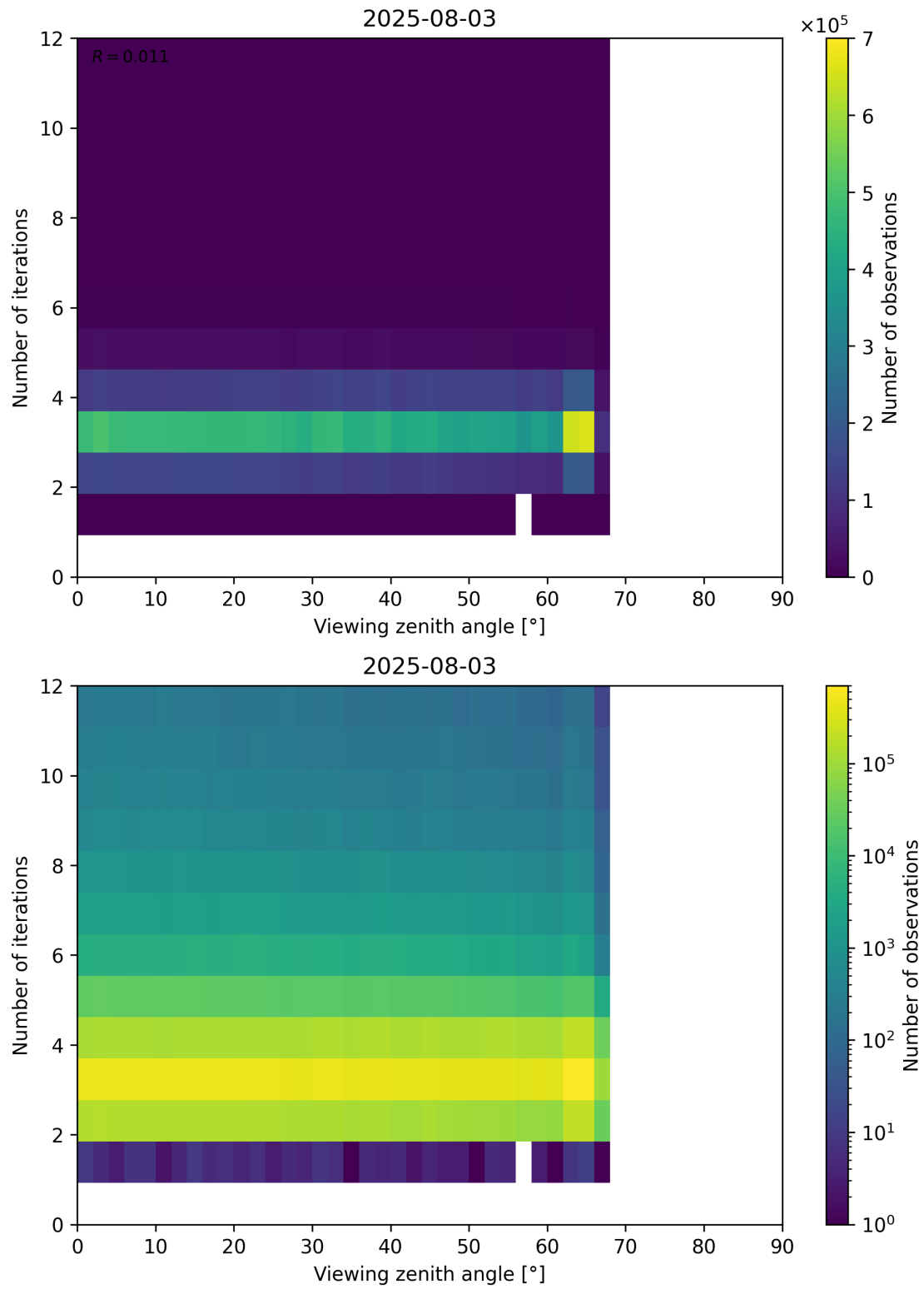
Figure 124: Scatter density plot of “Viewing zenith angle” against “Number of iterations” for 2025-08-03 to 2025-08-04.
