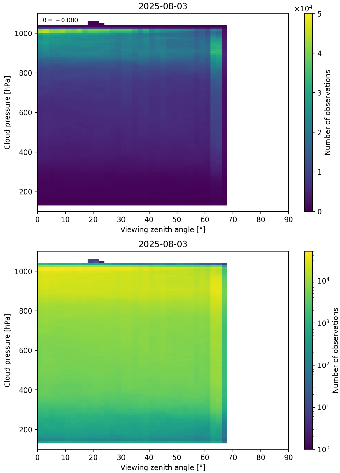
Figure 121: Scatter density plot of “Viewing zenith angle” against “Cloud pressure” for 2025-08-03 to 2025-08-04.
