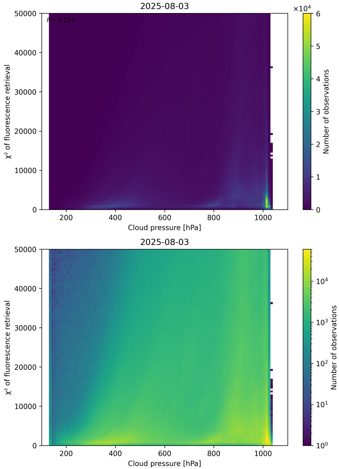
Figure 78: Scatter density plot of “Cloud pressure” against “ \chi^2 of fluorescence retrieval” for 2025-08-03 to 2025-08-04.
