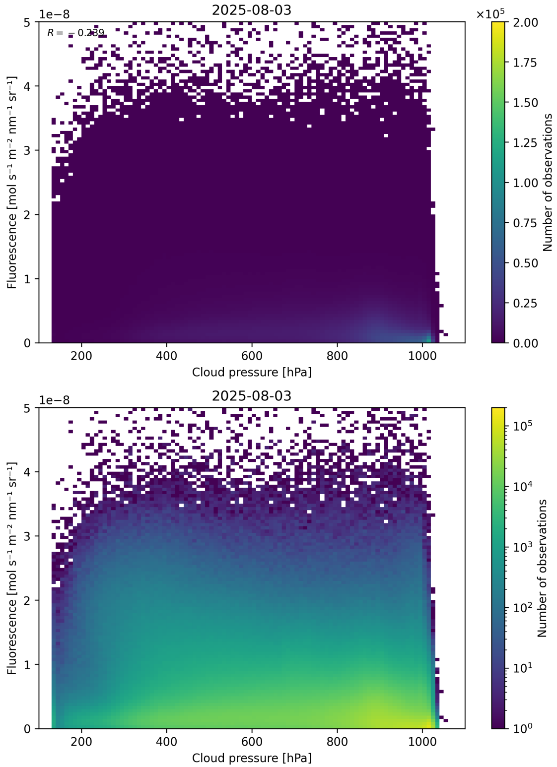
Figure 80: Scatter density plot of “Cloud pressure” against “Fluorescence” for 2025-08-03 to 2025-08-04.
