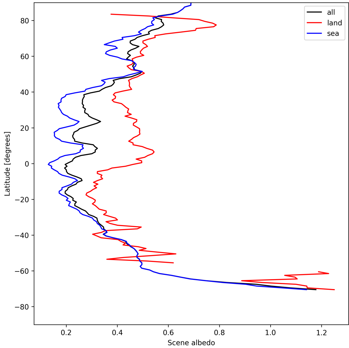
Figure 17: Zonal average of “Scene albedo” for 2025-08-03 to 2025-08-04.
