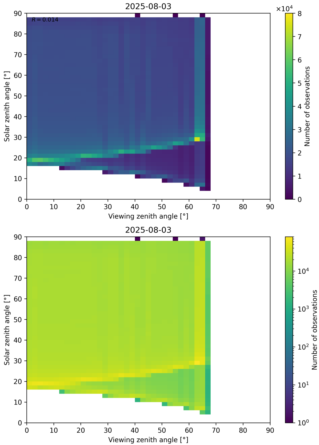
Figure 127: Scatter density plot of “Viewing zenith angle” against “Solar zenith angle” for 2025-08-03 to 2025-08-04.
