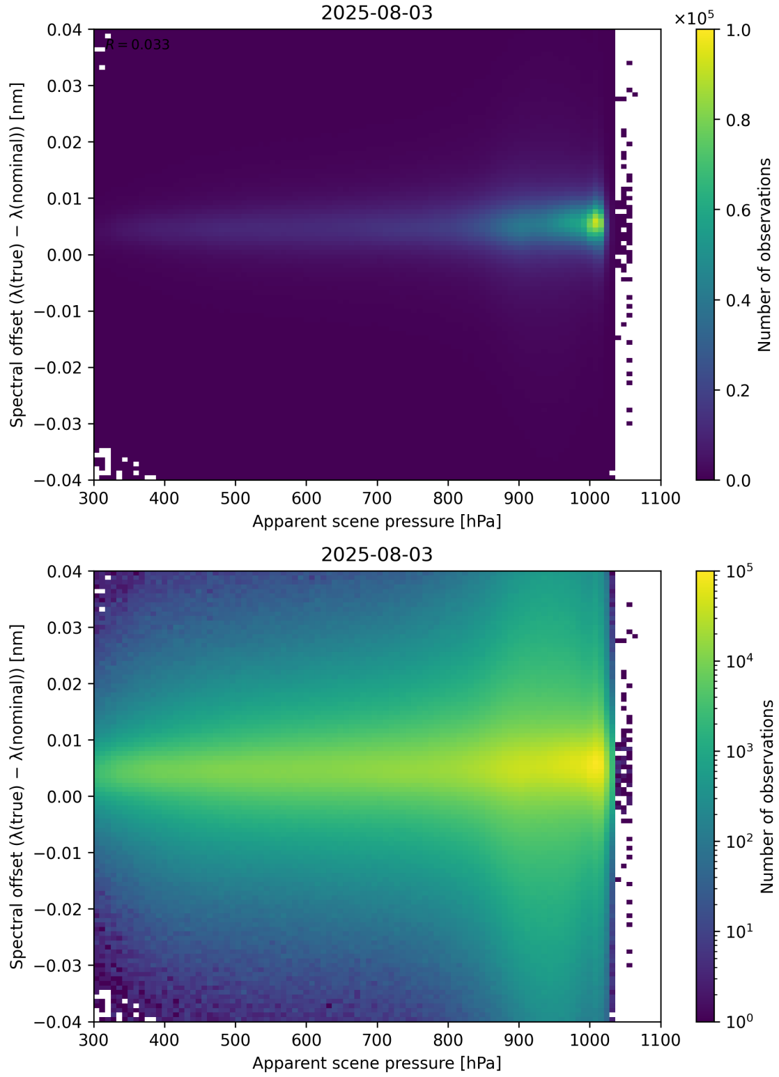
Figure 67: Scatter density plot of “Apparent scene pressure” against “Spectral offset ( \lambda_{\text{true}} - \lambda_{\text{nominal}} )” for 2025-08-03 to 2025-08-04.
