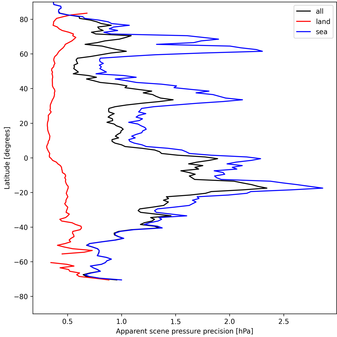
Figure 20: Zonal average of “Apparent scene pressure precision” for 2025-08-03 to 2025-08-04.
