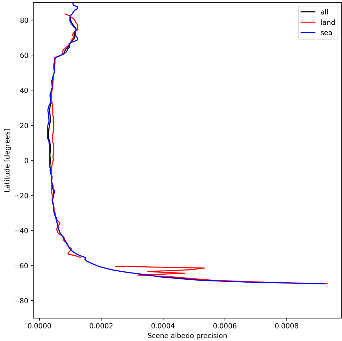
Figure 18: Zonal average of “Scene albedo precision” for 2025-08-03 to 2025-08-04.
