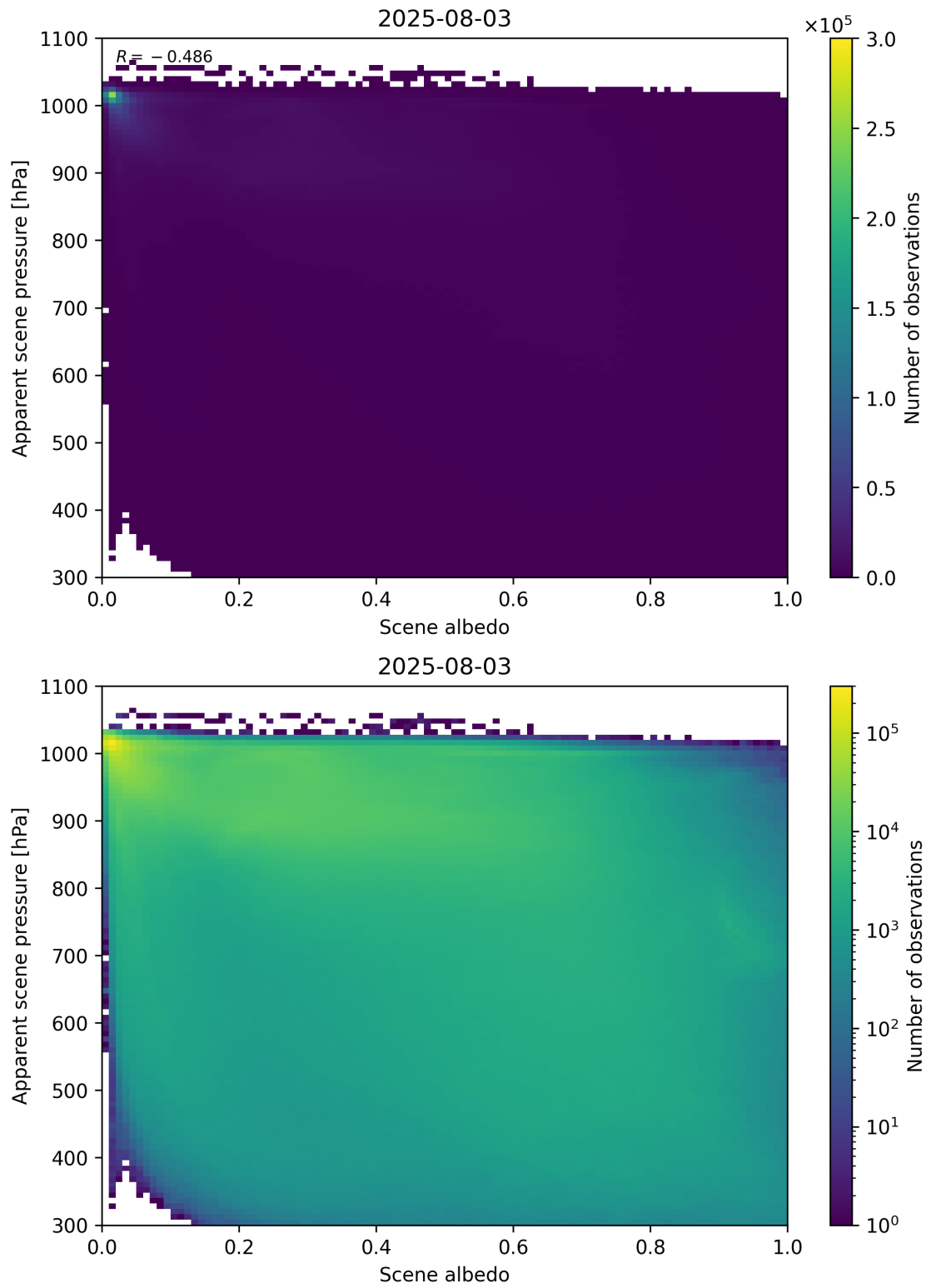
Figure 102: Scatter density plot of “Scene albedo” against “Apparent scene pressure” for 2025-08-03 to 2025-08-04.
