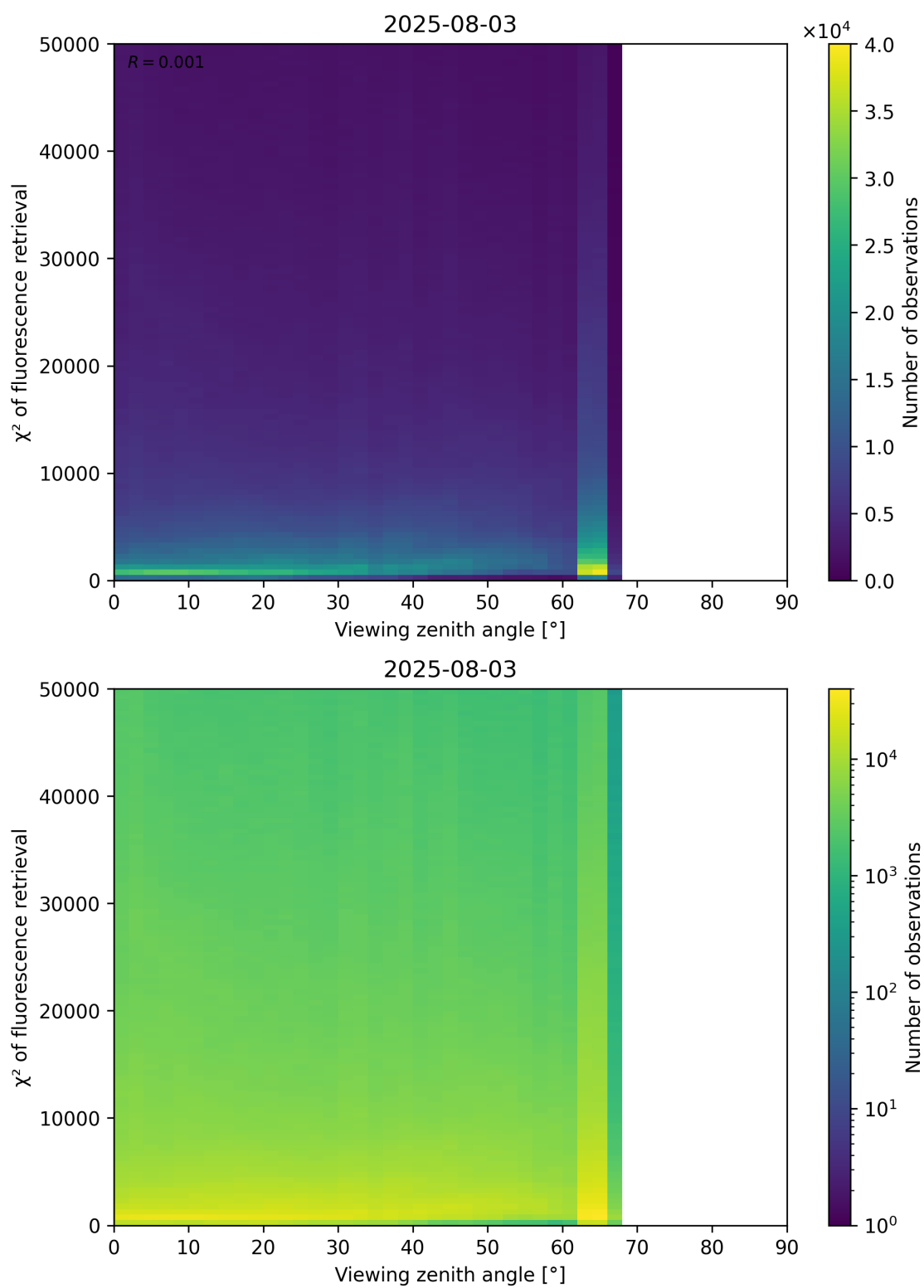
Figure 119: Scatter density plot of “Viewing zenith angle” against “ \chi^2 of fluorescence retrieval” for 2025-08-03 to 2025-08-04.
