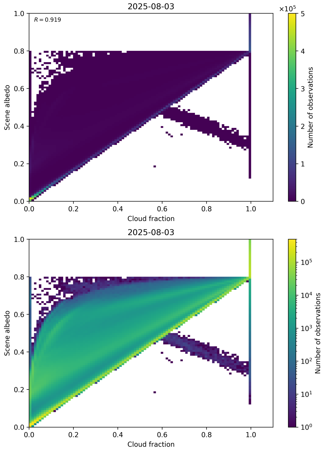
Figure 75: Scatter density plot of “Cloud fraction” against “Scene albedo” for 2025-08-03 to 2025-08-04.
