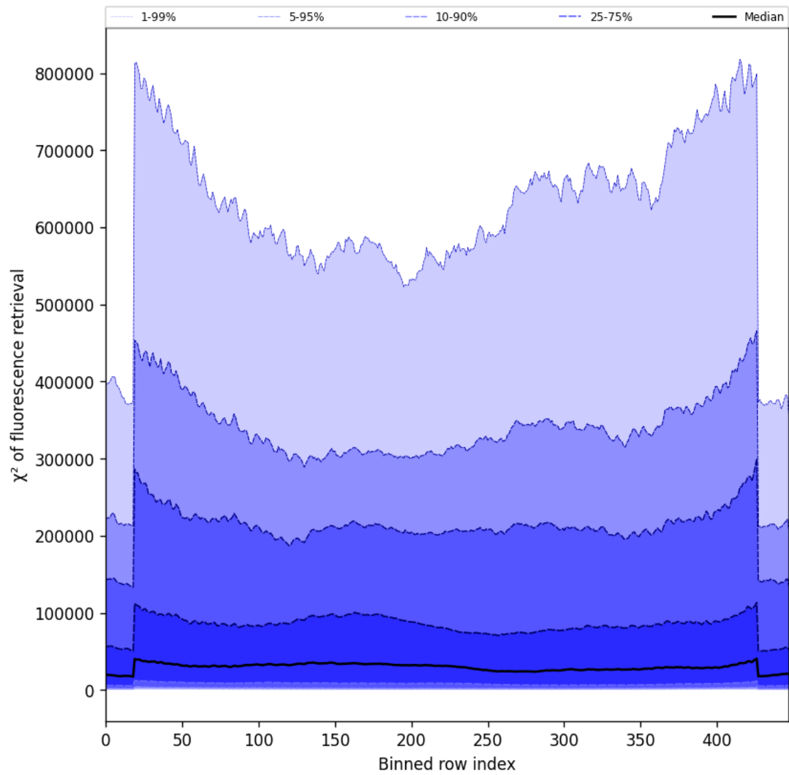
Figure 59: Along track statistics of “ \chi^2 of fluorescence retrieval” for 2025-08-03 to 2025-08-04
