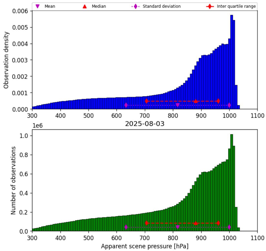
Figure 36: Histogram of “Apparent scene pressure” for 2025-08-03 to 2025-08-04
