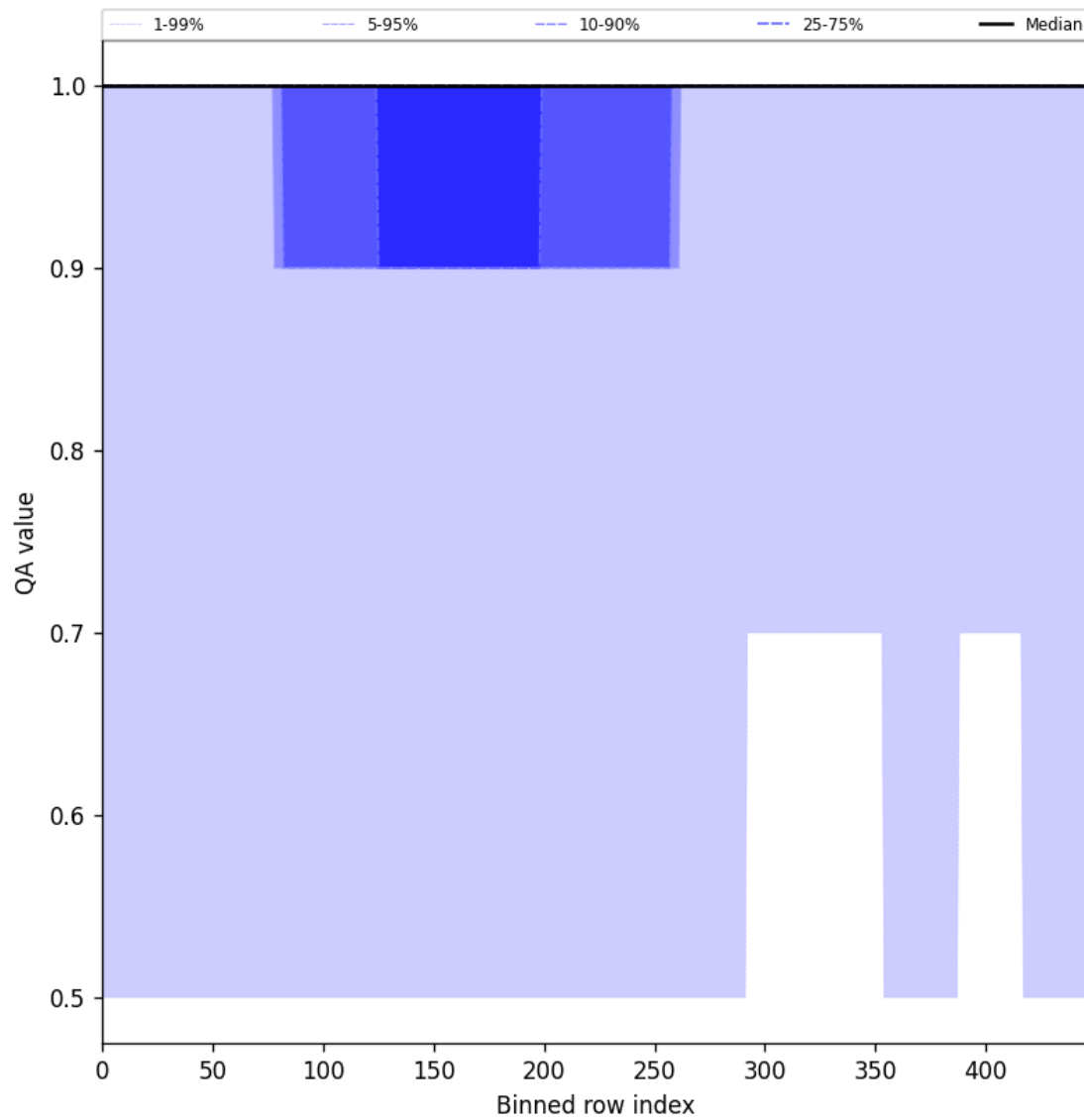
Figure 46: Along track statistics of “QA value” for 2025-08-03 to 2025-08-04
