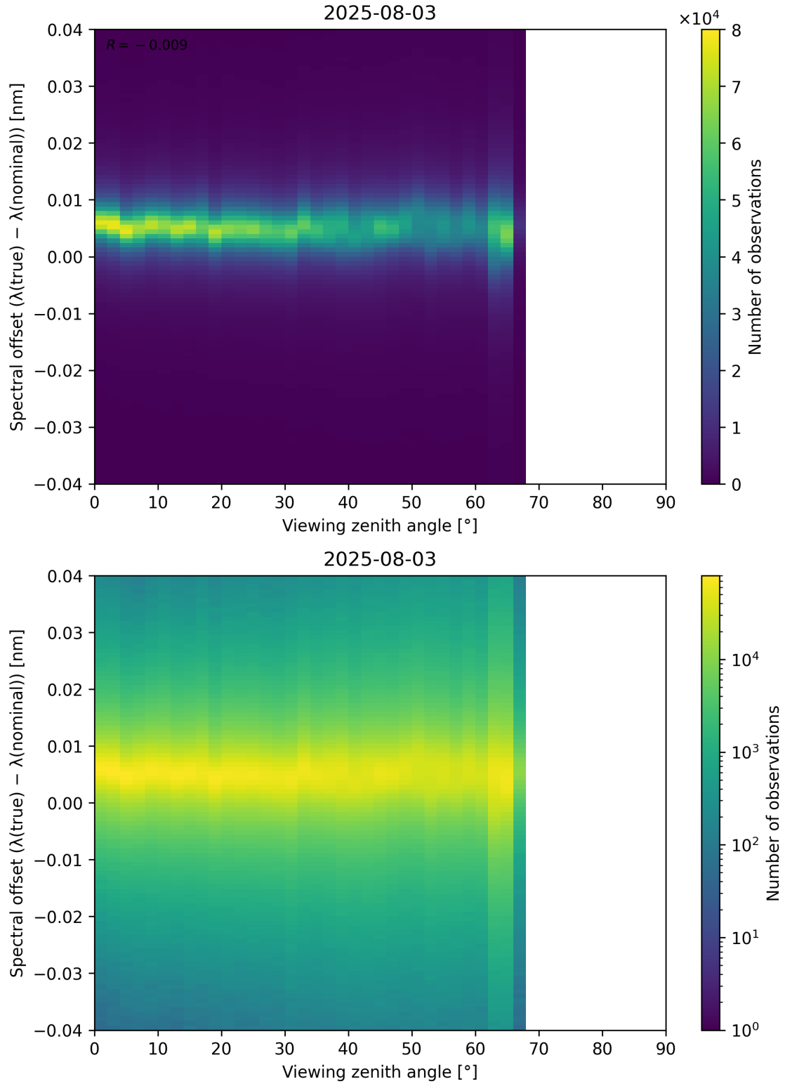
Figure 128: Scatter density plot of “Viewing zenith angle” against “Spectral offset ( \lambda_{\text{true}} - \lambda_{\text{nominal}} )” for 2025-08-03 to 2025-08-04.
