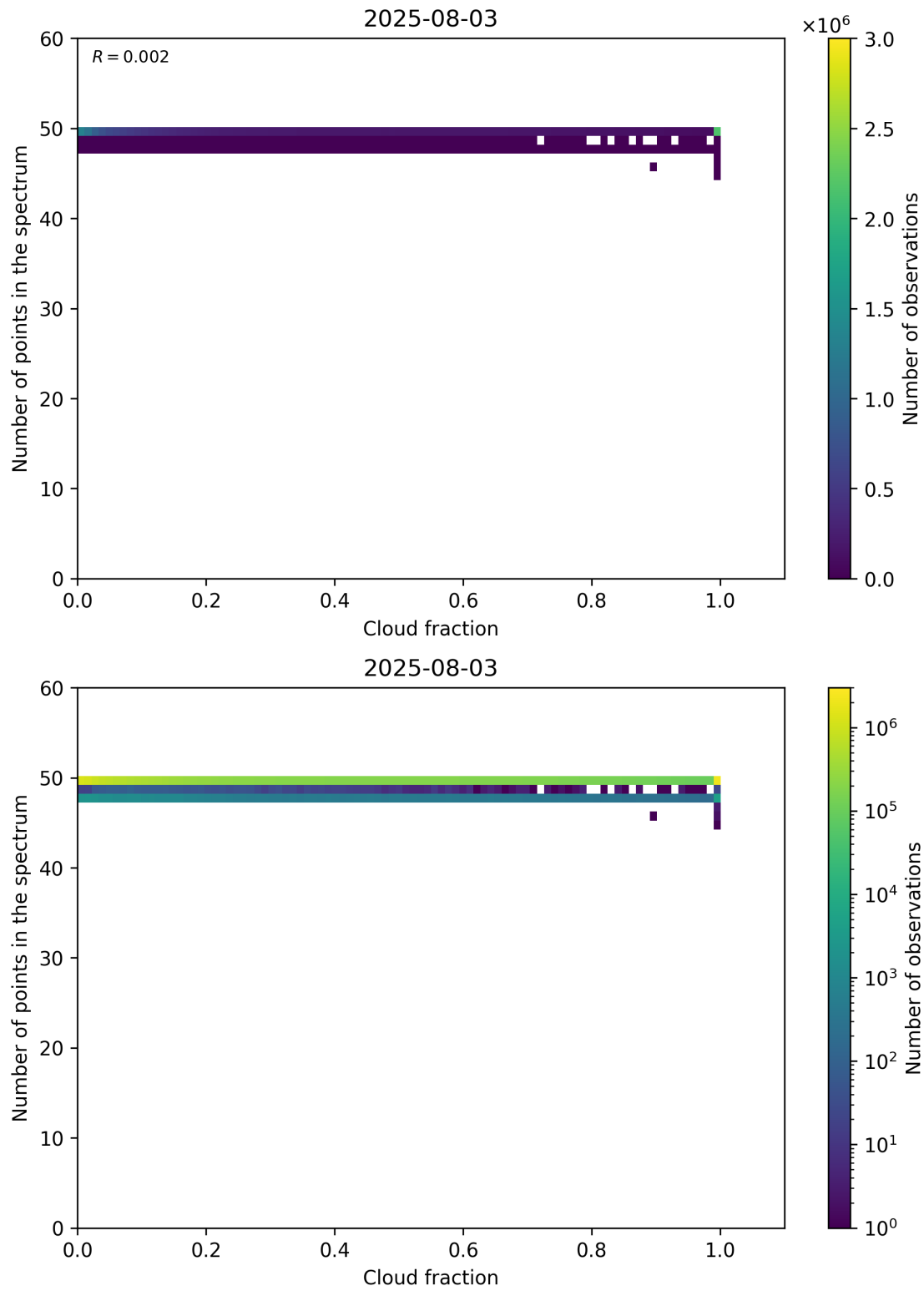
Figure 74: Scatter density plot of “Cloud fraction” against “Number of points in the spectrum” for 2025-08-03 to 2025-08-04.
