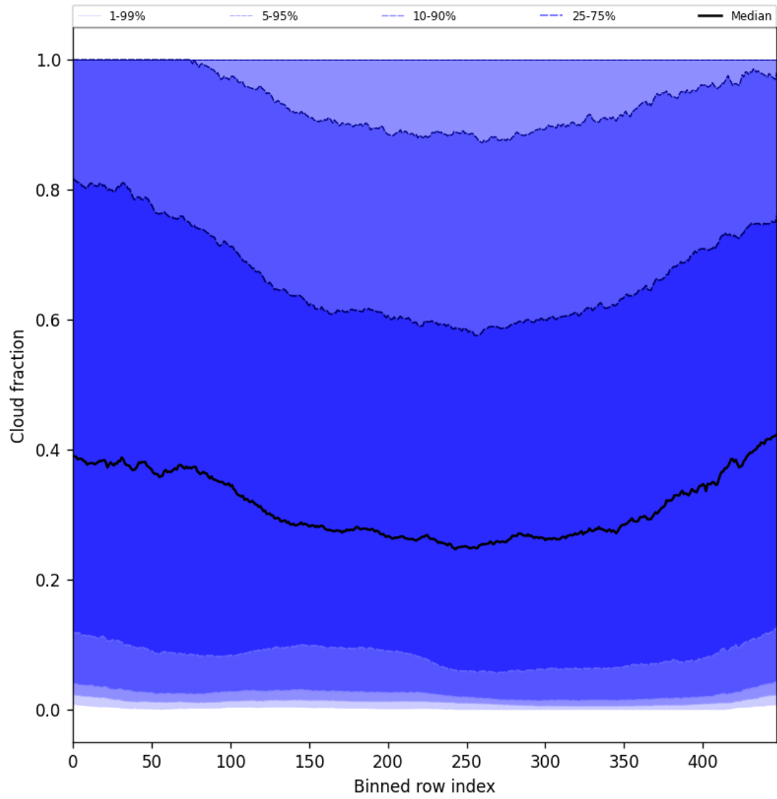
Figure 49: Along track statistics of “Cloud fraction” for 2025-08-03 to 2025-08-04
