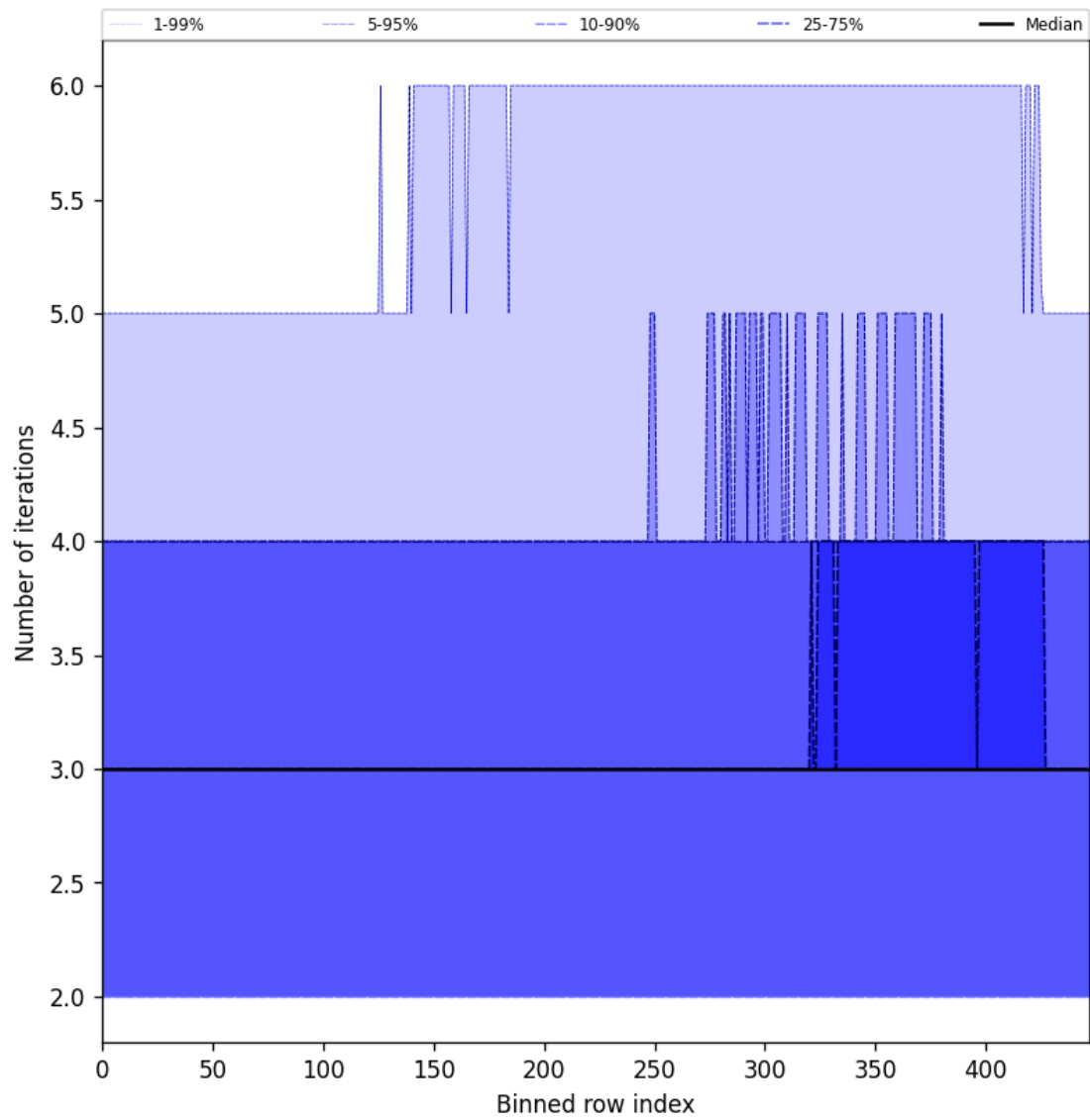
Figure 56: Along track statistics of “Number of iterations” for 2025-08-03 to 2025-08-04
