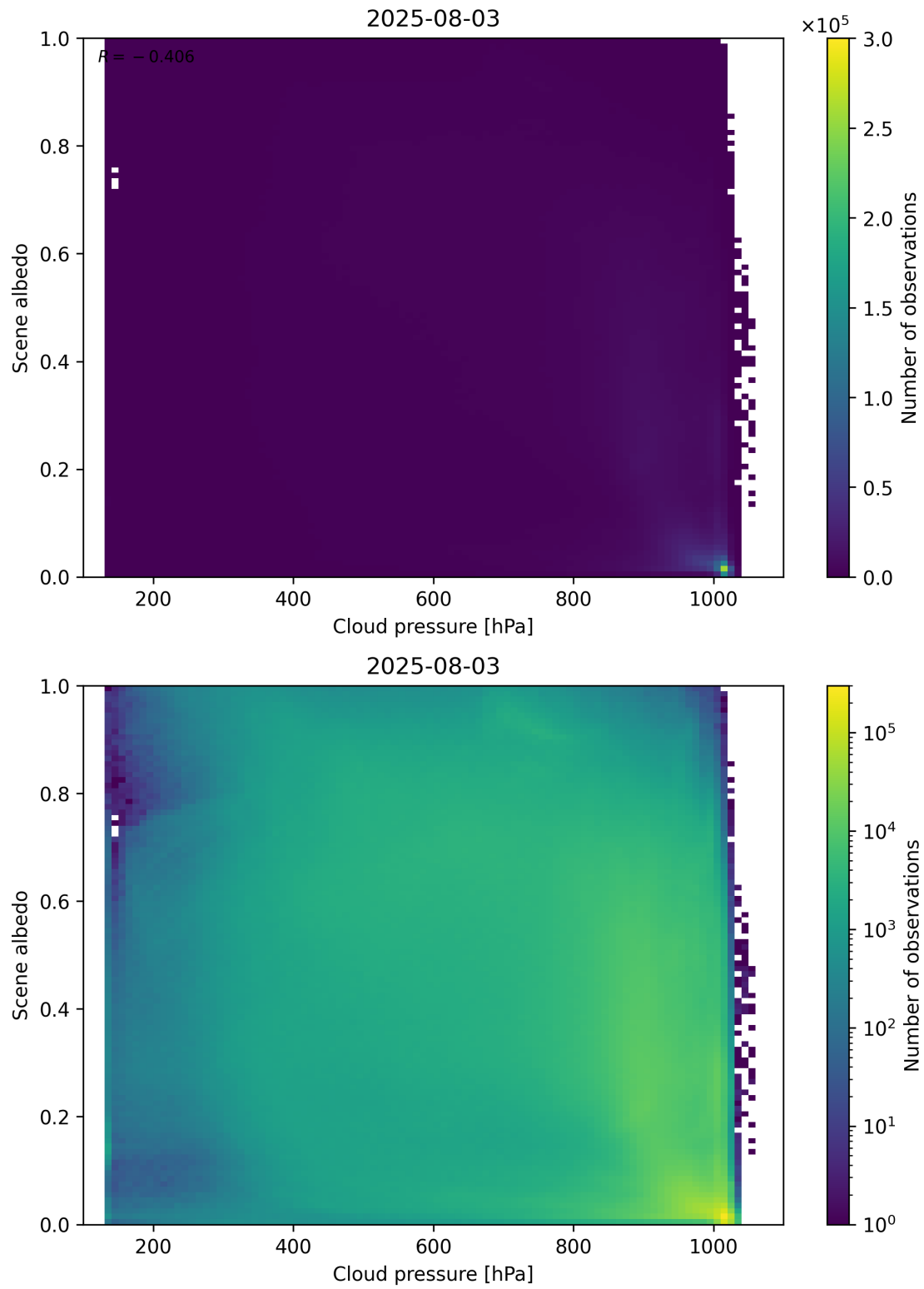
Figure 83: Scatter density plot of “Cloud pressure” against “Scene albedo” for 2025-08-03 to 2025-08-04.
