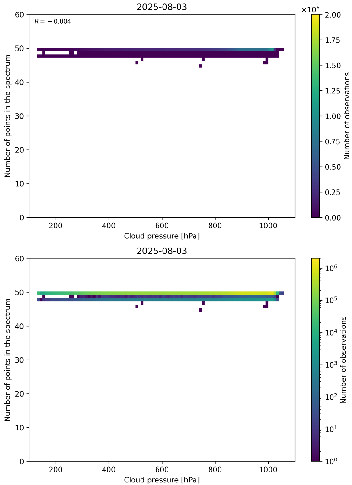
Figure 82: Scatter density plot of “Cloud pressure” against “Number of points in the spectrum” for 2025-08-03 to 2025-08-04.
