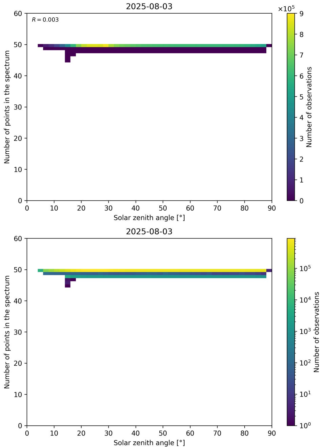
Figure 115: Scatter density plot of “Solar zenith angle” against “Number of points in the spectrum” for 2025-08-03 to 2025-08-04.
