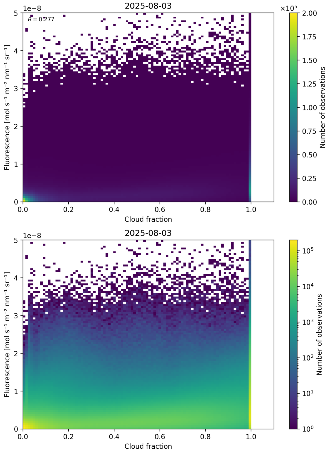
Figure 72: Scatter density plot of “Cloud fraction” against “Fluorescence” for 2025-08-03 to 2025-08-04.
