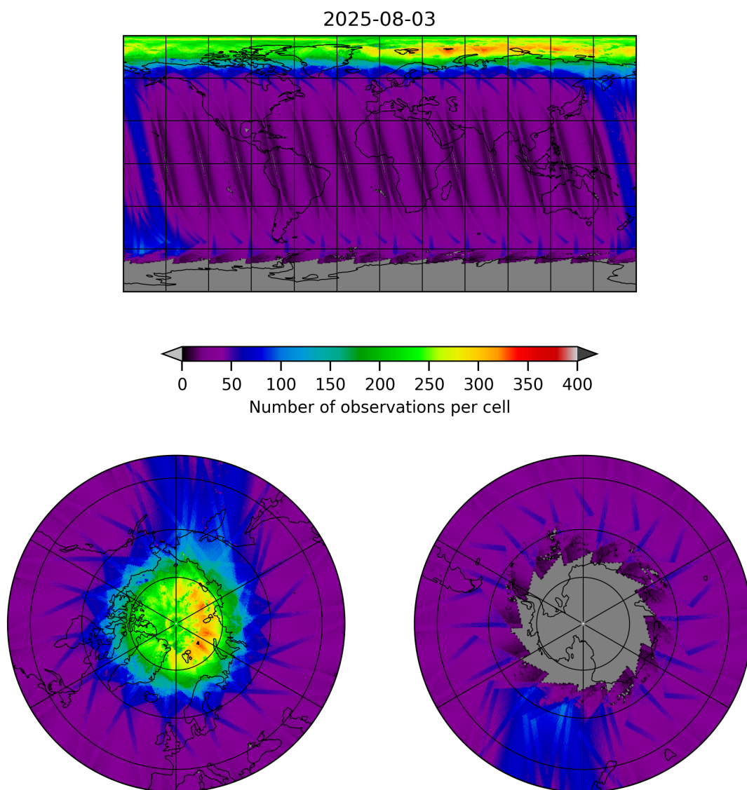
Figure 11: Map of the number of observations for 2025-08-03 to 2025-08-04
