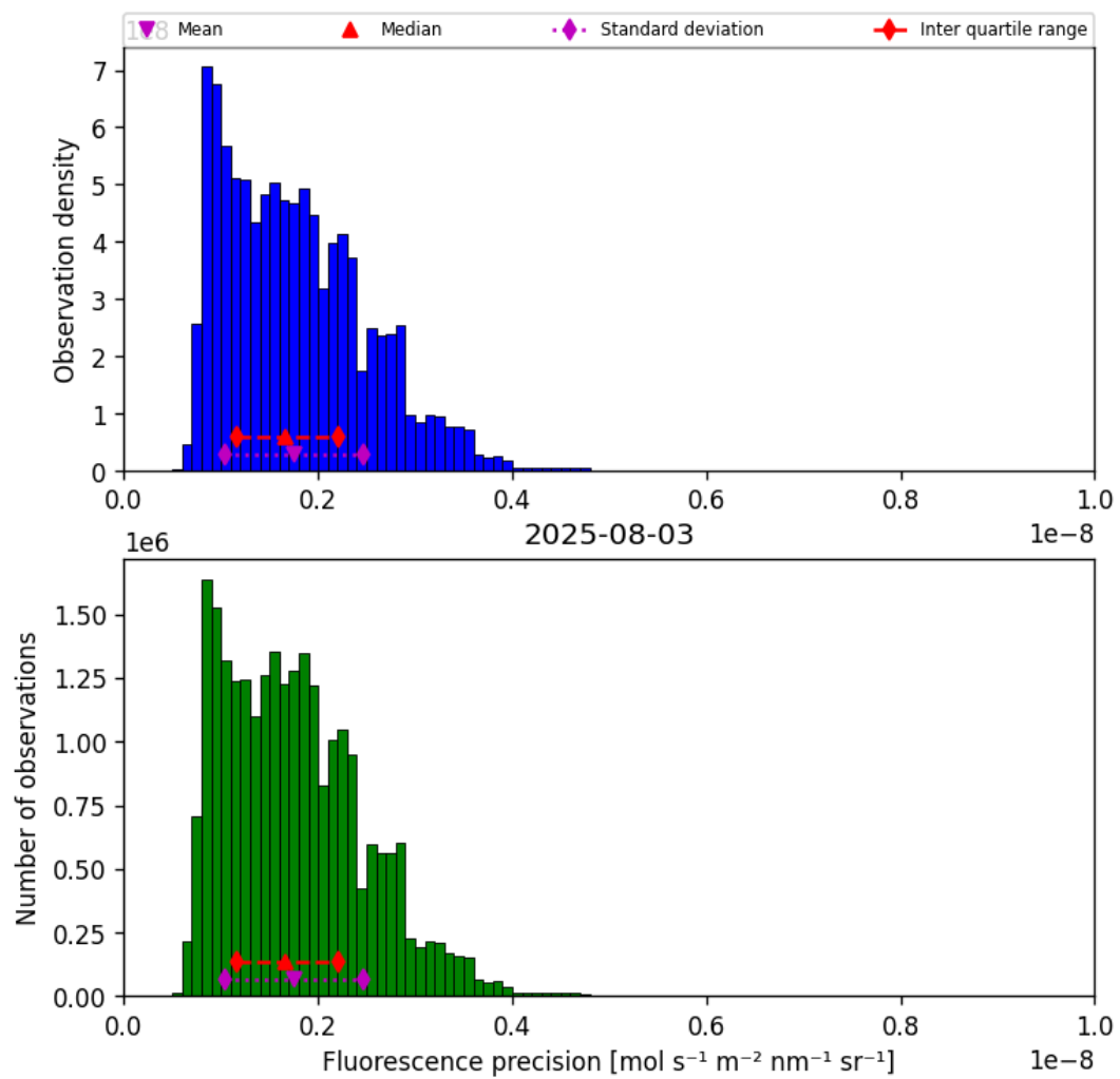
Figure 41: Histogram of “Fluorescence precision” for 2025-08-03 to 2025-08-04
