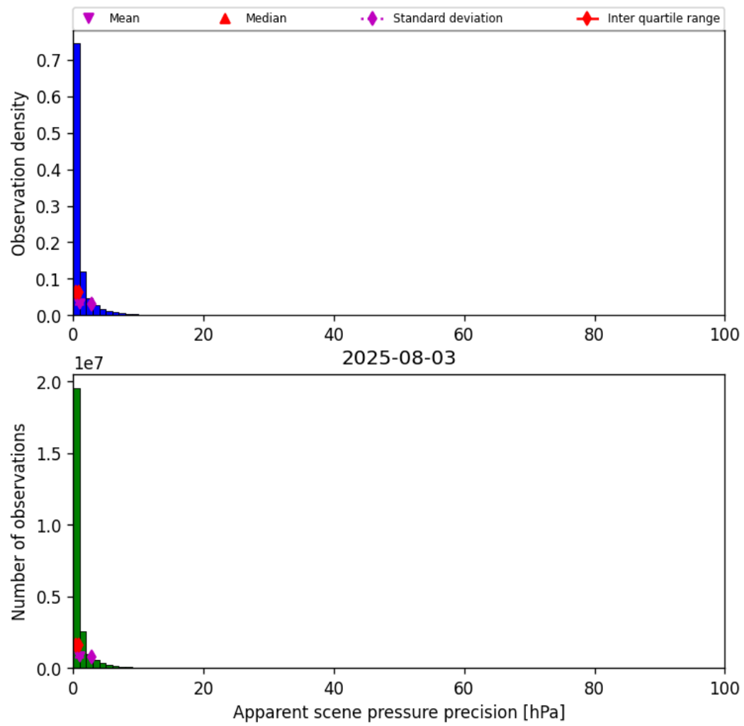
Figure 37: Histogram of “Apparent scene pressure precision” for 2025-08-03 to 2025-08-04
