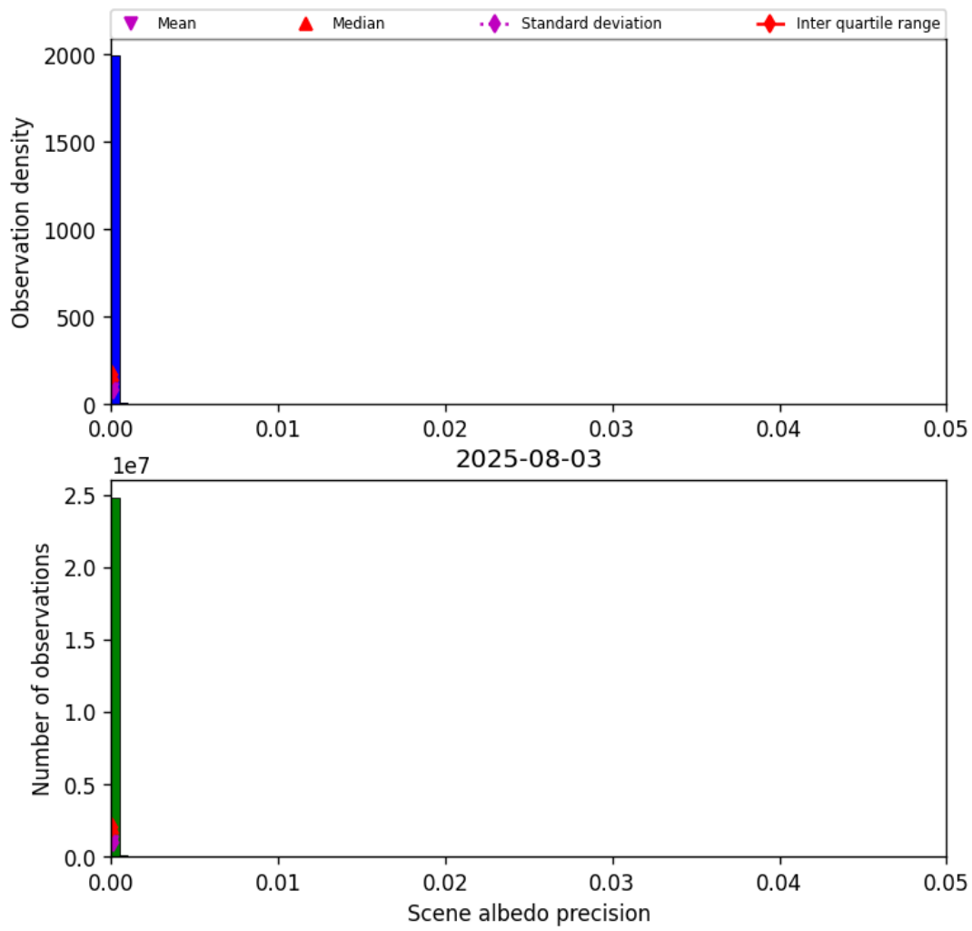
Figure 35: Histogram of “Scene albedo precision” for 2025-08-03 to 2025-08-04
