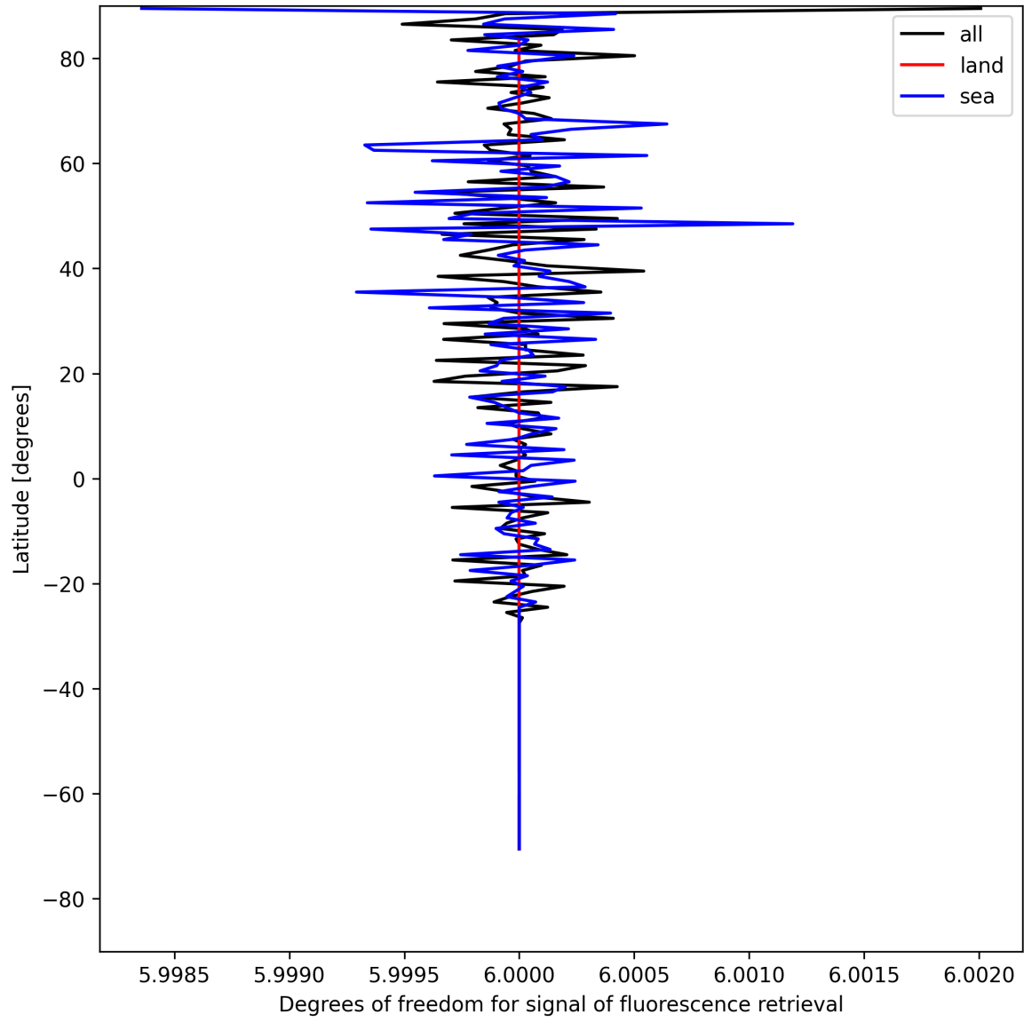
Figure 26: Zonal average of “Degrees of freedom for signal of fluorescence retrieval” for 2025-08-03 to 2025-08-04.
