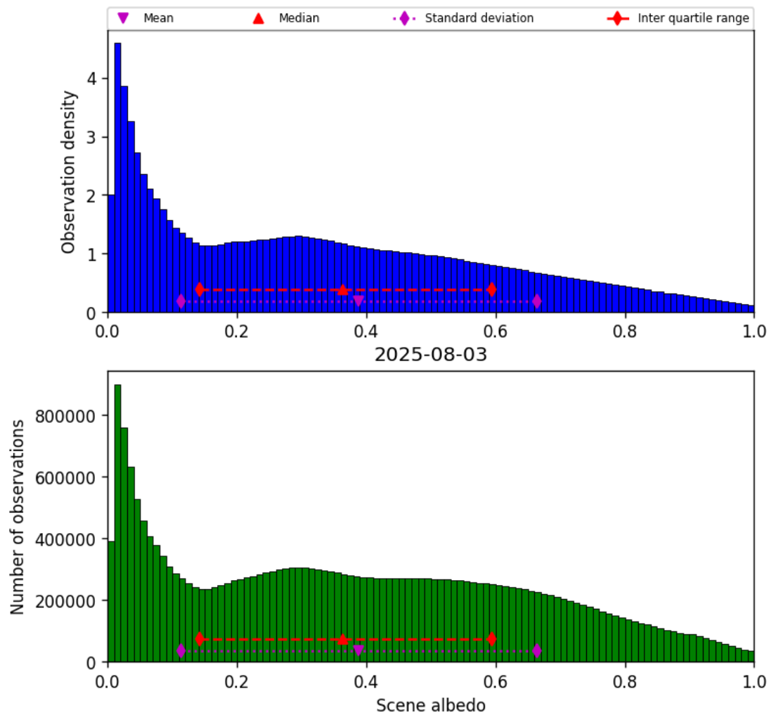
Figure 34: Histogram of “Scene albedo” for 2025-08-03 to 2025-08-04
