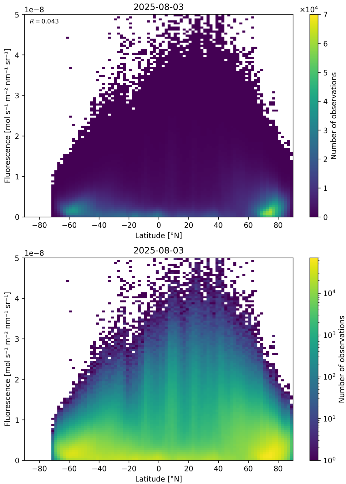
Figure 92: Scatter density plot of “Latitude” against “Fluorescence” for 2025-08-03 to 2025-08-04.
