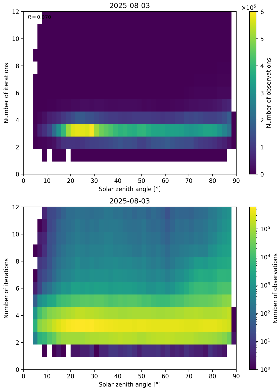
Figure 114: Scatter density plot of “Solar zenith angle” against “Number of iterations” for 2025-08-03 to 2025-08-04.
