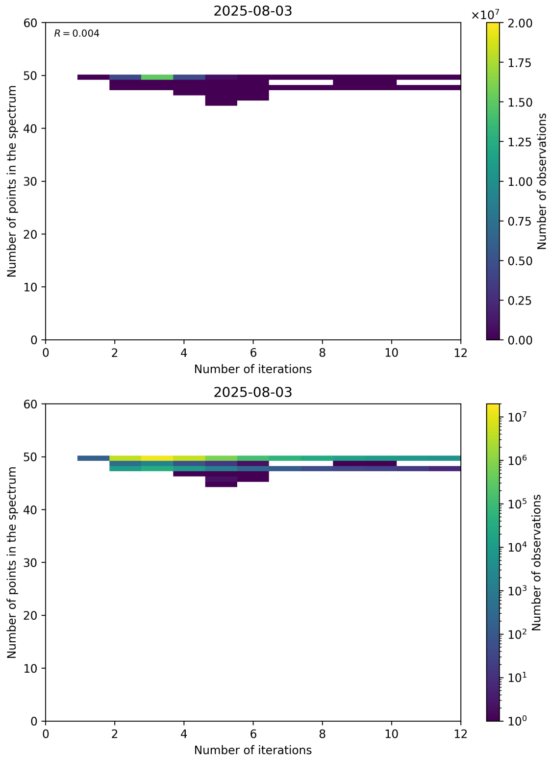
Figure 99: Scatter density plot of “Number of iterations” against “Number of points in the spectrum” for 2025-08-03 to 2025-08-04.
