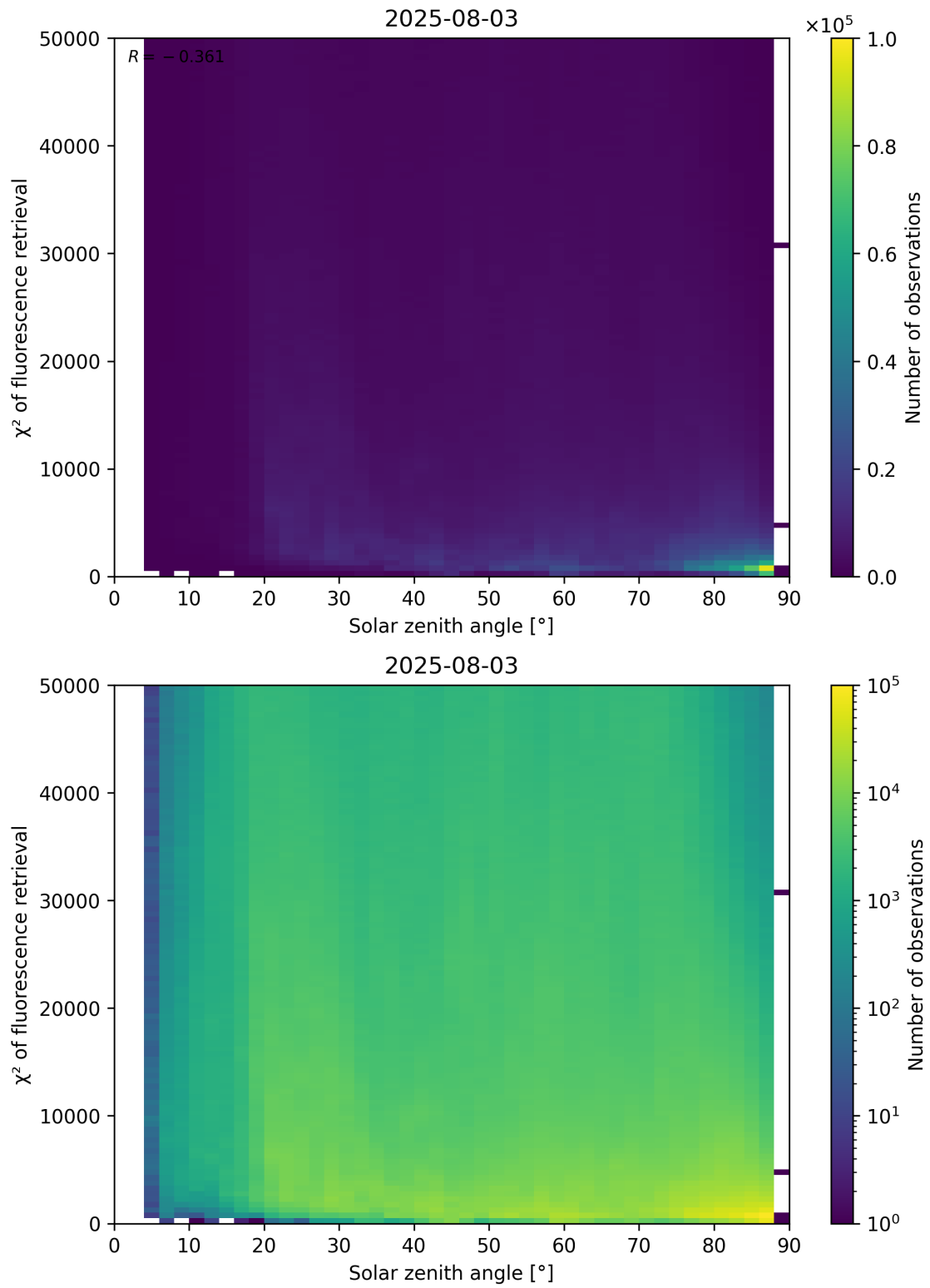
Figure 109: Scatter density plot of “Solar zenith angle” against “ \chi^2 of fluorescence retrieval” for 2025-08-03 to 2025-08-04.
