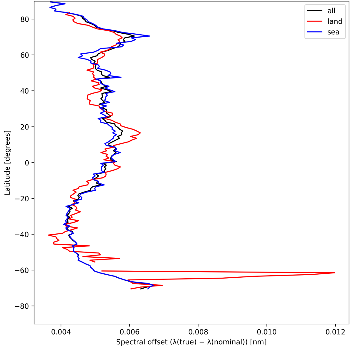
Figure 28: Zonal average of “Spectral offset ( \lambda_{\text{true}} - \lambda_{\text{nominal}} )” for 2025-08-03 to 2025-08-04.
