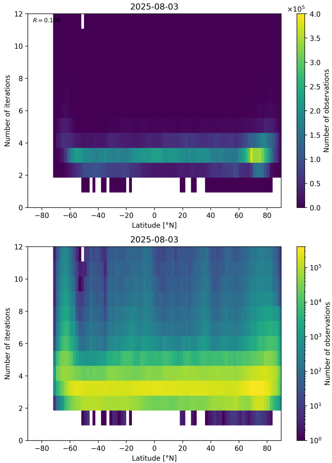
Figure 93: Scatter density plot of “Latitude” against “Number of iterations” for 2025-08-03 to 2025-08-04.
