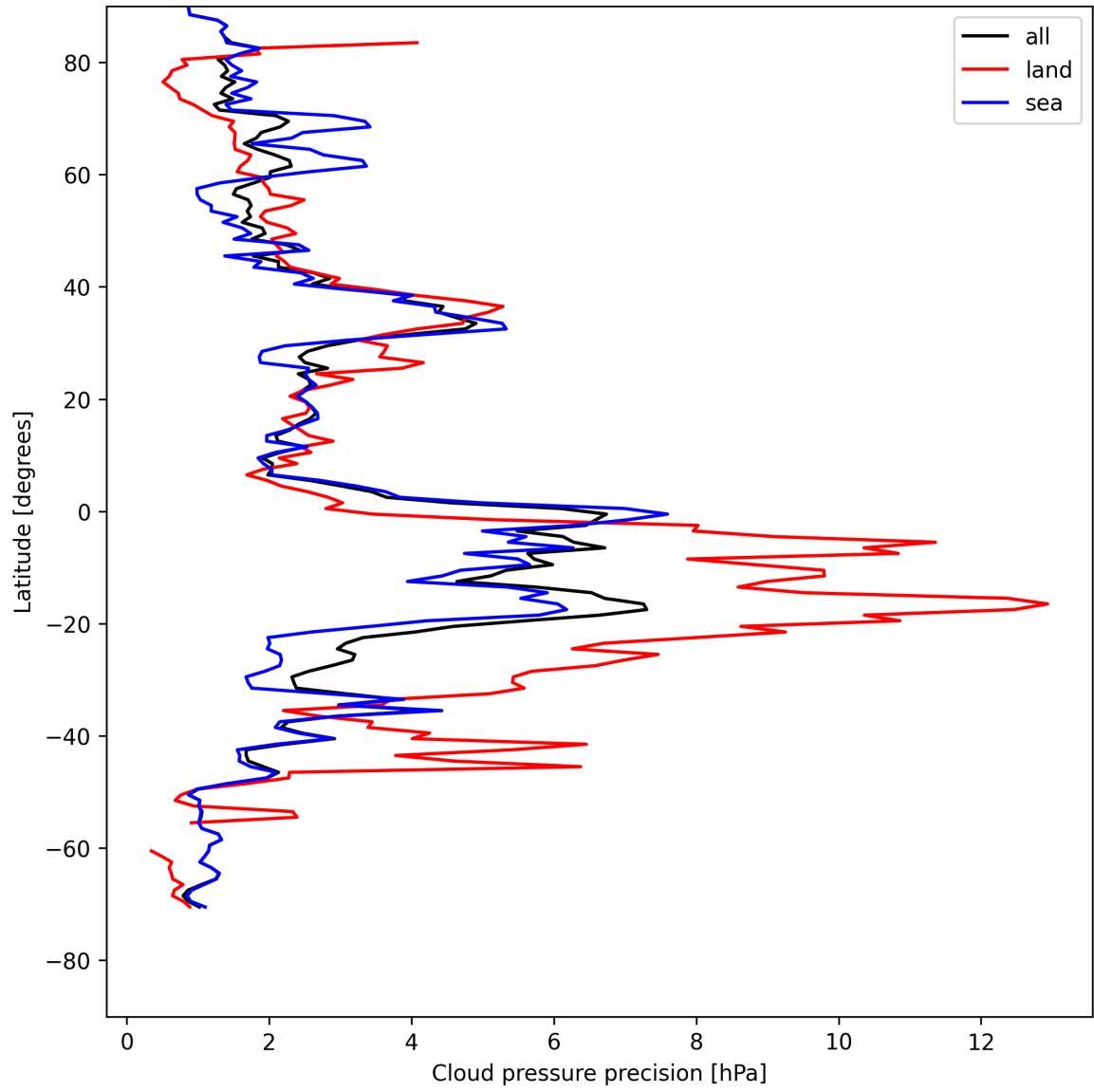
Figure 14: Zonal average of "Cloud pressure precision" for 2025-08-03 to 2025-08-04.
