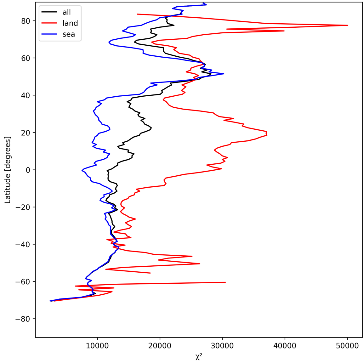
Figure 21: Zonal average of “ \chi^2 ” for 2025-08-03 to 2025-08-04.
