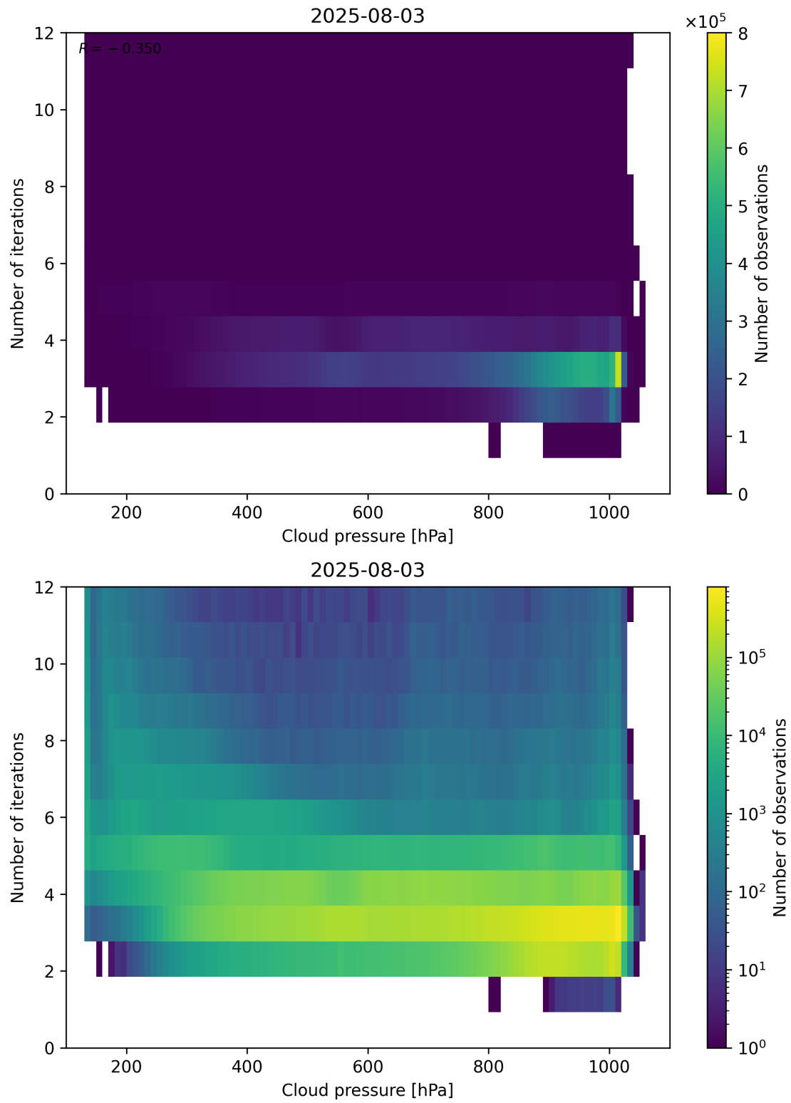
Figure 81: Scatter density plot of “Cloud pressure” against “Number of iterations” for 2025-08-03 to 2025-08-04.
