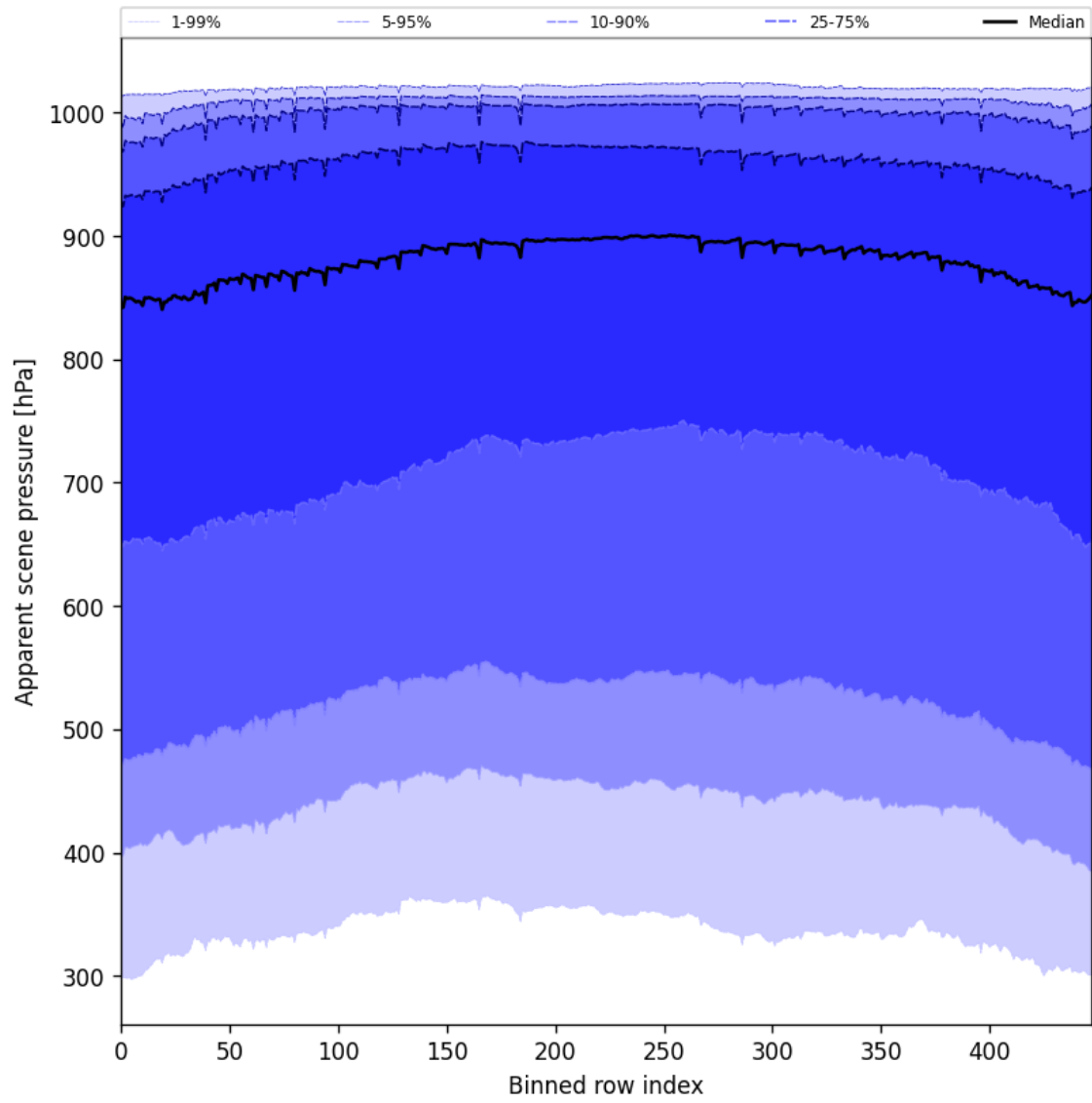
Figure 53: Along track statistics of “Apparent scene pressure” for 2025-08-03 to 2025-08-04
