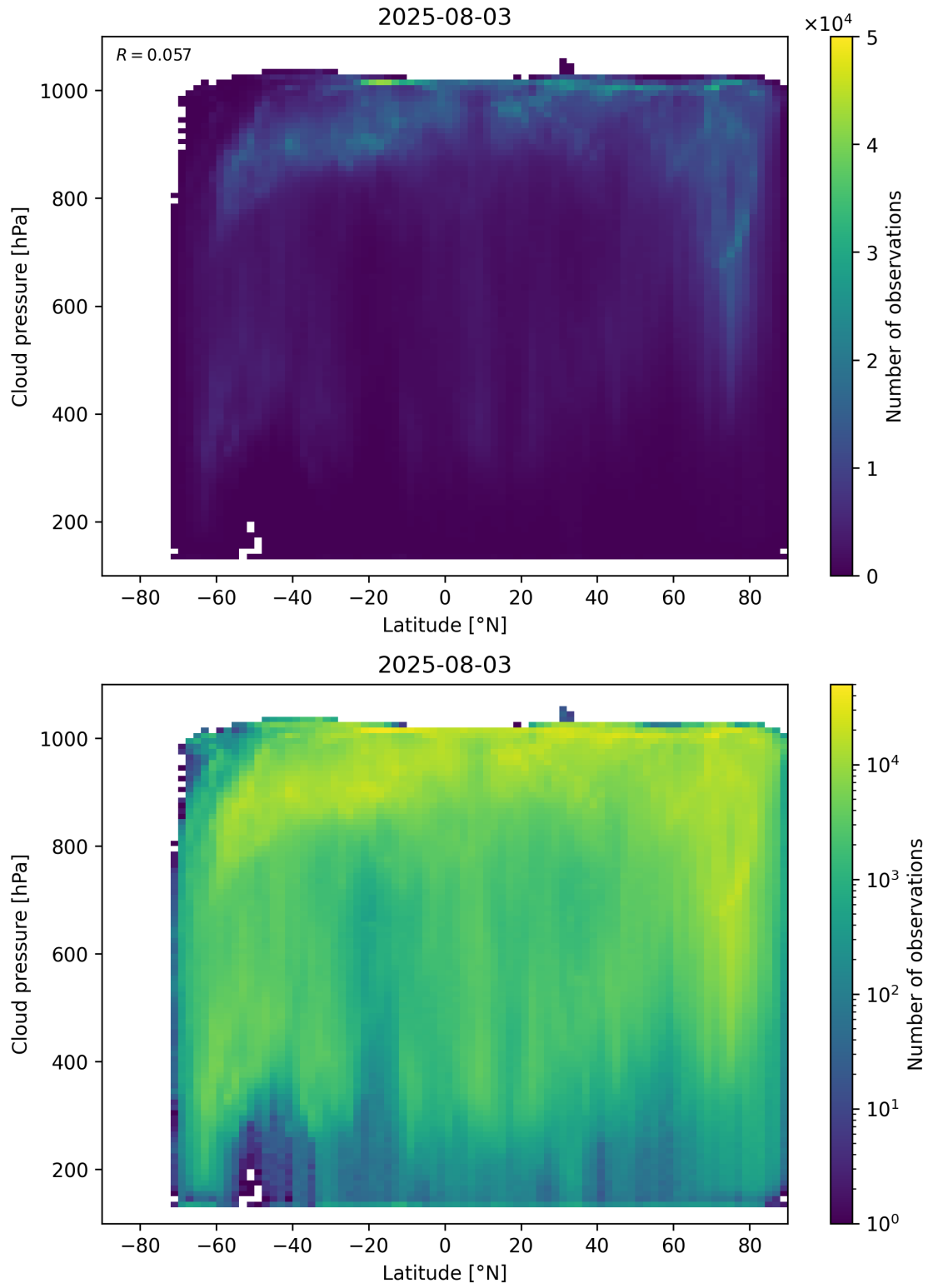
Figure 91: Scatter density plot of “Latitude” against “Cloud pressure” for 2025-08-03 to 2025-08-04.
