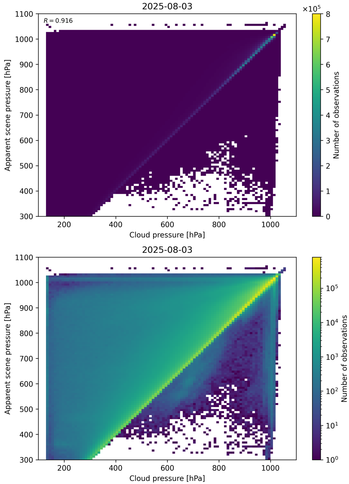
Figure 77: Scatter density plot of “Cloud pressure” against “Apparent scene pressure” for 2025-08-03 to 2025-08-04.
