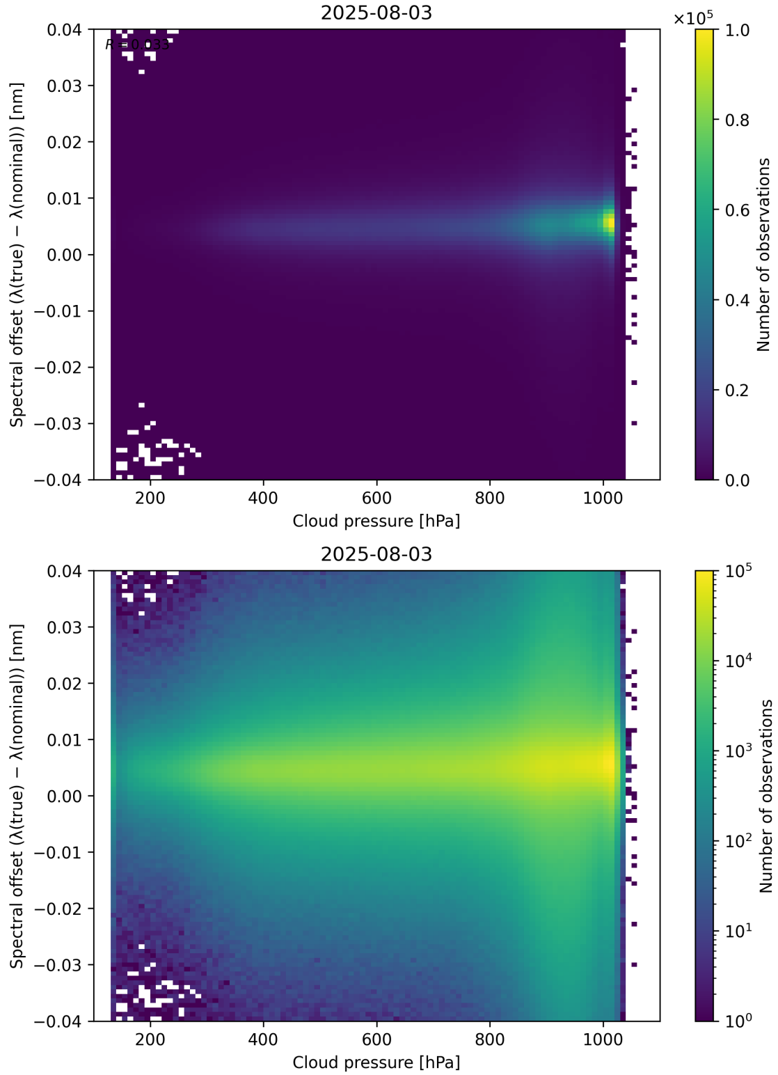
Figure 84: Scatter density plot of “Cloud pressure” against “Spectral offset ( \lambda_{\text{true}} - \lambda_{\text{nominal}} )” for 2025-08-03 to 2025-08-04.
