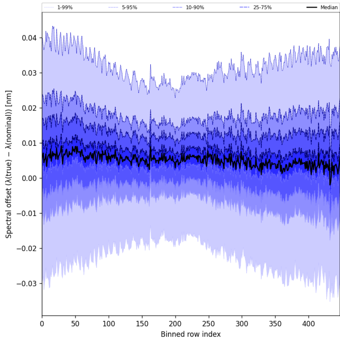
Figure 62: Along track statistics of “Spectral offset ( \lambda_{\text{true}} - \lambda_{\text{nominal}} )” for 2025-08-03 to 2025-08-04
