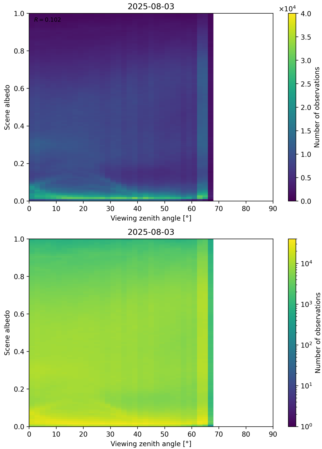
Figure 126: Scatter density plot of “Viewing zenith angle” against “Scene albedo” for 2025-08-03 to 2025-08-04.
