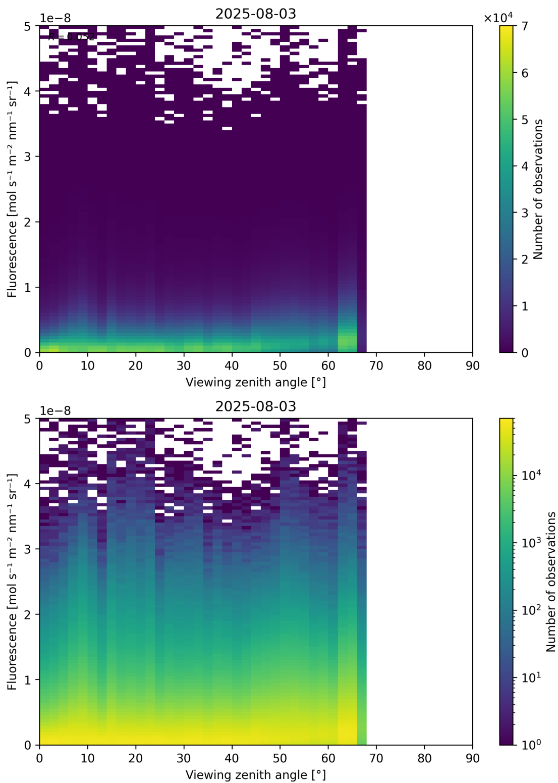
Figure 122: Scatter density plot of “Viewing zenith angle” against “Fluorescence” for 2025-08-03 to 2025-08-04.
