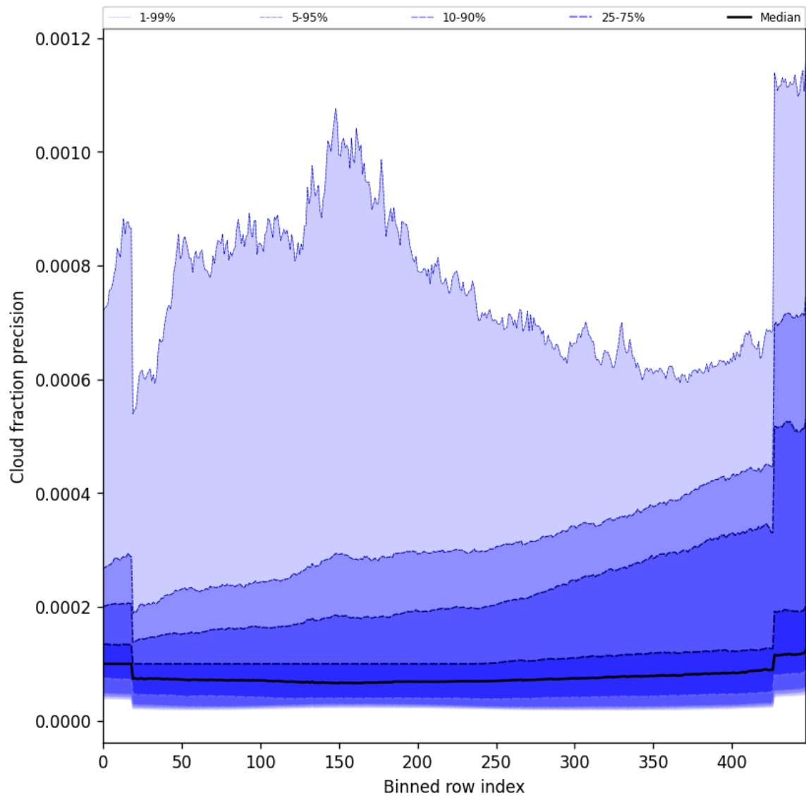
Figure 50: Along track statistics of “Cloud fraction precision” for 2025-08-03 to 2025-08-04
