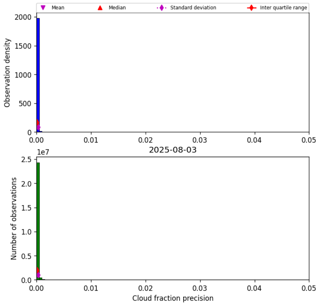
Figure 33: Histogram of “Cloud fraction precision” for 2025-08-03 to 2025-08-04
