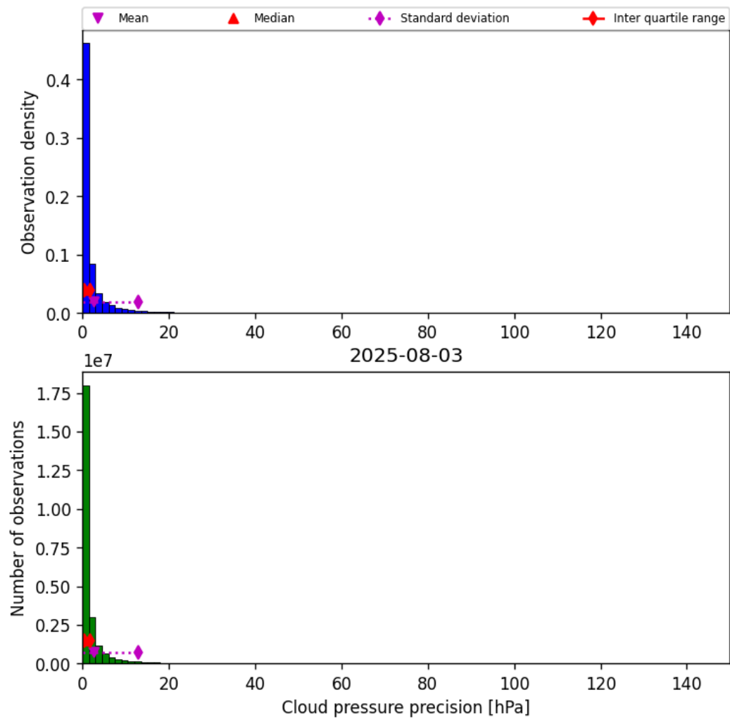
Figure 31: Histogram of “Cloud pressure precision” for 2025-08-03 to 2025-08-04
