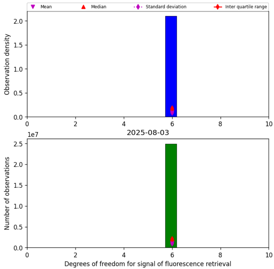
Figure 43: Histogram of “Degrees of freedom for signal of fluorescence retrieval” for 2025-08-03 to 2025-08-04
