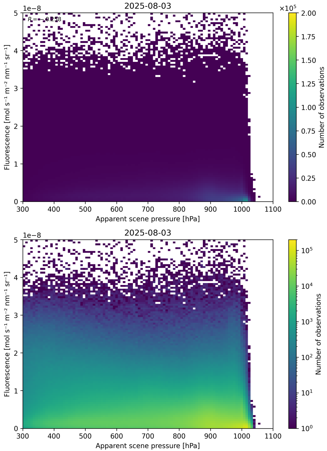
Figure 64: Scatter density plot of “Apparent scene pressure” against “Fluorescence” for 2025-08-03 to 2025-08-04.
