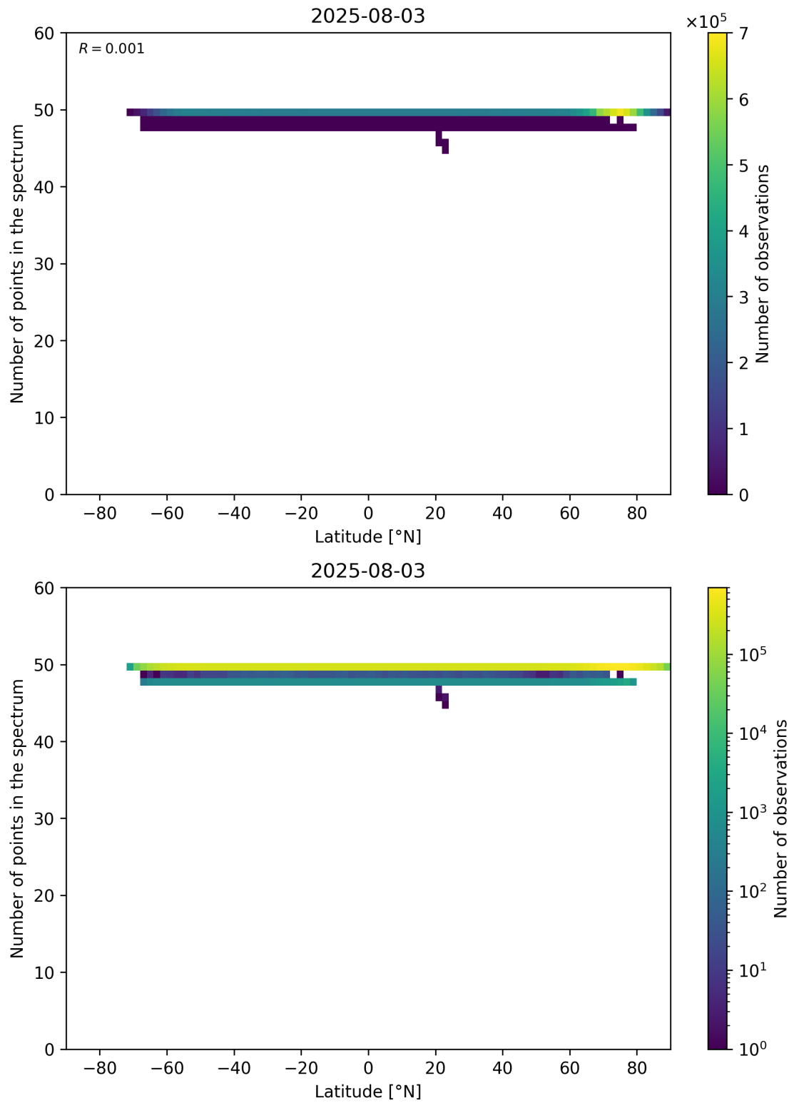
Figure 94: Scatter density plot of “Latitude” against “Number of points in the spectrum” for 2025-08-03 to 2025-08-04.
