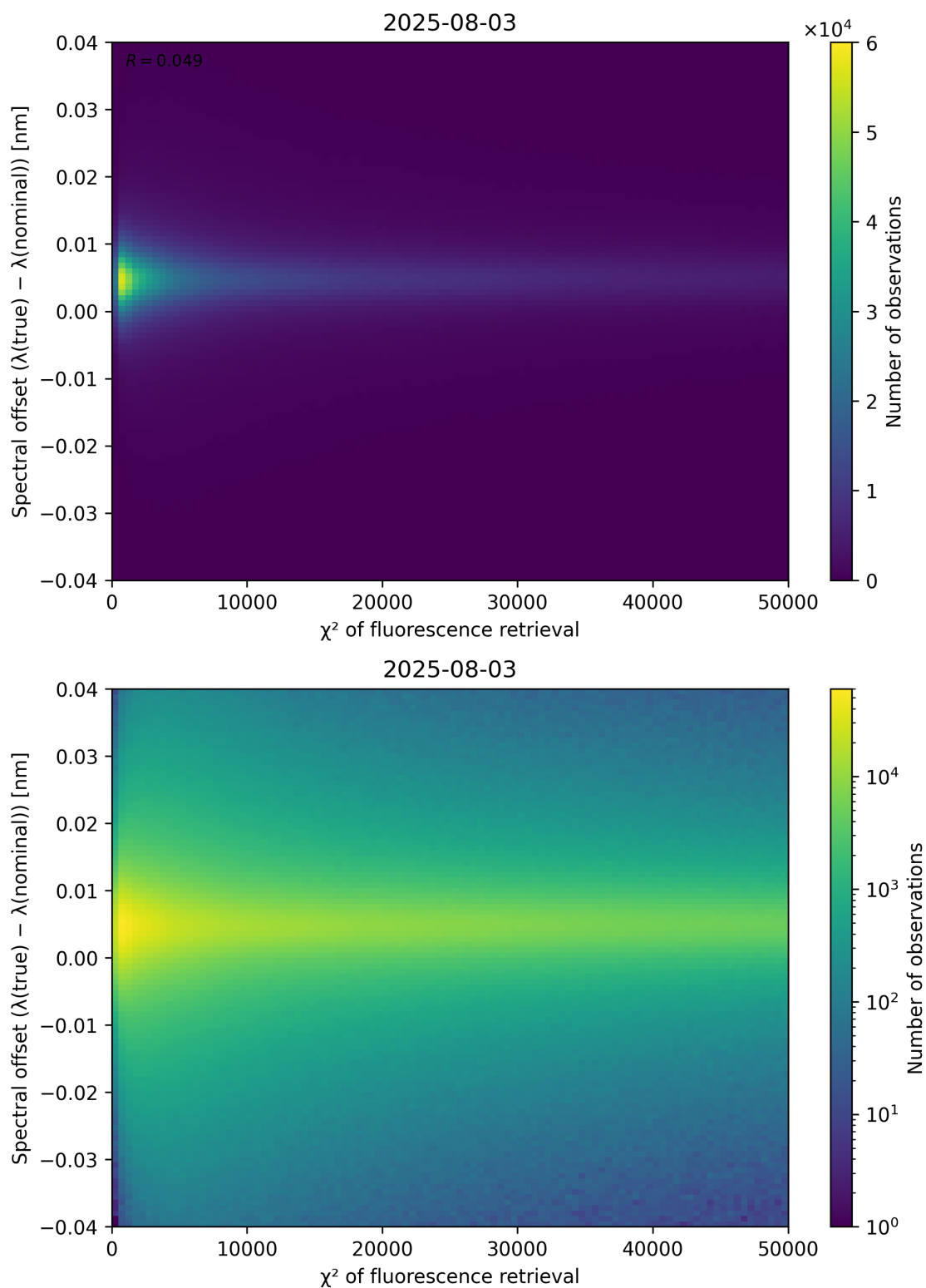
Figure 69: Scatter density plot of “ \chi^2 of fluorescence retrieval” against “Spectral offset ( \lambda_{\text{true}} - \lambda_{\text{nominal}} )” for 2025-08-03 to 2025-08-04.
