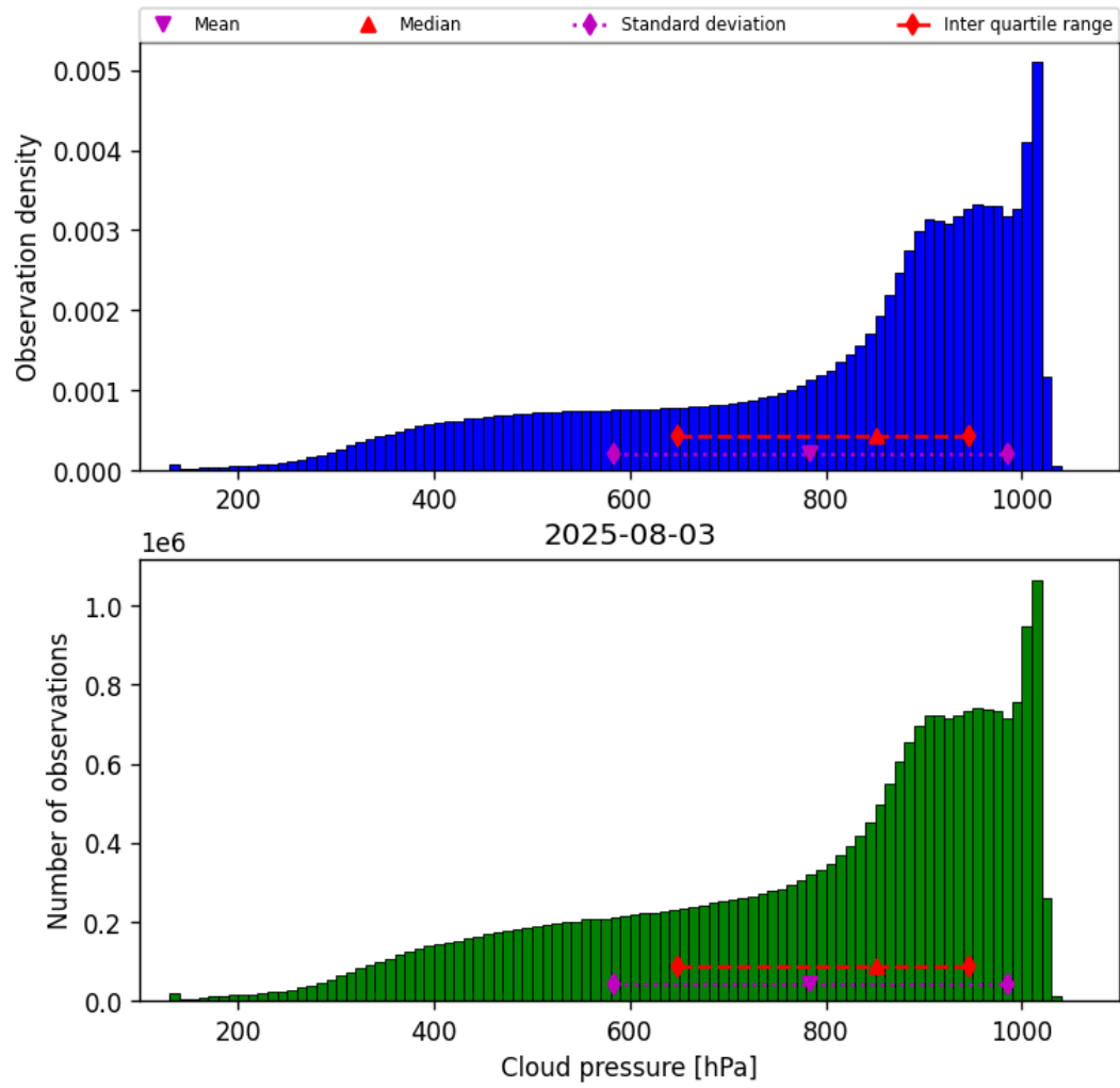
Figure 30: Histogram of “Cloud pressure” for 2025-08-03 to 2025-08-04
