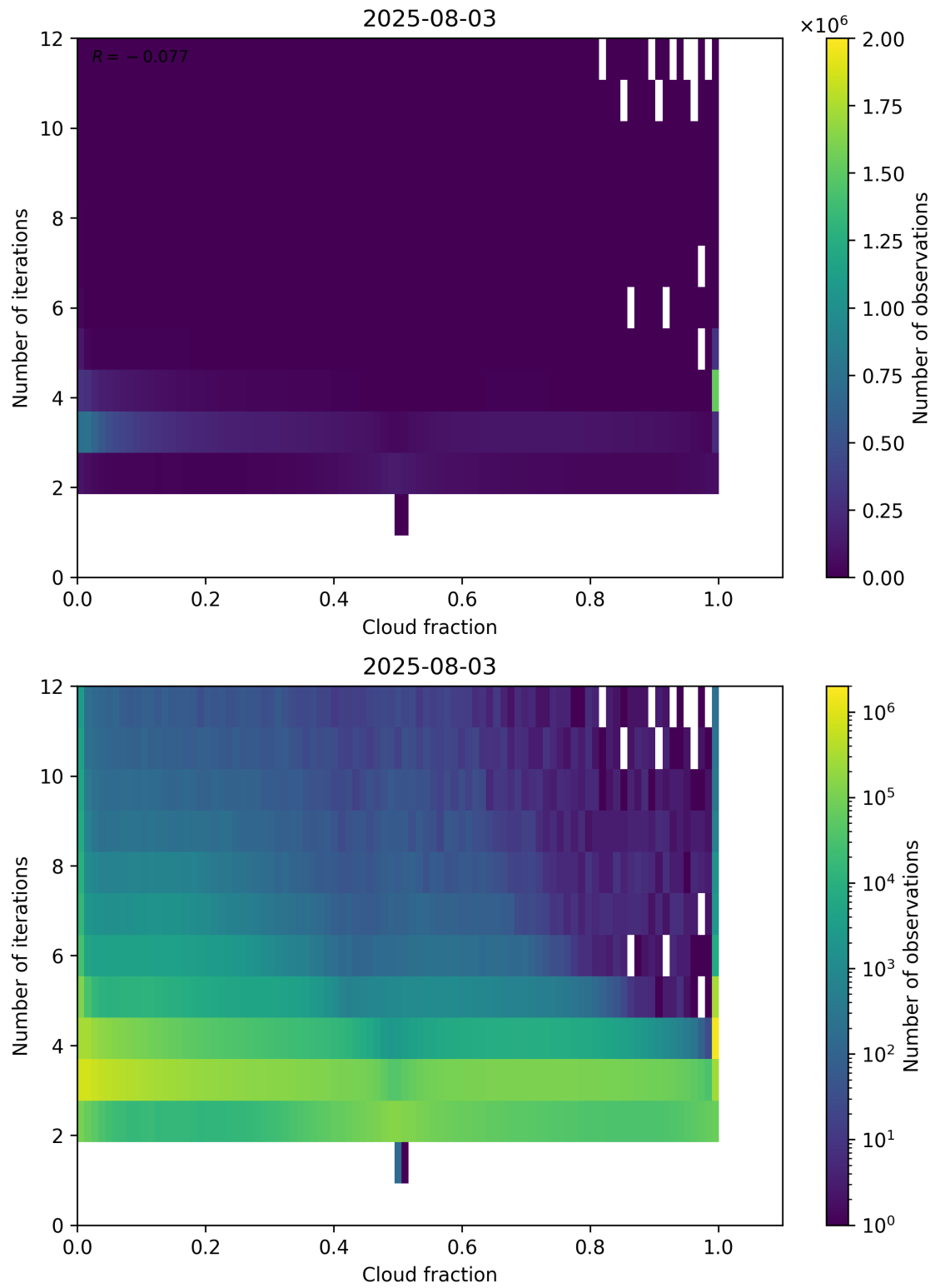
Figure 73: Scatter density plot of “Cloud fraction” against “Number of iterations” for 2025-08-03 to 2025-08-04.
