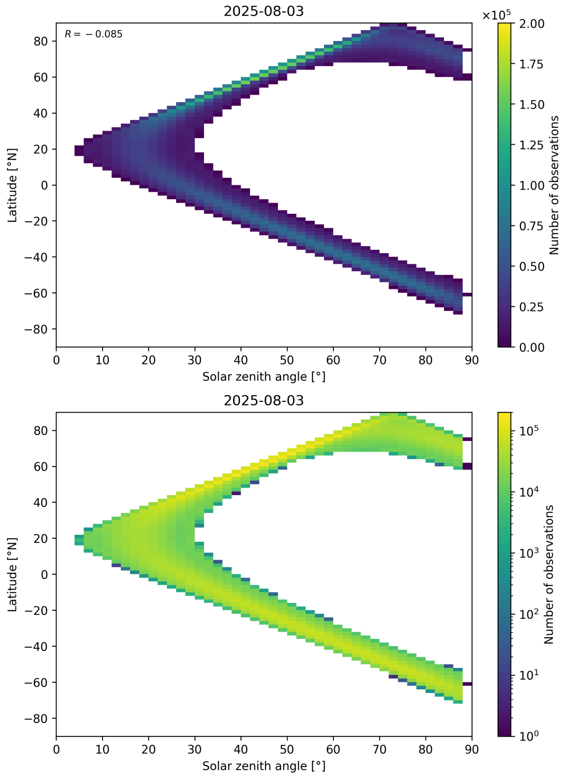
Figure 113: Scatter density plot of “Solar zenith angle” against “Latitude” for 2025-08-03 to 2025-08-04.
