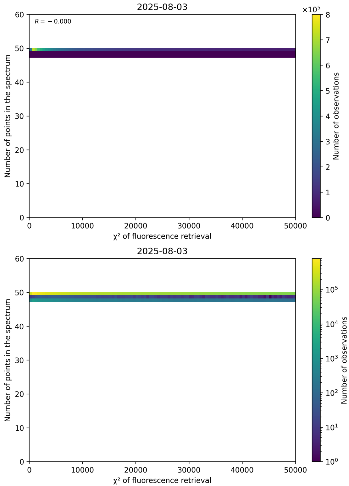
Figure 68: Scatter density plot of " \chi^2 of fluorescence retrieval" against "Number of points in the spectrum" for 2025-08-03 to 2025-08-04.
