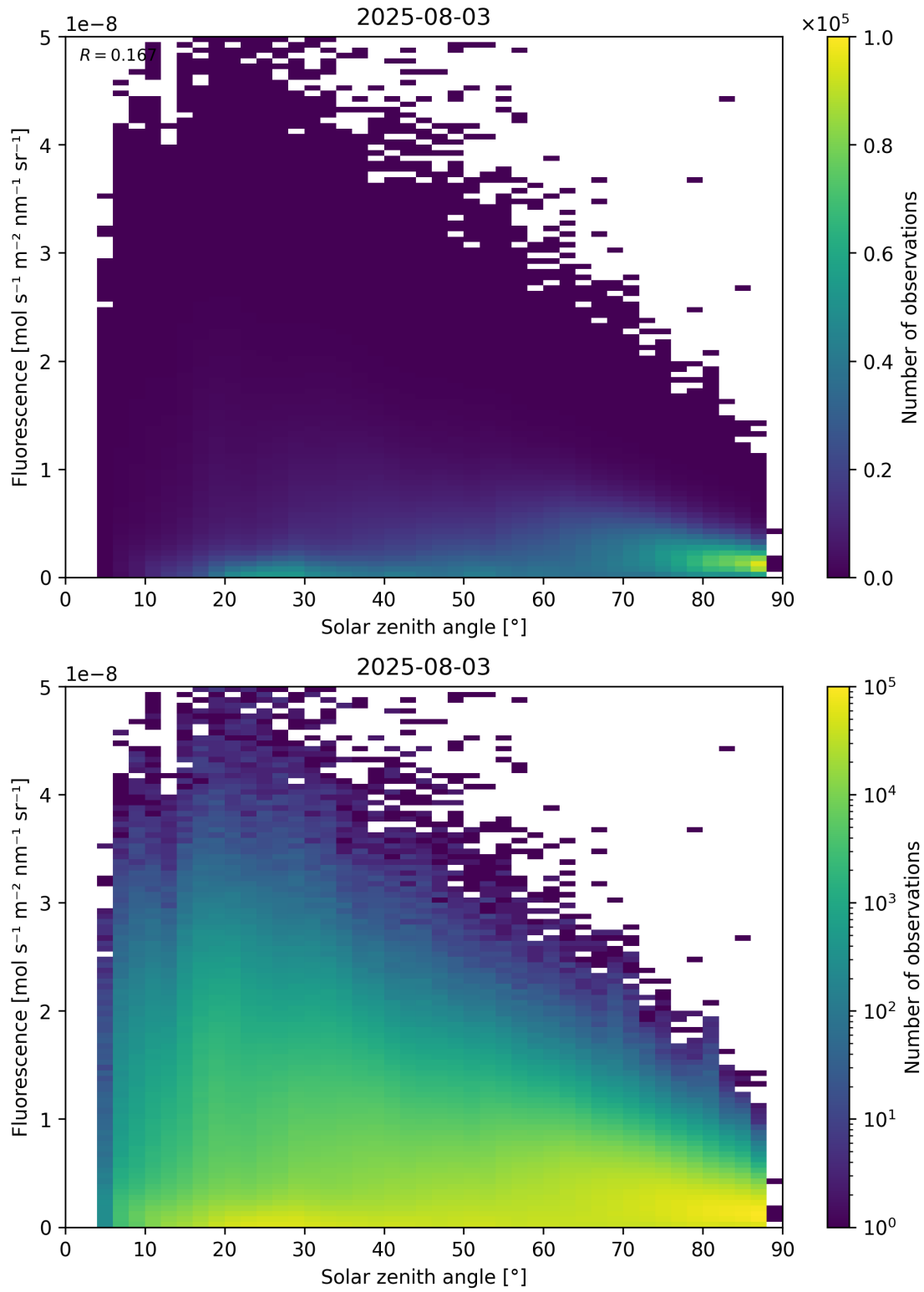
Figure 112: Scatter density plot of “Solar zenith angle” against “Fluorescence” for 2025-08-03 to 2025-08-04.
