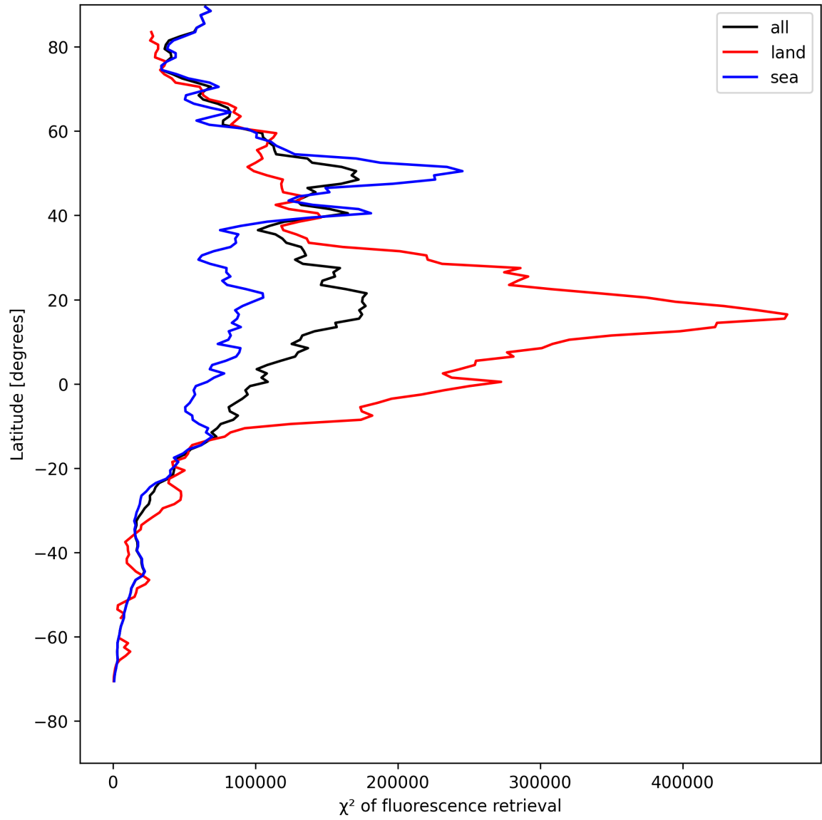
Figure 25: Zonal average of “ \chi^2 of fluorescence retrieval” for 2025-08-03 to 2025-08-04.
