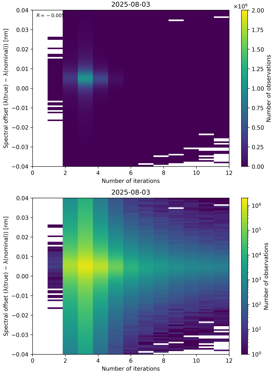
Figure 100: Scatter density plot of “Number of iterations” against “Spectral offset ( \lambda_{\text{true}} - \lambda_{\text{nominal}} )” for 2025-08-03 to 2025-08-04.
