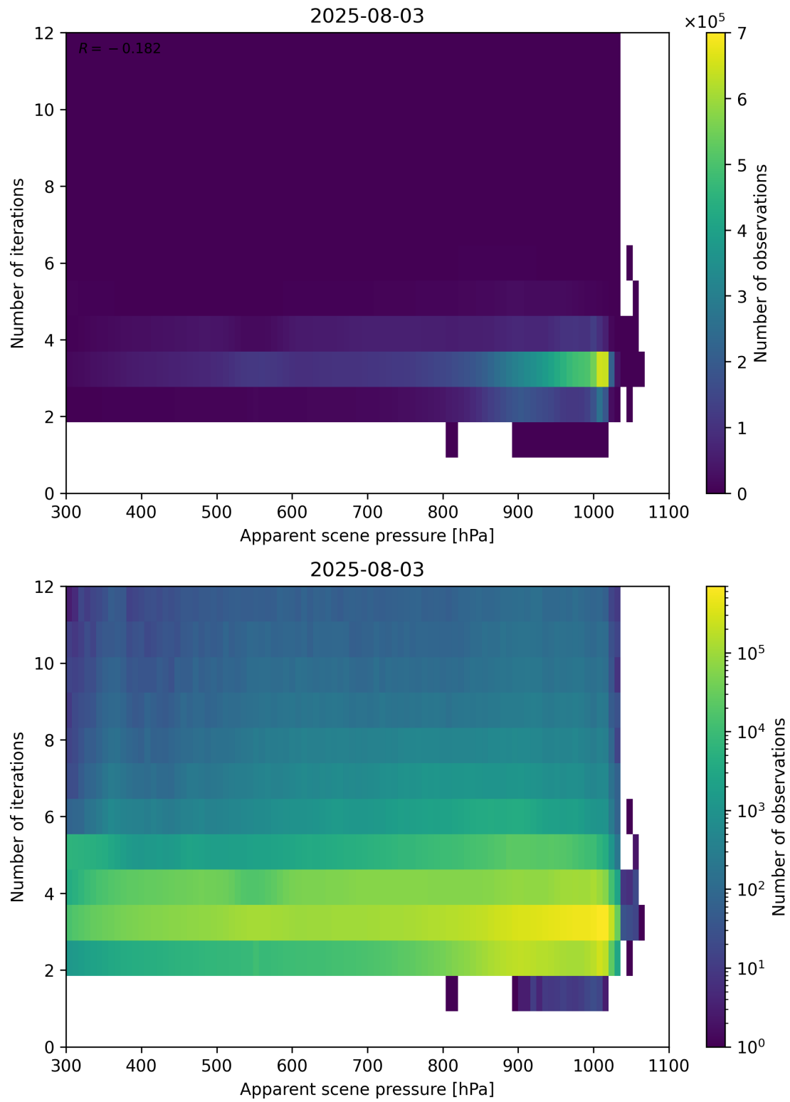
Figure 65: Scatter density plot of “Apparent scene pressure” against “Number of iterations” for 2025-08-03 to 2025-08-04.
