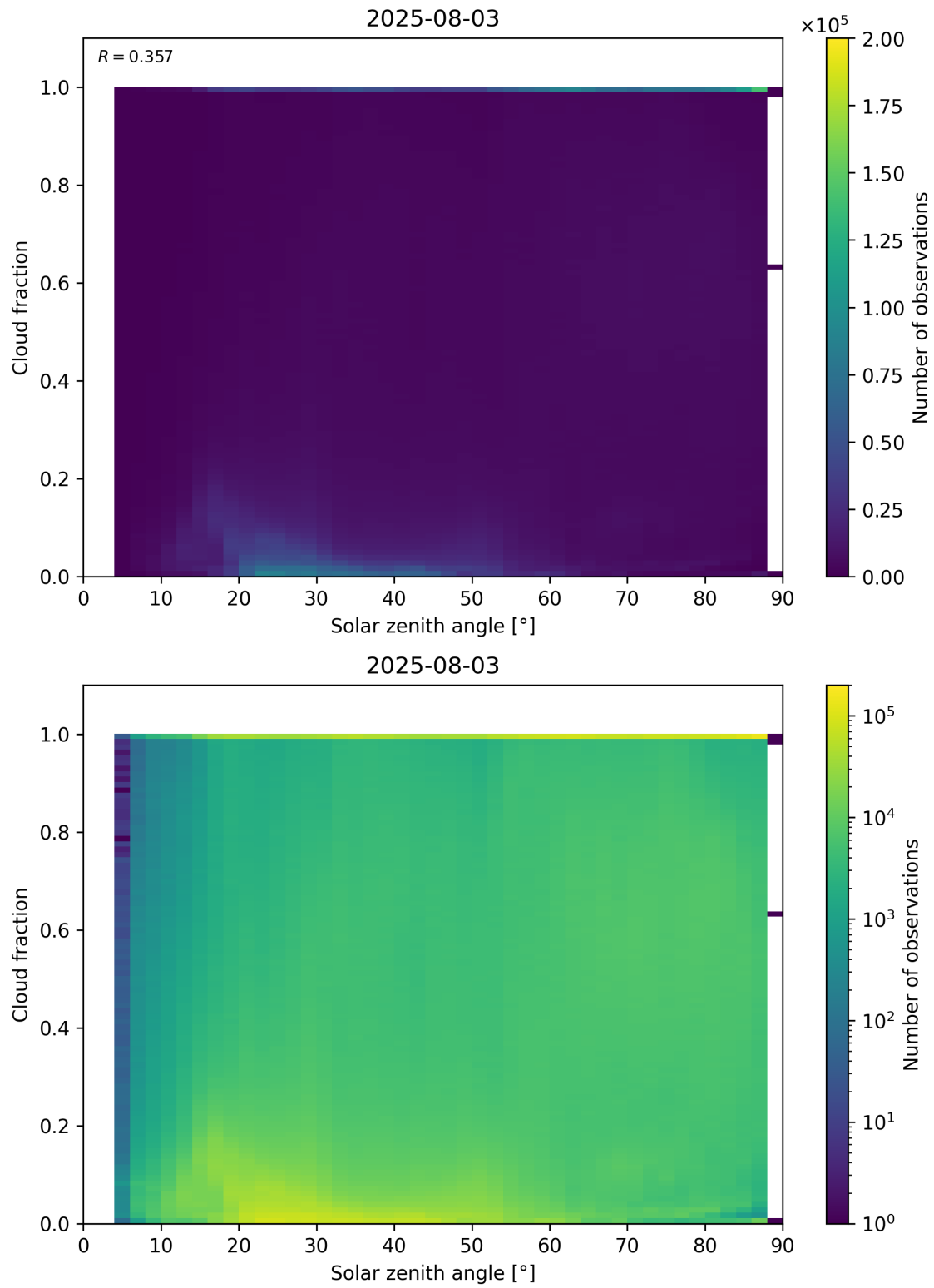
Figure 110: Scatter density plot of “Solar zenith angle” against “Cloud fraction” for 2025-08-03 to 2025-08-04.
