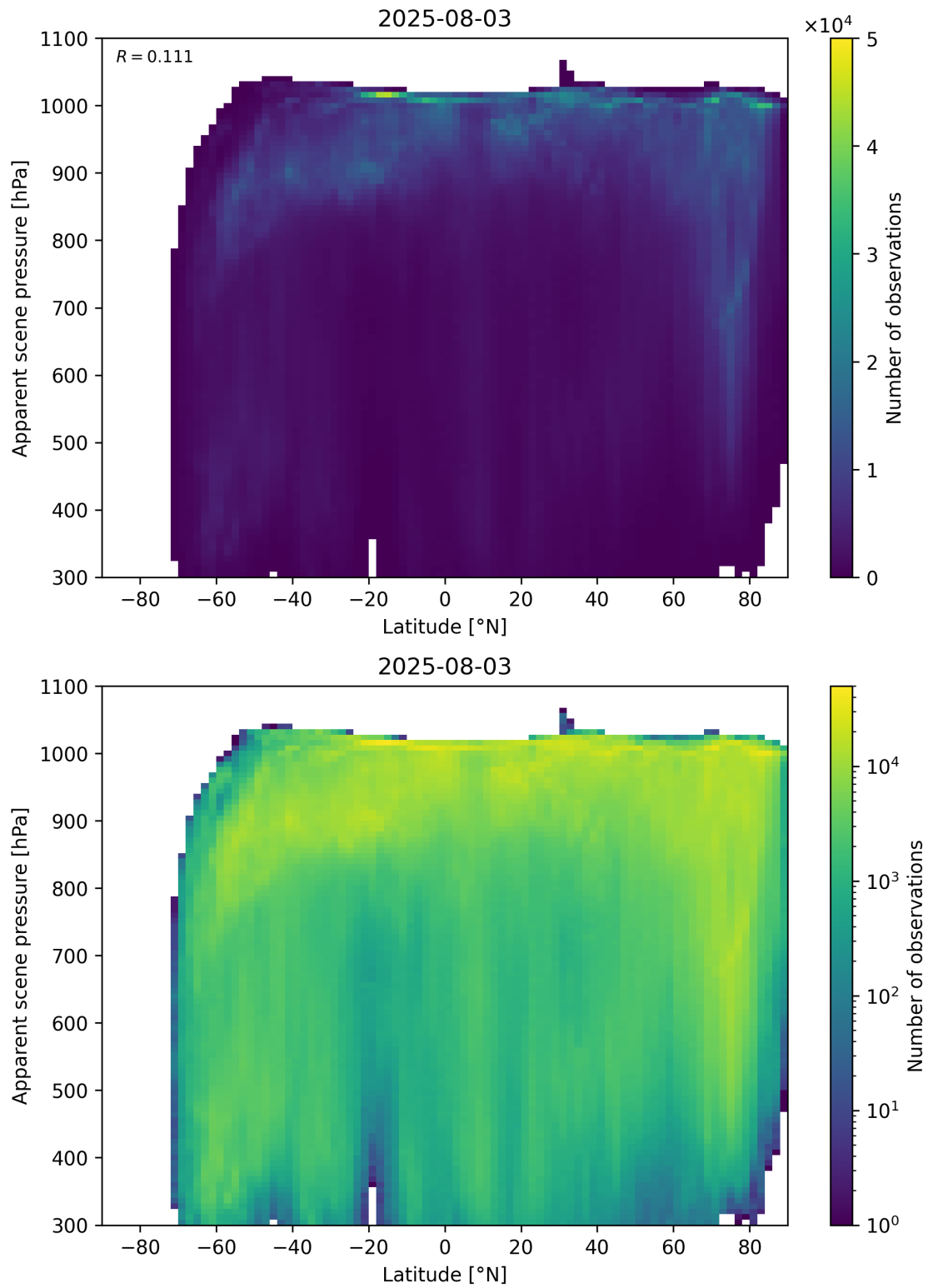
Figure 88: Scatter density plot of “Latitude” against “Apparent scene pressure” for 2025-08-03 to 2025-08-04.
