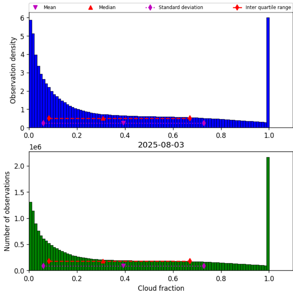
Figure 32: Histogram of “Cloud fraction” for 2025-08-03 to 2025-08-04
