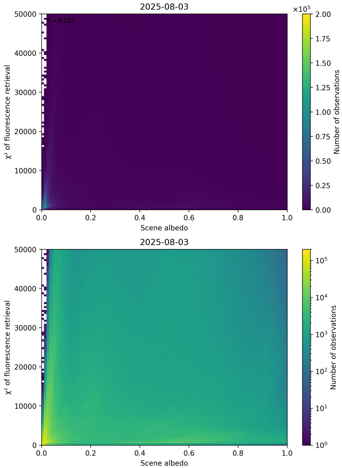
Figure 103: Scatter density plot of “Scene albedo” against “ \chi^2 of fluorescence retrieval” for 2025-08-03 to 2025-08-04.
