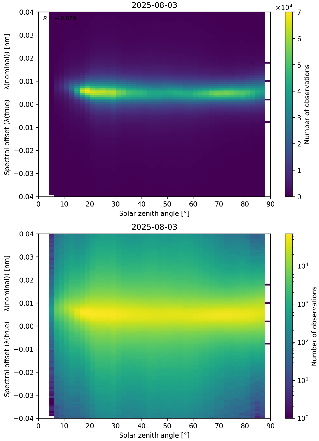
Figure 117: Scatter density plot of “Solar zenith angle” against “Spectral offset ( \lambda_{\text{true}} - \lambda_{\text{nominal}} )” for 2025-08-03 to 2025-08-04.
