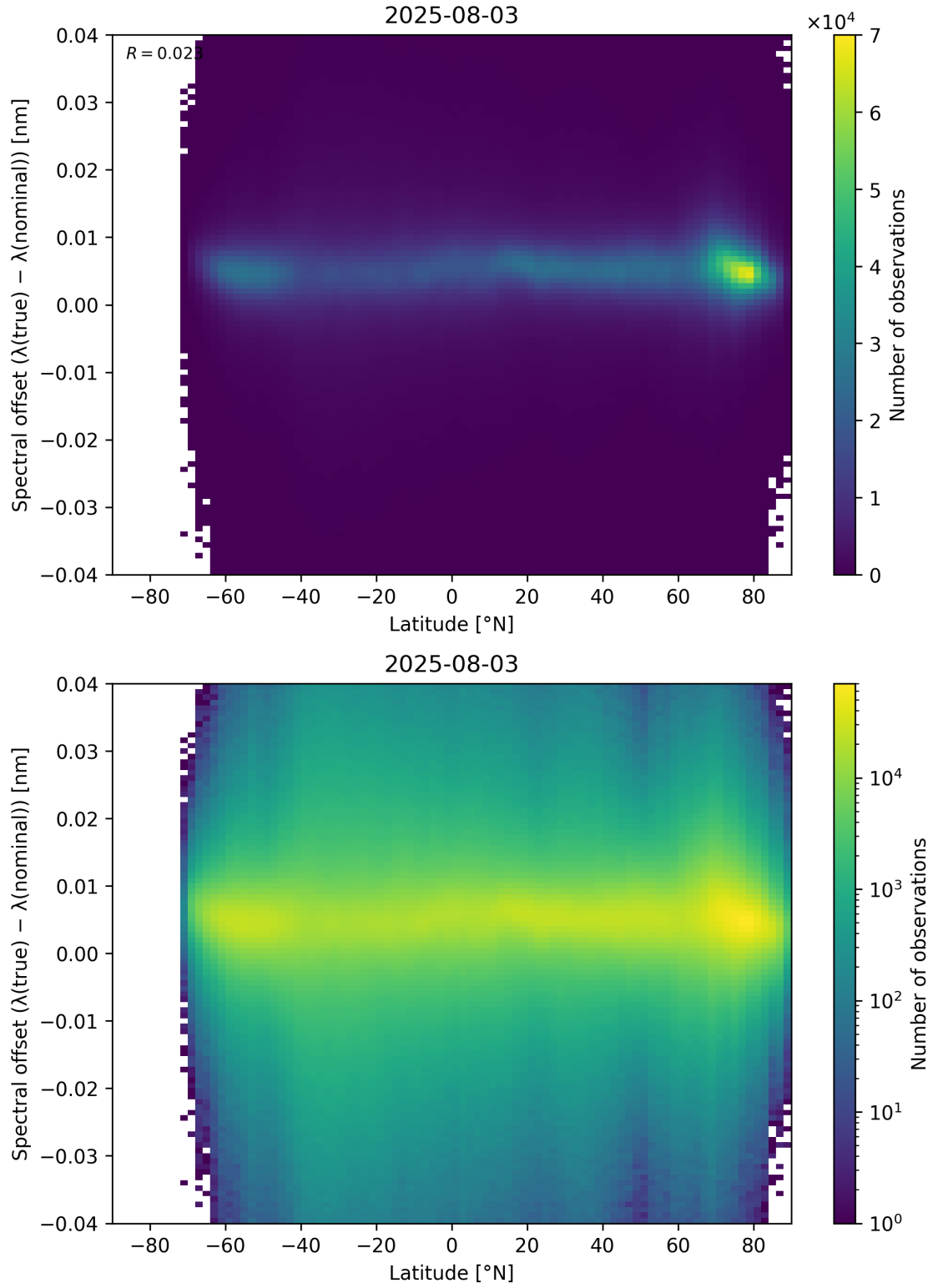
Figure 96: Scatter density plot of “Latitude” against “Spectral offset ( \lambda_{\text{true}} - \lambda_{\text{nominal}} )” for 2025-08-03 to 2025-08-04.
