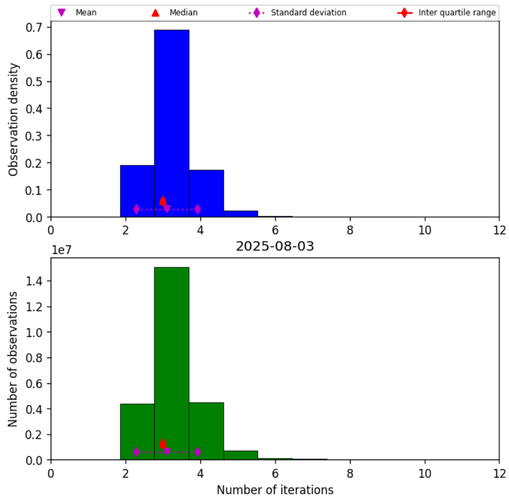
Figure 39: Histogram of “Number of iterations” for 2025-08-03 to 2025-08-04
