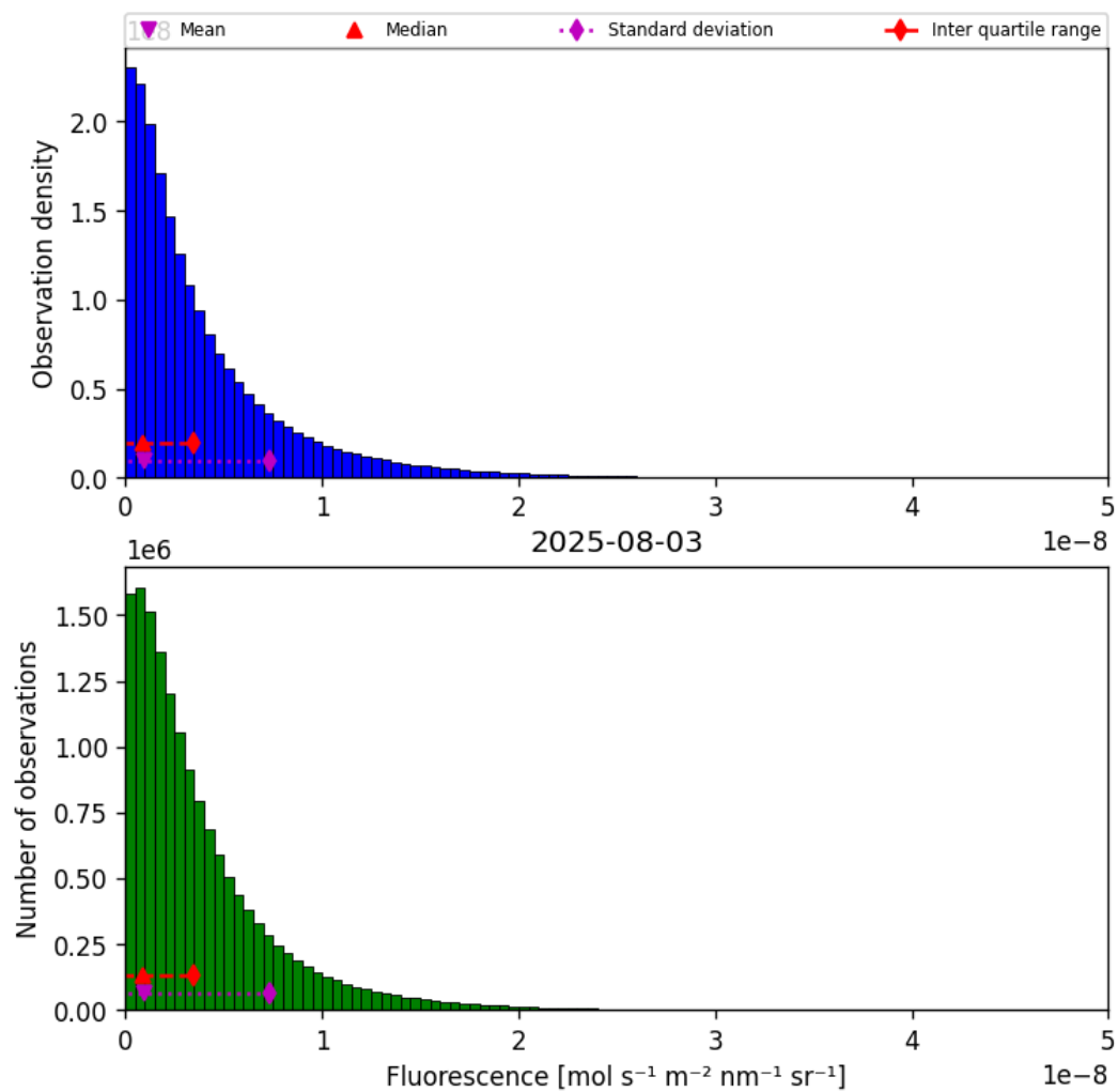
Figure 40: Histogram of “Fluorescence” for 2025-08-03 to 2025-08-04
