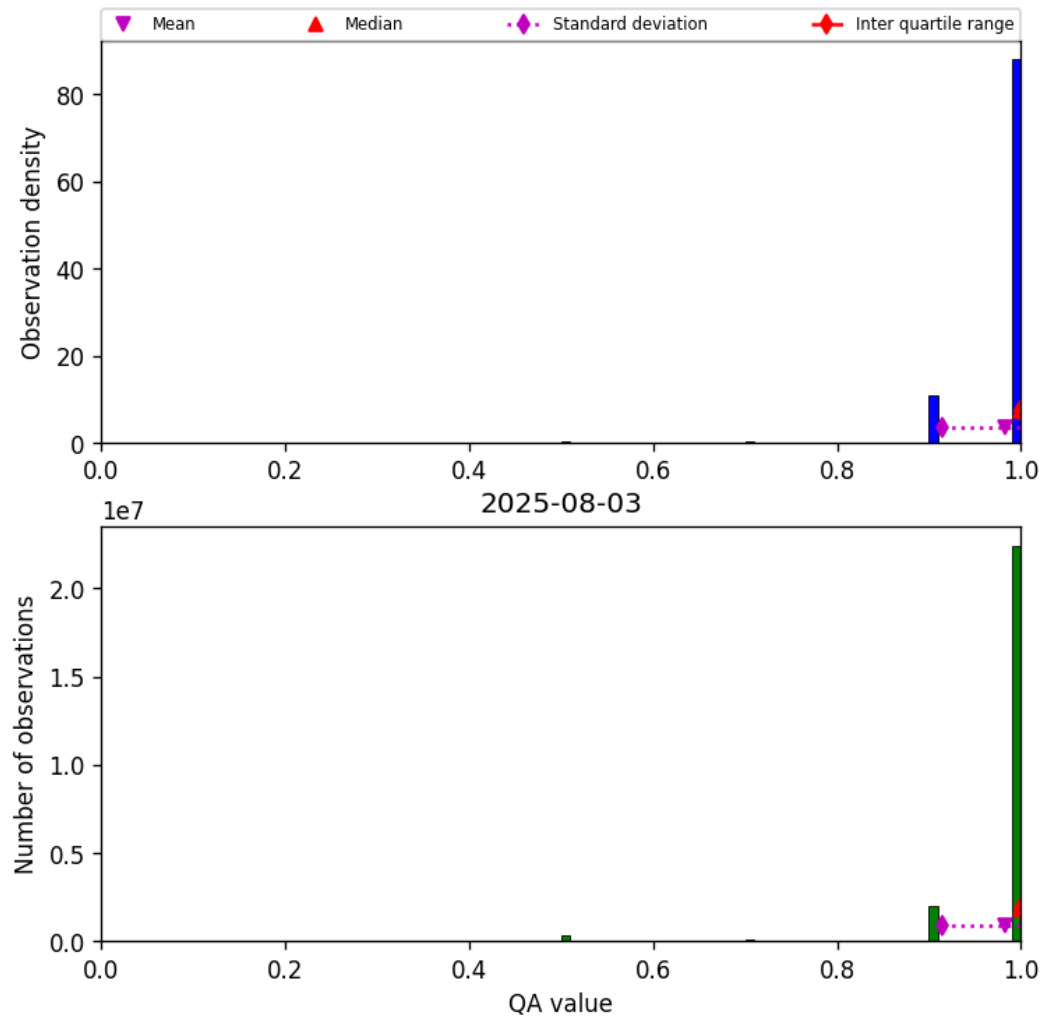
Figure 29: Histogram of “QA value” for 2025-08-03 to 2025-08-04
