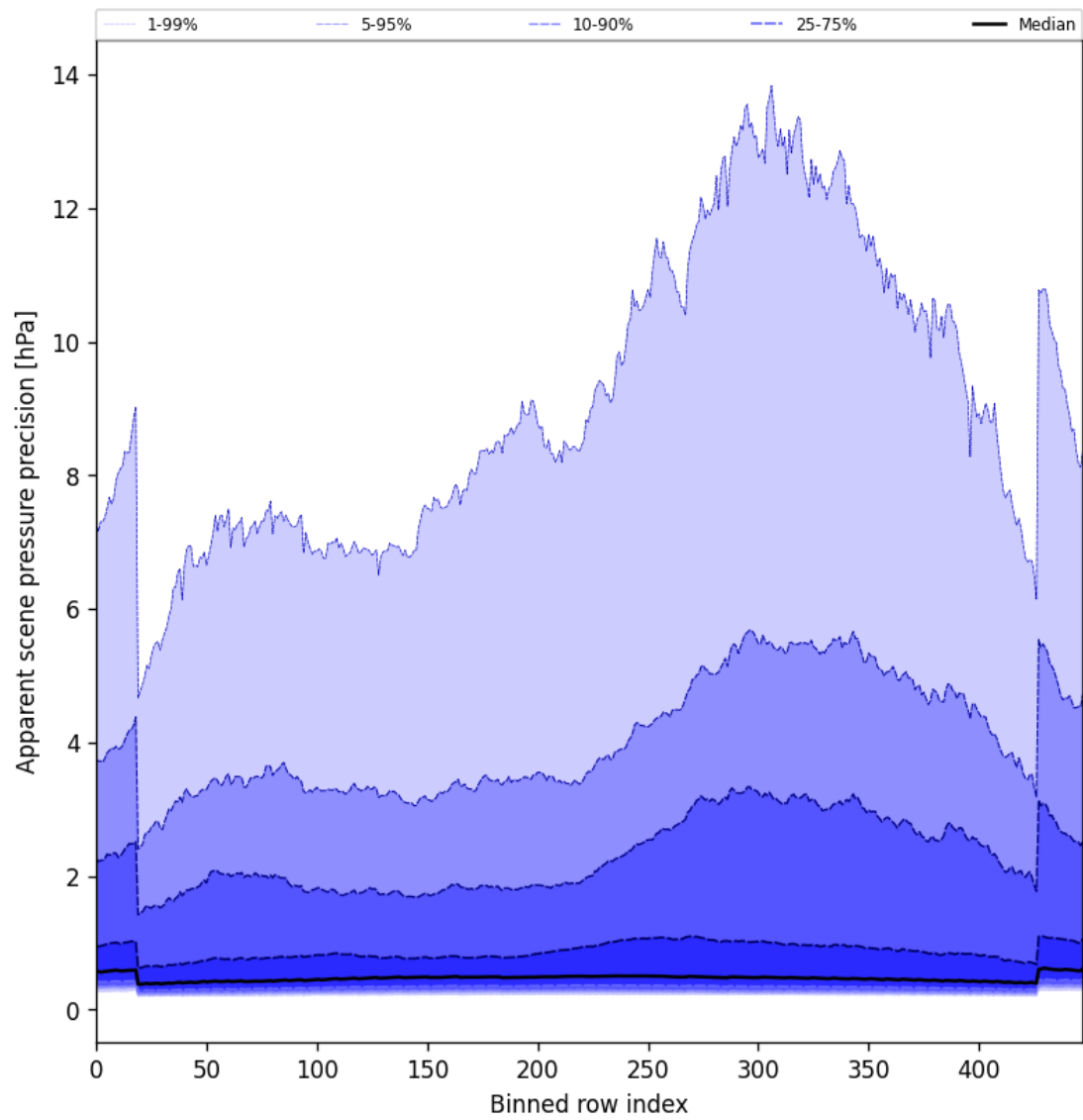
Figure 54: Along track statistics of “Apparent scene pressure precision” for 2025-08-03 to 2025-08-04
