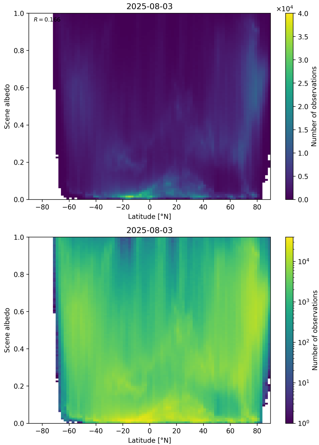
Figure 95: Scatter density plot of “Latitude” against “Scene albedo” for 2025-08-03 to 2025-08-04.
