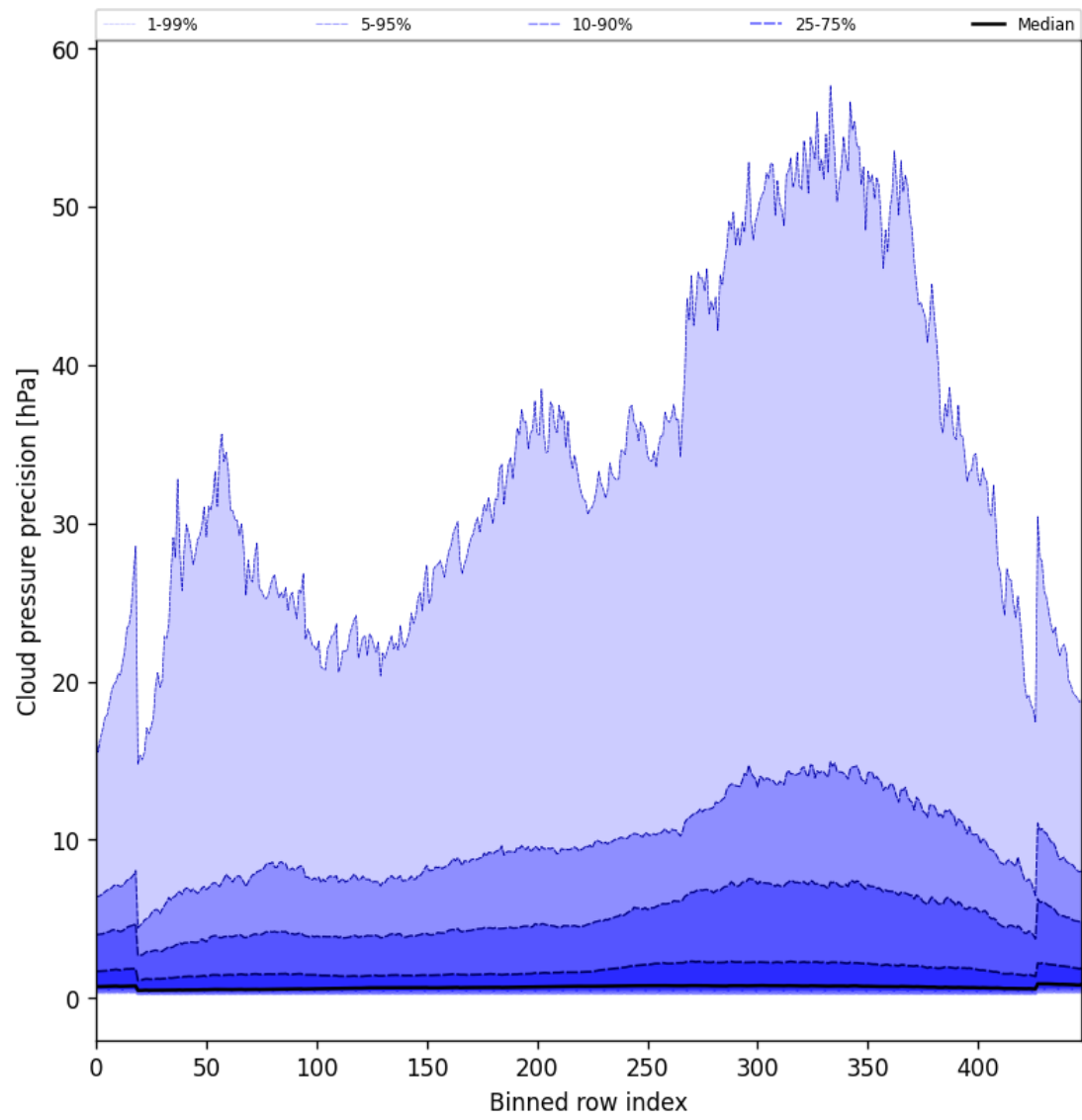
Figure 48: Along track statistics of “Cloud pressure precision” for 2025-08-03 to 2025-08-04
