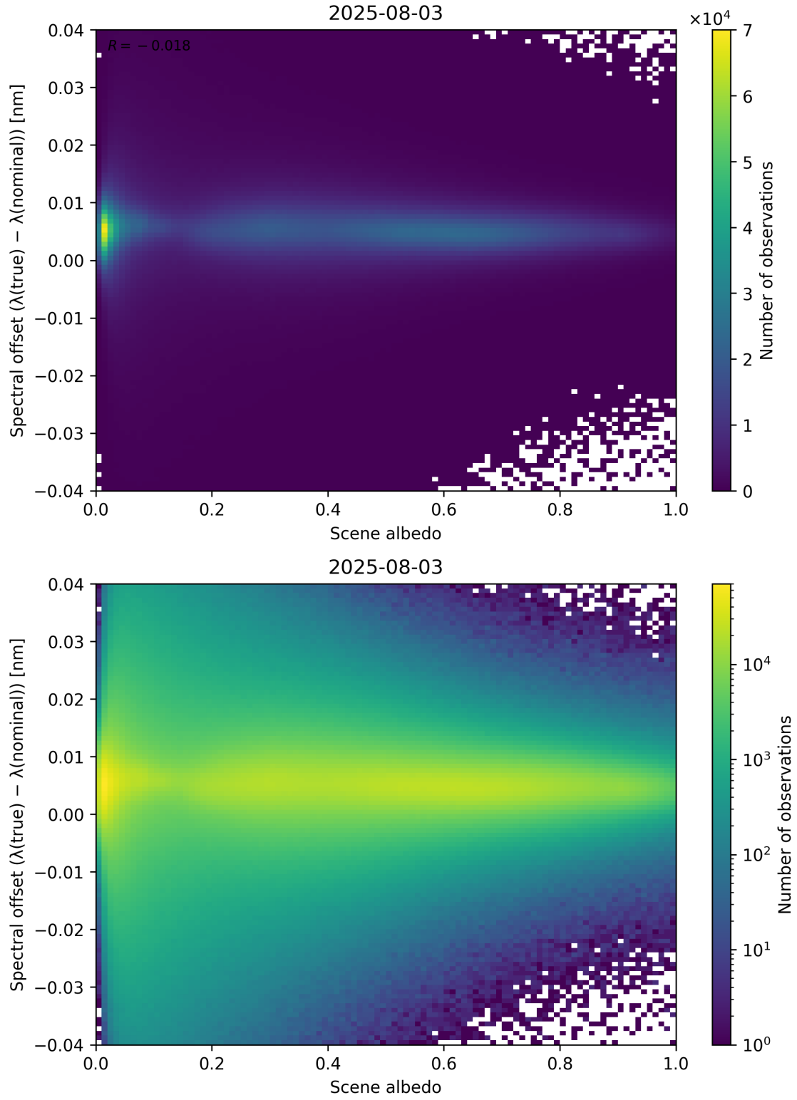
Figure 107: Scatter density plot of “Scene albedo” against “Spectral offset ( \lambda_{\text{true}} - \lambda_{\text{nominal}} )” for 2025-08-03 to 2025-08-04.
