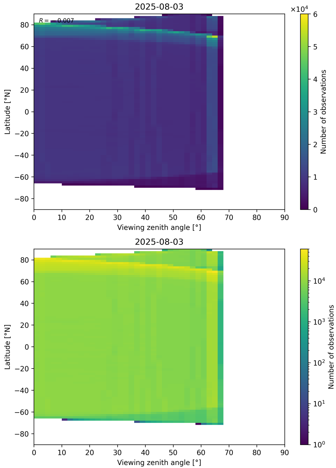
Figure 123: Scatter density plot of “Viewing zenith angle” against “Latitude” for 2025-08-03 to 2025-08-04.
