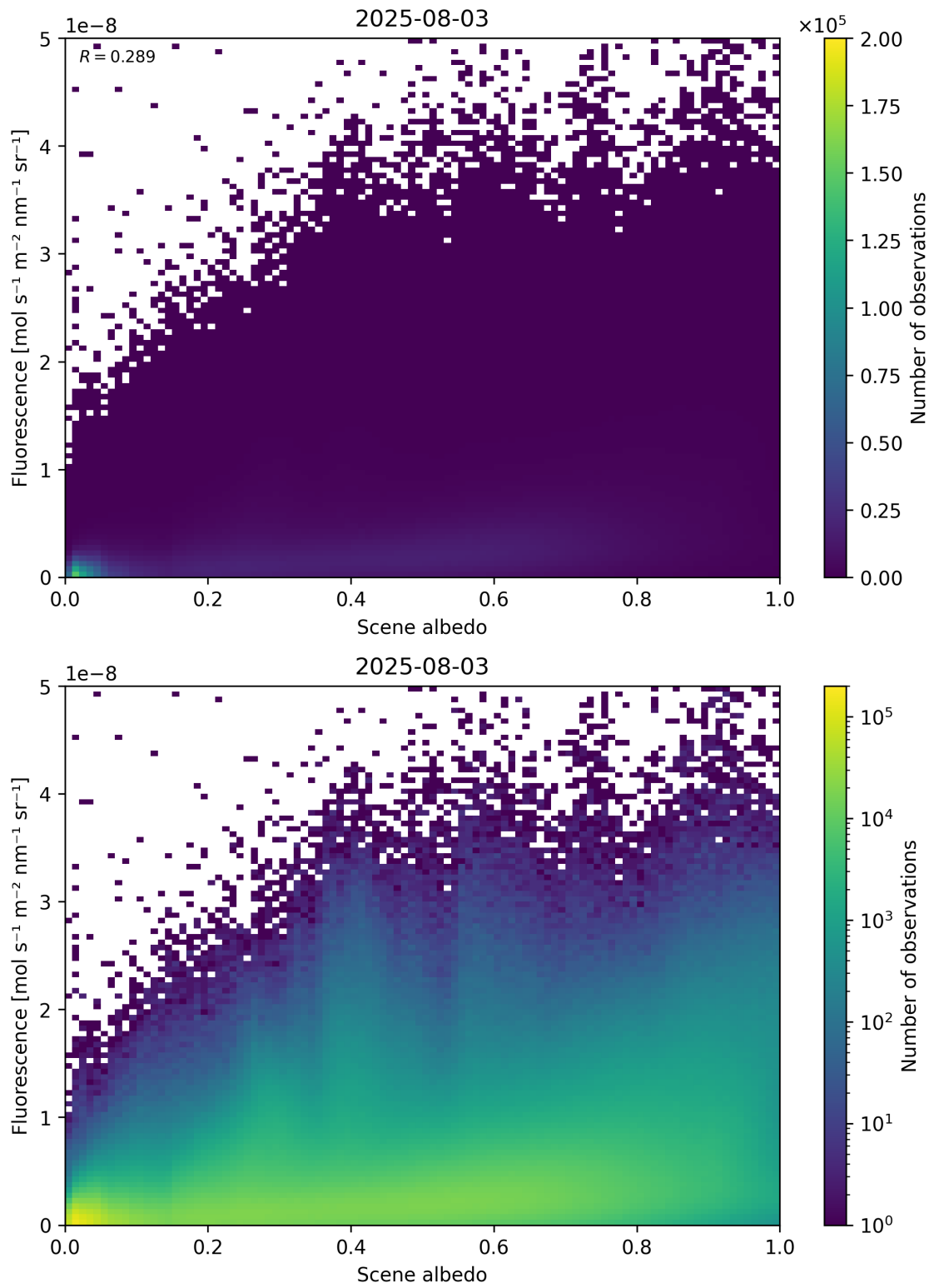
Figure 104: Scatter density plot of “Scene albedo” against “Fluorescence” for 2025-08-03 to 2025-08-04.
