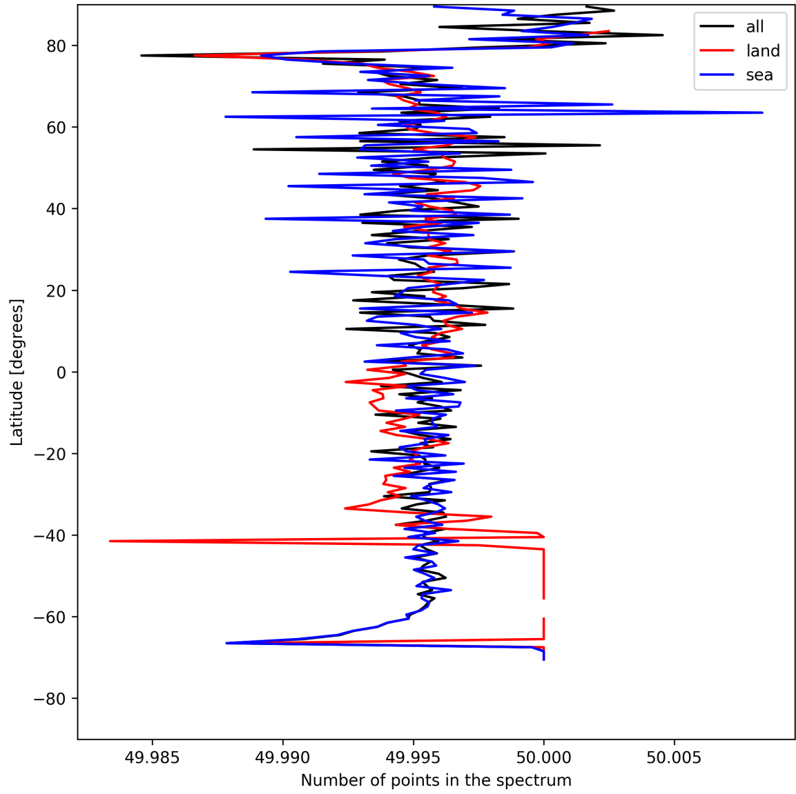
Figure 27: Zonal average of “Number of points in the spectrum” for 2025-08-03 to 2025-08-04.
