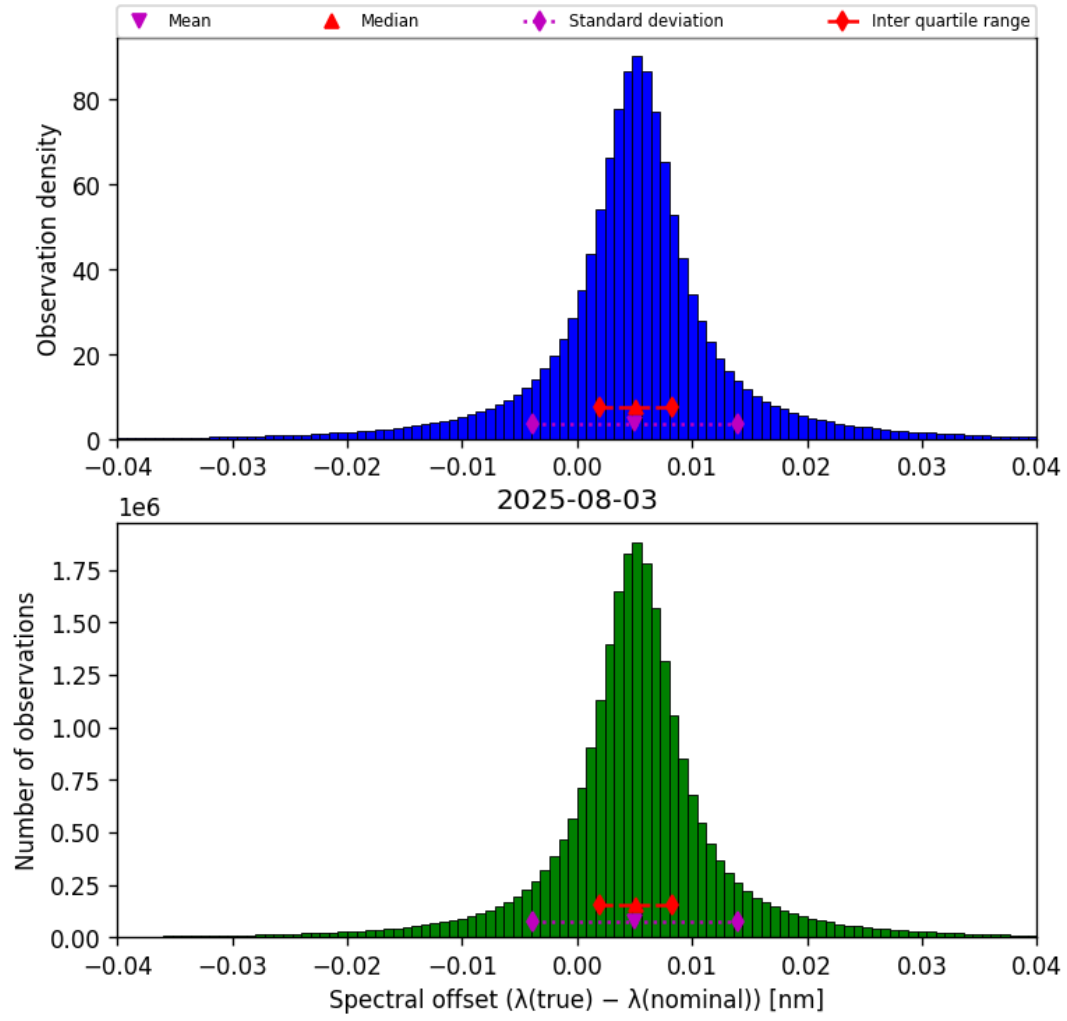
Figure 45: Histogram of “Spectral offset ( \lambda_{\text{true}} - \lambda_{\text{nominal}} )” for 2025-08-03 to 2025-08-04
