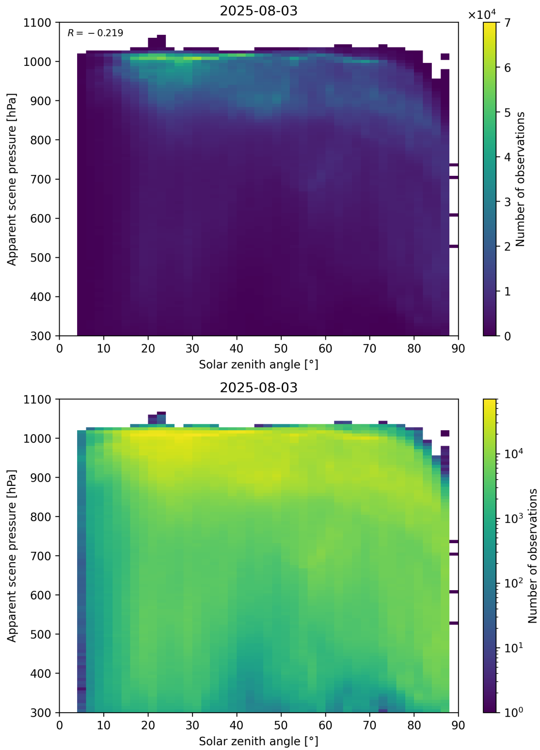
Figure 108: Scatter density plot of “Solar zenith angle” against “Apparent scene pressure” for 2025-08-03 to 2025-08-04.
