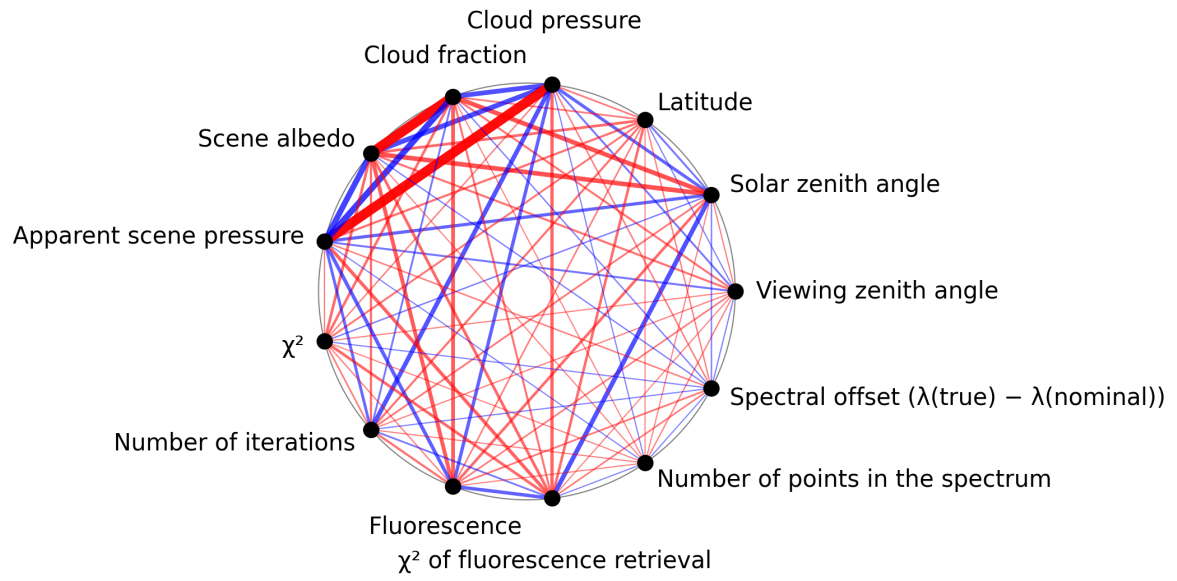
Figure 1: Map of correlation graph for 2025-08-03 to 2025-08-04.
