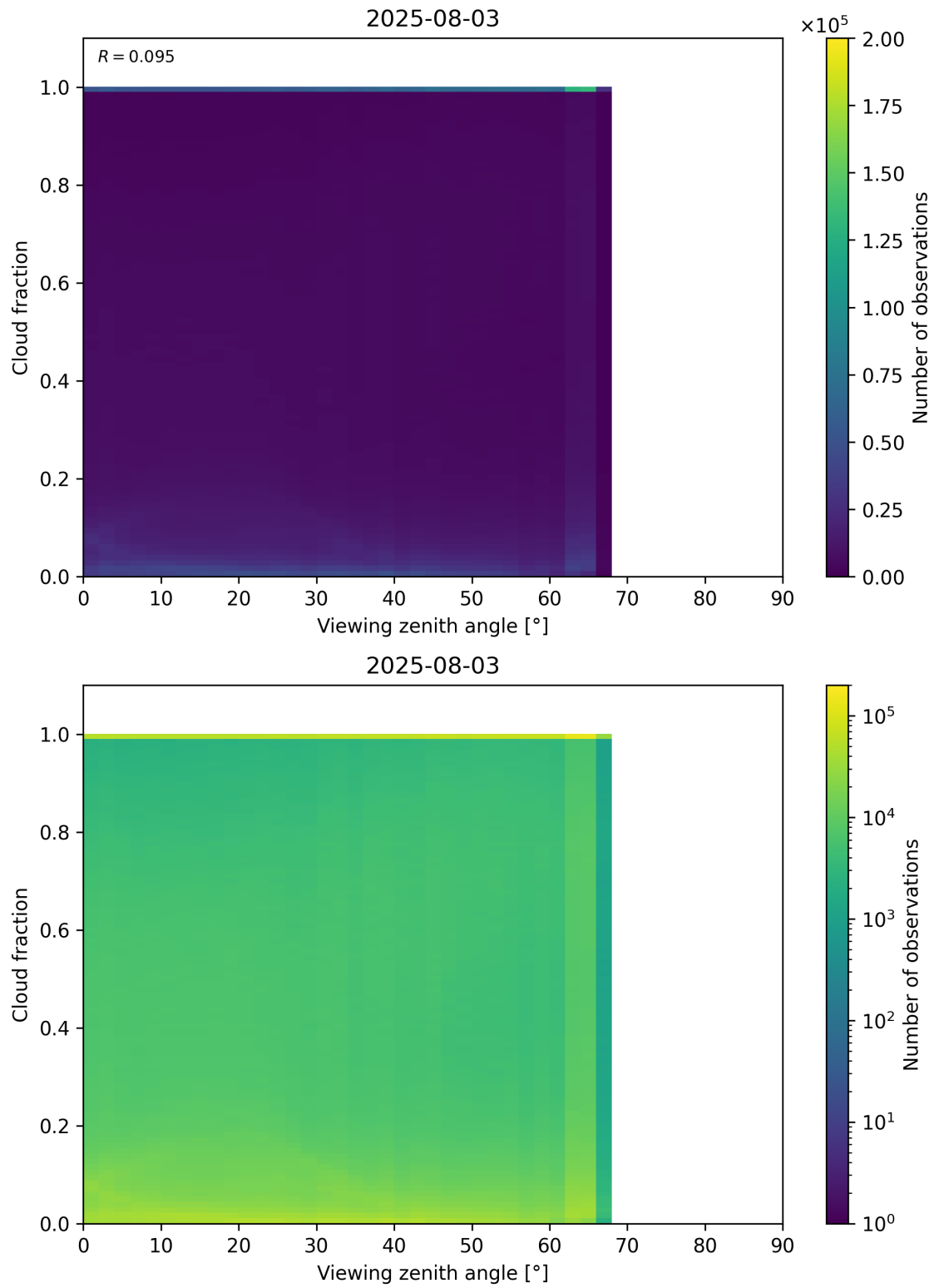
Figure 120: Scatter density plot of “Viewing zenith angle” against “Cloud fraction” for 2025-08-03 to 2025-08-04.
