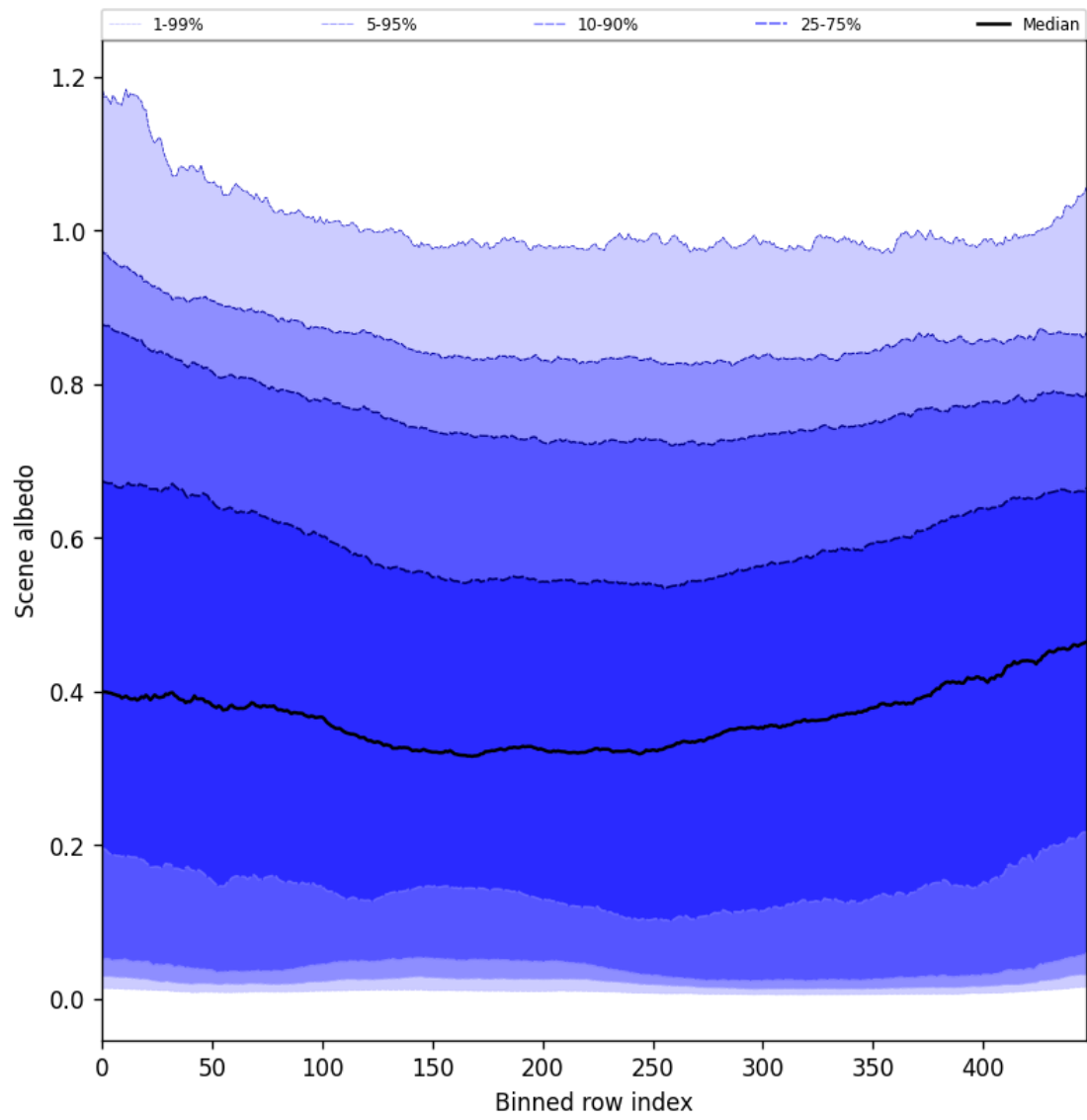
Figure 51: Along track statistics of “Scene albedo” for 2025-08-03 to 2025-08-04
