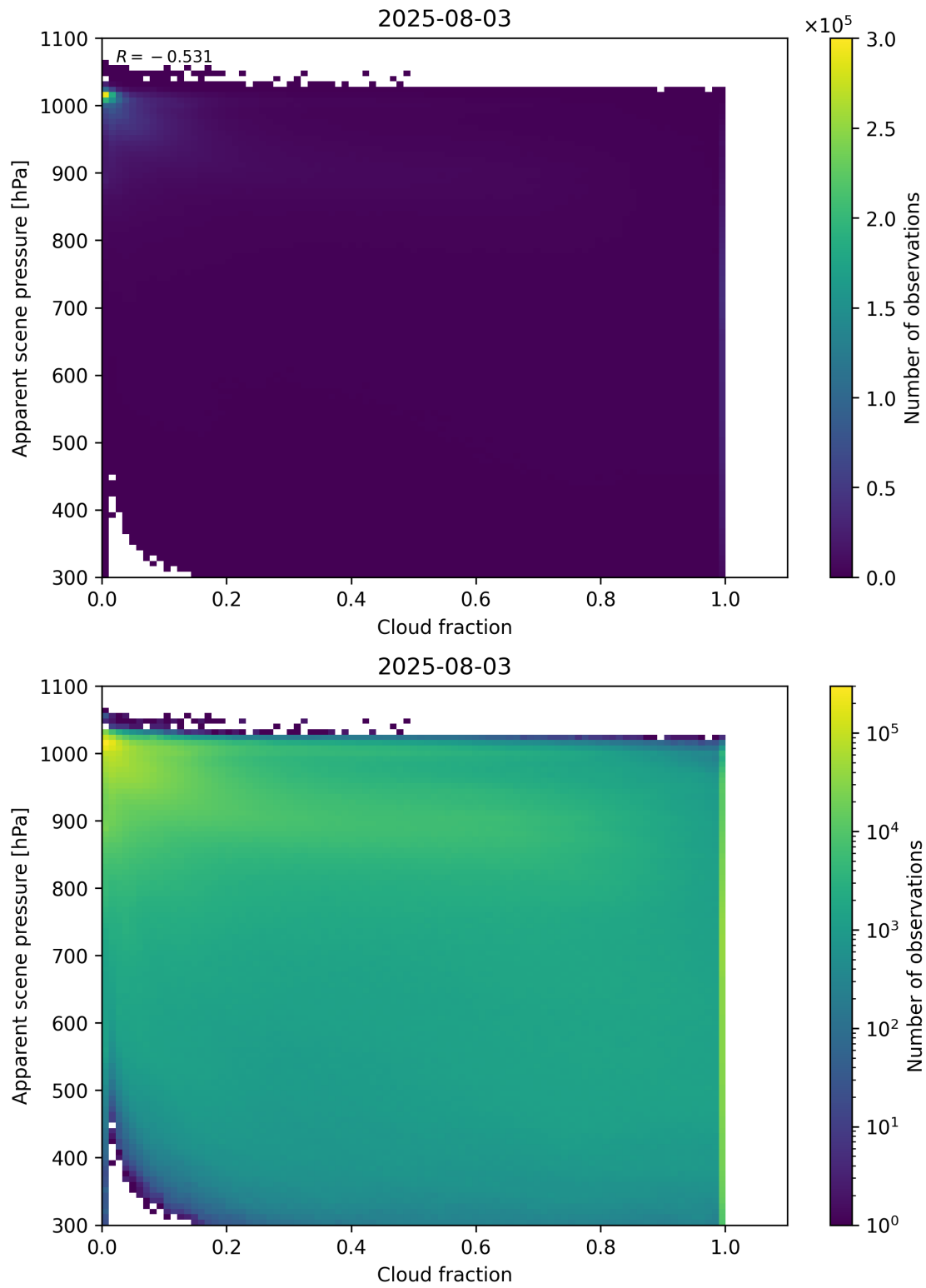
Figure 70: Scatter density plot of “Cloud fraction” against “Apparent scene pressure” for 2025-08-03 to 2025-08-04.
