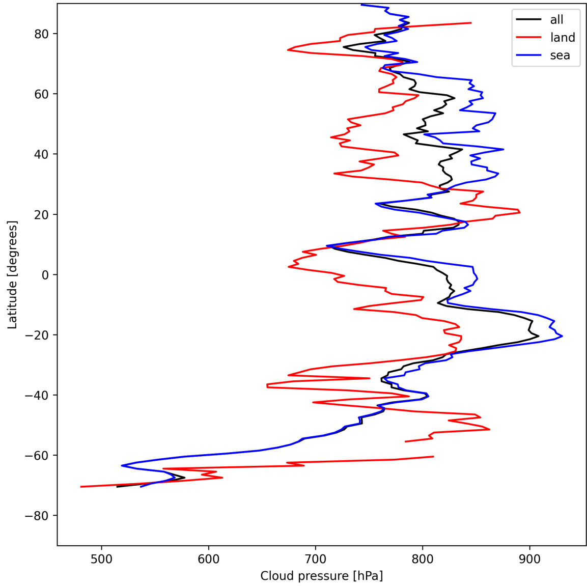
Figure 13: Zonal average of “Cloud pressure” for 2025-08-03 to 2025-08-04.
