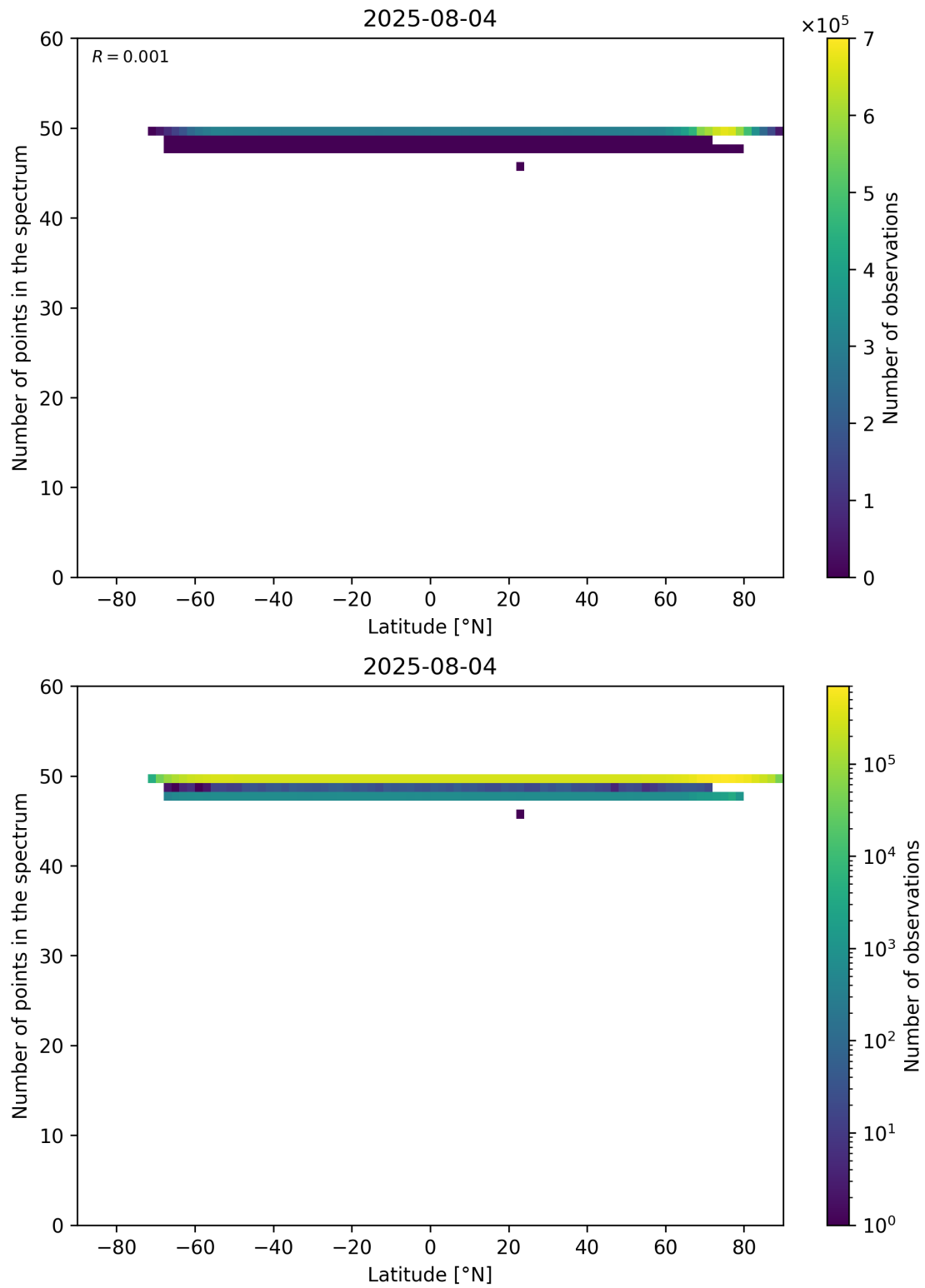
Figure 94: Scatter density plot of “Latitude” against “Number of points in the spectrum” for 2025-08-04 to 2025-08-05.
