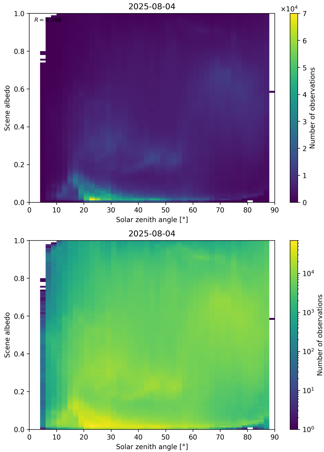
Figure 116: Scatter density plot of “Solar zenith angle” against “Scene albedo” for 2025-08-04 to 2025-08-05.
