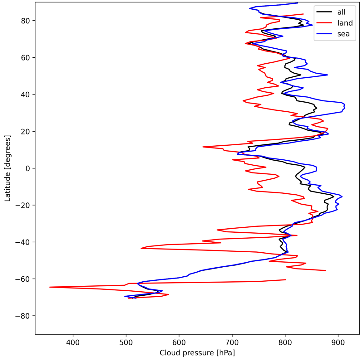
Figure 13: Zonal average of “Cloud pressure” for 2025-08-04 to 2025-08-05.
