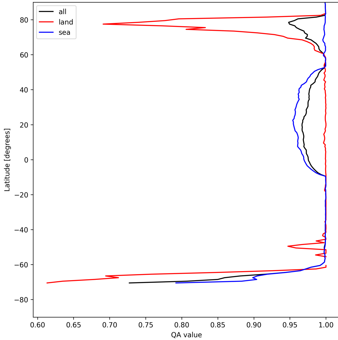
Figure 12: Zonal average of “QA value” for 2025-08-04 to 2025-08-05.
