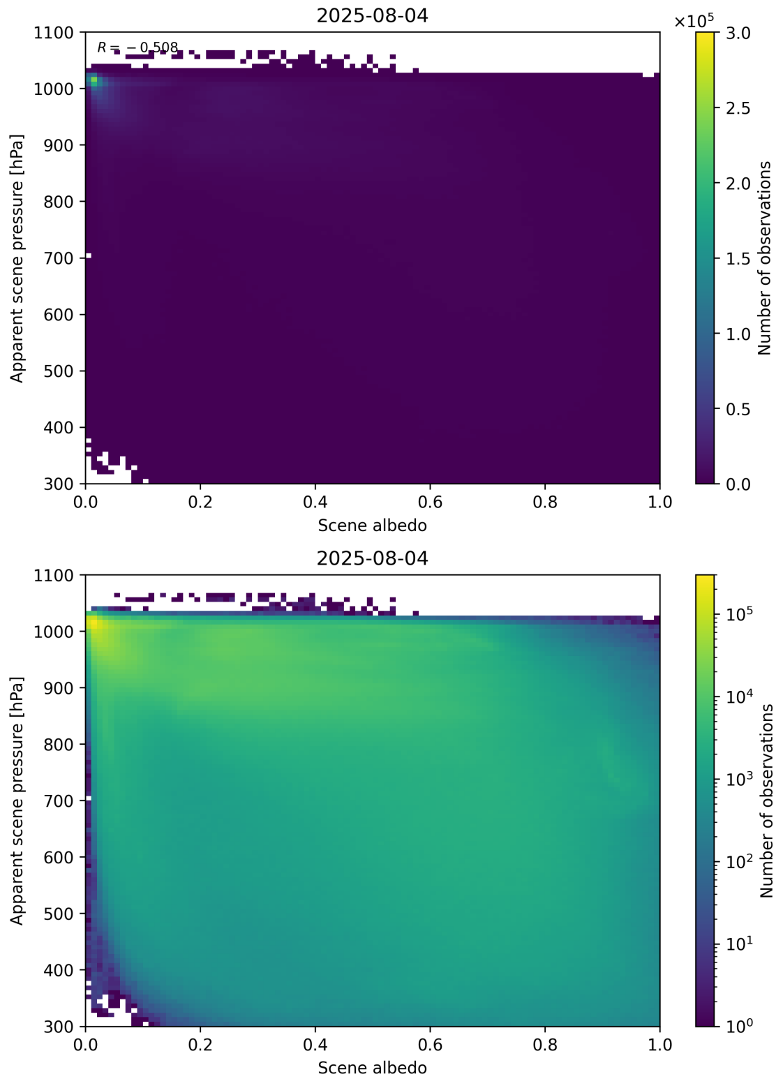
Figure 102: Scatter density plot of “Scene albedo” against “Apparent scene pressure” for 2025-08-04 to 2025-08-05.
