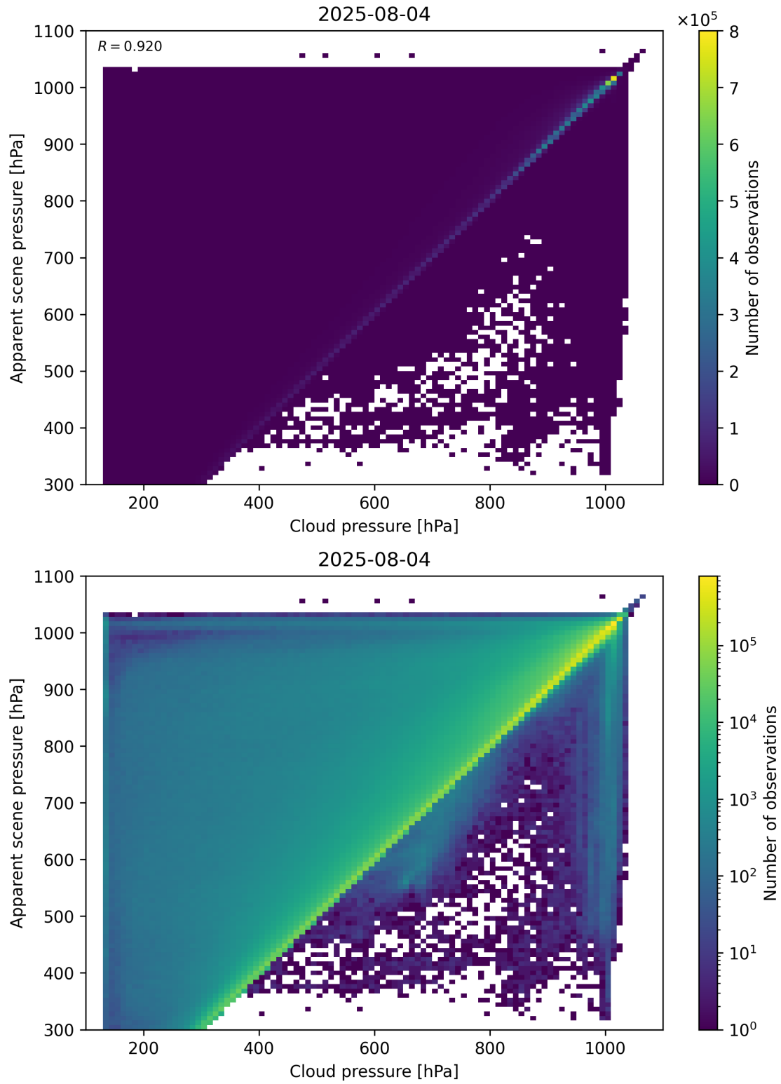
Figure 77: Scatter density plot of “Cloud pressure” against “Apparent scene pressure” for 2025-08-04 to 2025-08-05.
