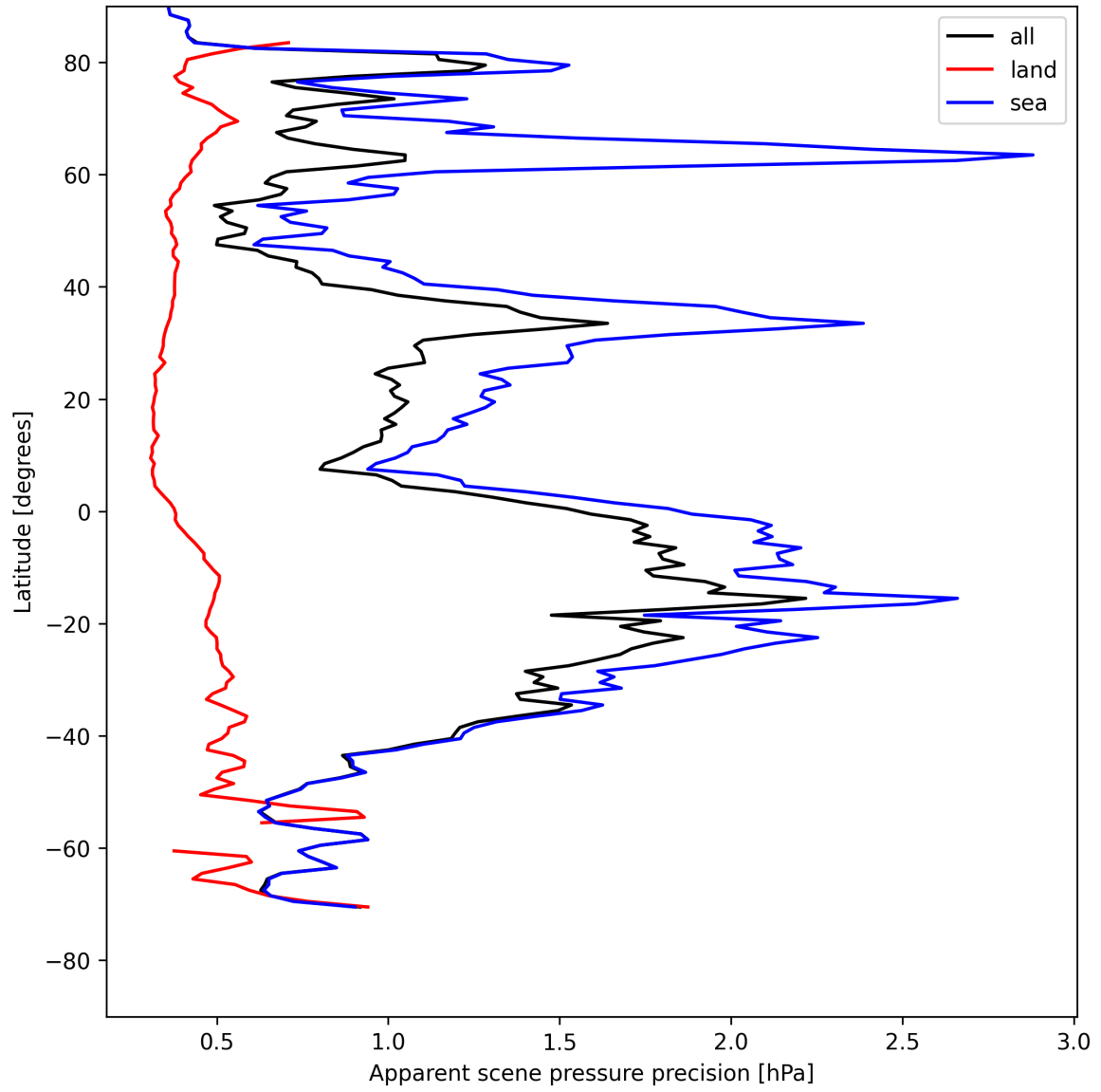
Figure 20: Zonal average of “Apparent scene pressure precision” for 2025-08-04 to 2025-08-05.
