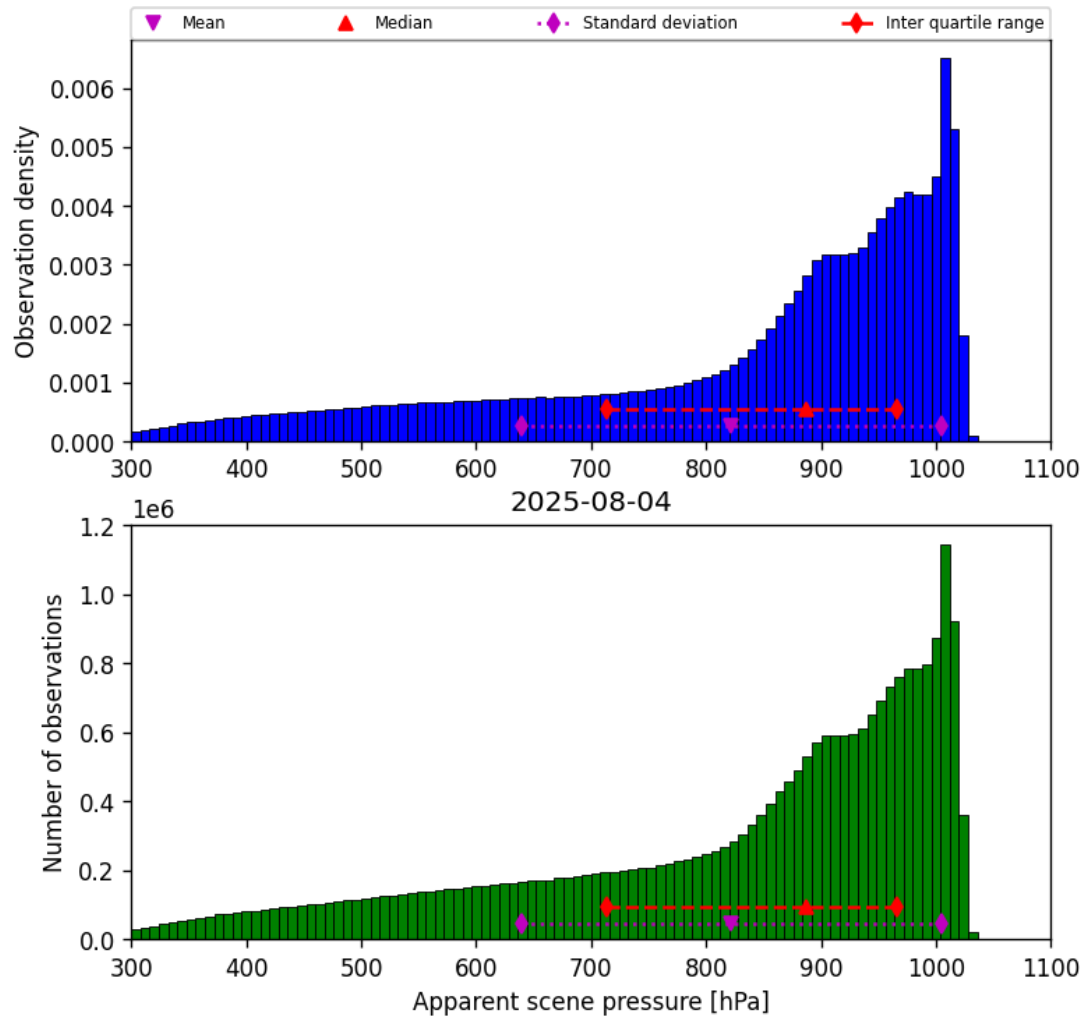
Figure 36: Histogram of “Apparent scene pressure” for 2025-08-04 to 2025-08-05
