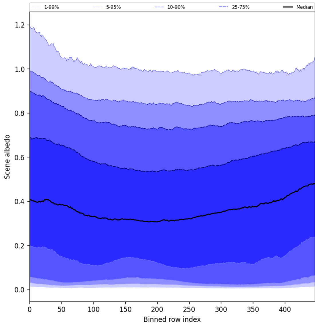
Figure 51: Along track statistics of “Scene albedo” for 2025-08-04 to 2025-08-05
