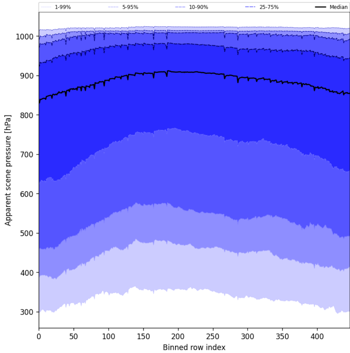
Figure 53: Along track statistics of “Apparent scene pressure” for 2025-08-04 to 2025-08-05
