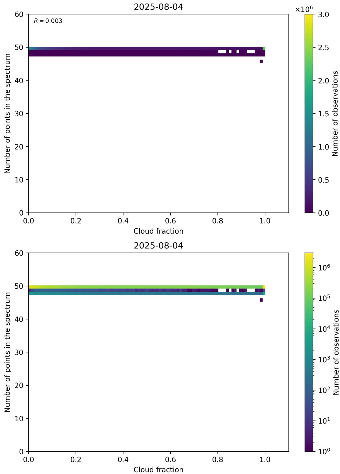
Figure 74: Scatter density plot of “Cloud fraction” against “Number of points in the spectrum” for 2025-08-04 to 2025-08-05.
