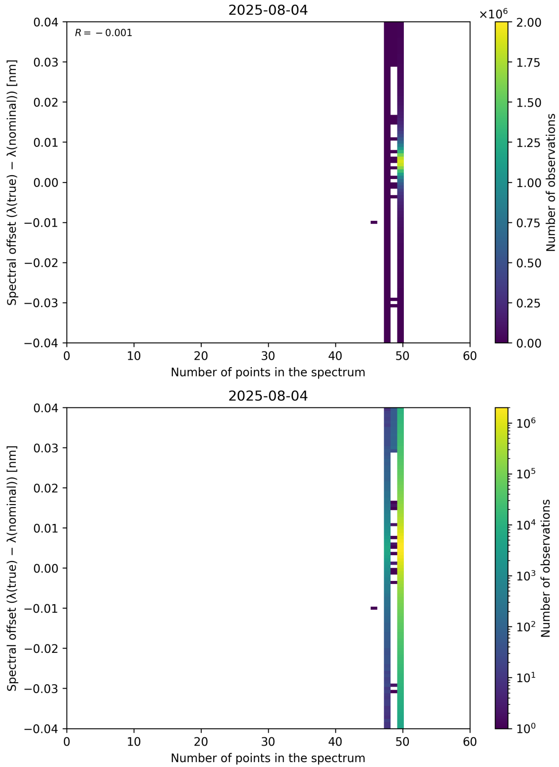
Figure 101: Scatter density plot of “Number of points in the spectrum” against “Spectral offset ( \lambda_{\text{true}} - \lambda_{\text{nominal}} )” for 2025-08-04 to 2025-08-05.
