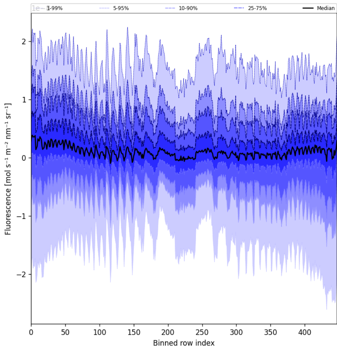
Figure 57: Along track statistics of "Fluorescence" for 2025-08-04 to 2025-08-05
