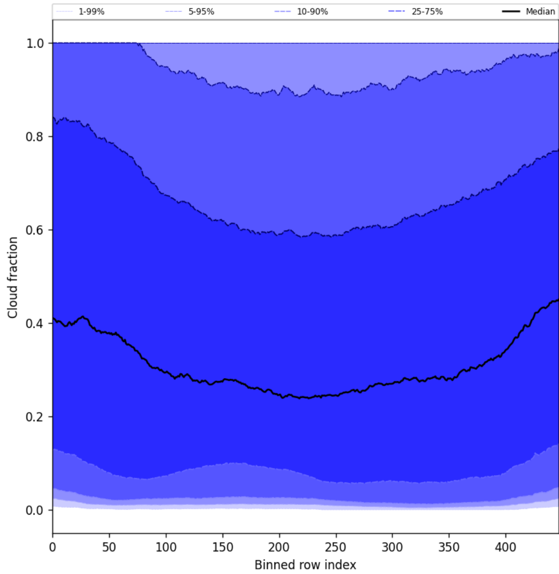
Figure 49: Along track statistics of “Cloud fraction” for 2025-08-04 to 2025-08-05
