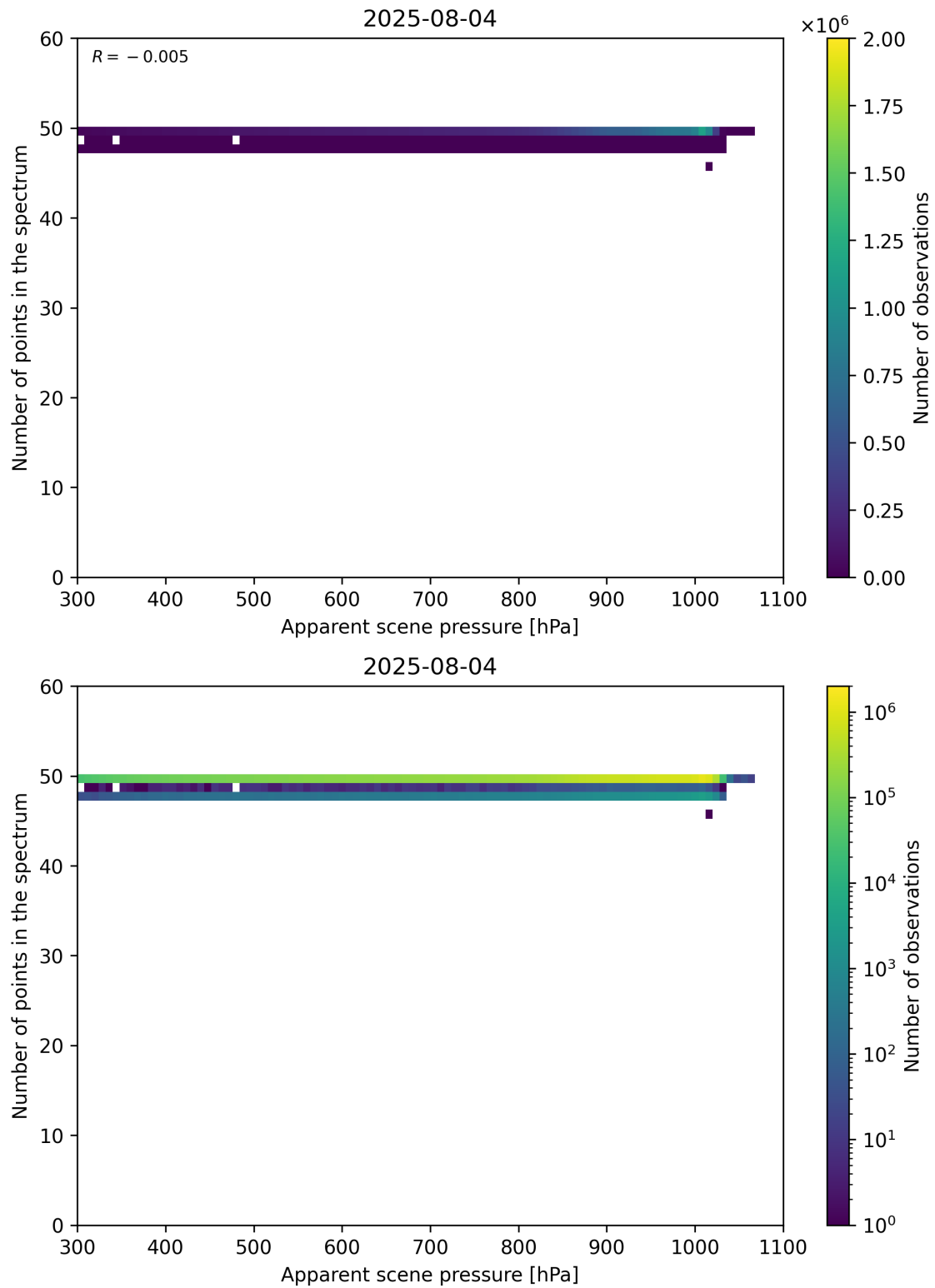
Figure 66: Scatter density plot of “Apparent scene pressure” against “Number of points in the spectrum” for 2025-08-04 to 2025-08-05.
