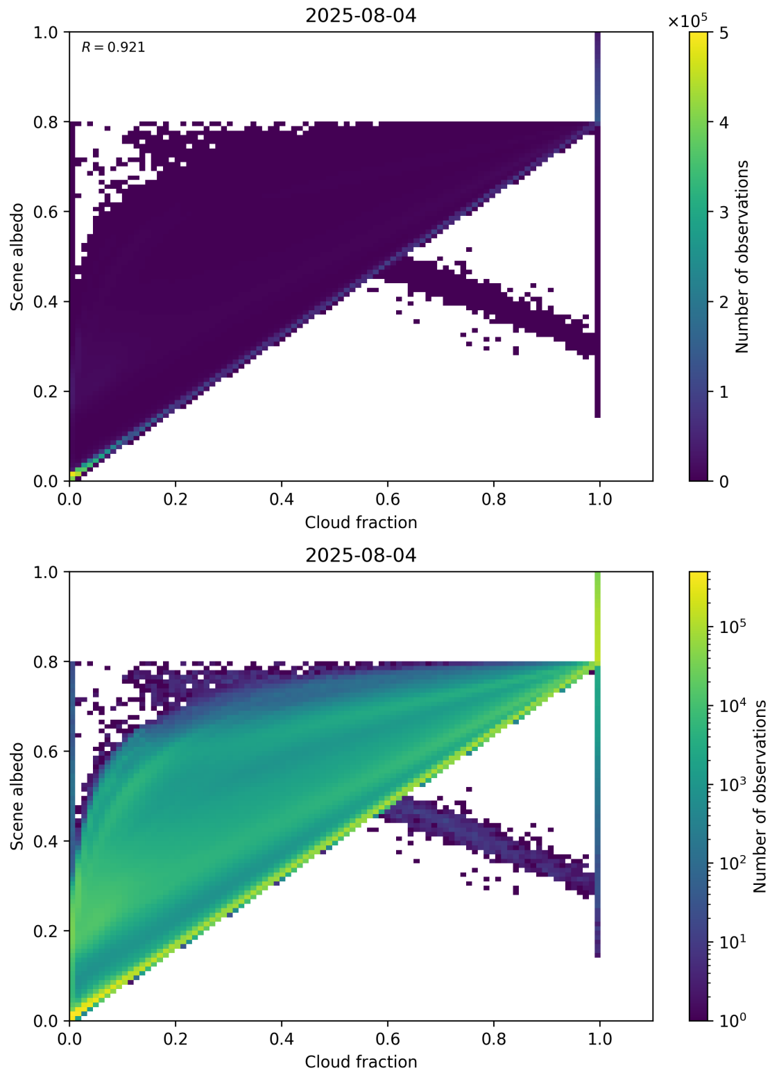
Figure 75: Scatter density plot of “Cloud fraction” against “Scene albedo” for 2025-08-04 to 2025-08-05.
