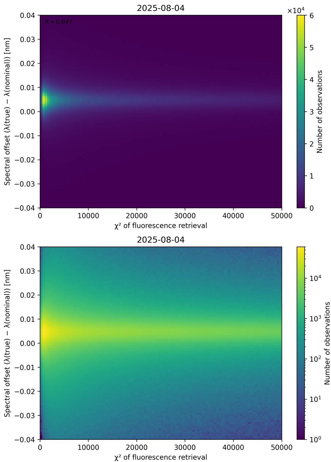
Figure 69: Scatter density plot of “ \chi^2 of fluorescence retrieval” against “Spectral offset ( \lambda_{\text{true}} - \lambda_{\text{nominal}} )” for 2025-08-04 to 2025-08-05.
