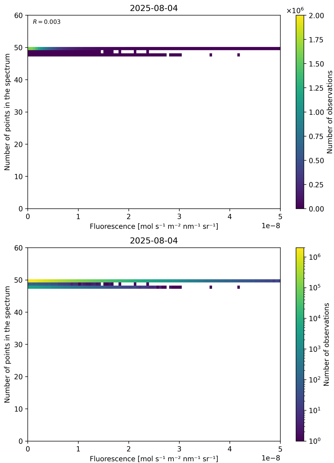
Figure 86: Scatter density plot of “Fluorescence” against “Number of points in the spectrum” for 2025-08-04 to 2025-08-05.
