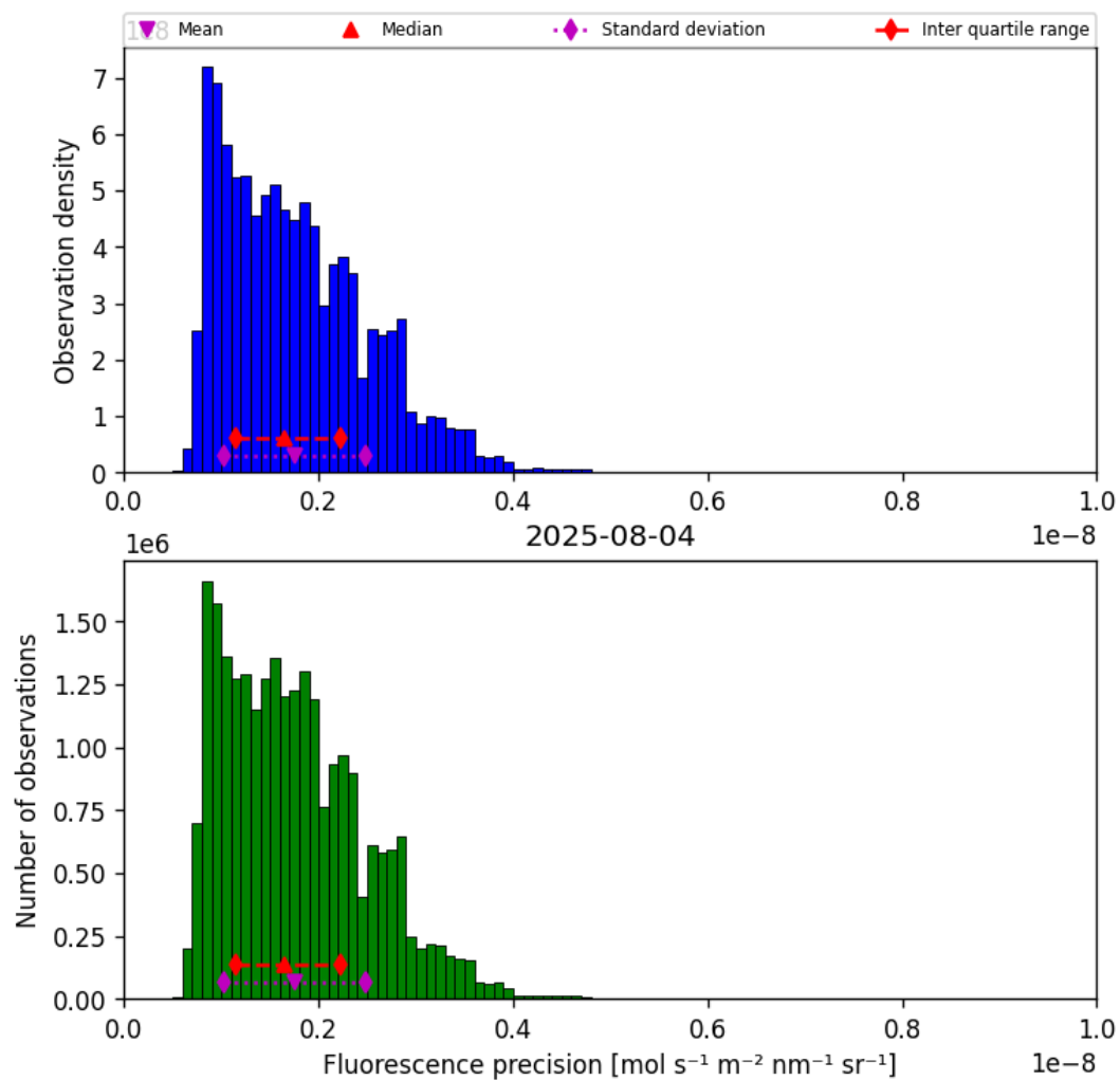
Figure 41: Histogram of “Fluorescence precision” for 2025-08-04 to 2025-08-05
