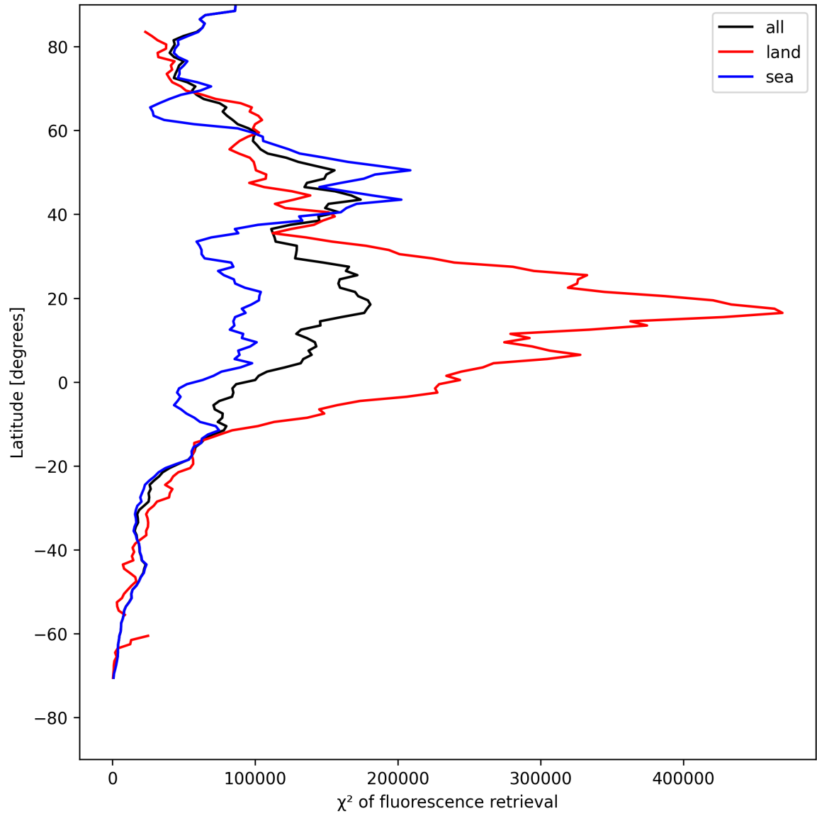
Figure 25: Zonal average of “ \chi^2 of fluorescence retrieval” for 2025-08-04 to 2025-08-05.
