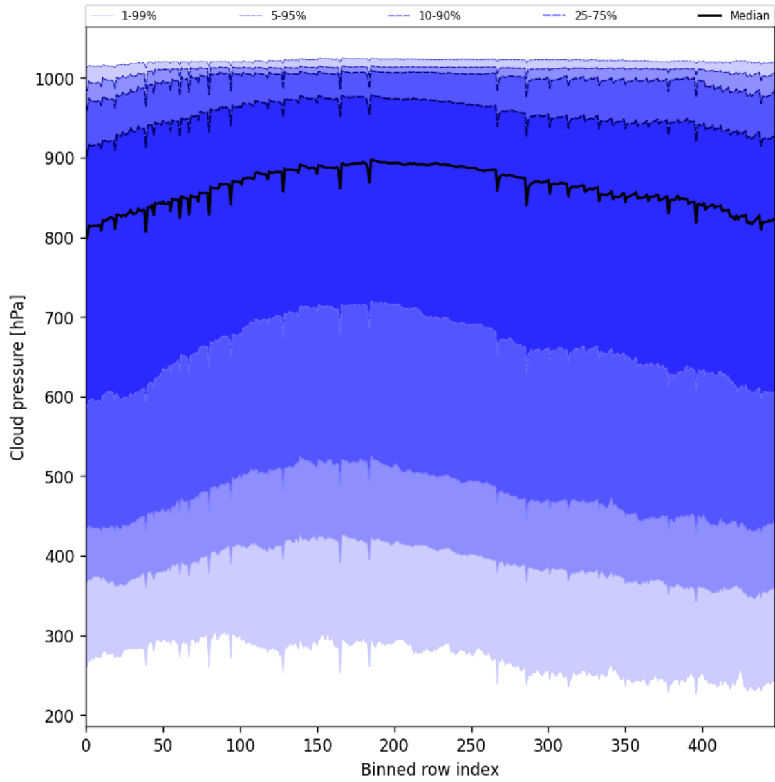
Figure 47: Along track statistics of “Cloud pressure” for 2025-08-04 to 2025-08-05
