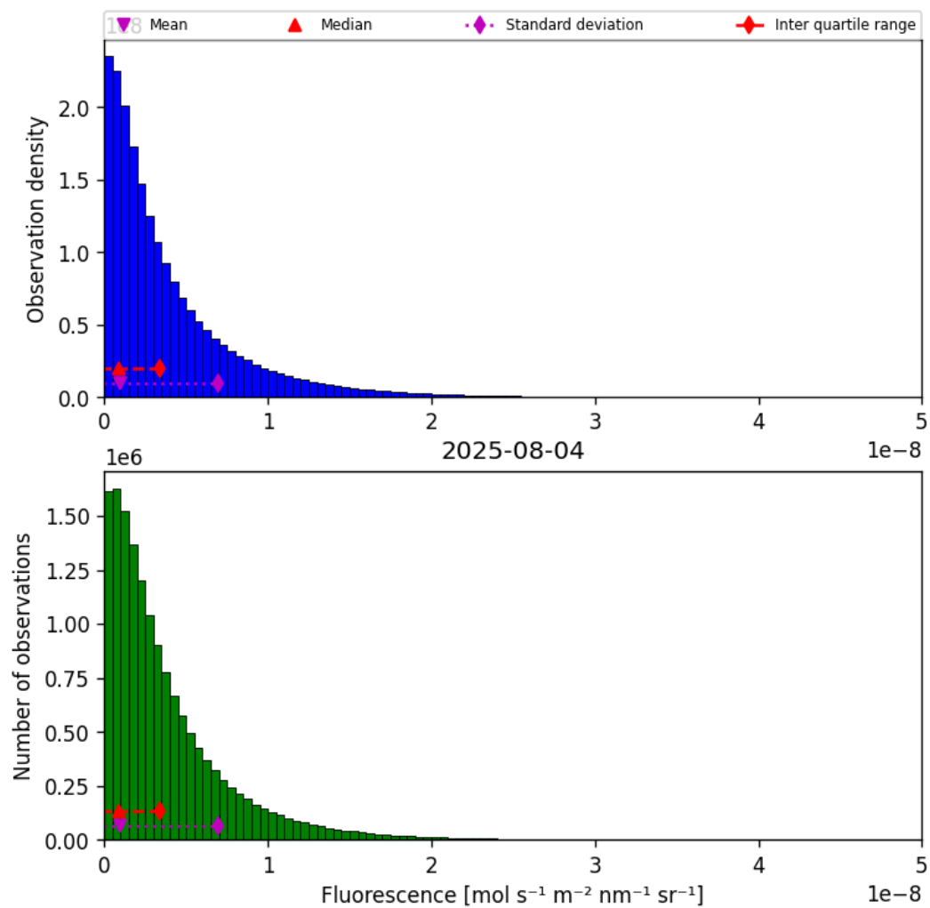
Figure 40: Histogram of “Fluorescence” for 2025-08-04 to 2025-08-05
