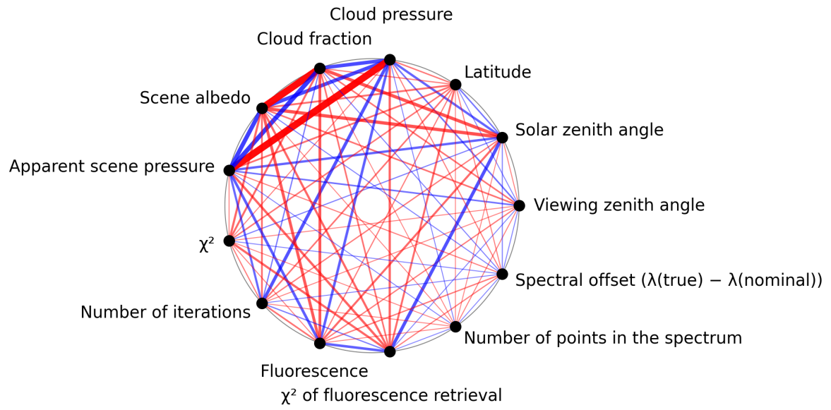
Figure 1: Map of correlation graph for 2025-08-04 to 2025-08-05.
