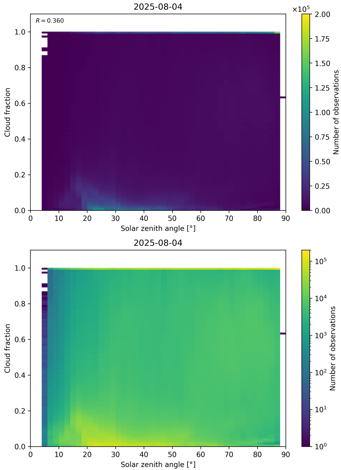
Figure 110: Scatter density plot of “Solar zenith angle” against “Cloud fraction” for 2025-08-04 to 2025-08-05.
