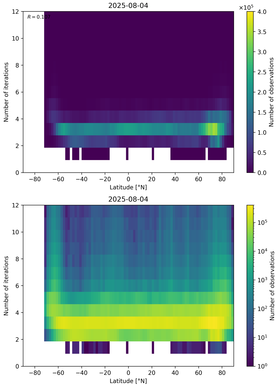
Figure 93: Scatter density plot of “Latitude” against “Number of iterations” for 2025-08-04 to 2025-08-05.
