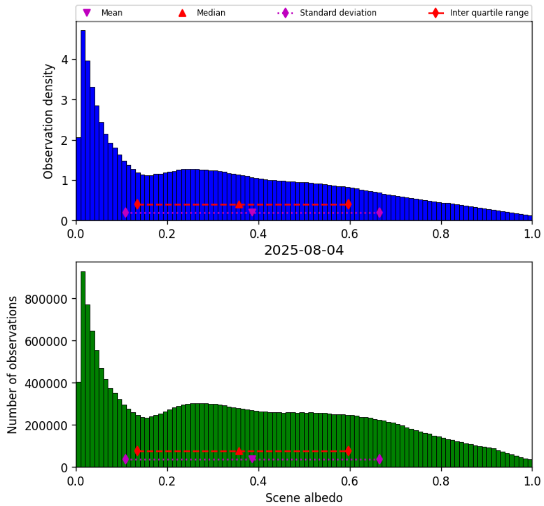
Figure 34: Histogram of “Scene albedo” for 2025-08-04 to 2025-08-05
