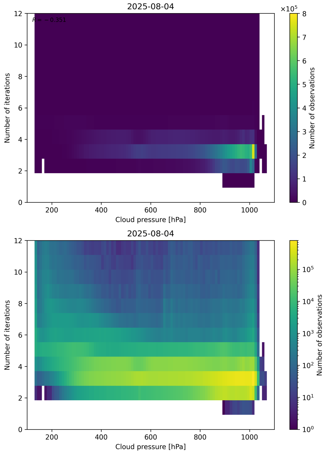
Figure 81: Scatter density plot of “Cloud pressure” against “Number of iterations” for 2025-08-04 to 2025-08-05.
