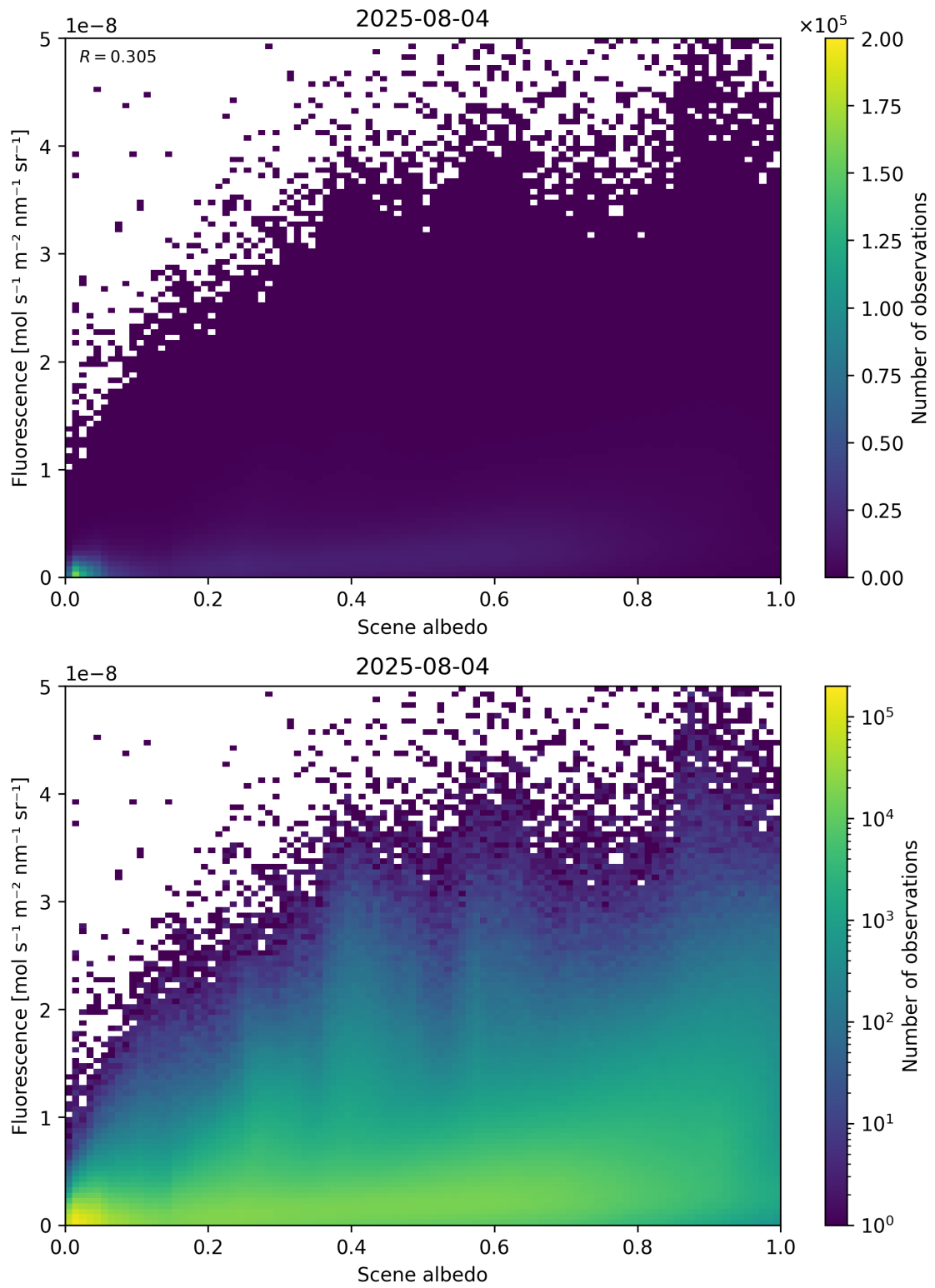
Figure 104: Scatter density plot of “Scene albedo” against “Fluorescence” for 2025-08-04 to 2025-08-05.
