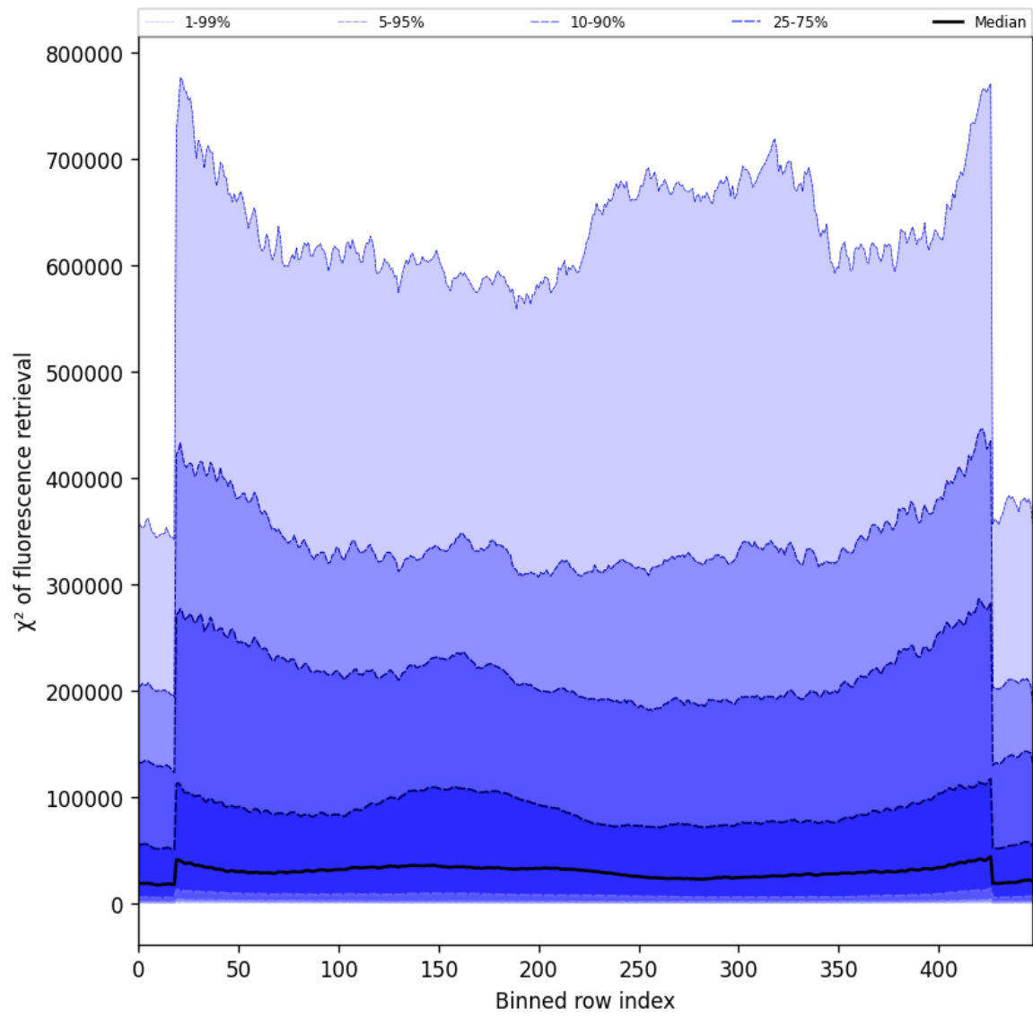
Figure 59: Along track statistics of “ \chi^2 of fluorescence retrieval” for 2025-08-04 to 2025-08-05
