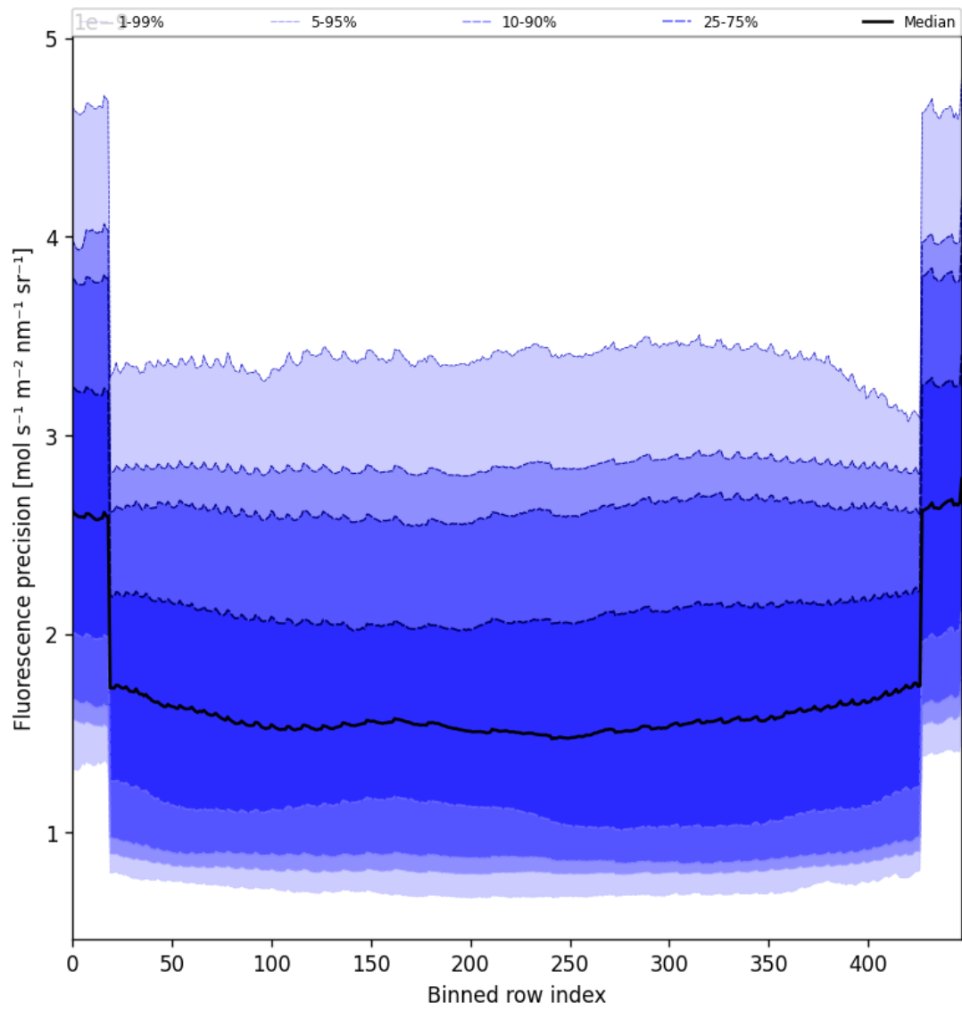
Figure 58: Along track statistics of “Fluorescence precision” for 2025-08-04 to 2025-08-05
