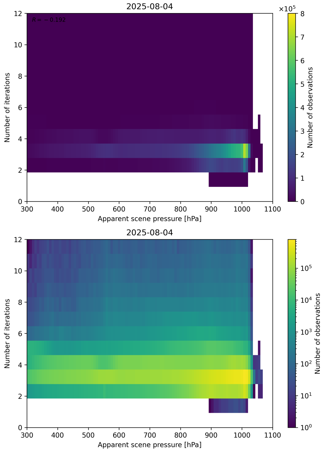
Figure 65: Scatter density plot of “Apparent scene pressure” against “Number of iterations” for 2025-08-04 to 2025-08-05.
