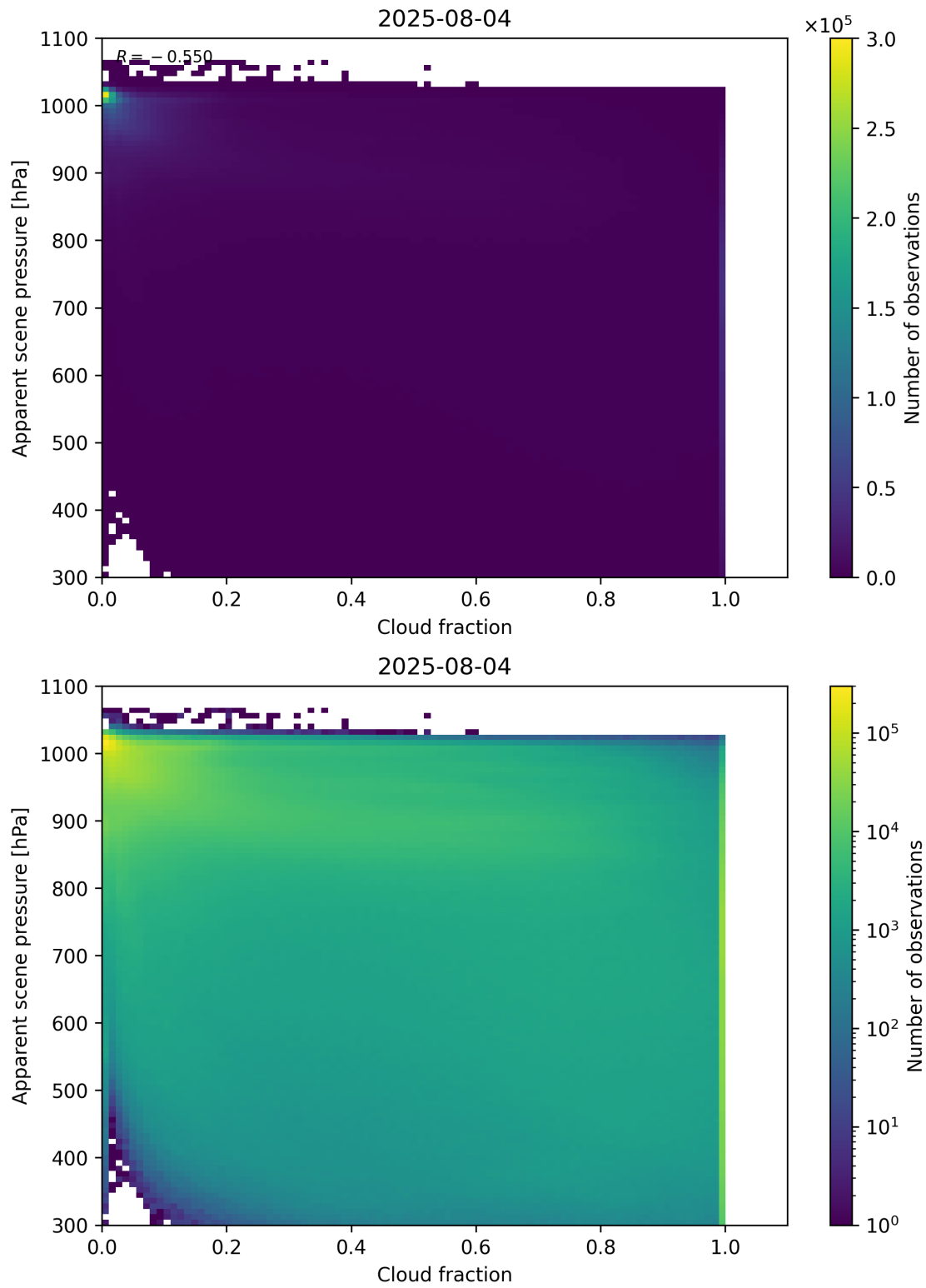
Figure 70: Scatter density plot of “Cloud fraction” against “Apparent scene pressure” for 2025-08-04 to 2025-08-05.
