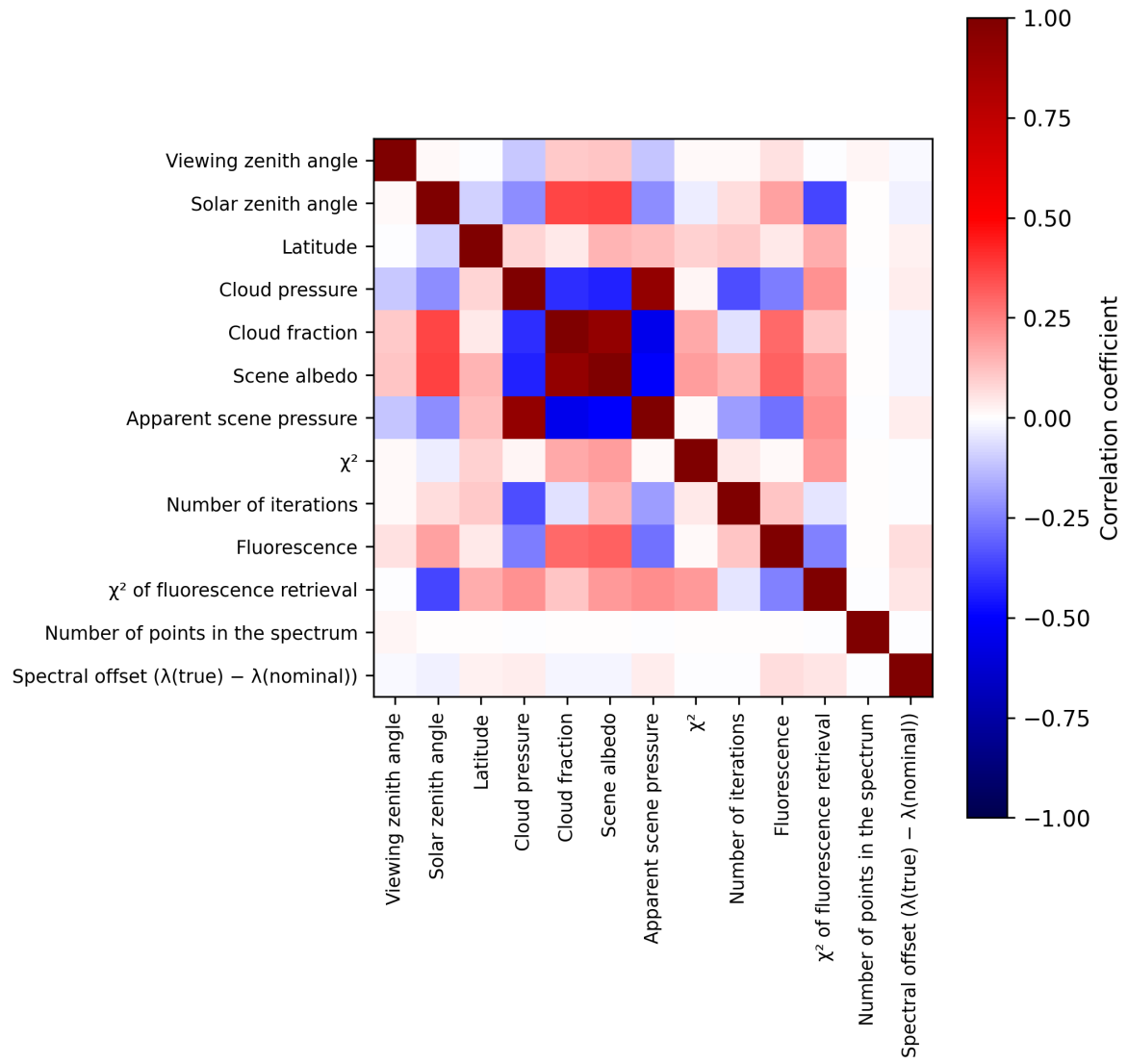
Figure 2: Map of correlation matrix for 2025-08-04 to 2025-08-05.
