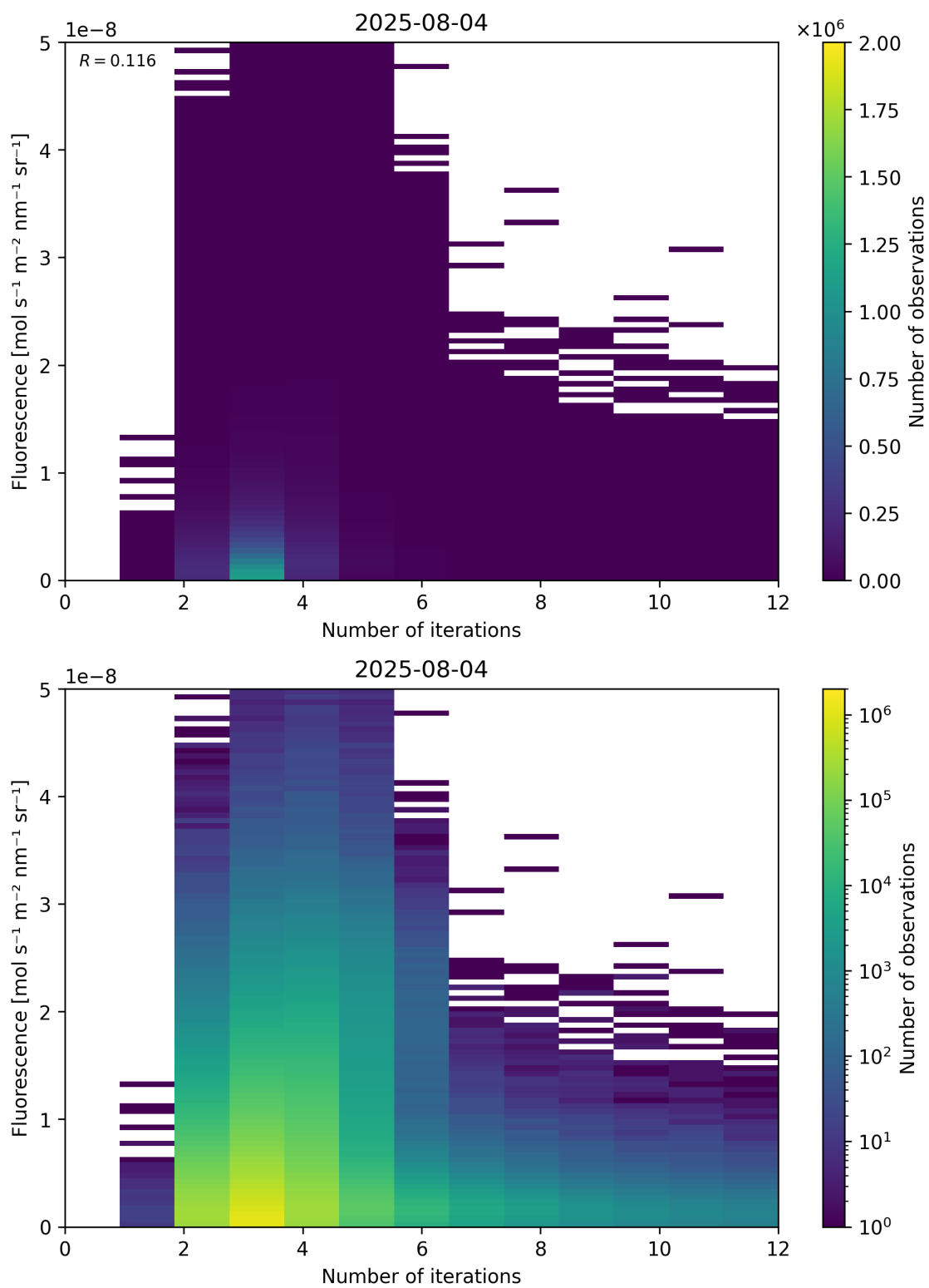
Figure 98: Scatter density plot of “Number of iterations” against “Fluorescence” for 2025-08-04 to 2025-08-05.
