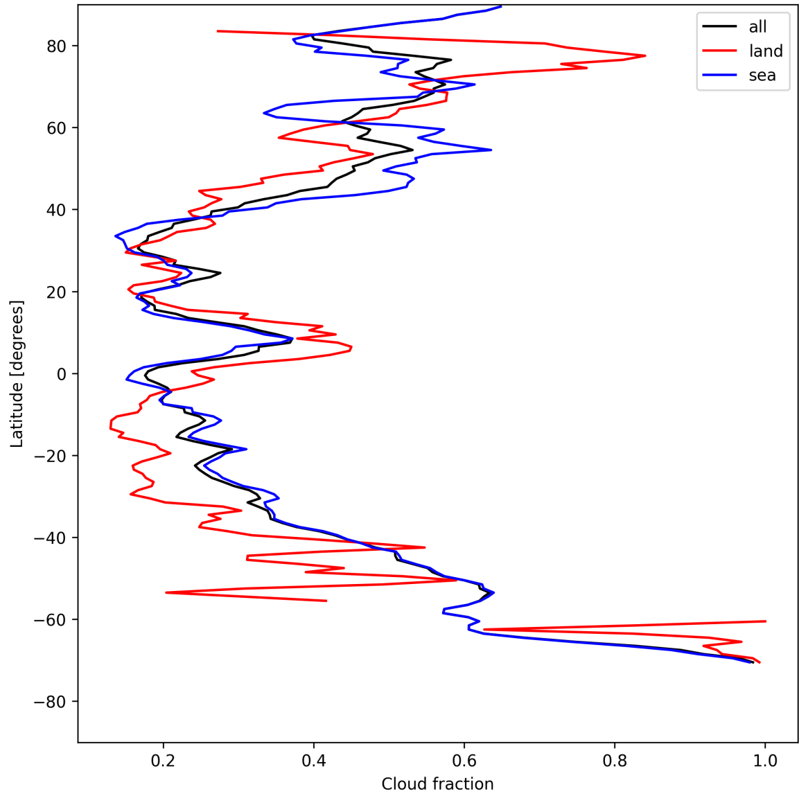
Figure 15: Zonal average of “Cloud fraction” for 2025-08-04 to 2025-08-05.
