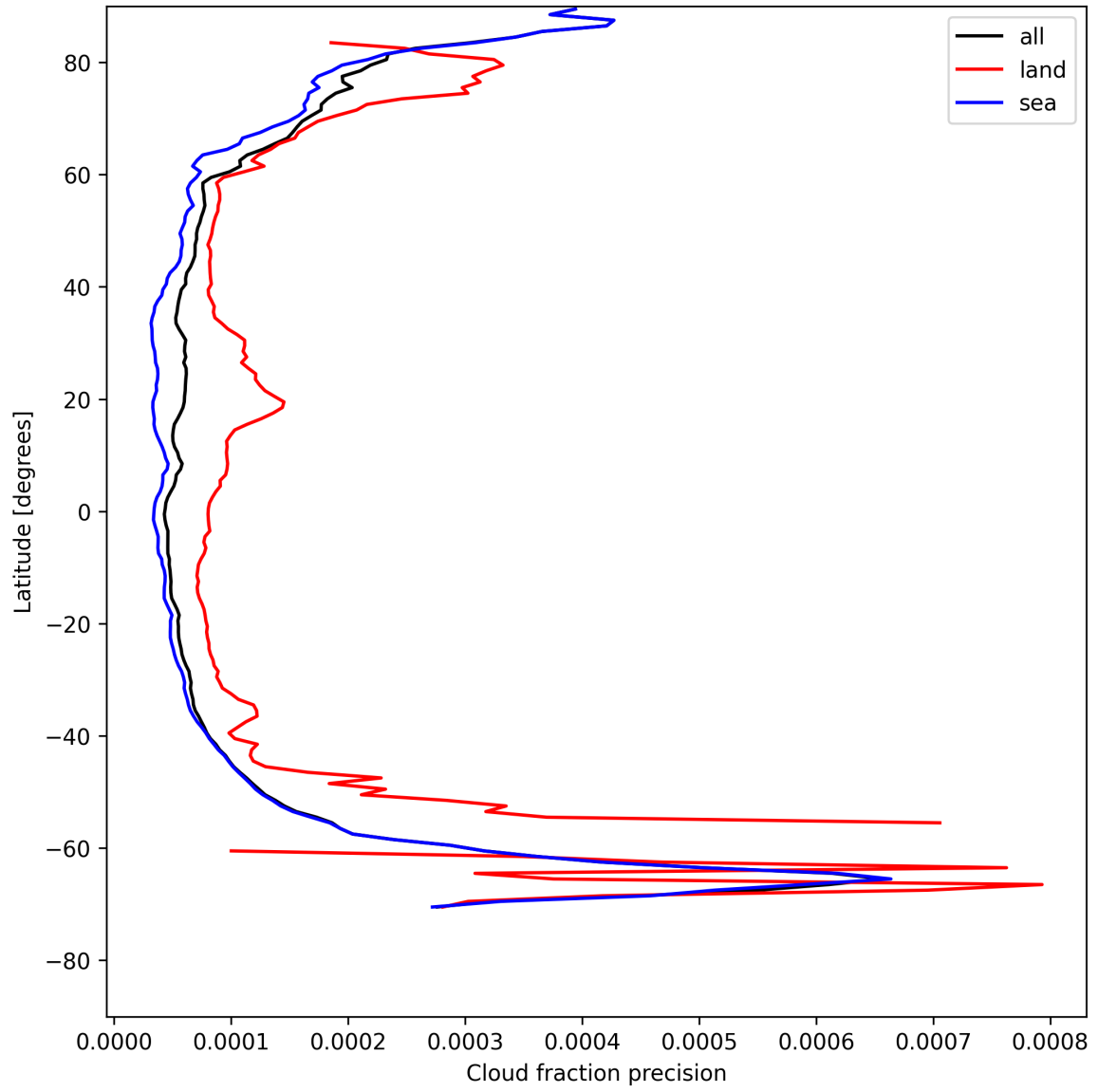
Figure 16: Zonal average of “Cloud fraction precision” for 2025-08-04 to 2025-08-05.
