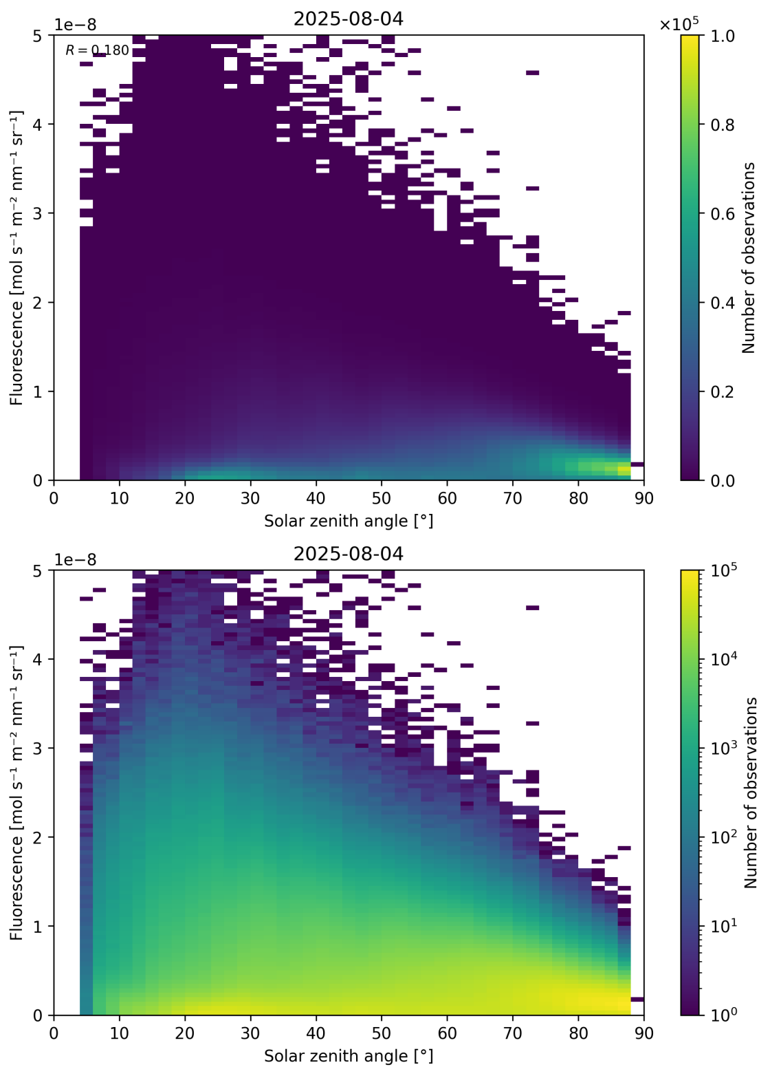
Figure 112: Scatter density plot of “Solar zenith angle” against “Fluorescence” for 2025-08-04 to 2025-08-05.
