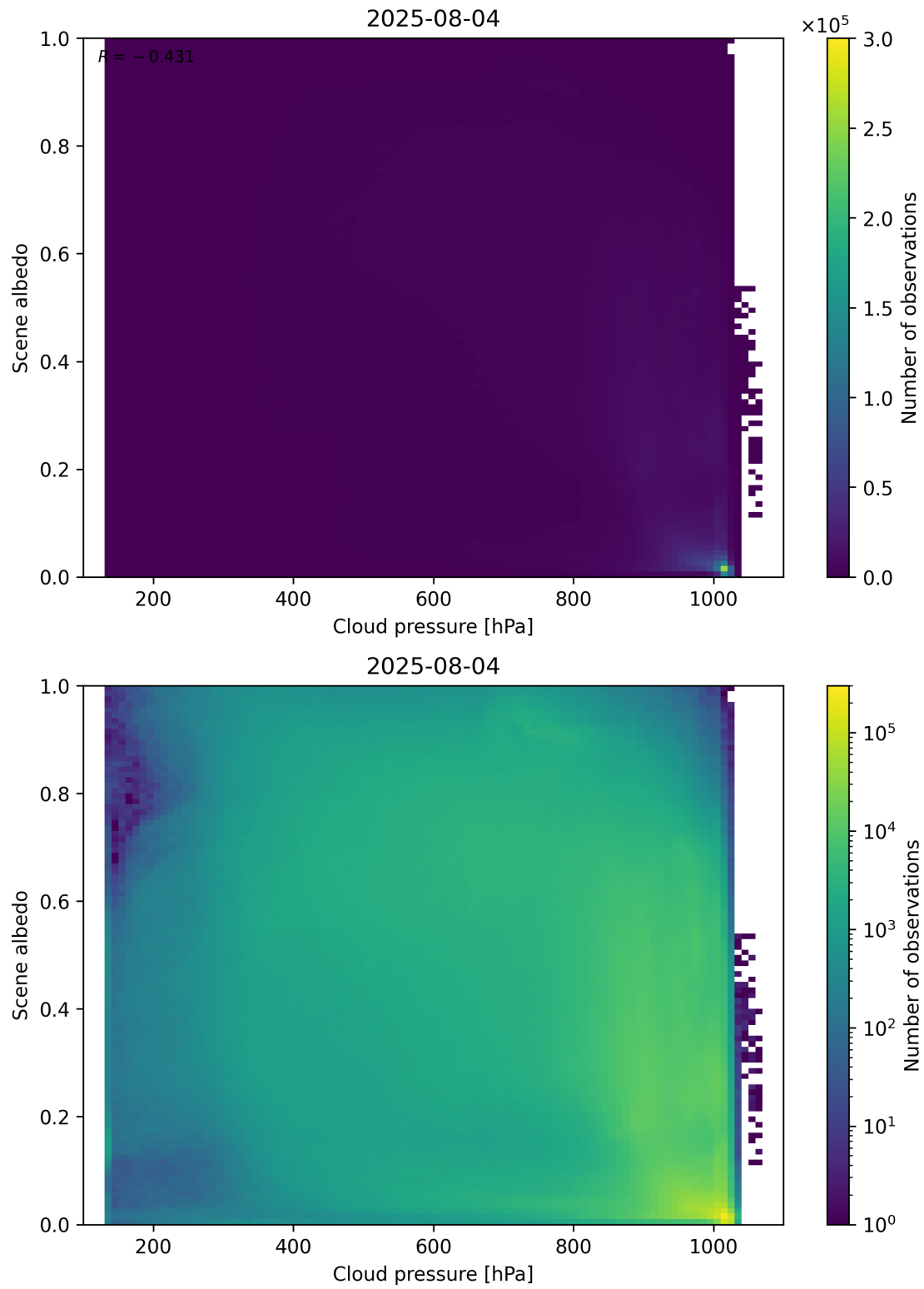
Figure 83: Scatter density plot of “Cloud pressure” against “Scene albedo” for 2025-08-04 to 2025-08-05.
