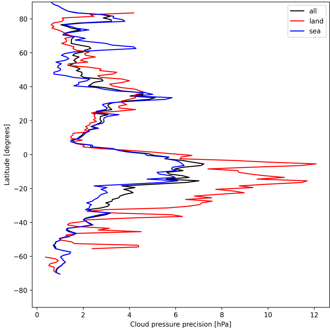
Figure 14: Zonal average of “Cloud pressure precision” for 2025-08-04 to 2025-08-05.
