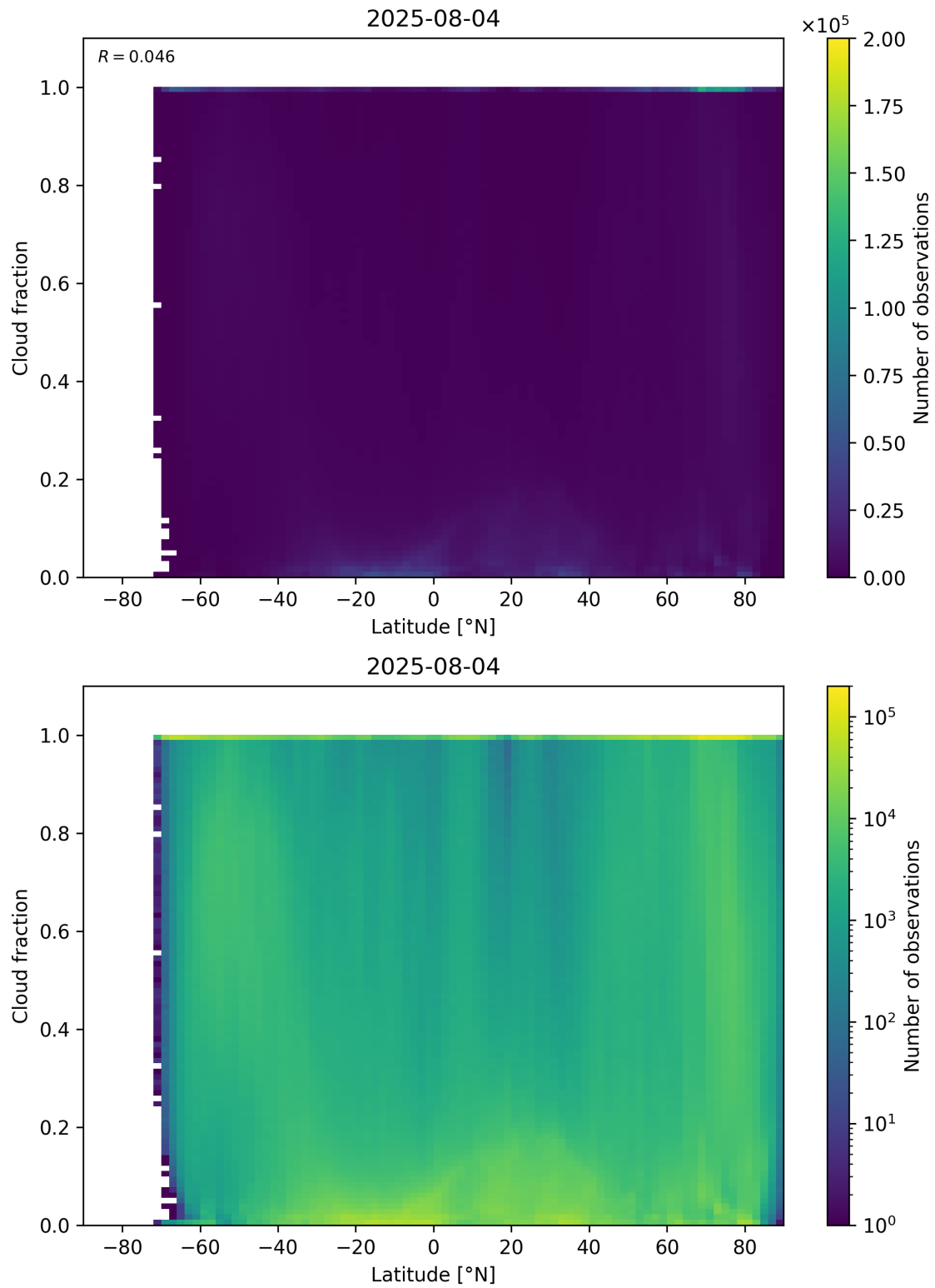
Figure 90: Scatter density plot of “Latitude” against “Cloud fraction” for 2025-08-04 to 2025-08-05.
