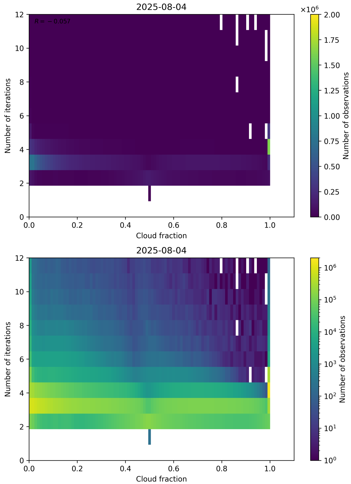
Figure 73: Scatter density plot of “Cloud fraction” against “Number of iterations” for 2025-08-04 to 2025-08-05.
