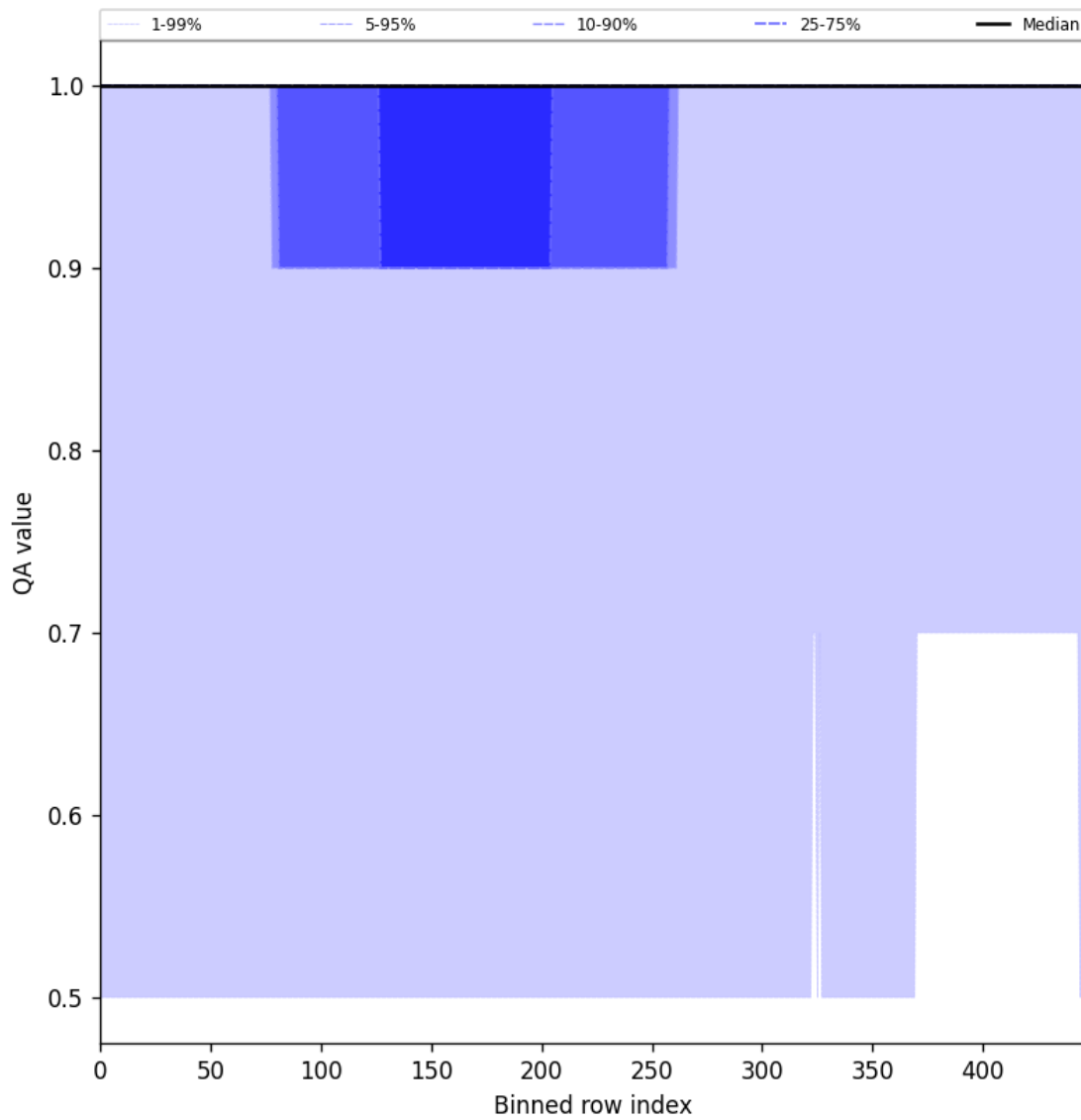
Figure 46: Along track statistics of “QA value” for 2025-08-04 to 2025-08-05
