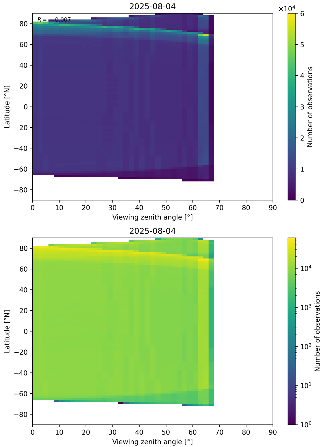
Figure 123: Scatter density plot of “Viewing zenith angle” against “Latitude” for 2025-08-04 to 2025-08-05.
