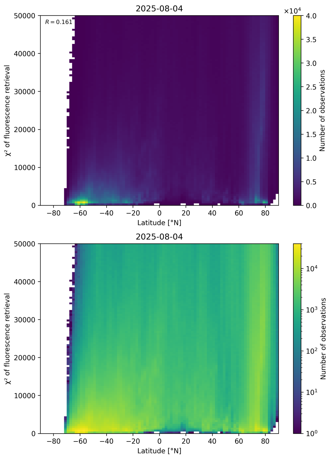
Figure 89: Scatter density plot of “Latitude” against “ \chi^2 of fluorescence retrieval” for 2025-08-04 to 2025-08-05.
