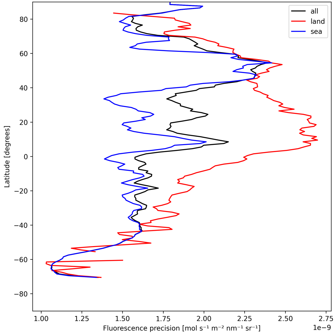
Figure 24: Zonal average of “Fluorescence precision” for 2025-08-04 to 2025-08-05.
