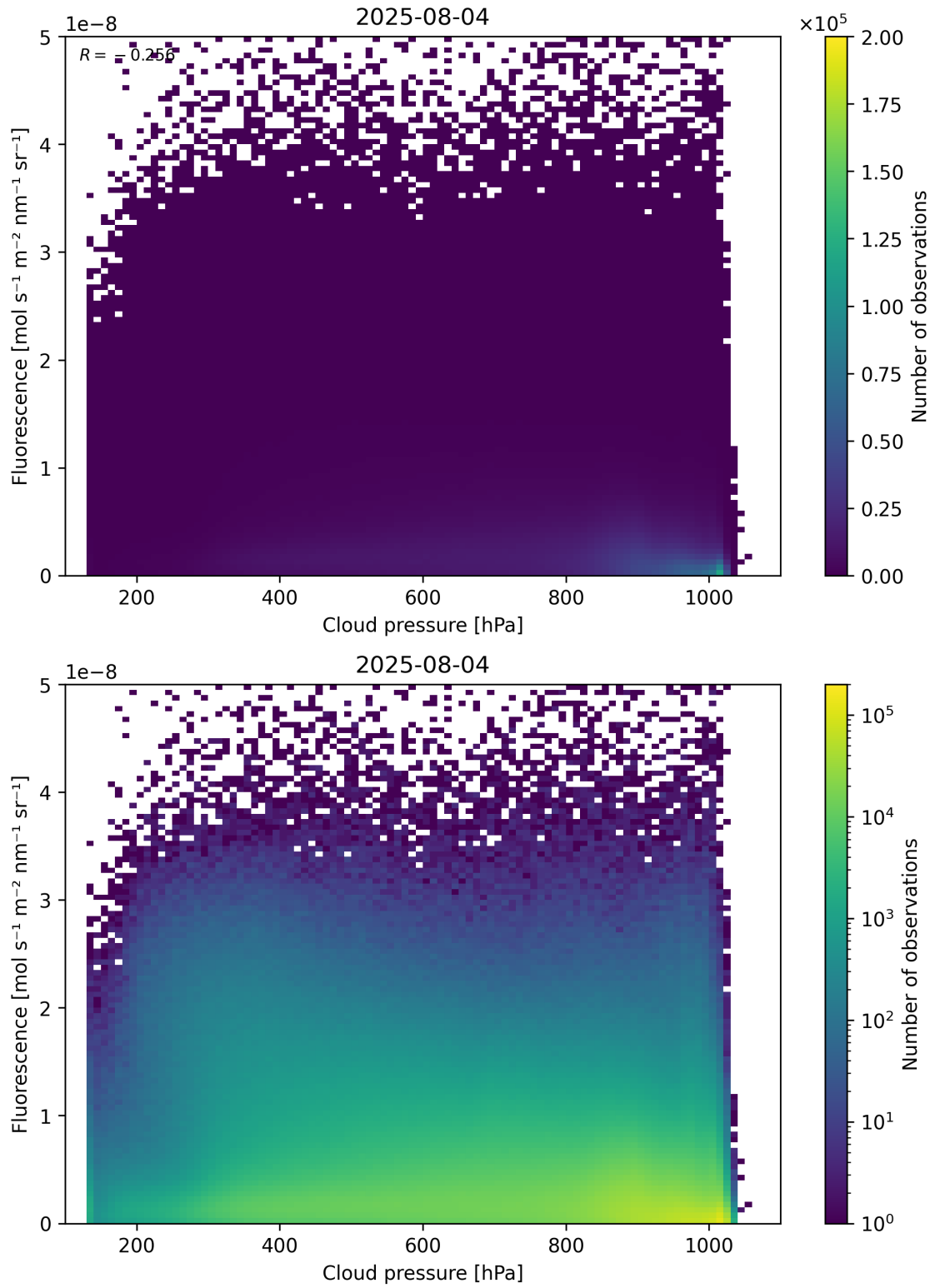
Figure 80: Scatter density plot of “Cloud pressure” against “Fluorescence” for 2025-08-04 to 2025-08-05.
