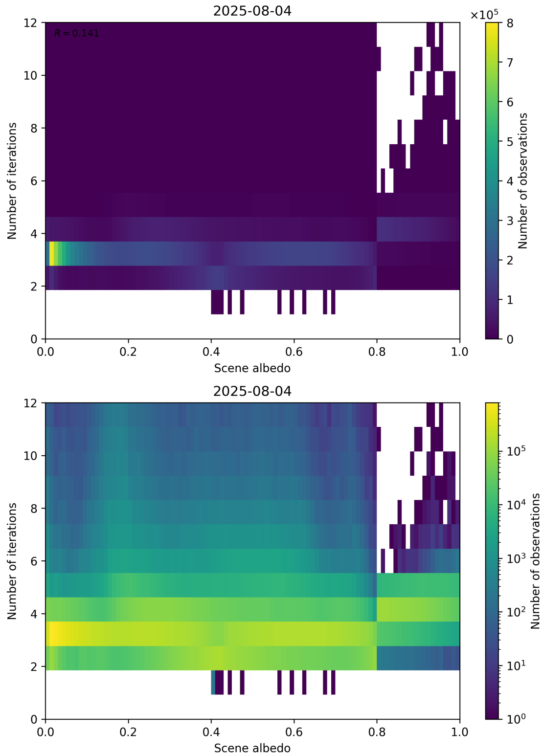
Figure 105: Scatter density plot of “Scene albedo” against “Number of iterations” for 2025-08-04 to 2025-08-05.
