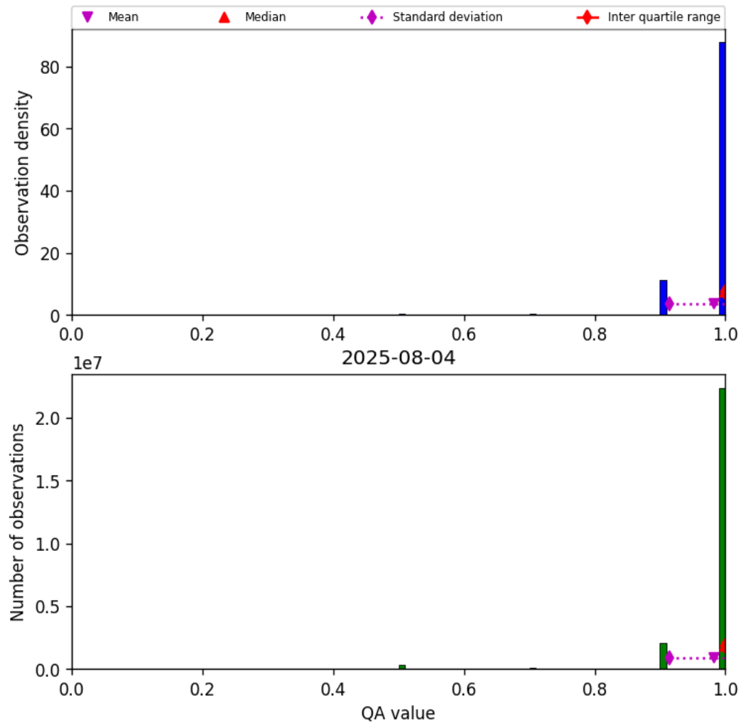
Figure 29: Histogram of “QA value” for 2025-08-04 to 2025-08-05
