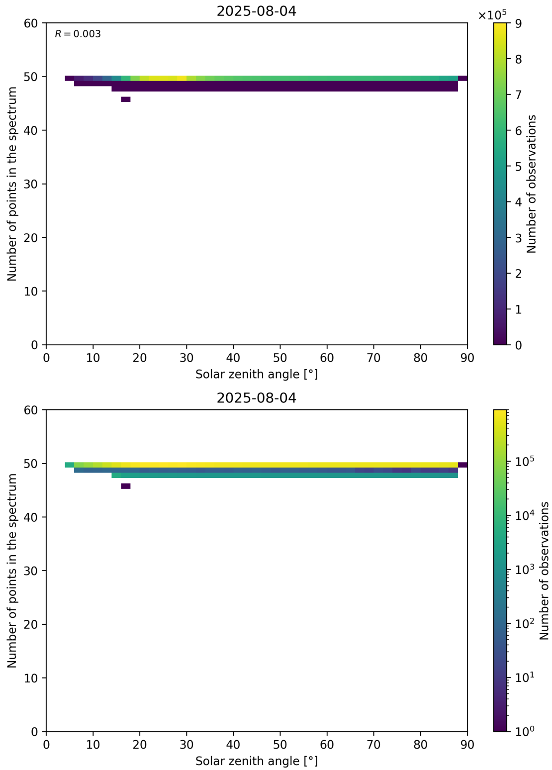
Figure 115: Scatter density plot of “Solar zenith angle” against “Number of points in the spectrum” for 2025-08-04 to 2025-08-05.
