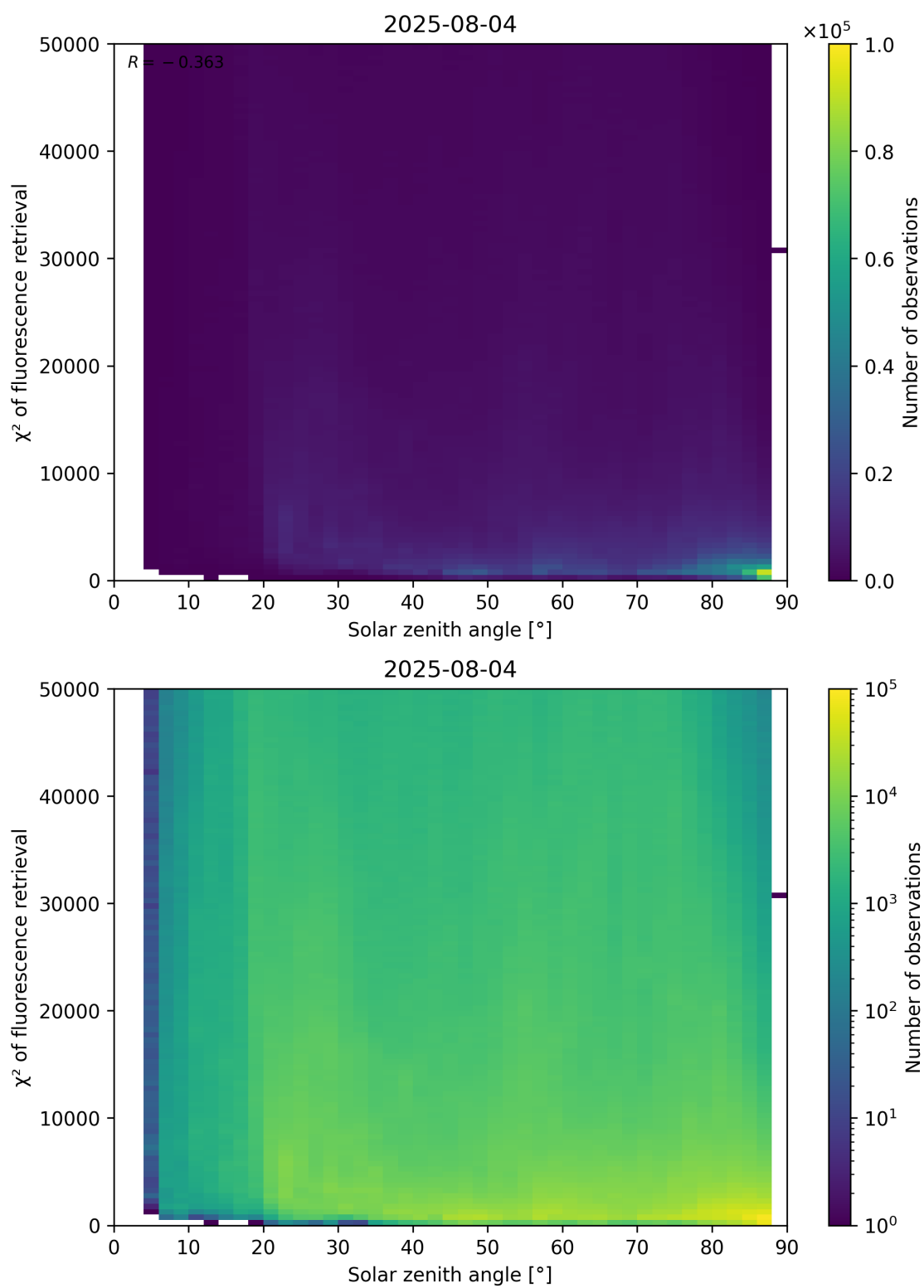
Figure 109: Scatter density plot of “Solar zenith angle” against “ \chi^2 of fluorescence retrieval” for 2025-08-04 to 2025-08-05.
