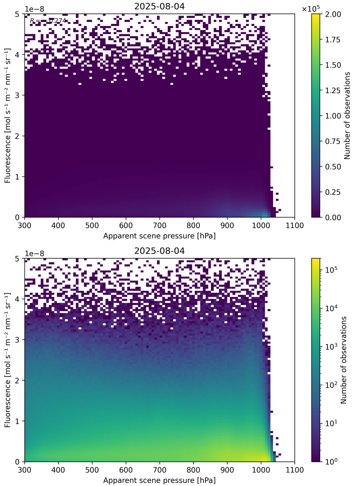
Figure 64: Scatter density plot of “Apparent scene pressure” against “Fluorescence” for 2025-08-04 to 2025-08-05.
