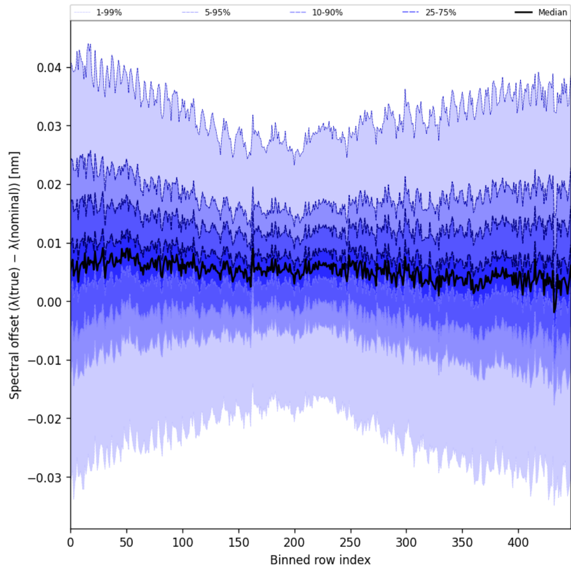
Figure 62: Along track statistics of “Spectral offset ( \lambda_{\text{true}} - \lambda_{\text{nominal}} )” for 2025-08-04 to 2025-08-05
