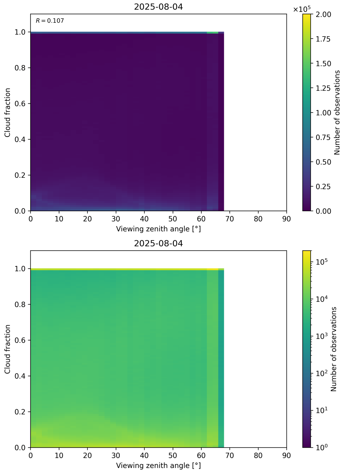
Figure 120: Scatter density plot of “Viewing zenith angle” against “Cloud fraction” for 2025-08-04 to 2025-08-05.
