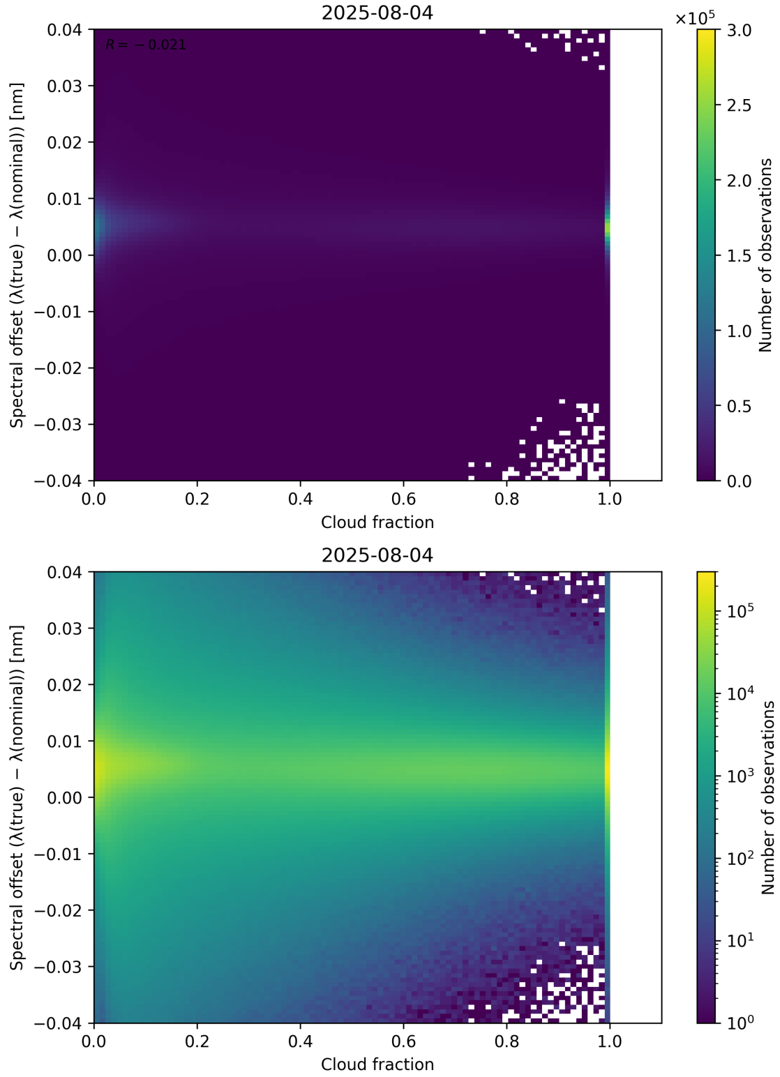
Figure 76: Scatter density plot of “Cloud fraction” against “Spectral offset ( \lambda_{\text{true}} - \lambda_{\text{nominal}} )” for 2025-08-04 to 2025-08-05.
