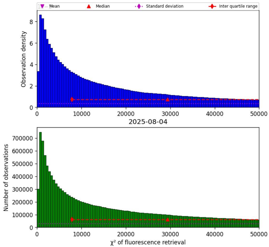
Figure 42: Histogram of “ \chi^2 of fluorescence retrieval” for 2025-08-04 to 2025-08-05
