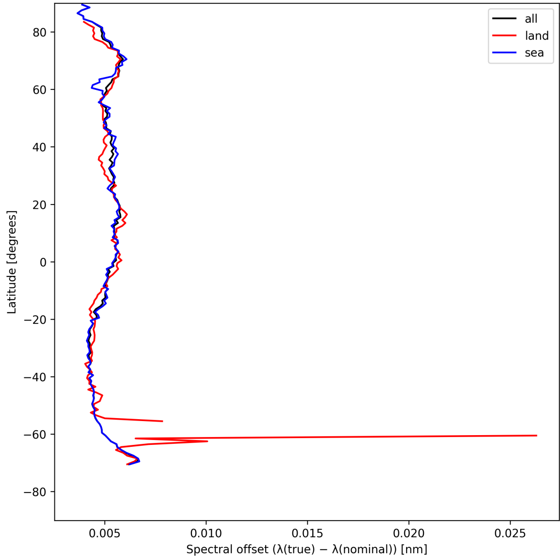
Figure 28: Zonal average of “Spectral offset ( \lambda_{\text{true}} - \lambda_{\text{nominal}} )” for 2025-08-04 to 2025-08-05.
