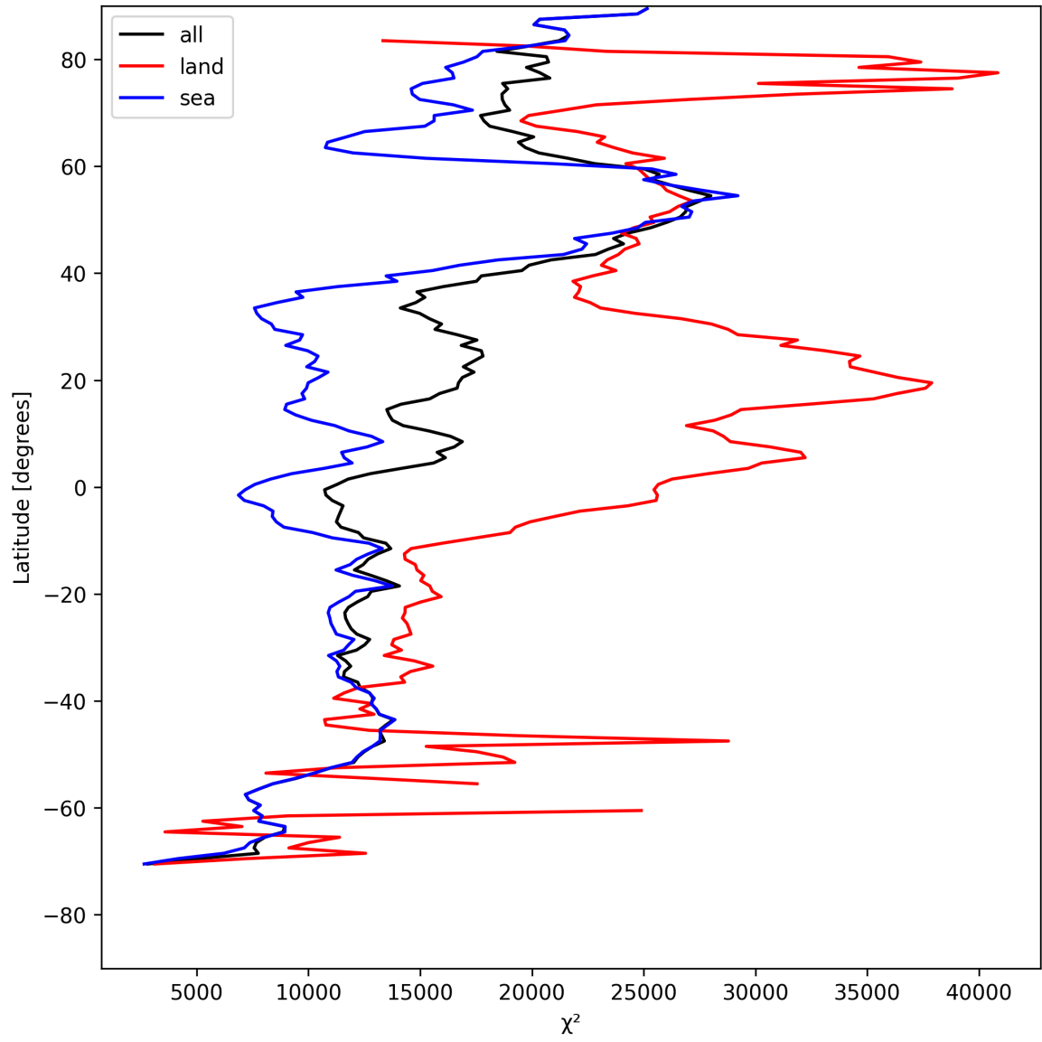
Figure 21: Zonal average of “ \chi^2 ” for 2025-08-04 to 2025-08-05.
