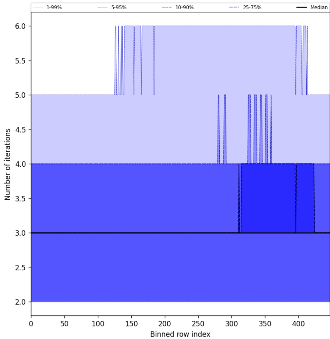
Figure 56: Along track statistics of “Number of iterations” for 2025-08-04 to 2025-08-05
