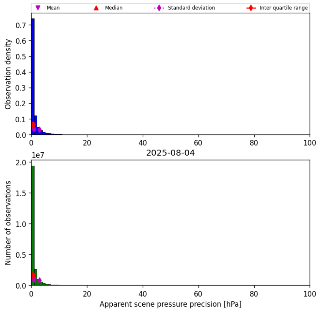
Figure 37: Histogram of “Apparent scene pressure precision” for 2025-08-04 to 2025-08-05
