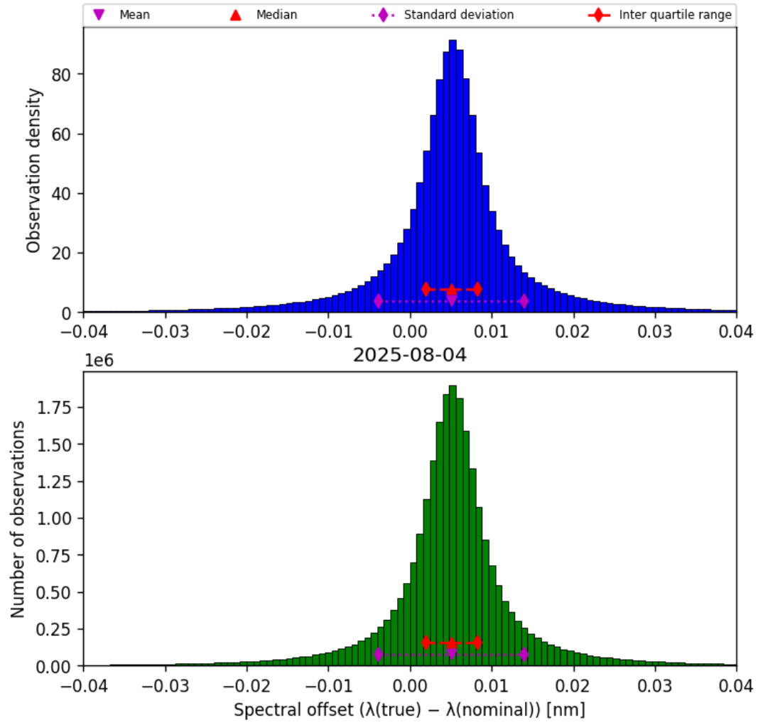
Figure 45: Histogram of “Spectral offset ( \lambda_{\text{true}} - \lambda_{\text{nominal}} )” for 2025-08-04 to 2025-08-05
