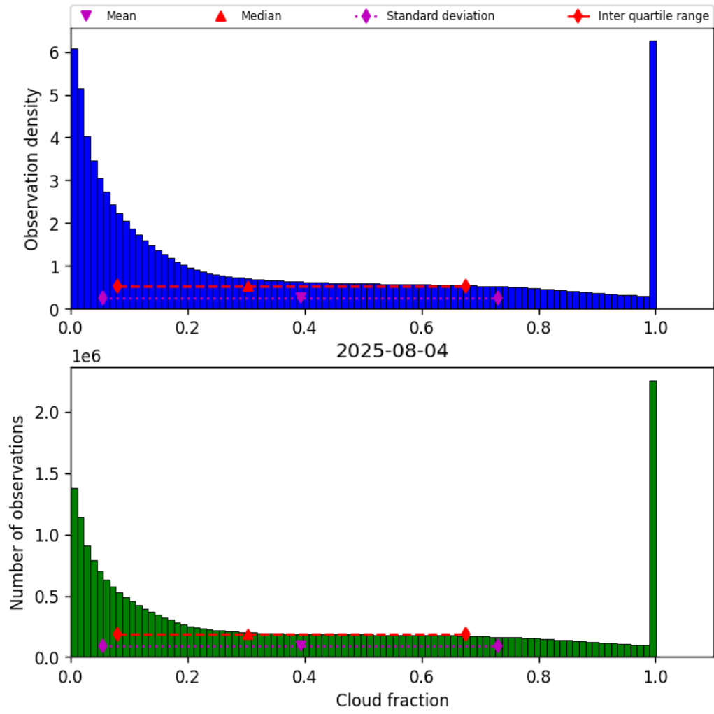
Figure 32: Histogram of “Cloud fraction” for 2025-08-04 to 2025-08-05
