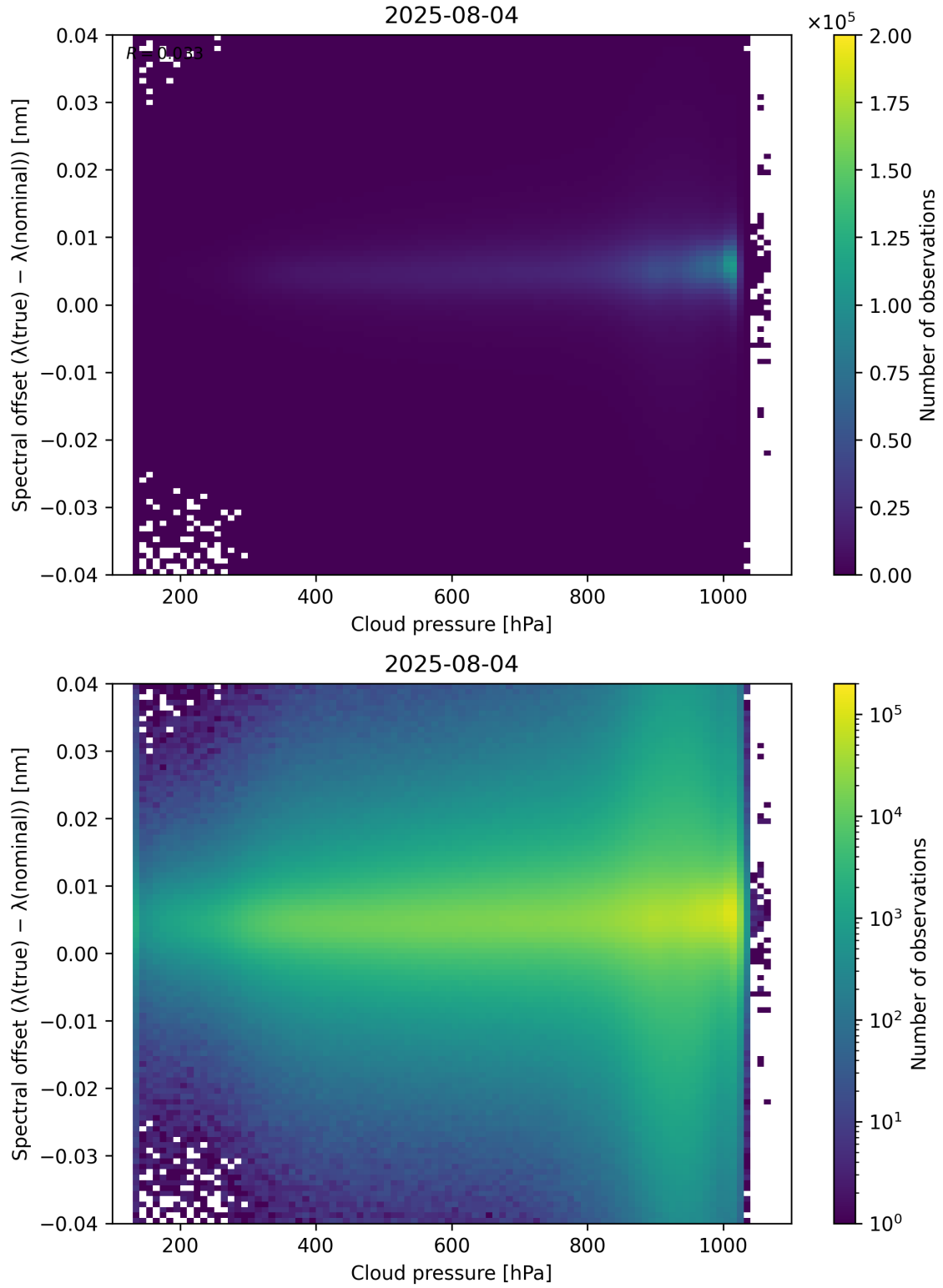
Figure 84: Scatter density plot of “Cloud pressure” against “Spectral offset ( \lambda_{\text{true}} - \lambda_{\text{nominal}} )” for 2025-08-04 to 2025-08-05.
