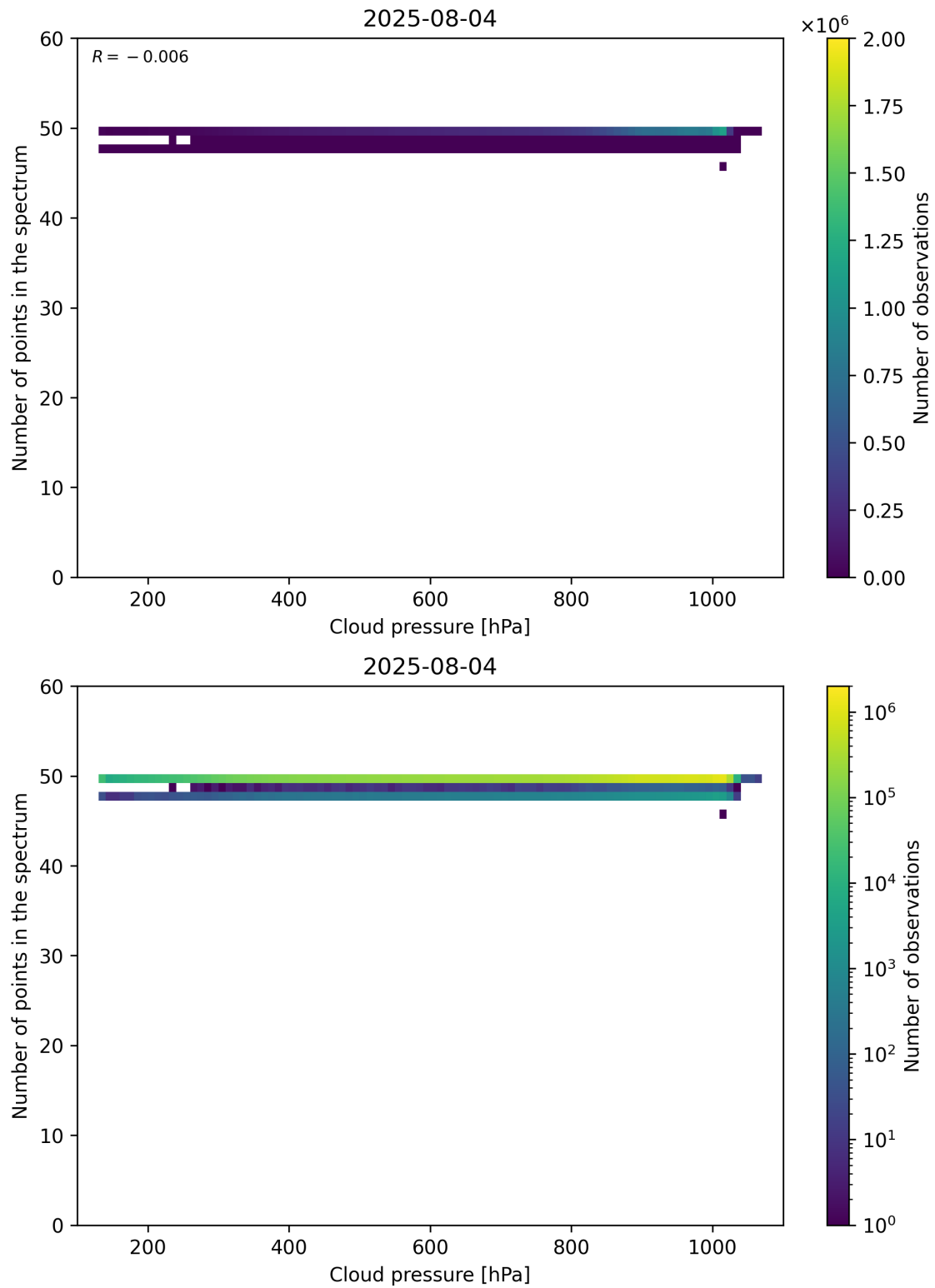
Figure 82: Scatter density plot of “Cloud pressure” against “Number of points in the spectrum” for 2025-08-04 to 2025-08-05.
