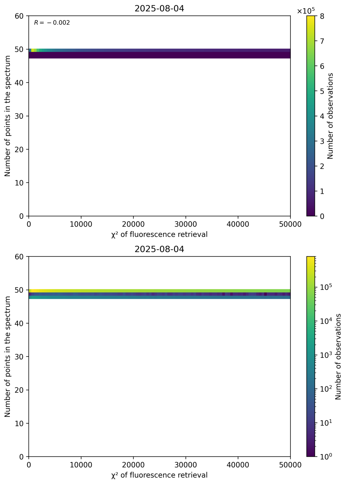
Figure 68: Scatter density plot of “ \chi^2 of fluorescence retrieval” against “Number of points in the spectrum” for 2025-08-04 to 2025-08-05.
