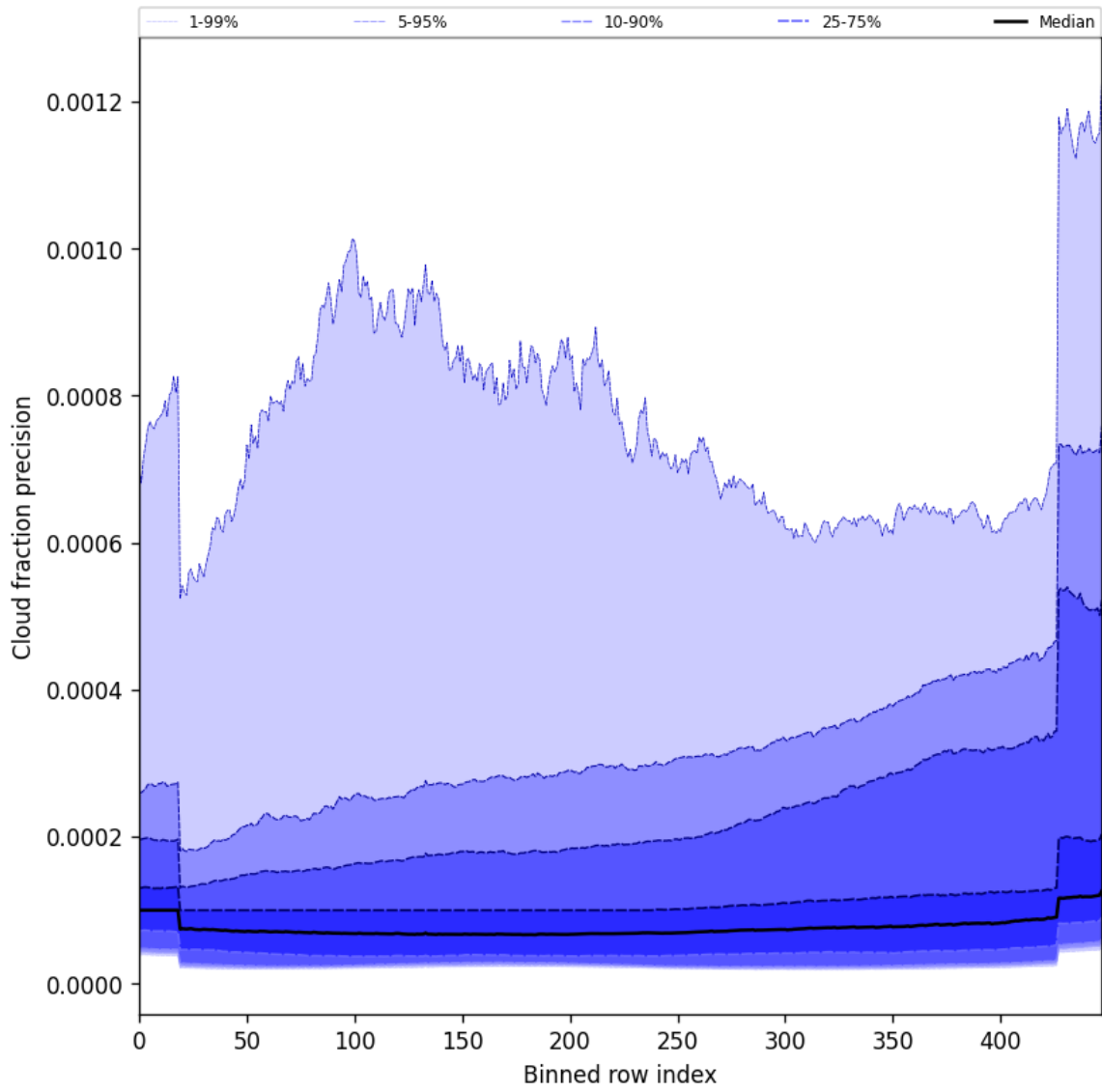
Figure 50: Along track statistics of “Cloud fraction precision” for 2025-08-04 to 2025-08-05
