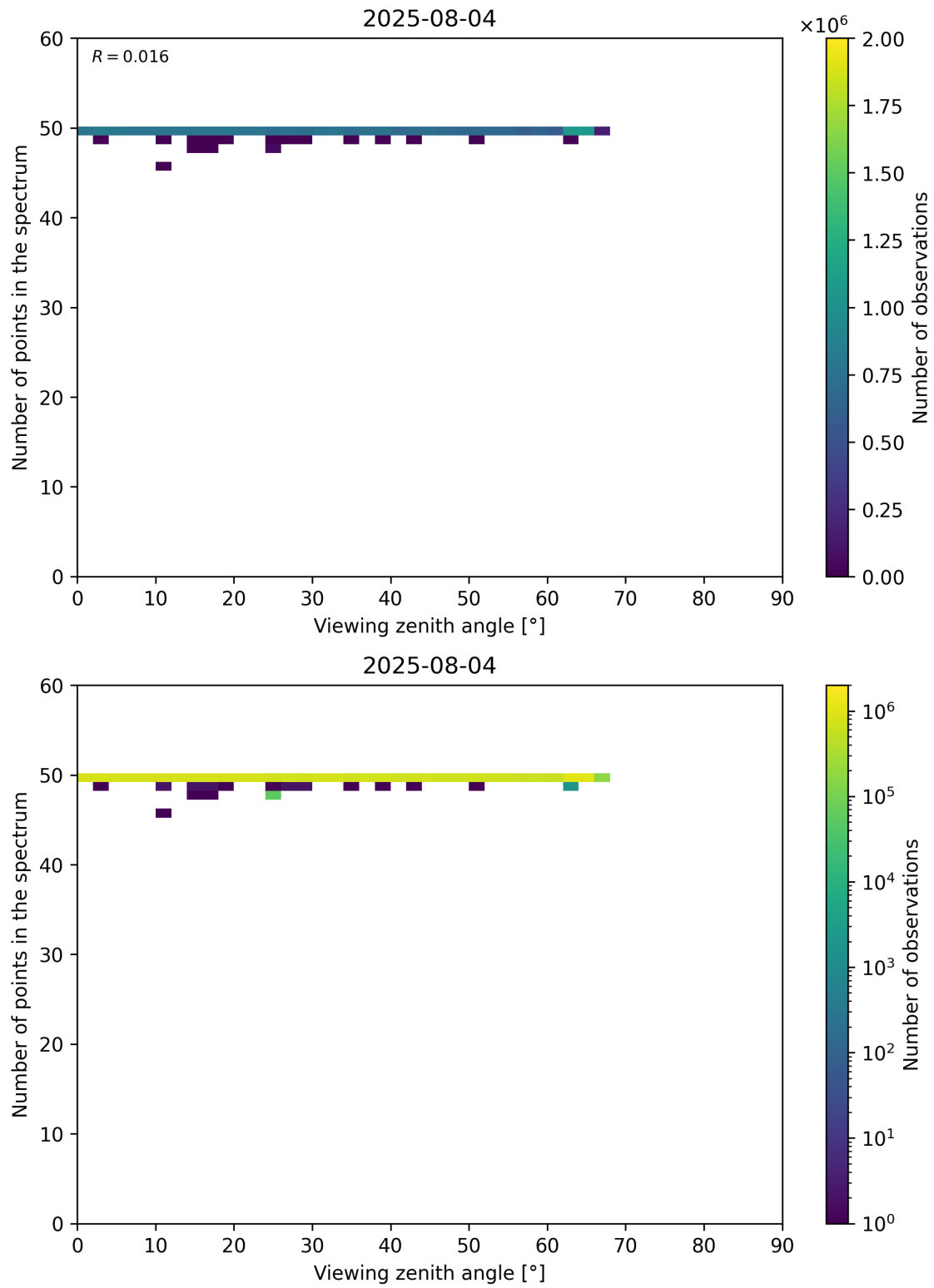
Figure 125: Scatter density plot of “Viewing zenith angle” against “Number of points in the spectrum” for 2025-08-04 to 2025-08-05.
