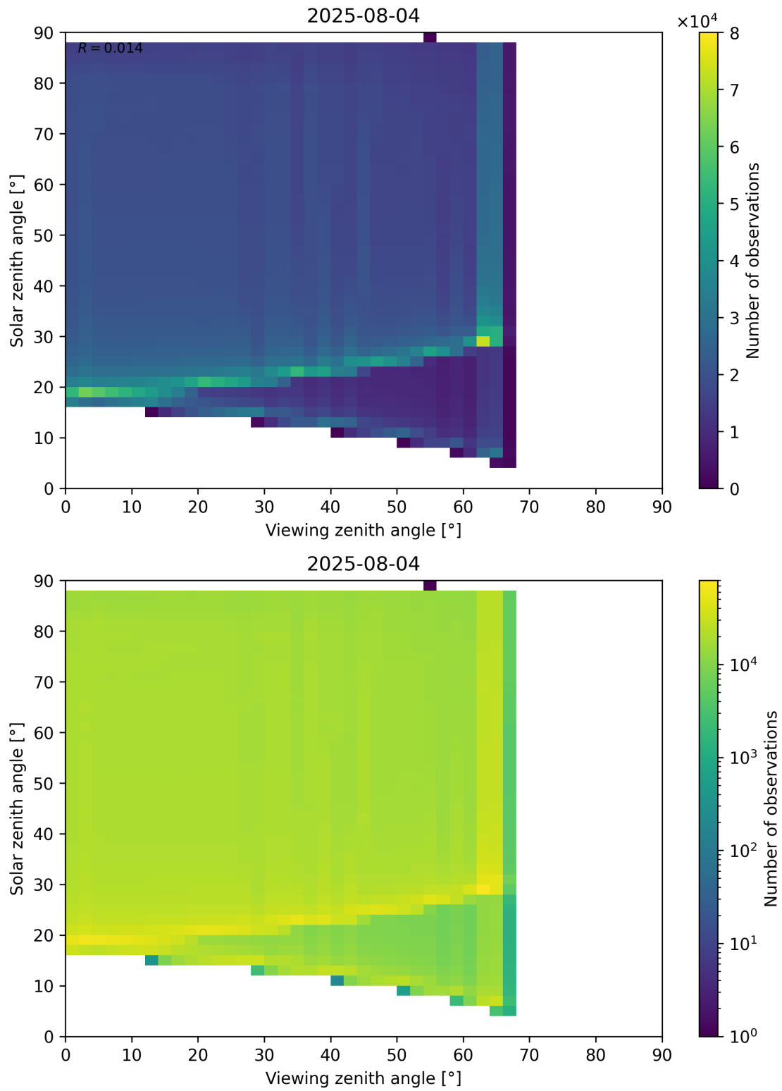
Figure 127: Scatter density plot of “Viewing zenith angle” against “Solar zenith angle” for 2025-08-04 to 2025-08-05.
