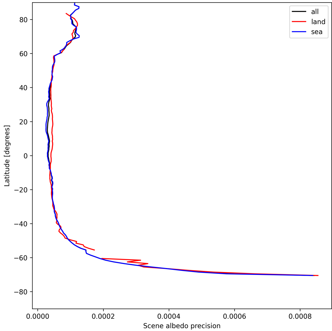
Figure 18: Zonal average of “Scene albedo precision” for 2025-08-04 to 2025-08-05.
