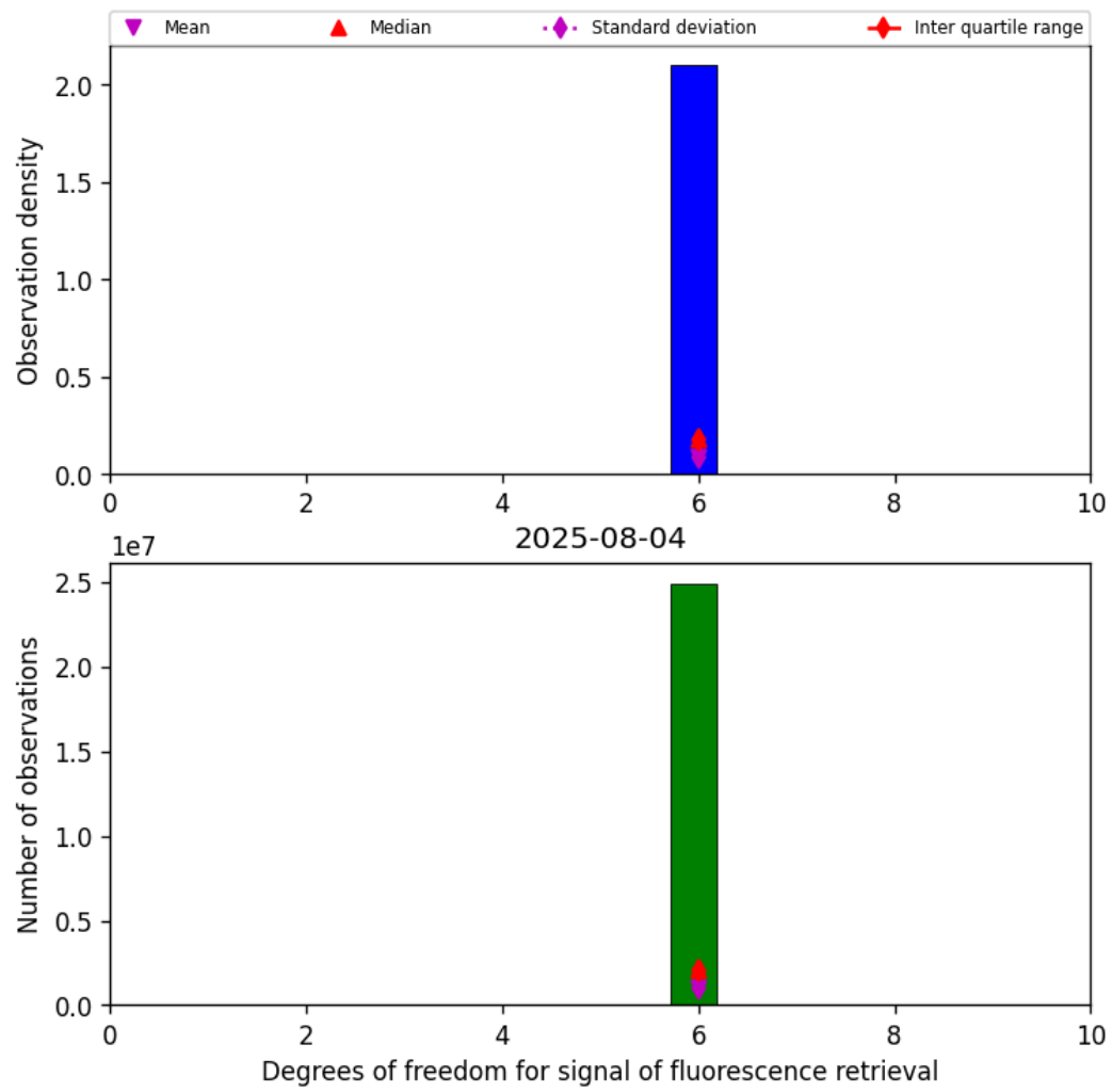
Figure 43: Histogram of “Degrees of freedom for signal of fluorescence retrieval” for 2025-08-04 to 2025-08-05
