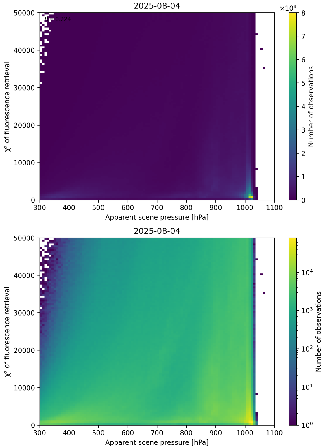
Figure 63: Scatter density plot of “Apparent scene pressure” against “ \chi^2 of fluorescence retrieval” for 2025-08-04 to 2025-08-05.
