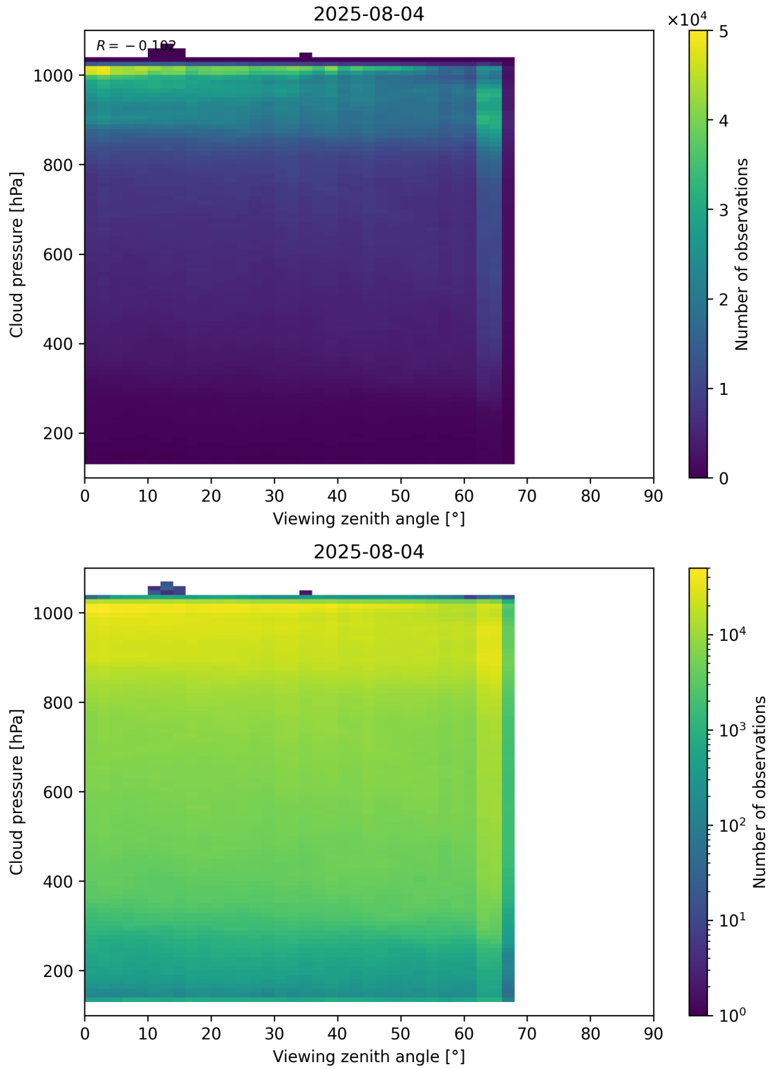
Figure 121: Scatter density plot of “Viewing zenith angle” against “Cloud pressure” for 2025-08-04 to 2025-08-05.
