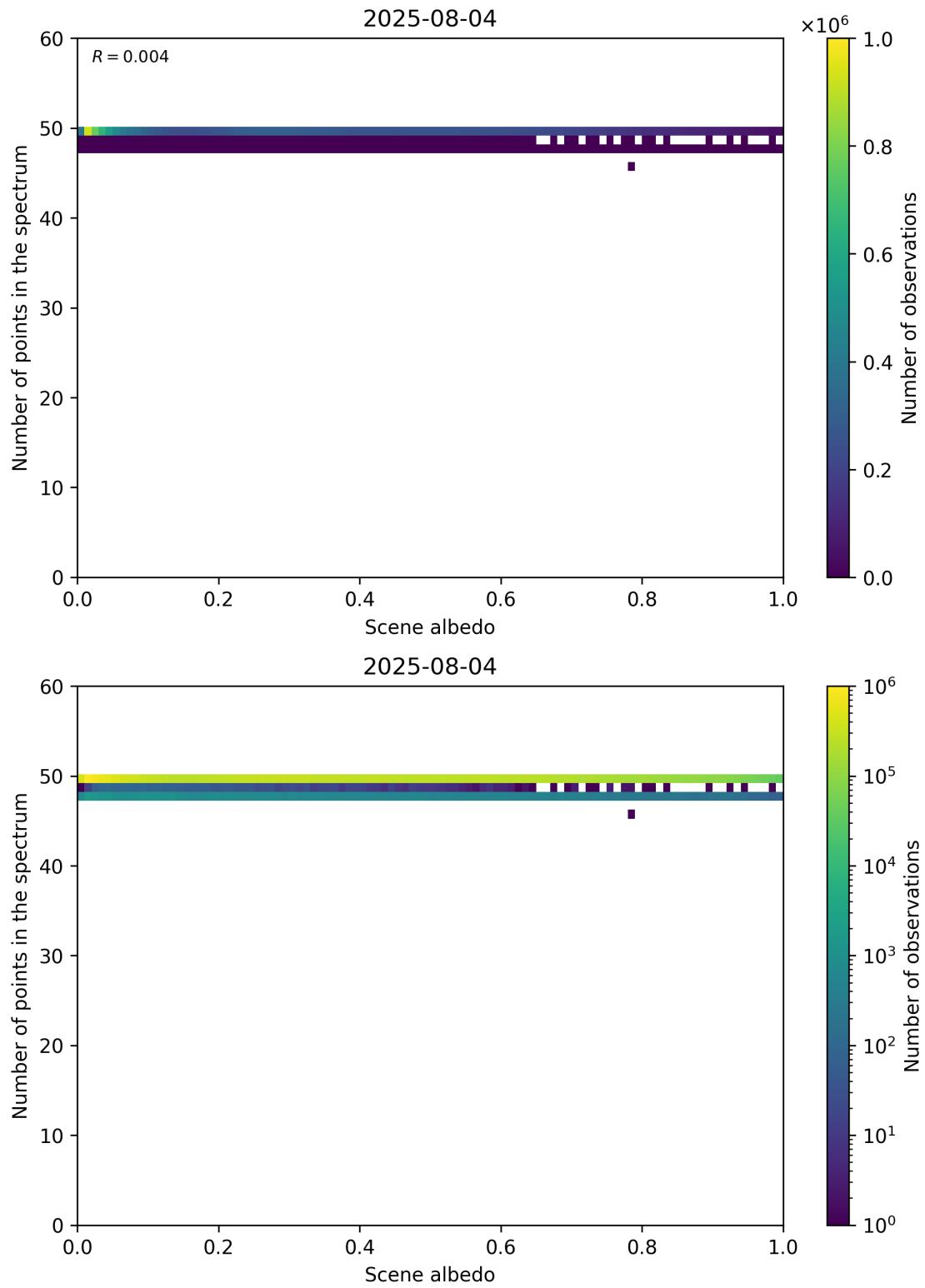
Figure 106: Scatter density plot of “Scene albedo” against “Number of points in the spectrum” for 2025-08-04 to 2025-08-05.
