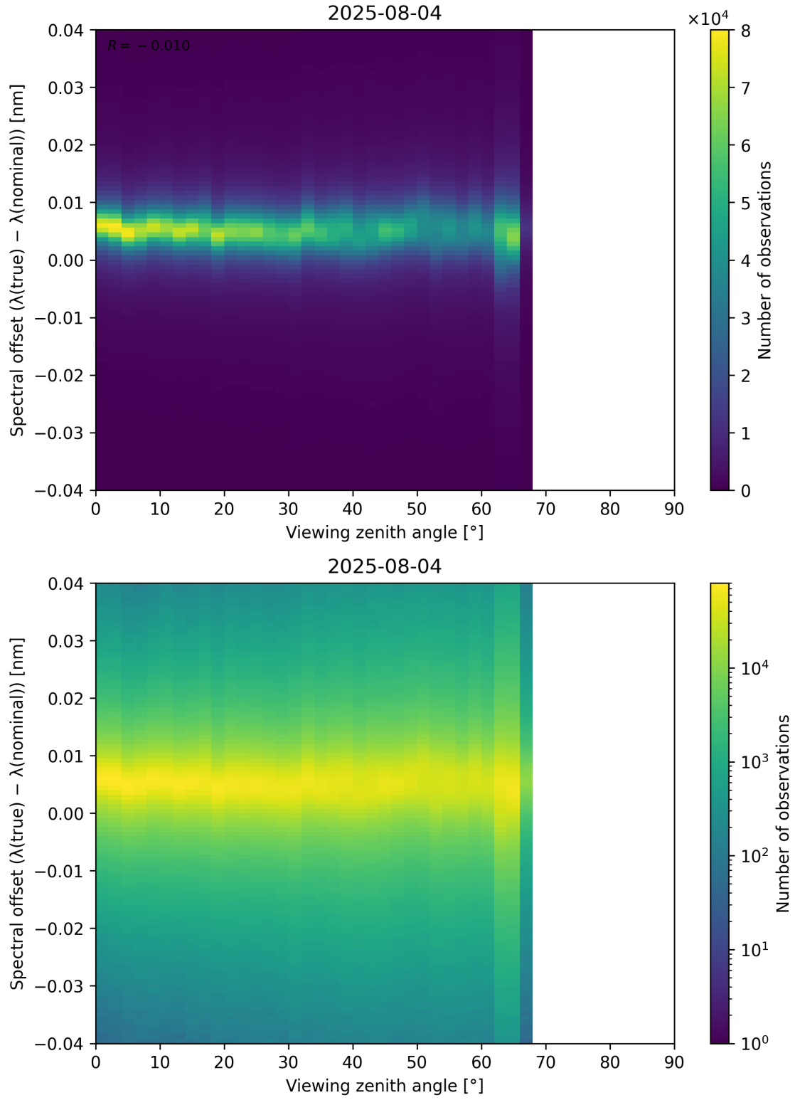
Figure 128: Scatter density plot of “Viewing zenith angle” against “Spectral offset ( \lambda_{\text{true}} - \lambda_{\text{nominal}} )” for 2025-08-04 to 2025-08-05.
