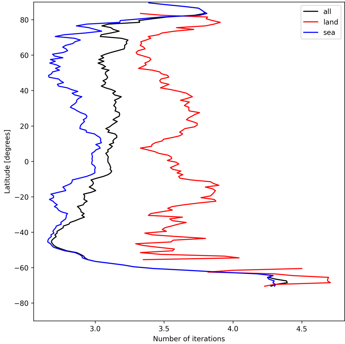
Figure 22: Zonal average of “Number of iterations” for 2025-08-04 to 2025-08-05.
