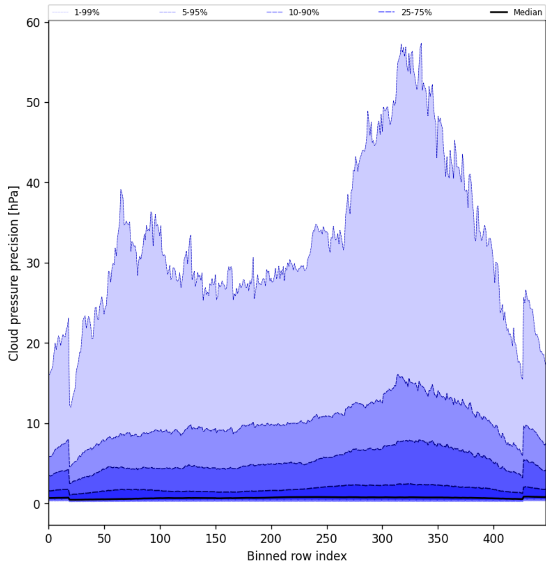
Figure 48: Along track statistics of “Cloud pressure precision” for 2025-08-04 to 2025-08-05
