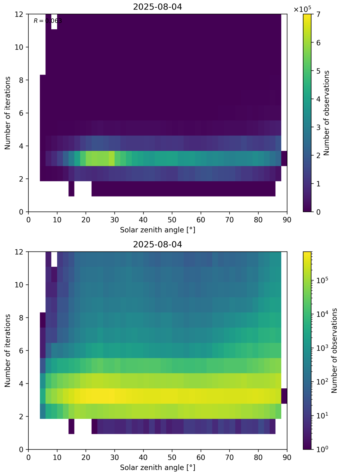
Figure 114: Scatter density plot of “Solar zenith angle” against “Number of iterations” for 2025-08-04 to 2025-08-05.
