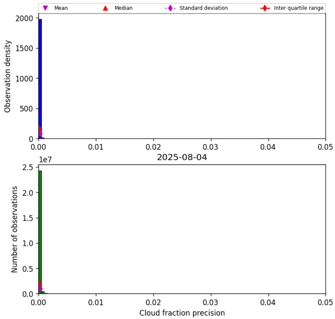
Figure 33: Histogram of “Cloud fraction precision” for 2025-08-04 to 2025-08-05
