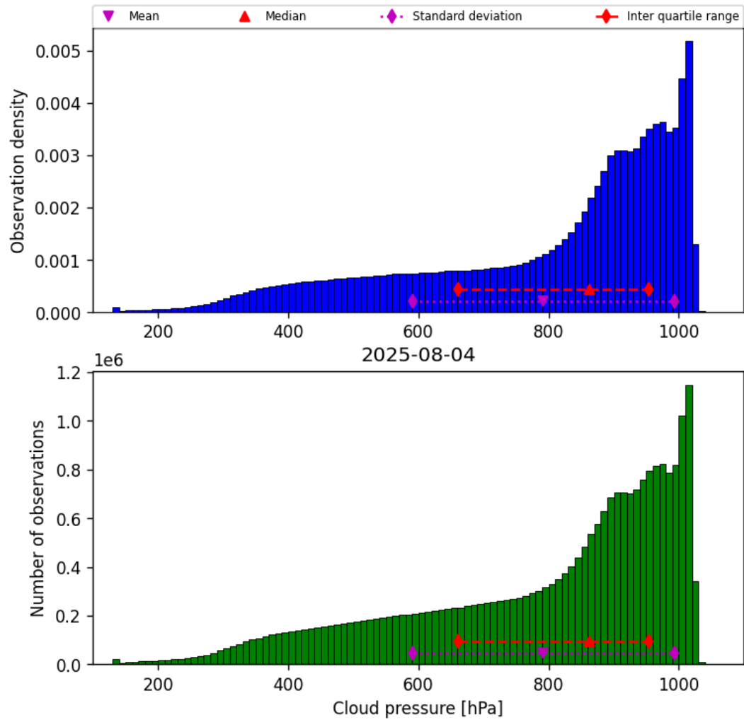
Figure 30: Histogram of “Cloud pressure” for 2025-08-04 to 2025-08-05
