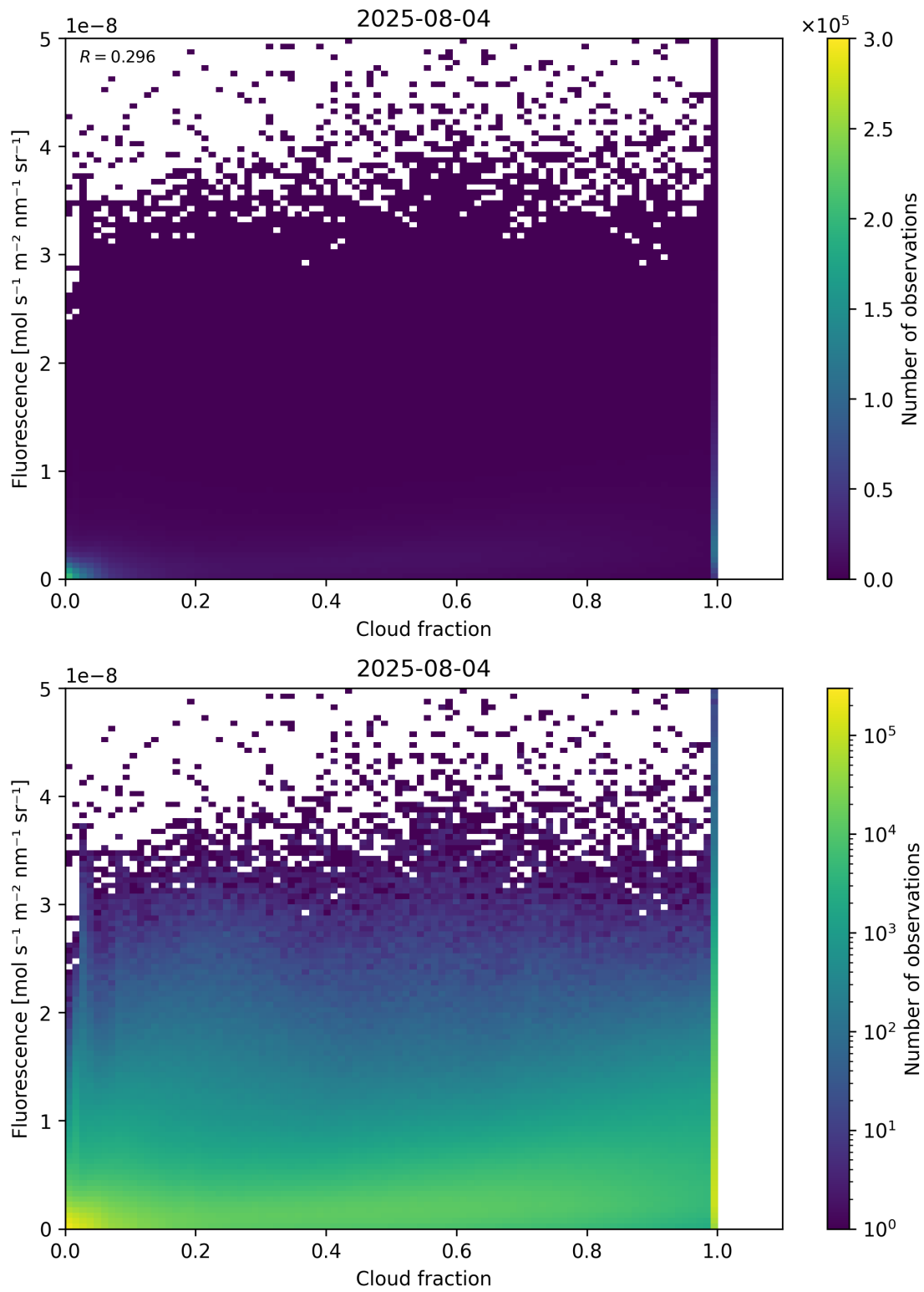
Figure 72: Scatter density plot of “Cloud fraction” against “Fluorescence” for 2025-08-04 to 2025-08-05.
