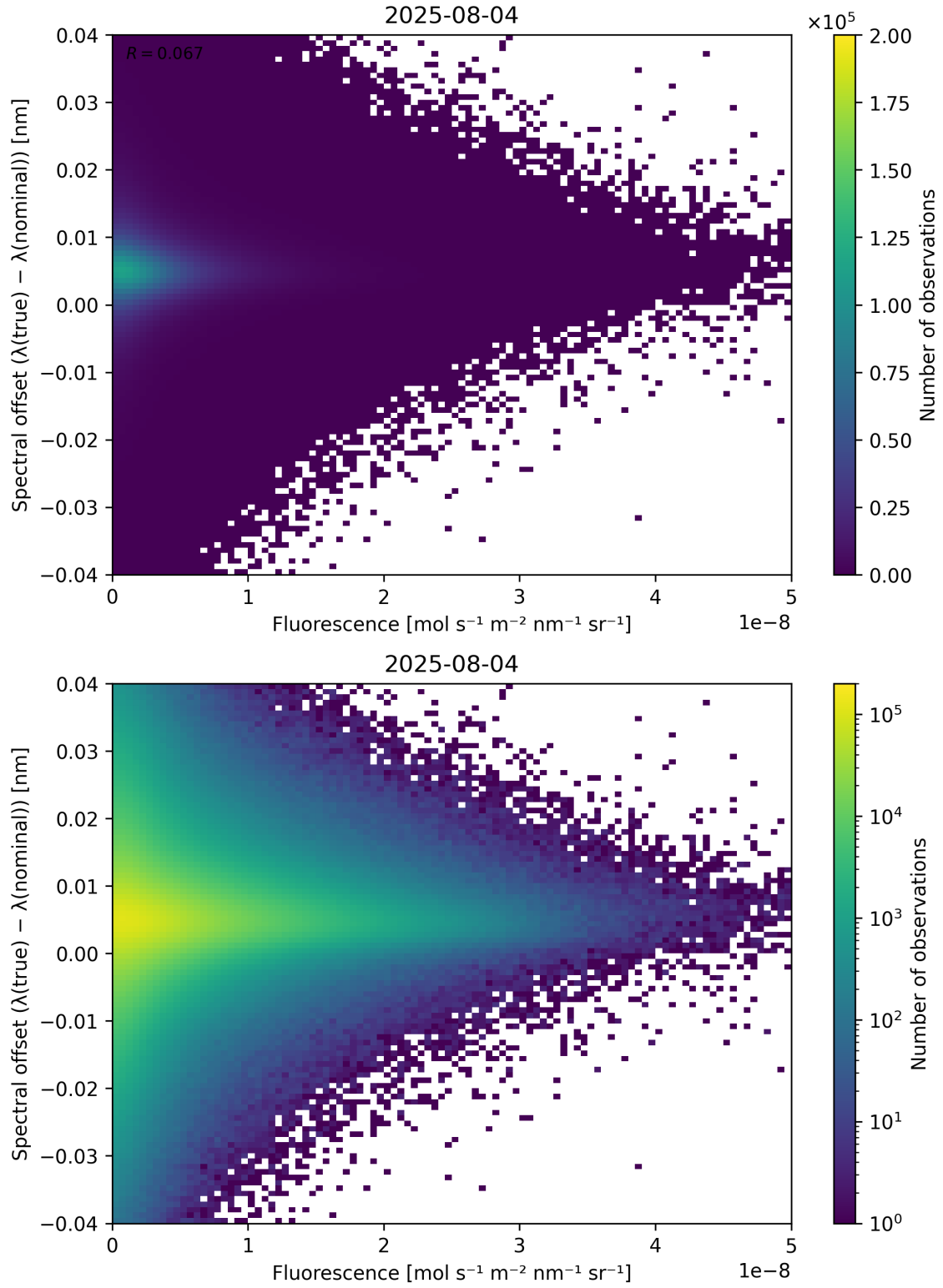
Figure 87: Scatter density plot of “Fluorescence” against “Spectral offset ( \lambda_{\text{true}} - \lambda_{\text{nominal}} )” for 2025-08-04 to 2025-08-05.
