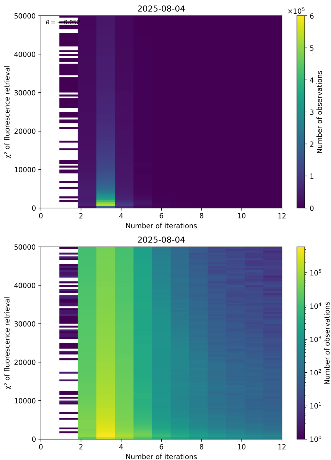
Figure 97: Scatter density plot of “Number of iterations” against “ \chi^2 of fluorescence retrieval” for 2025-08-04 to 2025-08-05.
