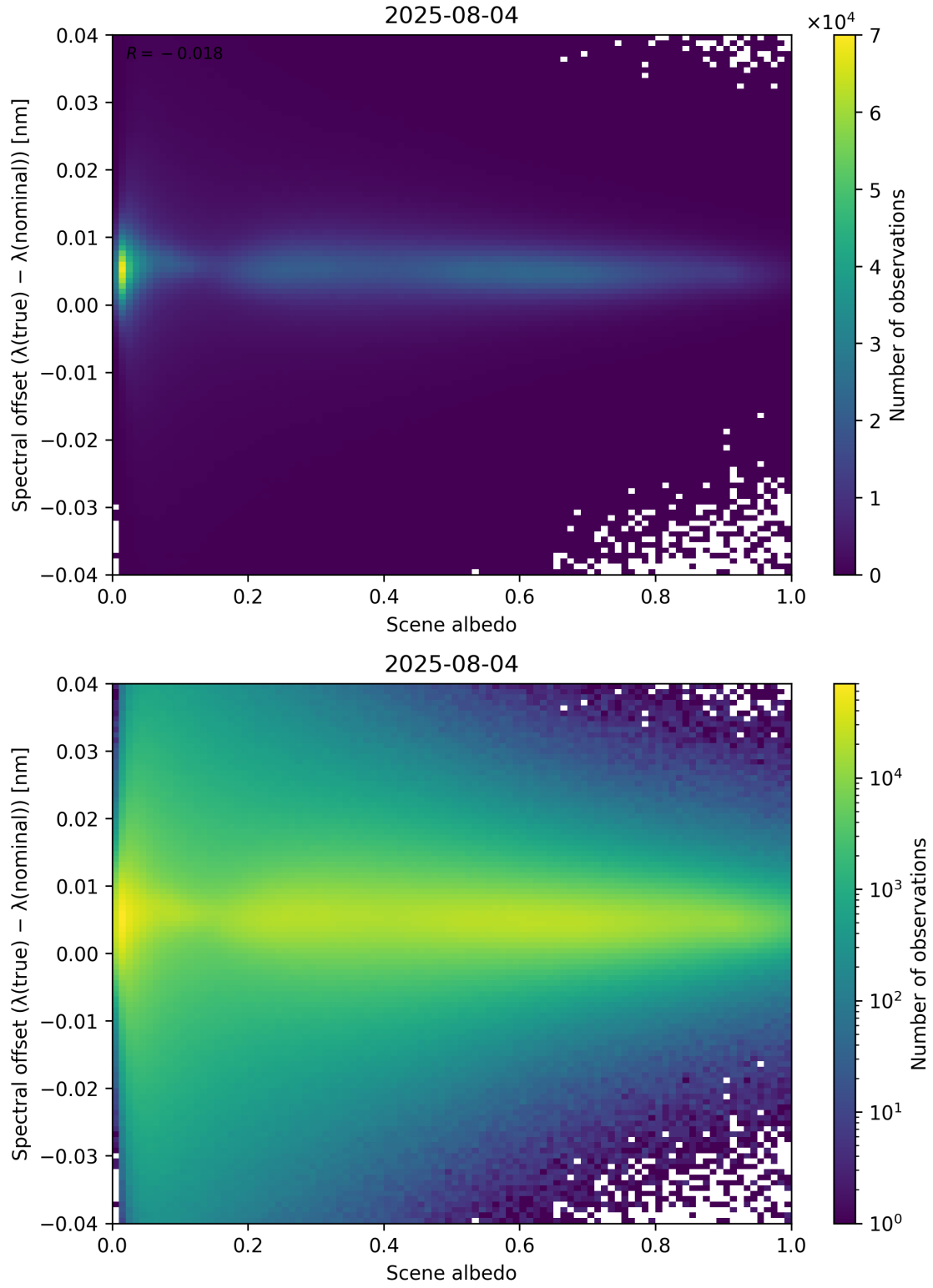
Figure 107: Scatter density plot of “Scene albedo” against “Spectral offset ( \lambda_{\text{true}} - \lambda_{\text{nominal}} )” for 2025-08-04 to 2025-08-05.
