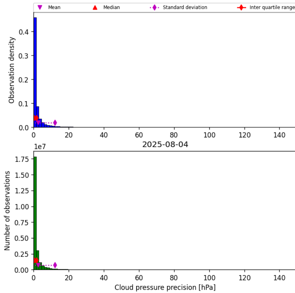
Figure 31: Histogram of “Cloud pressure precision” for 2025-08-04 to 2025-08-05
