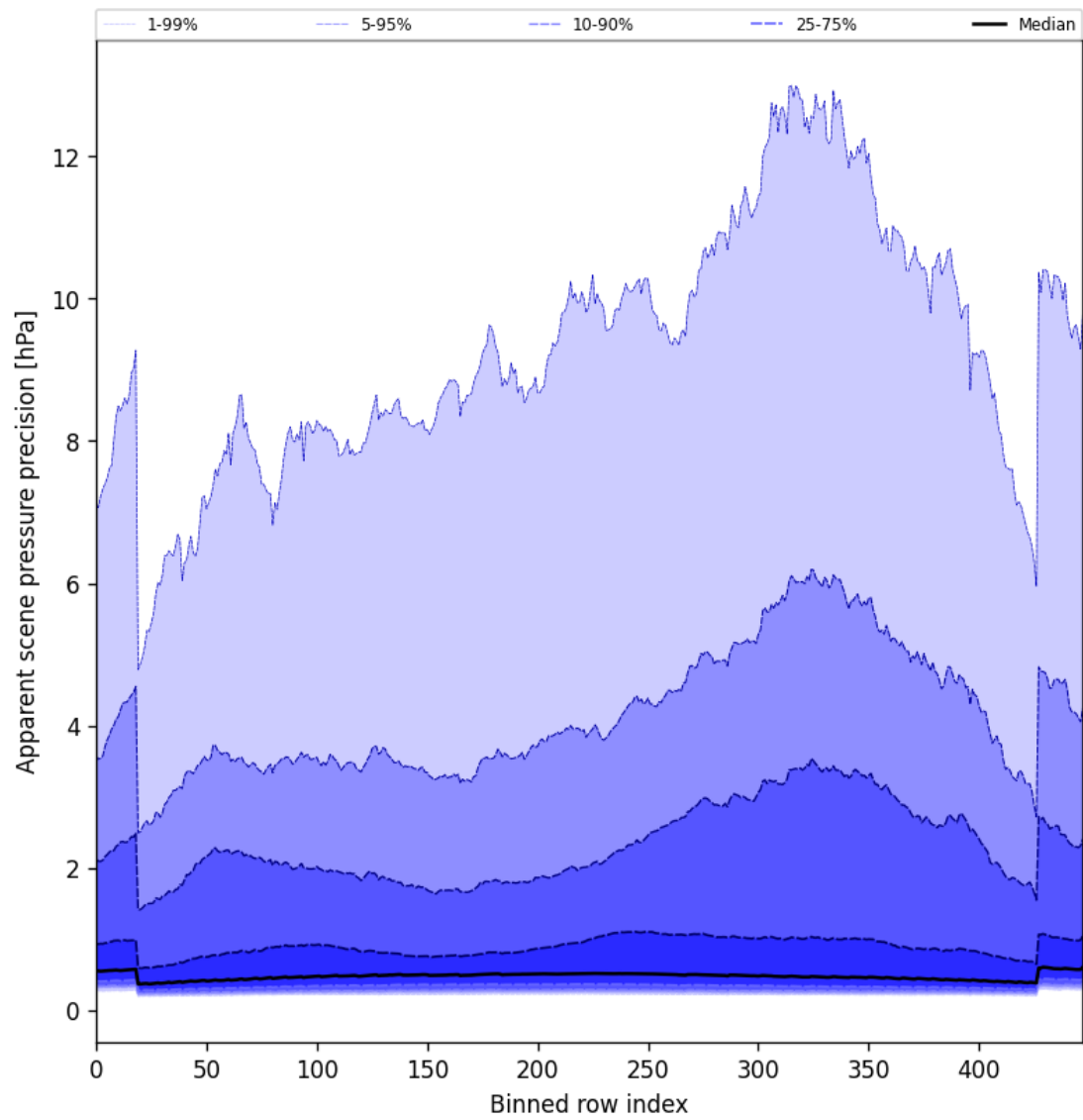
Figure 54: Along track statistics of “Apparent scene pressure precision” for 2025-08-04 to 2025-08-05
