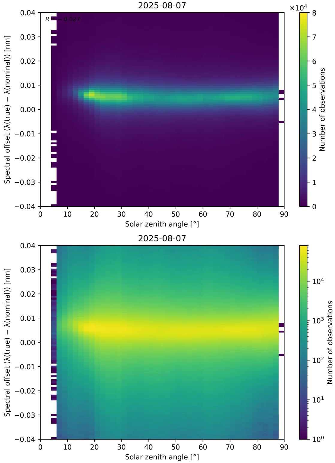
Figure 117: Scatter density plot of “Solar zenith angle” against “Spectral offset ( \lambda_{\text{true}} - \lambda_{\text{nominal}} )” for 2025-08-06 to 2025-08-08.
