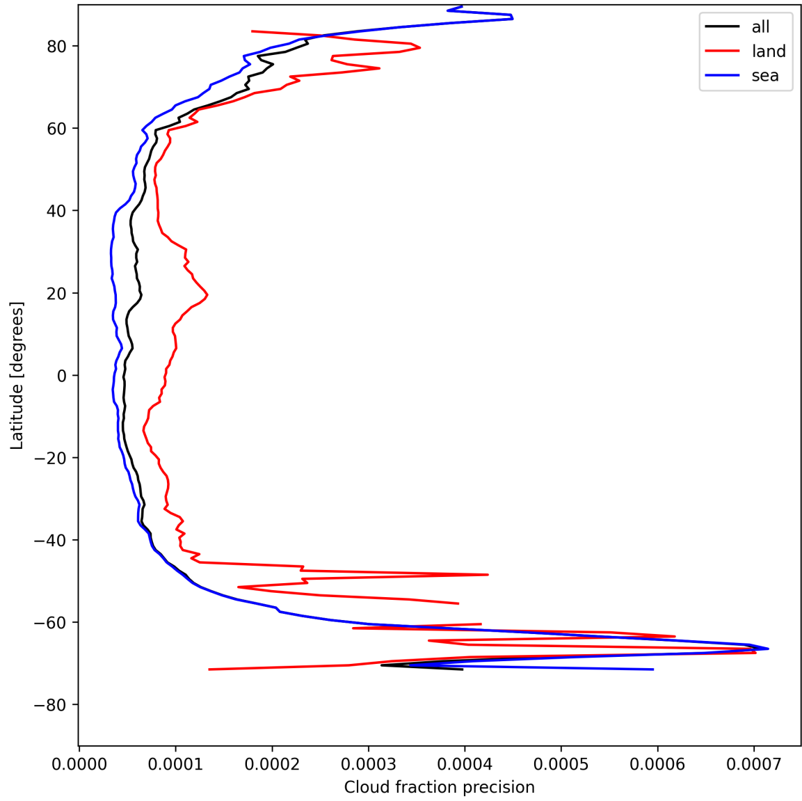
Figure 16: Zonal average of “Cloud fraction precision” for 2025-08-06 to 2025-08-08.
