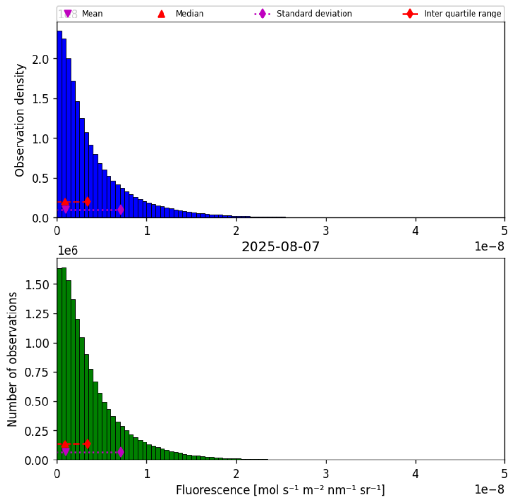
Figure 40: Histogram of “Fluorescence” for 2025-08-06 to 2025-08-08
