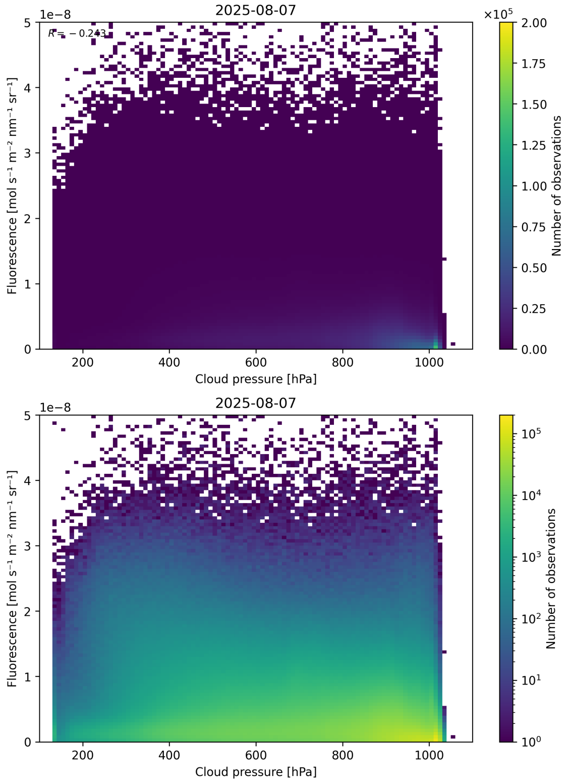
Figure 80: Scatter density plot of “Cloud pressure” against “Fluorescence” for 2025-08-06 to 2025-08-08.
