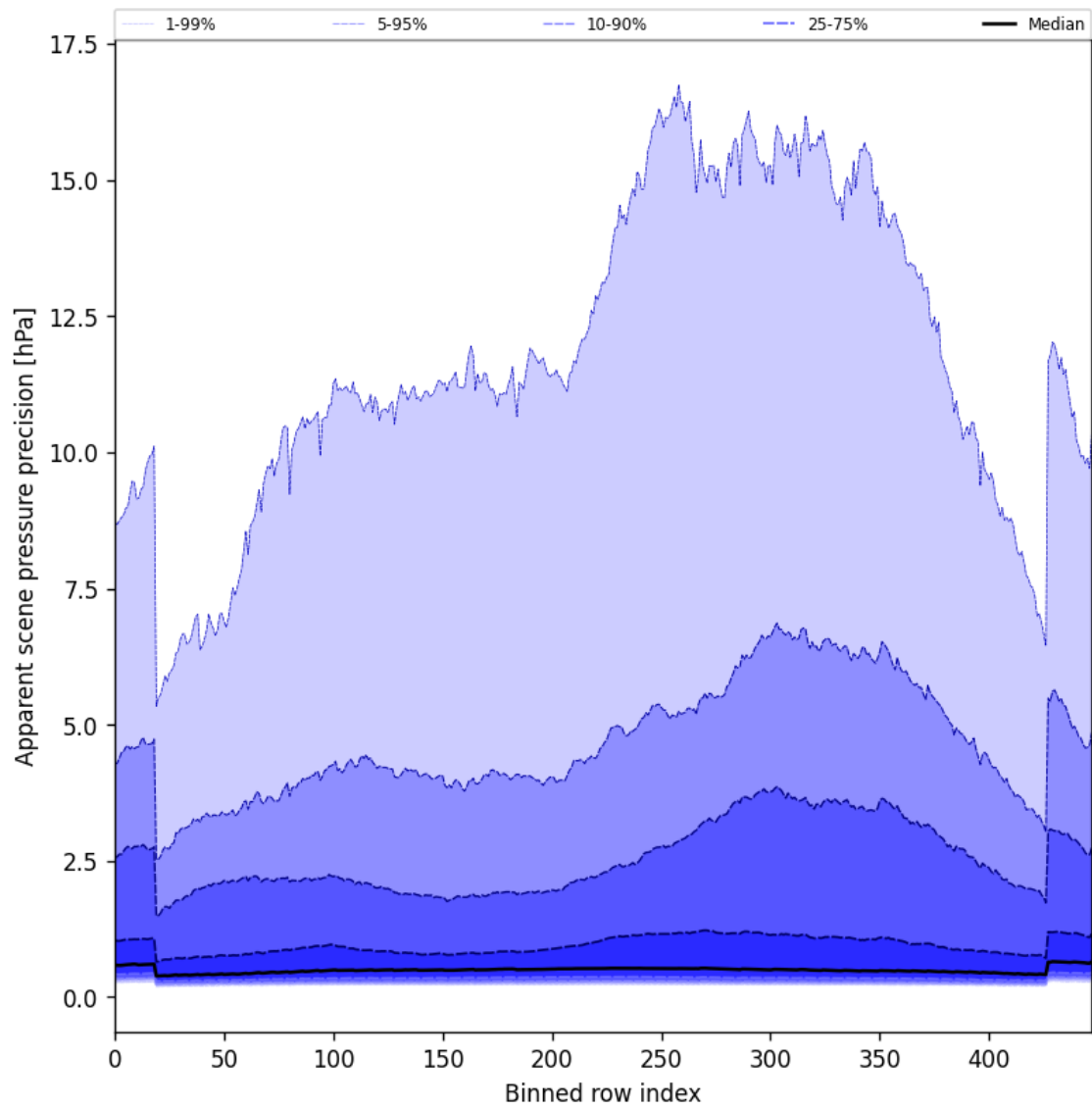
Figure 54: Along track statistics of “Apparent scene pressure precision” for 2025-08-06 to 2025-08-08
