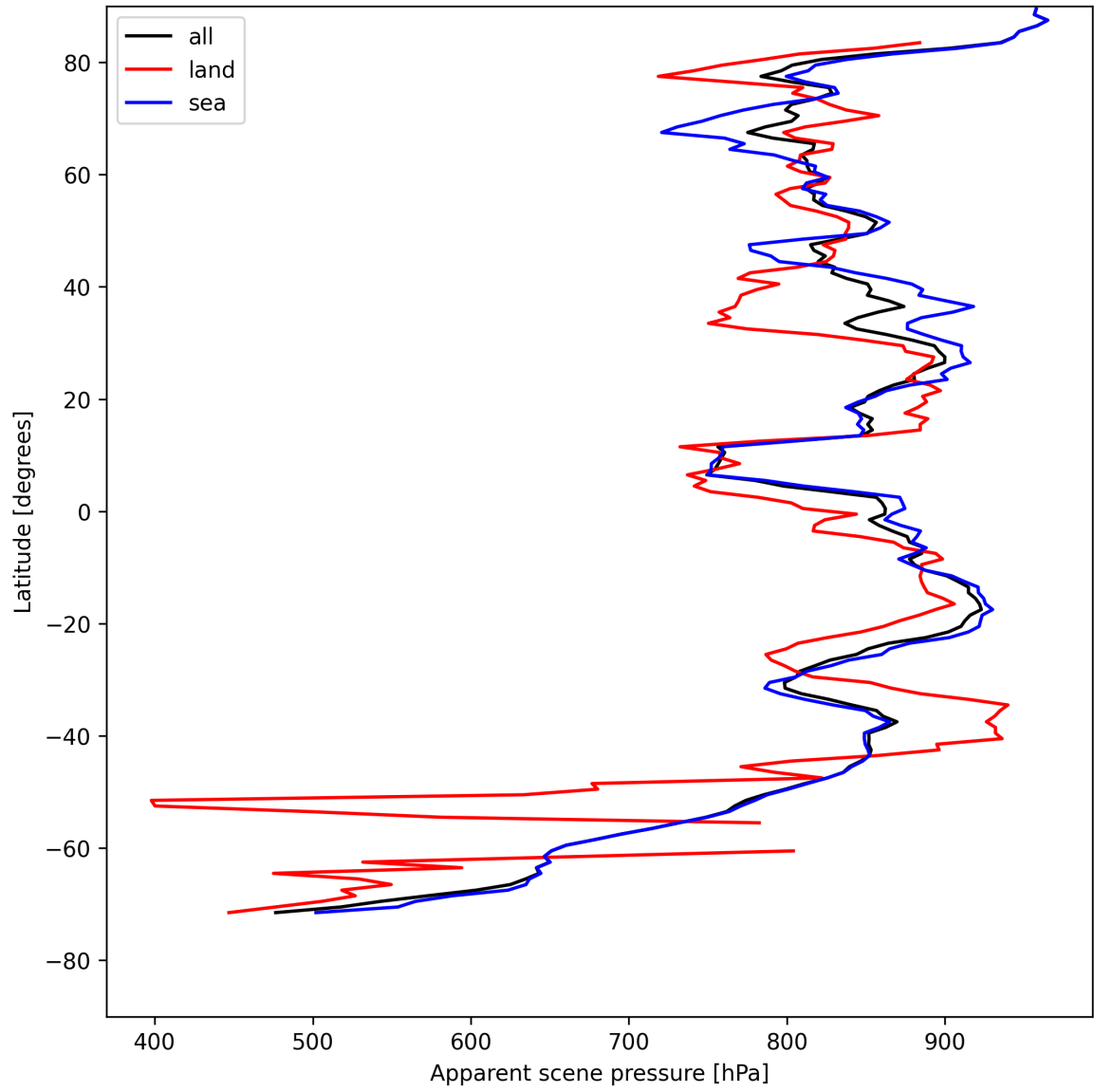
Figure 19: Zonal average of “Apparent scene pressure” for 2025-08-06 to 2025-08-08.
