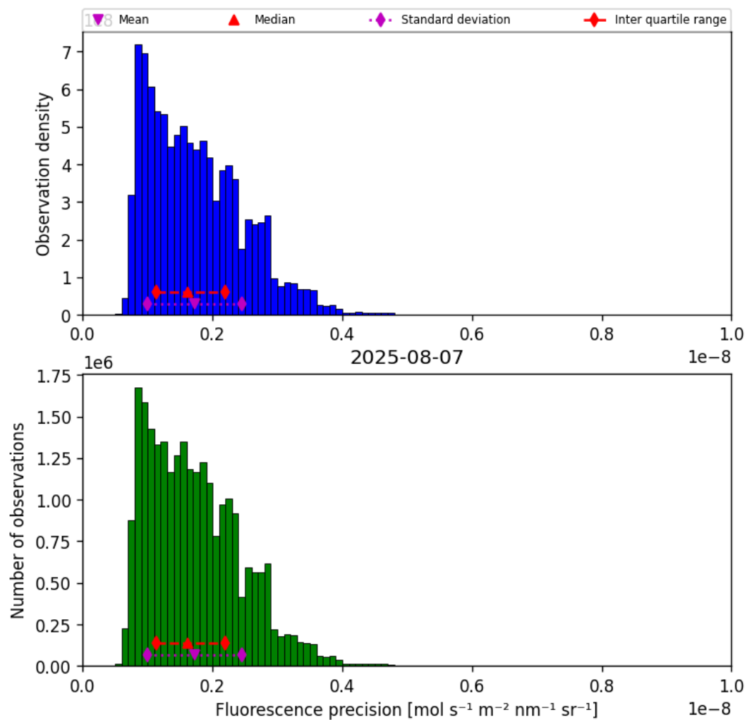
Figure 41: Histogram of “Fluorescence precision” for 2025-08-06 to 2025-08-08
