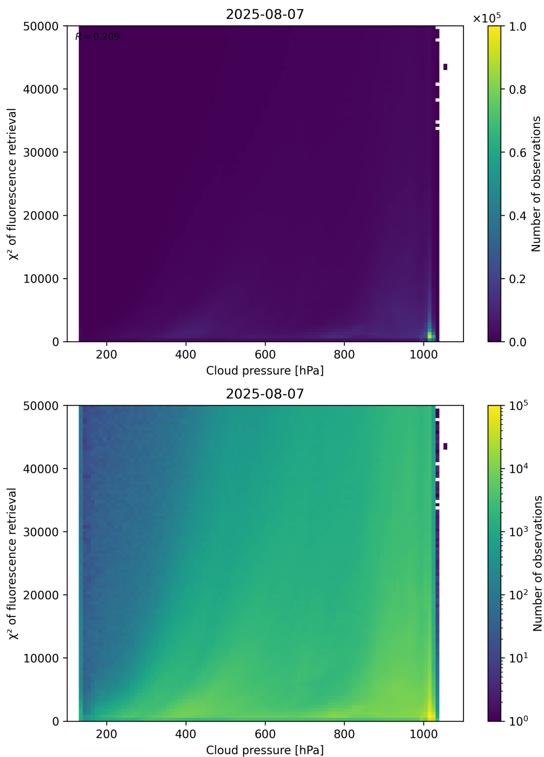
Figure 78: Scatter density plot of “Cloud pressure” against “ \chi^2 of fluorescence retrieval” for 2025-08-06 to 2025-08-08.
