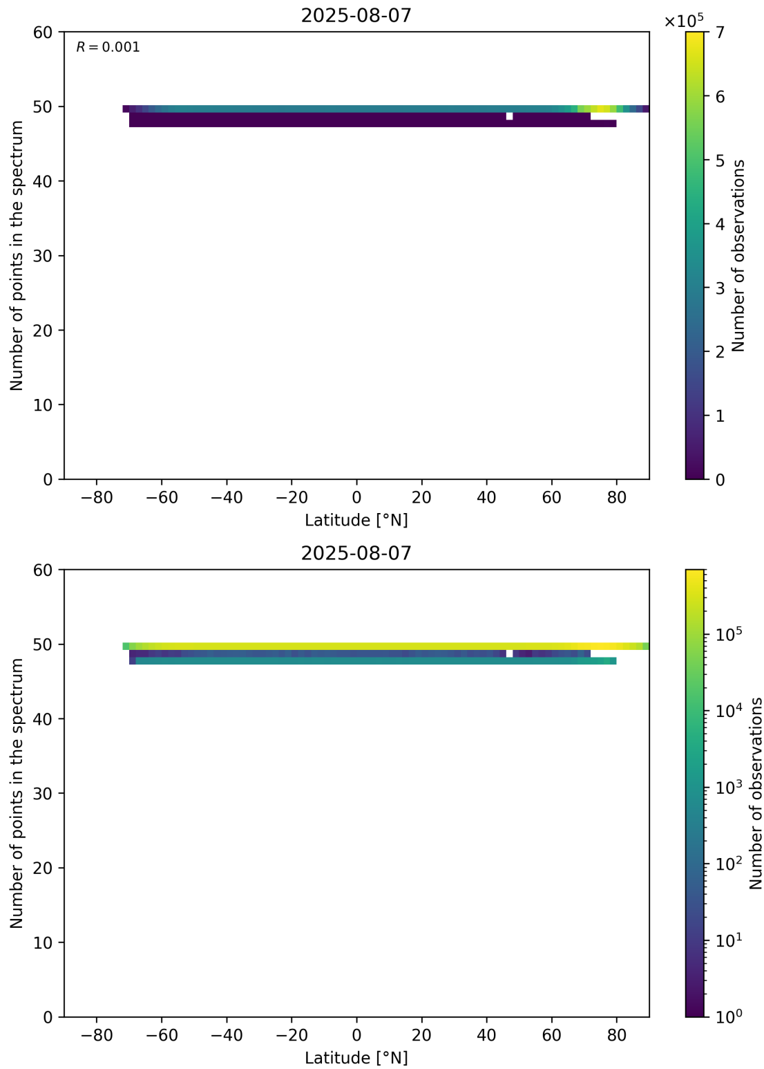
Figure 94: Scatter density plot of “Latitude” against “Number of points in the spectrum” for 2025-08-06 to 2025-08-08.
