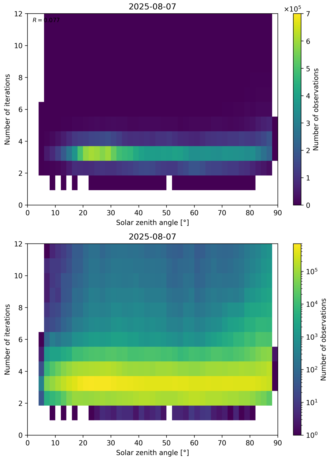
Figure 114: Scatter density plot of “Solar zenith angle” against “Number of iterations” for 2025-08-06 to 2025-08-08.
