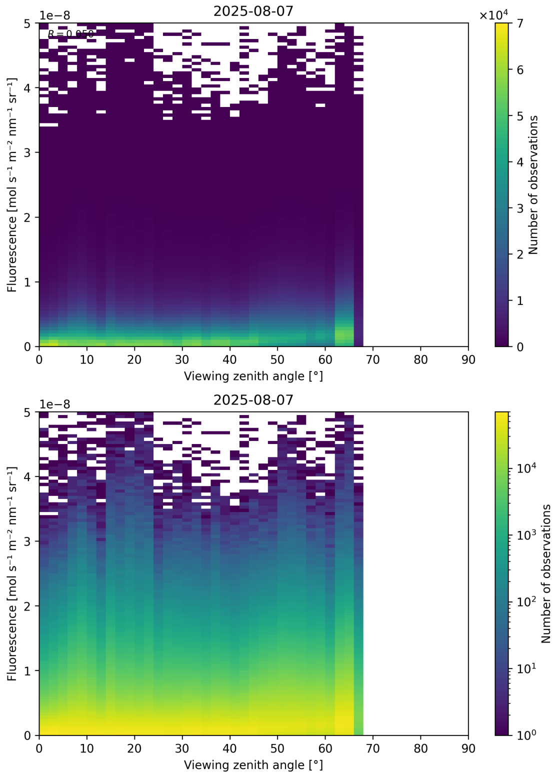
Figure 122: Scatter density plot of “Viewing zenith angle” against “Fluorescence” for 2025-08-06 to 2025-08-08.
