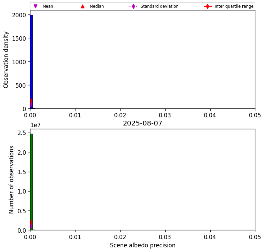
Figure 35: Histogram of “Scene albedo precision” for 2025-08-06 to 2025-08-08
