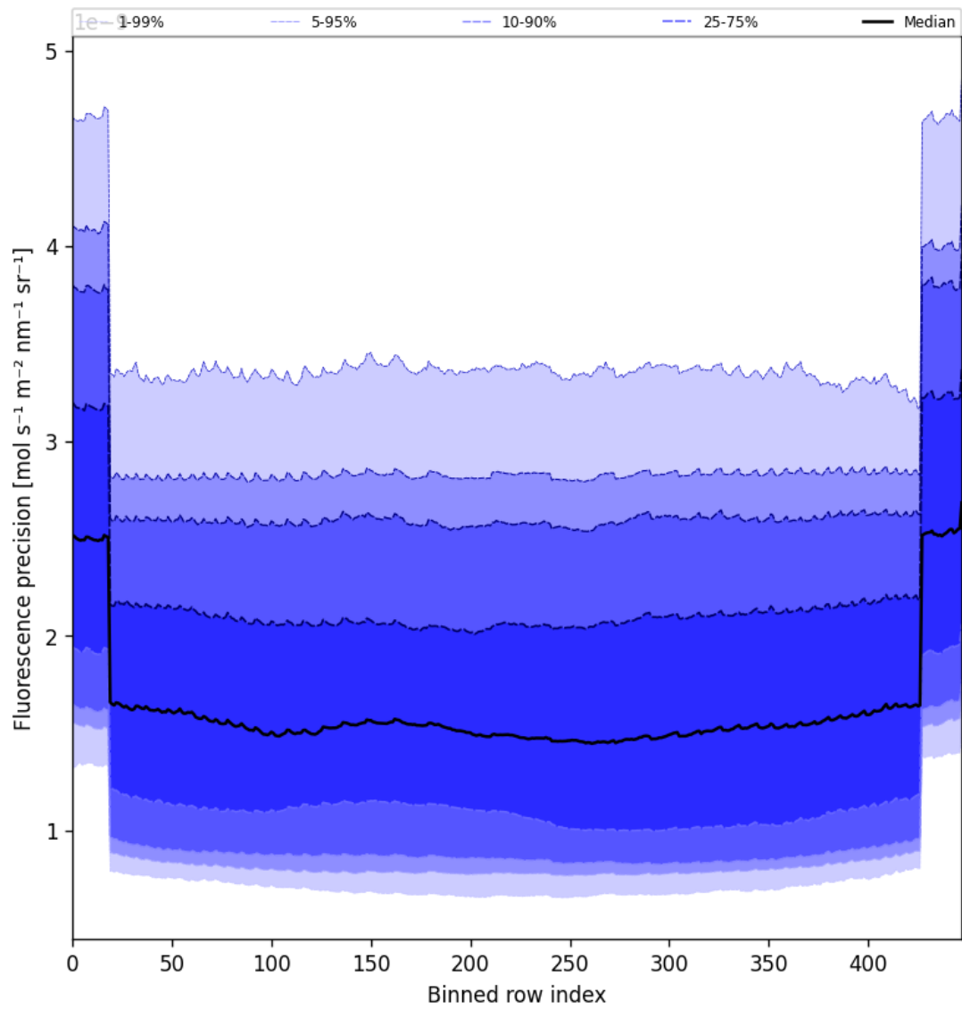
Figure 58: Along track statistics of “Fluorescence precision” for 2025-08-06 to 2025-08-08
