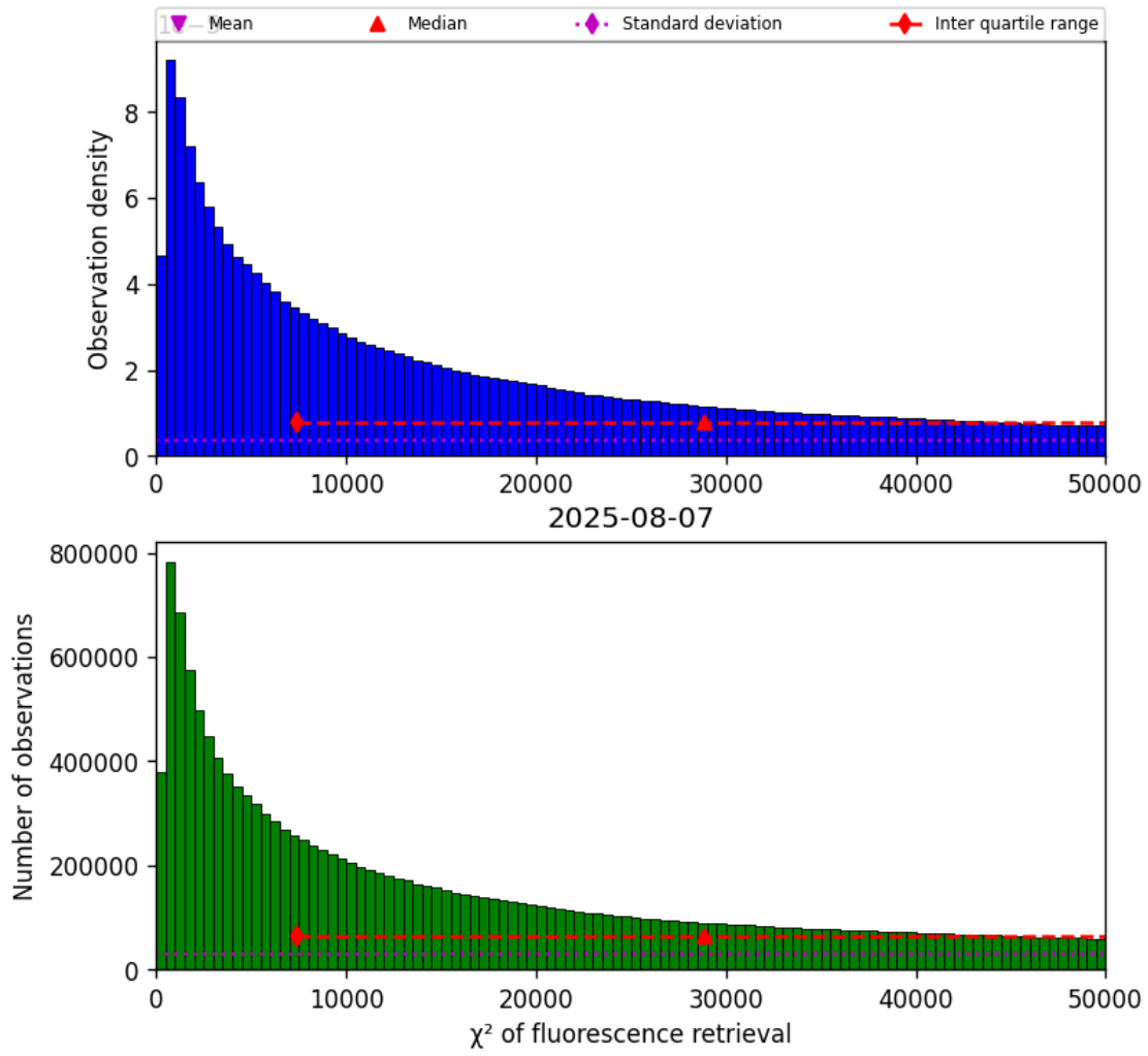
Figure 42: Histogram of “ \chi^2 of fluorescence retrieval” for 2025-08-06 to 2025-08-08
