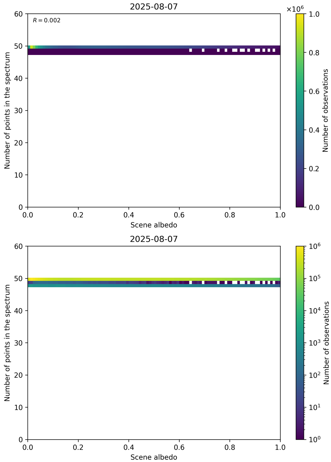
Figure 106: Scatter density plot of “Scene albedo” against “Number of points in the spectrum” for 2025-08-06 to 2025-08-08.
