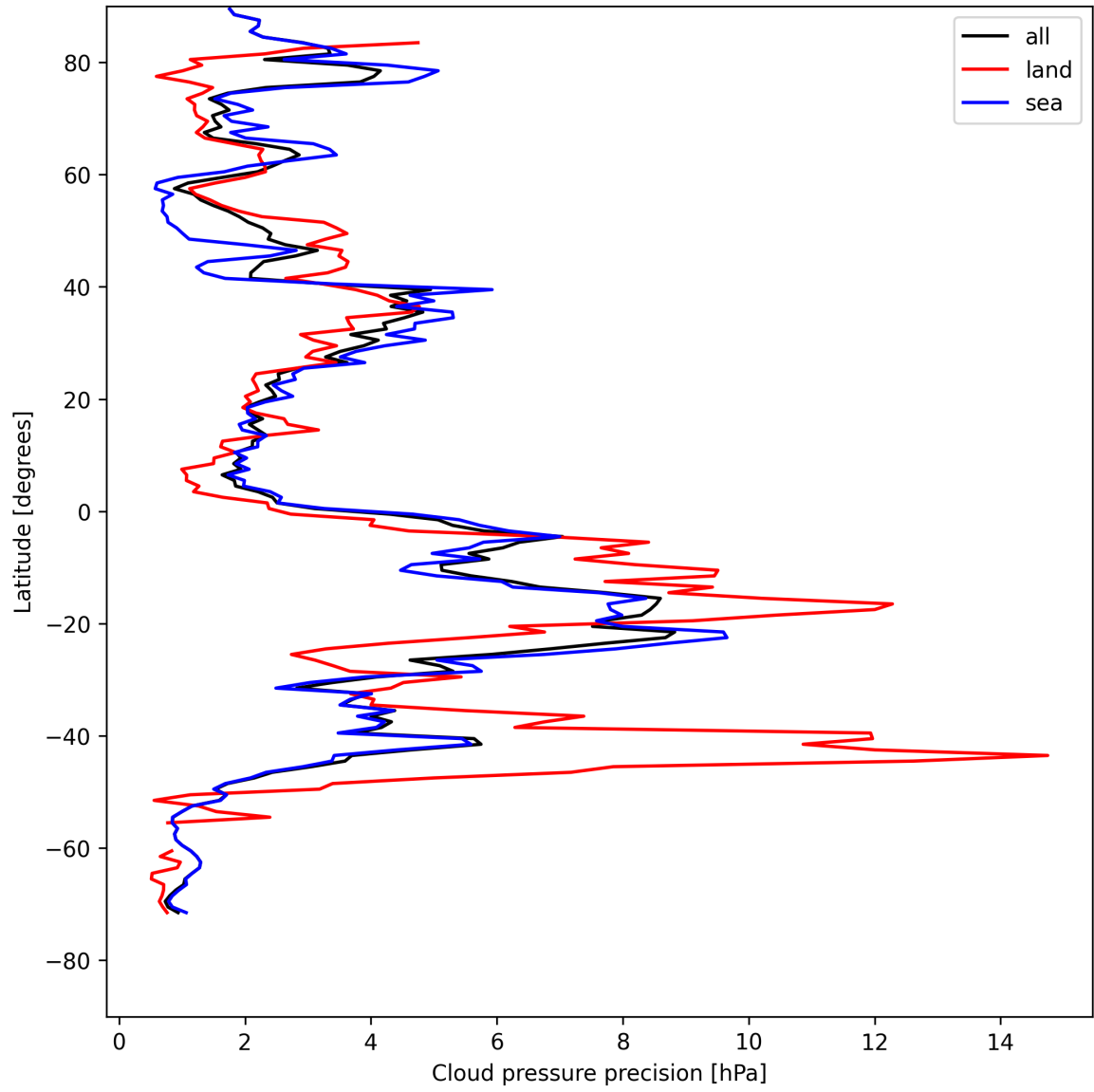
Figure 14: Zonal average of “Cloud pressure precision” for 2025-08-06 to 2025-08-08.
