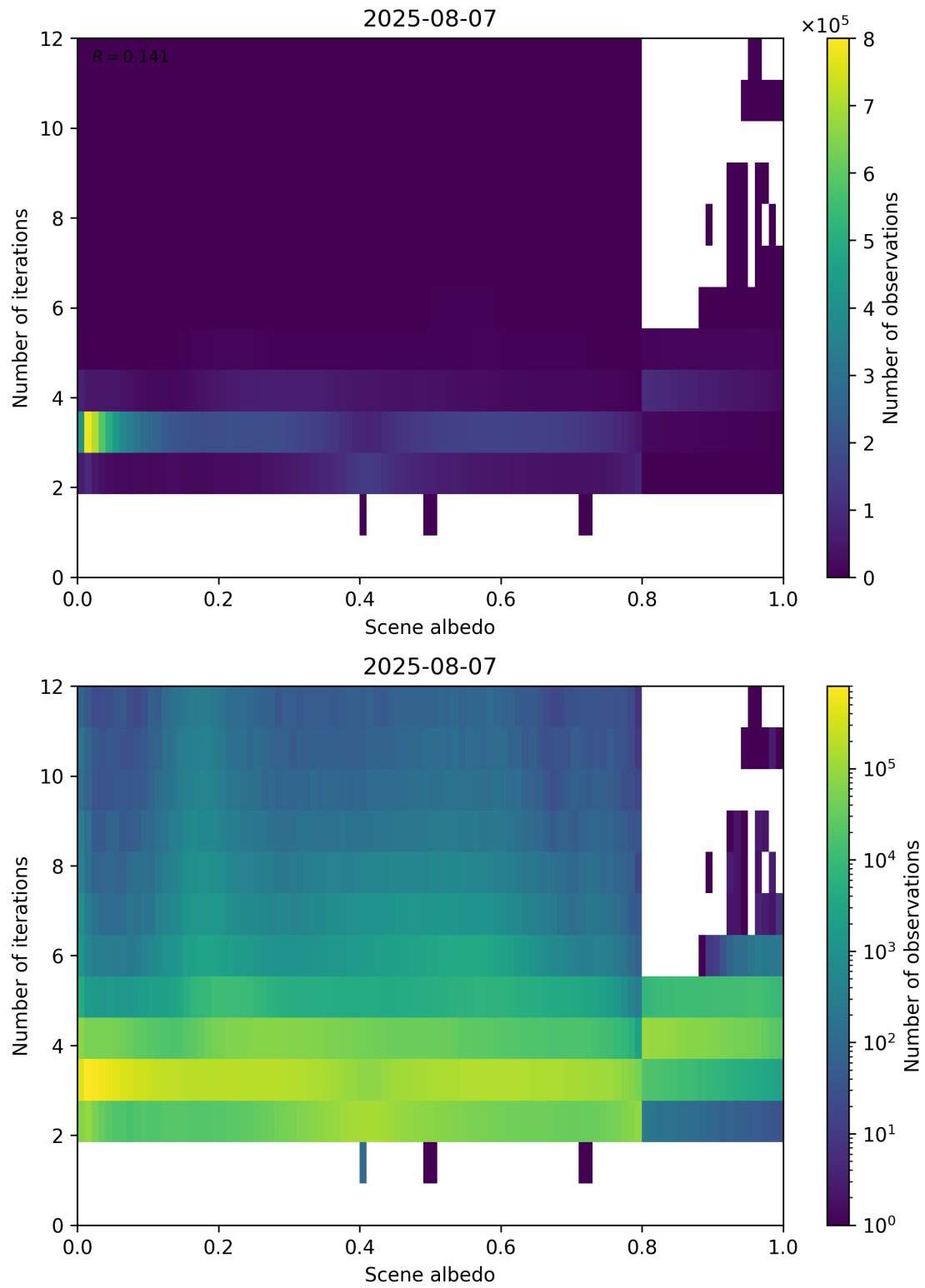
Figure 105: Scatter density plot of “Scene albedo” against “Number of iterations” for 2025-08-06 to 2025-08-08.
