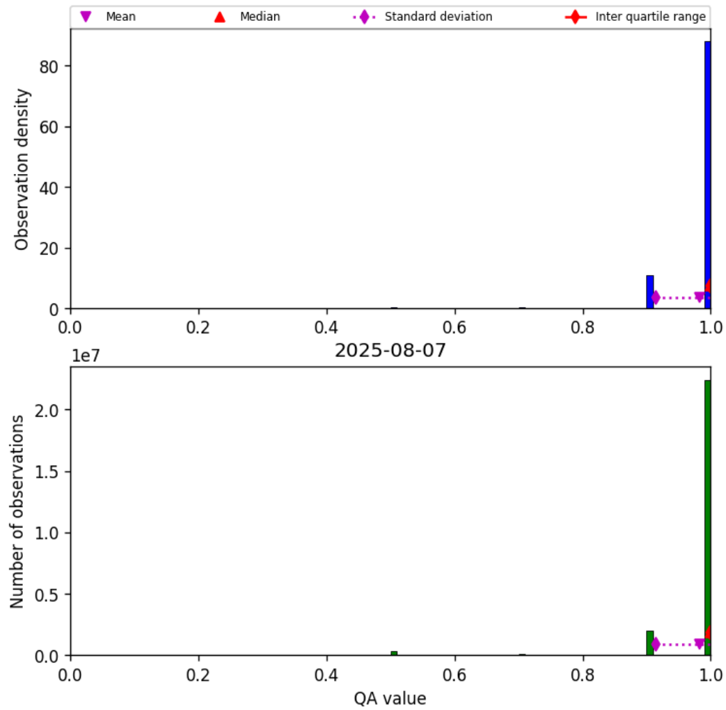
Figure 29: Histogram of “QA value” for 2025-08-06 to 2025-08-08
