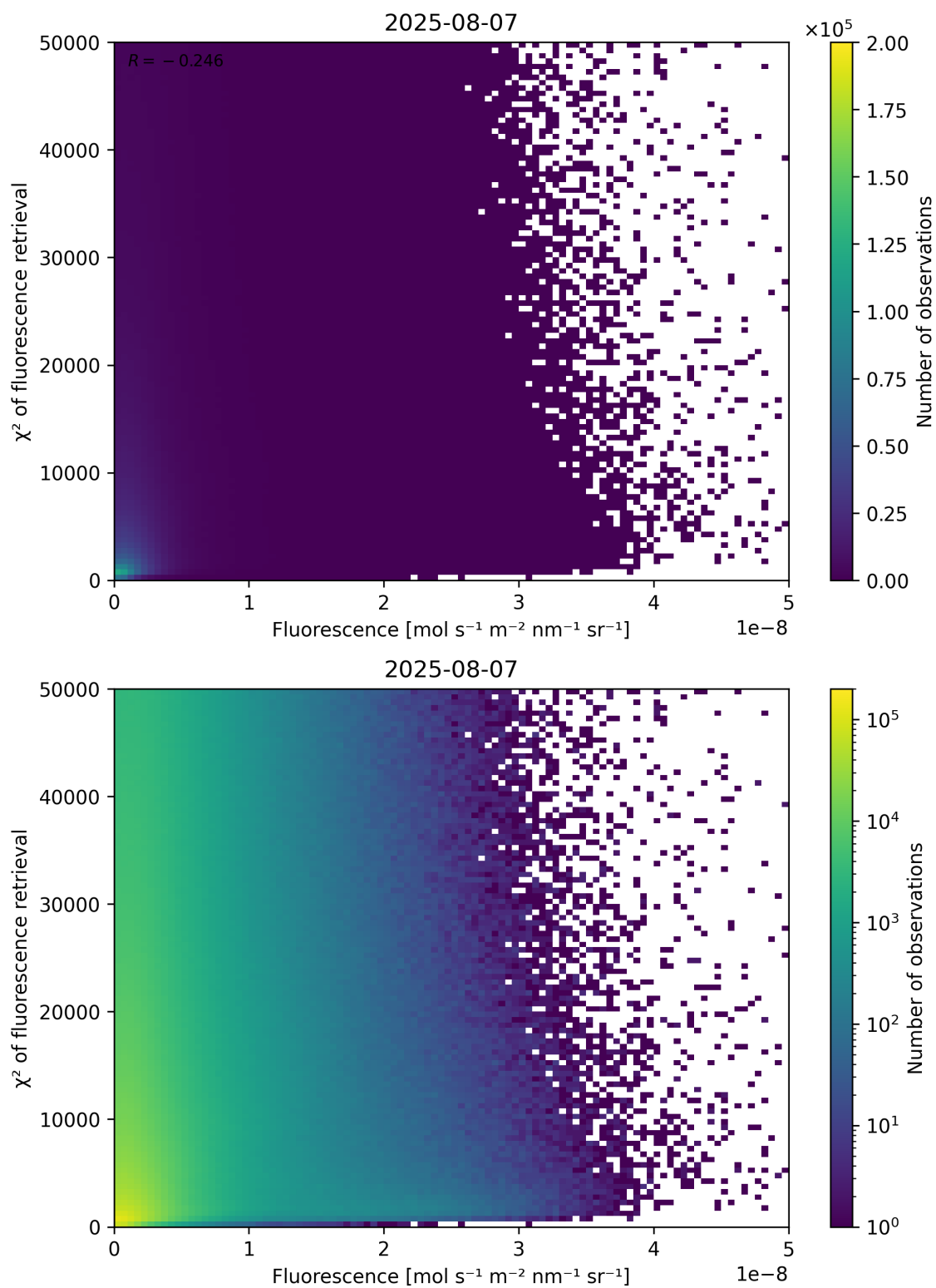
Figure 85: Scatter density plot of “Fluorescence” against “ \chi^2 of fluorescence retrieval” for 2025-08-06 to 2025-08-08.
