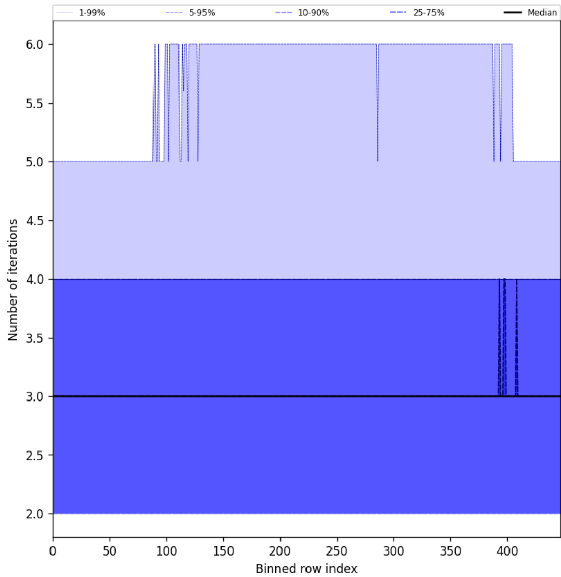
Figure 56: Along track statistics of “Number of iterations” for 2025-08-06 to 2025-08-08
