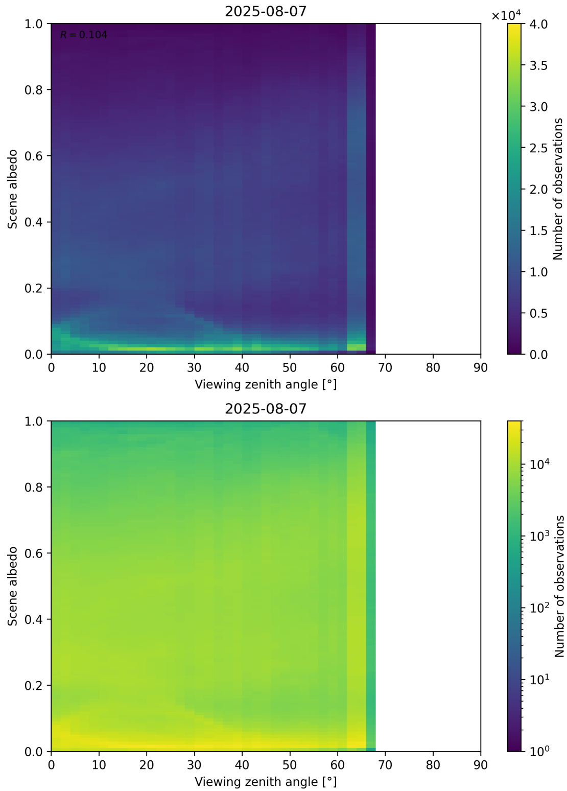
Figure 126: Scatter density plot of “Viewing zenith angle” against “Scene albedo” for 2025-08-06 to 2025-08-08.
