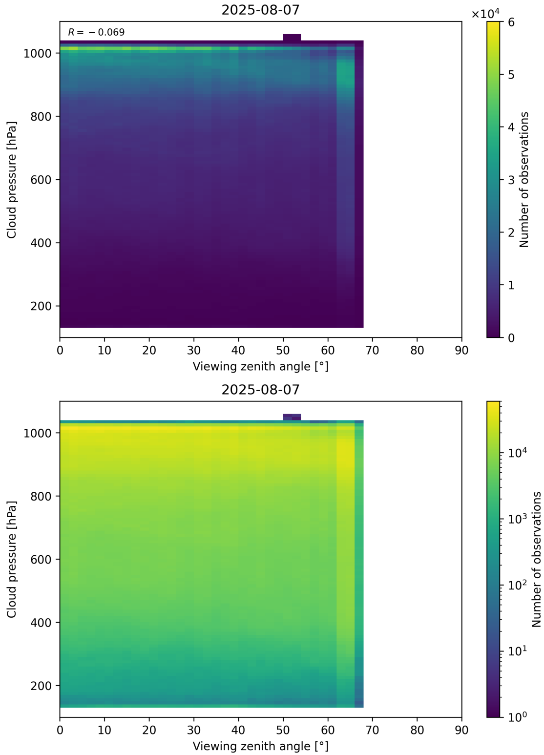
Figure 121: Scatter density plot of “Viewing zenith angle” against “Cloud pressure” for 2025-08-06 to 2025-08-08.
