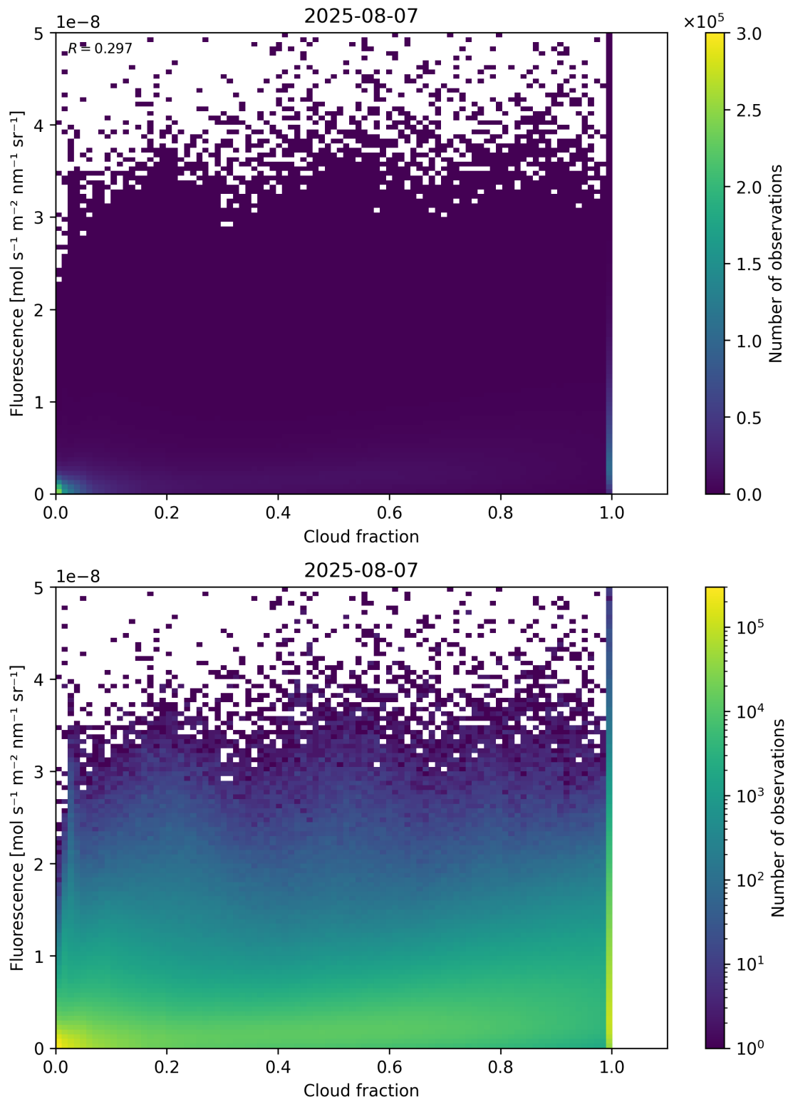
Figure 72: Scatter density plot of “Cloud fraction” against “Fluorescence” for 2025-08-06 to 2025-08-08.
