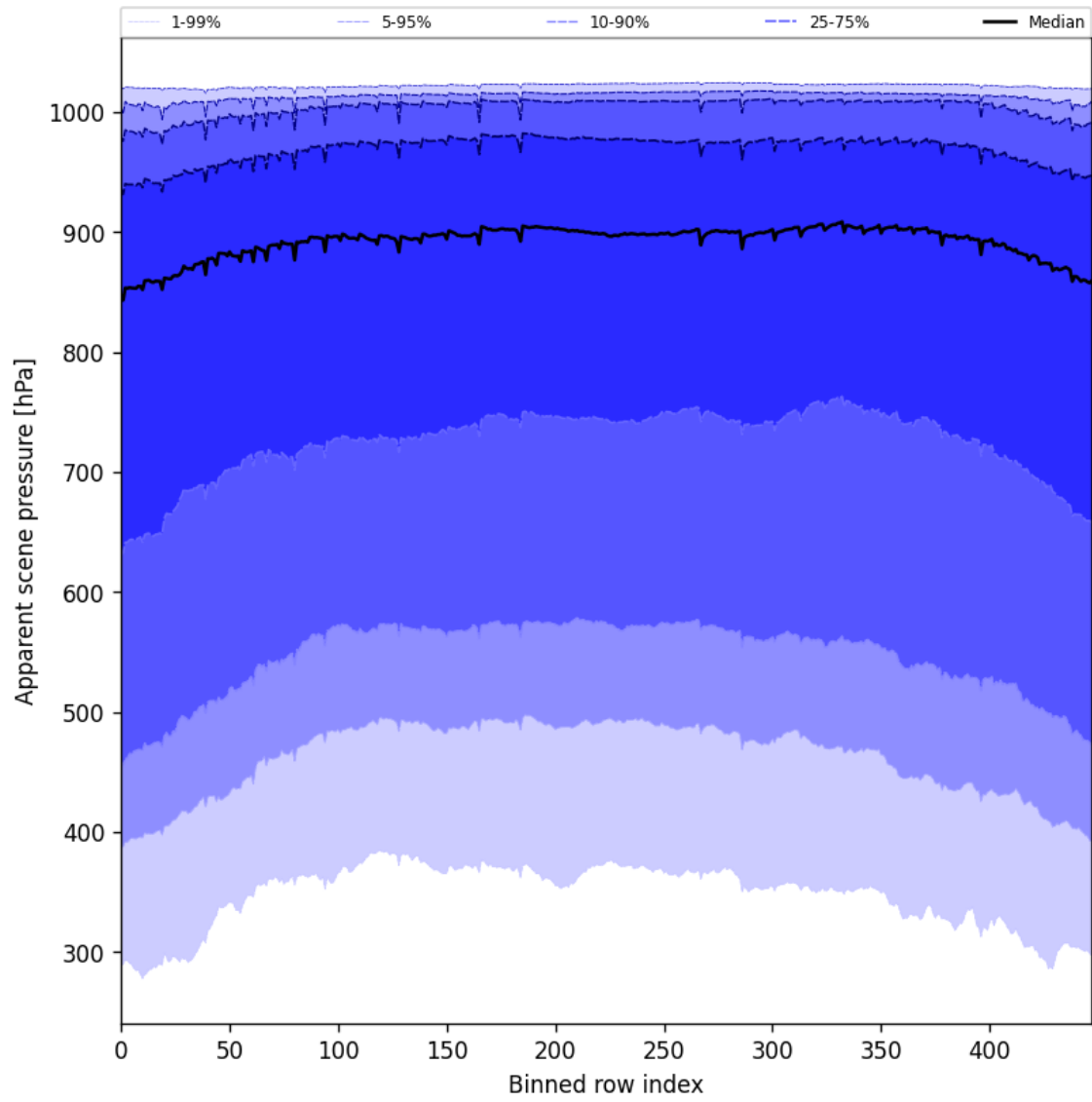
Figure 53: Along track statistics of “Apparent scene pressure” for 2025-08-06 to 2025-08-08
