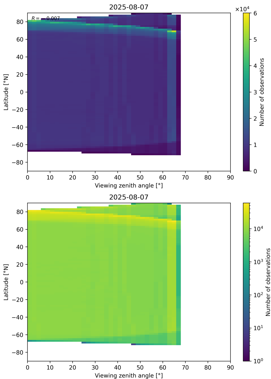
Figure 123: Scatter density plot of “Viewing zenith angle” against “Latitude” for 2025-08-06 to 2025-08-08.
