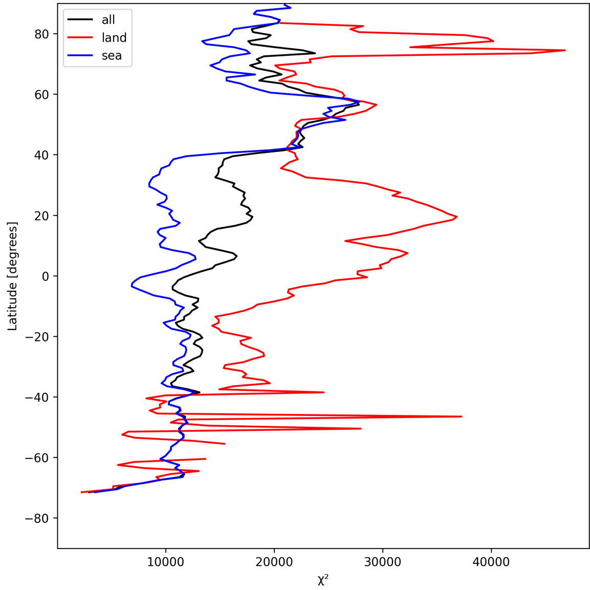
Figure 21: Zonal average of “ \chi^2 ” for 2025-08-06 to 2025-08-08.
