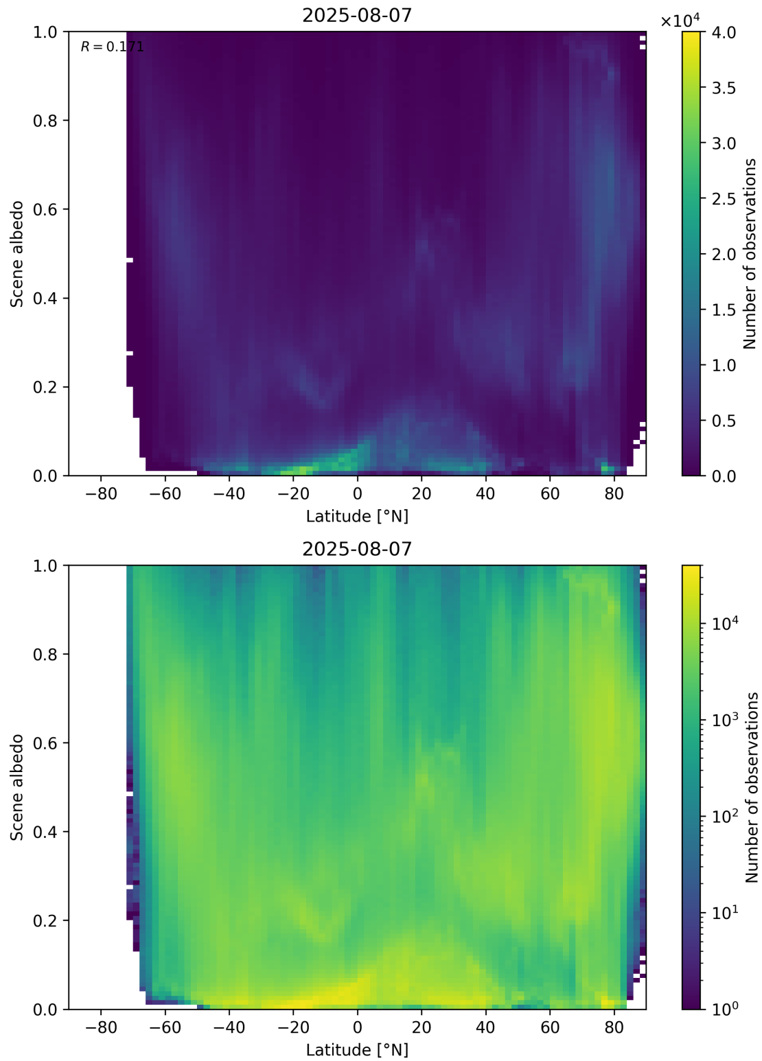
Figure 95: Scatter density plot of “Latitude” against “Scene albedo” for 2025-08-06 to 2025-08-08.
