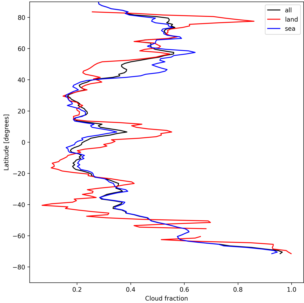
Figure 15: Zonal average of “Cloud fraction” for 2025-08-06 to 2025-08-08.
