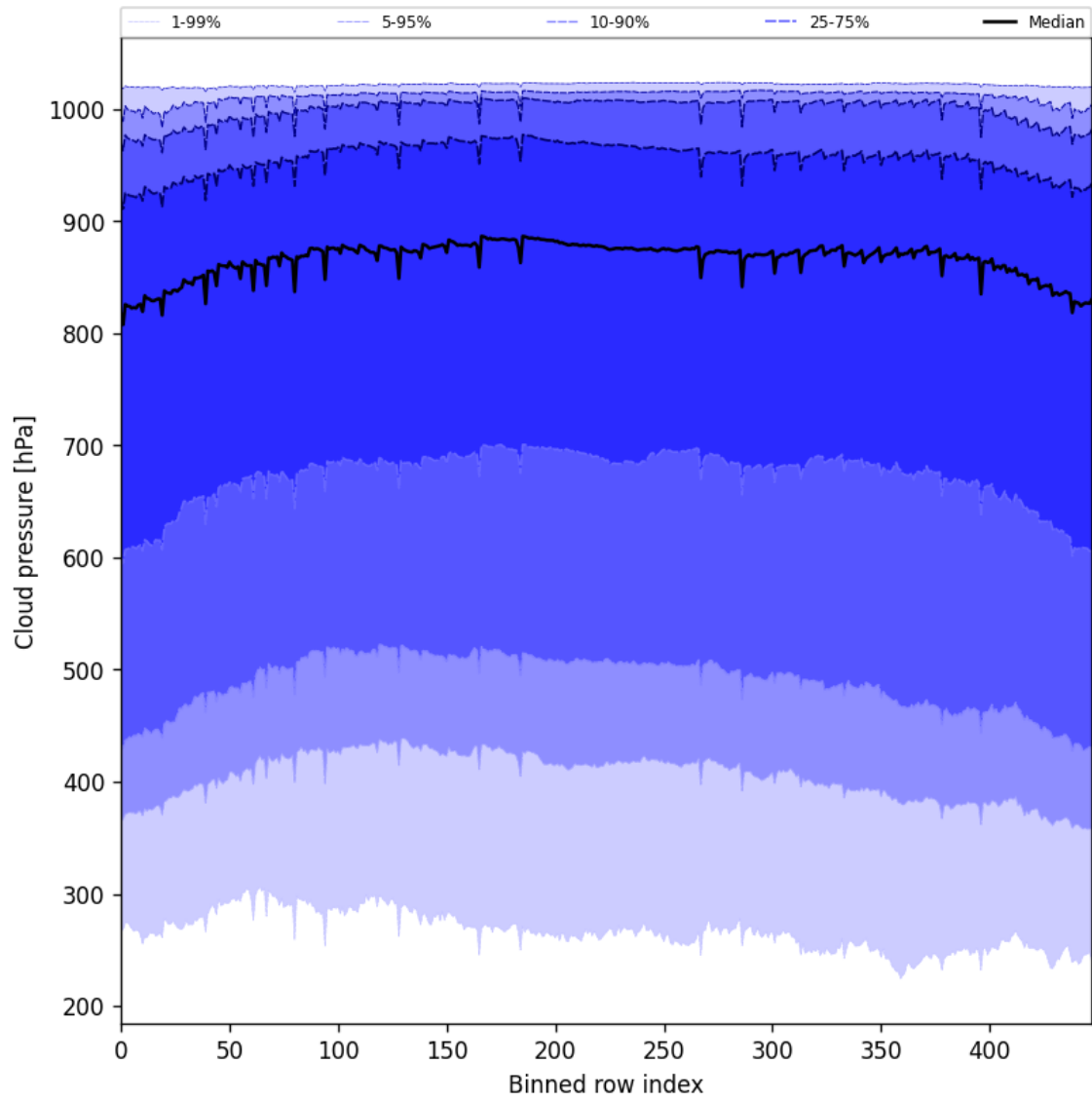
Figure 47: Along track statistics of “Cloud pressure” for 2025-08-06 to 2025-08-08
