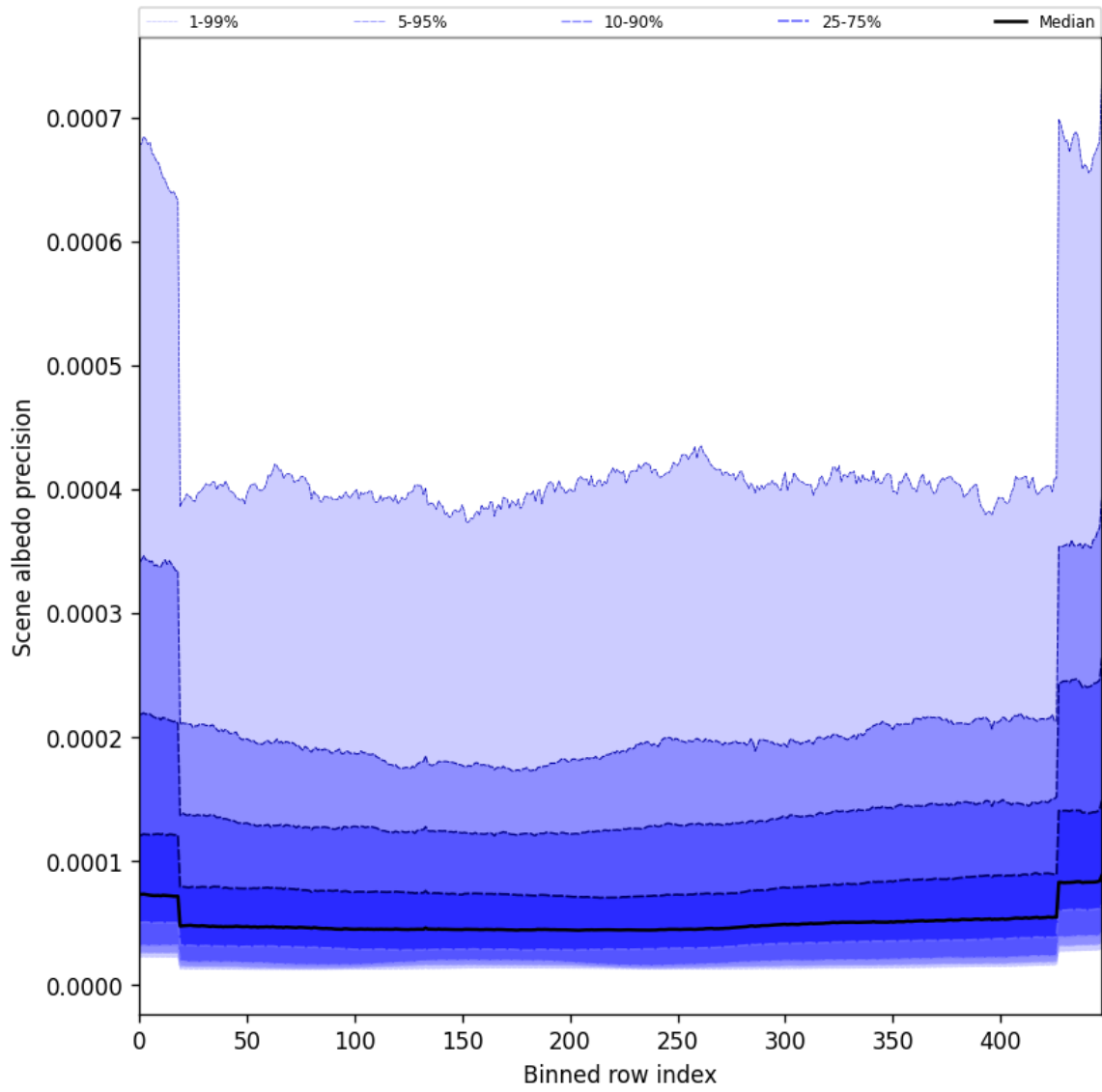
Figure 52: Along track statistics of “Scene albedo precision” for 2025-08-06 to 2025-08-08
