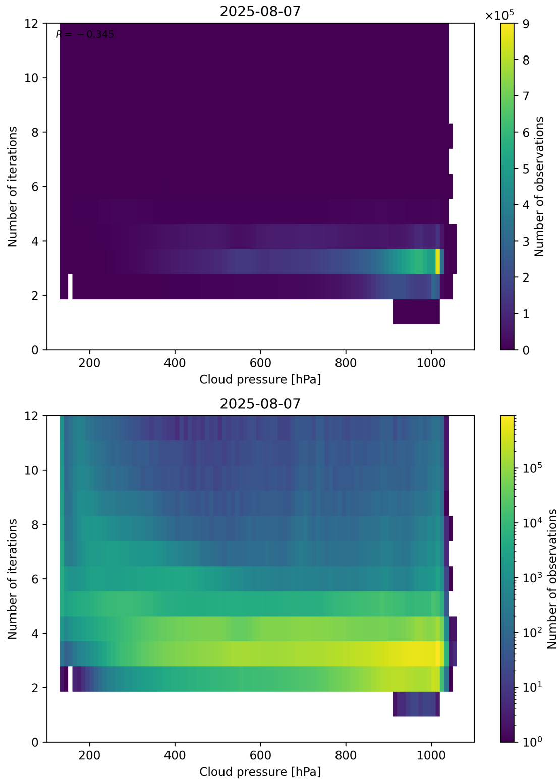
Figure 81: Scatter density plot of “Cloud pressure” against “Number of iterations” for 2025-08-06 to 2025-08-08.
