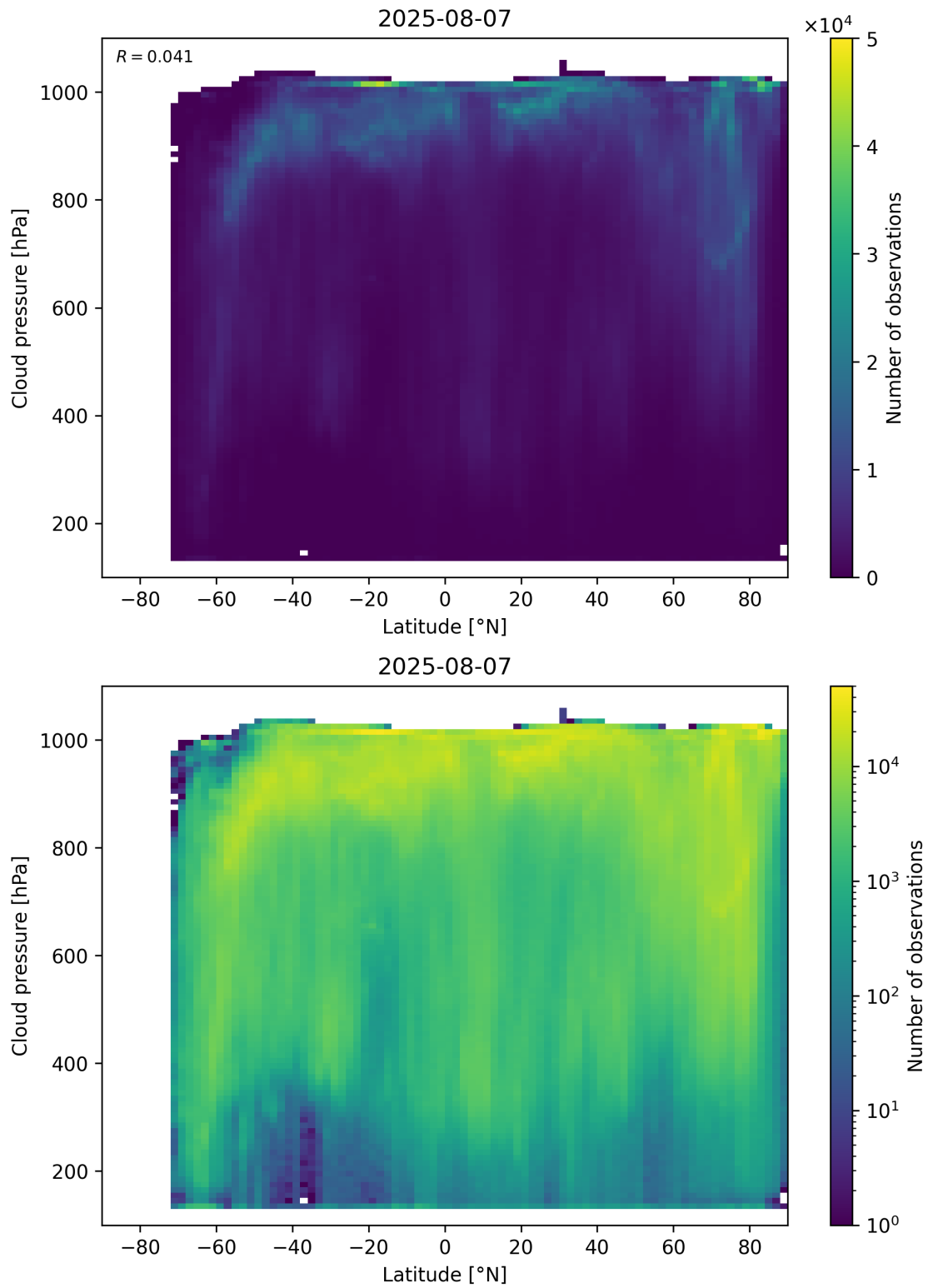
Figure 91: Scatter density plot of “Latitude” against “Cloud pressure” for 2025-08-06 to 2025-08-08.
