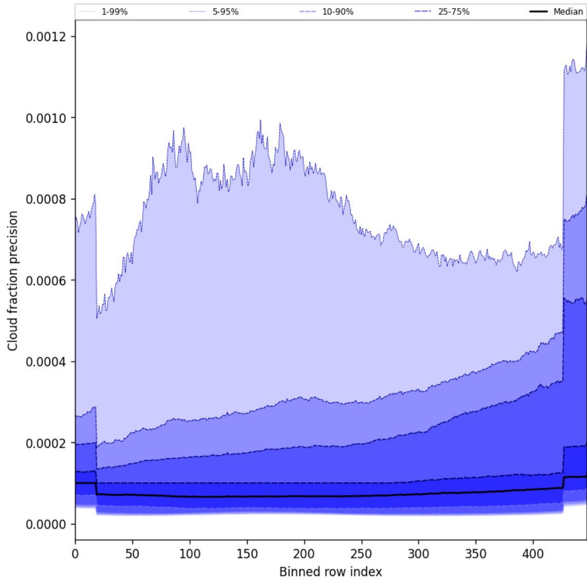
Figure 50: Along track statistics of “Cloud fraction precision” for 2025-08-06 to 2025-08-08
