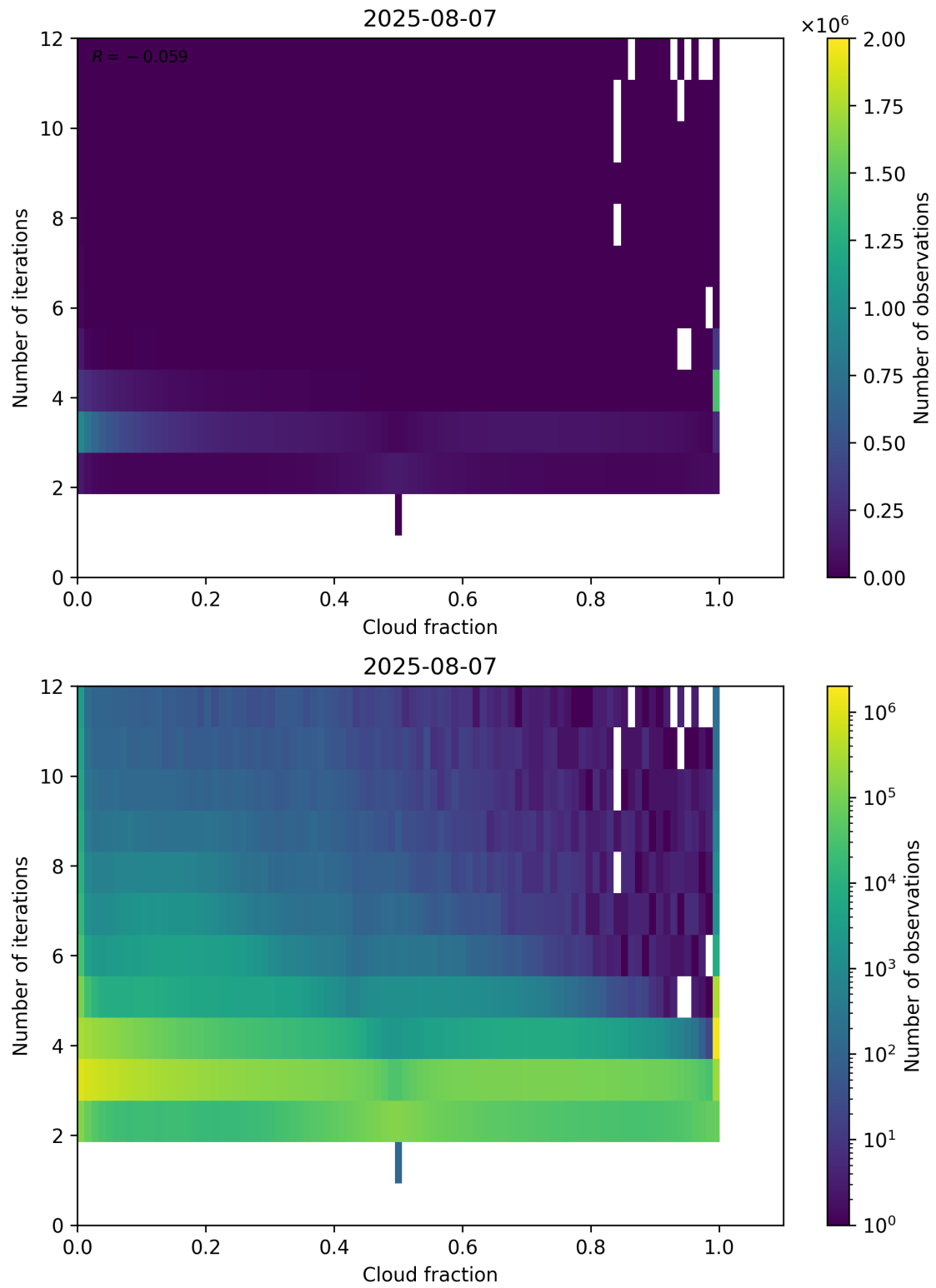
Figure 73: Scatter density plot of “Cloud fraction” against “Number of iterations” for 2025-08-06 to 2025-08-08.
