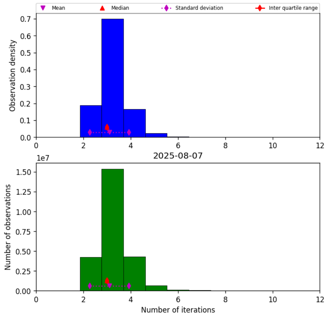
Figure 39: Histogram of “Number of iterations” for 2025-08-06 to 2025-08-08
