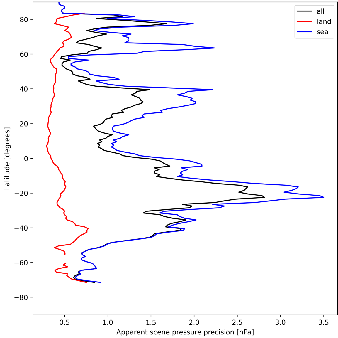
Figure 20: Zonal average of “Apparent scene pressure precision” for 2025-08-06 to 2025-08-08.
