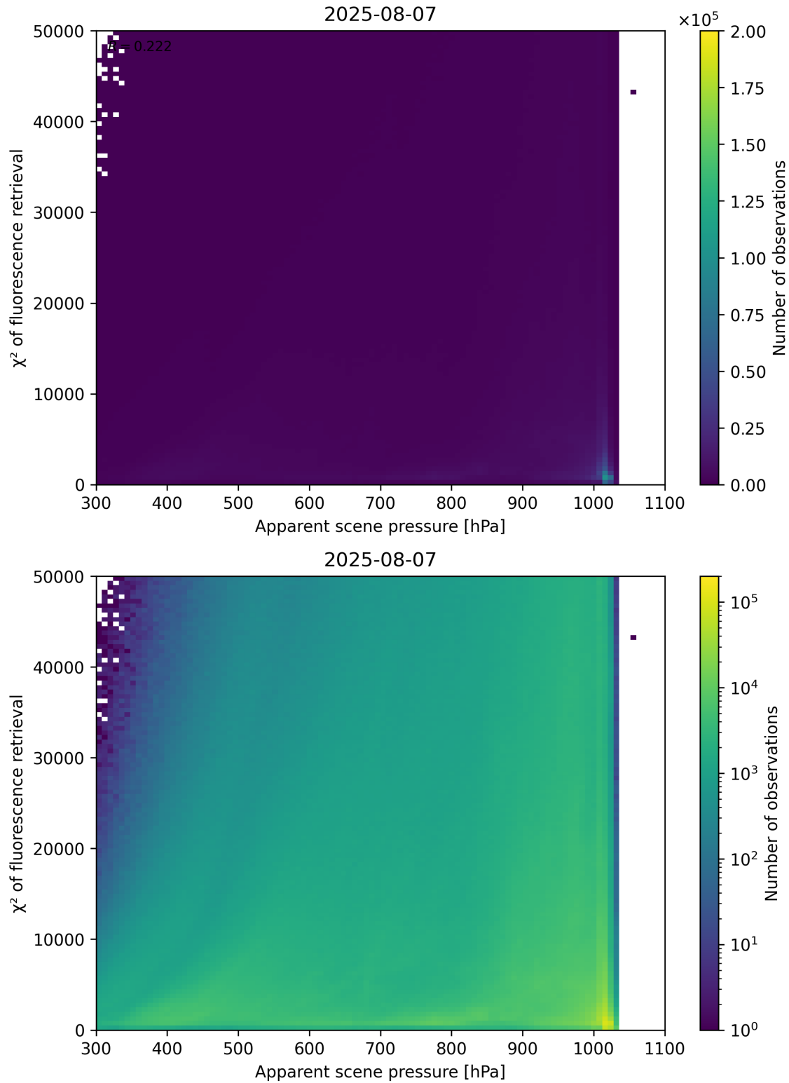
Figure 63: Scatter density plot of “Apparent scene pressure” against “ \chi^2 of fluorescence retrieval” for 2025-08-06 to 2025-08-08.
