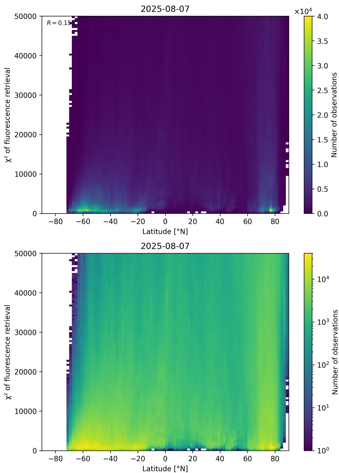
Figure 89: Scatter density plot of “Latitude” against “ \chi^2 of fluorescence retrieval” for 2025-08-06 to 2025-08-08.
