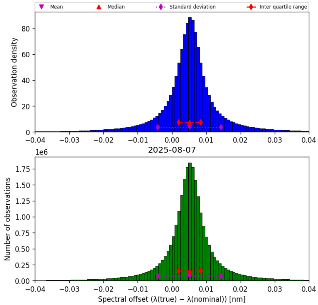
Figure 45: Histogram of “Spectral offset ( \lambda_{\text{true}} - \lambda_{\text{nominal}} )” for 2025-08-06 to 2025-08-08
