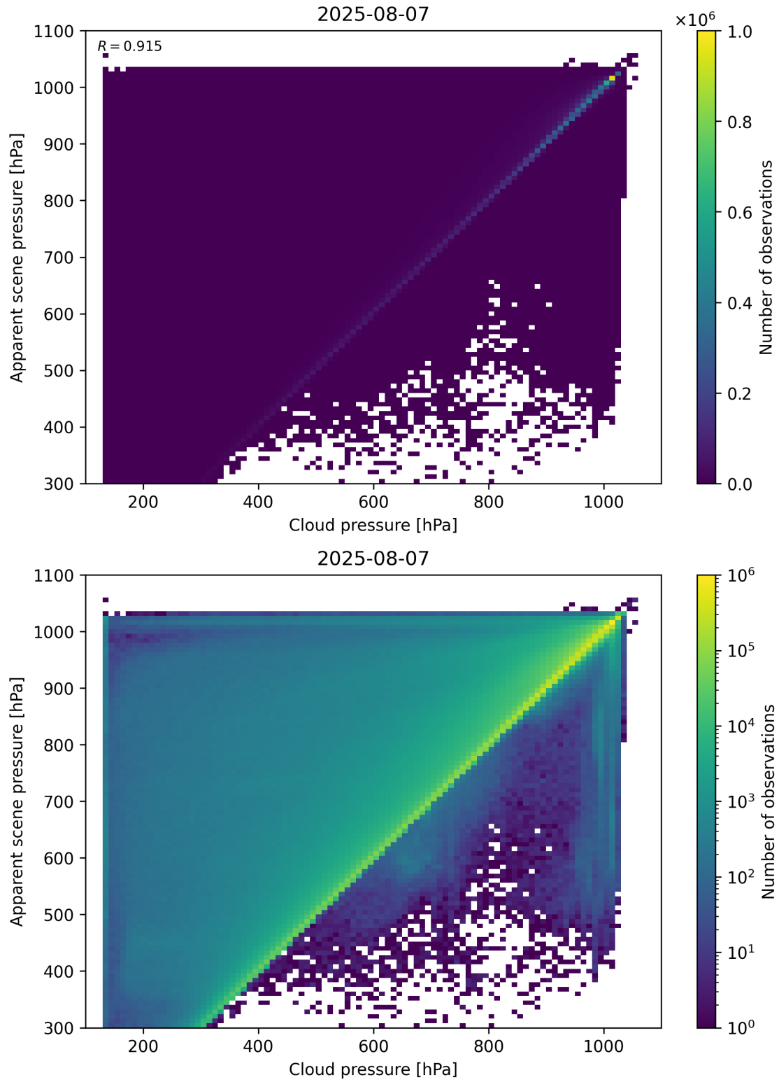
Figure 77: Scatter density plot of “Cloud pressure” against “Apparent scene pressure” for 2025-08-06 to 2025-08-08.
