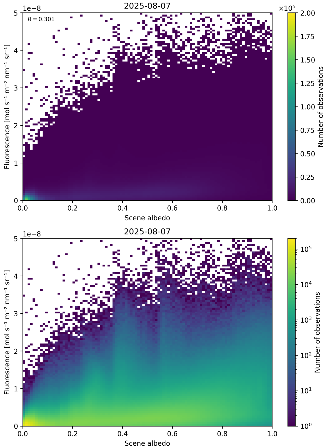
Figure 104: Scatter density plot of “Scene albedo” against “Fluorescence” for 2025-08-06 to 2025-08-08.
