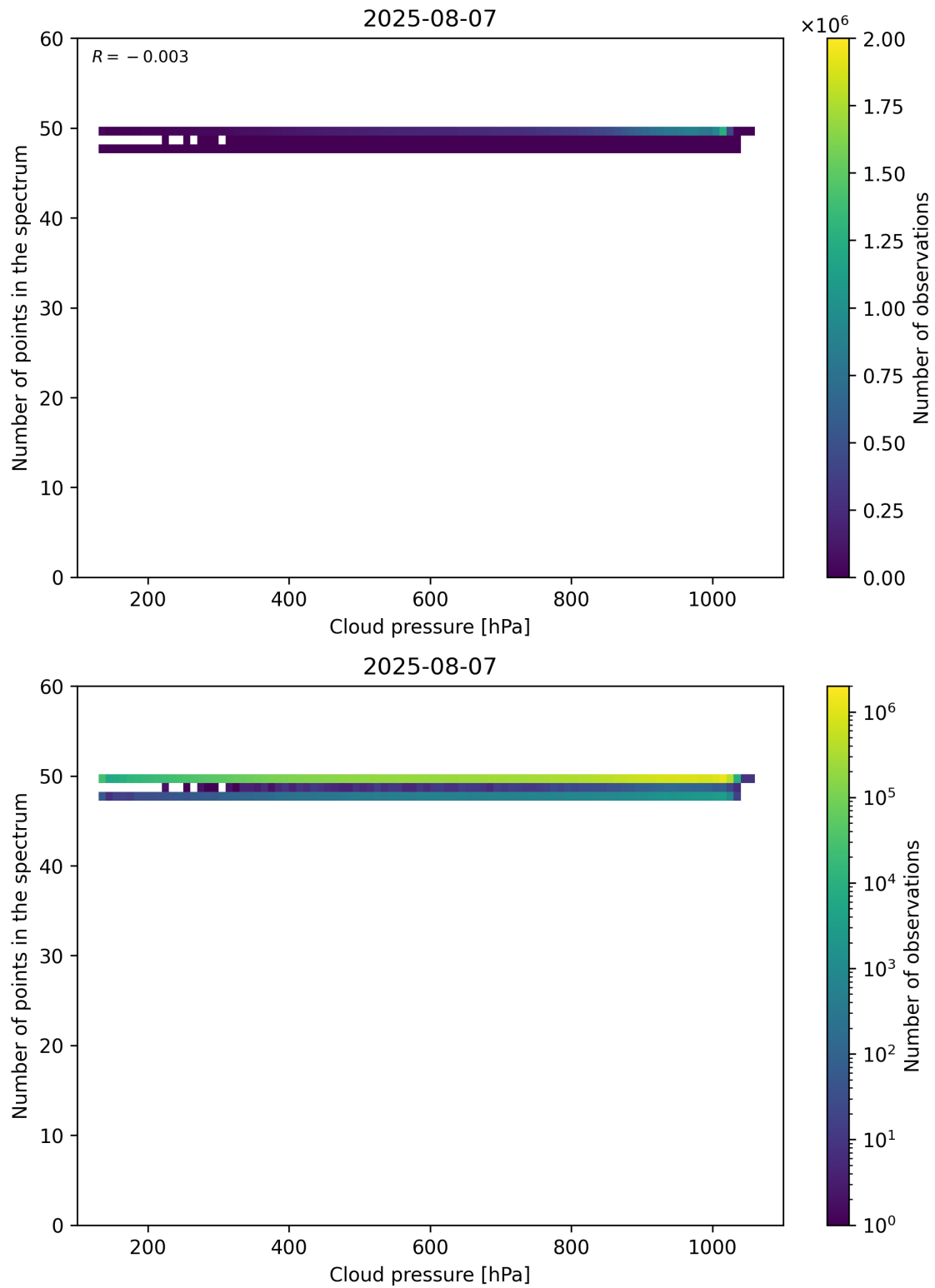
Figure 82: Scatter density plot of “Cloud pressure” against “Number of points in the spectrum” for 2025-08-06 to 2025-08-08.
