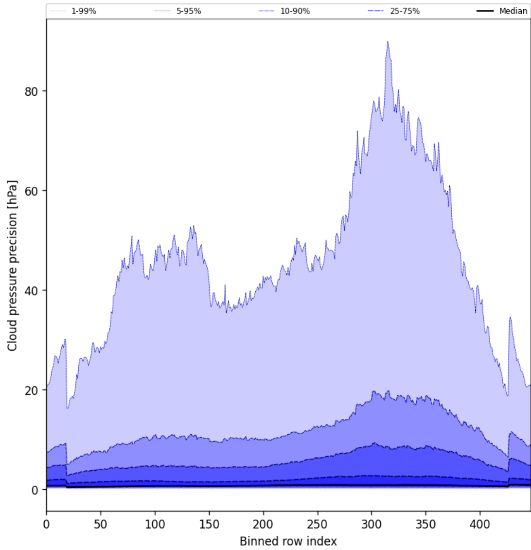
Figure 48: Along track statistics of “Cloud pressure precision” for 2025-08-06 to 2025-08-08
