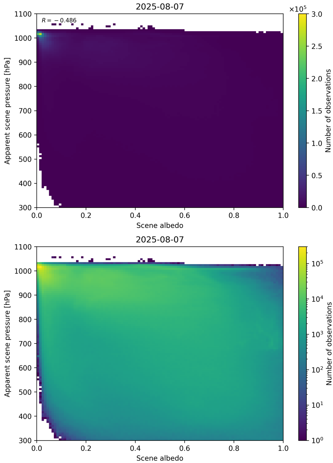
Figure 102: Scatter density plot of “Scene albedo” against “Apparent scene pressure” for 2025-08-06 to 2025-08-08.
