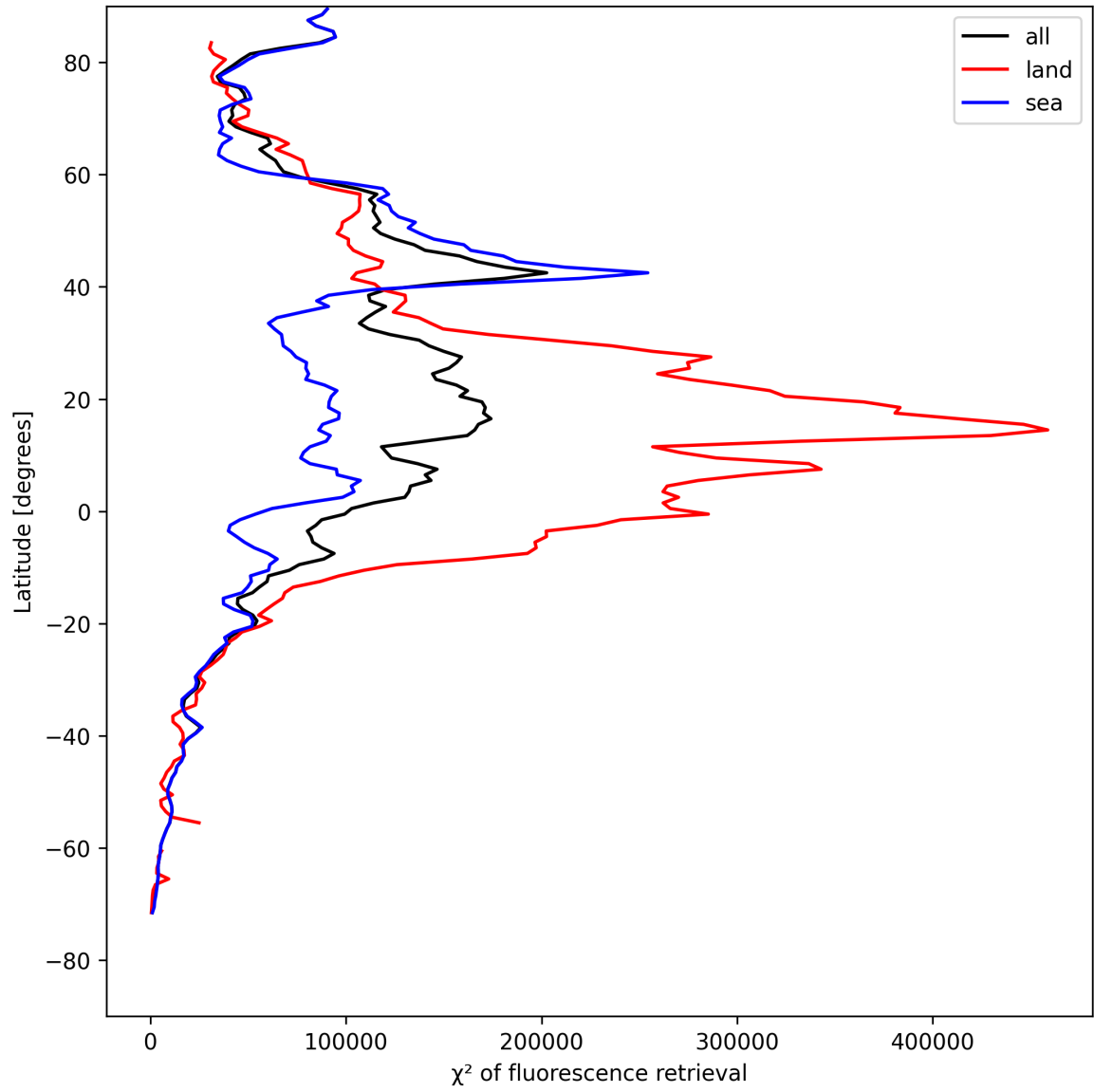
Figure 25: Zonal average of “ \chi^2 of fluorescence retrieval” for 2025-08-06 to 2025-08-08.
