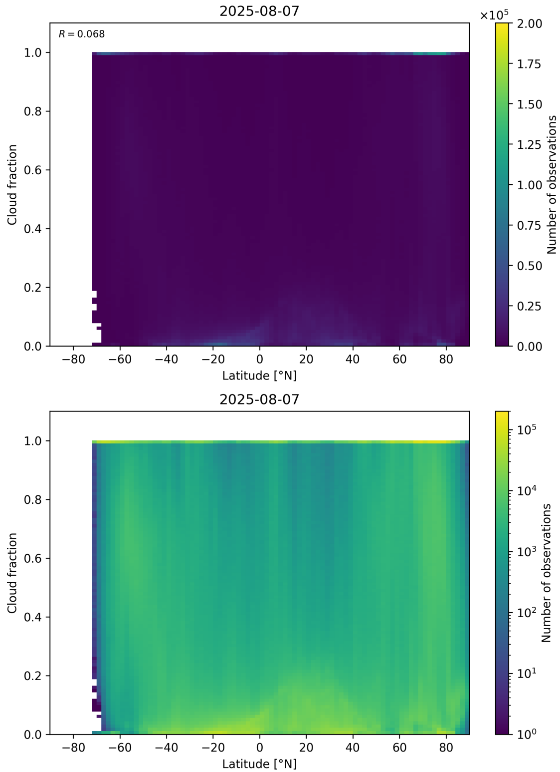
Figure 90: Scatter density plot of “Latitude” against “Cloud fraction” for 2025-08-06 to 2025-08-08.
