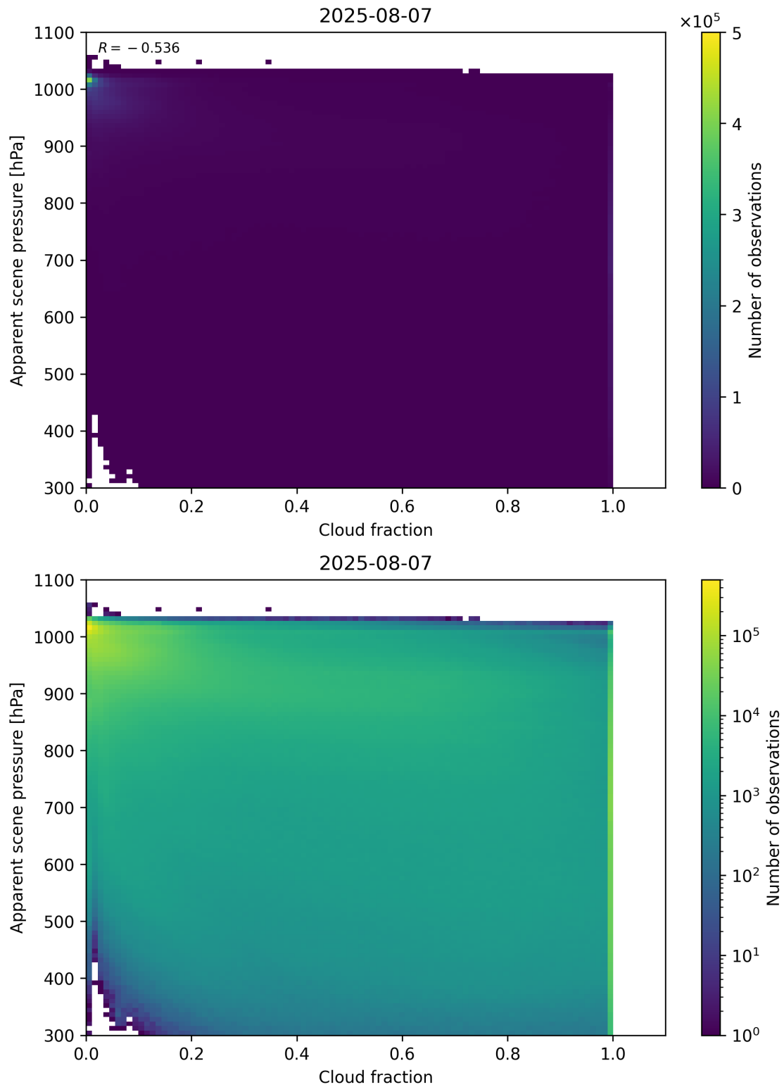
Figure 70: Scatter density plot of “Cloud fraction” against “Apparent scene pressure” for 2025-08-06 to 2025-08-08.
