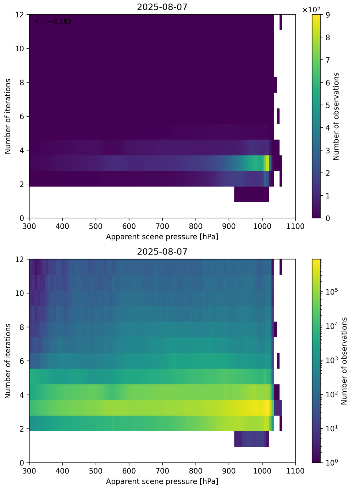
Figure 65: Scatter density plot of “Apparent scene pressure” against “Number of iterations” for 2025-08-06 to 2025-08-08.
