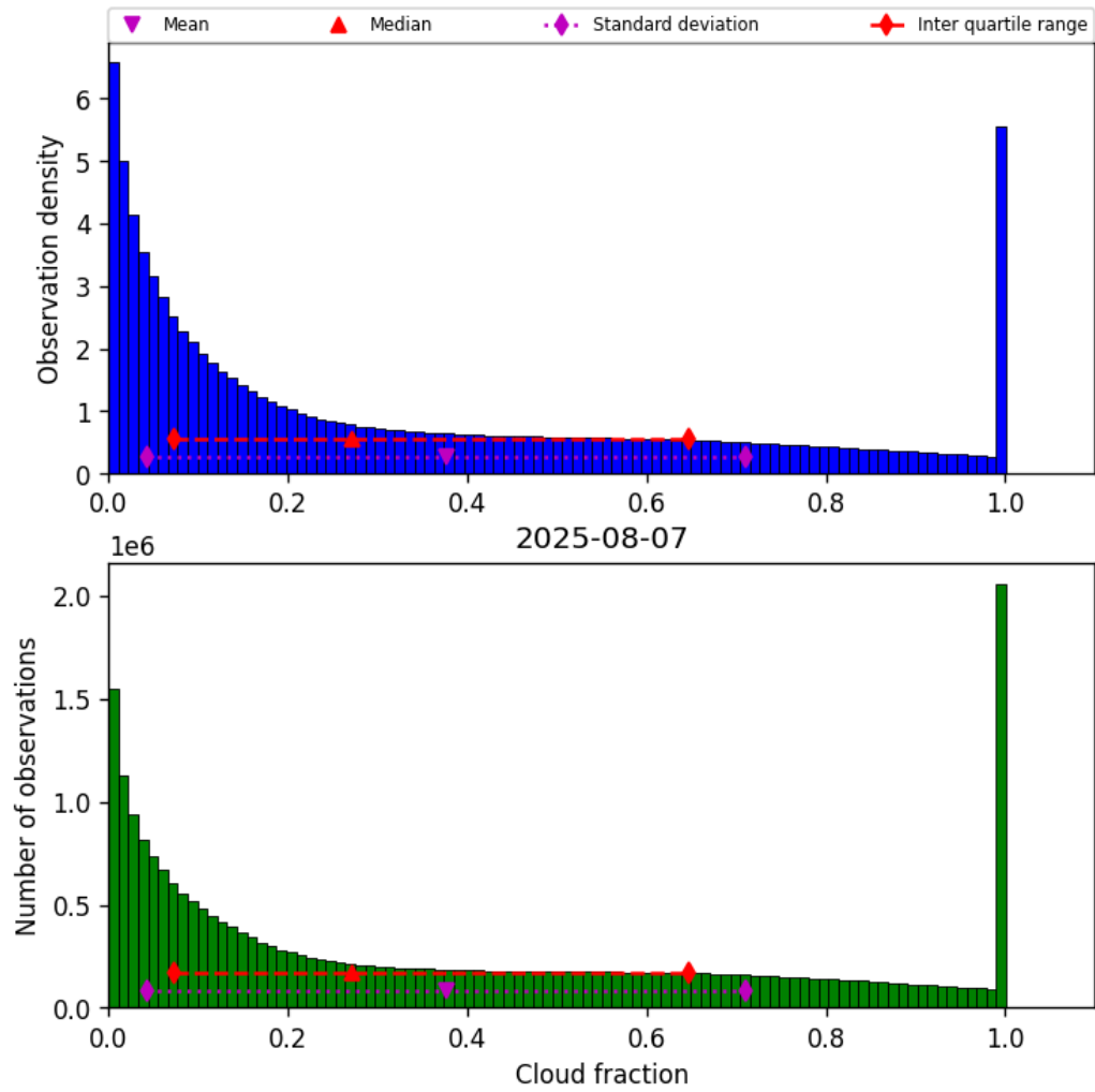
Figure 32: Histogram of “Cloud fraction” for 2025-08-06 to 2025-08-08
