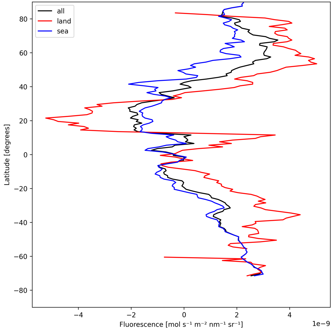
Figure 23: Zonal average of “Fluorescence” for 2025-08-06 to 2025-08-08.
