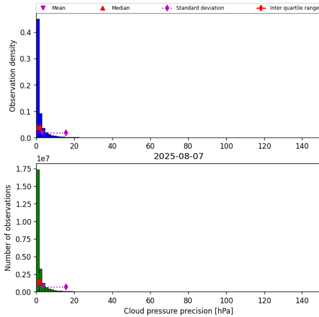
Figure 31: Histogram of “Cloud pressure precision” for 2025-08-06 to 2025-08-08
