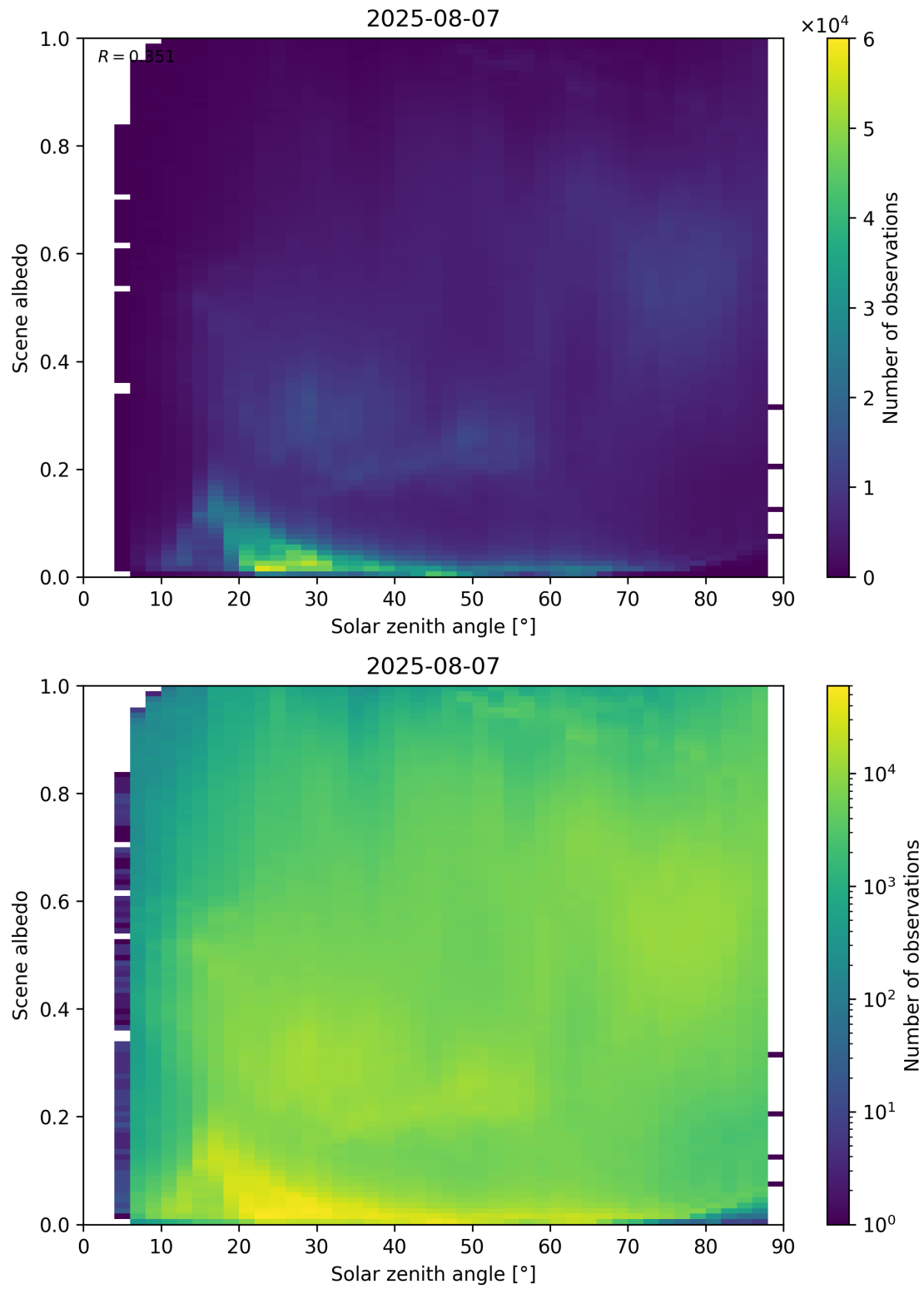
Figure 116: Scatter density plot of “Solar zenith angle” against “Scene albedo” for 2025-08-06 to 2025-08-08.
