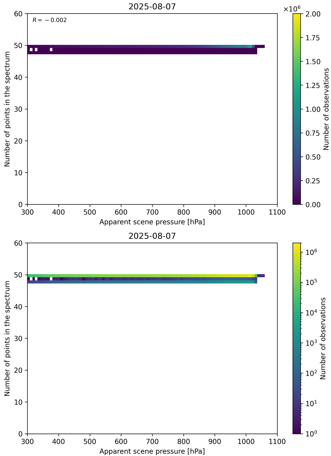
Figure 66: Scatter density plot of “Apparent scene pressure” against “Number of points in the spectrum” for 2025-08-06 to 2025-08-08.
