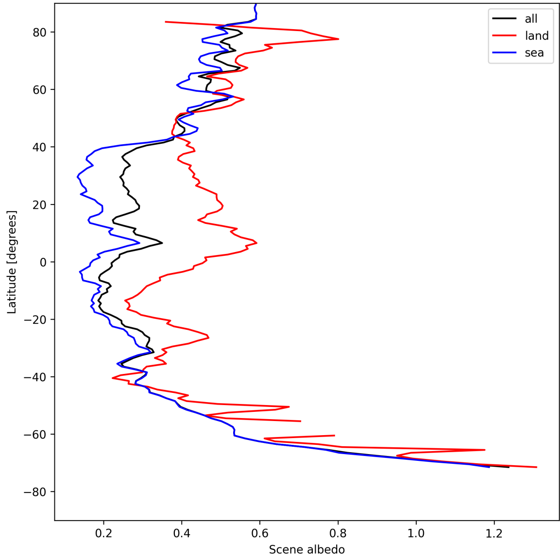
Figure 17: Zonal average of “Scene albedo” for 2025-08-06 to 2025-08-08.
