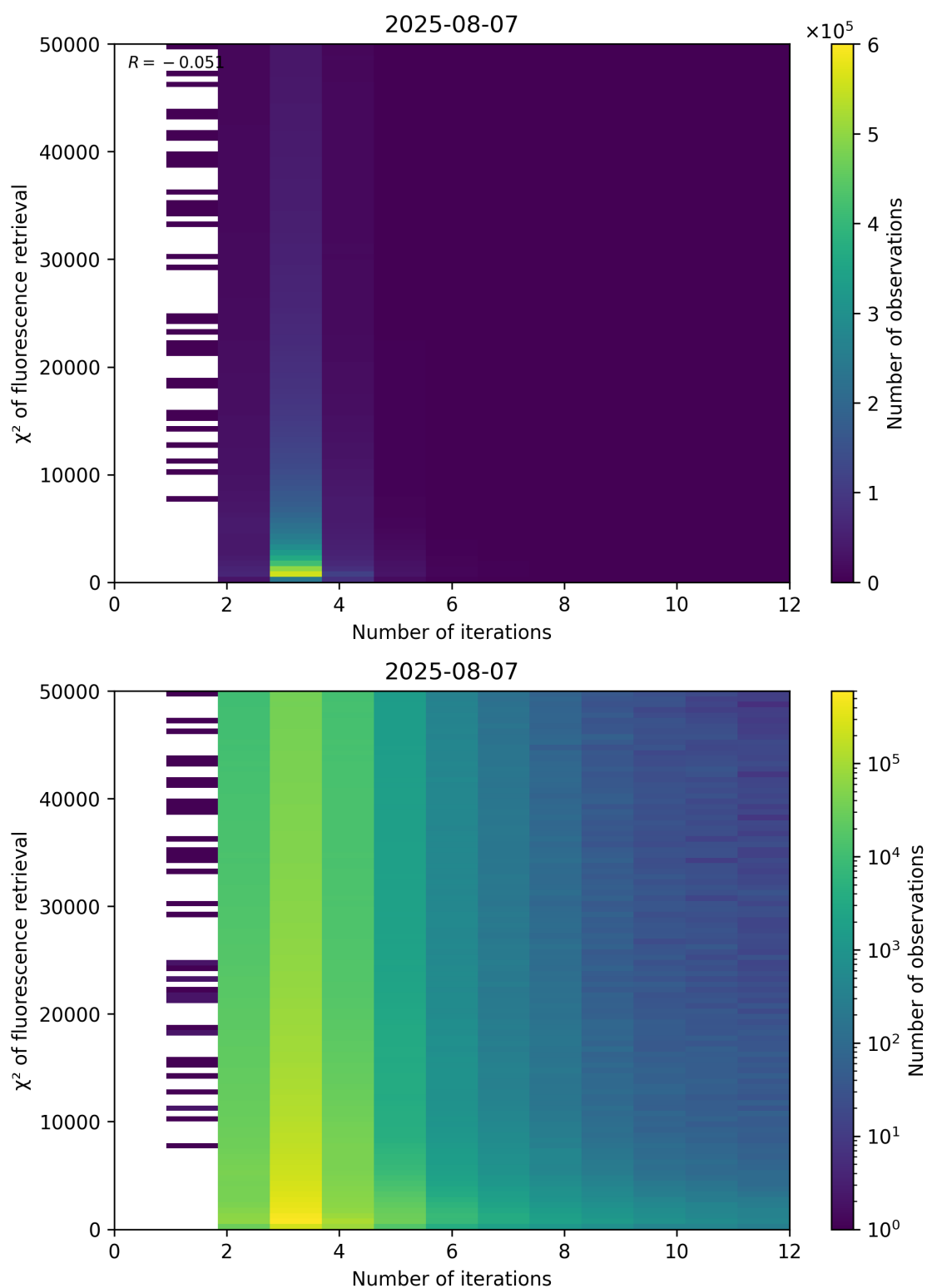
Figure 97: Scatter density plot of “Number of iterations” against “ \chi^2 of fluorescence retrieval” for 2025-08-06 to 2025-08-08.
