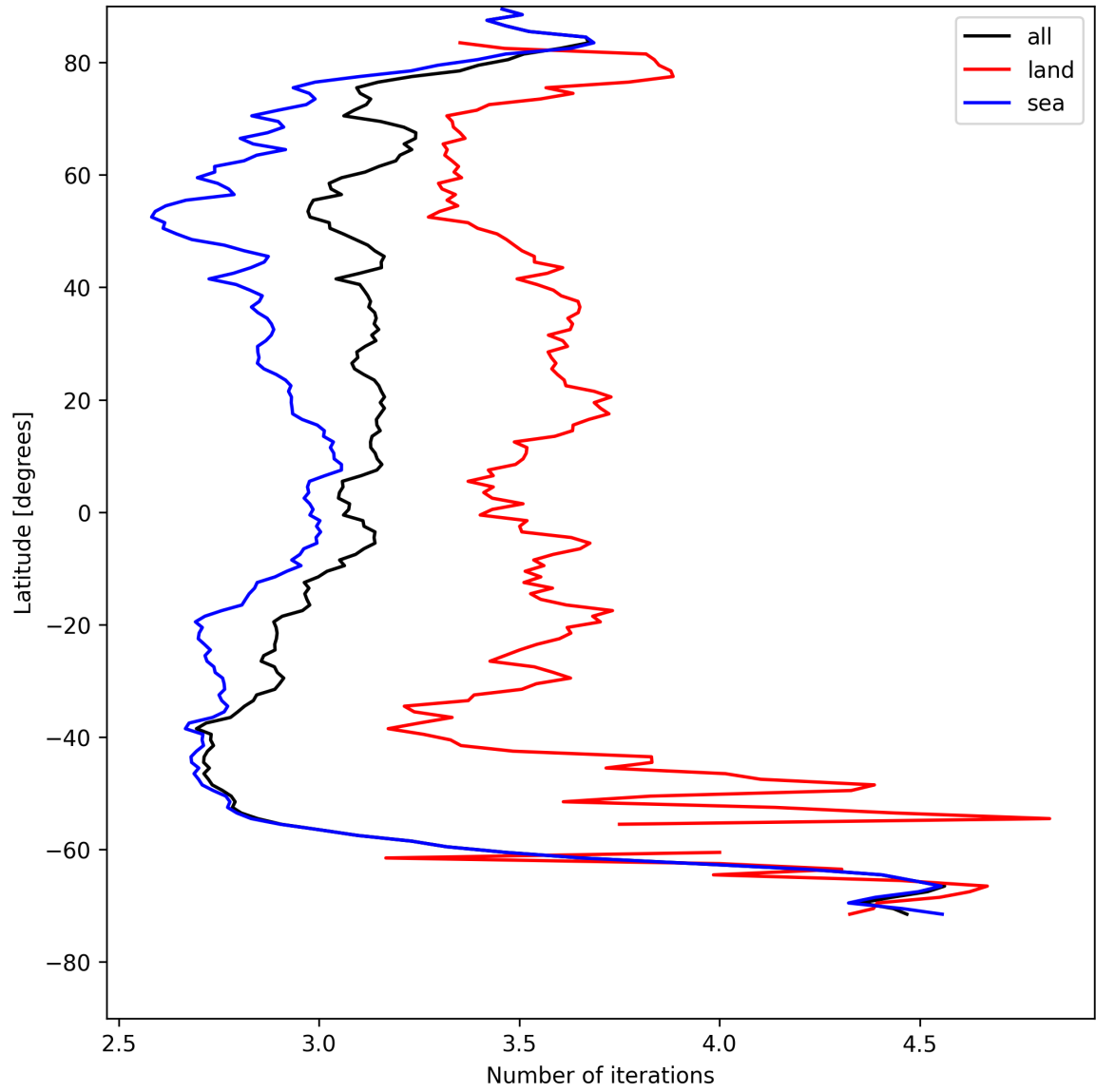
Figure 22: Zonal average of “Number of iterations” for 2025-08-06 to 2025-08-08.
