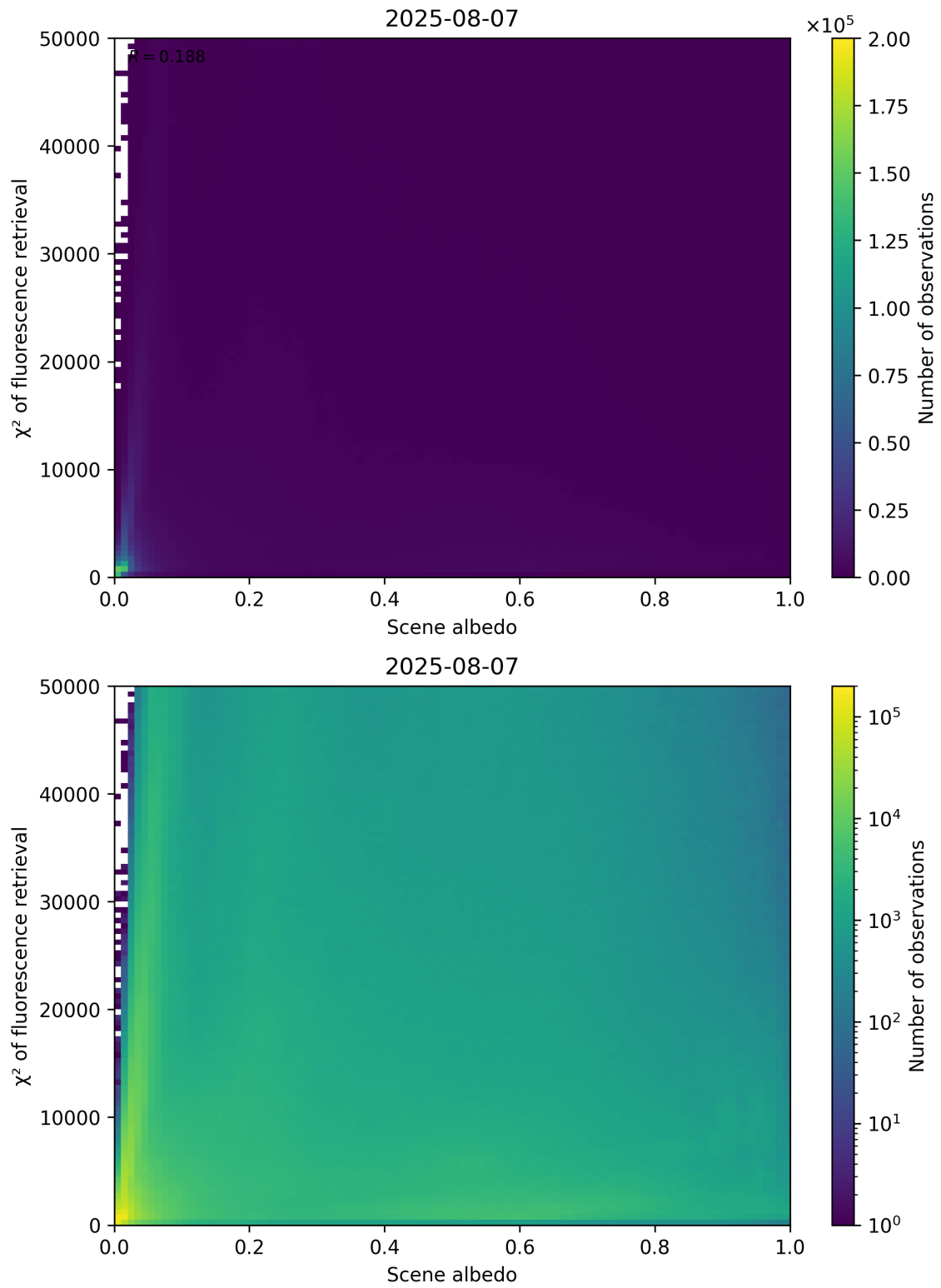
Figure 103: Scatter density plot of “Scene albedo” against “ \chi^2 of fluorescence retrieval” for 2025-08-06 to 2025-08-08.
