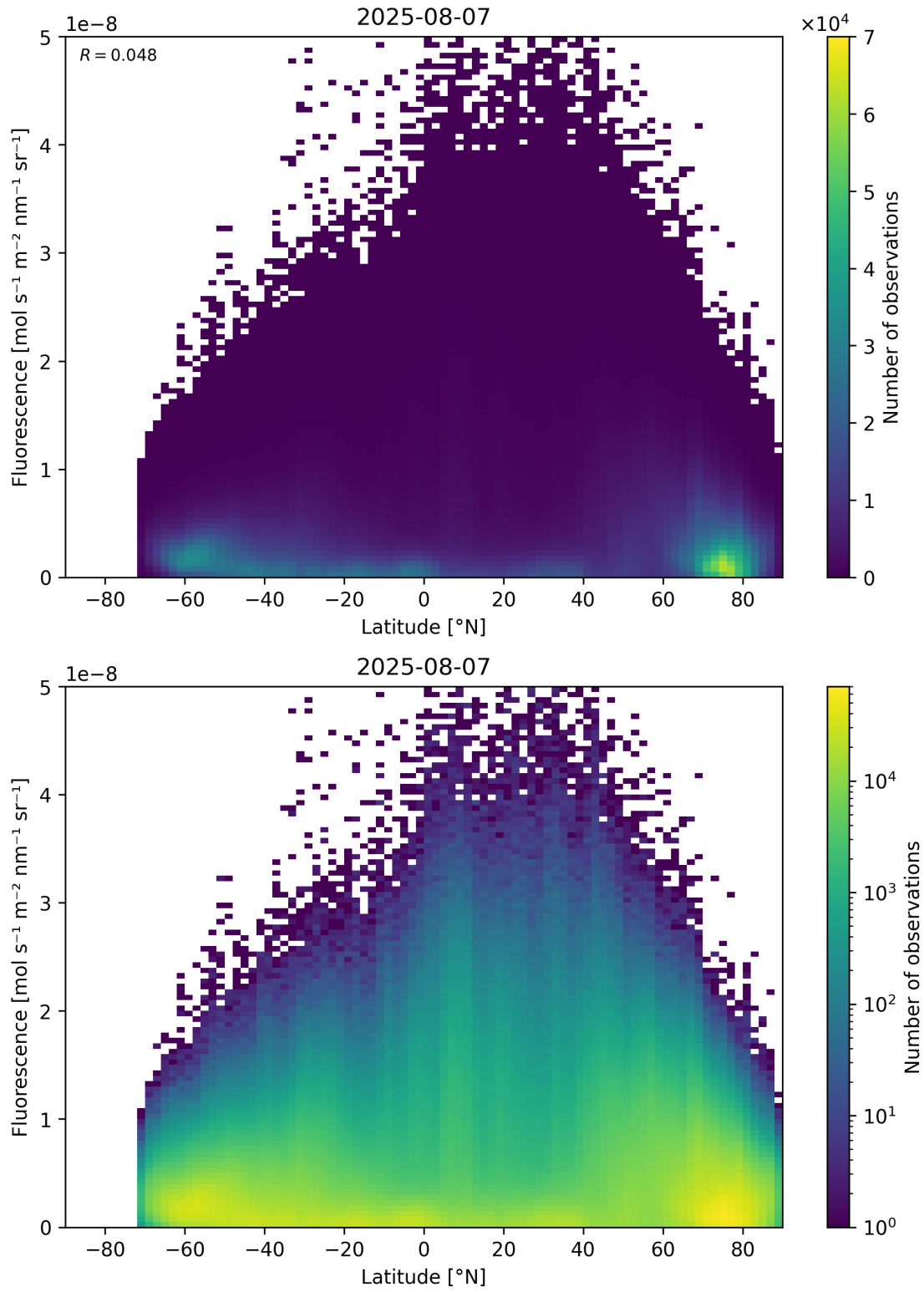
Figure 92: Scatter density plot of “Latitude” against “Fluorescence” for 2025-08-06 to 2025-08-08.
