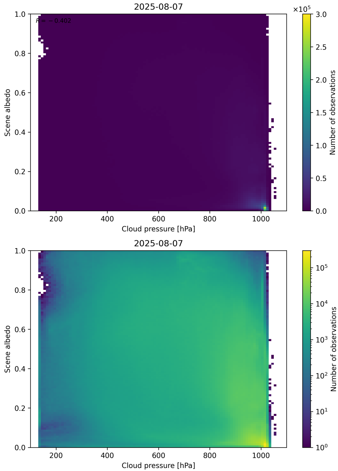
Figure 83: Scatter density plot of “Cloud pressure” against “Scene albedo” for 2025-08-06 to 2025-08-08.
