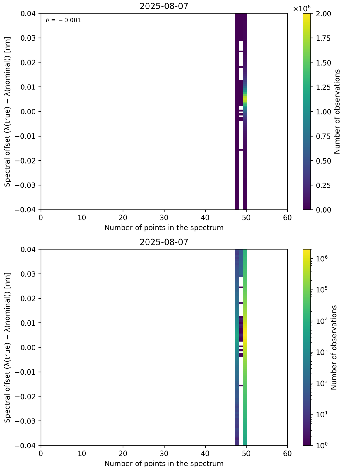
Figure 101: Scatter density plot of “Number of points in the spectrum” against “Spectral offset ( \lambda_{\text{true}} - \lambda_{\text{nominal}} )” for 2025-08-06 to 2025-08-08.
