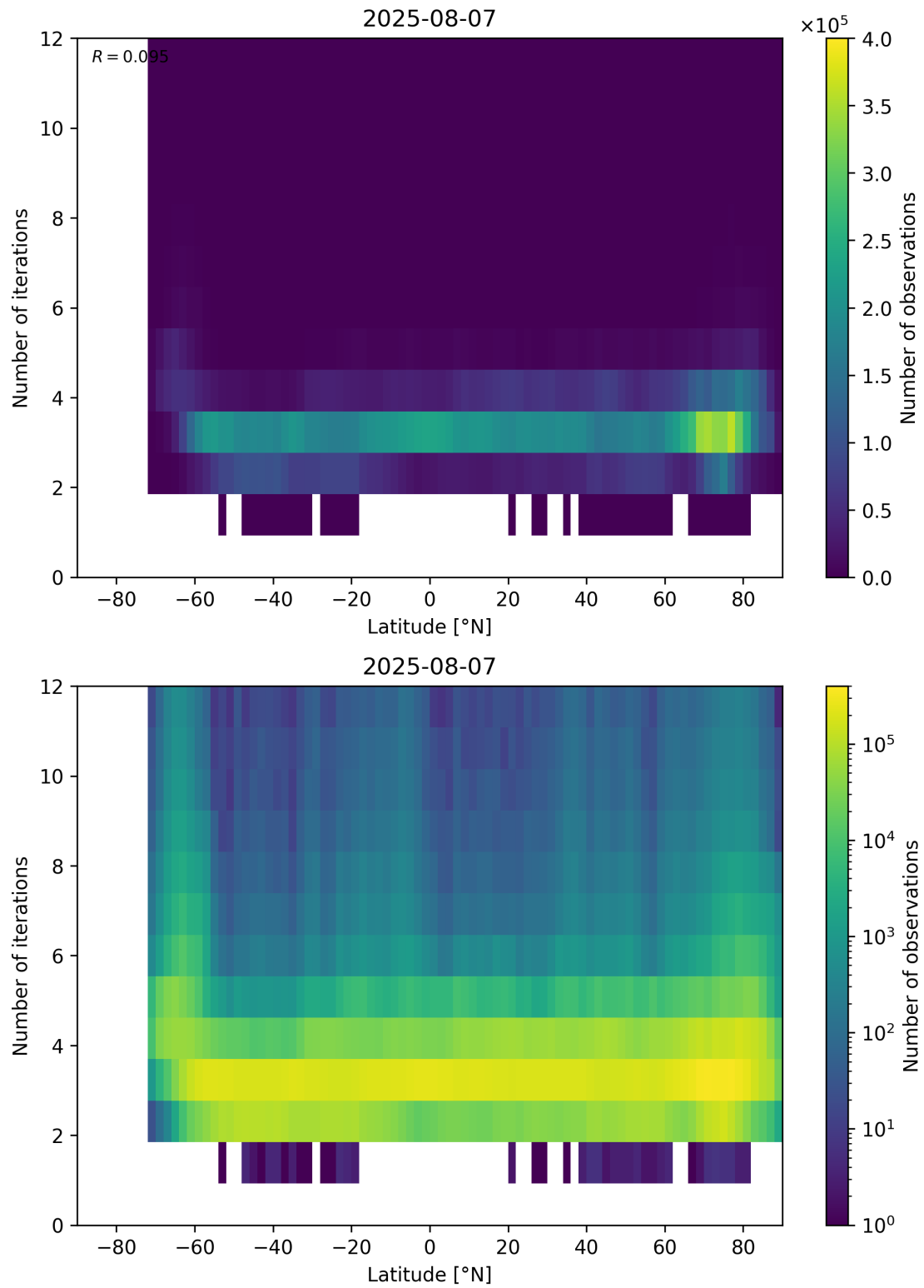
Figure 93: Scatter density plot of “Latitude” against “Number of iterations” for 2025-08-06 to 2025-08-08.
