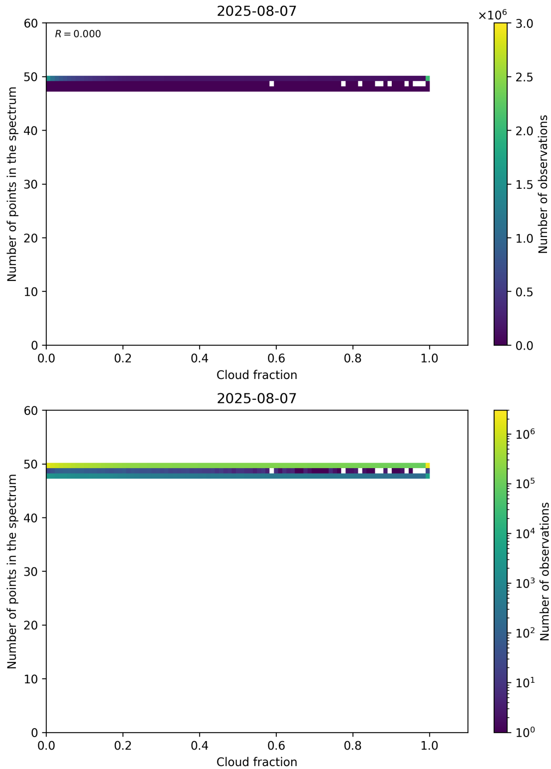
Figure 74: Scatter density plot of “Cloud fraction” against “Number of points in the spectrum” for 2025-08-06 to 2025-08-08.
