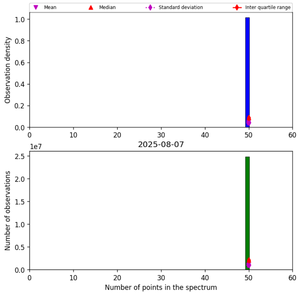
Figure 44: Histogram of “Number of points in the spectrum” for 2025-08-06 to 2025-08-08
