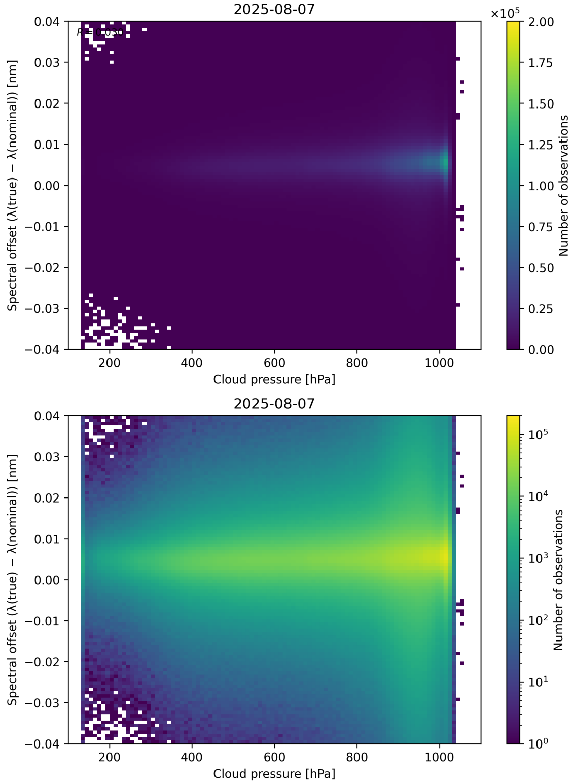
Figure 84: Scatter density plot of “Cloud pressure” against “Spectral offset ( \lambda_{\text{true}} - \lambda_{\text{nominal}} )” for 2025-08-06 to 2025-08-08.
