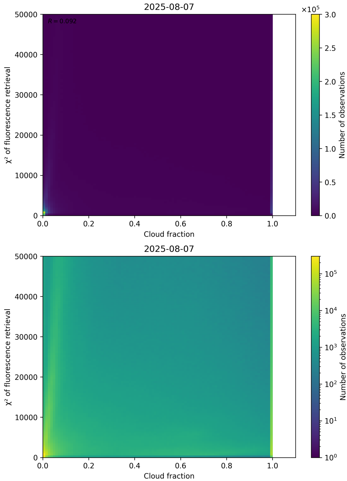
Figure 71: Scatter density plot of “Cloud fraction” against “ \chi^2 of fluorescence retrieval” for 2025-08-06 to 2025-08-08.
