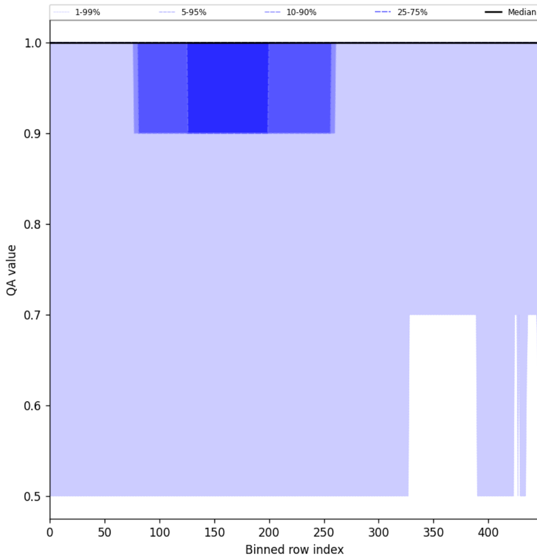
Figure 46: Along track statistics of “QA value” for 2025-08-06 to 2025-08-08
