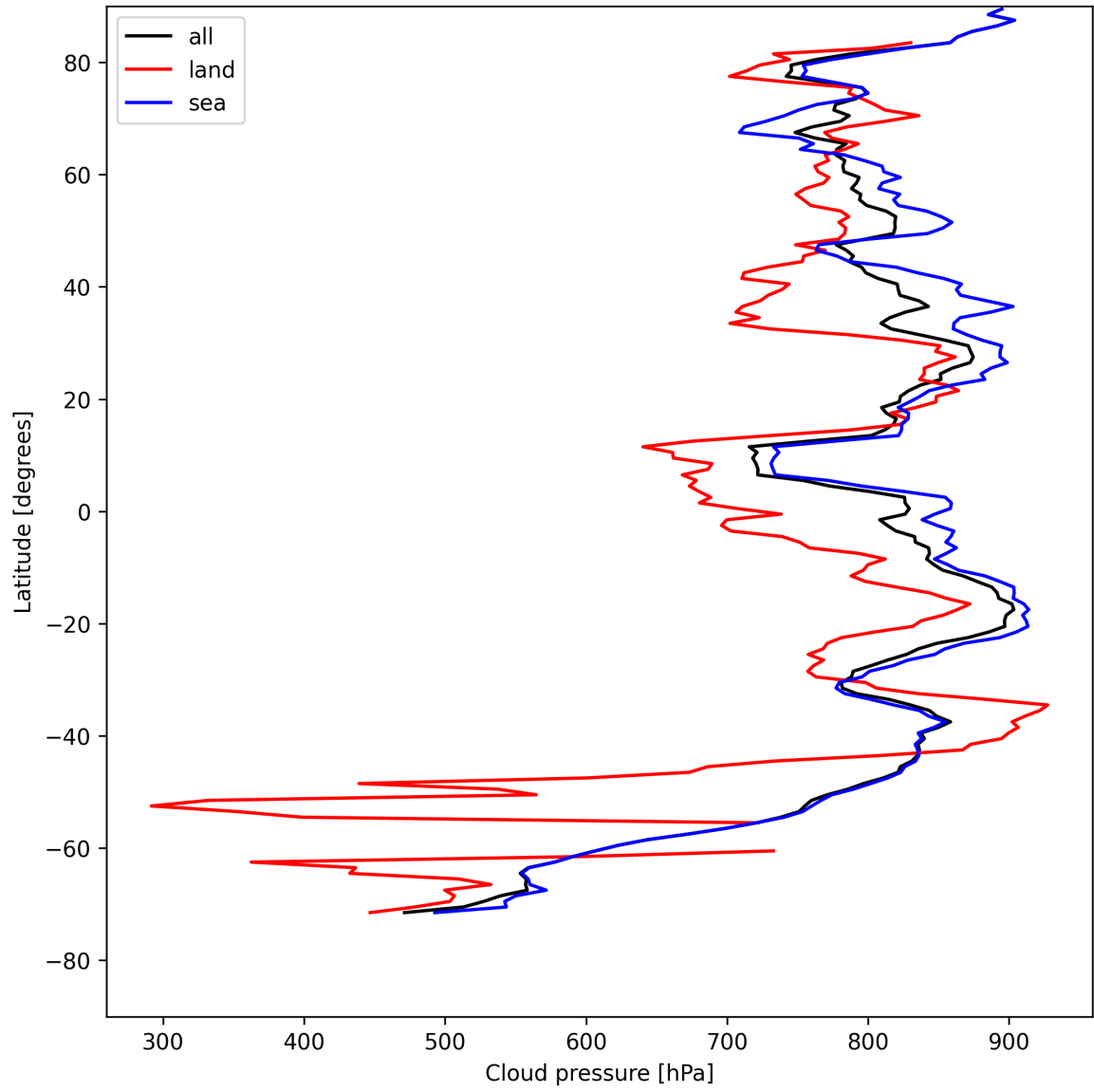
Figure 13: Zonal average of “Cloud pressure” for 2025-08-06 to 2025-08-08.
