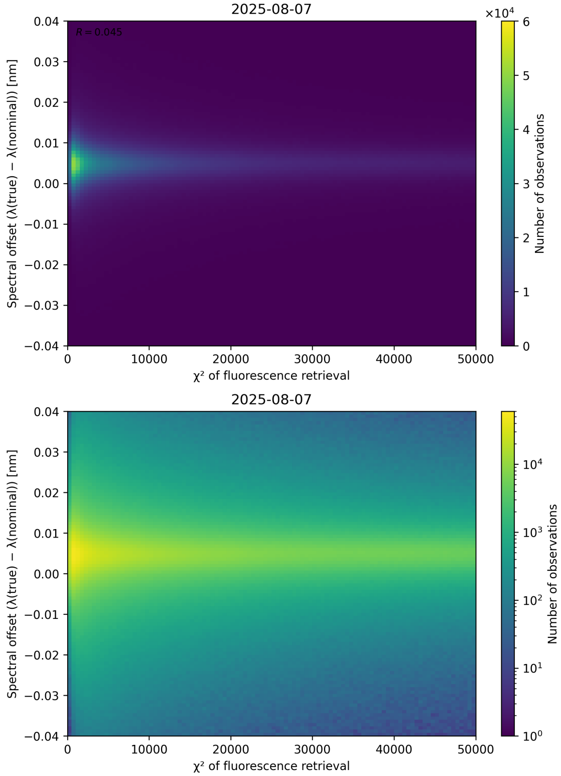
Figure 69: Scatter density plot of “ \chi^2 of fluorescence retrieval” against “Spectral offset ( \lambda_{\text{true}} - \lambda_{\text{nominal}} )” for 2025-08-06 to 2025-08-08.
