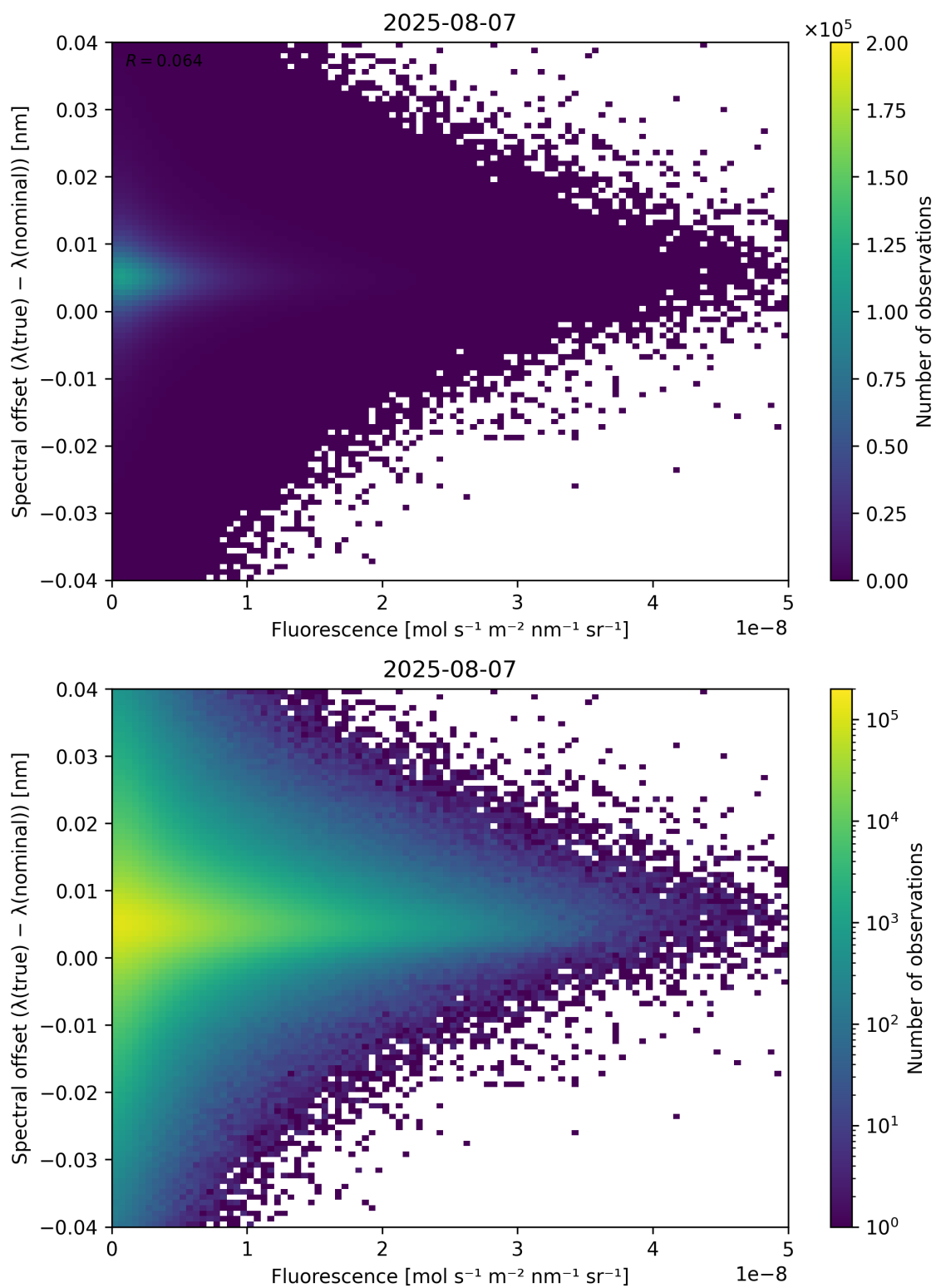
Figure 87: Scatter density plot of “Fluorescence” against “Spectral offset ( \lambda_{\text{true}} - \lambda_{\text{nominal}} )” for 2025-08-06 to 2025-08-08.
