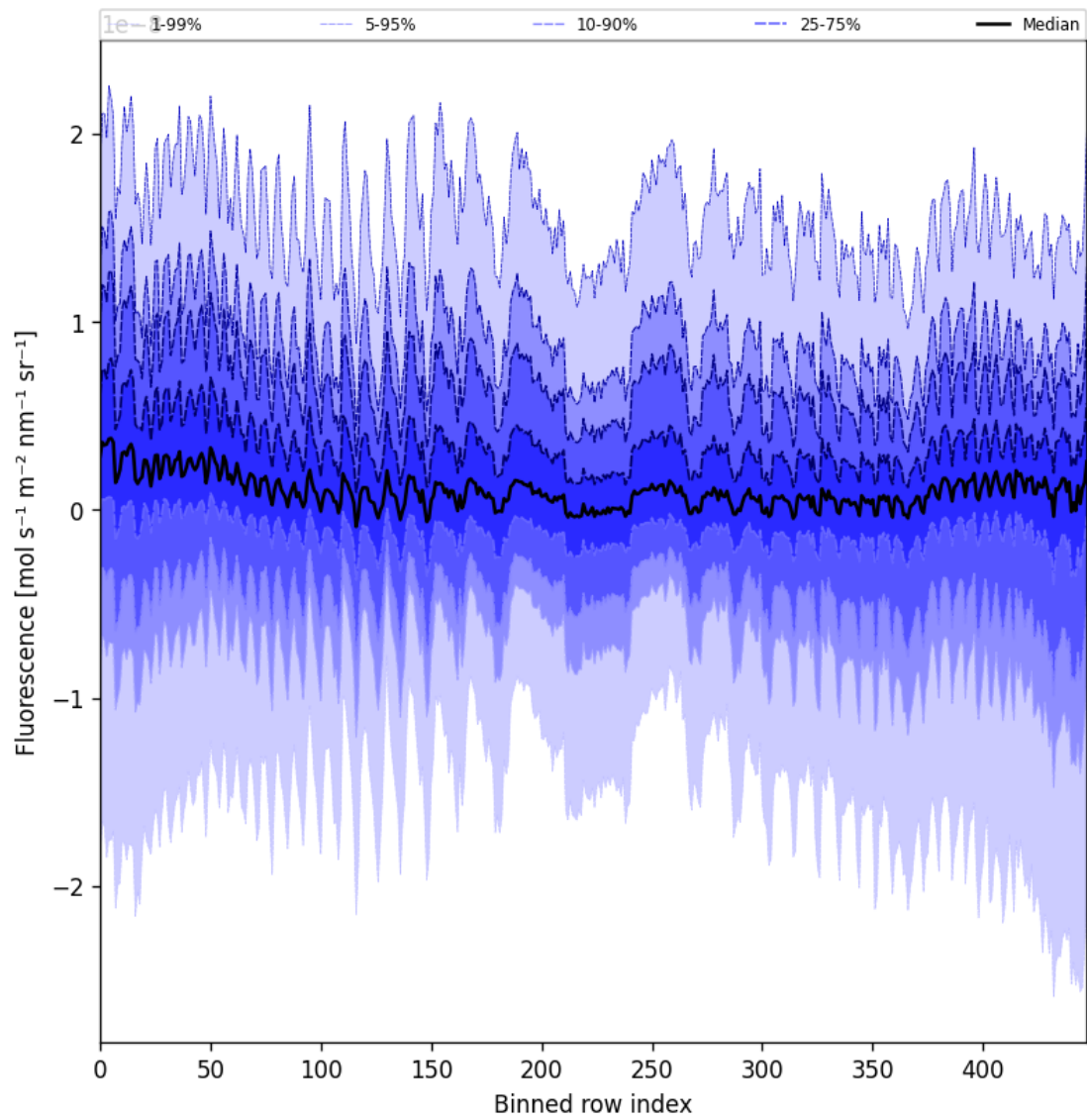
Figure 57: Along track statistics of “Fluorescence” for 2025-08-06 to 2025-08-08
