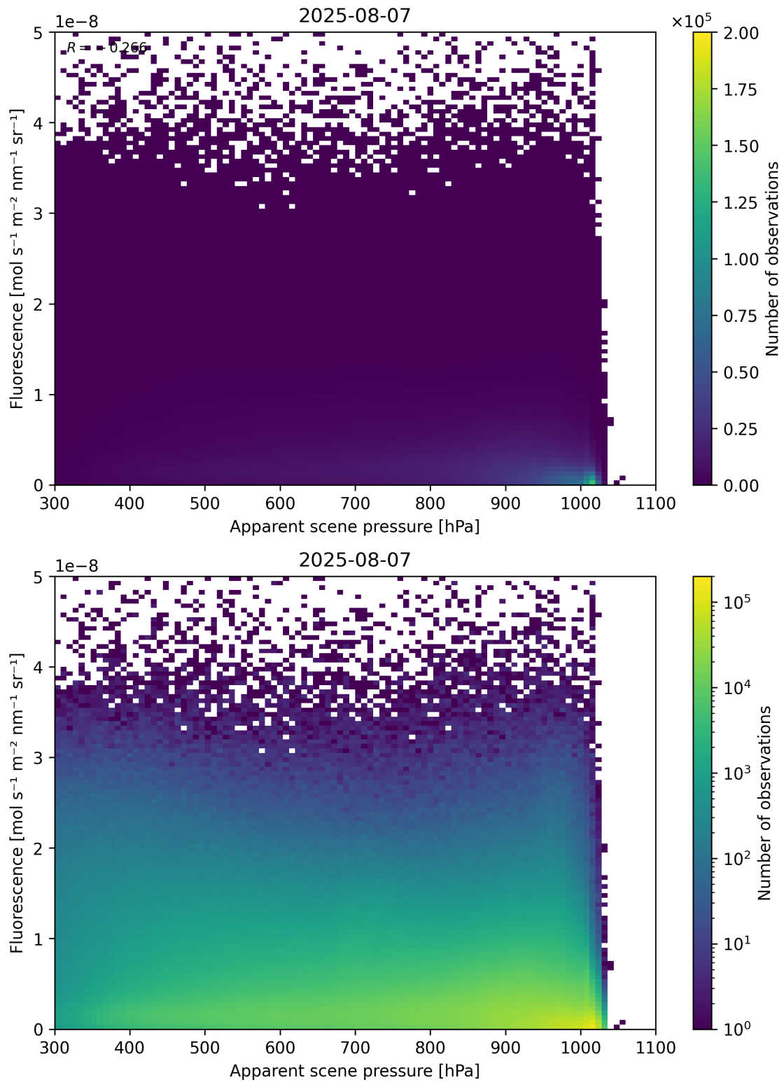
Figure 64: Scatter density plot of “Apparent scene pressure” against “Fluorescence” for 2025-08-06 to 2025-08-08.
