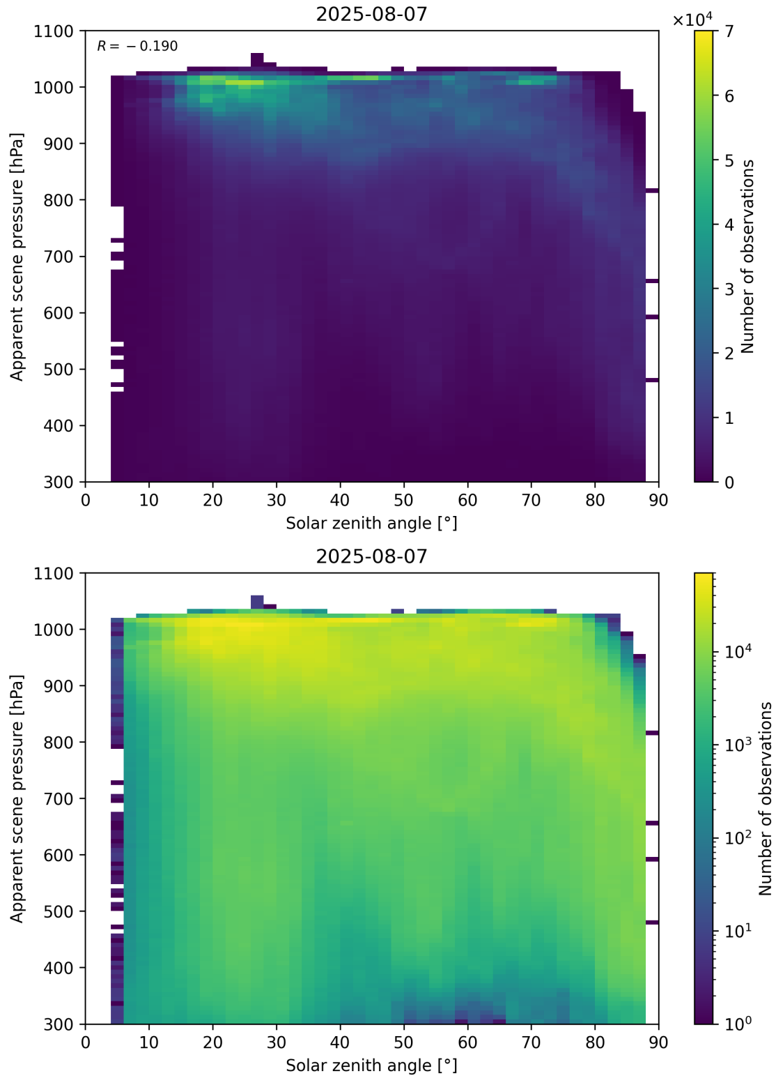
Figure 108: Scatter density plot of “Solar zenith angle” against “Apparent scene pressure” for 2025-08-06 to 2025-08-08.
