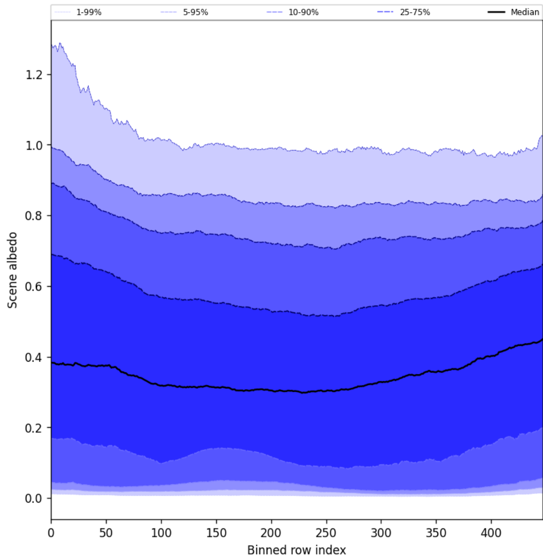
Figure 51: Along track statistics of “Scene albedo” for 2025-08-06 to 2025-08-08
