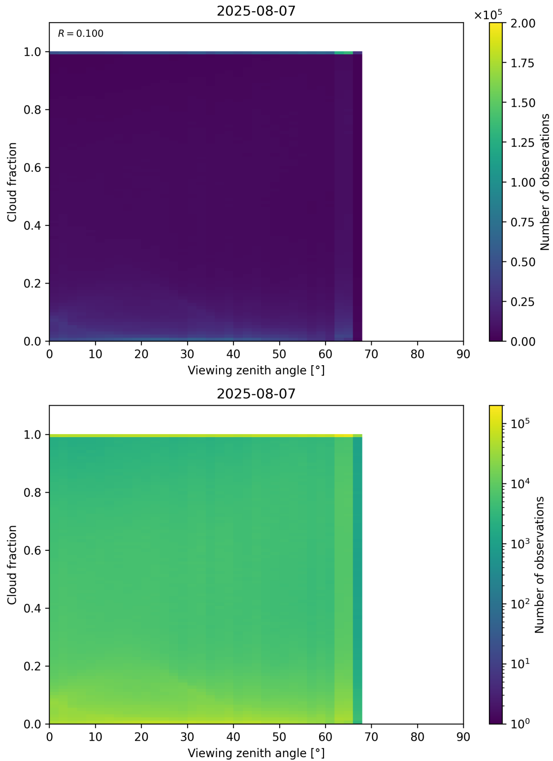
Figure 120: Scatter density plot of “Viewing zenith angle” against “Cloud fraction” for 2025-08-06 to 2025-08-08.
