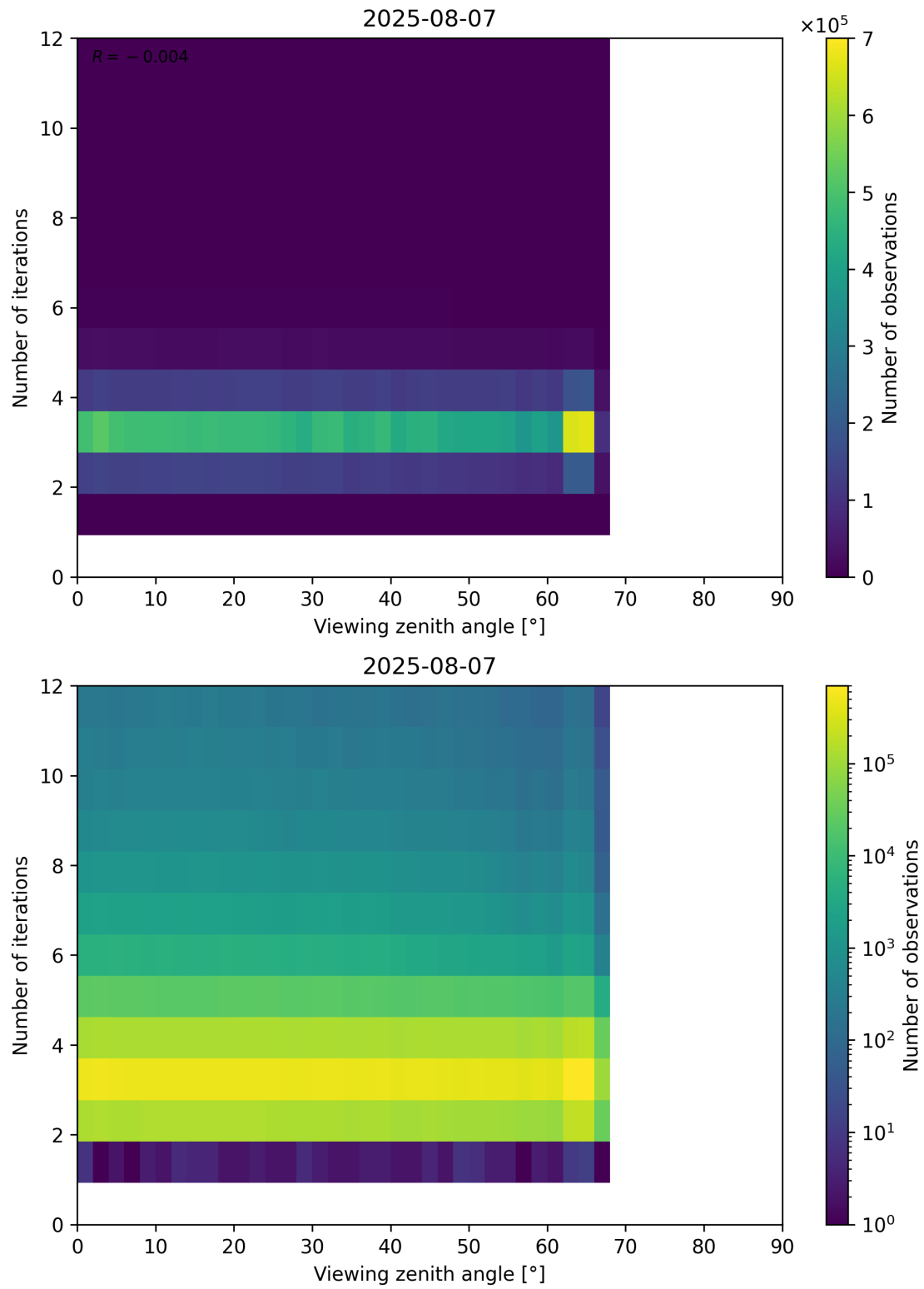
Figure 124: Scatter density plot of “Viewing zenith angle” against “Number of iterations” for 2025-08-06 to 2025-08-08.
