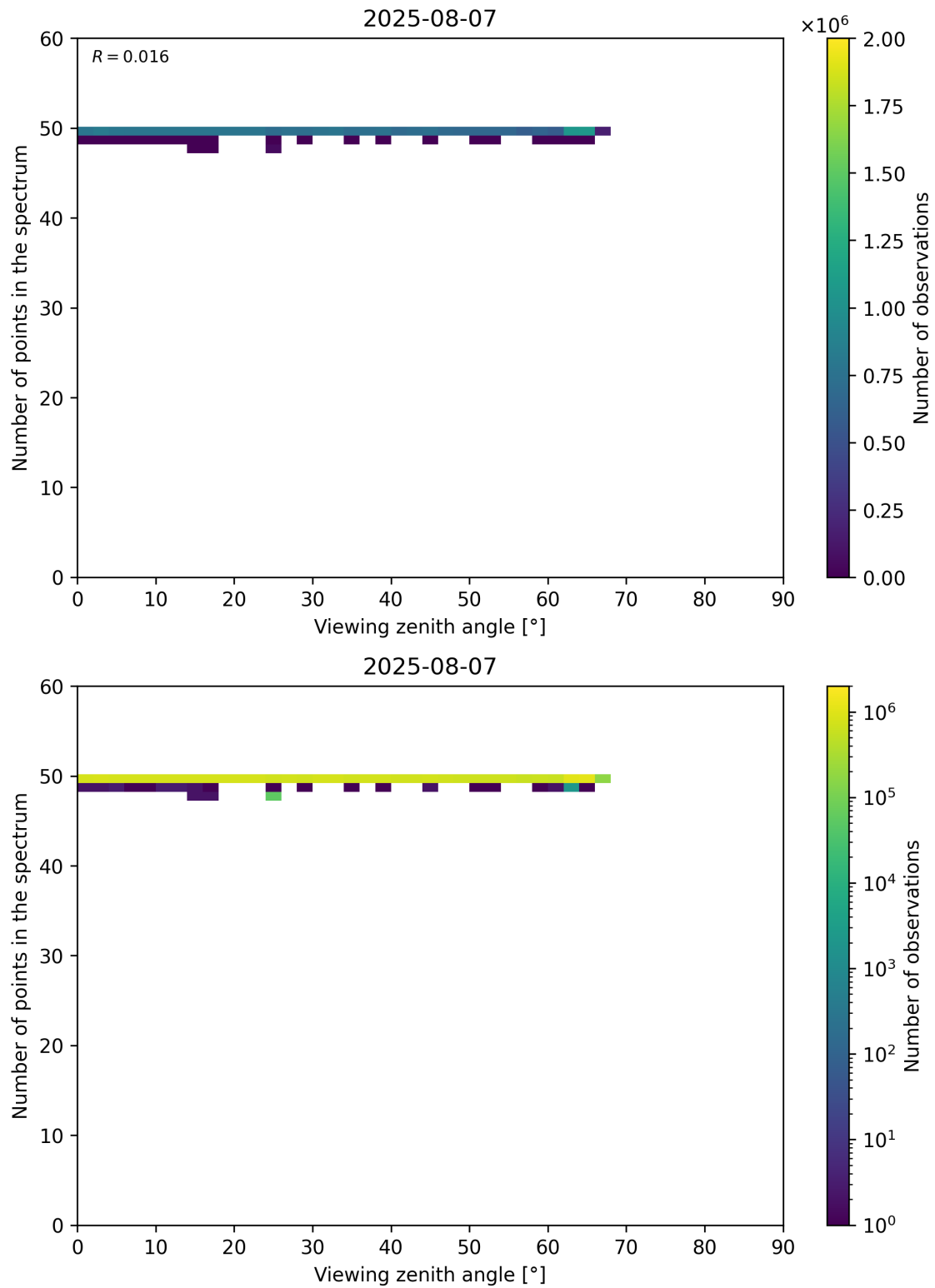
Figure 125: Scatter density plot of “Viewing zenith angle” against “Number of points in the spectrum” for 2025-08-06 to 2025-08-08.
