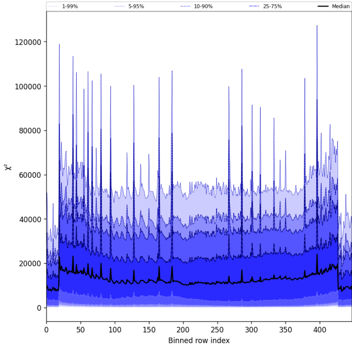
Figure 55: Along track statistics of “ \chi^2 ” for 2025-08-06 to 2025-08-08
