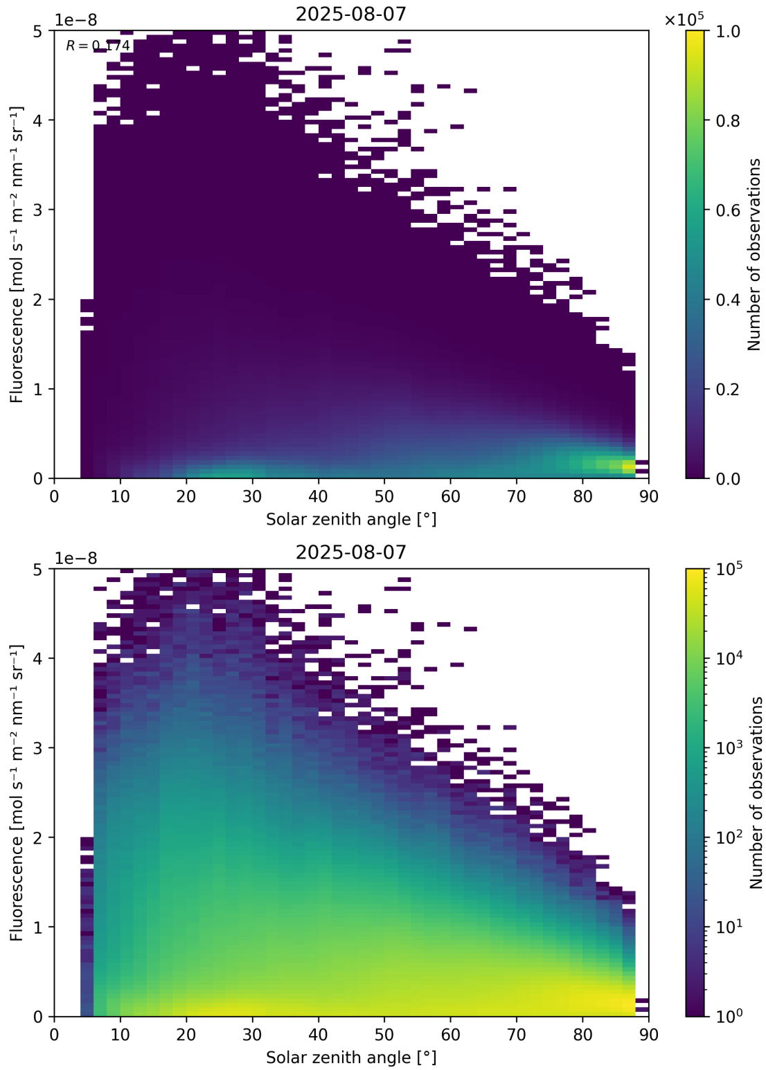
Figure 112: Scatter density plot of “Solar zenith angle” against “Fluorescence” for 2025-08-06 to 2025-08-08.
