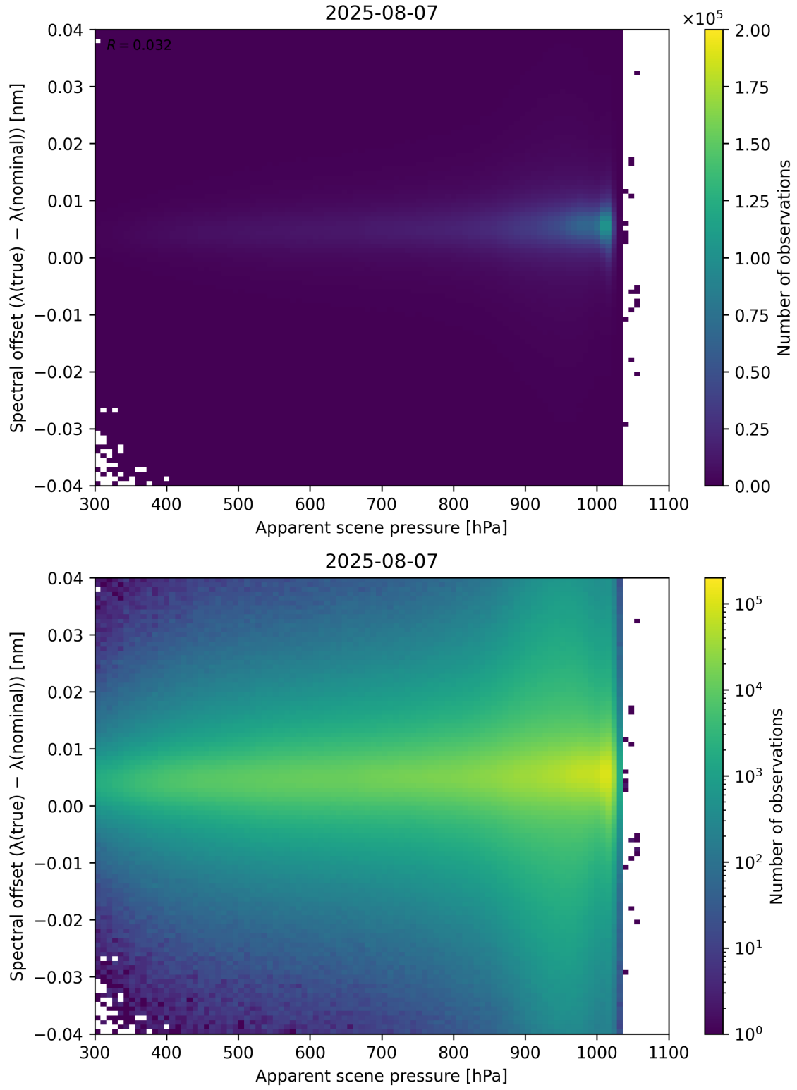
Figure 67: Scatter density plot of “Apparent scene pressure” against “Spectral offset ( \lambda_{\text{true}} - \lambda_{\text{nominal}} )” for 2025-08-06 to 2025-08-08.
