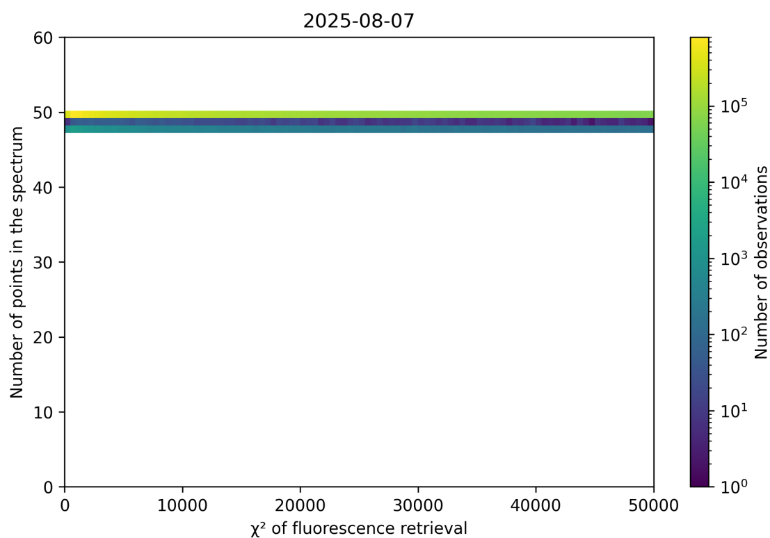
Figure 68: Scatter density plot of “ \chi^2 of fluorescence retrieval” against “Number of points in the spectrum” for 2025-08-06 to 2025-08-08.
