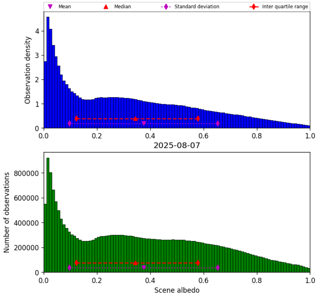
Figure 34: Histogram of “Scene albedo” for 2025-08-06 to 2025-08-08
