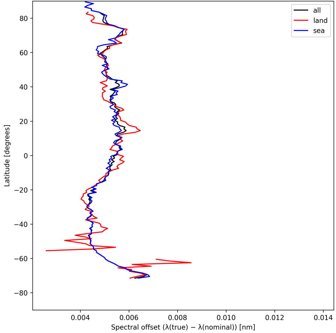
Figure 28: Zonal average of “Spectral offset ( \lambda_{\text{true}} - \lambda_{\text{nominal}} )” for 2025-08-06 to 2025-08-08.
