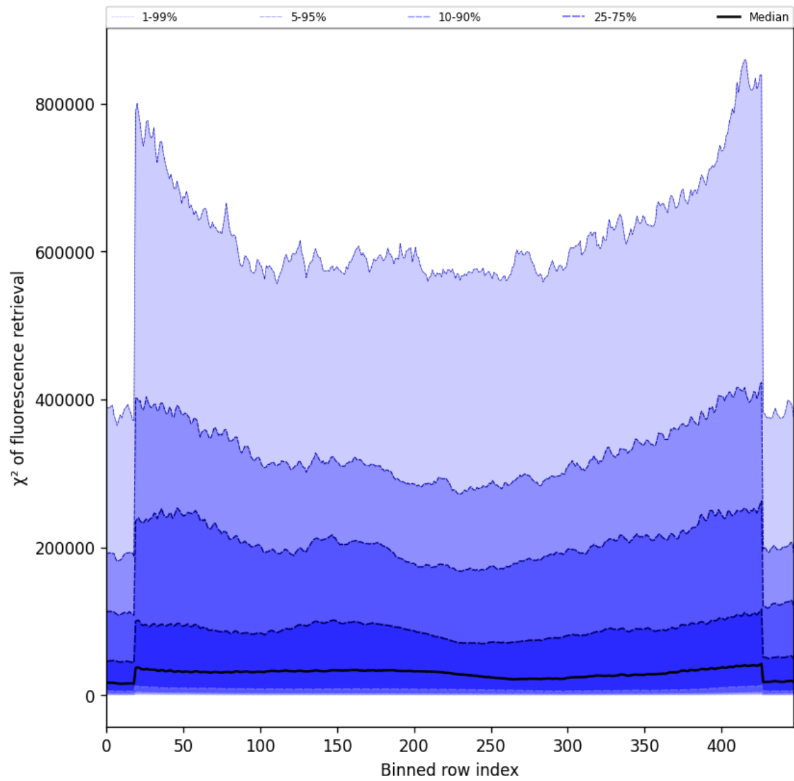
Figure 59: Along track statistics of “ \chi^2 of fluorescence retrieval” for 2025-08-06 to 2025-08-08
