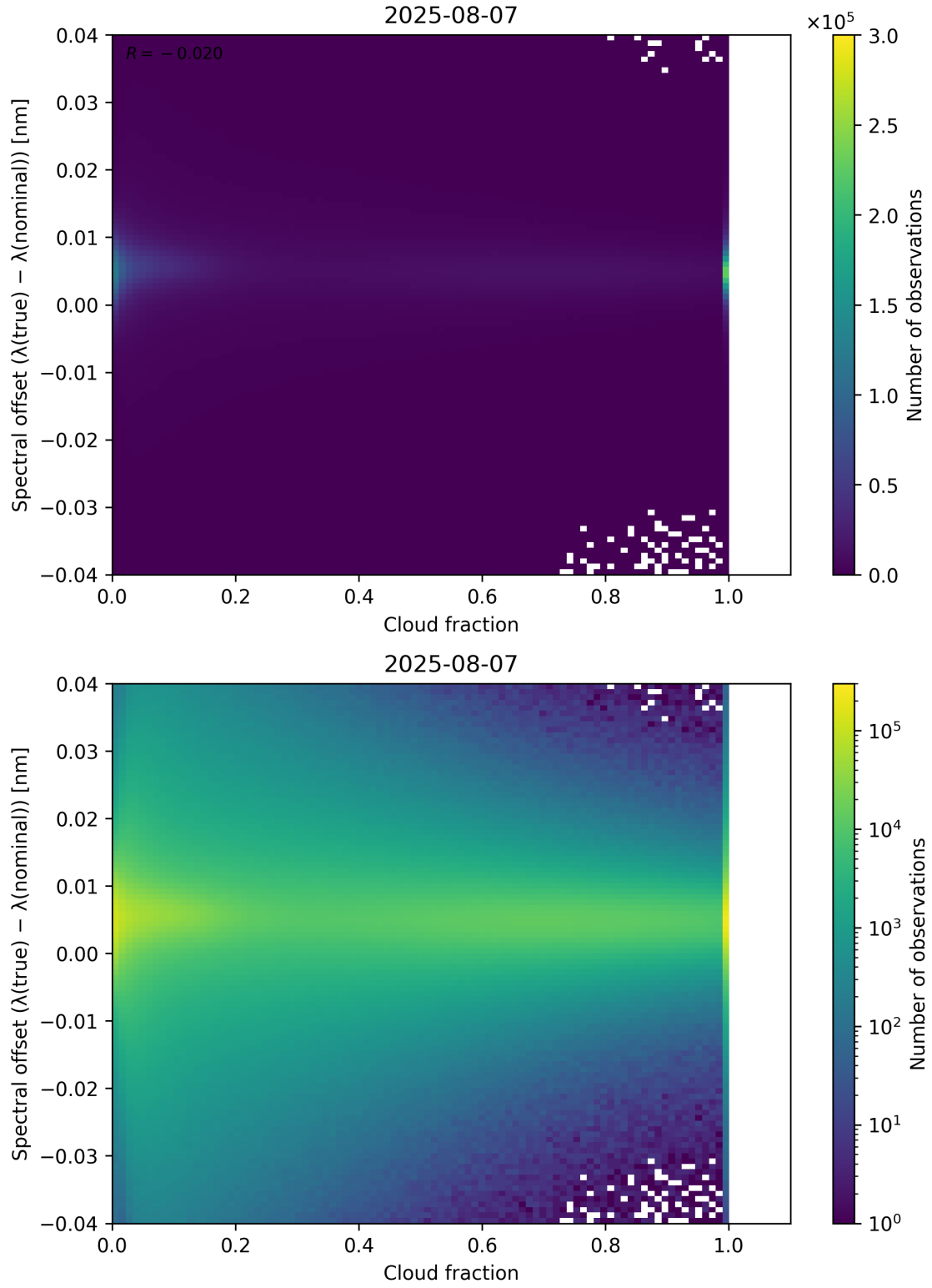
Figure 76: Scatter density plot of “Cloud fraction” against “Spectral offset ( \lambda_{\text{true}} - \lambda_{\text{nominal}} )” for 2025-08-06 to 2025-08-08.
