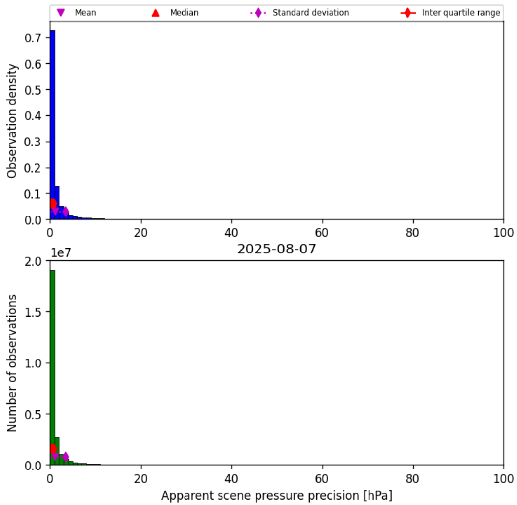
Figure 37: Histogram of “Apparent scene pressure precision” for 2025-08-06 to 2025-08-08
