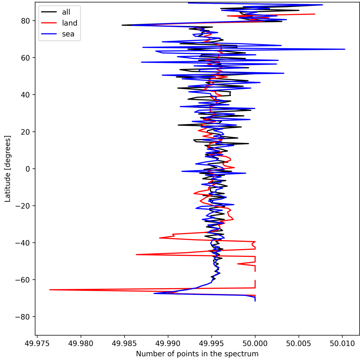
Figure 27: Zonal average of “Number of points in the spectrum” for 2025-08-06 to 2025-08-08.
