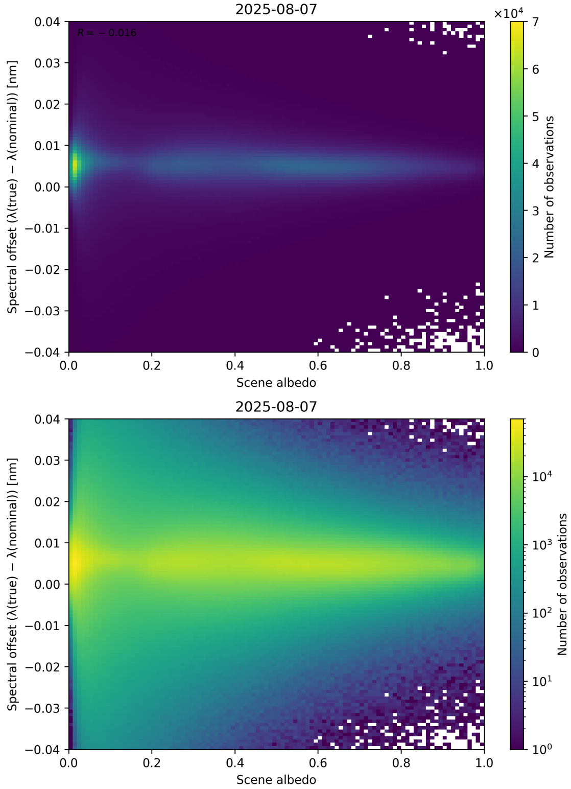
Figure 107: Scatter density plot of “Scene albedo” against “Spectral offset ( \lambda_{\text{true}} - \lambda_{\text{nominal}} )” for 2025-08-06 to 2025-08-08.
