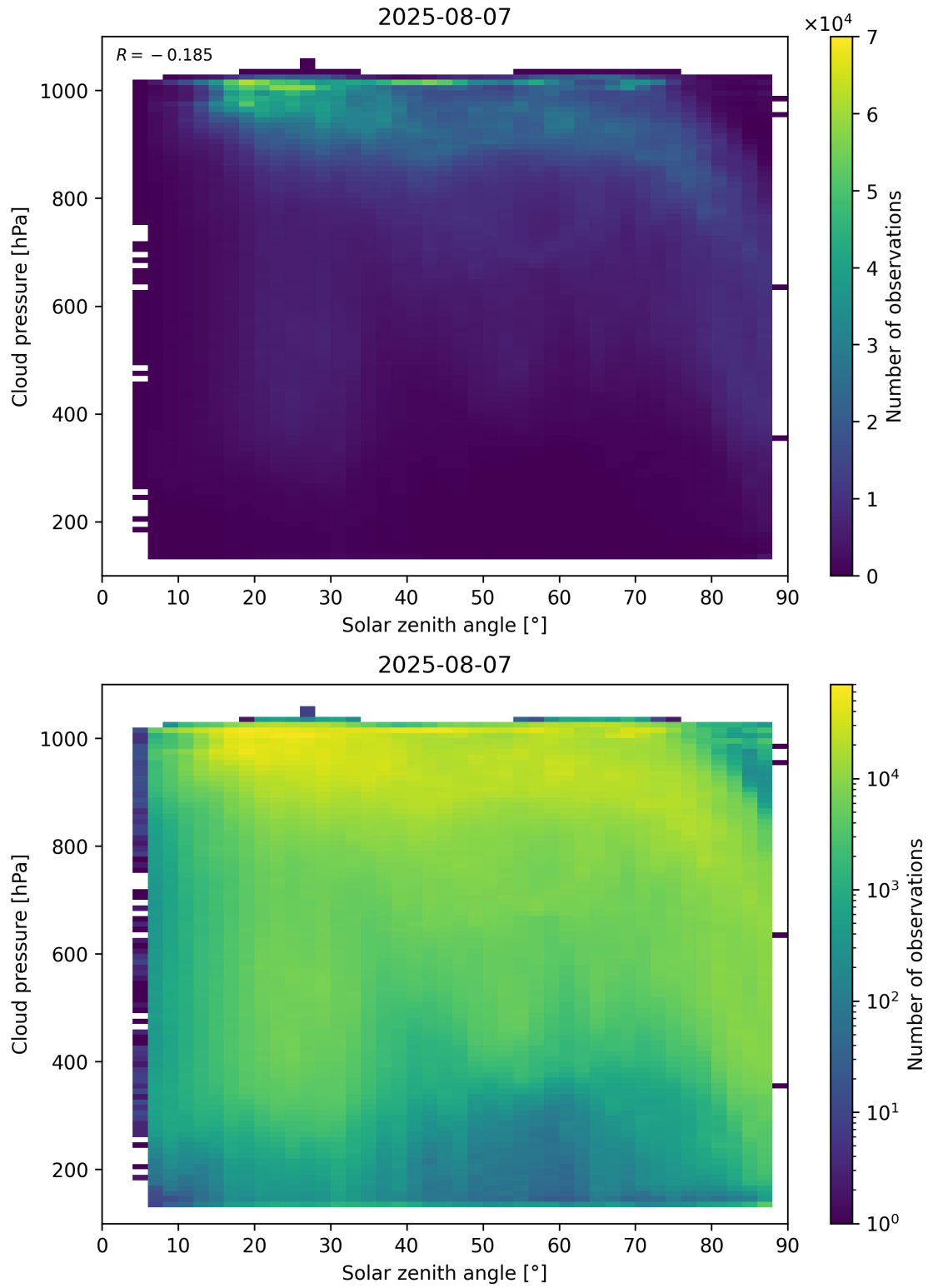
Figure 111: Scatter density plot of “Solar zenith angle” against “Cloud pressure” for 2025-08-06 to 2025-08-08.
