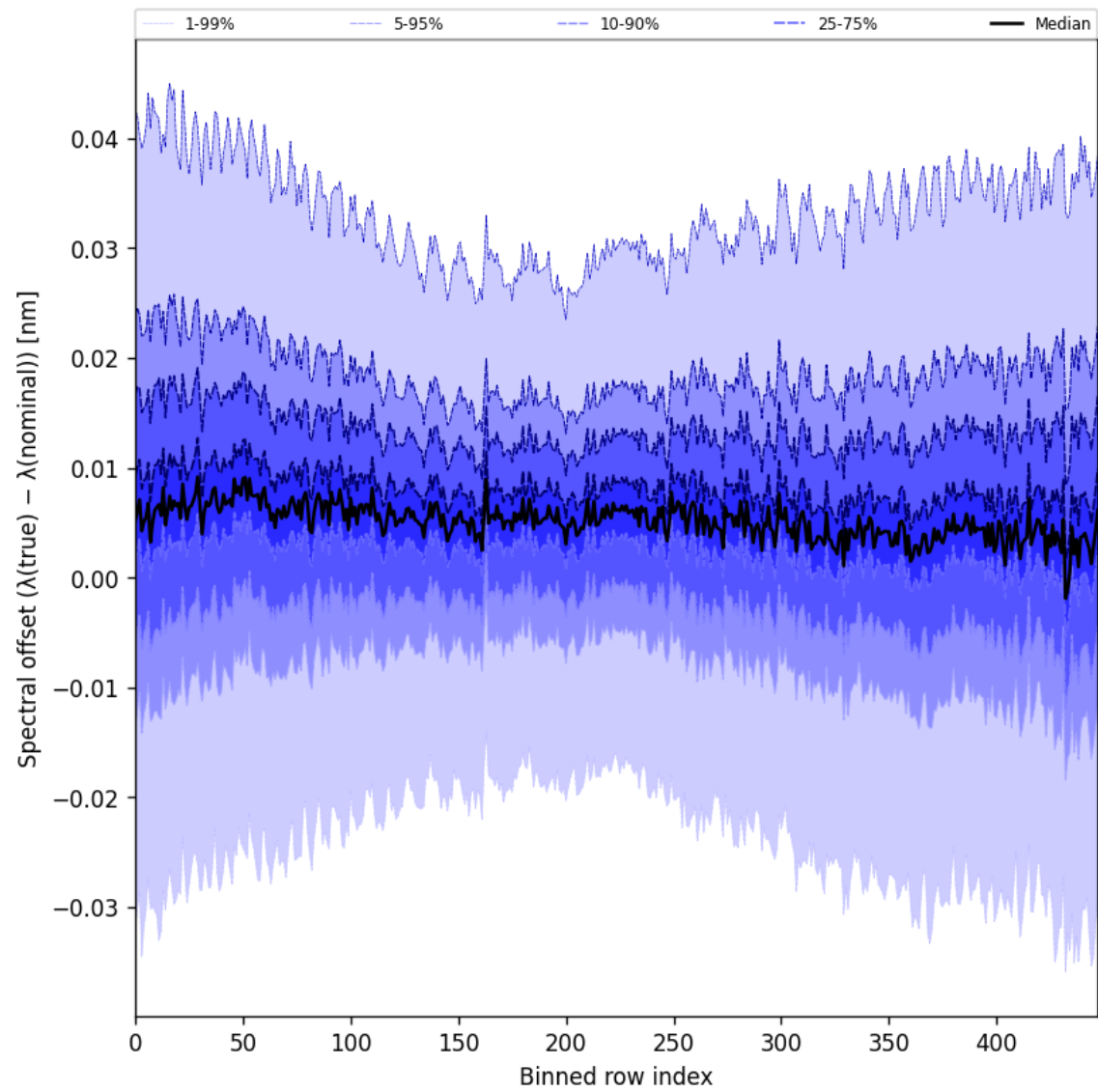
Figure 62: Along track statistics of “Spectral offset ( \lambda_{\text{true}} - \lambda_{\text{nominal}} )” for 2025-08-06 to 2025-08-08
