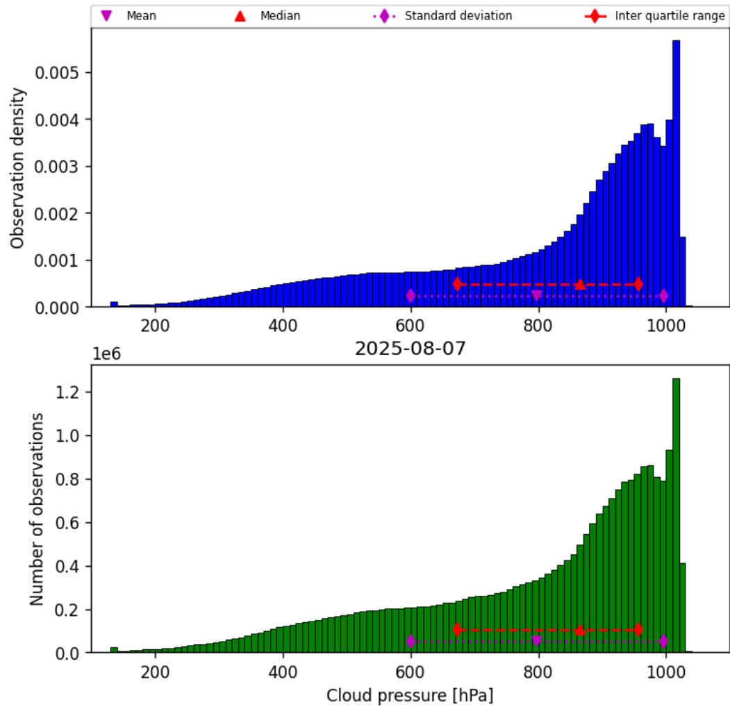
Figure 30: Histogram of “Cloud pressure” for 2025-08-06 to 2025-08-08
