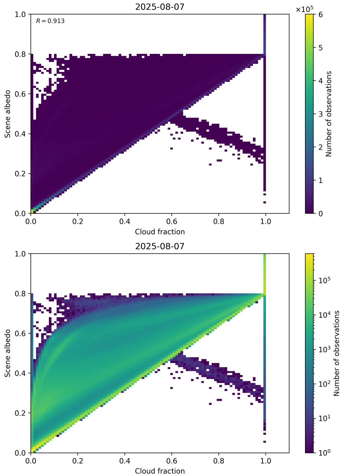
Figure 75: Scatter density plot of “Cloud fraction” against “Scene albedo” for 2025-08-06 to 2025-08-08.
