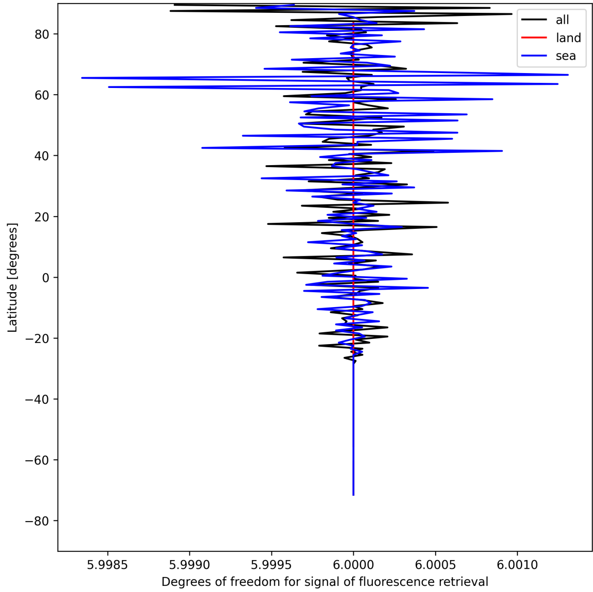
Figure 26: Zonal average of “Degrees of freedom for signal of fluorescence retrieval” for 2025-08-06 to 2025-08-08.
