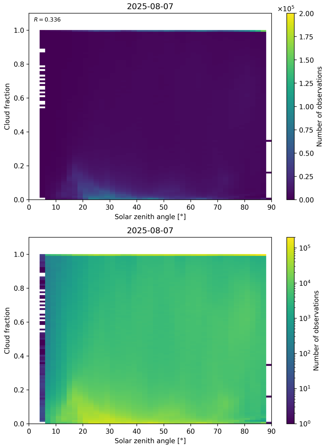
Figure 110: Scatter density plot of “Solar zenith angle” against “Cloud fraction” for 2025-08-06 to 2025-08-08.
