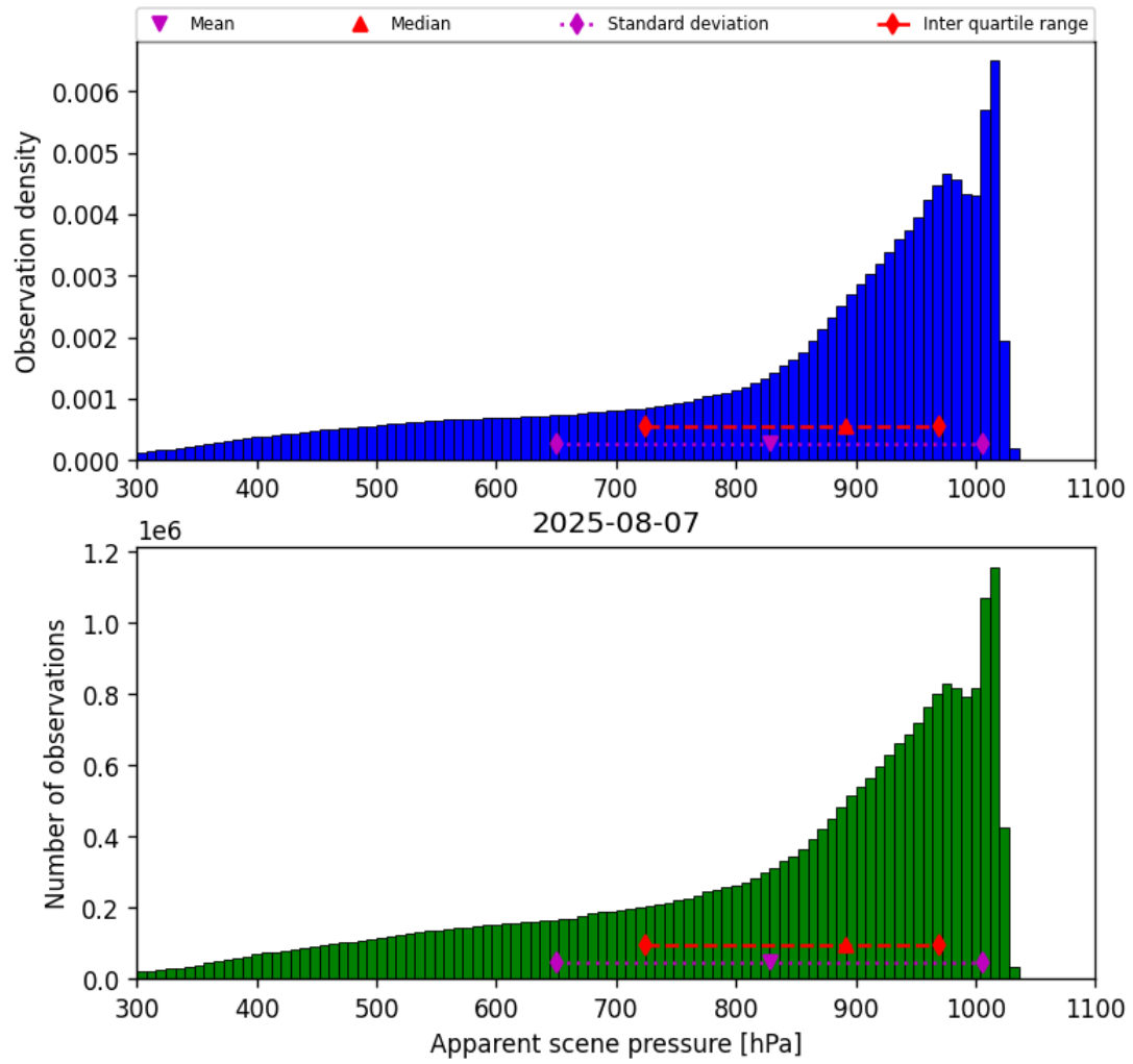
Figure 36: Histogram of “Apparent scene pressure” for 2025-08-06 to 2025-08-08
