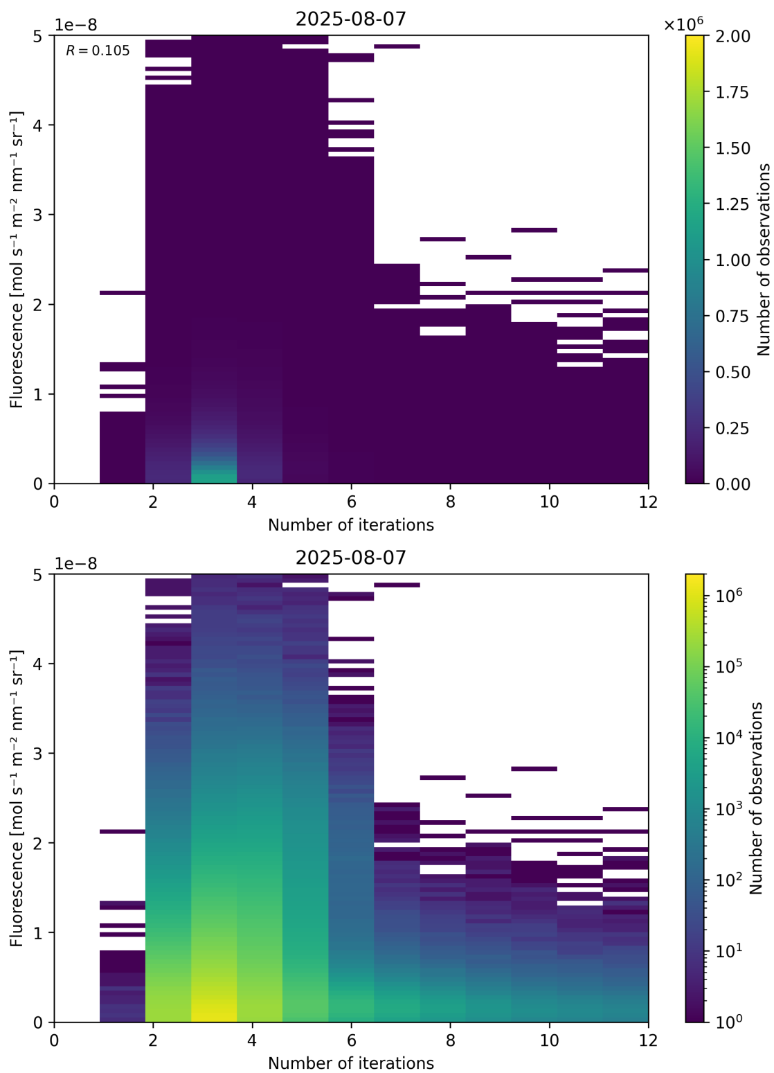
Figure 98: Scatter density plot of “Number of iterations” against “Fluorescence” for 2025-08-06 to 2025-08-08.
