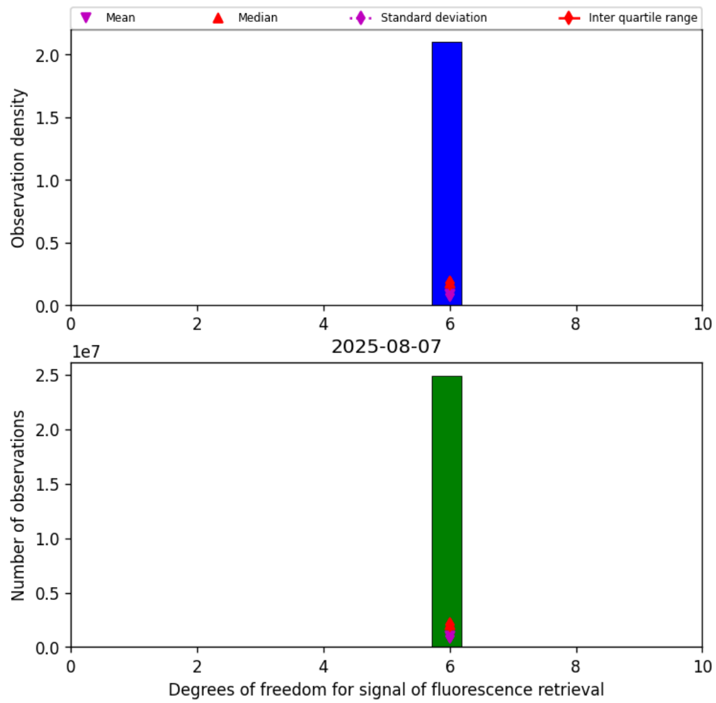
Figure 43: Histogram of “Degrees of freedom for signal of fluorescence retrieval” for 2025-08-06 to 2025-08-08
