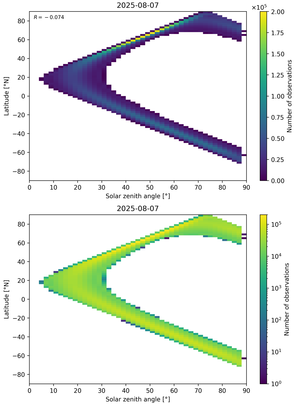
Figure 113: Scatter density plot of “Solar zenith angle” against “Latitude” for 2025-08-06 to 2025-08-08.
