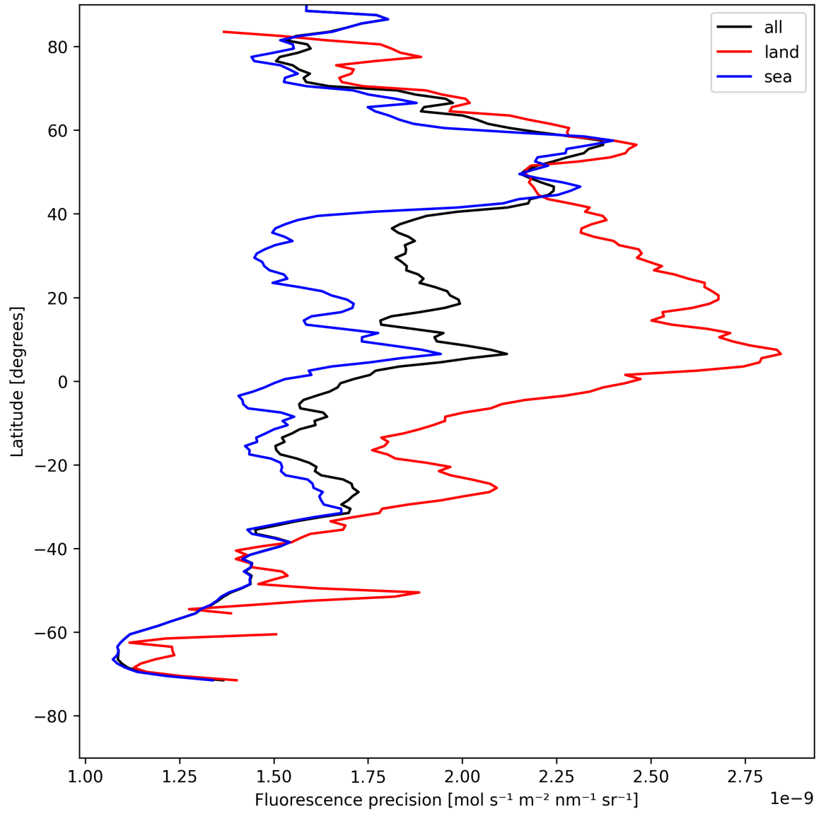
Figure 24: Zonal average of “Fluorescence precision” for 2025-08-06 to 2025-08-08.
