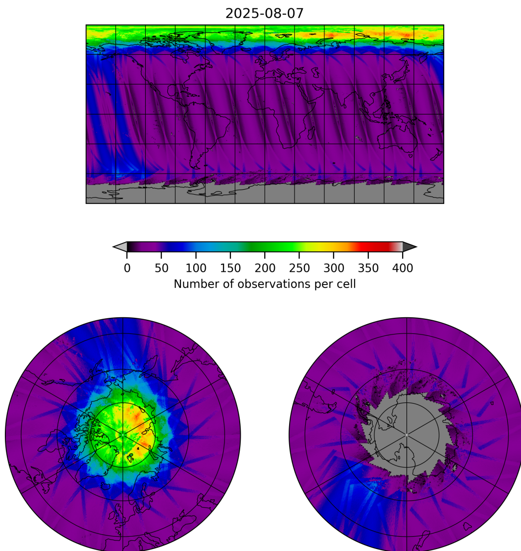
Figure 11: Map of the number of observations for 2025-08-06 to 2025-08-08
