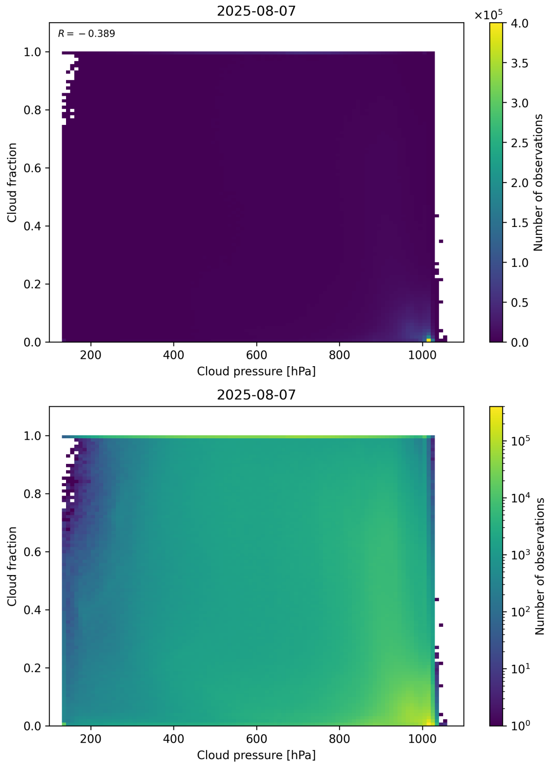
Figure 79: Scatter density plot of “Cloud pressure” against “Cloud fraction” for 2025-08-06 to 2025-08-08.
