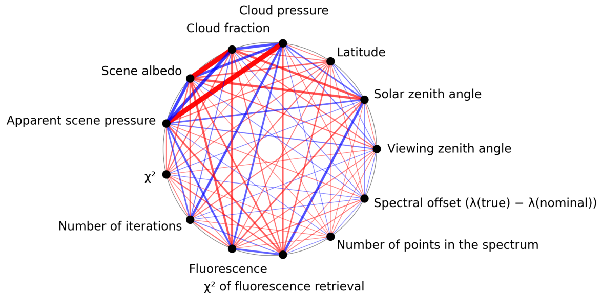
Figure 1: Map of correlation graph for 2025-08-06 to 2025-08-08.
