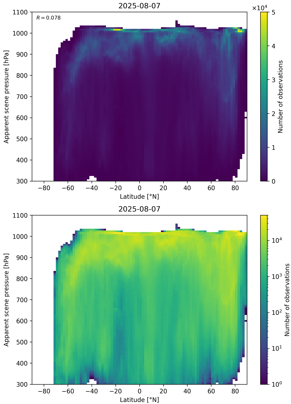
Figure 88: Scatter density plot of “Latitude” against “Apparent scene pressure” for 2025-08-06 to 2025-08-08.
