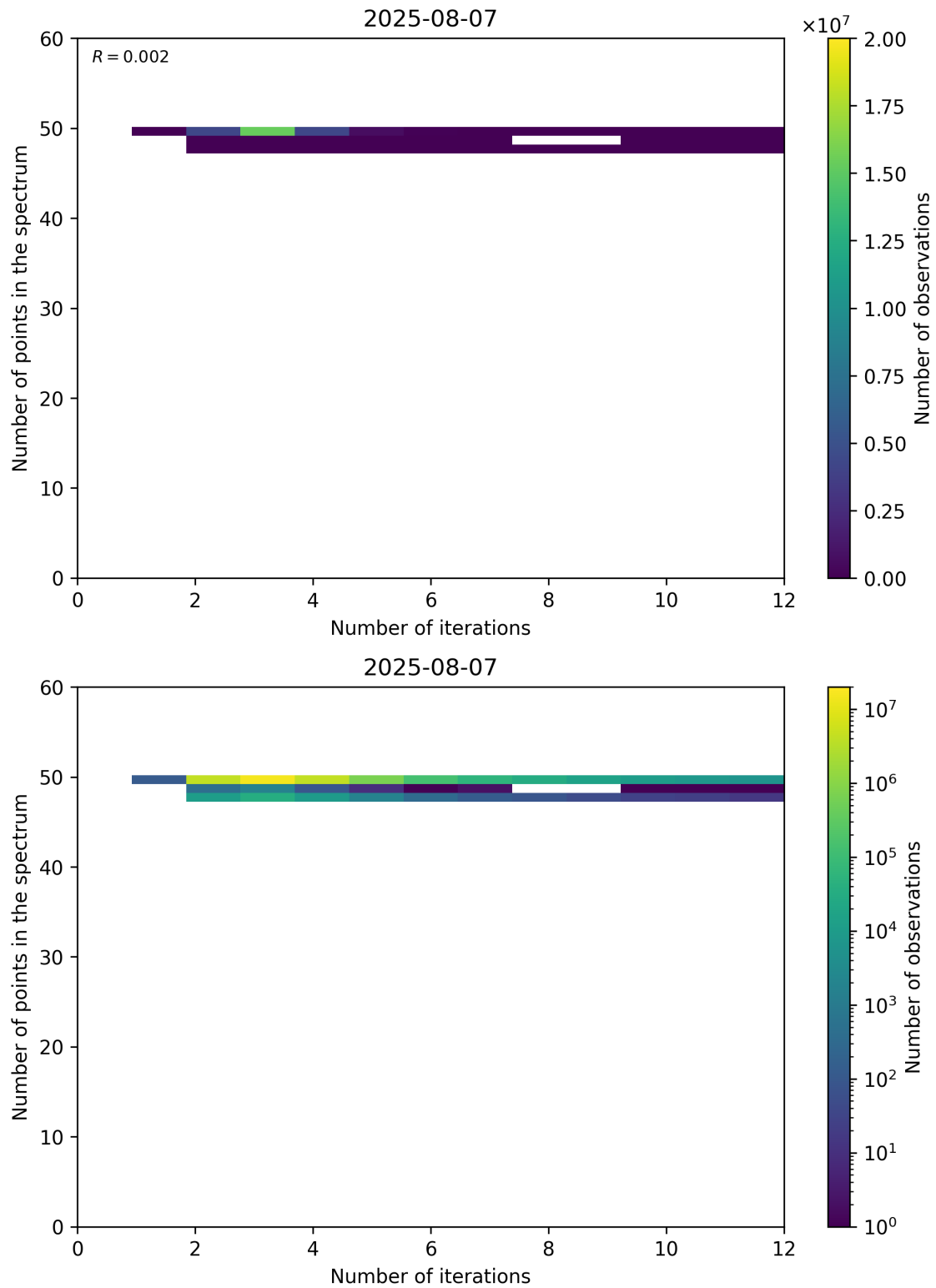
Figure 99: Scatter density plot of “Number of iterations” against “Number of points in the spectrum” for 2025-08-06 to 2025-08-08.
