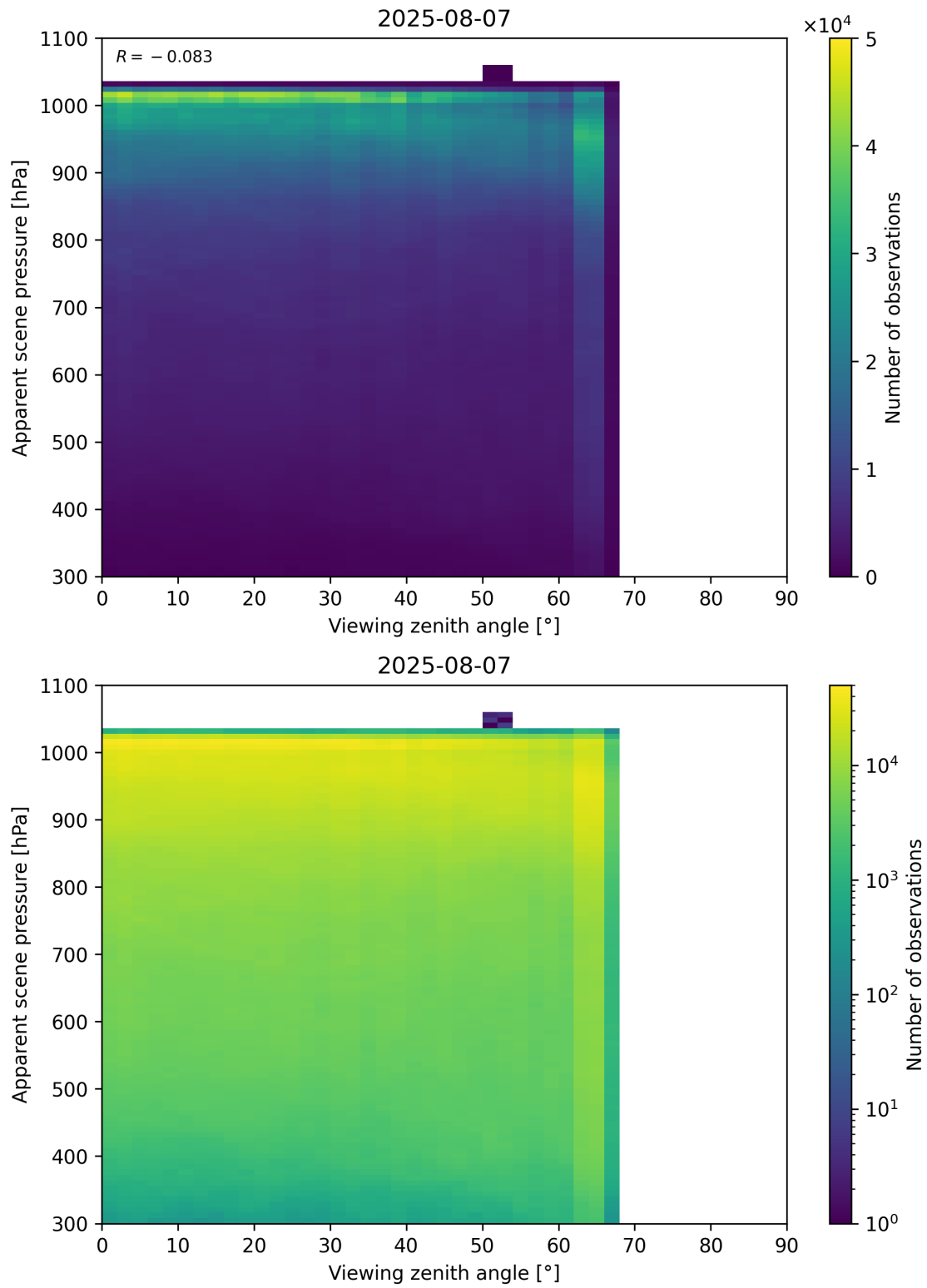
Figure 118: Scatter density plot of “Viewing zenith angle” against “Apparent scene pressure” for 2025-08-06 to 2025-08-08.
