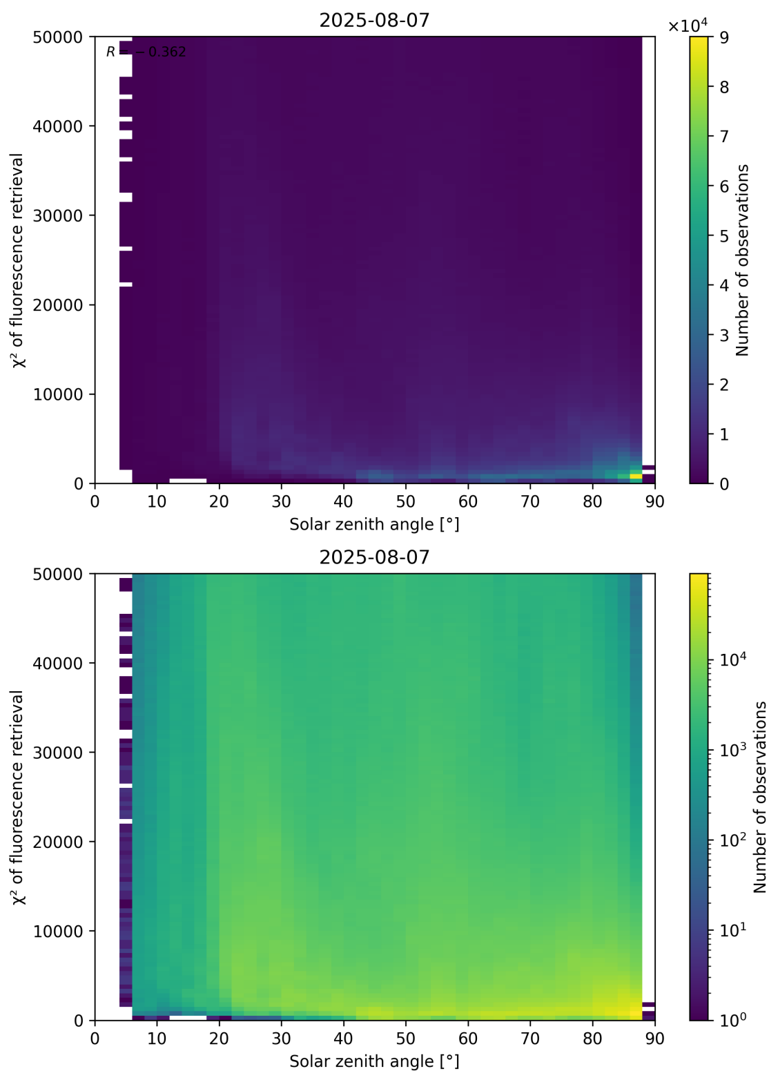
Figure 109: Scatter density plot of “Solar zenith angle” against “ \chi^2 of fluorescence retrieval” for 2025-08-06 to 2025-08-08.
