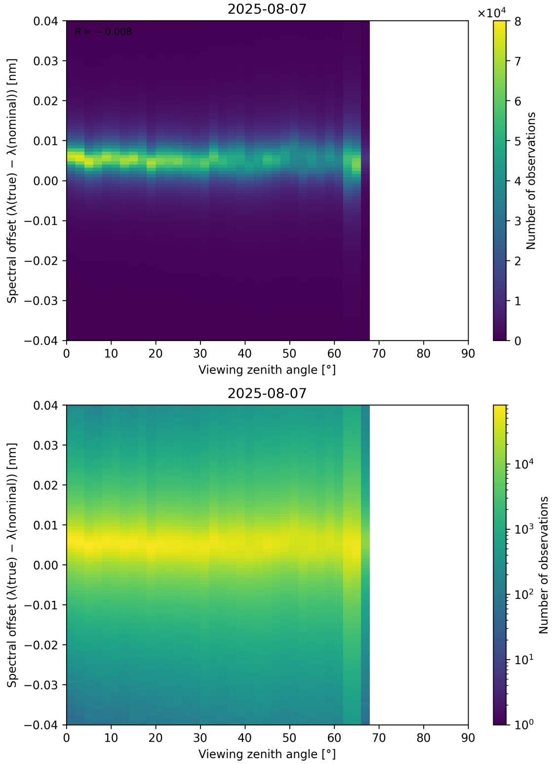
Figure 128: Scatter density plot of “Viewing zenith angle” against “Spectral offset ( \lambda_{\text{true}} - \lambda_{\text{nominal}} )” for 2025-08-06 to 2025-08-08.
