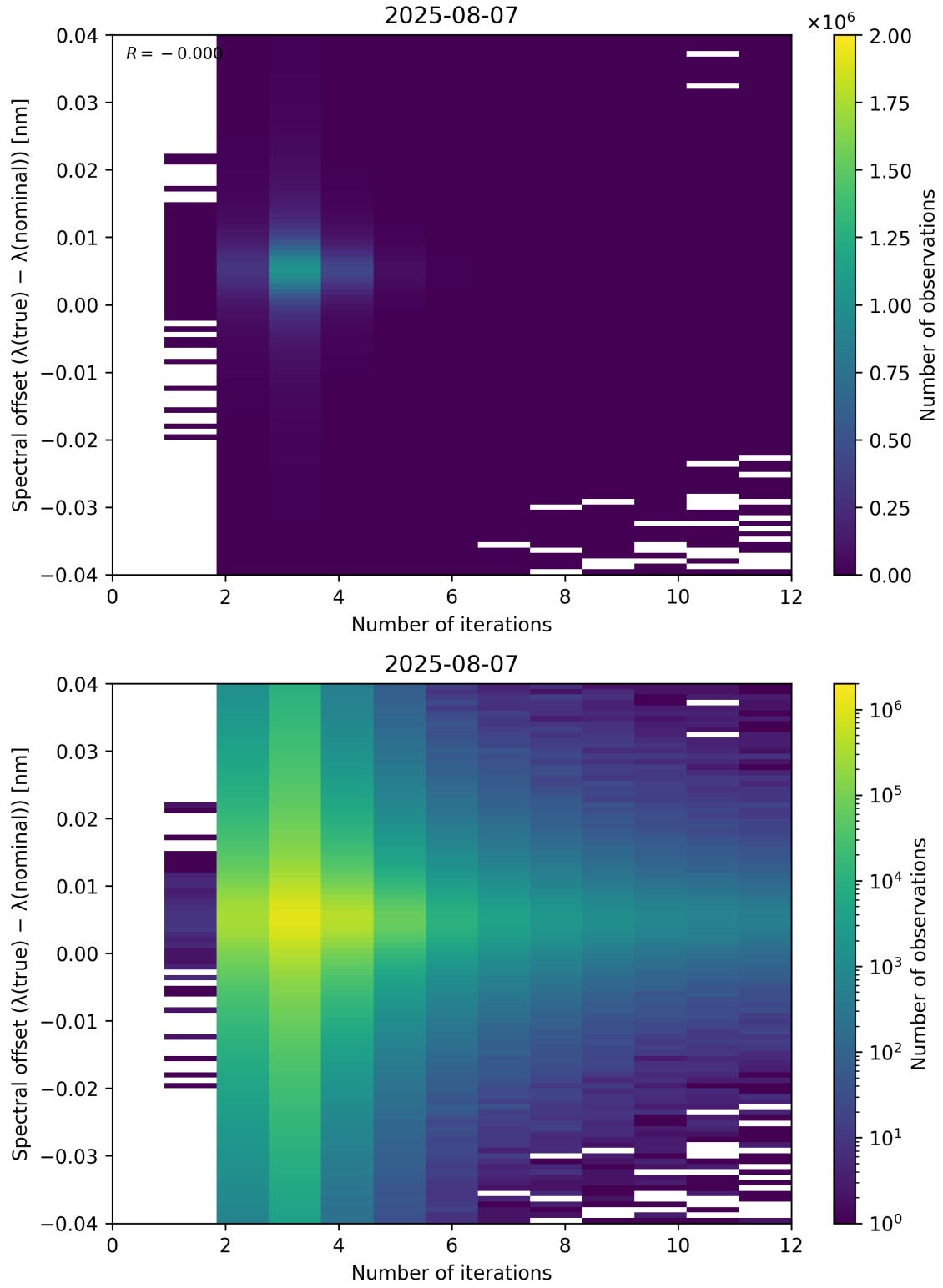
Figure 100: Scatter density plot of “Number of iterations” against “Spectral offset ( \lambda_{\text{true}} - \lambda_{\text{nominal}} )” for 2025-08-06 to 2025-08-08.
