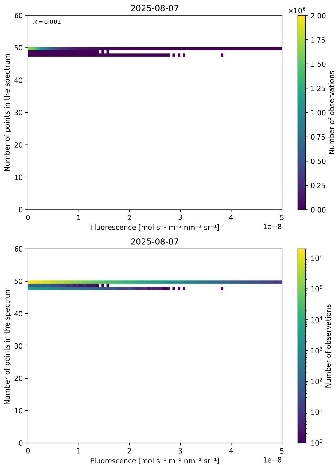
Figure 86: Scatter density plot of “Fluorescence” against “Number of points in the spectrum” for 2025-08-06 to 2025-08-08.
