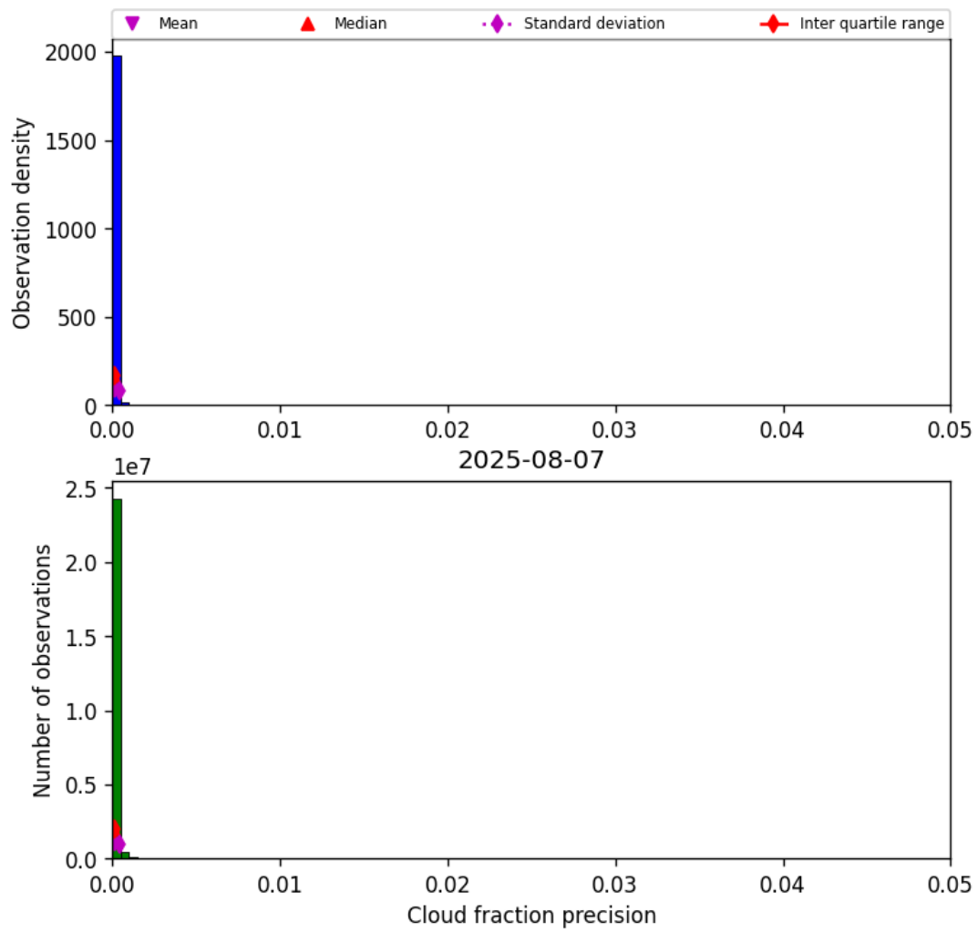
Figure 33: Histogram of “Cloud fraction precision” for 2025-08-06 to 2025-08-08
