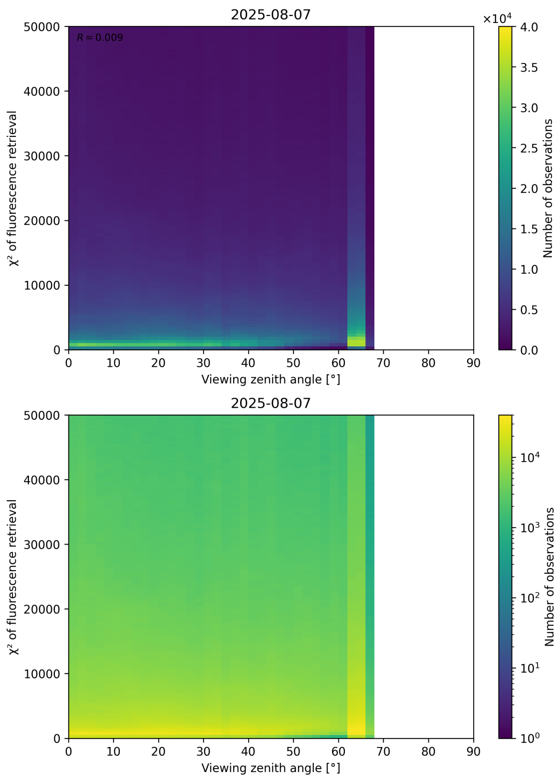
Figure 119: Scatter density plot of “Viewing zenith angle” against “ \chi^2 of fluorescence retrieval” for 2025-08-06 to 2025-08-08.
