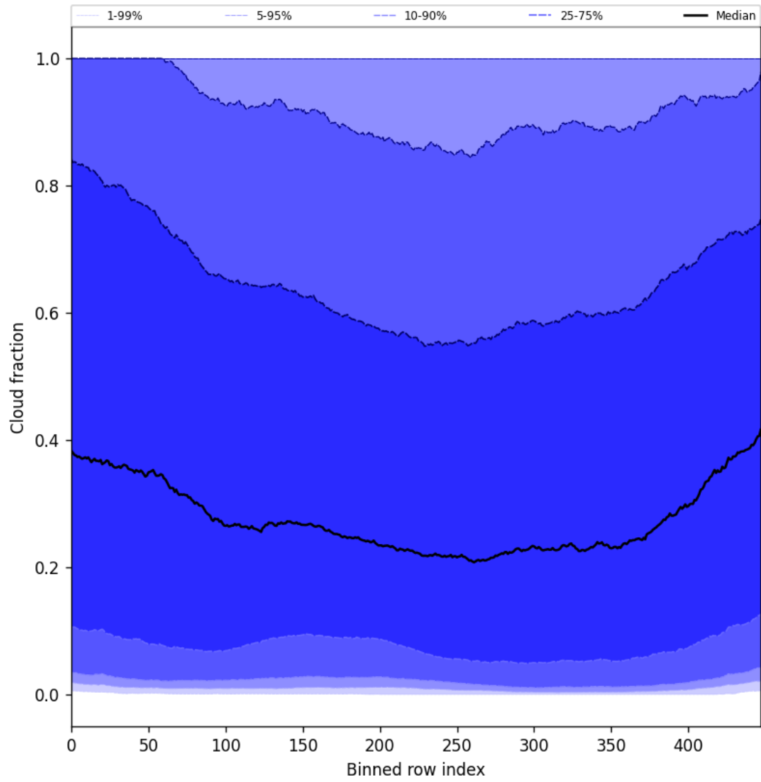
Figure 49: Along track statistics of “Cloud fraction” for 2025-08-06 to 2025-08-08
