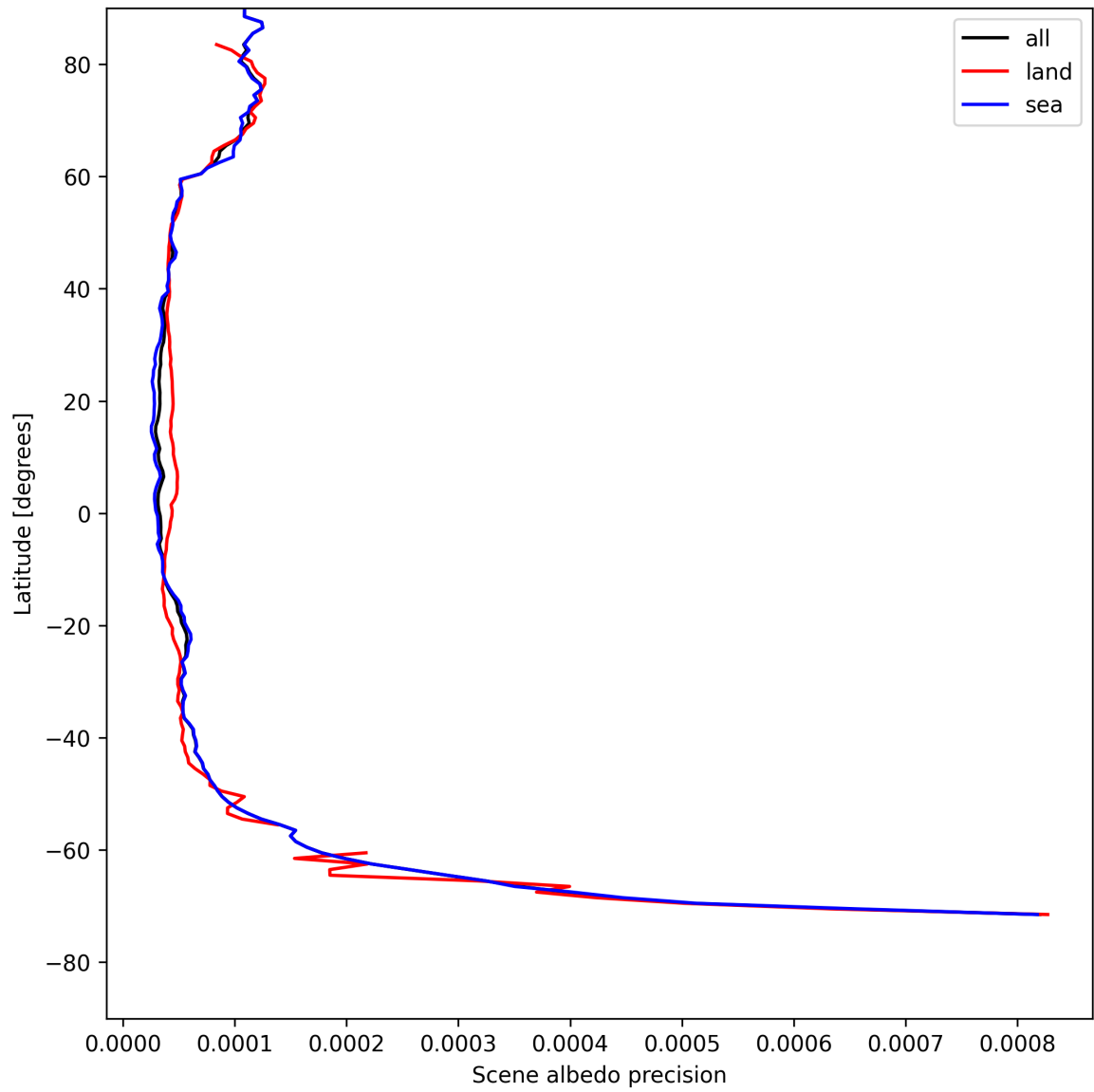
Figure 18: Zonal average of “Scene albedo precision” for 2025-08-06 to 2025-08-08.
