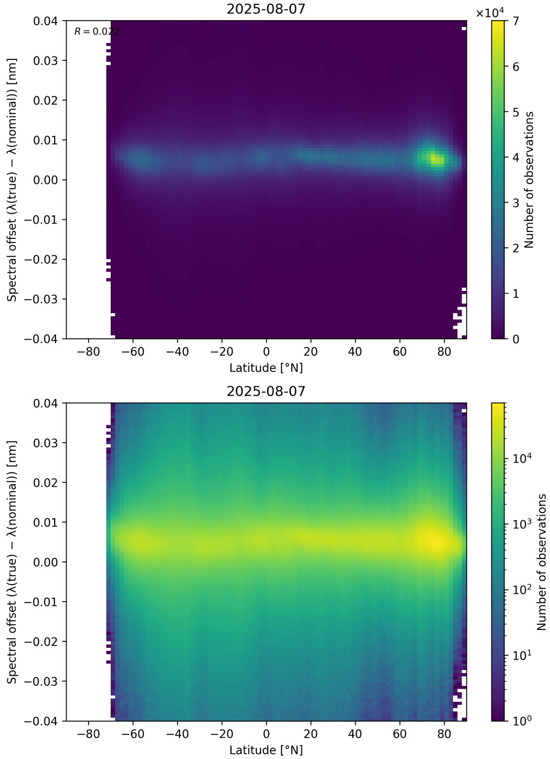
Figure 96: Scatter density plot of “Latitude” against “Spectral offset ( \lambda_{\text{true}} - \lambda_{\text{nominal}} )” for 2025-08-06 to 2025-08-08.
