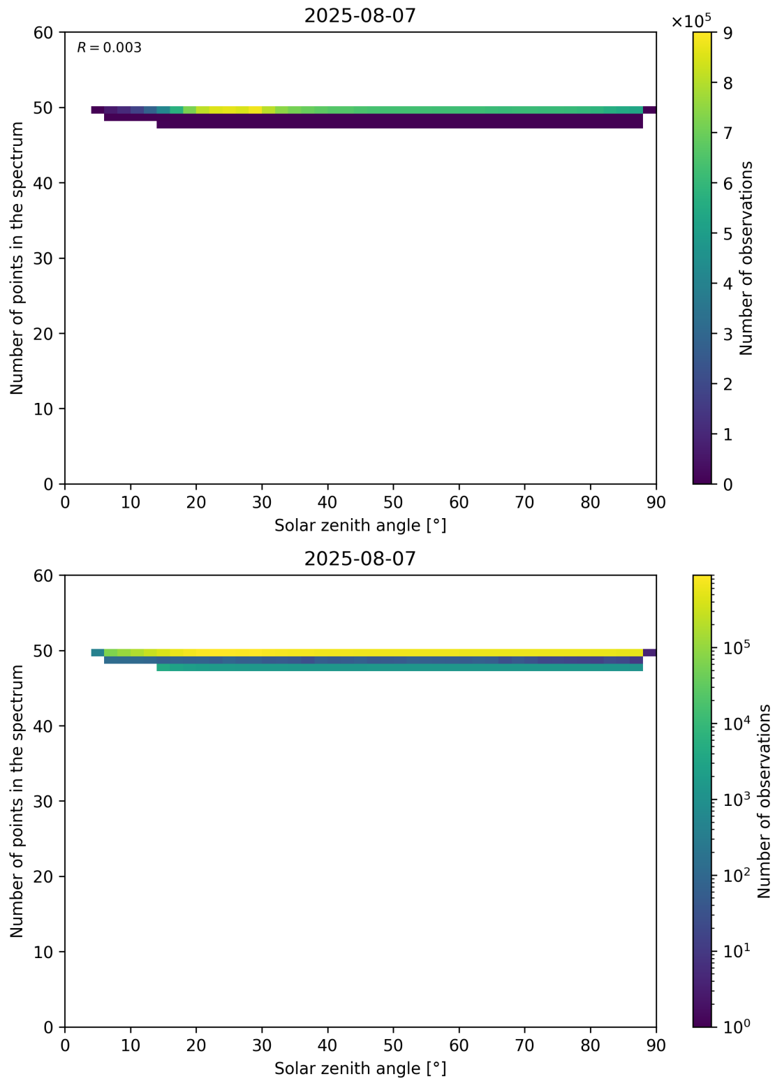
Figure 115: Scatter density plot of “Solar zenith angle” against “Number of points in the spectrum” for 2025-08-06 to 2025-08-08.
