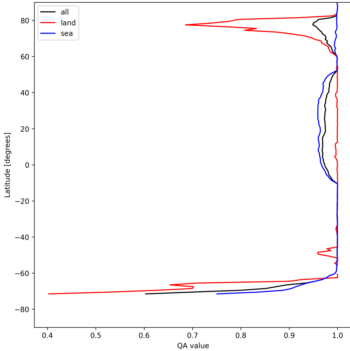
Figure 12: Zonal average of “QA value” for 2025-08-06 to 2025-08-08.
