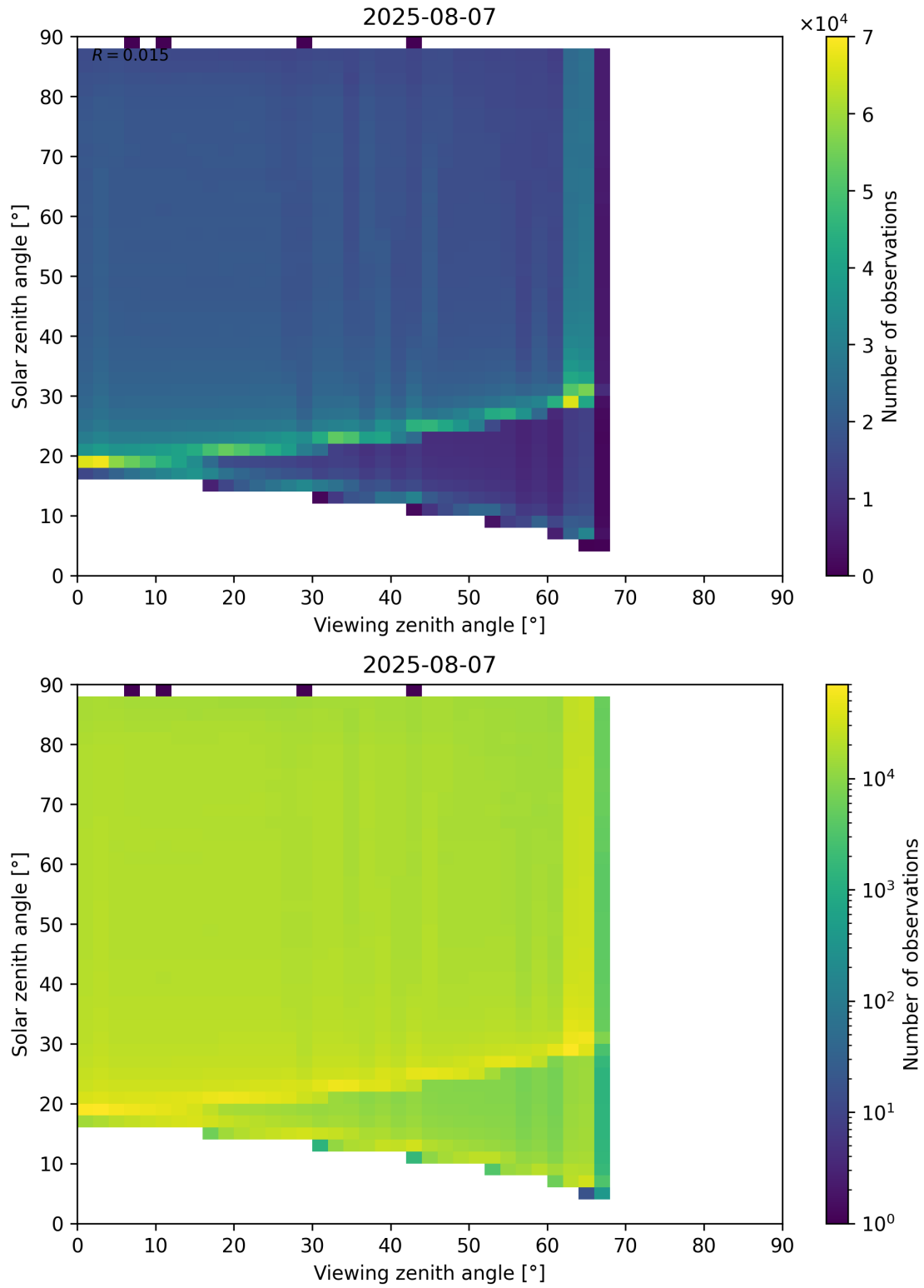
Figure 127: Scatter density plot of “Viewing zenith angle” against “Solar zenith angle” for 2025-08-06 to 2025-08-08.
