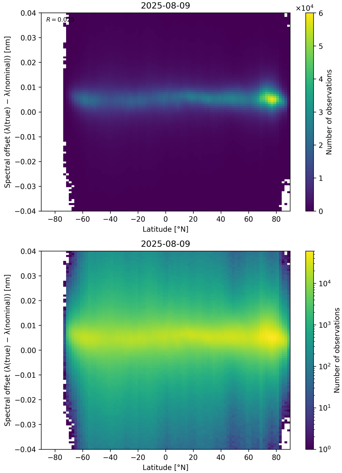
Figure 96: Scatter density plot of “Latitude” against “Spectral offset ( \lambda_{\text{true}} - \lambda_{\text{nominal}} )” for 2025-08-09 to 2025-08-10.
