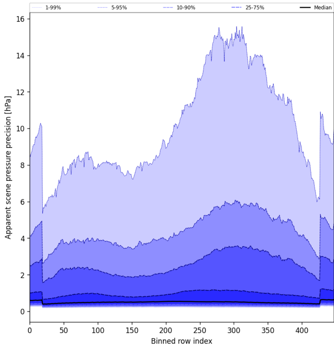
Figure 54: Along track statistics of “Apparent scene pressure precision” for 2025-08-09 to 2025-08-10
