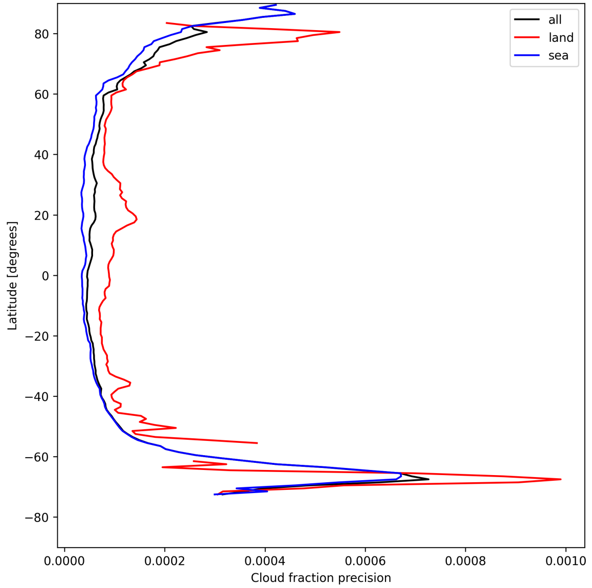
Figure 16: Zonal average of “Cloud fraction precision” for 2025-08-09 to 2025-08-10.
