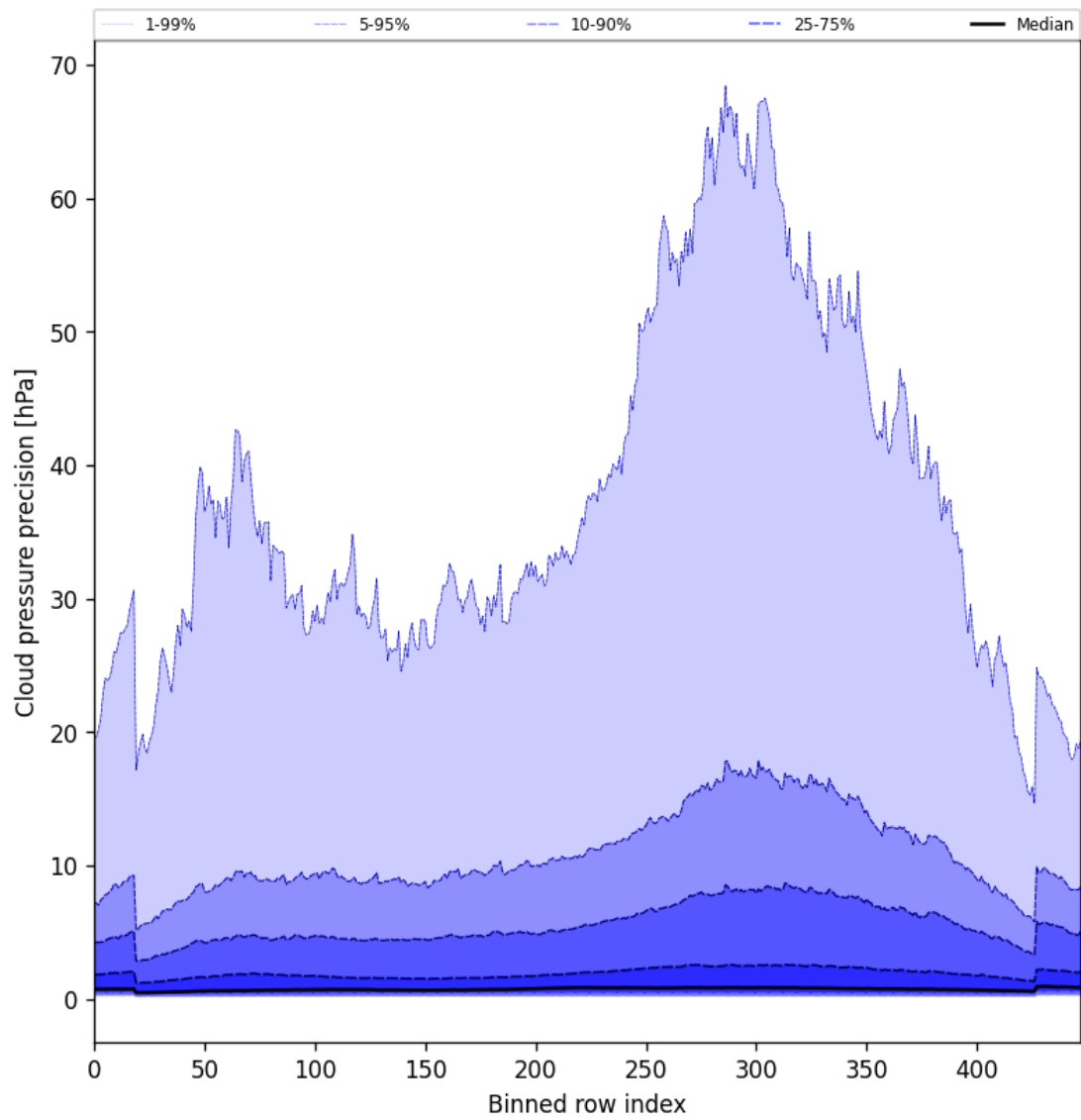
Figure 48: Along track statistics of “Cloud pressure precision” for 2025-08-09 to 2025-08-10
