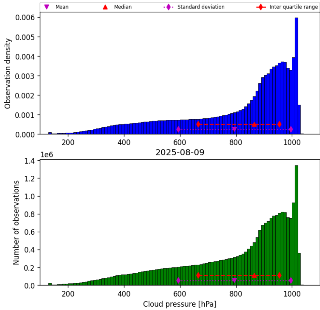
Figure 30: Histogram of “Cloud pressure” for 2025-08-09 to 2025-08-10
