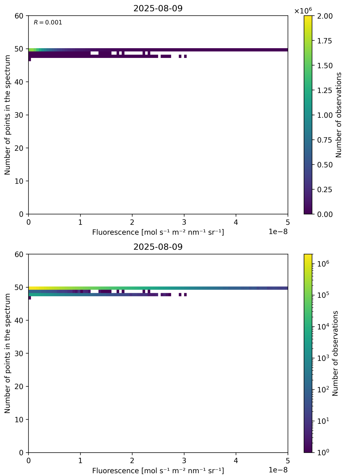
Figure 86: Scatter density plot of “Fluorescence” against “Number of points in the spectrum” for 2025-08-09 to 2025-08-10.
