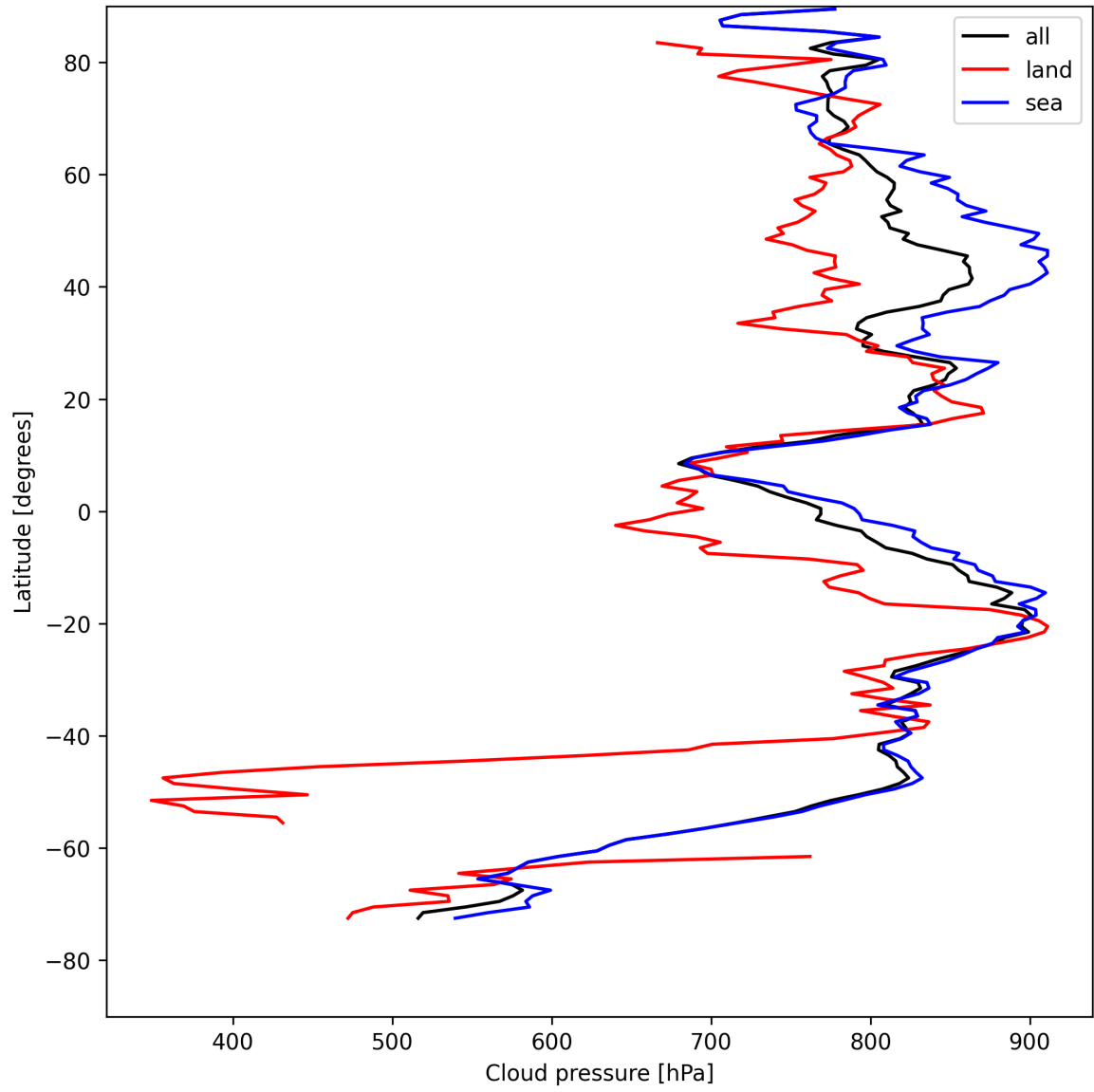
Figure 13: Zonal average of “Cloud pressure” for 2025-08-09 to 2025-08-10.
