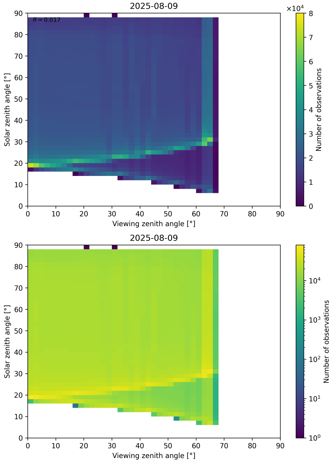
Figure 127: Scatter density plot of “Viewing zenith angle” against “Solar zenith angle” for 2025-08-09 to 2025-08-10.
