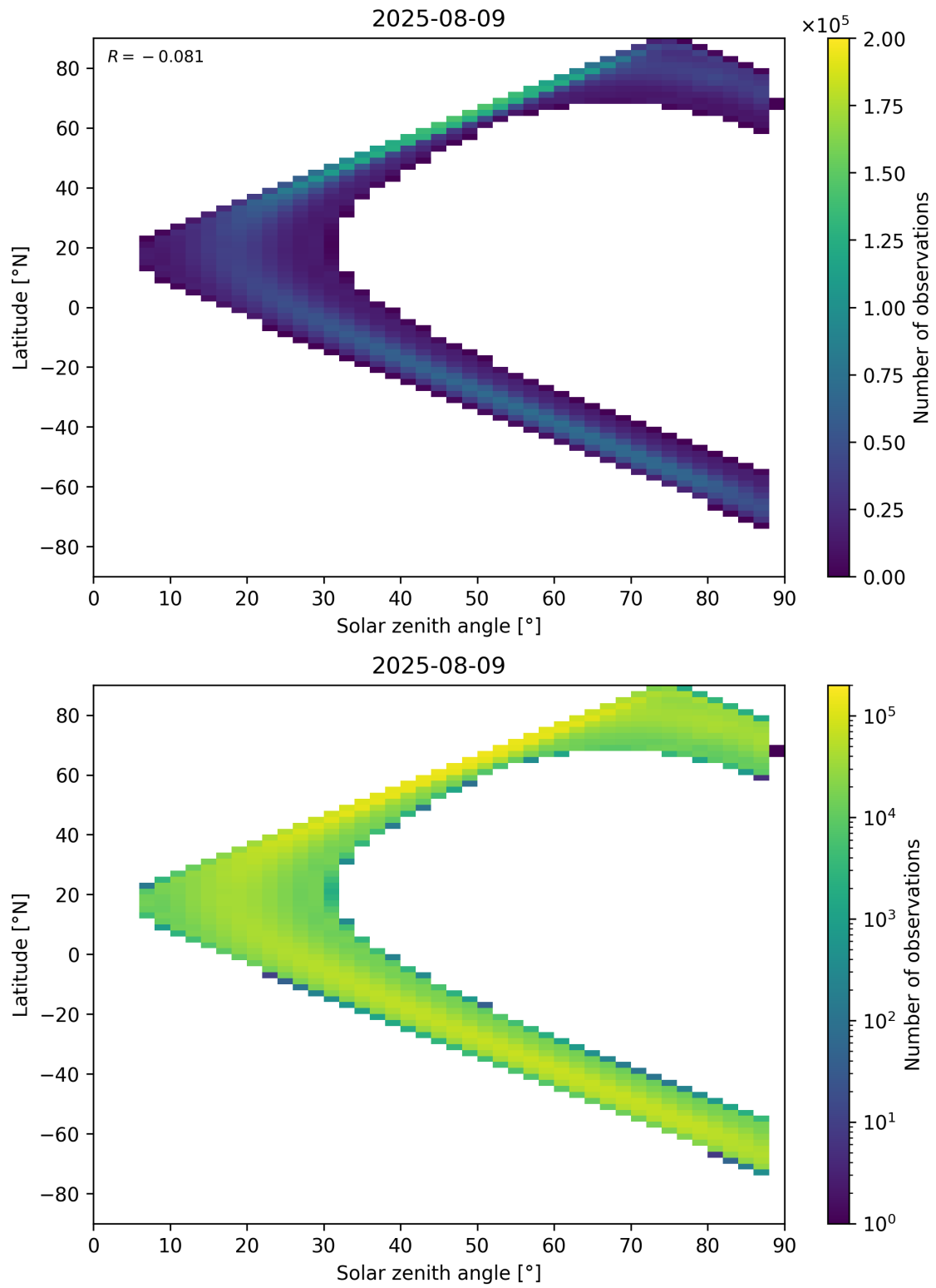
Figure 113: Scatter density plot of “Solar zenith angle” against “Latitude” for 2025-08-09 to 2025-08-10.
