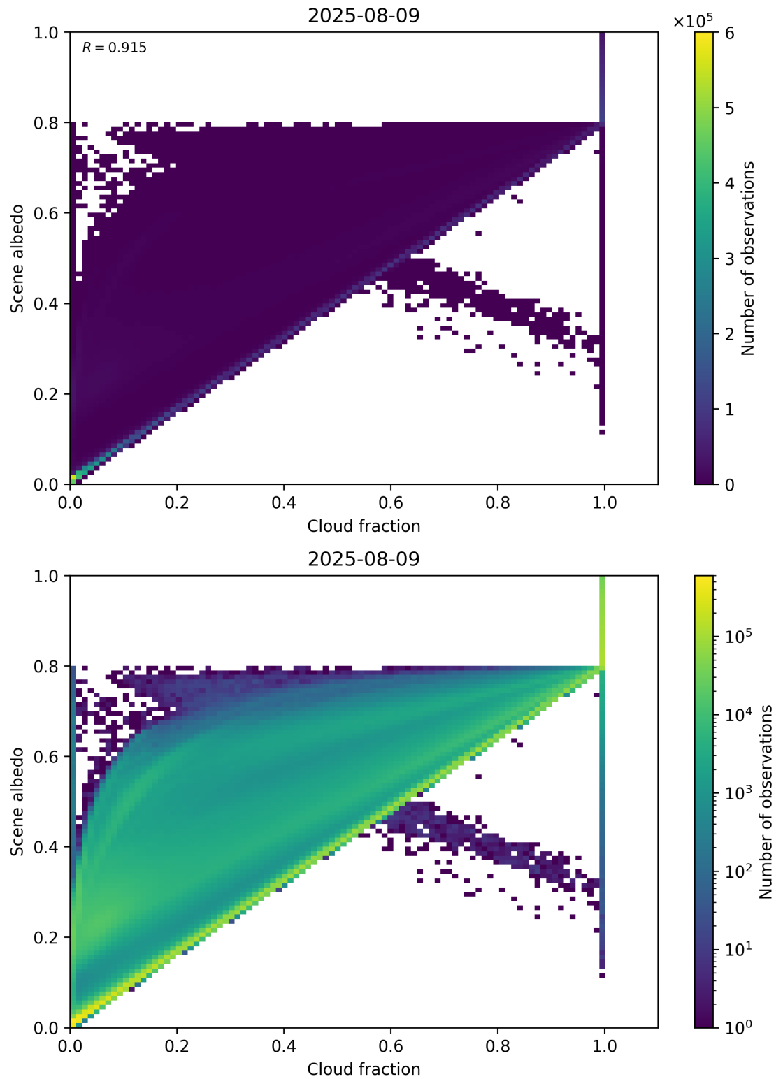
Figure 75: Scatter density plot of “Cloud fraction” against “Scene albedo” for 2025-08-09 to 2025-08-10.
