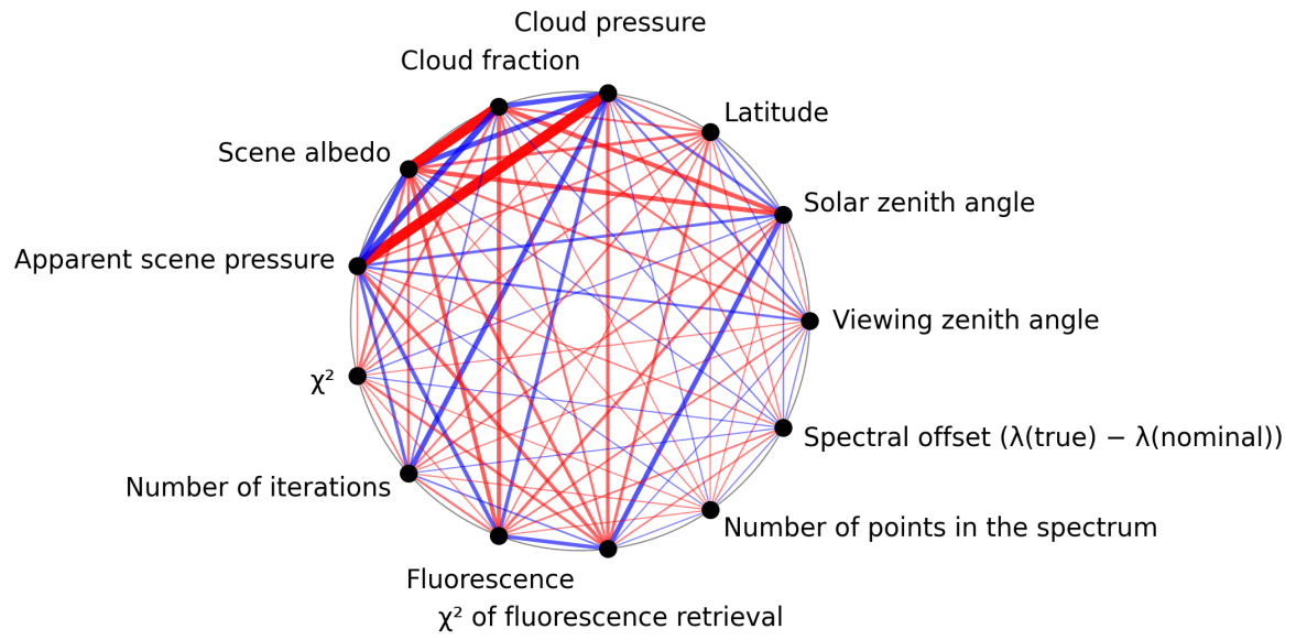
Figure 1: Map of correlation graph for 2025-08-09 to 2025-08-10.
