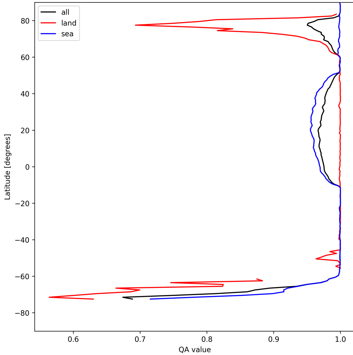
Figure 12: Zonal average of "QA value" for 2025-08-09 to 2025-08-10.
