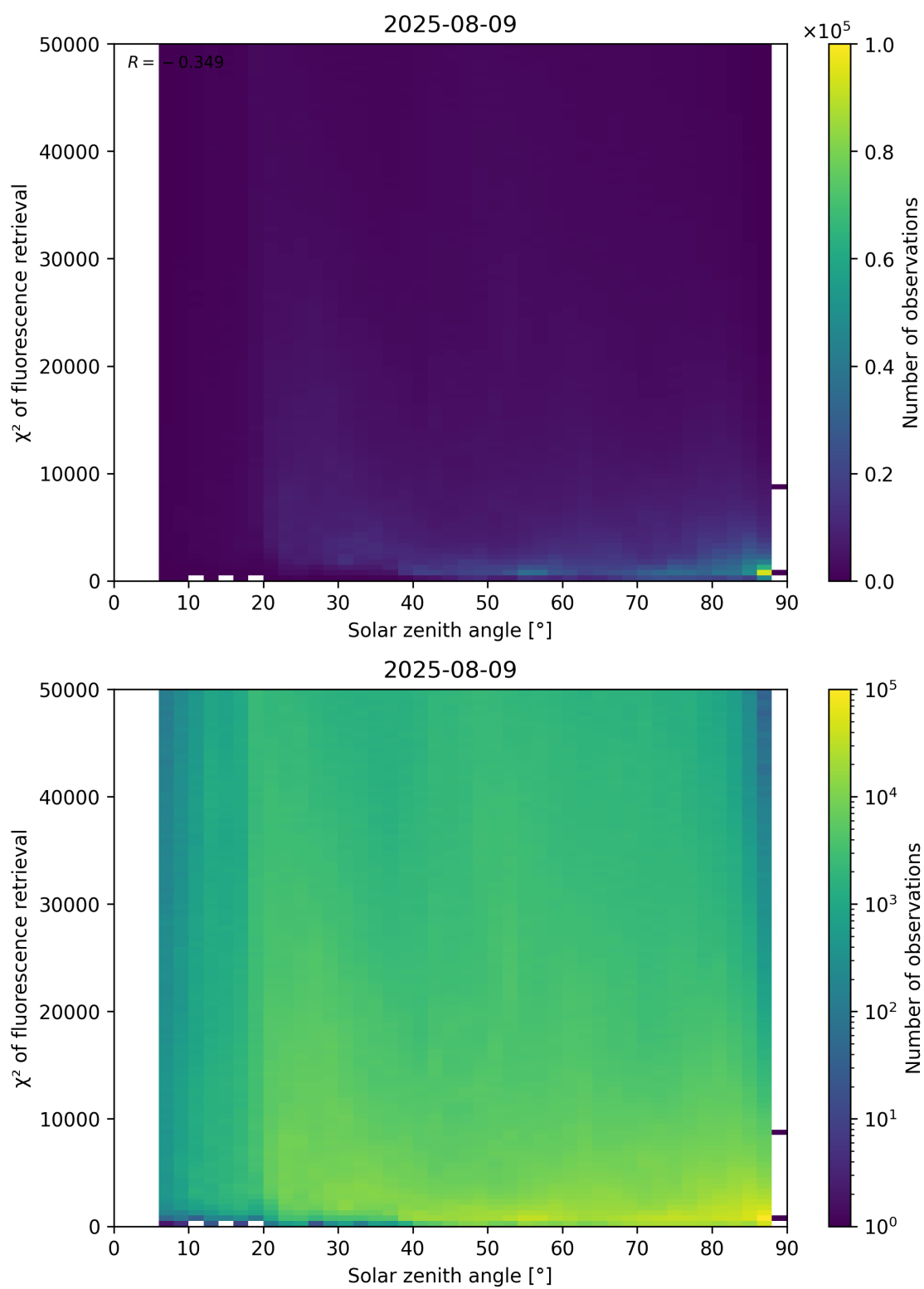
Figure 109: Scatter density plot of “Solar zenith angle” against “ \chi^2 of fluorescence retrieval” for 2025-08-09 to 2025-08-10.
