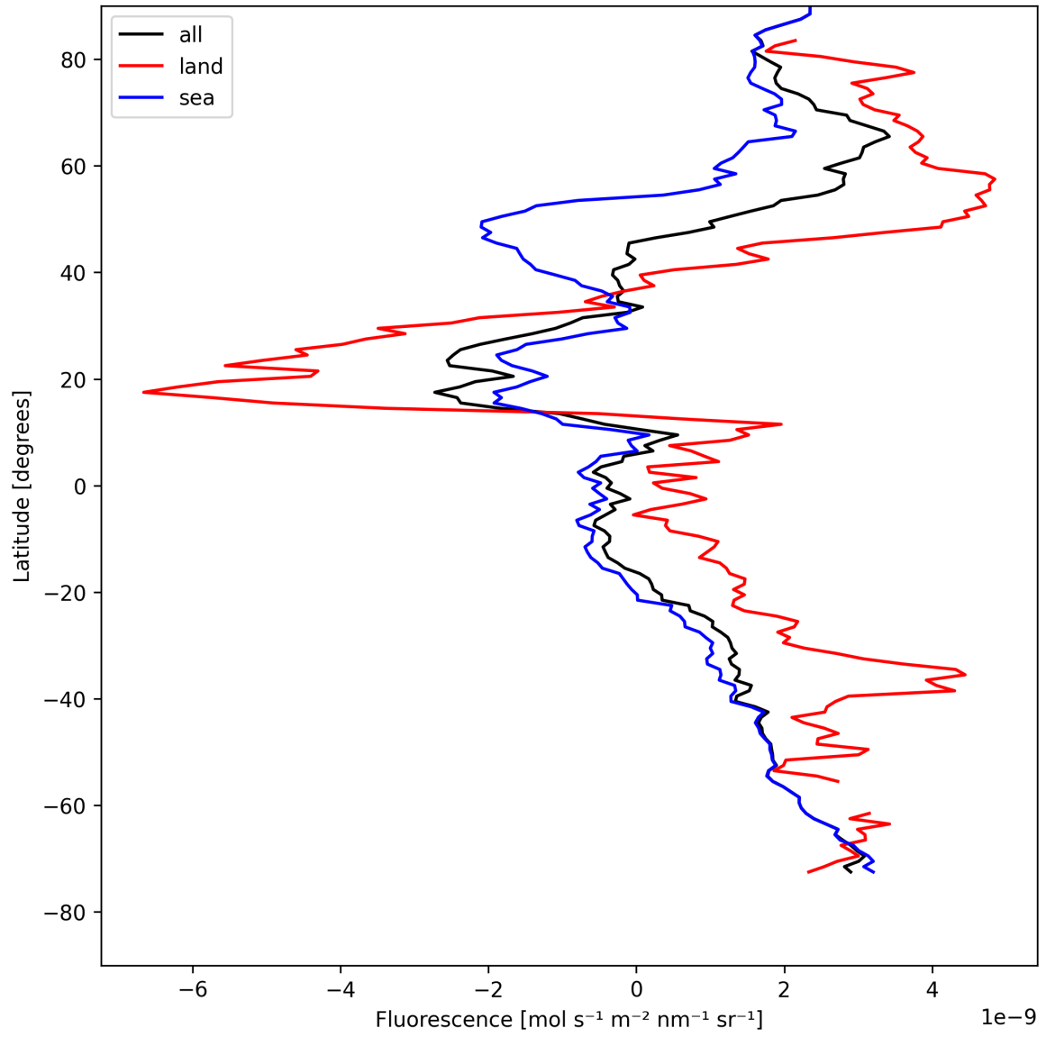
Figure 23: Zonal average of “Fluorescence” for 2025-08-09 to 2025-08-10.
