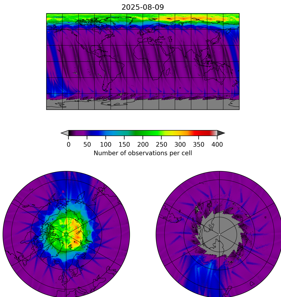
Figure 11: Map of the number of observations for 2025-08-09 to 2025-08-10
