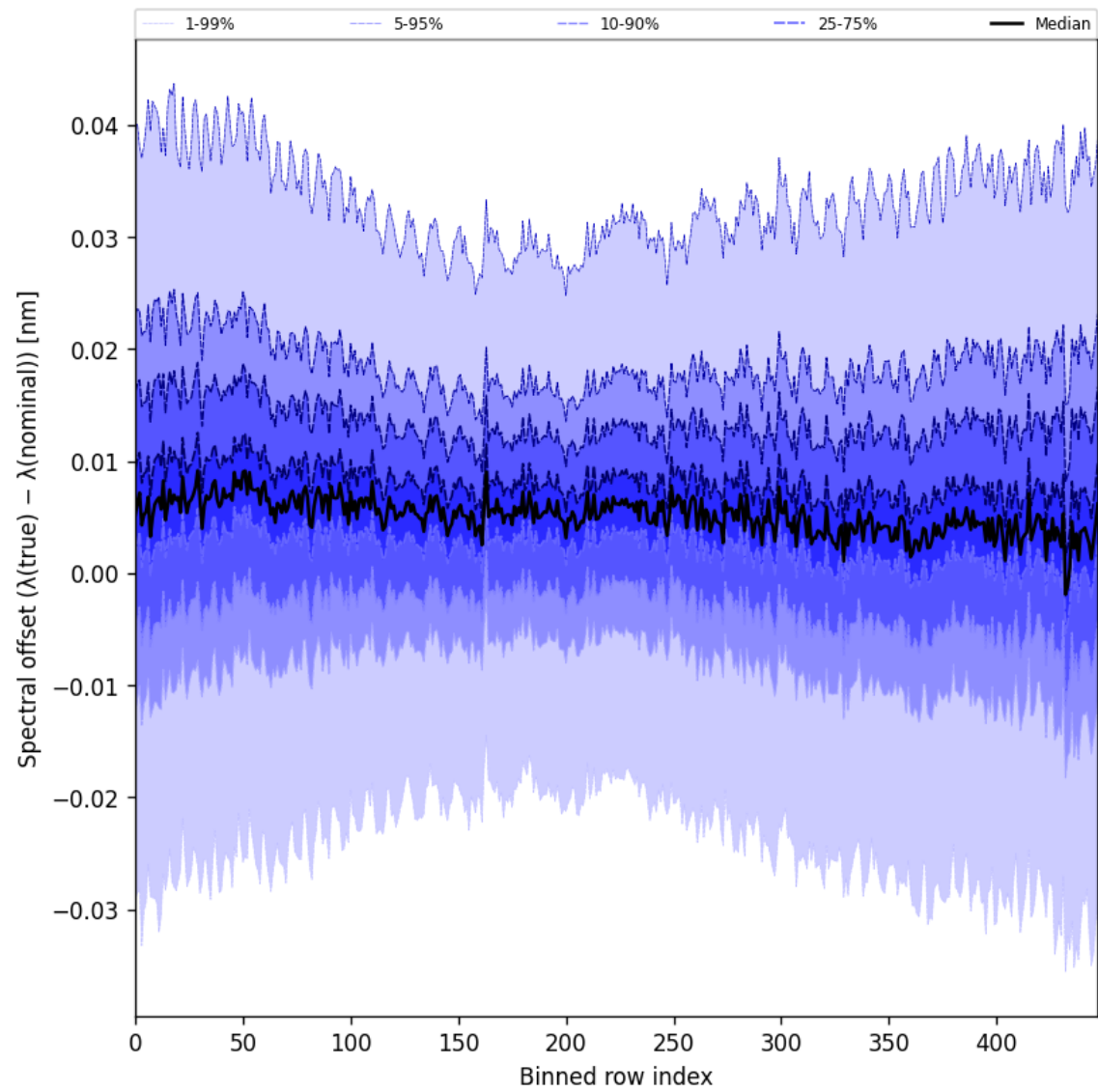
Figure 62: Along track statistics of “Spectral offset ( \lambda_{\text{true}} - \lambda_{\text{nominal}} )” for 2025-08-09 to 2025-08-10
