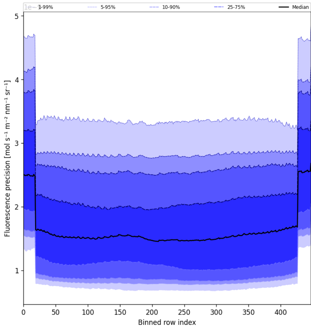
Figure 58: Along track statistics of “Fluorescence precision” for 2025-08-09 to 2025-08-10
