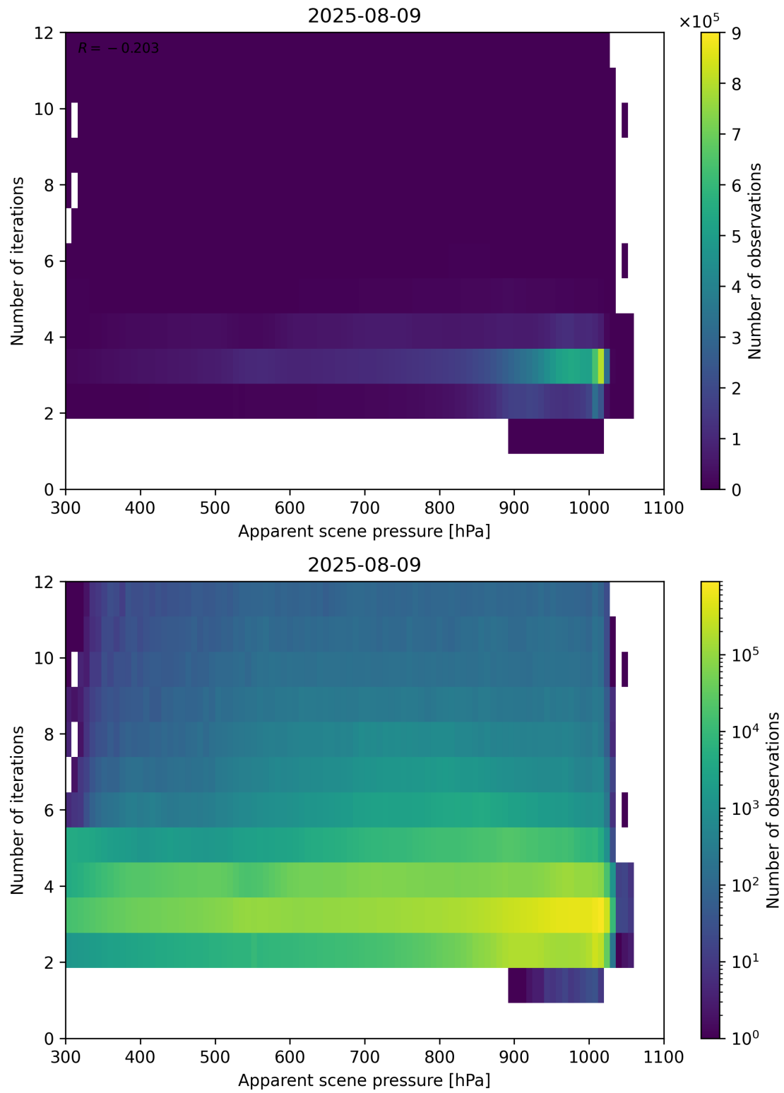
Figure 65: Scatter density plot of “Apparent scene pressure” against “Number of iterations” for 2025-08-09 to 2025-08-10.
