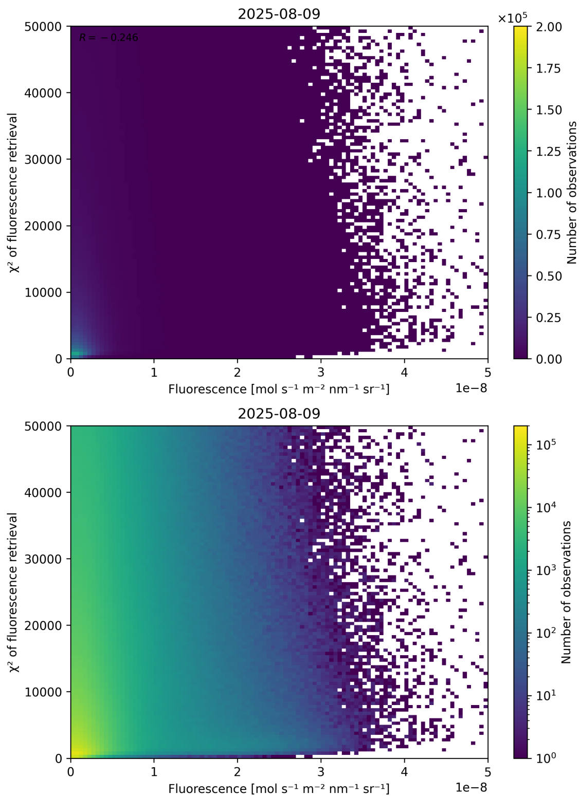
Figure 85: Scatter density plot of “Fluorescence” against “ \chi^2 of fluorescence retrieval” for 2025-08-09 to 2025-08-10.
