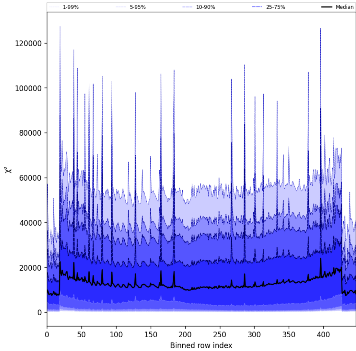
Figure 55: Along track statistics of “ \chi^2 ” for 2025-08-09 to 2025-08-10
