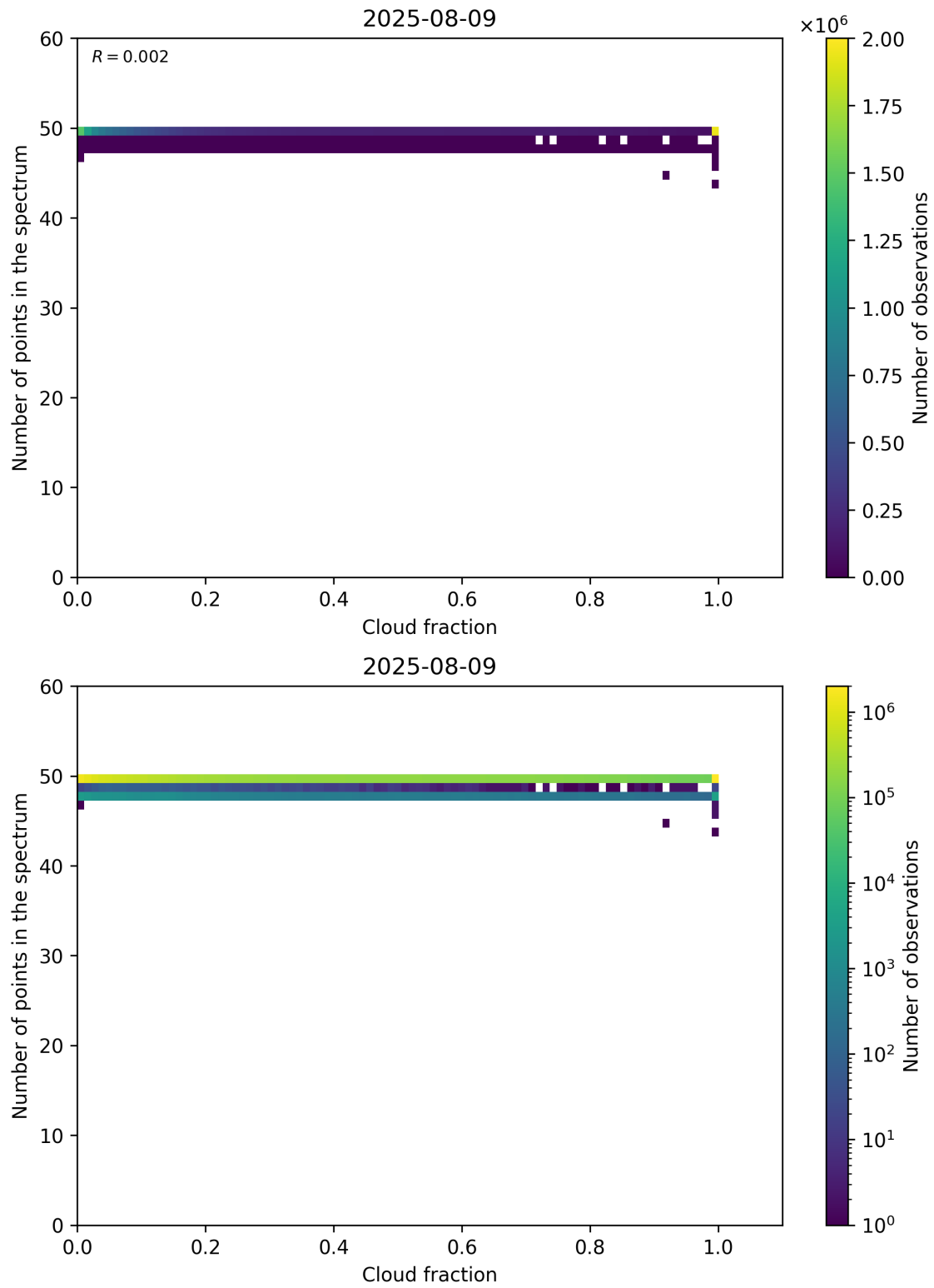
Figure 74: Scatter density plot of “Cloud fraction” against “Number of points in the spectrum” for 2025-08-09 to 2025-08-10.
