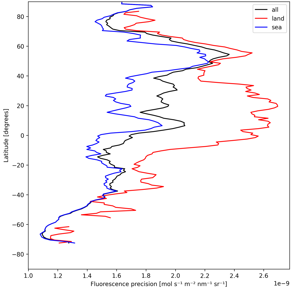
Figure 24: Zonal average of “Fluorescence precision” for 2025-08-09 to 2025-08-10.
