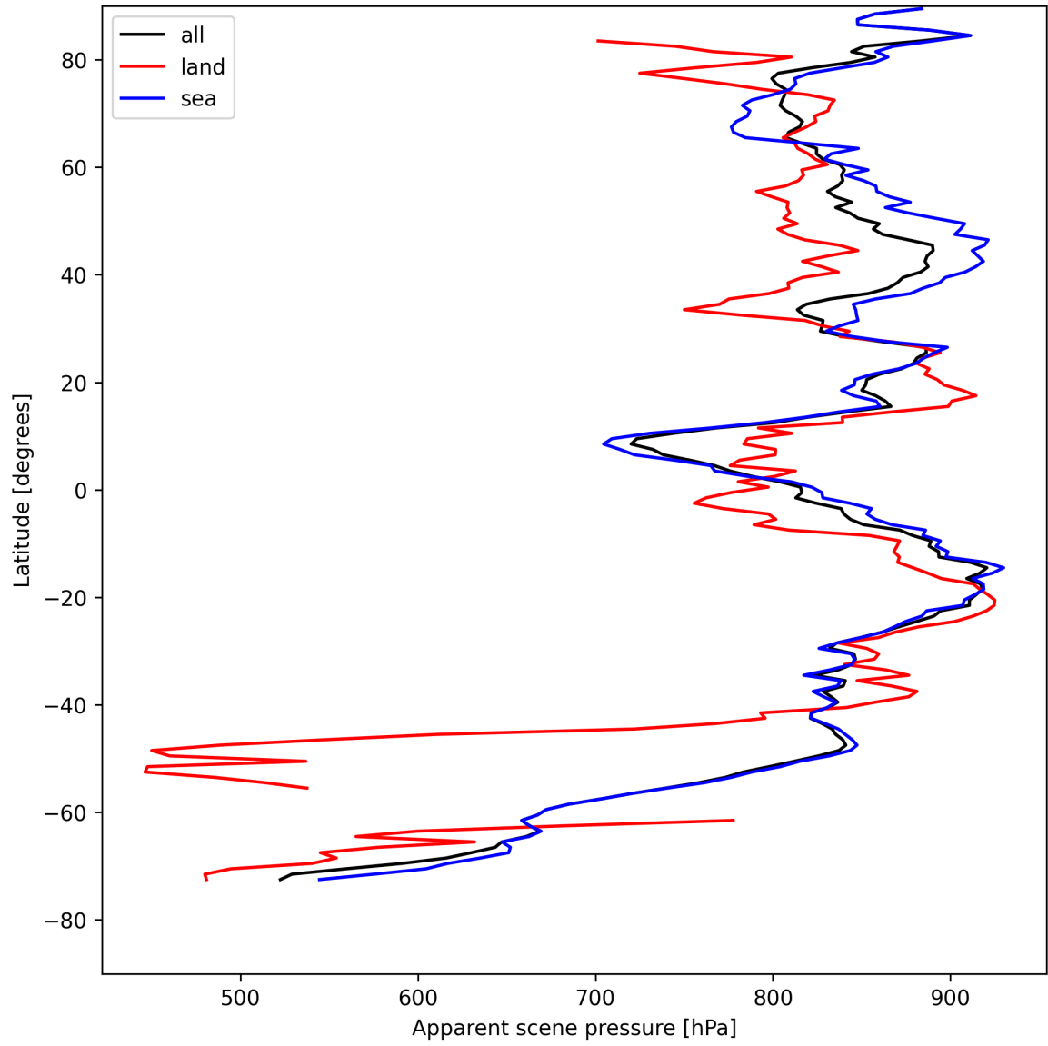
Figure 19: Zonal average of “Apparent scene pressure” for 2025-08-09 to 2025-08-10.
