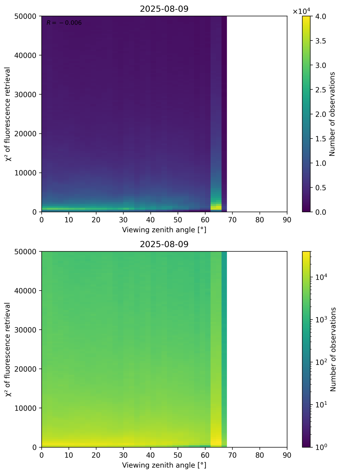
Figure 119: Scatter density plot of “Viewing zenith angle” against “ \chi^2 of fluorescence retrieval” for 2025-08-09 to 2025-08-10.
