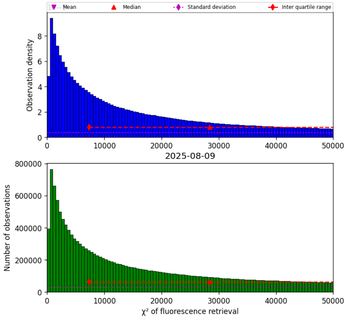
Figure 42: Histogram of “ \chi^2 of fluorescence retrieval” for 2025-08-09 to 2025-08-10
