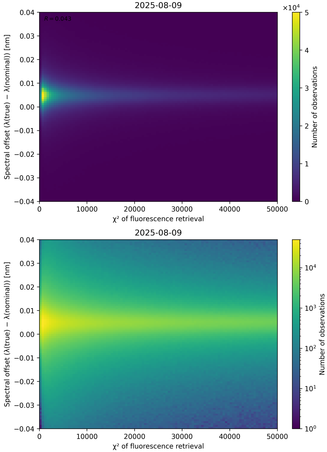
Figure 69: Scatter density plot of “ \chi^2 of fluorescence retrieval” against “Spectral offset ( \lambda_{\text{true}} - \lambda_{\text{nominal}} )” for 2025-08-09 to 2025-08-10.
