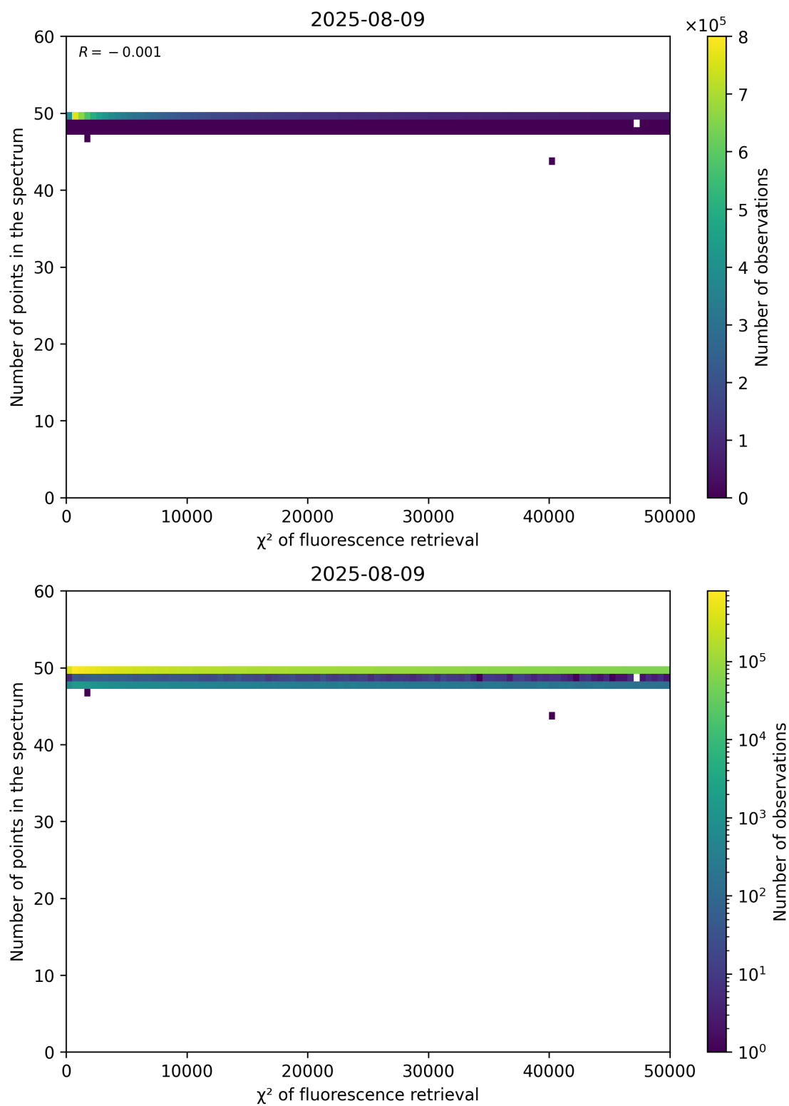
Figure 68: Scatter density plot of “ \chi^2 of fluorescence retrieval” against “Number of points in the spectrum” for 2025-08-09 to 2025-08-10.
