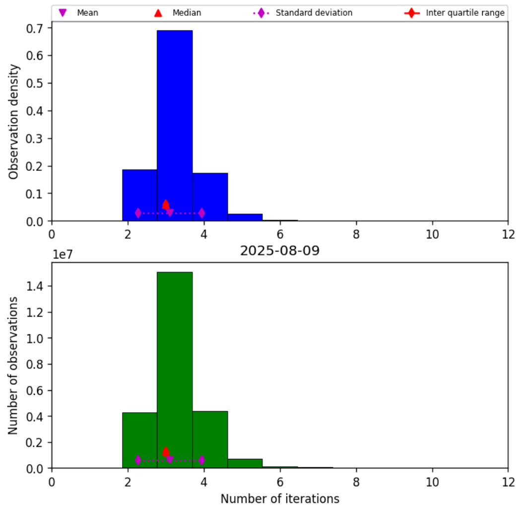
Figure 39: Histogram of “Number of iterations” for 2025-08-09 to 2025-08-10
