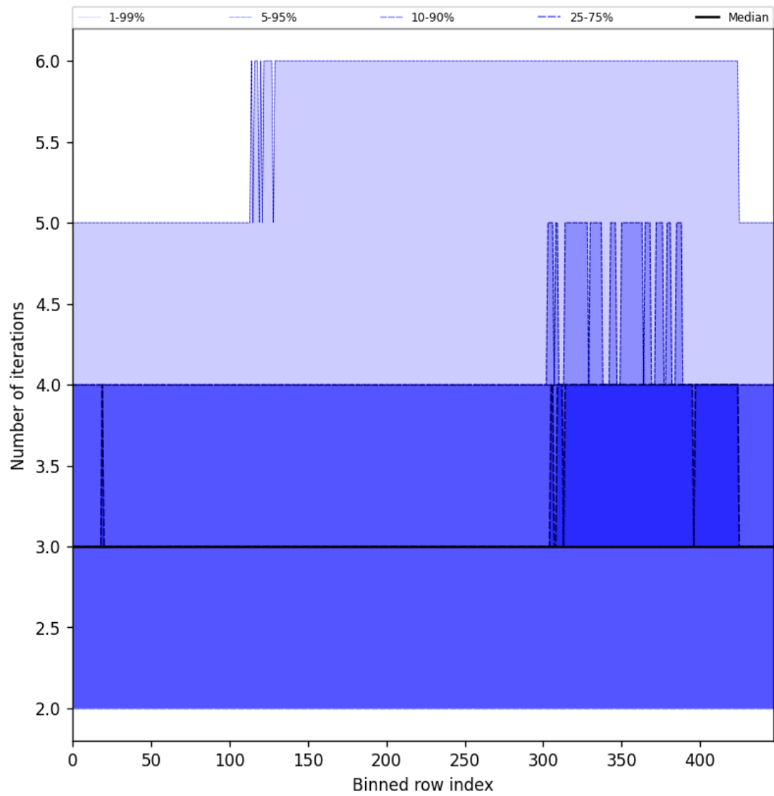
Figure 56: Along track statistics of “Number of iterations” for 2025-08-09 to 2025-08-10
