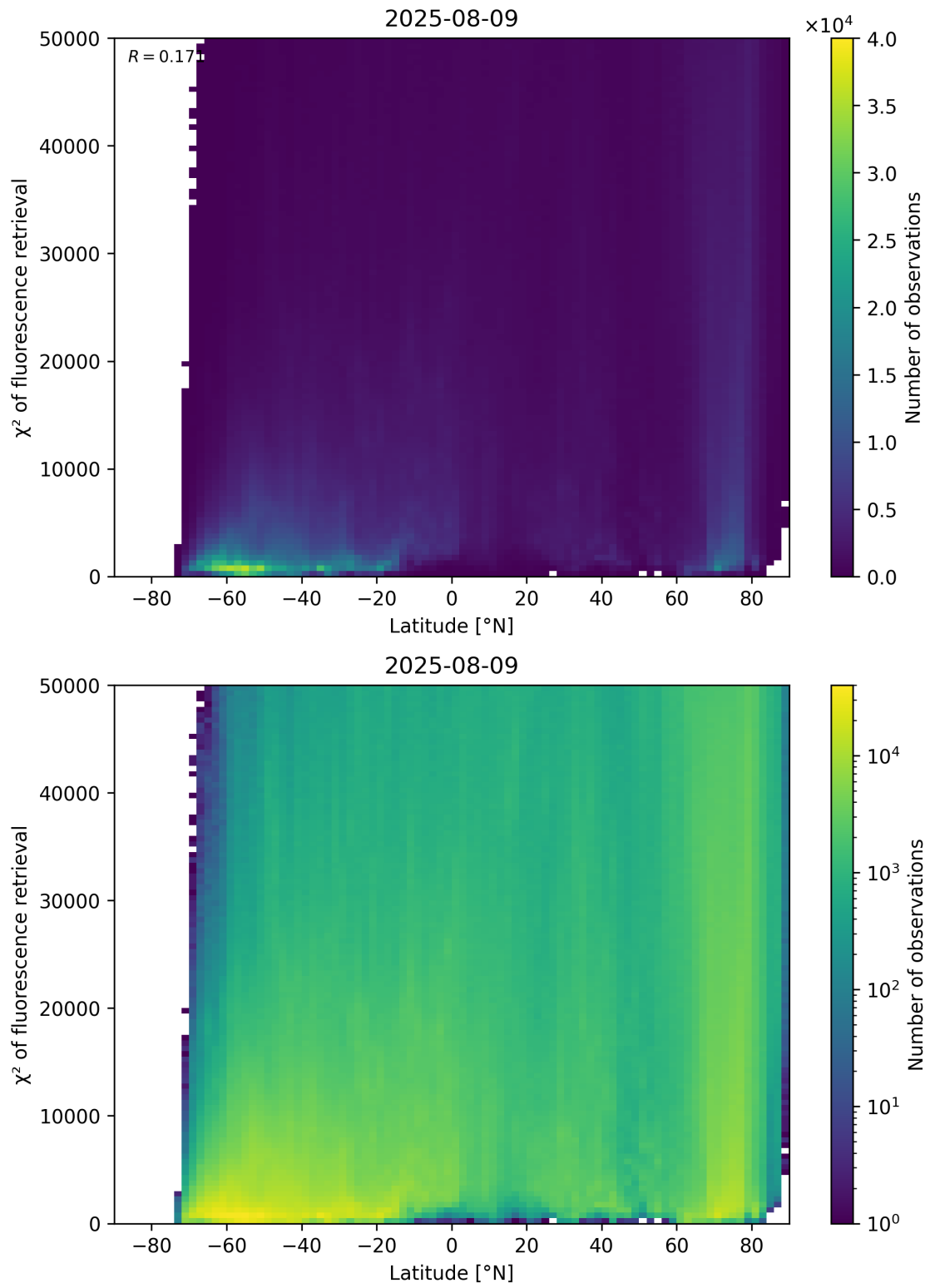
Figure 89: Scatter density plot of “Latitude” against “ \chi^2 of fluorescence retrieval” for 2025-08-09 to 2025-08-10.
