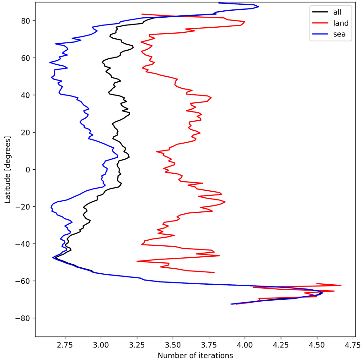
Figure 22: Zonal average of “Number of iterations” for 2025-08-09 to 2025-08-10.
