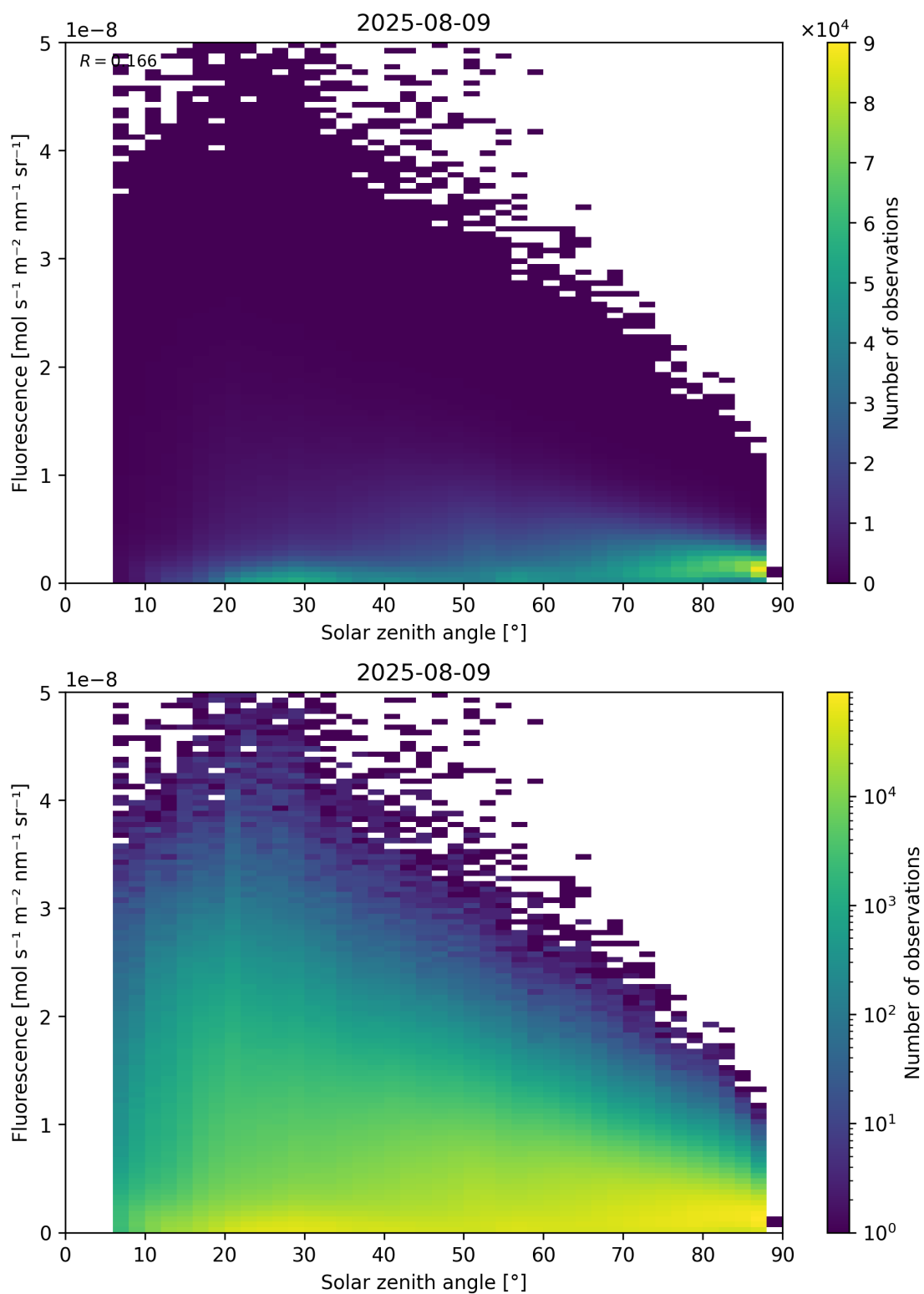
Figure 112: Scatter density plot of “Solar zenith angle” against “Fluorescence” for 2025-08-09 to 2025-08-10.
