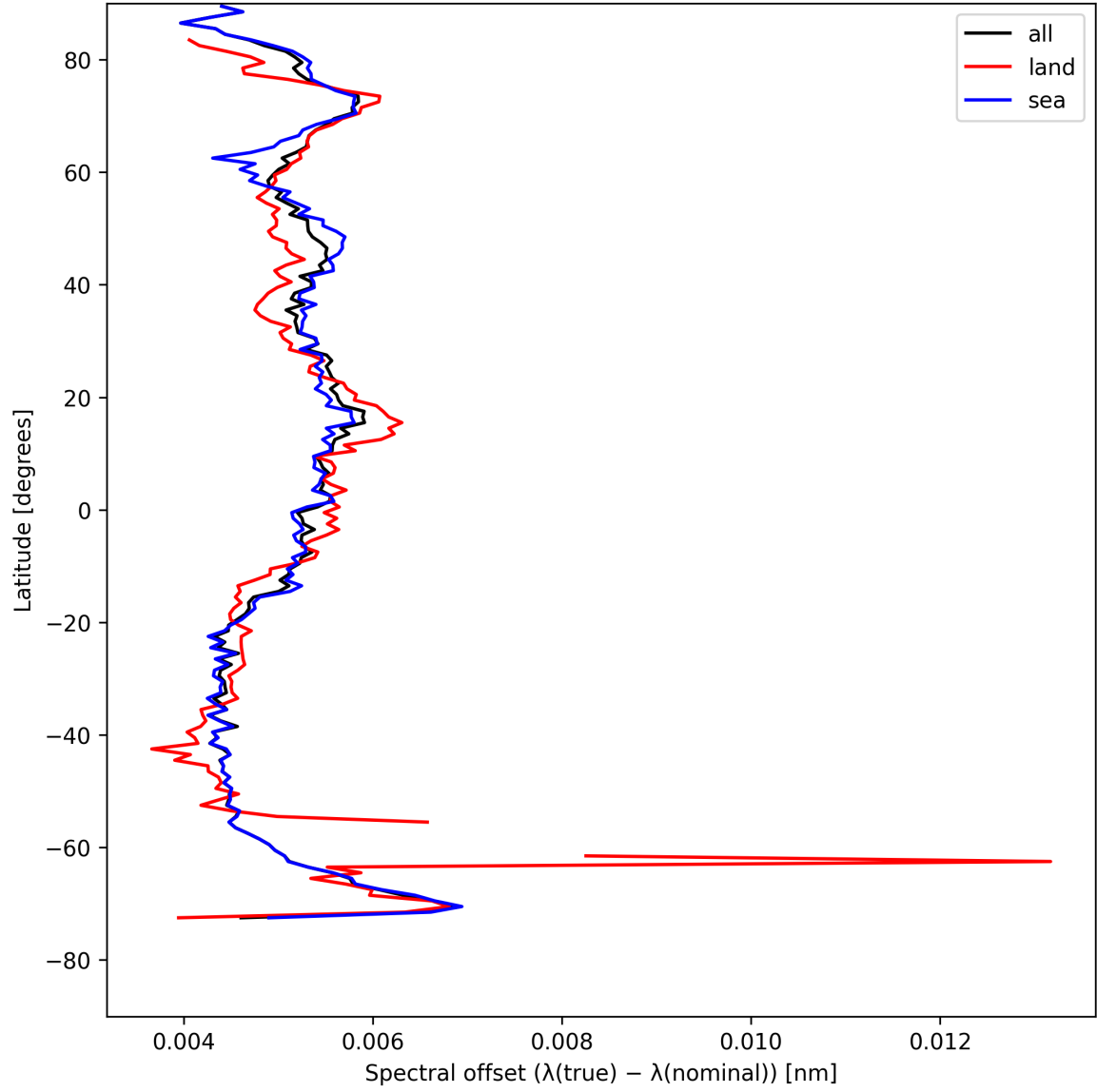
Figure 28: Zonal average of “Spectral offset ( \lambda_{\text{true}} - \lambda_{\text{nominal}} )” for 2025-08-09 to 2025-08-10.
