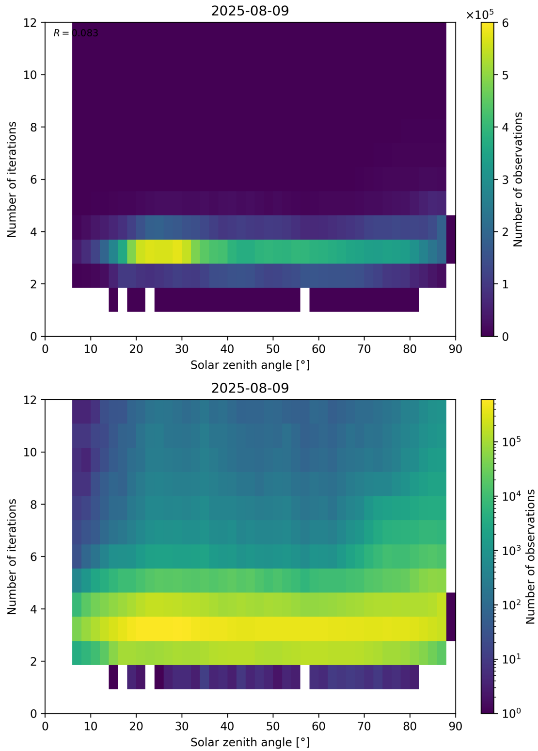
Figure 114: Scatter density plot of “Solar zenith angle” against “Number of iterations” for 2025-08-09 to 2025-08-10.
