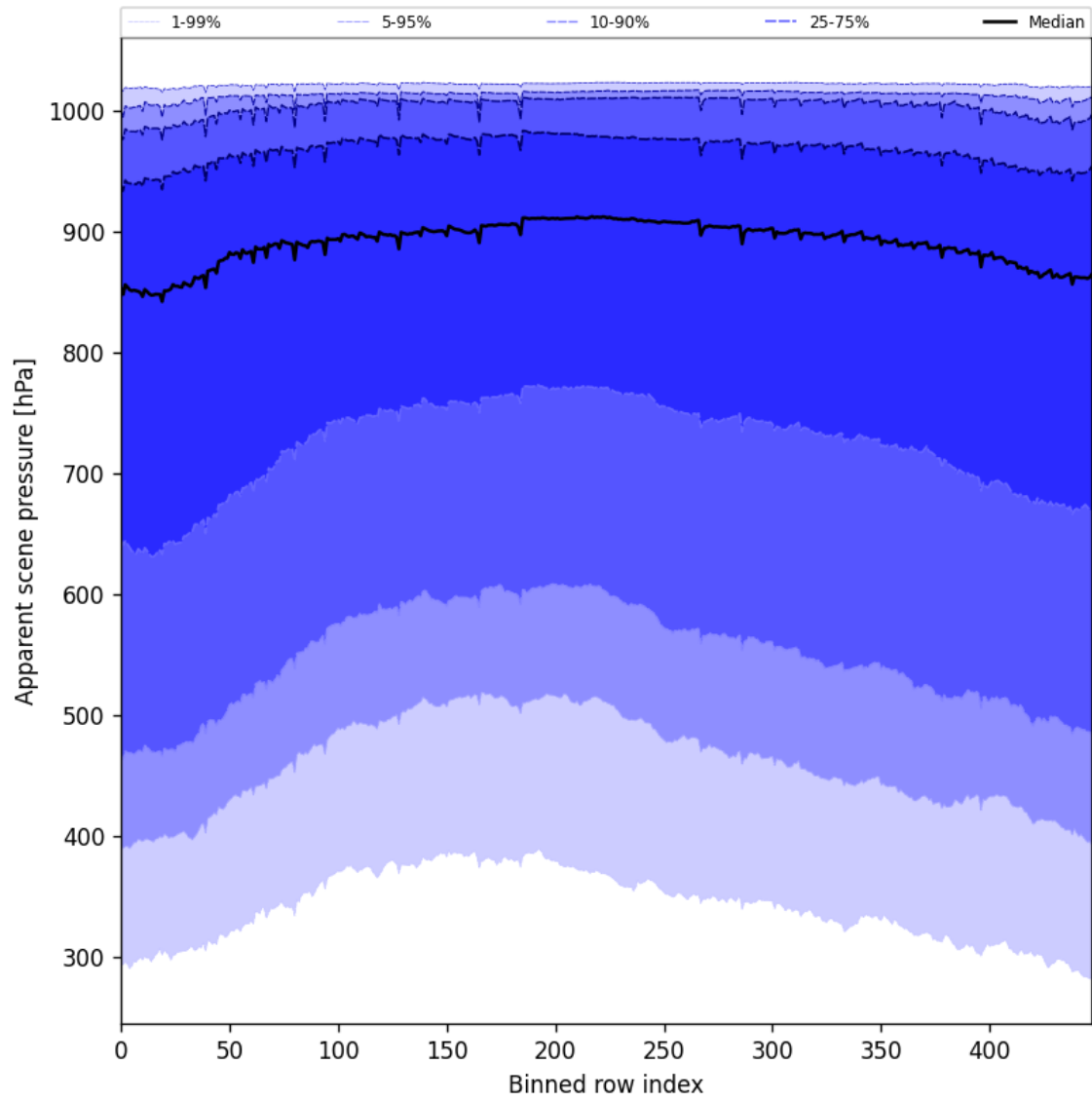
Figure 53: Along track statistics of “Apparent scene pressure” for 2025-08-09 to 2025-08-10
