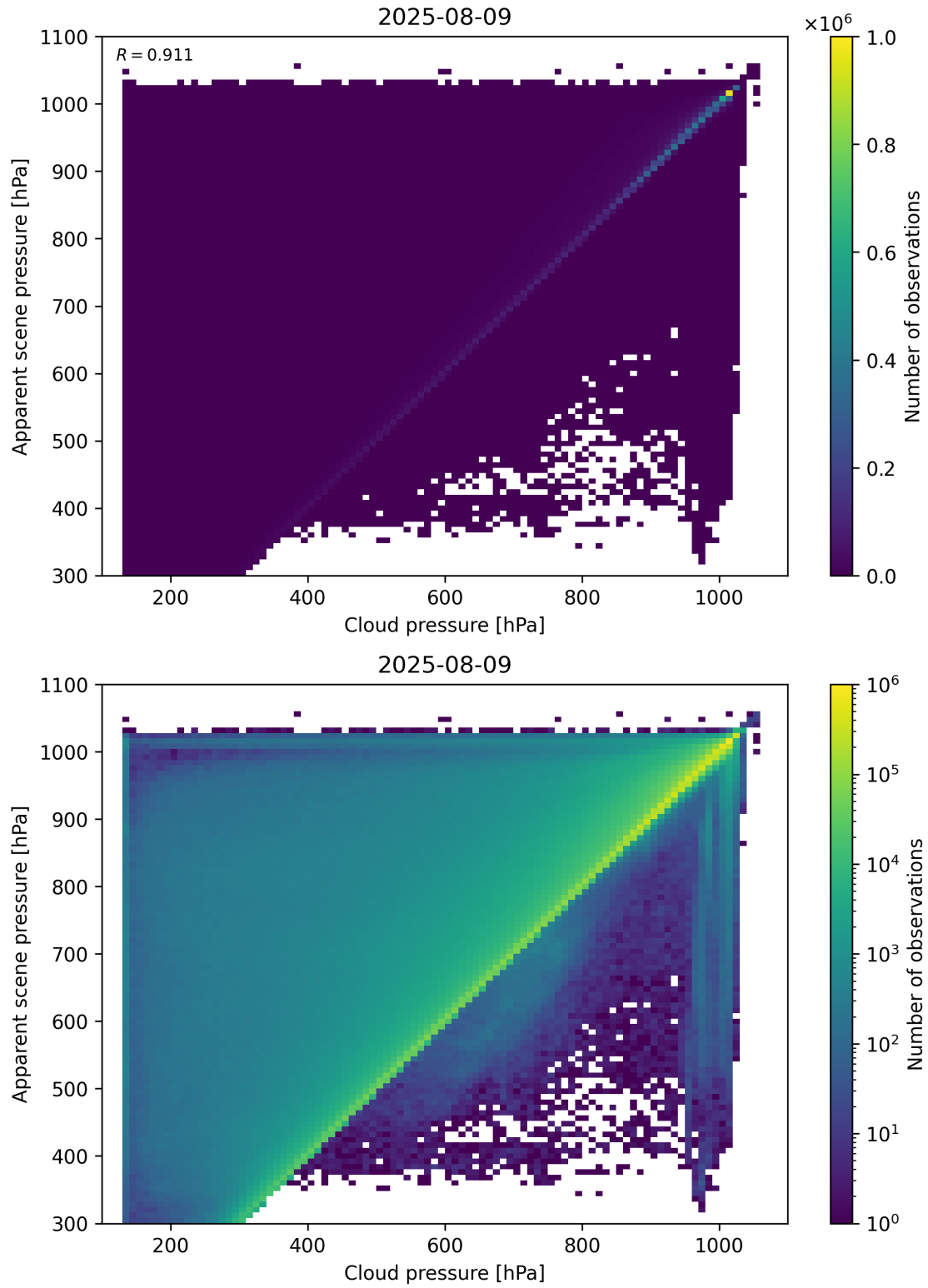
Figure 77: Scatter density plot of “Cloud pressure” against “Apparent scene pressure” for 2025-08-09 to 2025-08-10.
