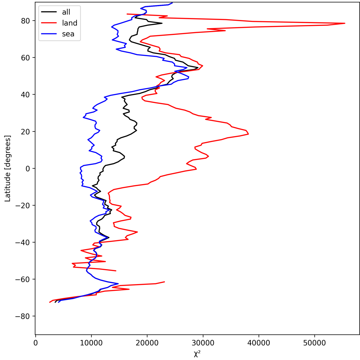
Figure 21: Zonal average of “ \chi^2 ” for 2025-08-09 to 2025-08-10.
