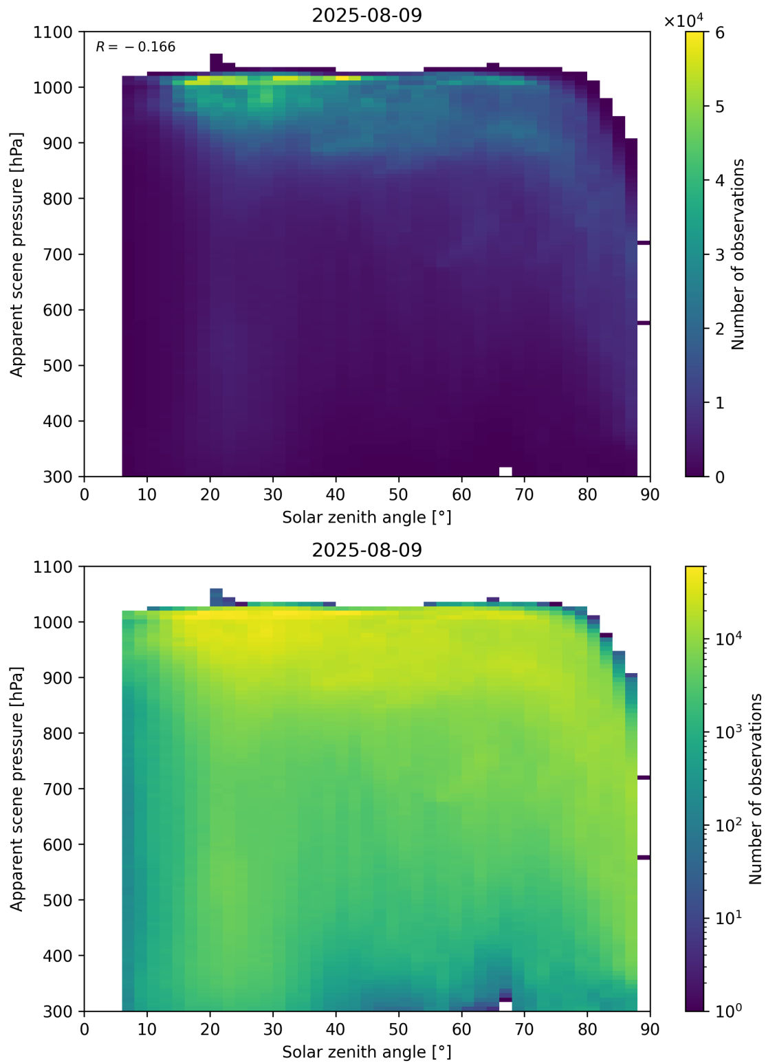
Figure 108: Scatter density plot of “Solar zenith angle” against “Apparent scene pressure” for 2025-08-09 to 2025-08-10.
