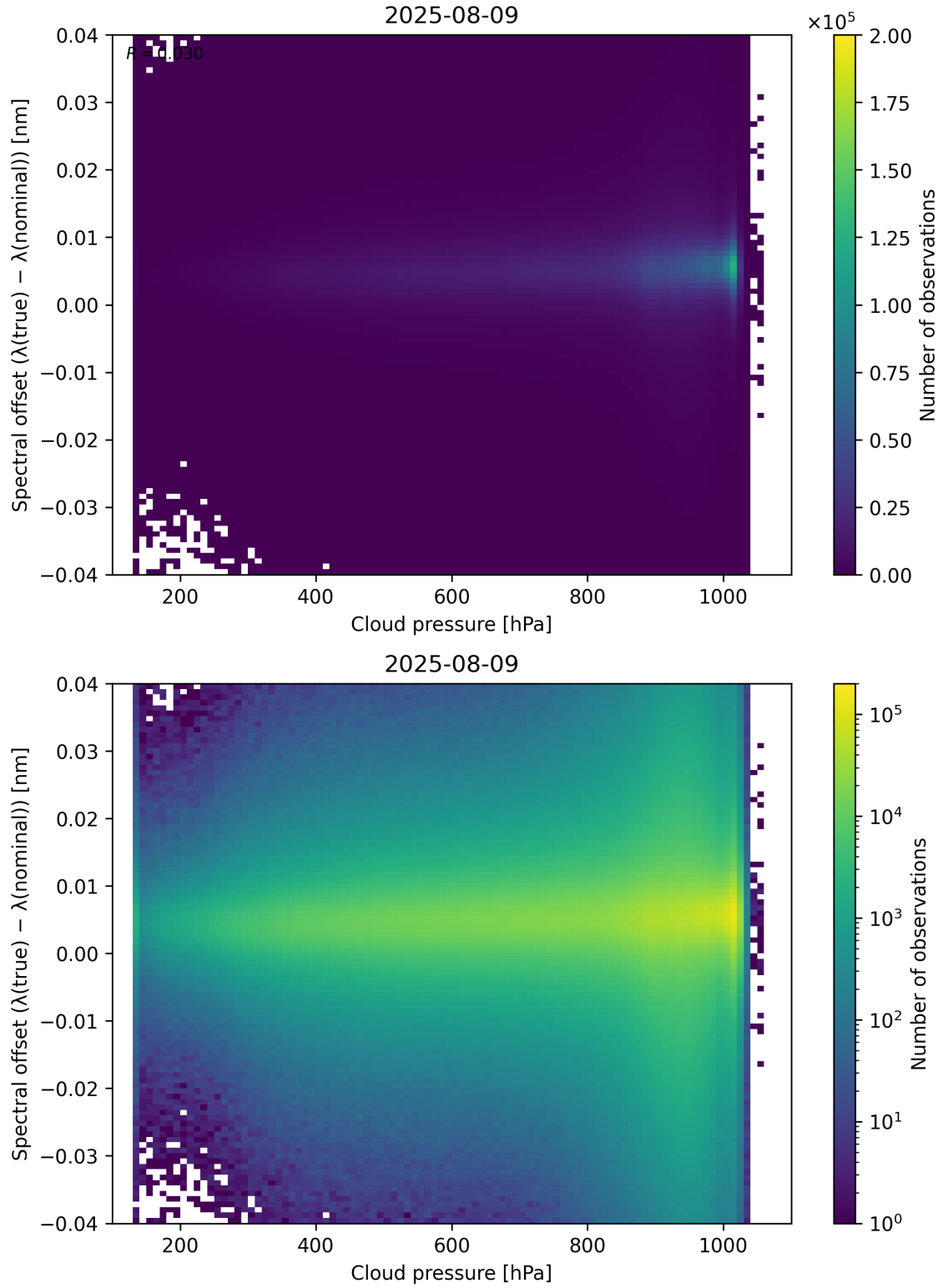
Figure 84: Scatter density plot of “Cloud pressure” against “Spectral offset ( \lambda_{\text{true}} - \lambda_{\text{nominal}} )” for 2025-08-09 to 2025-08-10.
