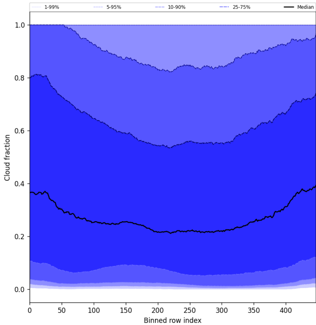
Figure 49: Along track statistics of “Cloud fraction” for 2025-08-09 to 2025-08-10
