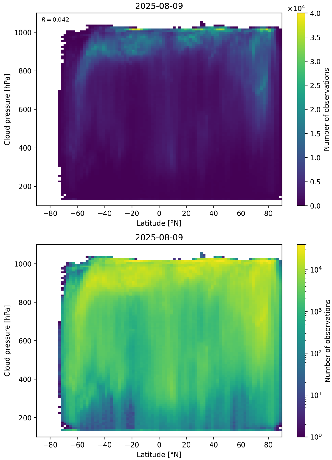
Figure 91: Scatter density plot of “Latitude” against “Cloud pressure” for 2025-08-09 to 2025-08-10.
