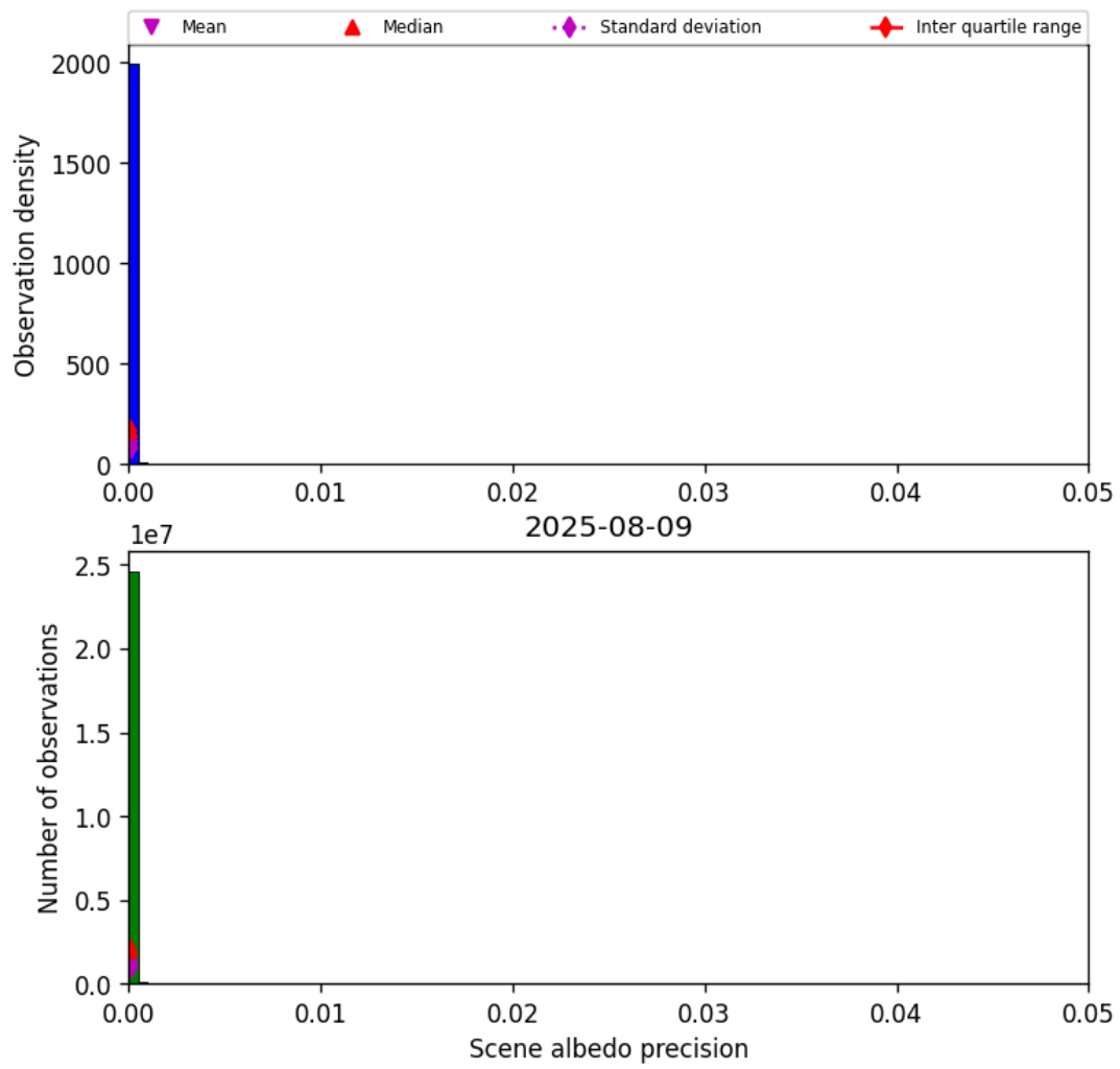
Figure 35: Histogram of “Scene albedo precision” for 2025-08-09 to 2025-08-10
