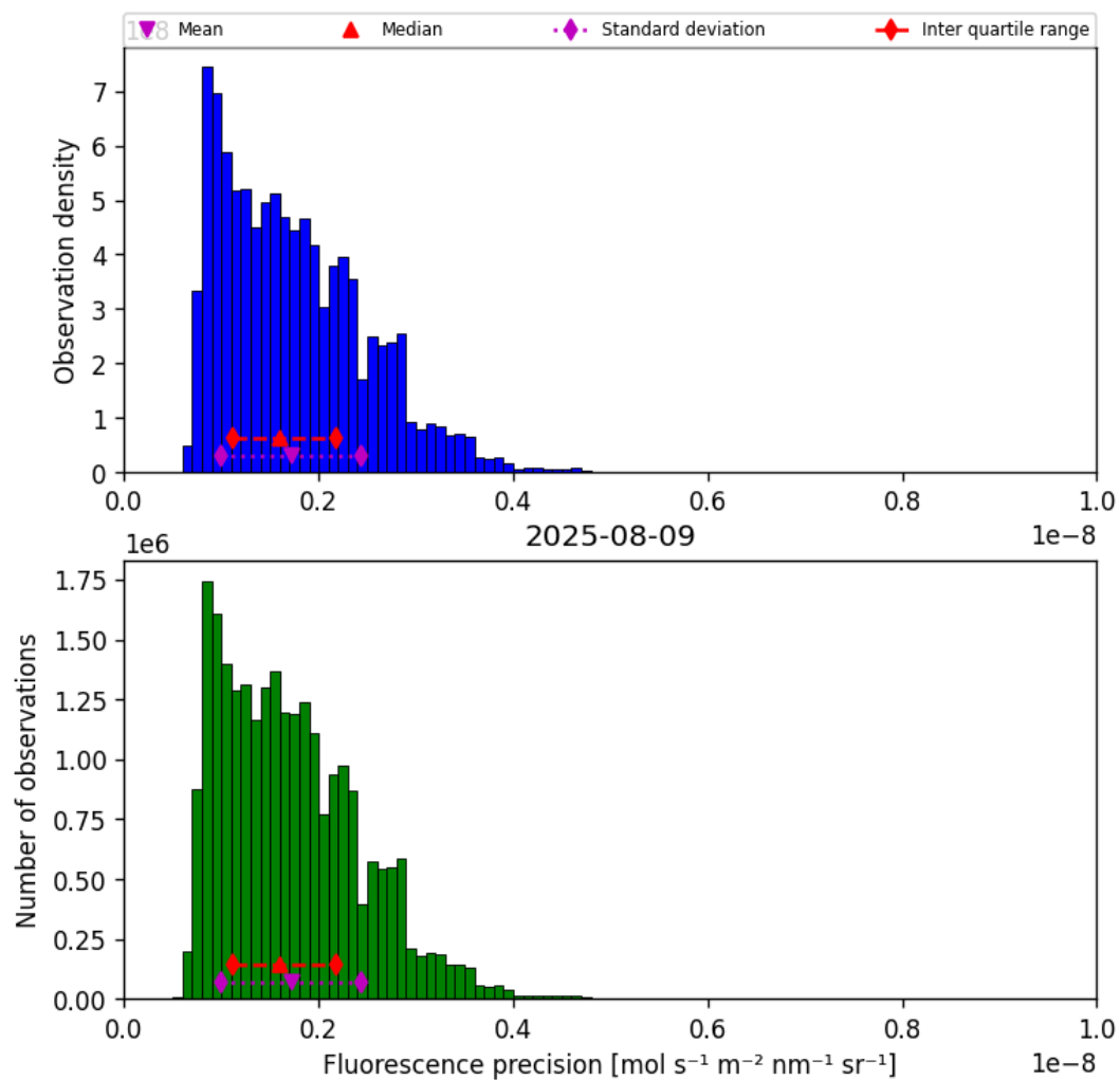
Figure 41: Histogram of “Fluorescence precision” for 2025-08-09 to 2025-08-10
