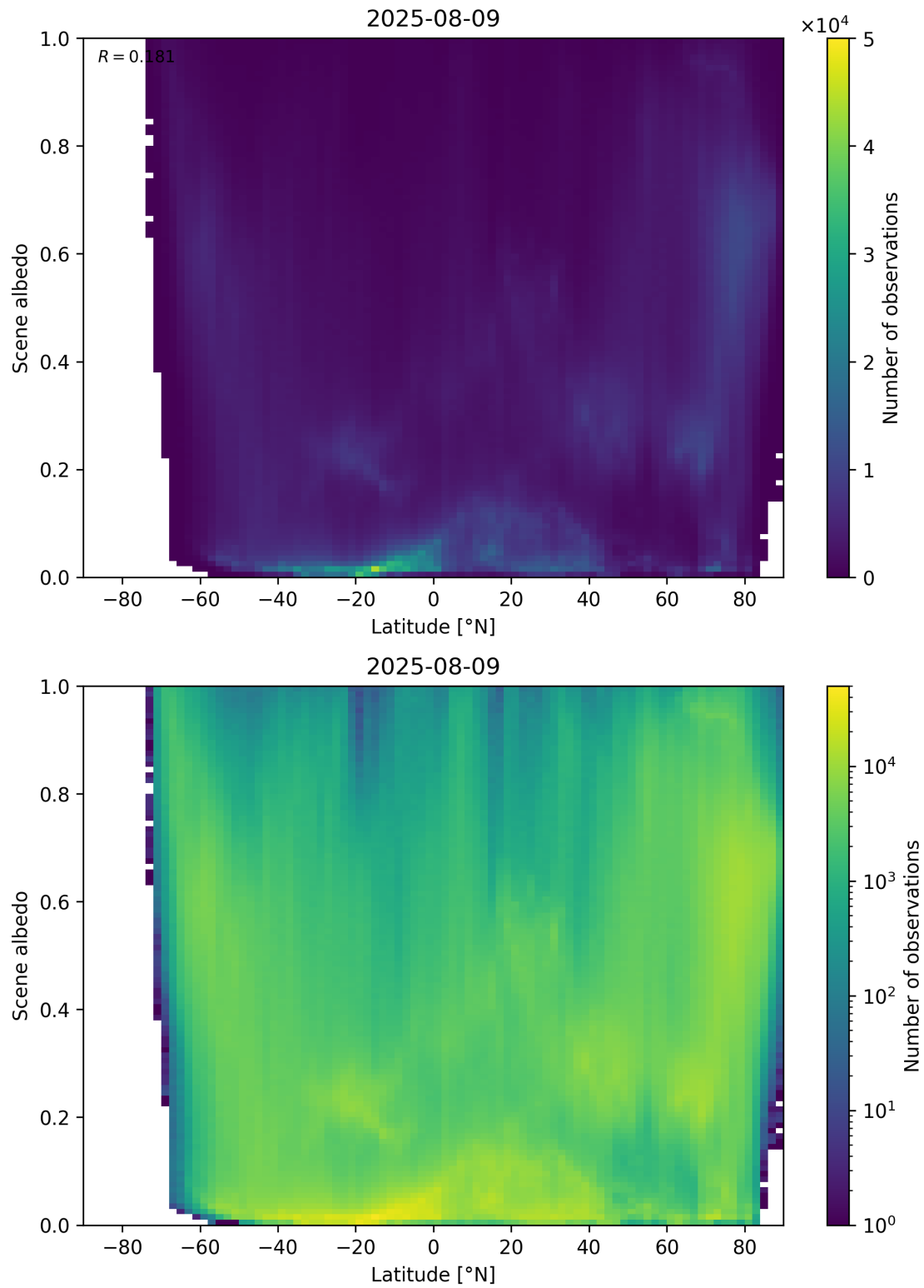
Figure 95: Scatter density plot of “Latitude” against “Scene albedo” for 2025-08-09 to 2025-08-10.
