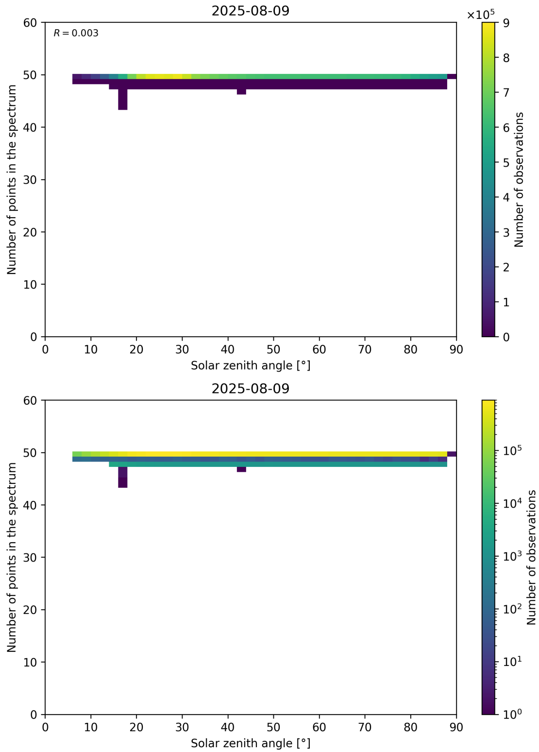
Figure 115: Scatter density plot of “Solar zenith angle” against “Number of points in the spectrum” for 2025-08-09 to 2025-08-10.
