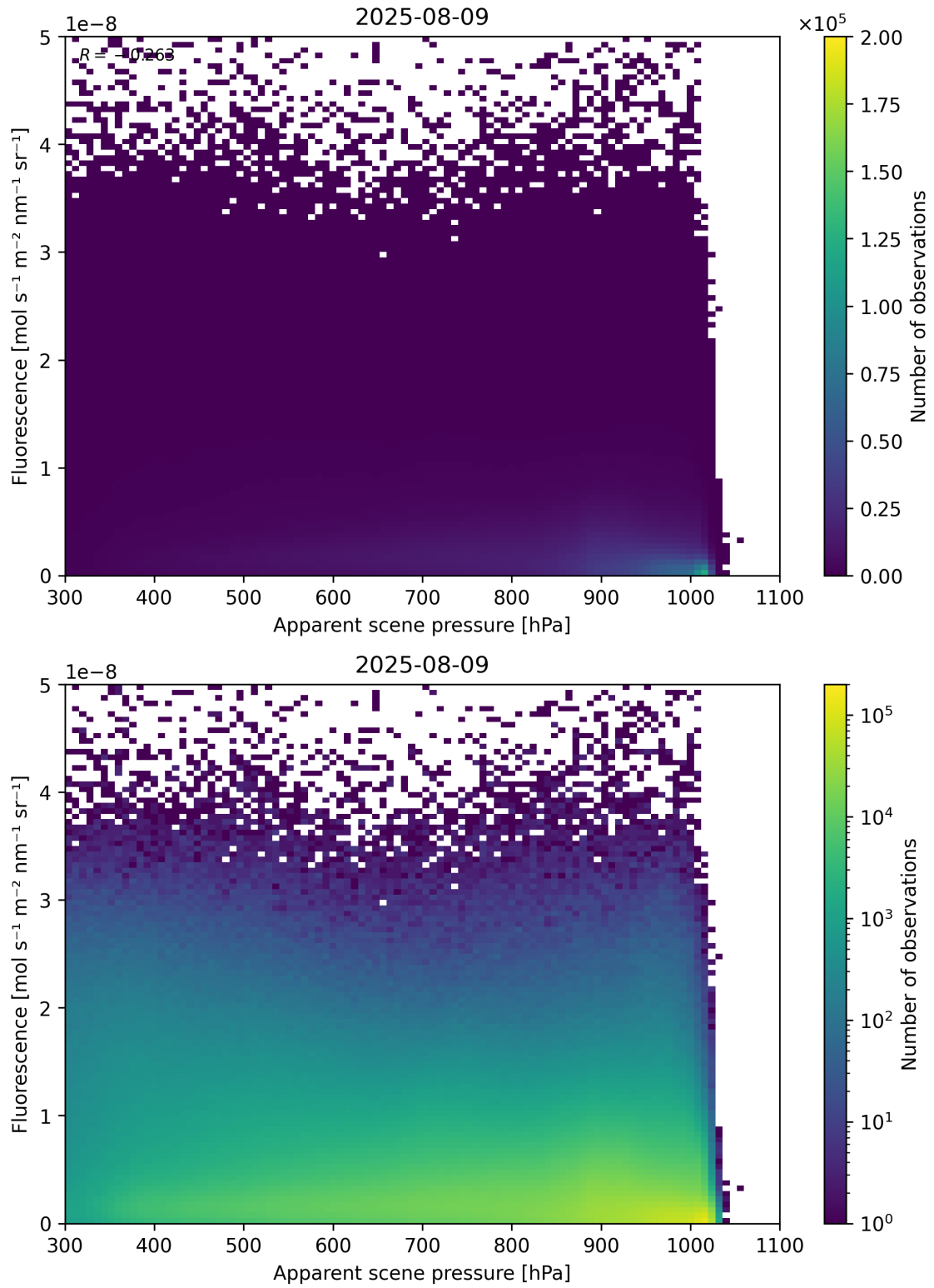
Figure 64: Scatter density plot of “Apparent scene pressure” against “Fluorescence” for 2025-08-09 to 2025-08-10.
