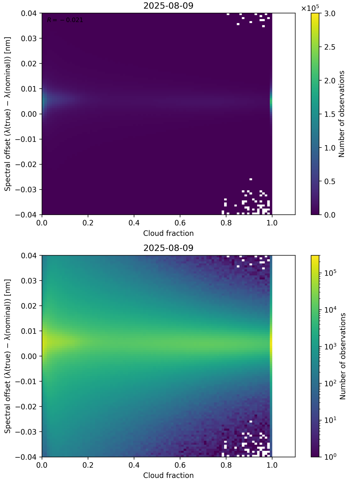
Figure 76: Scatter density plot of “Cloud fraction” against “Spectral offset ( \lambda_{\text{true}} - \lambda_{\text{nominal}} )” for 2025-08-09 to 2025-08-10.
