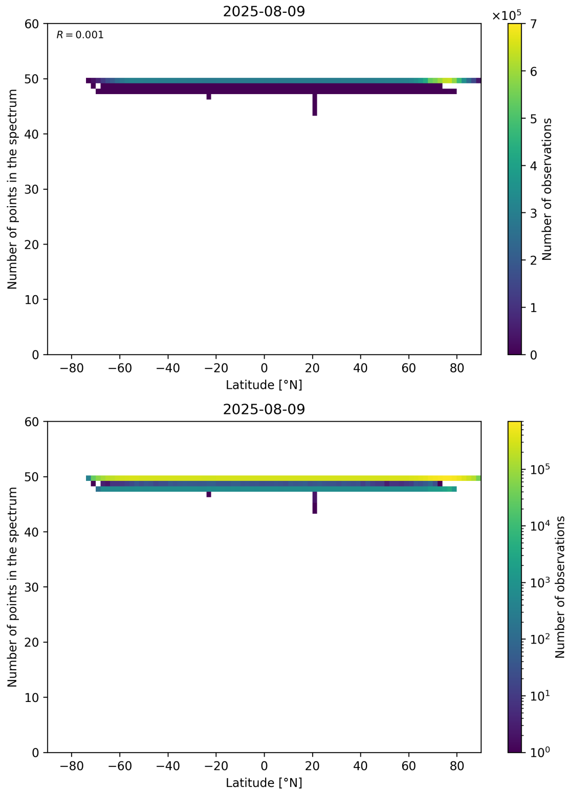
Figure 94: Scatter density plot of “Latitude” against “Number of points in the spectrum” for 2025-08-09 to 2025-08-10.
