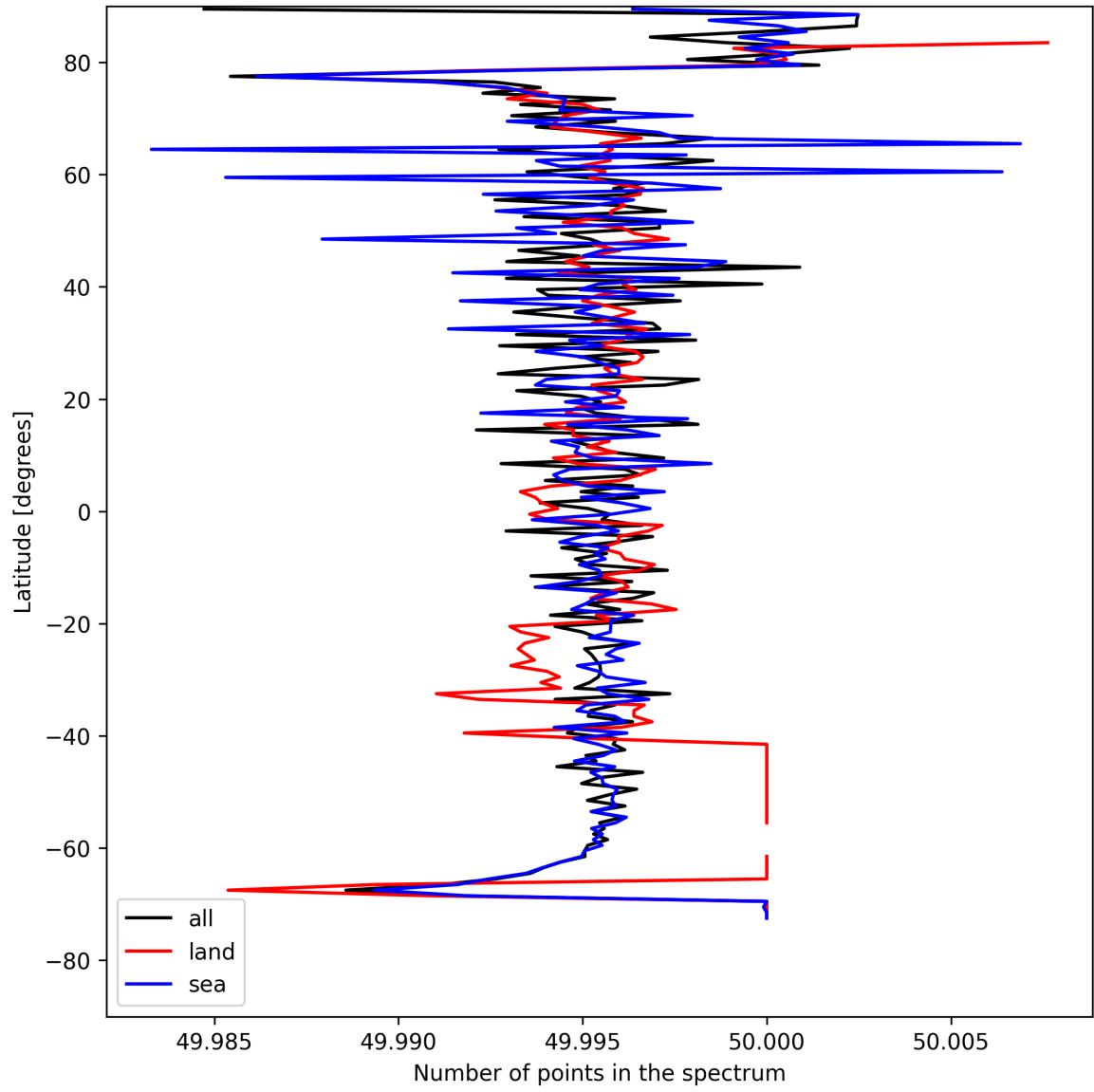
Figure 27: Zonal average of “Number of points in the spectrum” for 2025-08-09 to 2025-08-10.
