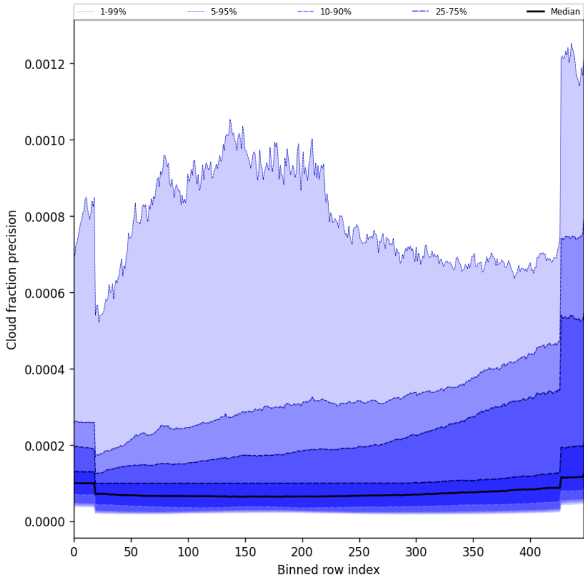
Figure 50: Along track statistics of “Cloud fraction precision” for 2025-08-09 to 2025-08-10
