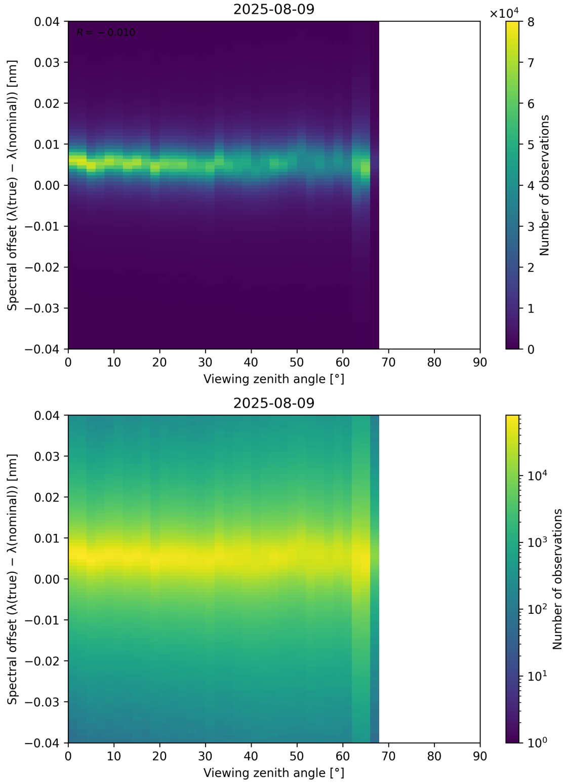
Figure 128: Scatter density plot of “Viewing zenith angle” against “Spectral offset ( \lambda_{\text{true}} - \lambda_{\text{nominal}} )” for 2025-08-09 to 2025-08-10.
