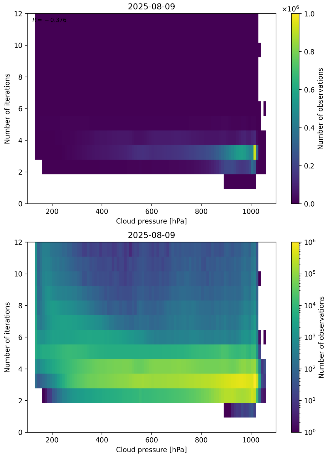
Figure 81: Scatter density plot of “Cloud pressure” against “Number of iterations” for 2025-08-09 to 2025-08-10.
