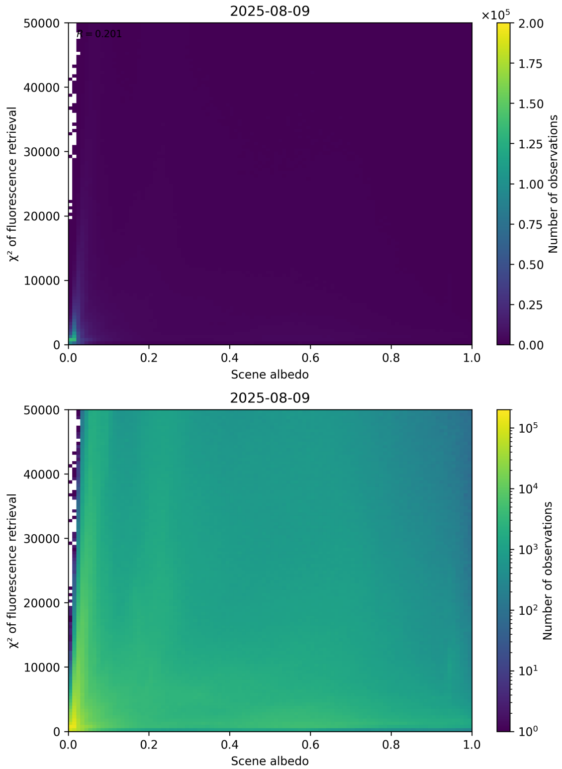
Figure 103: Scatter density plot of “Scene albedo” against “ \chi^2 of fluorescence retrieval” for 2025-08-09 to 2025-08-10.
