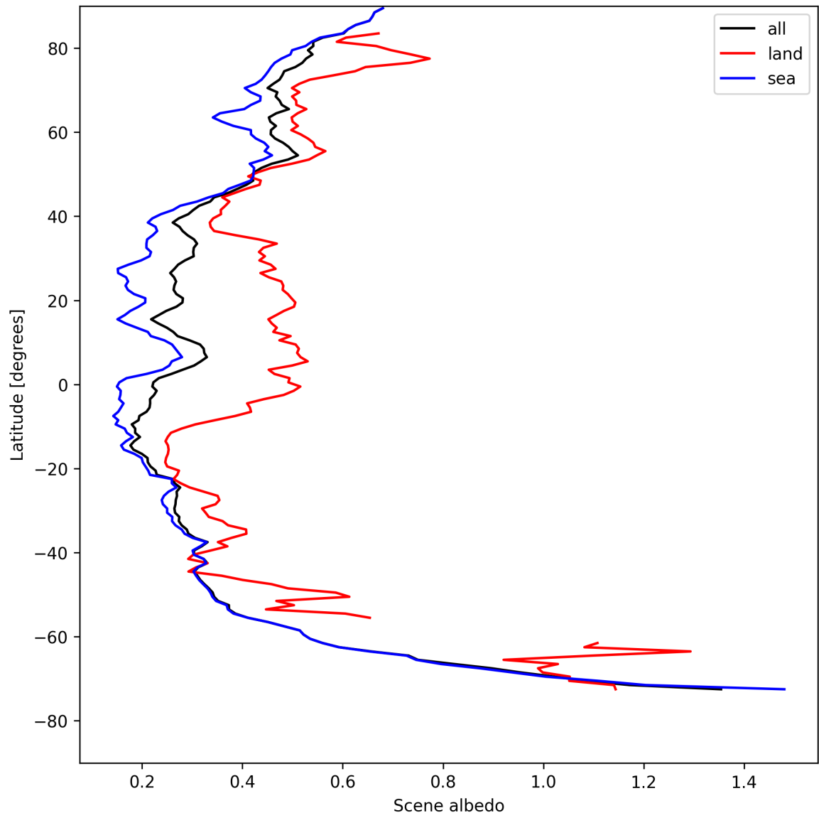
Figure 17: Zonal average of “Scene albedo” for 2025-08-09 to 2025-08-10.
