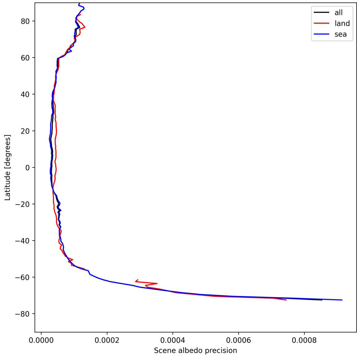
Figure 18: Zonal average of “Scene albedo precision” for 2025-08-09 to 2025-08-10.
