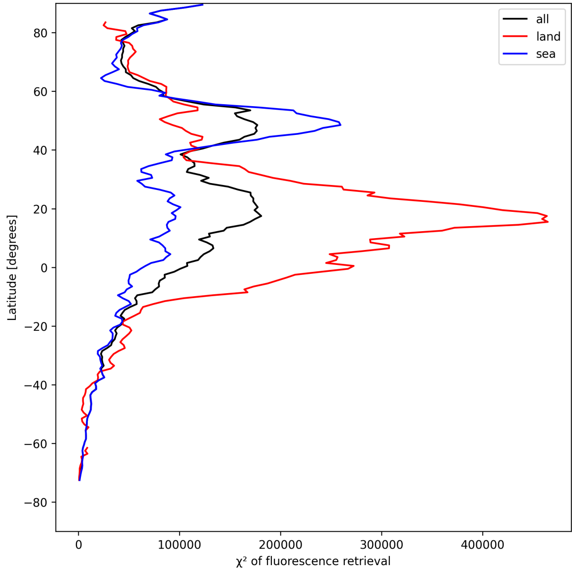
Figure 25: Zonal average of “ \chi^2 of fluorescence retrieval” for 2025-08-09 to 2025-08-10.
