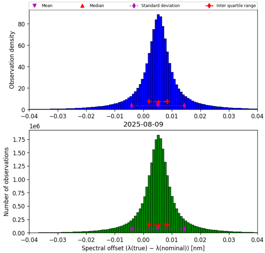
Figure 45: Histogram of “Spectral offset ( \lambda_{\text{true}} - \lambda_{\text{nominal}} )” for 2025-08-09 to 2025-08-10
