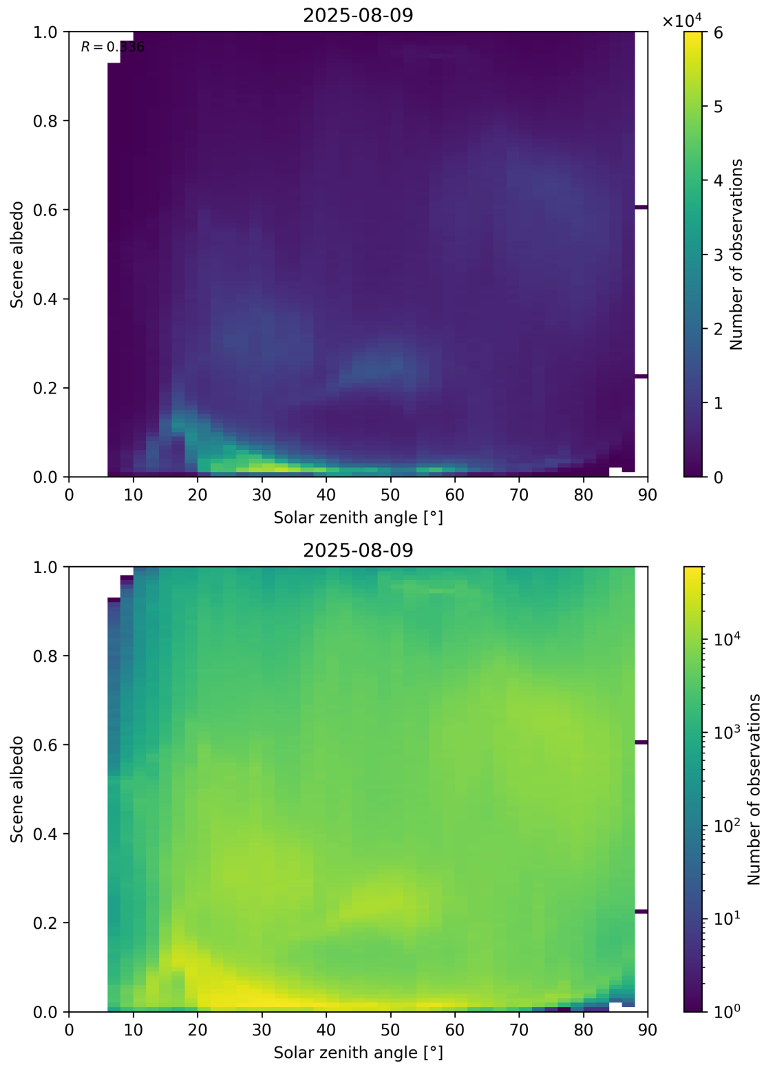
Figure 116: Scatter density plot of “Solar zenith angle” against “Scene albedo” for 2025-08-09 to 2025-08-10.
