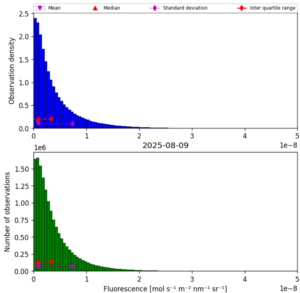
Figure 40: Histogram of “Fluorescence” for 2025-08-09 to 2025-08-10
