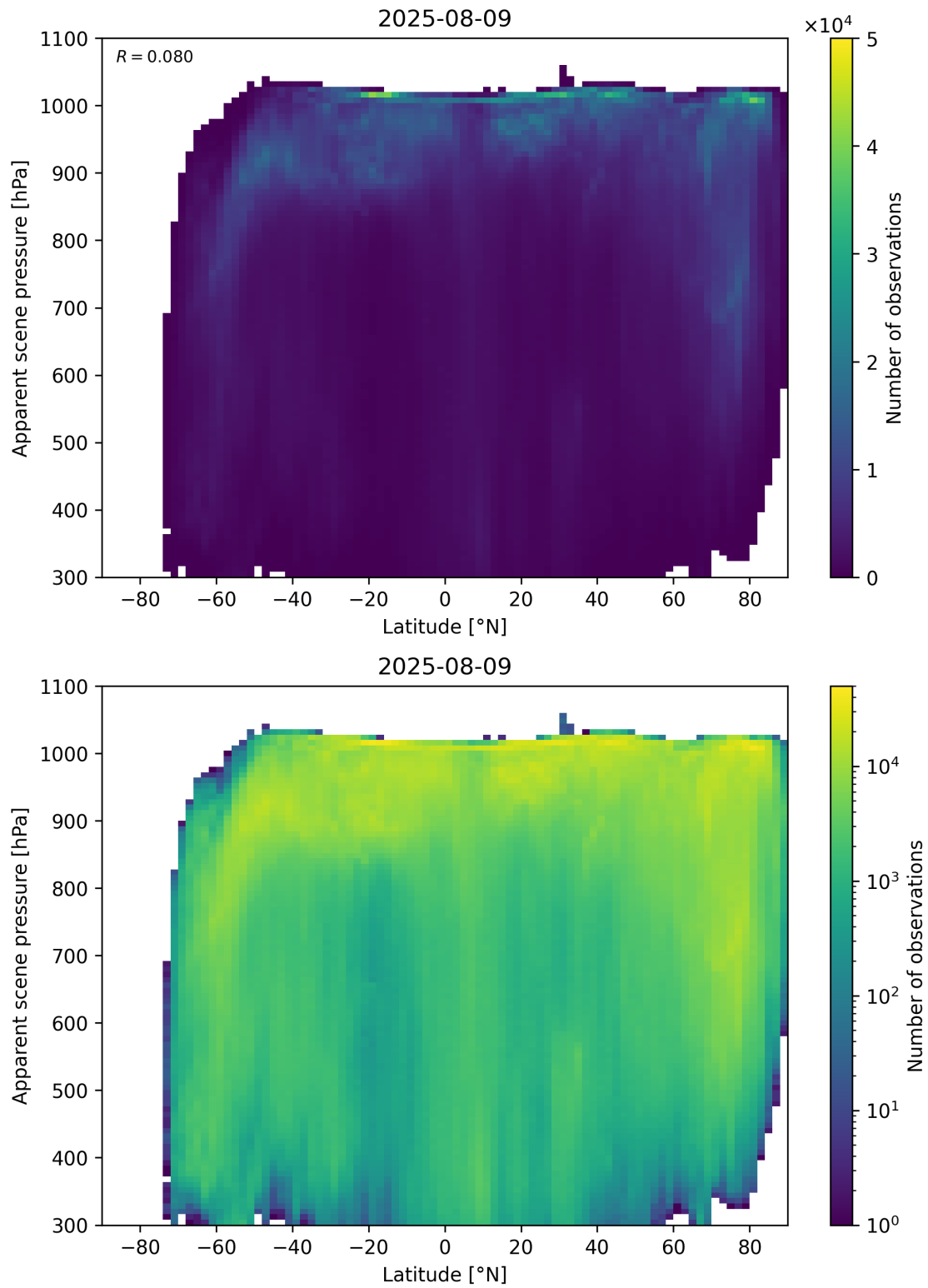
Figure 88: Scatter density plot of “Latitude” against “Apparent scene pressure” for 2025-08-09 to 2025-08-10.
