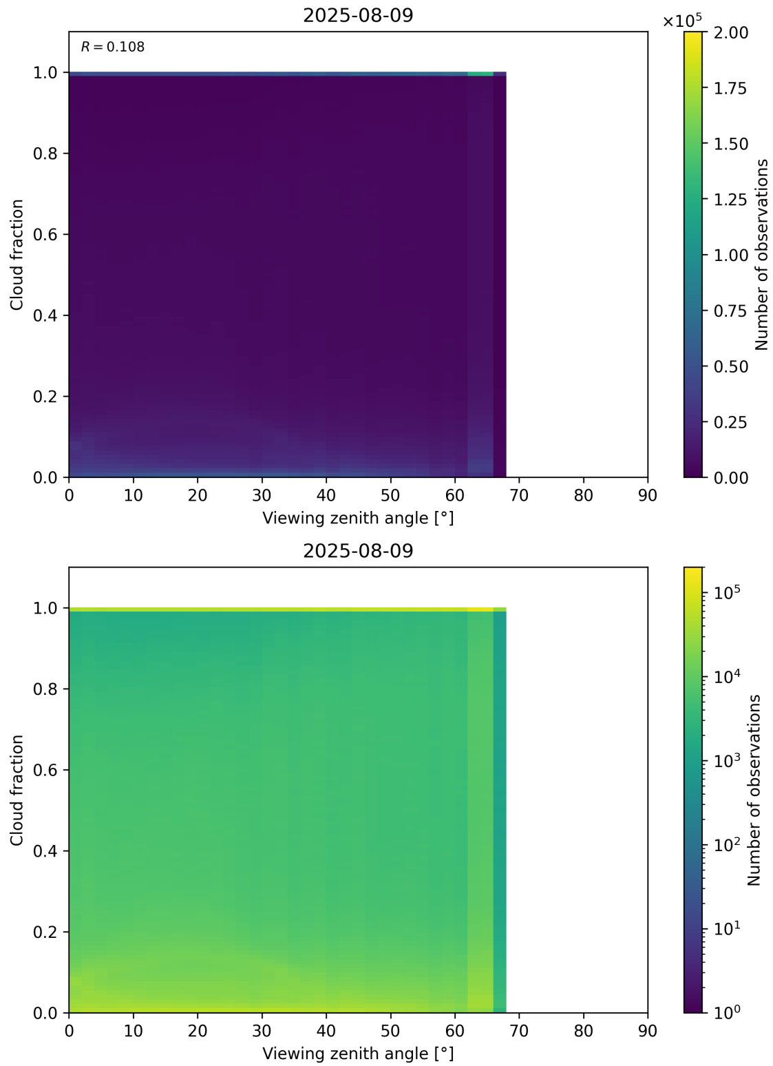
Figure 120: Scatter density plot of “Viewing zenith angle” against “Cloud fraction” for 2025-08-09 to 2025-08-10.
