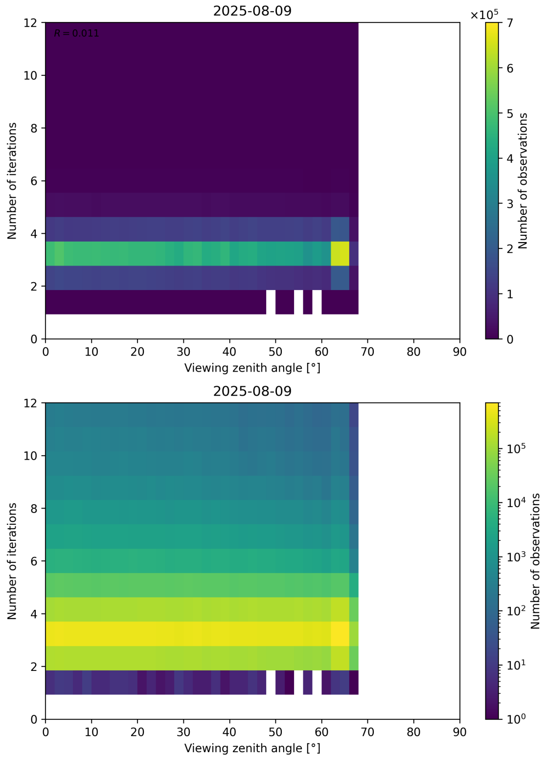
Figure 124: Scatter density plot of “Viewing zenith angle” against “Number of iterations” for 2025-08-09 to 2025-08-10.
