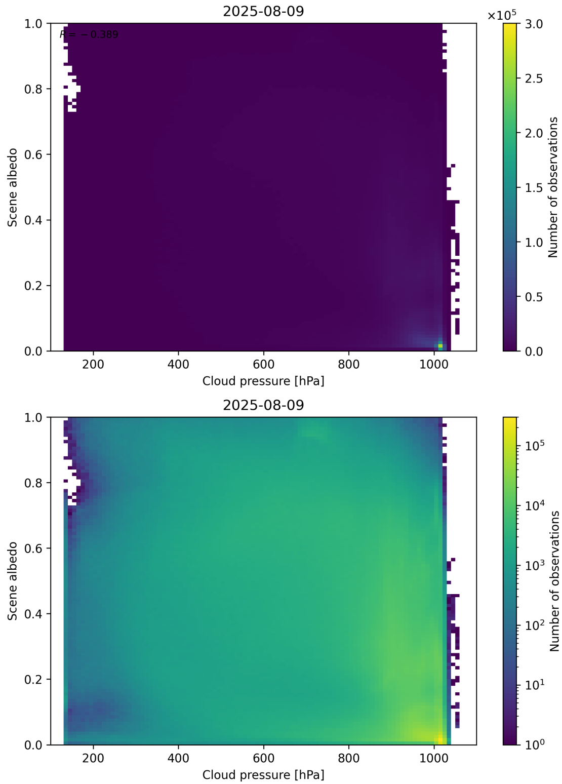
Figure 83: Scatter density plot of “Cloud pressure” against “Scene albedo” for 2025-08-09 to 2025-08-10.
