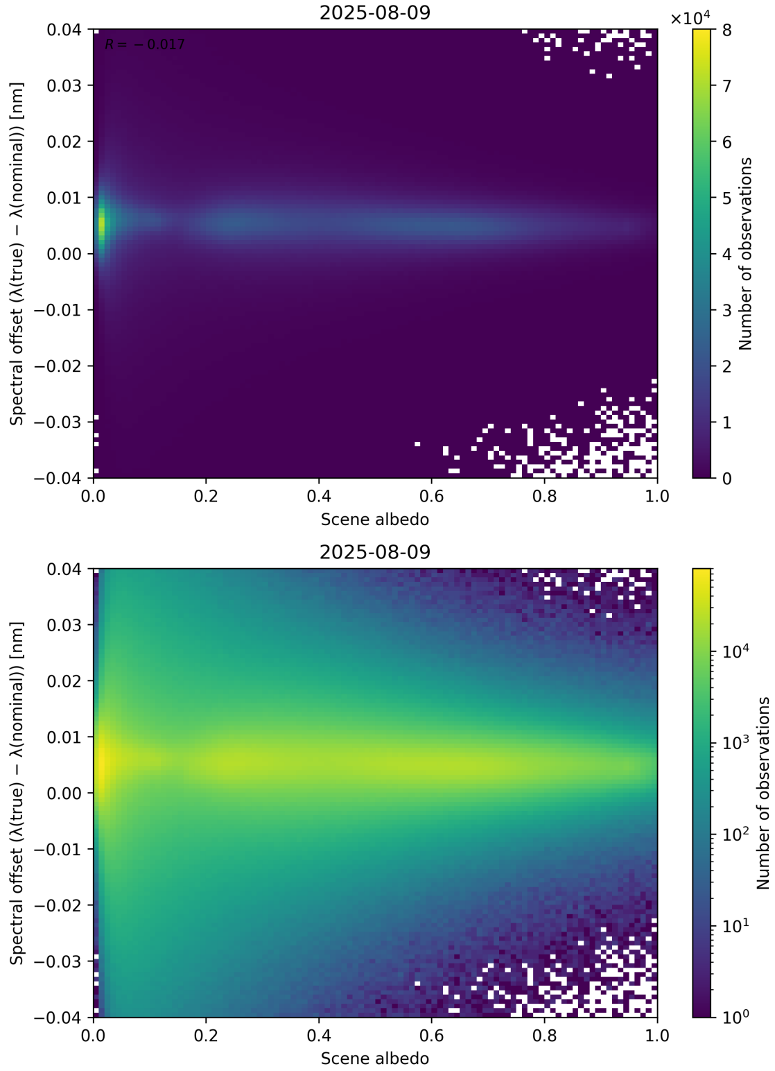
Figure 107: Scatter density plot of “Scene albedo” against “Spectral offset ( \lambda_{\text{true}} - \lambda_{\text{nominal}} )” for 2025-08-09 to 2025-08-10.
