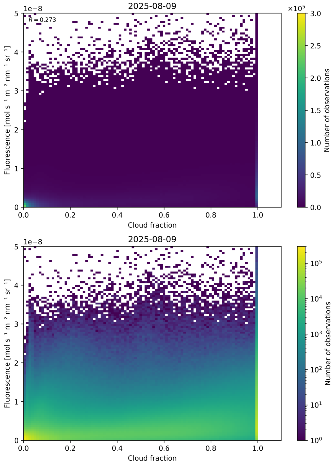
Figure 72: Scatter density plot of “Cloud fraction” against “Fluorescence” for 2025-08-09 to 2025-08-10.
