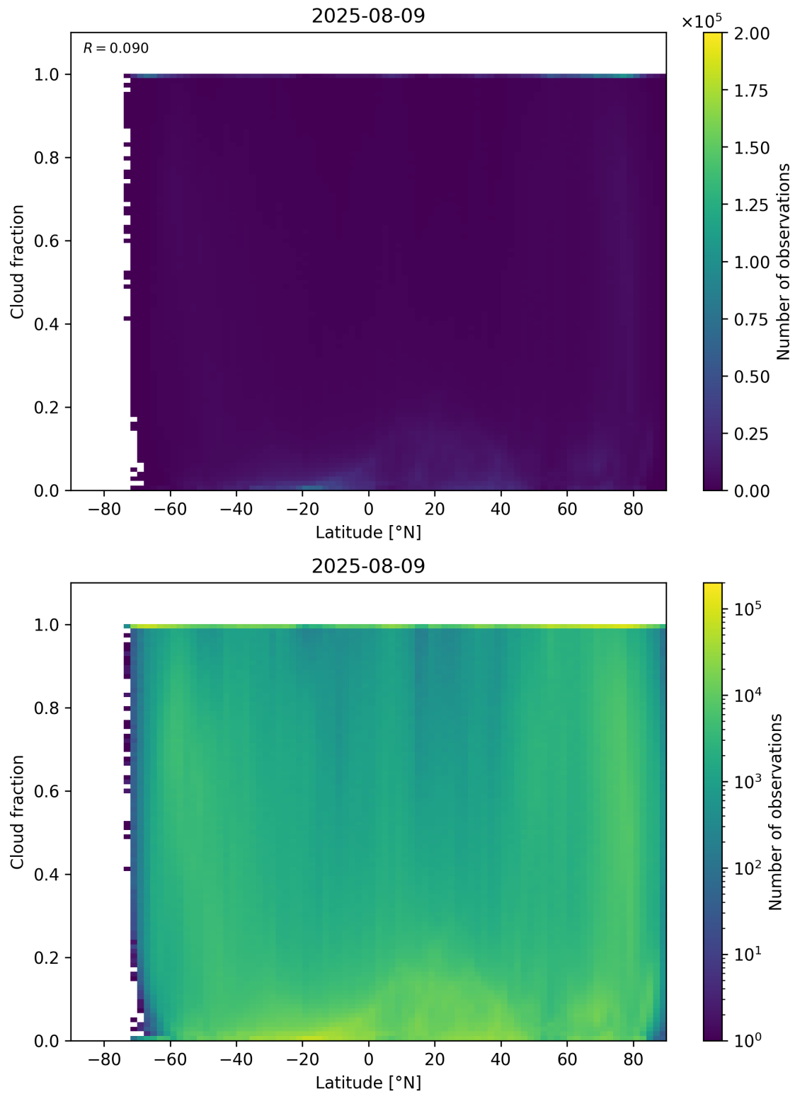
Figure 90: Scatter density plot of “Latitude” against “Cloud fraction” for 2025-08-09 to 2025-08-10.
