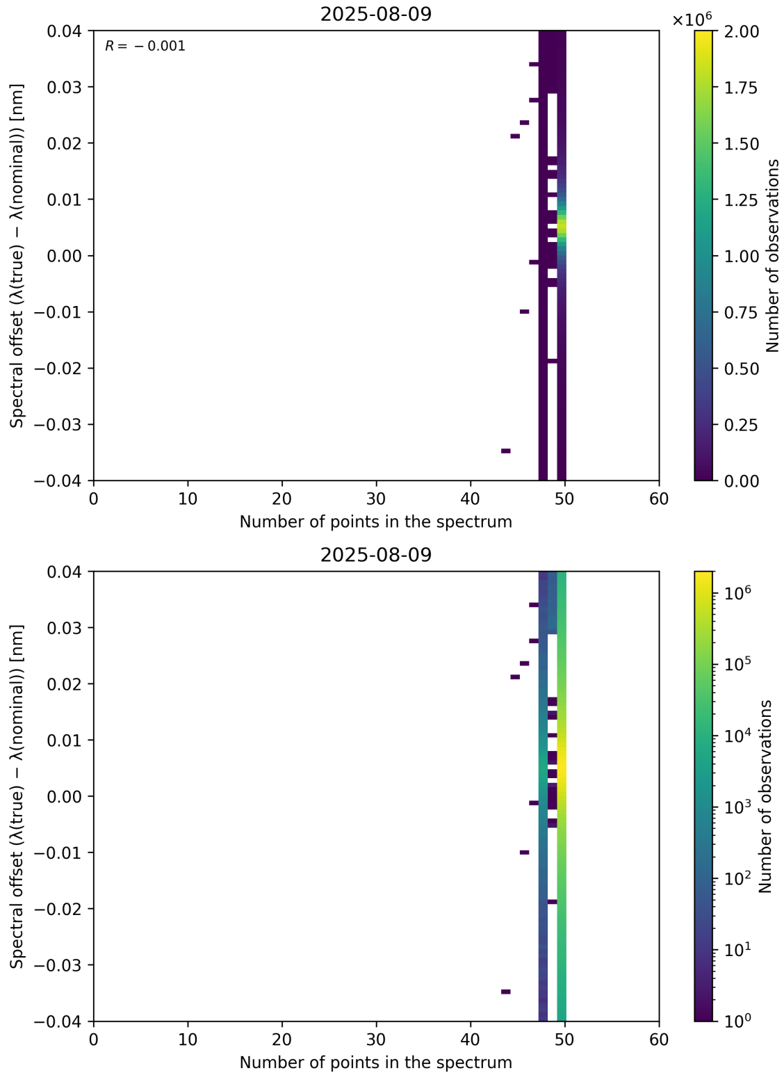
Figure 101: Scatter density plot of “Number of points in the spectrum” against “Spectral offset ( \lambda_{\text{true}} - \lambda_{\text{nominal}} )” for 2025-08-09 to 2025-08-10.
