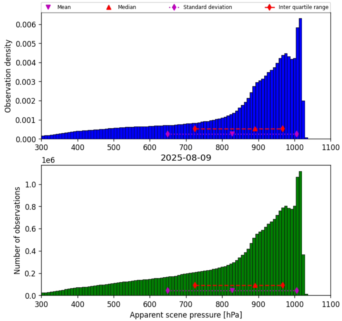
Figure 36: Histogram of “Apparent scene pressure” for 2025-08-09 to 2025-08-10
