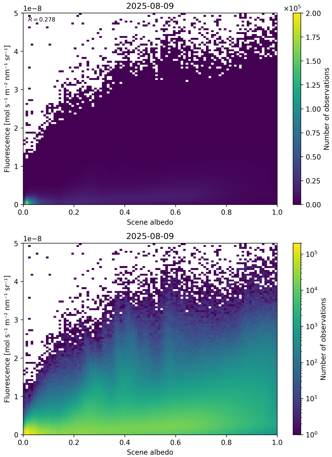
Figure 104: Scatter density plot of “Scene albedo” against “Fluorescence” for 2025-08-09 to 2025-08-10.
