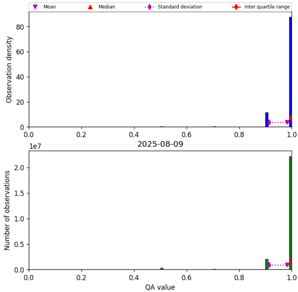
Figure 29: Histogram of “QA value” for 2025-08-09 to 2025-08-10
