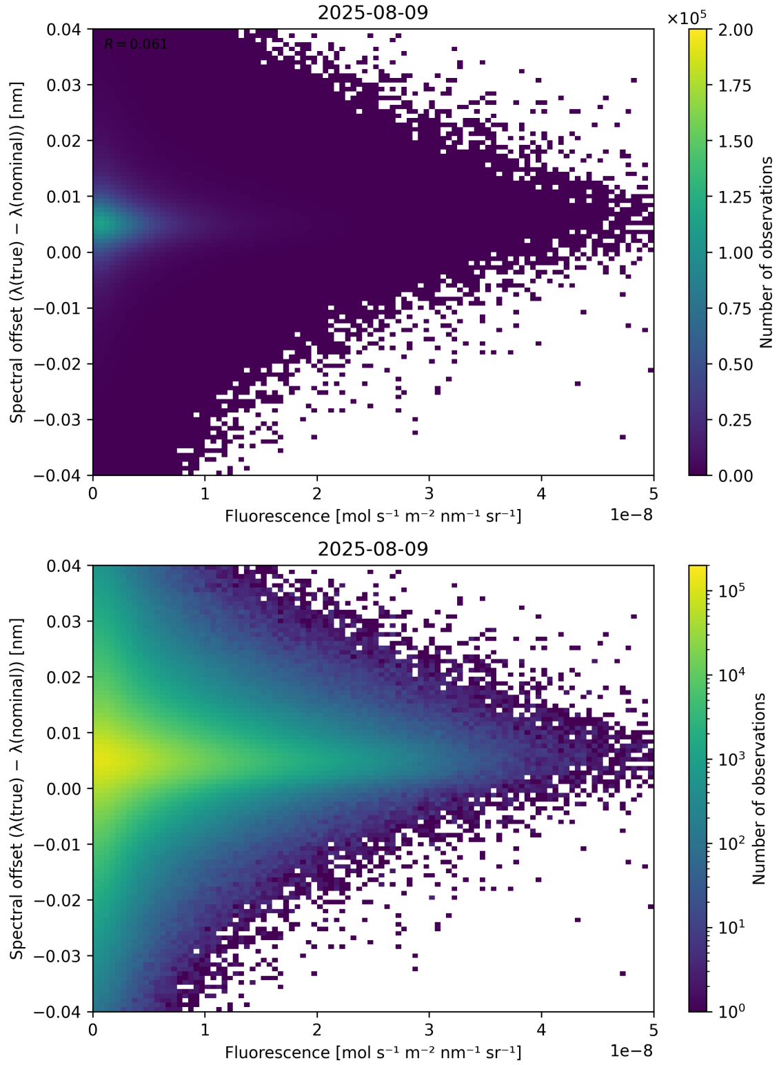
Figure 87: Scatter density plot of “Fluorescence” against “Spectral offset ( \lambda_{\text{true}} - \lambda_{\text{nominal}} )” for 2025-08-09 to 2025-08-10.
