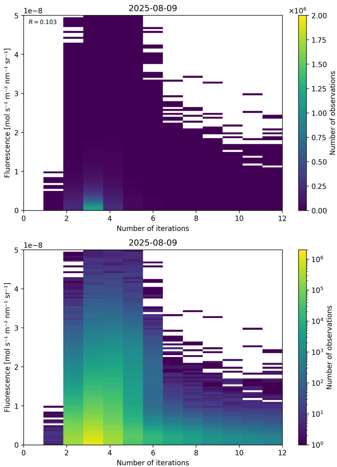
Figure 98: Scatter density plot of “Number of iterations” against “Fluorescence” for 2025-08-09 to 2025-08-10.
