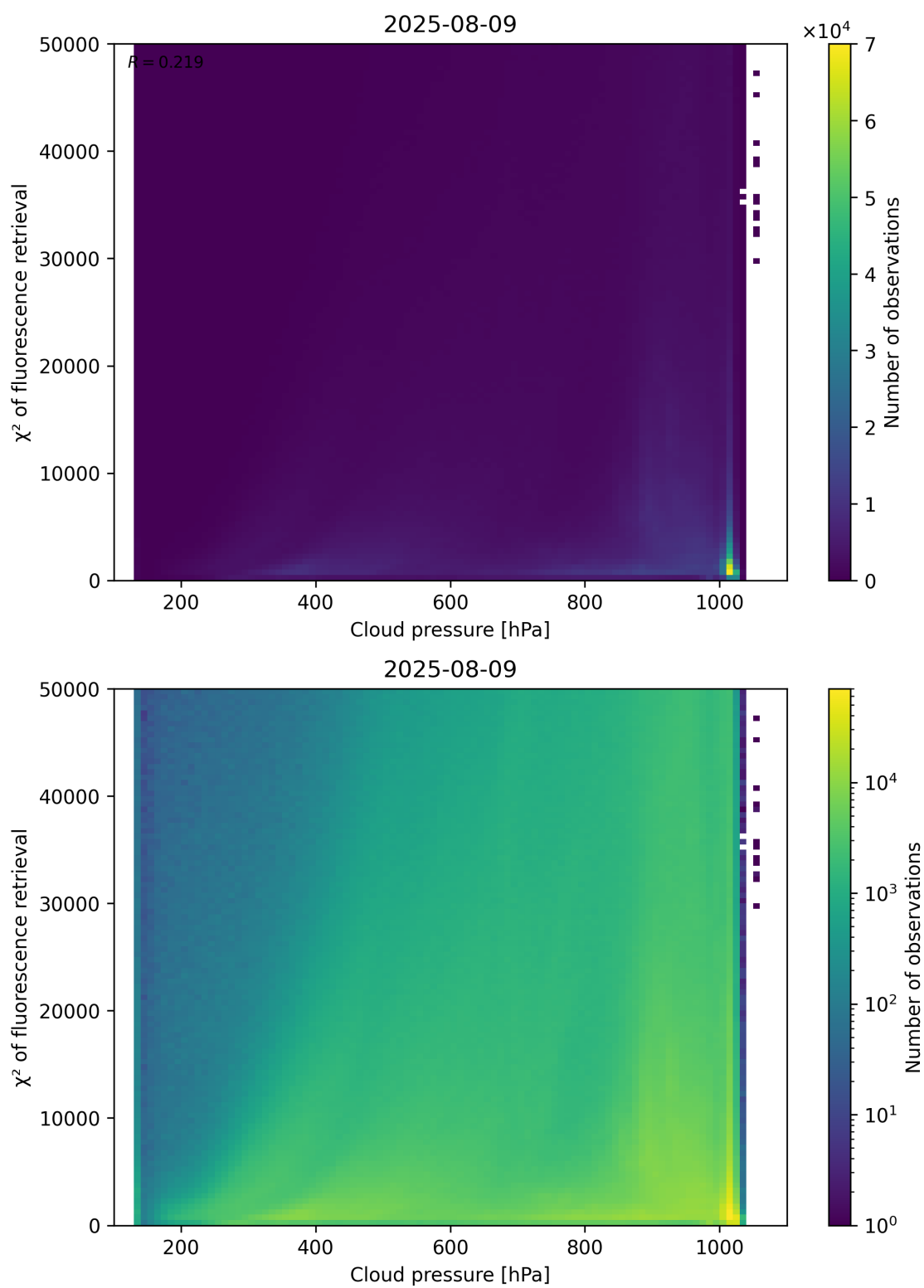
Figure 78: Scatter density plot of “Cloud pressure” against “ \chi^2 of fluorescence retrieval” for 2025-08-09 to 2025-08-10.
