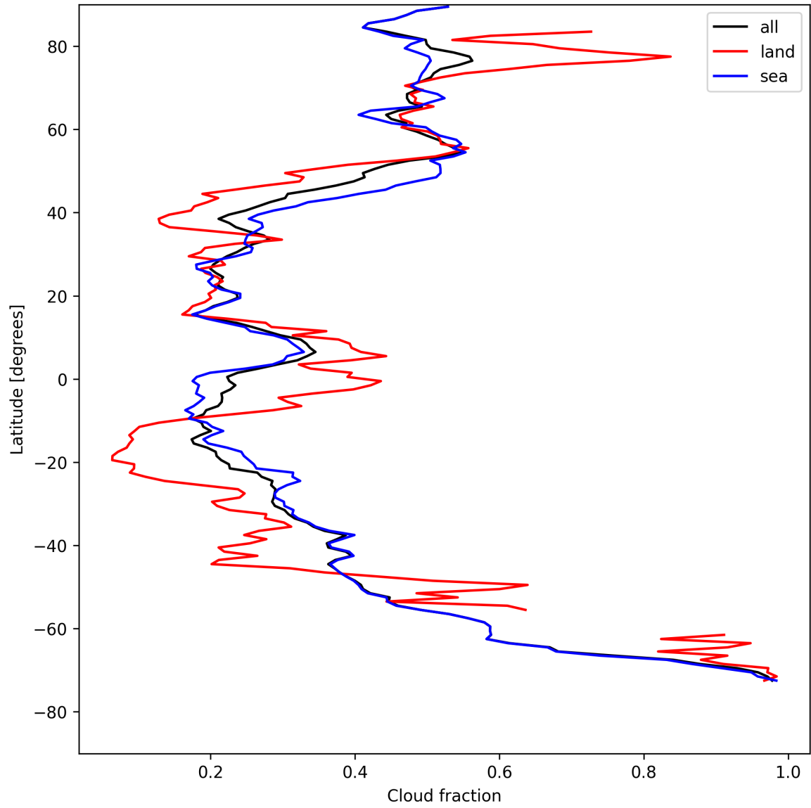
Figure 15: Zonal average of “Cloud fraction” for 2025-08-09 to 2025-08-10.
