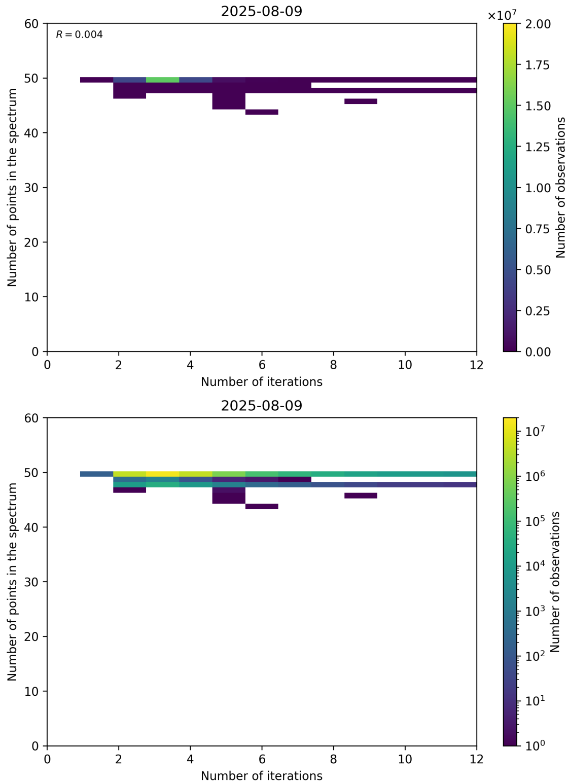
Figure 99: Scatter density plot of “Number of iterations” against “Number of points in the spectrum” for 2025-08-09 to 2025-08-10.
