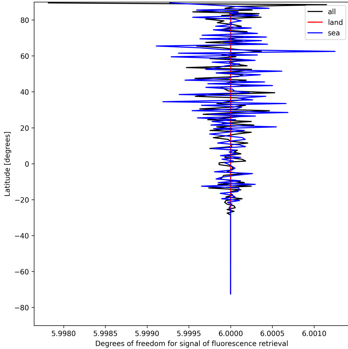
Figure 26: Zonal average of “Degrees of freedom for signal of fluorescence retrieval” for 2025-08-09 to 2025-08-10.
