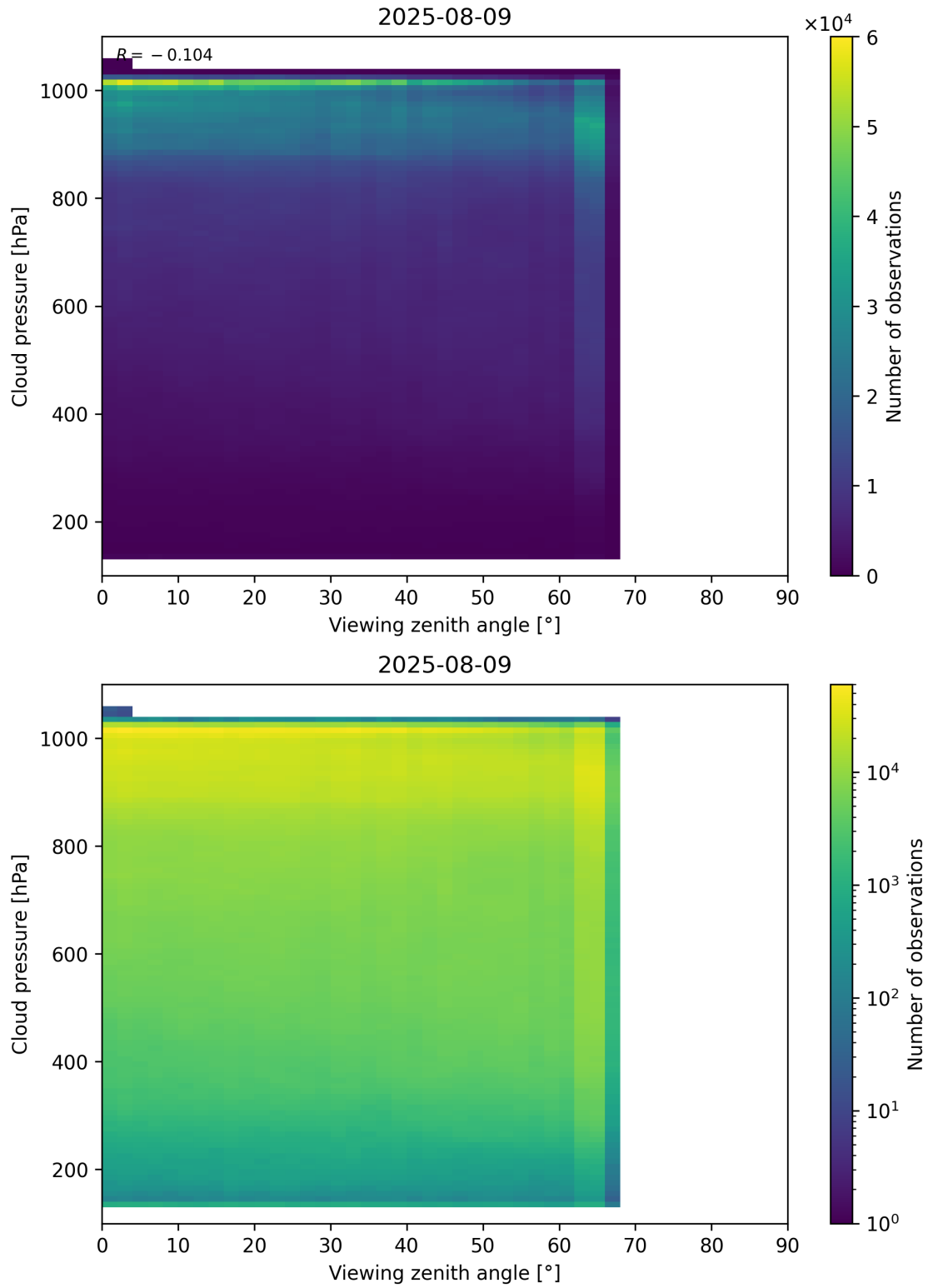
Figure 121: Scatter density plot of “Viewing zenith angle” against “Cloud pressure” for 2025-08-09 to 2025-08-10.
