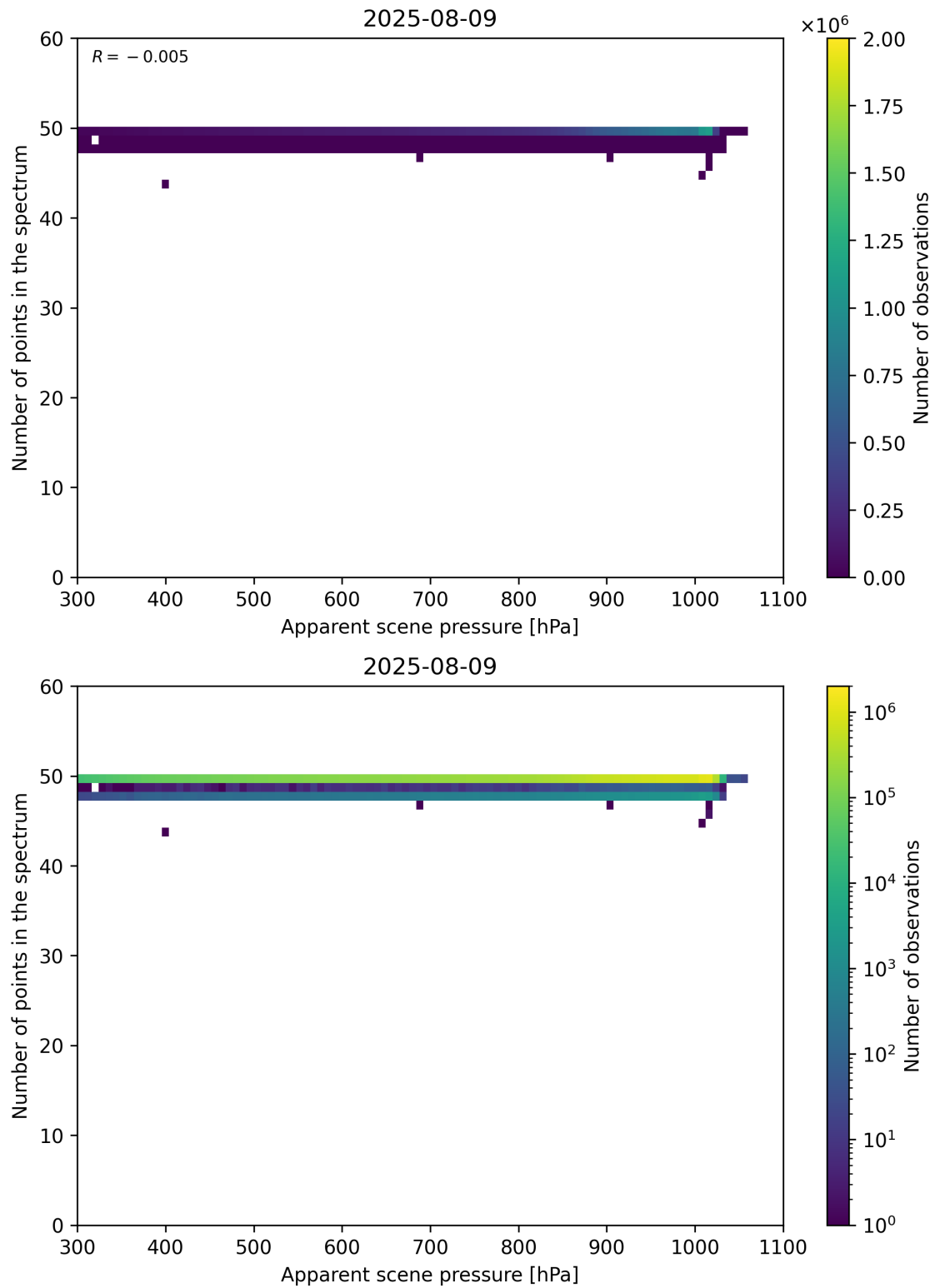
Figure 66: Scatter density plot of “Apparent scene pressure” against “Number of points in the spectrum” for 2025-08-09 to 2025-08-10.
