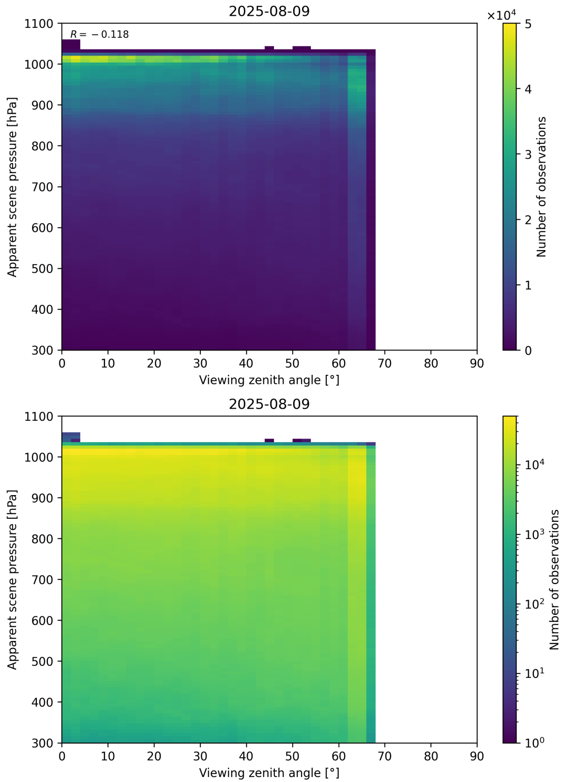
Figure 118: Scatter density plot of “Viewing zenith angle” against “Apparent scene pressure” for 2025-08-09 to 2025-08-10.
