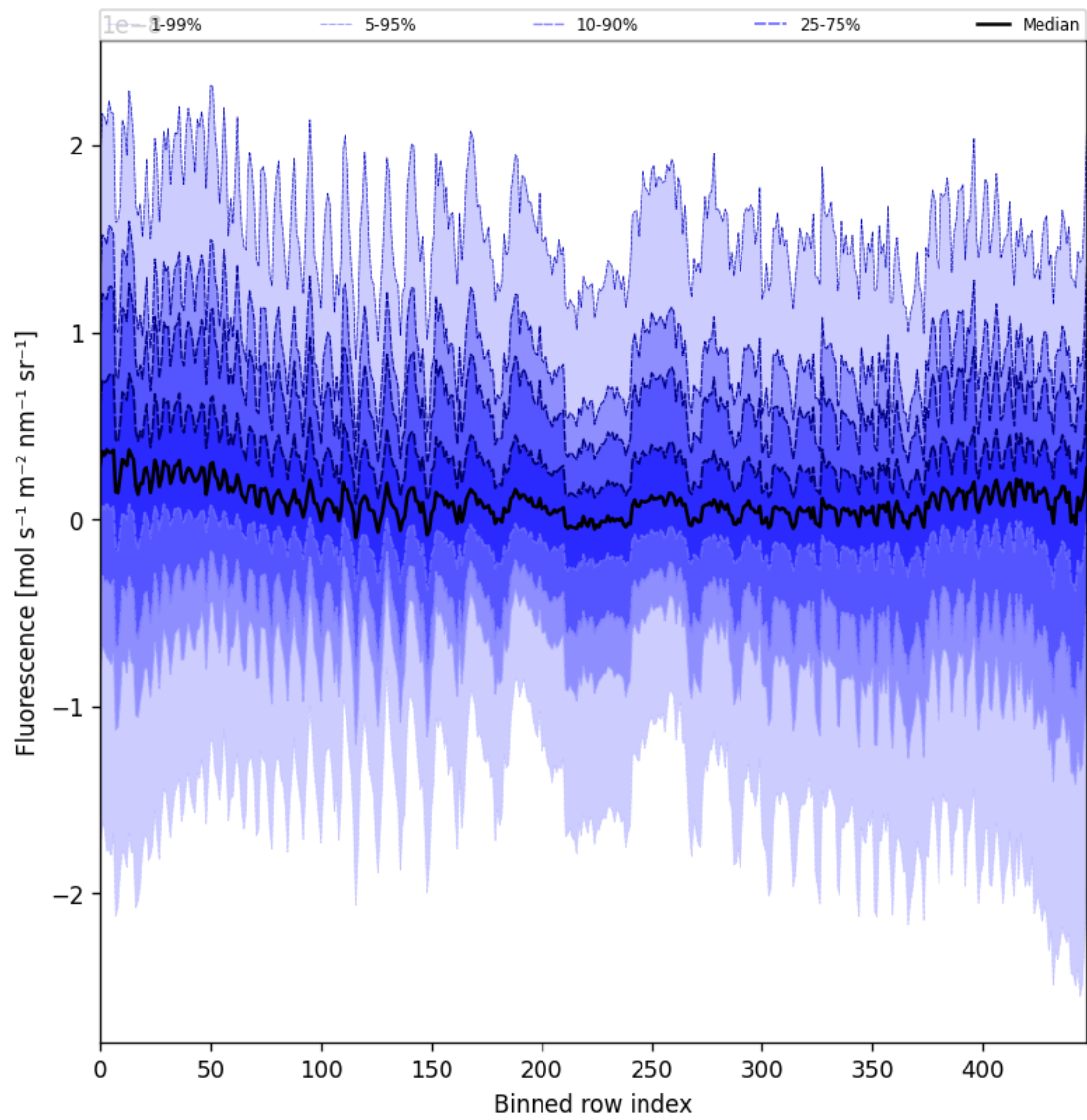
Figure 57: Along track statistics of “Fluorescence” for 2025-08-09 to 2025-08-10
