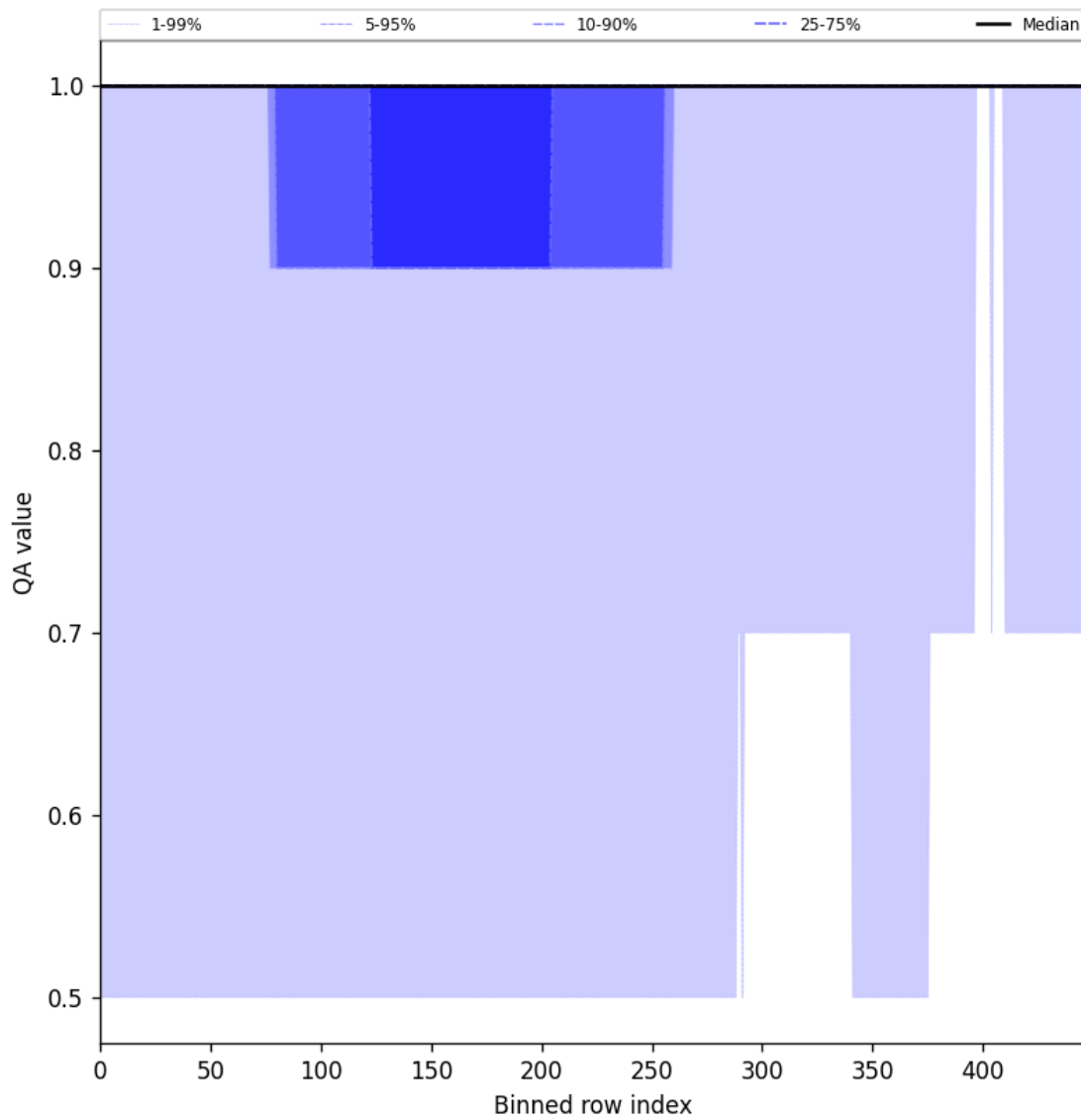
Figure 46: Along track statistics of “QA value” for 2025-08-09 to 2025-08-10
