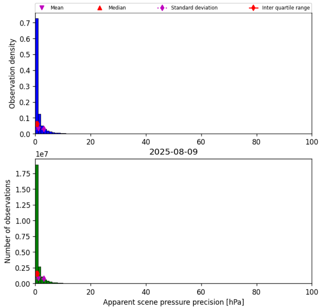
Figure 37: Histogram of “Apparent scene pressure precision” for 2025-08-09 to 2025-08-10
