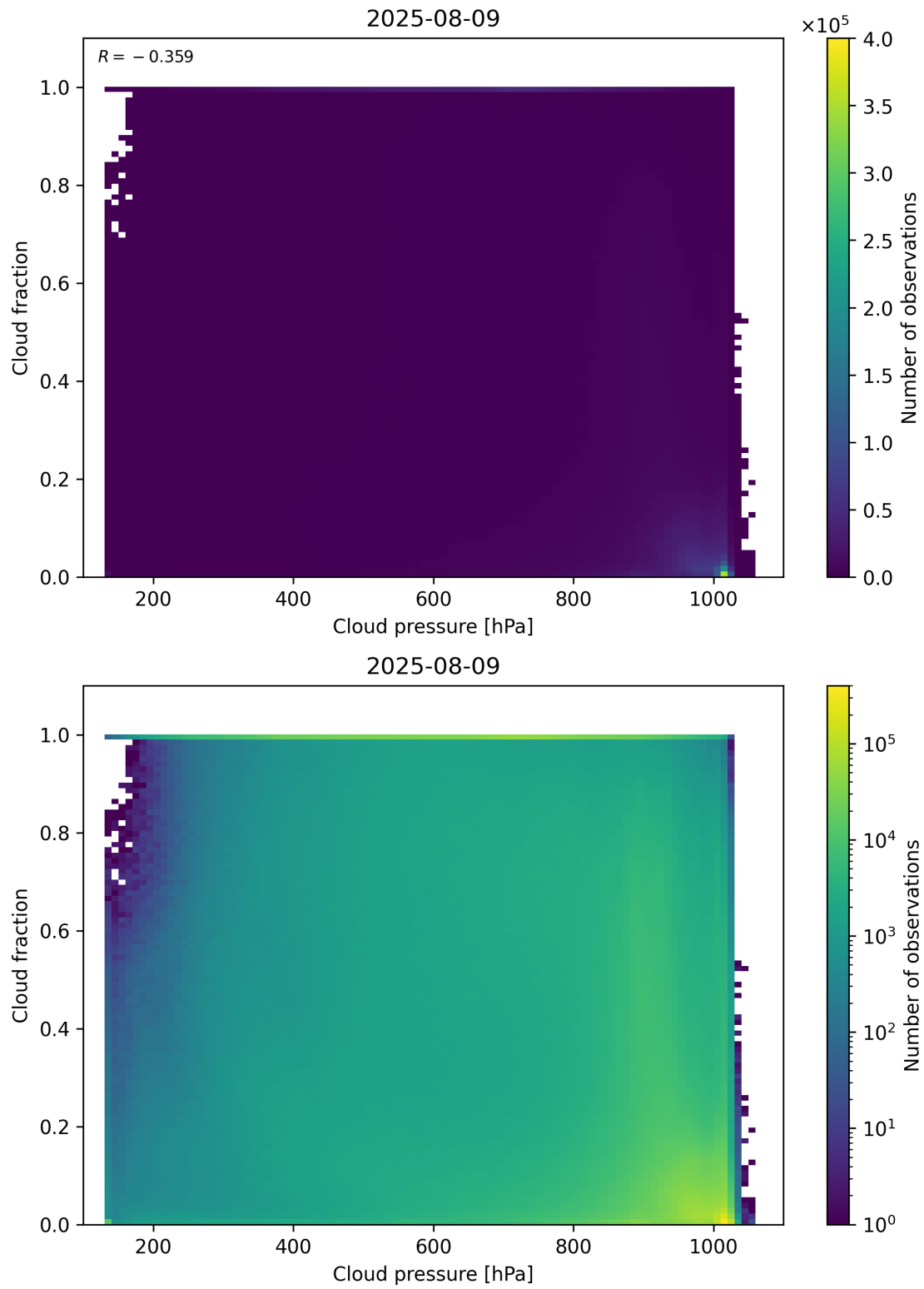
Figure 79: Scatter density plot of “Cloud pressure” against “Cloud fraction” for 2025-08-09 to 2025-08-10.
