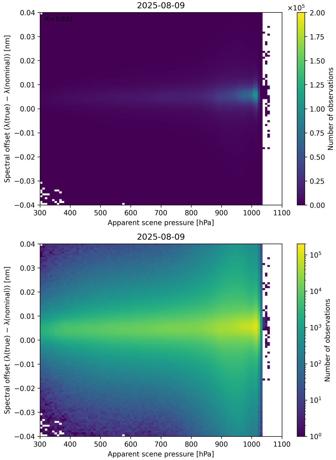
Figure 67: Scatter density plot of “Apparent scene pressure” against “Spectral offset ( \lambda_{\text{true}} - \lambda_{\text{nominal}} )” for 2025-08-09 to 2025-08-10.
