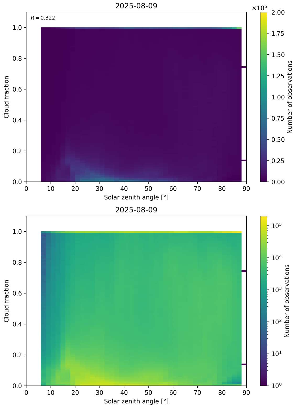
Figure 110: Scatter density plot of “Solar zenith angle” against “Cloud fraction” for 2025-08-09 to 2025-08-10.
