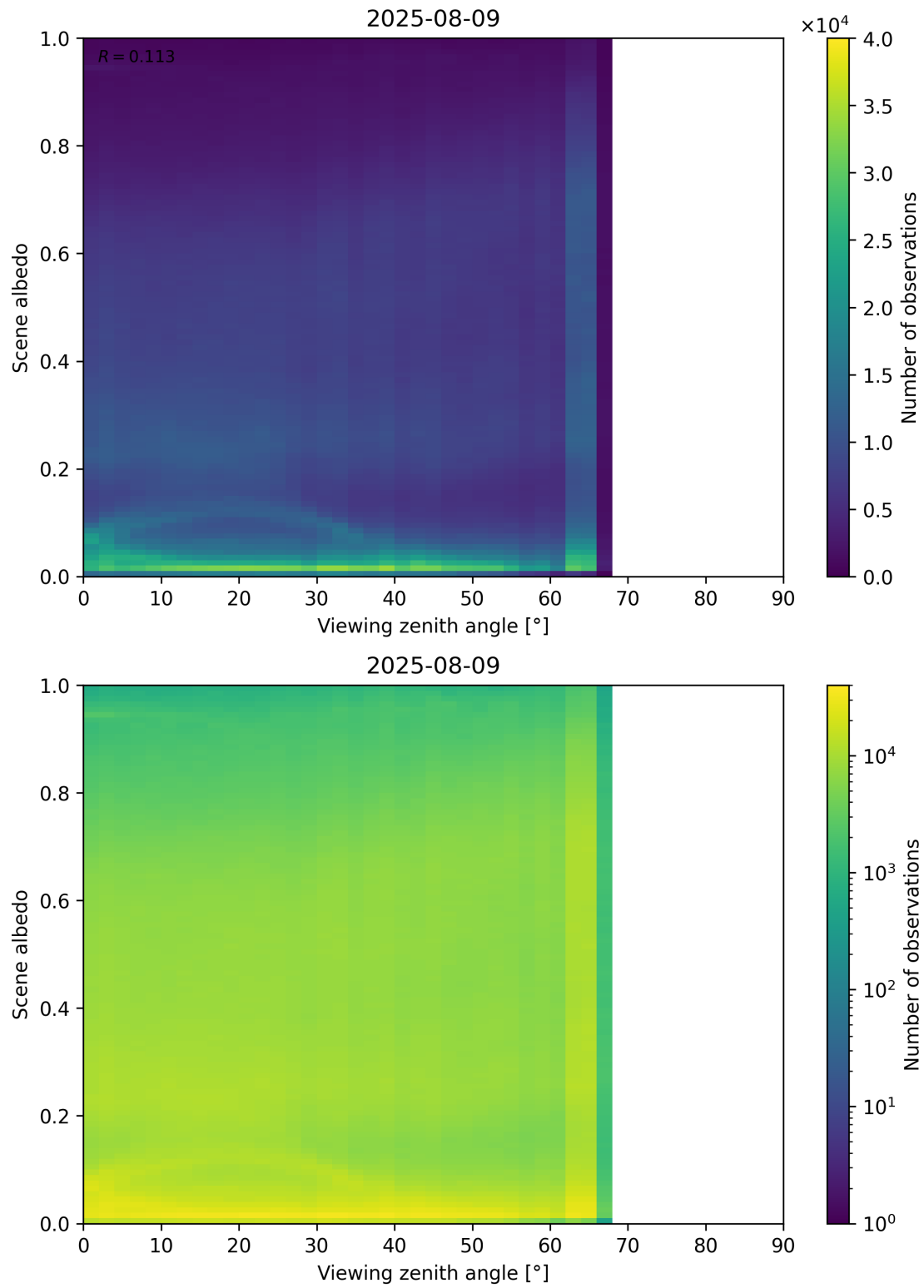
Figure 126: Scatter density plot of “Viewing zenith angle” against “Scene albedo” for 2025-08-09 to 2025-08-10.
