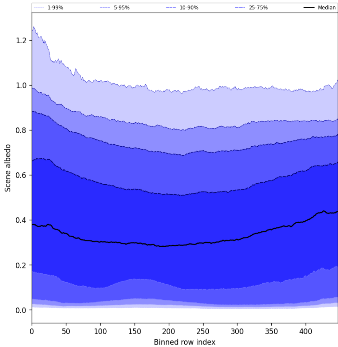
Figure 51: Along track statistics of “Scene albedo” for 2025-08-09 to 2025-08-10
