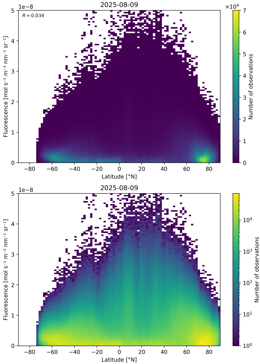
Figure 92: Scatter density plot of “Latitude” against “Fluorescence” for 2025-08-09 to 2025-08-10.
