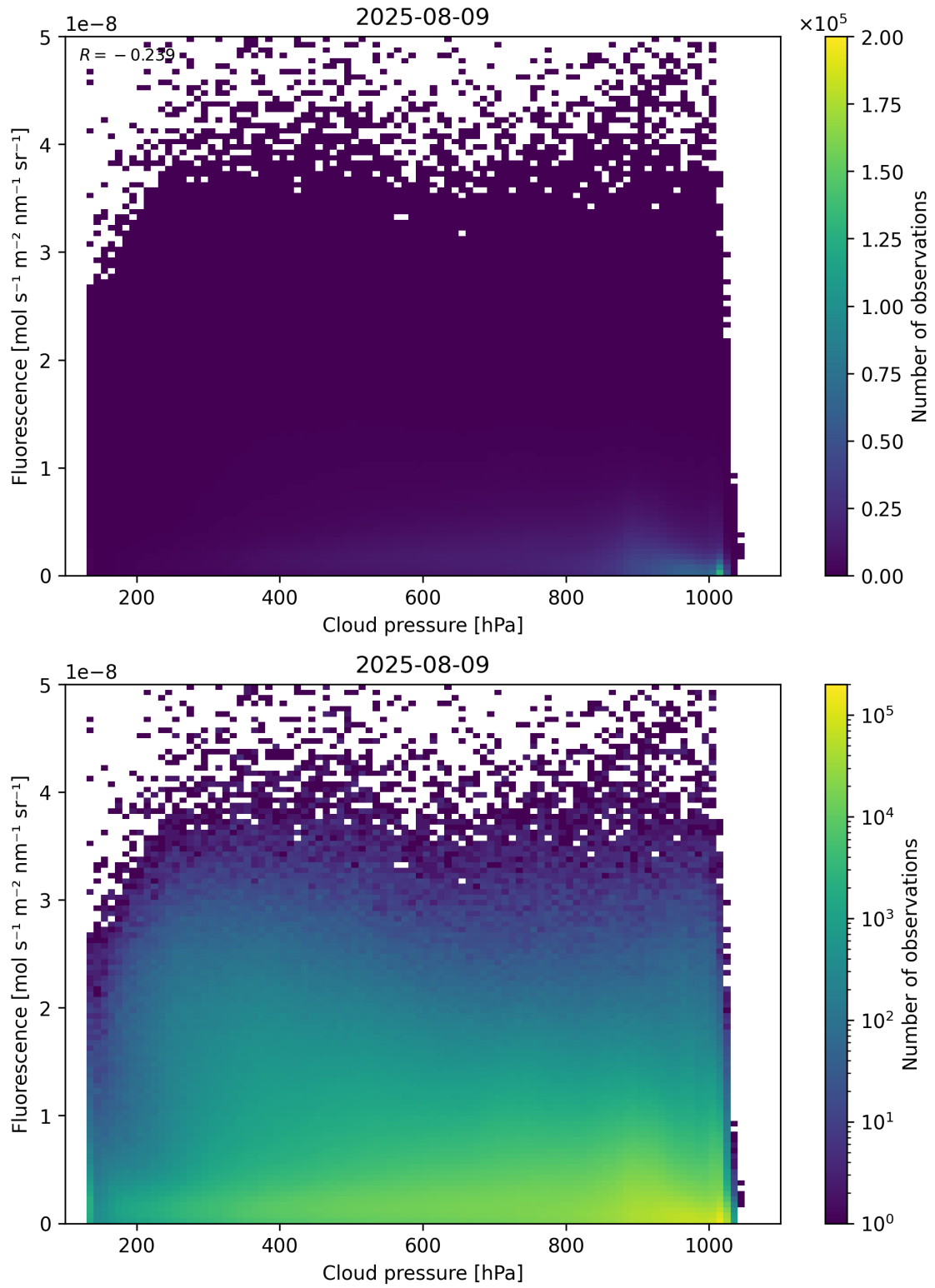
Figure 80: Scatter density plot of “Cloud pressure” against “Fluorescence” for 2025-08-09 to 2025-08-10.
