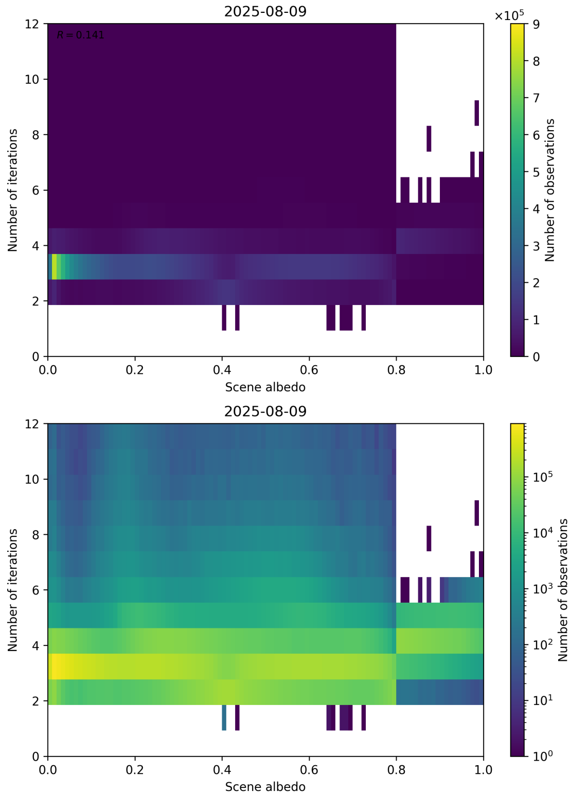
Figure 105: Scatter density plot of “Scene albedo” against “Number of iterations” for 2025-08-09 to 2025-08-10.
