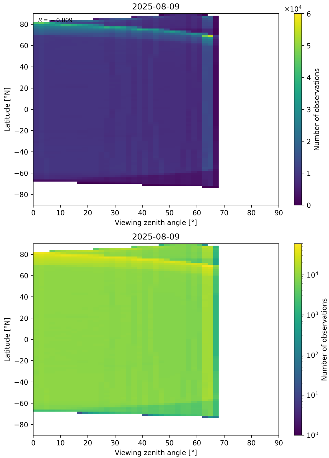
Figure 123: Scatter density plot of “Viewing zenith angle” against “Latitude” for 2025-08-09 to 2025-08-10.
