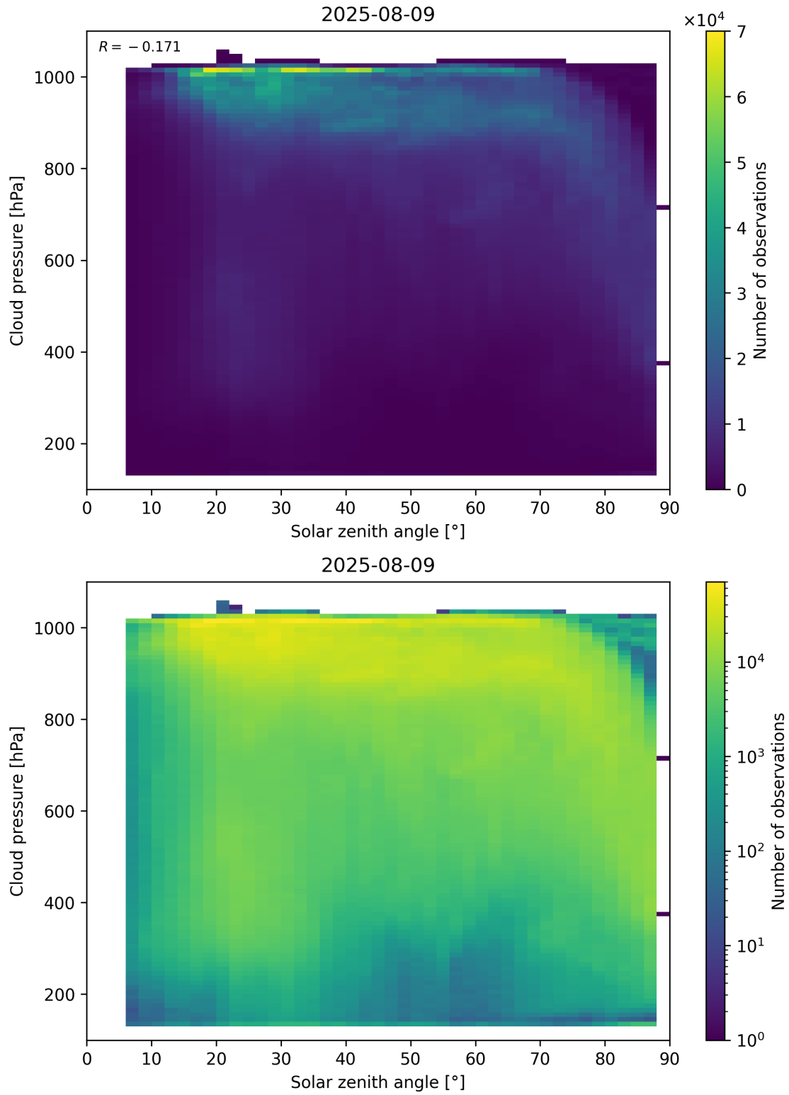
Figure 111: Scatter density plot of “Solar zenith angle” against “Cloud pressure” for 2025-08-09 to 2025-08-10.
