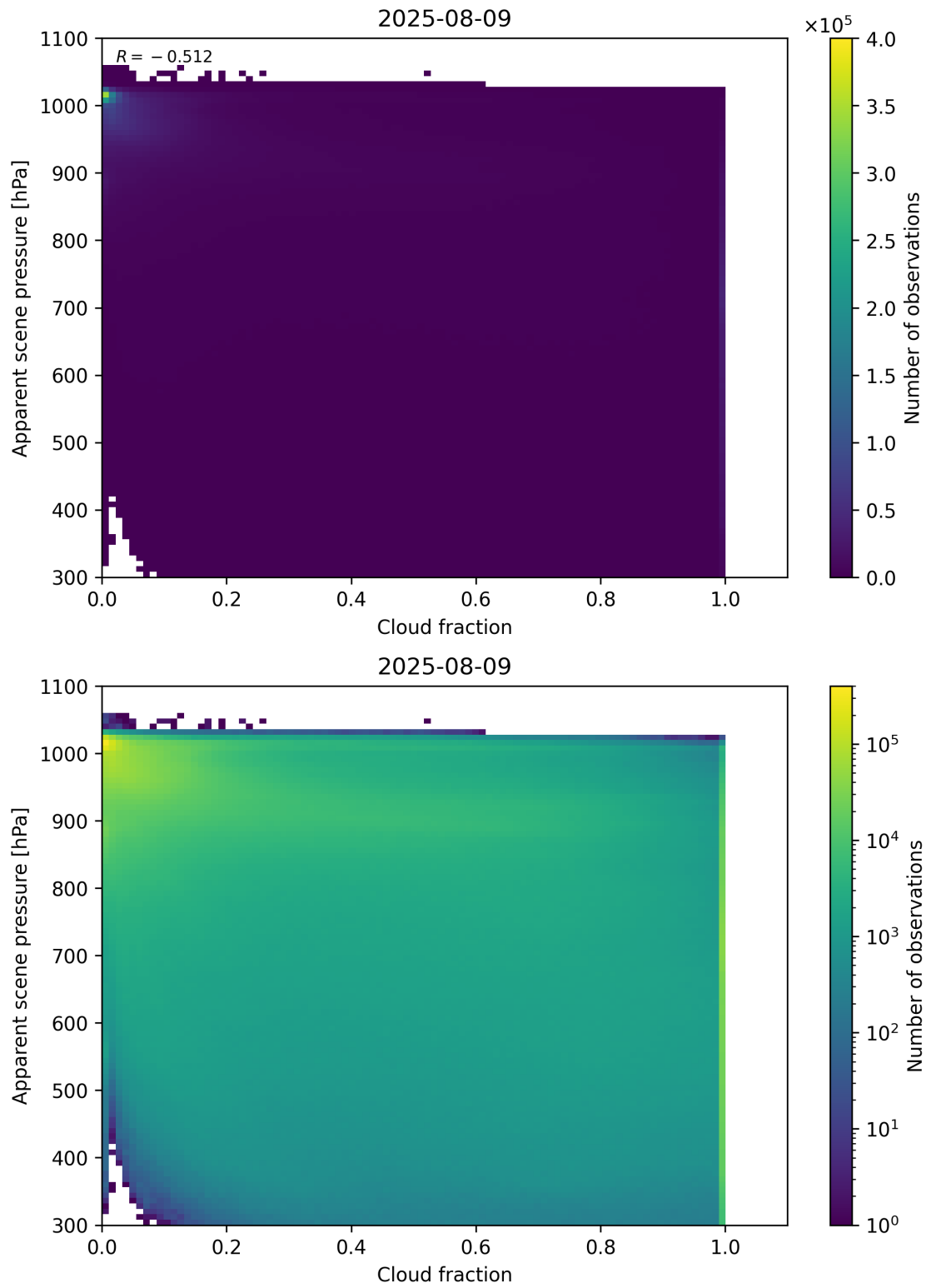
Figure 70: Scatter density plot of “Cloud fraction” against “Apparent scene pressure” for 2025-08-09 to 2025-08-10.
