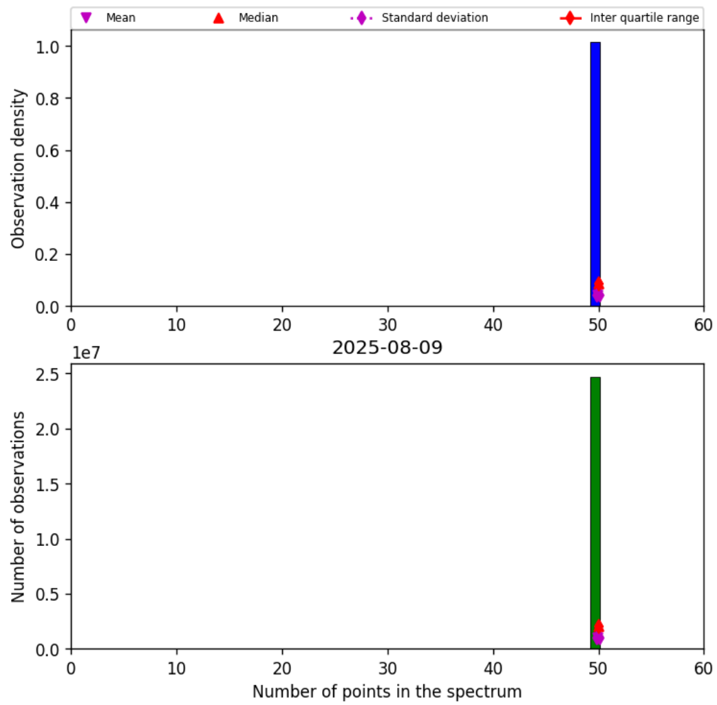
Figure 44: Histogram of “Number of points in the spectrum” for 2025-08-09 to 2025-08-10
