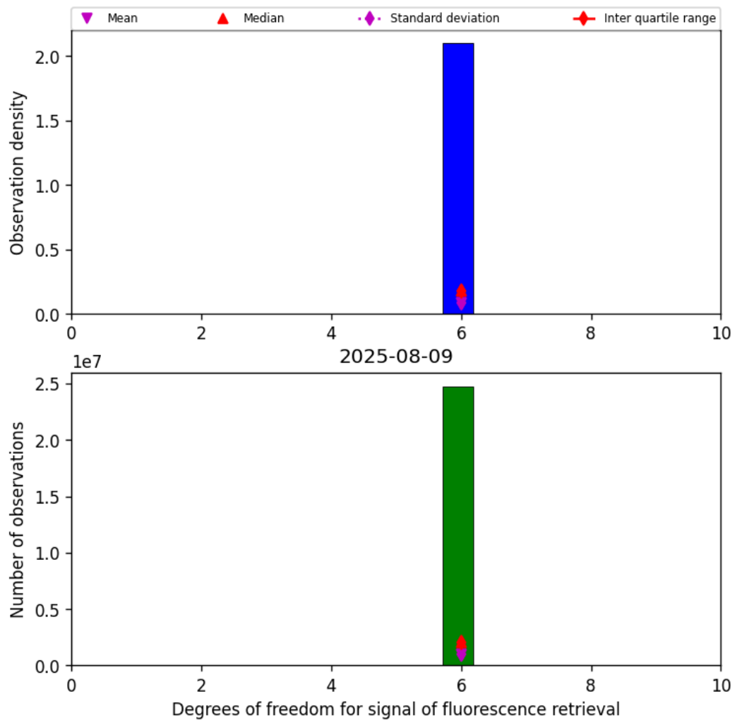
Figure 43: Histogram of “Degrees of freedom for signal of fluorescence retrieval” for 2025-08-09 to 2025-08-10
