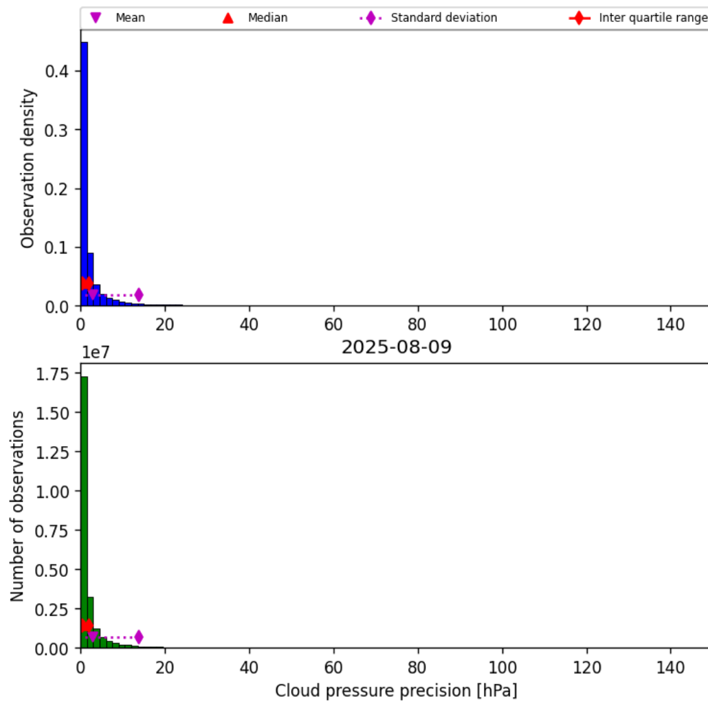
Figure 31: Histogram of “Cloud pressure precision” for 2025-08-09 to 2025-08-10
