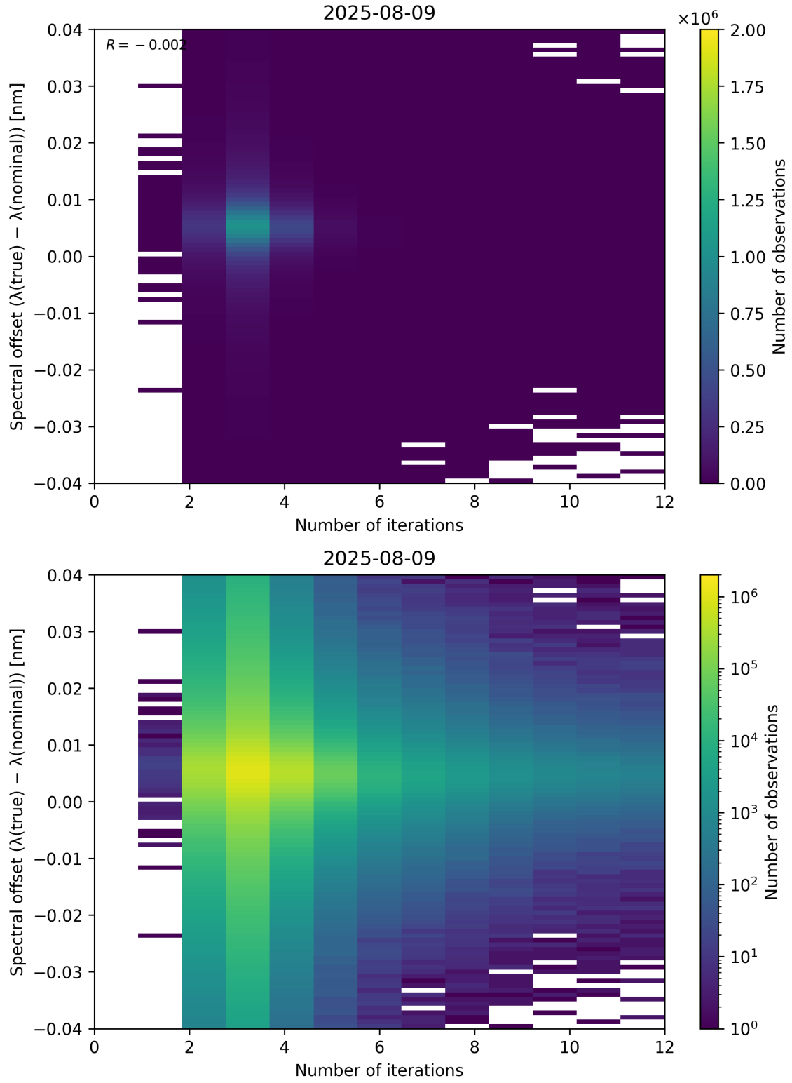
Figure 100: Scatter density plot of “Number of iterations” against “Spectral offset ( \lambda_{\text{true}} - \lambda_{\text{nominal}} )” for 2025-08-09 to 2025-08-10.
