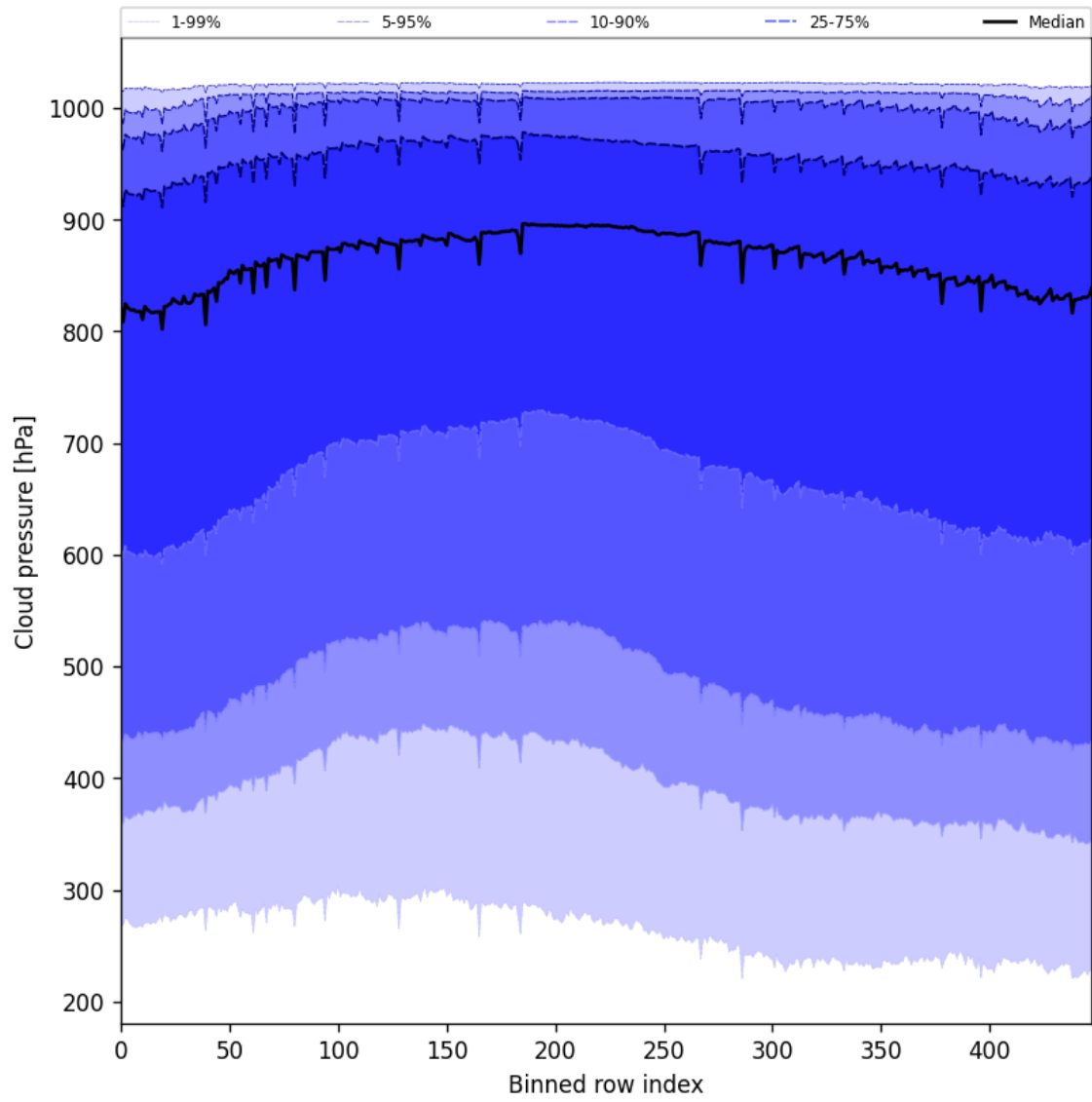
Figure 47: Along track statistics of “Cloud pressure” for 2025-08-09 to 2025-08-10
