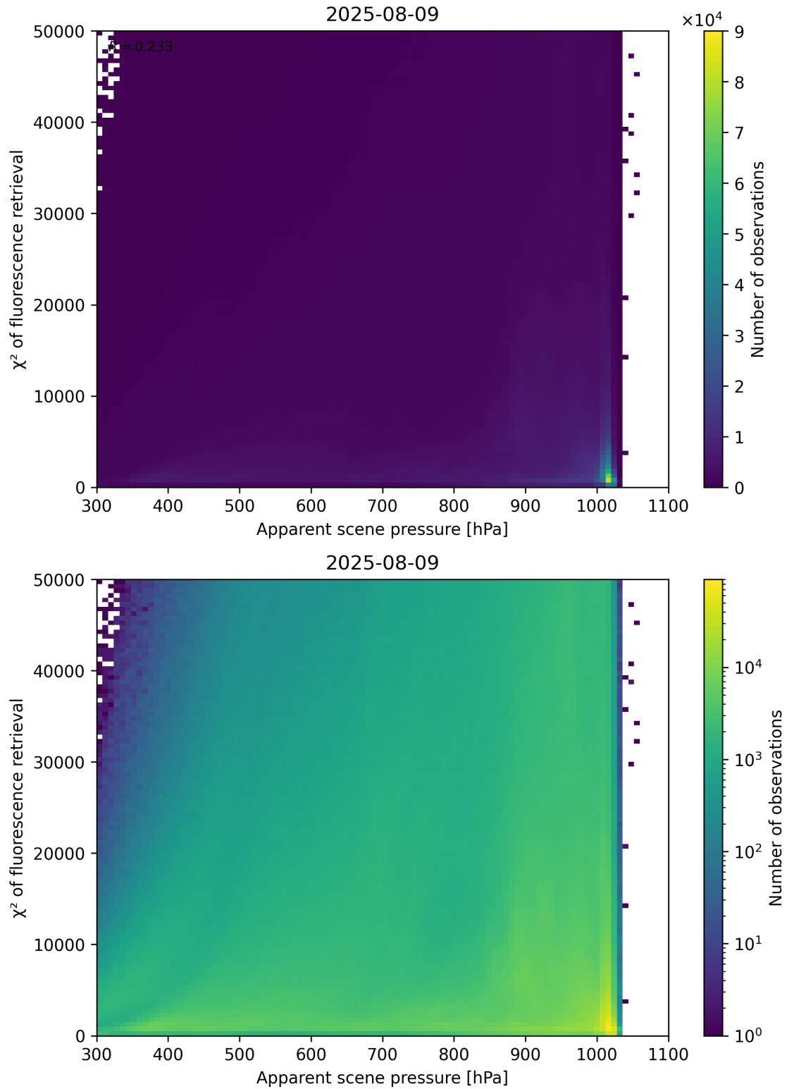
Figure 63: Scatter density plot of “Apparent scene pressure” against “ \chi^2 of fluorescence retrieval” for 2025-08-09 to 2025-08-10.
