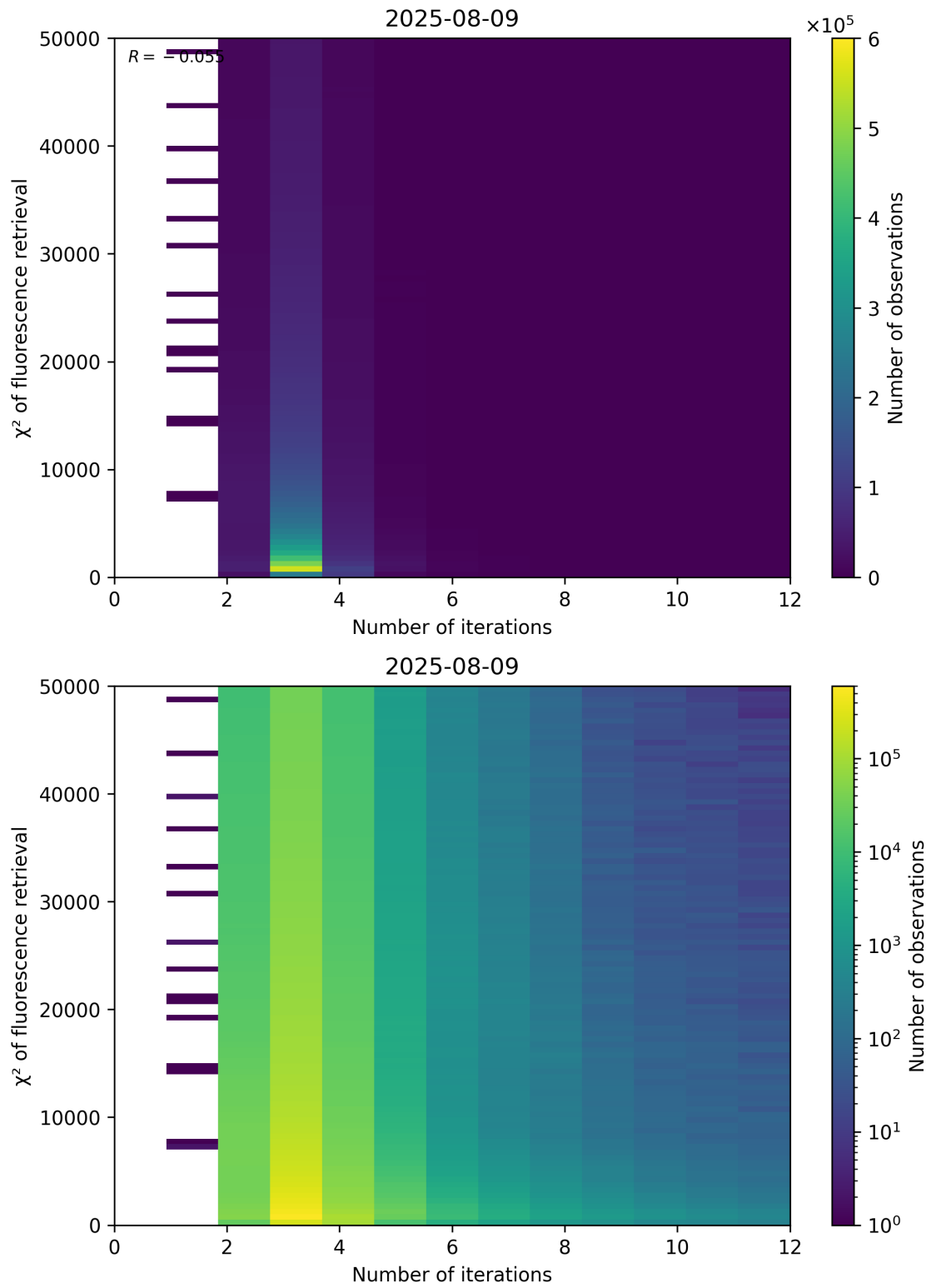
Figure 97: Scatter density plot of “Number of iterations” against “ \chi^2 of fluorescence retrieval” for 2025-08-09 to 2025-08-10.
