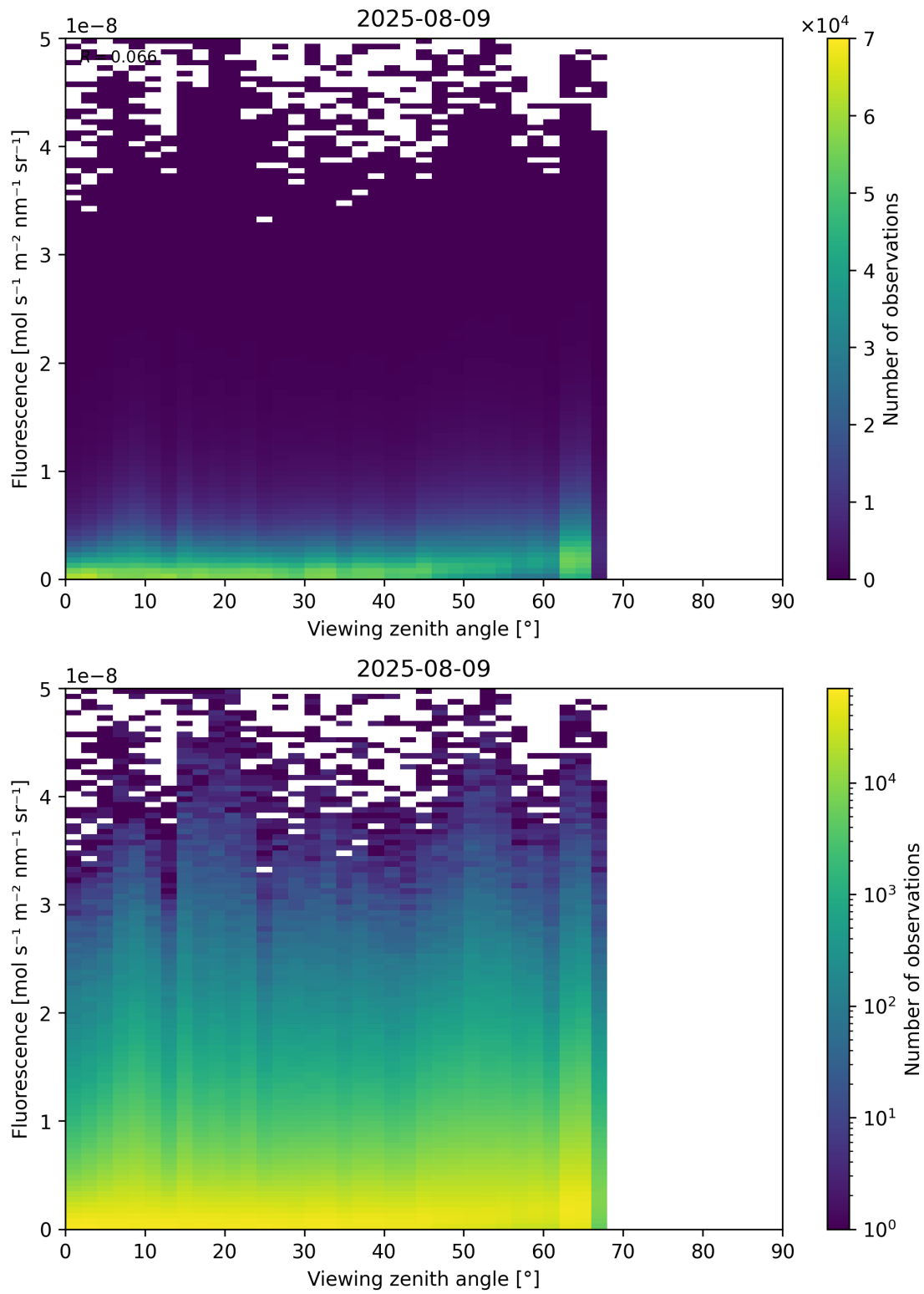
Figure 122: Scatter density plot of “Viewing zenith angle” against “Fluorescence” for 2025-08-09 to 2025-08-10.
