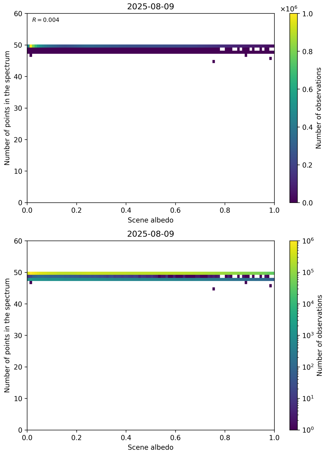
Figure 106: Scatter density plot of “Scene albedo” against “Number of points in the spectrum” for 2025-08-09 to 2025-08-10.
