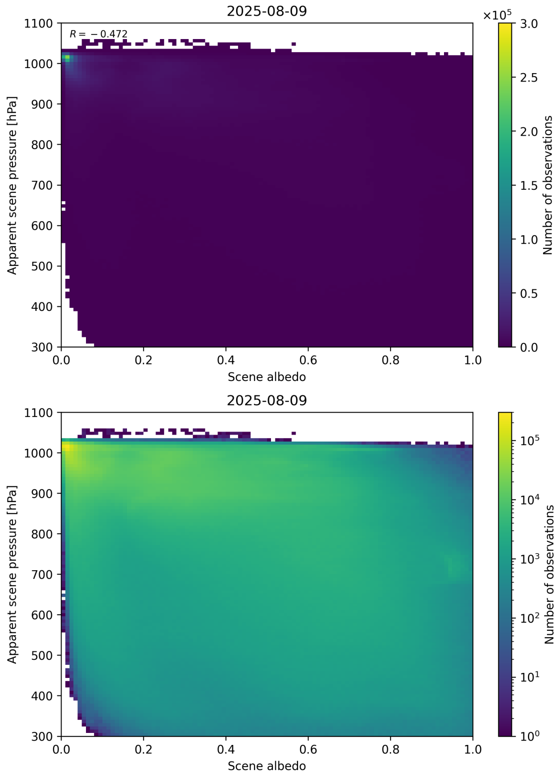
Figure 102: Scatter density plot of “Scene albedo” against “Apparent scene pressure” for 2025-08-09 to 2025-08-10.
