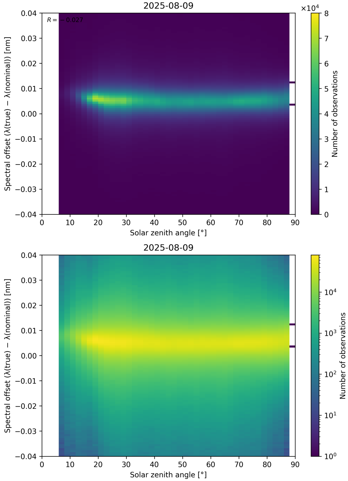
Figure 117: Scatter density plot of “Solar zenith angle” against “Spectral offset ( \lambda_{\text{true}} - \lambda_{\text{nominal}} )” for 2025-08-09 to 2025-08-10.
