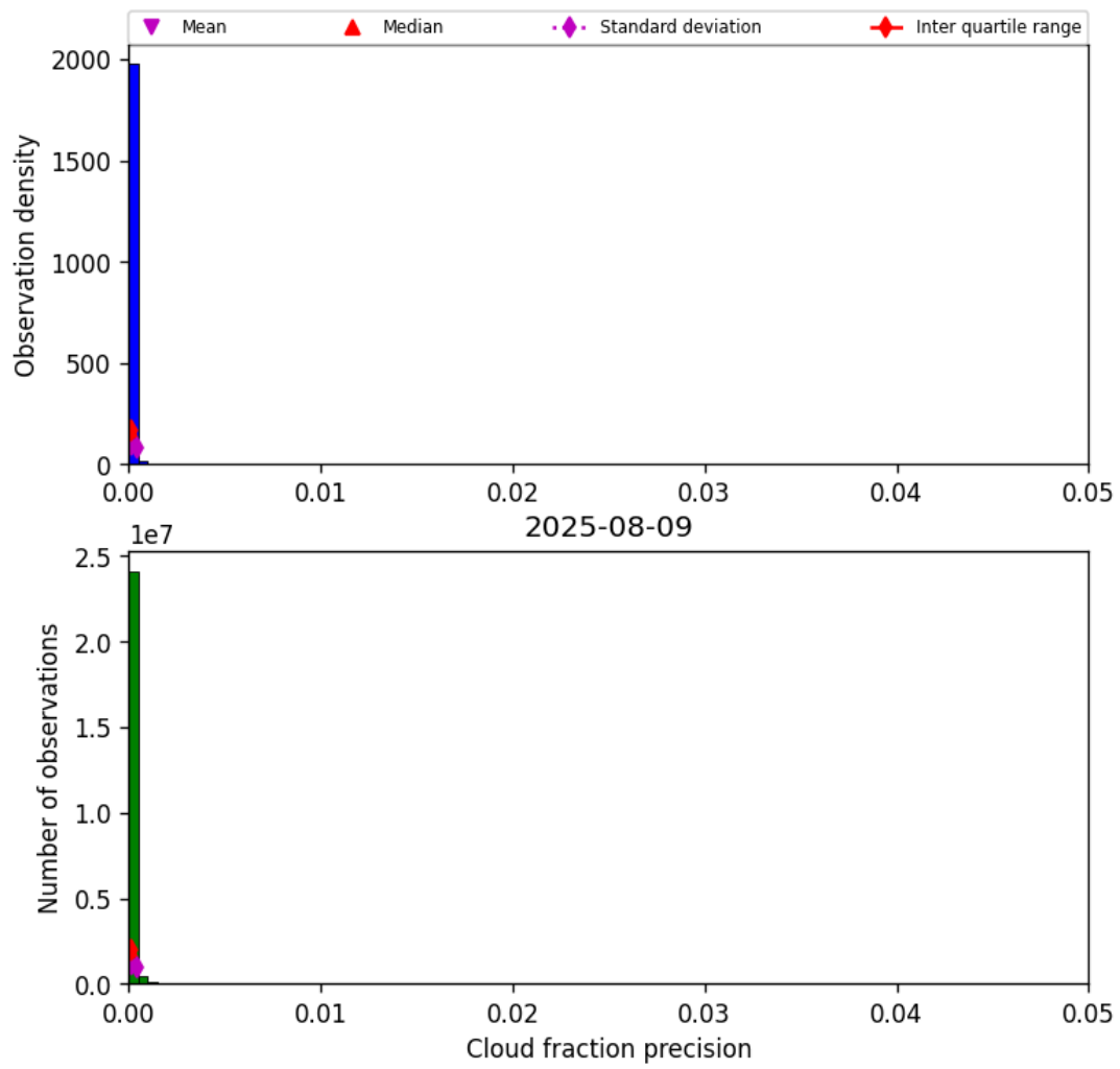
Figure 33: Histogram of “Cloud fraction precision” for 2025-08-09 to 2025-08-10
