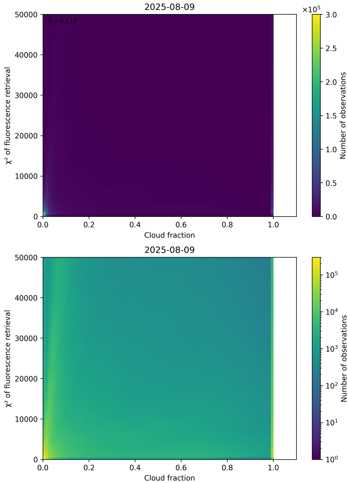
Figure 71: Scatter density plot of “Cloud fraction” against “ \chi^2 of fluorescence retrieval” for 2025-08-09 to 2025-08-10.
