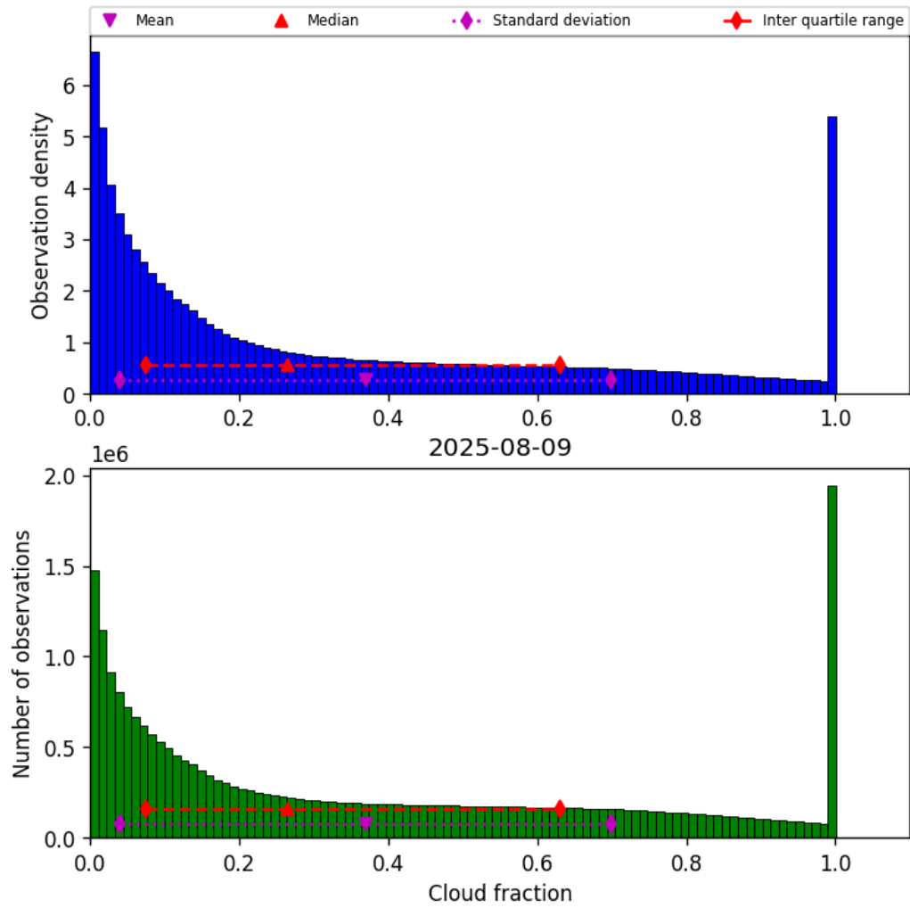
Figure 32: Histogram of “Cloud fraction” for 2025-08-09 to 2025-08-10
