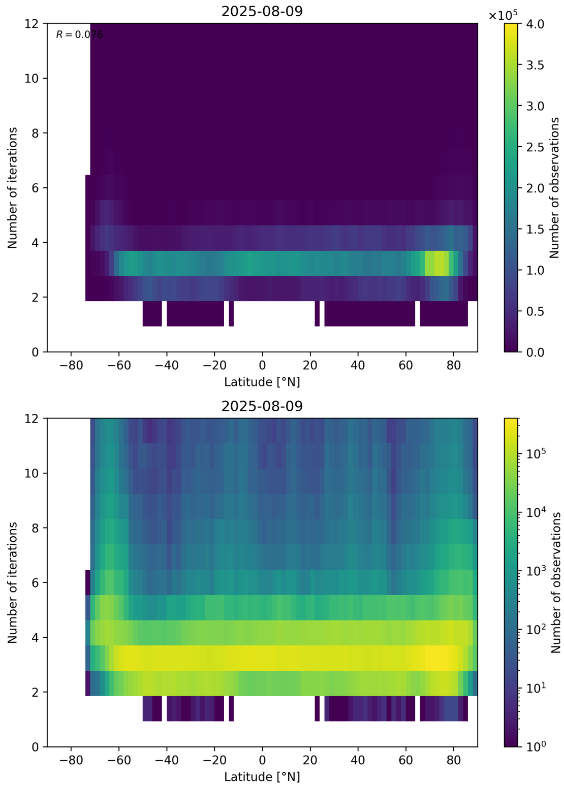
Figure 93: Scatter density plot of “Latitude” against “Number of iterations” for 2025-08-09 to 2025-08-10.
