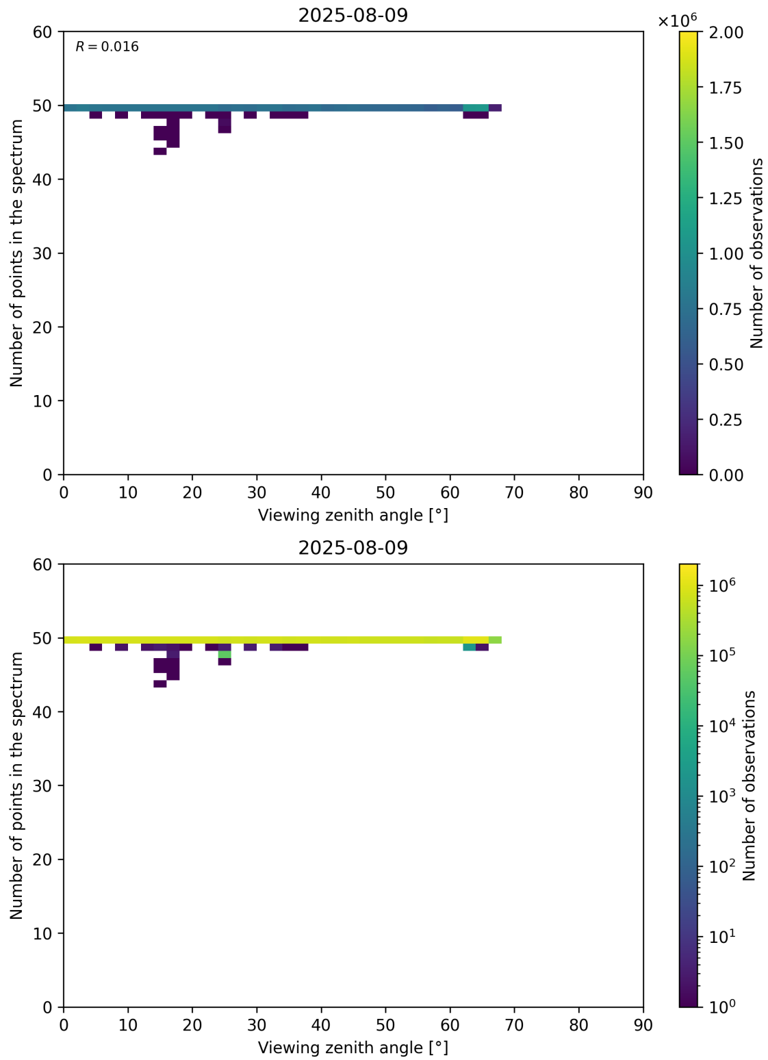
Figure 125: Scatter density plot of “Viewing zenith angle” against “Number of points in the spectrum” for 2025-08-09 to 2025-08-10.
