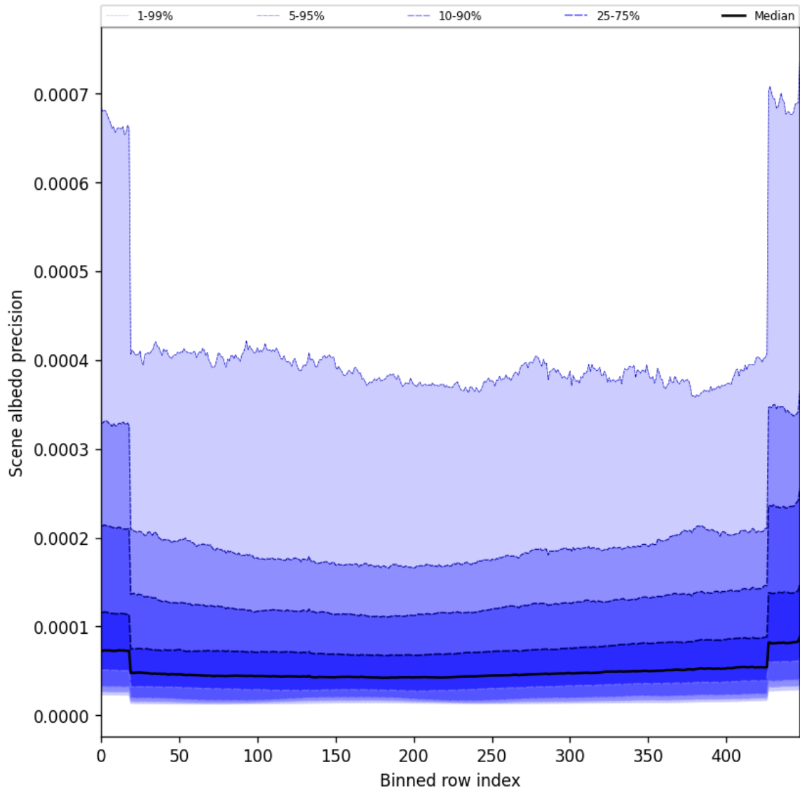
Figure 52: Along track statistics of “Scene albedo precision” for 2025-08-09 to 2025-08-10
