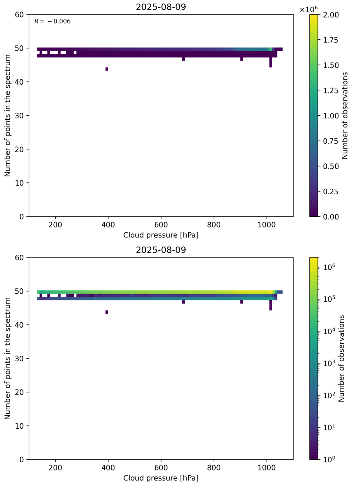
Figure 82: Scatter density plot of “Cloud pressure” against “Number of points in the spectrum” for 2025-08-09 to 2025-08-10.
