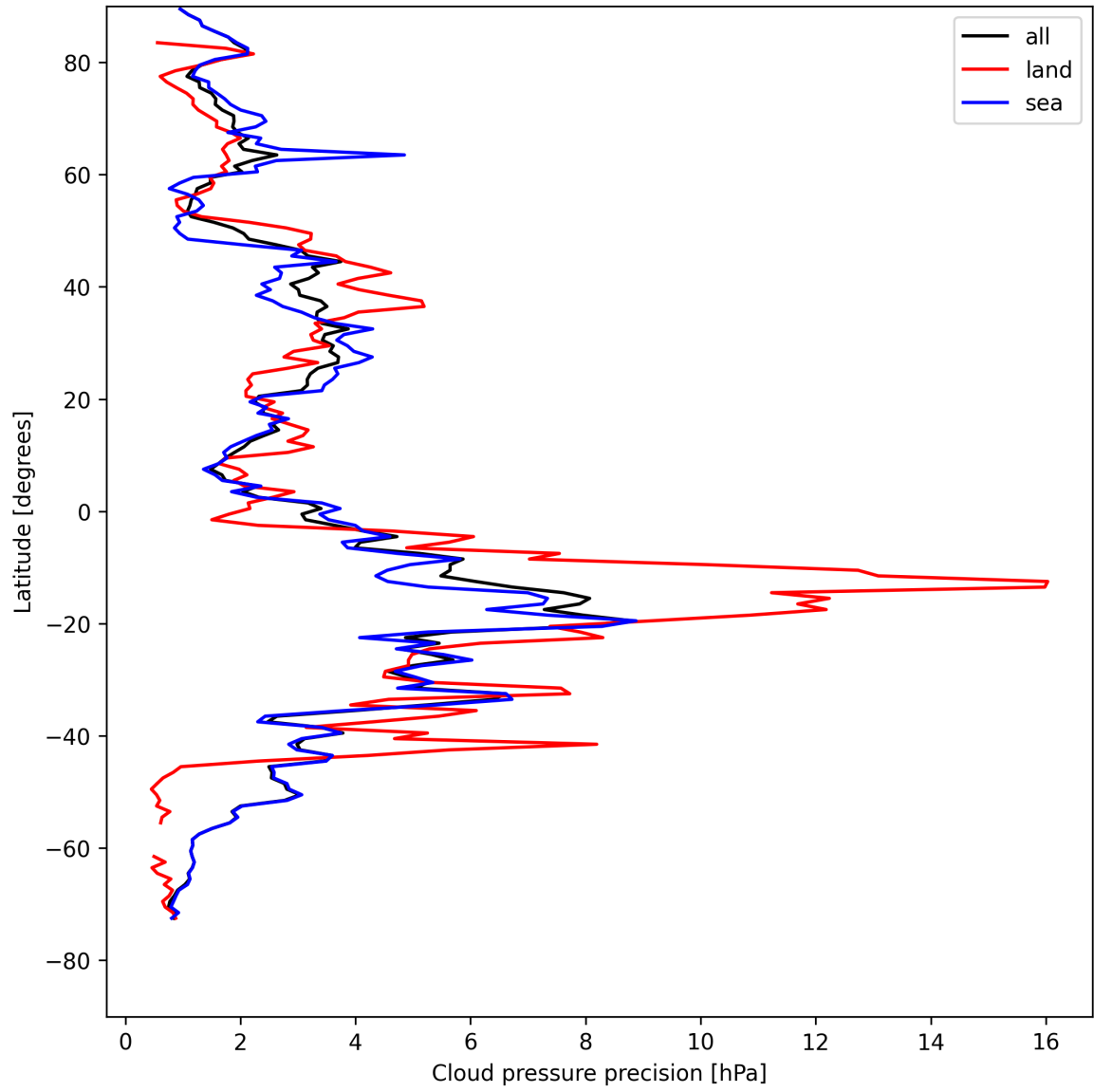
Figure 14: Zonal average of “Cloud pressure precision” for 2025-08-09 to 2025-08-10.
