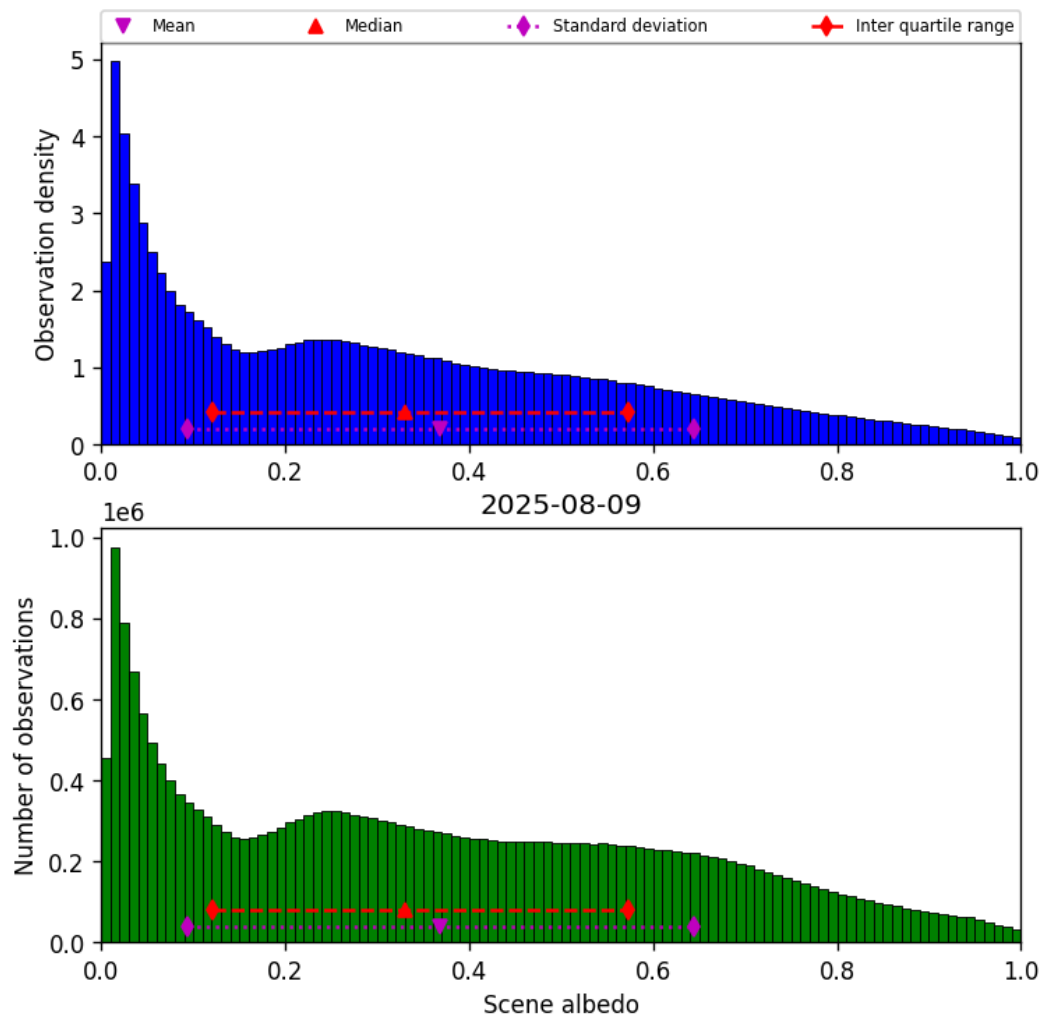
Figure 34: Histogram of “Scene albedo” for 2025-08-09 to 2025-08-10
