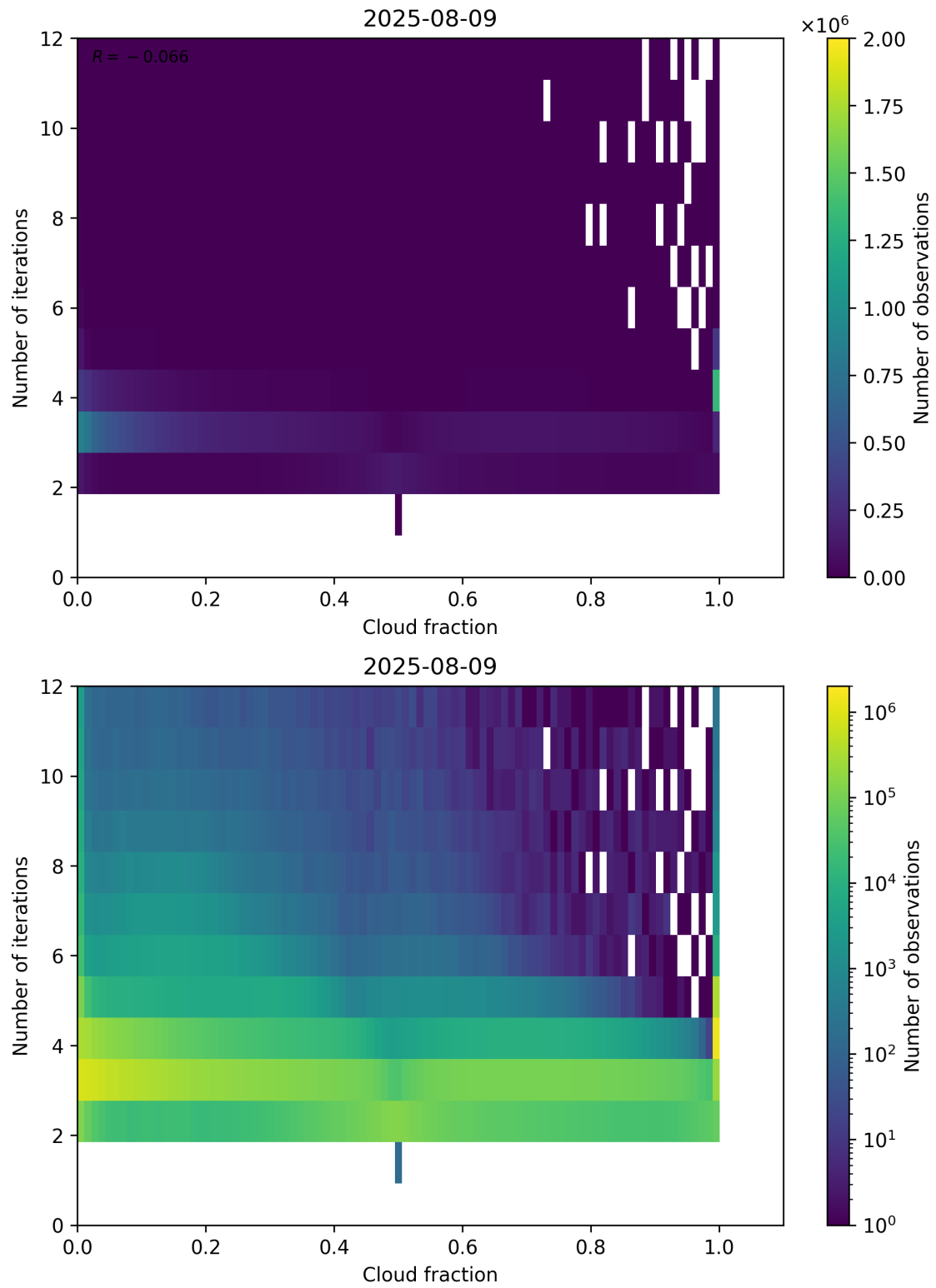
Figure 73: Scatter density plot of “Cloud fraction” against “Number of iterations” for 2025-08-09 to 2025-08-10.
