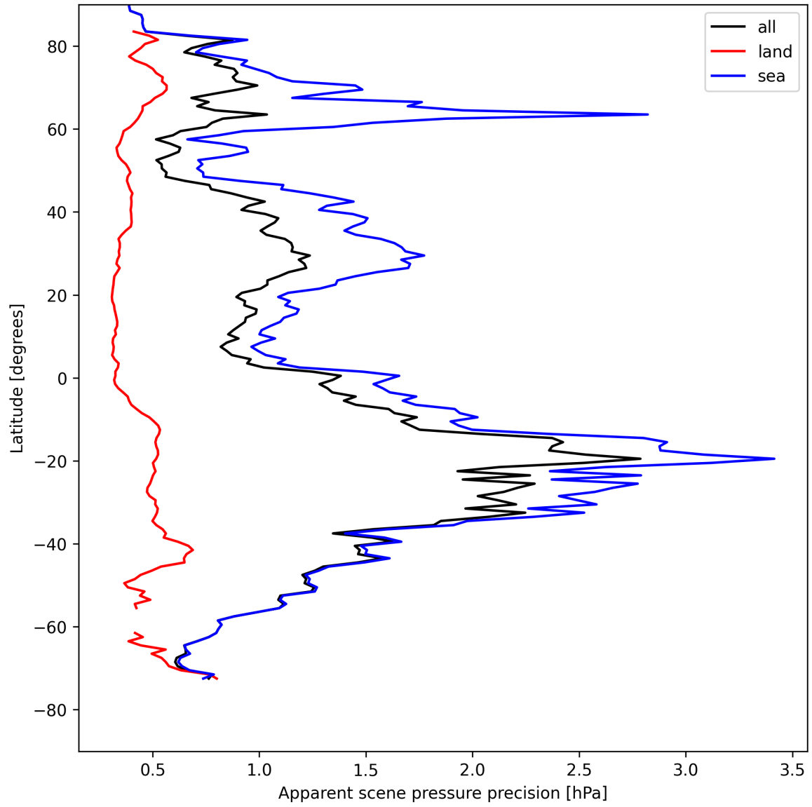
Figure 20: Zonal average of “Apparent scene pressure precision” for 2025-08-09 to 2025-08-10.
