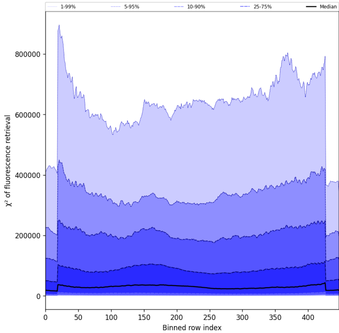
Figure 59: Along track statistics of “ \chi^2 of fluorescence retrieval” for 2025-08-09 to 2025-08-10
