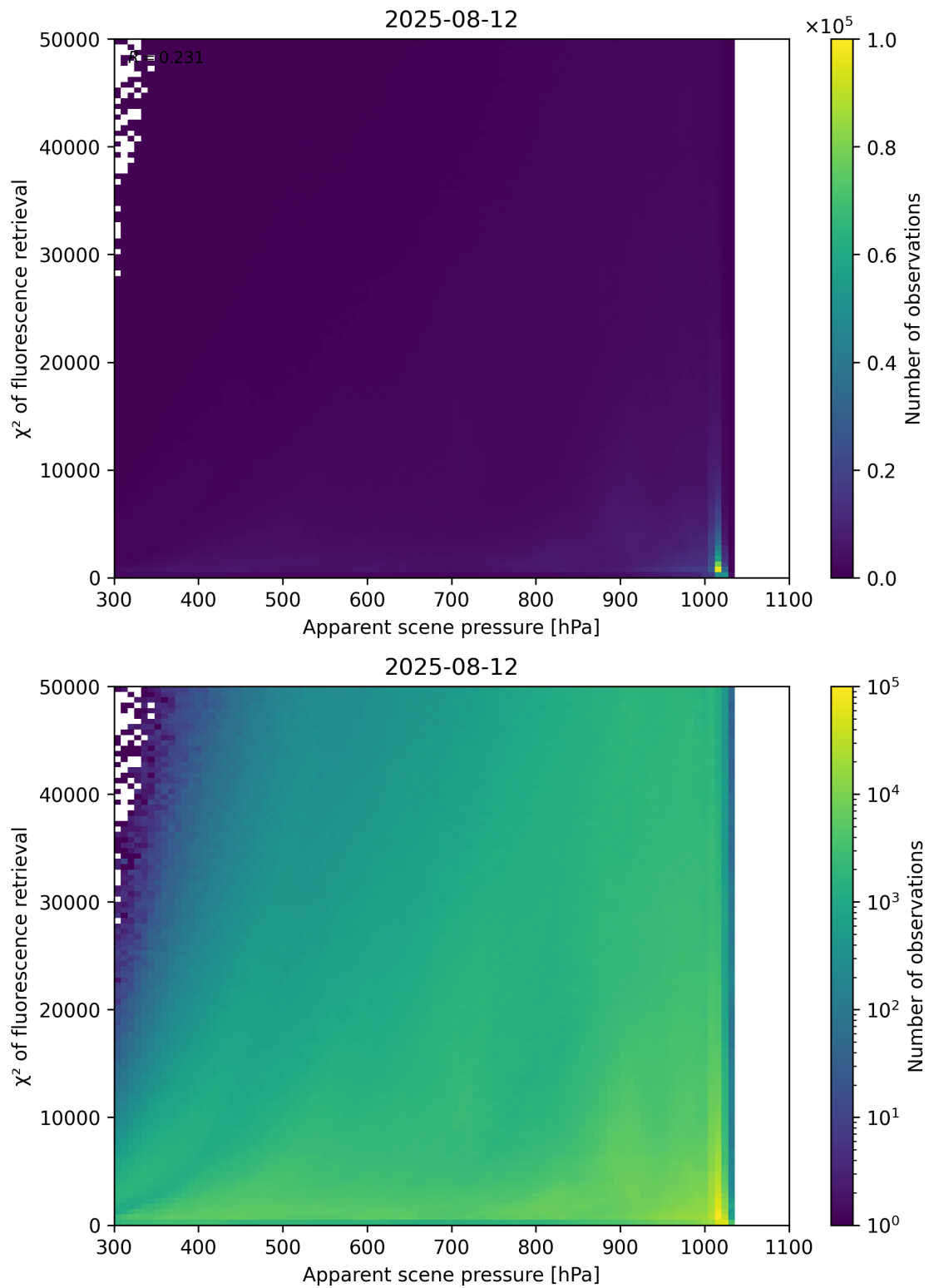
Figure 63: Scatter density plot of “Apparent scene pressure” against “ \chi^2 of fluorescence retrieval” for 2025-08-11 to 2025-08-13.
