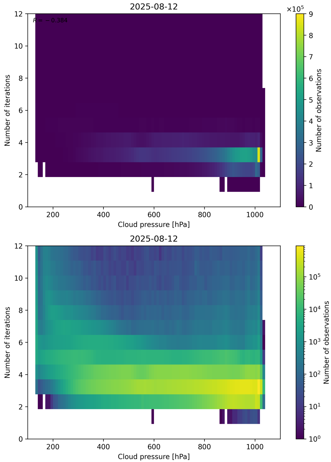
Figure 81: Scatter density plot of “Cloud pressure” against “Number of iterations” for 2025-08-11 to 2025-08-13.
