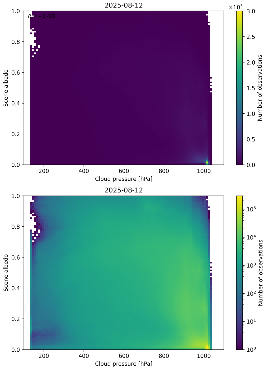
Figure 83: Scatter density plot of “Cloud pressure” against “Scene albedo” for 2025-08-11 to 2025-08-13.
