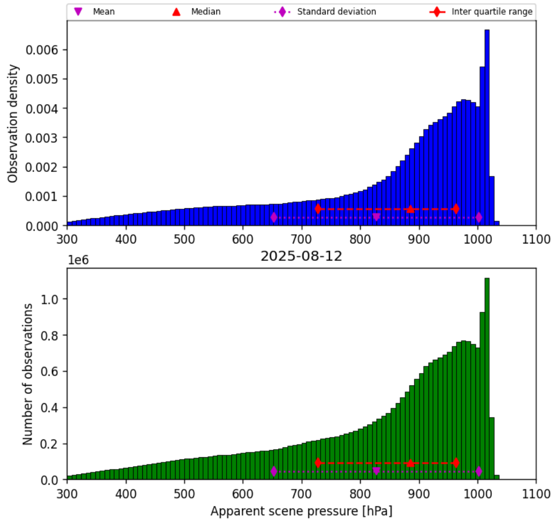
Figure 36: Histogram of “Apparent scene pressure” for 2025-08-11 to 2025-08-13
