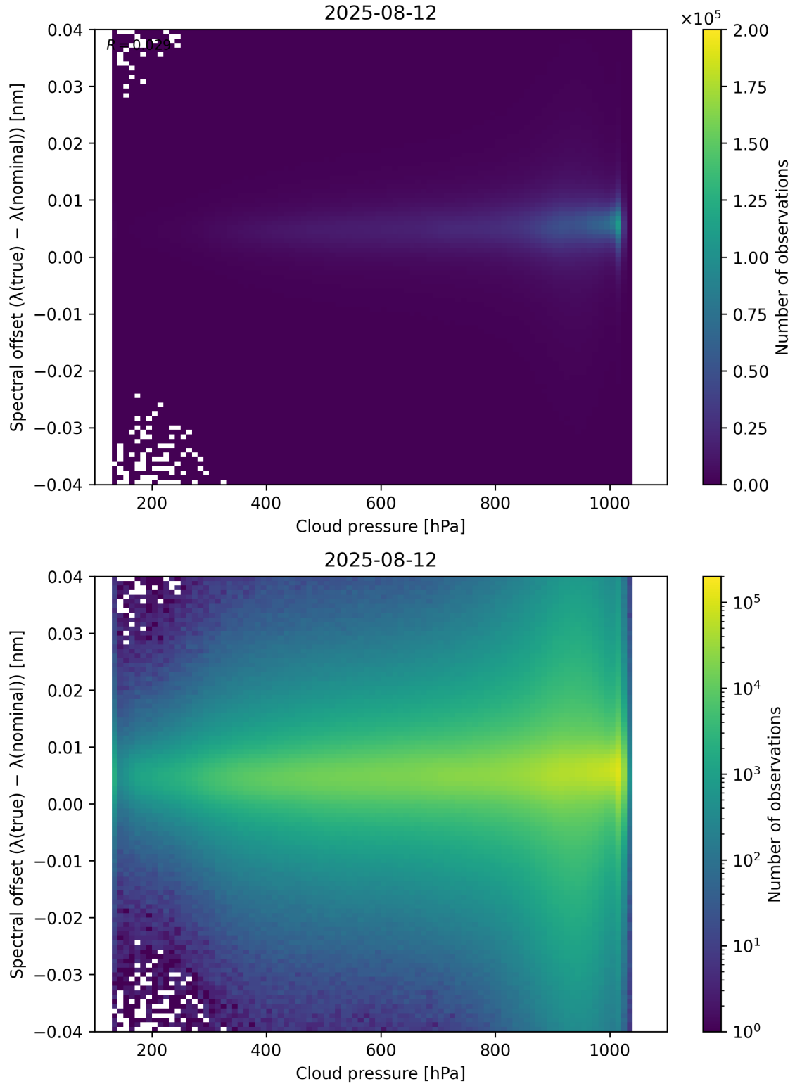
Figure 84: Scatter density plot of “Cloud pressure” against “Spectral offset ( \lambda_{\text{true}} - \lambda_{\text{nominal}} )” for 2025-08-11 to 2025-08-13.
