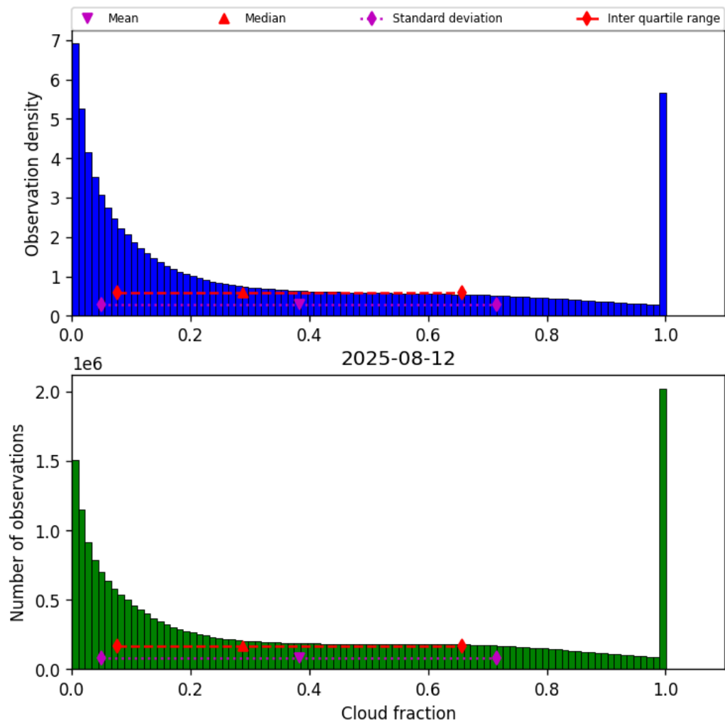
Figure 32: Histogram of “Cloud fraction” for 2025-08-11 to 2025-08-13
