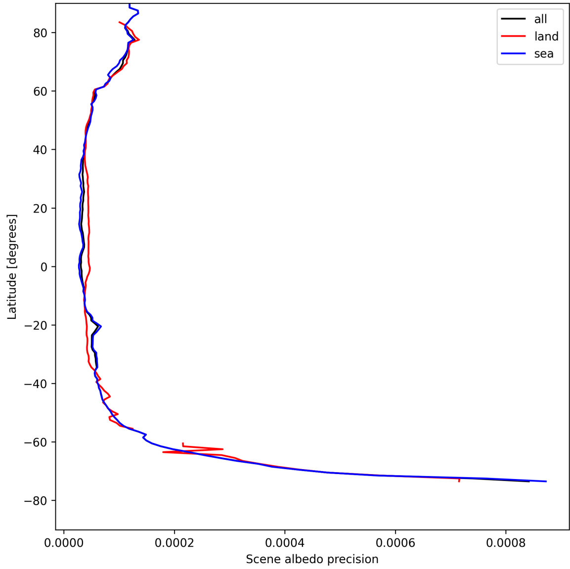
Figure 18: Zonal average of “Scene albedo precision” for 2025-08-11 to 2025-08-13.
