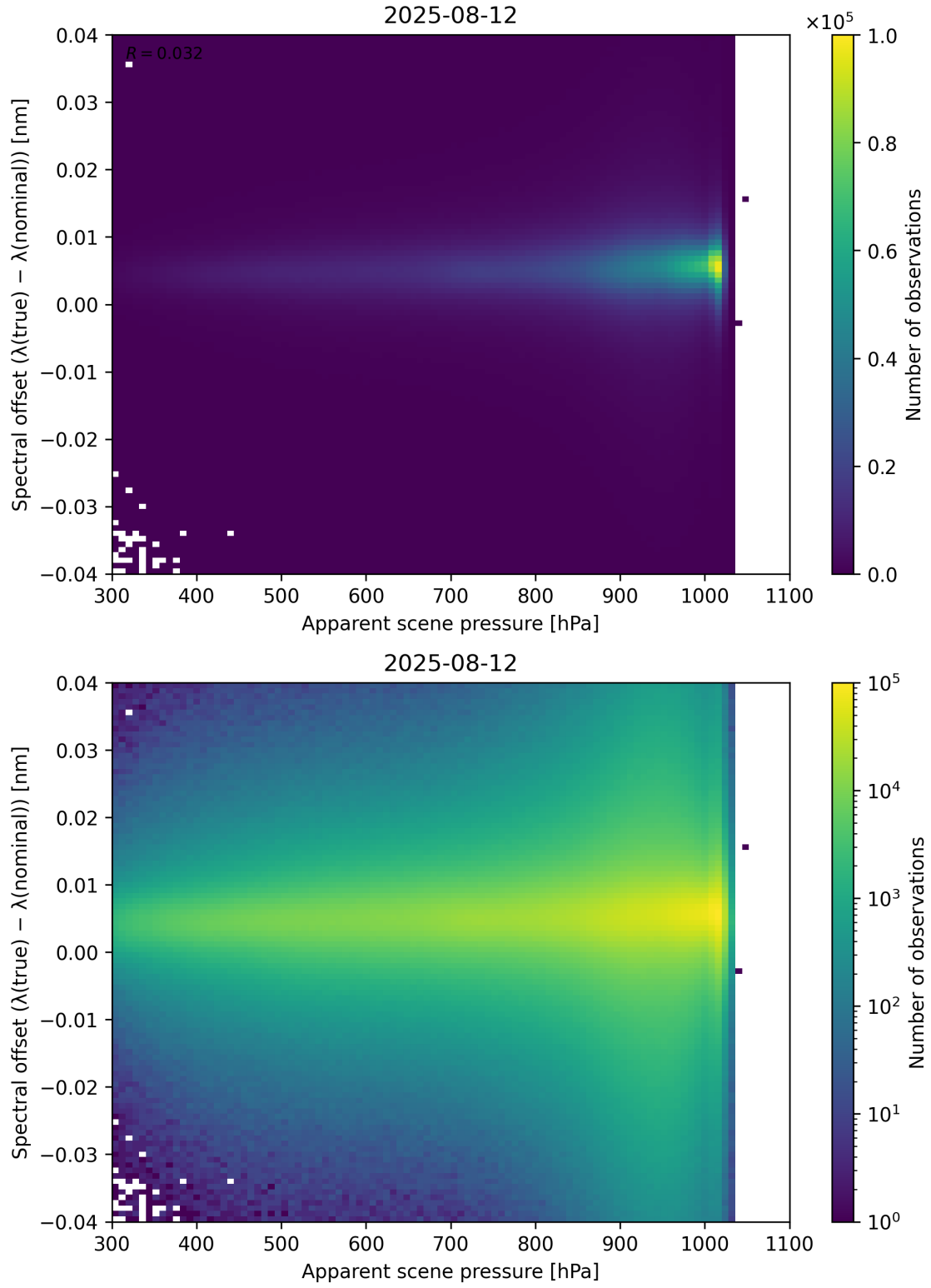
Figure 67: Scatter density plot of “Apparent scene pressure” against “Spectral offset ( \lambda_{\text{true}} - \lambda_{\text{nominal}} )” for 2025-08-11 to 2025-08-13.
