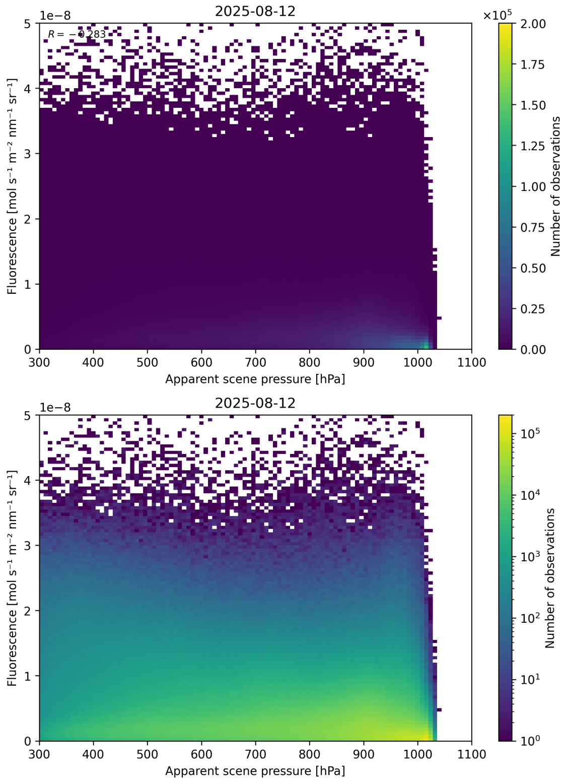
Figure 64: Scatter density plot of “Apparent scene pressure” against “Fluorescence” for 2025-08-11 to 2025-08-13.
