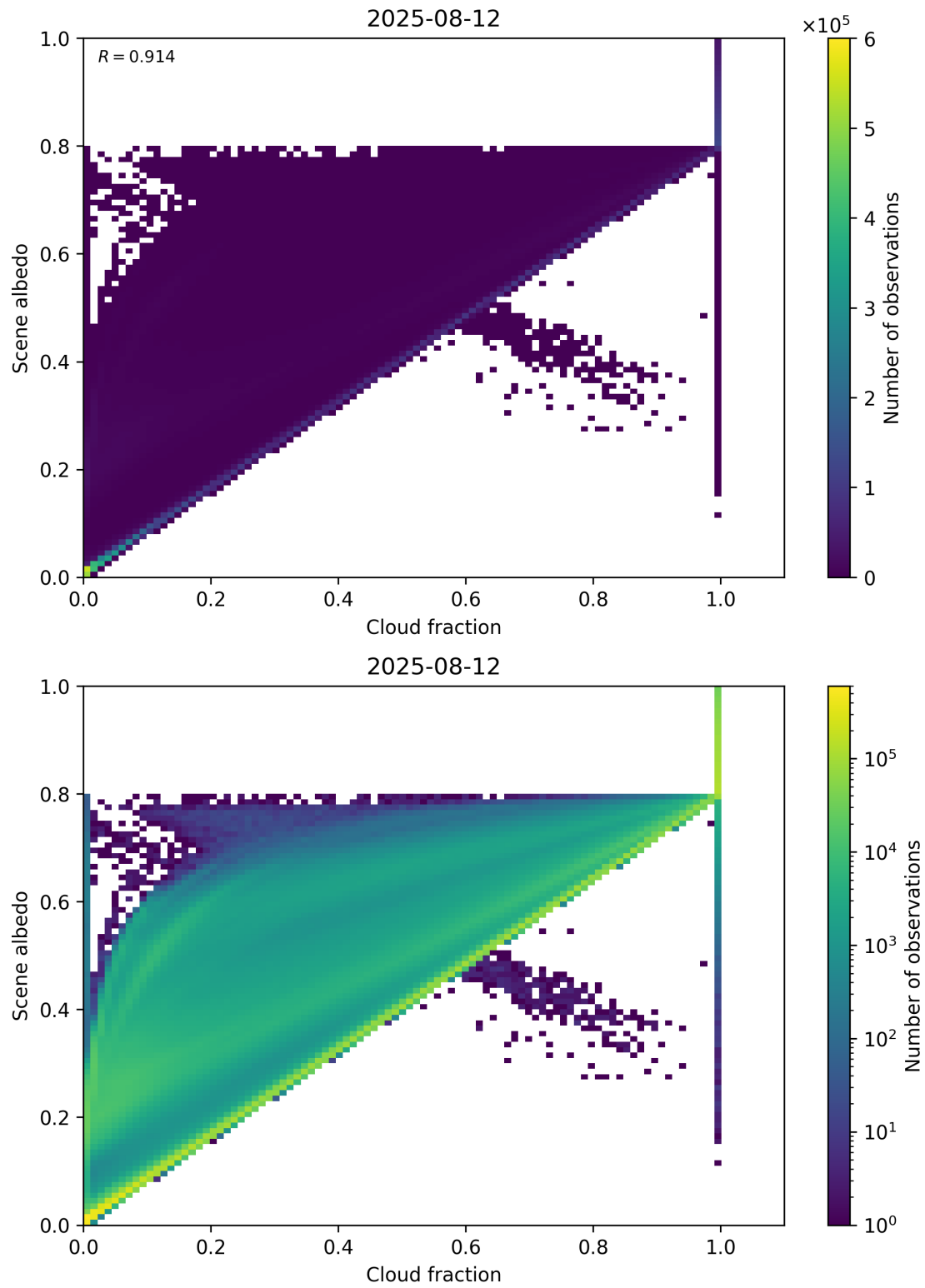
Figure 75: Scatter density plot of “Cloud fraction” against “Scene albedo” for 2025-08-11 to 2025-08-13.
