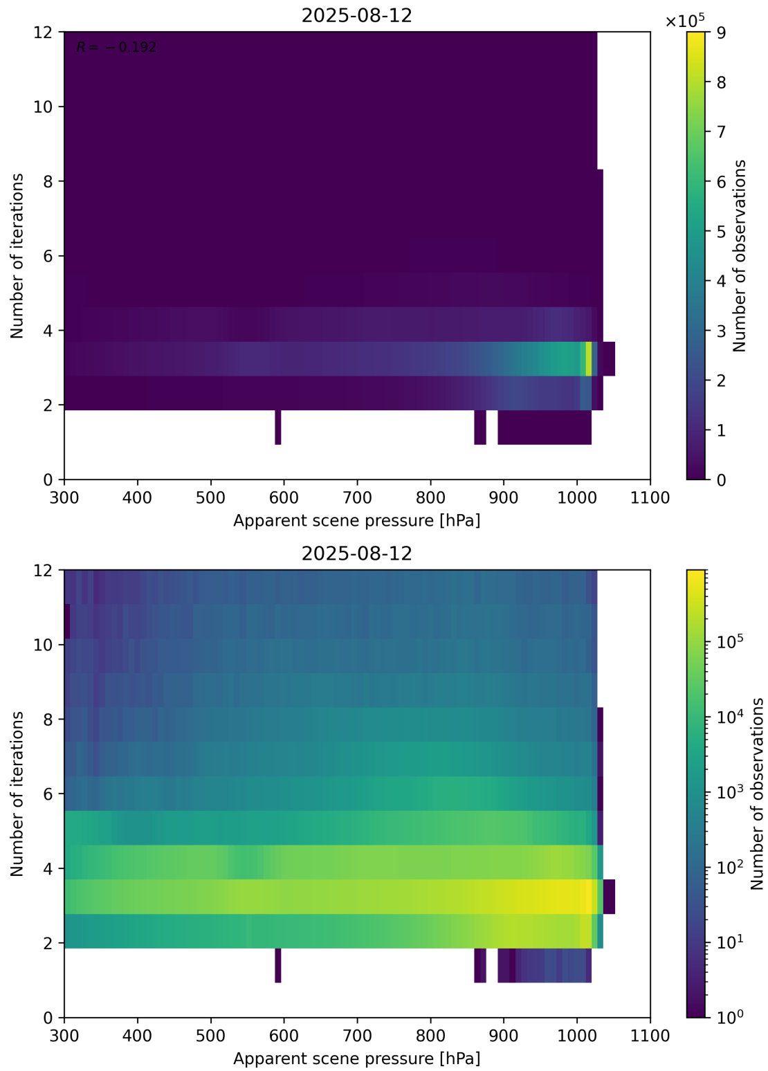
Figure 65: Scatter density plot of “Apparent scene pressure” against “Number of iterations” for 2025-08-11 to 2025-08-13.
