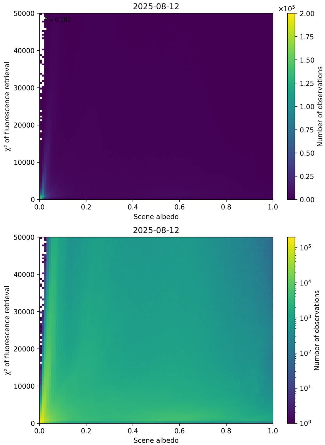
Figure 103: Scatter density plot of “Scene albedo” against “ \chi^2 of fluorescence retrieval” for 2025-08-11 to 2025-08-13.
