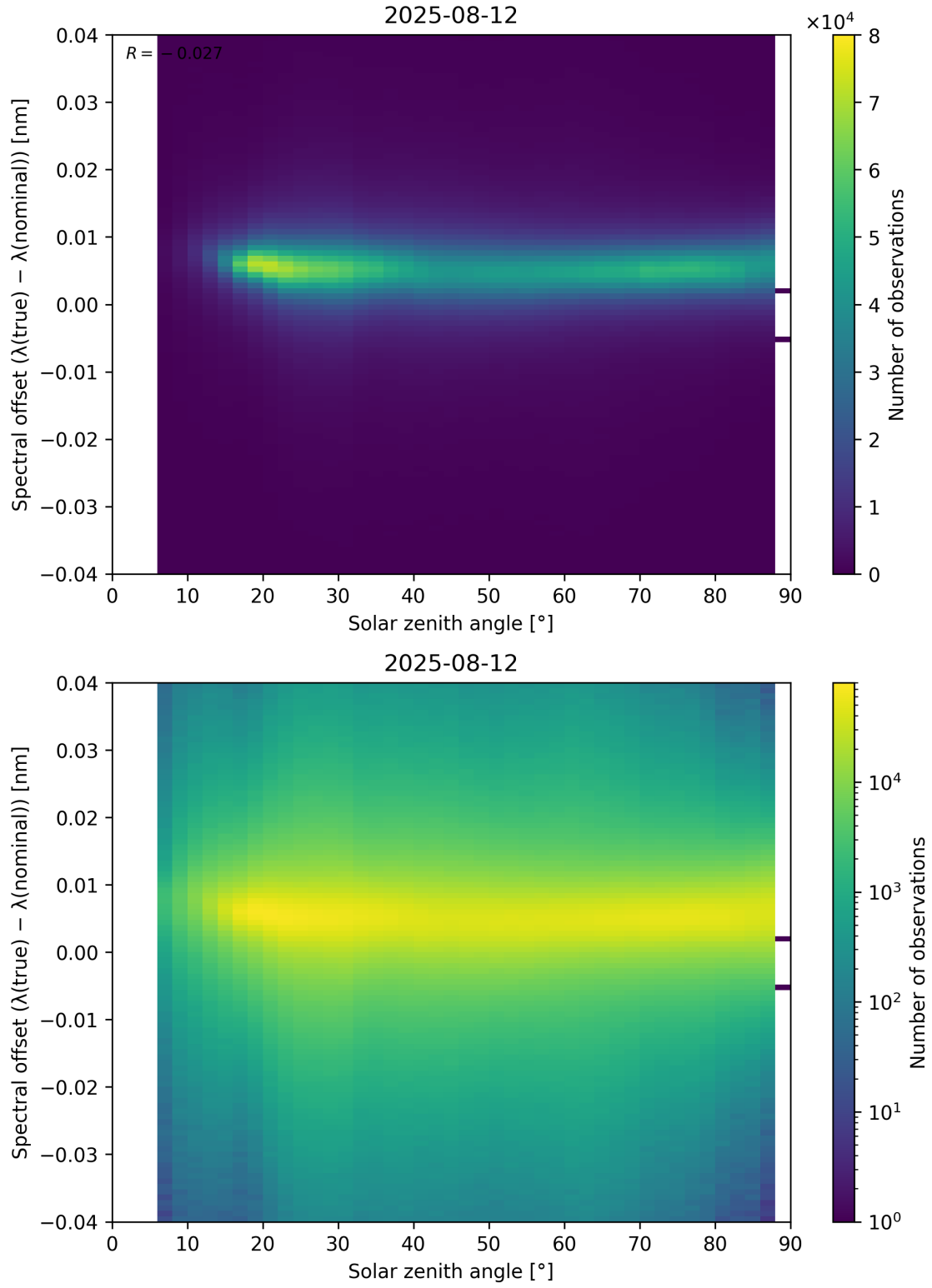
Figure 117: Scatter density plot of “Solar zenith angle” against “Spectral offset ( \lambda_{\text{true}} - \lambda_{\text{nominal}} )” for 2025-08-11 to 2025-08-13.
