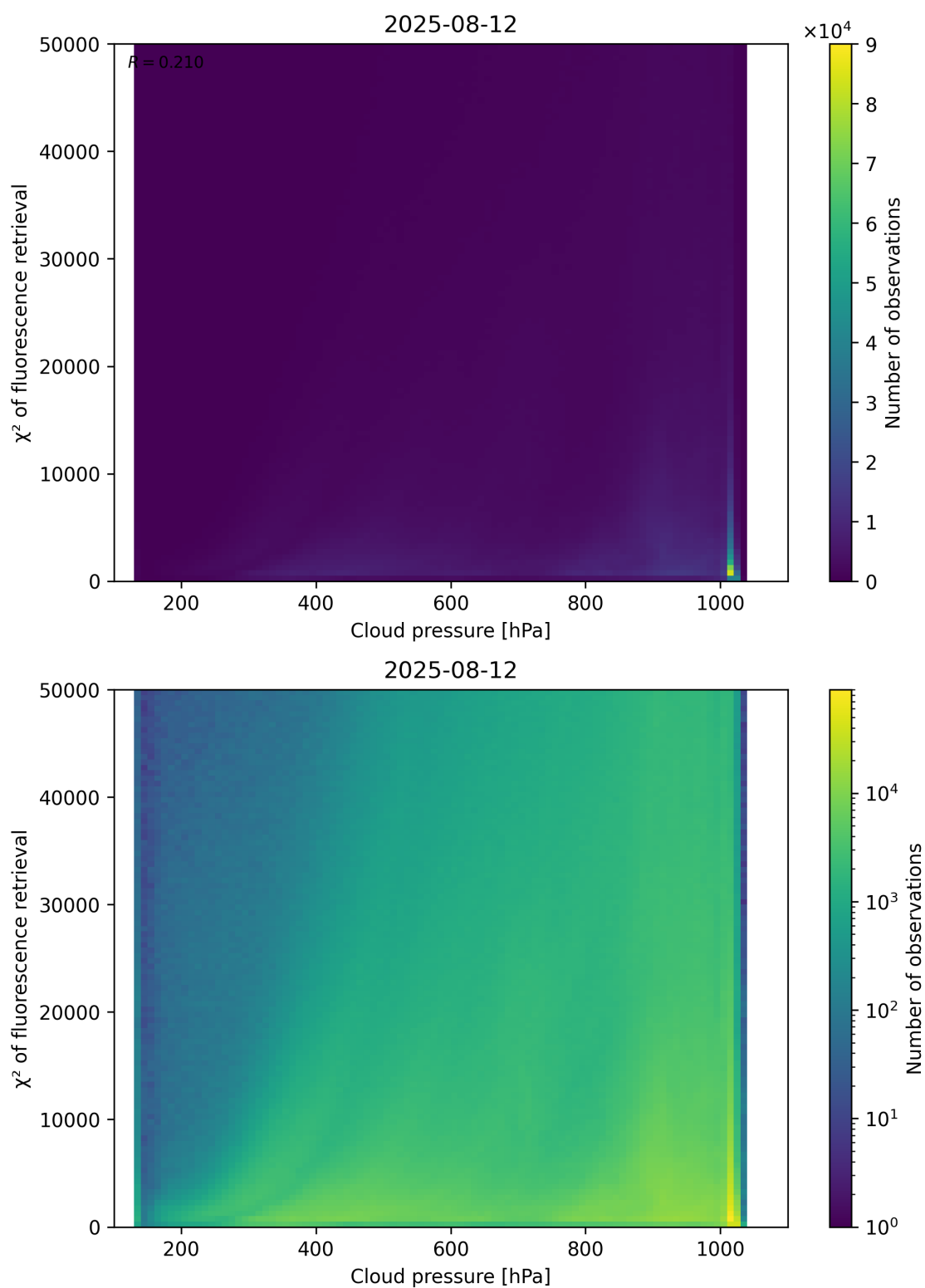
Figure 78: Scatter density plot of “Cloud pressure” against “ \chi^2 of fluorescence retrieval” for 2025-08-11 to 2025-08-13.
