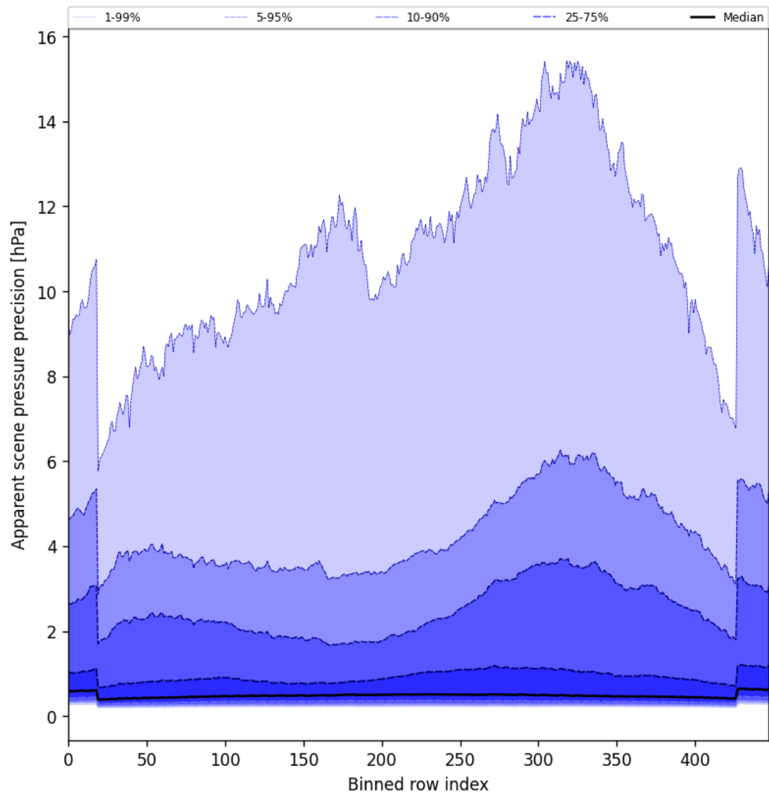
Figure 54: Along track statistics of “Apparent scene pressure precision” for 2025-08-11 to 2025-08-13
