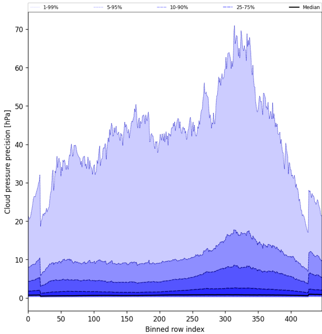
Figure 48: Along track statistics of “Cloud pressure precision” for 2025-08-11 to 2025-08-13
