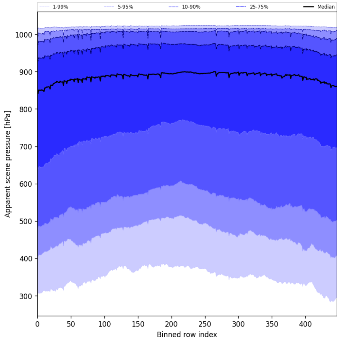
Figure 53: Along track statistics of “Apparent scene pressure” for 2025-08-11 to 2025-08-13
