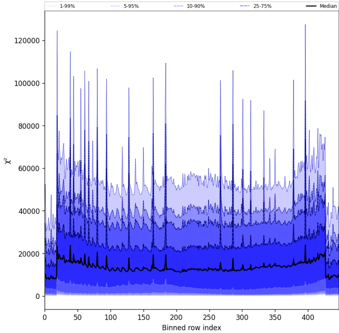
Figure 55: Along track statistics of “ \chi^2 ” for 2025-08-11 to 2025-08-13
