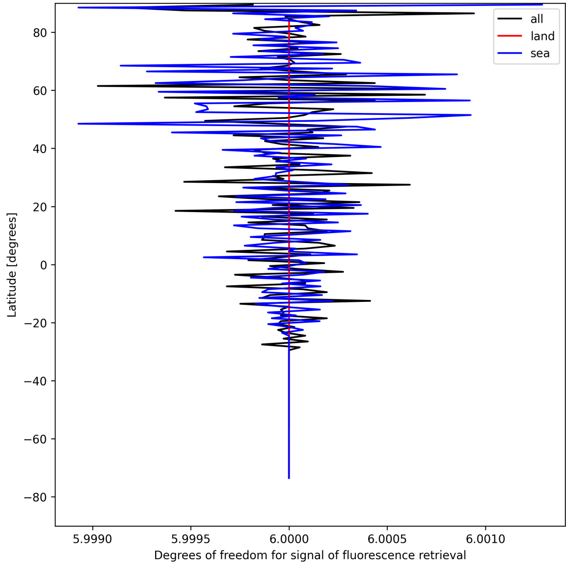
Figure 26: Zonal average of “Degrees of freedom for signal of fluorescence retrieval” for 2025-08-11 to 2025-08-13.
