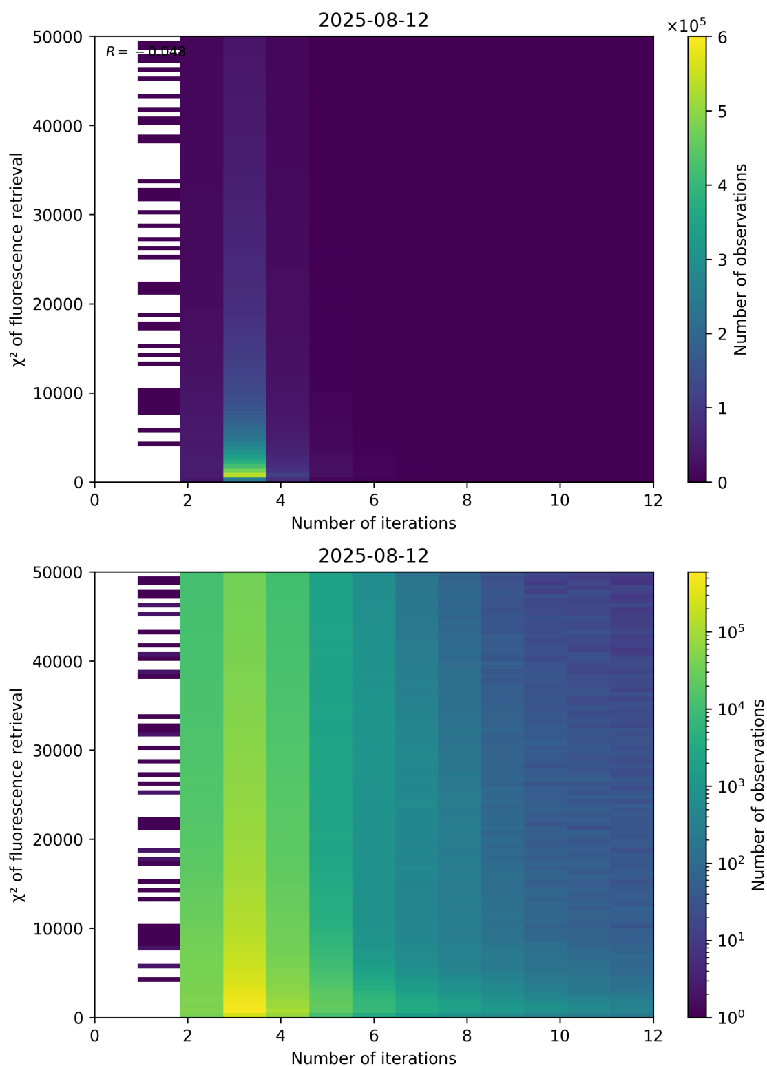
Figure 97: Scatter density plot of “Number of iterations” against “ \chi^2 of fluorescence retrieval” for 2025-08-11 to 2025-08-13.
