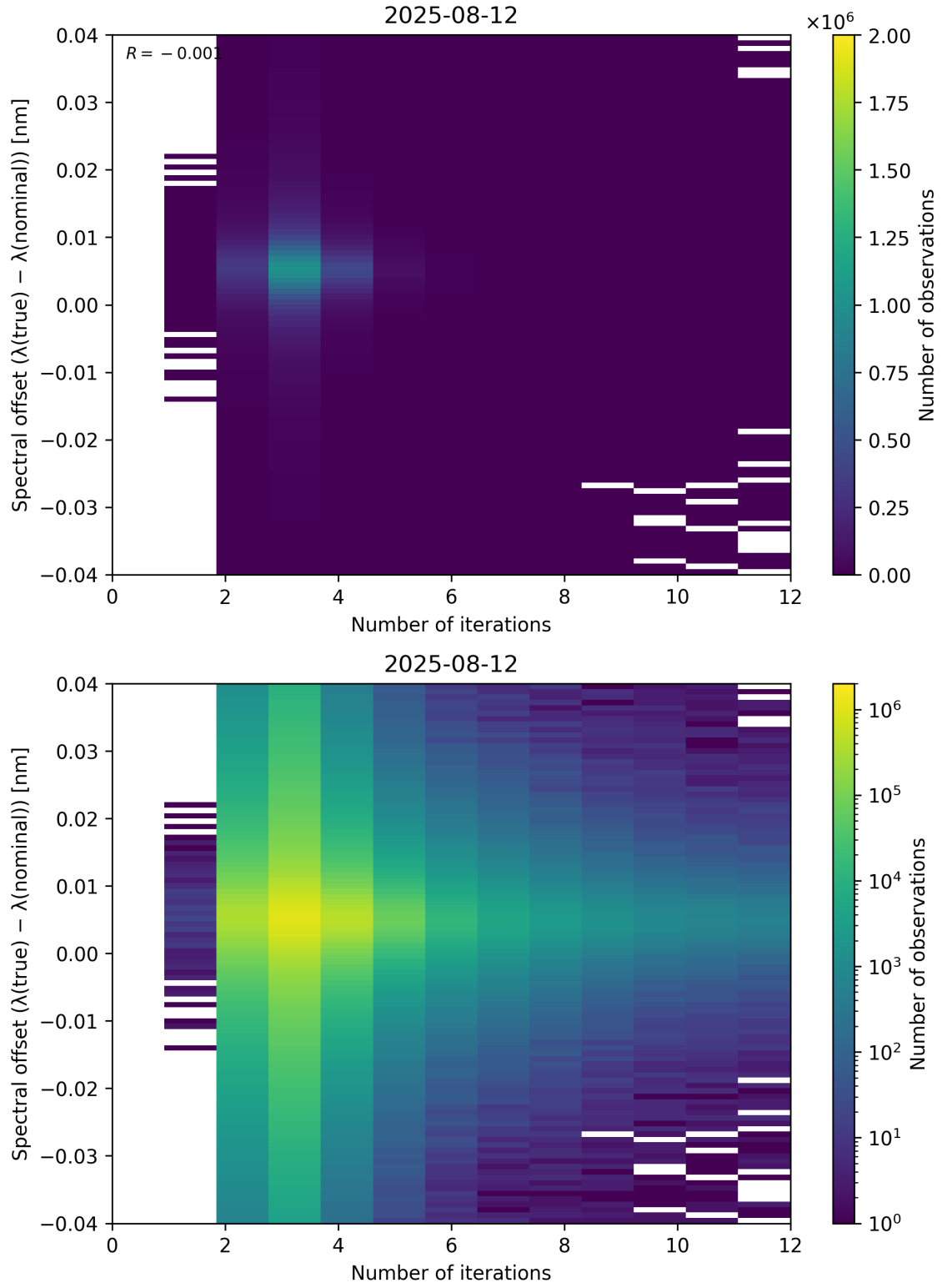
Figure 100: Scatter density plot of “Number of iterations” against “Spectral offset ( \lambda_{\text{true}} - \lambda_{\text{nominal}} )” for 2025-08-11 to 2025-08-13.
