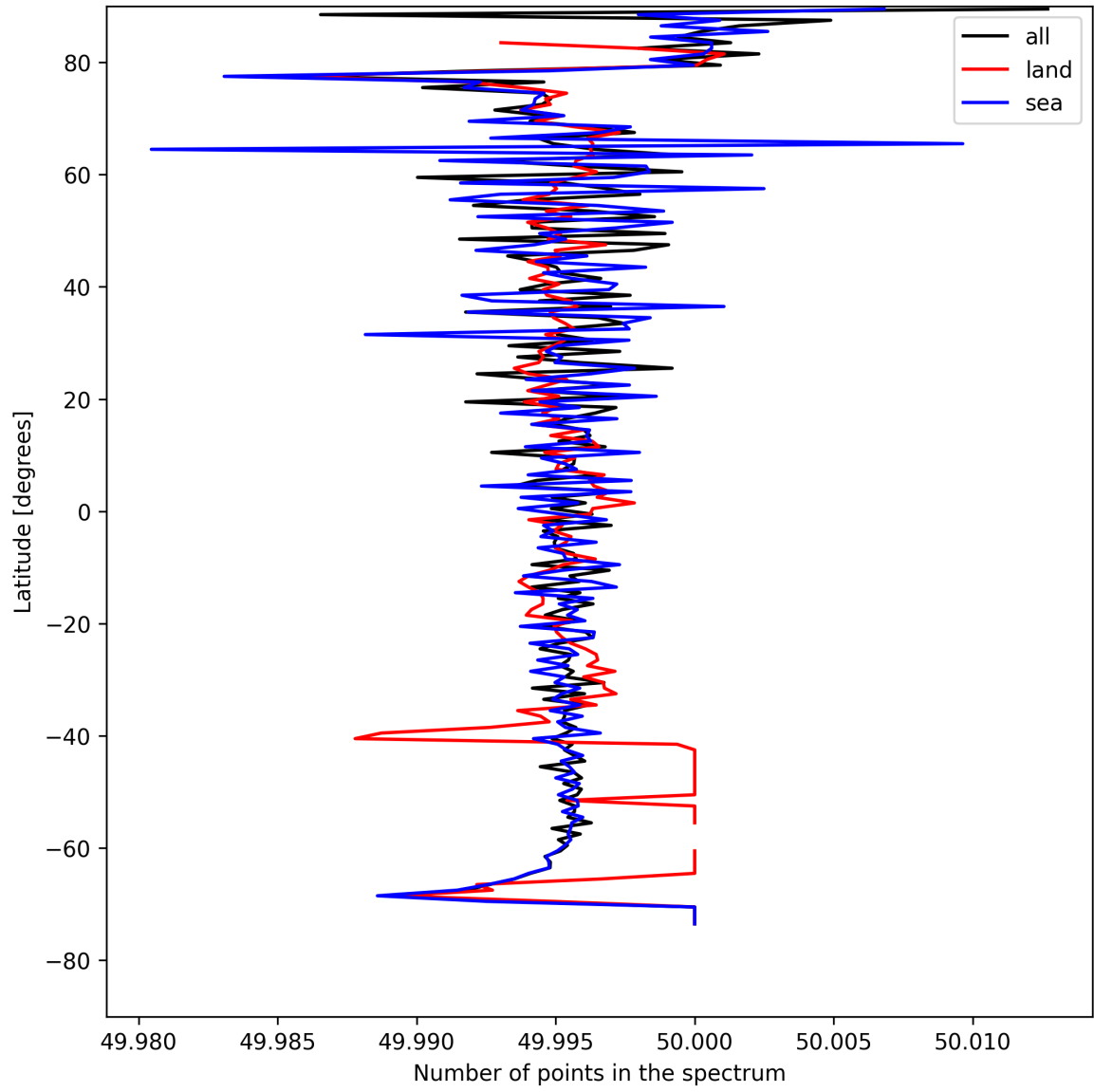
Figure 27: Zonal average of “Number of points in the spectrum” for 2025-08-11 to 2025-08-13.
