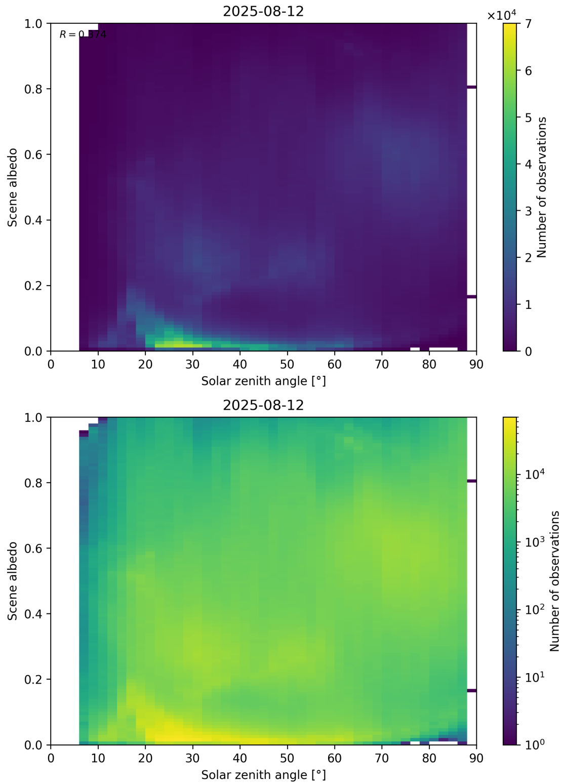
Figure 116: Scatter density plot of “Solar zenith angle” against “Scene albedo” for 2025-08-11 to 2025-08-13.
