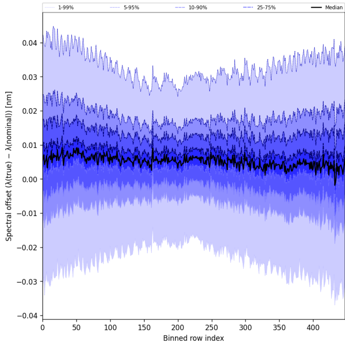
Figure 62: Along track statistics of “Spectral offset ( \lambda_{\text{true}} - \lambda_{\text{nominal}} )” for 2025-08-11 to 2025-08-13
