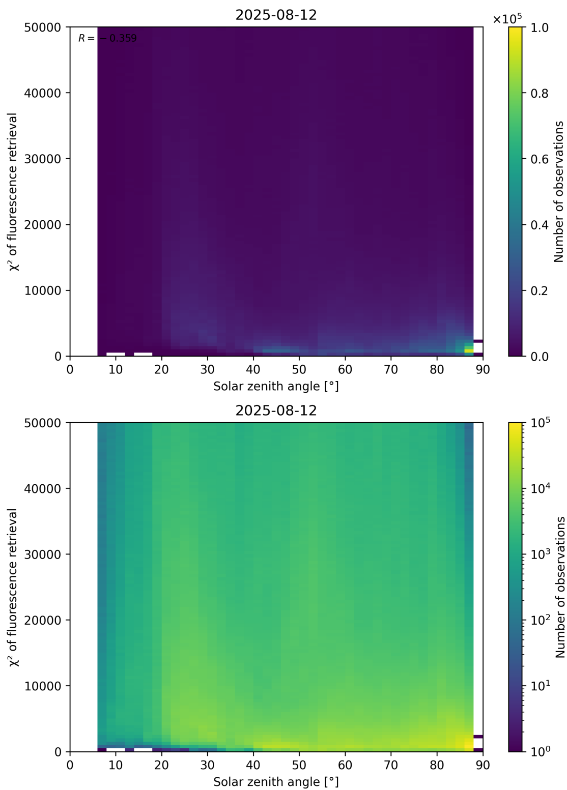
Figure 109: Scatter density plot of “Solar zenith angle” against “ \chi^2 of fluorescence retrieval” for 2025-08-11 to 2025-08-13.
