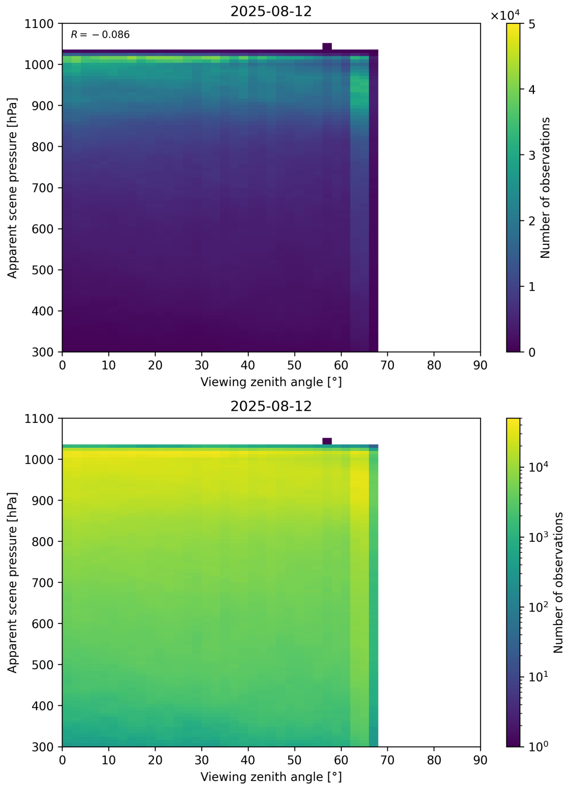
Figure 118: Scatter density plot of “Viewing zenith angle” against “Apparent scene pressure” for 2025-08-11 to 2025-08-13.
