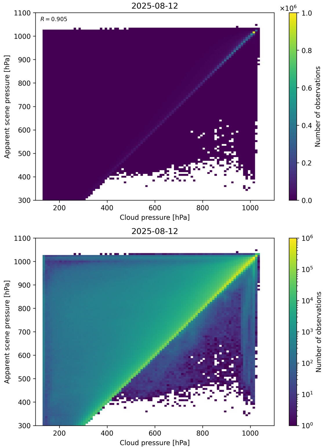
Figure 77: Scatter density plot of “Cloud pressure” against “Apparent scene pressure” for 2025-08-11 to 2025-08-13.
