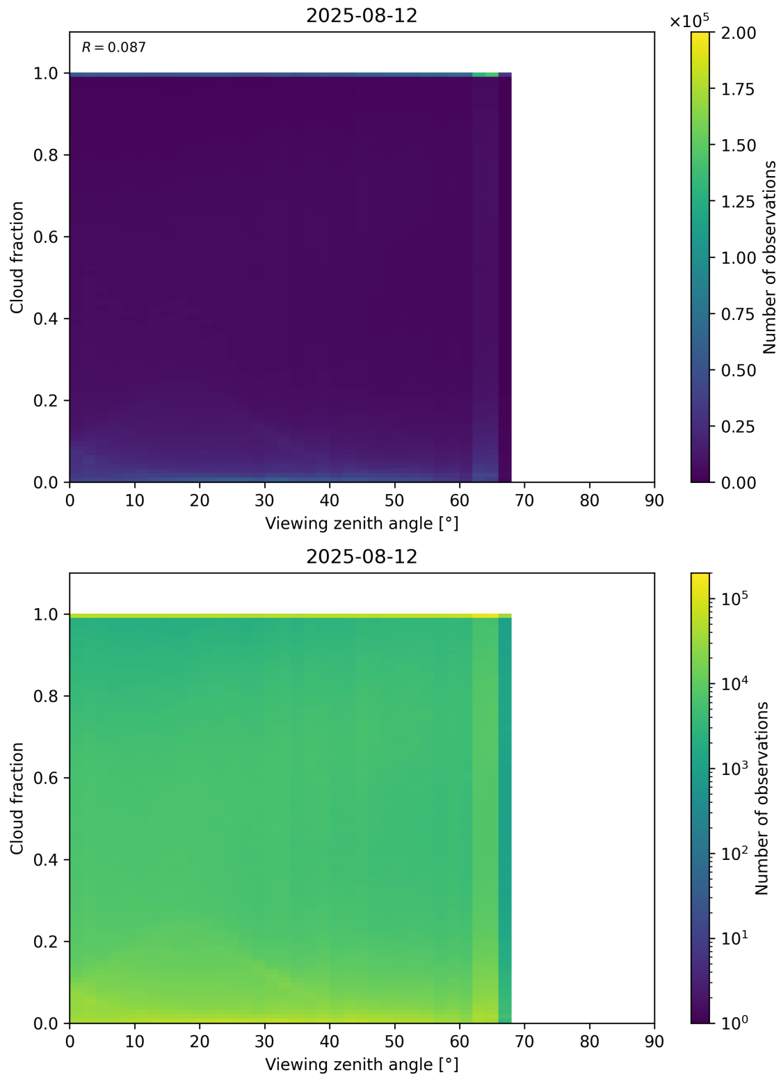
Figure 120: Scatter density plot of “Viewing zenith angle” against “Cloud fraction” for 2025-08-11 to 2025-08-13.
