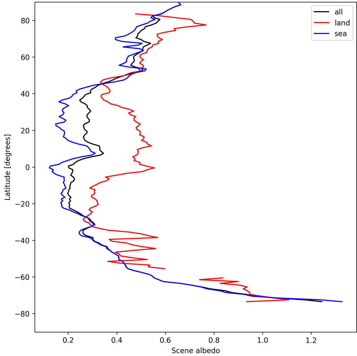
Figure 17: Zonal average of “Scene albedo” for 2025-08-11 to 2025-08-13.
