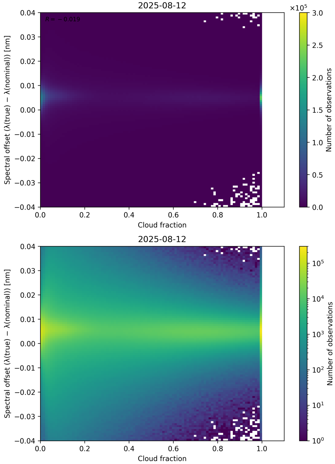
Figure 76: Scatter density plot of “Cloud fraction” against “Spectral offset ( \lambda_{\text{true}} - \lambda_{\text{nominal}} )” for 2025-08-11 to 2025-08-13.
