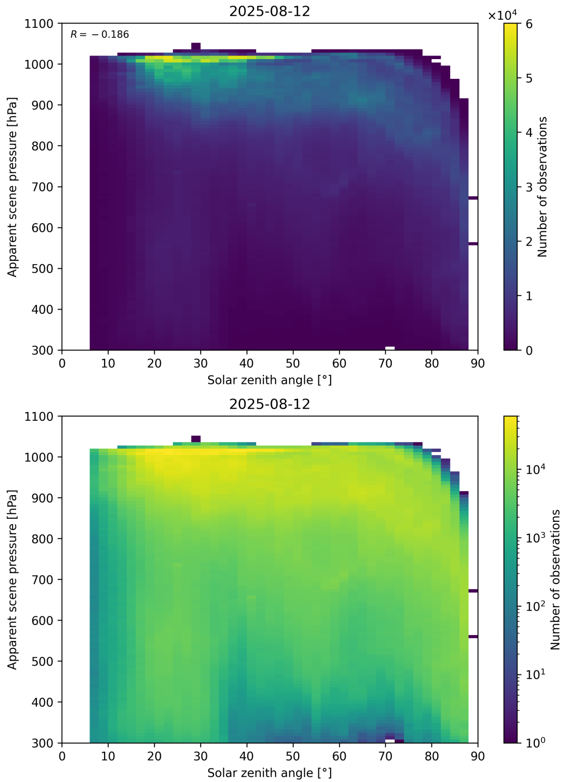
Figure 108: Scatter density plot of “Solar zenith angle” against “Apparent scene pressure” for 2025-08-11 to 2025-08-13.
