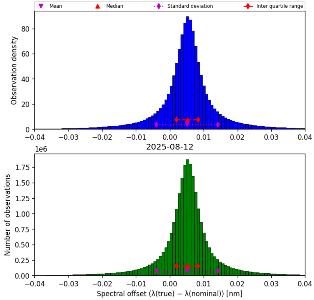
Figure 45: Histogram of “Spectral offset ( \lambda_{\text{true}} - \lambda_{\text{nominal}} )” for 2025-08-11 to 2025-08-13
