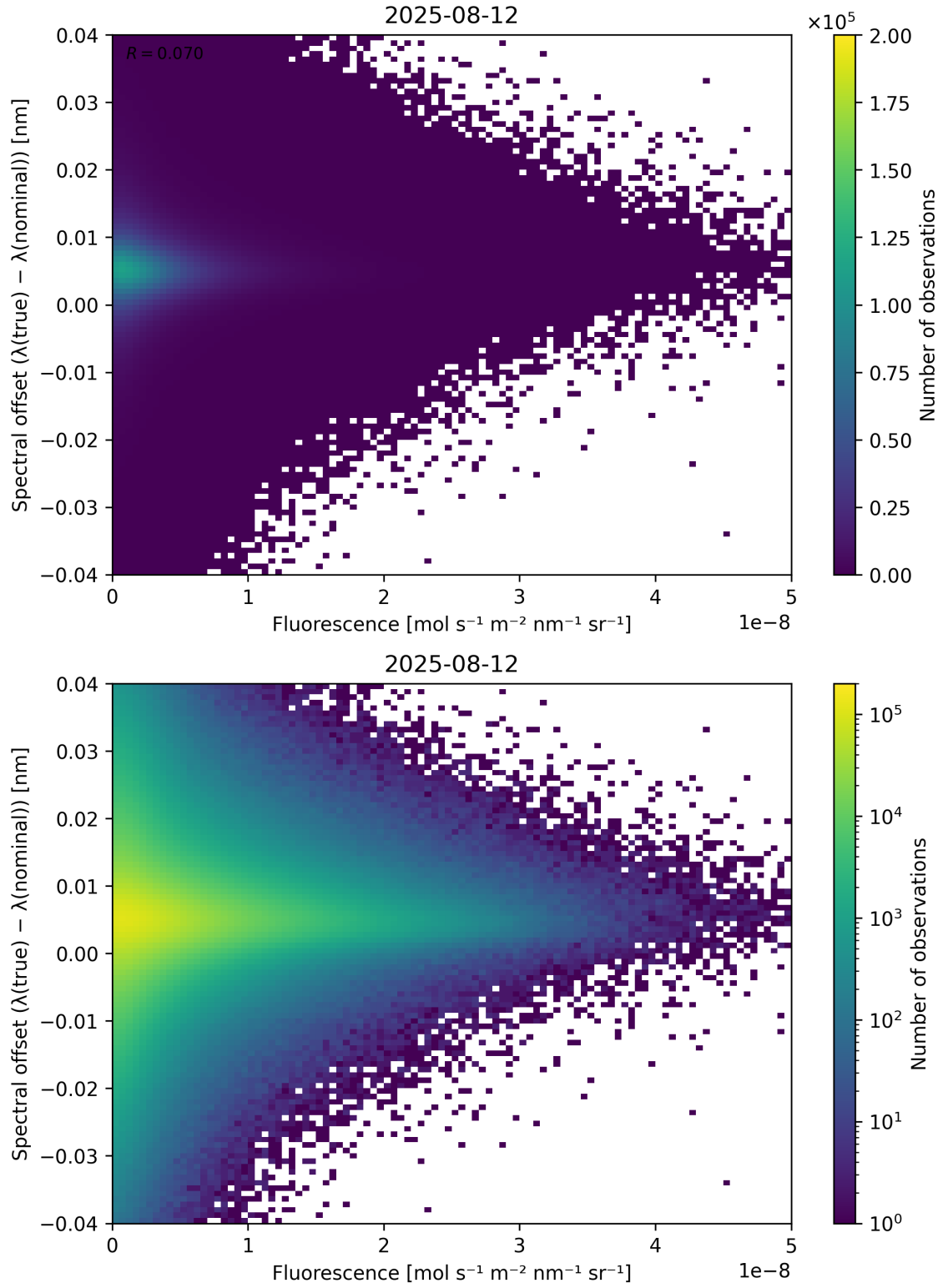
Figure 87: Scatter density plot of “Fluorescence” against “Spectral offset ( \lambda_{\text{true}} - \lambda_{\text{nominal}} )” for 2025-08-11 to 2025-08-13.
