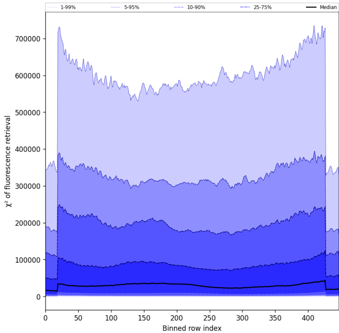
Figure 59: Along track statistics of “ \chi^2 of fluorescence retrieval” for 2025-08-11 to 2025-08-13
