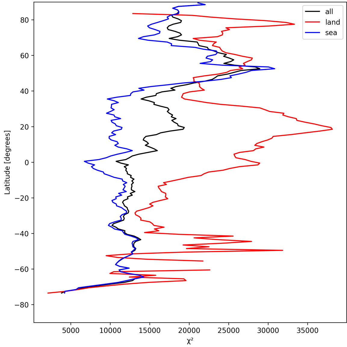
Figure 21: Zonal average of “ \chi^2 ” for 2025-08-11 to 2025-08-13.
