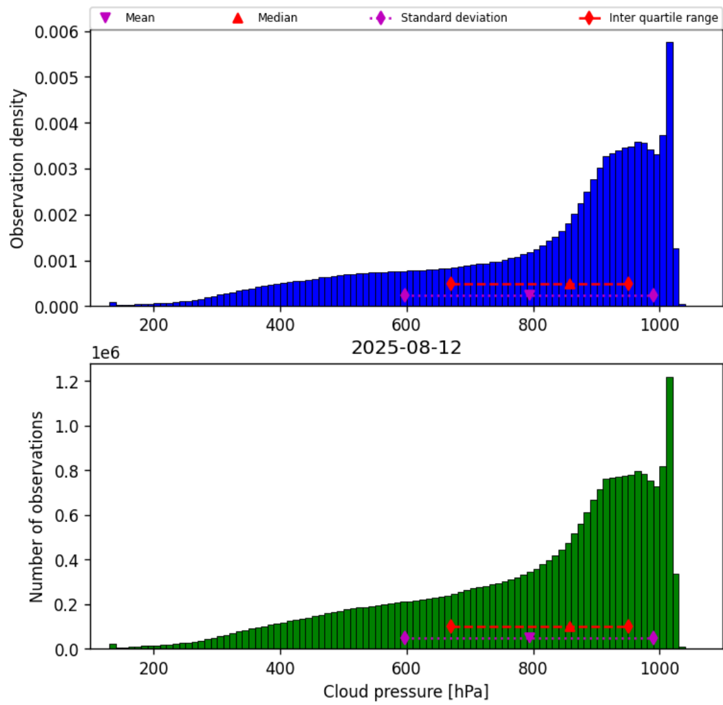
Figure 30: Histogram of “Cloud pressure” for 2025-08-11 to 2025-08-13
