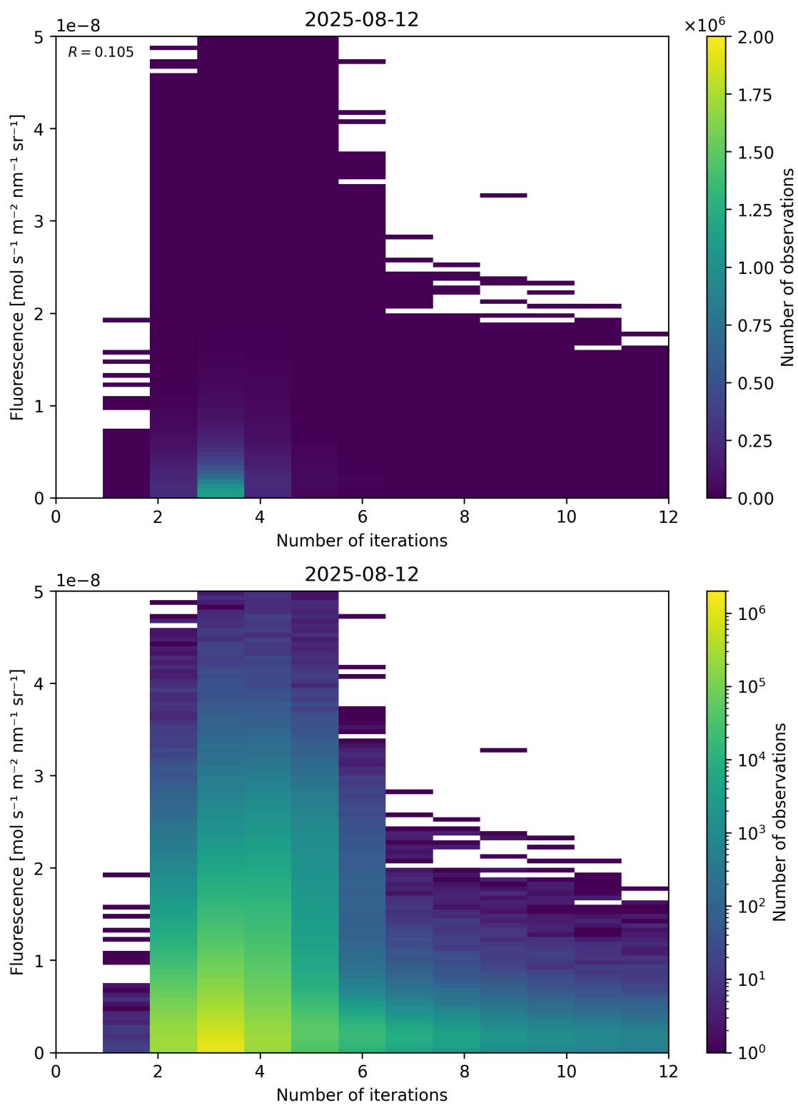
Figure 98: Scatter density plot of “Number of iterations” against “Fluorescence” for 2025-08-11 to 2025-08-13.
