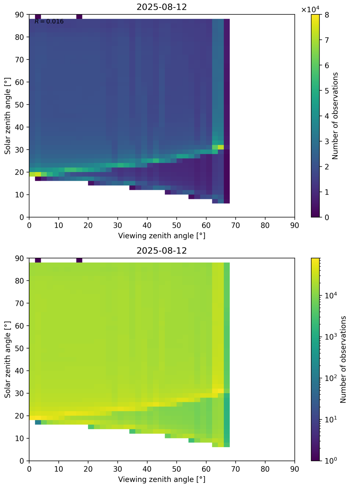
Figure 127: Scatter density plot of “Viewing zenith angle” against “Solar zenith angle” for 2025-08-11 to 2025-08-13.
