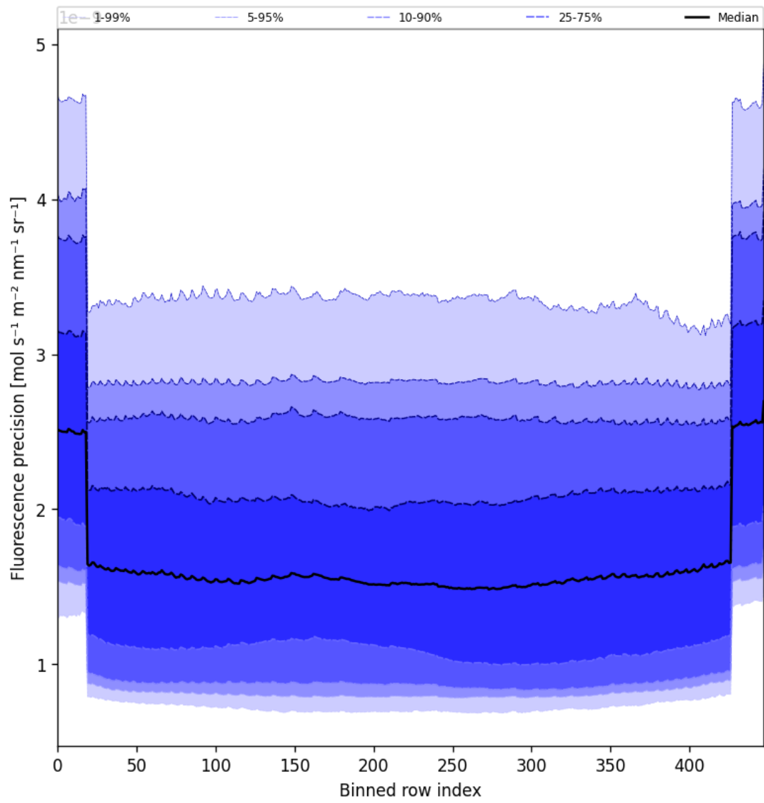
Figure 58: Along track statistics of “Fluorescence precision” for 2025-08-11 to 2025-08-13
