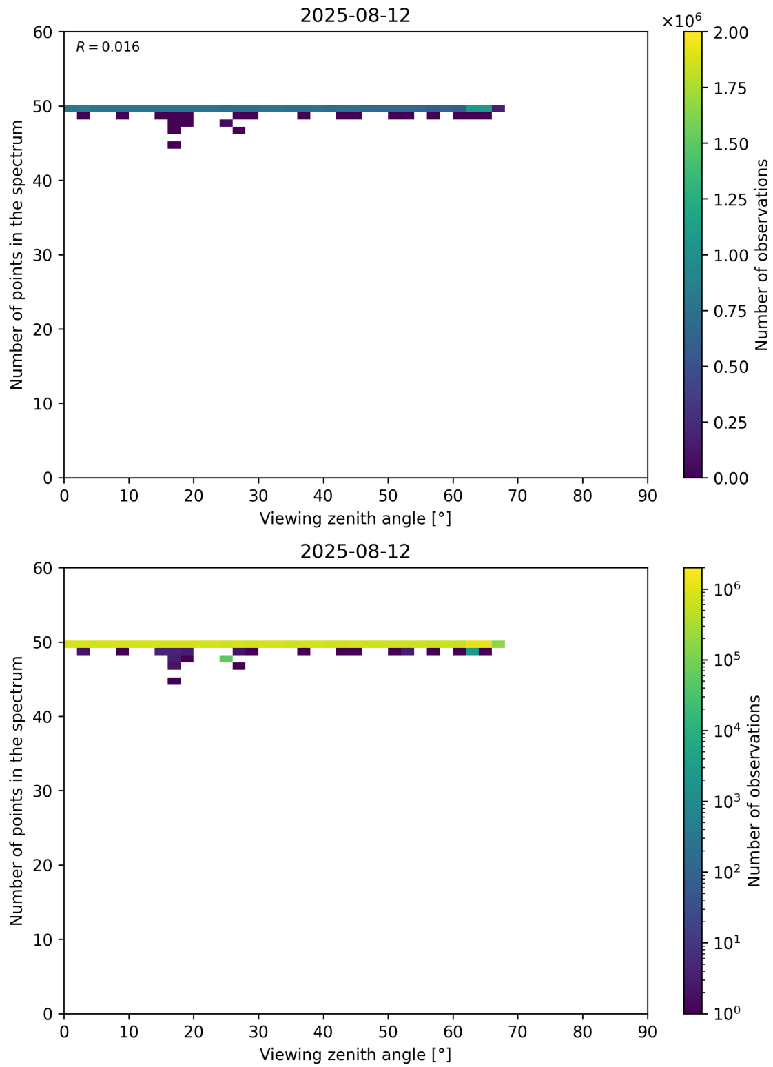
Figure 125: Scatter density plot of “Viewing zenith angle” against “Number of points in the spectrum” for 2025-08-11 to 2025-08-13.
