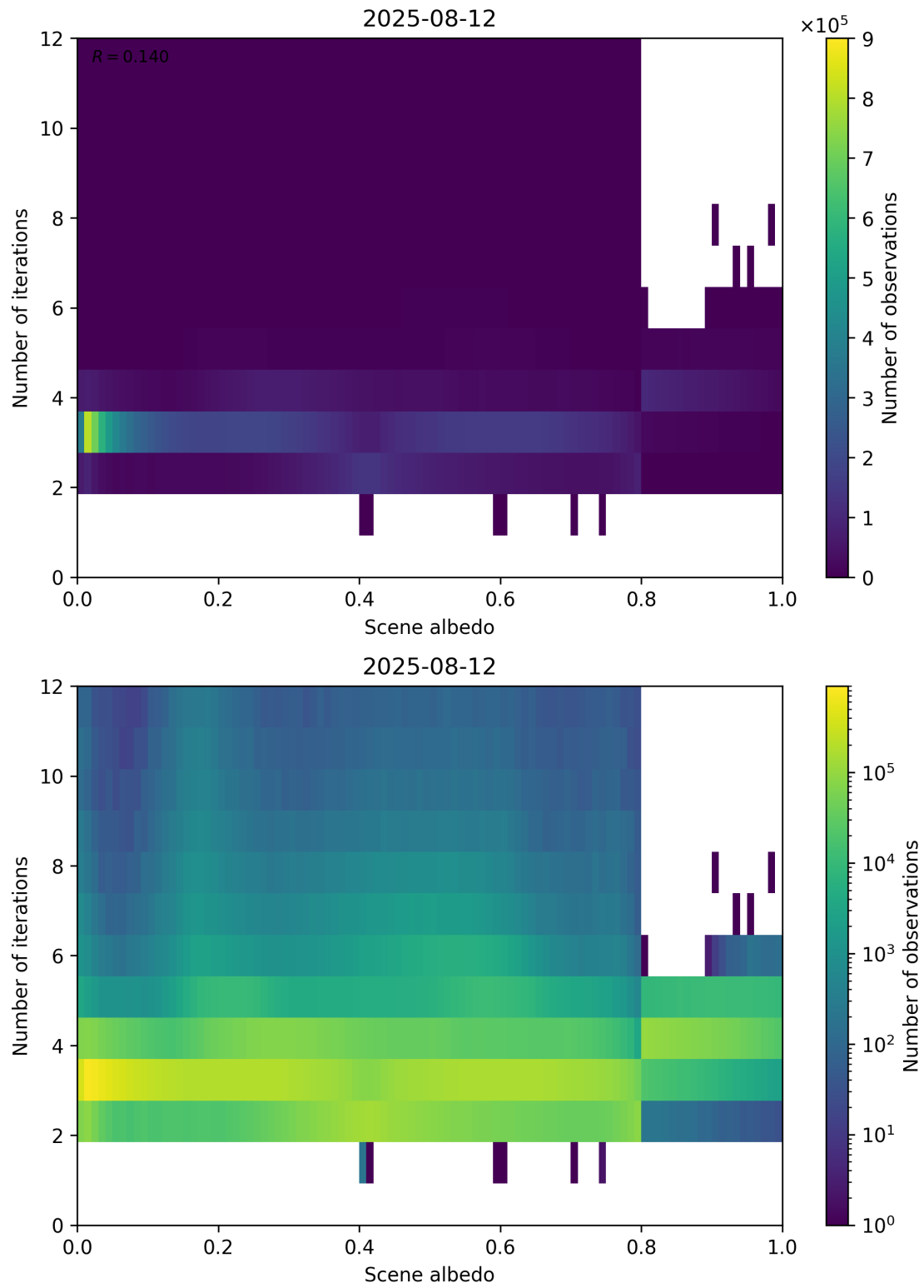
Figure 105: Scatter density plot of “Scene albedo” against “Number of iterations” for 2025-08-11 to 2025-08-13.
