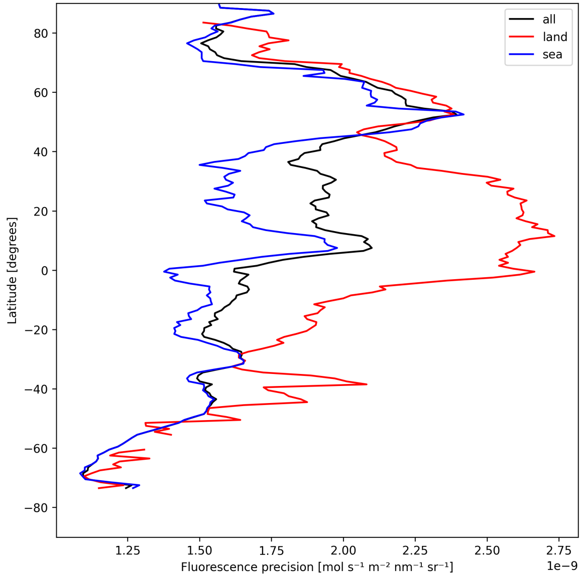
Figure 24: Zonal average of “Fluorescence precision” for 2025-08-11 to 2025-08-13.
