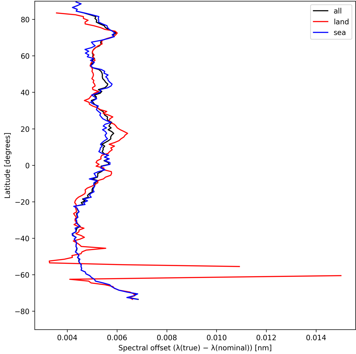
Figure 28: Zonal average of “Spectral offset ( \lambda_{\text{true}} - \lambda_{\text{nominal}} )” for 2025-08-11 to 2025-08-13.
