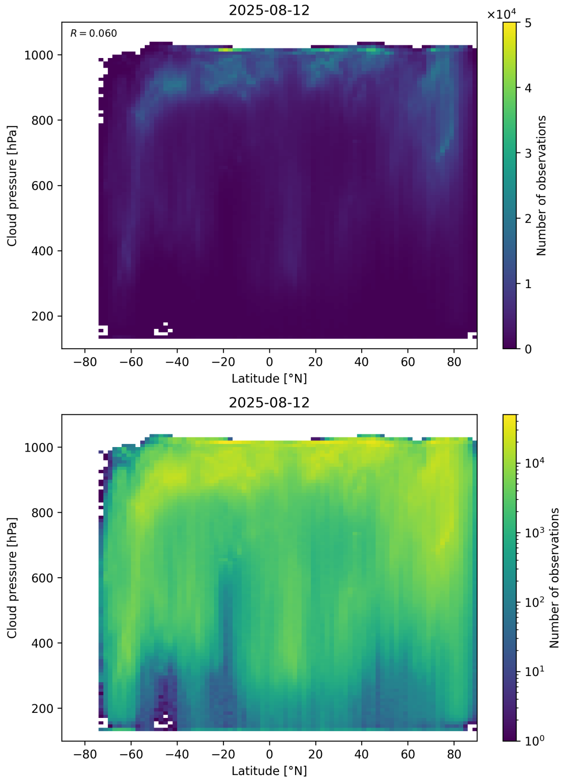
Figure 91: Scatter density plot of “Latitude” against “Cloud pressure” for 2025-08-11 to 2025-08-13.
