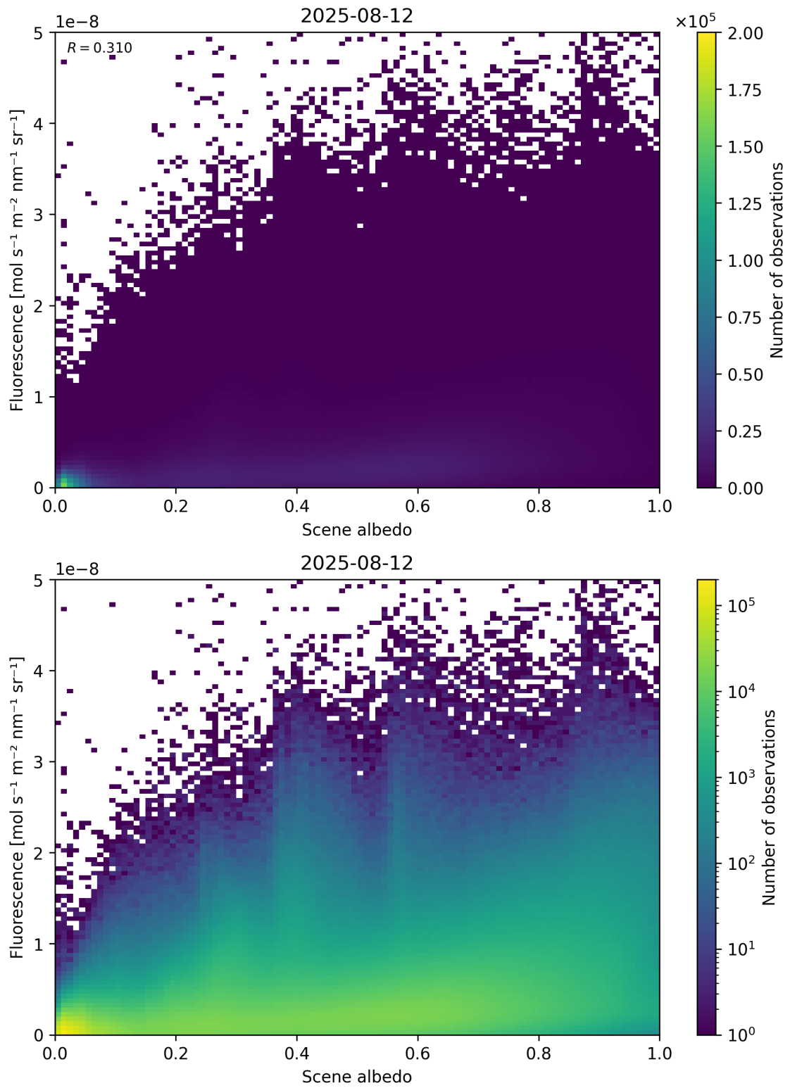
Figure 104: Scatter density plot of “Scene albedo” against “Fluorescence” for 2025-08-11 to 2025-08-13.
