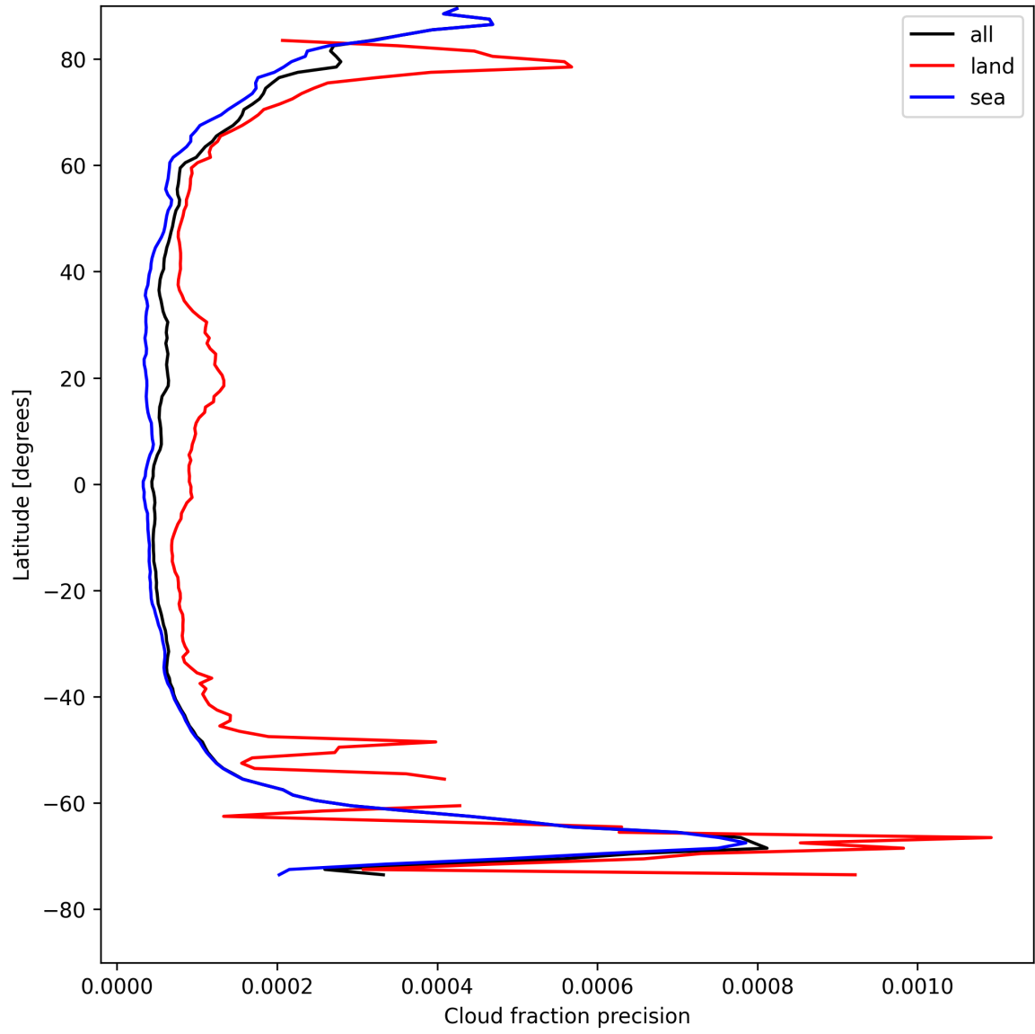
Figure 16: Zonal average of “Cloud fraction precision” for 2025-08-11 to 2025-08-13.
