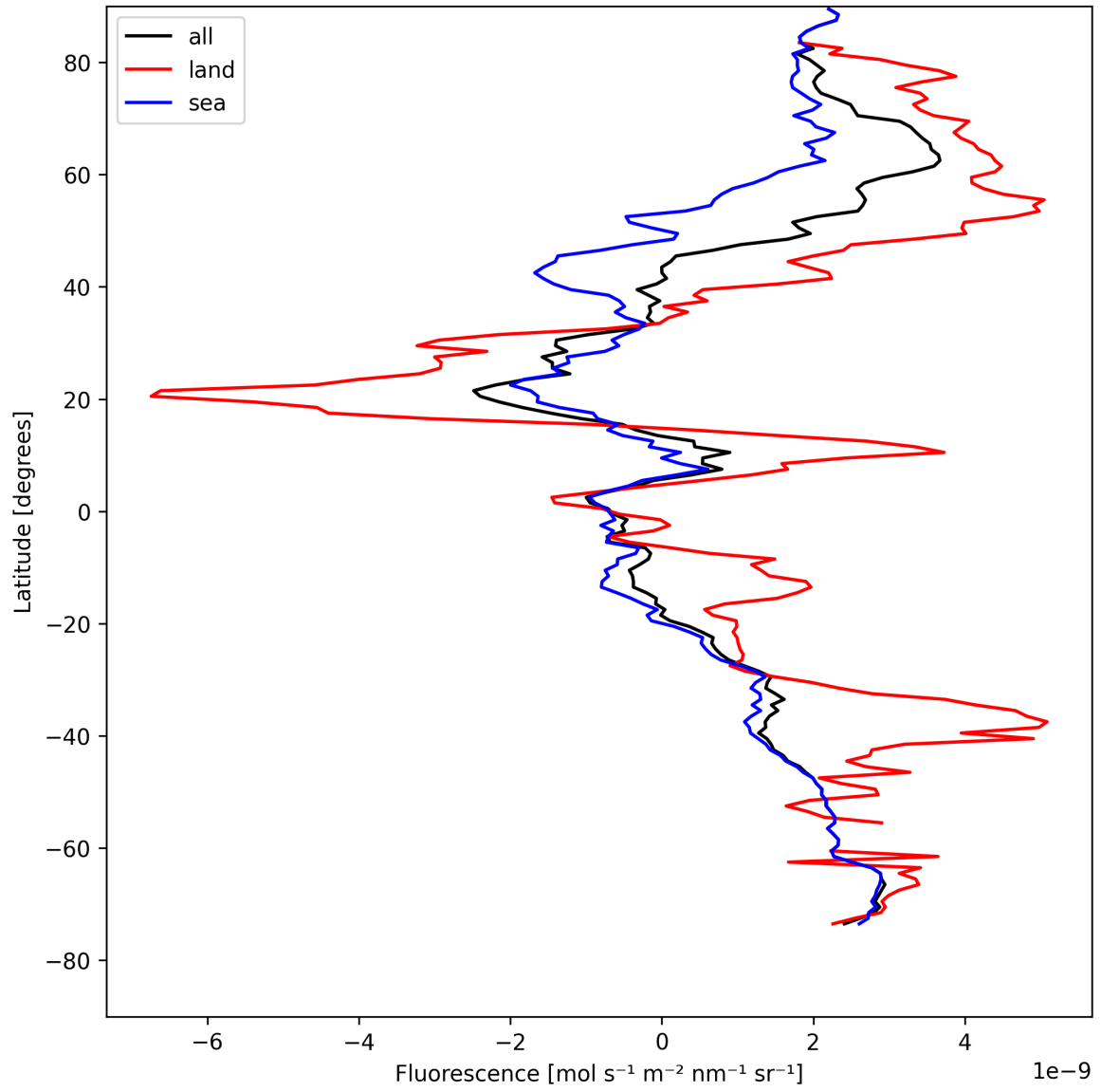
Figure 23: Zonal average of “Fluorescence” for 2025-08-12 to 2025-08-14.
