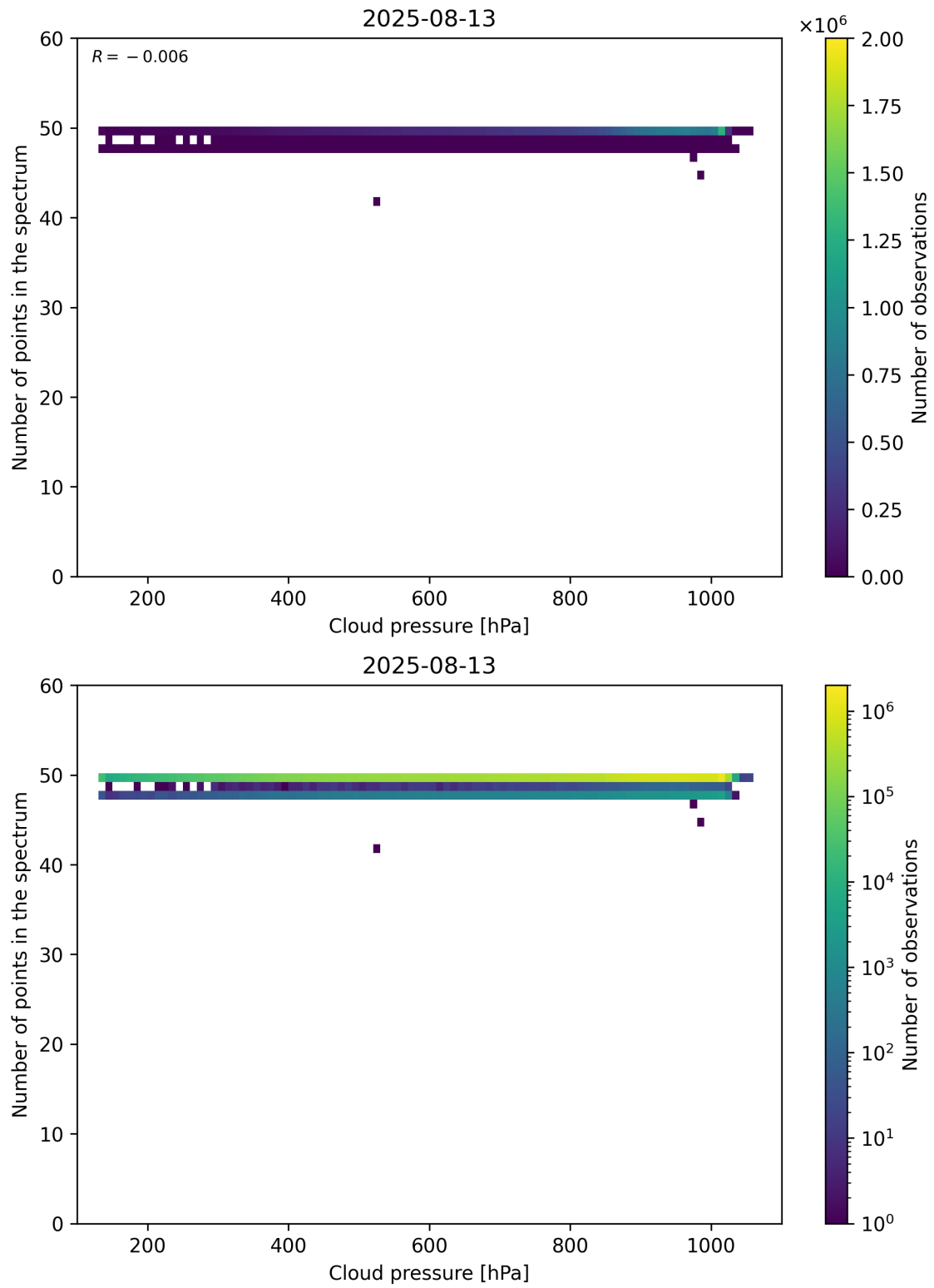
Figure 82: Scatter density plot of “Cloud pressure” against “Number of points in the spectrum” for 2025-08-12 to 2025-08-14.
