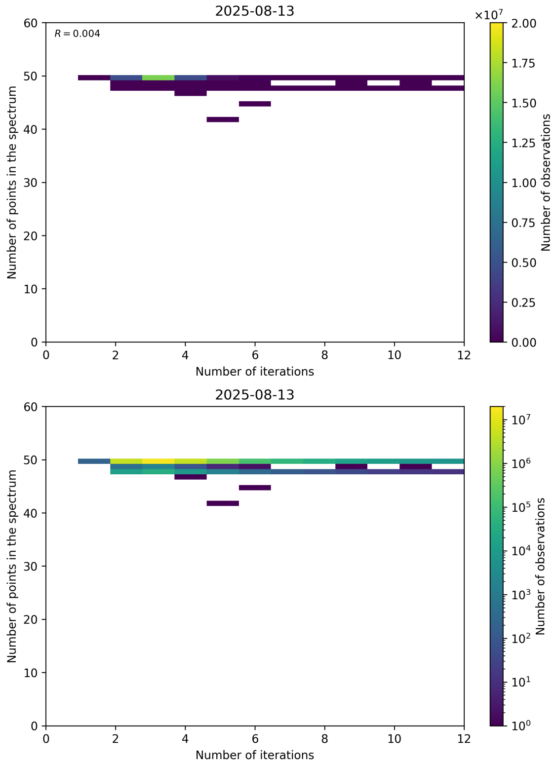
Figure 99: Scatter density plot of “Number of iterations” against “Number of points in the spectrum” for 2025-08-12 to 2025-08-14.
