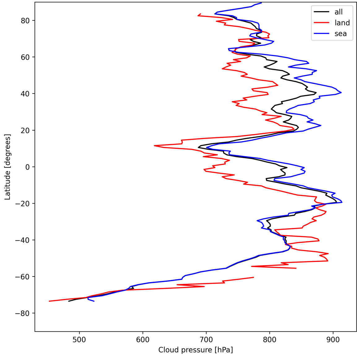
Figure 13: Zonal average of “Cloud pressure” for 2025-08-12 to 2025-08-14.
