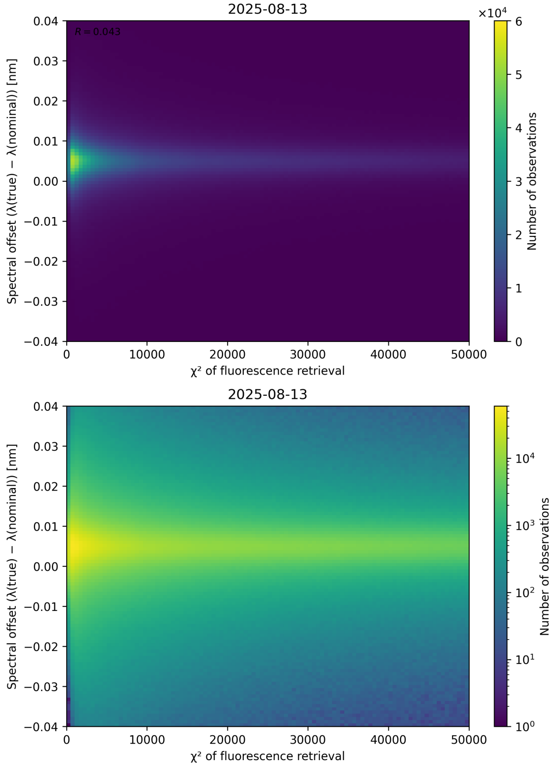
Figure 69: Scatter density plot of “ \chi^2 of fluorescence retrieval” against “Spectral offset ( \lambda_{\text{true}} - \lambda_{\text{nominal}} )” for 2025-08-12 to 2025-08-14.
