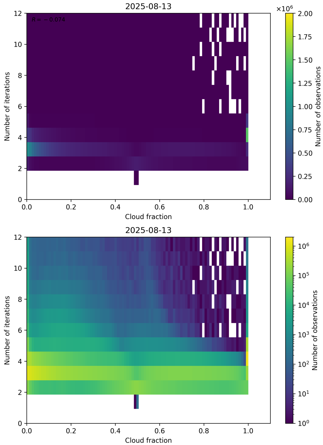
Figure 73: Scatter density plot of “Cloud fraction” against “Number of iterations” for 2025-08-12 to 2025-08-14.
