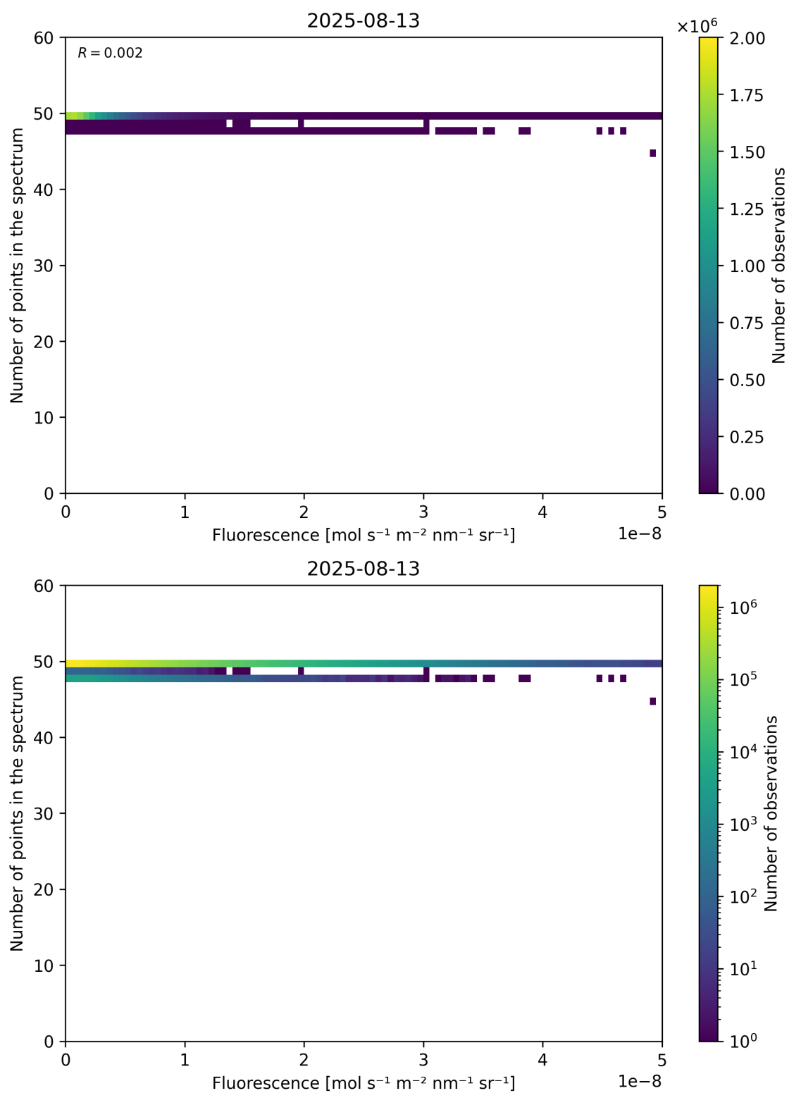
Figure 86: Scatter density plot of “Fluorescence” against “Number of points in the spectrum” for 2025-08-12 to 2025-08-14.
