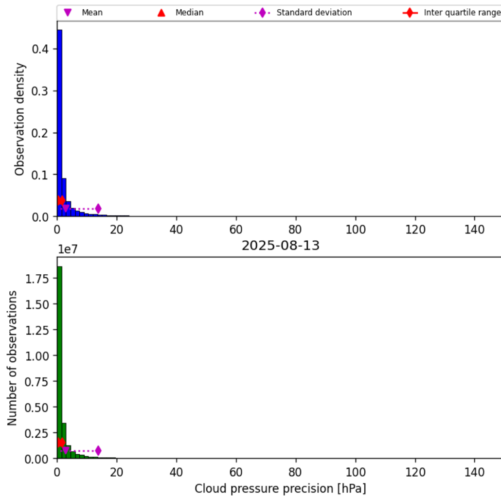
Figure 31: Histogram of “Cloud pressure precision” for 2025-08-12 to 2025-08-14
