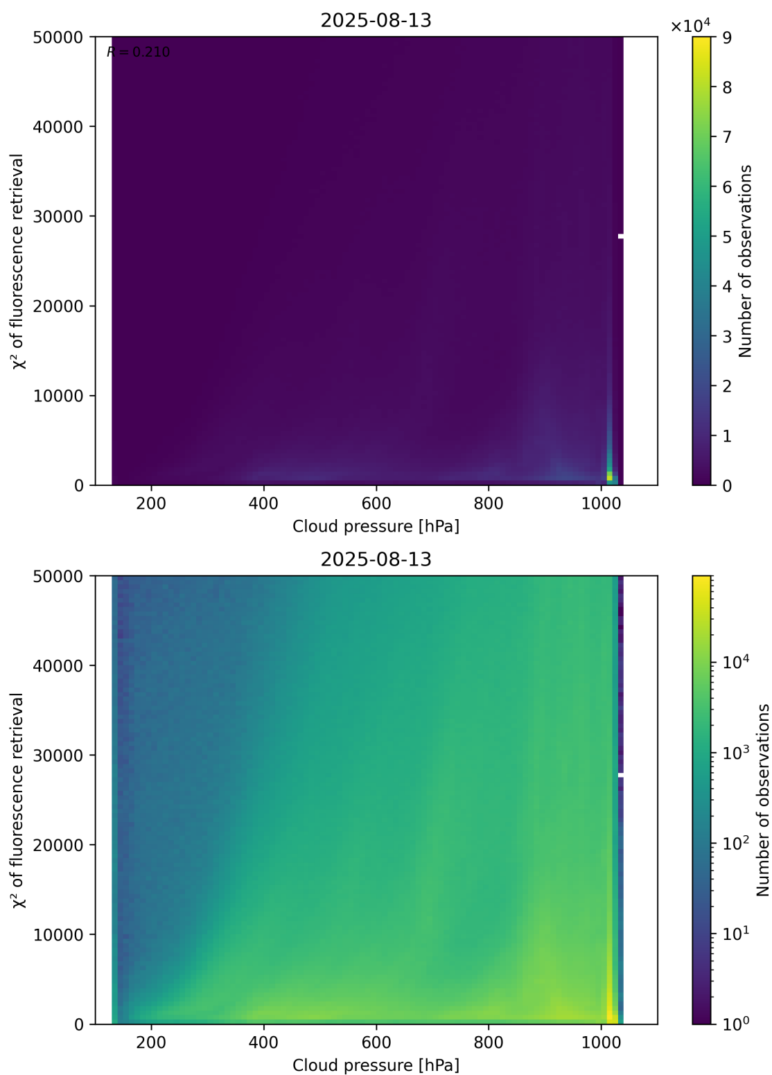
Figure 78: Scatter density plot of “Cloud pressure” against “ \chi^2 of fluorescence retrieval” for 2025-08-12 to 2025-08-14.
