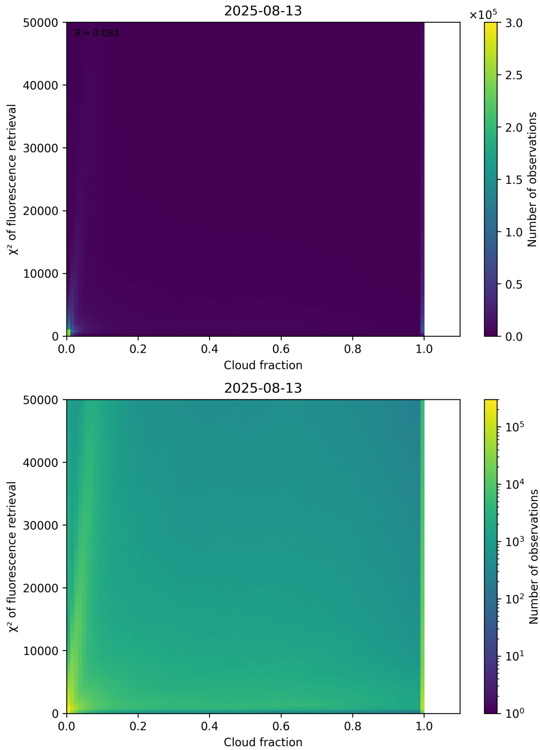
Figure 71: Scatter density plot of “Cloud fraction” against “ \chi^2 of fluorescence retrieval” for 2025-08-12 to 2025-08-14.
