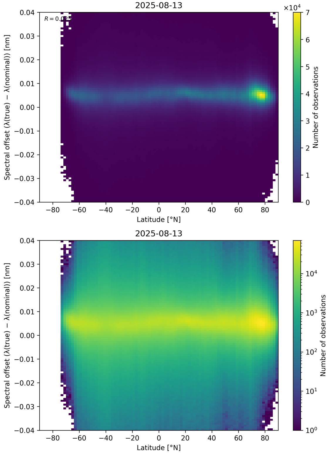
Figure 96: Scatter density plot of “Latitude” against “Spectral offset ( \lambda_{\text{true}} - \lambda_{\text{nominal}} )” for 2025-08-12 to 2025-08-14.
