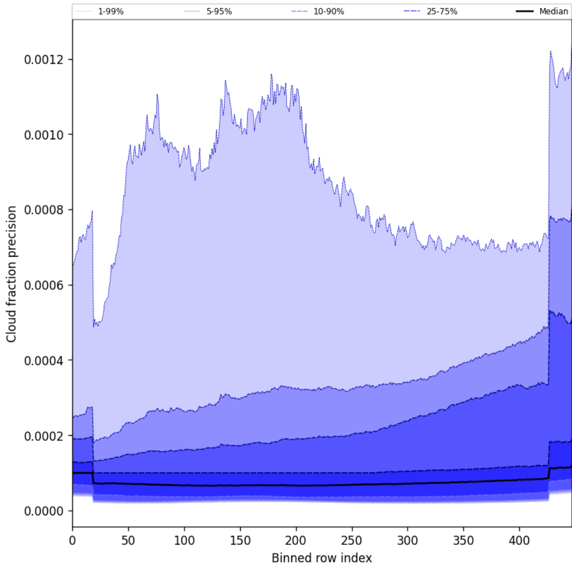
Figure 50: Along track statistics of “Cloud fraction precision” for 2025-08-12 to 2025-08-14
