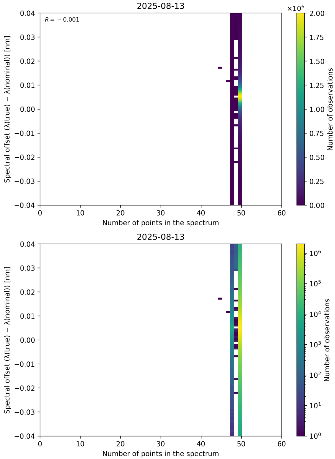
Figure 101: Scatter density plot of “Number of points in the spectrum” against “Spectral offset ( \lambda_{\text{true}} - \lambda_{\text{nominal}} )” for 2025-08-12 to 2025-08-14.
