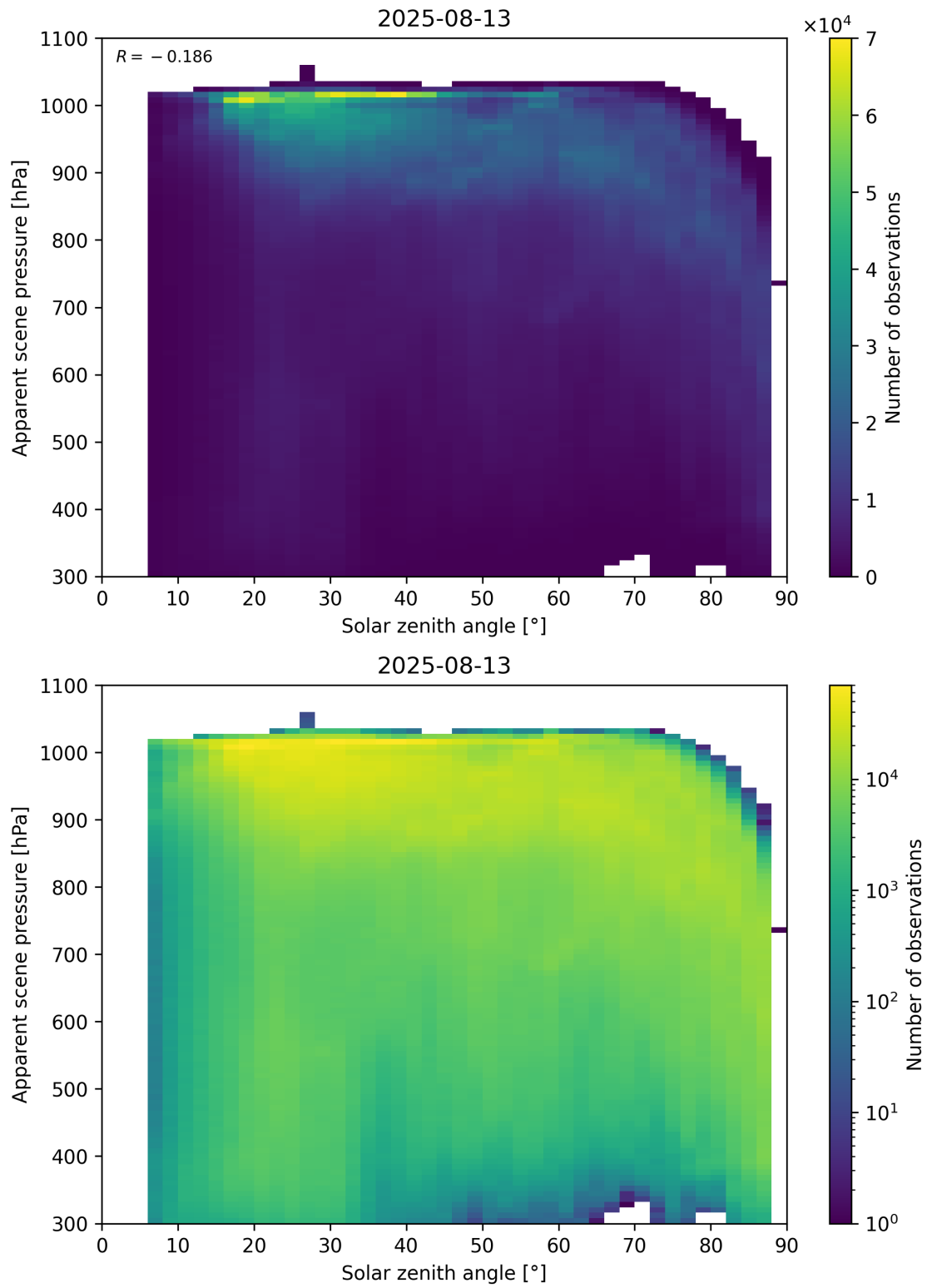
Figure 108: Scatter density plot of “Solar zenith angle” against “Apparent scene pressure” for 2025-08-12 to 2025-08-14.
