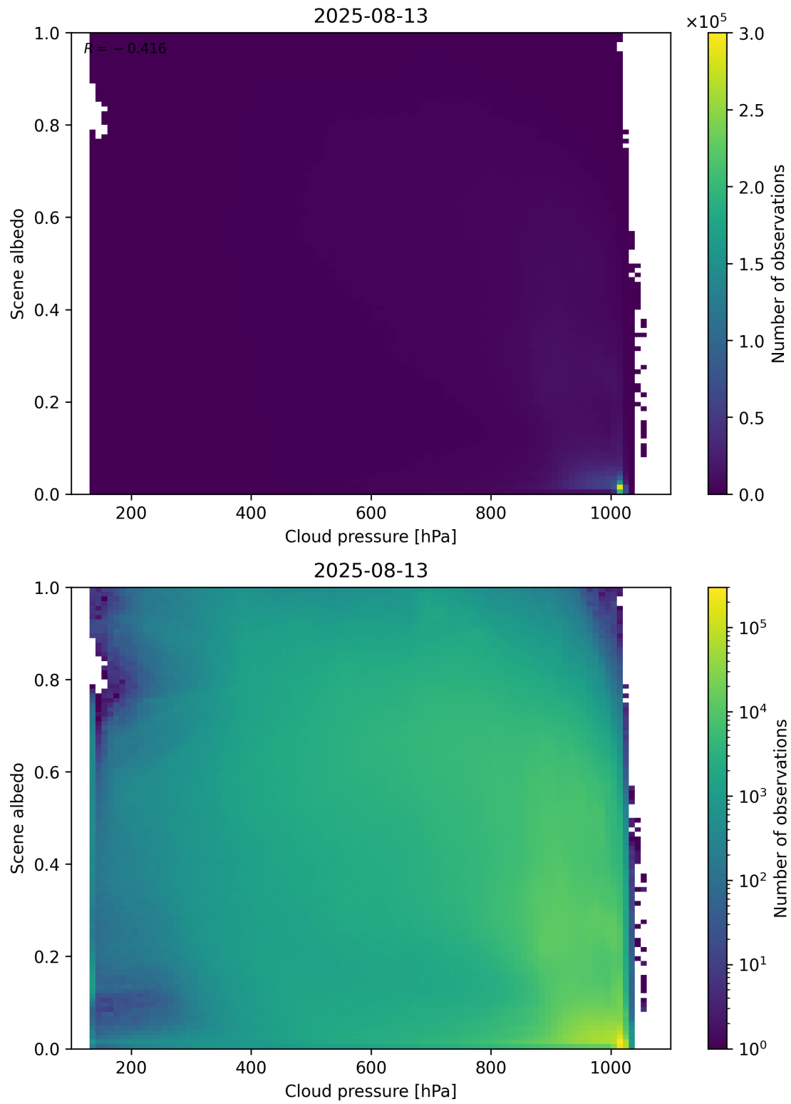
Figure 83: Scatter density plot of “Cloud pressure” against “Scene albedo” for 2025-08-12 to 2025-08-14.
