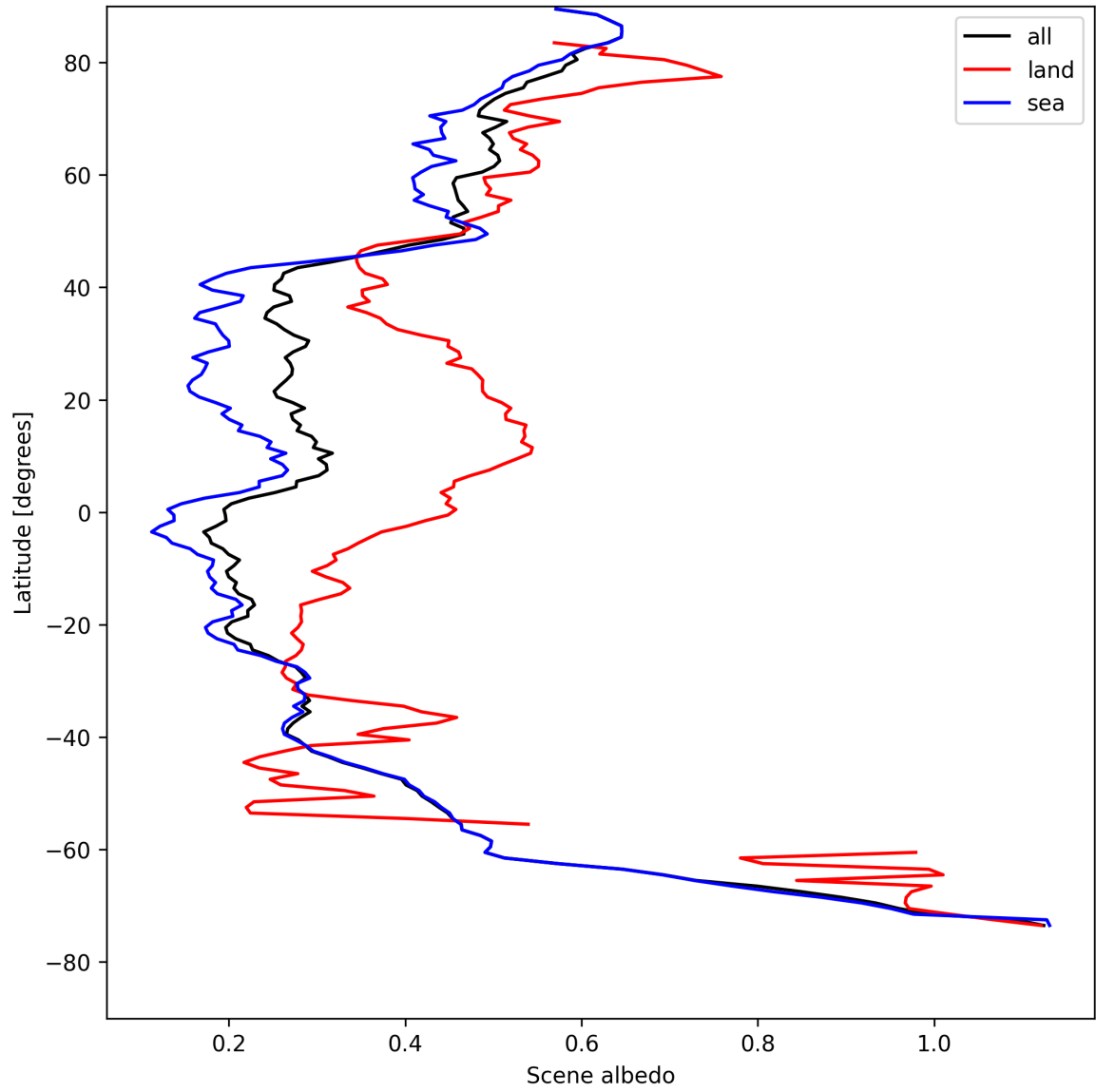
Figure 17: Zonal average of “Scene albedo” for 2025-08-12 to 2025-08-14.
