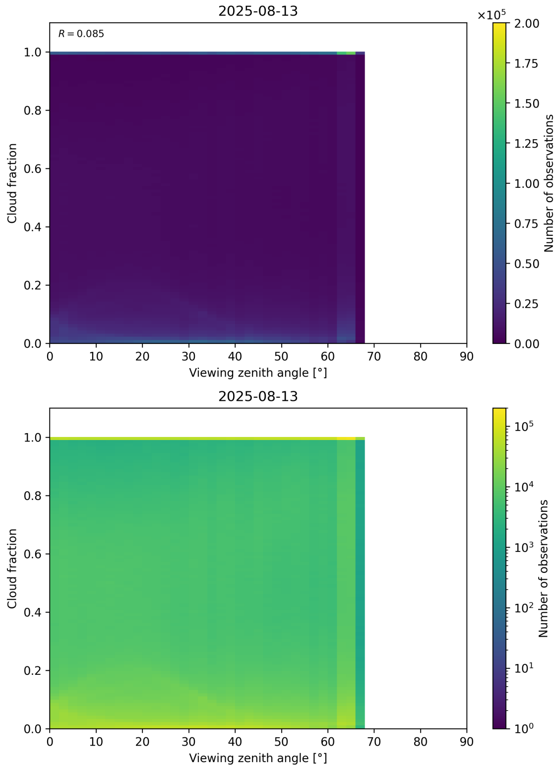
Figure 120: Scatter density plot of “Viewing zenith angle” against “Cloud fraction” for 2025-08-12 to 2025-08-14.
