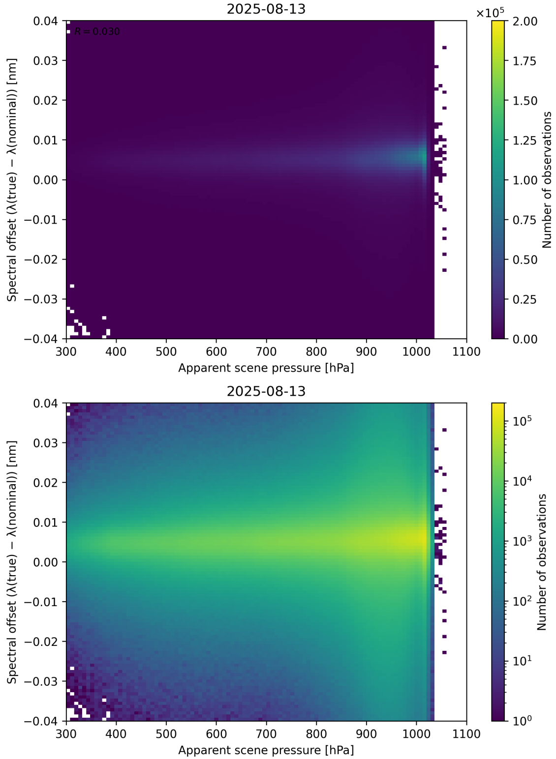
Figure 67: Scatter density plot of “Apparent scene pressure” against “Spectral offset ( \lambda_{\text{true}} - \lambda_{\text{nominal}} )” for 2025-08-12 to 2025-08-14.
