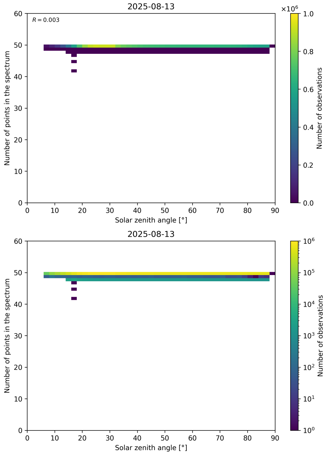
Figure 115: Scatter density plot of “Solar zenith angle” against “Number of points in the spectrum” for 2025-08-12 to 2025-08-14.
