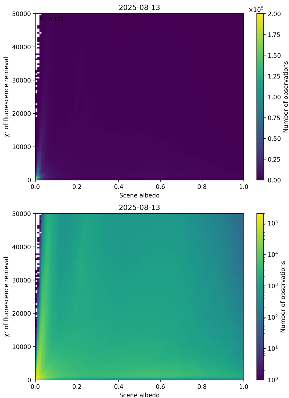
Figure 103: Scatter density plot of “Scene albedo” against “ \chi^2 of fluorescence retrieval” for 2025-08-12 to 2025-08-14.
