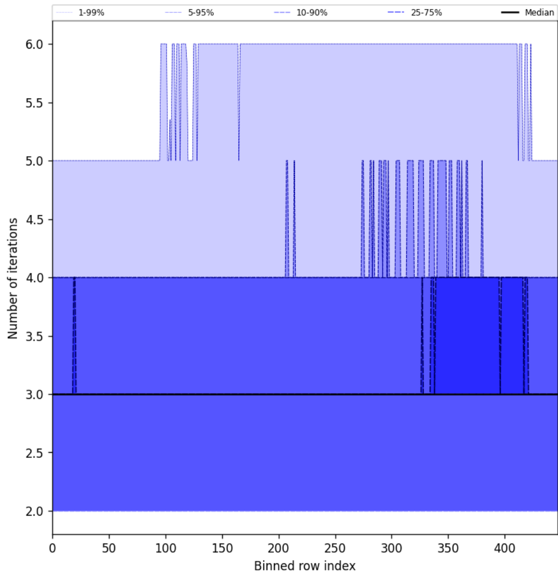
Figure 56: Along track statistics of “Number of iterations” for 2025-08-12 to 2025-08-14
