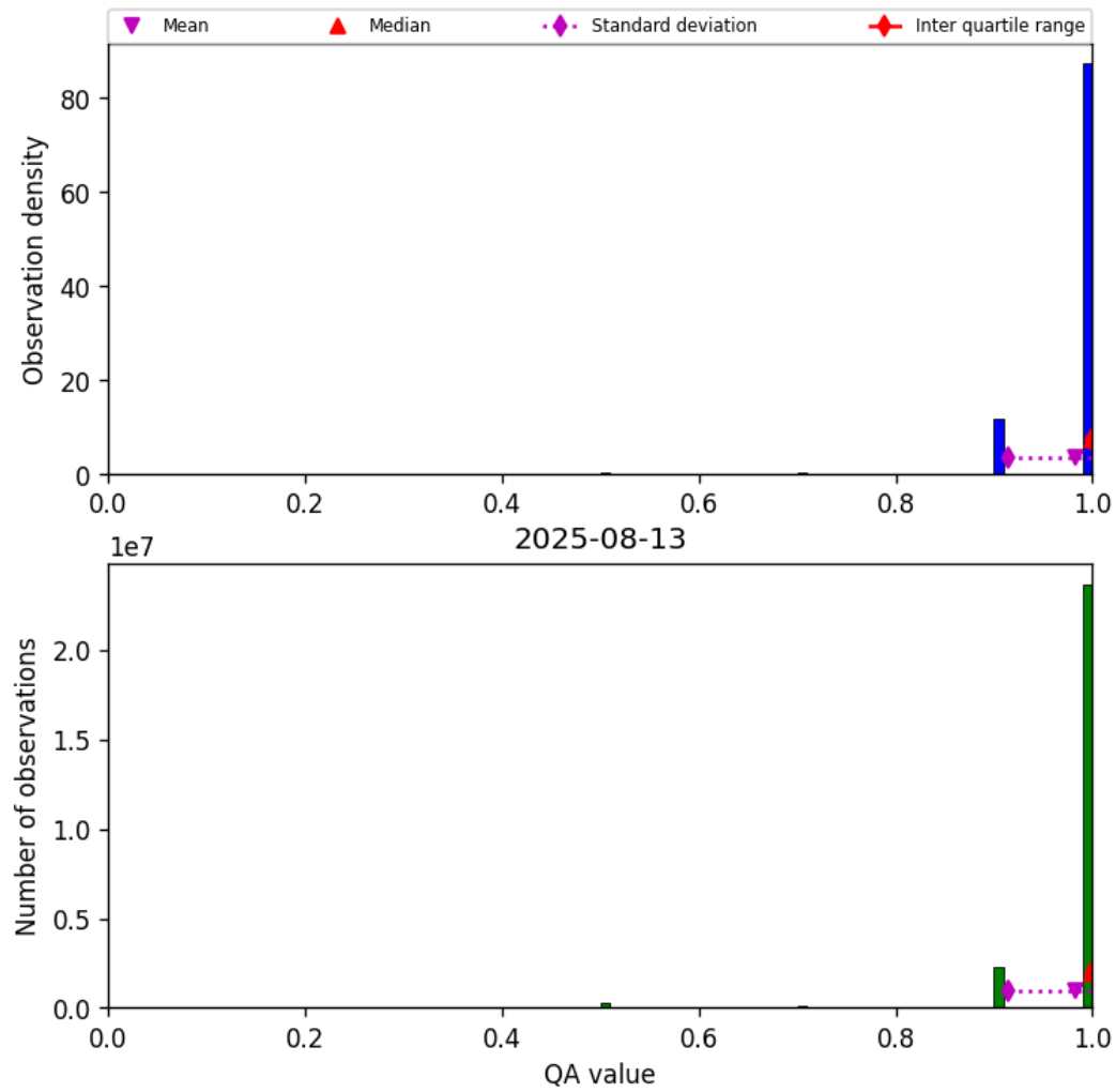
Figure 29: Histogram of “QA value” for 2025-08-12 to 2025-08-14
