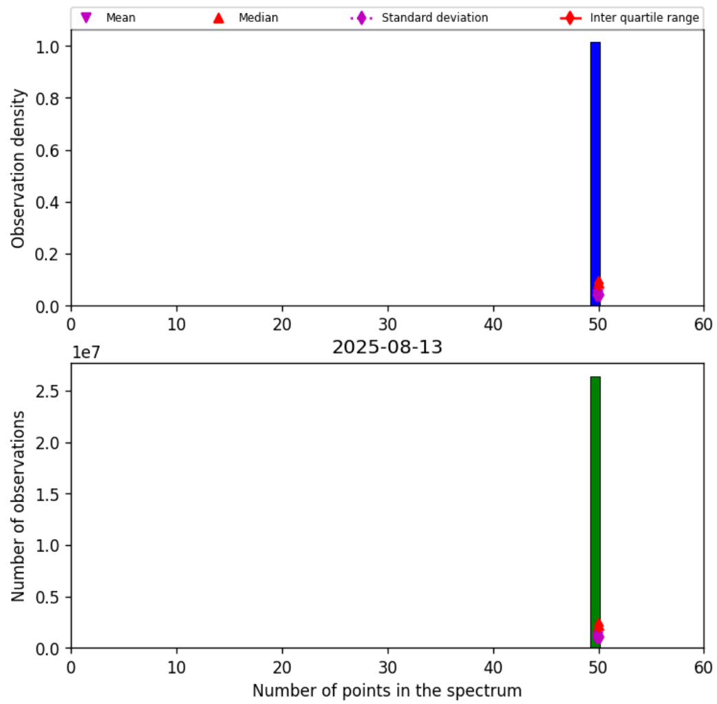
Figure 44: Histogram of “Number of points in the spectrum” for 2025-08-12 to 2025-08-14
