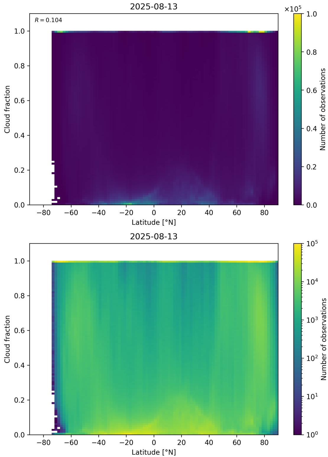
Figure 90: Scatter density plot of “Latitude” against “Cloud fraction” for 2025-08-12 to 2025-08-14.
