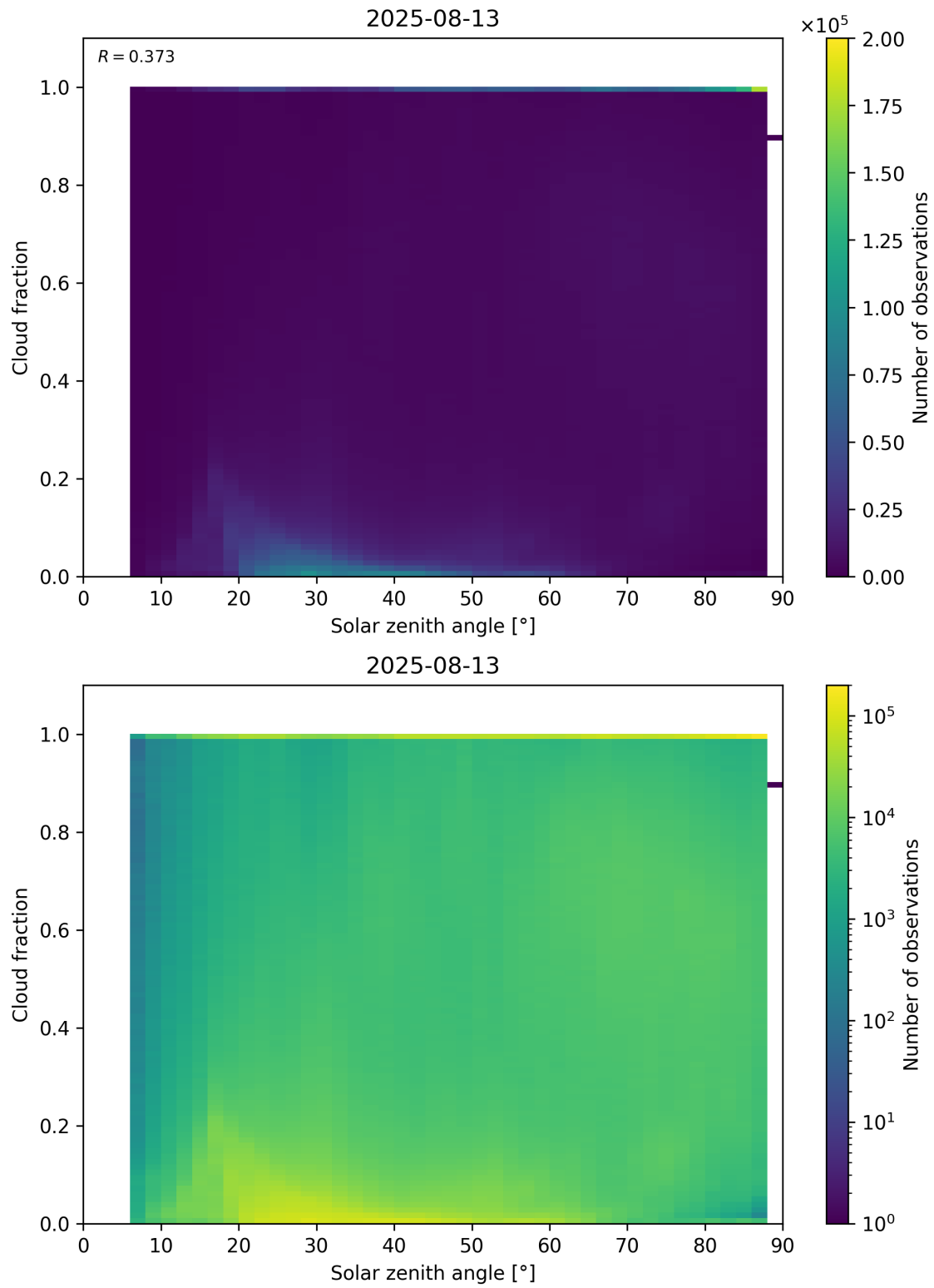
Figure 110: Scatter density plot of “Solar zenith angle” against “Cloud fraction” for 2025-08-12 to 2025-08-14.
