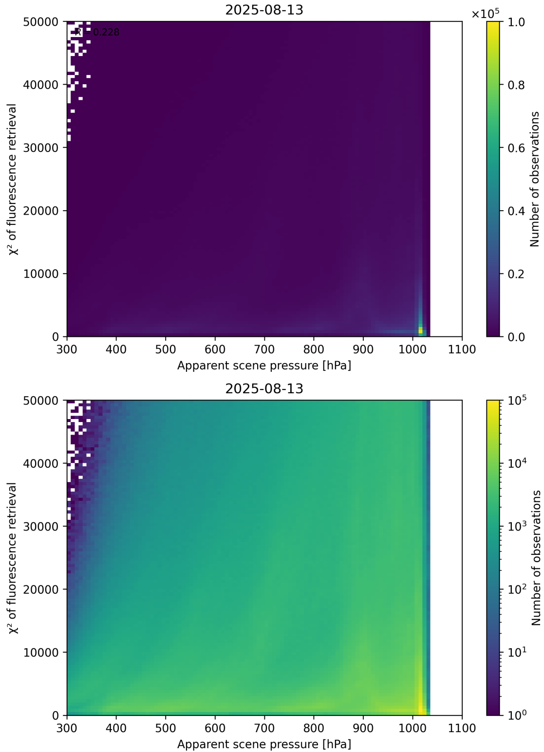
Figure 63: Scatter density plot of “Apparent scene pressure” against “ \chi^2 of fluorescence retrieval” for 2025-08-12 to 2025-08-14.
