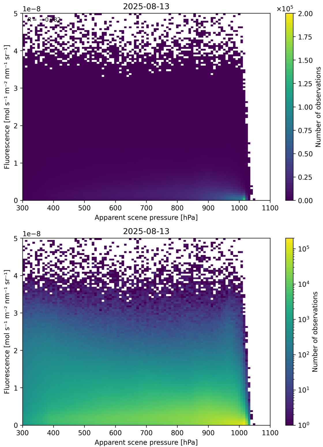
Figure 64: Scatter density plot of “Apparent scene pressure” against “Fluorescence” for 2025-08-12 to 2025-08-14.
