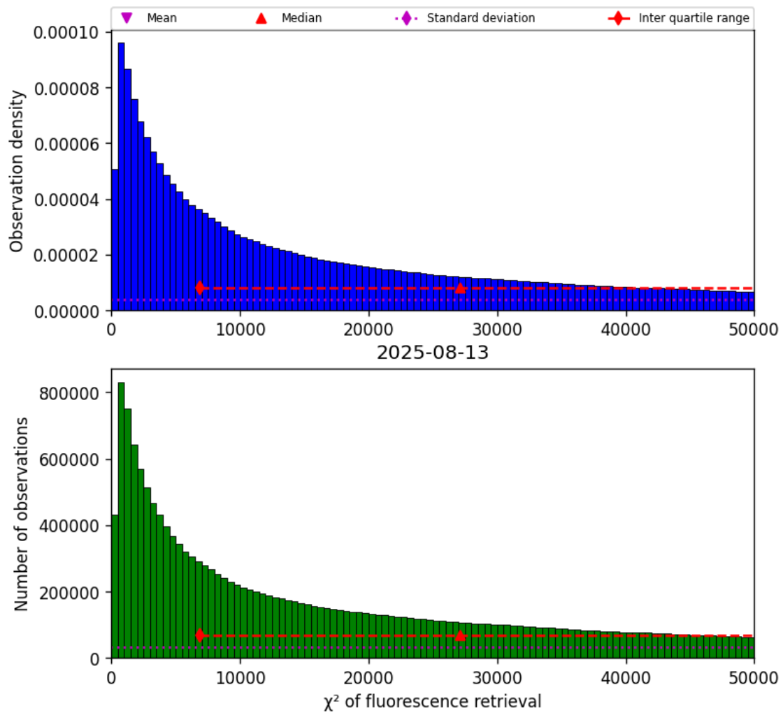
Figure 42: Histogram of “ \chi^2 of fluorescence retrieval” for 2025-08-12 to 2025-08-14
