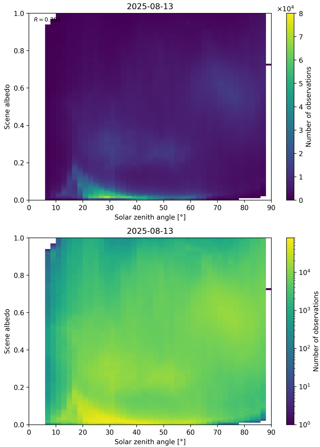
Figure 116: Scatter density plot of “Solar zenith angle” against “Scene albedo” for 2025-08-12 to 2025-08-14.
