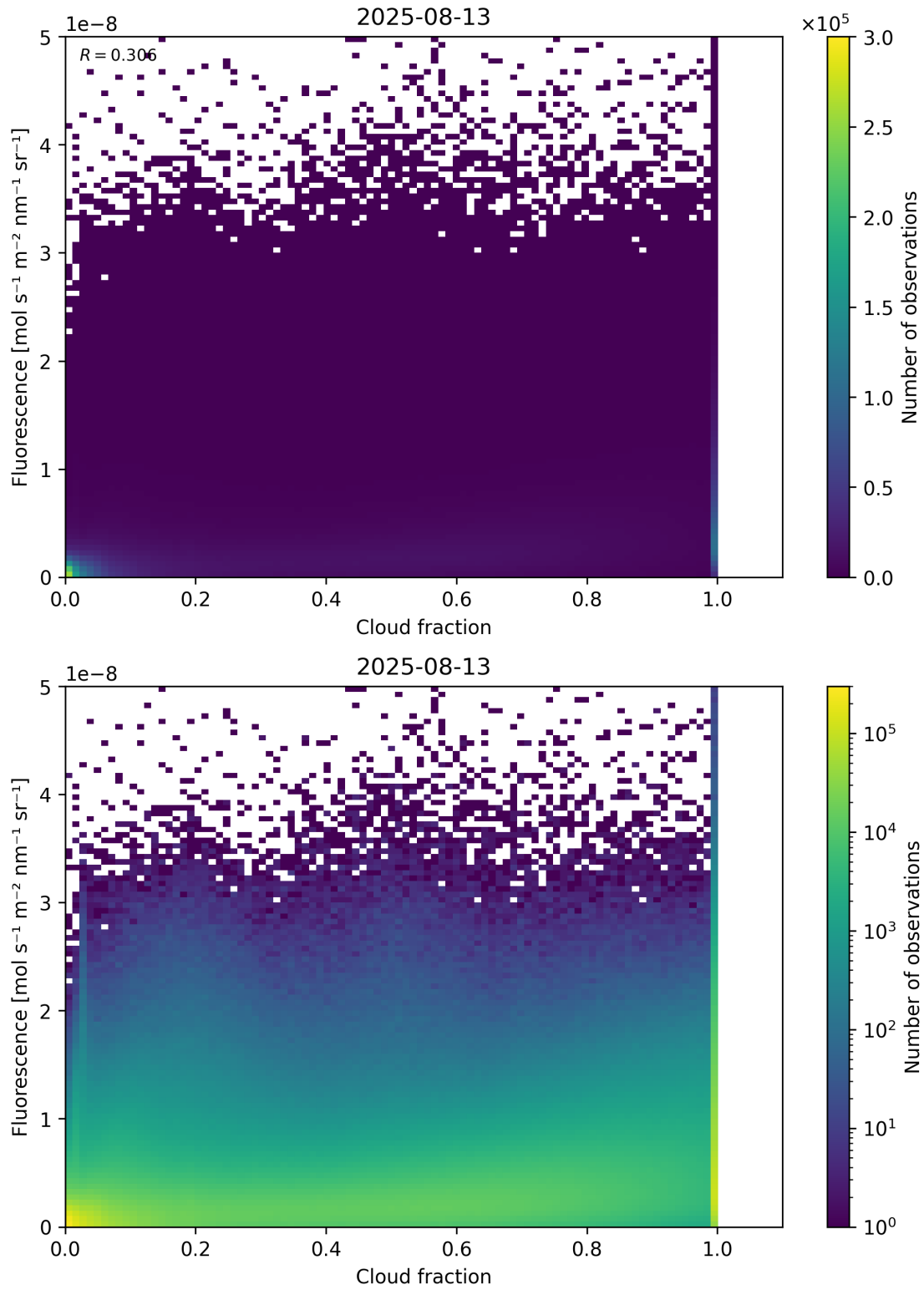
Figure 72: Scatter density plot of “Cloud fraction” against “Fluorescence” for 2025-08-12 to 2025-08-14.
