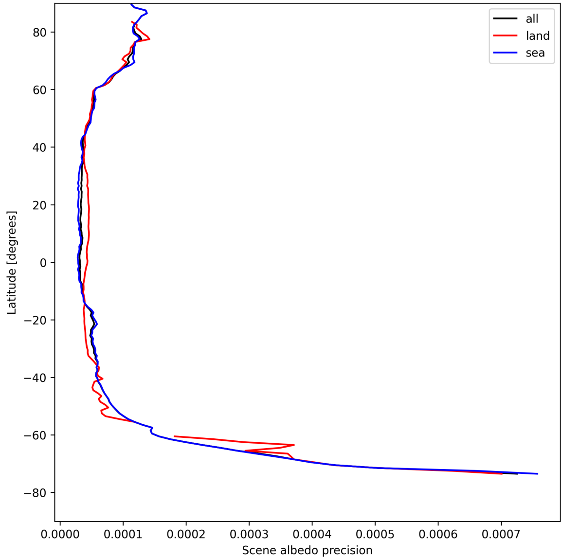
Figure 18: Zonal average of “Scene albedo precision” for 2025-08-12 to 2025-08-14.
