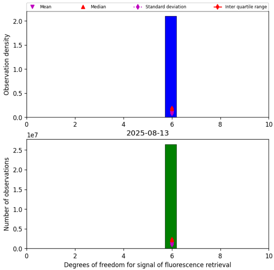
Figure 43: Histogram of “Degrees of freedom for signal of fluorescence retrieval” for 2025-08-12 to 2025-08-14
