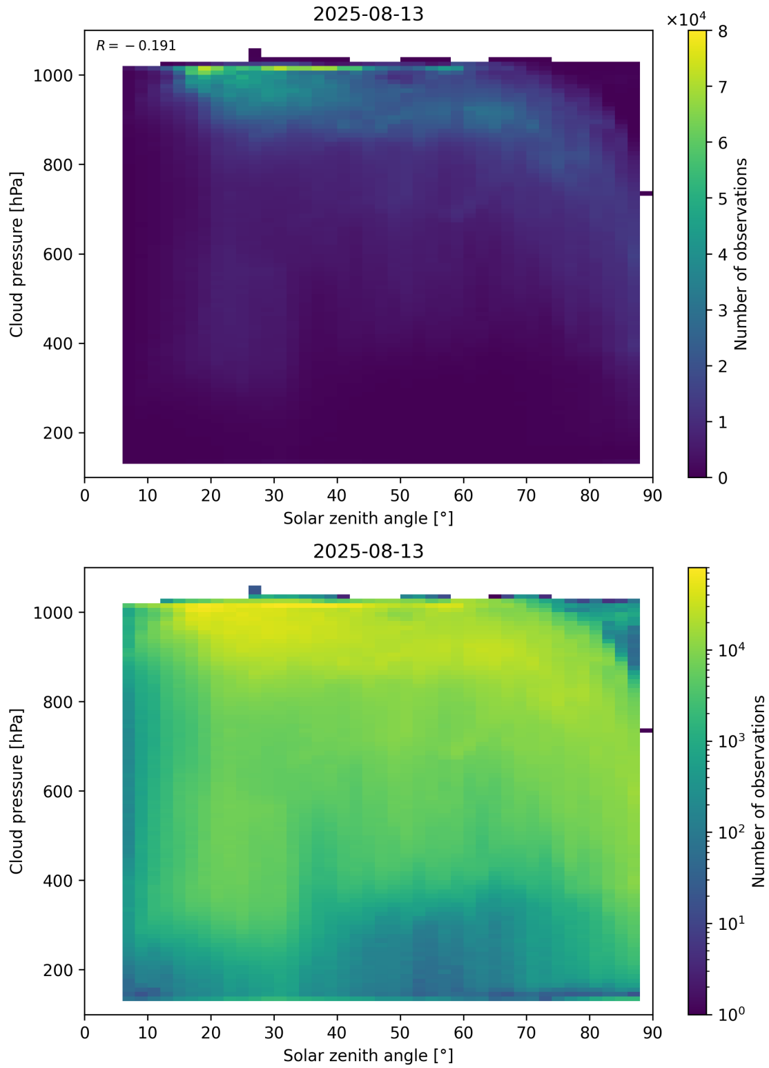
Figure 111: Scatter density plot of “Solar zenith angle” against “Cloud pressure” for 2025-08-12 to 2025-08-14.
