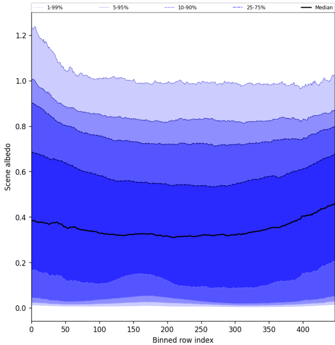
Figure 51: Along track statistics of “Scene albedo” for 2025-08-12 to 2025-08-14
