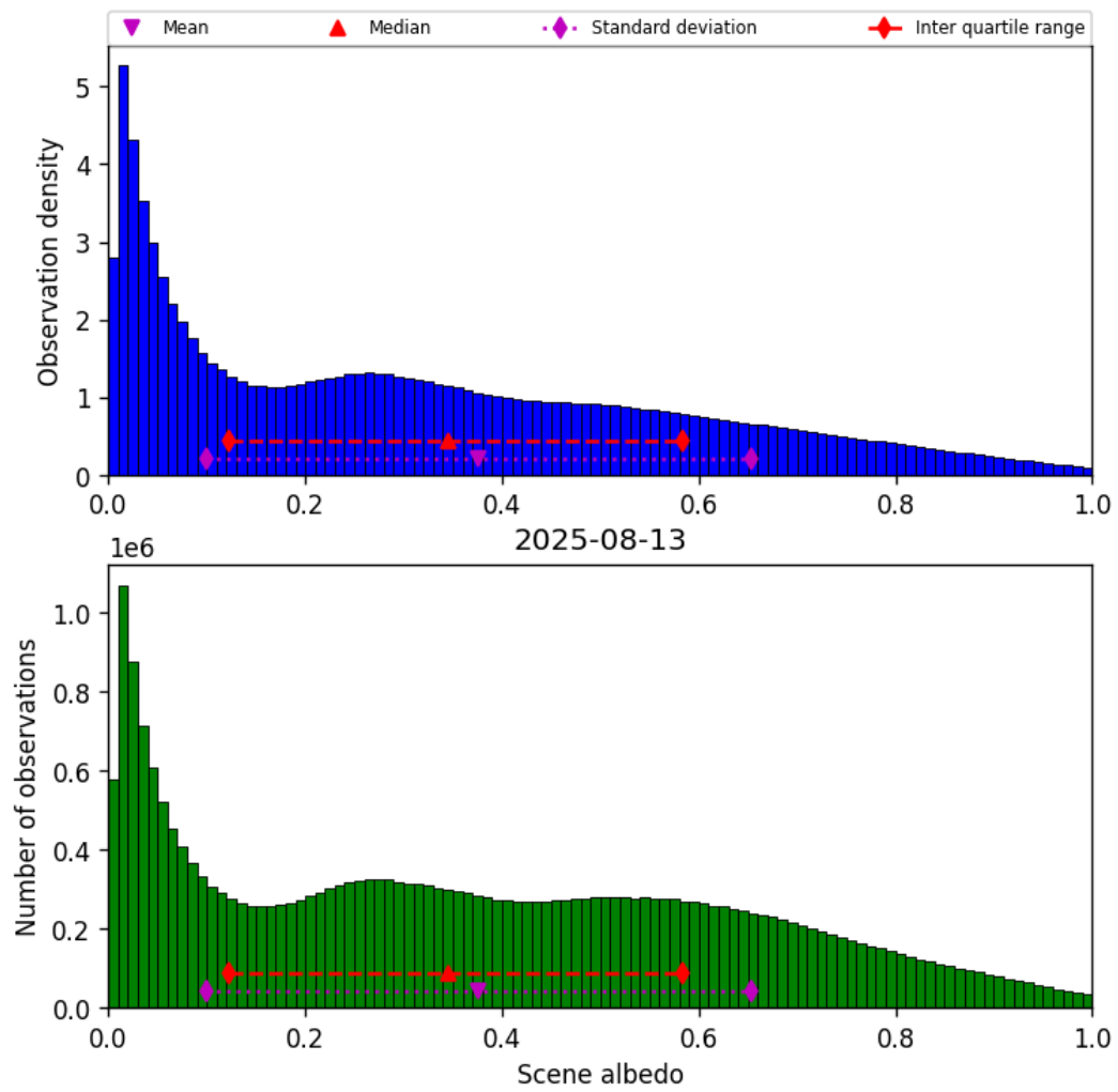
Figure 34: Histogram of “Scene albedo” for 2025-08-12 to 2025-08-14
