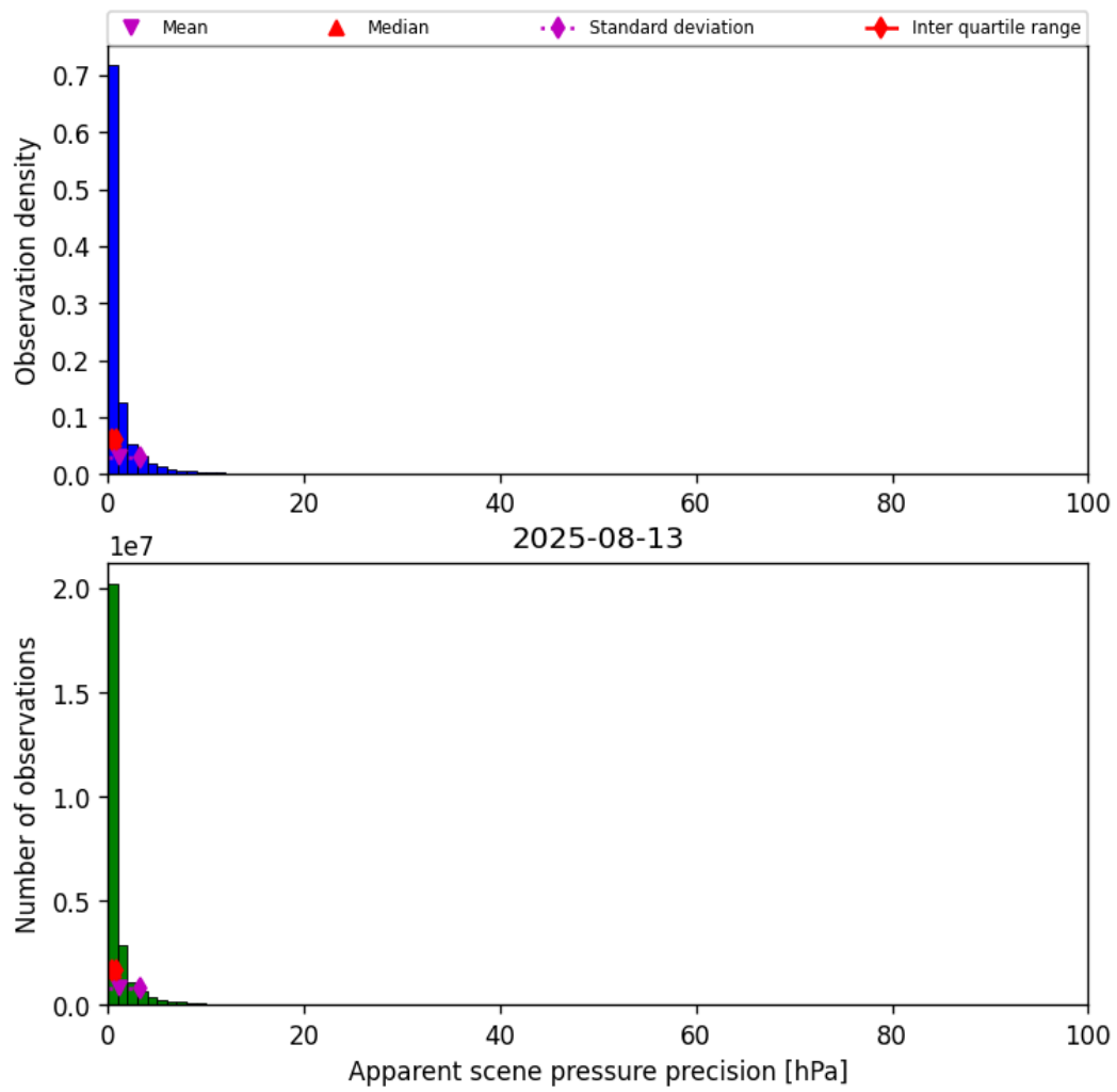
Figure 37: Histogram of “Apparent scene pressure precision” for 2025-08-12 to 2025-08-14
