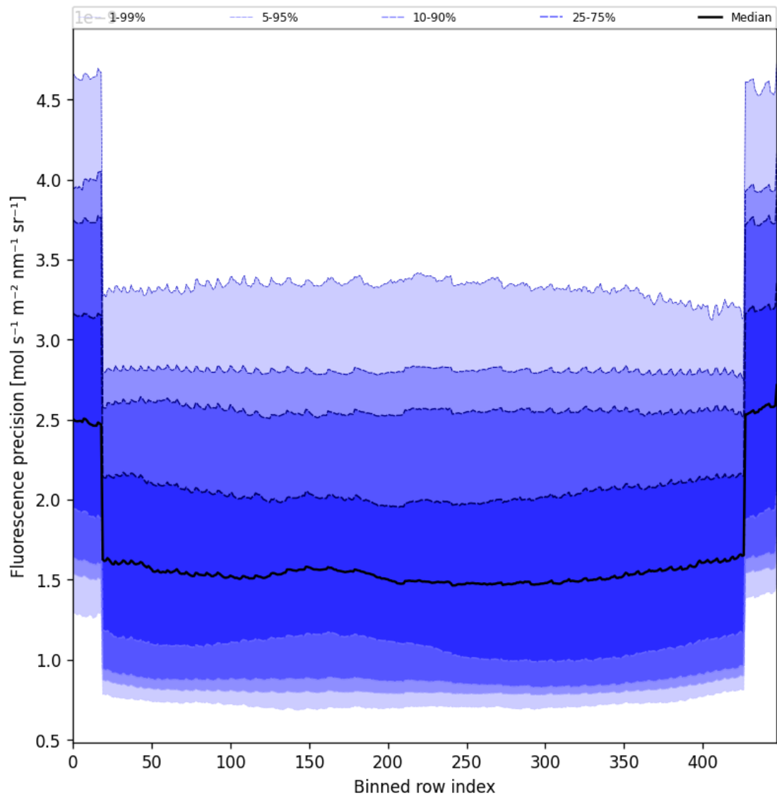
Figure 58: Along track statistics of “Fluorescence precision” for 2025-08-12 to 2025-08-14
