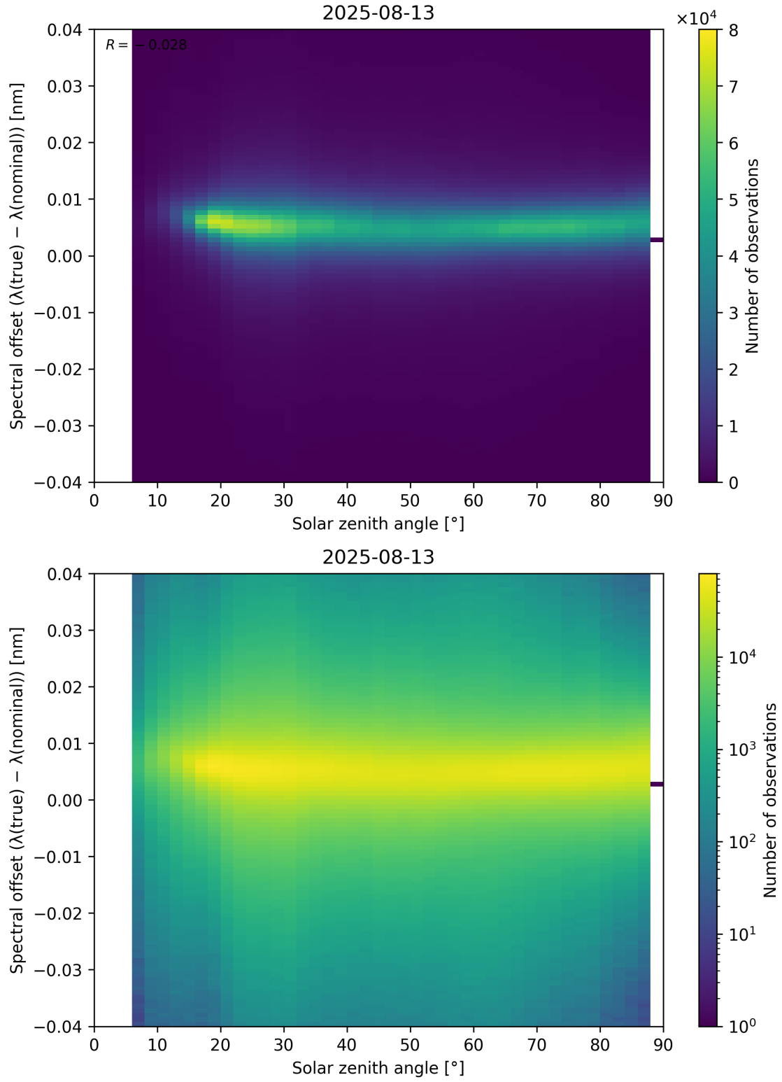
Figure 117: Scatter density plot of “Solar zenith angle” against “Spectral offset ( \lambda_{\text{true}} - \lambda_{\text{nominal}} )” for 2025-08-12 to 2025-08-14.
