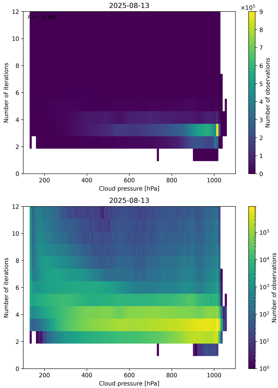
Figure 81: Scatter density plot of “Cloud pressure” against “Number of iterations” for 2025-08-12 to 2025-08-14.
