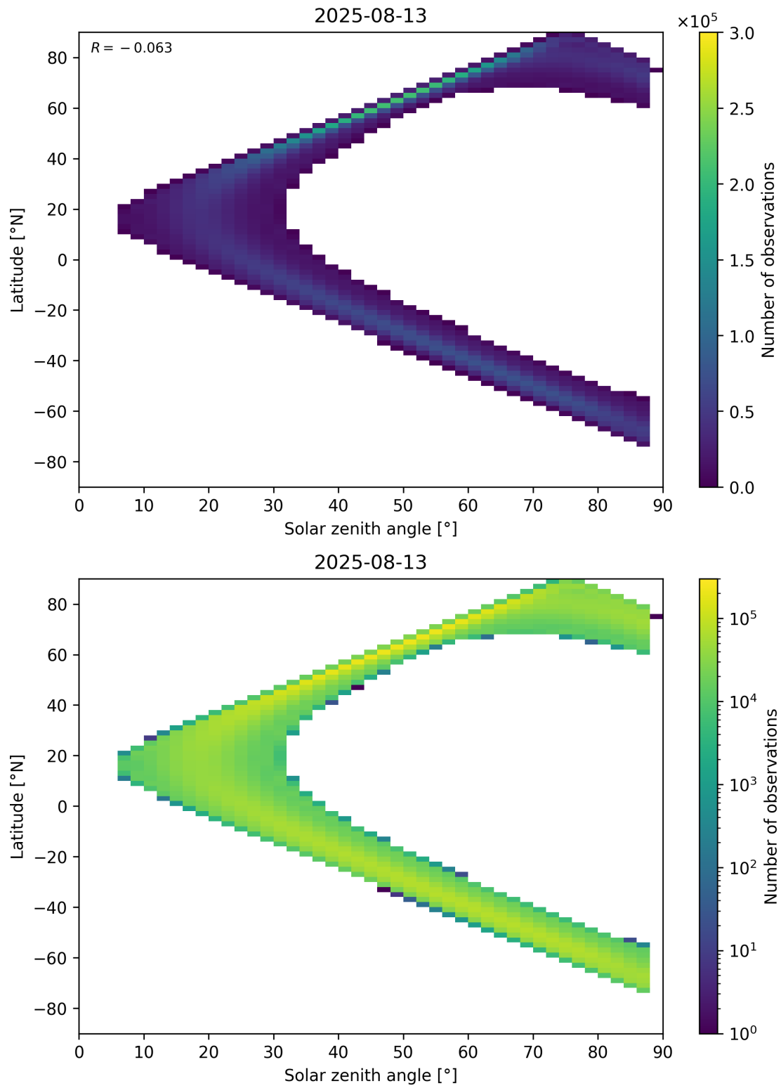
Figure 113: Scatter density plot of “Solar zenith angle” against “Latitude” for 2025-08-12 to 2025-08-14.
