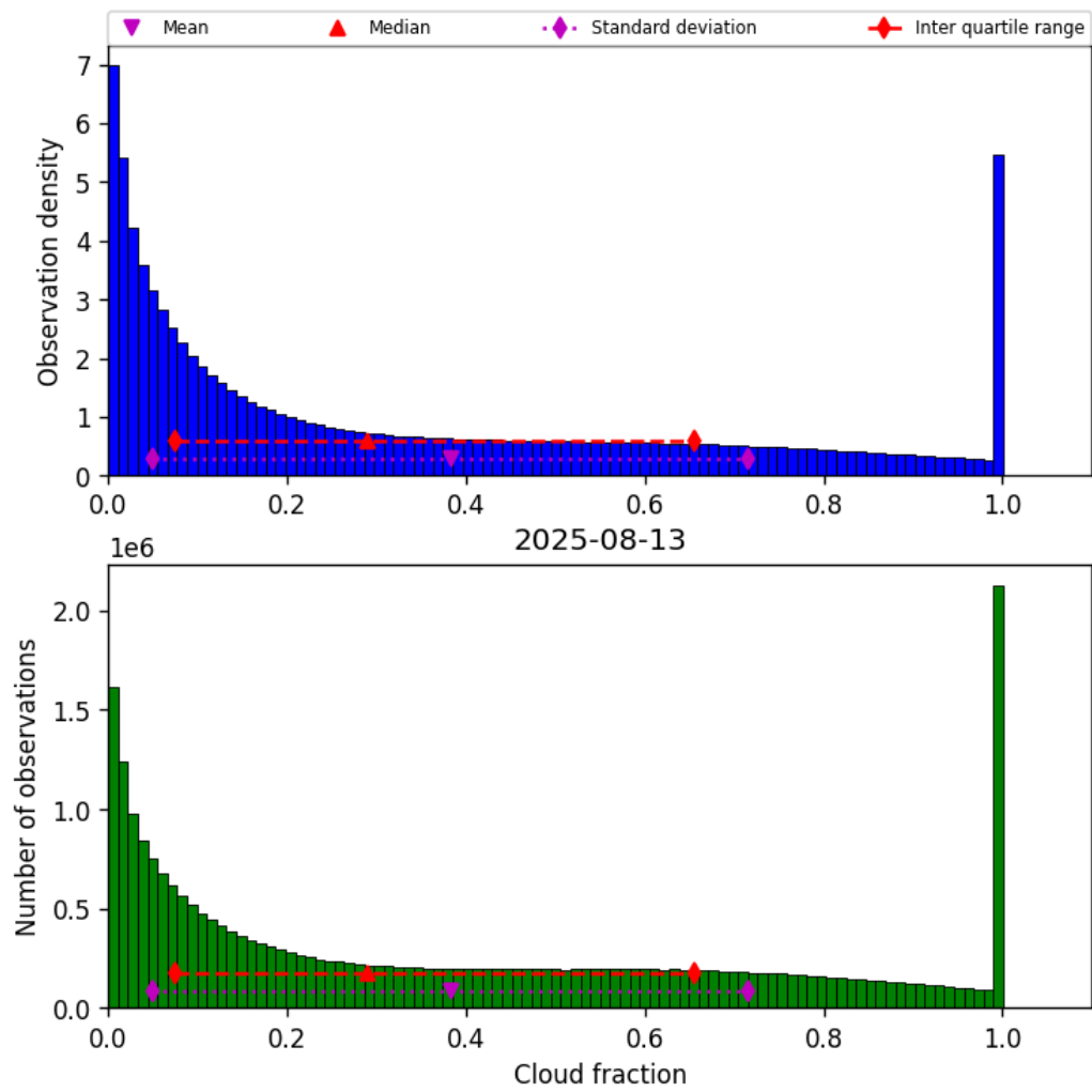
Figure 32: Histogram of “Cloud fraction” for 2025-08-12 to 2025-08-14
