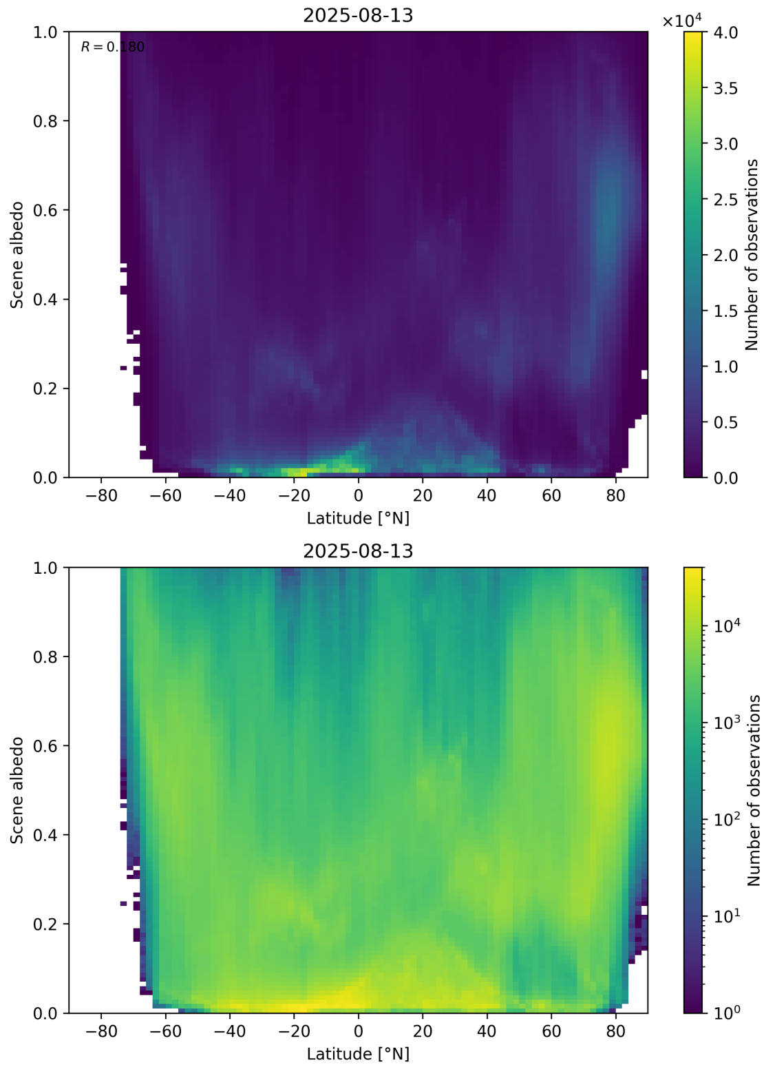
Figure 95: Scatter density plot of “Latitude” against “Scene albedo” for 2025-08-12 to 2025-08-14.
