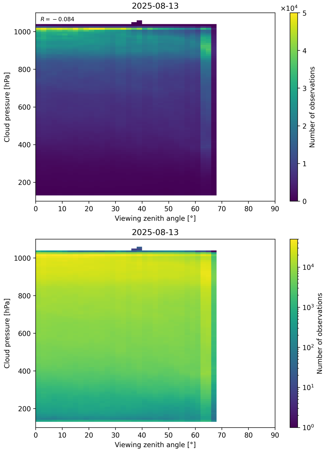
Figure 121: Scatter density plot of “Viewing zenith angle” against “Cloud pressure” for 2025-08-12 to 2025-08-14.
