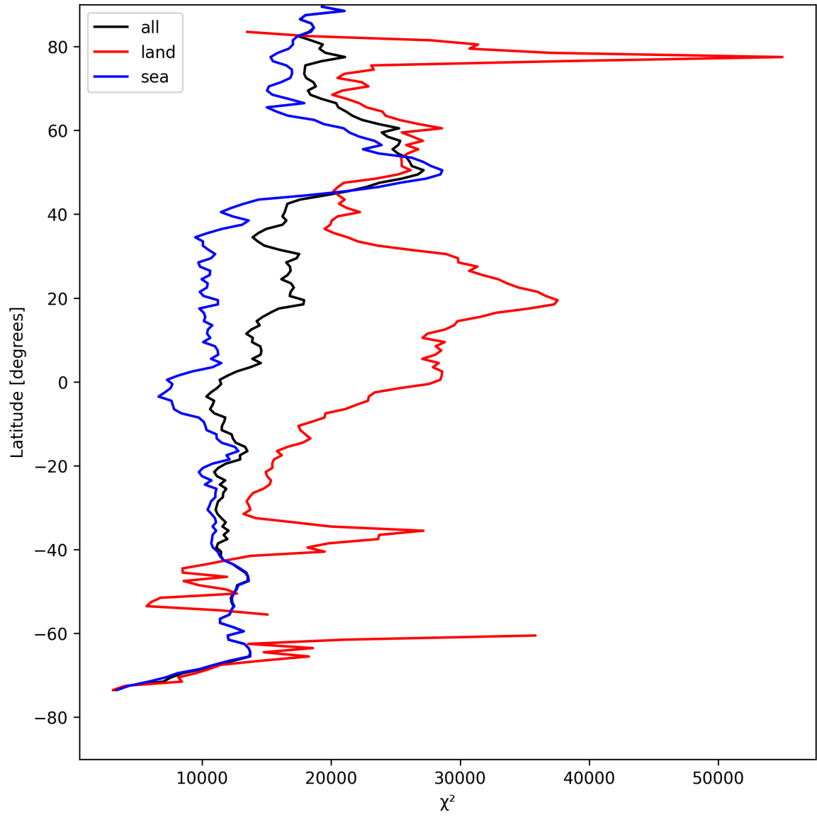
Figure 21: Zonal average of “ \chi^2 ” for 2025-08-12 to 2025-08-14.
