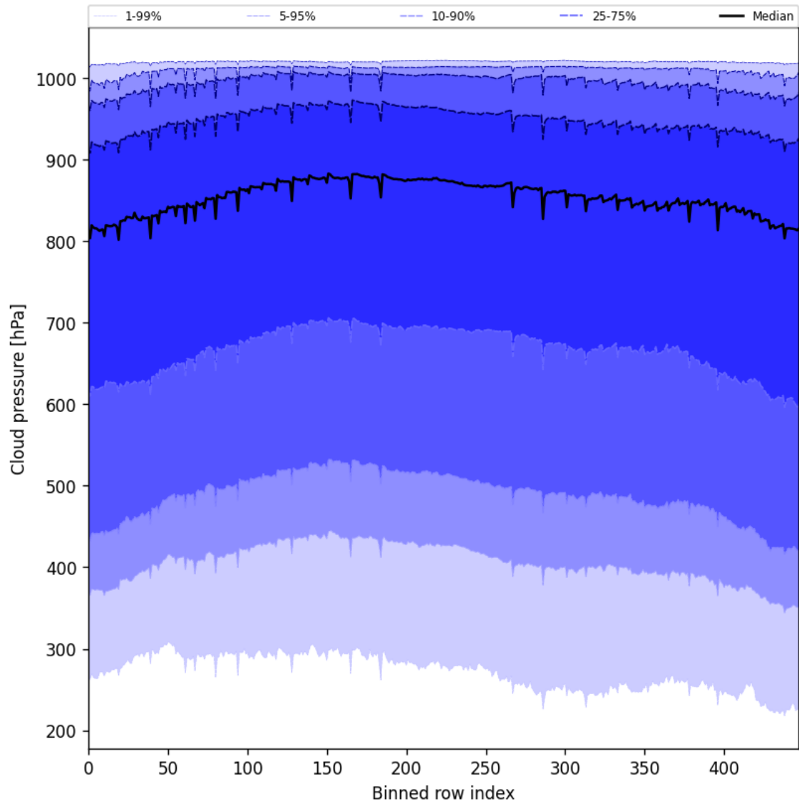
Figure 47: Along track statistics of “Cloud pressure” for 2025-08-12 to 2025-08-14
