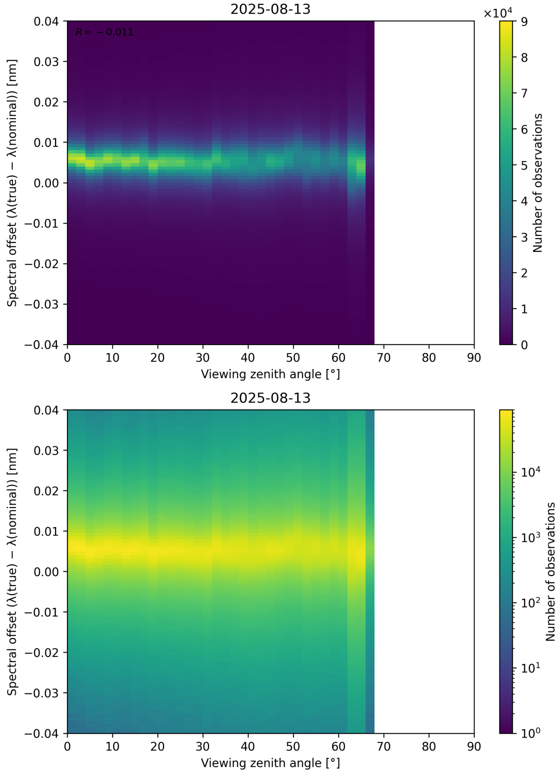
Figure 128: Scatter density plot of “Viewing zenith angle” against “Spectral offset ( \lambda_{\text{true}} - \lambda_{\text{nominal}} )” for 2025-08-12 to 2025-08-14.
