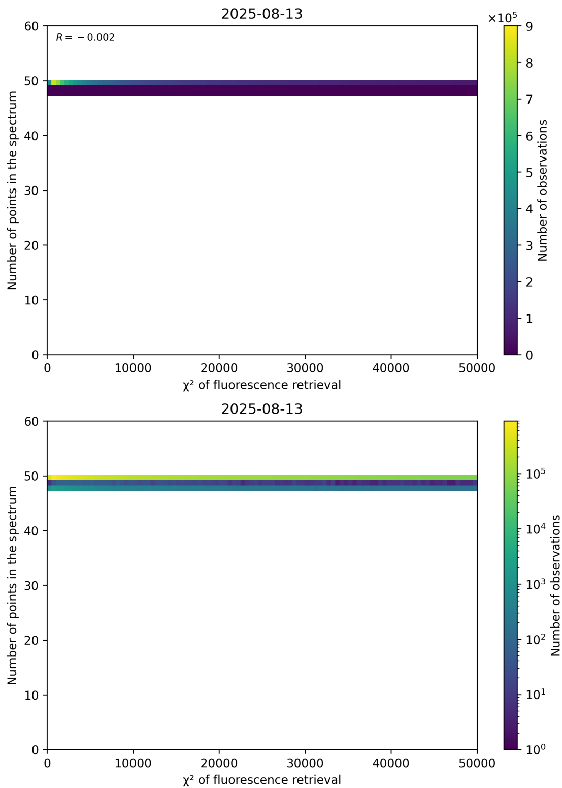
Figure 68: Scatter density plot of “ \chi^2 of fluorescence retrieval” against “Number of points in the spectrum” for 2025-08-12 to 2025-08-14.
