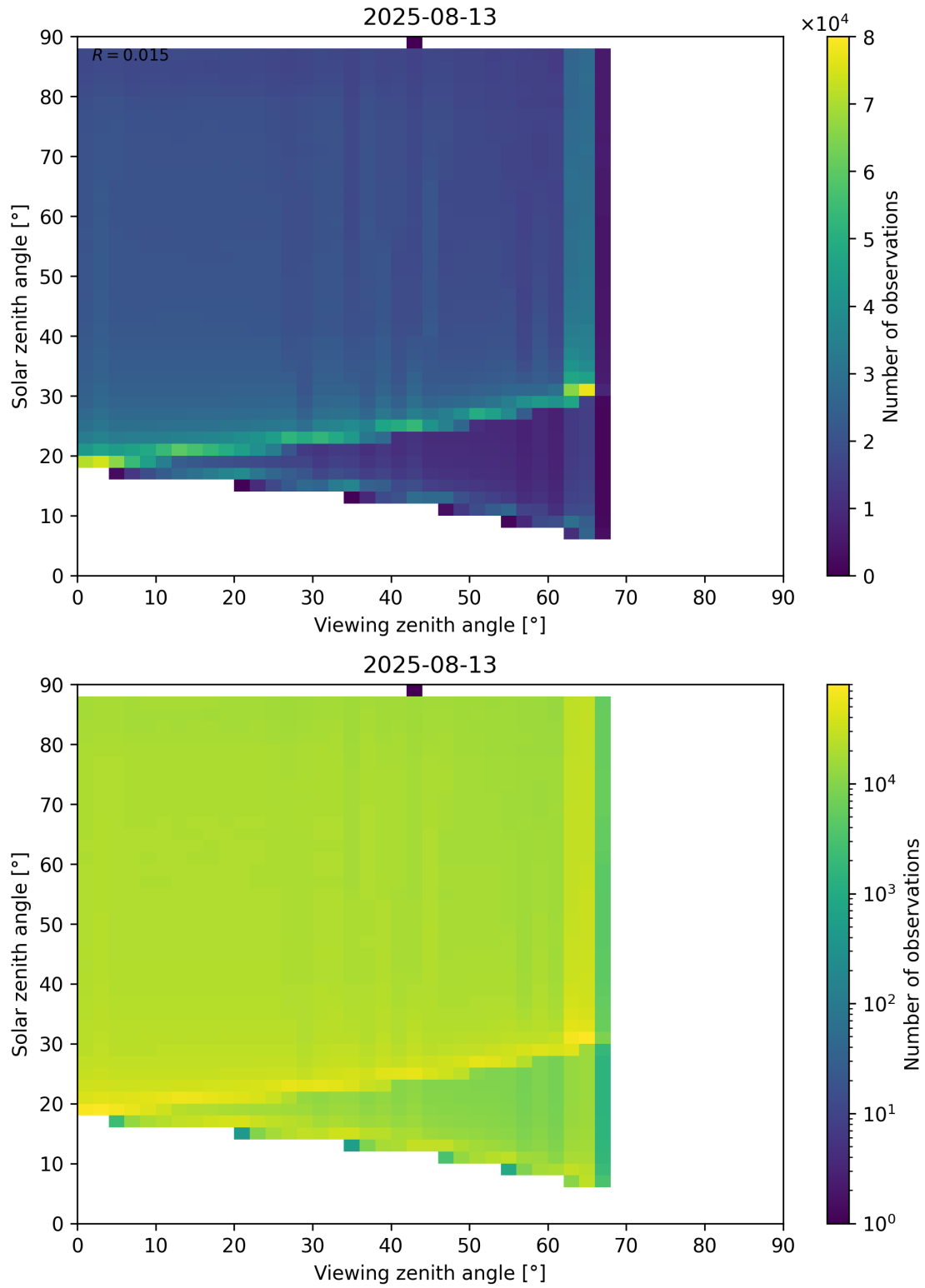
Figure 127: Scatter density plot of “Viewing zenith angle” against “Solar zenith angle” for 2025-08-12 to 2025-08-14.
