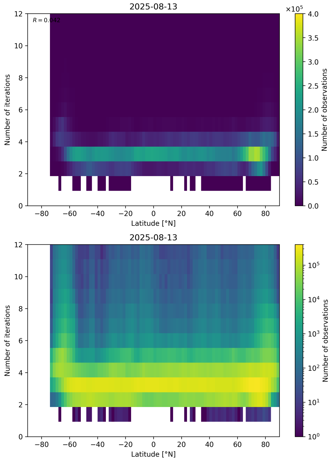
Figure 93: Scatter density plot of “Latitude” against “Number of iterations” for 2025-08-12 to 2025-08-14.
