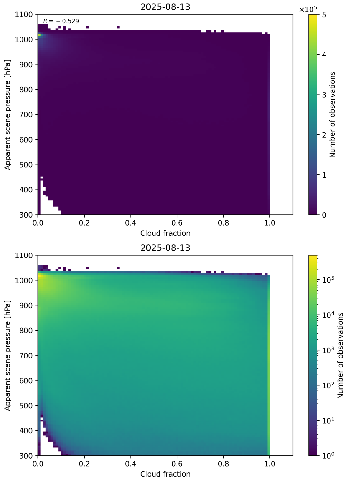
Figure 70: Scatter density plot of “Cloud fraction” against “Apparent scene pressure” for 2025-08-12 to 2025-08-14.
