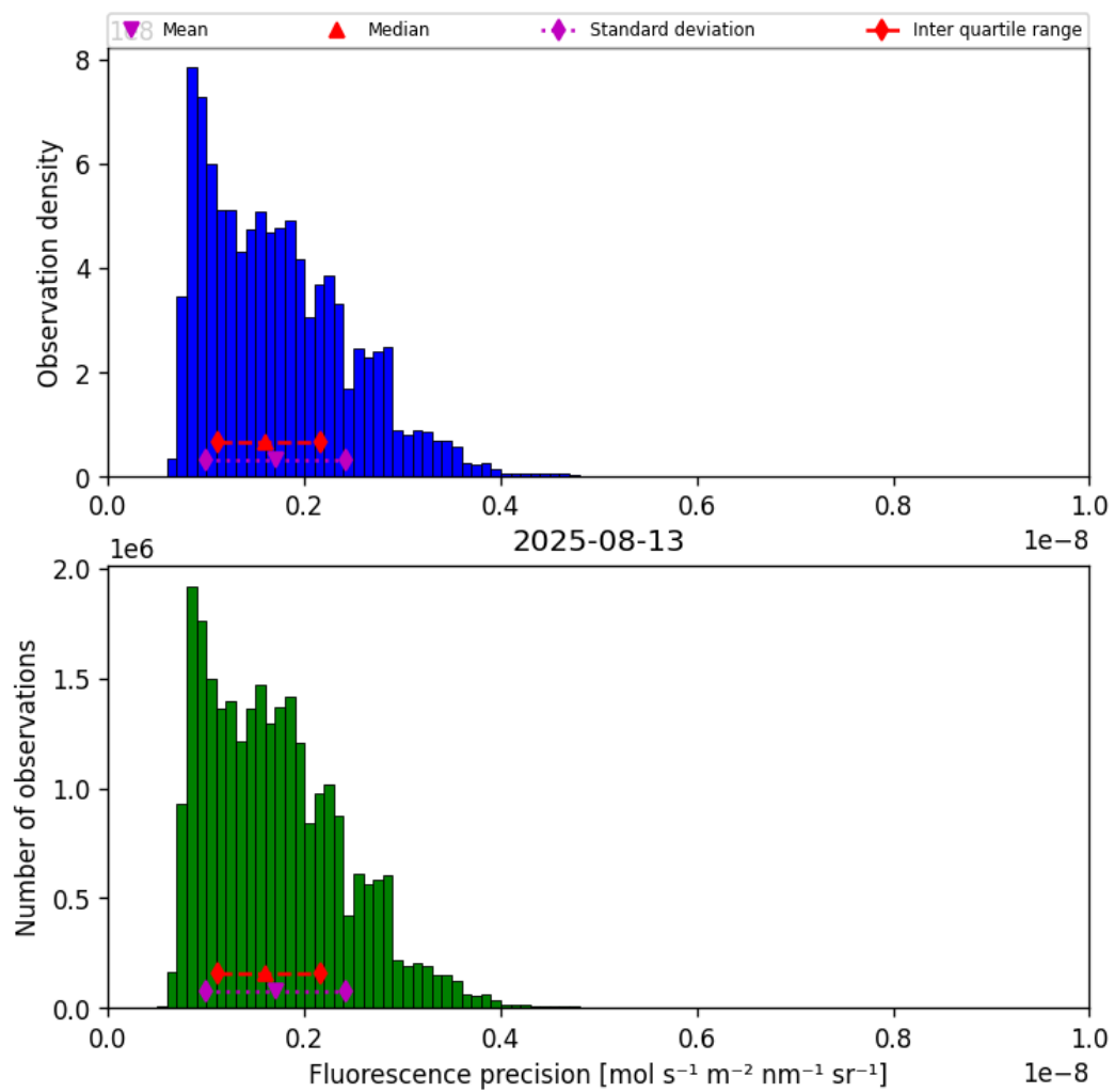
Figure 41: Histogram of “Fluorescence precision” for 2025-08-12 to 2025-08-14
