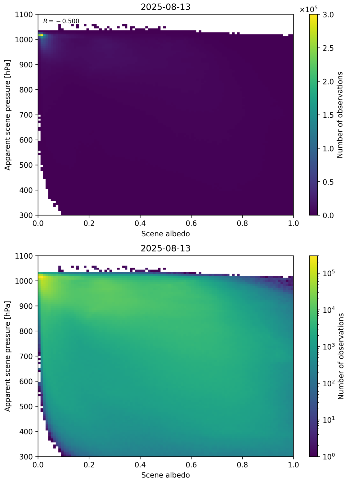
Figure 102: Scatter density plot of “Scene albedo” against “Apparent scene pressure” for 2025-08-12 to 2025-08-14.
