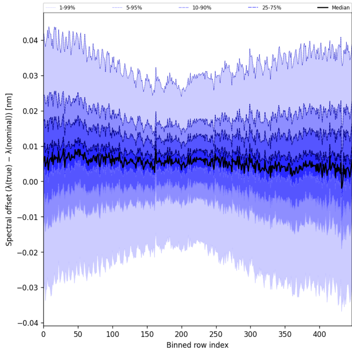
Figure 62: Along track statistics of “Spectral offset ( \lambda_{\text{true}} - \lambda_{\text{nominal}} )” for 2025-08-12 to 2025-08-14
