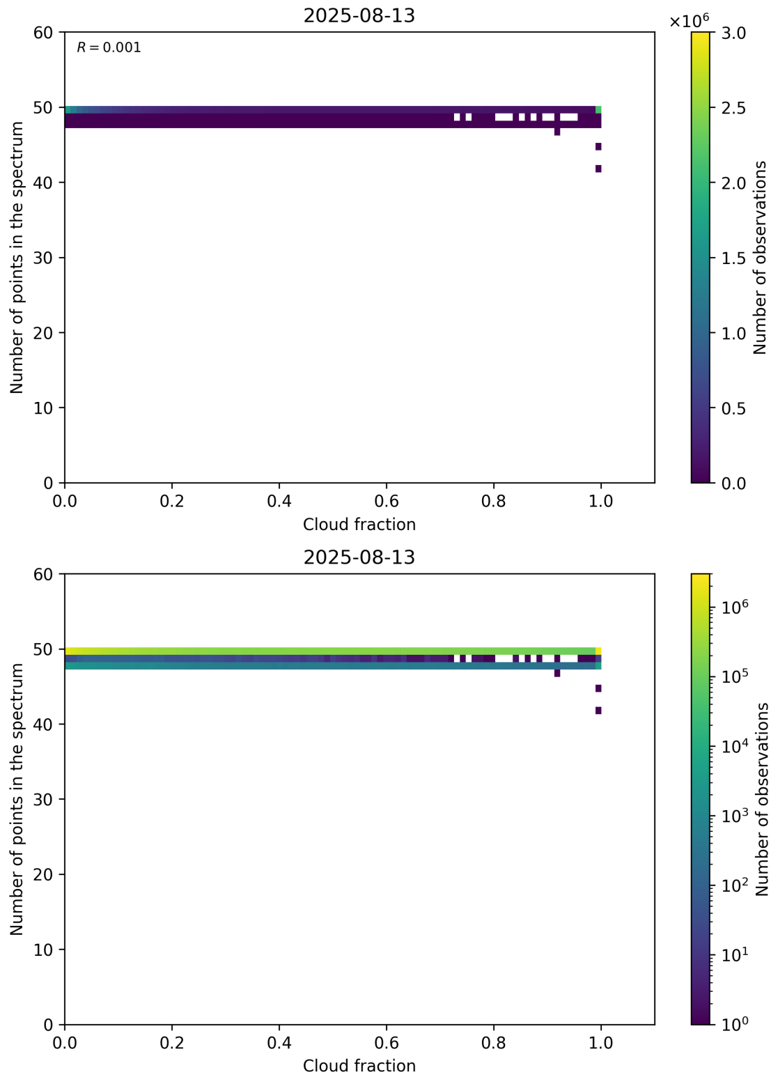
Figure 74: Scatter density plot of “Cloud fraction” against “Number of points in the spectrum” for 2025-08-12 to 2025-08-14.
