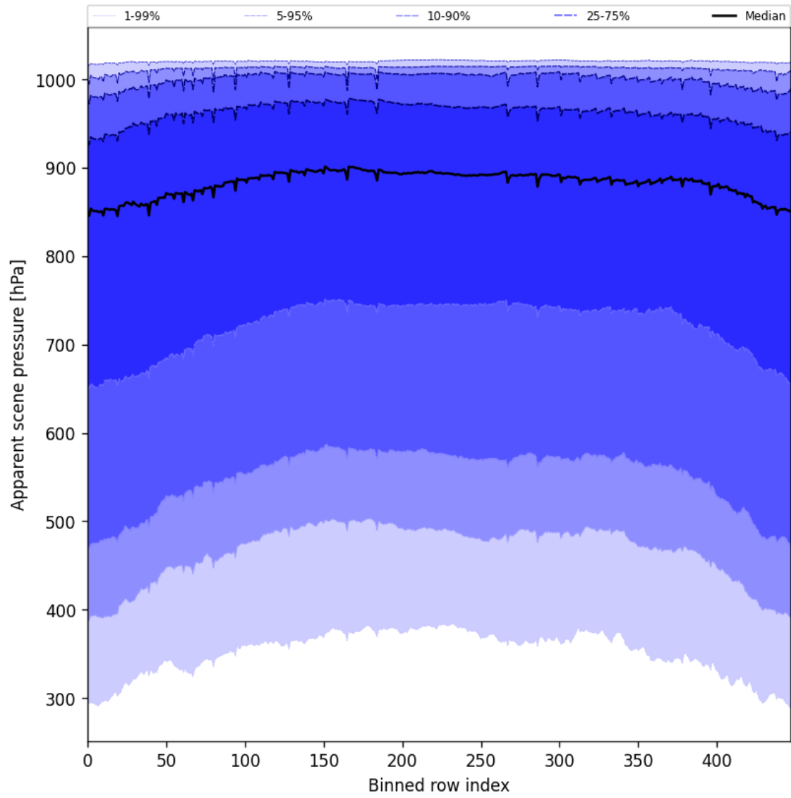
Figure 53: Along track statistics of “Apparent scene pressure” for 2025-08-12 to 2025-08-14
