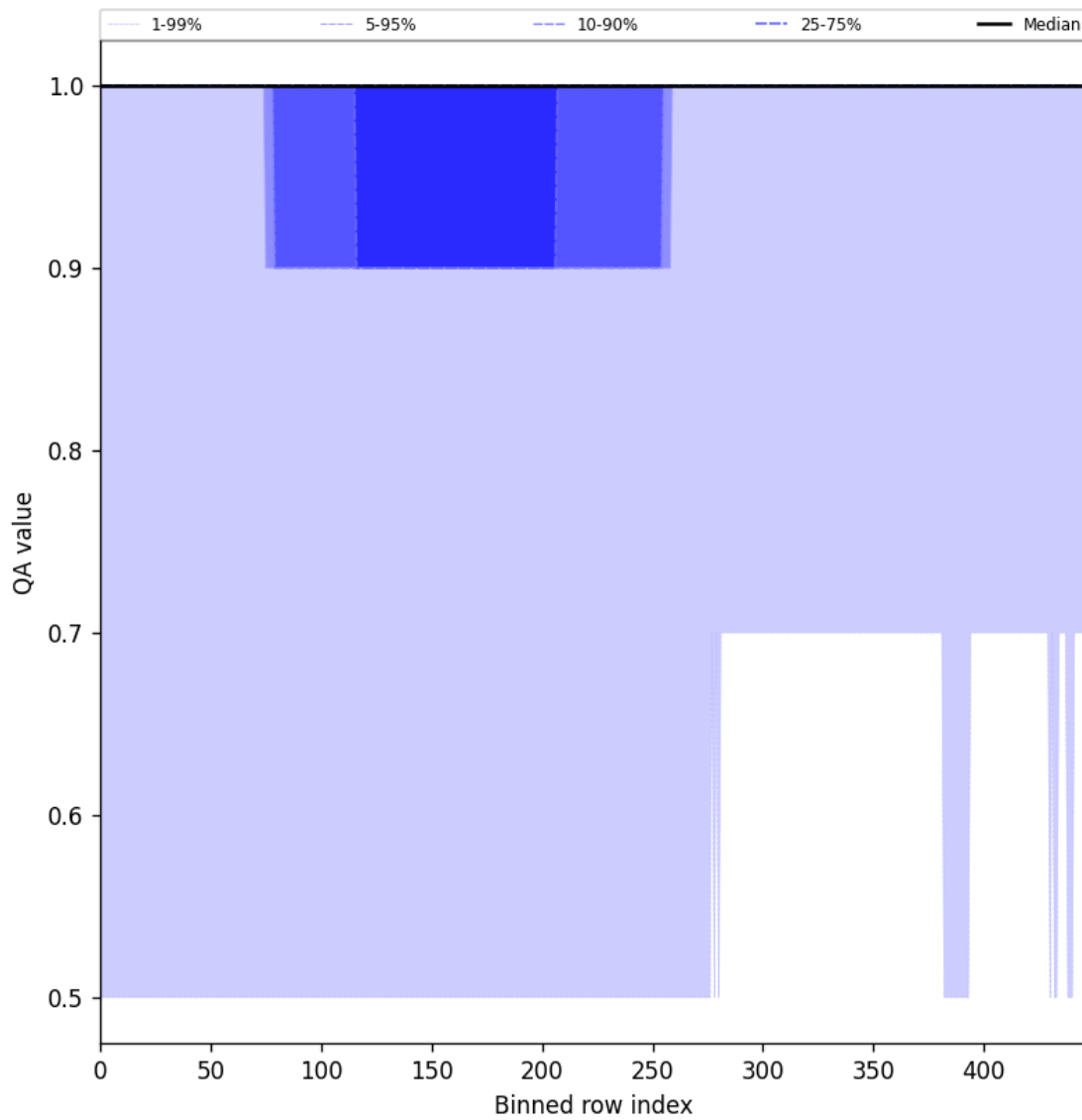
Figure 46: Along track statistics of “QA value” for 2025-08-12 to 2025-08-14
