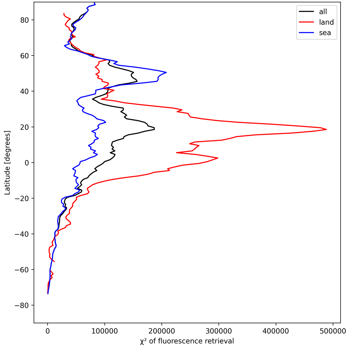
Figure 25: Zonal average of “ \chi^2 of fluorescence retrieval” for 2025-08-12 to 2025-08-14.
