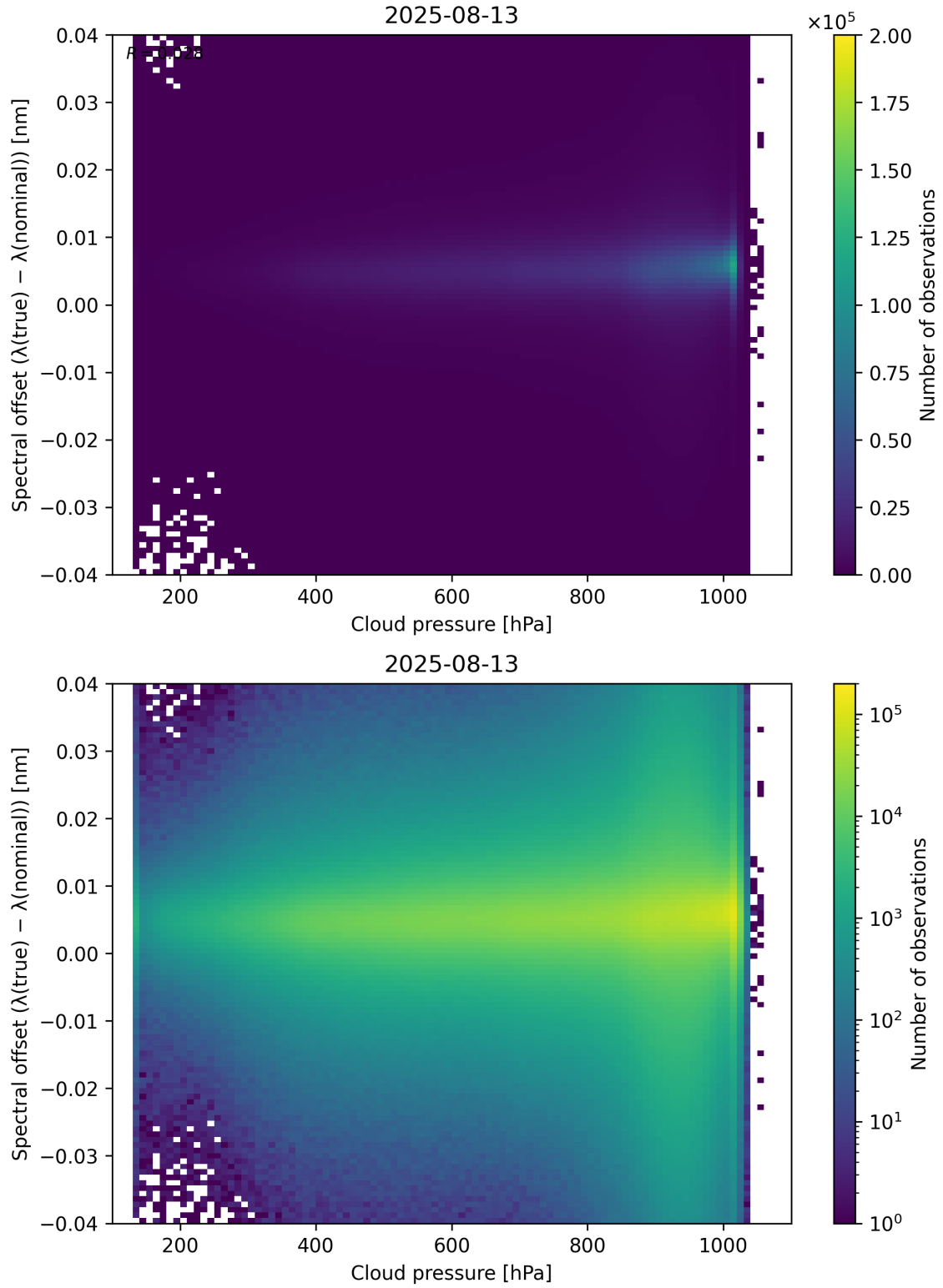
Figure 84: Scatter density plot of “Cloud pressure” against “Spectral offset ( \lambda_{\text{true}} - \lambda_{\text{nominal}} )” for 2025-08-12 to 2025-08-14.
