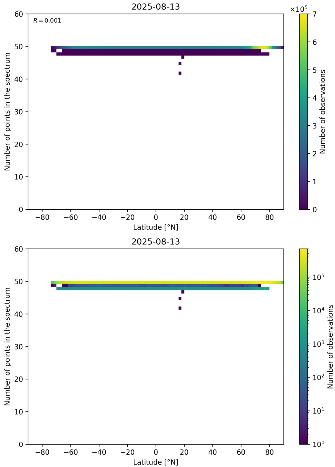
Figure 94: Scatter density plot of “Latitude” against “Number of points in the spectrum” for 2025-08-12 to 2025-08-14.
