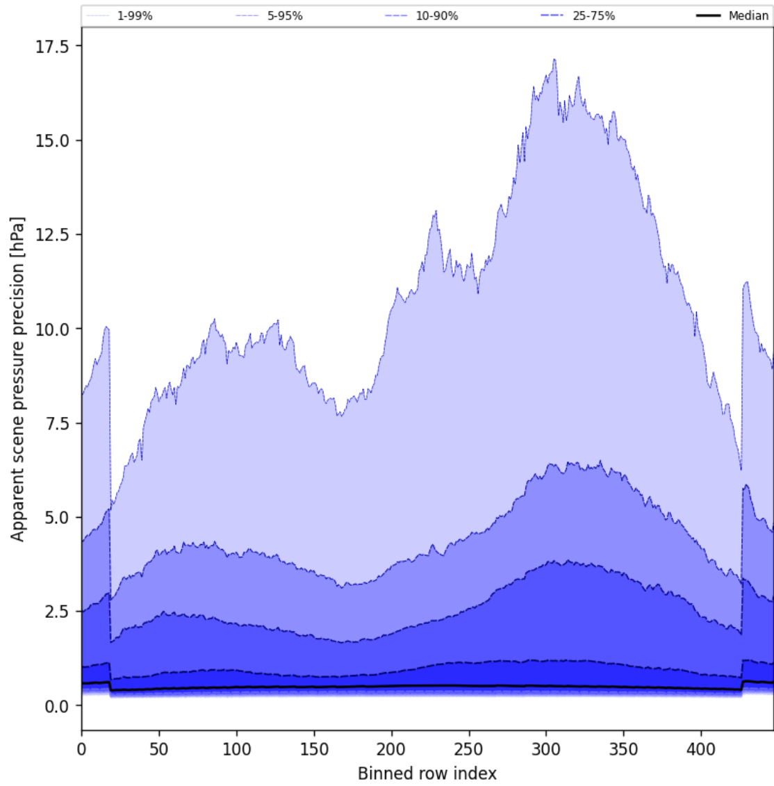
Figure 54: Along track statistics of “Apparent scene pressure precision” for 2025-08-12 to 2025-08-14
