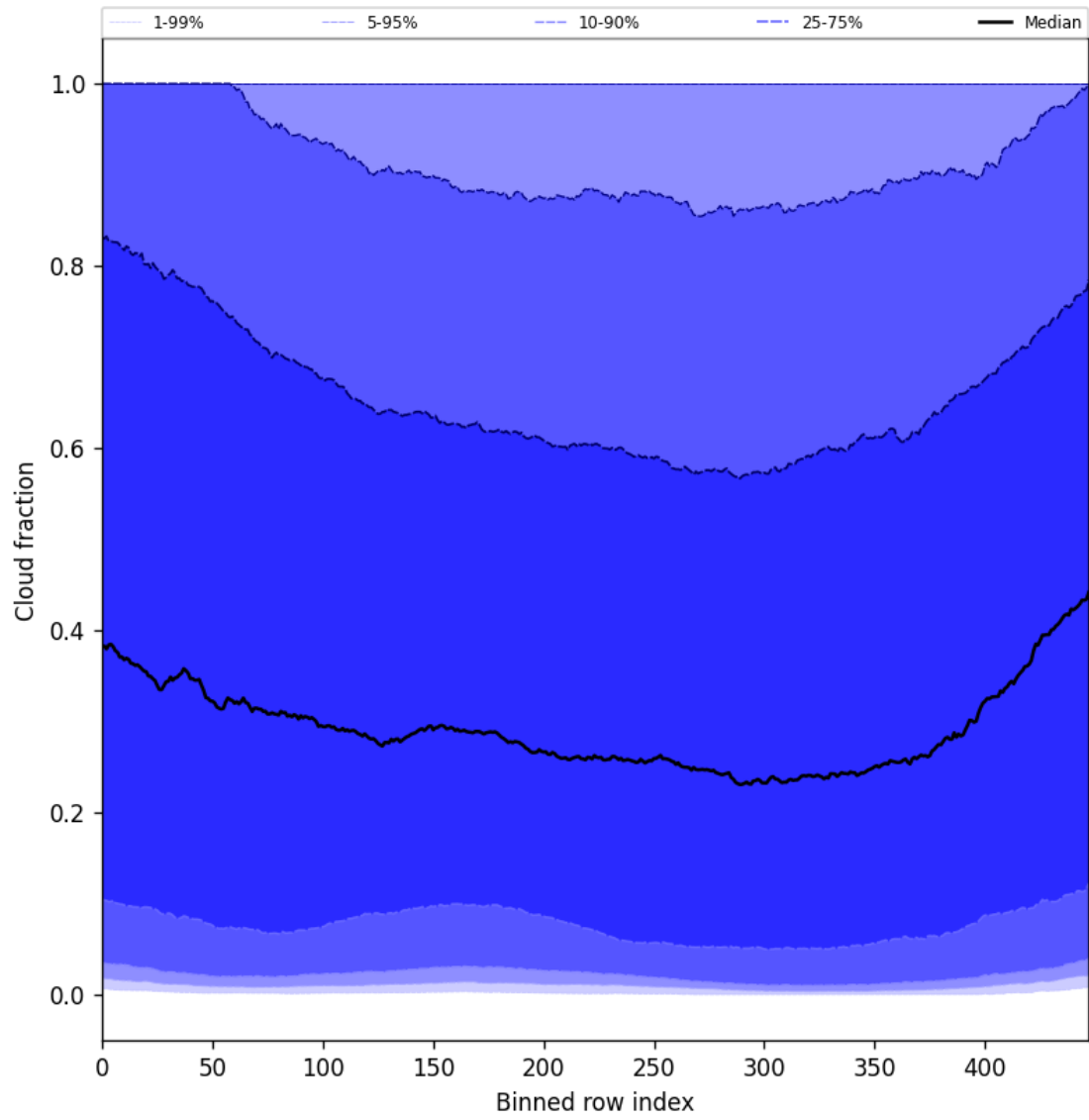
Figure 49: Along track statistics of “Cloud fraction” for 2025-08-12 to 2025-08-14
