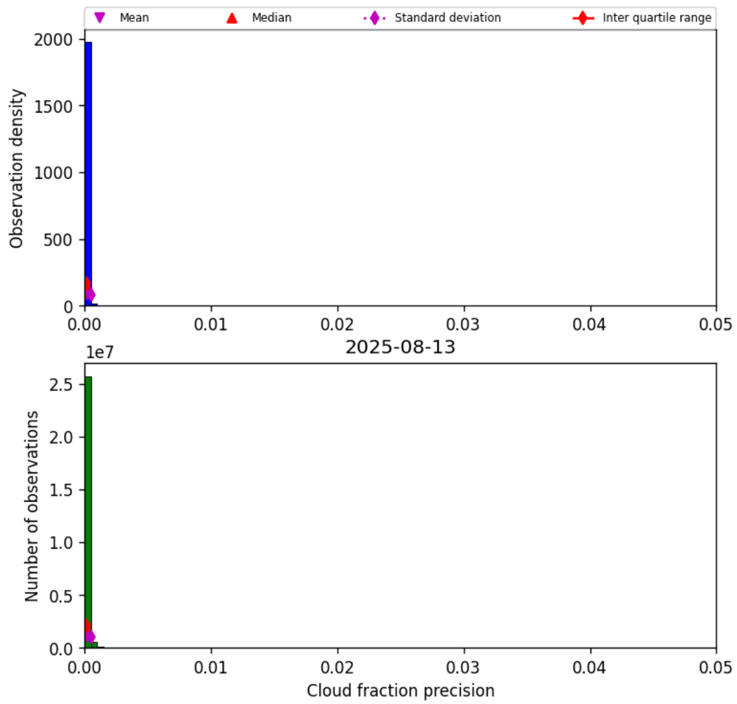
Figure 33: Histogram of “Cloud fraction precision” for 2025-08-12 to 2025-08-14
