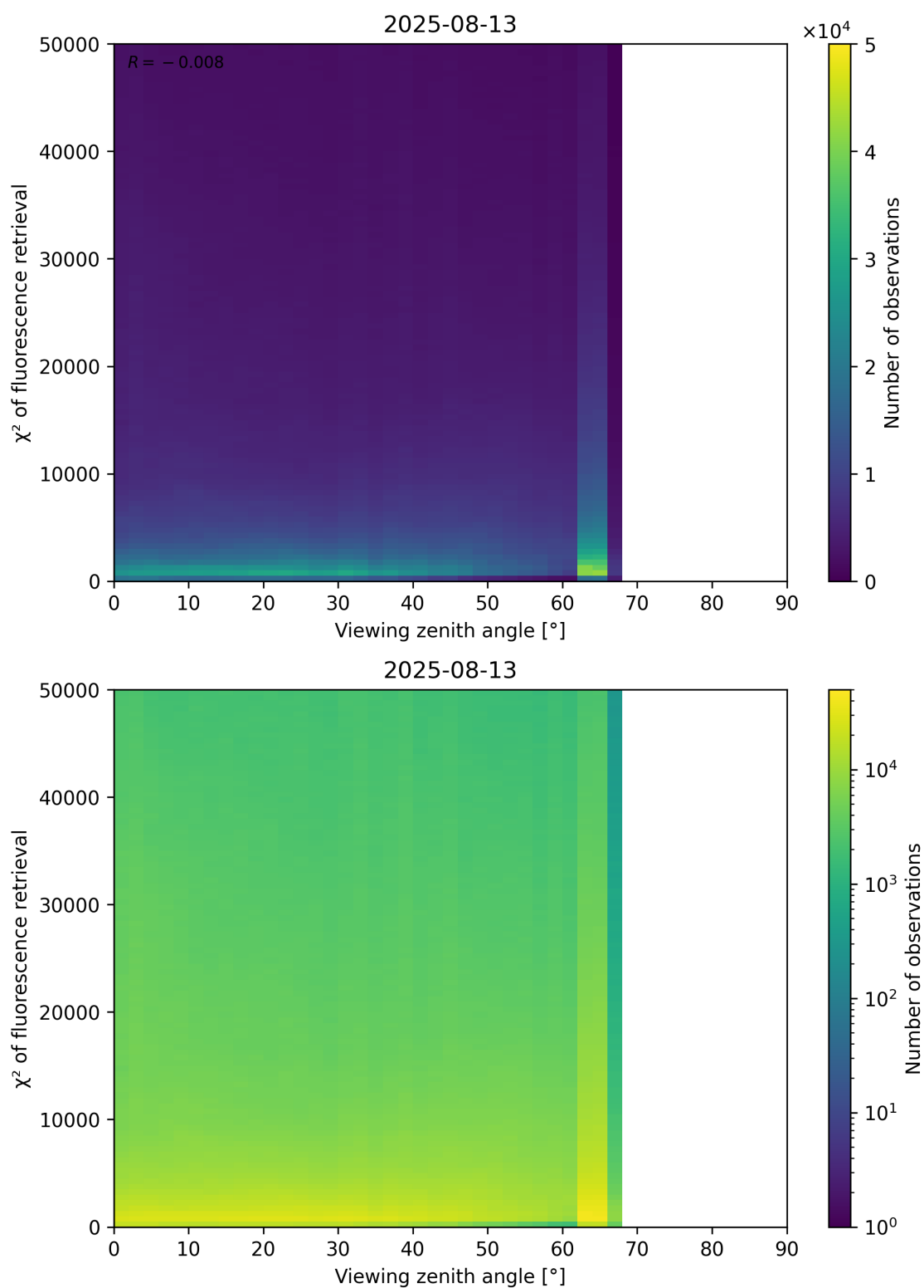
Figure 119: Scatter density plot of “Viewing zenith angle” against “ \chi^2 of fluorescence retrieval” for 2025-08-12 to 2025-08-14.
