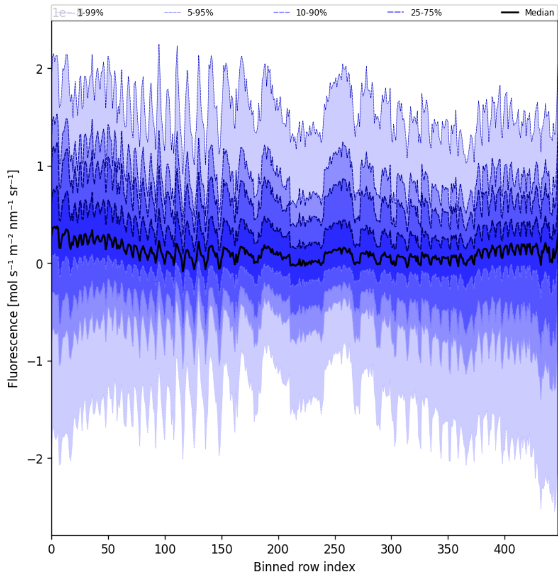
Figure 57: Along track statistics of “Fluorescence” for 2025-08-12 to 2025-08-14
