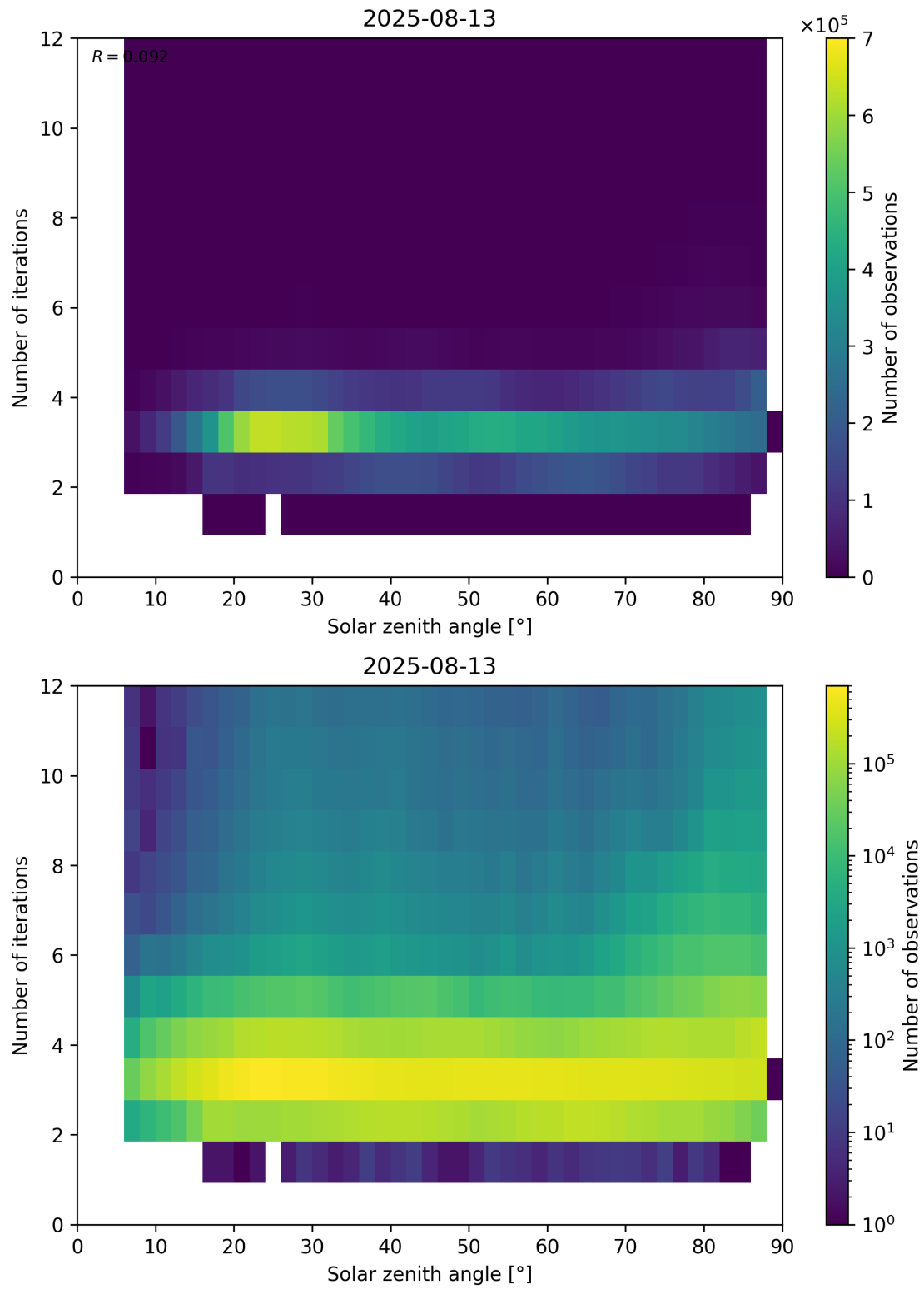
Figure 114: Scatter density plot of “Solar zenith angle” against “Number of iterations” for 2025-08-12 to 2025-08-14.
