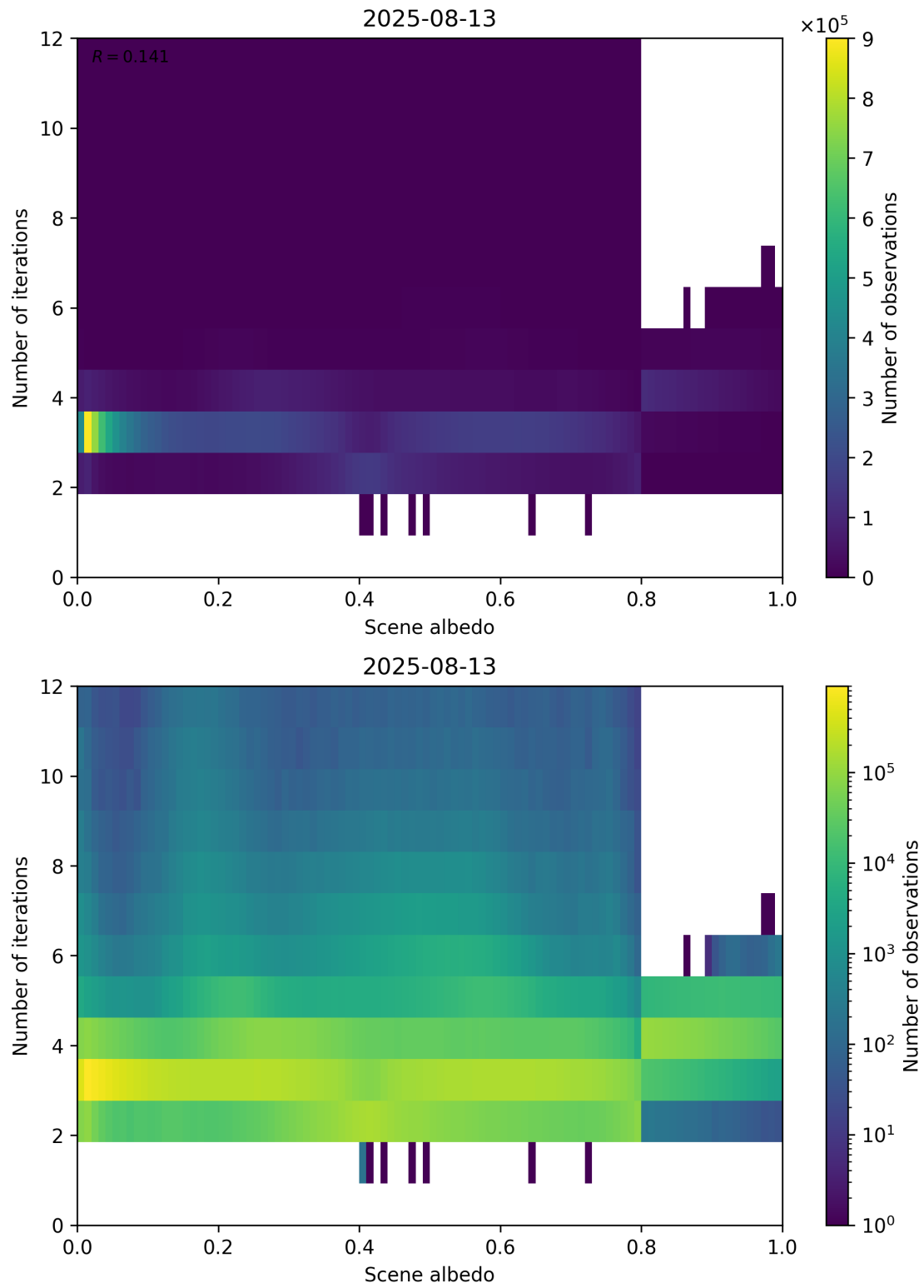
Figure 105: Scatter density plot of “Scene albedo” against “Number of iterations” for 2025-08-12 to 2025-08-14.
