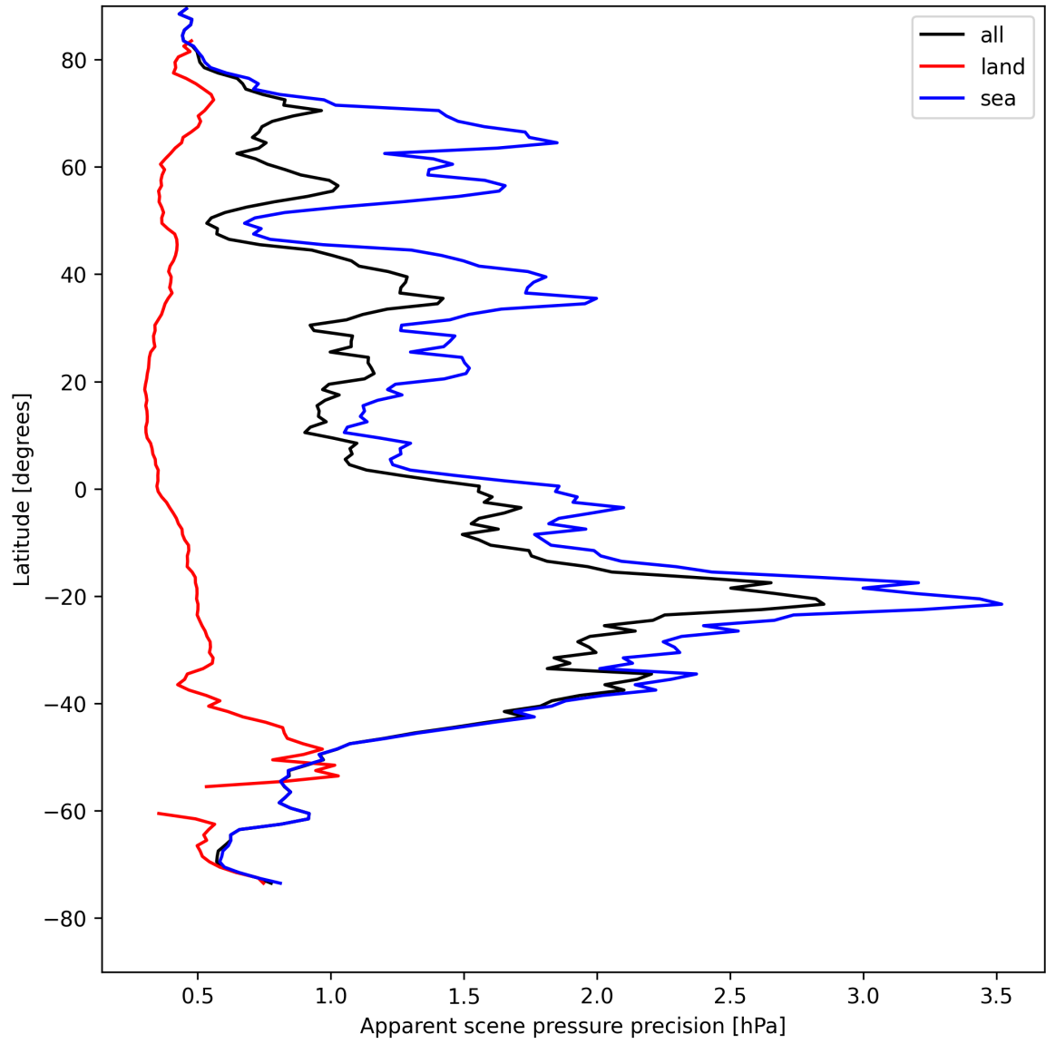
Figure 20: Zonal average of “Apparent scene pressure precision” for 2025-08-12 to 2025-08-14.
