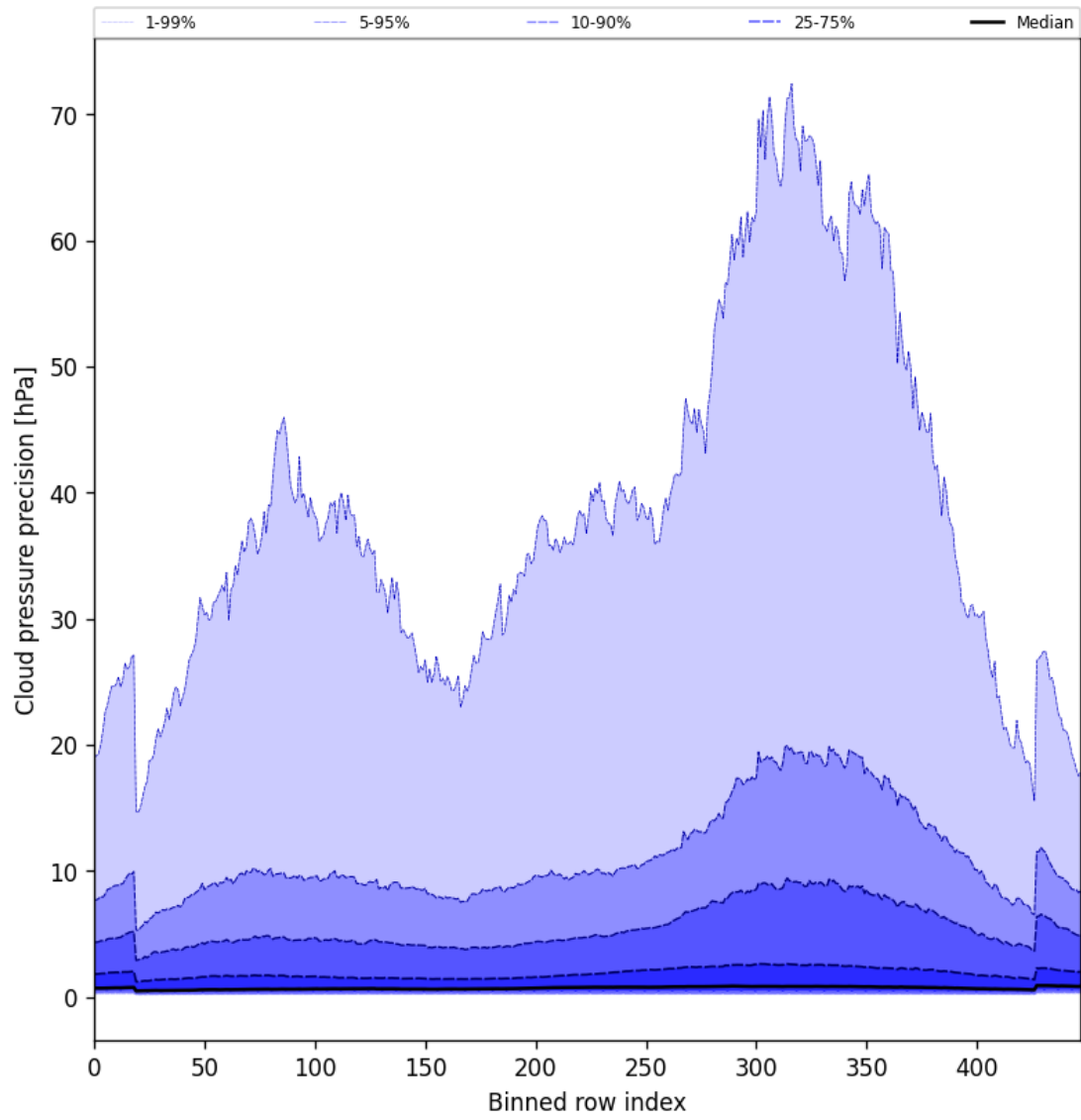
Figure 48: Along track statistics of “Cloud pressure precision” for 2025-08-12 to 2025-08-14
