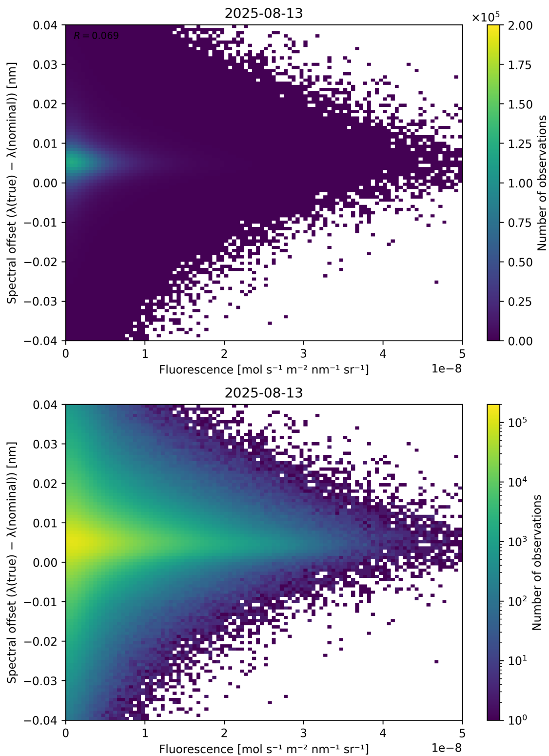
Figure 87: Scatter density plot of “Fluorescence” against “Spectral offset ( \lambda_{\text{true}} - \lambda_{\text{nominal}} )” for 2025-08-12 to 2025-08-14.
