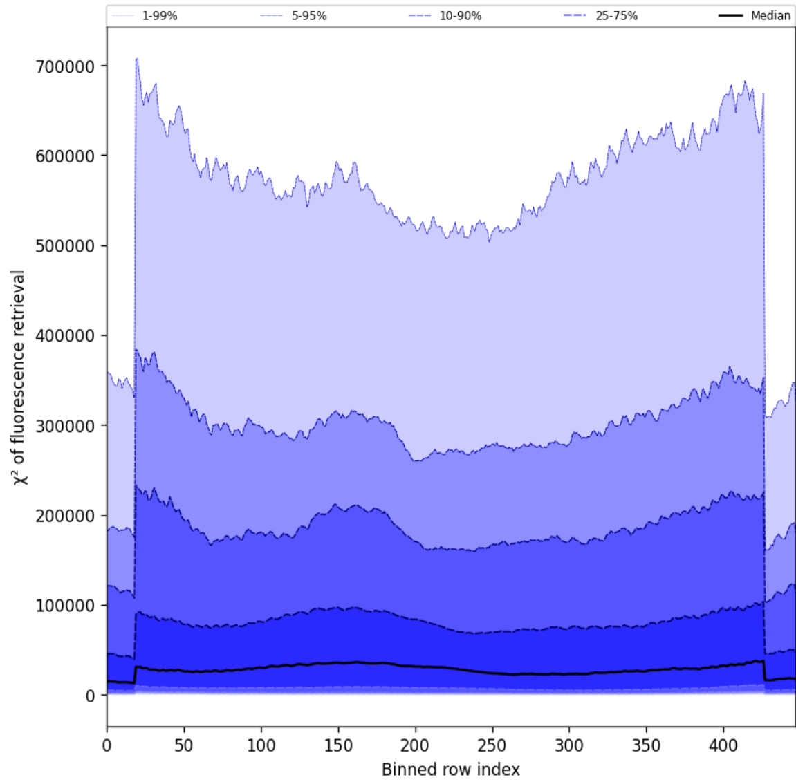
Figure 59: Along track statistics of “ \chi^2 of fluorescence retrieval” for 2025-08-12 to 2025-08-14
