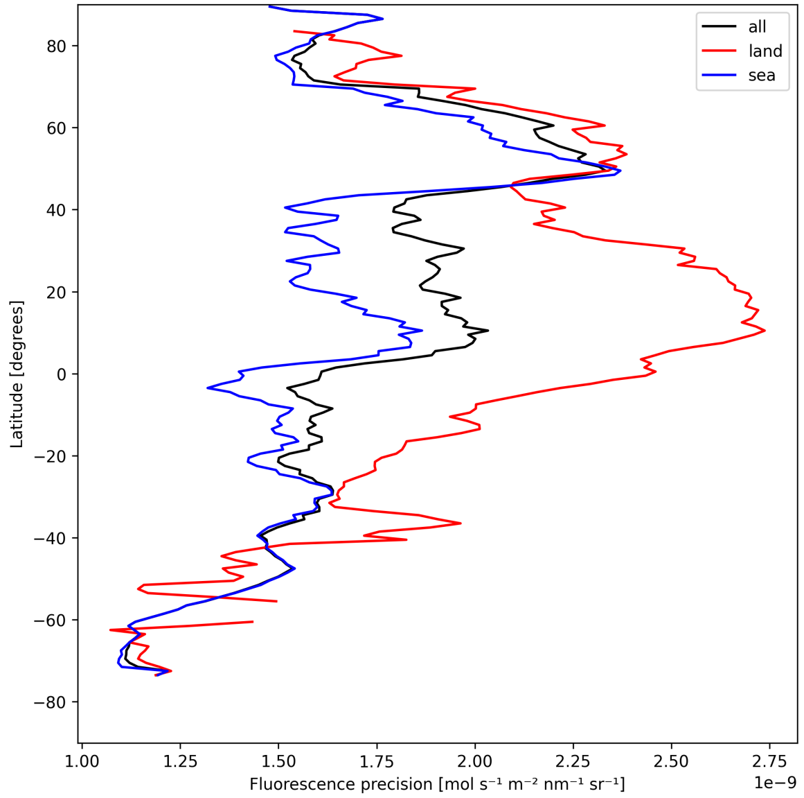
Figure 24: Zonal average of “Fluorescence precision” for 2025-08-12 to 2025-08-14.
