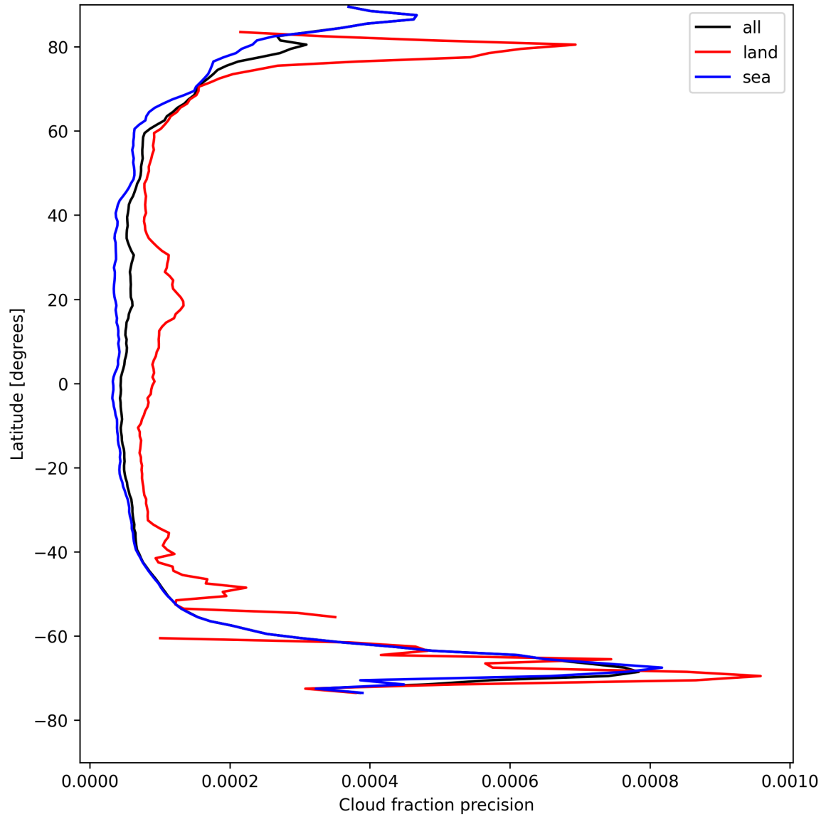
Figure 16: Zonal average of “Cloud fraction precision” for 2025-08-12 to 2025-08-14.
