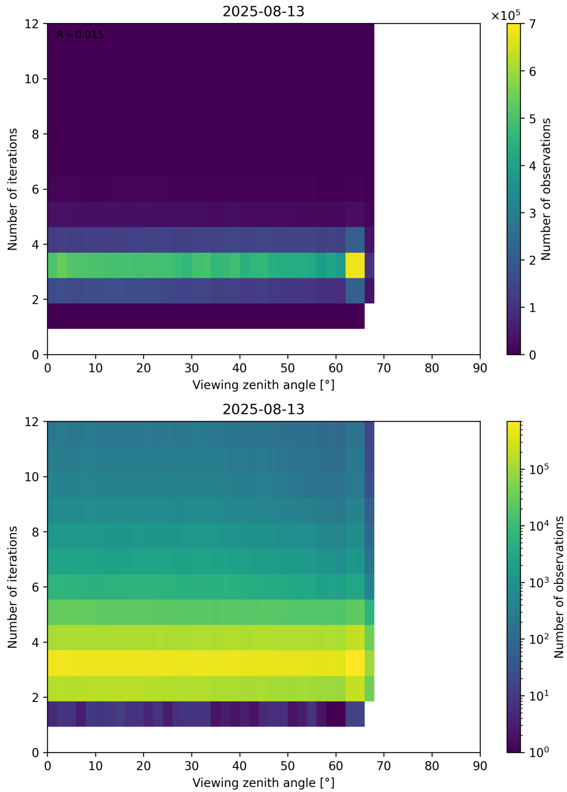
Figure 124: Scatter density plot of “Viewing zenith angle” against “Number of iterations” for 2025-08-12 to 2025-08-14.
