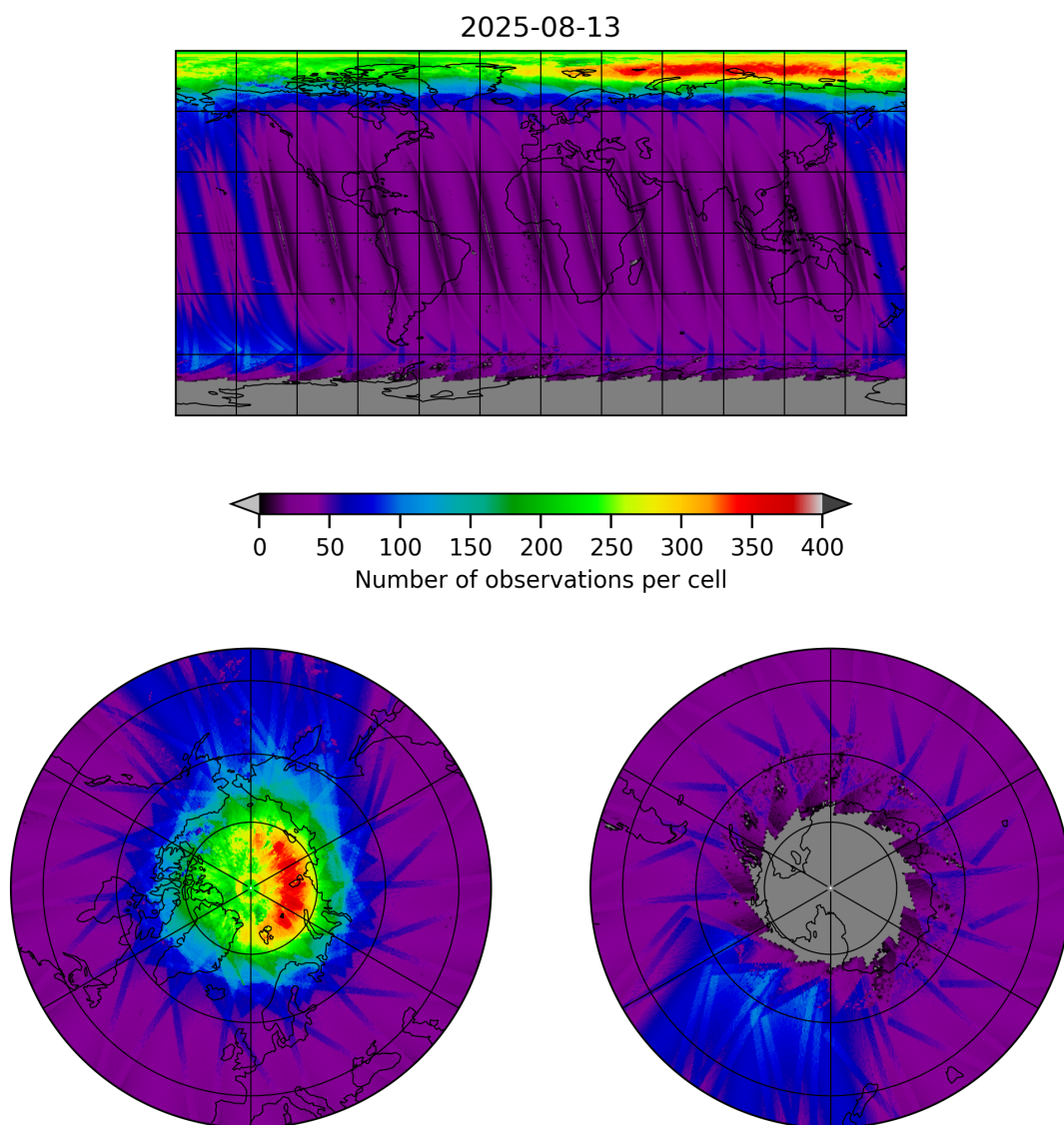
Figure 11: Map of the number of observations for 2025-08-12 to 2025-08-14
