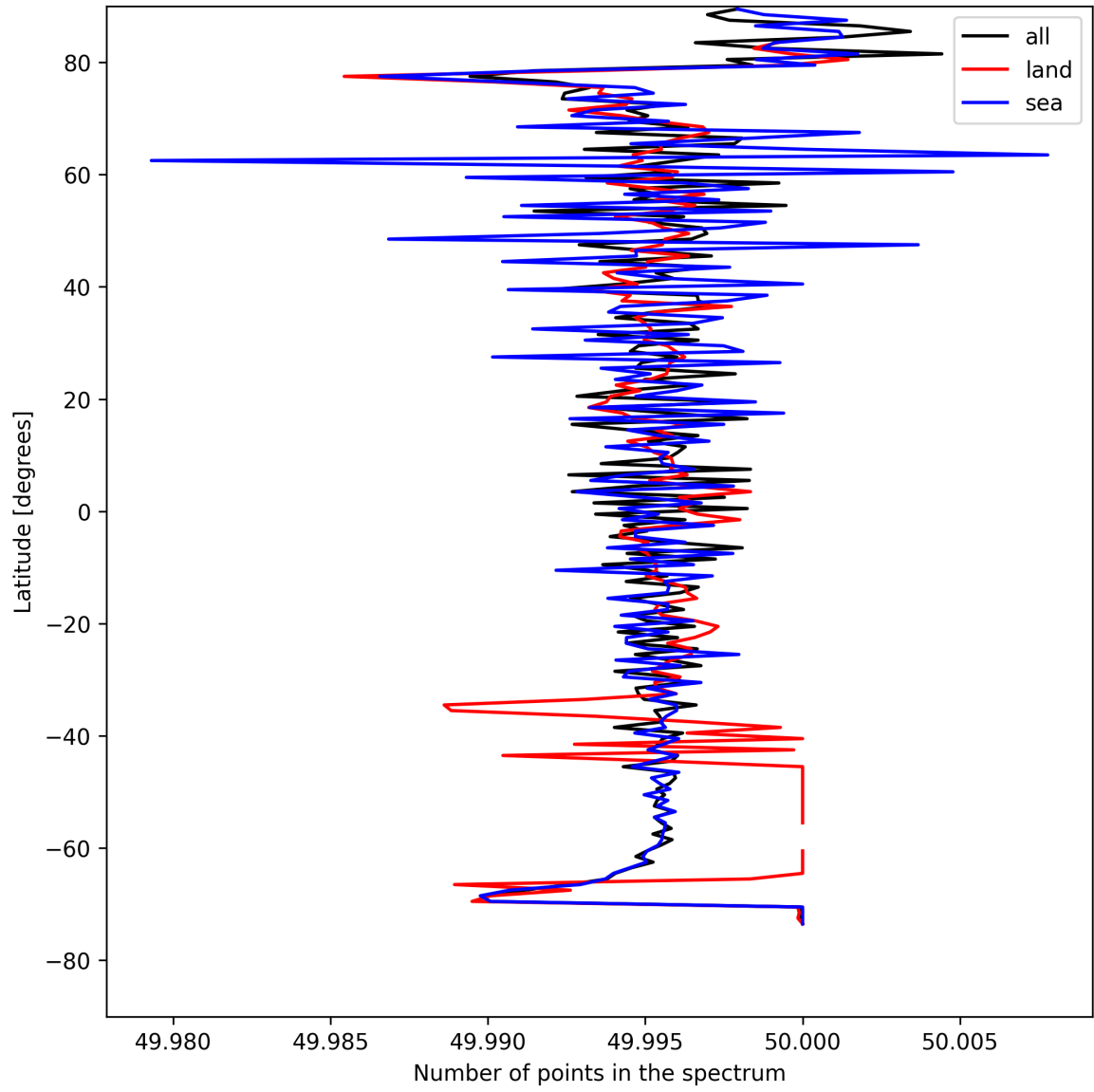
Figure 27: Zonal average of “Number of points in the spectrum” for 2025-08-12 to 2025-08-14.
