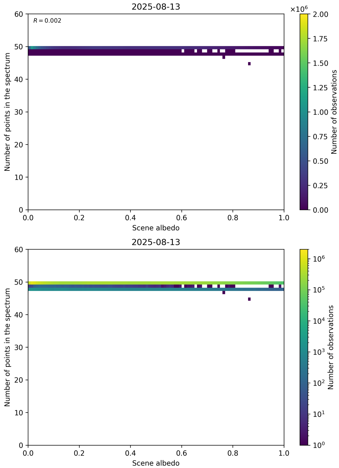
Figure 106: Scatter density plot of “Scene albedo” against “Number of points in the spectrum” for 2025-08-12 to 2025-08-14.
