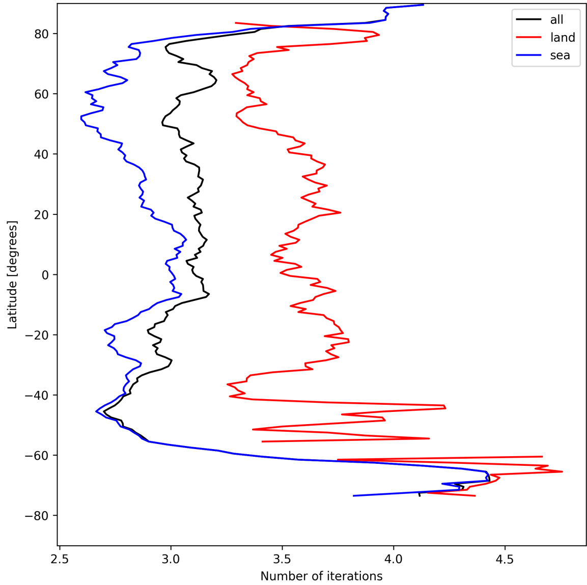
Figure 22: Zonal average of “Number of iterations” for 2025-08-12 to 2025-08-14.
