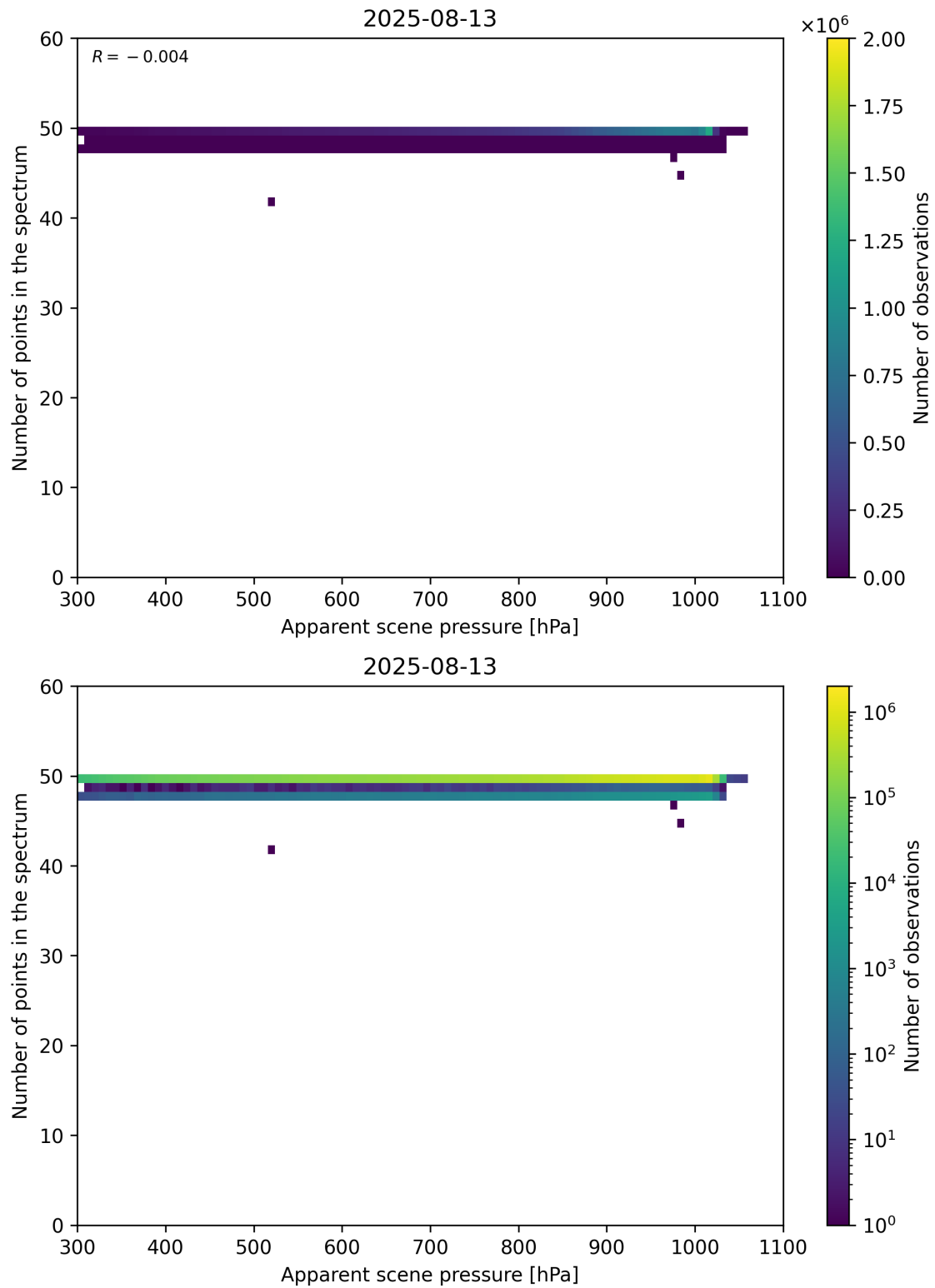
Figure 66: Scatter density plot of “Apparent scene pressure” against “Number of points in the spectrum” for 2025-08-12 to 2025-08-14.
