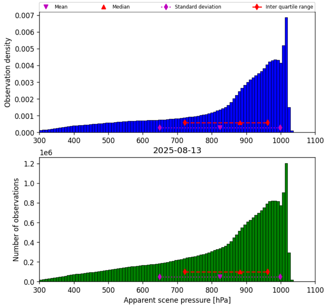
Figure 36: Histogram of “Apparent scene pressure” for 2025-08-12 to 2025-08-14
