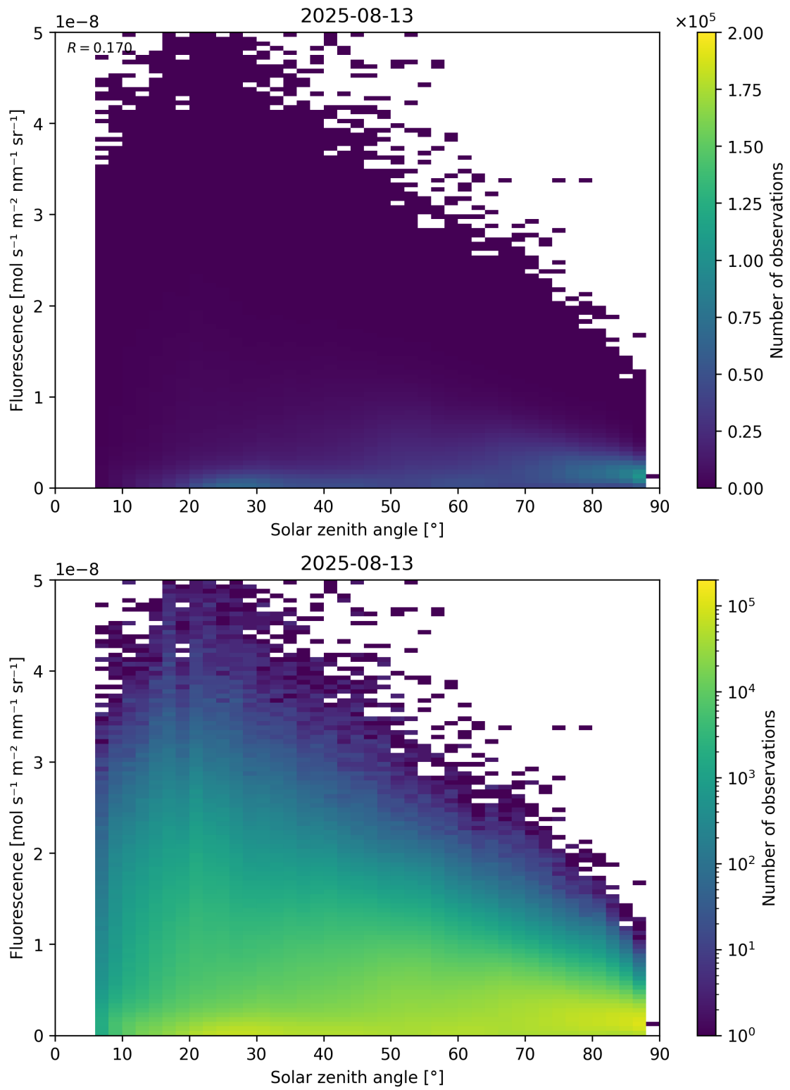
Figure 112: Scatter density plot of “Solar zenith angle” against “Fluorescence” for 2025-08-12 to 2025-08-14.
