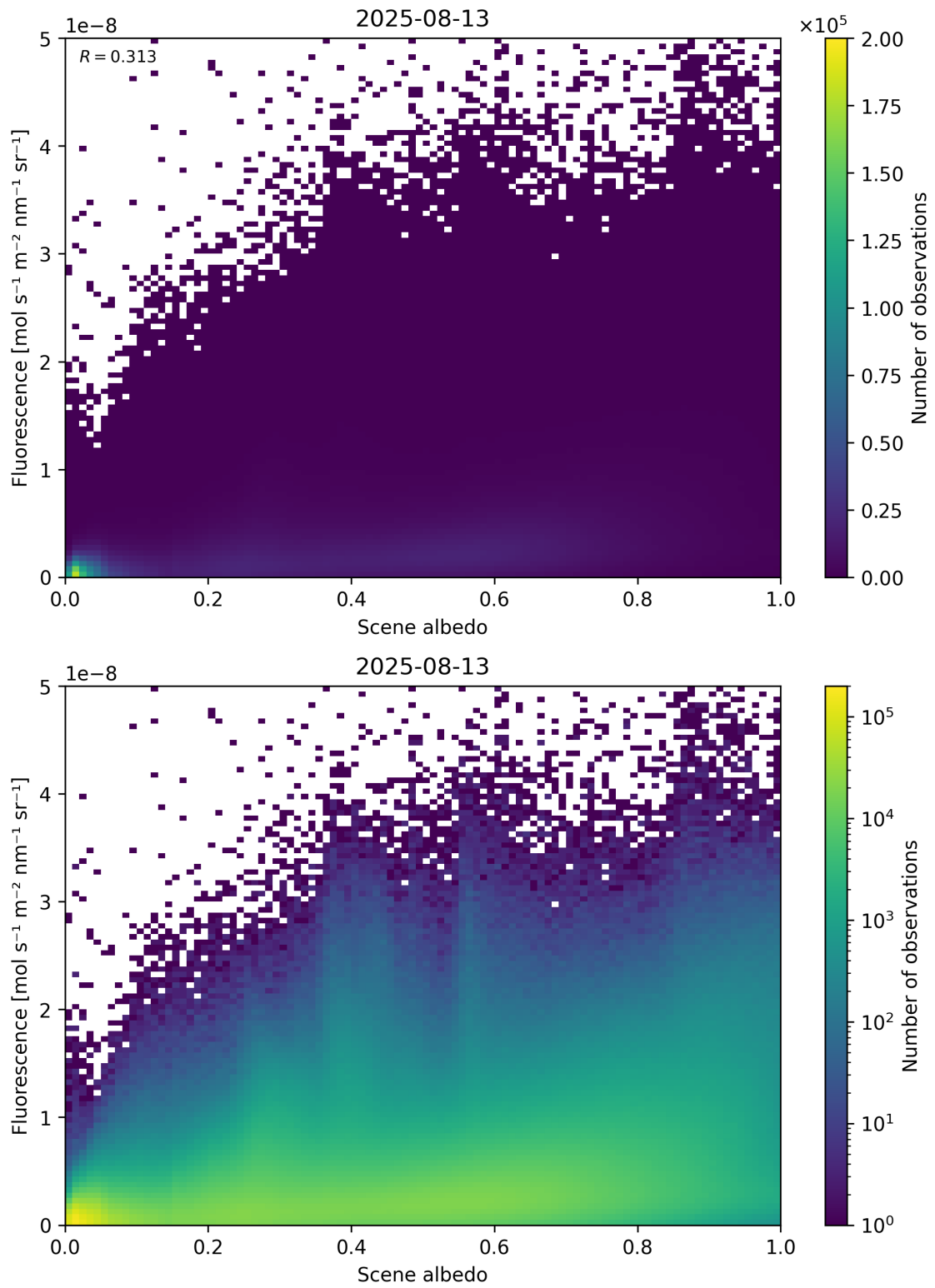
Figure 104: Scatter density plot of “Scene albedo” against “Fluorescence” for 2025-08-12 to 2025-08-14.
