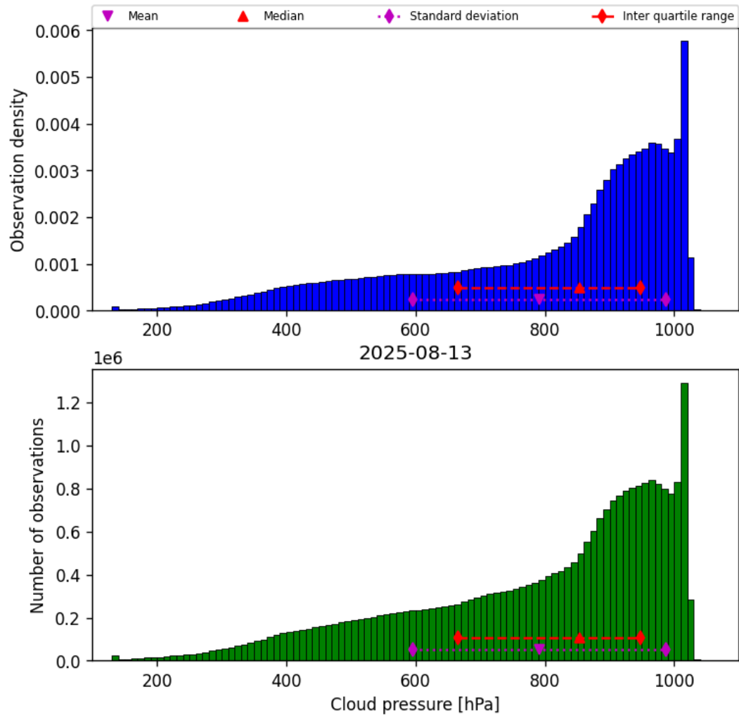
Figure 30: Histogram of “Cloud pressure” for 2025-08-12 to 2025-08-14
