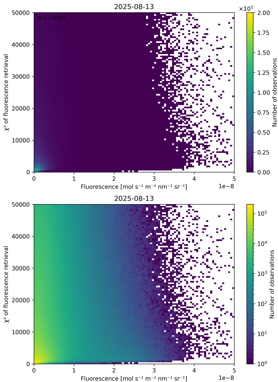
Figure 85: Scatter density plot of “Fluorescence” against “ \chi^2 of fluorescence retrieval” for 2025-08-12 to 2025-08-14.
