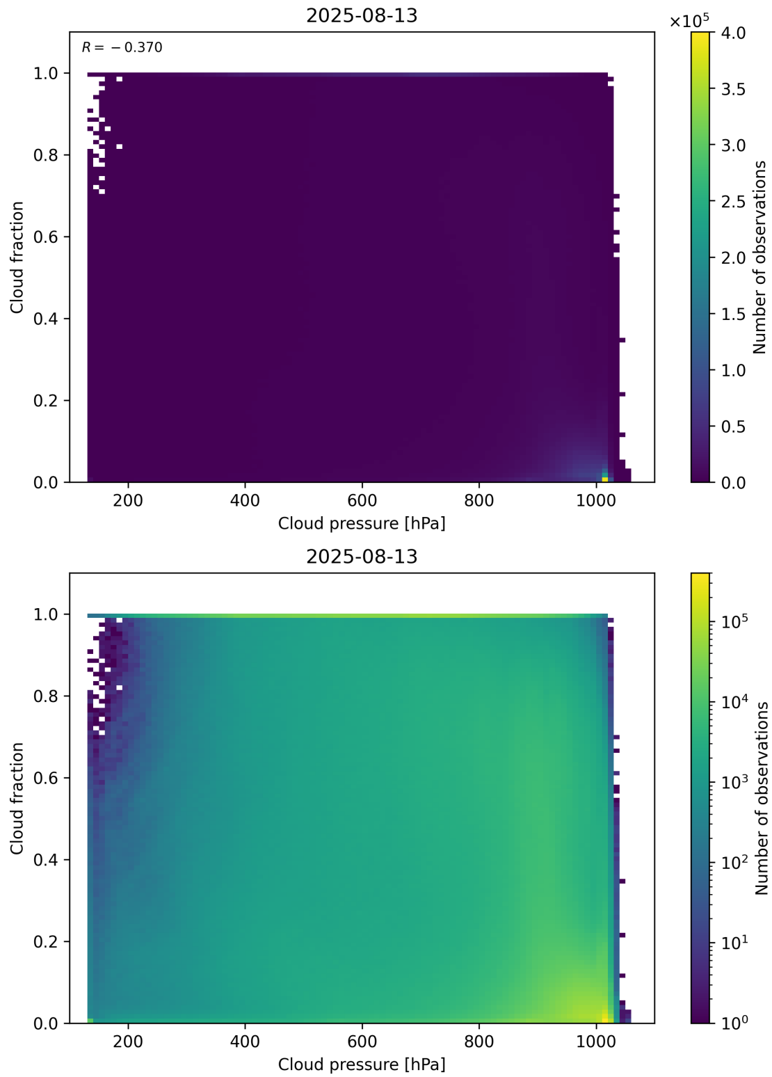
Figure 79: Scatter density plot of “Cloud pressure” against “Cloud fraction” for 2025-08-12 to 2025-08-14.
