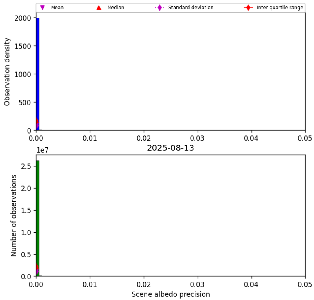
Figure 35: Histogram of “Scene albedo precision” for 2025-08-12 to 2025-08-14
