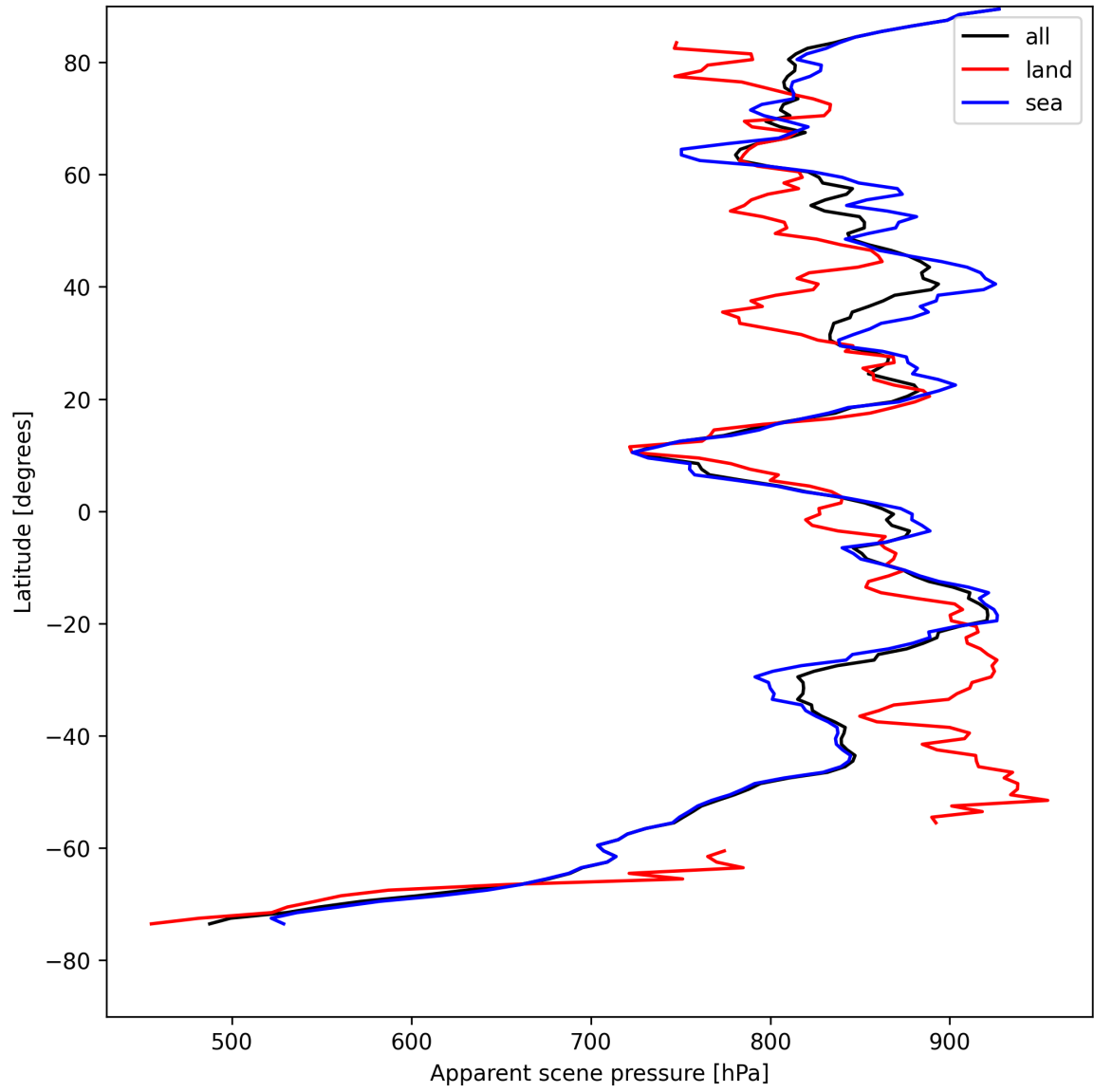
Figure 19: Zonal average of “Apparent scene pressure” for 2025-08-12 to 2025-08-14.
