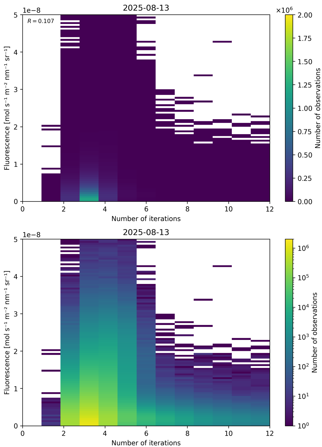
Figure 98: Scatter density plot of “Number of iterations” against “Fluorescence” for 2025-08-12 to 2025-08-14.
