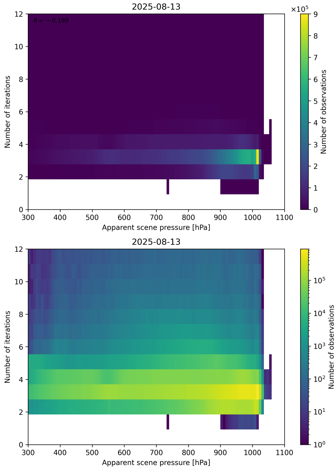
Figure 65: Scatter density plot of “Apparent scene pressure” against “Number of iterations” for 2025-08-12 to 2025-08-14.
