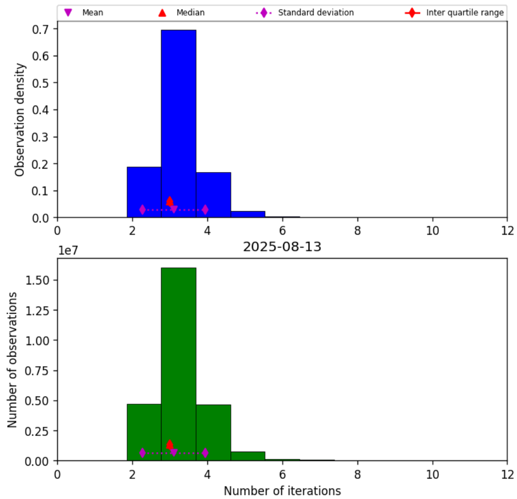
Figure 39: Histogram of “Number of iterations” for 2025-08-12 to 2025-08-14
