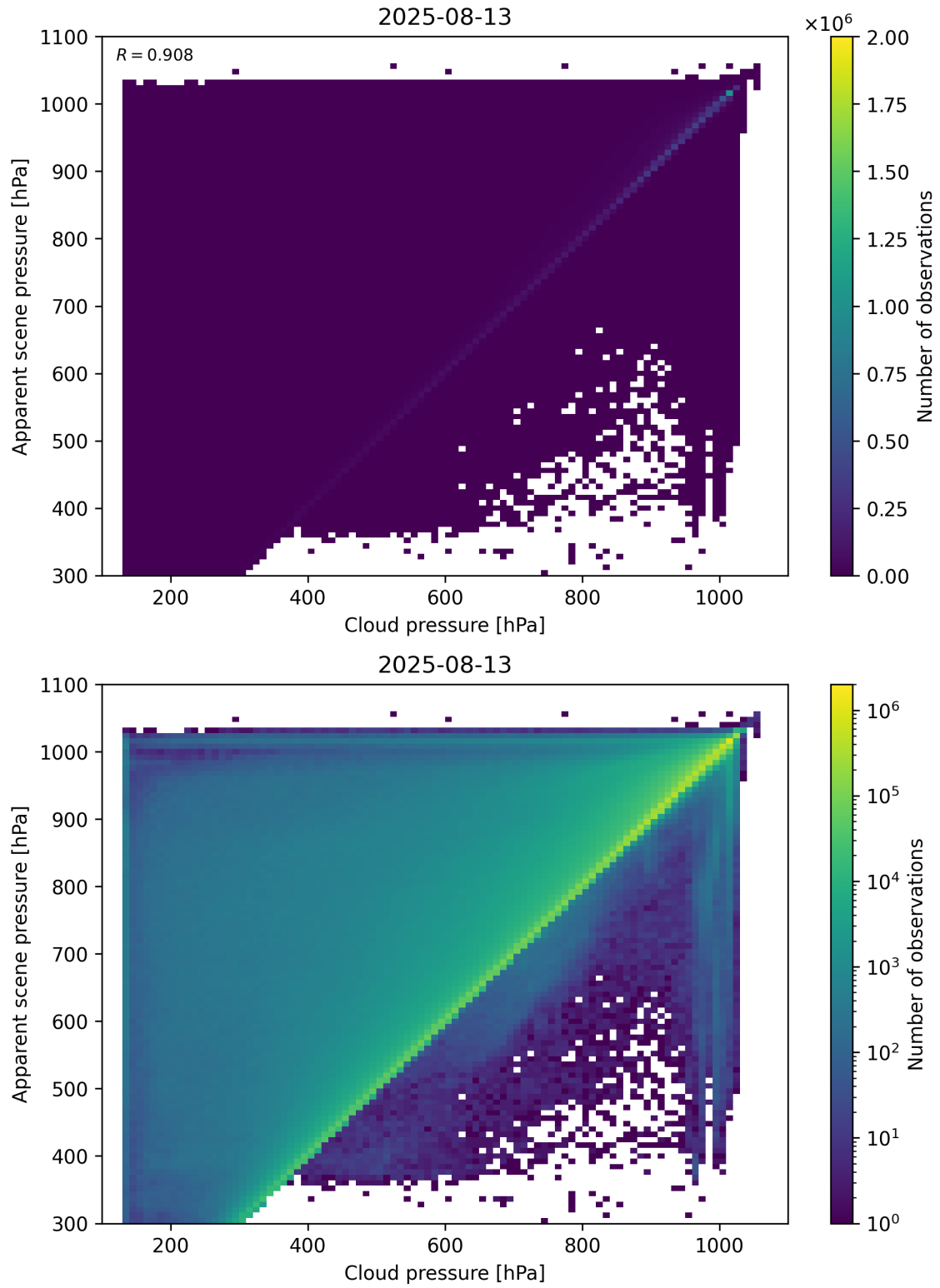
Figure 77: Scatter density plot of “Cloud pressure” against “Apparent scene pressure” for 2025-08-12 to 2025-08-14.
