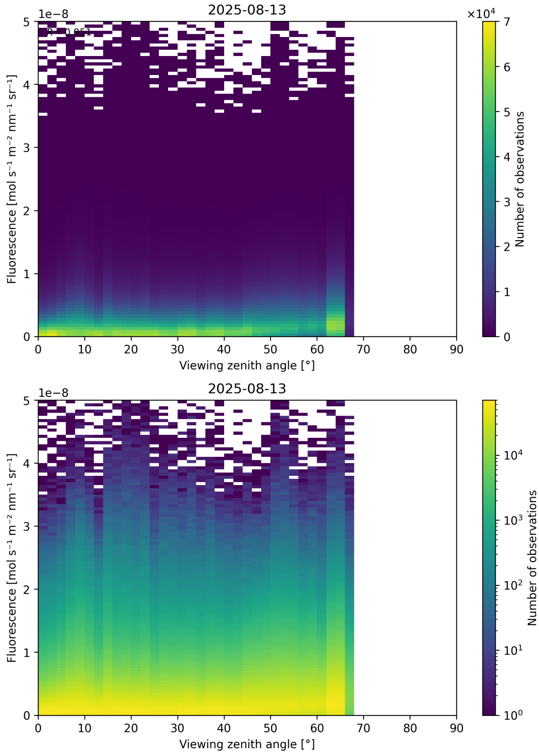
Figure 122: Scatter density plot of “Viewing zenith angle” against “Fluorescence” for 2025-08-12 to 2025-08-14.
