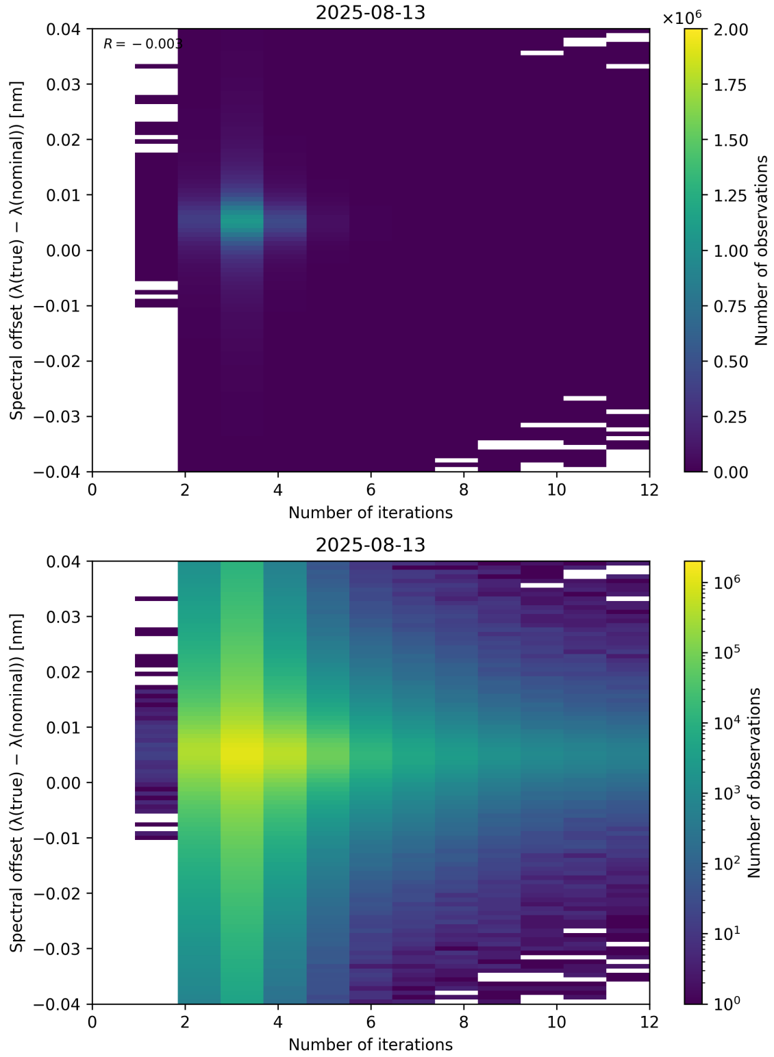
Figure 100: Scatter density plot of “Number of iterations” against “Spectral offset ( \lambda_{\text{true}} - \lambda_{\text{nominal}} )” for 2025-08-12 to 2025-08-14.
