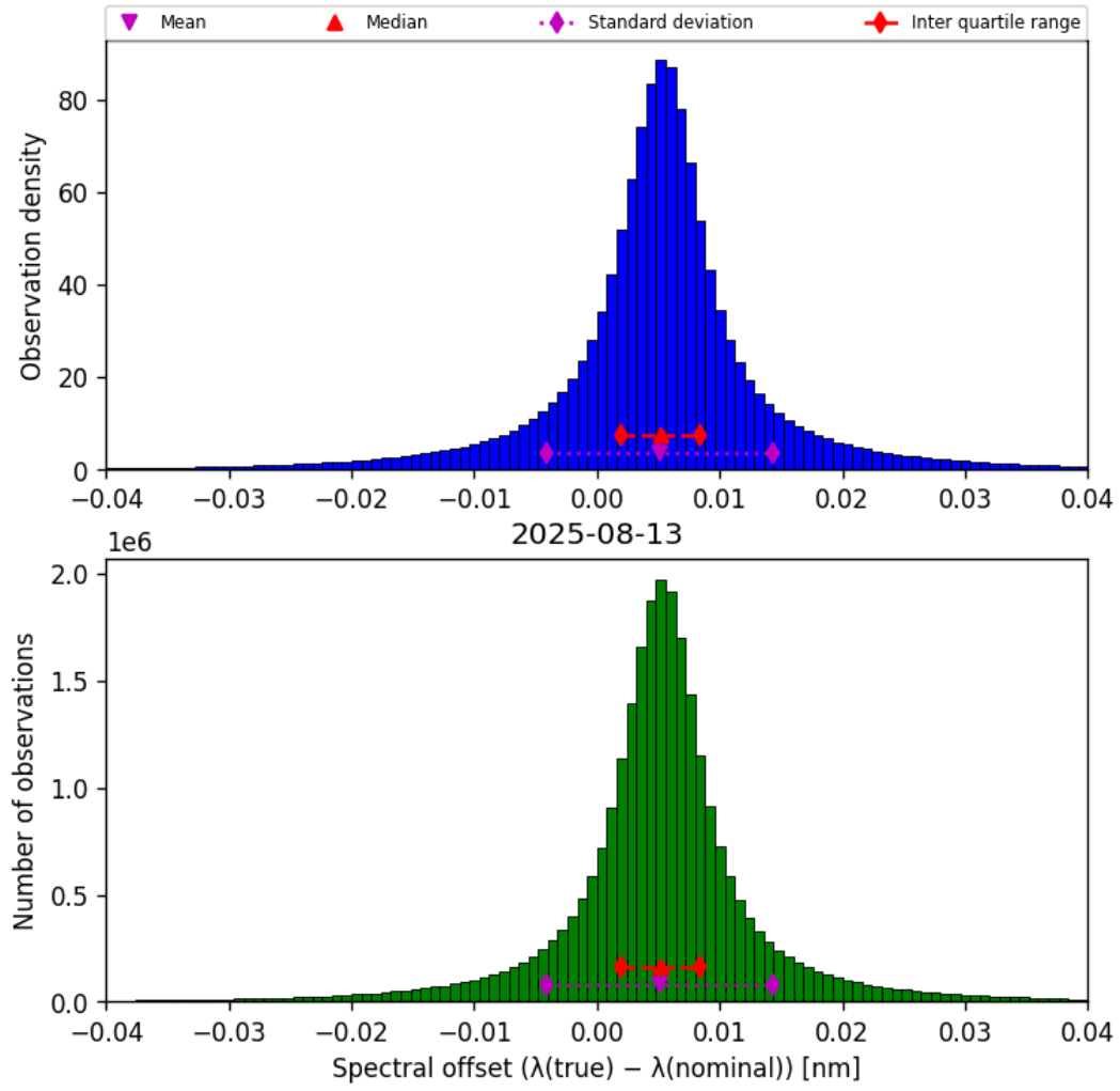
Figure 45: Histogram of “Spectral offset ( \lambda_{\text{true}} - \lambda_{\text{nominal}} )” for 2025-08-12 to 2025-08-14
