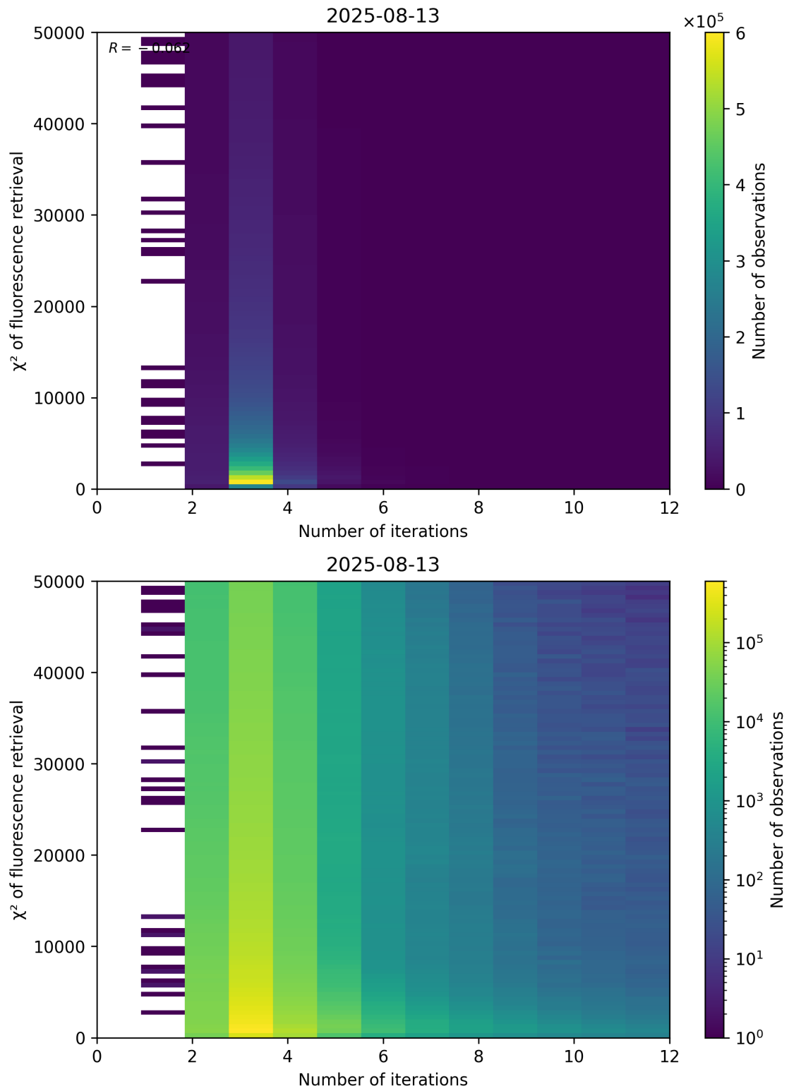
Figure 97: Scatter density plot of “Number of iterations” against “ \chi^2 of fluorescence retrieval” for 2025-08-12 to 2025-08-14.
