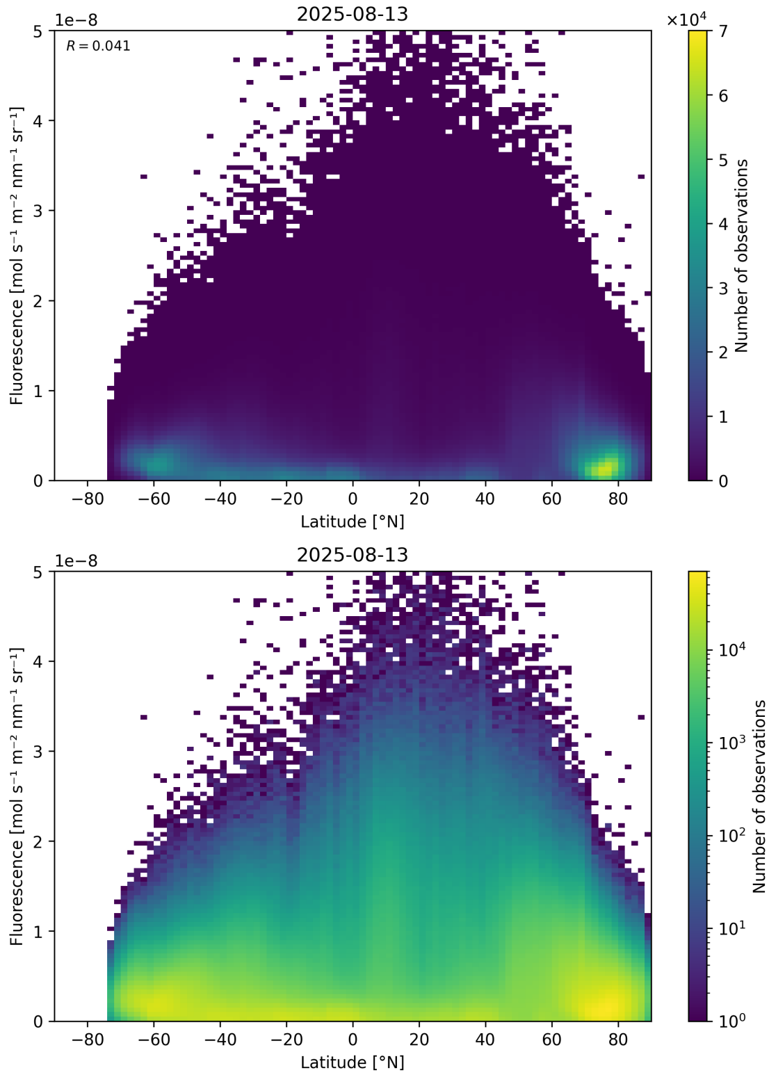
Figure 92: Scatter density plot of “Latitude” against “Fluorescence” for 2025-08-12 to 2025-08-14.
