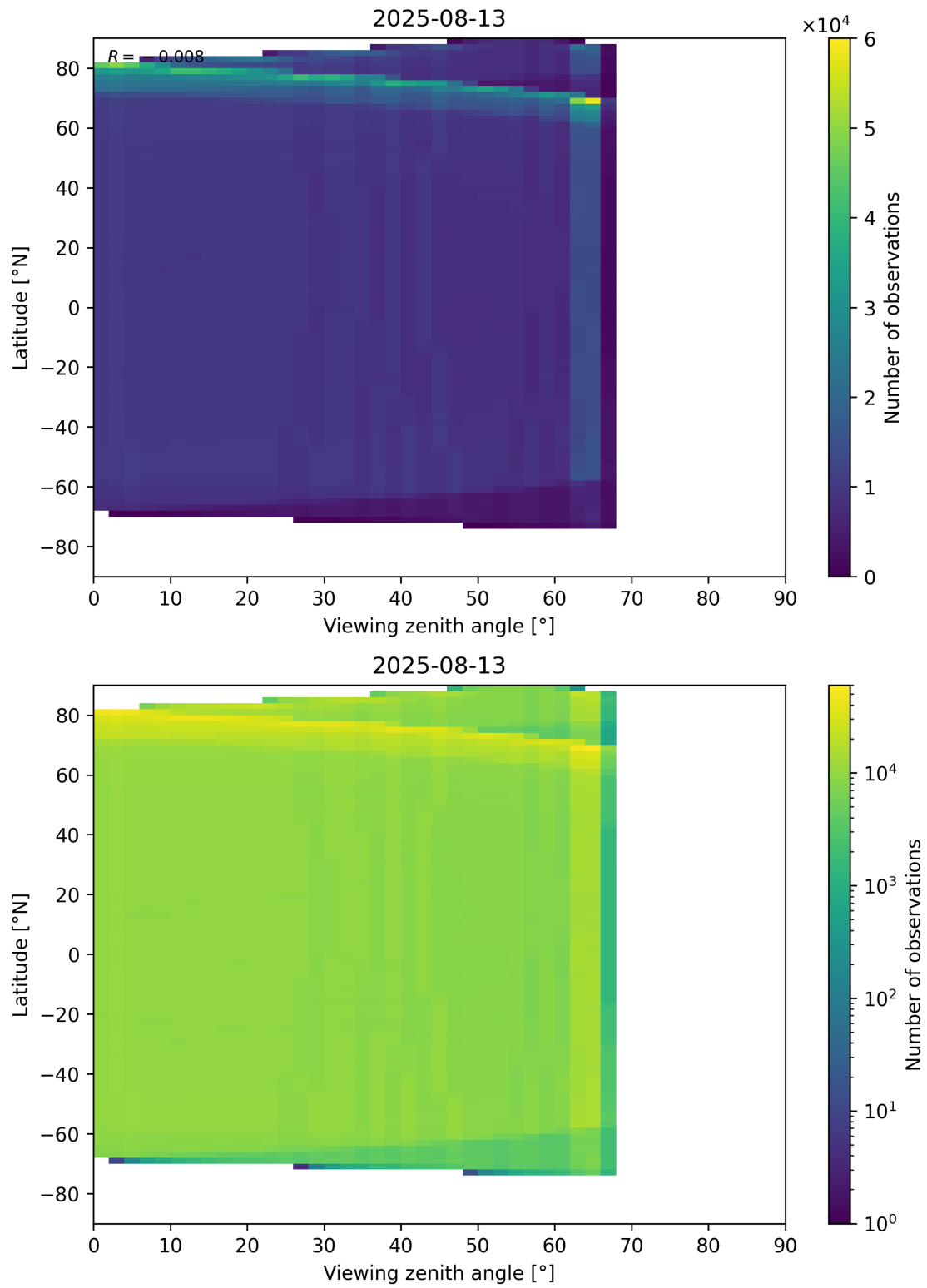
Figure 123: Scatter density plot of “Viewing zenith angle” against “Latitude” for 2025-08-12 to 2025-08-14.
