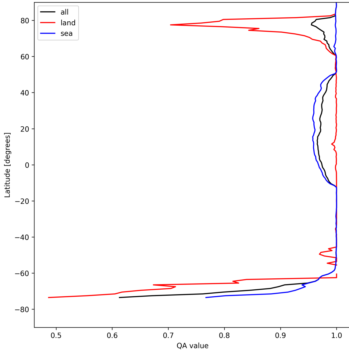
Figure 12: Zonal average of “QA value” for 2025-08-12 to 2025-08-14.
