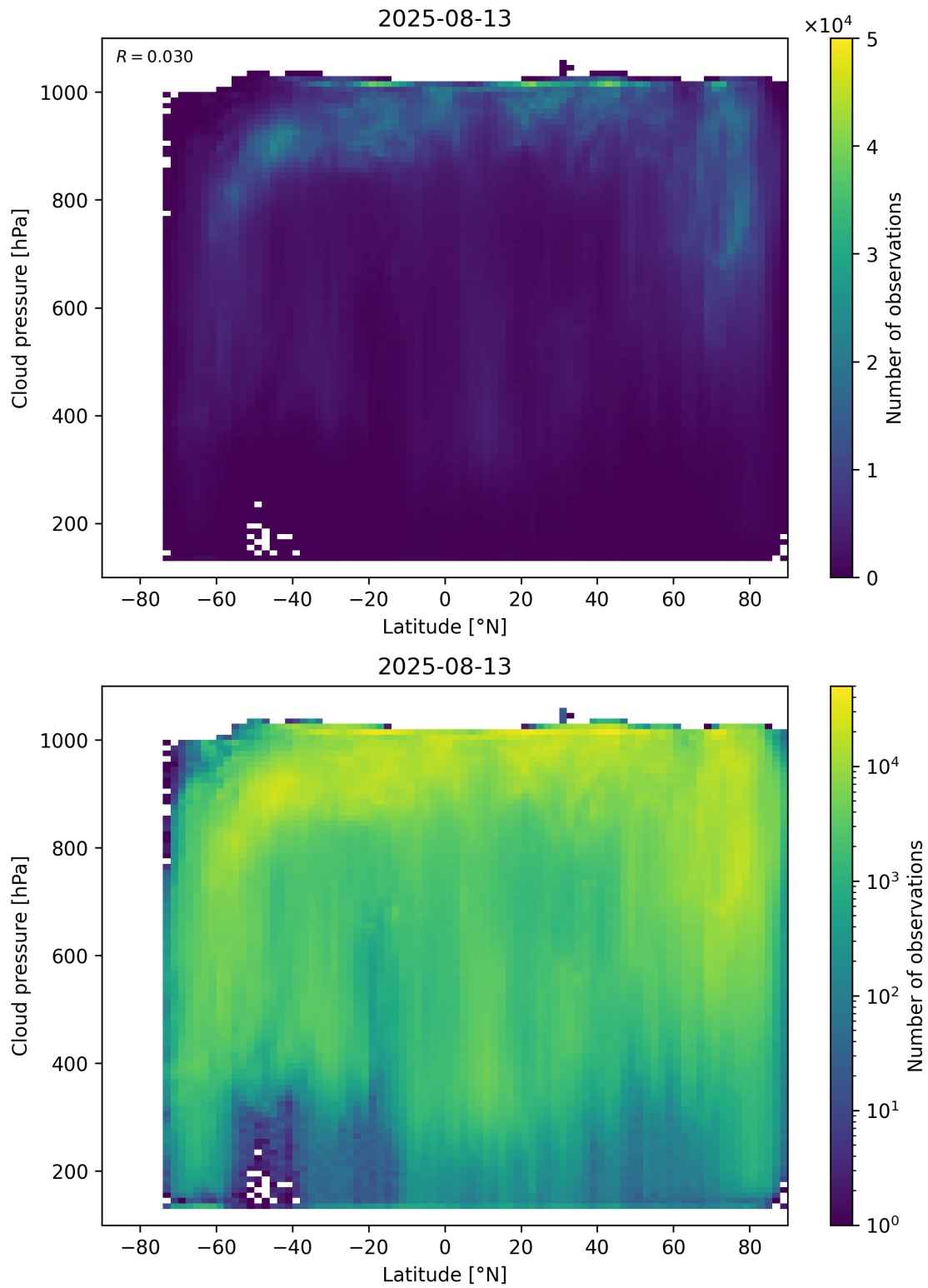
Figure 91: Scatter density plot of “Latitude” against “Cloud pressure” for 2025-08-12 to 2025-08-14.
