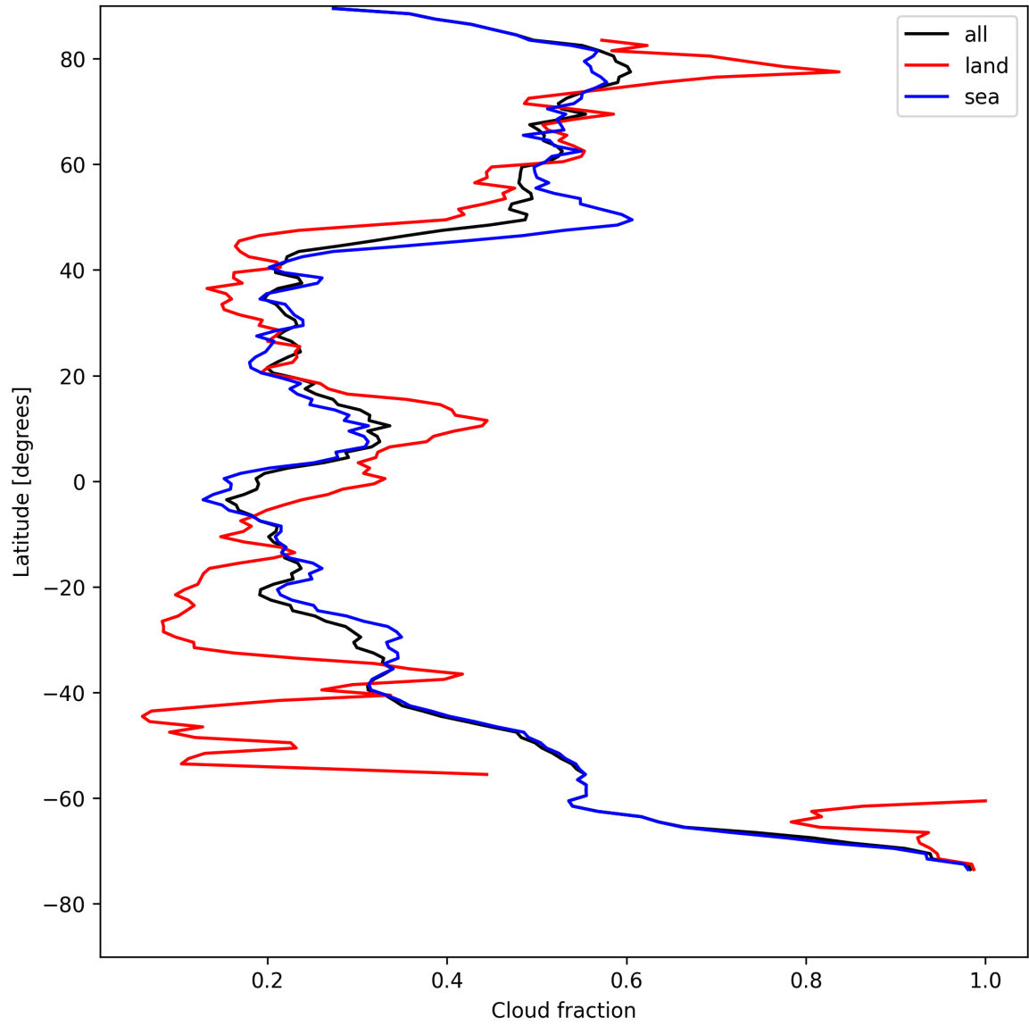
Figure 15: Zonal average of “Cloud fraction” for 2025-08-12 to 2025-08-14.
