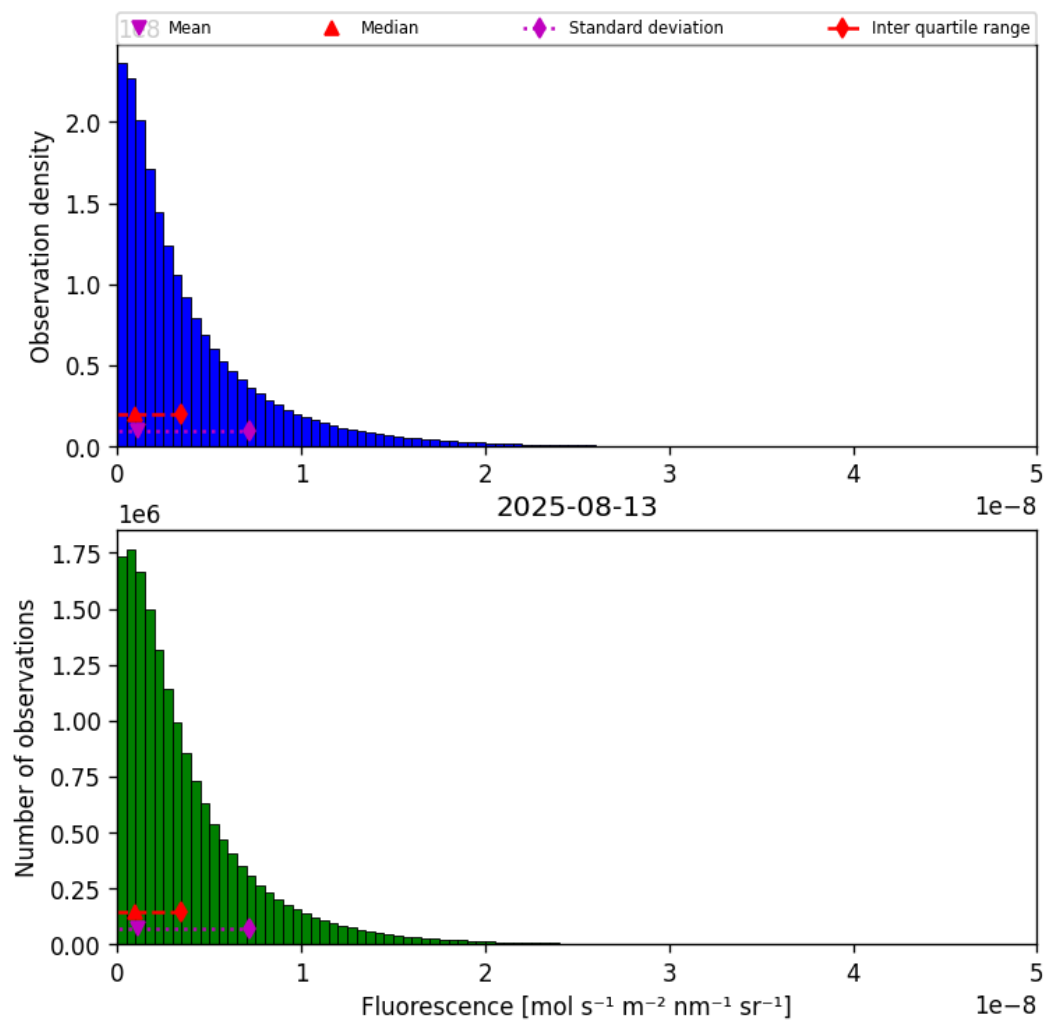
Figure 40: Histogram of “Fluorescence” for 2025-08-12 to 2025-08-14
