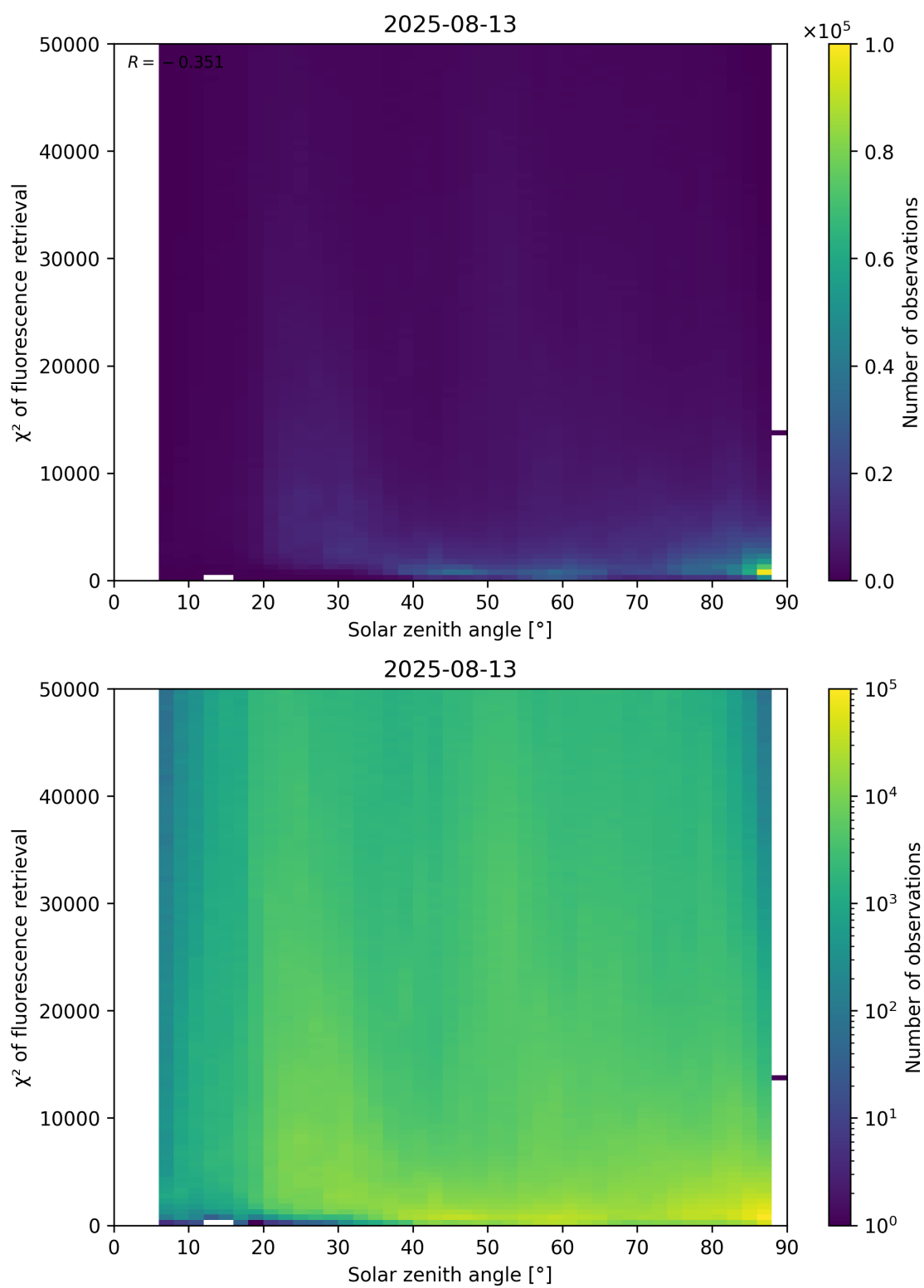
Figure 109: Scatter density plot of “Solar zenith angle” against “ \chi^2 of fluorescence retrieval” for 2025-08-12 to 2025-08-14.
