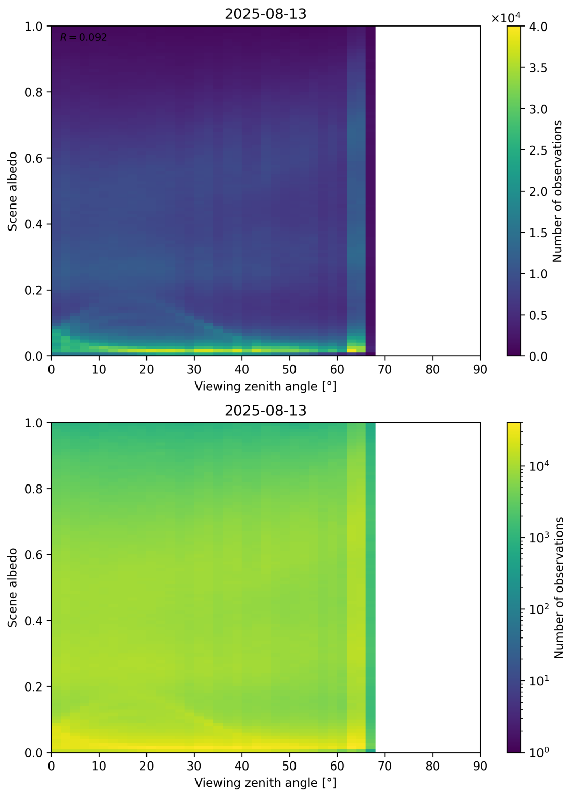
Figure 126: Scatter density plot of “Viewing zenith angle” against “Scene albedo” for 2025-08-12 to 2025-08-14.
