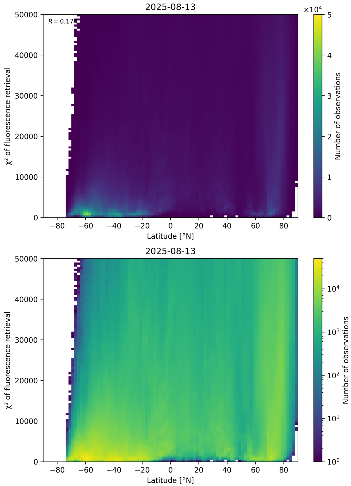
Figure 89: Scatter density plot of “Latitude” against “ \chi^2 of fluorescence retrieval” for 2025-08-12 to 2025-08-14.
