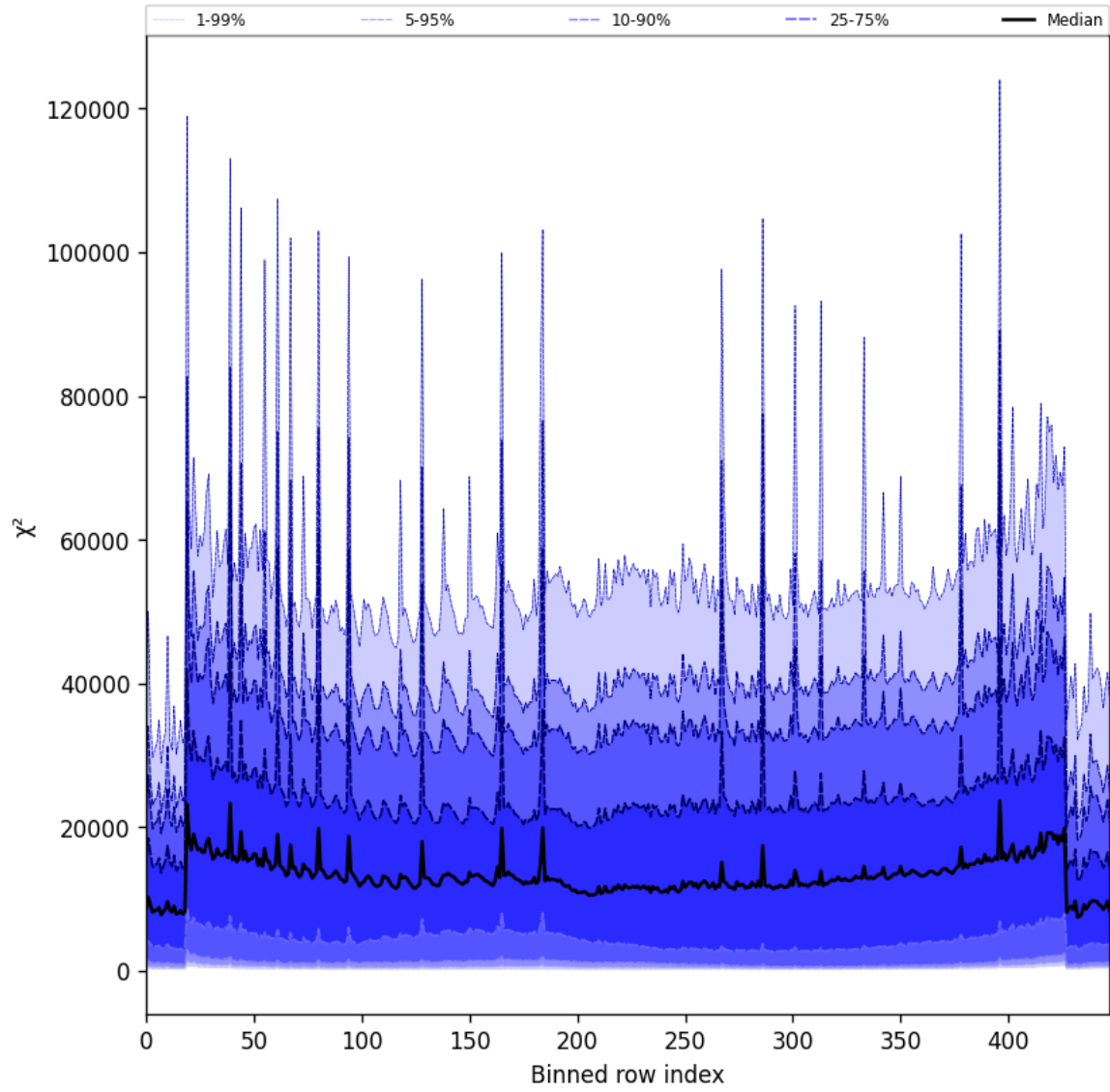
Figure 55: Along track statistics of " \chi^2 " for 2025-08-12 to 2025-08-14
