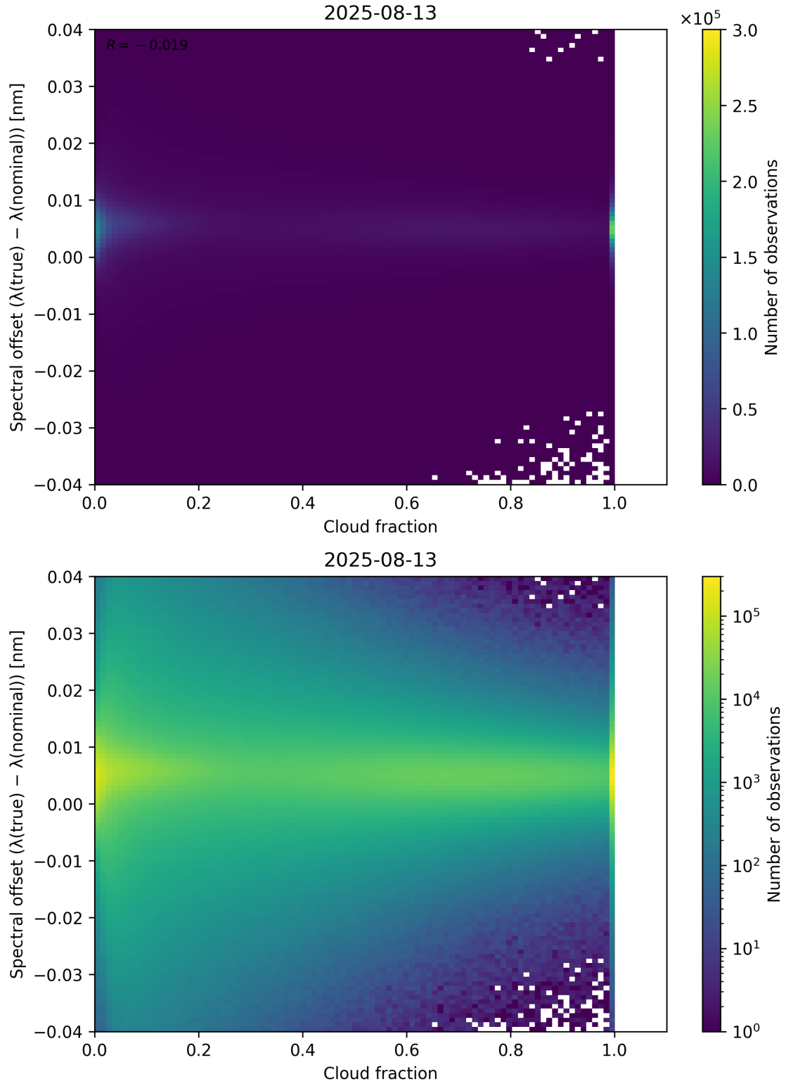
Figure 76: Scatter density plot of “Cloud fraction” against “Spectral offset ( \lambda_{\text{true}} - \lambda_{\text{nominal}} )” for 2025-08-12 to 2025-08-14.
