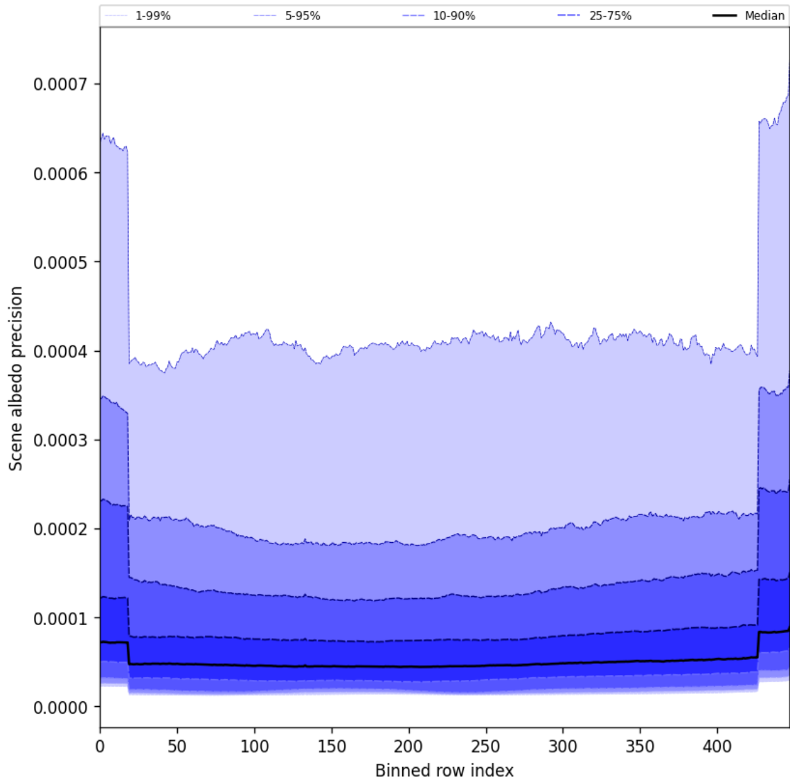
Figure 52: Along track statistics of “Scene albedo precision” for 2025-08-12 to 2025-08-14
