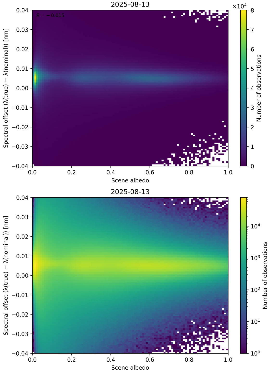
Figure 107: Scatter density plot of “Scene albedo” against “Spectral offset ( \lambda_{\text{true}} - \lambda_{\text{nominal}} )” for 2025-08-12 to 2025-08-14.
