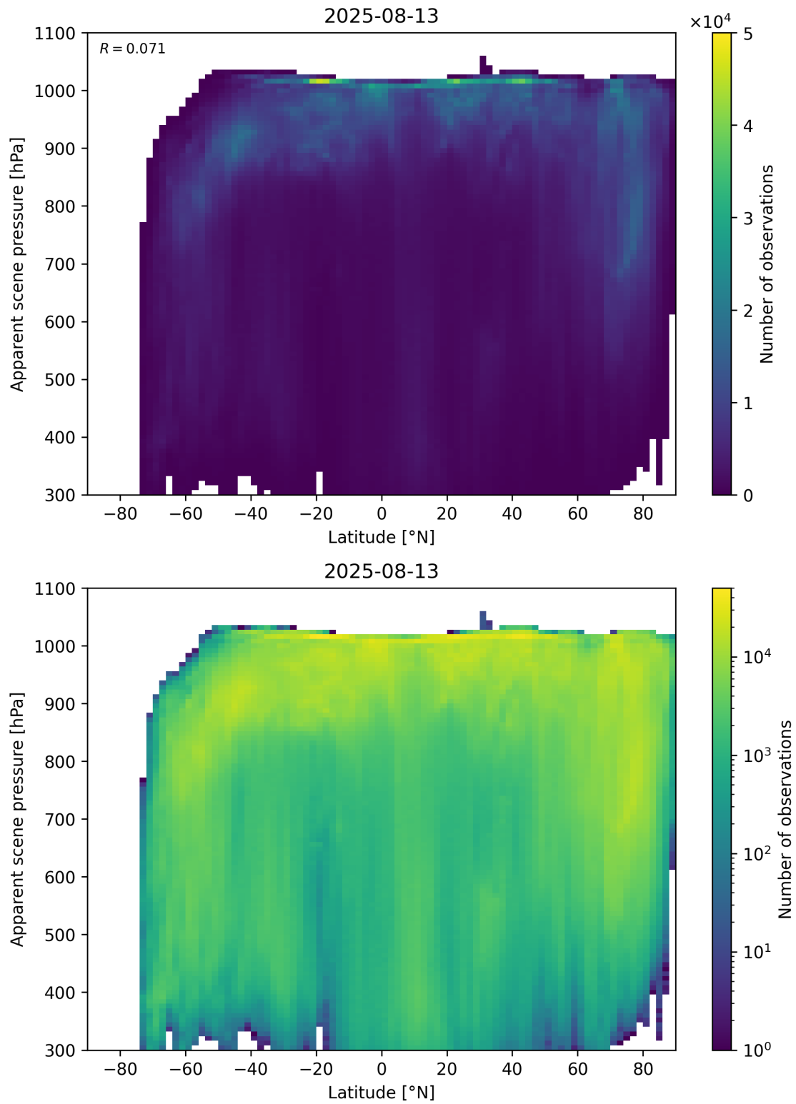
Figure 88: Scatter density plot of “Latitude” against “Apparent scene pressure” for 2025-08-12 to 2025-08-14.
