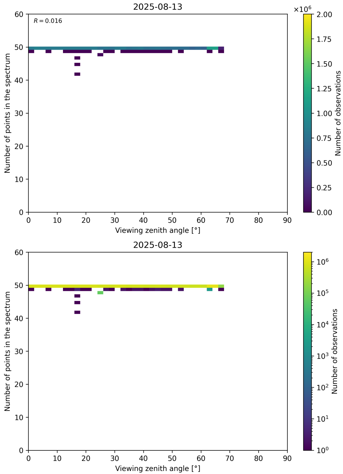
Figure 125: Scatter density plot of “Viewing zenith angle” against “Number of points in the spectrum” for 2025-08-12 to 2025-08-14.
