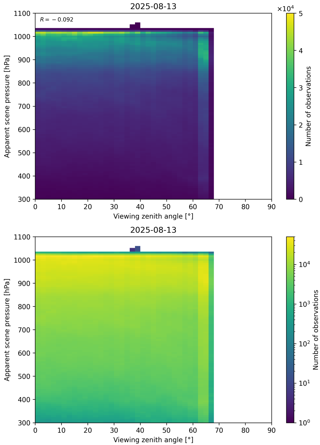
Figure 118: Scatter density plot of “Viewing zenith angle” against “Apparent scene pressure” for 2025-08-12 to 2025-08-14.
