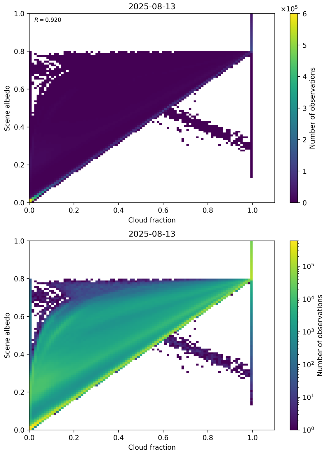
Figure 75: Scatter density plot of “Cloud fraction” against “Scene albedo” for 2025-08-12 to 2025-08-14.
