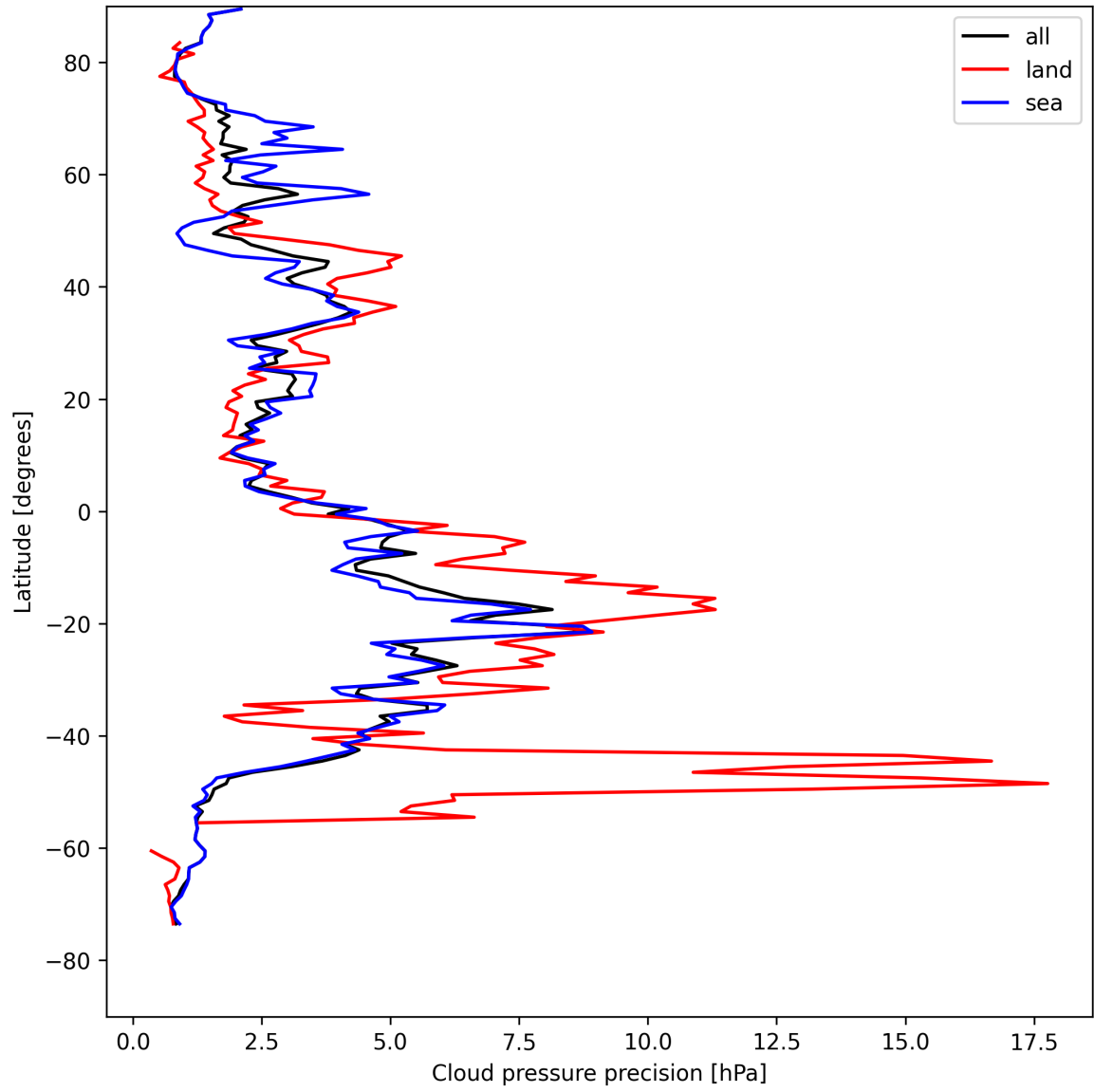
Figure 14: Zonal average of “Cloud pressure precision” for 2025-08-12 to 2025-08-14.
