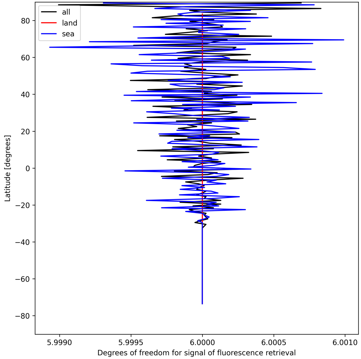
Figure 26: Zonal average of “Degrees of freedom for signal of fluorescence retrieval” for 2025-08-12 to 2025-08-14.
