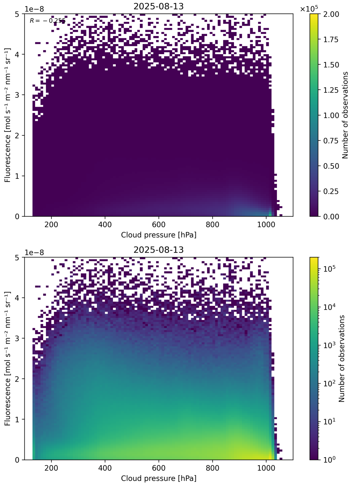
Figure 80: Scatter density plot of “Cloud pressure” against “Fluorescence” for 2025-08-12 to 2025-08-14.
