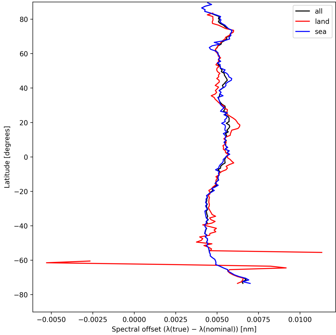
Figure 28: Zonal average of “Spectral offset ( \lambda_{\text{true}} - \lambda_{\text{nominal}} )” for 2025-08-12 to 2025-08-14.
