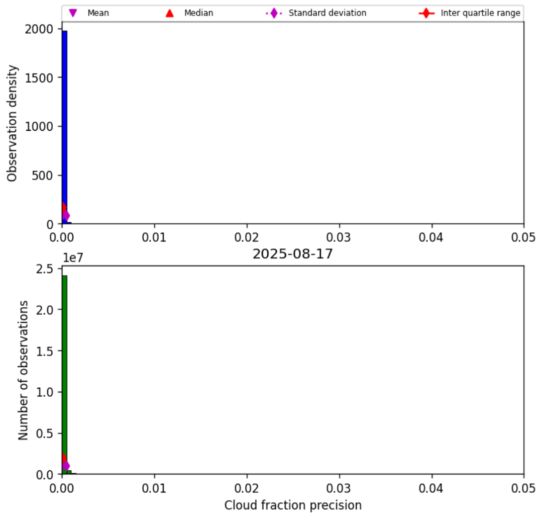
Figure 33: Histogram of “Cloud fraction precision” for 2025-08-16 to 2025-08-18
