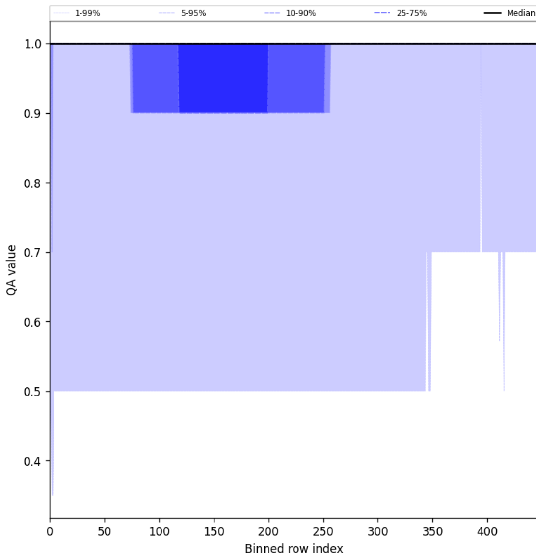
Figure 46: Along track statistics of “QA value” for 2025-08-16 to 2025-08-18
