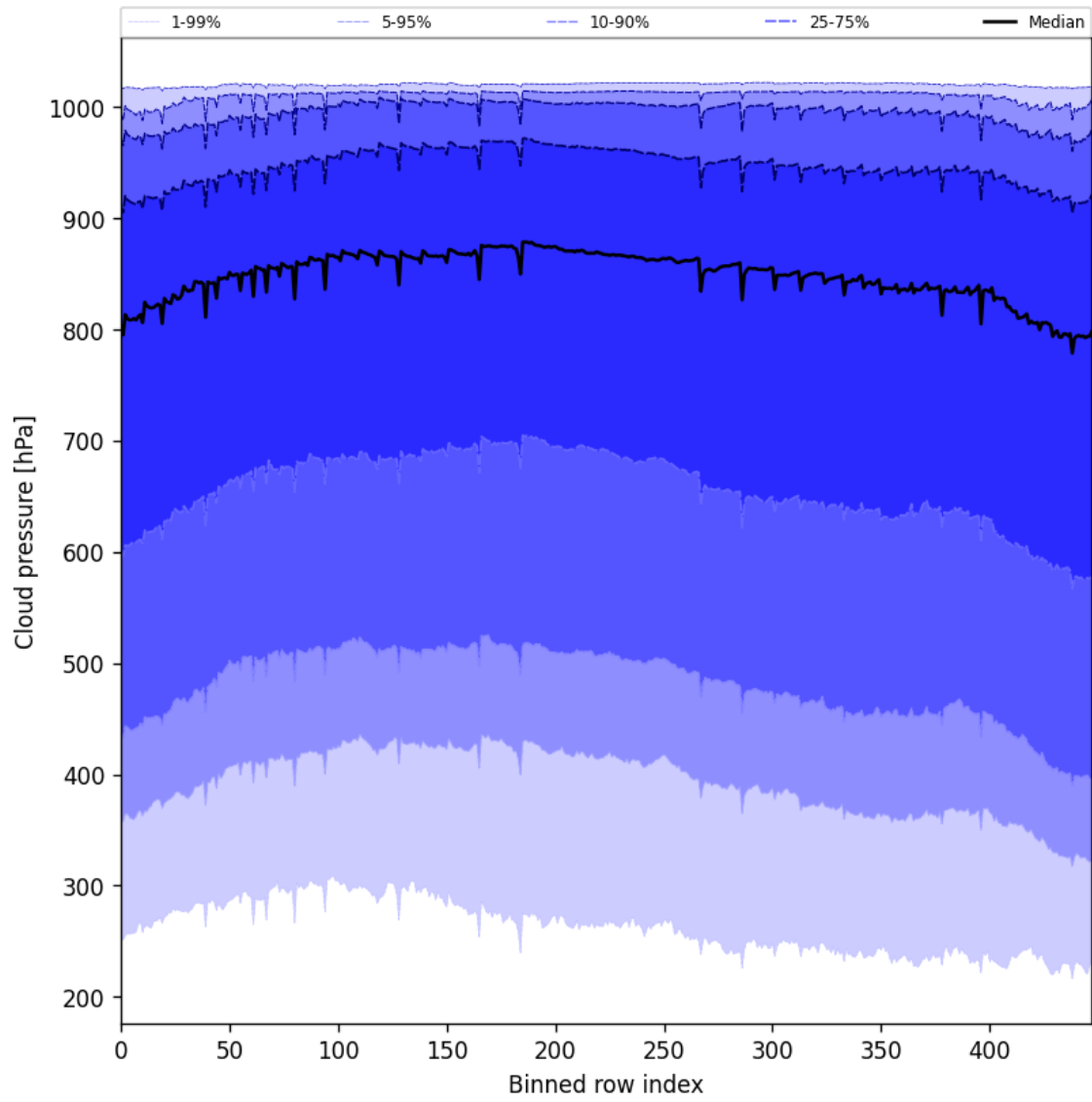
Figure 47: Along track statistics of “Cloud pressure” for 2025-08-16 to 2025-08-18
