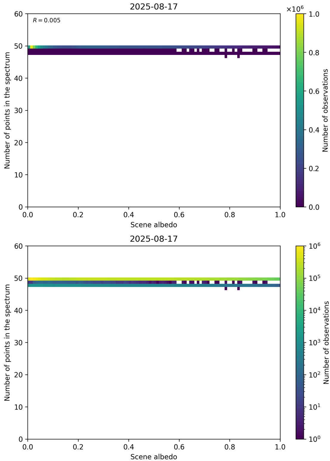
Figure 106: Scatter density plot of “Scene albedo” against “Number of points in the spectrum” for 2025-08-16 to 2025-08-18.
