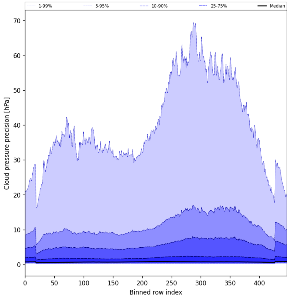
Figure 48: Along track statistics of “Cloud pressure precision” for 2025-08-16 to 2025-08-18
