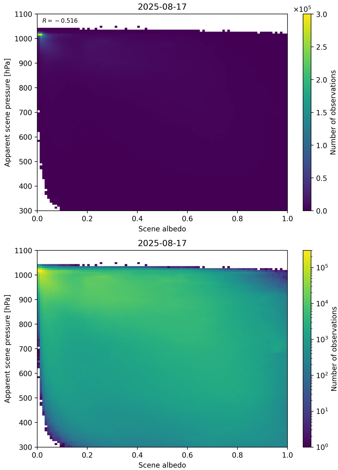
Figure 102: Scatter density plot of “Scene albedo” against “Apparent scene pressure” for 2025-08-16 to 2025-08-18.
