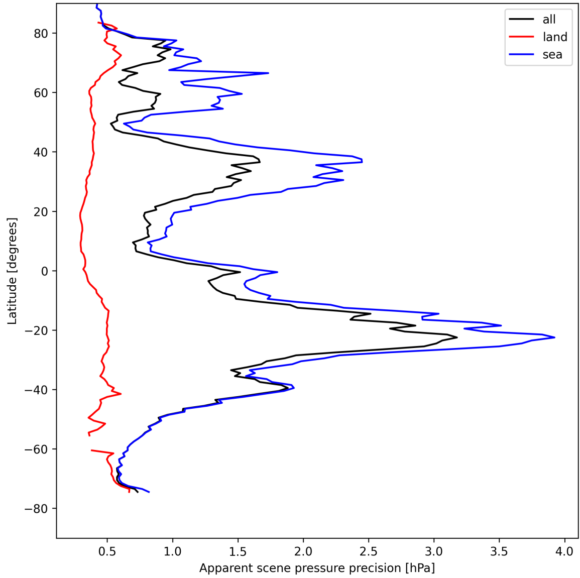
Figure 20: Zonal average of “Apparent scene pressure precision” for 2025-08-16 to 2025-08-18.
