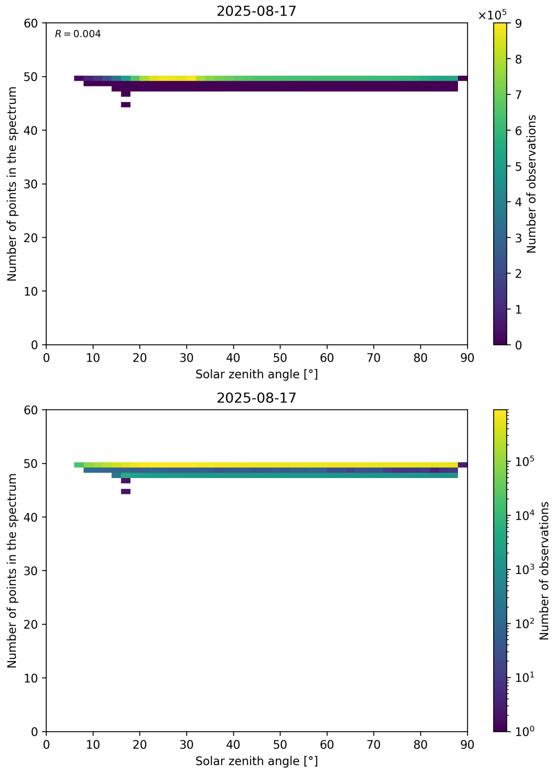
Figure 115: Scatter density plot of “Solar zenith angle” against “Number of points in the spectrum” for 2025-08-16 to 2025-08-18.
