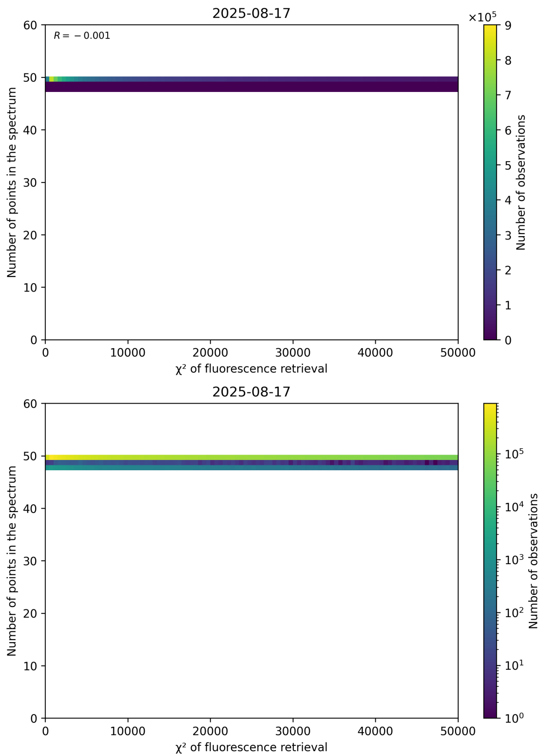
Figure 68: Scatter density plot of " \chi^2 of fluorescence retrieval" against "Number of points in the spectrum" for 2025-08-16 to 2025-08-18.
