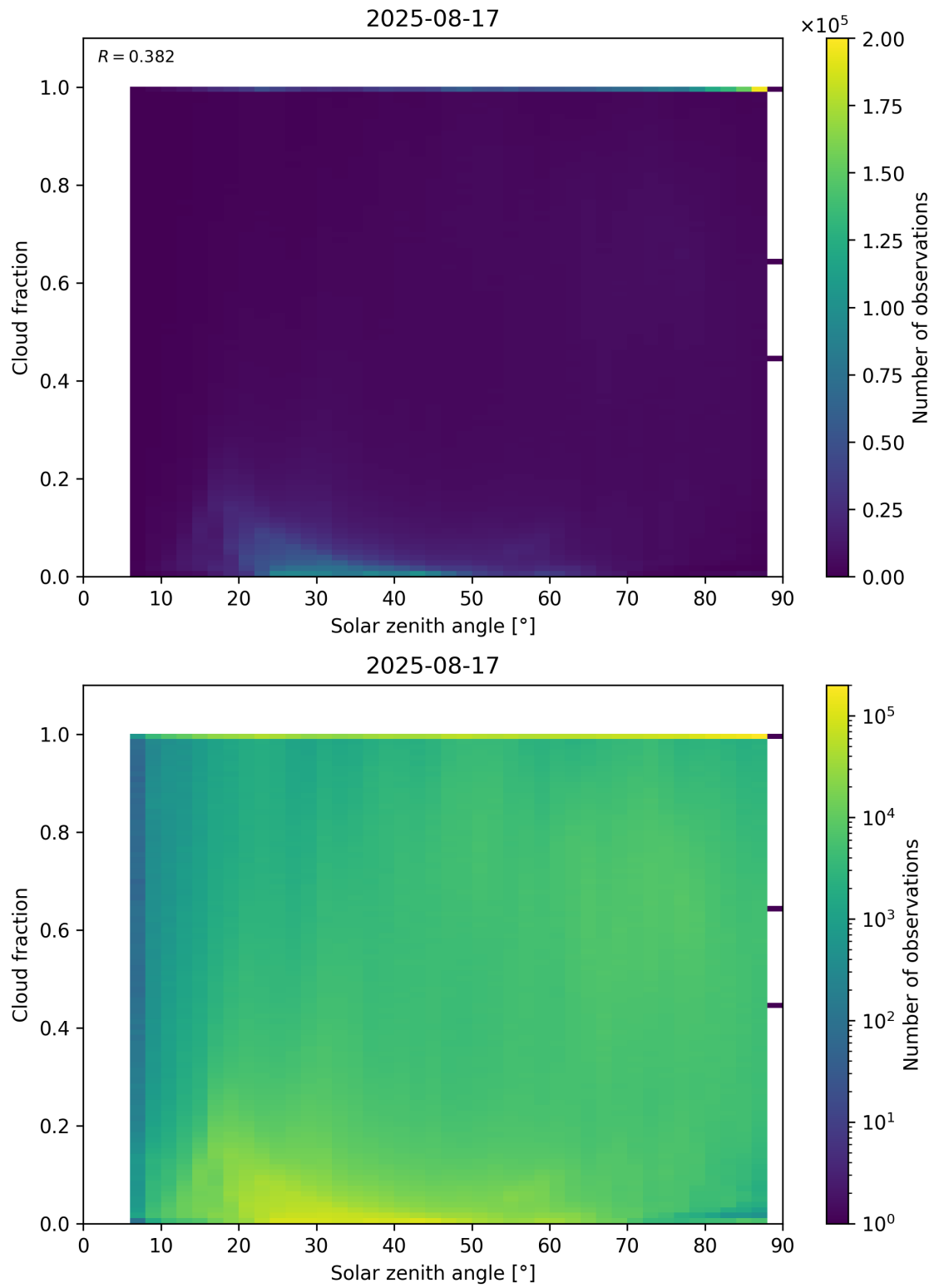
Figure 110: Scatter density plot of “Solar zenith angle” against “Cloud fraction” for 2025-08-16 to 2025-08-18.
