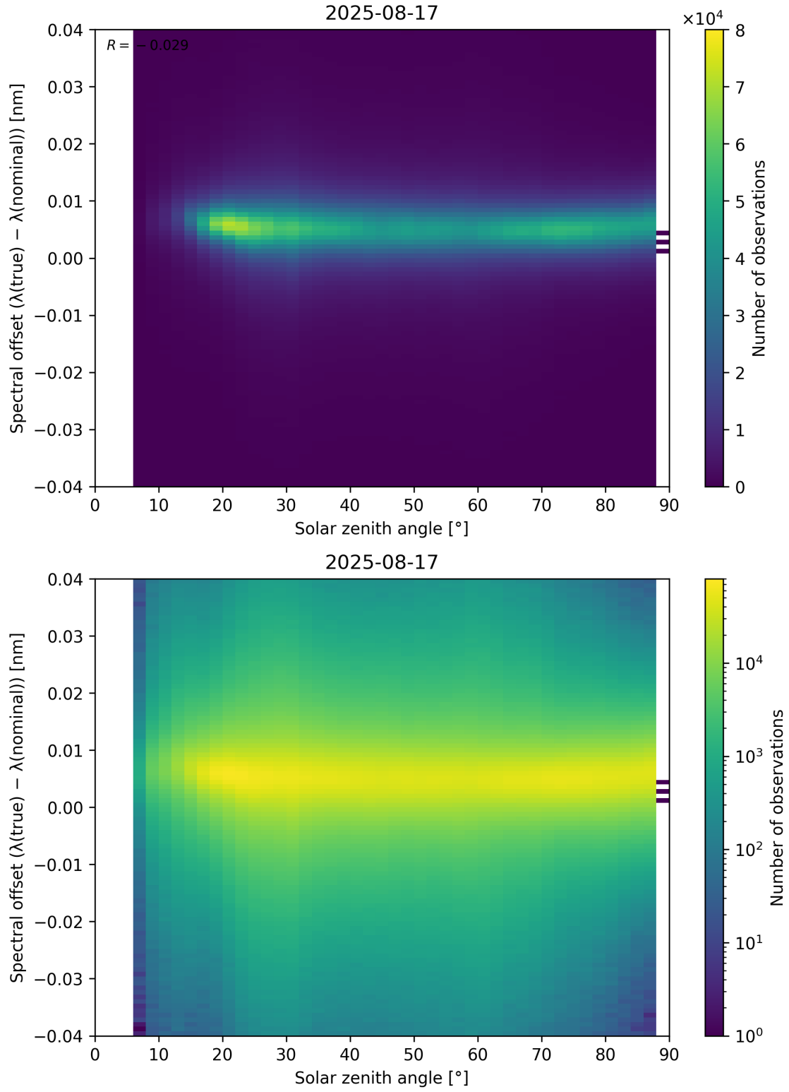
Figure 117: Scatter density plot of “Solar zenith angle” against “Spectral offset ( \lambda_{\text{true}} - \lambda_{\text{nominal}} )” for 2025-08-16 to 2025-08-18.
