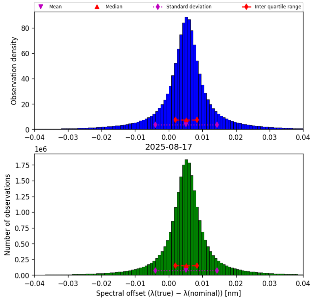
Figure 45: Histogram of “Spectral offset ( \lambda_{\text{true}} - \lambda_{\text{nominal}} )” for 2025-08-16 to 2025-08-18
