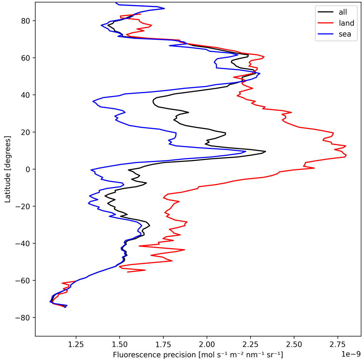
Figure 24: Zonal average of “Fluorescence precision” for 2025-08-16 to 2025-08-18.
