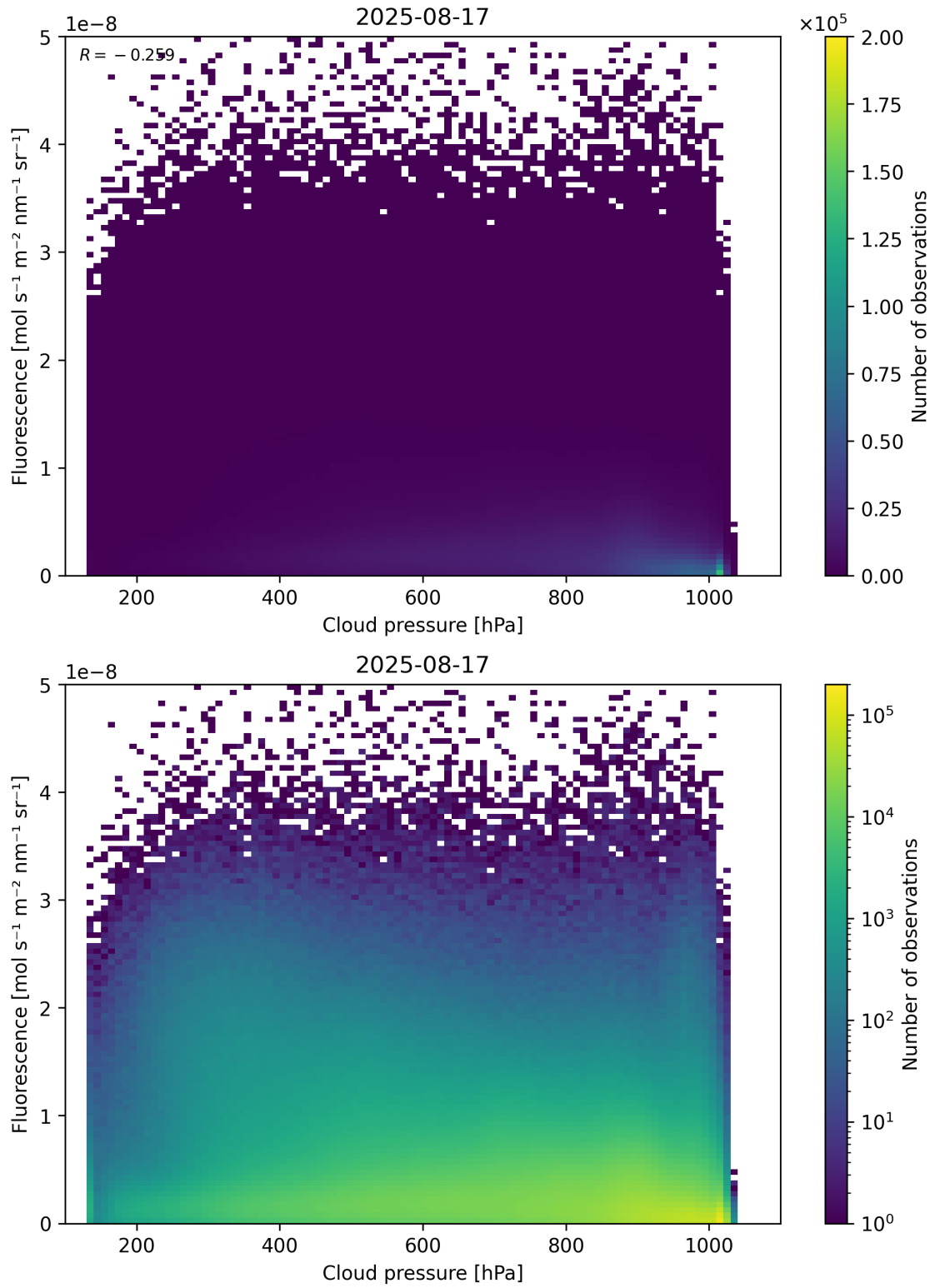
Figure 80: Scatter density plot of “Cloud pressure” against “Fluorescence” for 2025-08-16 to 2025-08-18.
