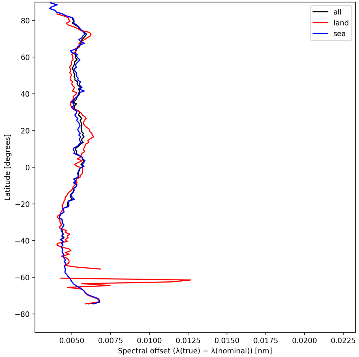
Figure 28: Zonal average of “Spectral offset ( \lambda_{\text{true}} - \lambda_{\text{nominal}} )” for 2025-08-16 to 2025-08-18.
