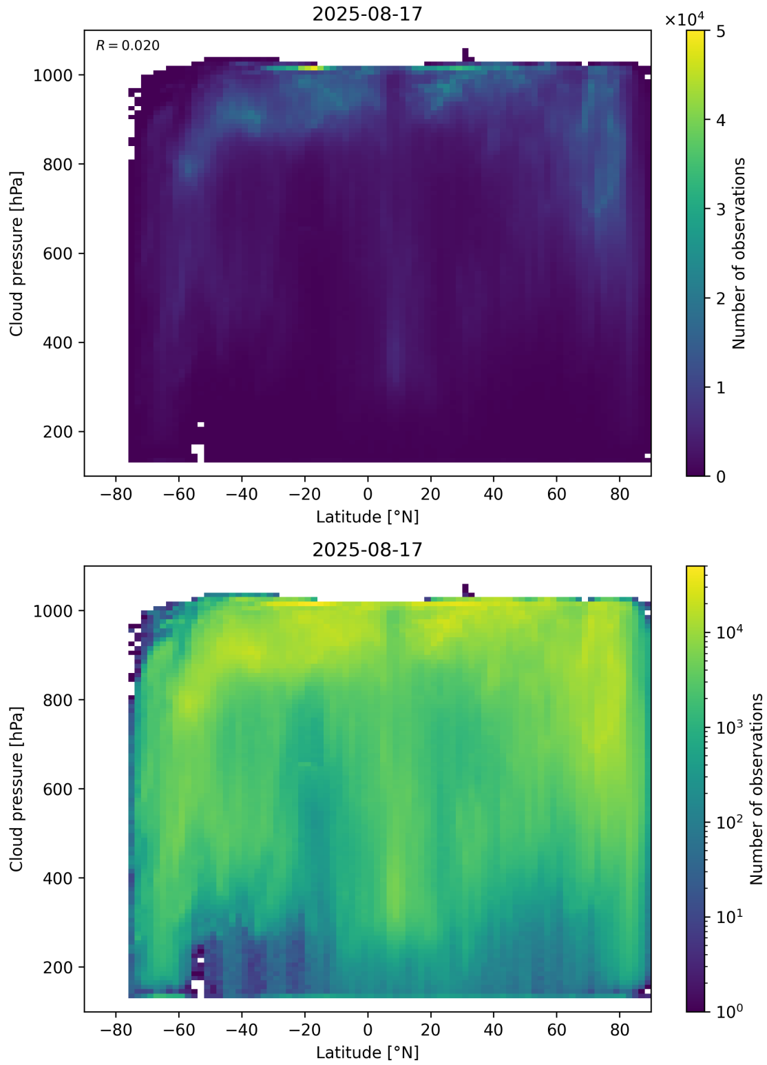
Figure 91: Scatter density plot of “Latitude” against “Cloud pressure” for 2025-08-16 to 2025-08-18.
