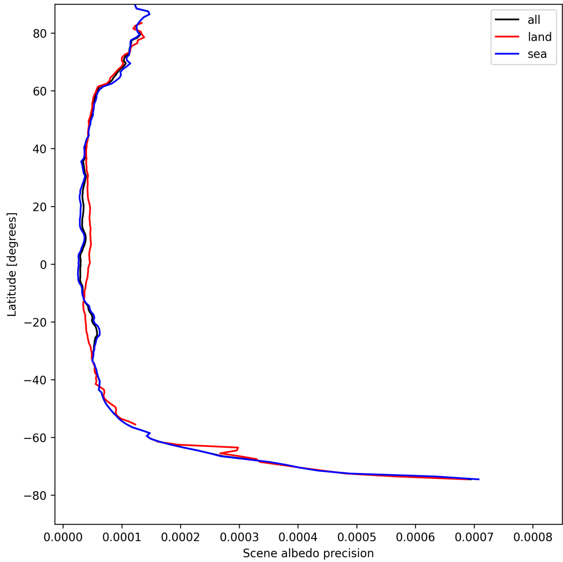
Figure 18: Zonal average of “Scene albedo precision” for 2025-08-16 to 2025-08-18.
