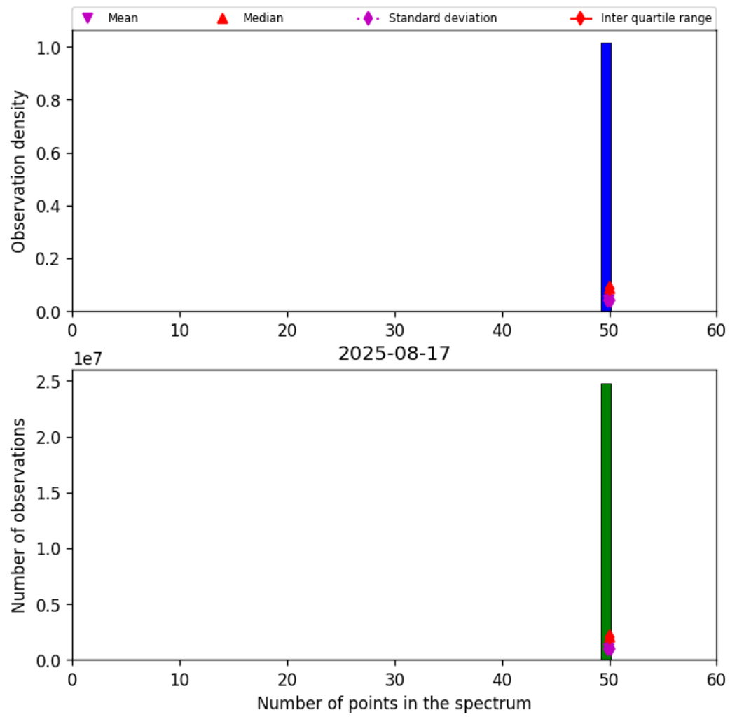
Figure 44: Histogram of “Number of points in the spectrum” for 2025-08-16 to 2025-08-18
