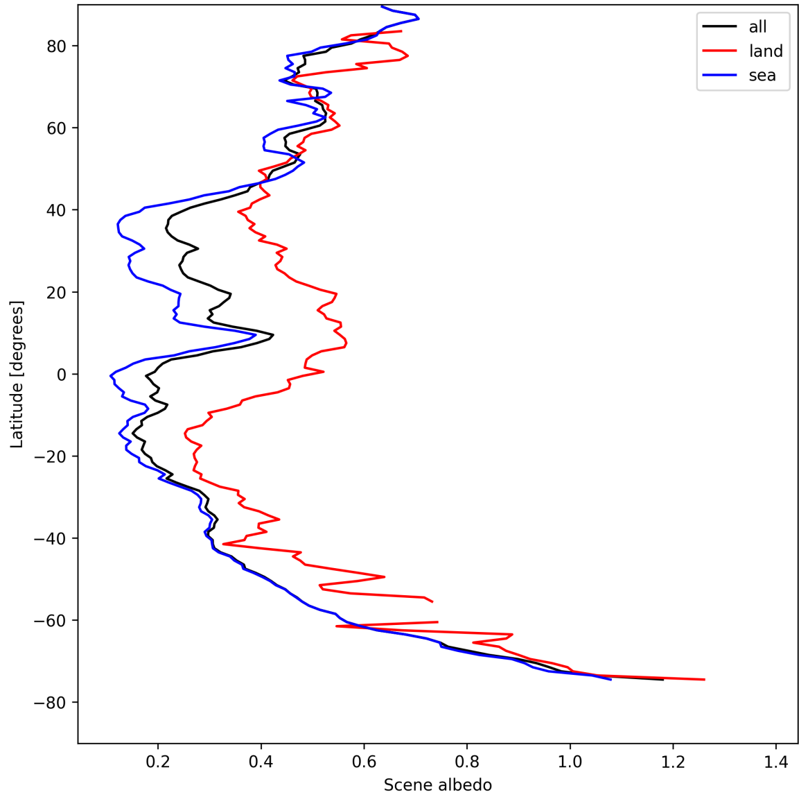
Figure 17: Zonal average of “Scene albedo” for 2025-08-16 to 2025-08-18.
