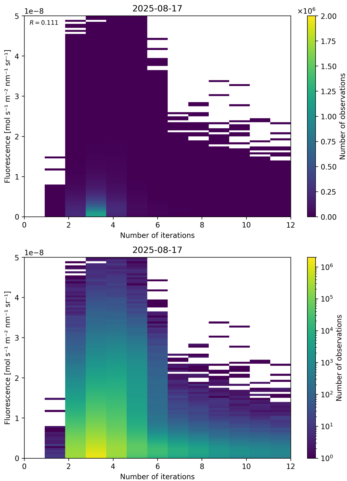
Figure 98: Scatter density plot of “Number of iterations” against “Fluorescence” for 2025-08-16 to 2025-08-18.
