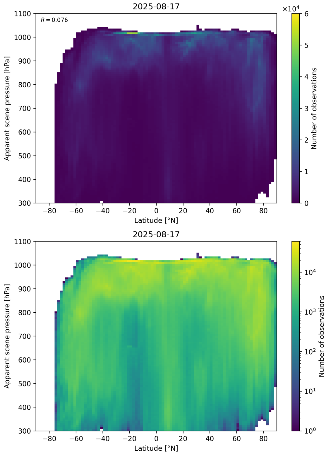
Figure 88: Scatter density plot of “Latitude” against “Apparent scene pressure” for 2025-08-16 to 2025-08-18.
