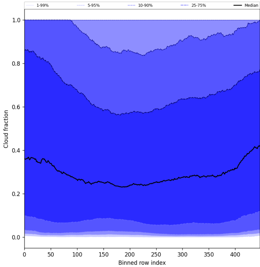
Figure 49: Along track statistics of “Cloud fraction” for 2025-08-16 to 2025-08-18
