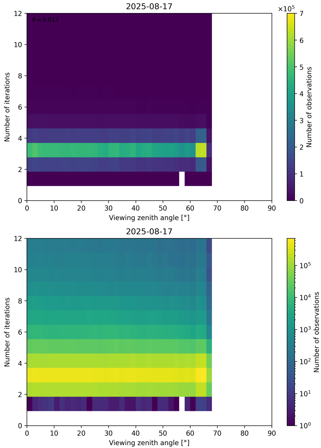
Figure 124: Scatter density plot of “Viewing zenith angle” against “Number of iterations” for 2025-08-16 to 2025-08-18.
