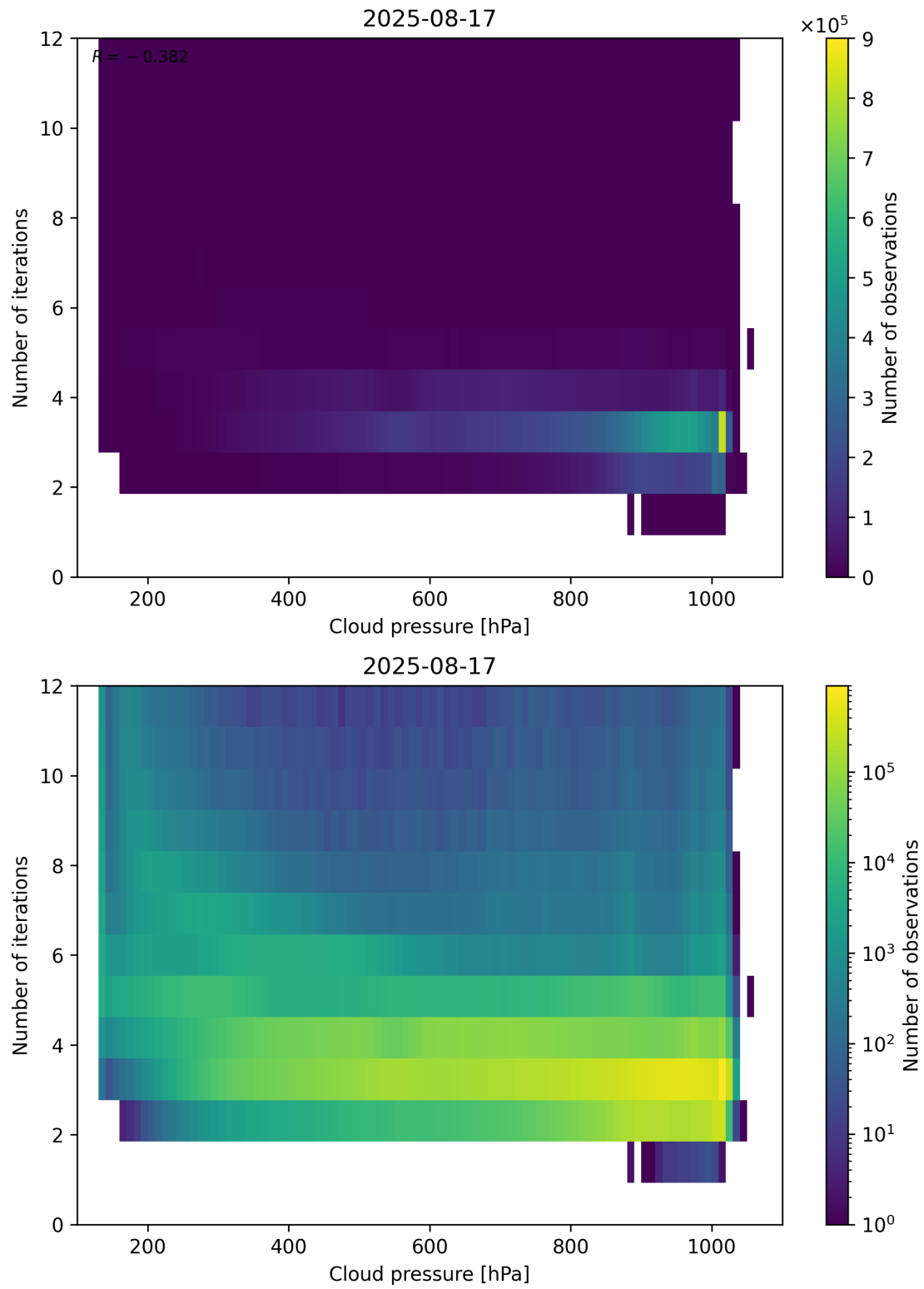
Figure 81: Scatter density plot of “Cloud pressure” against “Number of iterations” for 2025-08-16 to 2025-08-18.
