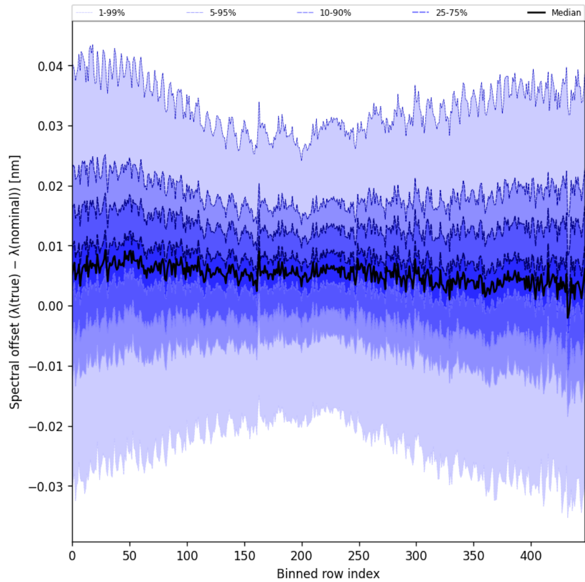
Figure 62: Along track statistics of “Spectral offset ( \lambda_{\text{true}} - \lambda_{\text{nominal}} )” for 2025-08-16 to 2025-08-18
