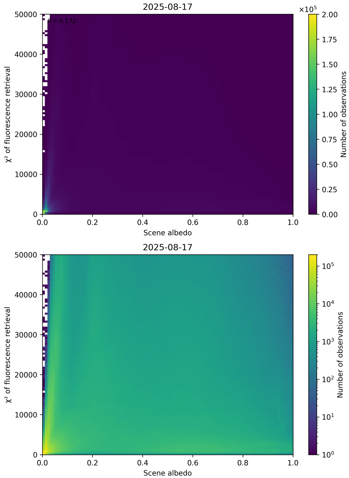
Figure 103: Scatter density plot of “Scene albedo” against “ \chi^2 of fluorescence retrieval” for 2025-08-16 to 2025-08-18.
