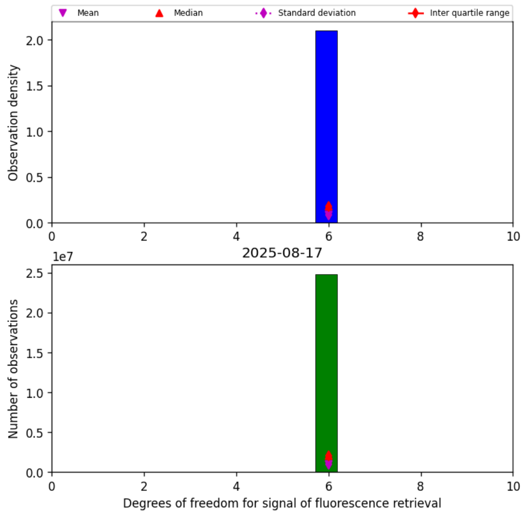
Figure 43: Histogram of "Degrees of freedom for signal of fluorescence retrieval" for 2025-08-16 to 2025-08-18
