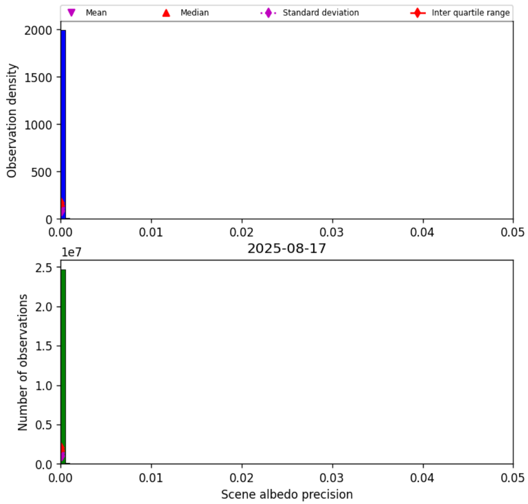
Figure 35: Histogram of “Scene albedo precision” for 2025-08-16 to 2025-08-18
