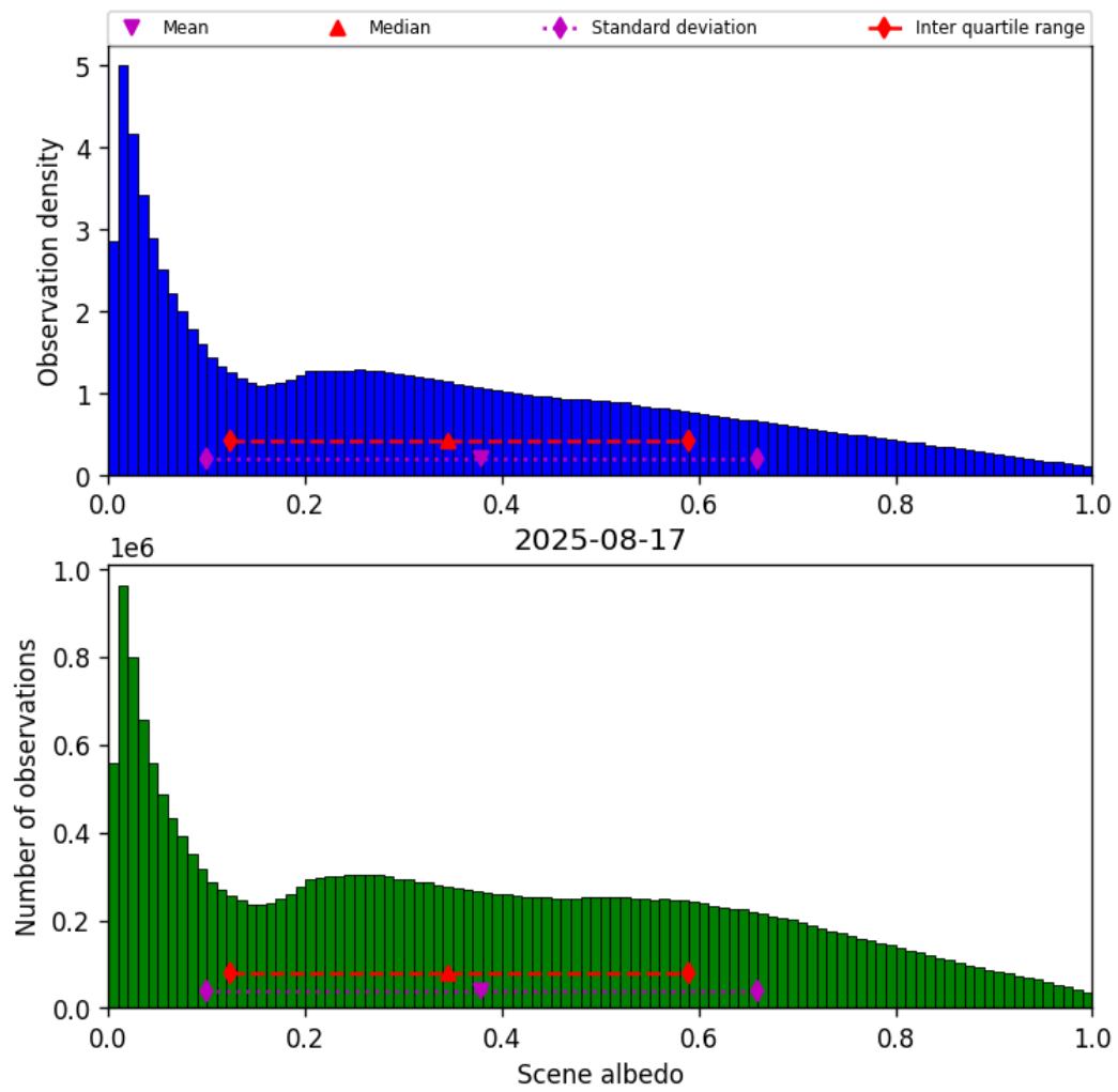
Figure 34: Histogram of “Scene albedo” for 2025-08-16 to 2025-08-18
