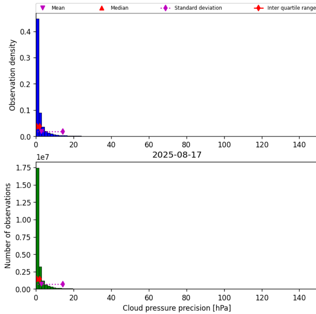
Figure 31: Histogram of “Cloud pressure precision” for 2025-08-16 to 2025-08-18
