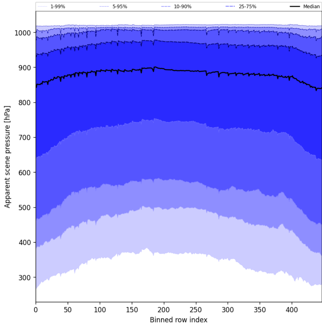
Figure 53: Along track statistics of “Apparent scene pressure” for 2025-08-16 to 2025-08-18
