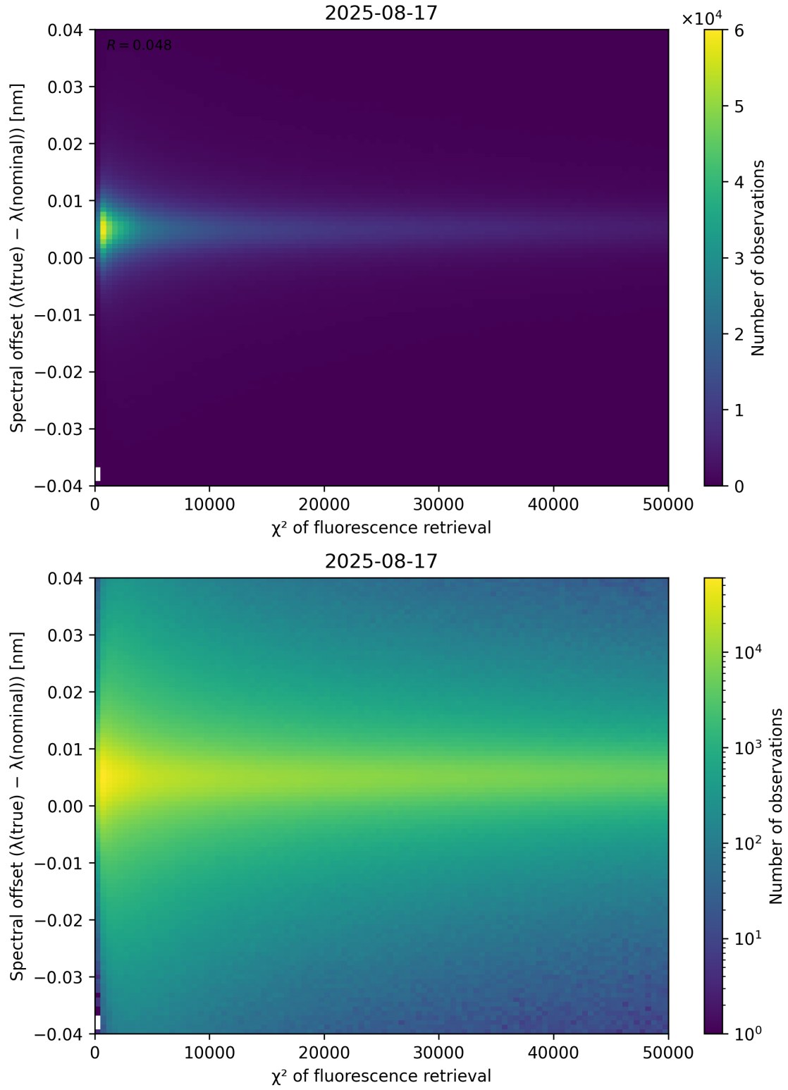
Figure 69: Scatter density plot of “ \chi^2 of fluorescence retrieval” against “Spectral offset ( \lambda_{\text{true}} - \lambda_{\text{nominal}} )” for 2025-08-16 to 2025-08-18.
