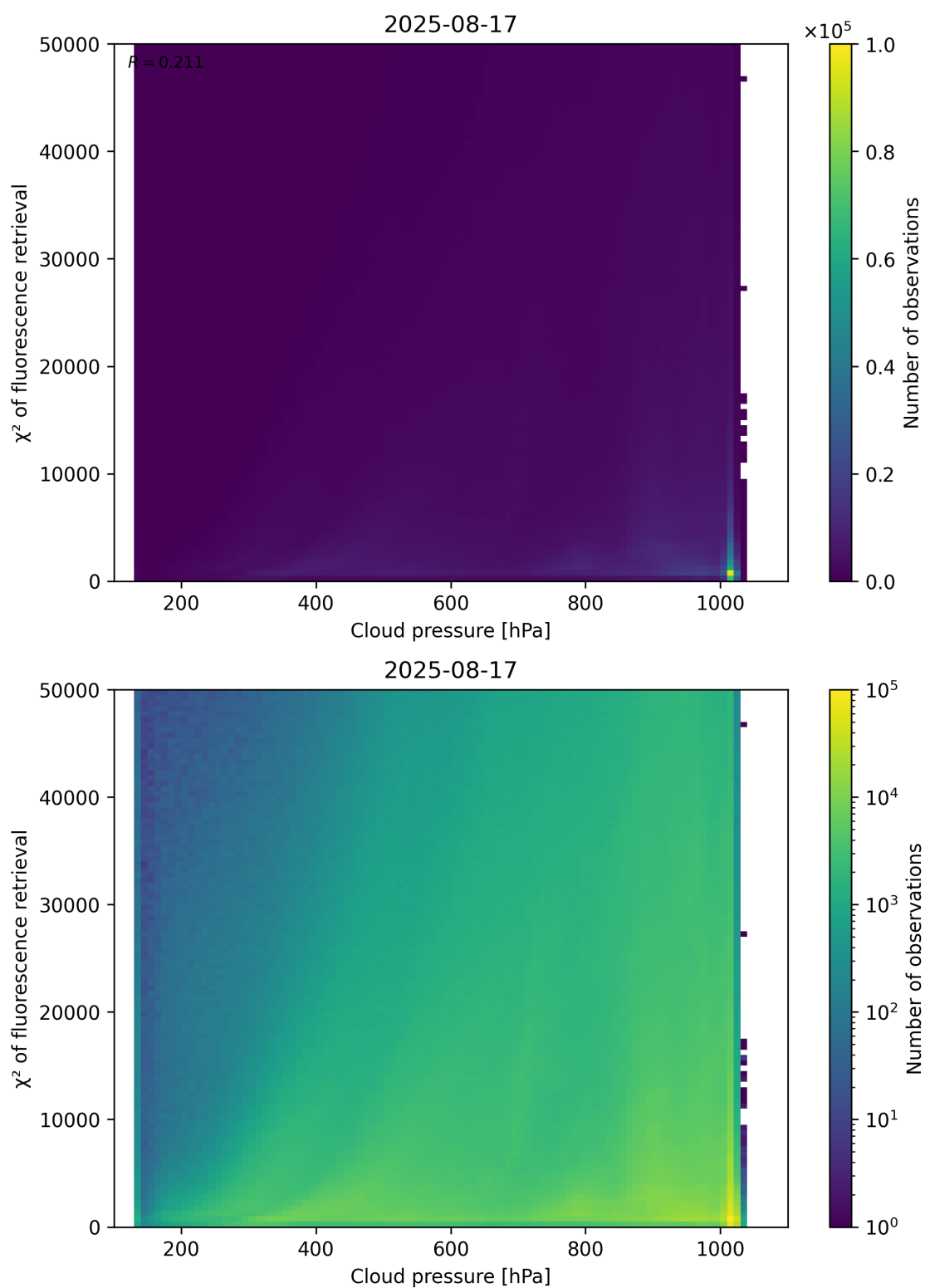
Figure 78: Scatter density plot of “Cloud pressure” against “ \chi^2 of fluorescence retrieval” for 2025-08-16 to 2025-08-18.
