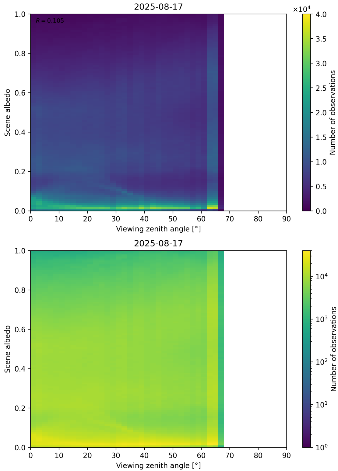
Figure 126: Scatter density plot of “Viewing zenith angle” against “Scene albedo” for 2025-08-16 to 2025-08-18.
