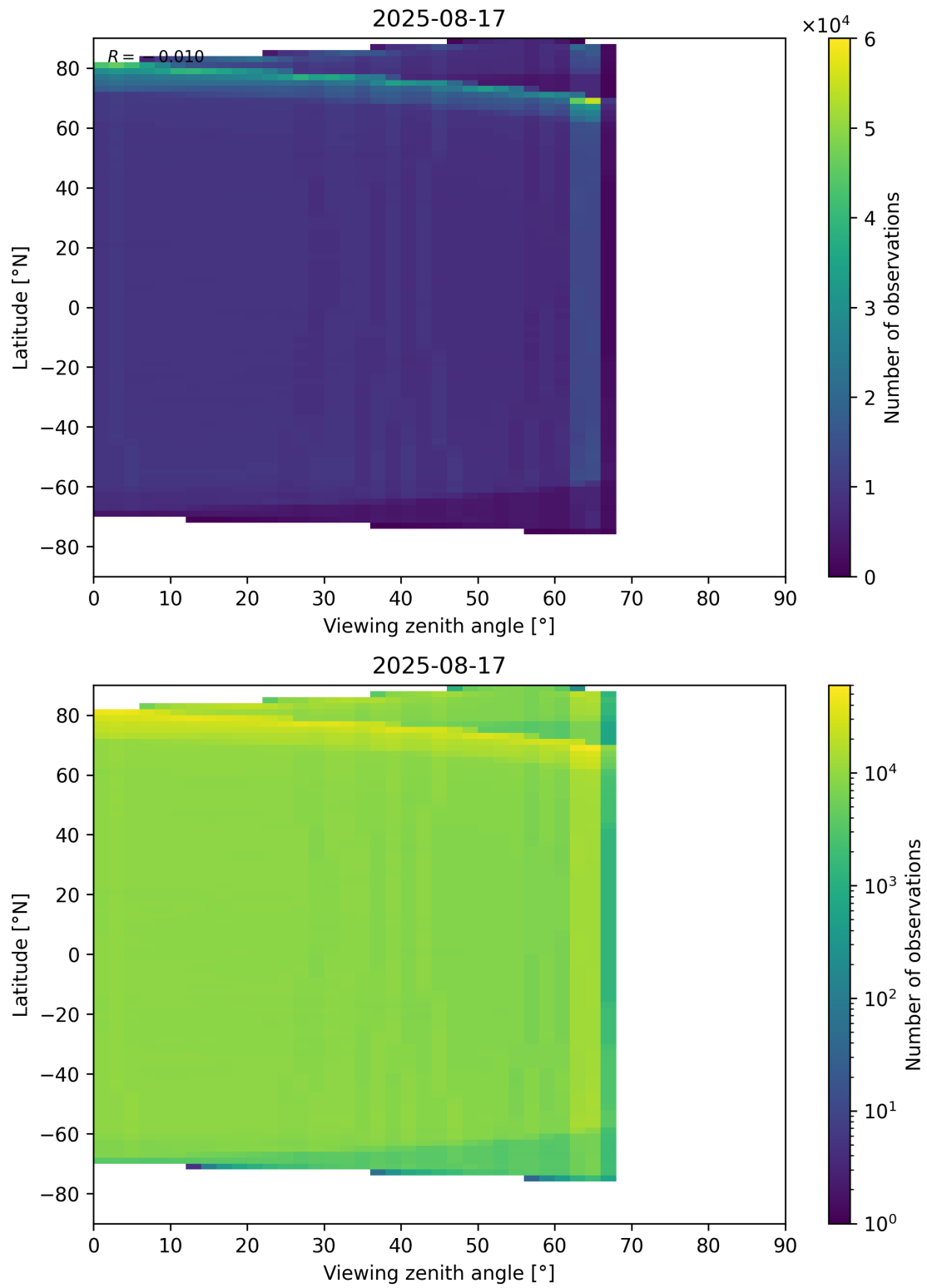
Figure 123: Scatter density plot of “Viewing zenith angle” against “Latitude” for 2025-08-16 to 2025-08-18.
