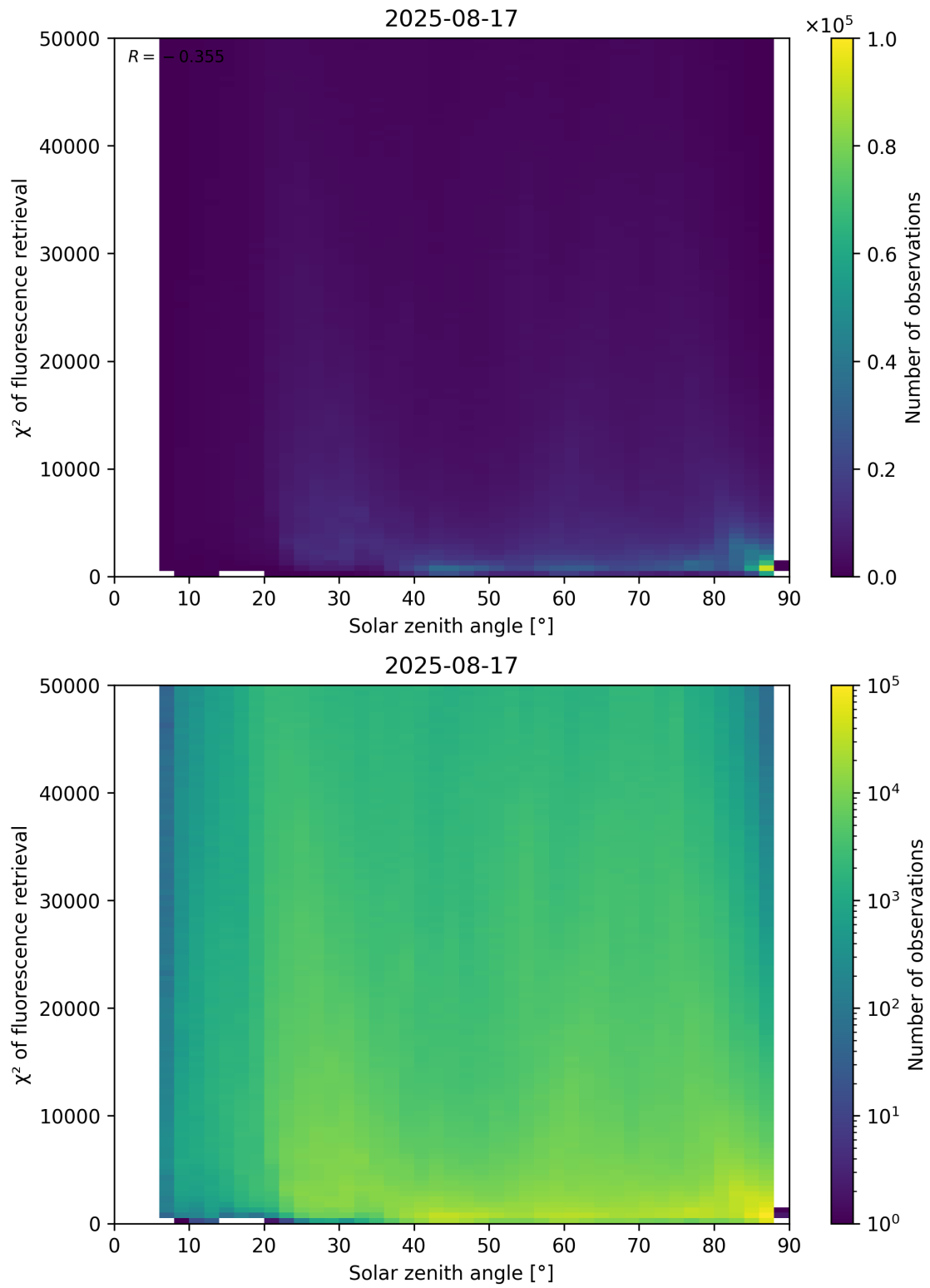
Figure 109: Scatter density plot of “Solar zenith angle” against “ \chi^2 of fluorescence retrieval” for 2025-08-16 to 2025-08-18.
