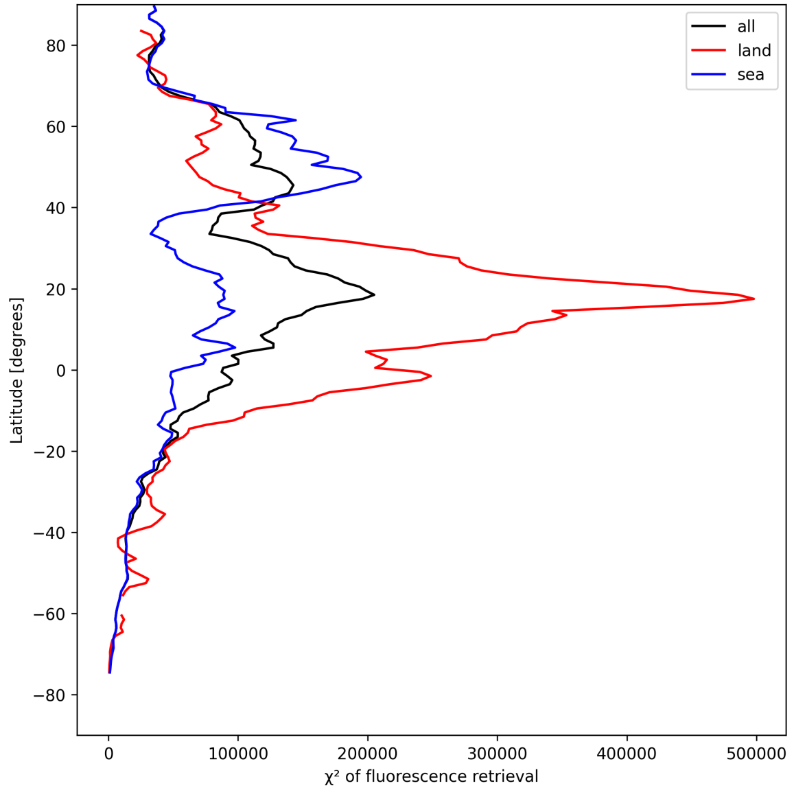
Figure 25: Zonal average of “ \chi^2 of fluorescence retrieval” for 2025-08-16 to 2025-08-18.
