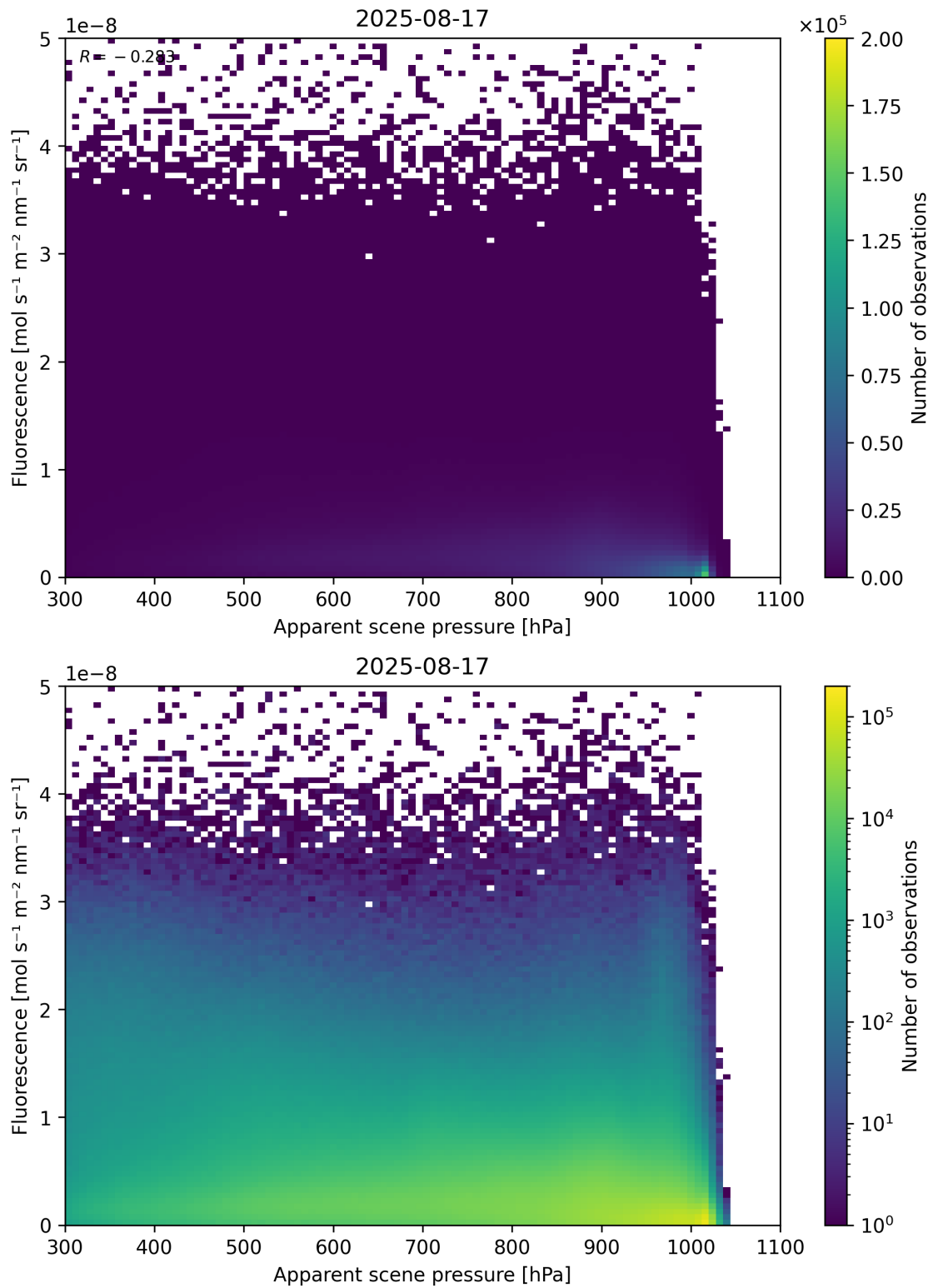
Figure 64: Scatter density plot of “Apparent scene pressure” against “Fluorescence” for 2025-08-16 to 2025-08-18.
