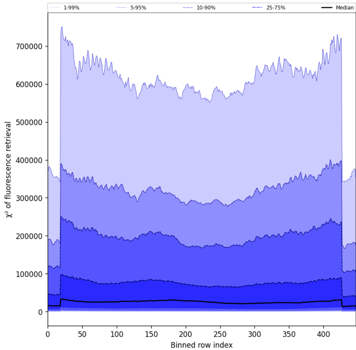
Figure 59: Along track statistics of “ \chi^2 of fluorescence retrieval” for 2025-08-16 to 2025-08-18
