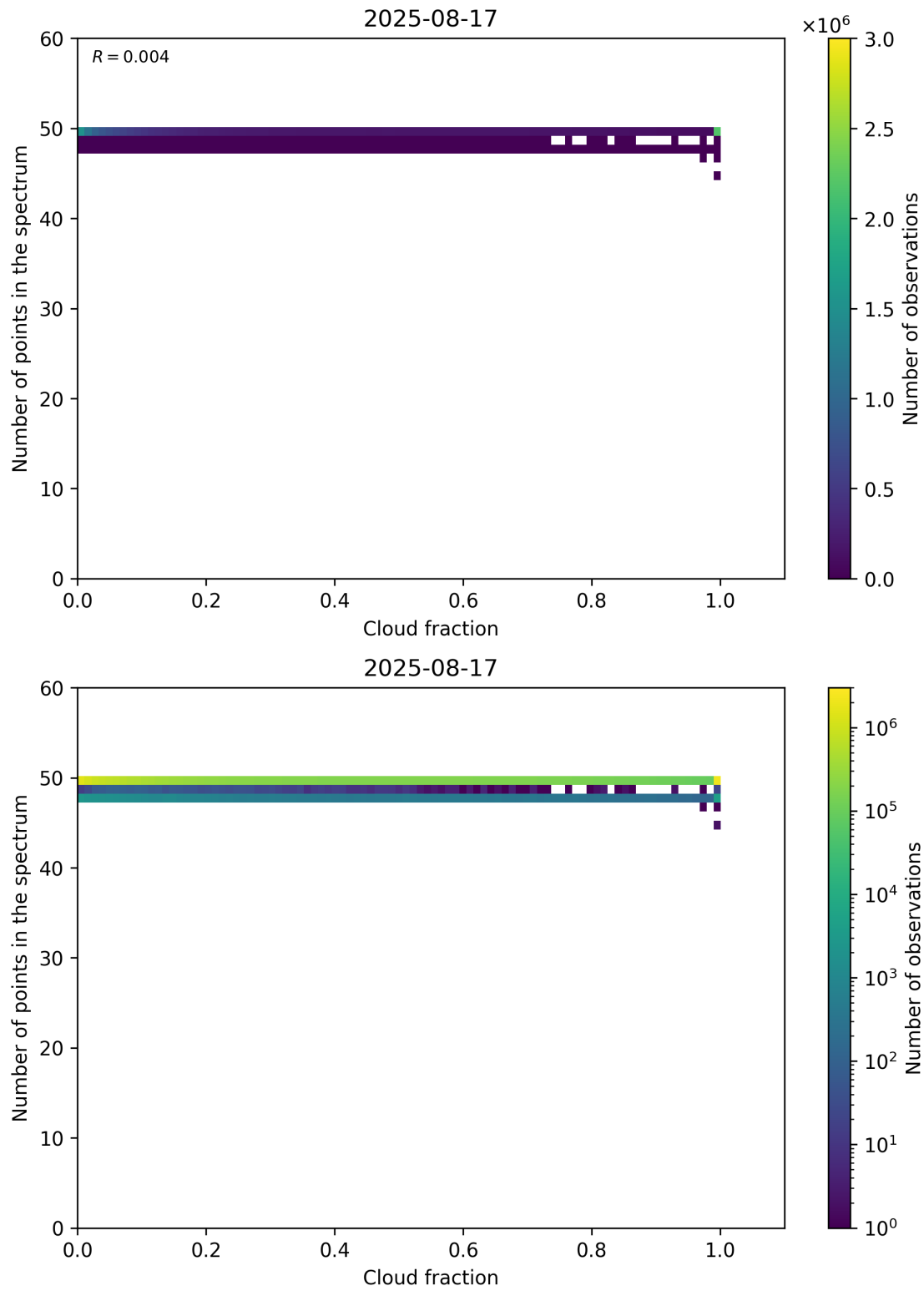
Figure 74: Scatter density plot of “Cloud fraction” against “Number of points in the spectrum” for 2025-08-16 to 2025-08-18.
