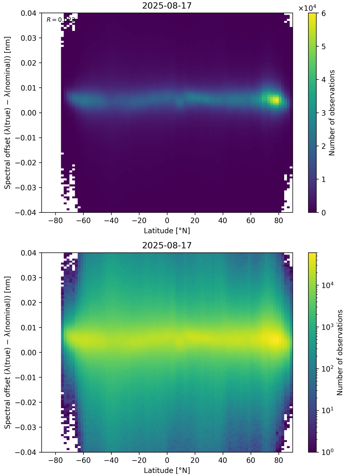
Figure 96: Scatter density plot of “Latitude” against “Spectral offset ( \lambda_{\text{true}} - \lambda_{\text{nominal}} )” for 2025-08-16 to 2025-08-18.
