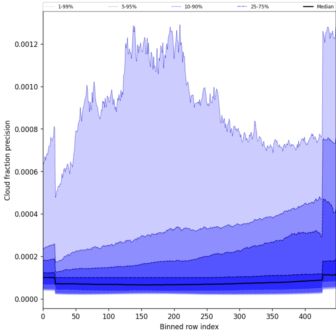
Figure 50: Along track statistics of “Cloud fraction precision” for 2025-08-16 to 2025-08-18
