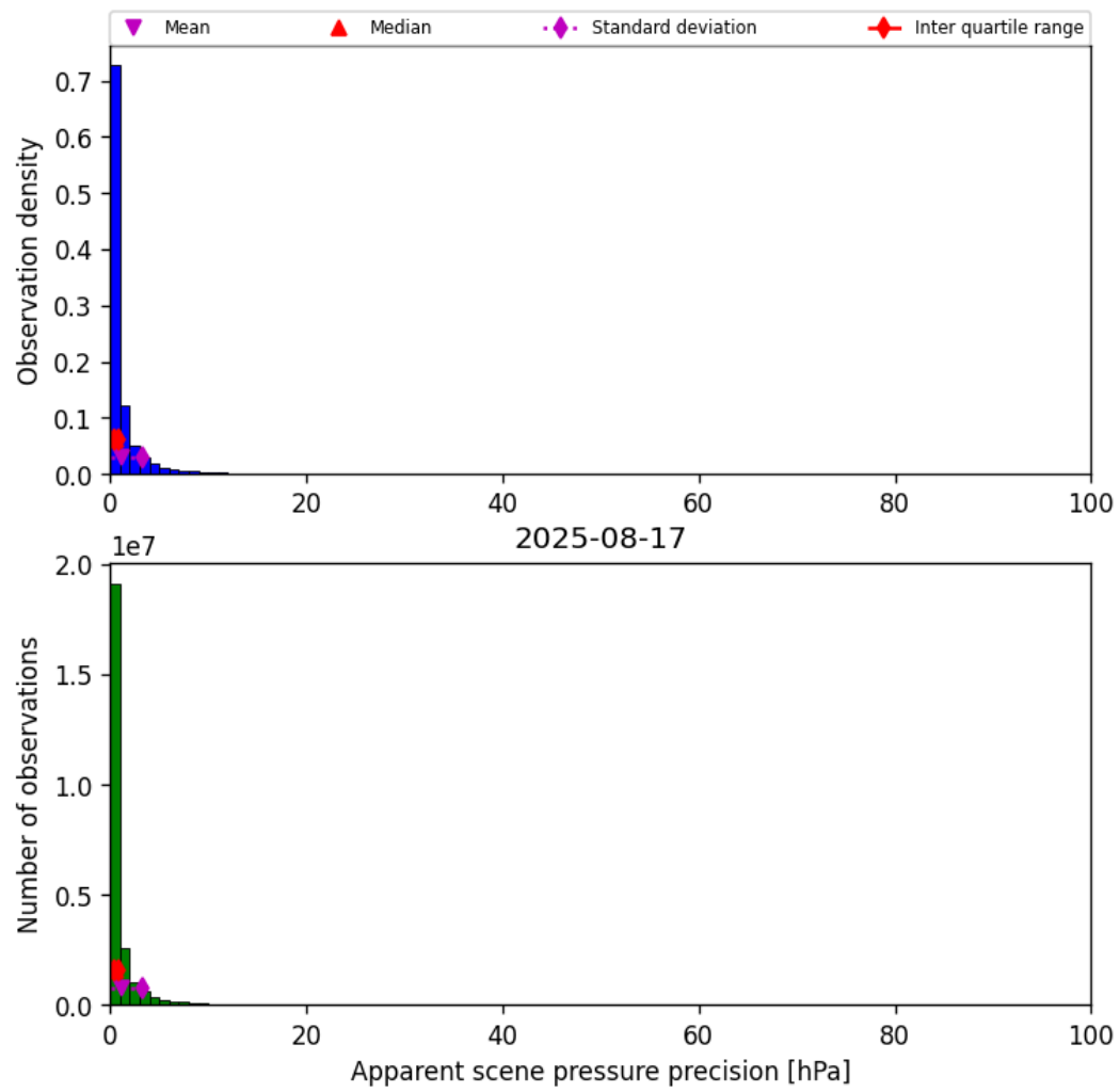
Figure 37: Histogram of “Apparent scene pressure precision” for 2025-08-16 to 2025-08-18
