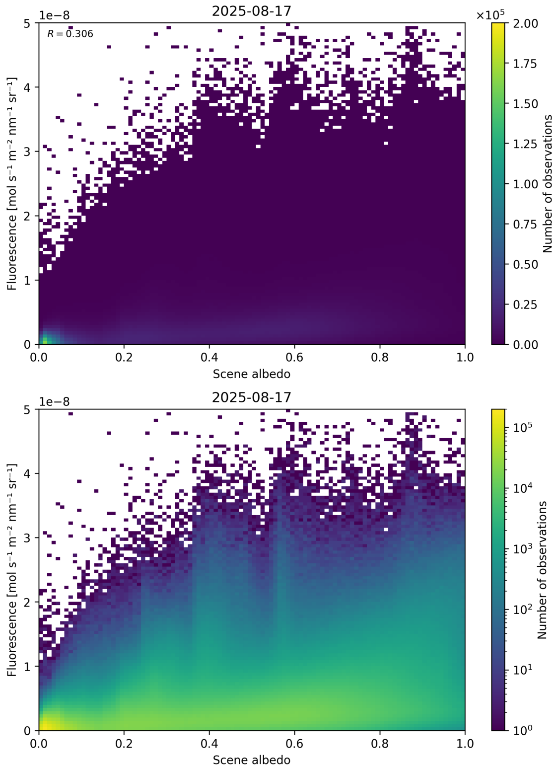
Figure 104: Scatter density plot of “Scene albedo” against “Fluorescence” for 2025-08-16 to 2025-08-18.
