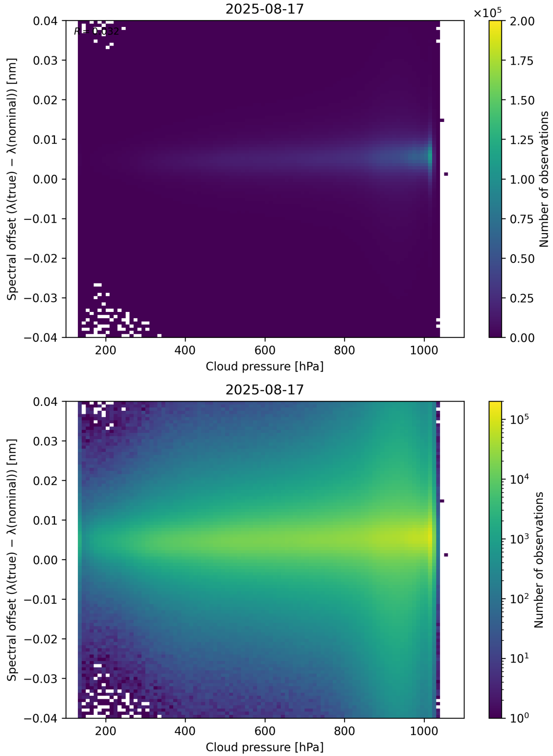
Figure 84: Scatter density plot of “Cloud pressure” against “Spectral offset ( \lambda_{\text{true}} - \lambda_{\text{nominal}} )” for 2025-08-16 to 2025-08-18.
