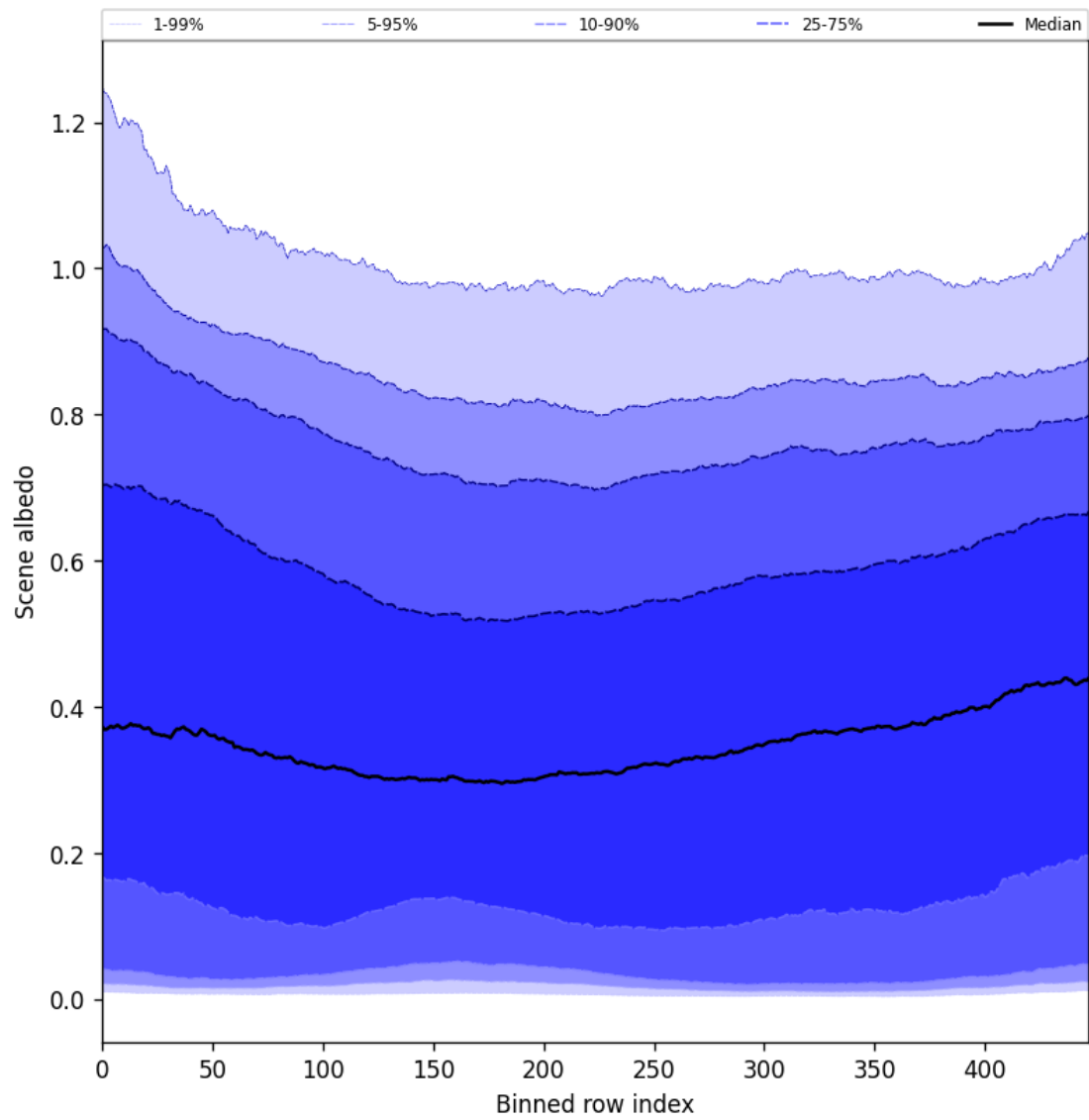
Figure 51: Along track statistics of “Scene albedo” for 2025-08-16 to 2025-08-18
