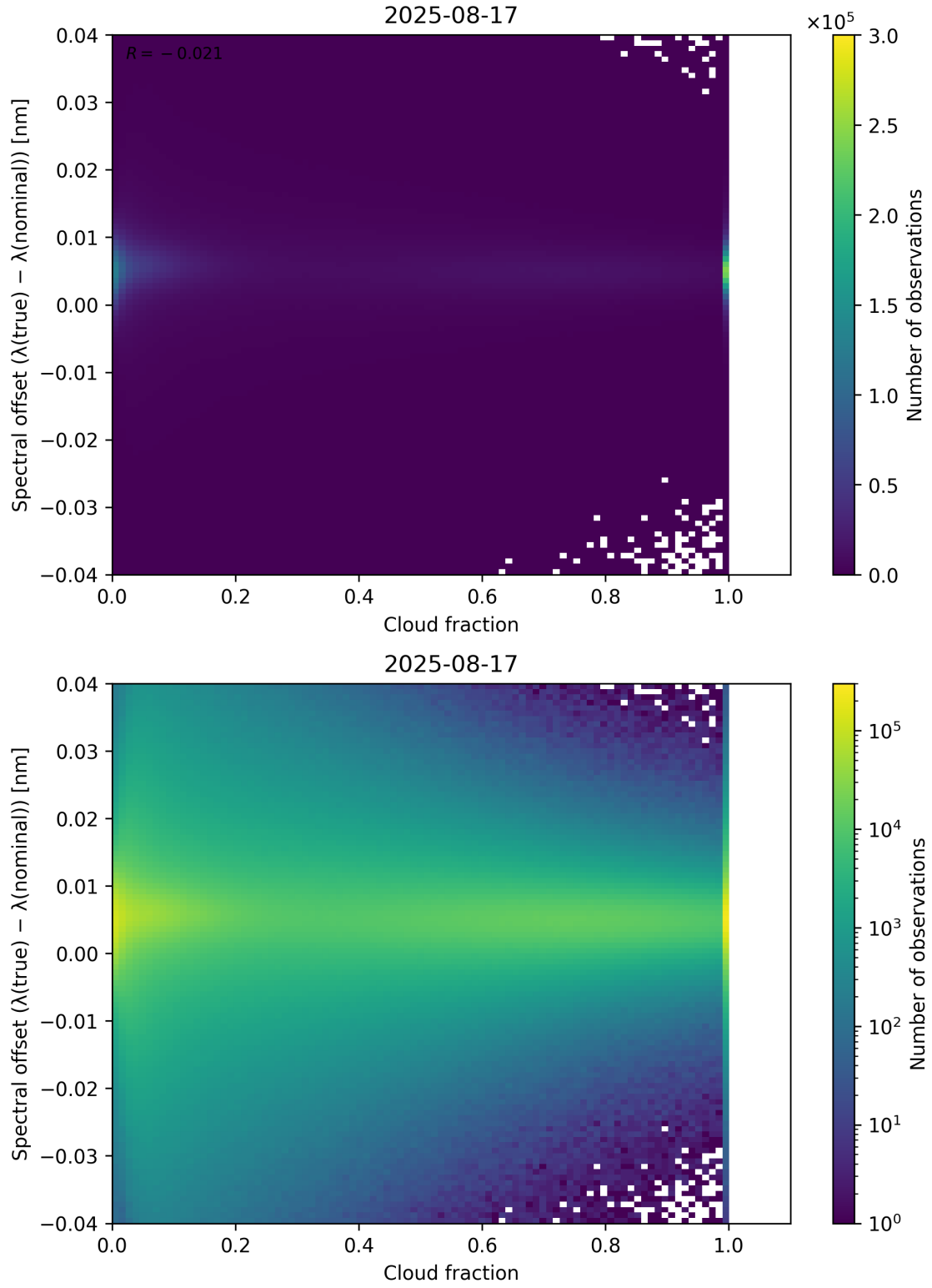
Figure 76: Scatter density plot of “Cloud fraction” against “Spectral offset ( \lambda_{\text{true}} - \lambda_{\text{nominal}} )” for 2025-08-16 to 2025-08-18.
