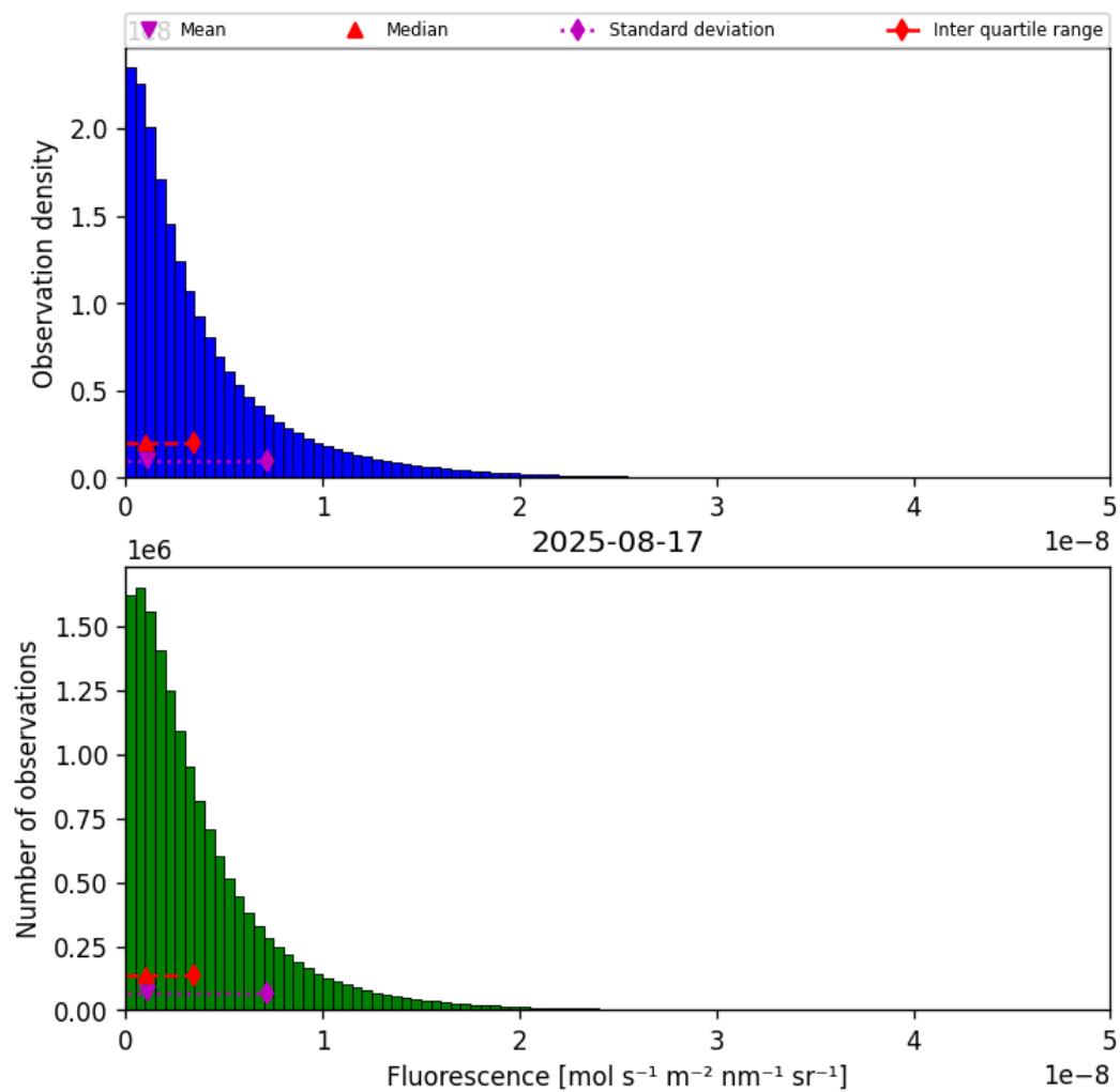
Figure 40: Histogram of “Fluorescence” for 2025-08-16 to 2025-08-18
