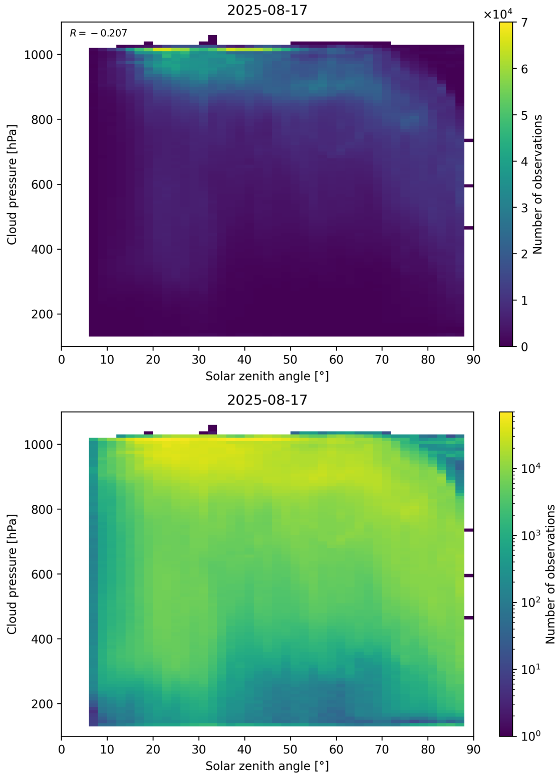
Figure 111: Scatter density plot of “Solar zenith angle” against “Cloud pressure” for 2025-08-16 to 2025-08-18.
