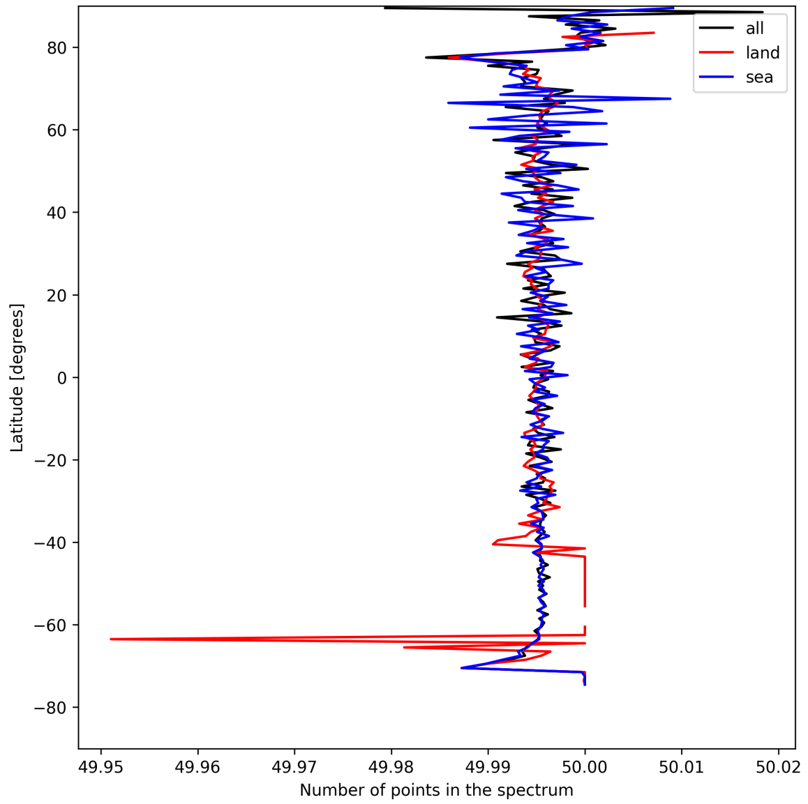
Figure 27: Zonal average of “Number of points in the spectrum” for 2025-08-16 to 2025-08-18.
