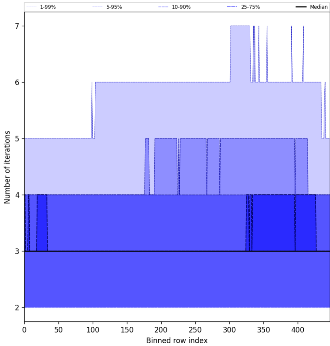
Figure 56: Along track statistics of “Number of iterations” for 2025-08-16 to 2025-08-18
