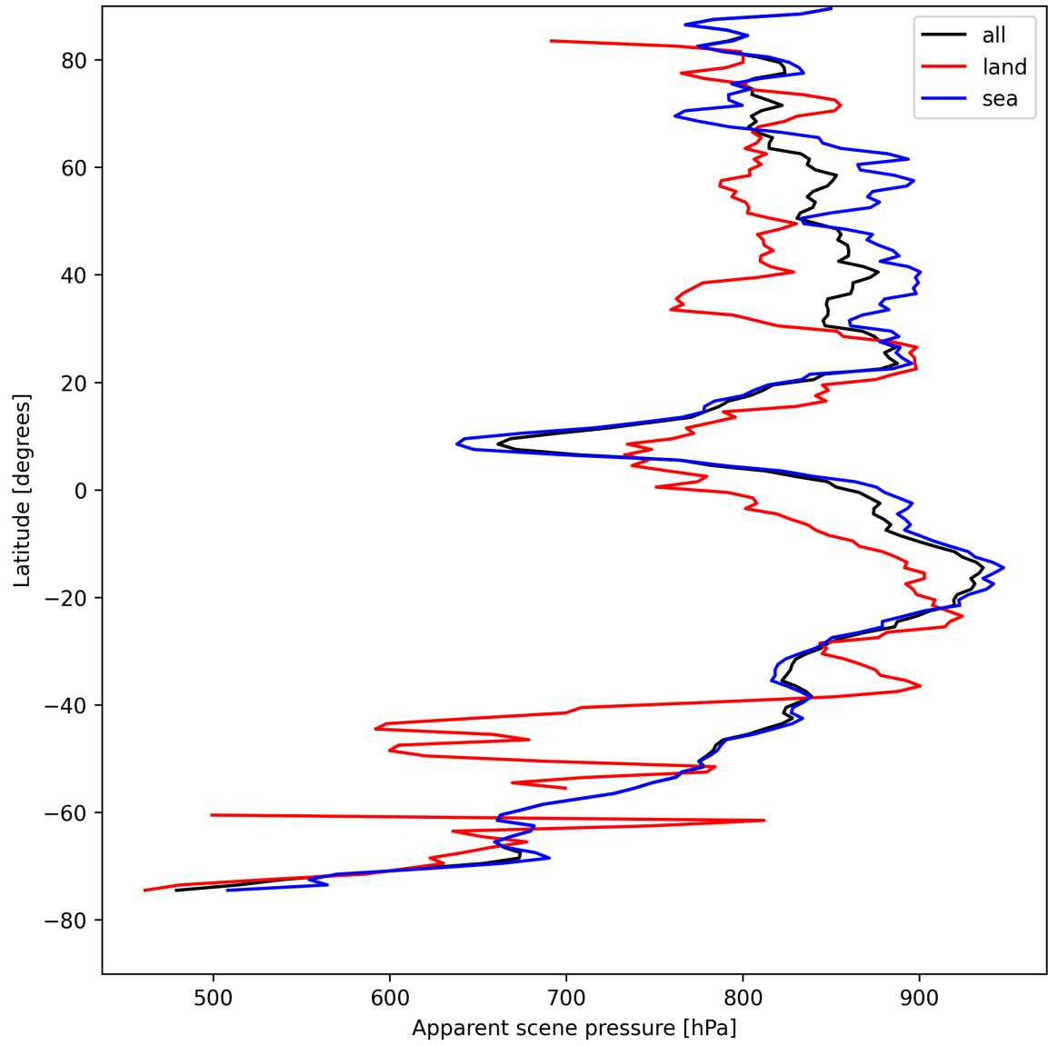
Figure 19: Zonal average of “Apparent scene pressure” for 2025-08-16 to 2025-08-18.
