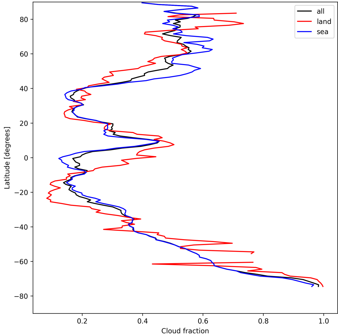
Figure 15: Zonal average of “Cloud fraction” for 2025-08-16 to 2025-08-18.
