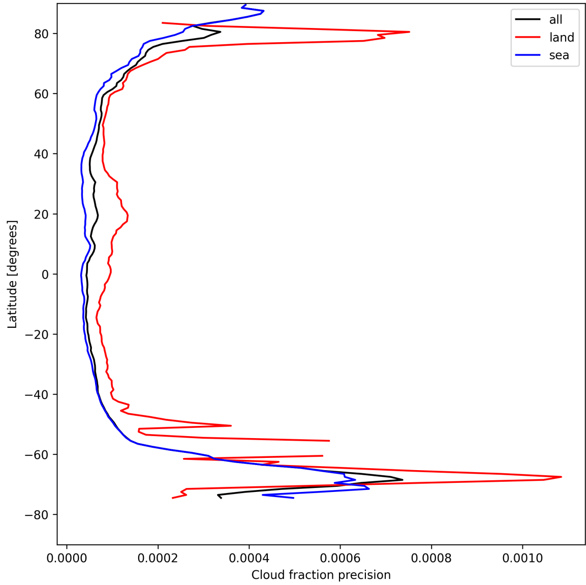
Figure 16: Zonal average of “Cloud fraction precision” for 2025-08-16 to 2025-08-18.
