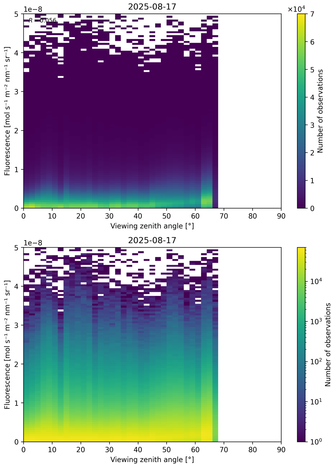
Figure 122: Scatter density plot of “Viewing zenith angle” against “Fluorescence” for 2025-08-16 to 2025-08-18.
