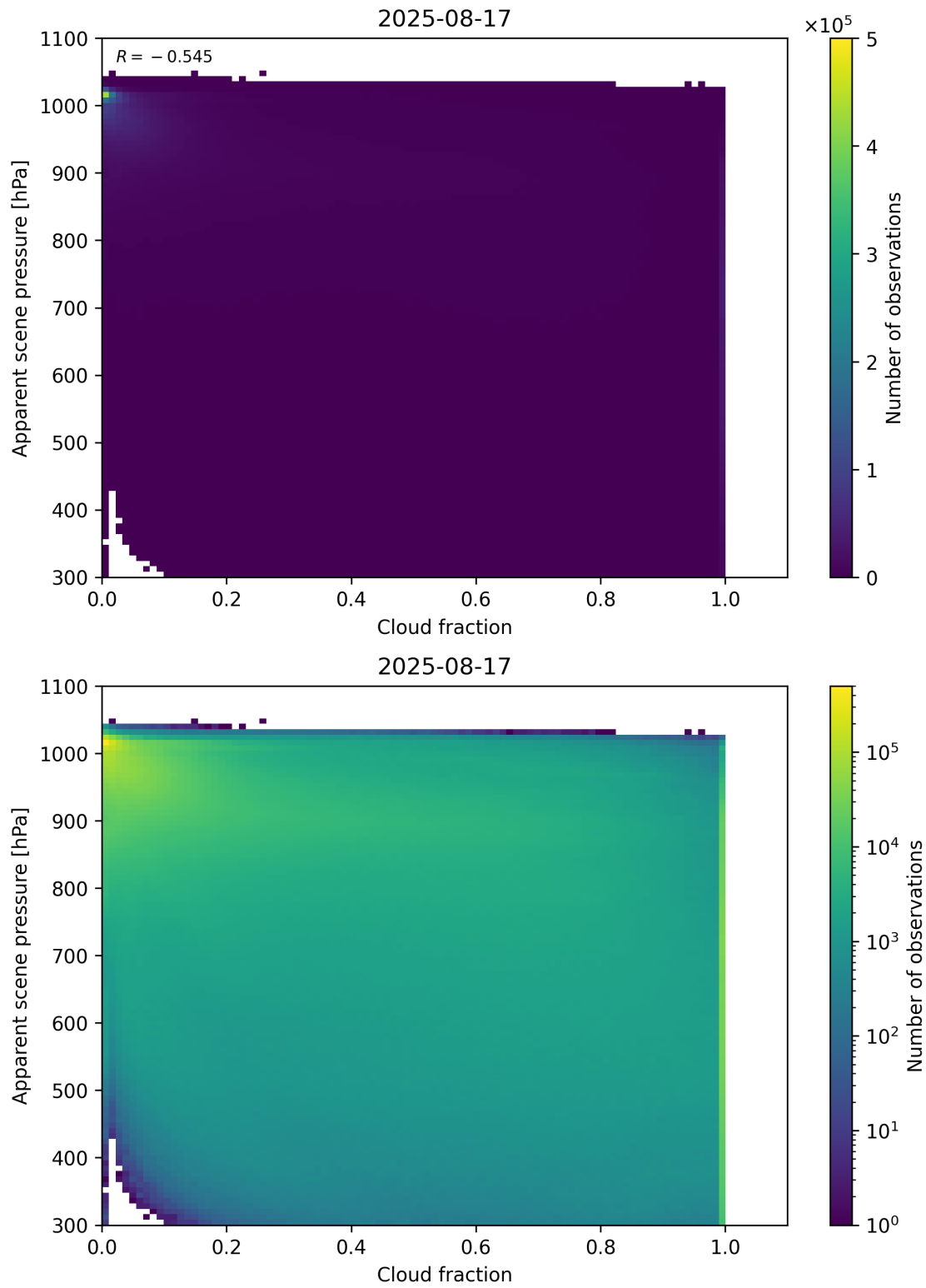
Figure 70: Scatter density plot of “Cloud fraction” against “Apparent scene pressure” for 2025-08-16 to 2025-08-18.
