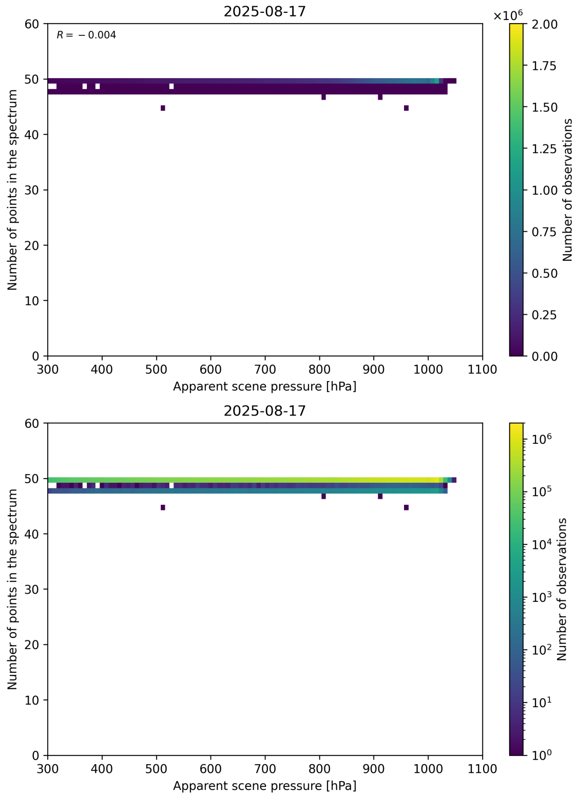
Figure 66: Scatter density plot of “Apparent scene pressure” against “Number of points in the spectrum” for 2025-08-16 to 2025-08-18.
