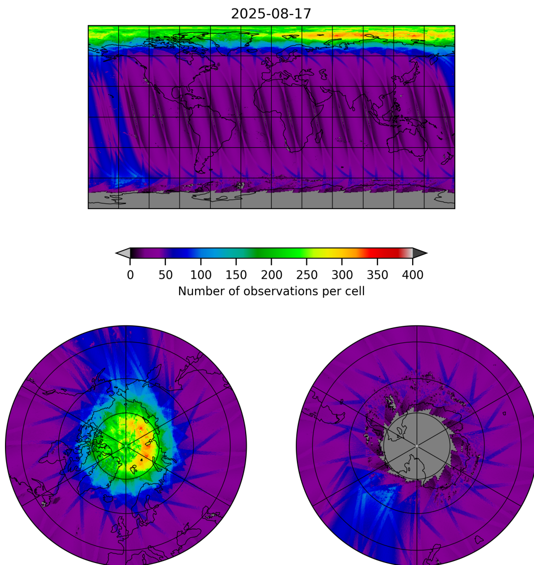
Figure 11: Map of the number of observations for 2025-08-16 to 2025-08-18
