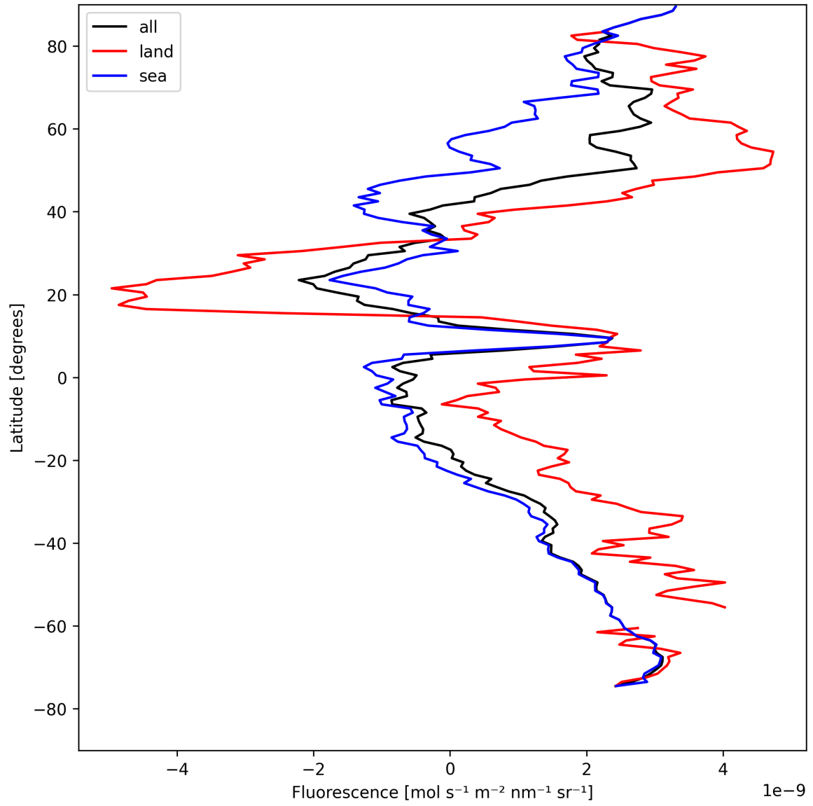
Figure 23: Zonal average of “Fluorescence” for 2025-08-16 to 2025-08-18.
