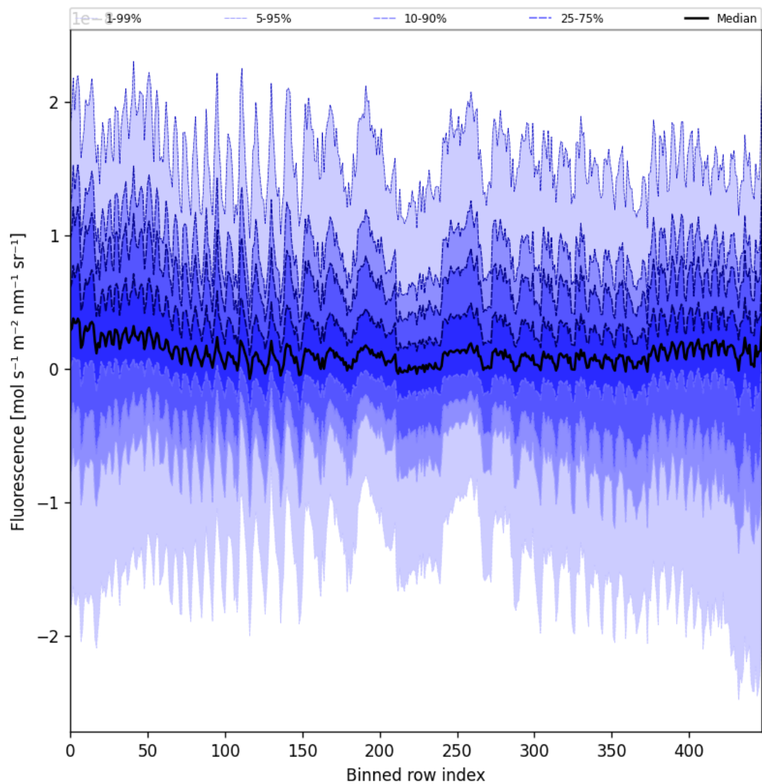
Figure 57: Along track statistics of “Fluorescence” for 2025-08-16 to 2025-08-18
