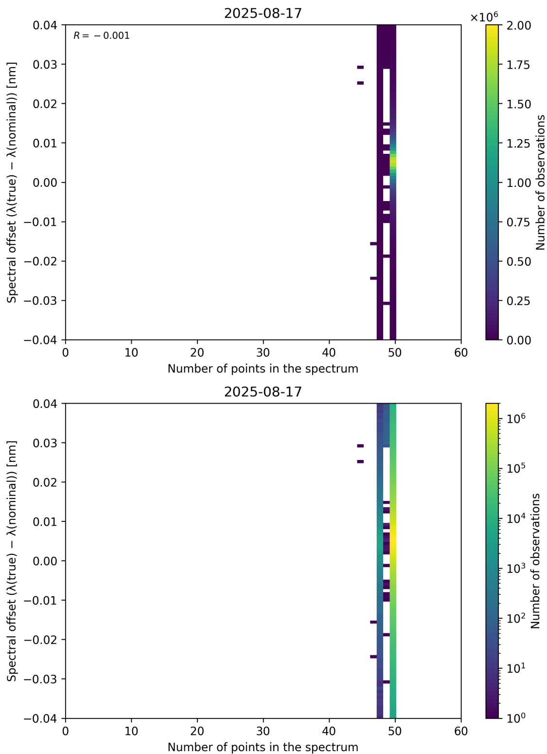
Figure 101: Scatter density plot of “Number of points in the spectrum” against “Spectral offset ( \lambda_{\text{true}} - \lambda_{\text{nominal}} )” for 2025-08-16 to 2025-08-18.
