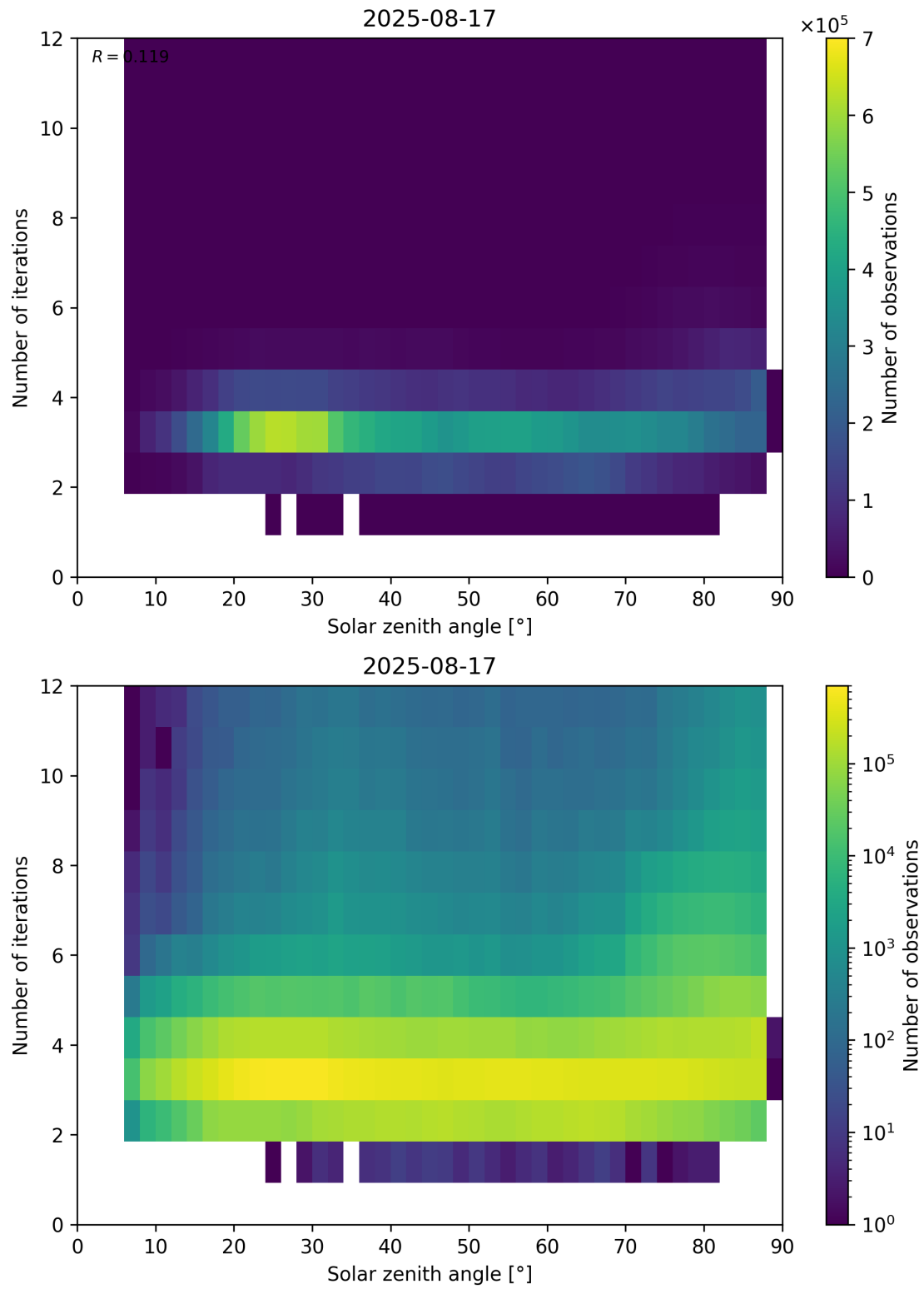
Figure 114: Scatter density plot of “Solar zenith angle” against “Number of iterations” for 2025-08-16 to 2025-08-18.
