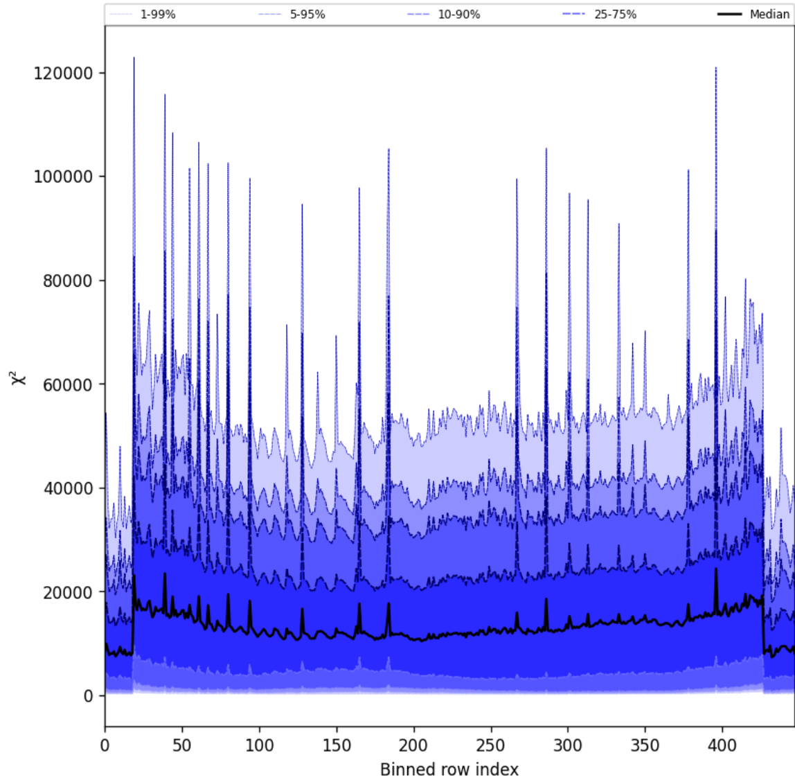
Figure 55: Along track statistics of “ \chi^2 ” for 2025-08-16 to 2025-08-18
