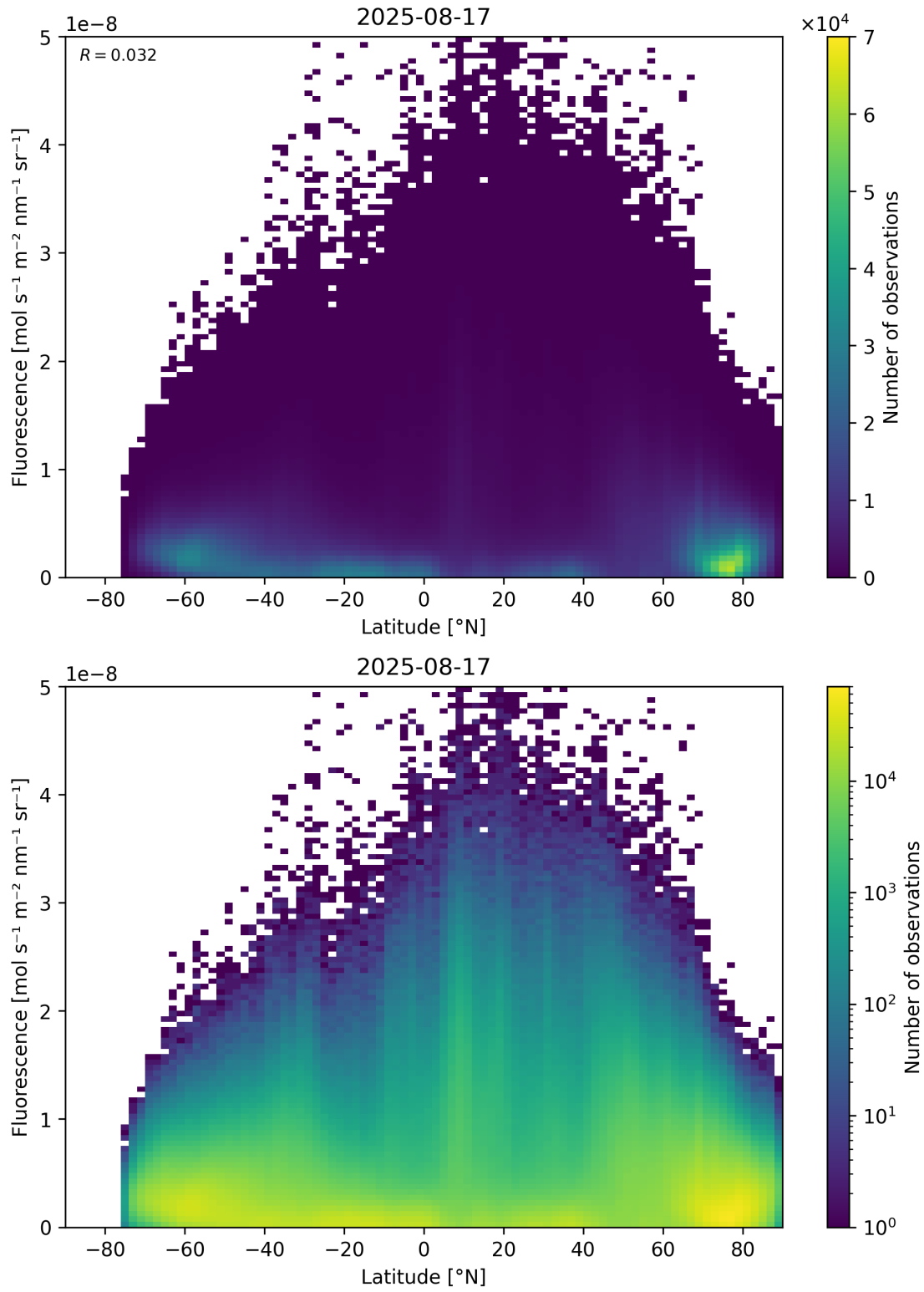
Figure 92: Scatter density plot of “Latitude” against “Fluorescence” for 2025-08-16 to 2025-08-18.
