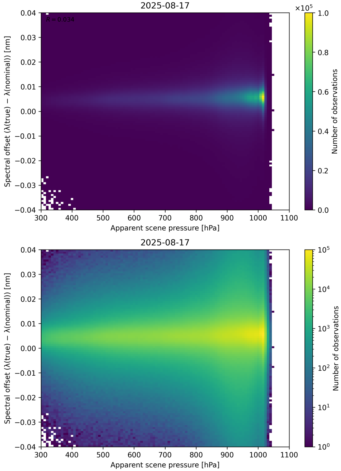
Figure 67: Scatter density plot of “Apparent scene pressure” against “Spectral offset ( \lambda_{\text{true}} - \lambda_{\text{nominal}} )” for 2025-08-16 to 2025-08-18.
