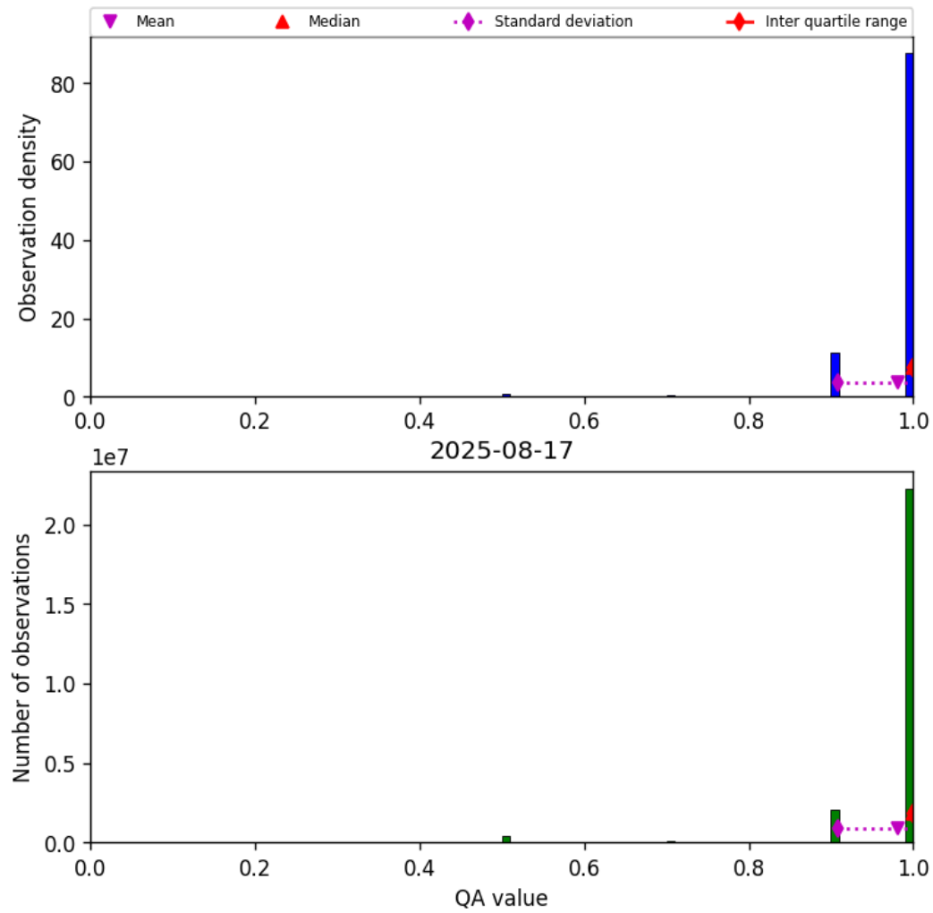
Figure 29: Histogram of “QA value” for 2025-08-16 to 2025-08-18
