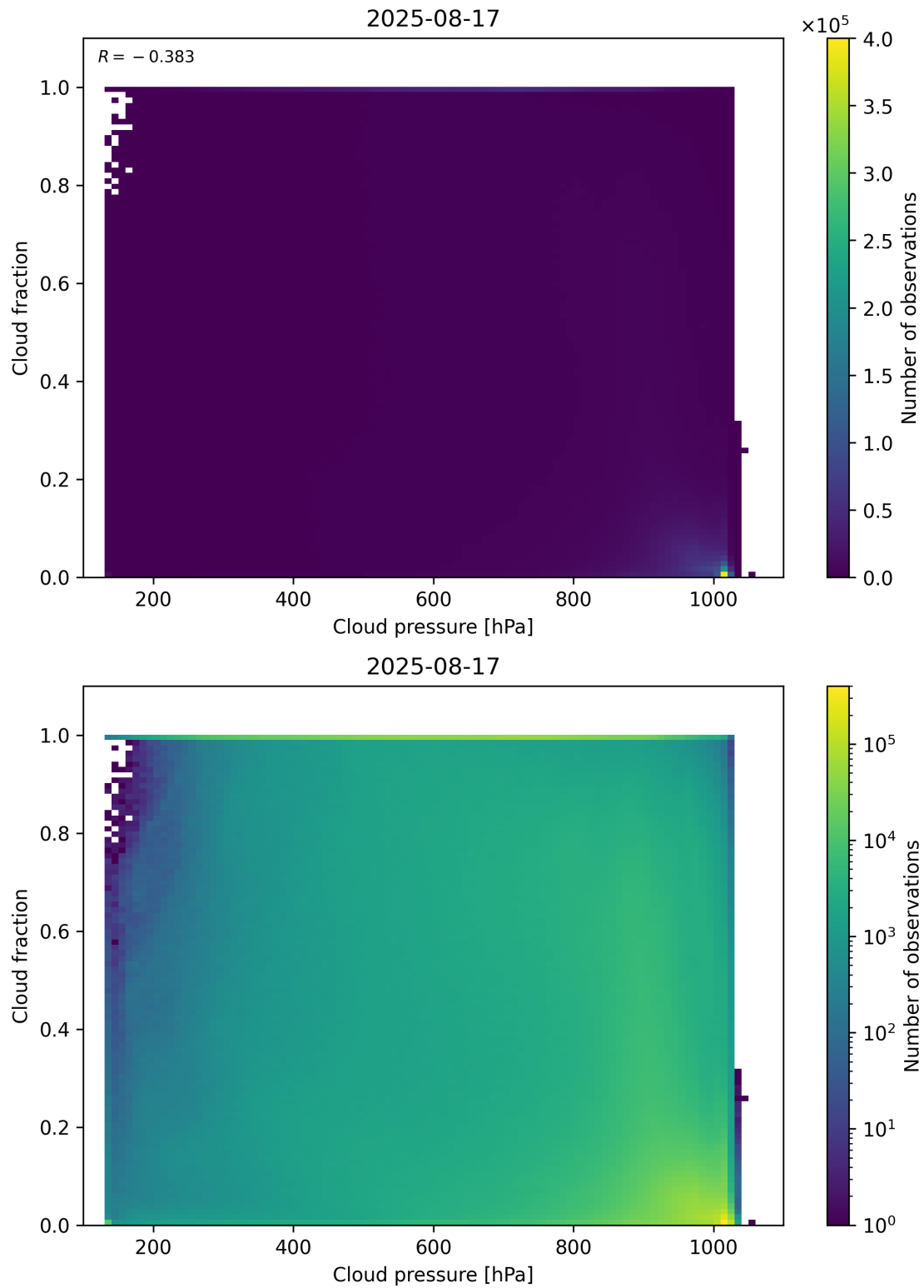
Figure 79: Scatter density plot of “Cloud pressure” against “Cloud fraction” for 2025-08-16 to 2025-08-18.
