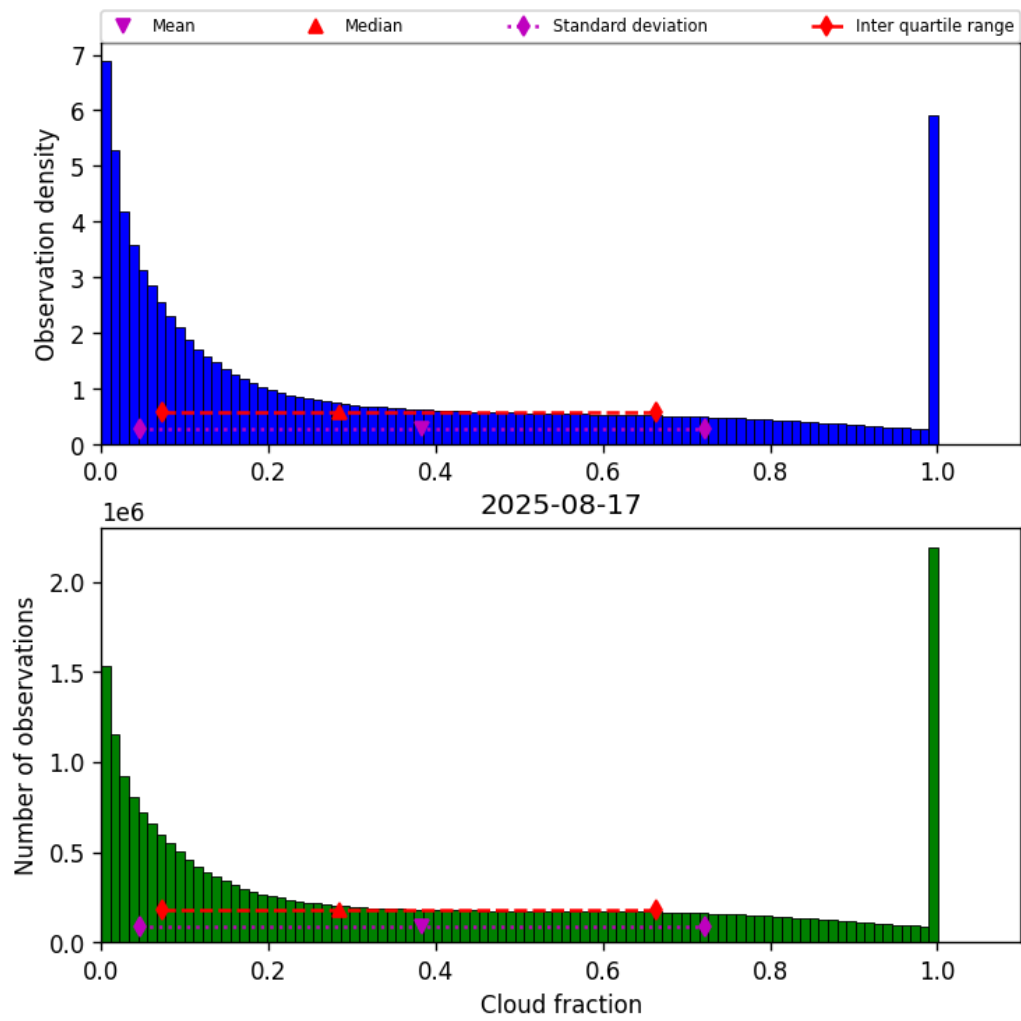
Figure 32: Histogram of “Cloud fraction” for 2025-08-16 to 2025-08-18
