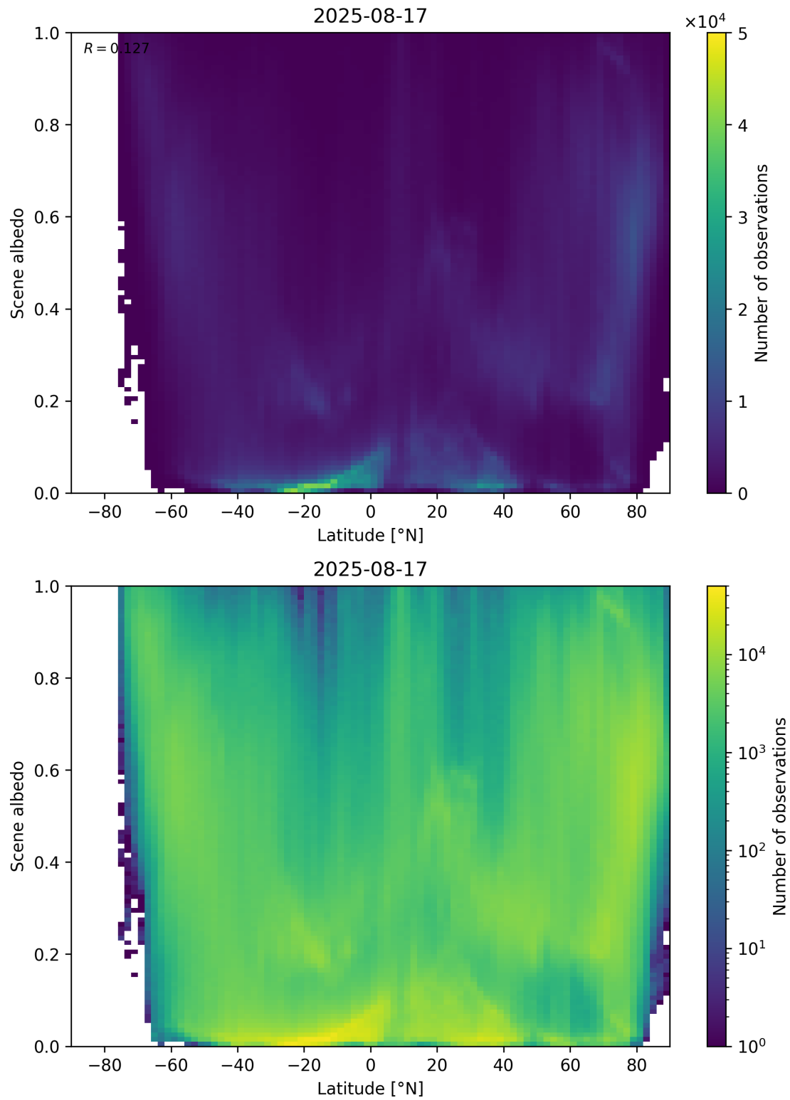
Figure 95: Scatter density plot of “Latitude” against “Scene albedo” for 2025-08-16 to 2025-08-18.
