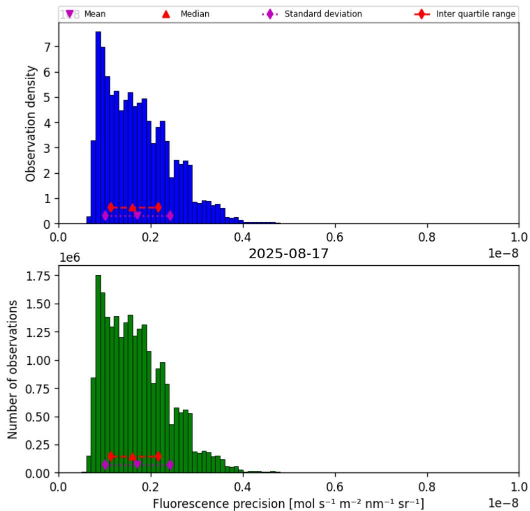
Figure 41: Histogram of “Fluorescence precision” for 2025-08-16 to 2025-08-18
