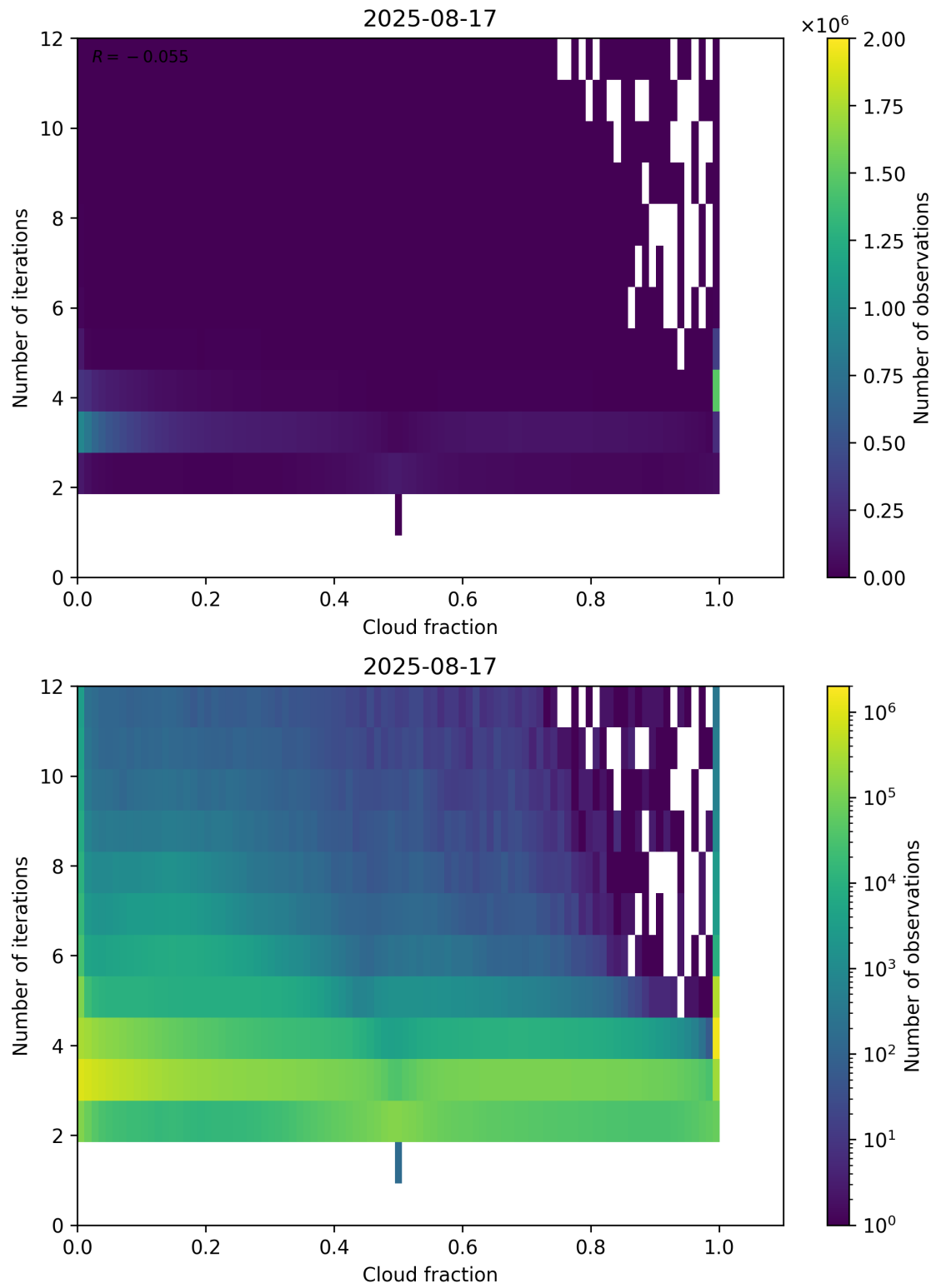
Figure 73: Scatter density plot of “Cloud fraction” against “Number of iterations” for 2025-08-16 to 2025-08-18.
