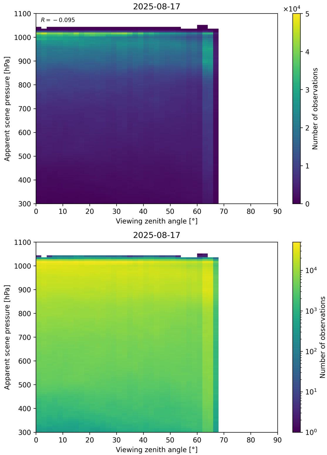
Figure 118: Scatter density plot of “Viewing zenith angle” against “Apparent scene pressure” for 2025-08-16 to 2025-08-18.
