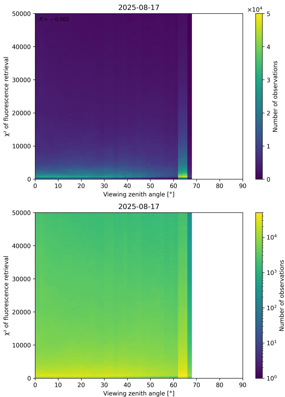
Figure 119: Scatter density plot of “Viewing zenith angle” against “ \chi^2 of fluorescence retrieval” for 2025-08-16 to 2025-08-18.
