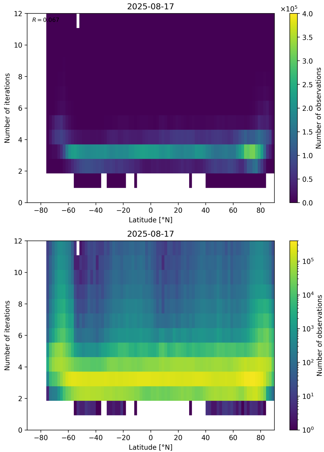
Figure 93: Scatter density plot of “Latitude” against “Number of iterations” for 2025-08-16 to 2025-08-18.
