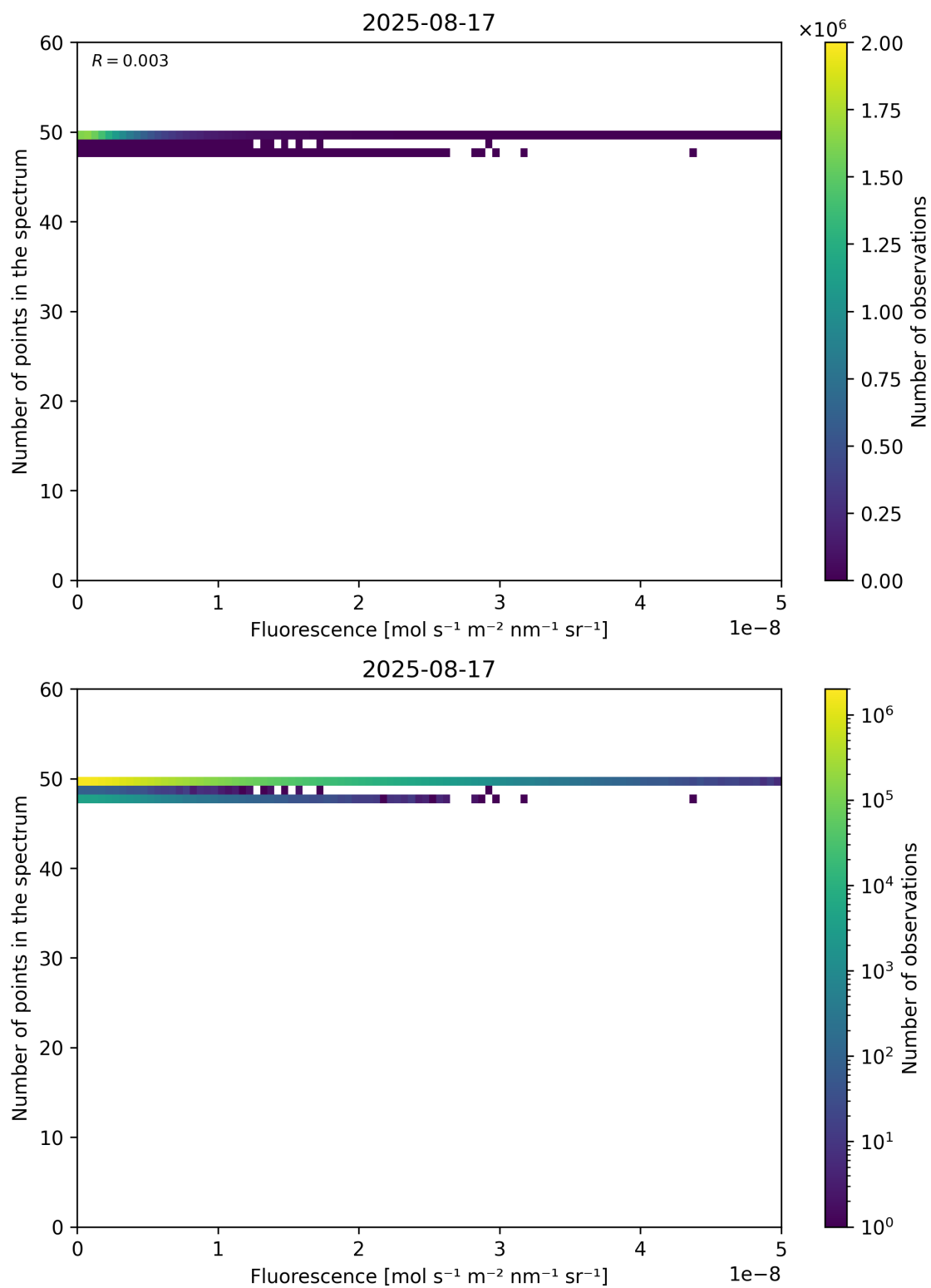
Figure 86: Scatter density plot of “Fluorescence” against “Number of points in the spectrum” for 2025-08-16 to 2025-08-18.
