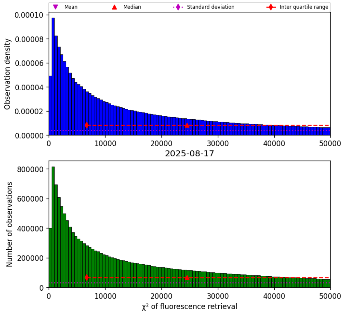
Figure 42: Histogram of “ \chi^2 of fluorescence retrieval” for 2025-08-16 to 2025-08-18
