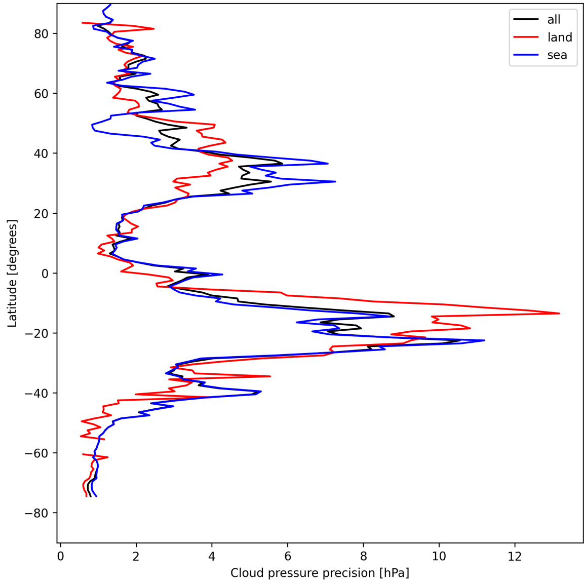
Figure 14: Zonal average of “Cloud pressure precision” for 2025-08-16 to 2025-08-18.
