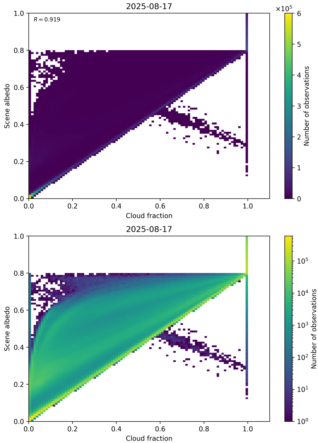
Figure 75: Scatter density plot of “Cloud fraction” against “Scene albedo” for 2025-08-16 to 2025-08-18.
