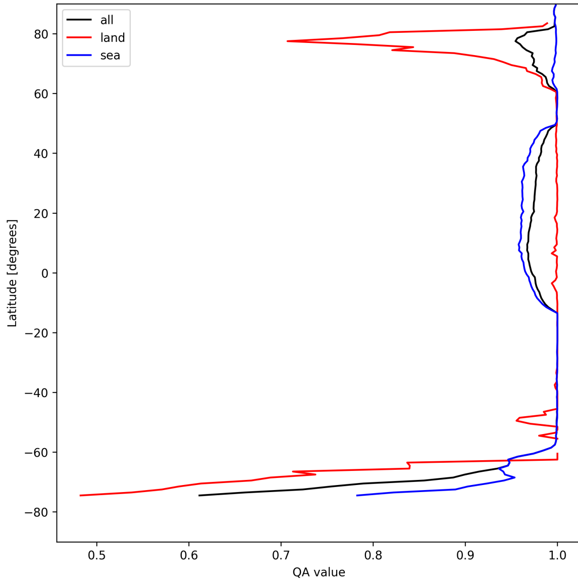
Figure 12: Zonal average of “QA value” for 2025-08-16 to 2025-08-18.
