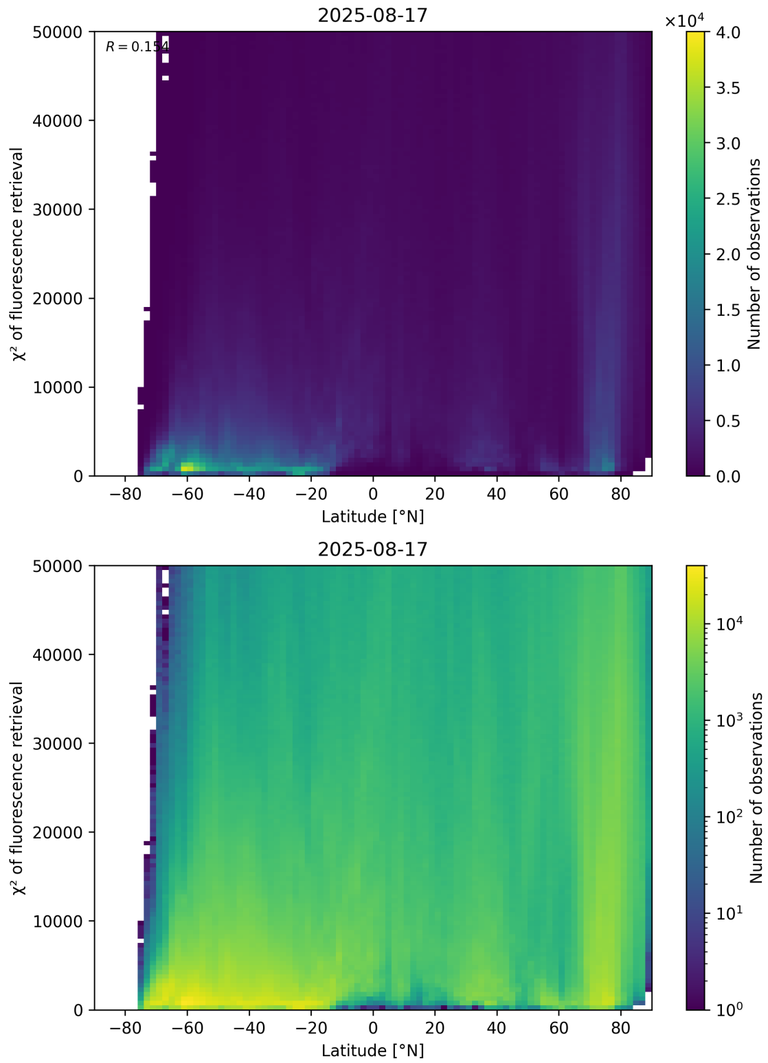
Figure 89: Scatter density plot of “Latitude” against “ \chi^2 of fluorescence retrieval” for 2025-08-16 to 2025-08-18.
