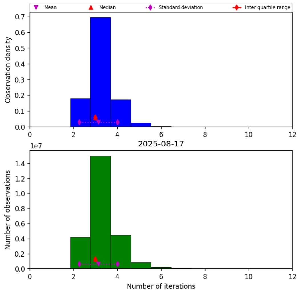
Figure 39: Histogram of “Number of iterations” for 2025-08-16 to 2025-08-18
