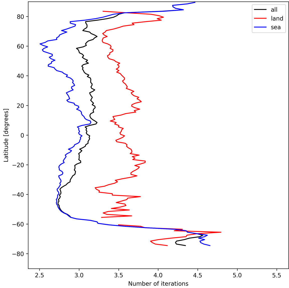
Figure 22: Zonal average of “Number of iterations” for 2025-08-16 to 2025-08-18.
