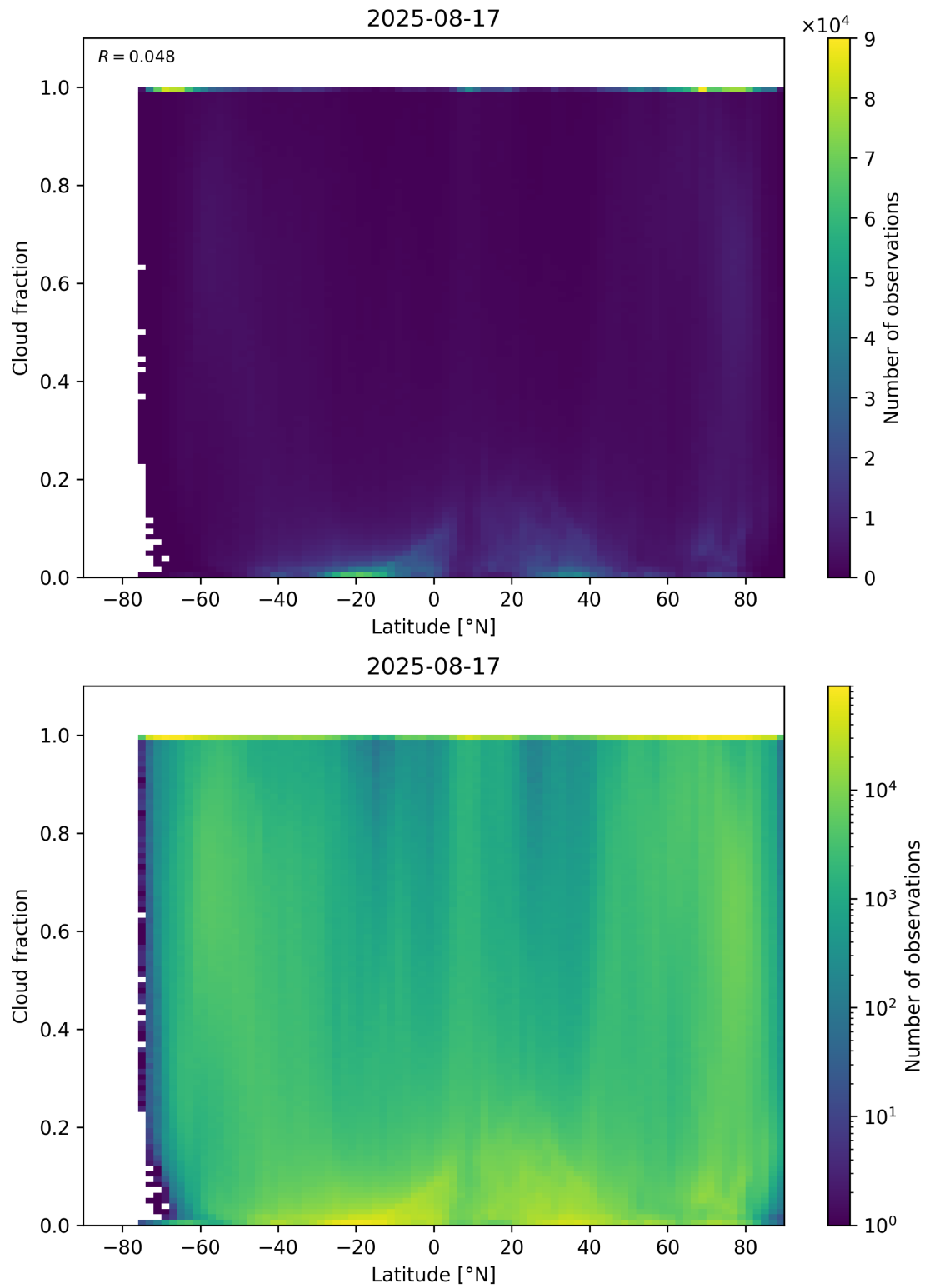
Figure 90: Scatter density plot of “Latitude” against “Cloud fraction” for 2025-08-16 to 2025-08-18.
