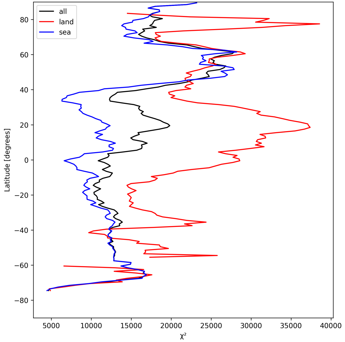
Figure 21: Zonal average of “ \chi^2 ” for 2025-08-16 to 2025-08-18.
