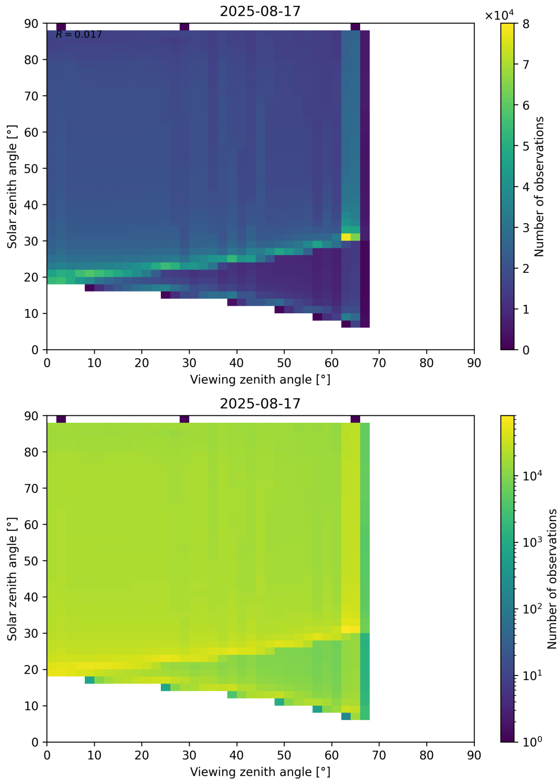
Figure 127: Scatter density plot of “Viewing zenith angle” against “Solar zenith angle” for 2025-08-16 to 2025-08-18.
