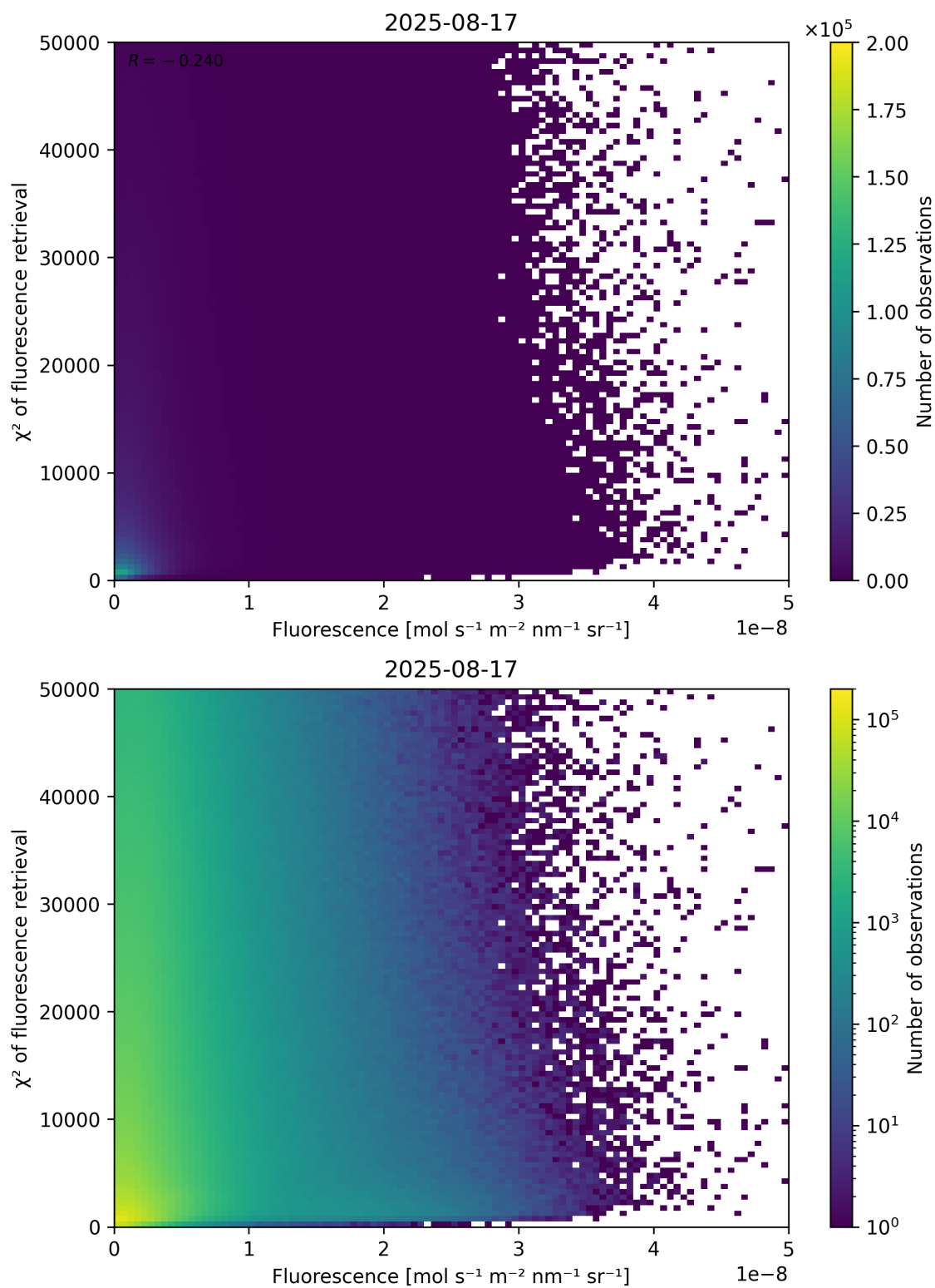
Figure 85: Scatter density plot of “Fluorescence” against “ \chi^2 of fluorescence retrieval” for 2025-08-16 to 2025-08-18.
