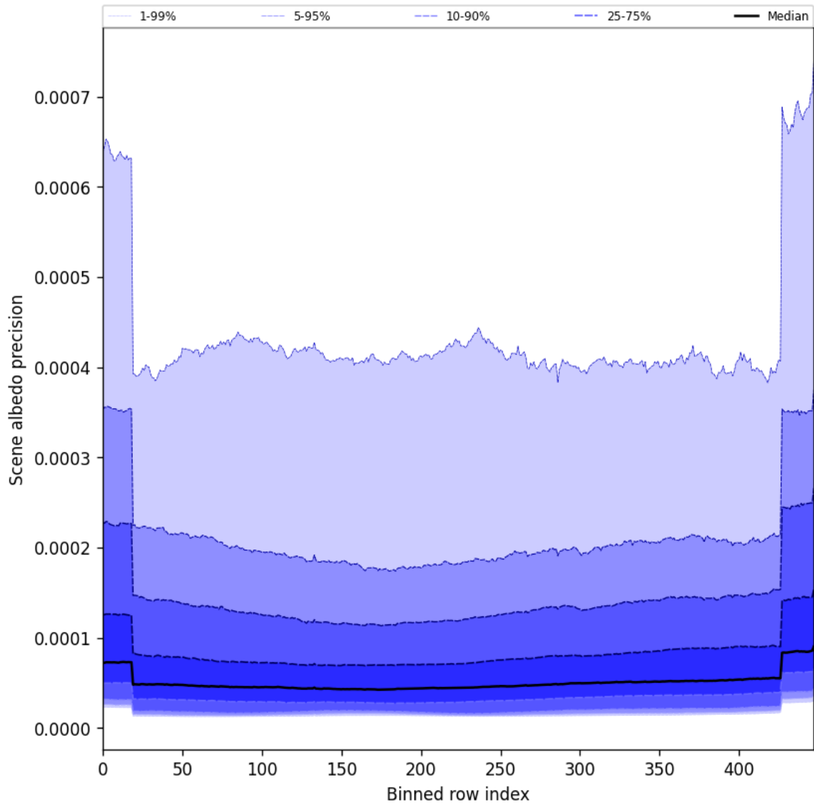
Figure 52: Along track statistics of “Scene albedo precision” for 2025-08-16 to 2025-08-18
