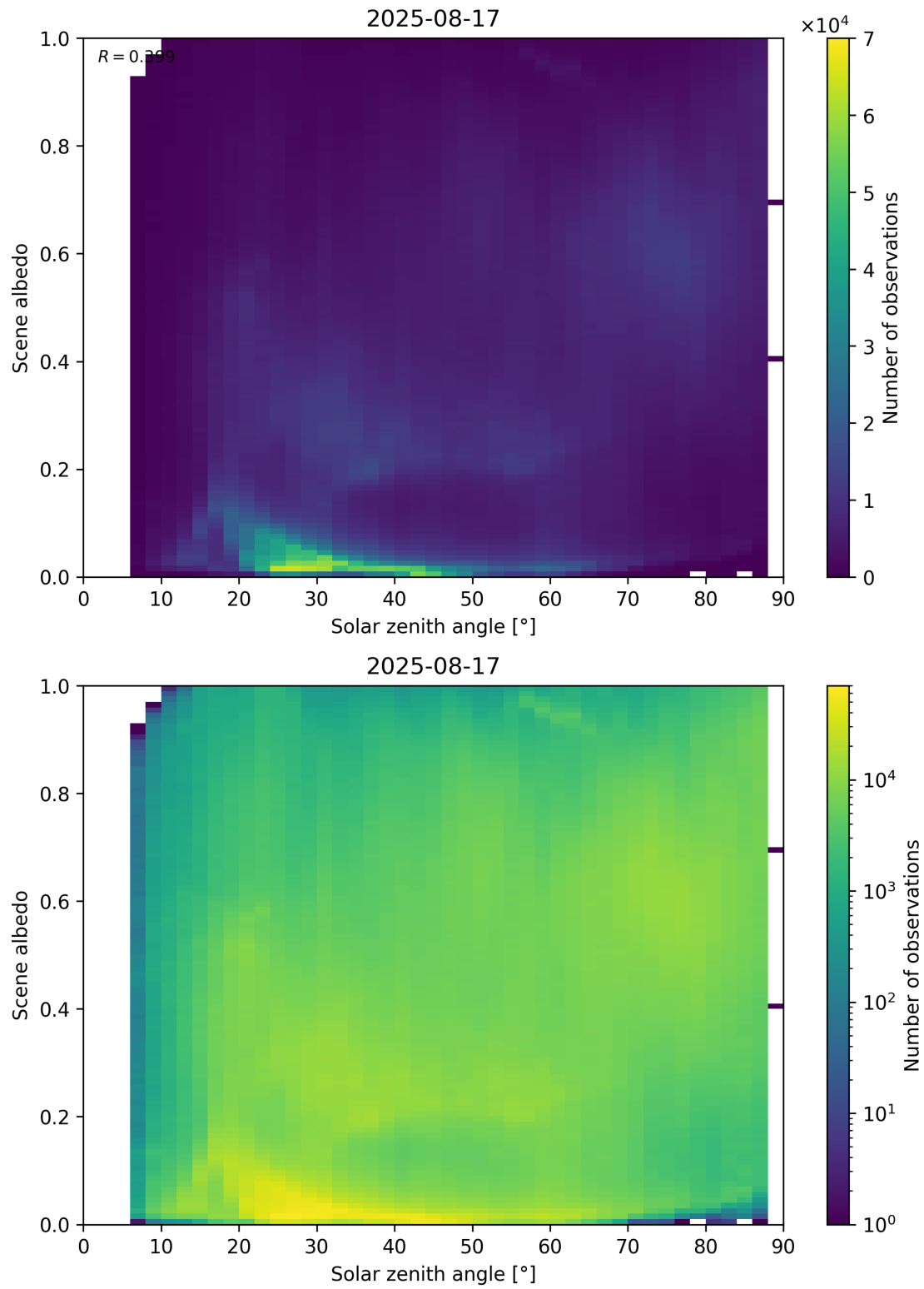
Figure 116: Scatter density plot of “Solar zenith angle” against “Scene albedo” for 2025-08-16 to 2025-08-18.
