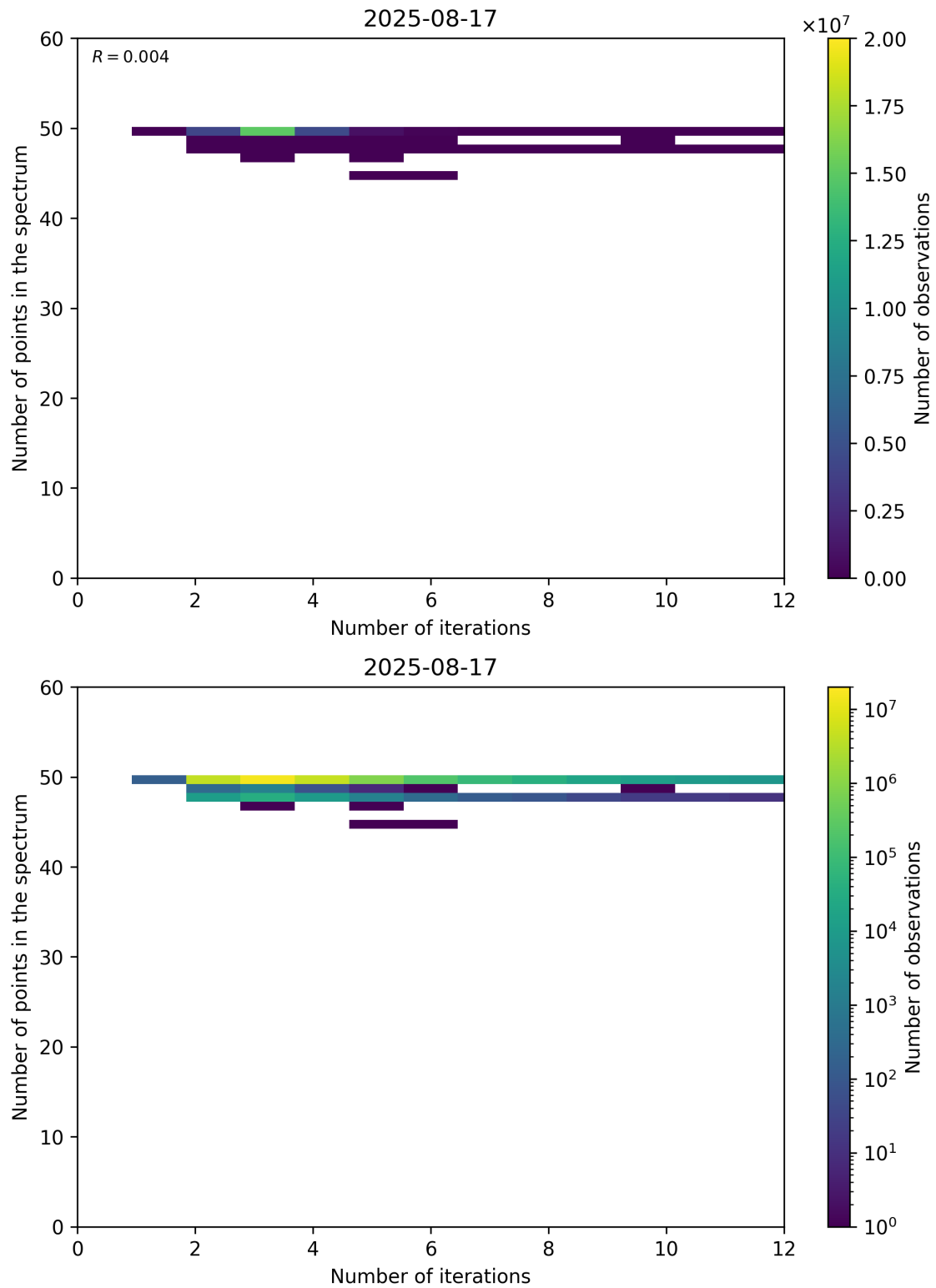
Figure 99: Scatter density plot of “Number of iterations” against “Number of points in the spectrum” for 2025-08-16 to 2025-08-18.
