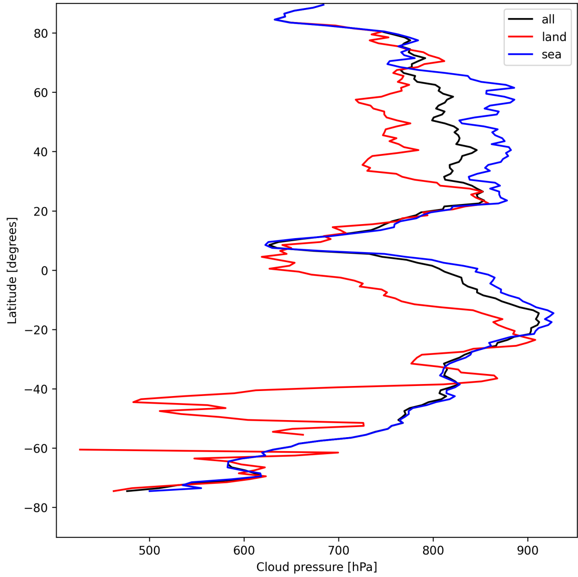
Figure 13: Zonal average of “Cloud pressure” for 2025-08-16 to 2025-08-18.
