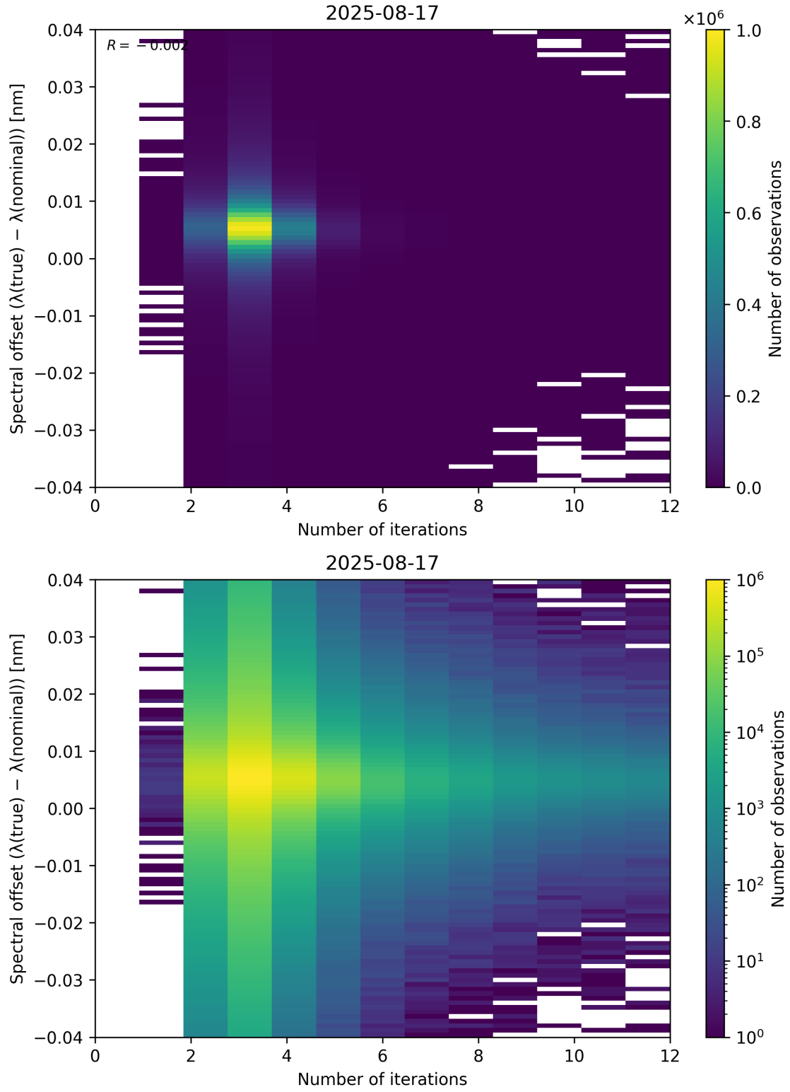
Figure 100: Scatter density plot of “Number of iterations” against “Spectral offset ( \lambda_{\text{true}} - \lambda_{\text{nominal}} )” for 2025-08-16 to 2025-08-18.
