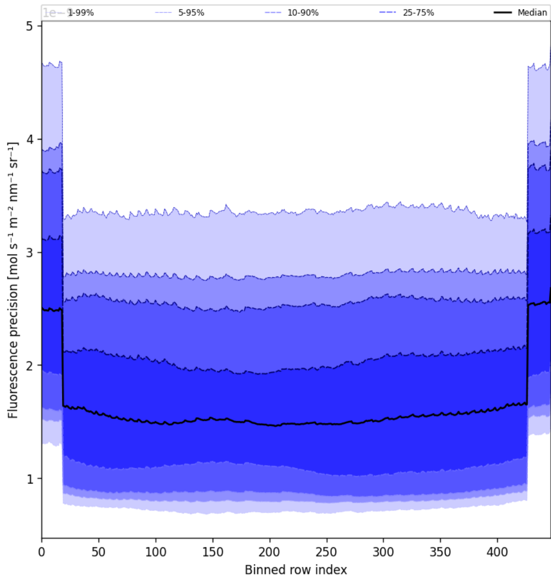
Figure 58: Along track statistics of “Fluorescence precision” for 2025-08-16 to 2025-08-18
