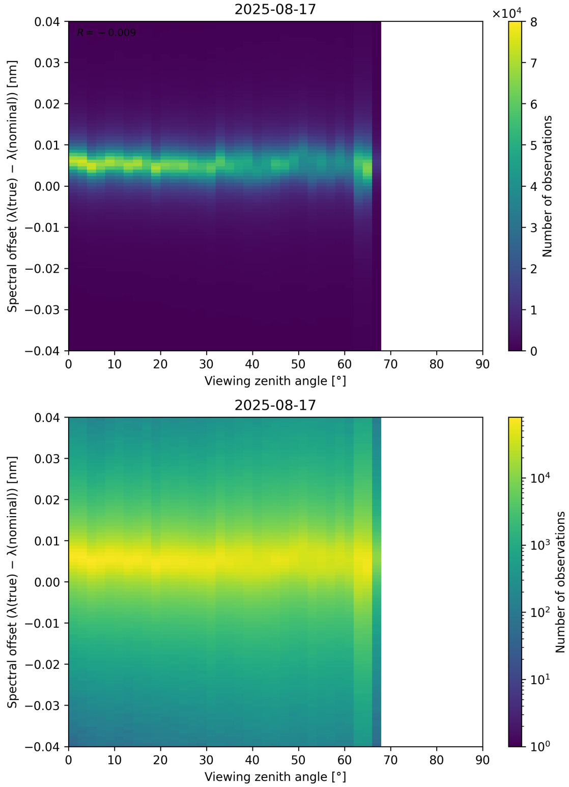
Figure 128: Scatter density plot of “Viewing zenith angle” against “Spectral offset ( \lambda_{\text{true}} - \lambda_{\text{nominal}} )” for 2025-08-16 to 2025-08-18.
