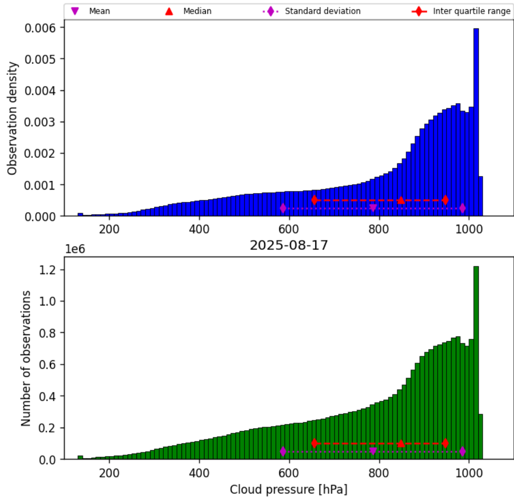
Figure 30: Histogram of “Cloud pressure” for 2025-08-16 to 2025-08-18
