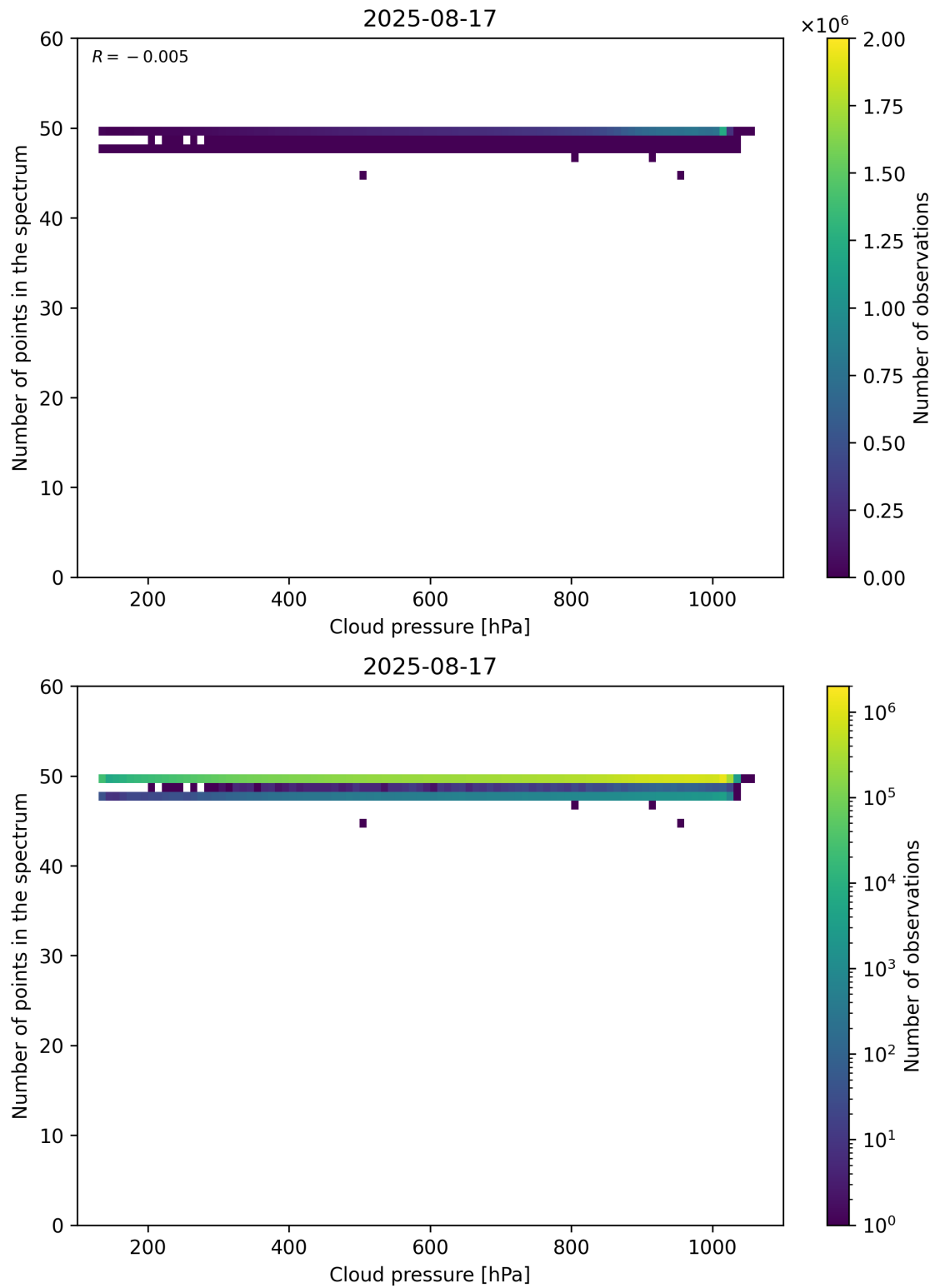
Figure 82: Scatter density plot of “Cloud pressure” against “Number of points in the spectrum” for 2025-08-16 to 2025-08-18.
