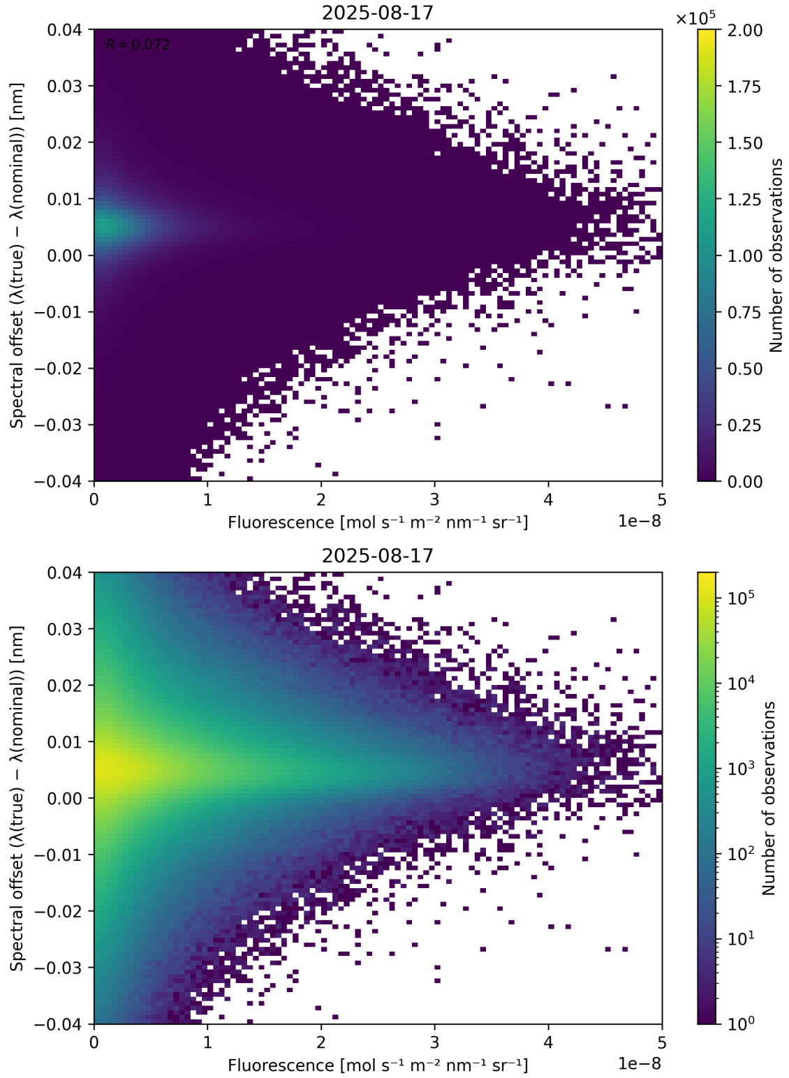
Figure 87: Scatter density plot of “Fluorescence” against “Spectral offset ( \lambda_{\text{true}} - \lambda_{\text{nominal}} )” for 2025-08-16 to 2025-08-18.
