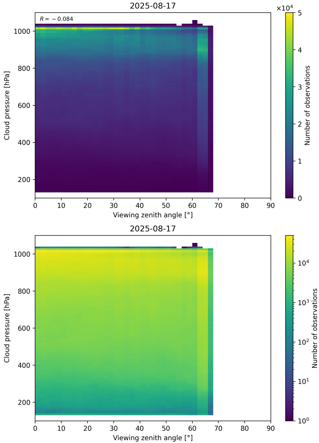
Figure 121: Scatter density plot of “Viewing zenith angle” against “Cloud pressure” for 2025-08-16 to 2025-08-18.
