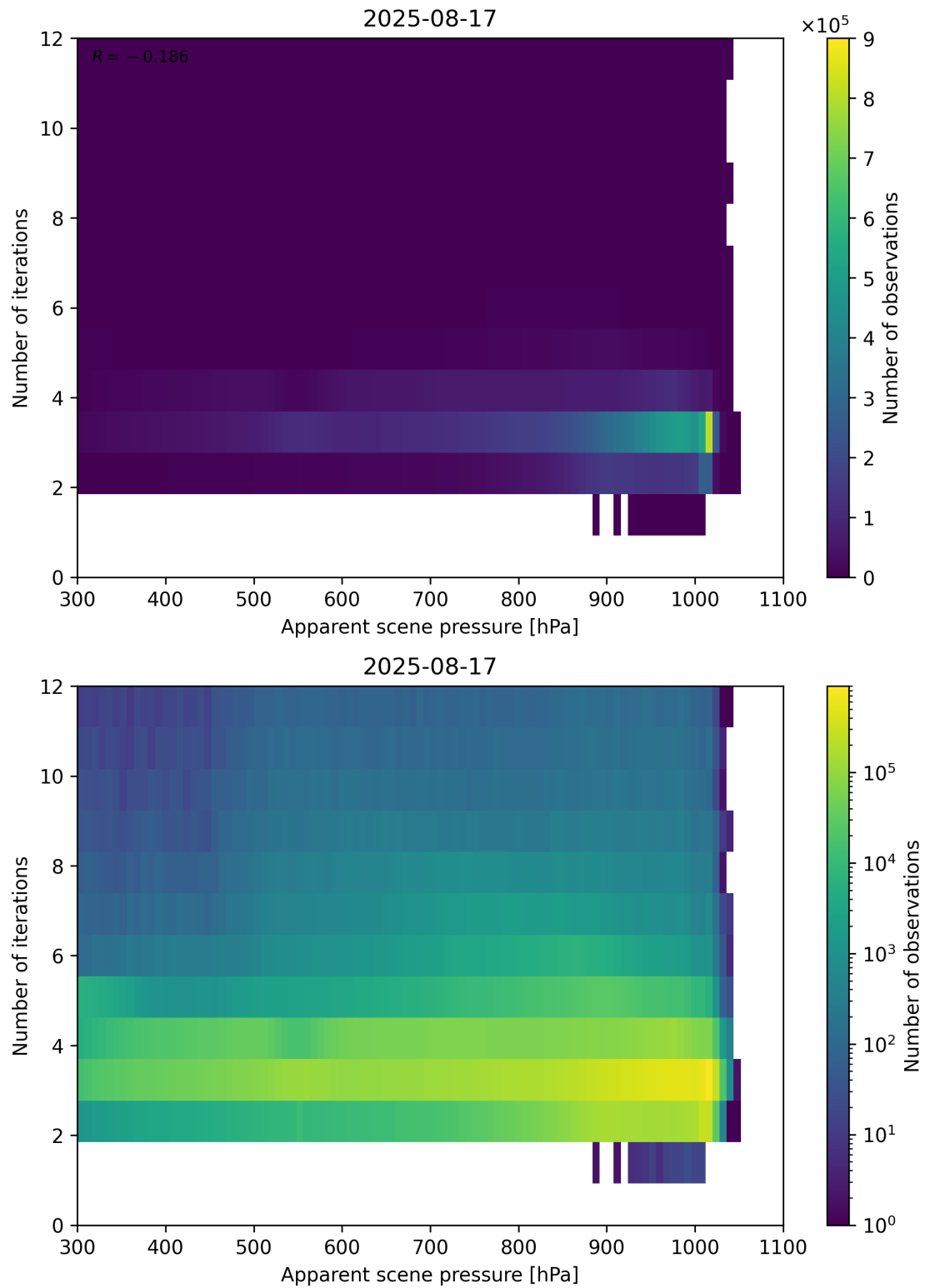
Figure 65: Scatter density plot of “Apparent scene pressure” against “Number of iterations” for 2025-08-16 to 2025-08-18.
