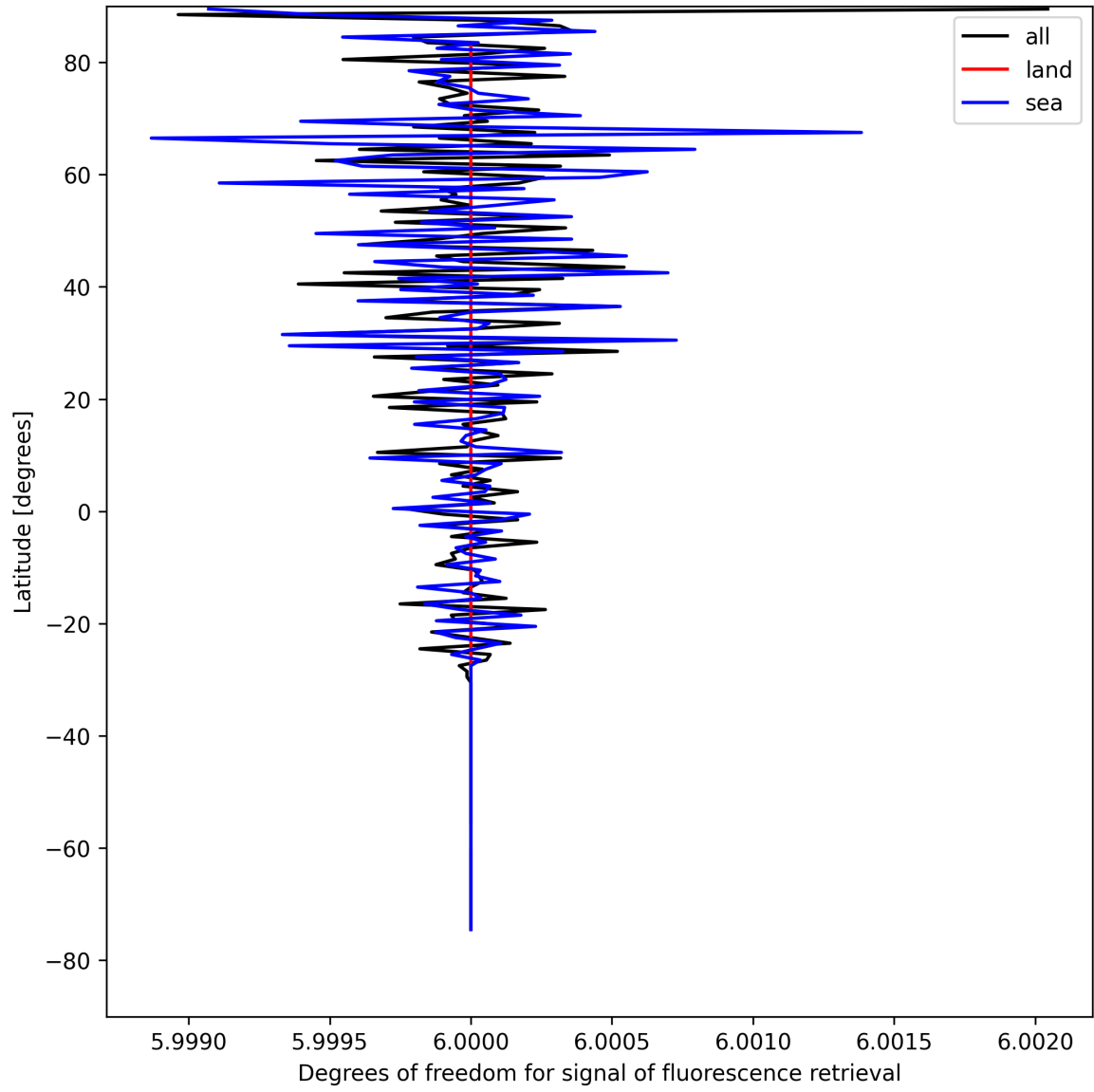
Figure 26: Zonal average of “Degrees of freedom for signal of fluorescence retrieval” for 2025-08-16 to 2025-08-18.
