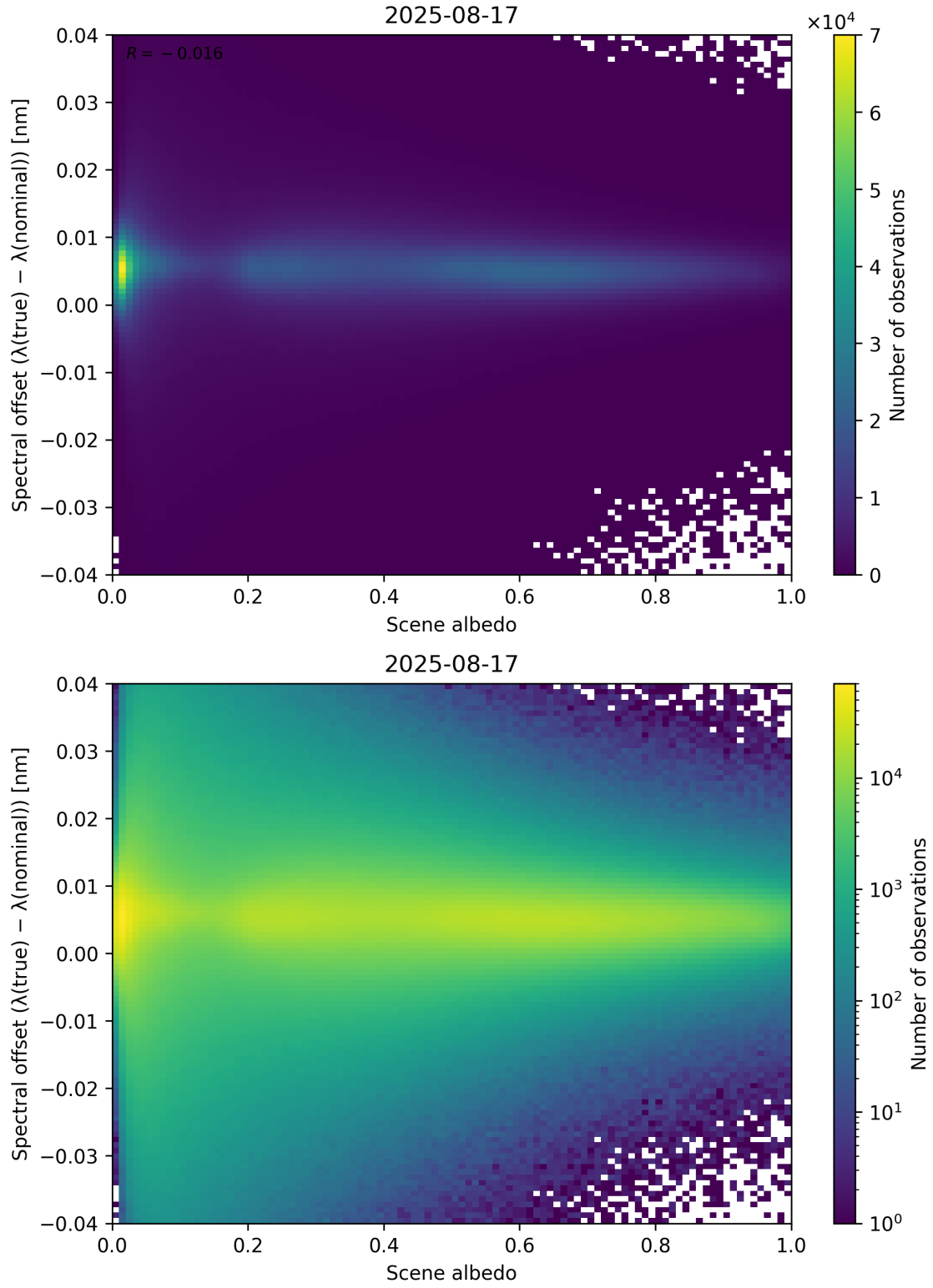
Figure 107: Scatter density plot of “Scene albedo” against “Spectral offset ( \lambda_{\text{true}} - \lambda_{\text{nominal}} )” for 2025-08-16 to 2025-08-18.
