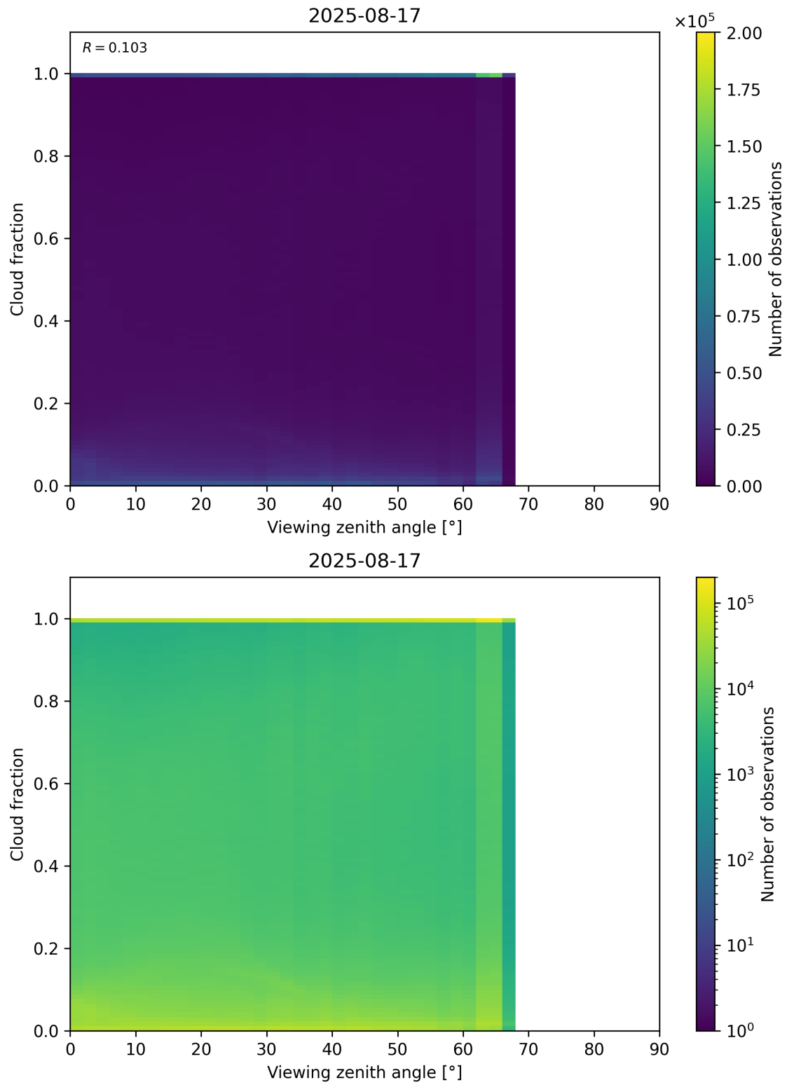
Figure 120: Scatter density plot of “Viewing zenith angle” against “Cloud fraction” for 2025-08-16 to 2025-08-18.
