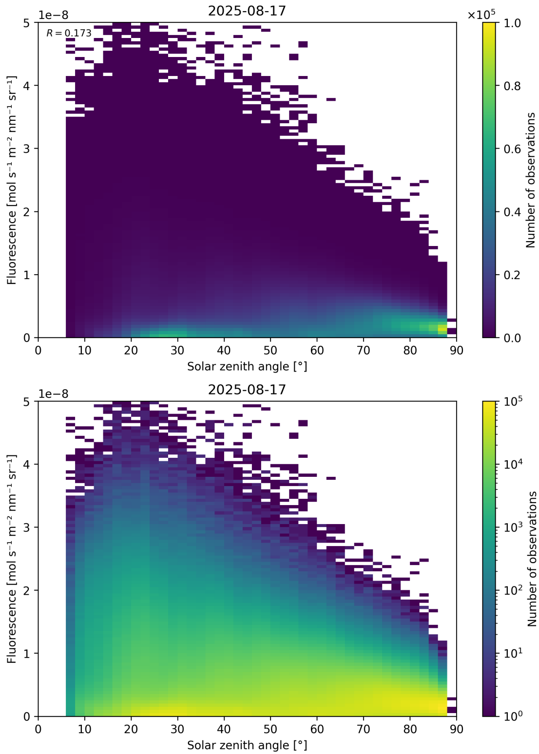
Figure 112: Scatter density plot of “Solar zenith angle” against “Fluorescence” for 2025-08-16 to 2025-08-18.
