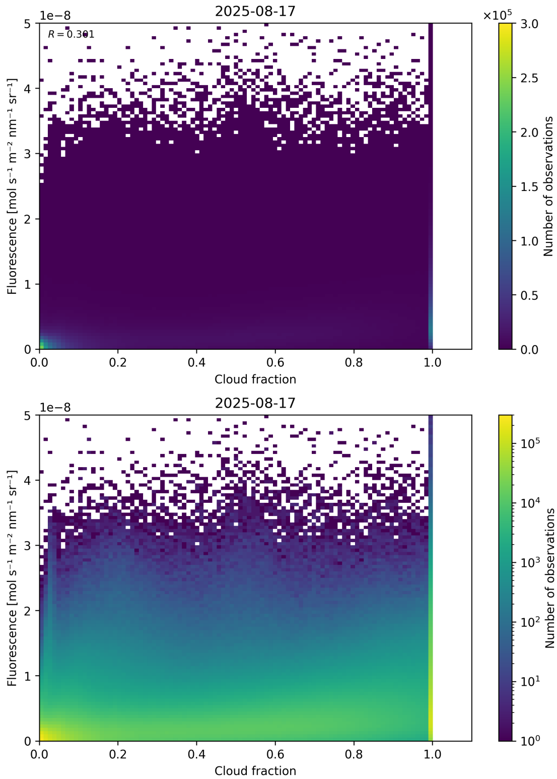
Figure 72: Scatter density plot of “Cloud fraction” against “Fluorescence” for 2025-08-16 to 2025-08-18.
