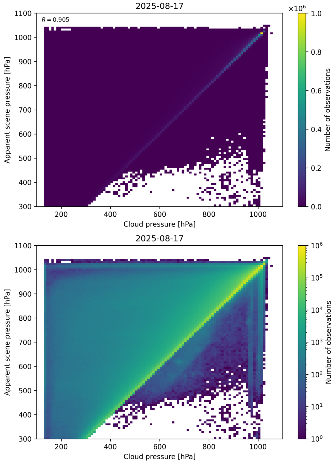
Figure 77: Scatter density plot of “Cloud pressure” against “Apparent scene pressure” for 2025-08-16 to 2025-08-18.
