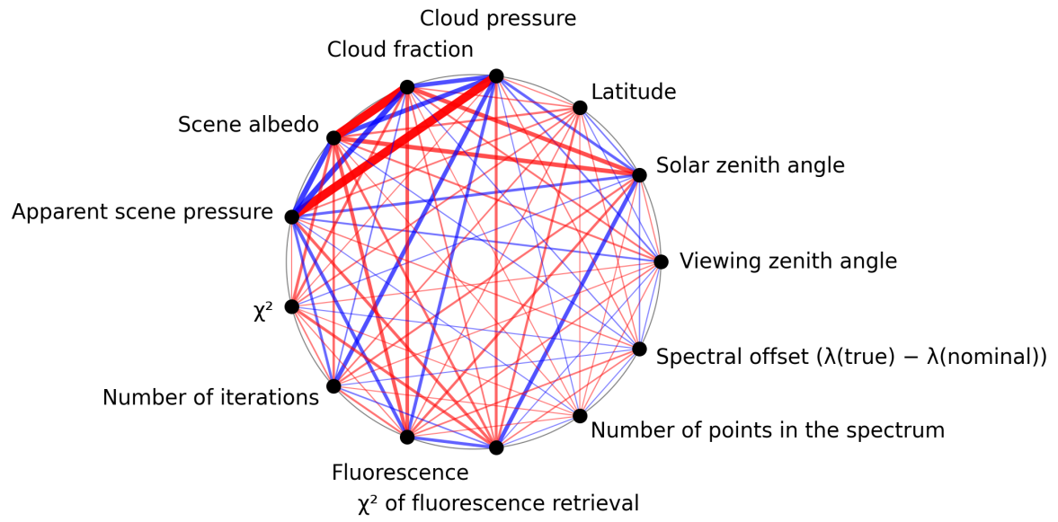
Figure 1: Map of correlation graph for 2025-08-16 to 2025-08-18.
