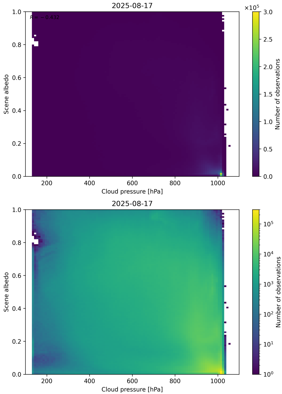
Figure 83: Scatter density plot of “Cloud pressure” against “Scene albedo” for 2025-08-16 to 2025-08-18.
