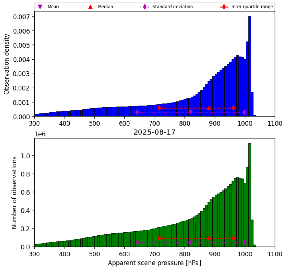
Figure 36: Histogram of “Apparent scene pressure” for 2025-08-16 to 2025-08-18
