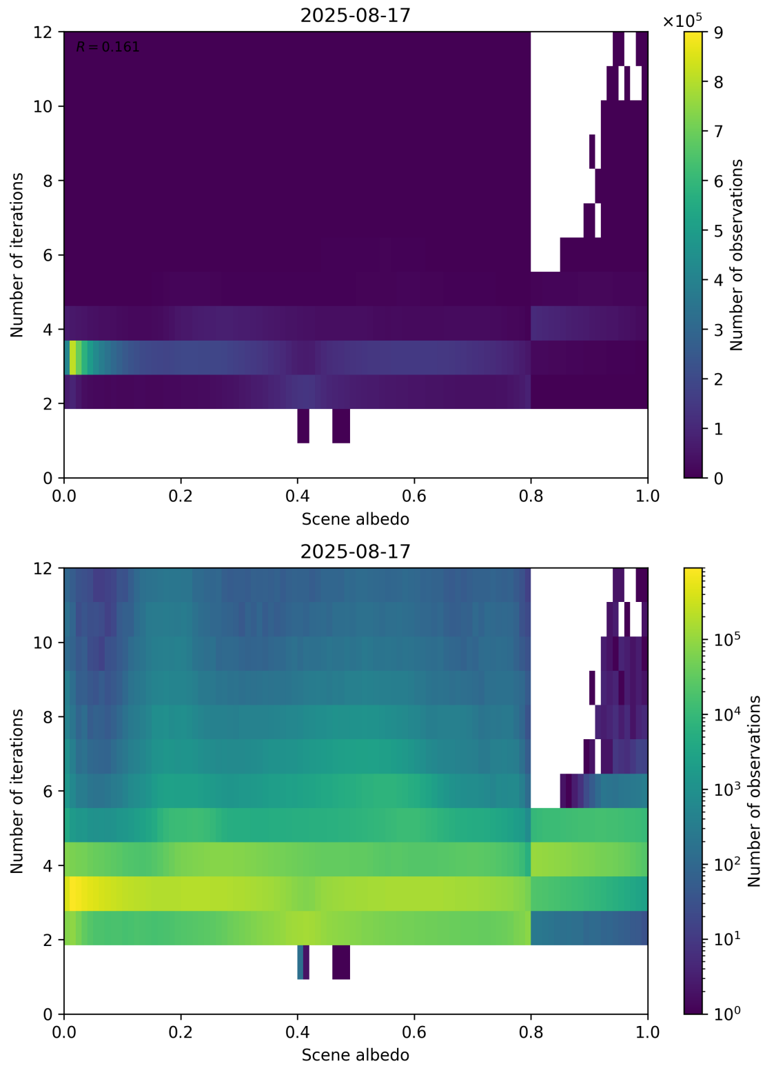
Figure 105: Scatter density plot of “Scene albedo” against “Number of iterations” for 2025-08-16 to 2025-08-18.
