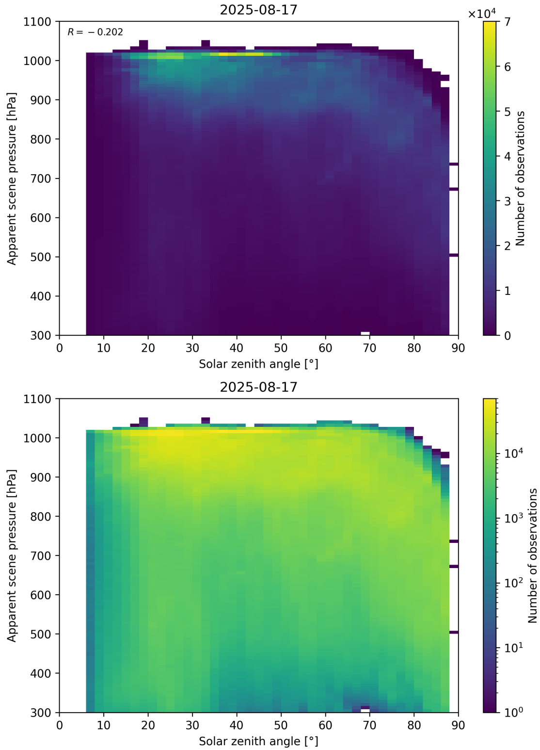
Figure 108: Scatter density plot of “Solar zenith angle” against “Apparent scene pressure” for 2025-08-16 to 2025-08-18.
