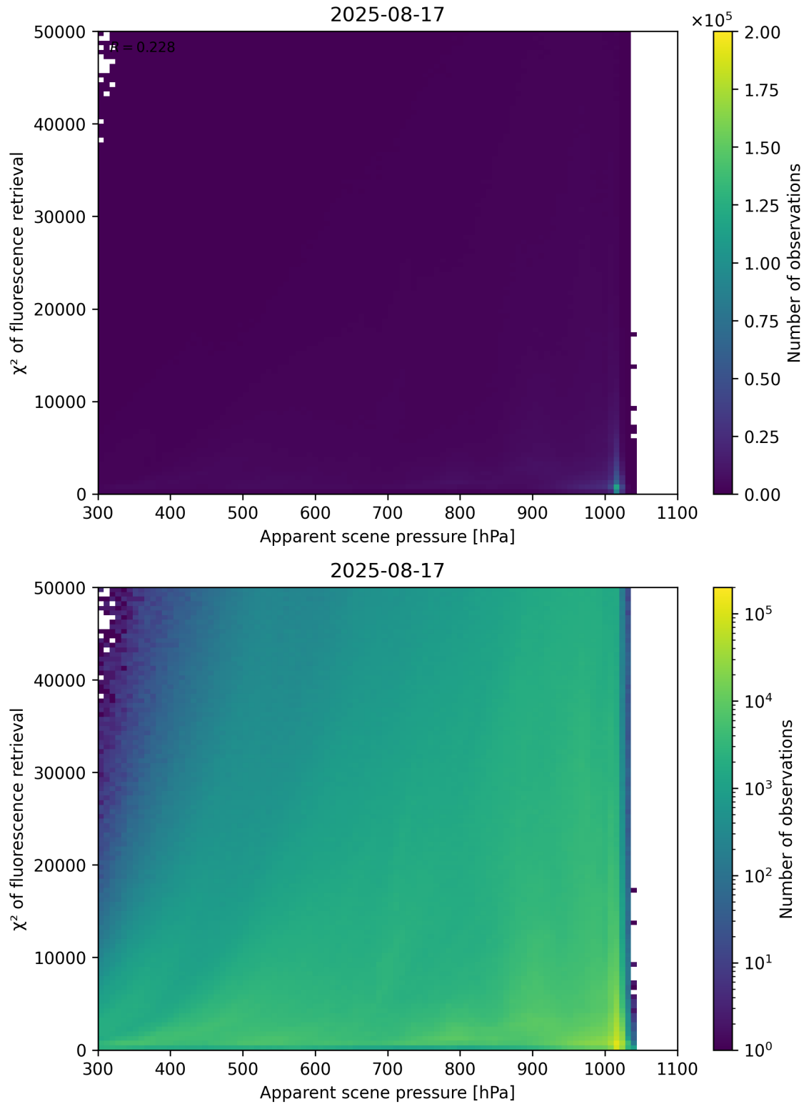
Figure 63: Scatter density plot of “Apparent scene pressure” against “ \chi^2 of fluorescence retrieval” for 2025-08-16 to 2025-08-18.
