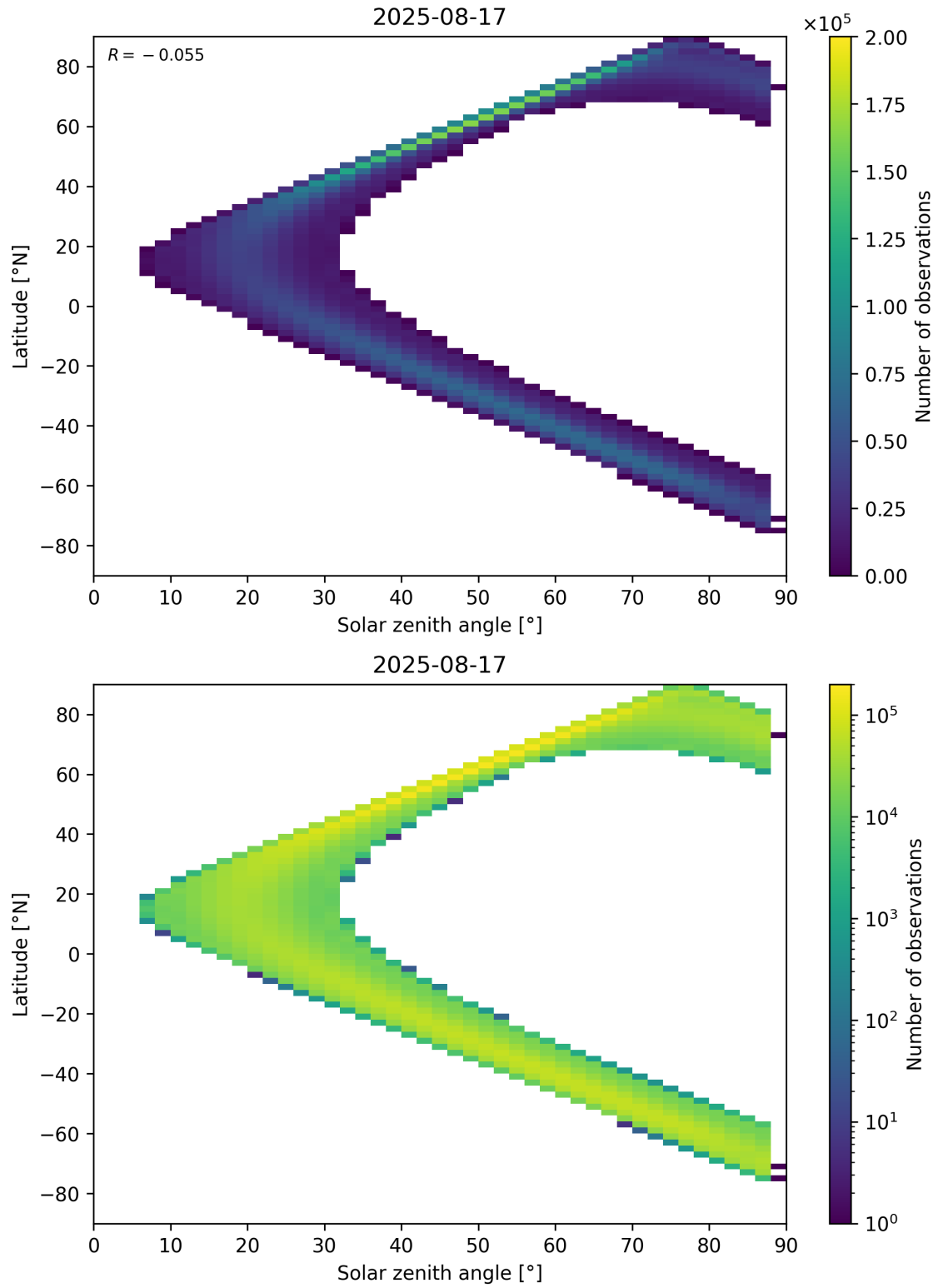
Figure 113: Scatter density plot of “Solar zenith angle” against “Latitude” for 2025-08-16 to 2025-08-18.
