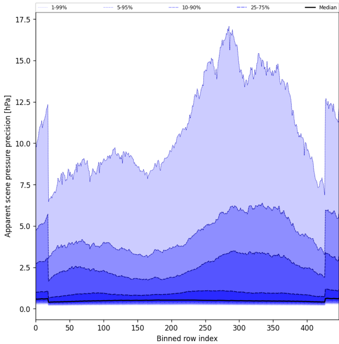
Figure 54: Along track statistics of “Apparent scene pressure precision” for 2025-08-16 to 2025-08-18
