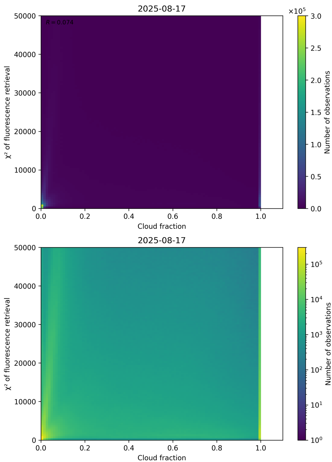
Figure 71: Scatter density plot of “Cloud fraction” against “ \chi^2 of fluorescence retrieval” for 2025-08-16 to 2025-08-18.
