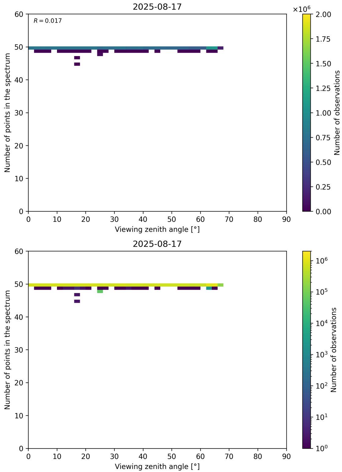
Figure 125: Scatter density plot of “Viewing zenith angle” against “Number of points in the spectrum” for 2025-08-16 to 2025-08-18.
