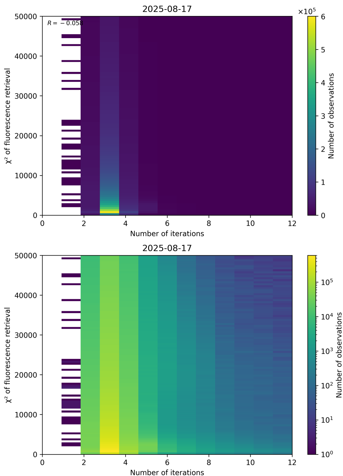
Figure 97: Scatter density plot of “Number of iterations” against “ \chi^2 of fluorescence retrieval” for 2025-08-16 to 2025-08-18.
