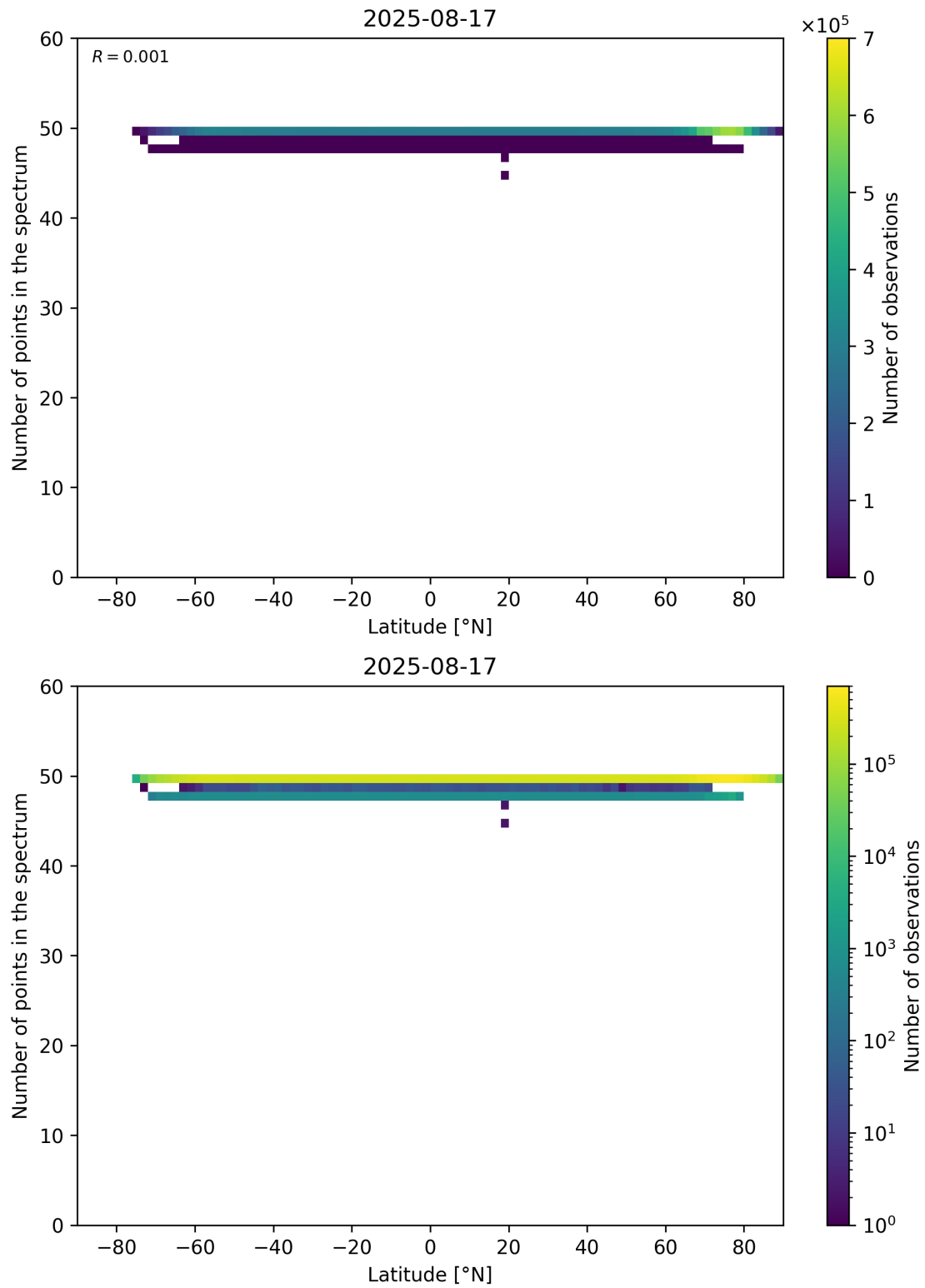
Figure 94: Scatter density plot of “Latitude” against “Number of points in the spectrum” for 2025-08-16 to 2025-08-18.
