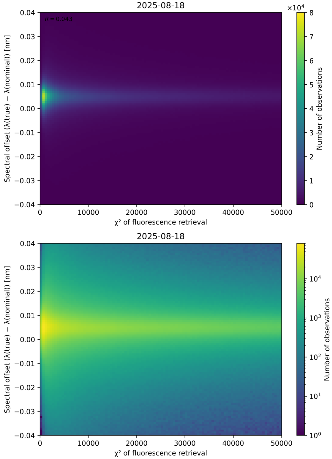
Figure 69: Scatter density plot of “ \chi^2 of fluorescence retrieval” against “Spectral offset ( \lambda_{\text{true}} - \lambda_{\text{nominal}} )” for 2025-08-17 to 2025-08-19.
