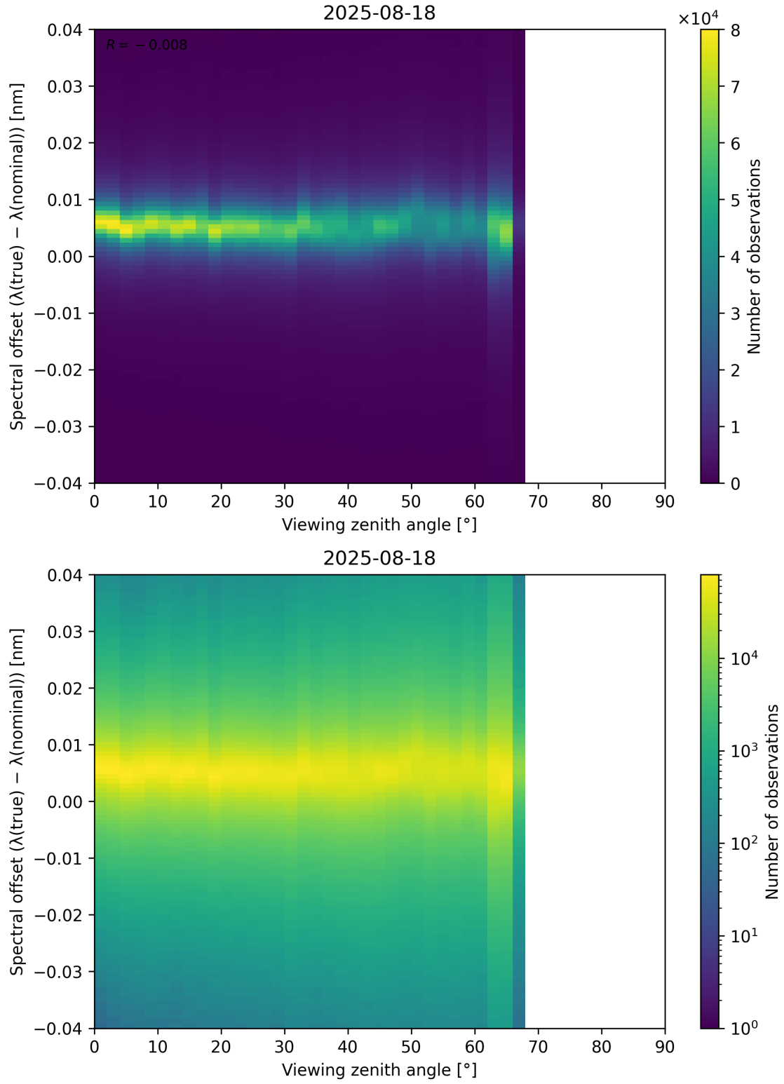
Figure 128: Scatter density plot of “Viewing zenith angle” against “Spectral offset ( \lambda_{\text{true}} - \lambda_{\text{nominal}} )” for 2025-08-17 to 2025-08-19.
