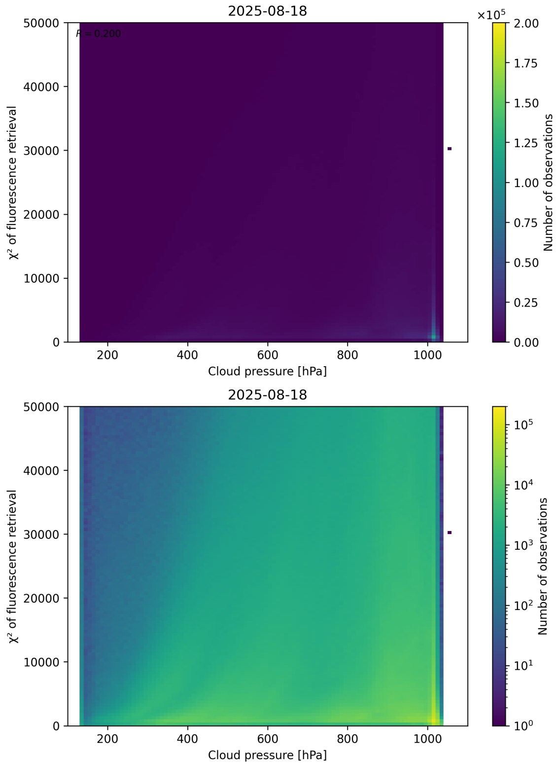
Figure 78: Scatter density plot of “Cloud pressure” against “ \chi^2 of fluorescence retrieval” for 2025-08-17 to 2025-08-19.
