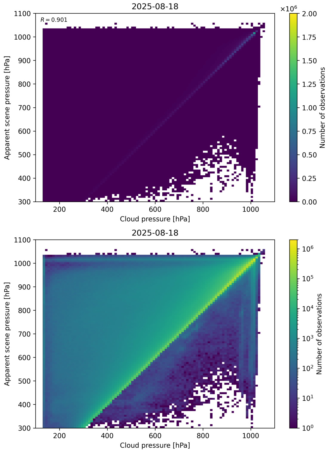
Figure 77: Scatter density plot of “Cloud pressure” against “Apparent scene pressure” for 2025-08-17 to 2025-08-19.
