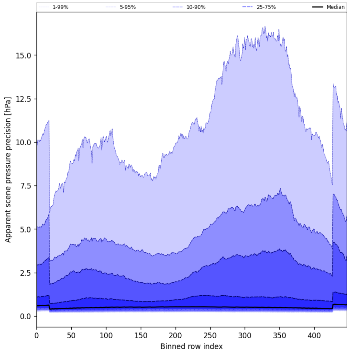
Figure 54: Along track statistics of “Apparent scene pressure precision” for 2025-08-17 to 2025-08-19
