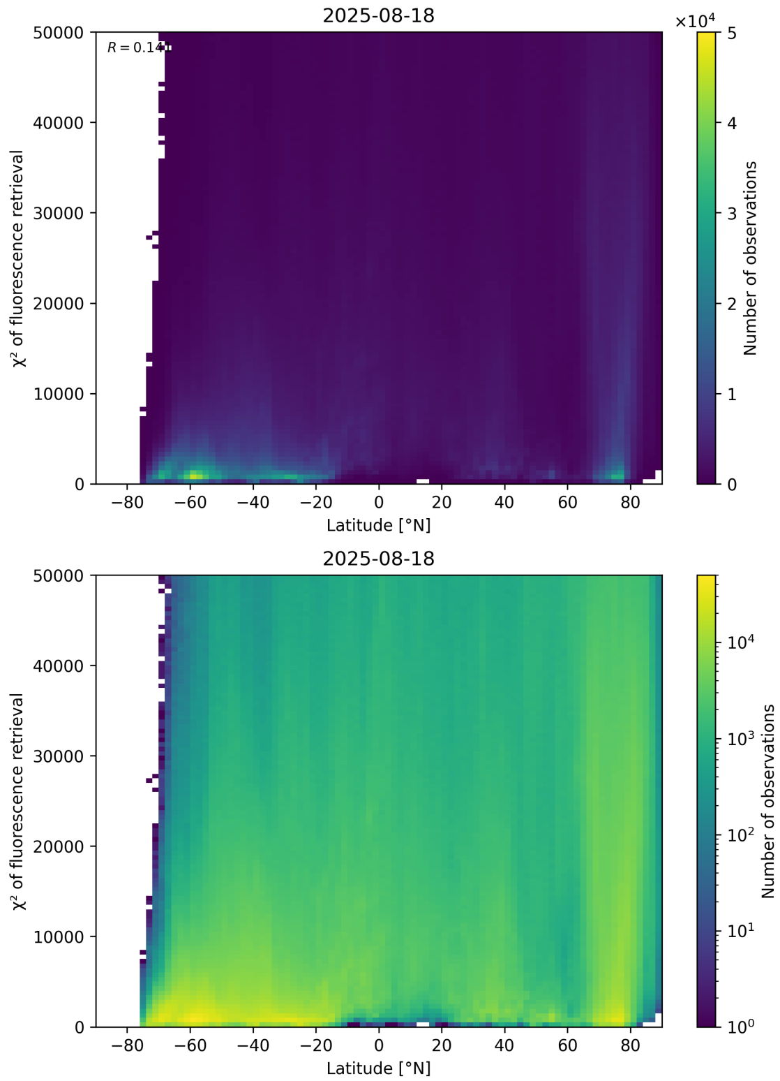
Figure 89: Scatter density plot of “Latitude” against “ \chi^2 of fluorescence retrieval” for 2025-08-17 to 2025-08-19.
