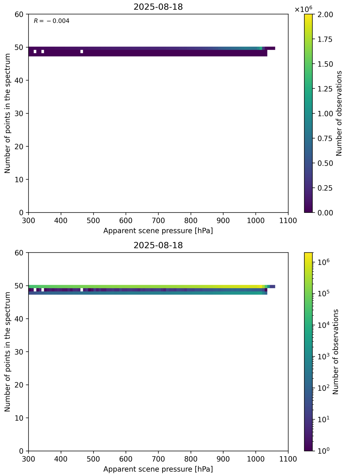
Figure 66: Scatter density plot of “Apparent scene pressure” against “Number of points in the spectrum” for 2025-08-17 to 2025-08-19.
