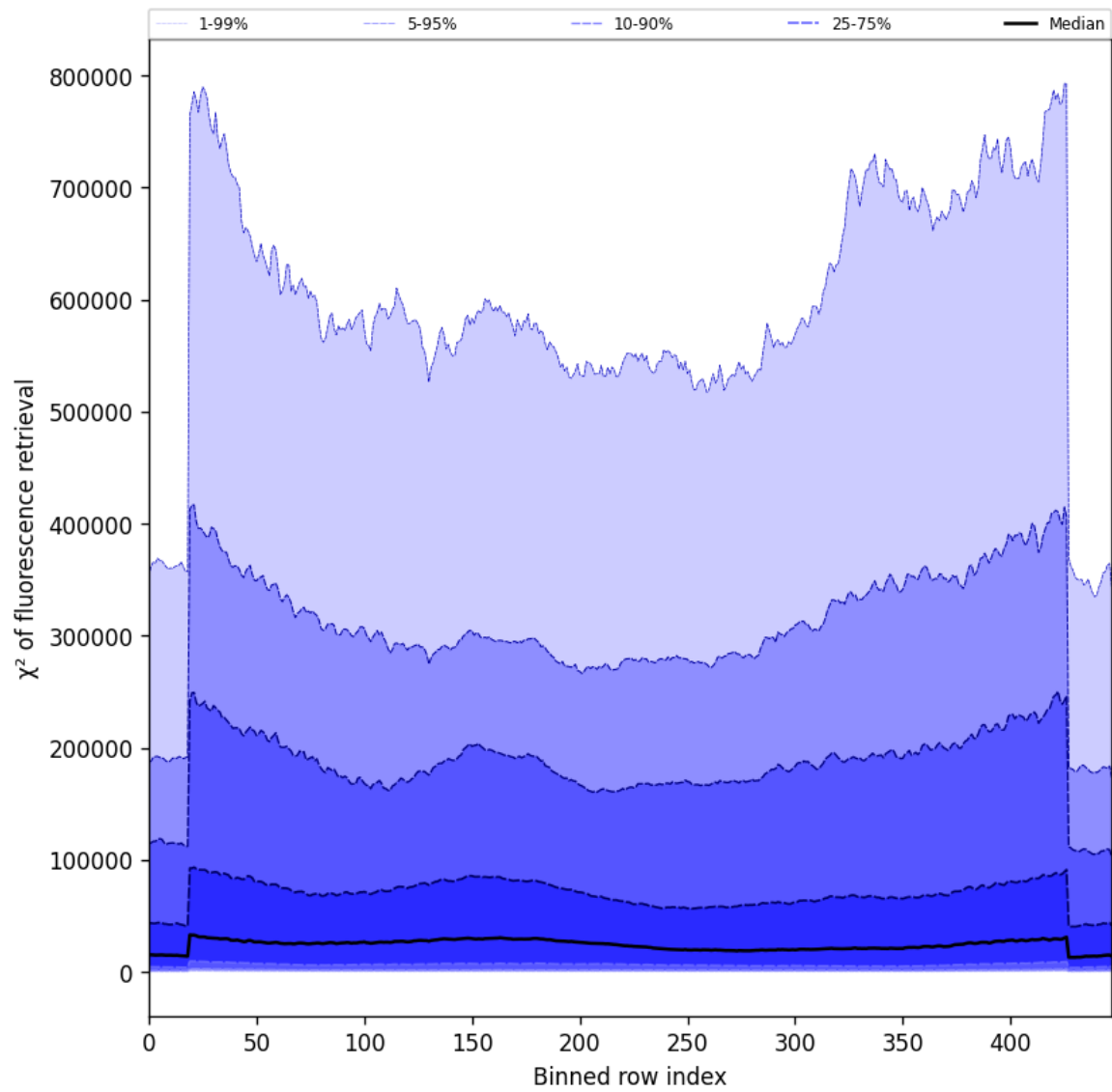
Figure 59: Along track statistics of “ \chi^2 of fluorescence retrieval” for 2025-08-17 to 2025-08-19
