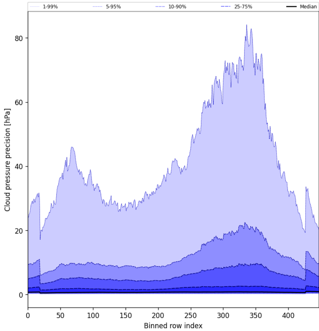
Figure 48: Along track statistics of “Cloud pressure precision” for 2025-08-17 to 2025-08-19
