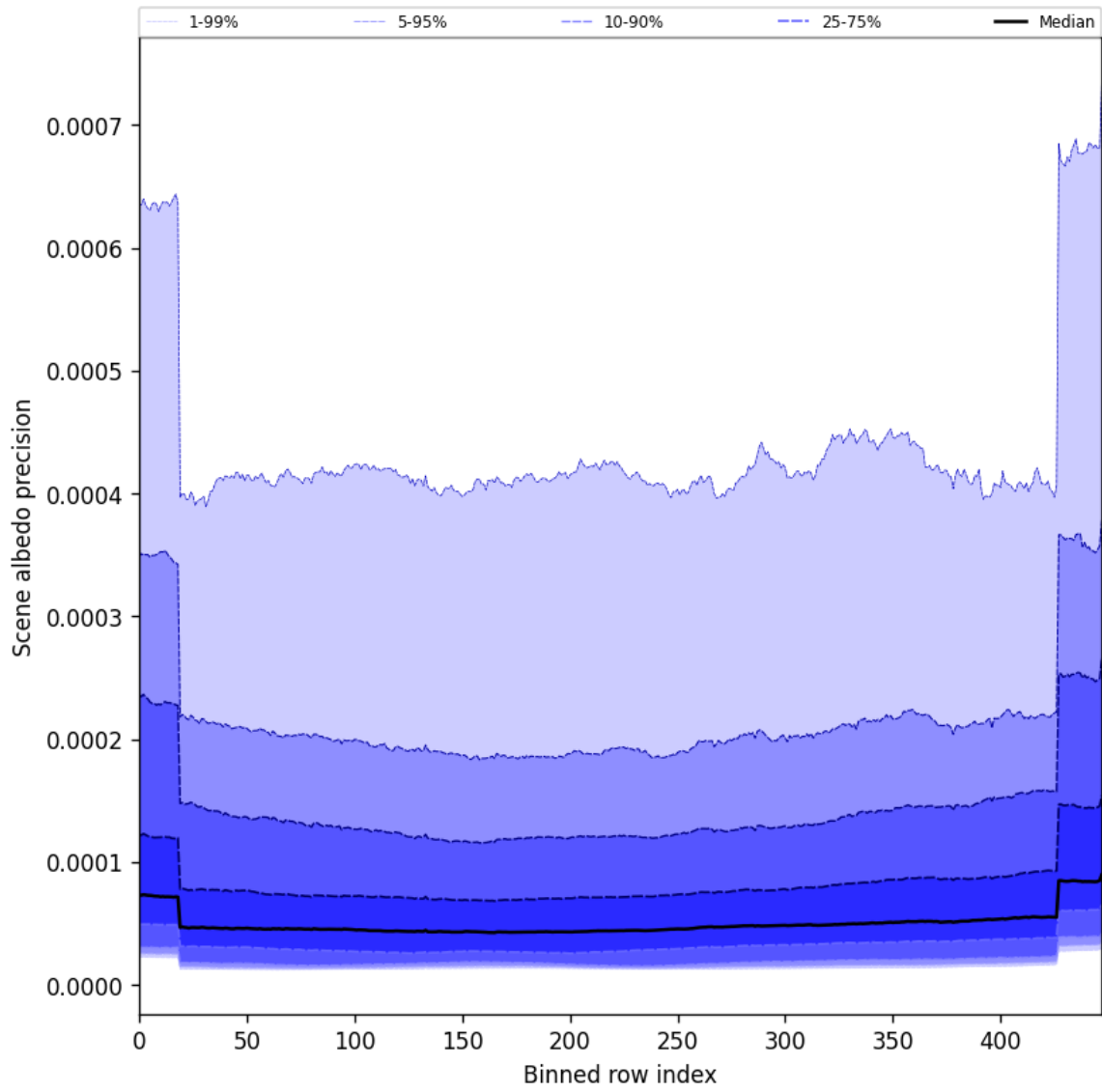
Figure 52: Along track statistics of “Scene albedo precision” for 2025-08-17 to 2025-08-19
