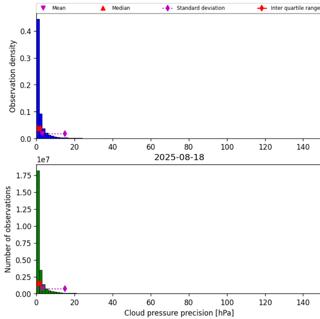
Figure 31: Histogram of “Cloud pressure precision” for 2025-08-17 to 2025-08-19
