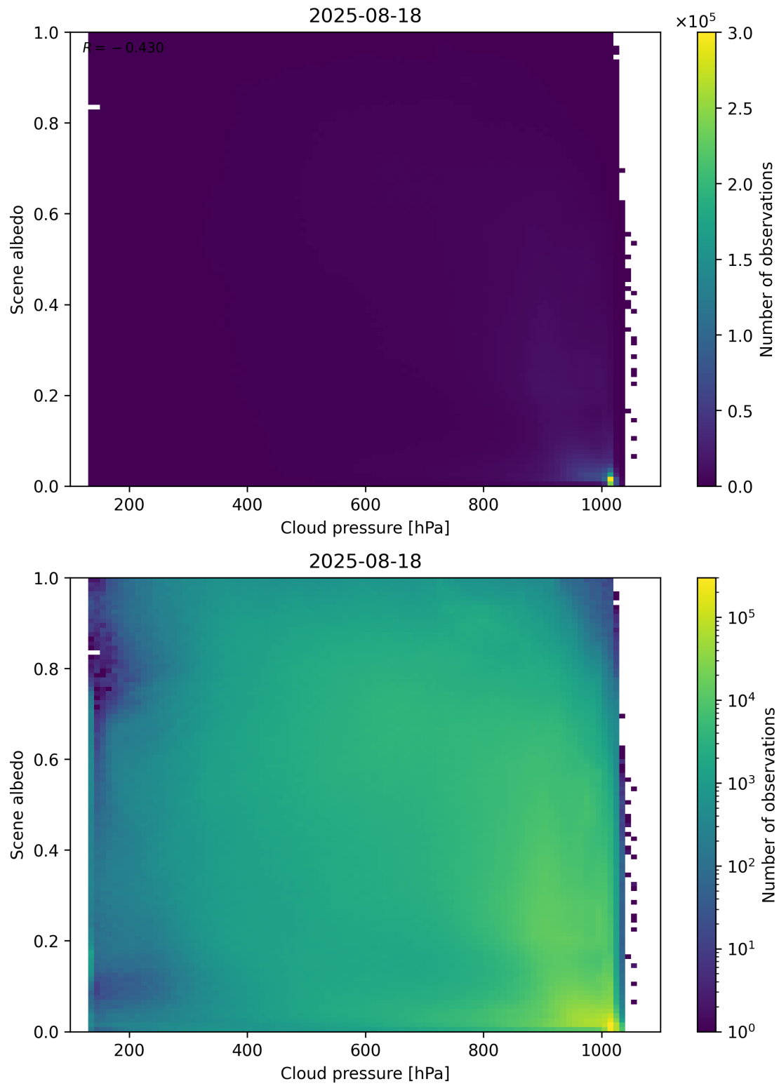
Figure 83: Scatter density plot of “Cloud pressure” against “Scene albedo” for 2025-08-17 to 2025-08-19.
