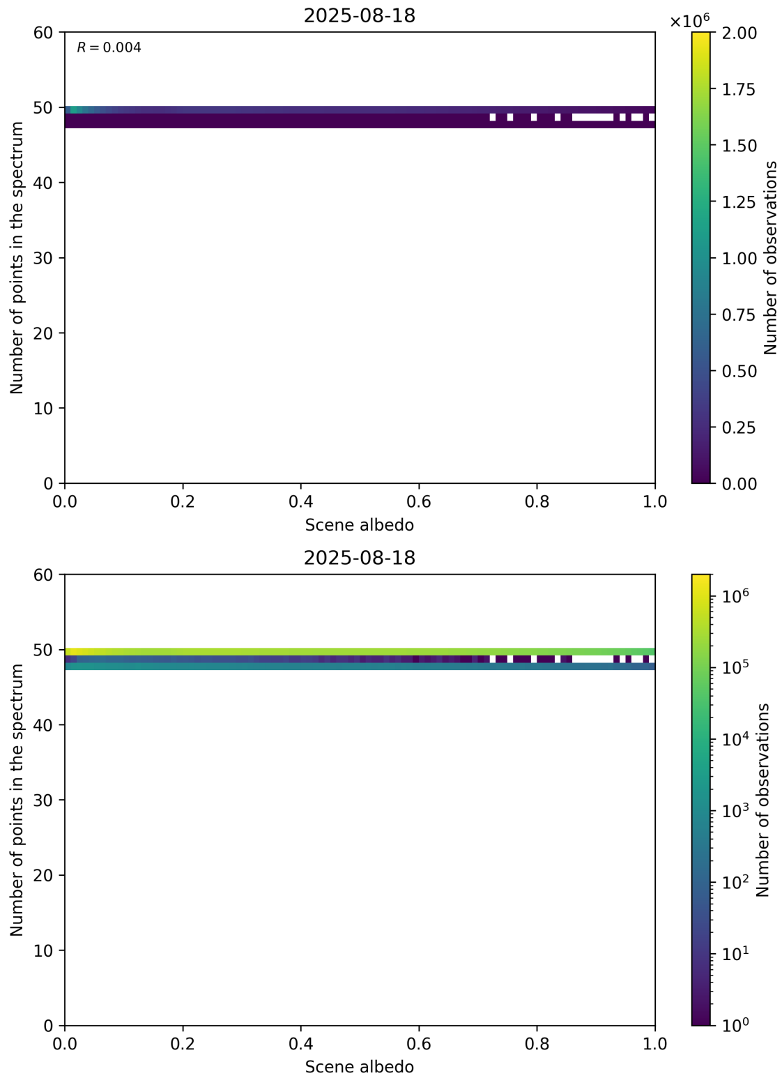
Figure 106: Scatter density plot of “Scene albedo” against “Number of points in the spectrum” for 2025-08-17 to 2025-08-19.
