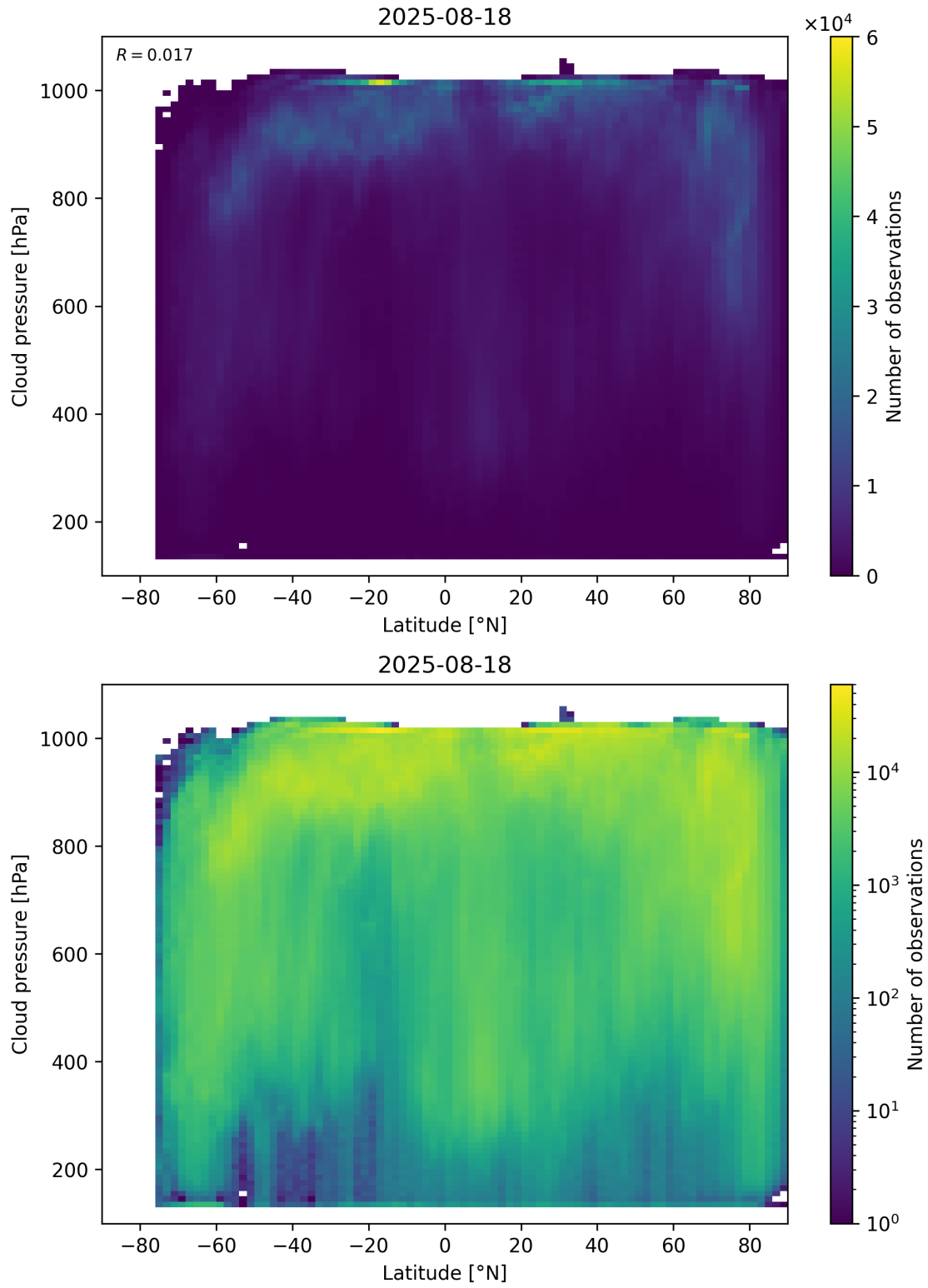
Figure 91: Scatter density plot of “Latitude” against “Cloud pressure” for 2025-08-17 to 2025-08-19.
