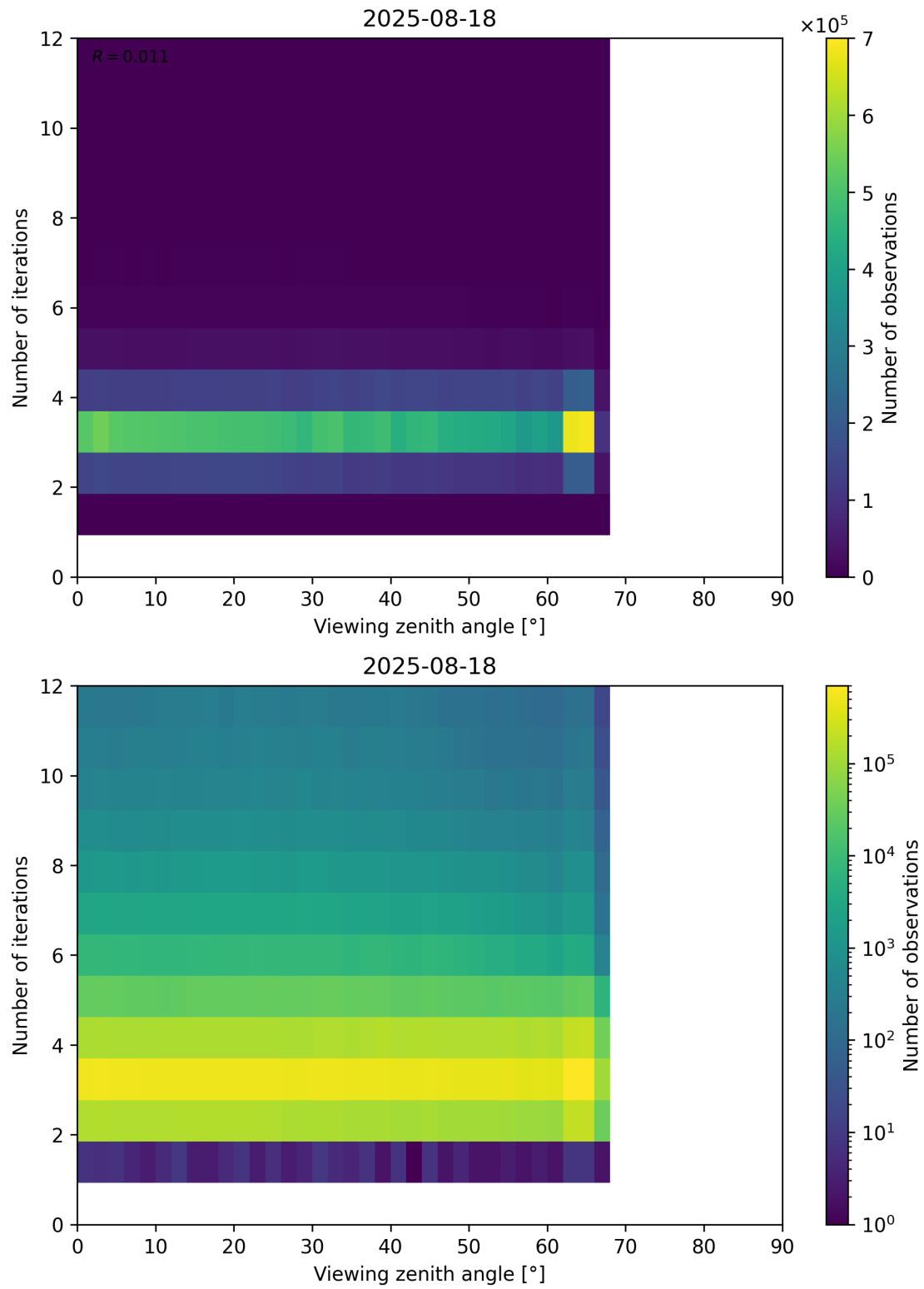
Figure 124: Scatter density plot of “Viewing zenith angle” against “Number of iterations” for 2025-08-17 to 2025-08-19.
