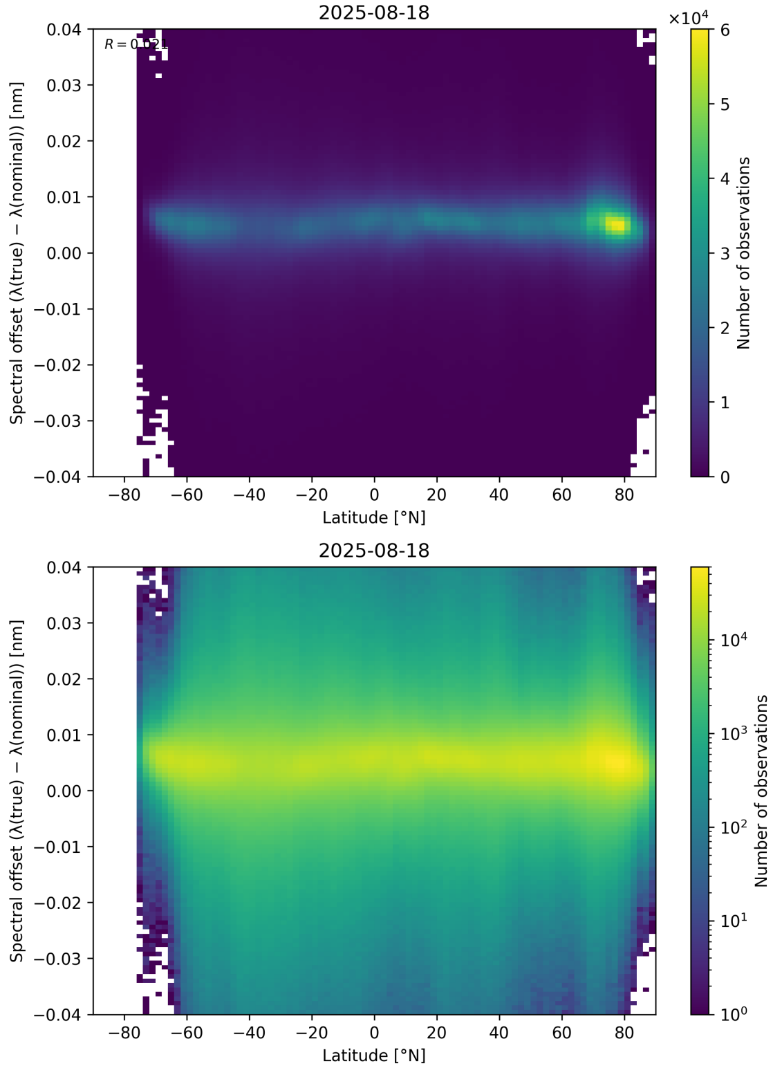
Figure 96: Scatter density plot of “Latitude” against “Spectral offset ( \lambda_{\text{true}} - \lambda_{\text{nominal}} )” for 2025-08-17 to 2025-08-19.
