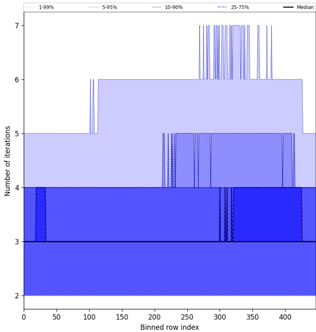
Figure 56: Along track statistics of “Number of iterations” for 2025-08-17 to 2025-08-19
