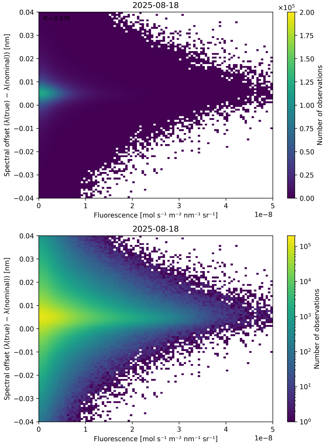
Figure 87: Scatter density plot of “Fluorescence” against “Spectral offset ( \lambda_{\text{true}} - \lambda_{\text{nominal}} )” for 2025-08-17 to 2025-08-19.
