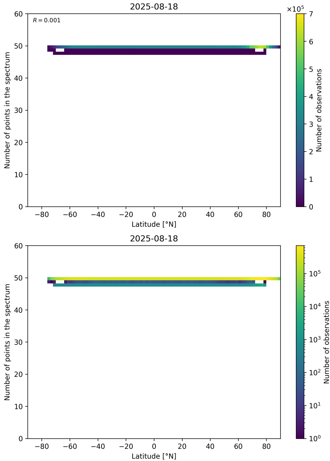
Figure 94: Scatter density plot of “Latitude” against “Number of points in the spectrum” for 2025-08-17 to 2025-08-19.
