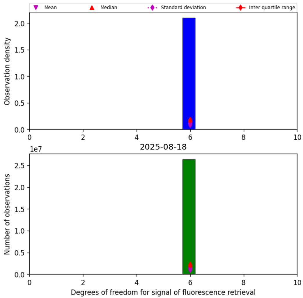
Figure 43: Histogram of "Degrees of freedom for signal of fluorescence retrieval" for 2025-08-17 to 2025-08-19
