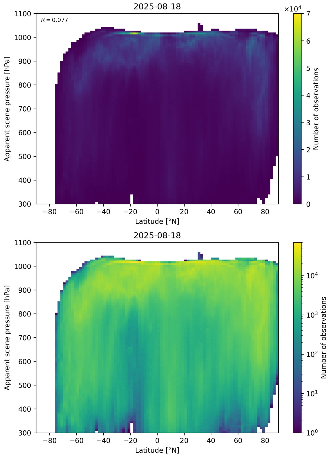
Figure 88: Scatter density plot of “Latitude” against “Apparent scene pressure” for 2025-08-17 to 2025-08-19.
