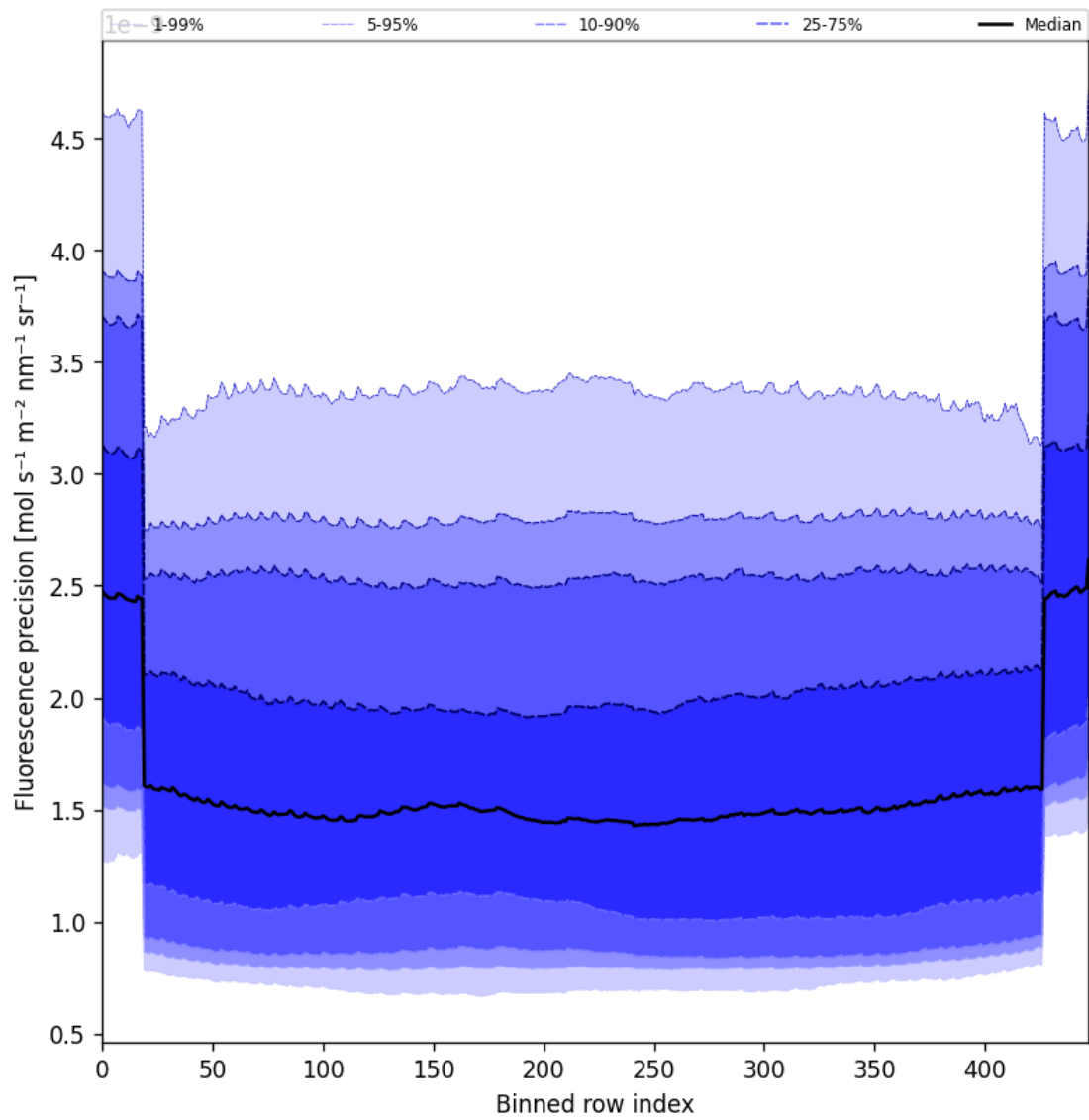
Figure 58: Along track statistics of “Fluorescence precision” for 2025-08-17 to 2025-08-19
