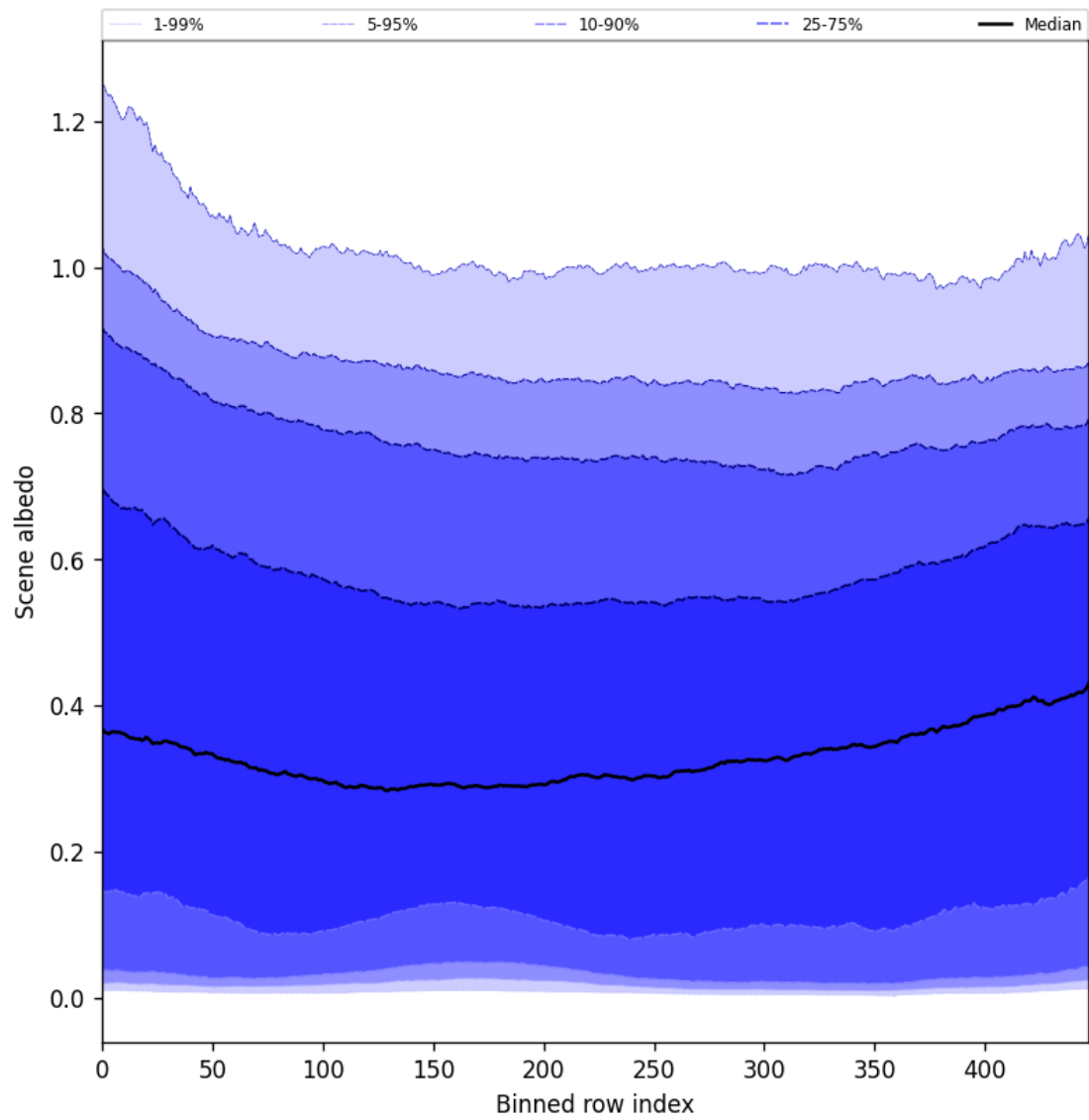
Figure 51: Along track statistics of “Scene albedo” for 2025-08-17 to 2025-08-19
