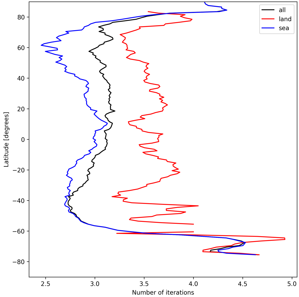
Figure 22: Zonal average of “Number of iterations” for 2025-08-17 to 2025-08-19.
