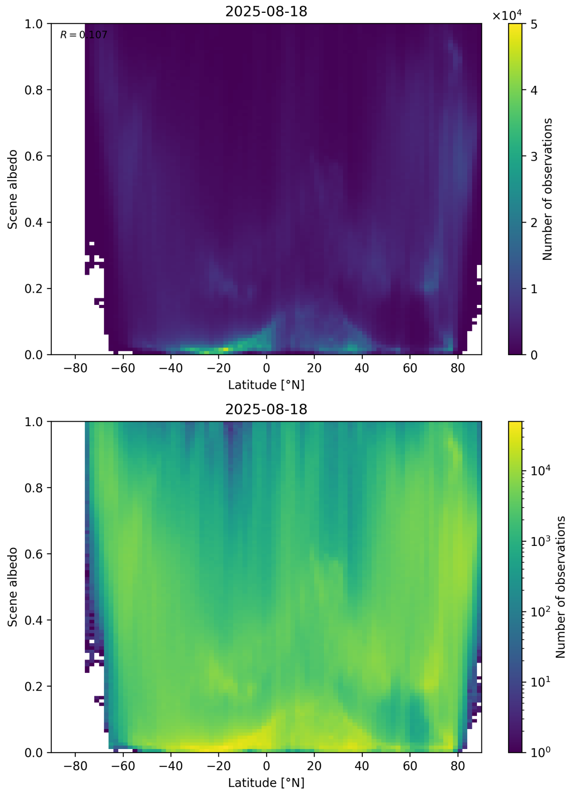
Figure 95: Scatter density plot of “Latitude” against “Scene albedo” for 2025-08-17 to 2025-08-19.
