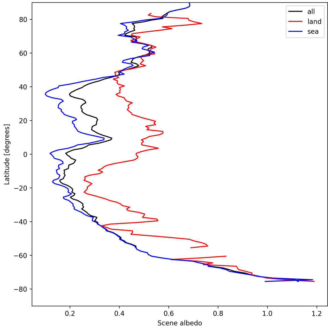
Figure 17: Zonal average of “Scene albedo” for 2025-08-17 to 2025-08-19.
