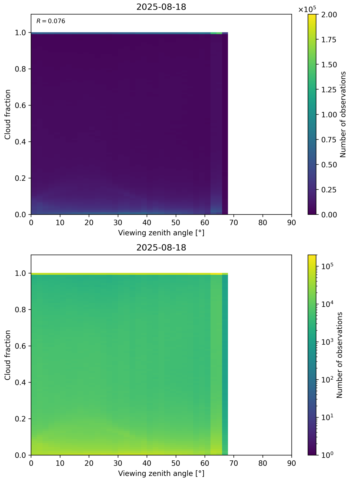
Figure 120: Scatter density plot of “Viewing zenith angle” against “Cloud fraction” for 2025-08-17 to 2025-08-19.
