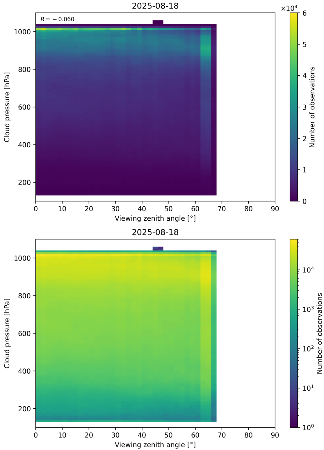
Figure 121: Scatter density plot of “Viewing zenith angle” against “Cloud pressure” for 2025-08-17 to 2025-08-19.
