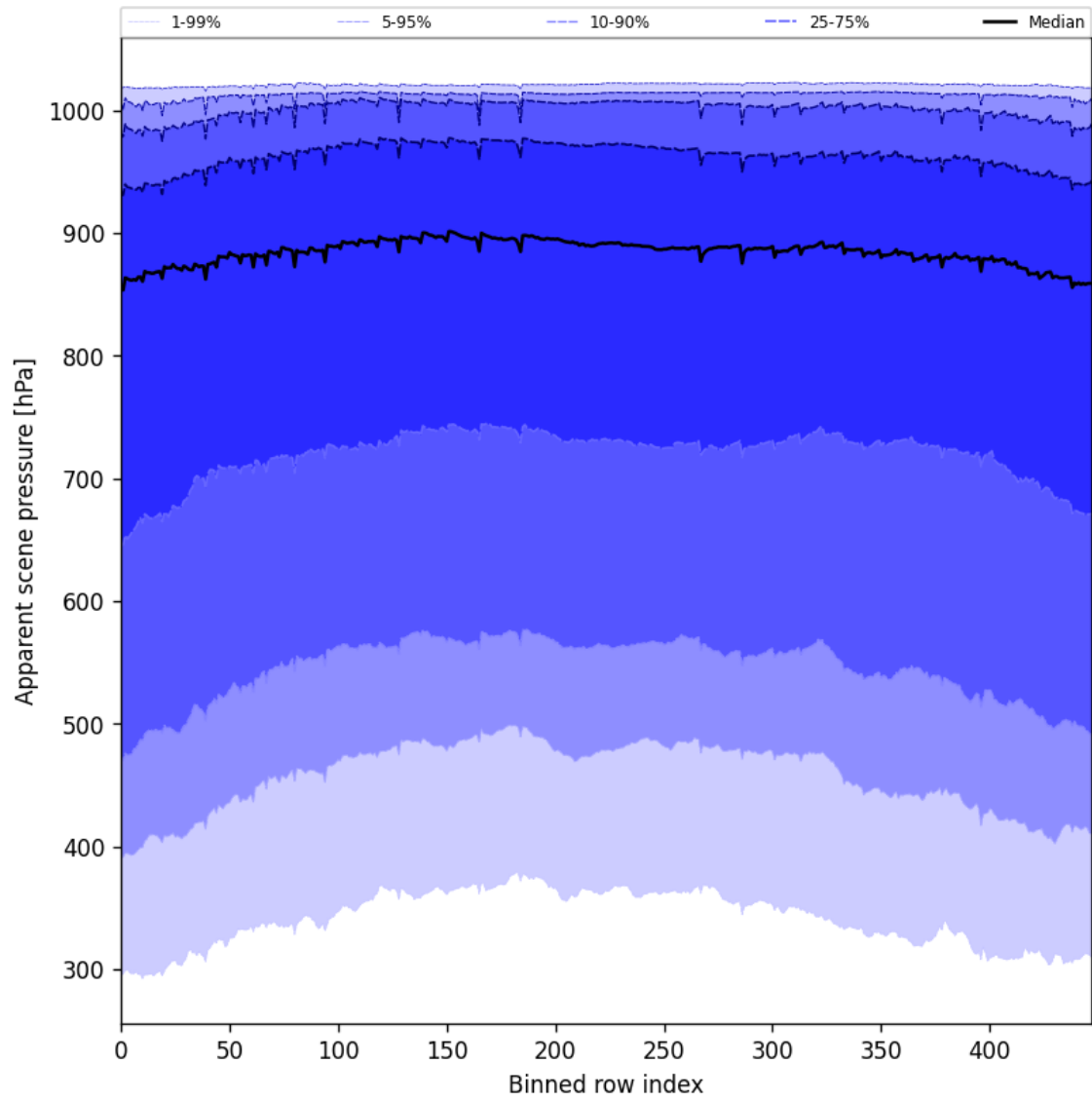
Figure 53: Along track statistics of “Apparent scene pressure” for 2025-08-17 to 2025-08-19
