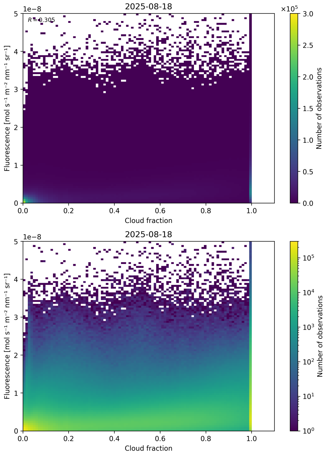
Figure 72: Scatter density plot of “Cloud fraction” against “Fluorescence” for 2025-08-17 to 2025-08-19.
