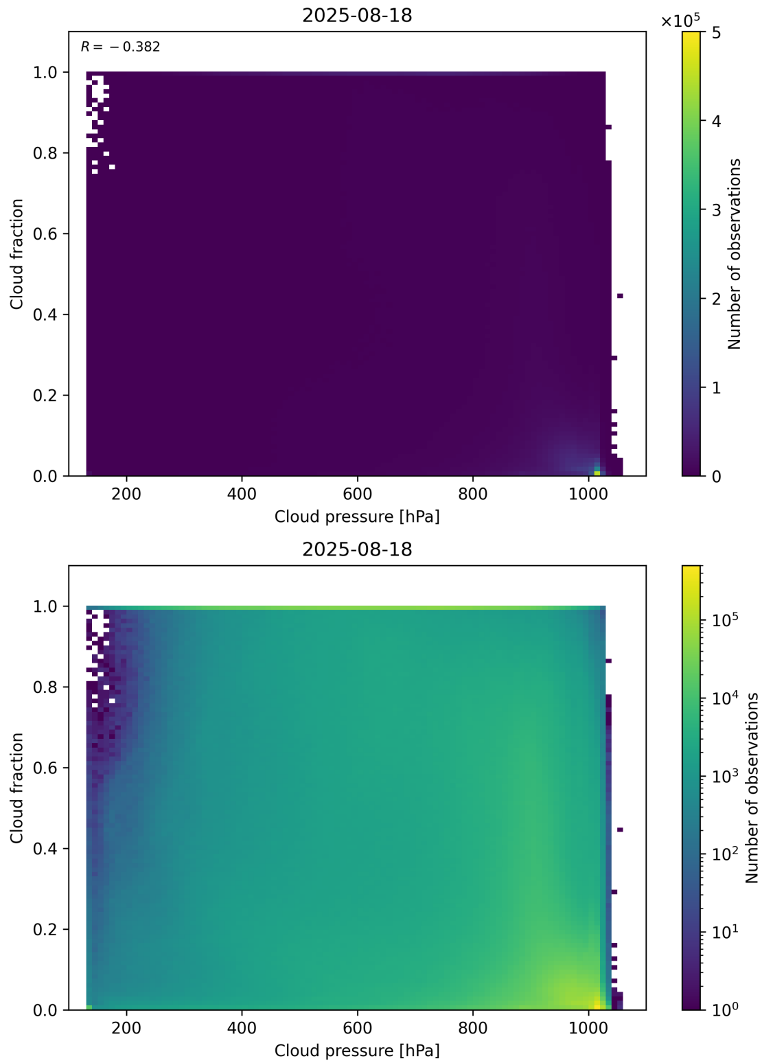
Figure 79: Scatter density plot of “Cloud pressure” against “Cloud fraction” for 2025-08-17 to 2025-08-19.
