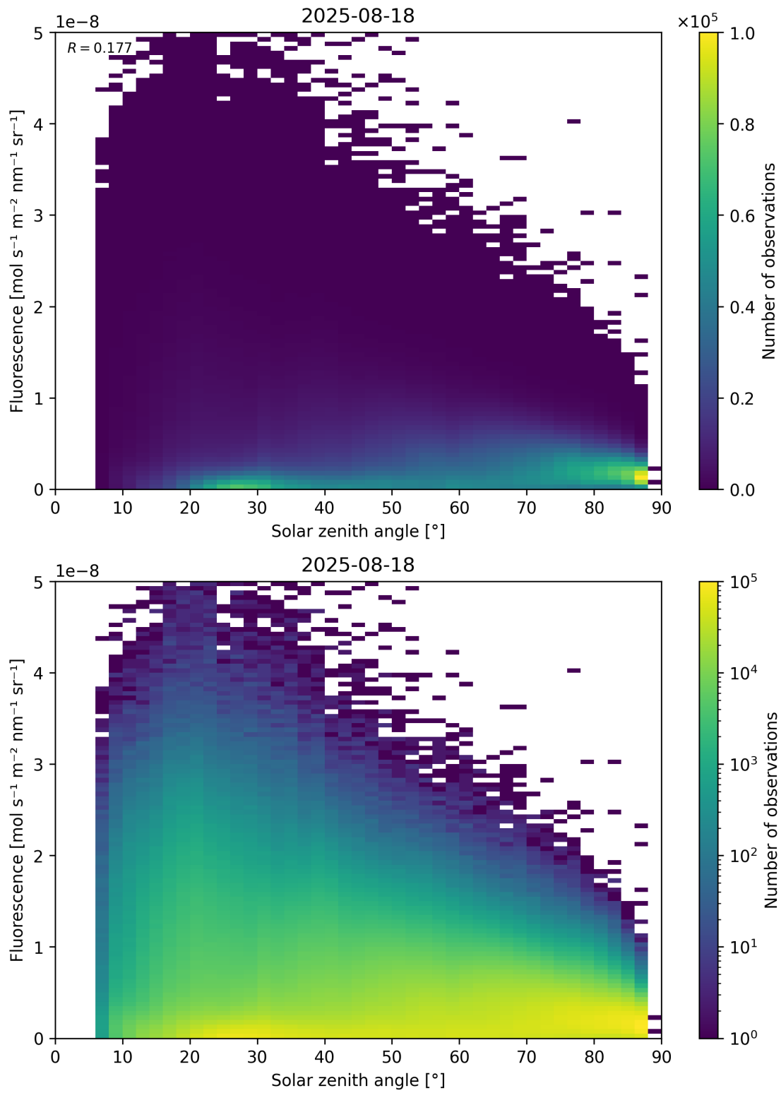
Figure 112: Scatter density plot of “Solar zenith angle” against “Fluorescence” for 2025-08-17 to 2025-08-19.
