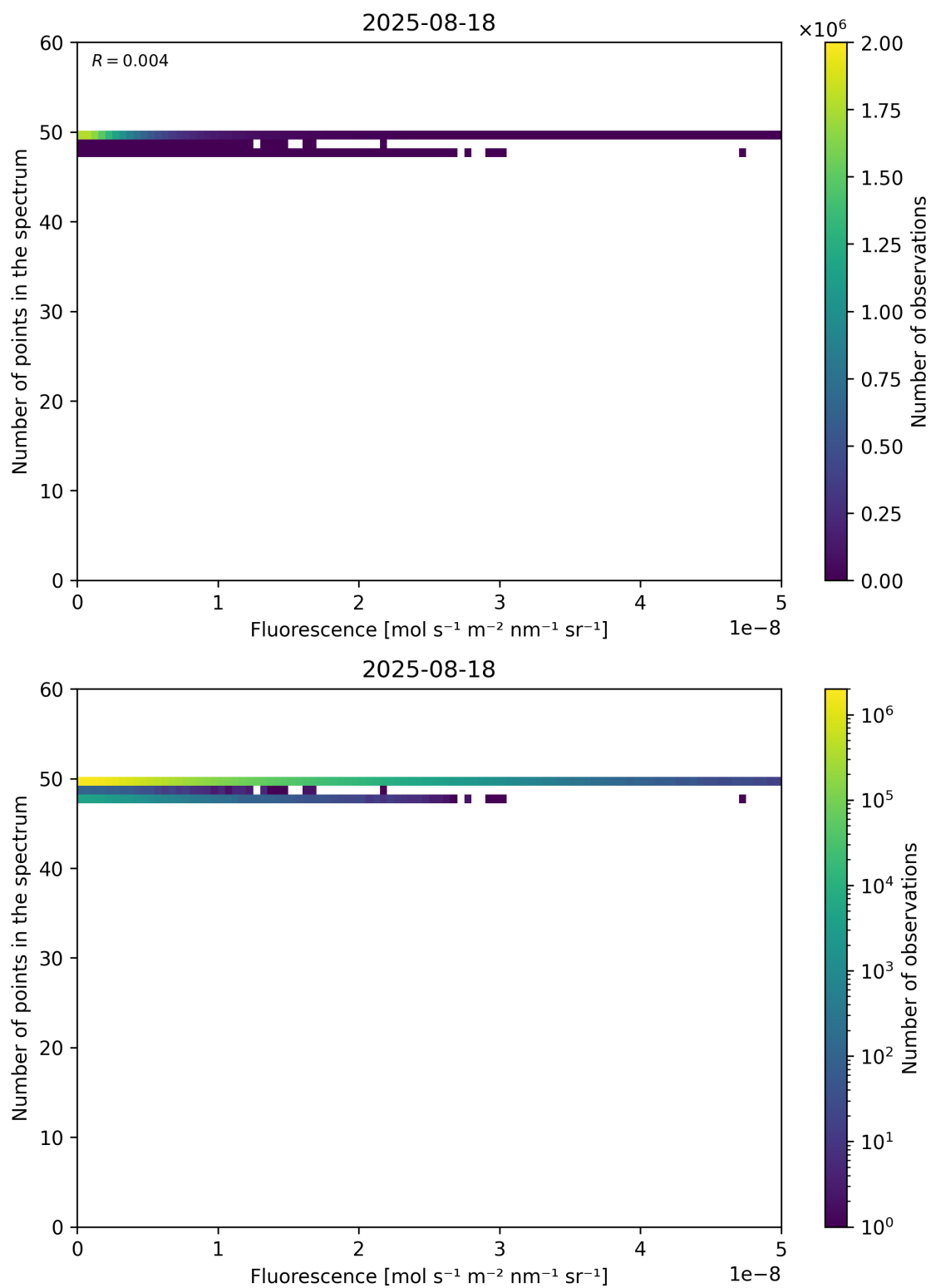
Figure 86: Scatter density plot of “Fluorescence” against “Number of points in the spectrum” for 2025-08-17 to 2025-08-19.
