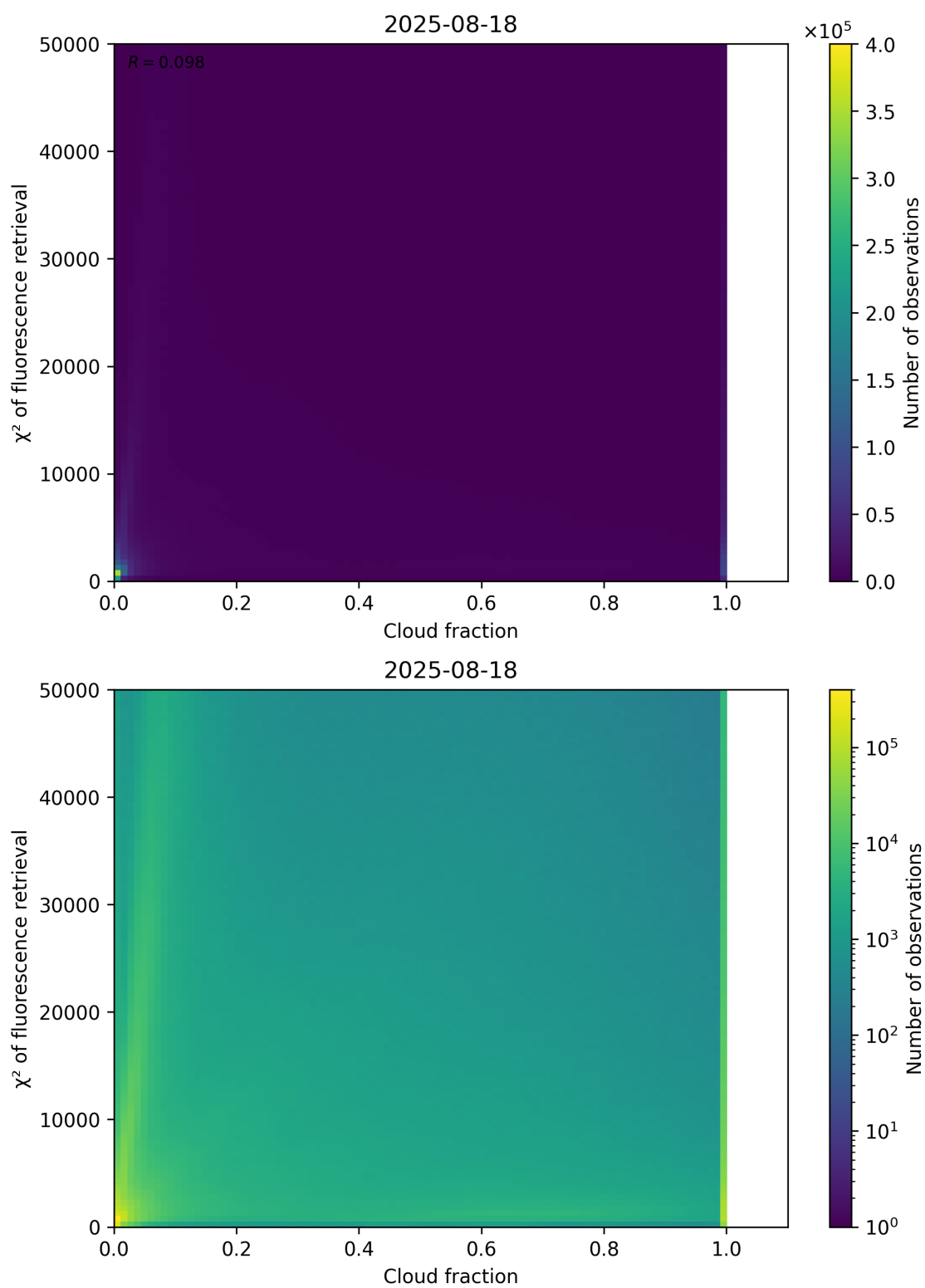
Figure 71: Scatter density plot of “Cloud fraction” against “ \chi^2 of fluorescence retrieval” for 2025-08-17 to 2025-08-19.
