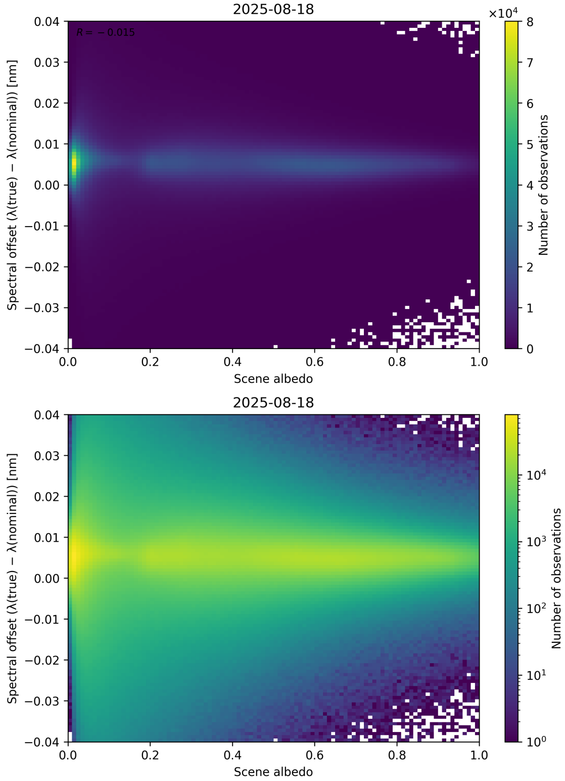
Figure 107: Scatter density plot of “Scene albedo” against “Spectral offset ( \lambda_{\text{true}} - \lambda_{\text{nominal}} )” for 2025-08-17 to 2025-08-19.
