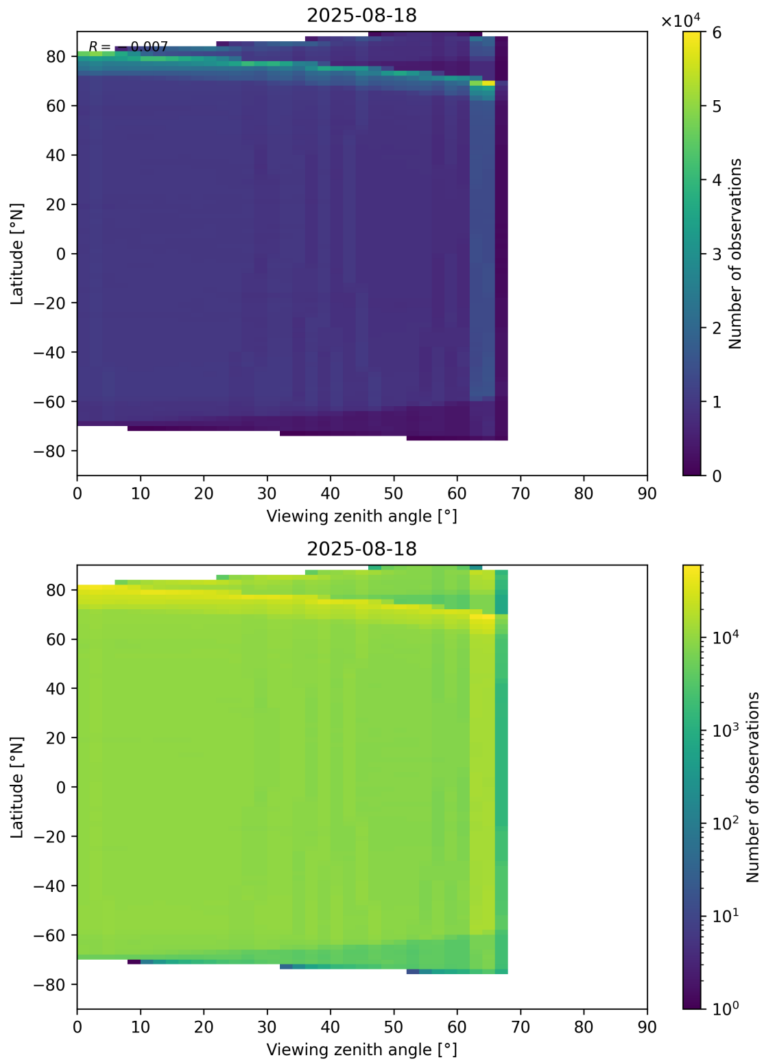
Figure 123: Scatter density plot of “Viewing zenith angle” against “Latitude” for 2025-08-17 to 2025-08-19.
