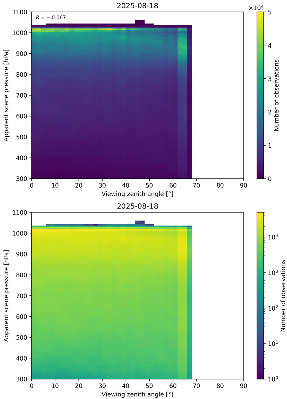
Figure 118: Scatter density plot of “Viewing zenith angle” against “Apparent scene pressure” for 2025-08-17 to 2025-08-19.
