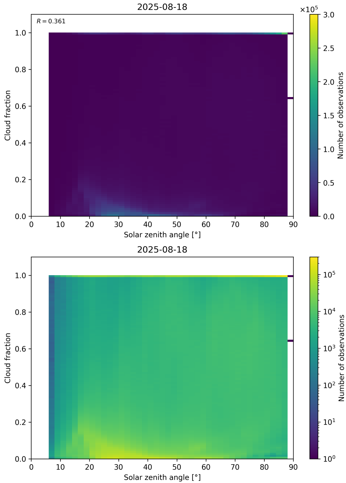
Figure 110: Scatter density plot of “Solar zenith angle” against “Cloud fraction” for 2025-08-17 to 2025-08-19.
