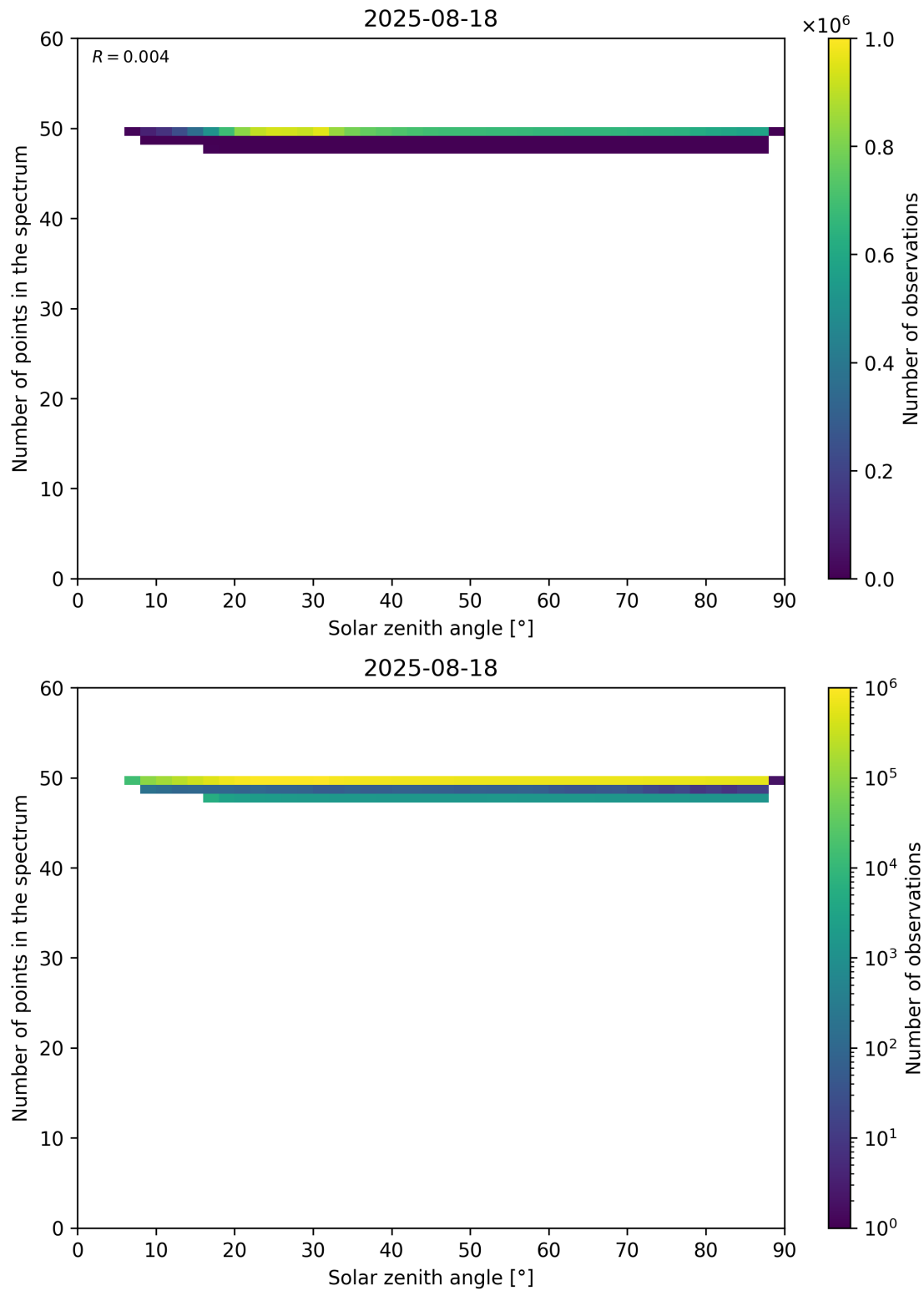
Figure 115: Scatter density plot of “Solar zenith angle” against “Number of points in the spectrum” for 2025-08-17 to 2025-08-19.
