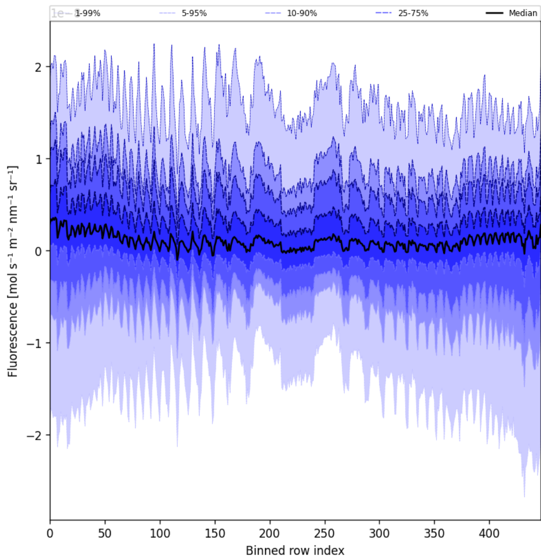
Figure 57: Along track statistics of "Fluorescence" for 2025-08-17 to 2025-08-19
