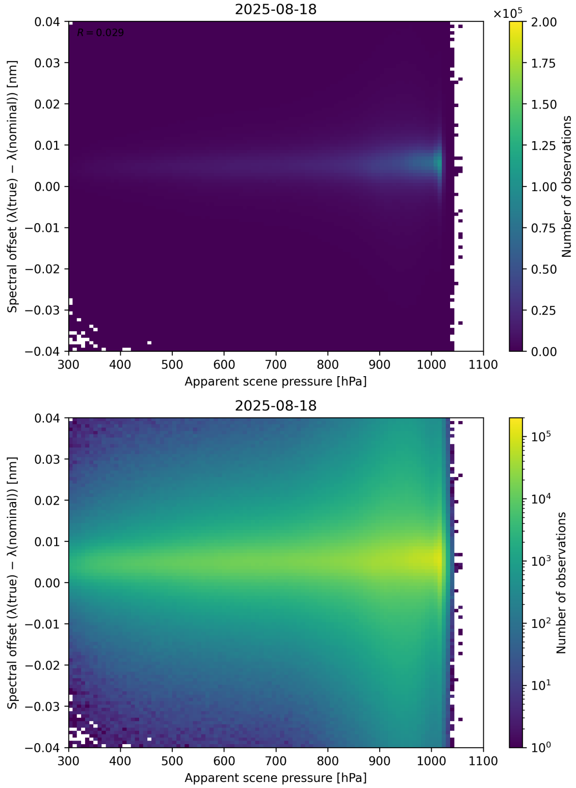
Figure 67: Scatter density plot of “Apparent scene pressure” against “Spectral offset ( \lambda_{\text{true}} - \lambda_{\text{nominal}} )” for 2025-08-17 to 2025-08-19.
