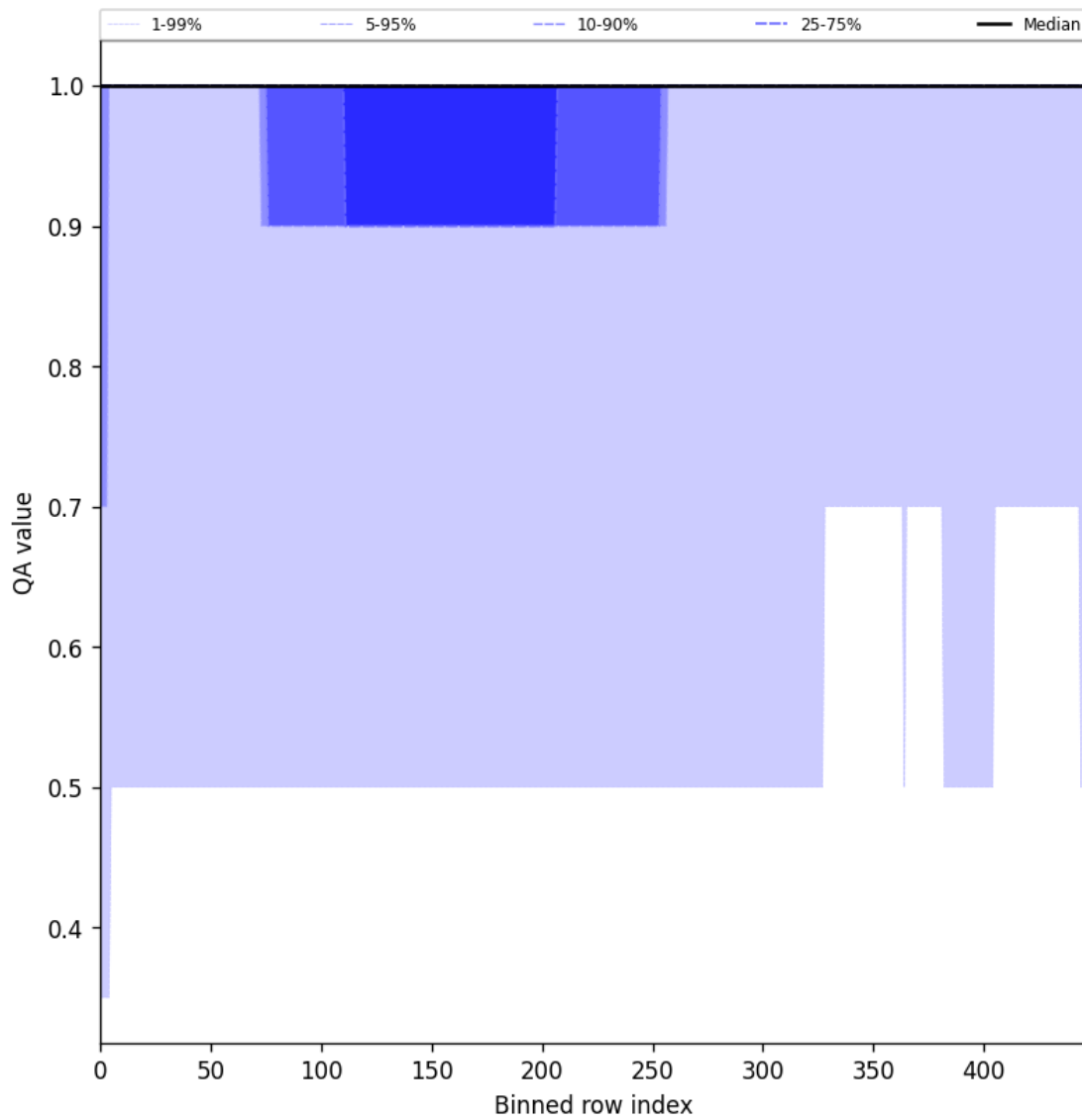
Figure 46: Along track statistics of “QA value” for 2025-08-17 to 2025-08-19
