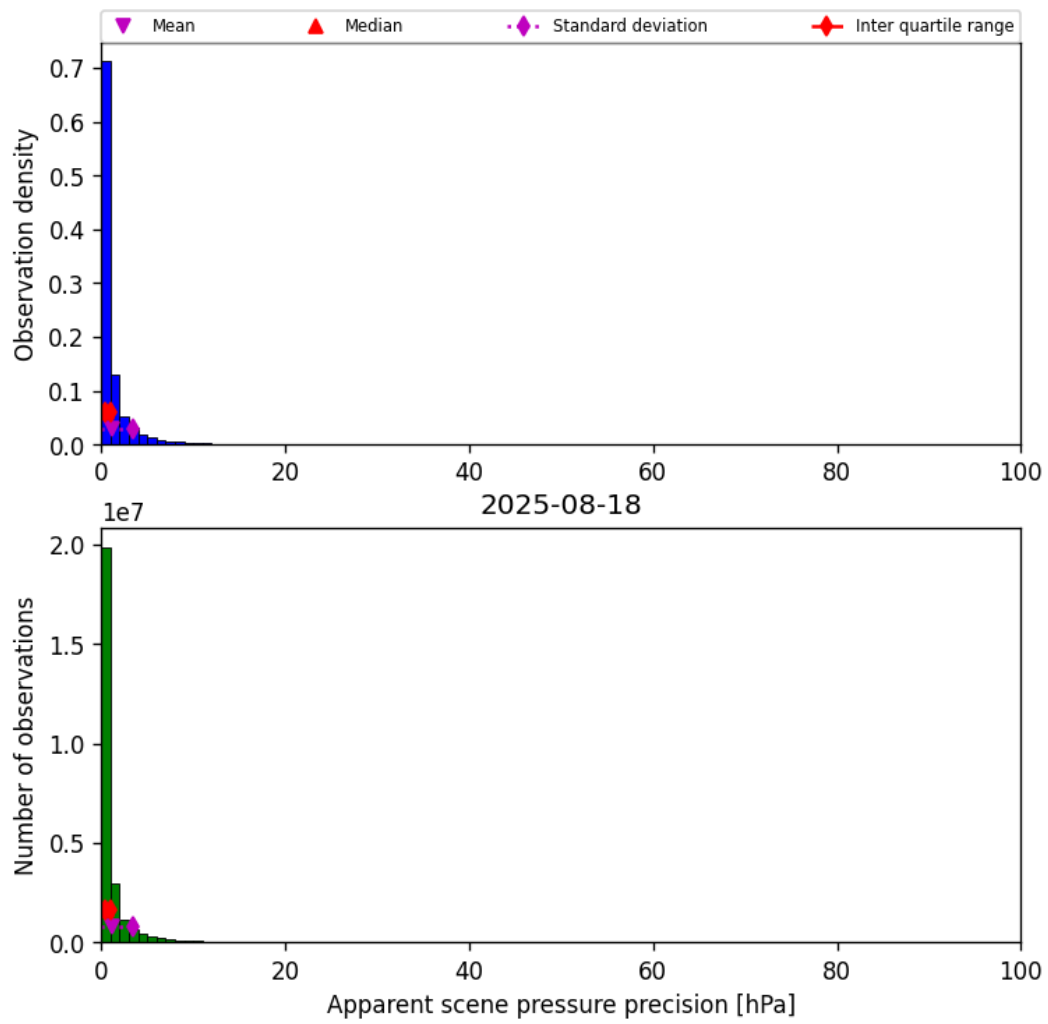
Figure 37: Histogram of “Apparent scene pressure precision” for 2025-08-17 to 2025-08-19
