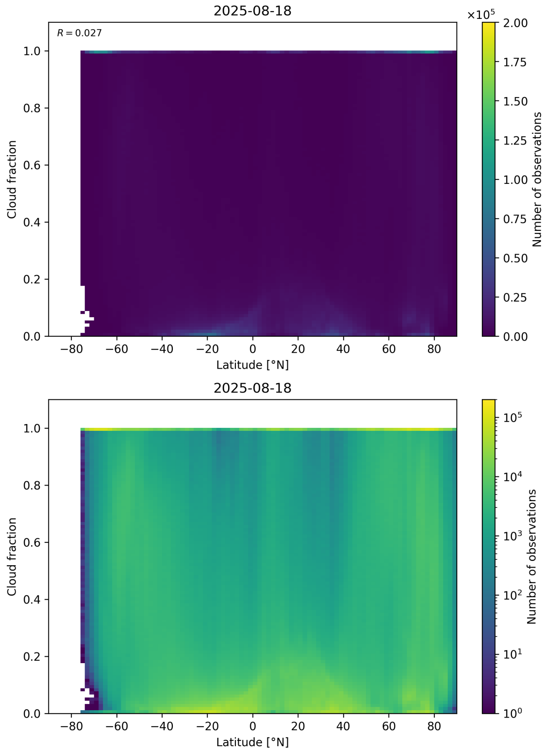
Figure 90: Scatter density plot of “Latitude” against “Cloud fraction” for 2025-08-17 to 2025-08-19.
