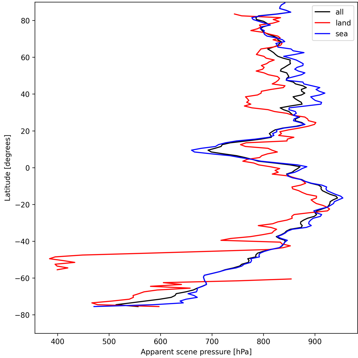
Figure 19: Zonal average of “Apparent scene pressure” for 2025-08-17 to 2025-08-19.
