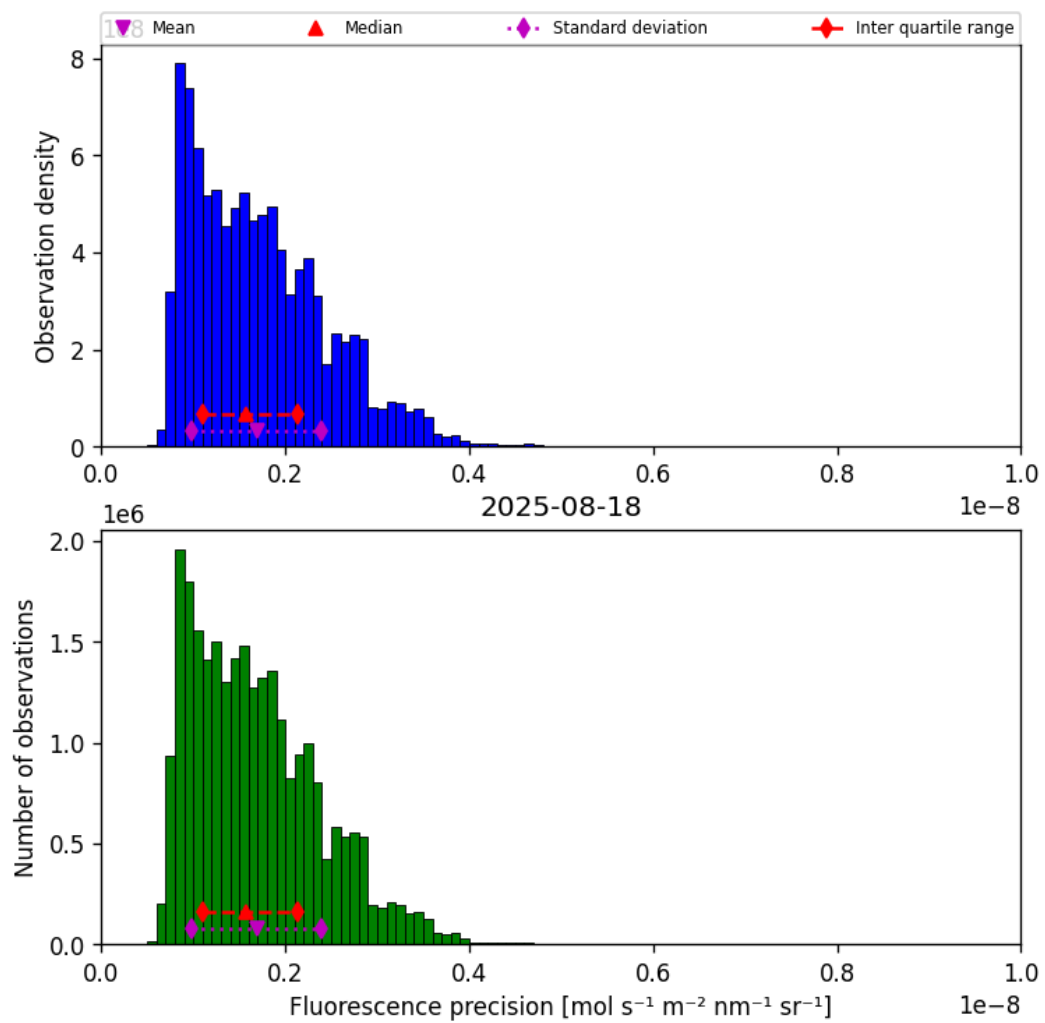
Figure 41: Histogram of “Fluorescence precision” for 2025-08-17 to 2025-08-19
