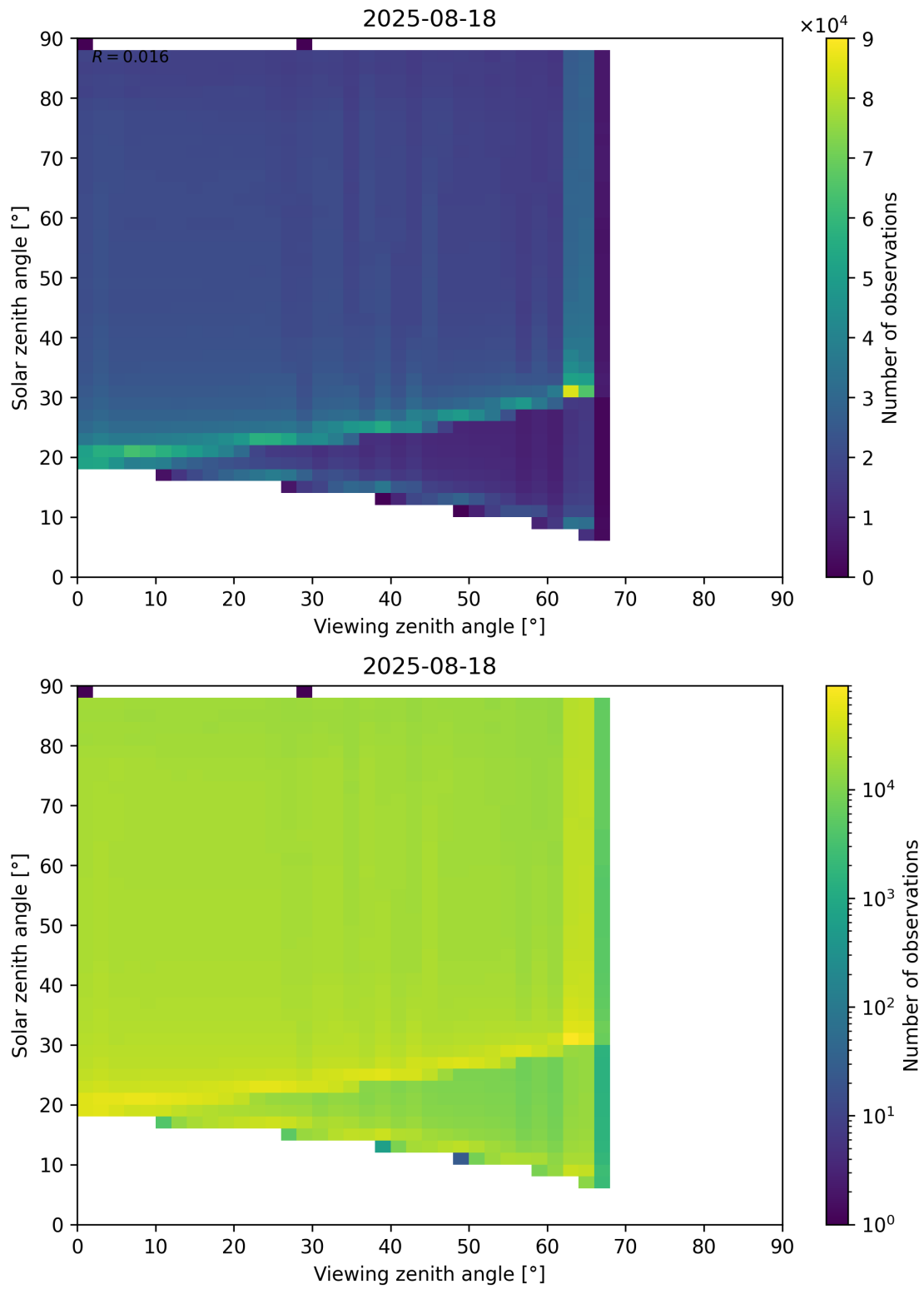
Figure 127: Scatter density plot of “Viewing zenith angle” against “Solar zenith angle” for 2025-08-17 to 2025-08-19.
