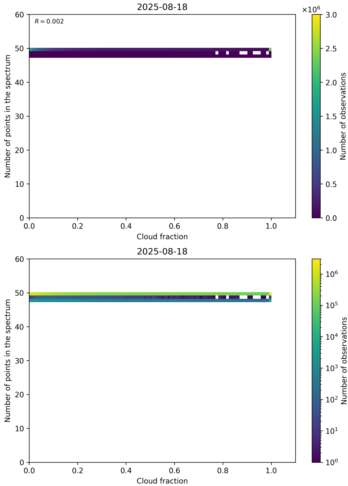
Figure 74: Scatter density plot of “Cloud fraction” against “Number of points in the spectrum” for 2025-08-17 to 2025-08-19.
