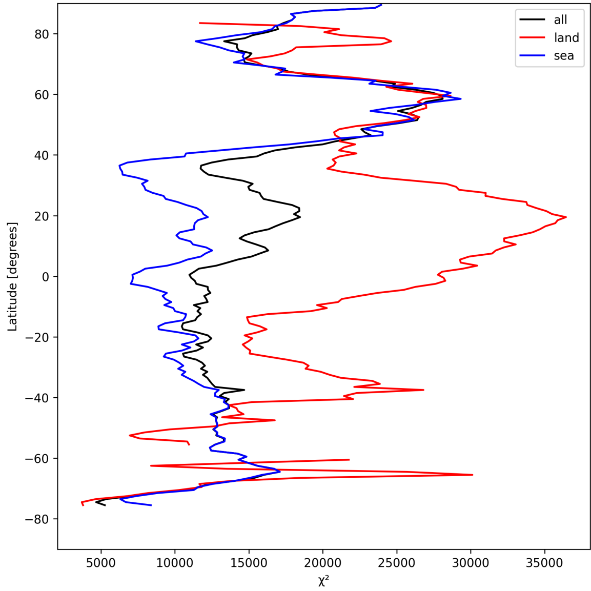
Figure 21: Zonal average of “ \chi^2 ” for 2025-08-17 to 2025-08-19.
