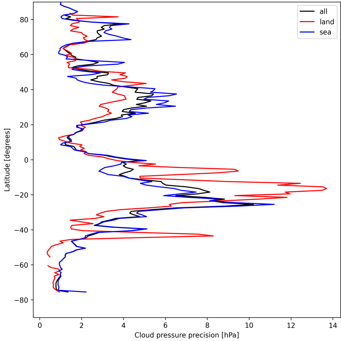
Figure 14: Zonal average of “Cloud pressure precision” for 2025-08-17 to 2025-08-19.
