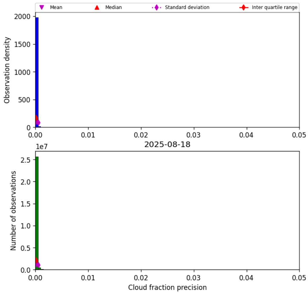
Figure 33: Histogram of “Cloud fraction precision” for 2025-08-17 to 2025-08-19
