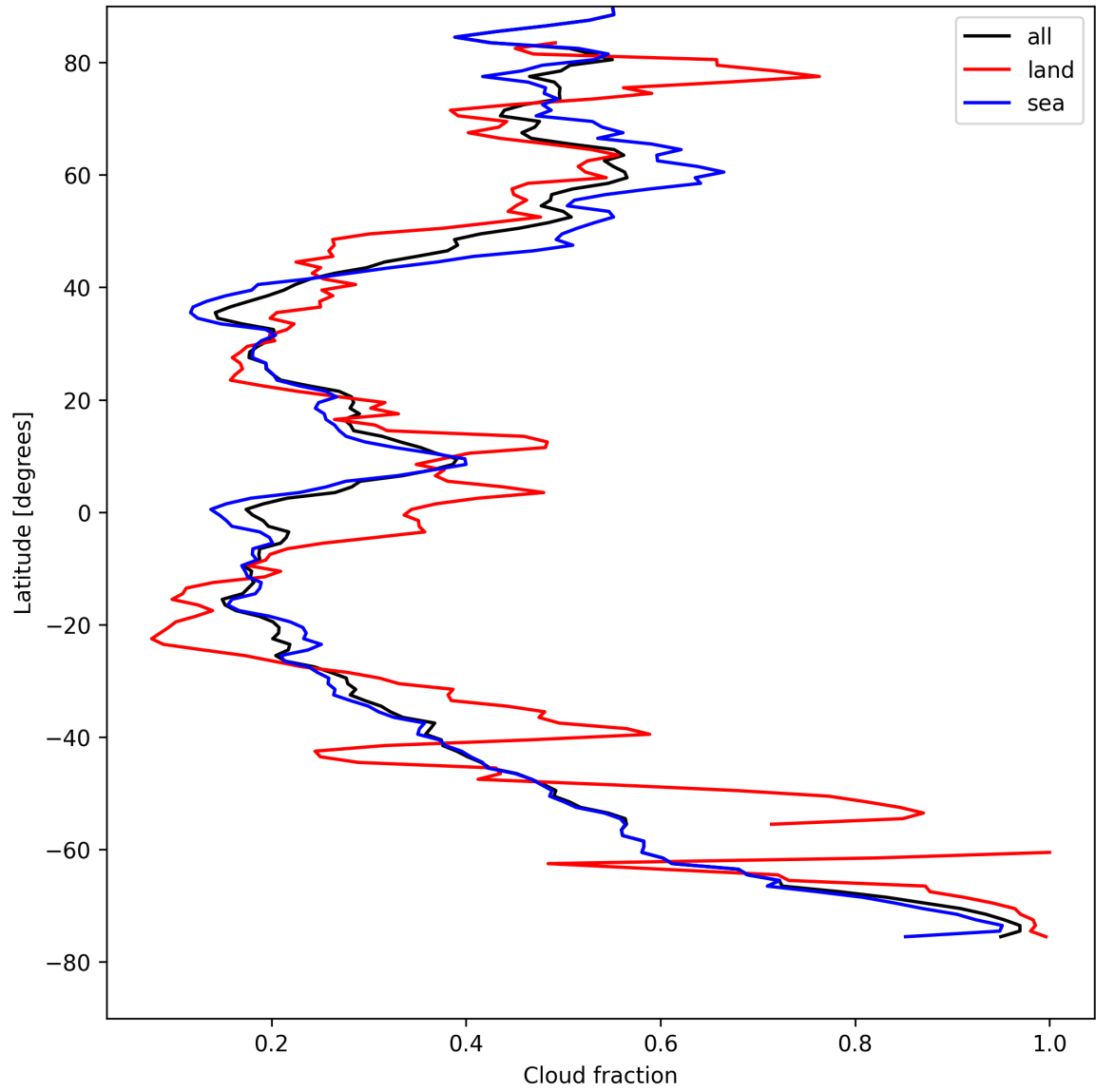
Figure 15: Zonal average of “Cloud fraction” for 2025-08-17 to 2025-08-19.
