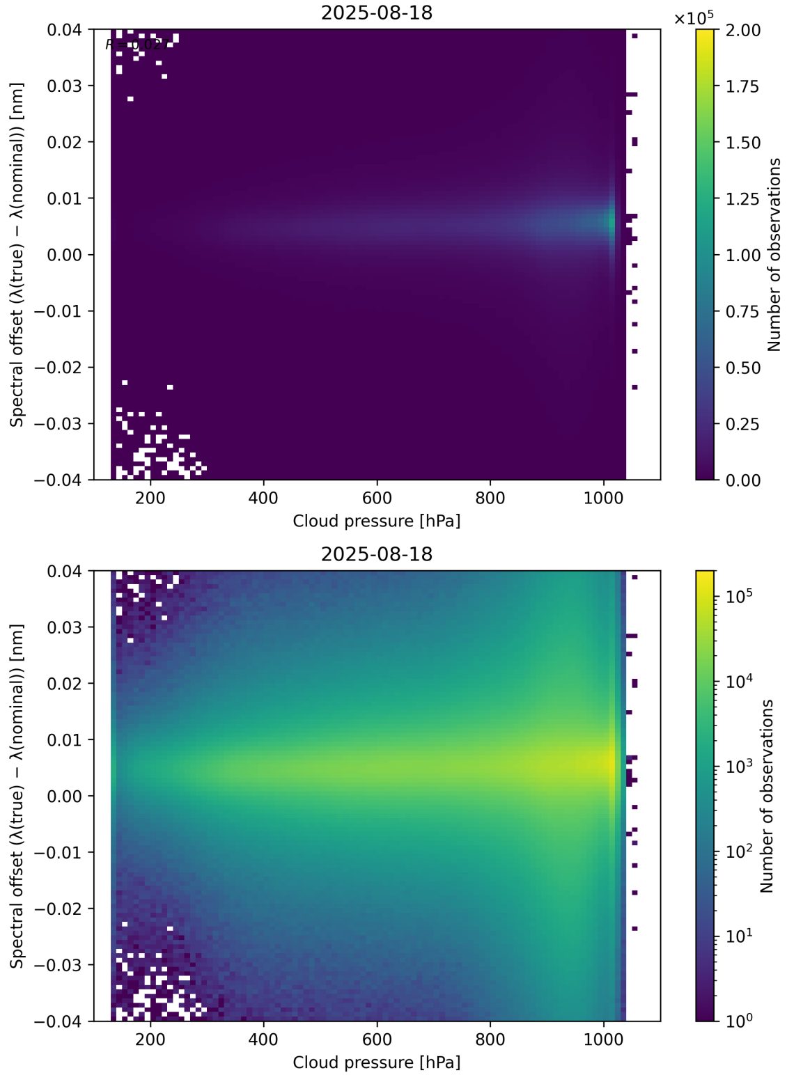
Figure 84: Scatter density plot of “Cloud pressure” against “Spectral offset ( \lambda_{\text{true}} - \lambda_{\text{nominal}} )” for 2025-08-17 to 2025-08-19.
