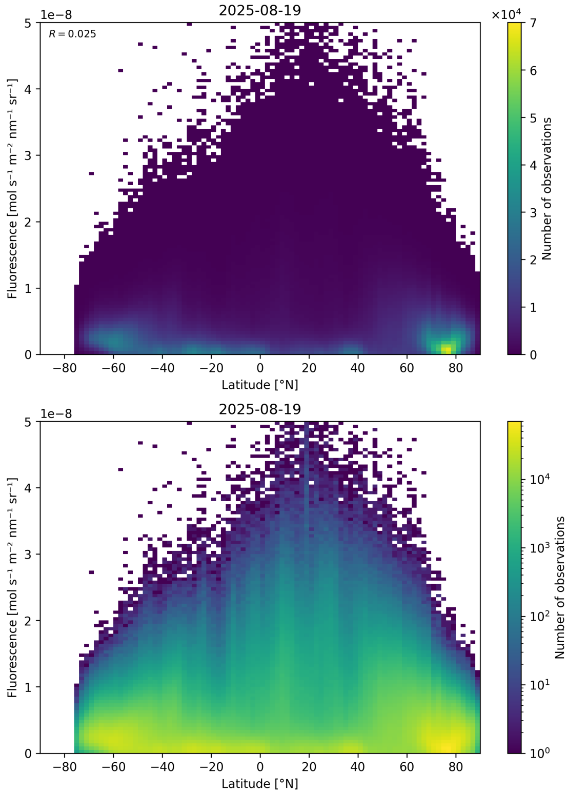
Figure 92: Scatter density plot of “Latitude” against “Fluorescence” for 2025-08-19 to 2025-08-20.
