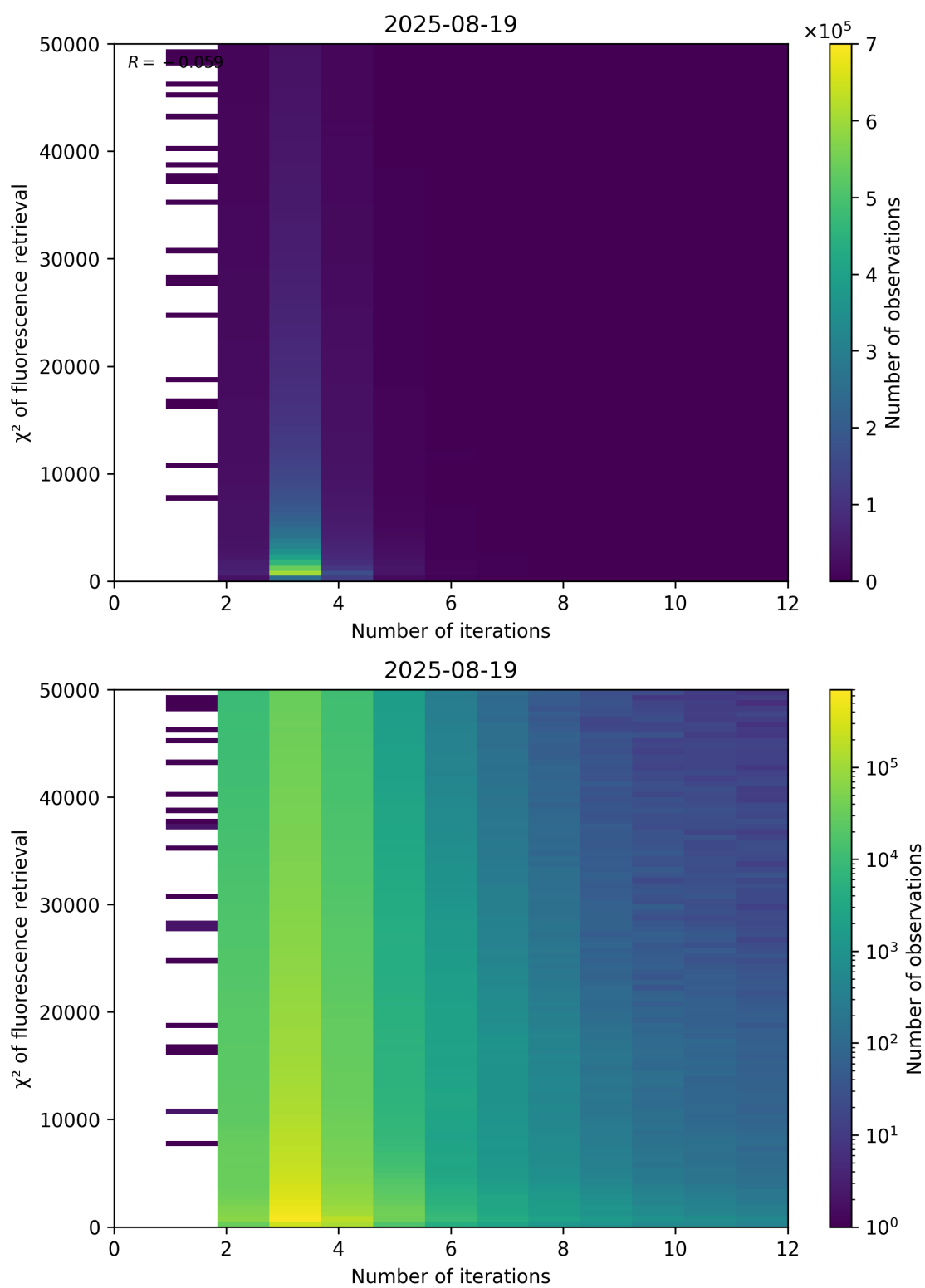
Figure 97: Scatter density plot of “Number of iterations” against “ \chi^2 of fluorescence retrieval” for 2025-08-19 to 2025-08-20.
