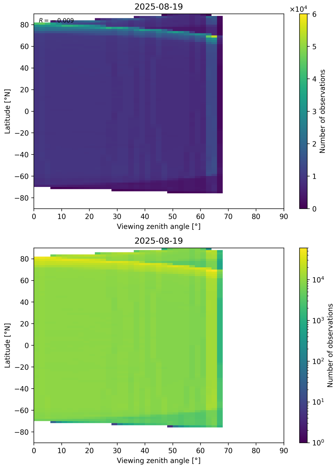
Figure 123: Scatter density plot of “Viewing zenith angle” against “Latitude” for 2025-08-19 to 2025-08-20.
