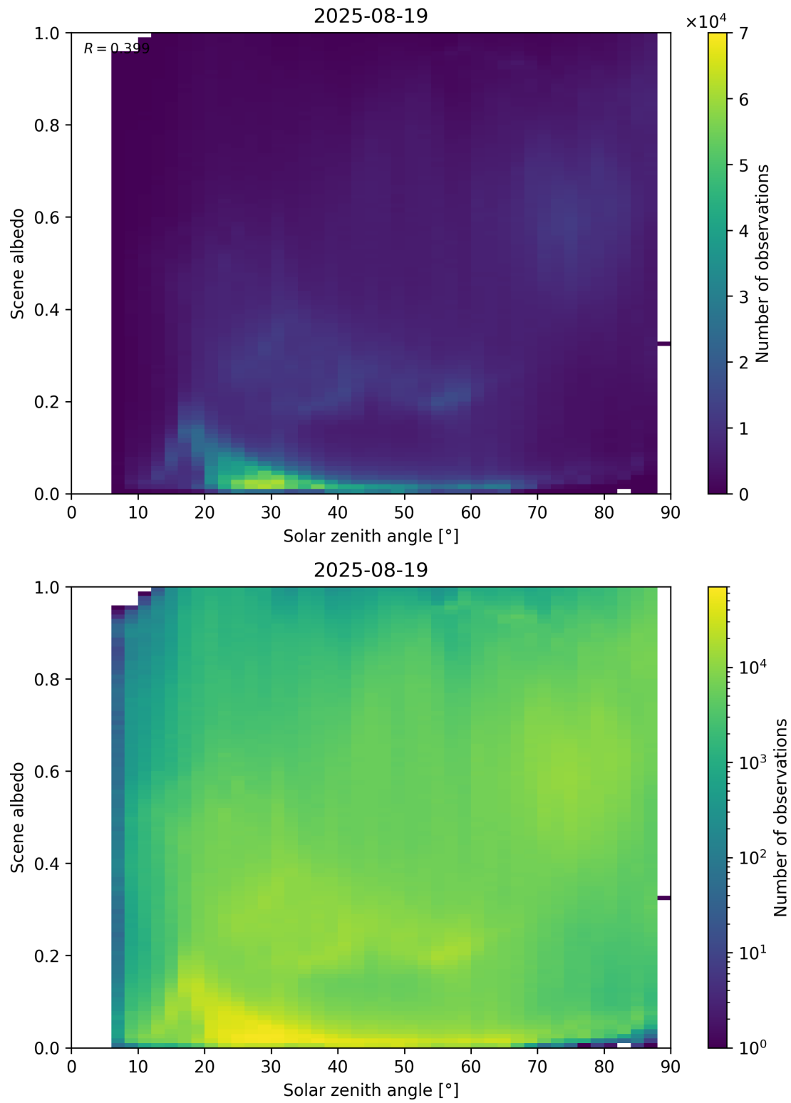
Figure 116: Scatter density plot of “Solar zenith angle” against “Scene albedo” for 2025-08-19 to 2025-08-20.
