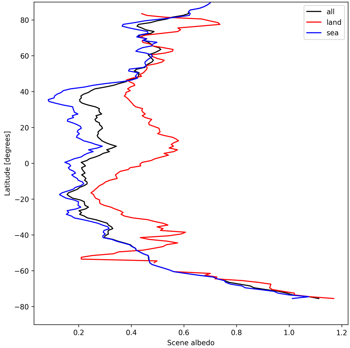
Figure 17: Zonal average of “Scene albedo” for 2025-08-19 to 2025-08-20.
