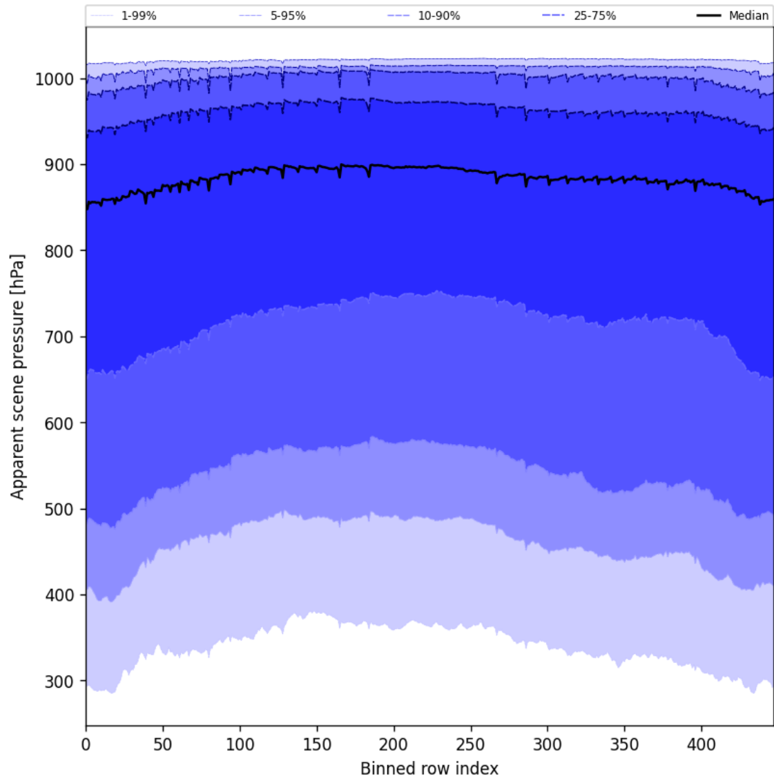
Figure 53: Along track statistics of “Apparent scene pressure” for 2025-08-19 to 2025-08-20
