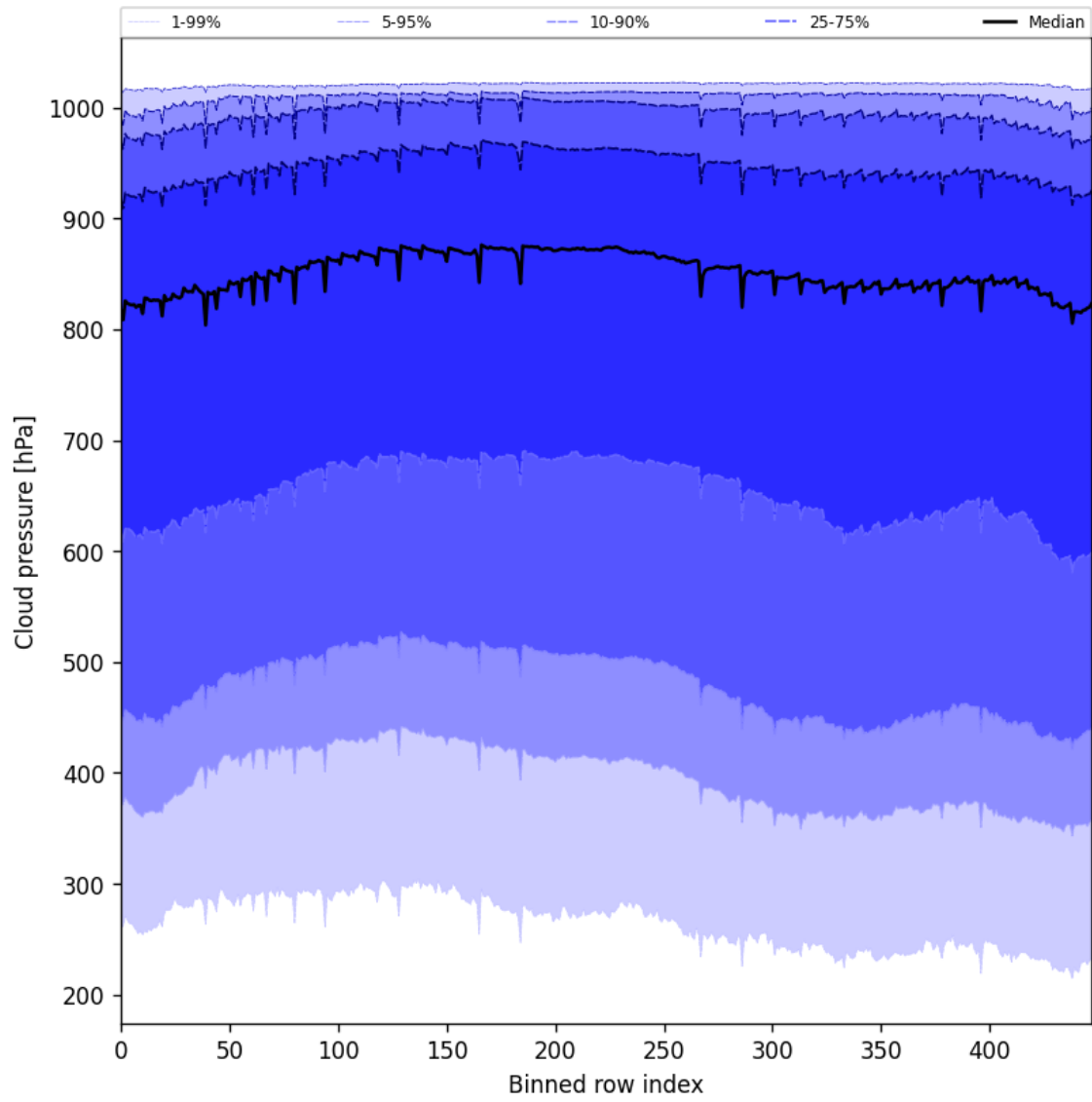
Figure 47: Along track statistics of “Cloud pressure” for 2025-08-19 to 2025-08-20
