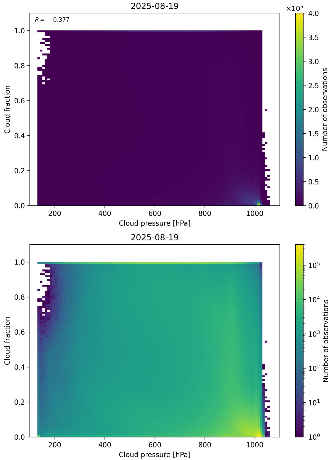
Figure 79: Scatter density plot of “Cloud pressure” against “Cloud fraction” for 2025-08-19 to 2025-08-20.
