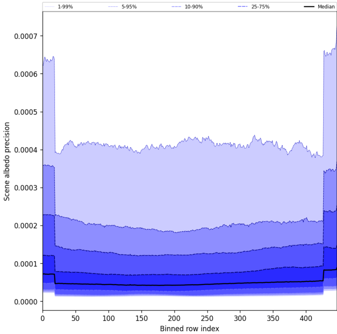
Figure 52: Along track statistics of “Scene albedo precision” for 2025-08-19 to 2025-08-20
