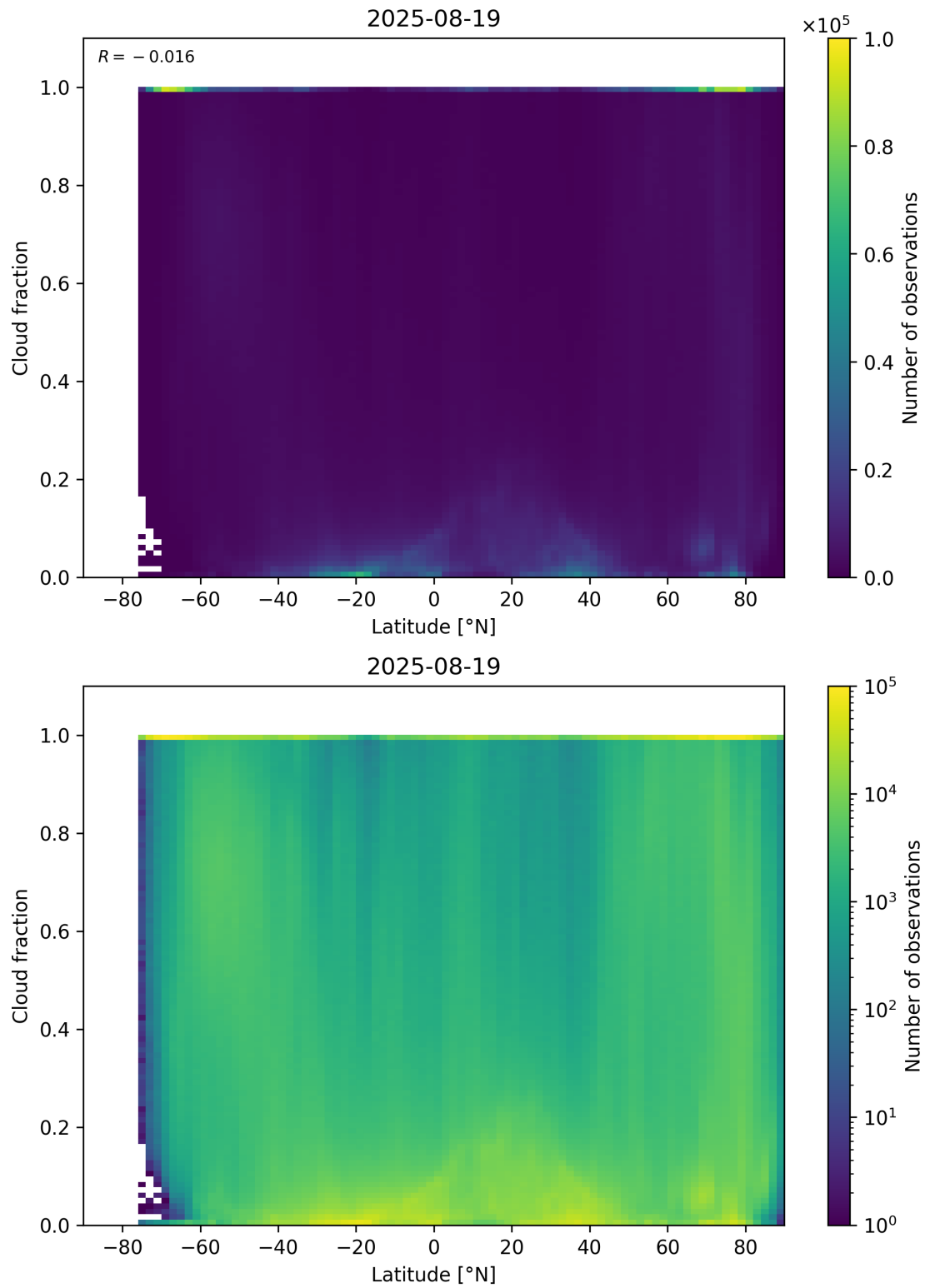
Figure 90: Scatter density plot of “Latitude” against “Cloud fraction” for 2025-08-19 to 2025-08-20.
