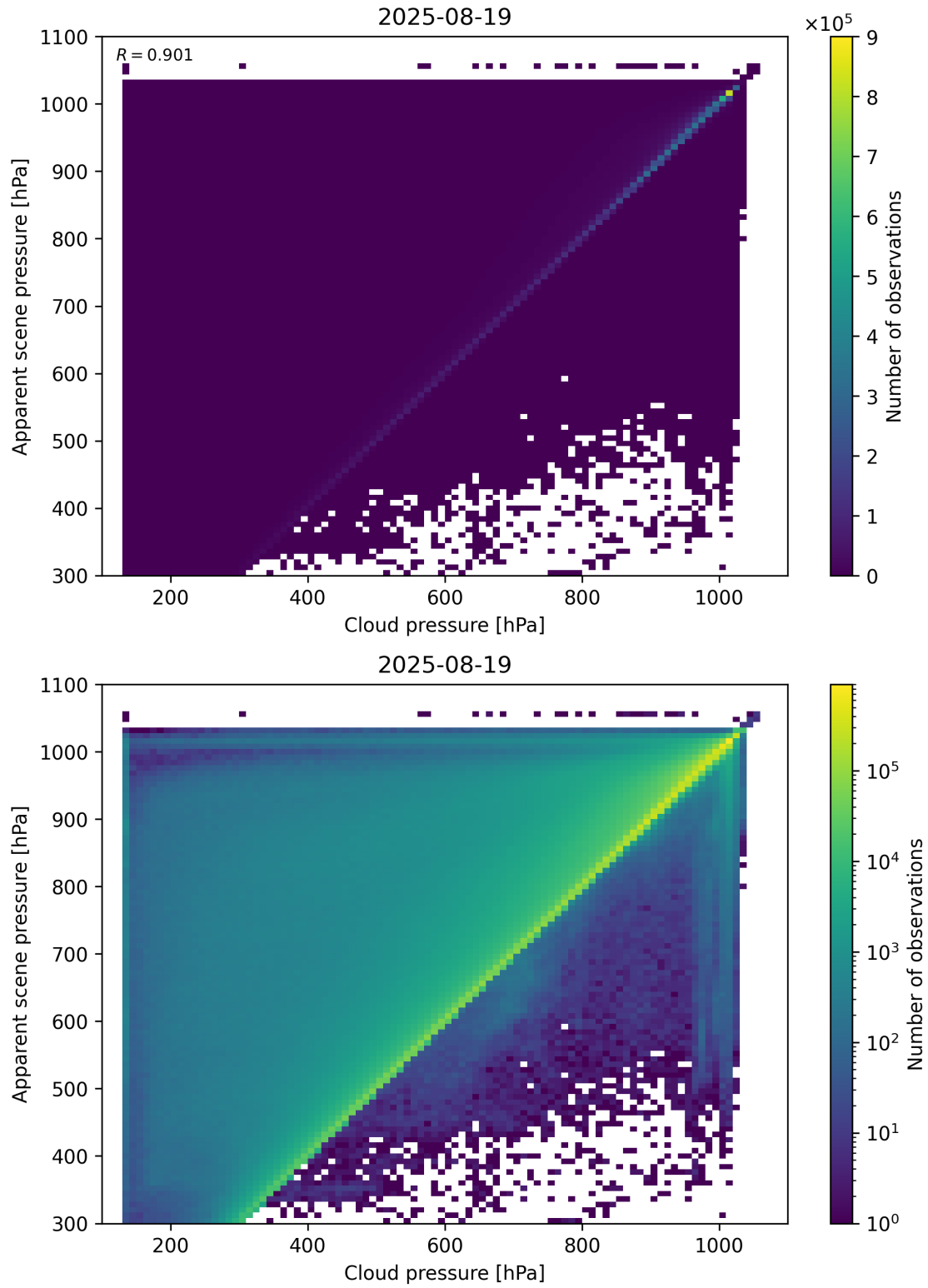
Figure 77: Scatter density plot of “Cloud pressure” against “Apparent scene pressure” for 2025-08-19 to 2025-08-20.
