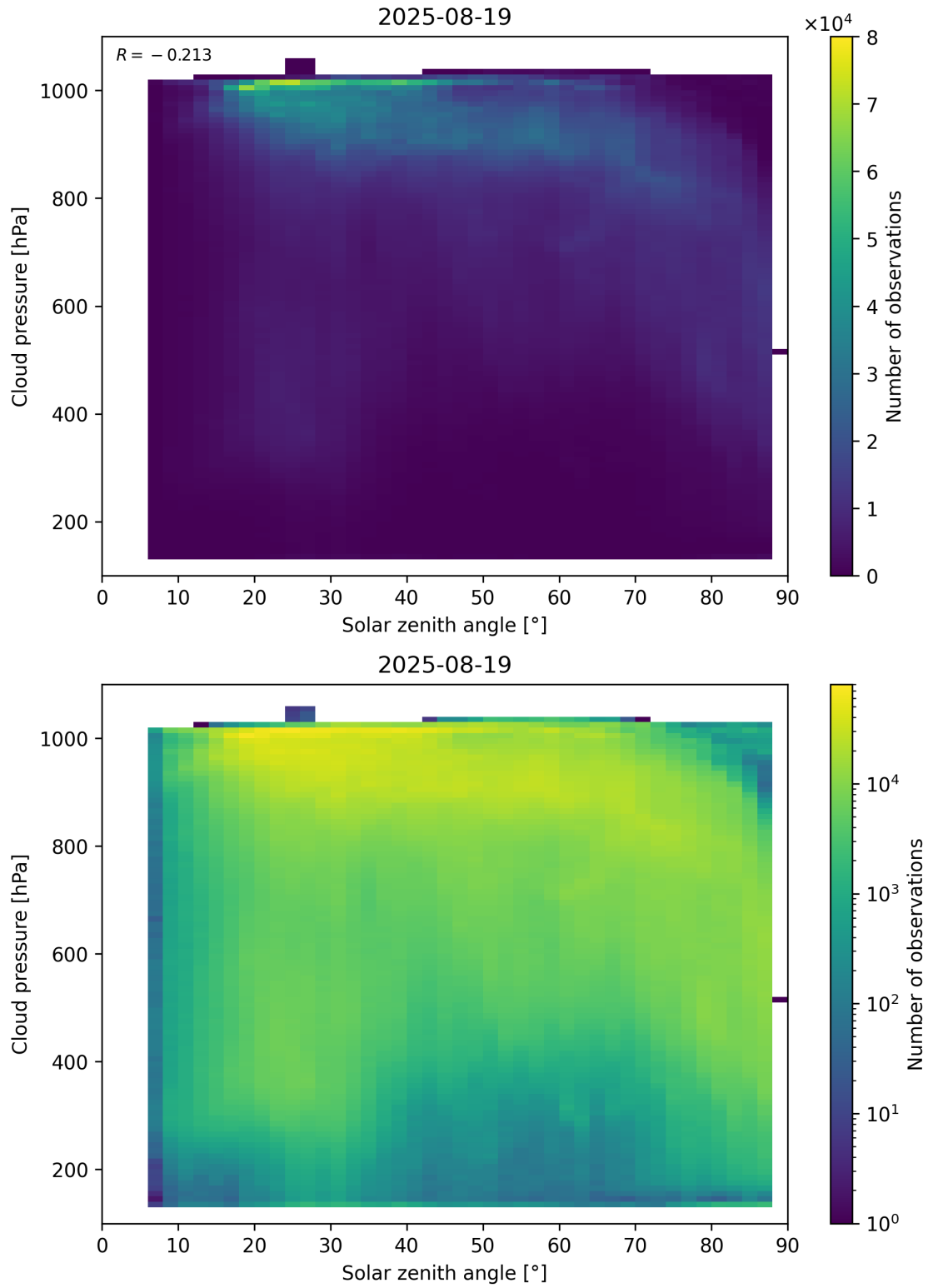
Figure 111: Scatter density plot of “Solar zenith angle” against “Cloud pressure” for 2025-08-19 to 2025-08-20.
