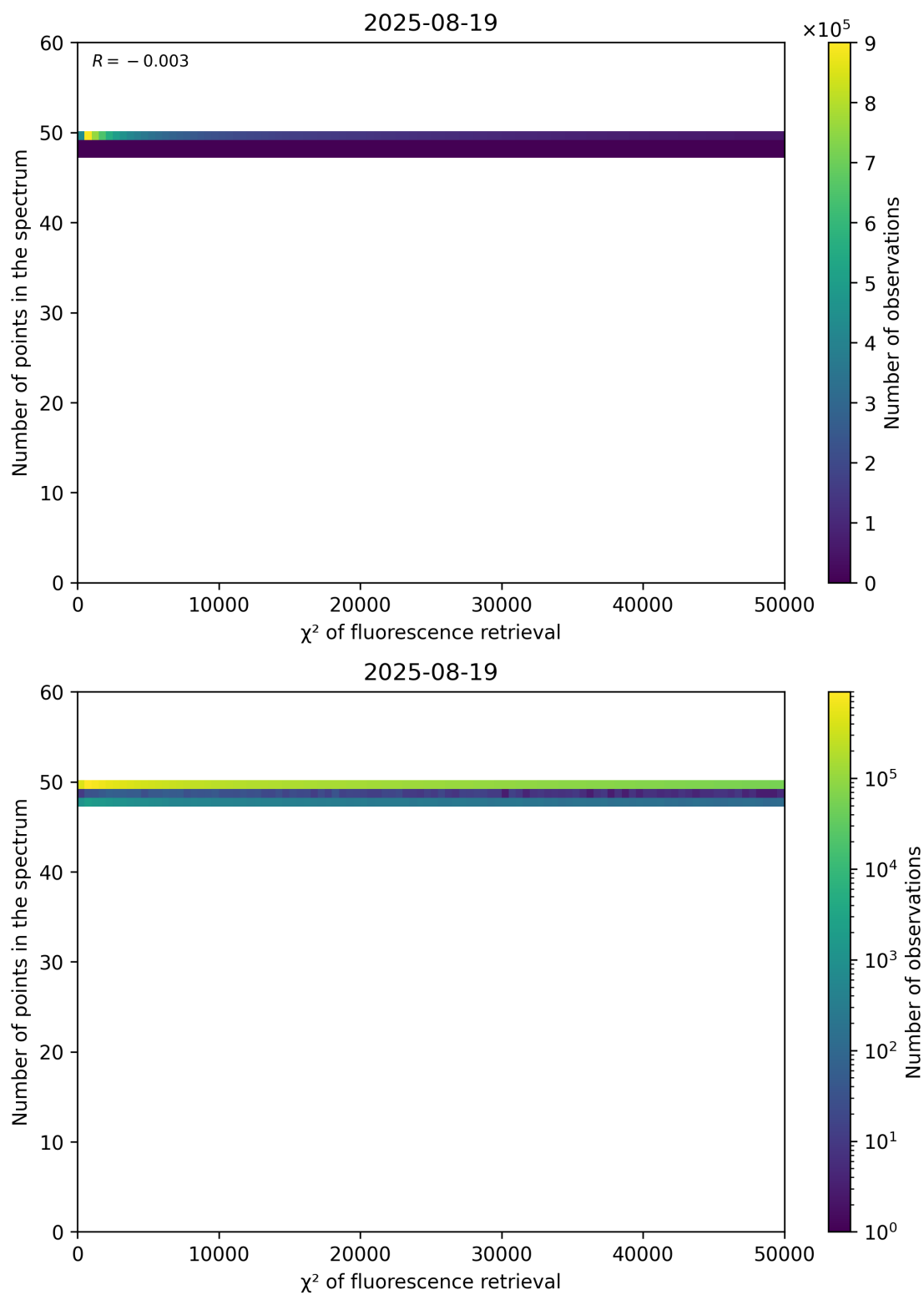
Figure 68: Scatter density plot of “ \chi^2 of fluorescence retrieval” against “Number of points in the spectrum” for 2025-08-19 to 2025-08-20.
