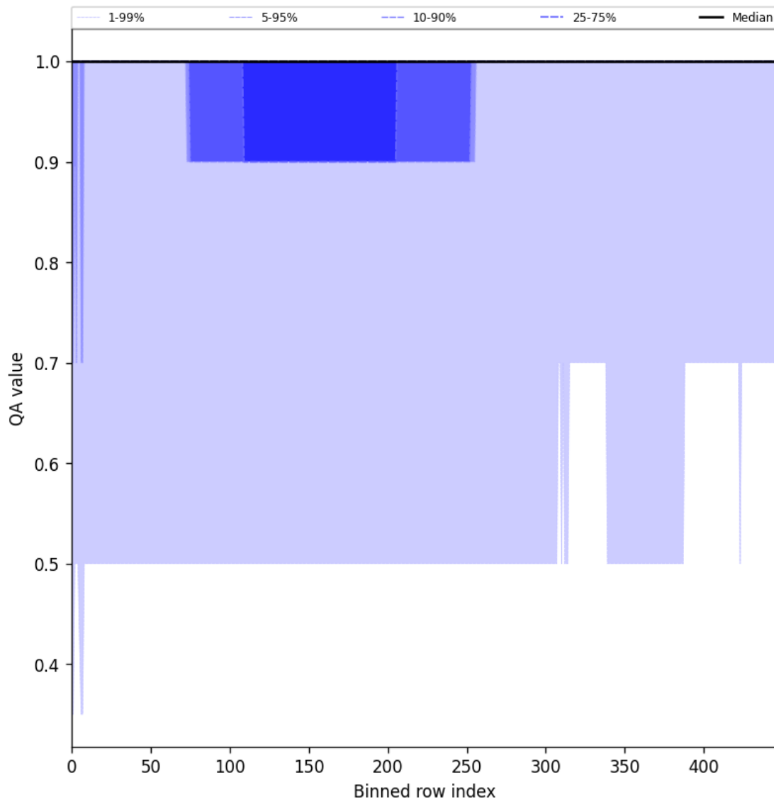
Figure 46: Along track statistics of “QA value” for 2025-08-19 to 2025-08-20
