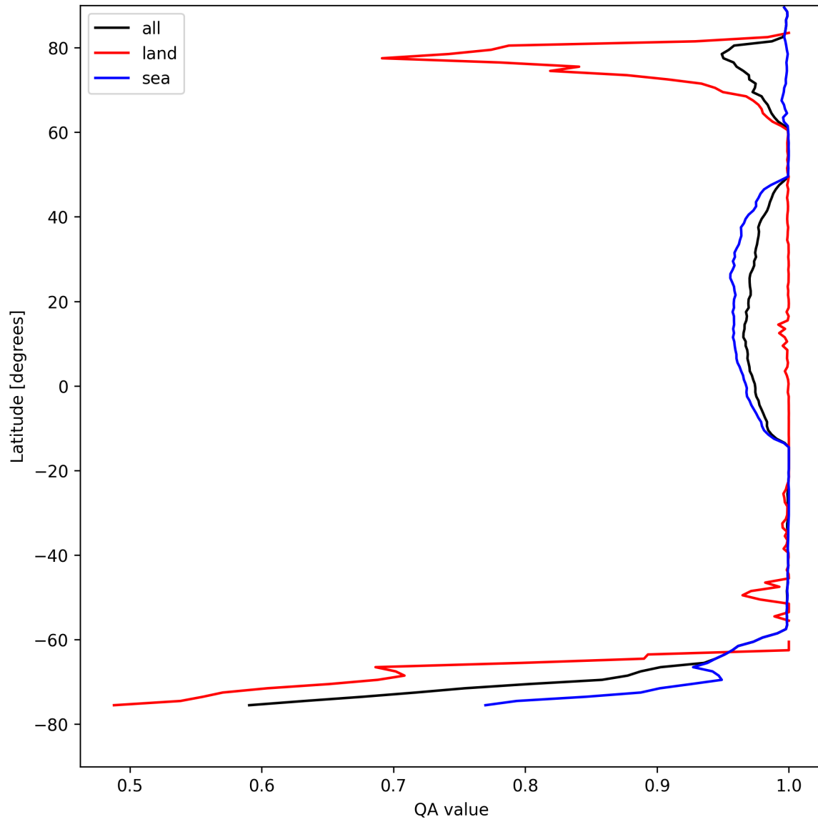
Figure 12: Zonal average of “QA value” for 2025-08-19 to 2025-08-20.
