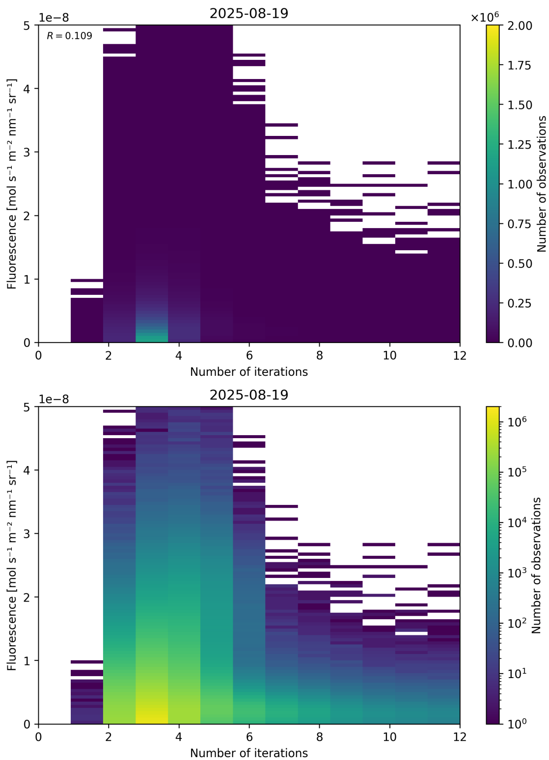
Figure 98: Scatter density plot of “Number of iterations” against “Fluorescence” for 2025-08-19 to 2025-08-20.
