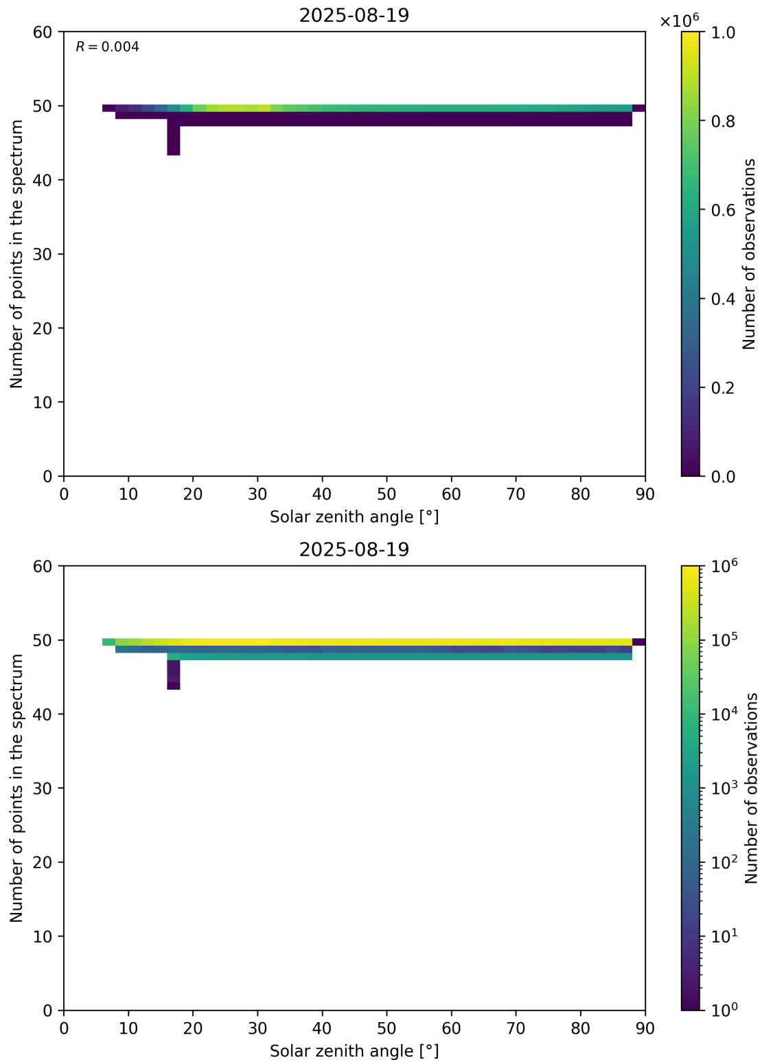
Figure 115: Scatter density plot of “Solar zenith angle” against “Number of points in the spectrum” for 2025-08-19 to 2025-08-20.
