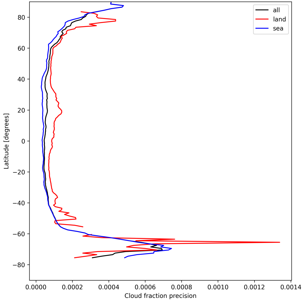
Figure 16: Zonal average of “Cloud fraction precision” for 2025-08-19 to 2025-08-20.
