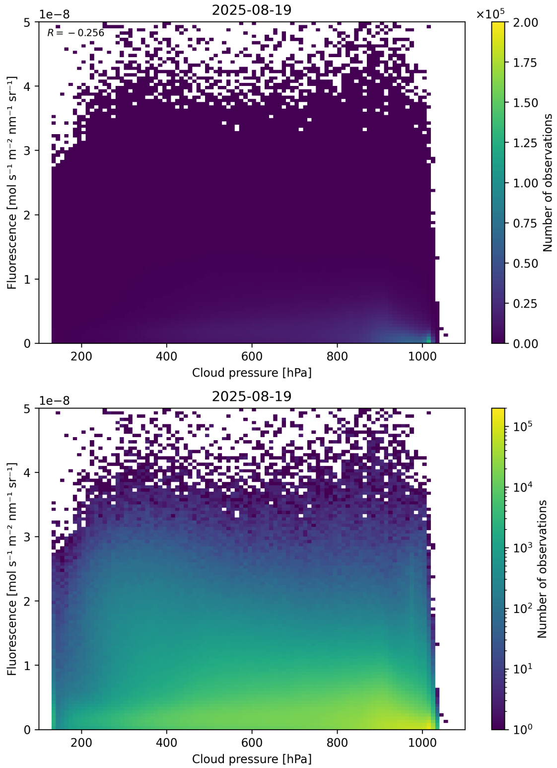
Figure 80: Scatter density plot of “Cloud pressure” against “Fluorescence” for 2025-08-19 to 2025-08-20.
