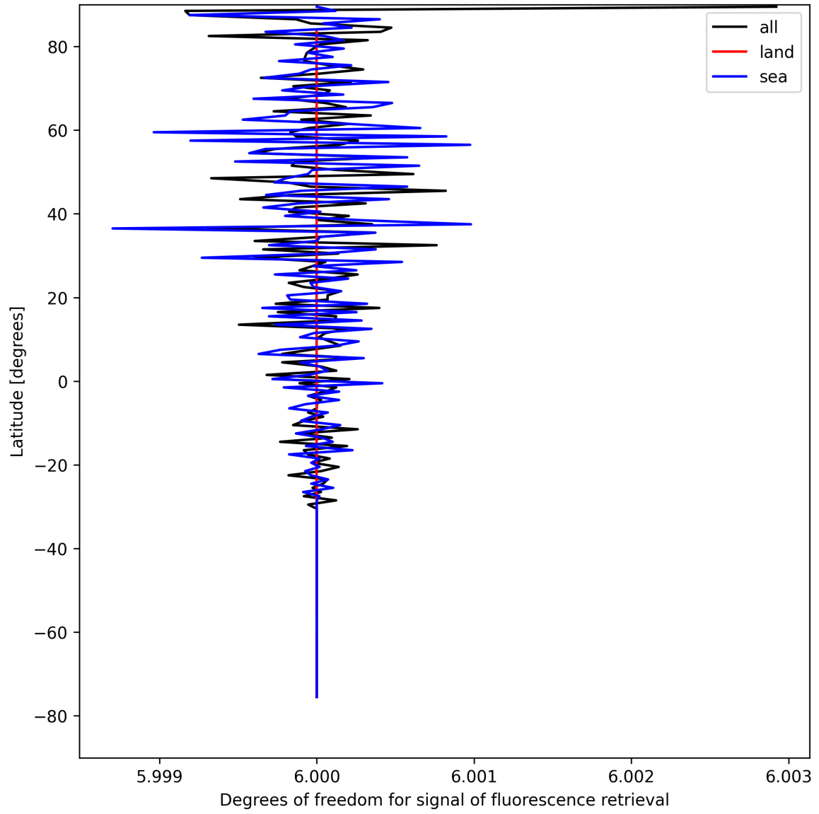
Figure 26: Zonal average of “Degrees of freedom for signal of fluorescence retrieval” for 2025-08-19 to 2025-08-20.
