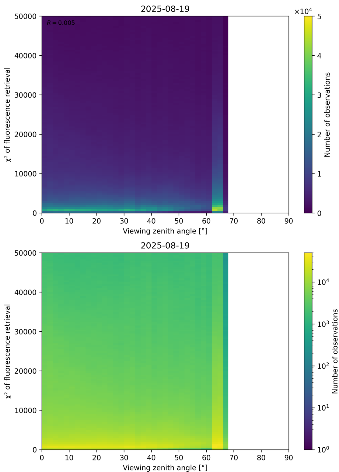
Figure 119: Scatter density plot of “Viewing zenith angle” against “ \chi^2 of fluorescence retrieval” for 2025-08-19 to 2025-08-20.
