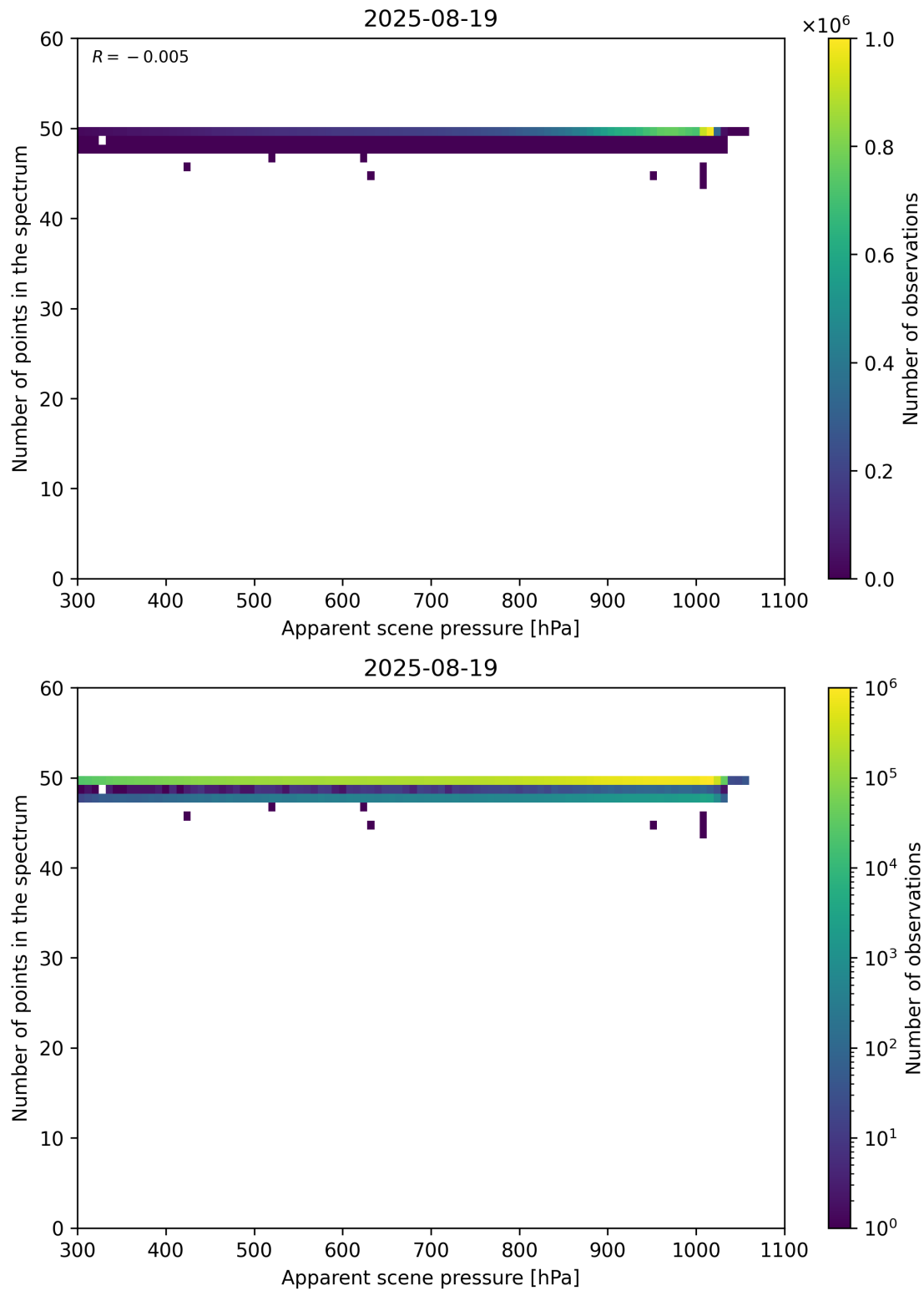
Figure 66: Scatter density plot of “Apparent scene pressure” against “Number of points in the spectrum” for 2025-08-19 to 2025-08-20.
