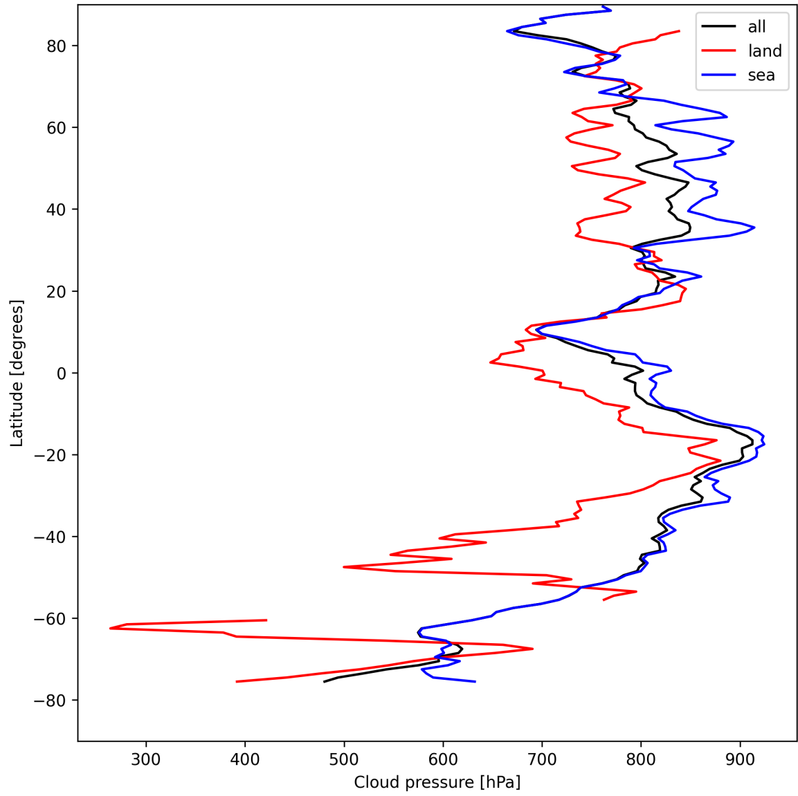
Figure 13: Zonal average of “Cloud pressure” for 2025-08-19 to 2025-08-20.
