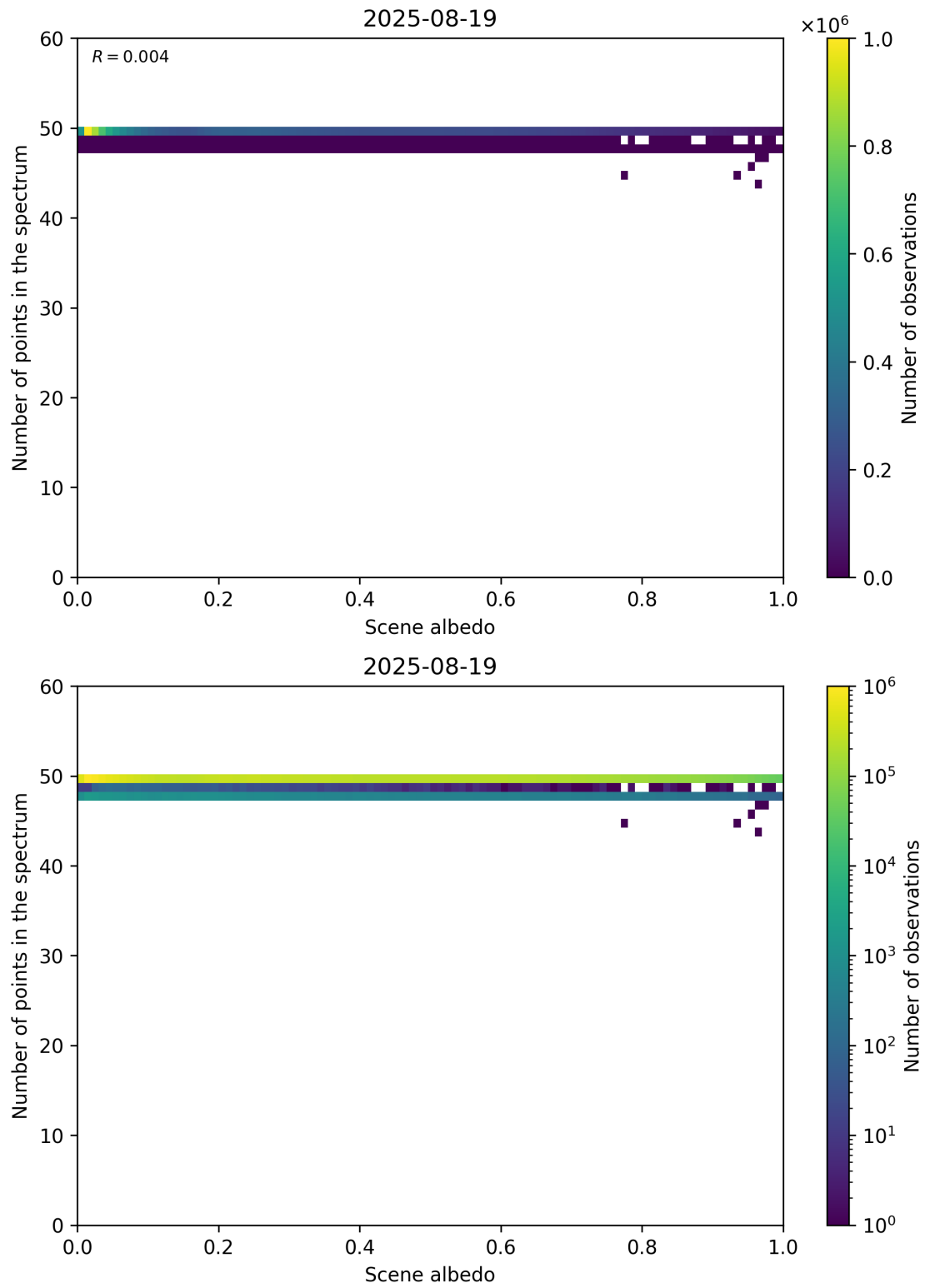
Figure 106: Scatter density plot of “Scene albedo” against “Number of points in the spectrum” for 2025-08-19 to 2025-08-20.
