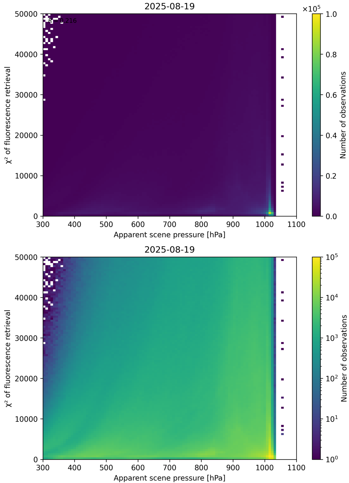
Figure 63: Scatter density plot of “Apparent scene pressure” against “ \chi^2 of fluorescence retrieval” for 2025-08-19 to 2025-08-20.
