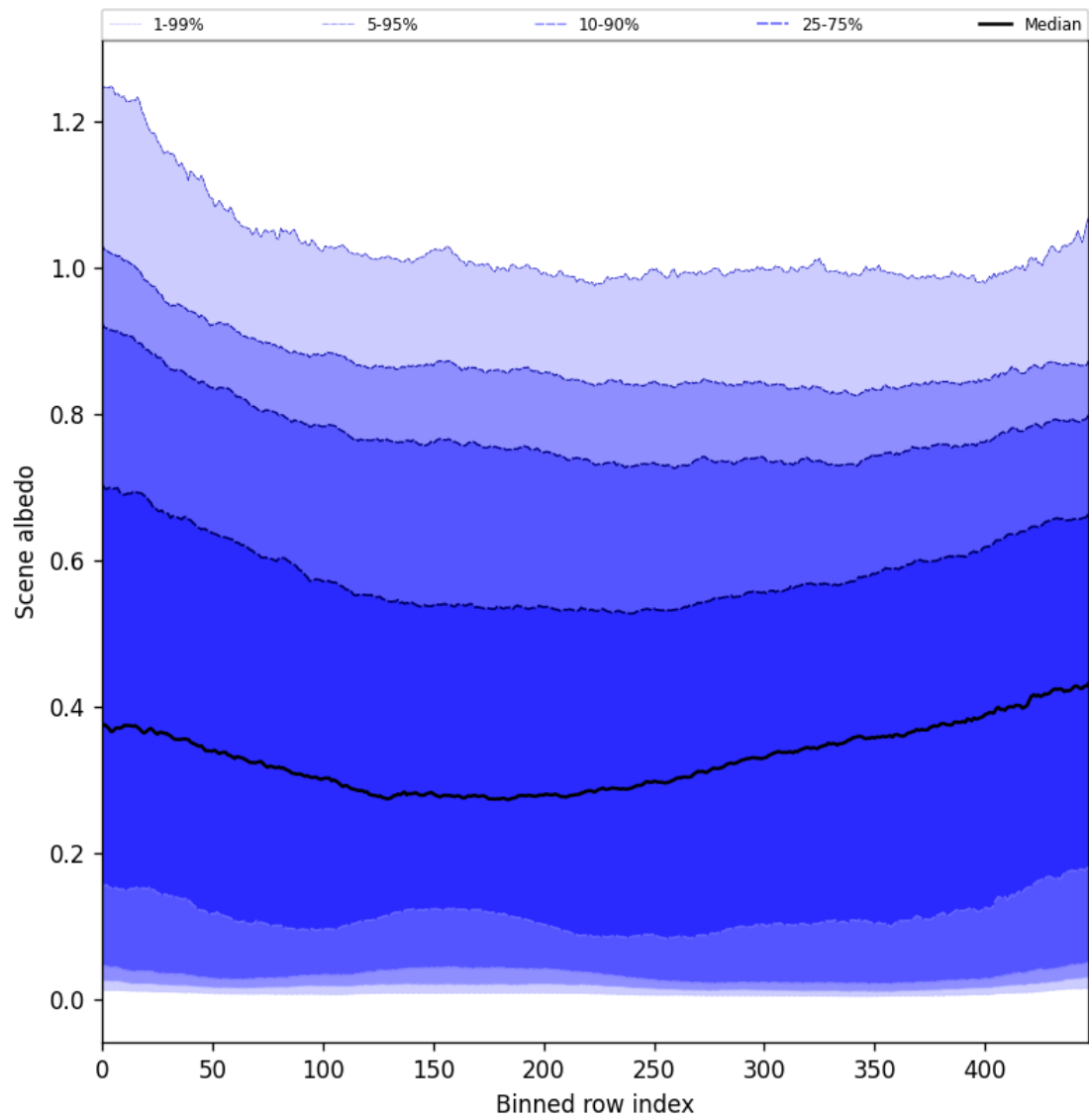
Figure 51: Along track statistics of “Scene albedo” for 2025-08-19 to 2025-08-20
