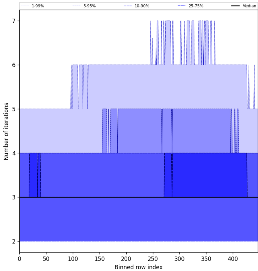
Figure 56: Along track statistics of “Number of iterations” for 2025-08-19 to 2025-08-20
