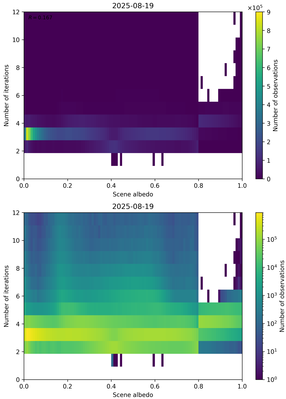
Figure 105: Scatter density plot of “Scene albedo” against “Number of iterations” for 2025-08-19 to 2025-08-20.
