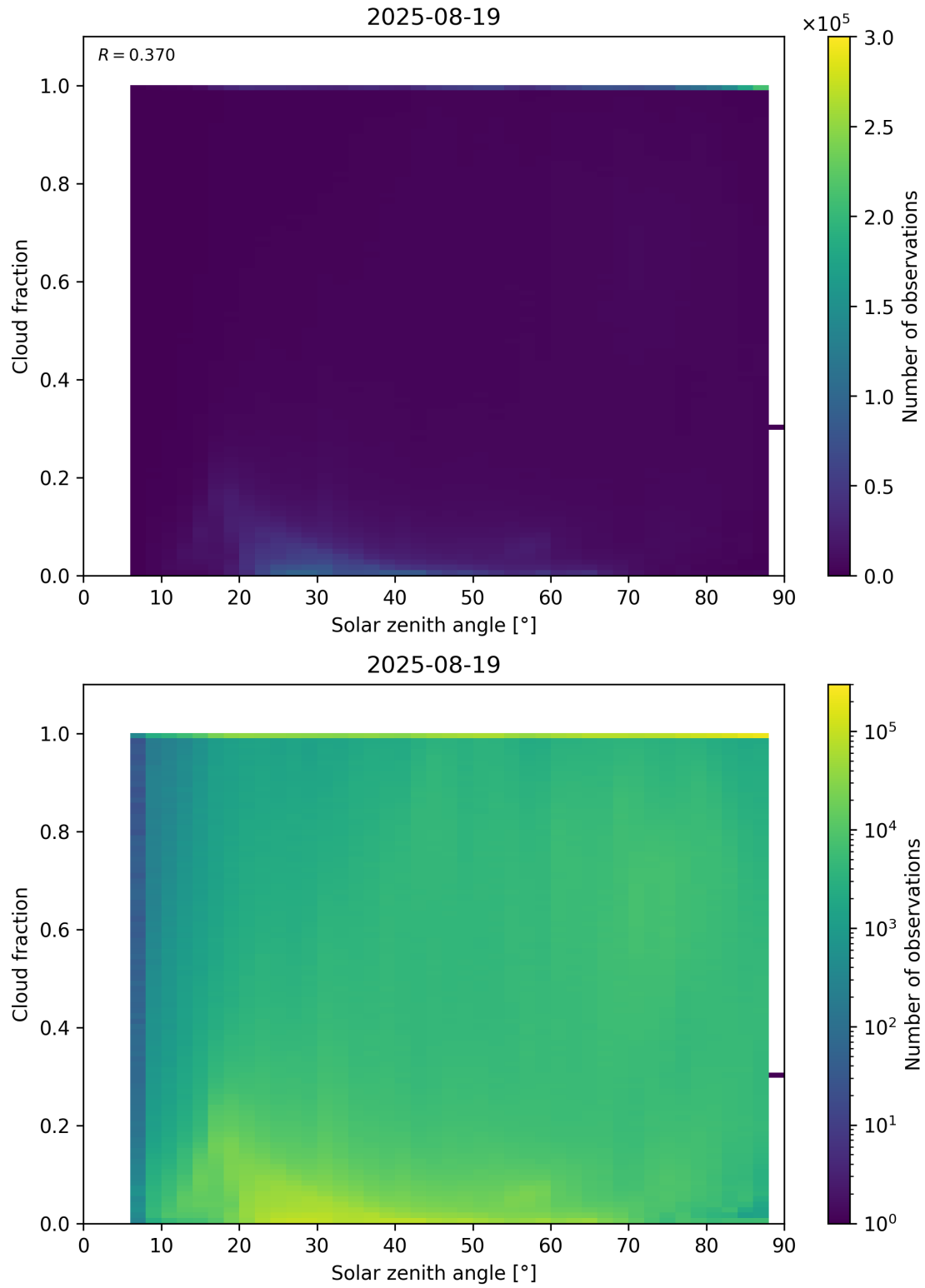
Figure 110: Scatter density plot of “Solar zenith angle” against “Cloud fraction” for 2025-08-19 to 2025-08-20.
