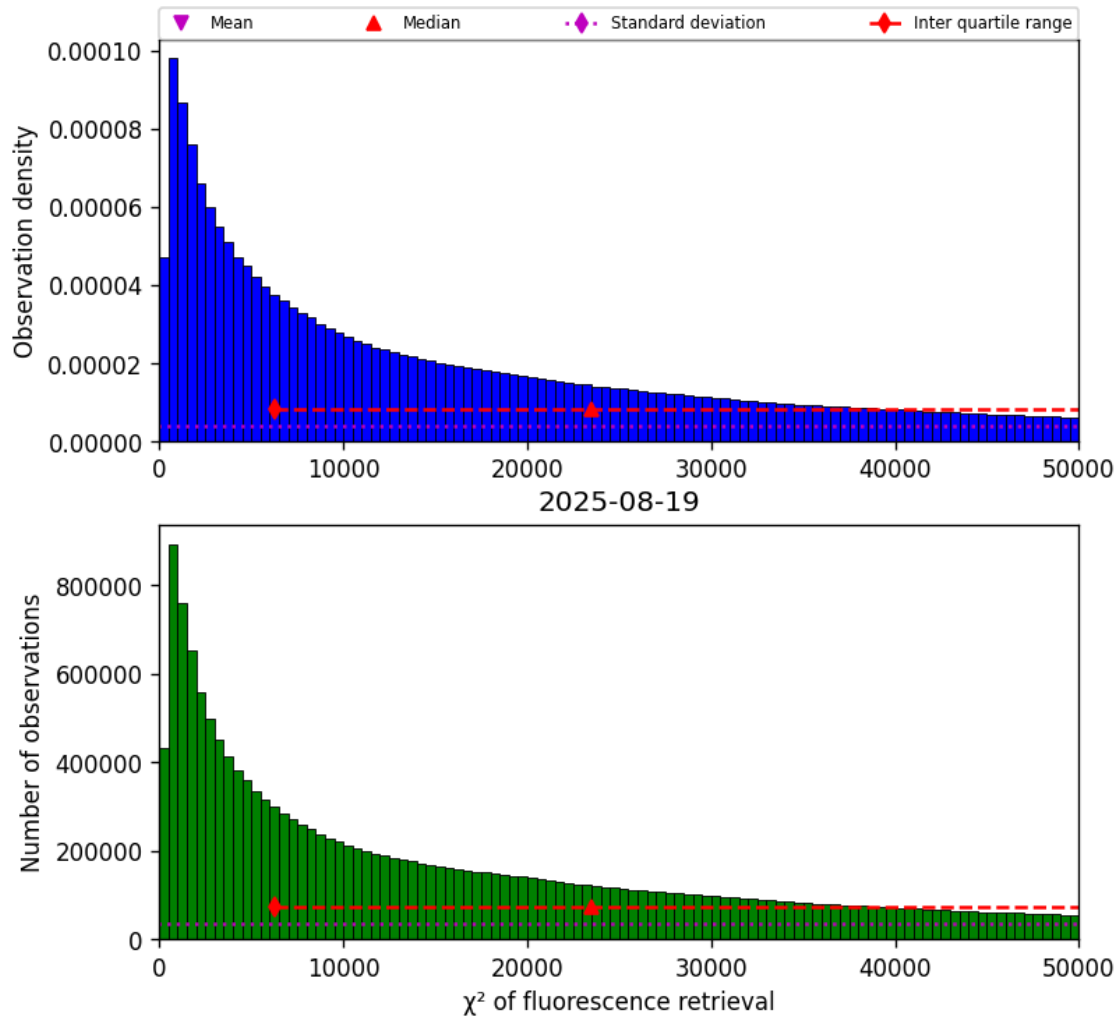
Figure 42: Histogram of “ \chi^2 of fluorescence retrieval” for 2025-08-19 to 2025-08-20
