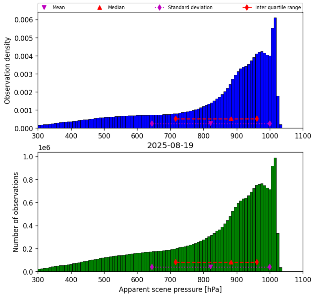
Figure 36: Histogram of “Apparent scene pressure” for 2025-08-19 to 2025-08-20
