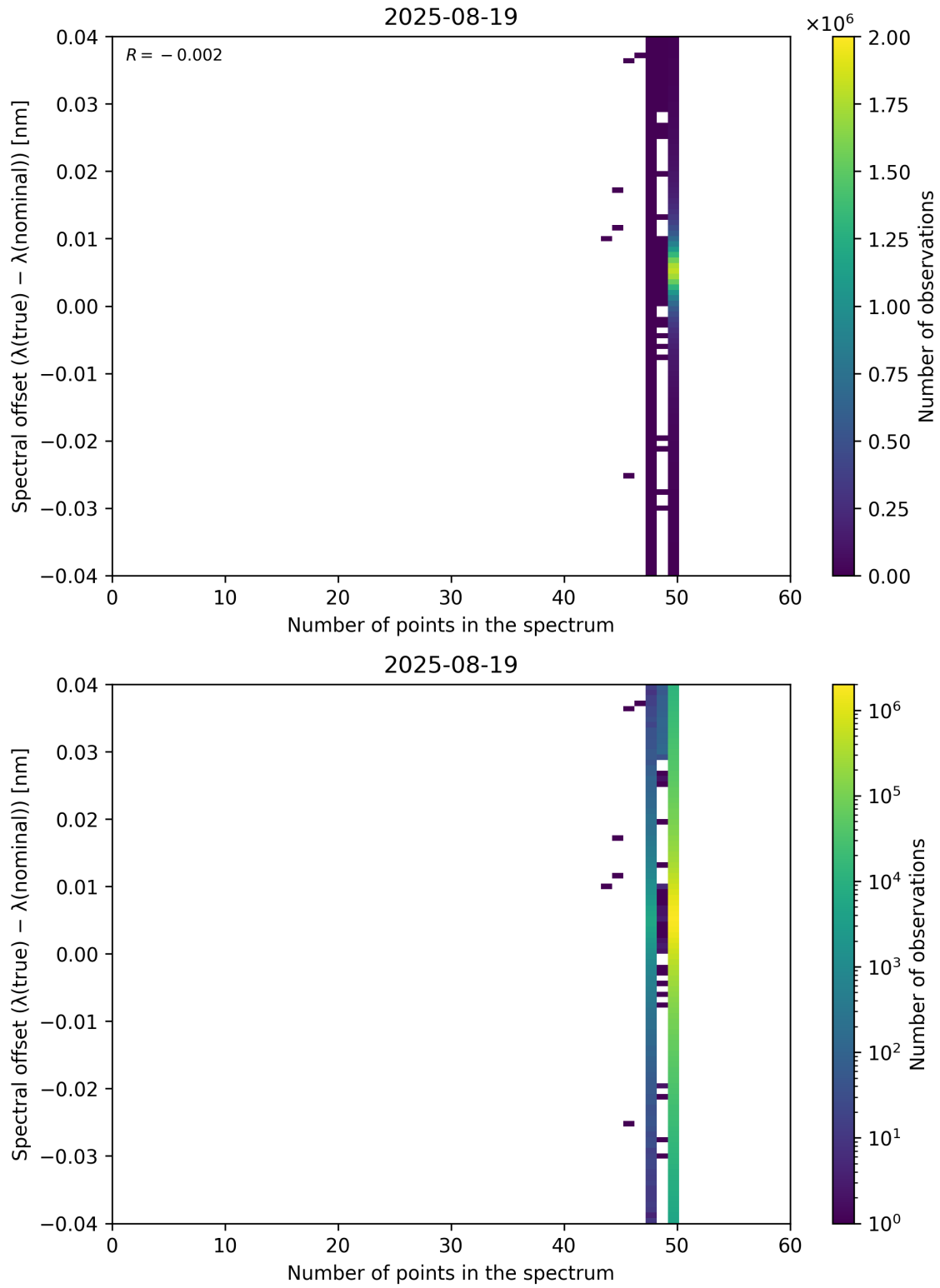
Figure 101: Scatter density plot of “Number of points in the spectrum” against “Spectral offset ( \lambda_{\text{true}} - \lambda_{\text{nominal}} )” for 2025-08-19 to 2025-08-20.
