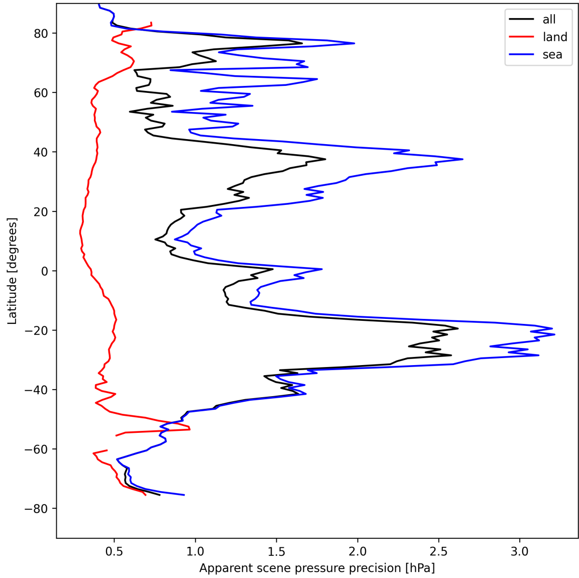
Figure 20: Zonal average of “Apparent scene pressure precision” for 2025-08-19 to 2025-08-20.
