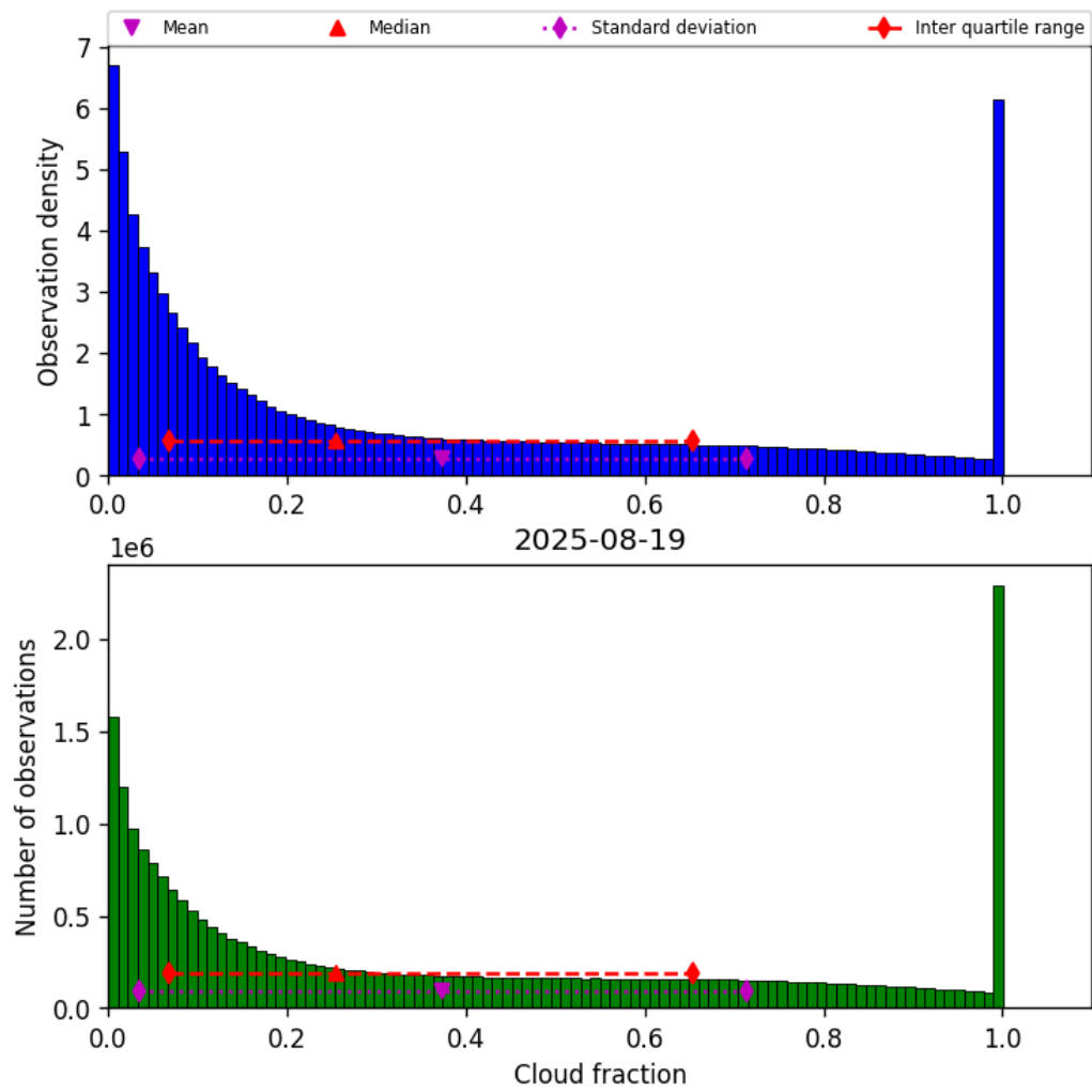
Figure 32: Histogram of “Cloud fraction” for 2025-08-19 to 2025-08-20
