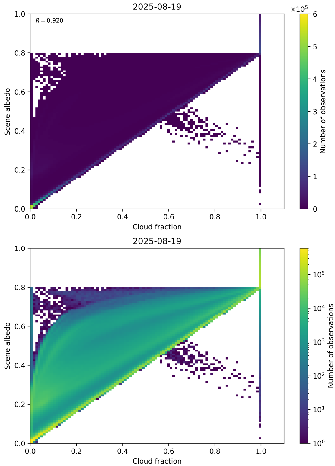
Figure 75: Scatter density plot of “Cloud fraction” against “Scene albedo” for 2025-08-19 to 2025-08-20.
