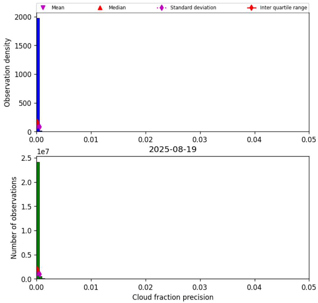
Figure 33: Histogram of “Cloud fraction precision” for 2025-08-19 to 2025-08-20
