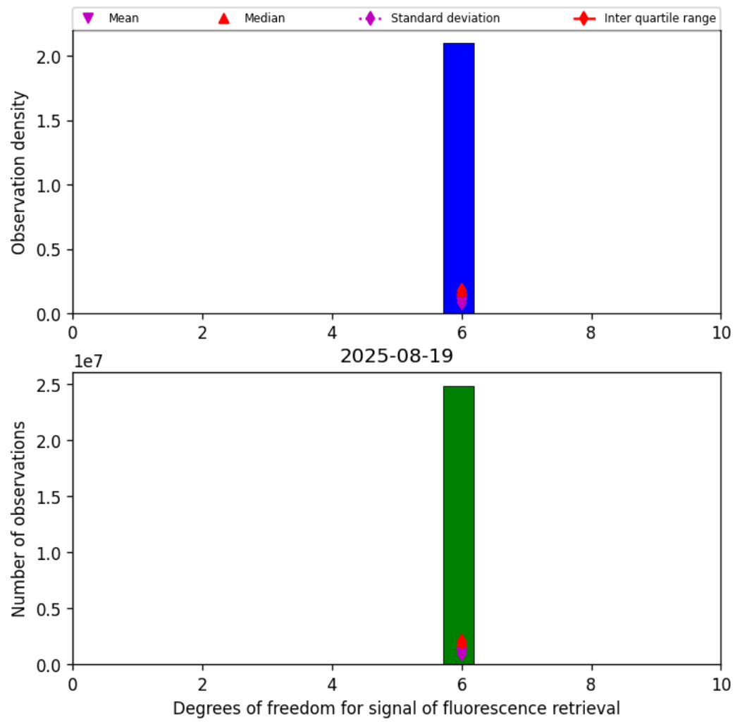
Figure 43: Histogram of “Degrees of freedom for signal of fluorescence retrieval” for 2025-08-19 to 2025-08-20
