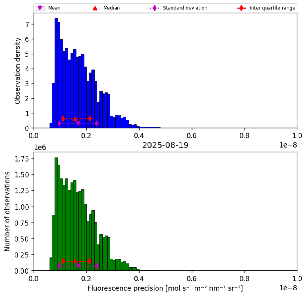
Figure 41: Histogram of “Fluorescence precision” for 2025-08-19 to 2025-08-20
