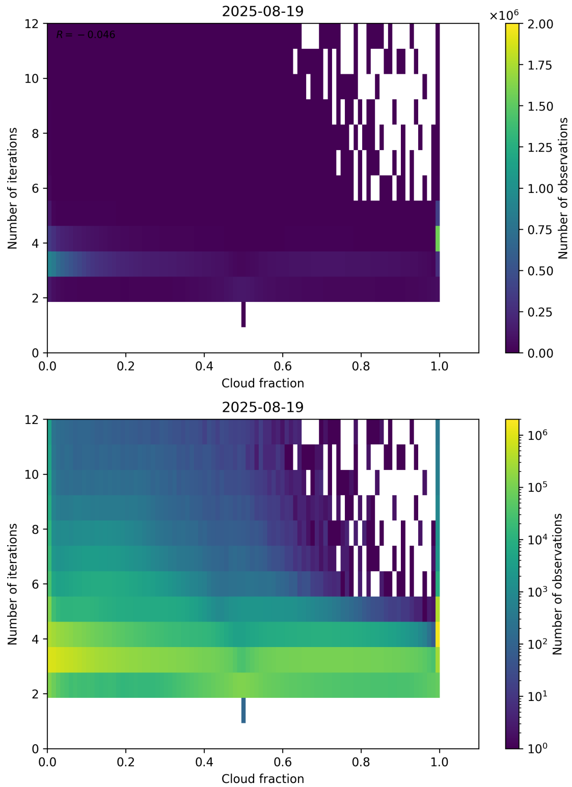
Figure 73: Scatter density plot of “Cloud fraction” against “Number of iterations” for 2025-08-19 to 2025-08-20.
