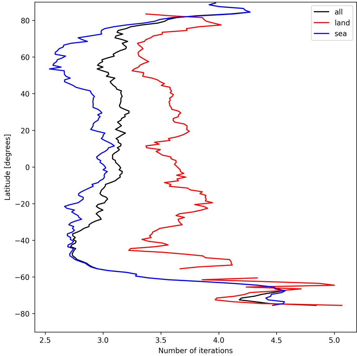
Figure 22: Zonal average of “Number of iterations” for 2025-08-19 to 2025-08-20.
