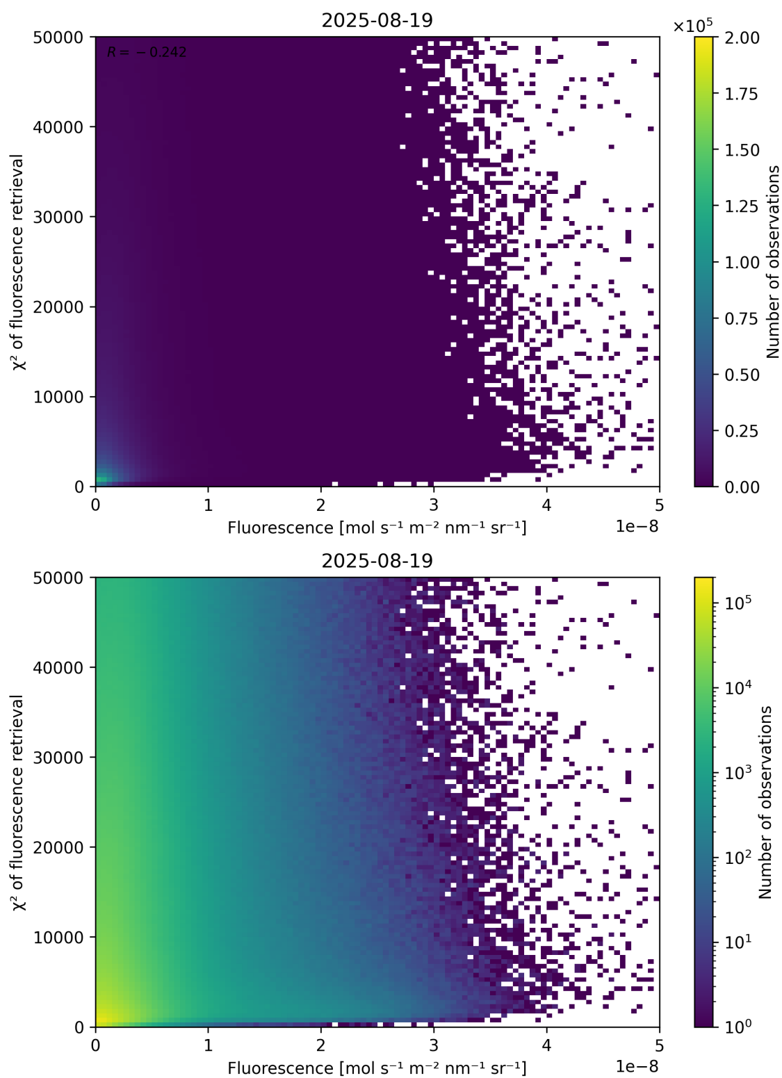
Figure 85: Scatter density plot of “Fluorescence” against “ \chi^2 of fluorescence retrieval” for 2025-08-19 to 2025-08-20.
