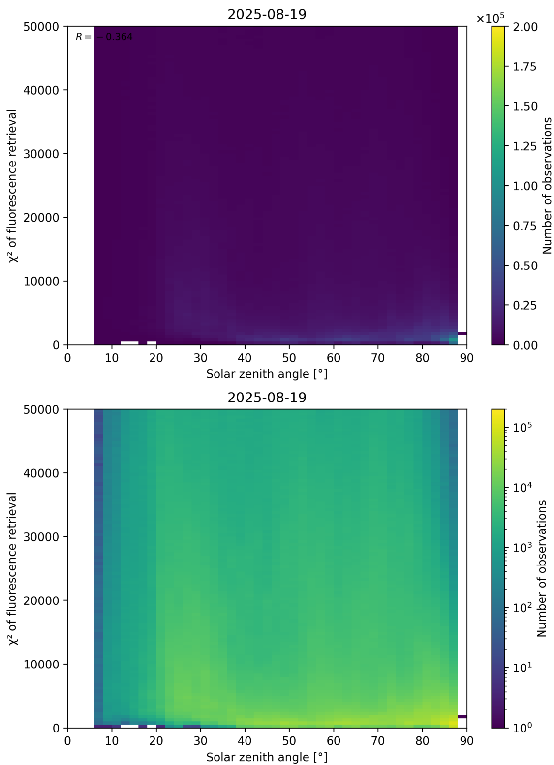
Figure 109: Scatter density plot of “Solar zenith angle” against “ \chi^2 of fluorescence retrieval” for 2025-08-19 to 2025-08-20.
