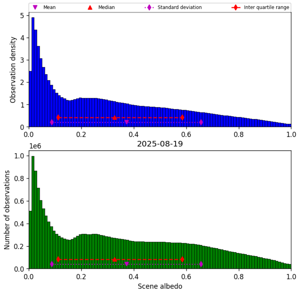
Figure 34: Histogram of “Scene albedo” for 2025-08-19 to 2025-08-20
