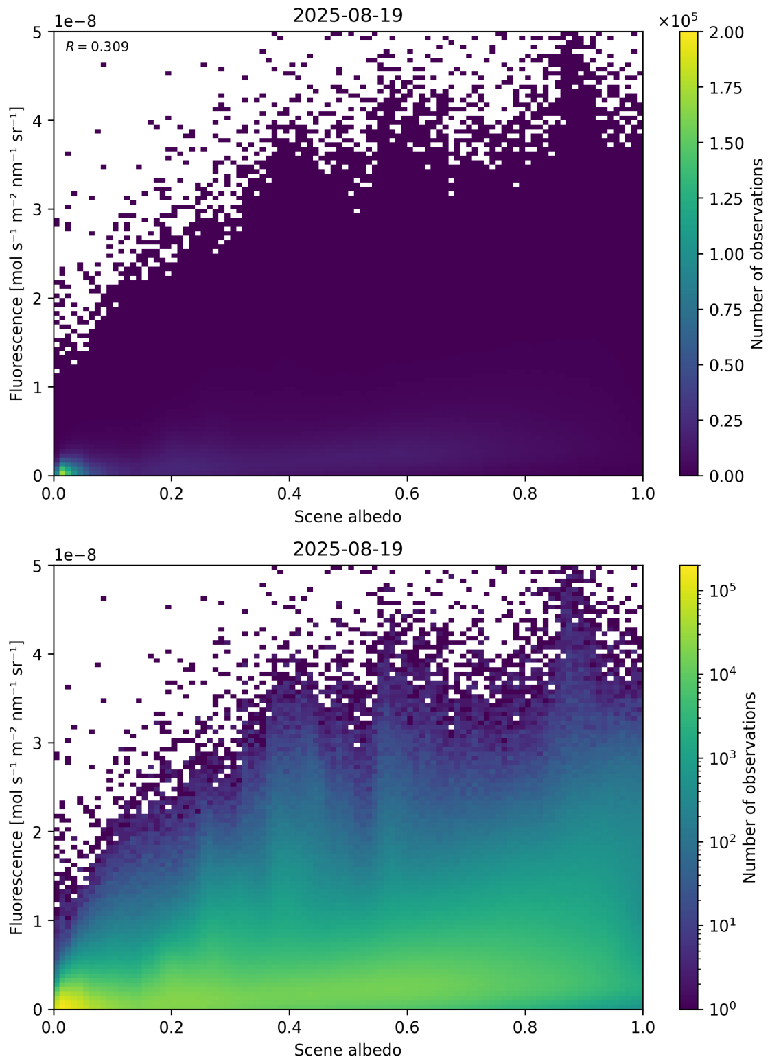
Figure 104: Scatter density plot of “Scene albedo” against “Fluorescence” for 2025-08-19 to 2025-08-20.
