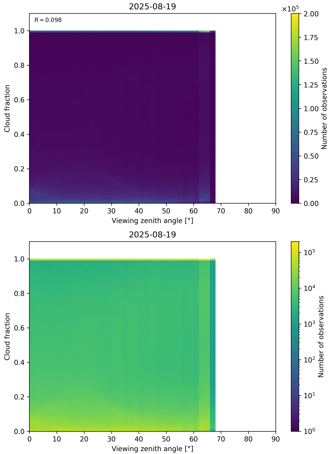
Figure 120: Scatter density plot of “Viewing zenith angle” against “Cloud fraction” for 2025-08-19 to 2025-08-20.
