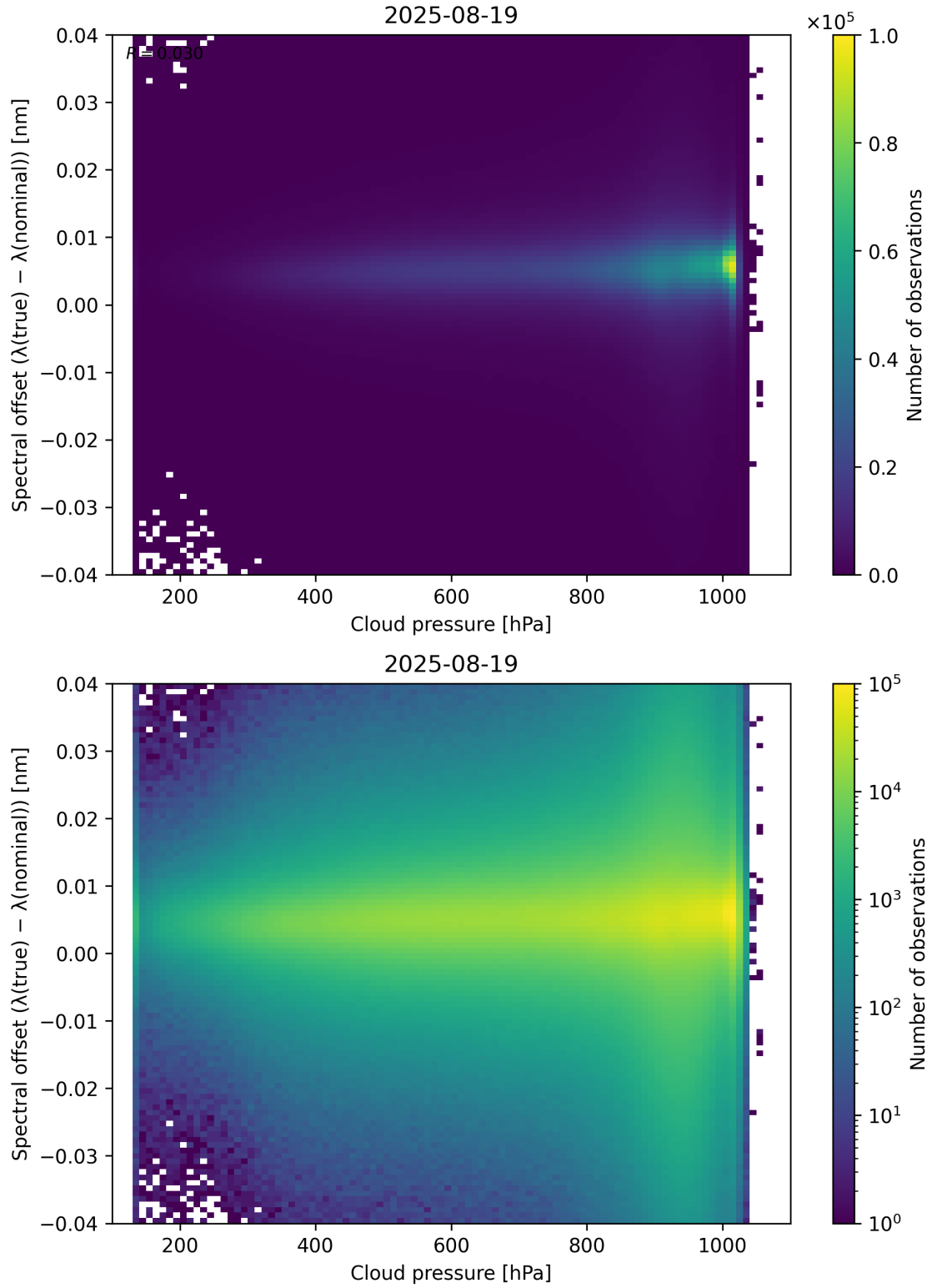
Figure 84: Scatter density plot of “Cloud pressure” against “Spectral offset ( \lambda_{\text{true}} - \lambda_{\text{nominal}} )” for 2025-08-19 to 2025-08-20.
