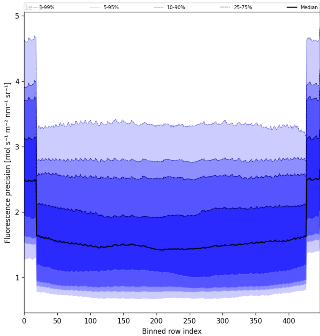
Figure 58: Along track statistics of “Fluorescence precision” for 2025-08-19 to 2025-08-20
