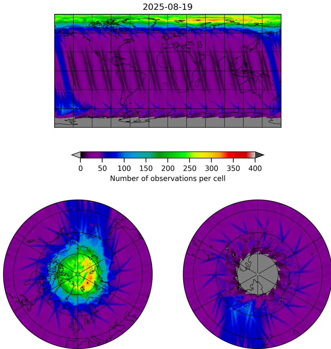
Figure 11: Map of the number of observations for 2025-08-19 to 2025-08-20
