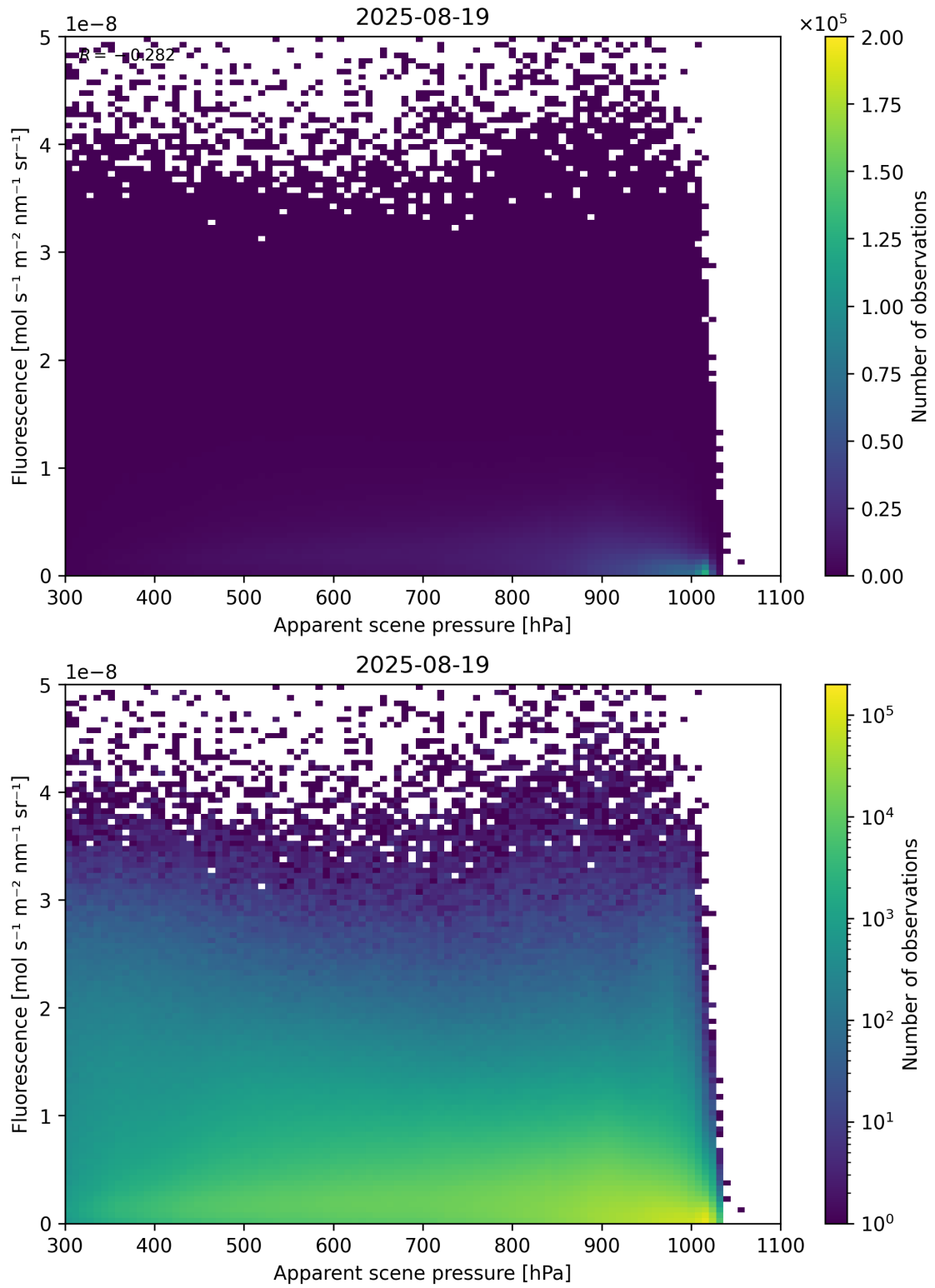
Figure 64: Scatter density plot of “Apparent scene pressure” against “Fluorescence” for 2025-08-19 to 2025-08-20.
