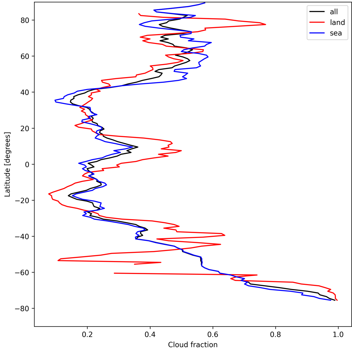
Figure 15: Zonal average of “Cloud fraction” for 2025-08-19 to 2025-08-20.
