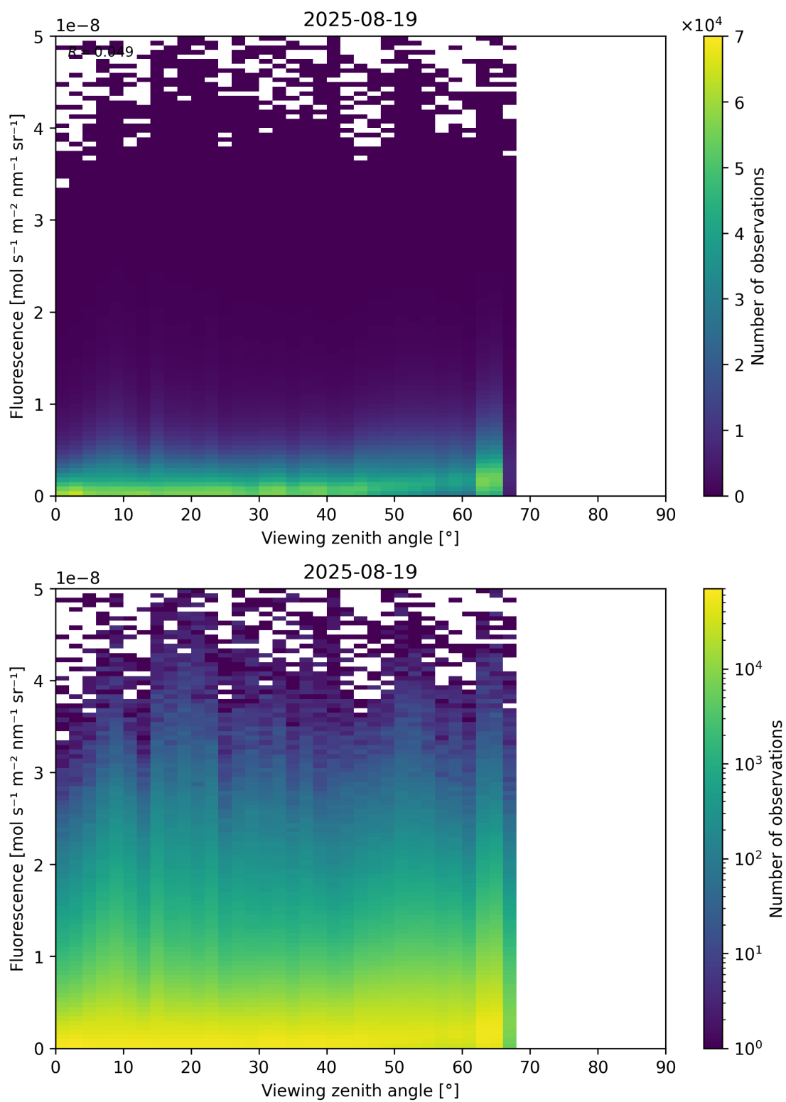
Figure 122: Scatter density plot of “Viewing zenith angle” against “Fluorescence” for 2025-08-19 to 2025-08-20.
