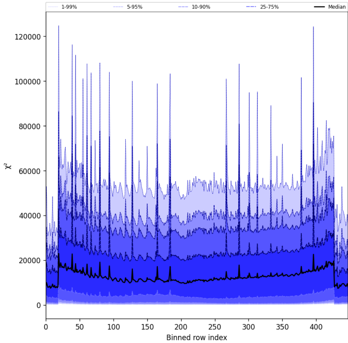
Figure 55: Along track statistics of “ \chi^2 ” for 2025-08-19 to 2025-08-20
