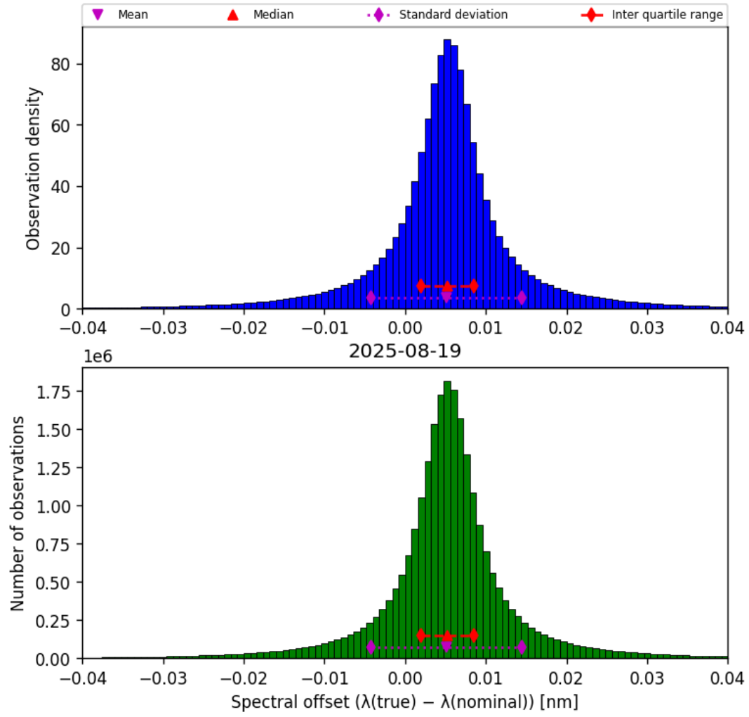
Figure 45: Histogram of “Spectral offset ( \lambda_{\text{true}} - \lambda_{\text{nominal}} )” for 2025-08-19 to 2025-08-20
