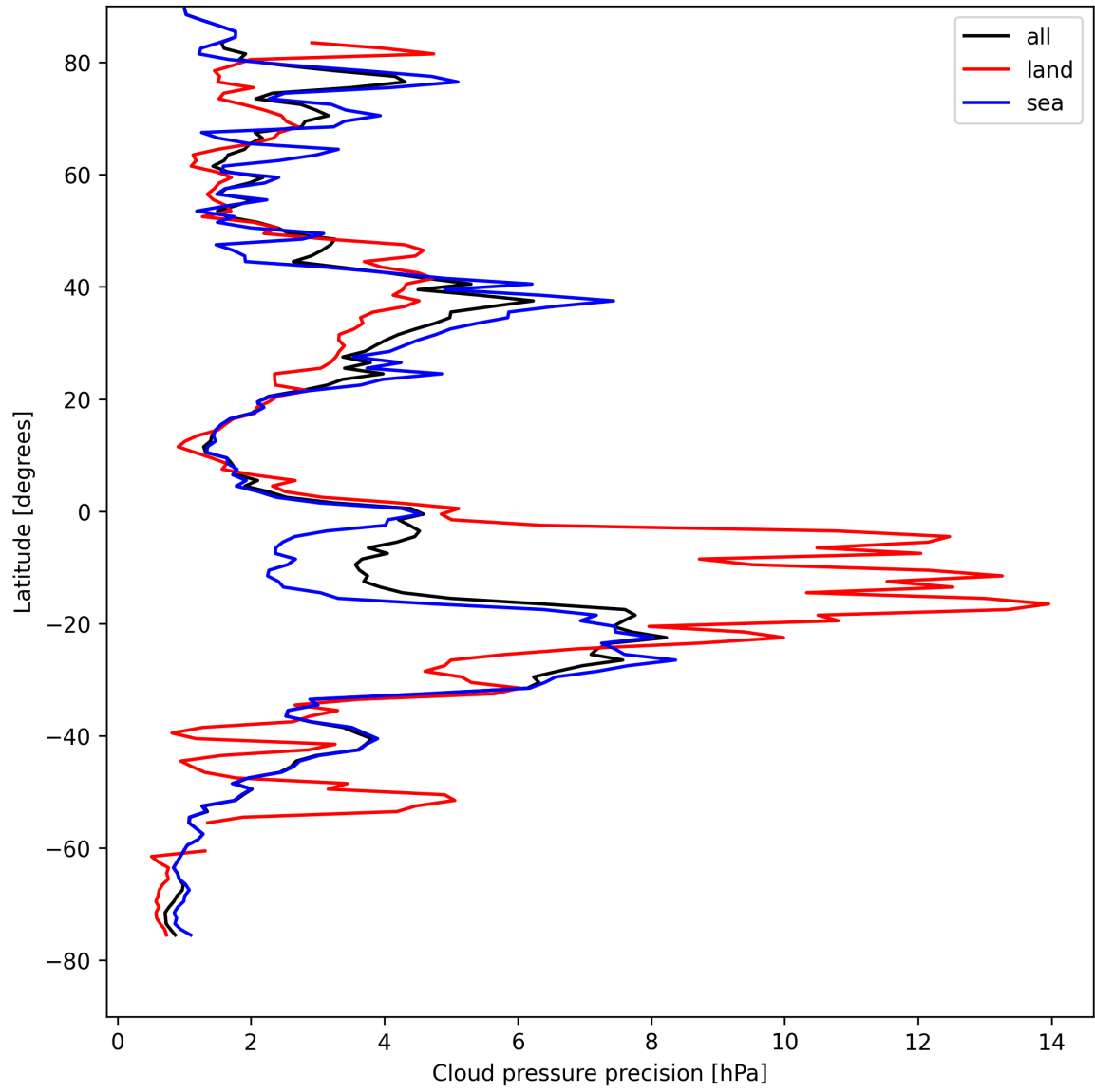
Figure 14: Zonal average of "Cloud pressure precision" for 2025-08-19 to 2025-08-20.
