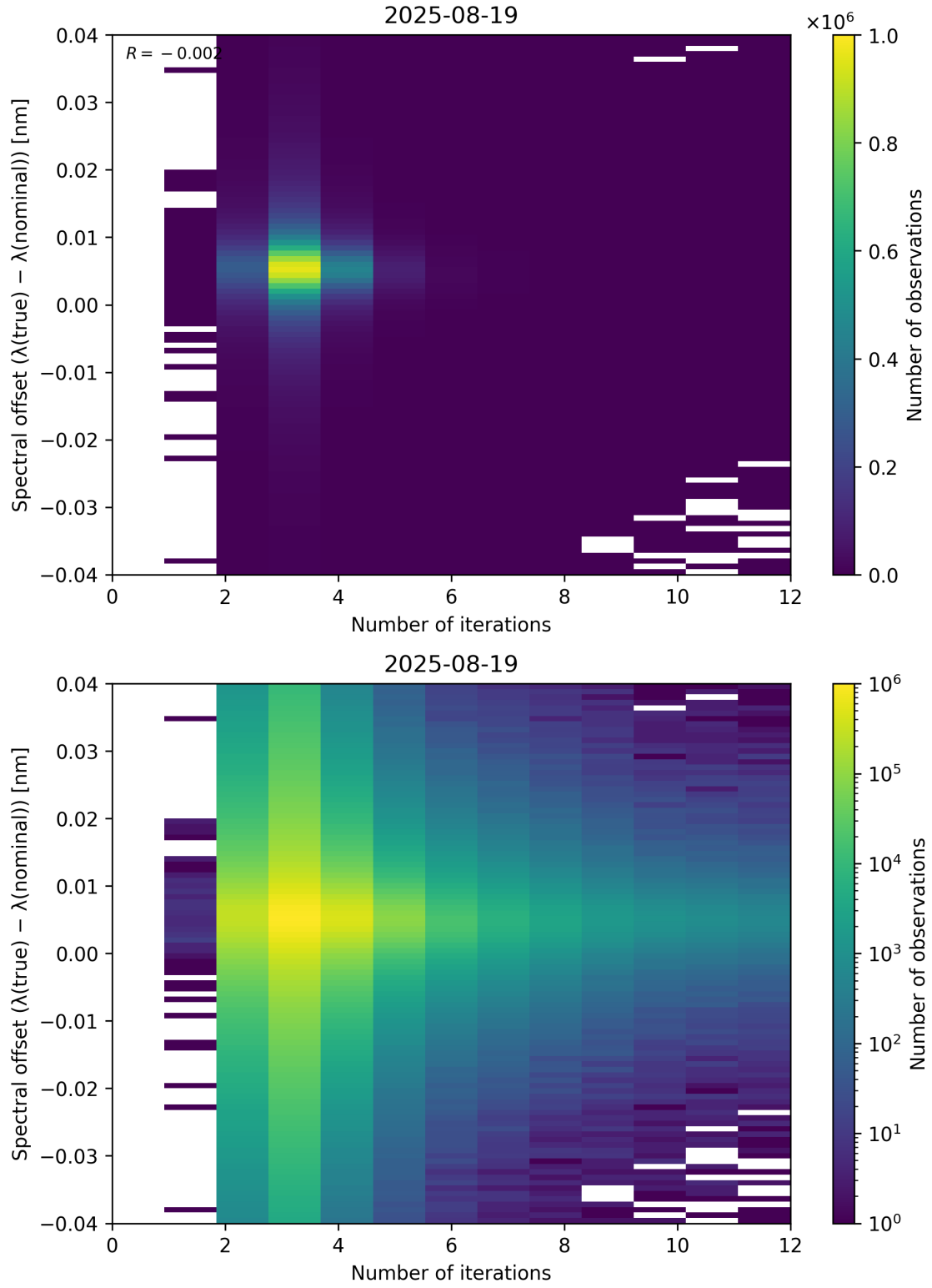
Figure 100: Scatter density plot of “Number of iterations” against “Spectral offset ( \lambda_{\text{true}} - \lambda_{\text{nominal}} )” for 2025-08-19 to 2025-08-20.
