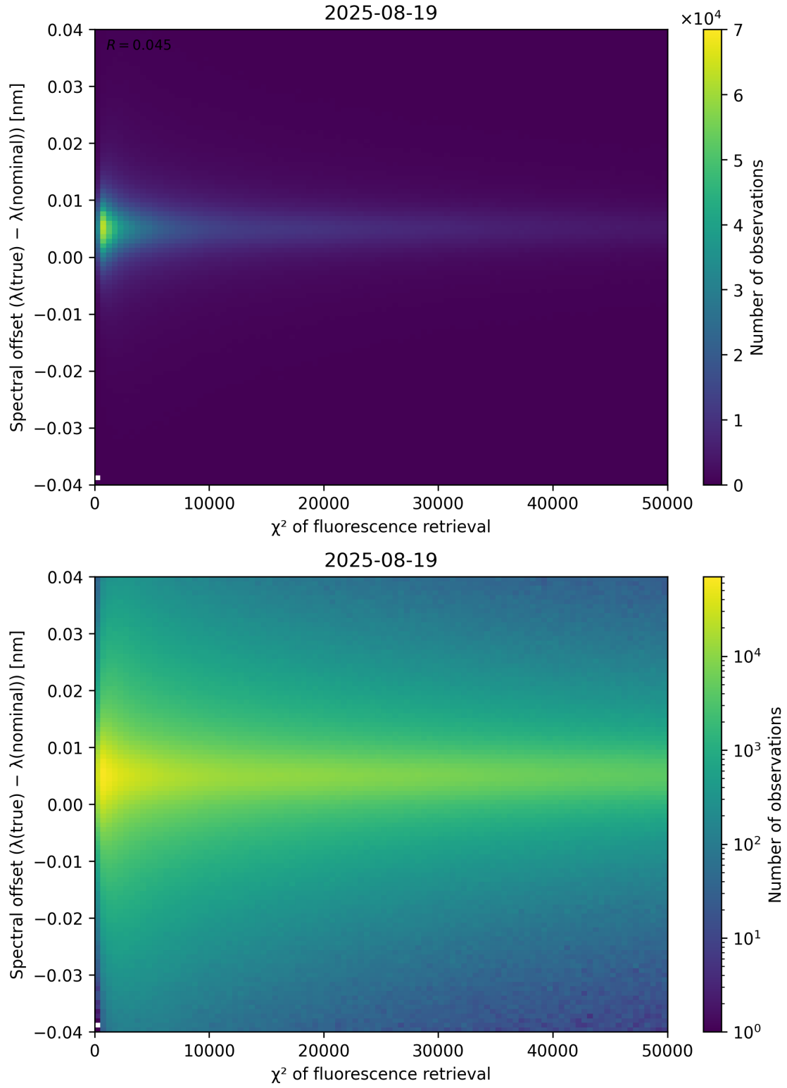
Figure 69: Scatter density plot of “ \chi^2 of fluorescence retrieval” against “Spectral offset ( \lambda_{\text{true}} - \lambda_{\text{nominal}} )” for 2025-08-19 to 2025-08-20.
