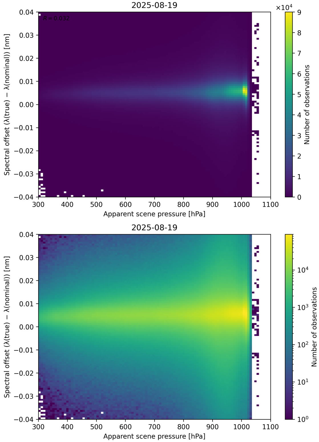
Figure 67: Scatter density plot of “Apparent scene pressure” against “Spectral offset ( \lambda_{\text{true}} - \lambda_{\text{nominal}} )” for 2025-08-19 to 2025-08-20.
