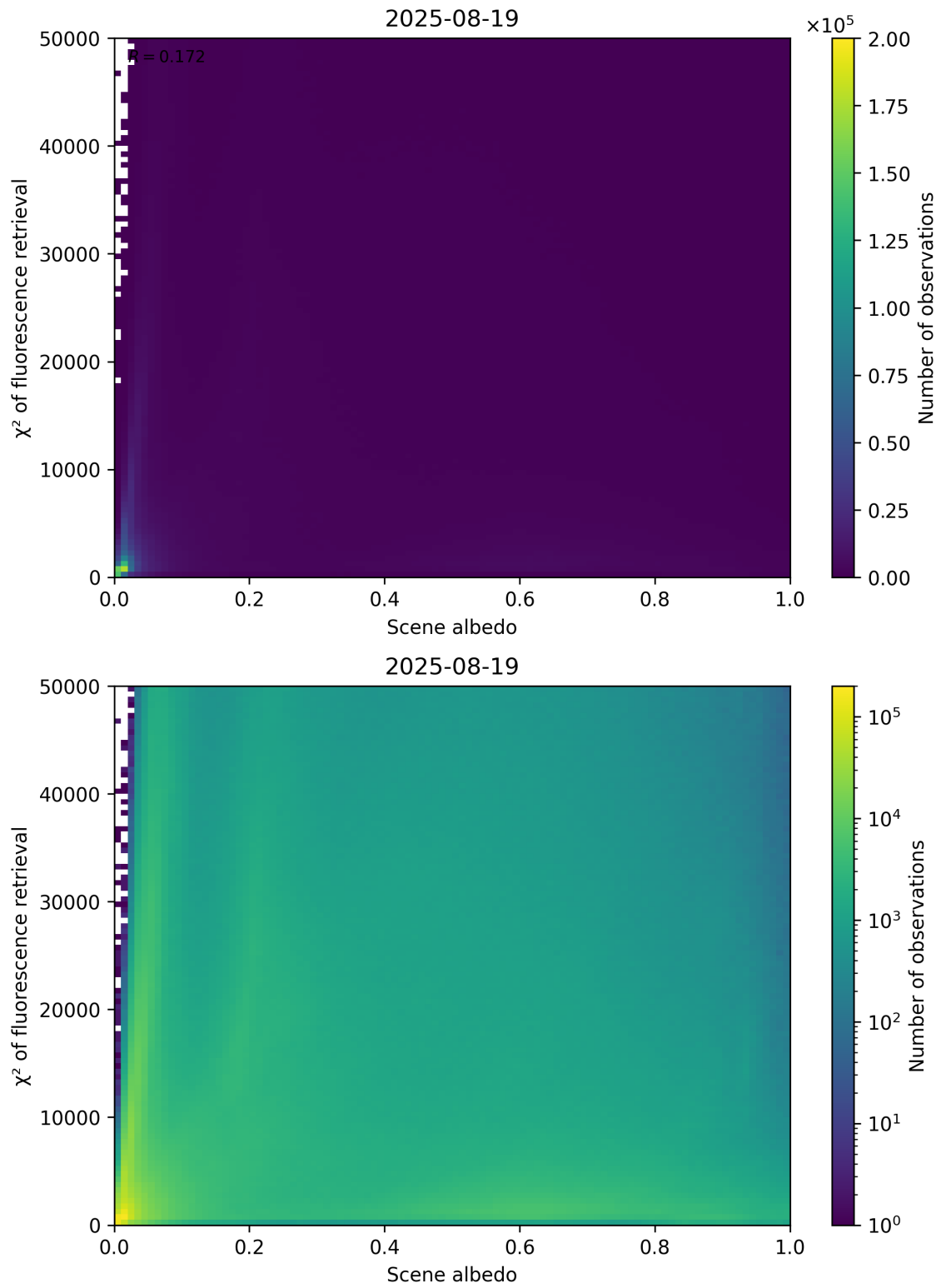
Figure 103: Scatter density plot of “Scene albedo” against “ \chi^2 of fluorescence retrieval” for 2025-08-19 to 2025-08-20.
