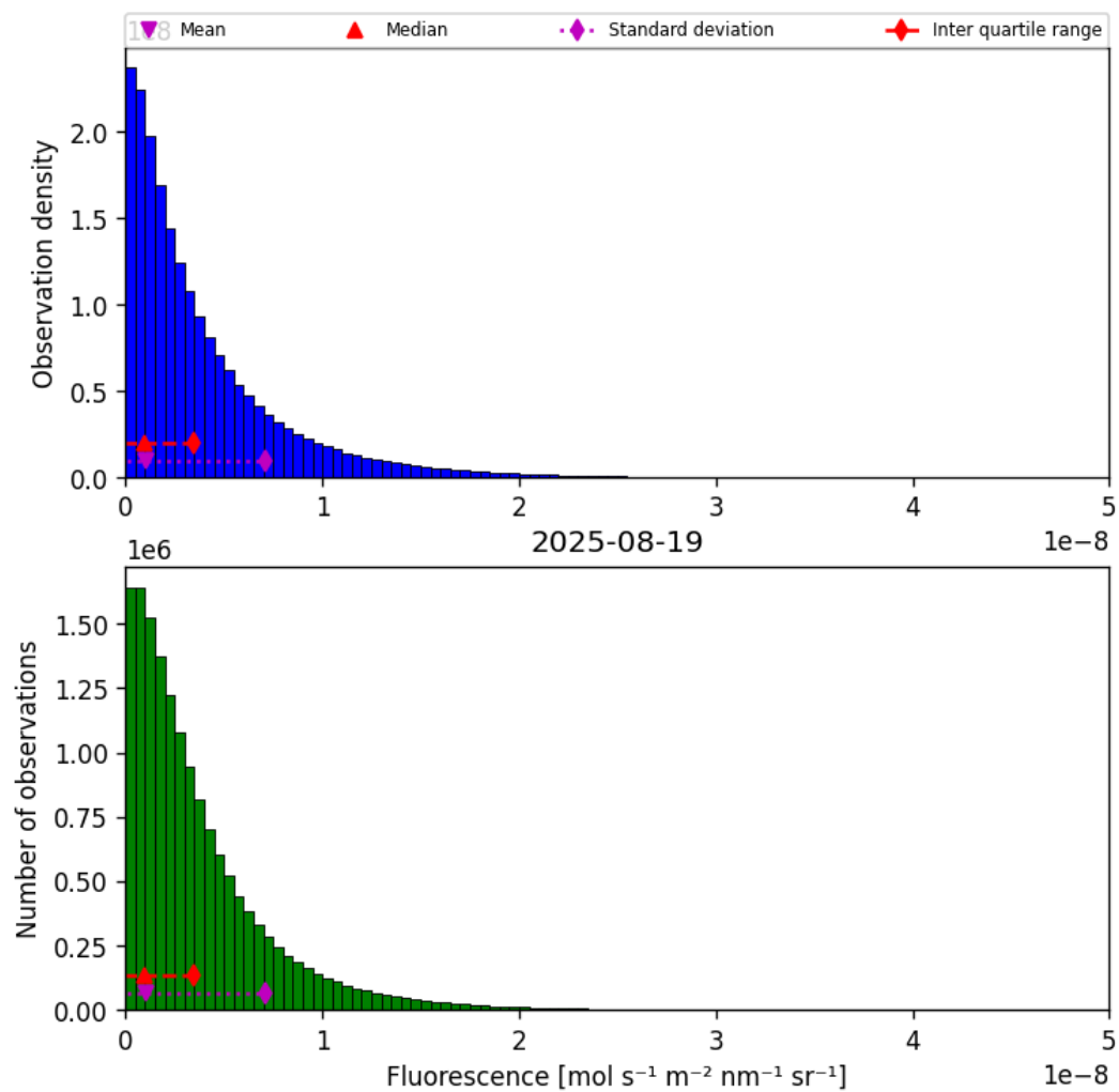
Figure 40: Histogram of “Fluorescence” for 2025-08-19 to 2025-08-20
