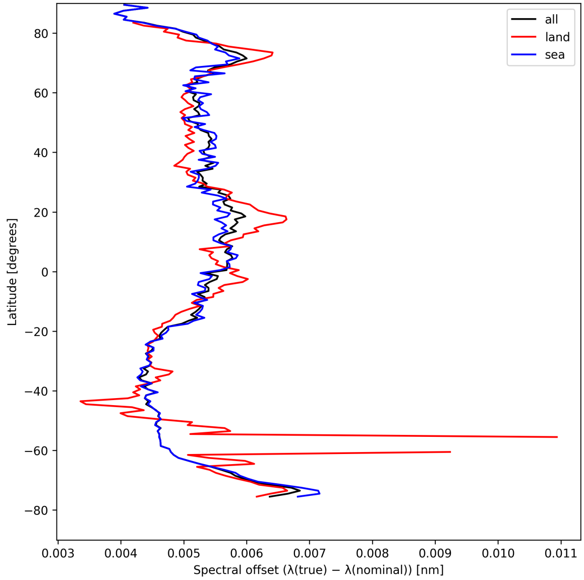
Figure 28: Zonal average of “Spectral offset ( \lambda_{\text{true}} - \lambda_{\text{nominal}} )” for 2025-08-19 to 2025-08-20.
