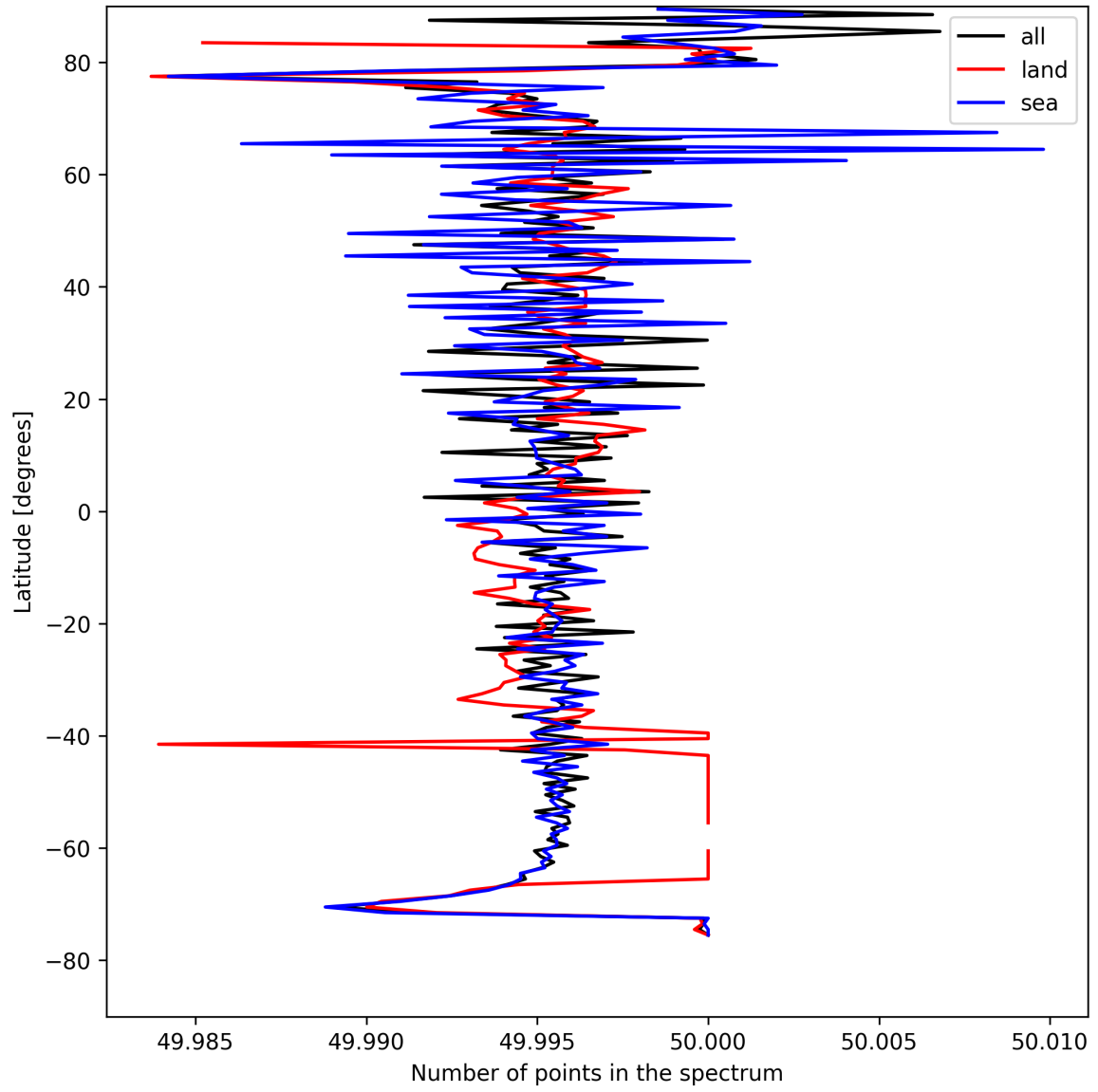
Figure 27: Zonal average of “Number of points in the spectrum” for 2025-08-19 to 2025-08-20.
