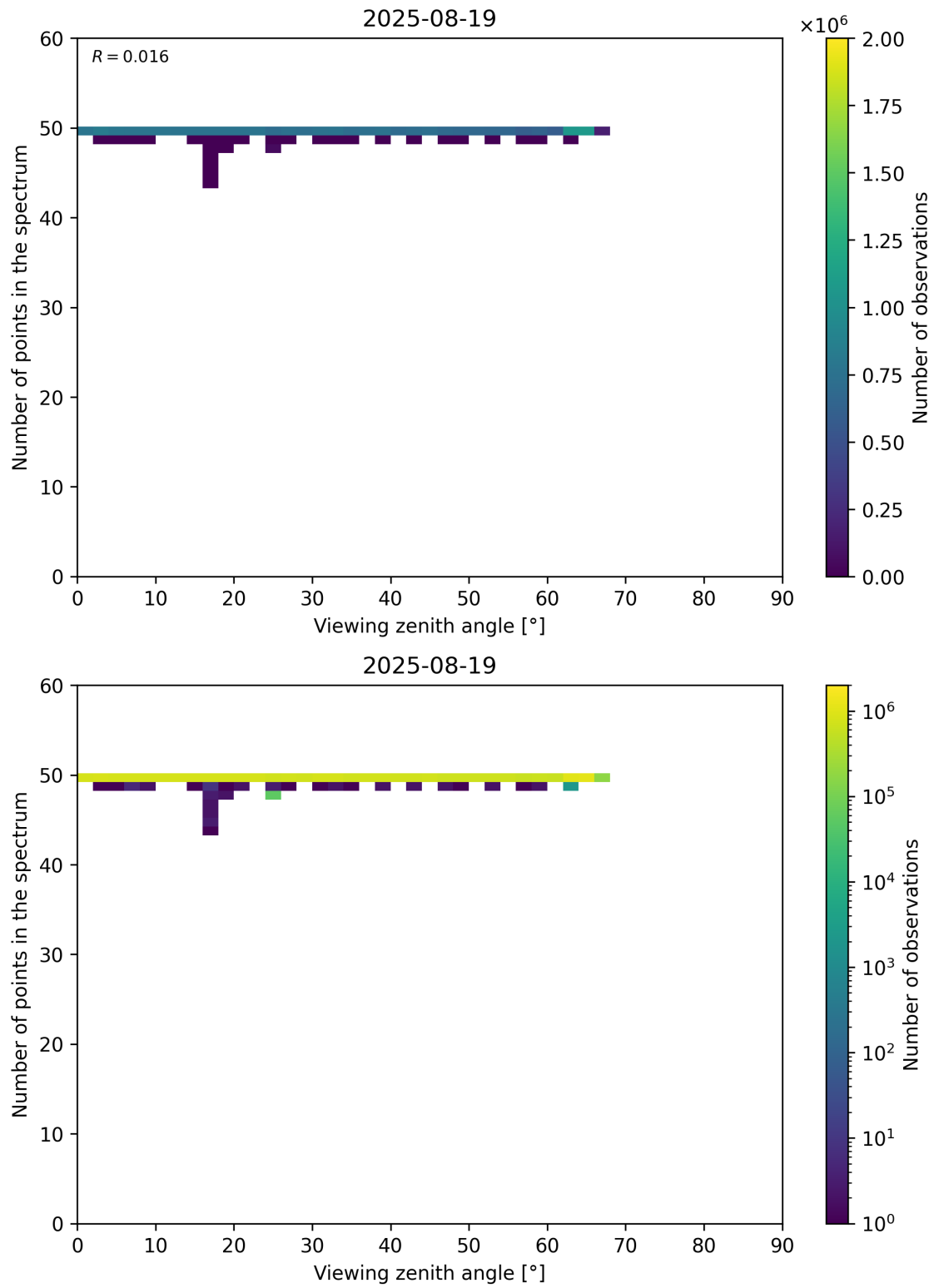
Figure 125: Scatter density plot of “Viewing zenith angle” against “Number of points in the spectrum” for 2025-08-19 to 2025-08-20.
