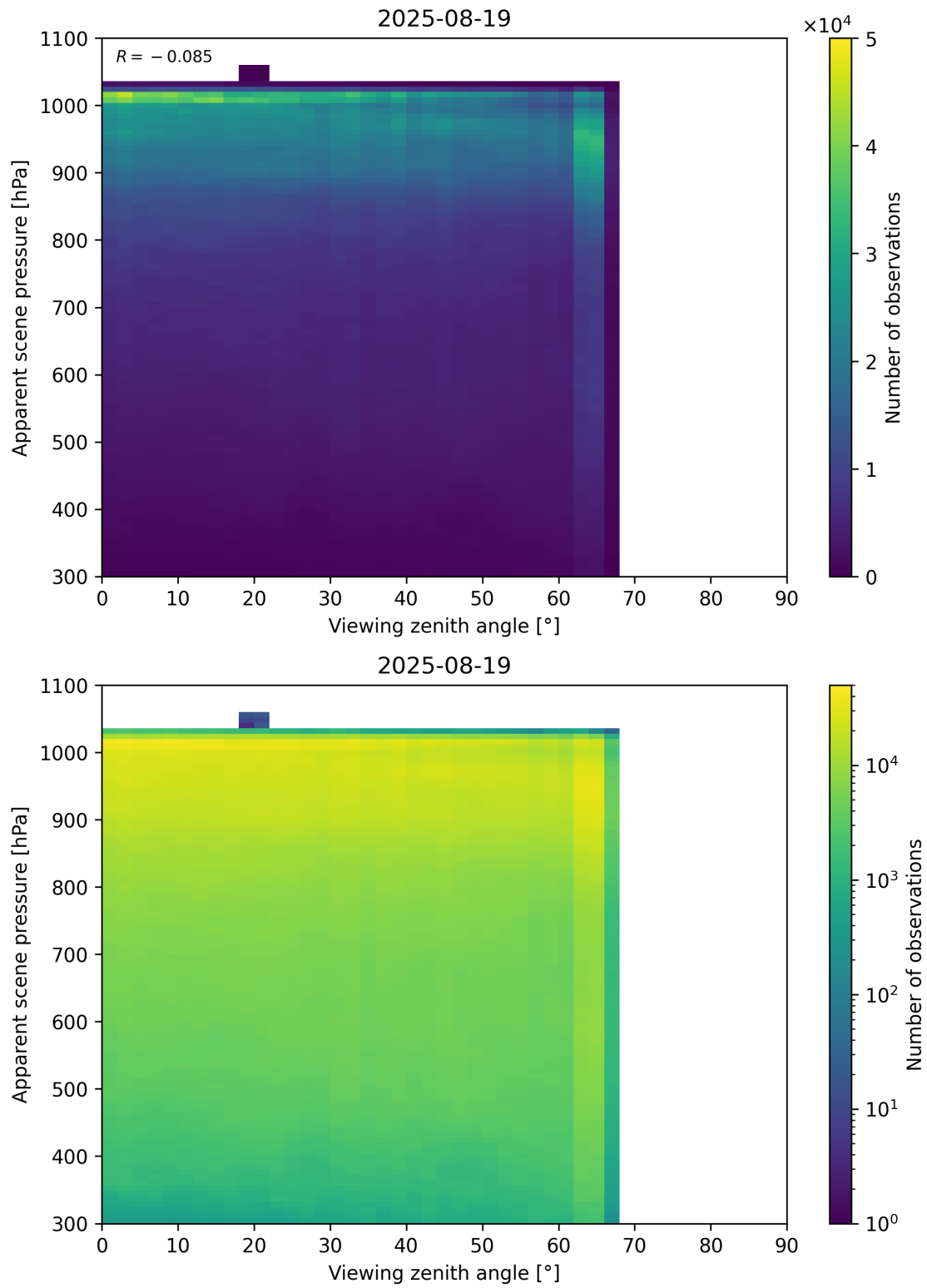
Figure 118: Scatter density plot of “Viewing zenith angle” against “Apparent scene pressure” for 2025-08-19 to 2025-08-20.
