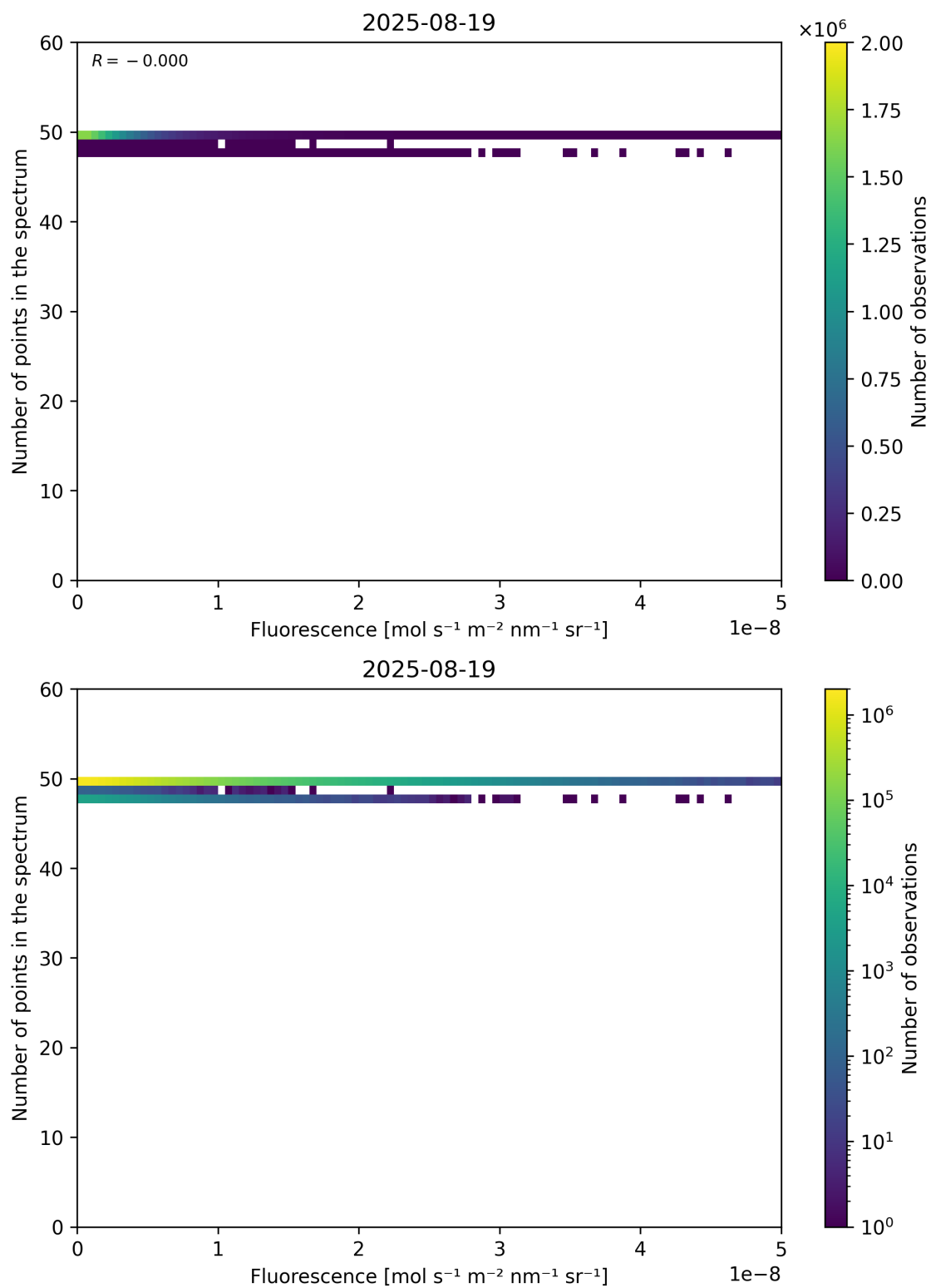
Figure 86: Scatter density plot of “Fluorescence” against “Number of points in the spectrum” for 2025-08-19 to 2025-08-20.
