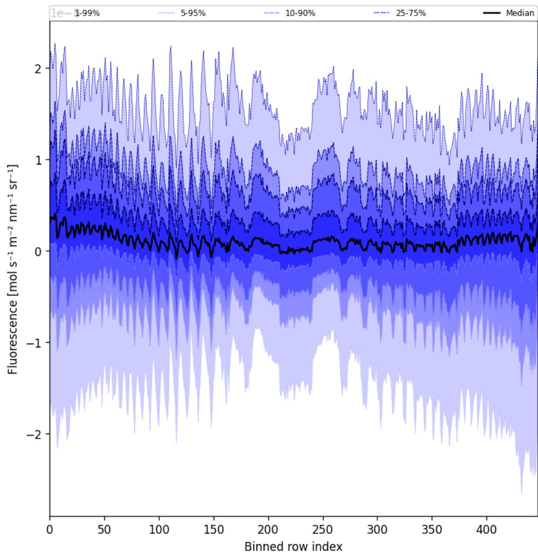
Figure 57: Along track statistics of “Fluorescence” for 2025-08-19 to 2025-08-20
