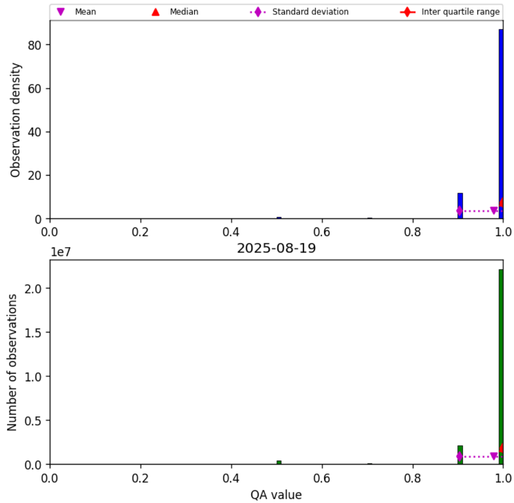
Figure 29: Histogram of “QA value” for 2025-08-19 to 2025-08-20
