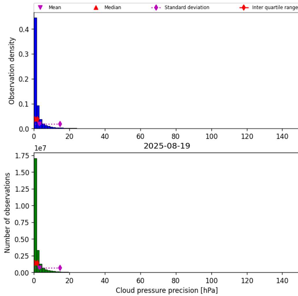
Figure 31: Histogram of “Cloud pressure precision” for 2025-08-19 to 2025-08-20
