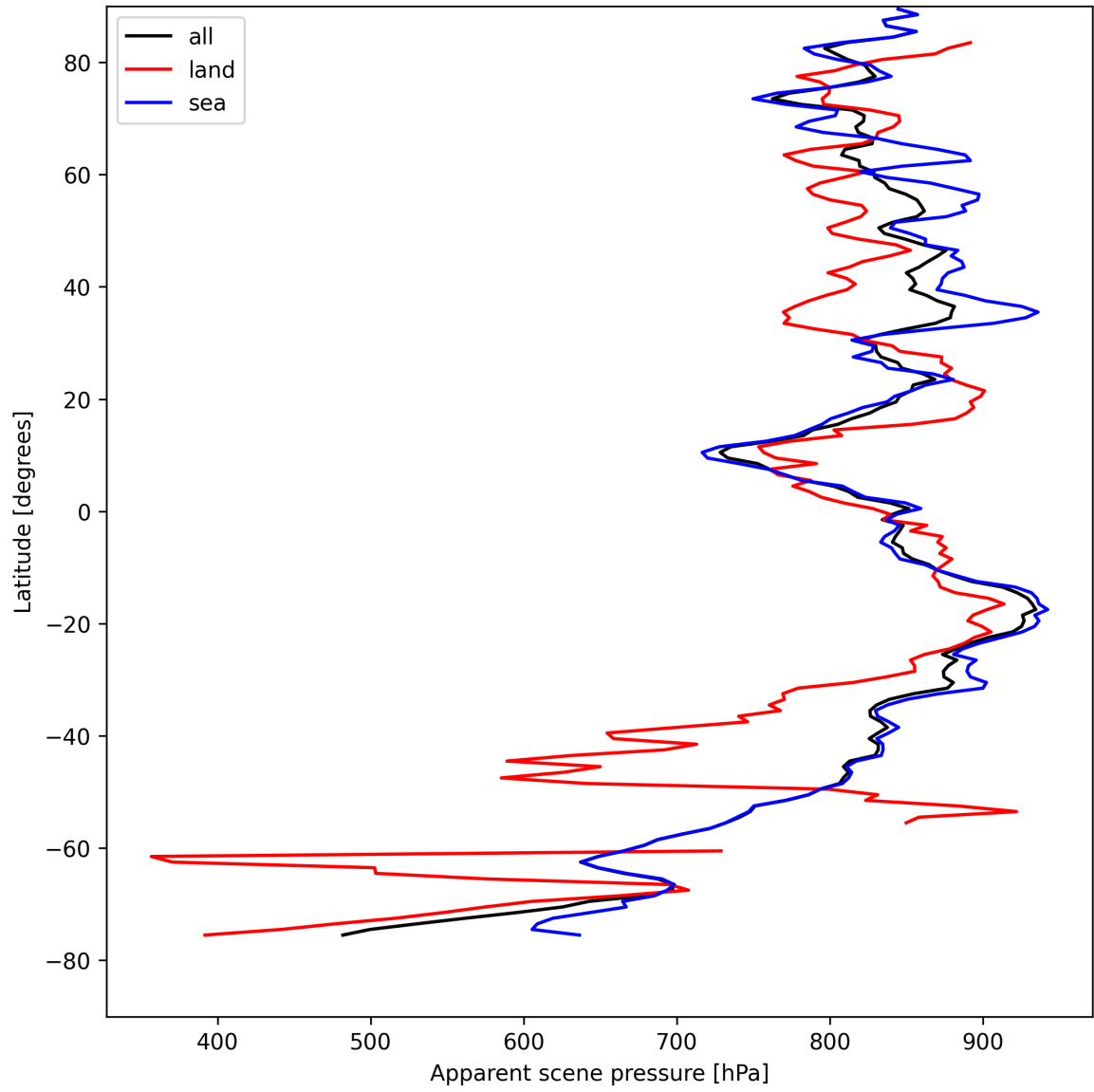
Figure 19: Zonal average of “Apparent scene pressure” for 2025-08-19 to 2025-08-20.
