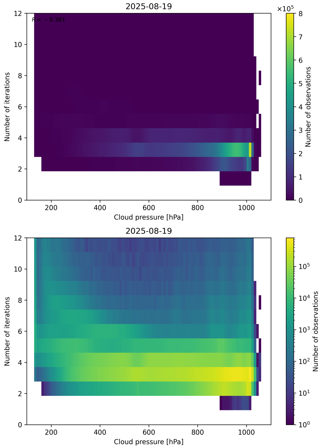
Figure 81: Scatter density plot of “Cloud pressure” against “Number of iterations” for 2025-08-19 to 2025-08-20.
