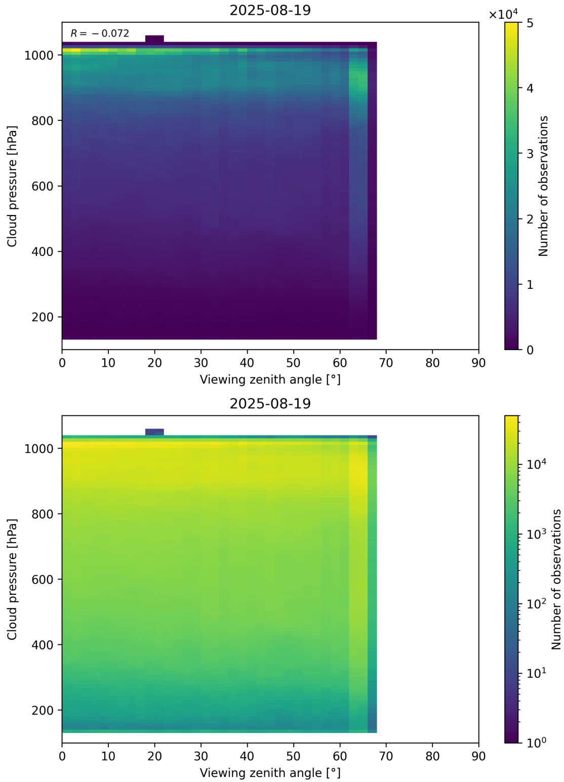
Figure 121: Scatter density plot of “Viewing zenith angle” against “Cloud pressure” for 2025-08-19 to 2025-08-20.
