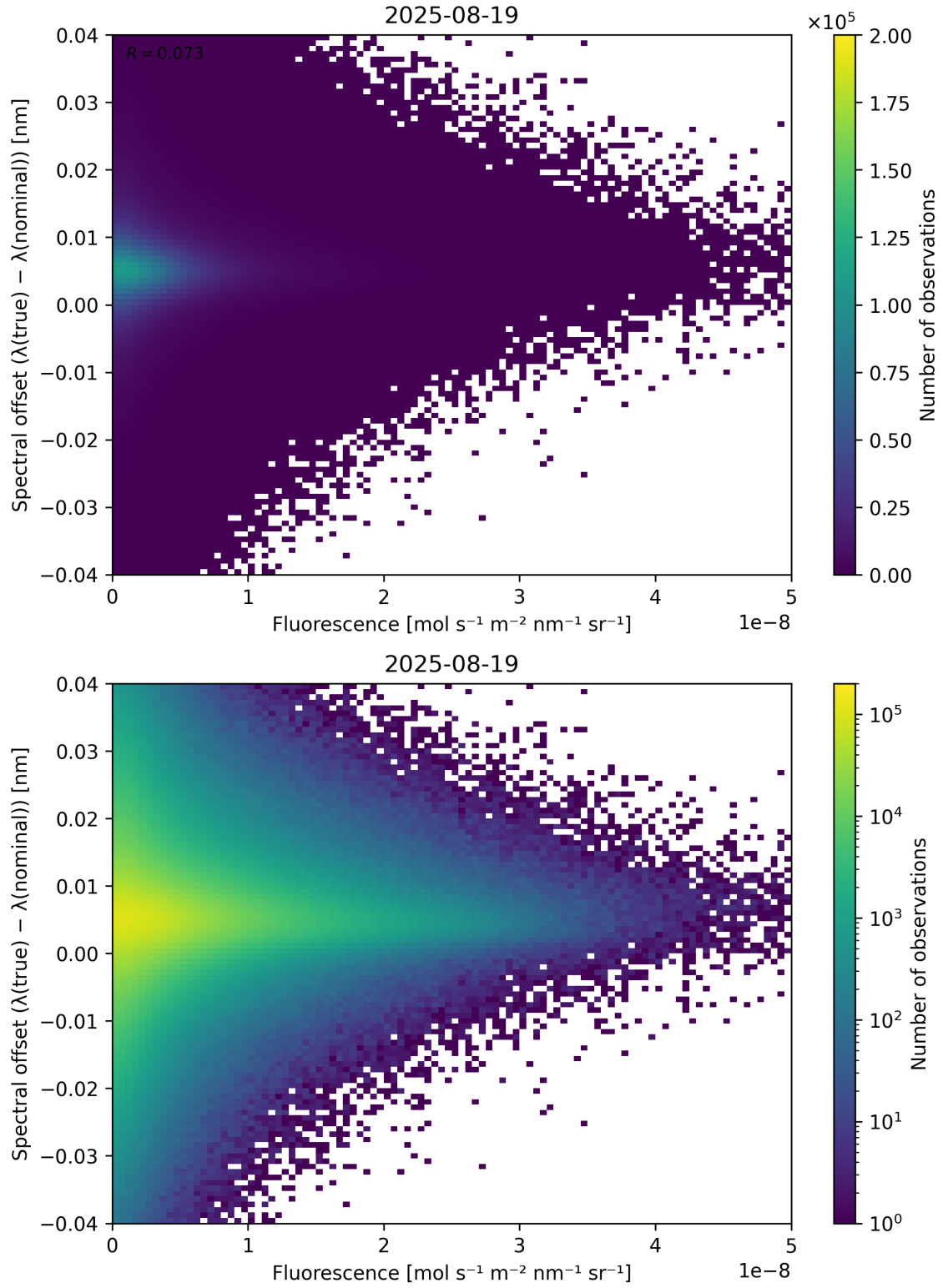
Figure 87: Scatter density plot of “Fluorescence” against “Spectral offset ( \lambda_{\text{true}} - \lambda_{\text{nominal}} )” for 2025-08-19 to 2025-08-20.
