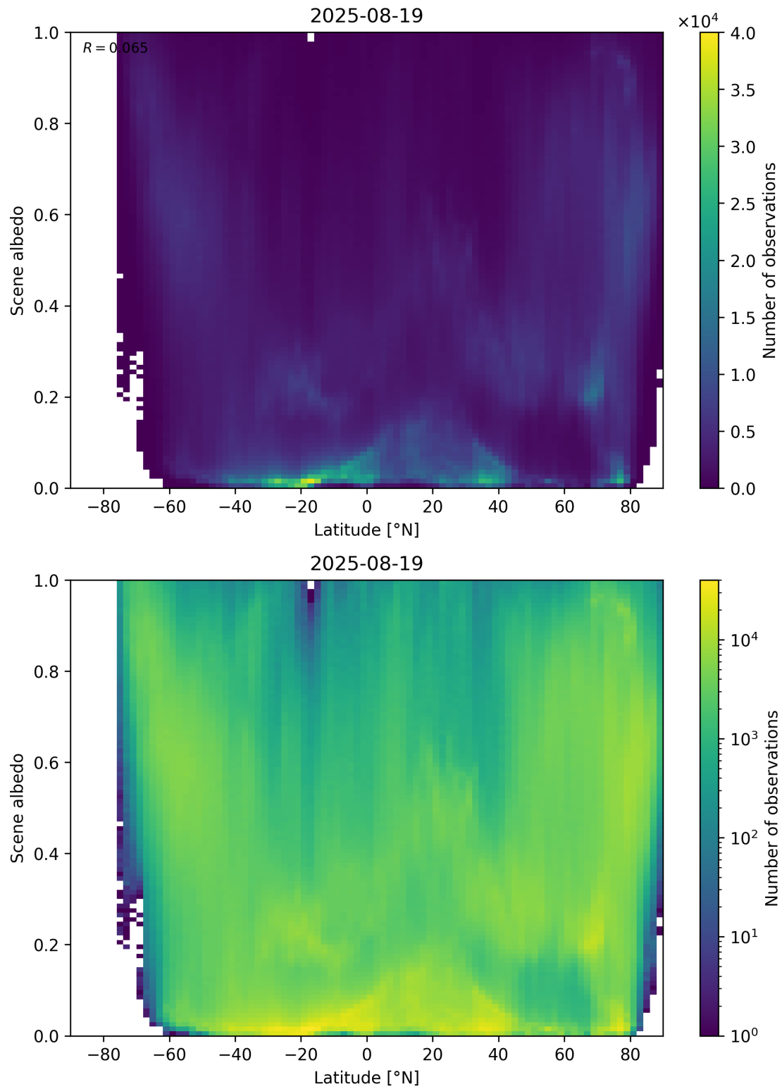
Figure 95: Scatter density plot of “Latitude” against “Scene albedo” for 2025-08-19 to 2025-08-20.
