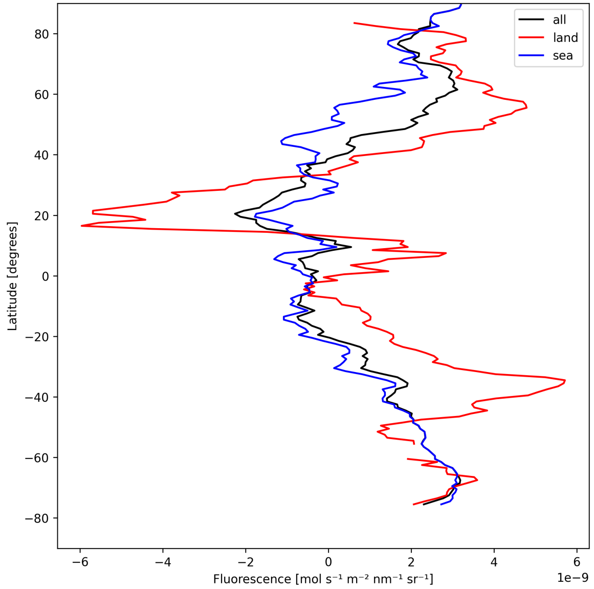
Figure 23: Zonal average of “Fluorescence” for 2025-08-19 to 2025-08-20.
