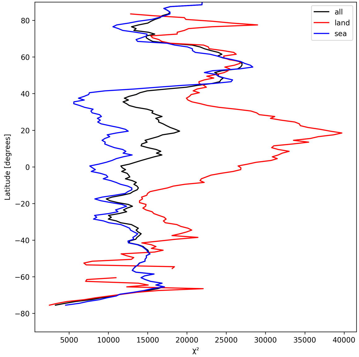
Figure 21: Zonal average of “ \chi^2 ” for 2025-08-19 to 2025-08-20.
