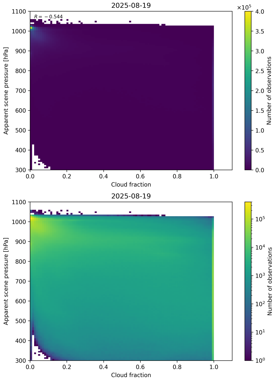
Figure 70: Scatter density plot of “Cloud fraction” against “Apparent scene pressure” for 2025-08-19 to 2025-08-20.
