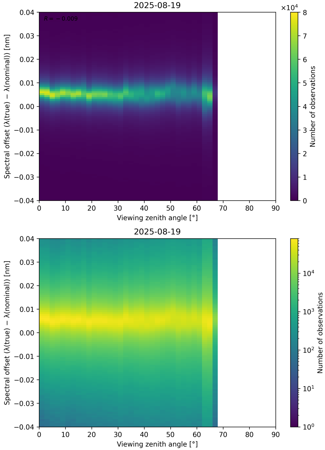
Figure 128: Scatter density plot of “Viewing zenith angle” against “Spectral offset ( \lambda_{\text{true}} - \lambda_{\text{nominal}} )” for 2025-08-19 to 2025-08-20.
