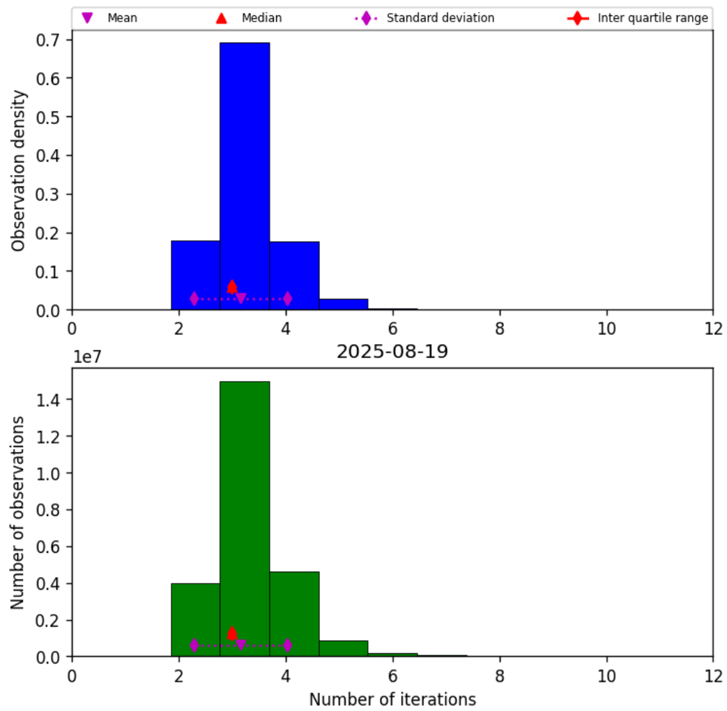
Figure 39: Histogram of “Number of iterations” for 2025-08-19 to 2025-08-20
