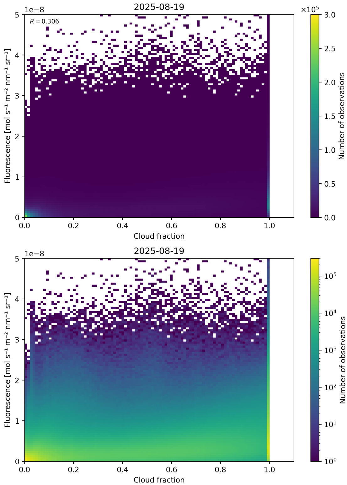
Figure 72: Scatter density plot of “Cloud fraction” against “Fluorescence” for 2025-08-19 to 2025-08-20.
