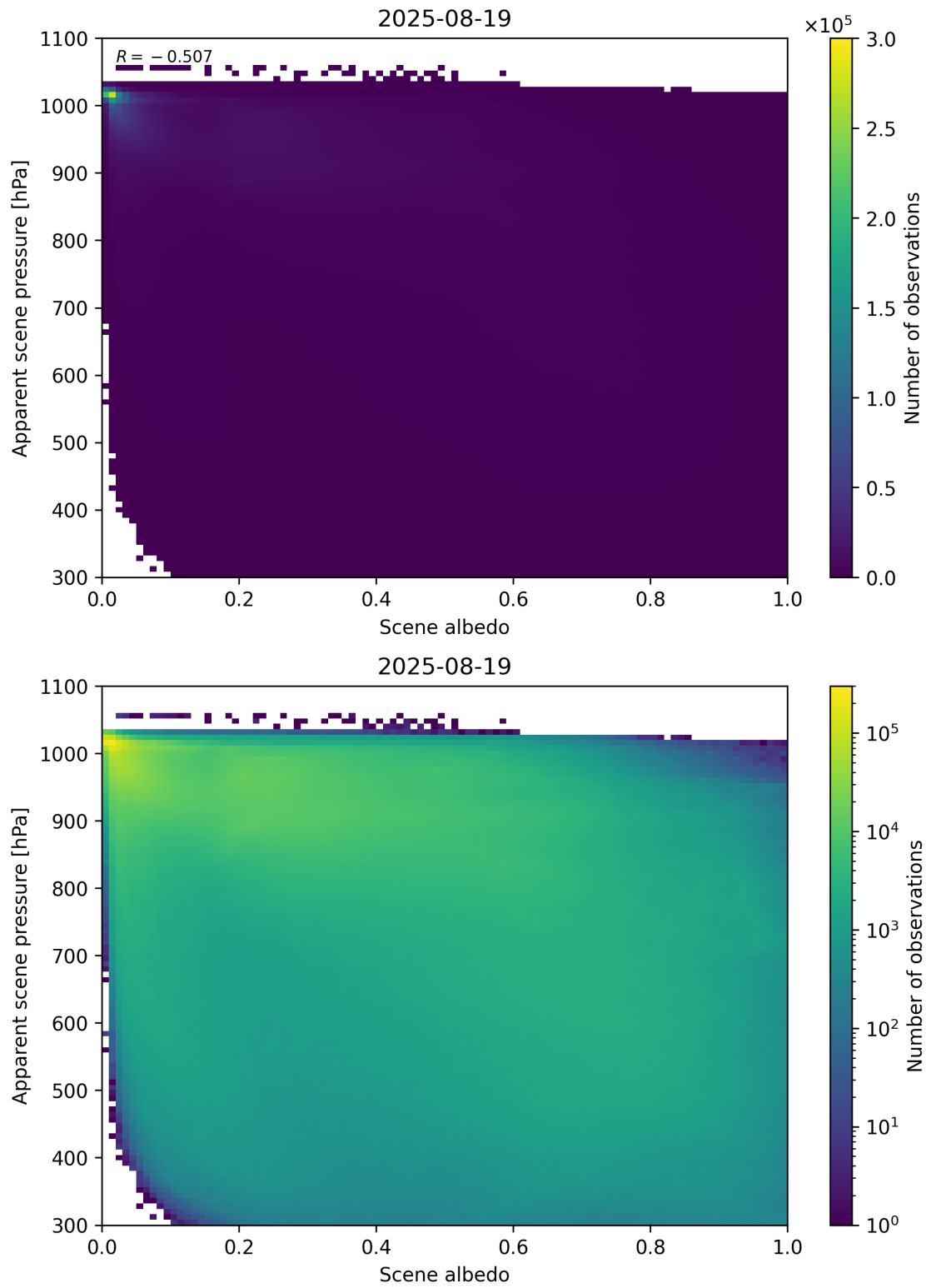
Figure 102: Scatter density plot of “Scene albedo” against “Apparent scene pressure” for 2025-08-19 to 2025-08-20.
