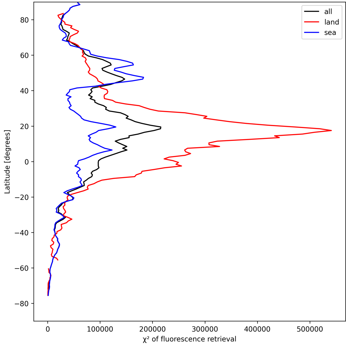
Figure 25: Zonal average of “ \chi^2 of fluorescence retrieval” for 2025-08-19 to 2025-08-20.
