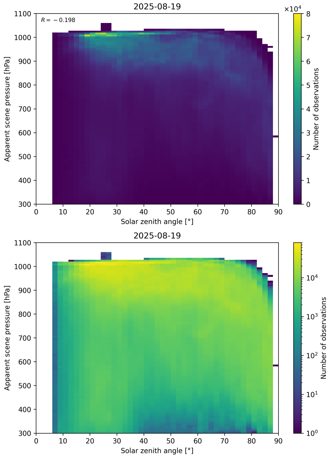
Figure 108: Scatter density plot of “Solar zenith angle” against “Apparent scene pressure” for 2025-08-19 to 2025-08-20.
