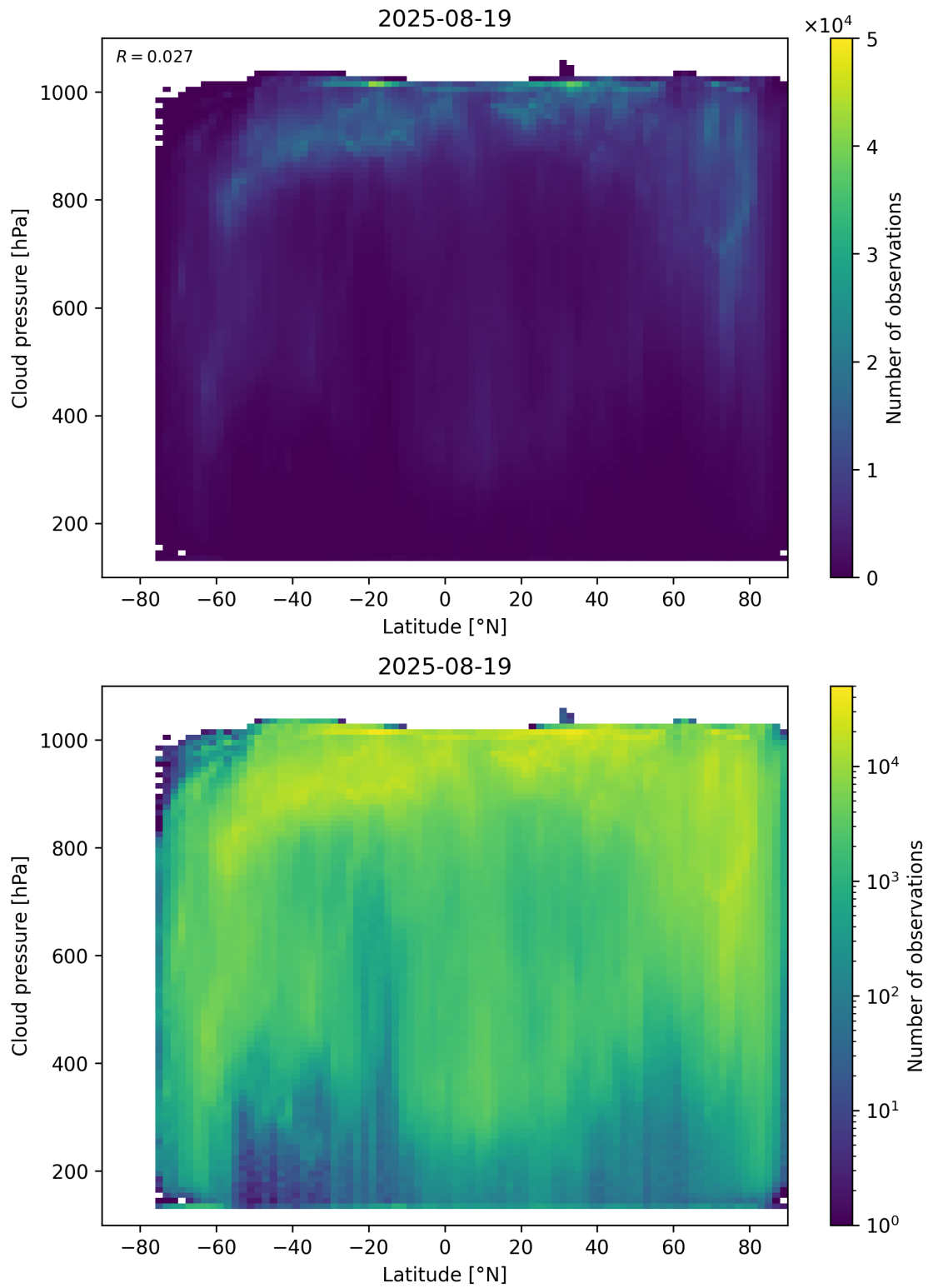
Figure 91: Scatter density plot of “Latitude” against “Cloud pressure” for 2025-08-19 to 2025-08-20.
