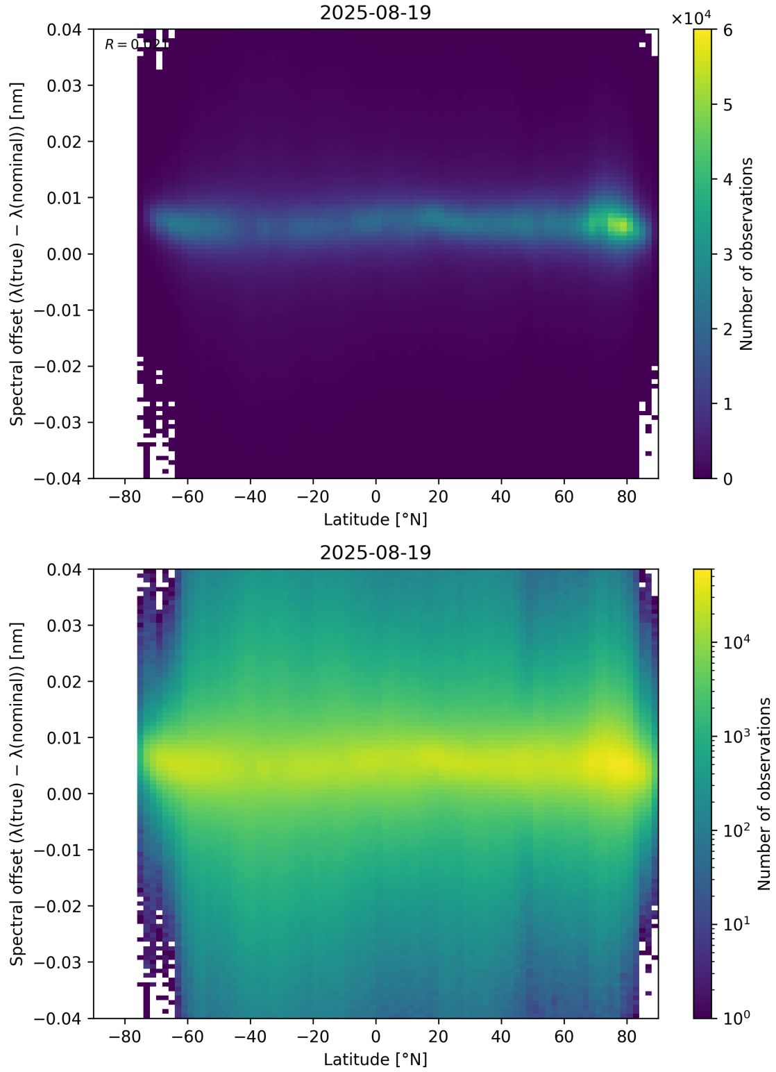
Figure 96: Scatter density plot of “Latitude” against “Spectral offset ( \lambda_{\text{true}} - \lambda_{\text{nominal}} )” for 2025-08-19 to 2025-08-20.
