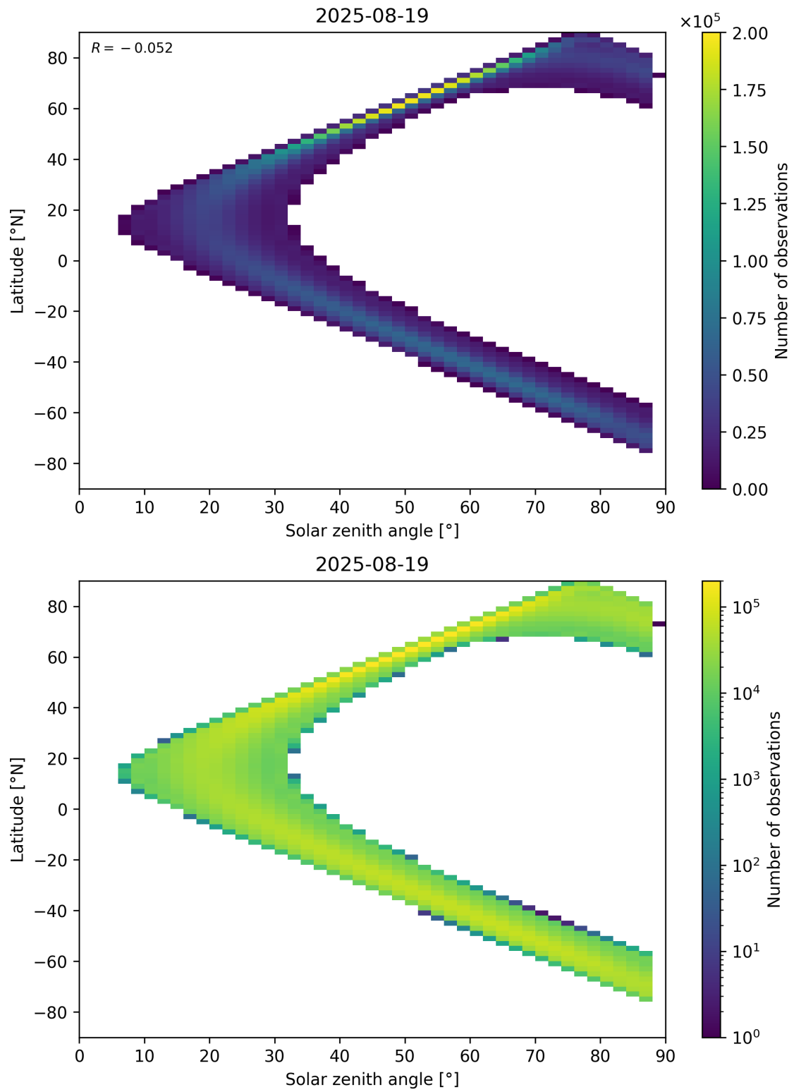
Figure 113: Scatter density plot of “Solar zenith angle” against “Latitude” for 2025-08-19 to 2025-08-20.
