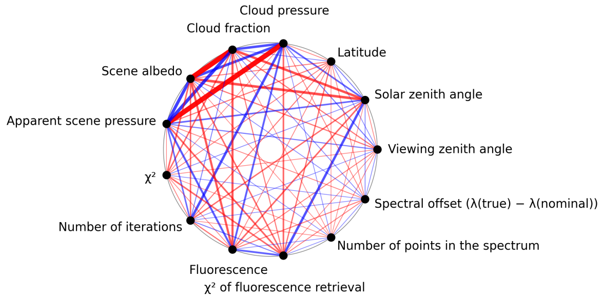
Figure 1: Map of correlation graph for 2025-08-19 to 2025-08-20.
