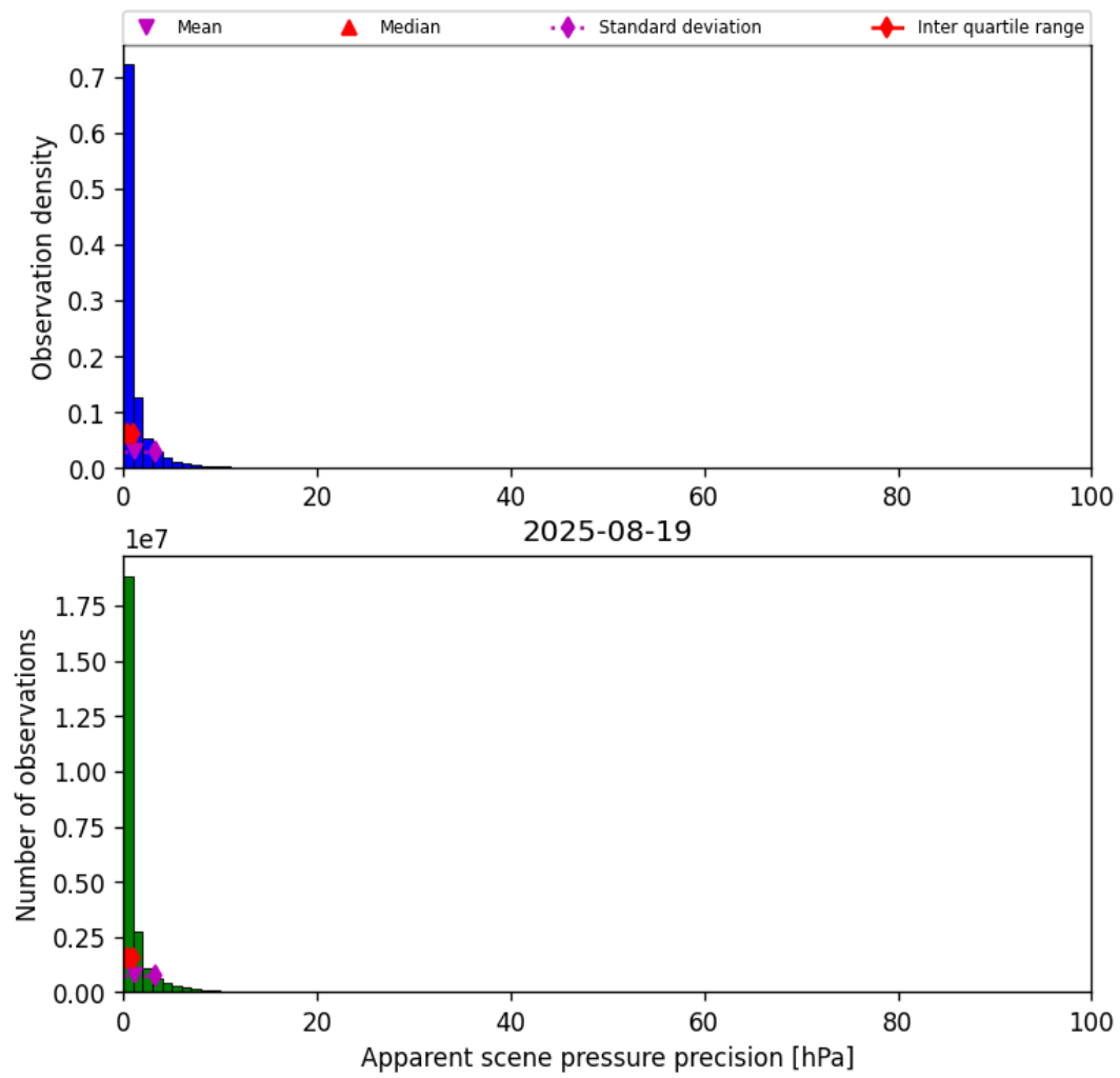
Figure 37: Histogram of “Apparent scene pressure precision” for 2025-08-19 to 2025-08-20
