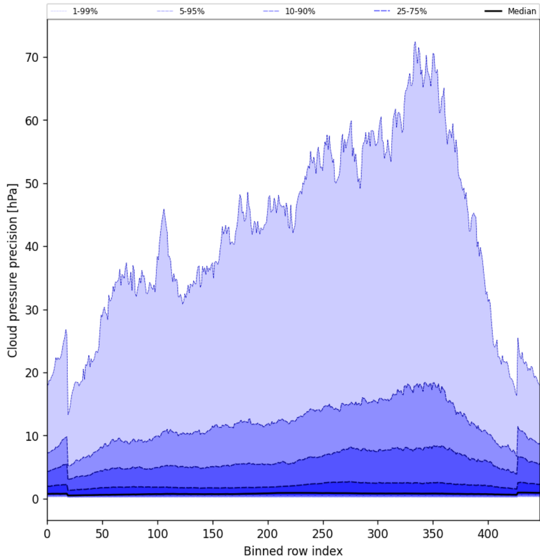
Figure 48: Along track statistics of “Cloud pressure precision” for 2025-08-19 to 2025-08-20
