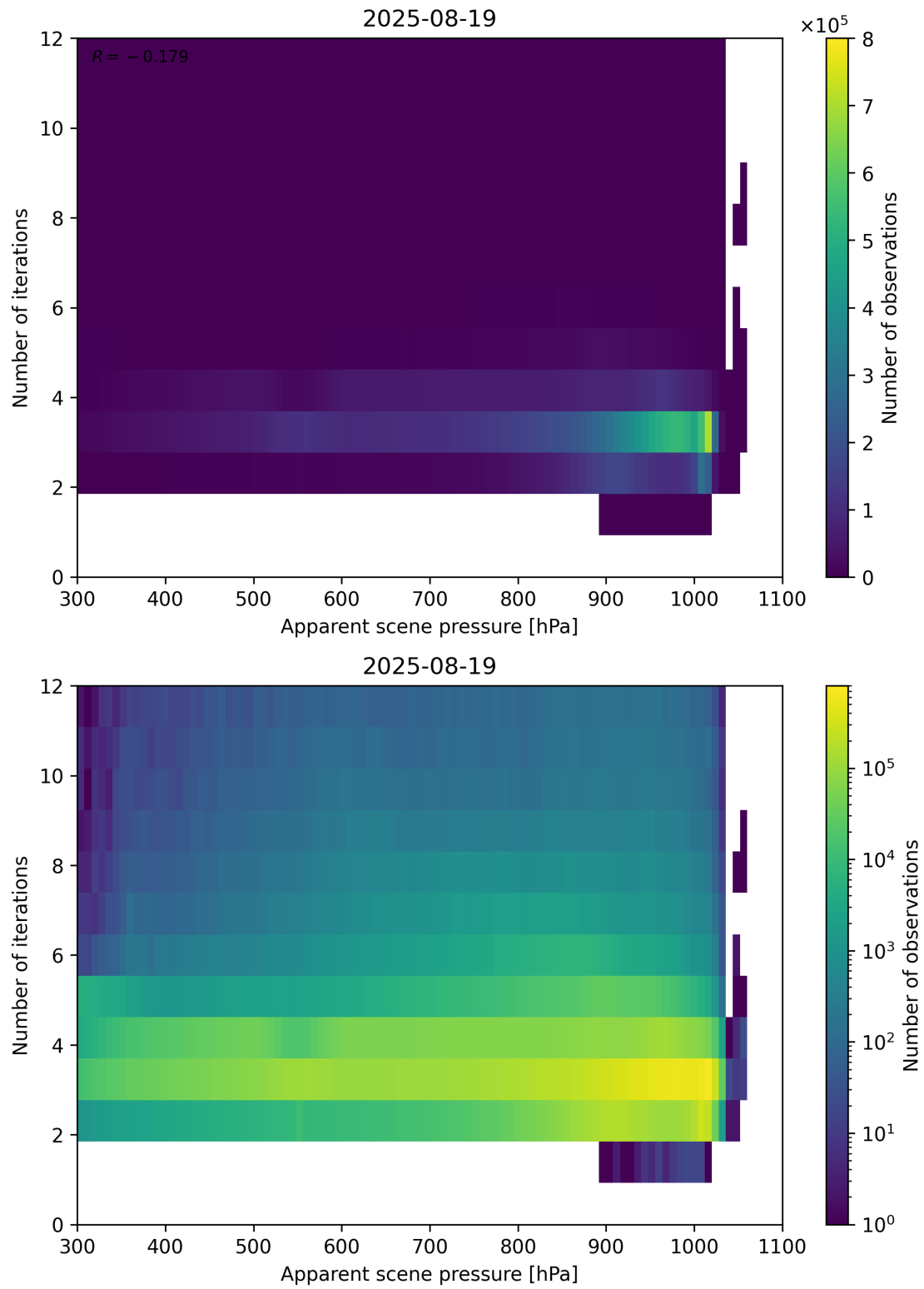
Figure 65: Scatter density plot of “Apparent scene pressure” against “Number of iterations” for 2025-08-19 to 2025-08-20.
