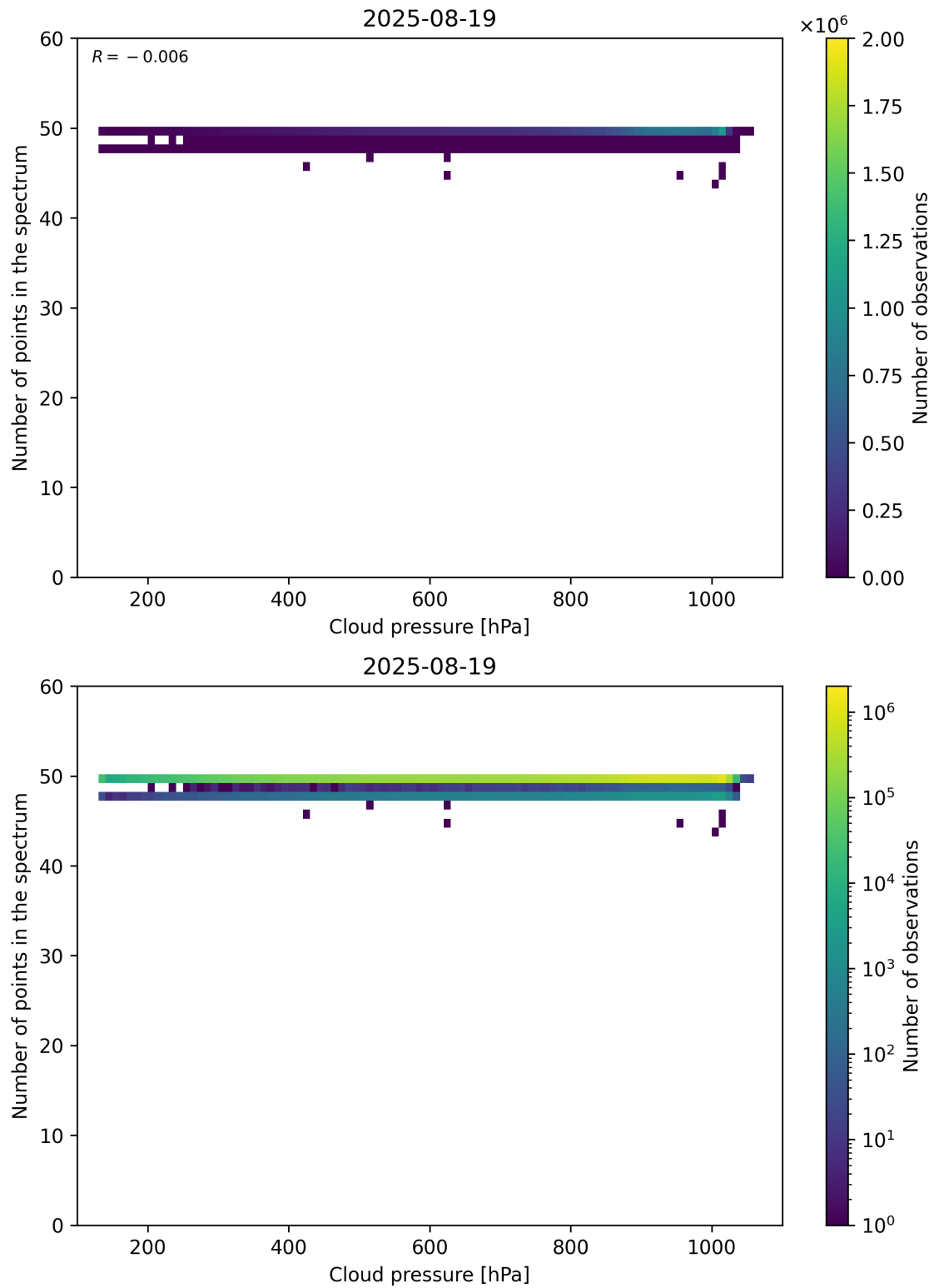
Figure 82: Scatter density plot of “Cloud pressure” against “Number of points in the spectrum” for 2025-08-19 to 2025-08-20.
