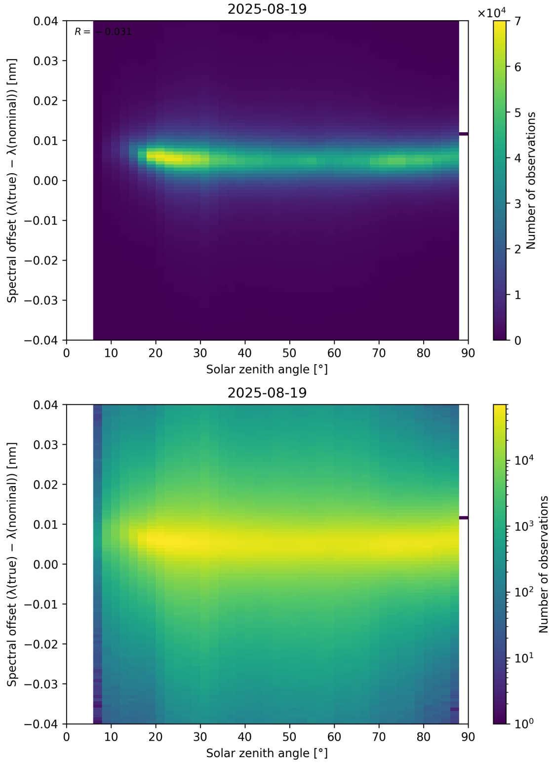
Figure 117: Scatter density plot of “Solar zenith angle” against “Spectral offset ( \lambda_{\text{true}} - \lambda_{\text{nominal}} )” for 2025-08-19 to 2025-08-20.
