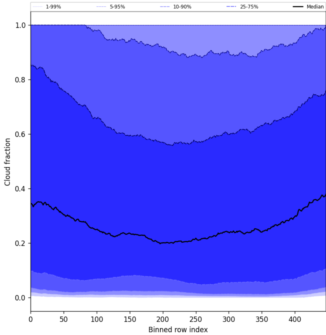
Figure 49: Along track statistics of “Cloud fraction” for 2025-08-19 to 2025-08-20
