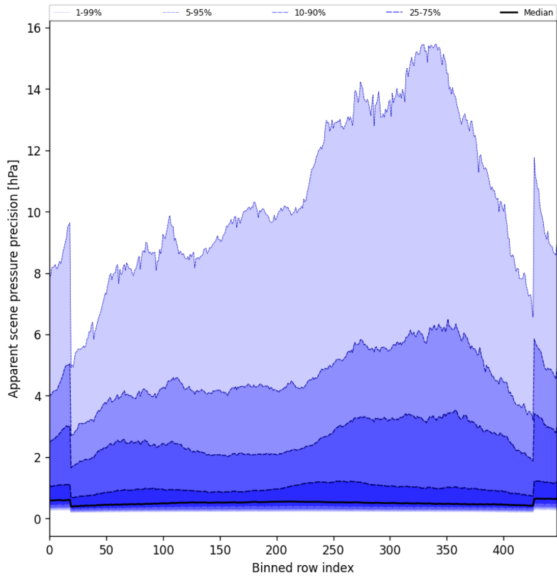
Figure 54: Along track statistics of “Apparent scene pressure precision” for 2025-08-19 to 2025-08-20
