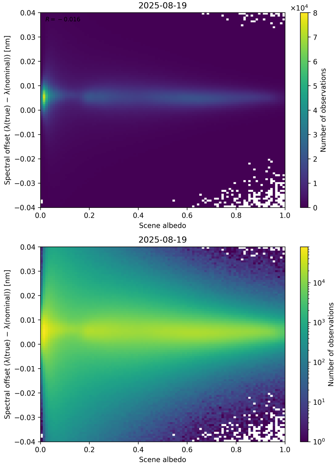
Figure 107: Scatter density plot of “Scene albedo” against “Spectral offset ( \lambda_{\text{true}} - \lambda_{\text{nominal}} )” for 2025-08-19 to 2025-08-20.
