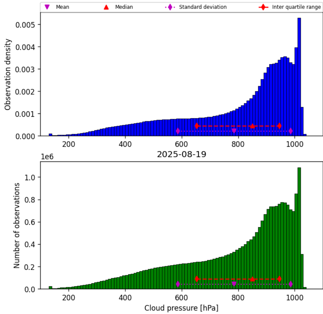
Figure 30: Histogram of “Cloud pressure” for 2025-08-19 to 2025-08-20
