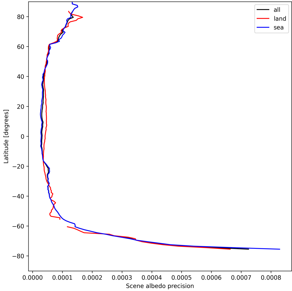
Figure 18: Zonal average of “Scene albedo precision” for 2025-08-19 to 2025-08-20.
