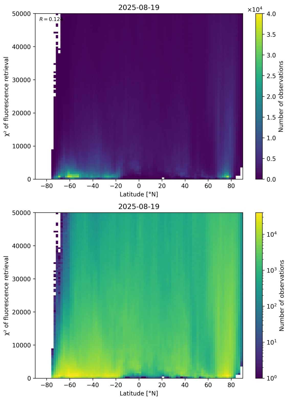
Figure 89: Scatter density plot of “Latitude” against “ \chi^2 of fluorescence retrieval” for 2025-08-19 to 2025-08-20.
