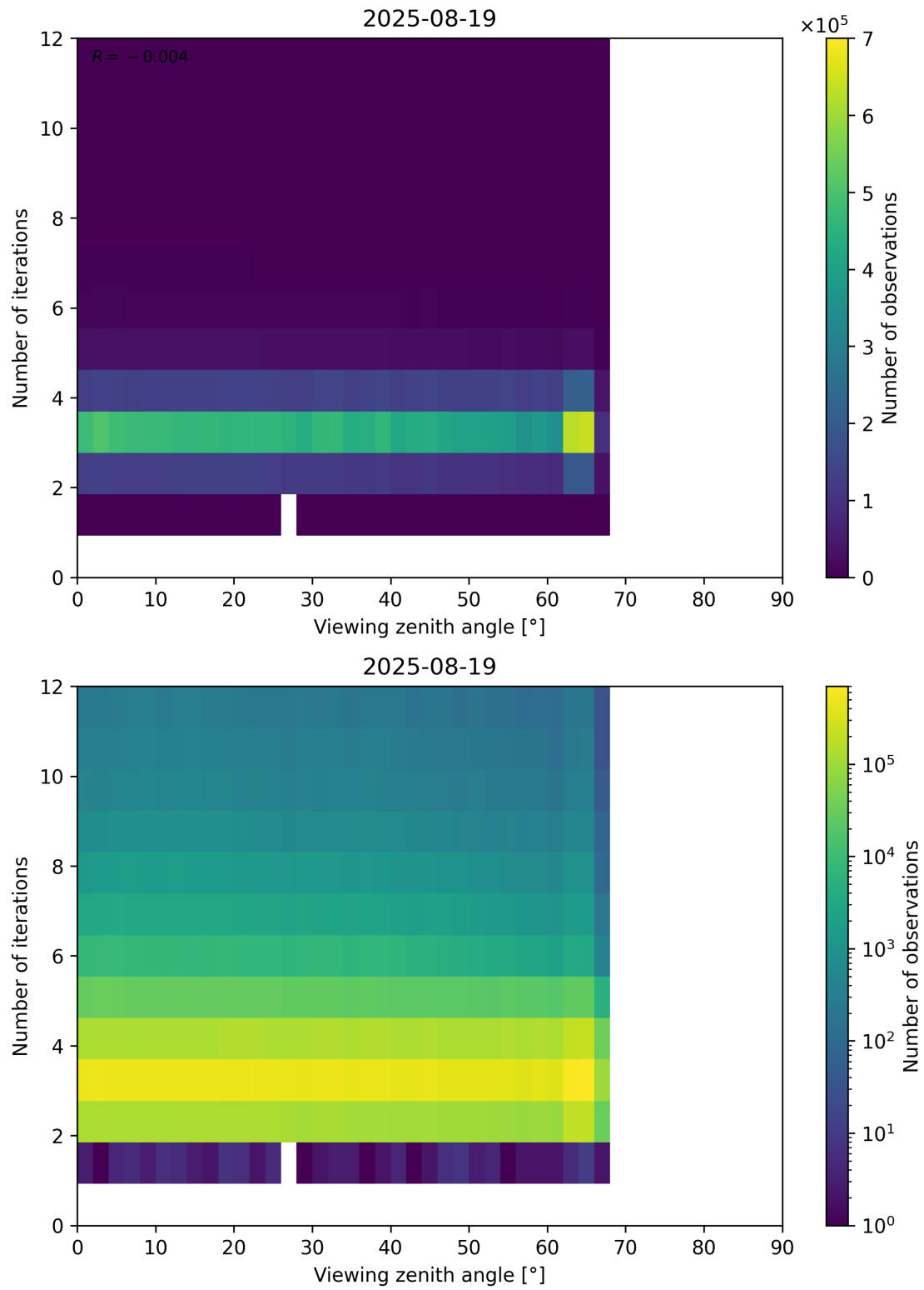
Figure 124: Scatter density plot of “Viewing zenith angle” against “Number of iterations” for 2025-08-19 to 2025-08-20.
