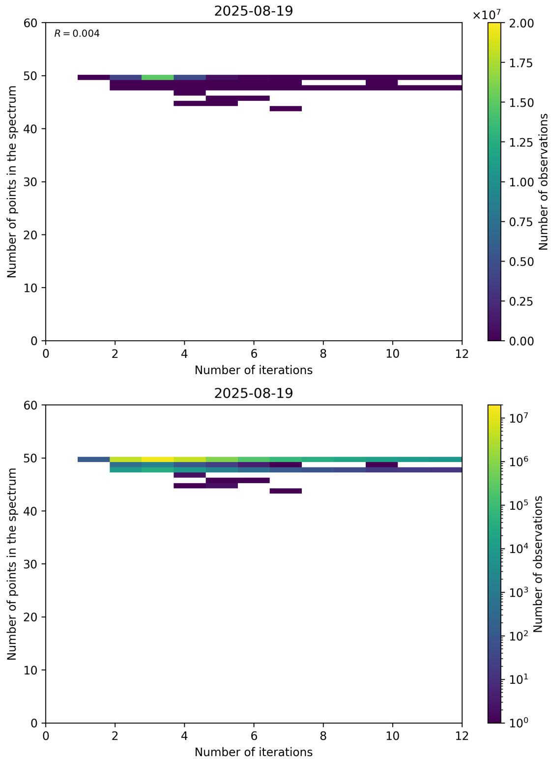
Figure 99: Scatter density plot of “Number of iterations” against “Number of points in the spectrum” for 2025-08-19 to 2025-08-20.
