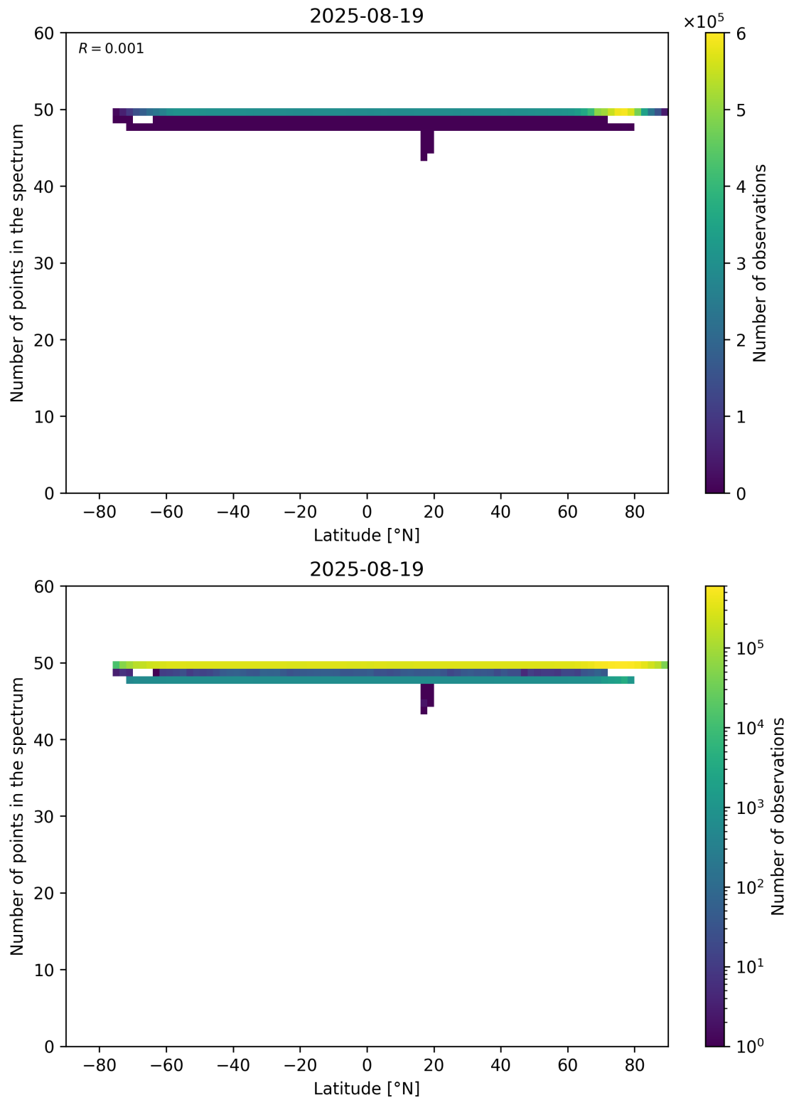
Figure 94: Scatter density plot of “Latitude” against “Number of points in the spectrum” for 2025-08-19 to 2025-08-20.
