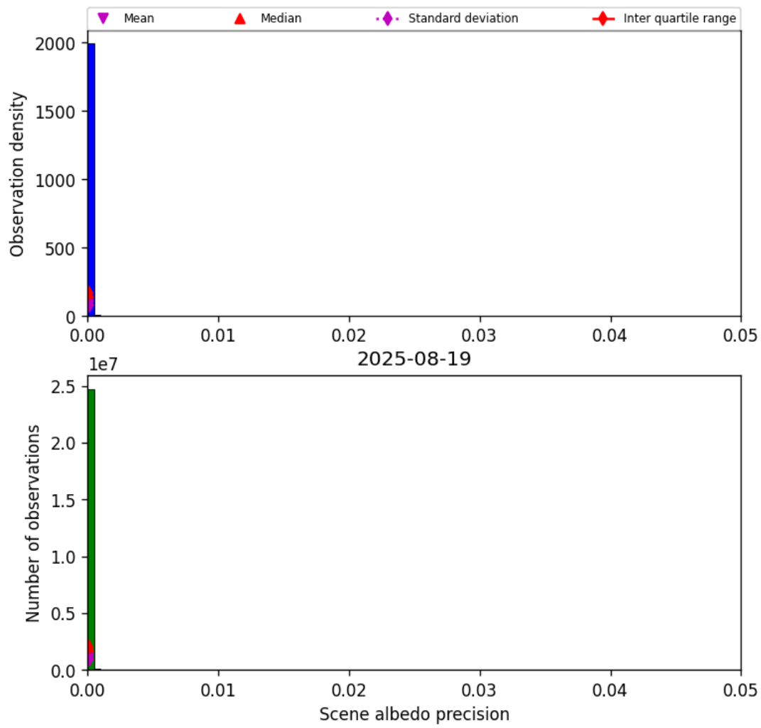
Figure 35: Histogram of “Scene albedo precision” for 2025-08-19 to 2025-08-20
