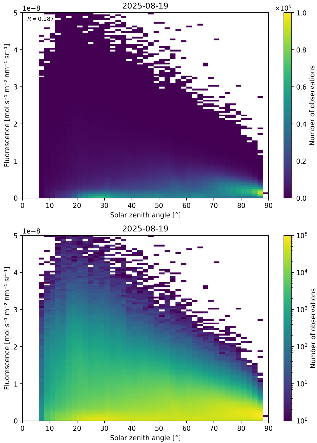
Figure 112: Scatter density plot of “Solar zenith angle” against “Fluorescence” for 2025-08-19 to 2025-08-20.
