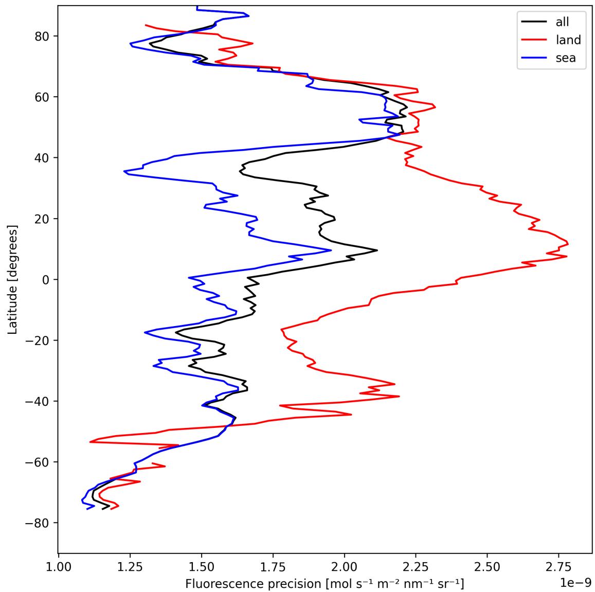
Figure 24: Zonal average of “Fluorescence precision” for 2025-08-19 to 2025-08-20.
