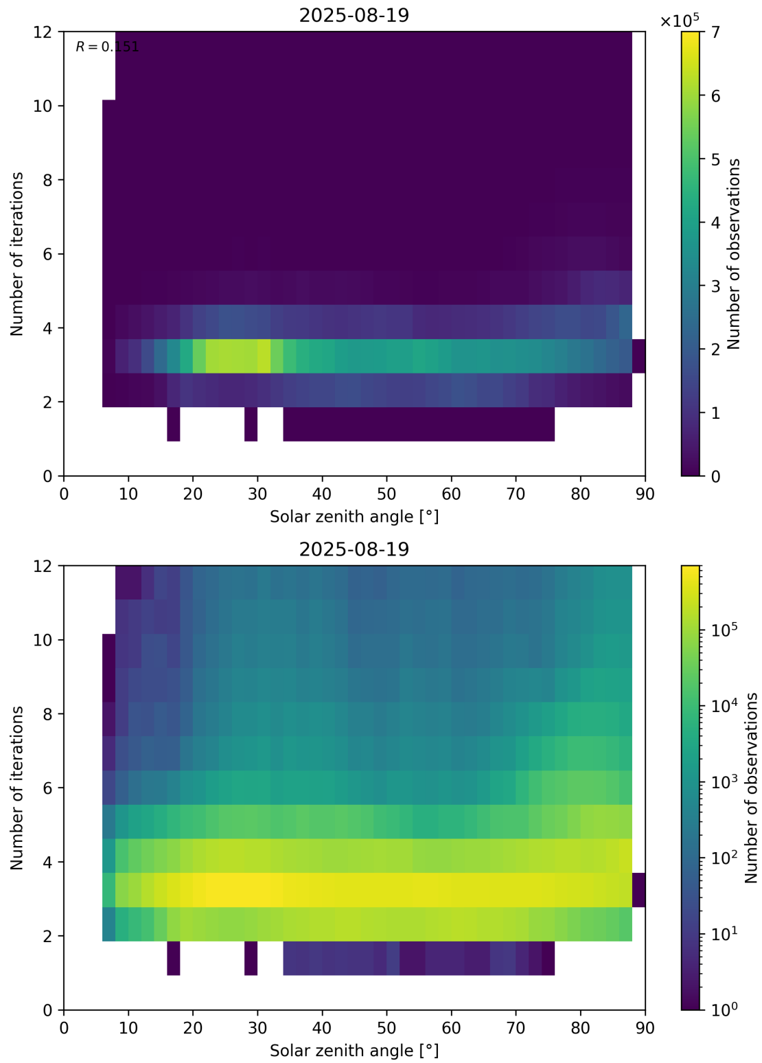
Figure 114: Scatter density plot of “Solar zenith angle” against “Number of iterations” for 2025-08-19 to 2025-08-20.
