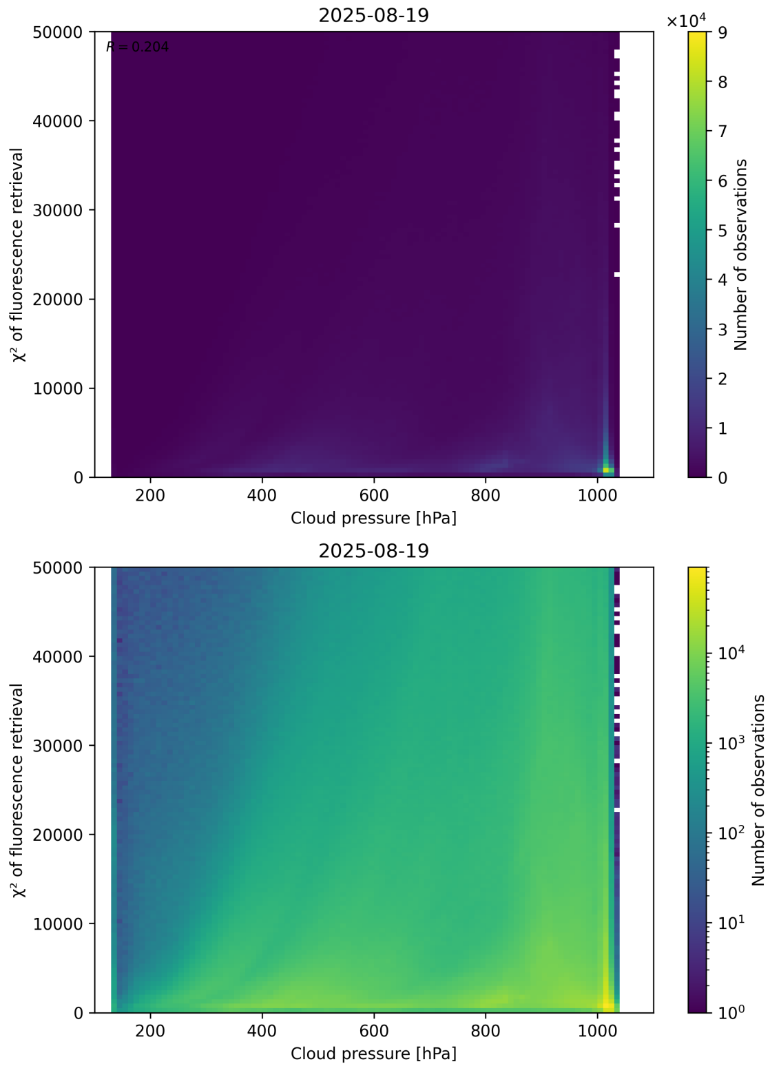
Figure 78: Scatter density plot of “Cloud pressure” against “ \chi^2 of fluorescence retrieval” for 2025-08-19 to 2025-08-20.
