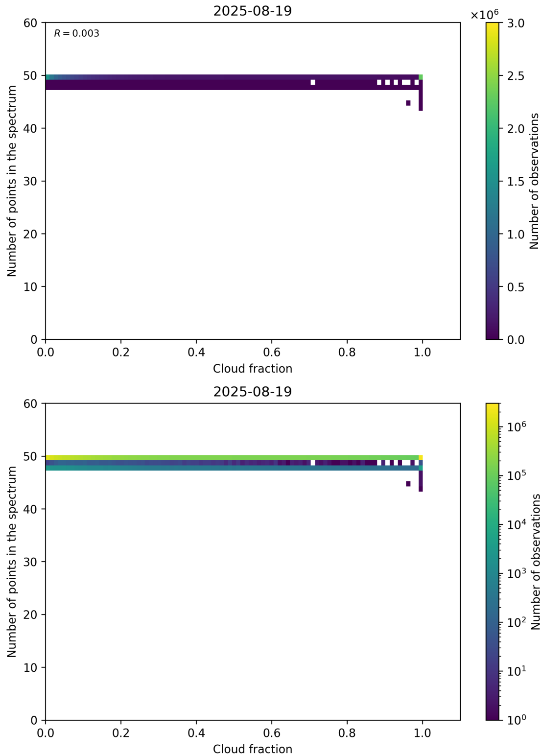
Figure 74: Scatter density plot of “Cloud fraction” against “Number of points in the spectrum” for 2025-08-19 to 2025-08-20.
