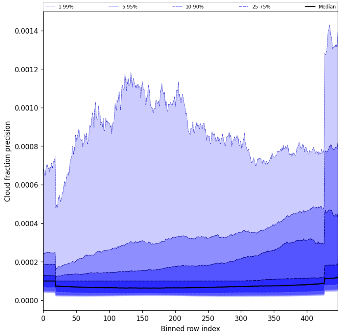
Figure 50: Along track statistics of “Cloud fraction precision” for 2025-08-19 to 2025-08-20
