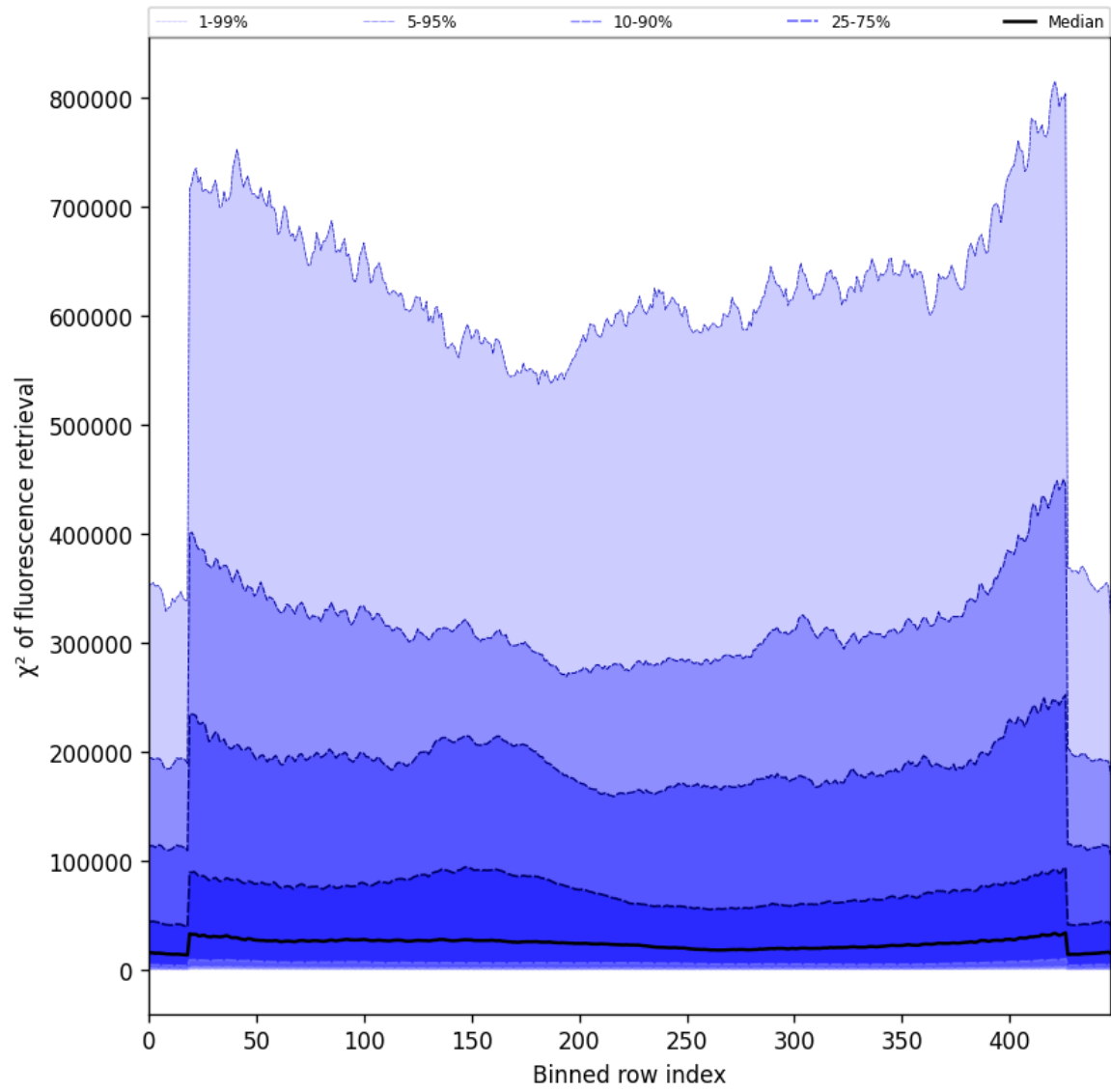
Figure 59: Along track statistics of “ \chi^2 of fluorescence retrieval” for 2025-08-19 to 2025-08-20
