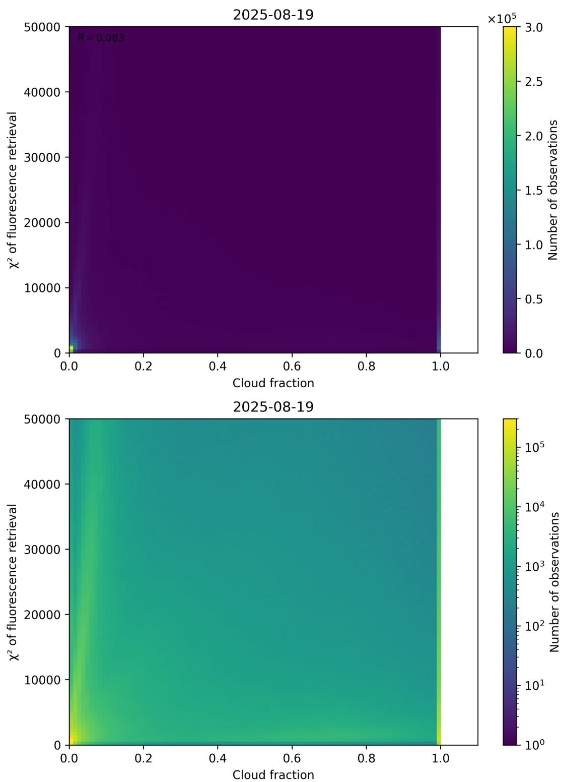
Figure 71: Scatter density plot of “Cloud fraction” against “ \chi^2 of fluorescence retrieval” for 2025-08-19 to 2025-08-20.
