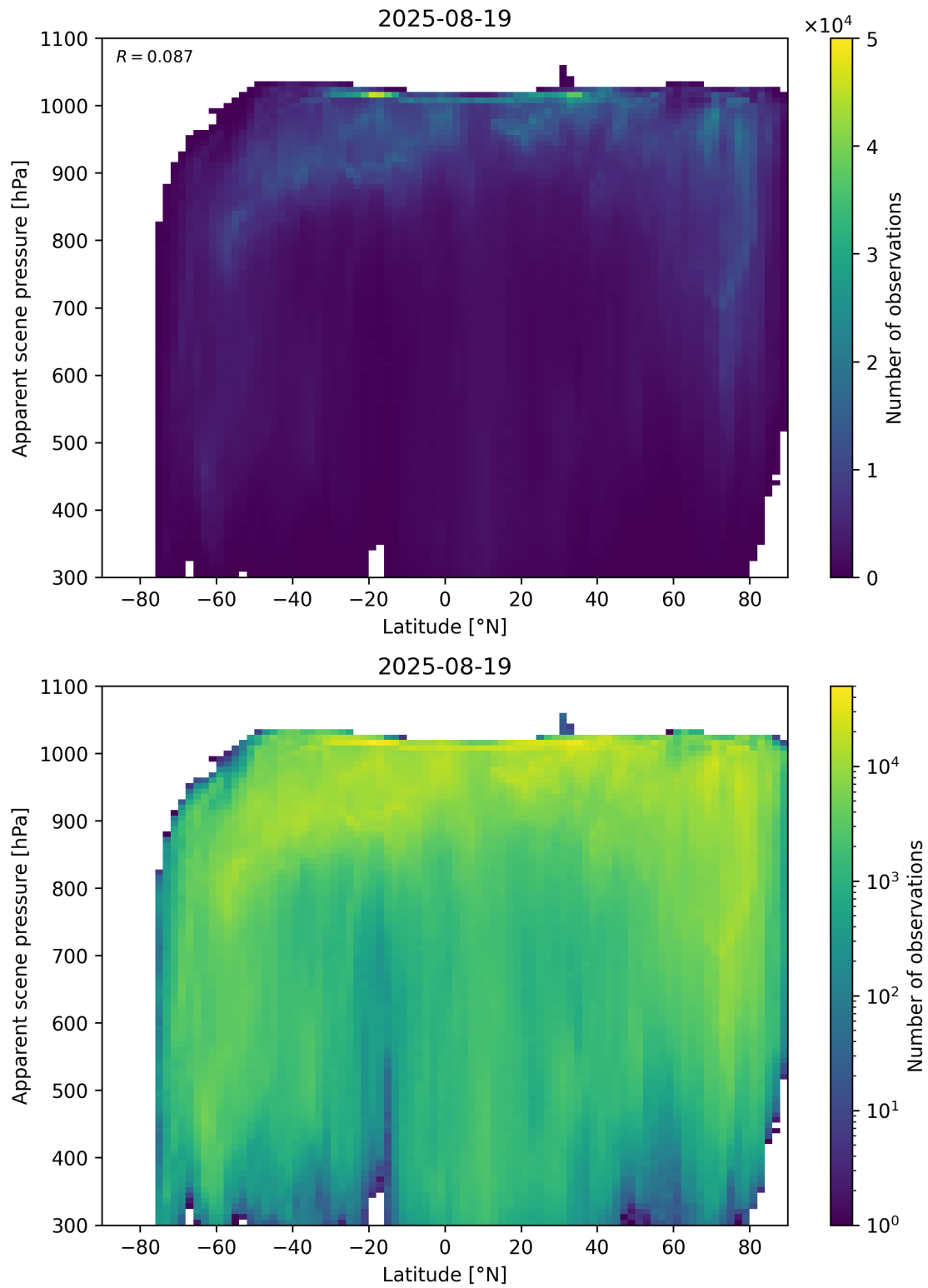
Figure 88: Scatter density plot of “Latitude” against “Apparent scene pressure” for 2025-08-19 to 2025-08-20.
