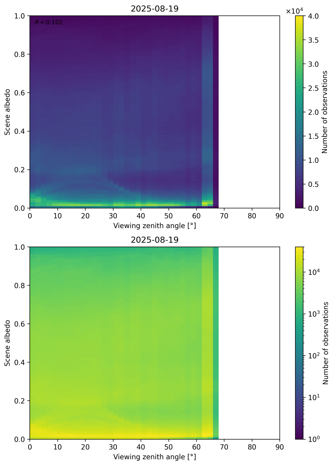
Figure 126: Scatter density plot of “Viewing zenith angle” against “Scene albedo” for 2025-08-19 to 2025-08-20.
