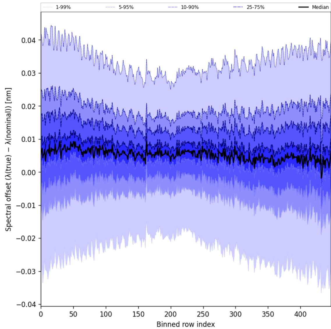
Figure 62: Along track statistics of “Spectral offset ( \lambda_{\text{true}} - \lambda_{\text{nominal}} )” for 2025-08-19 to 2025-08-20
