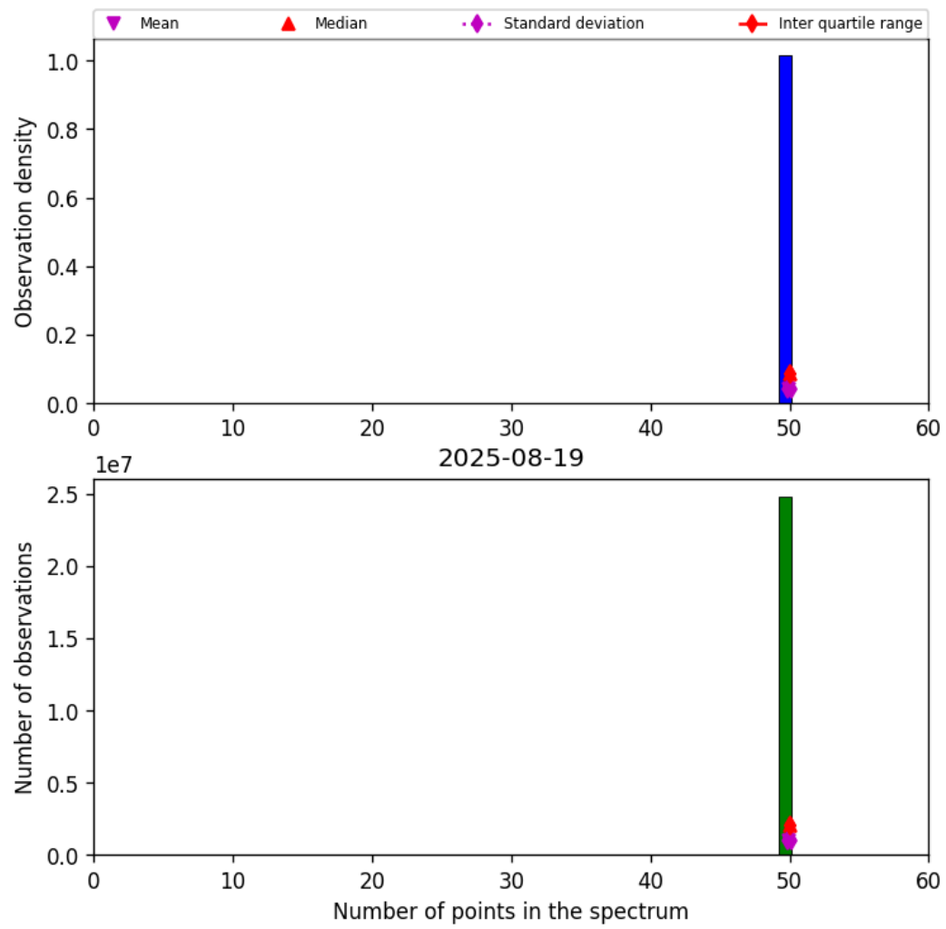
Figure 44: Histogram of “Number of points in the spectrum” for 2025-08-19 to 2025-08-20
