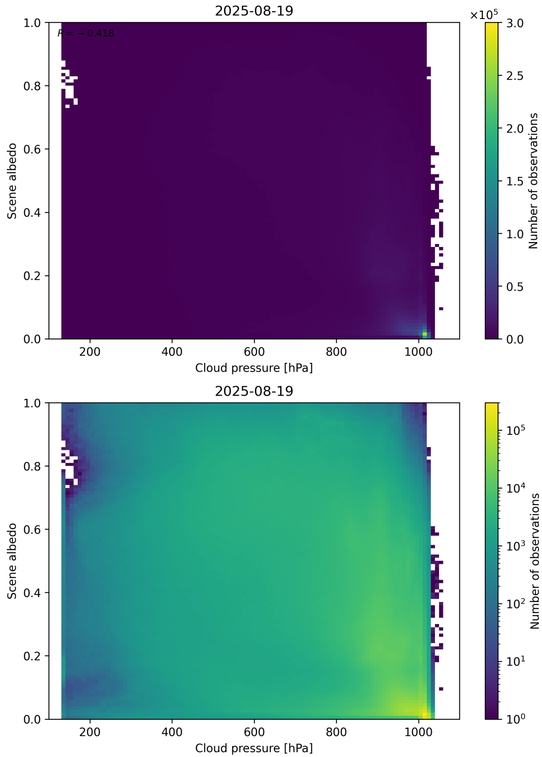
Figure 83: Scatter density plot of “Cloud pressure” against “Scene albedo” for 2025-08-19 to 2025-08-20.
