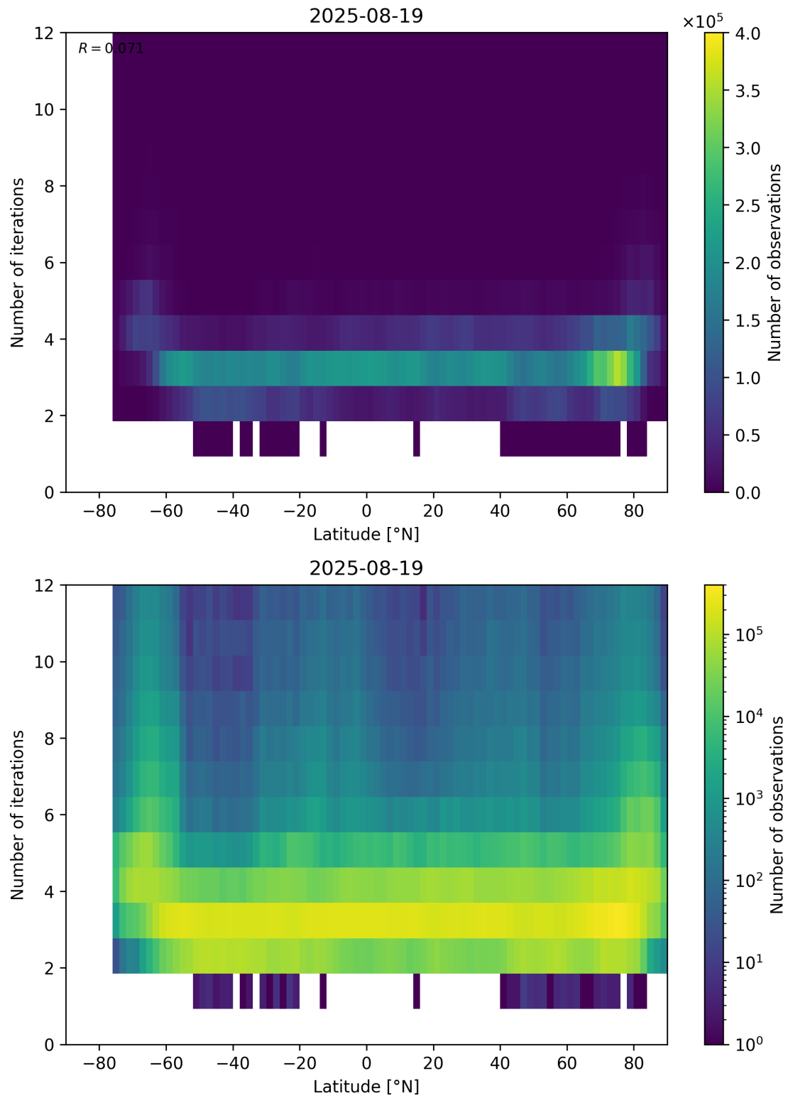
Figure 93: Scatter density plot of “Latitude” against “Number of iterations” for 2025-08-19 to 2025-08-20.
