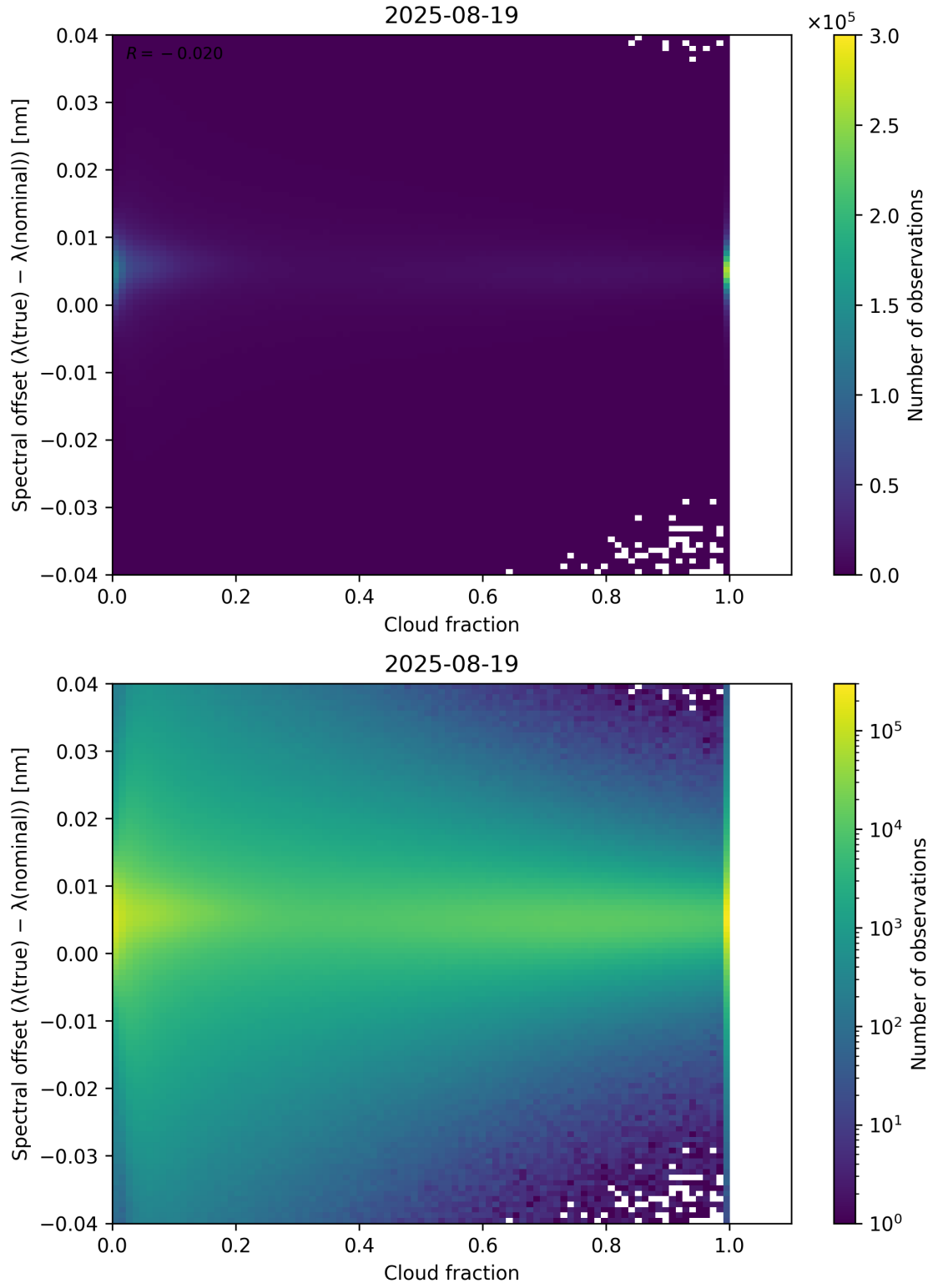
Figure 76: Scatter density plot of “Cloud fraction” against “Spectral offset ( \lambda_{\text{true}} - \lambda_{\text{nominal}} )” for 2025-08-19 to 2025-08-20.
