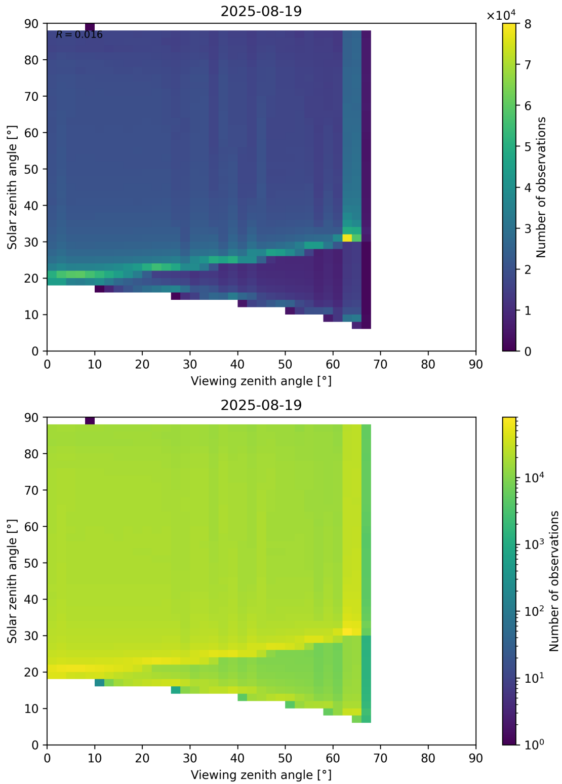
Figure 127: Scatter density plot of “Viewing zenith angle” against “Solar zenith angle” for 2025-08-19 to 2025-08-20.
