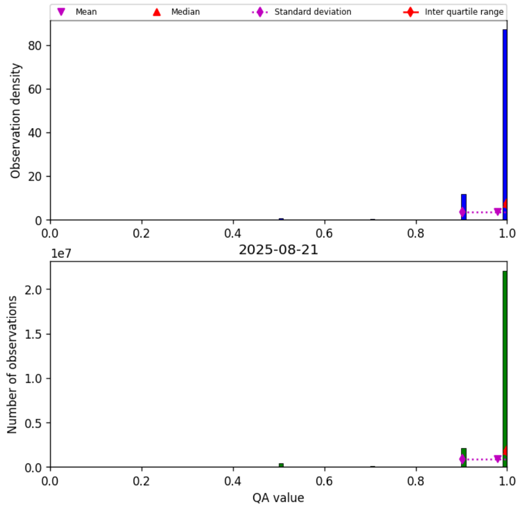
Figure 29: Histogram of “QA value” for 2025-08-20 to 2025-08-22
