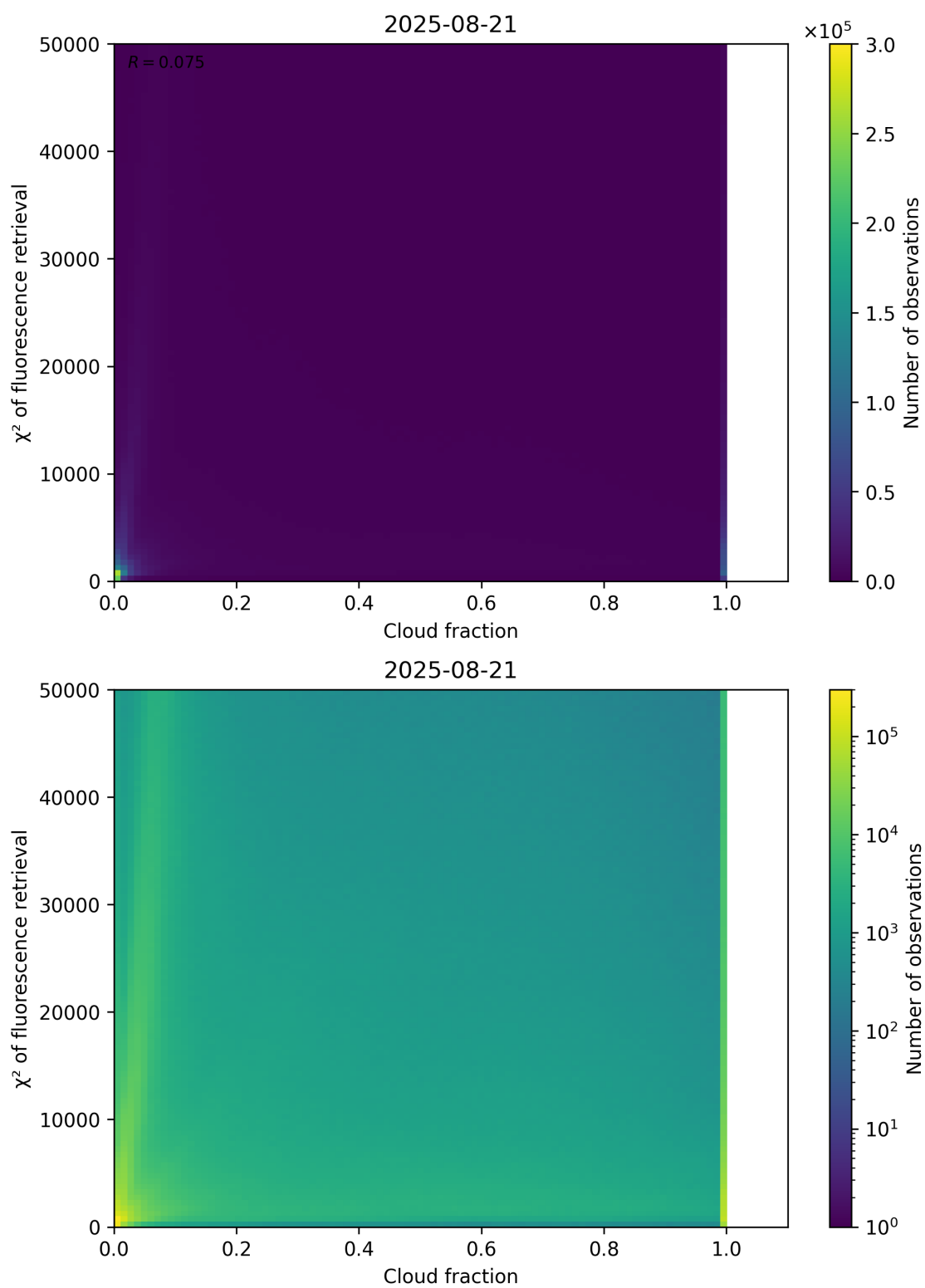
Figure 71: Scatter density plot of “Cloud fraction” against “ \chi^2 of fluorescence retrieval” for 2025-08-20 to 2025-08-22.
