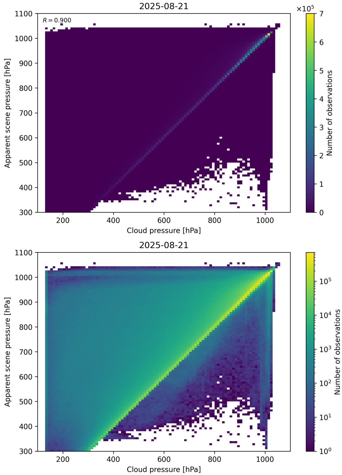
Figure 77: Scatter density plot of “Cloud pressure” against “Apparent scene pressure” for 2025-08-20 to 2025-08-22.
