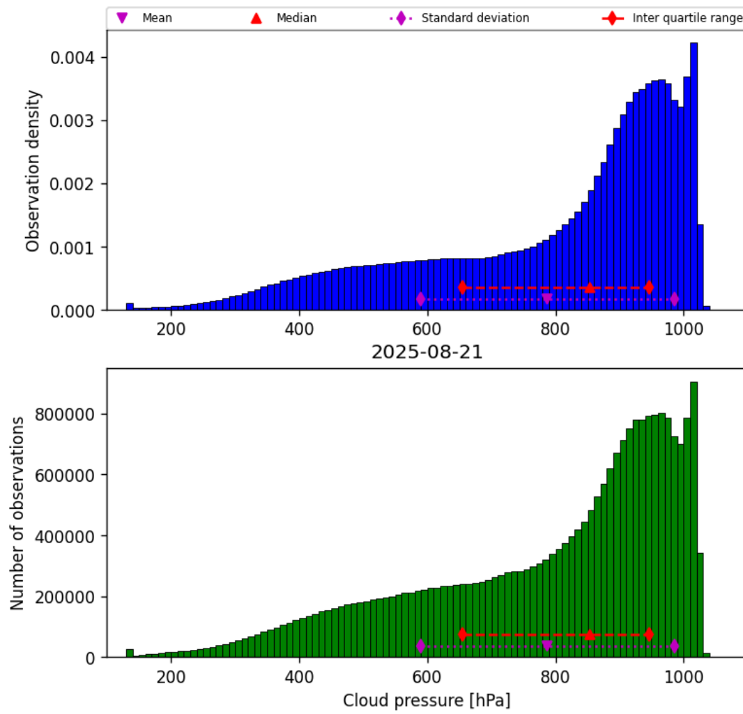
Figure 30: Histogram of “Cloud pressure” for 2025-08-20 to 2025-08-22
