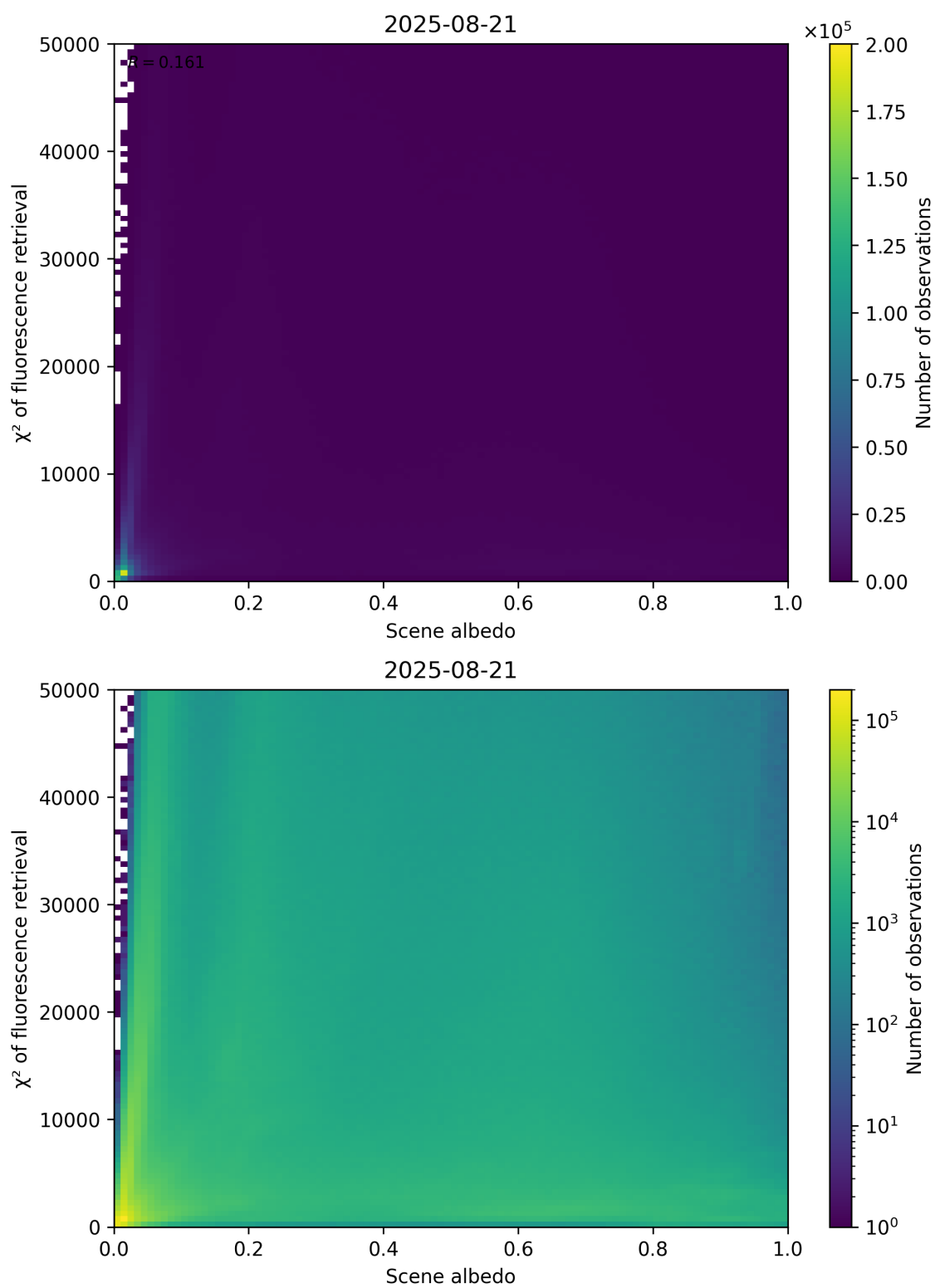
Figure 103: Scatter density plot of “Scene albedo” against “ \chi^2 of fluorescence retrieval” for 2025-08-20 to 2025-08-22.
