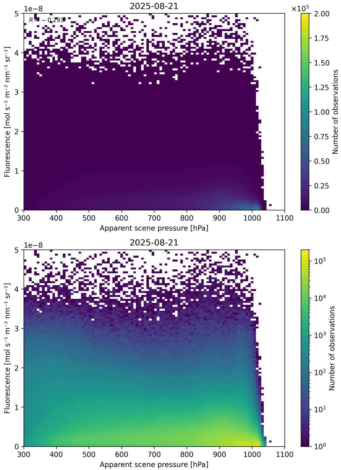
Figure 64: Scatter density plot of “Apparent scene pressure” against “Fluorescence” for 2025-08-20 to 2025-08-22.
