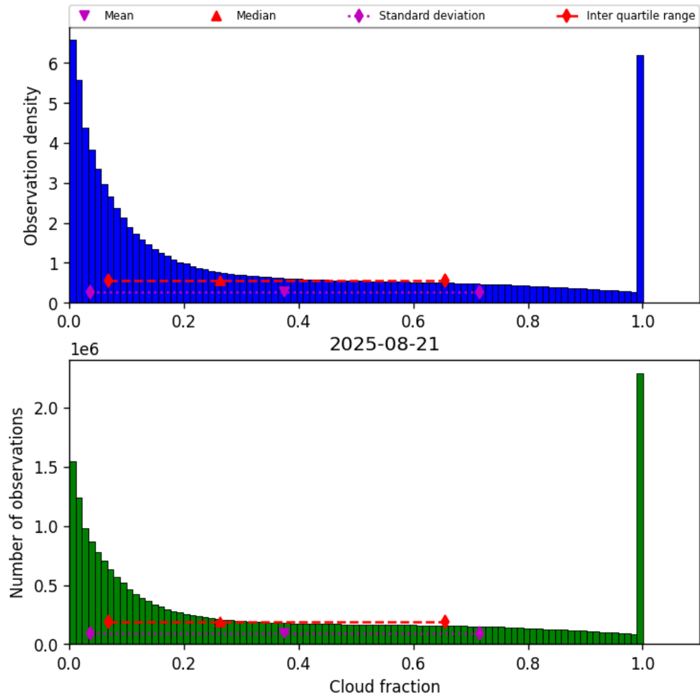
Figure 32: Histogram of “Cloud fraction” for 2025-08-20 to 2025-08-22
