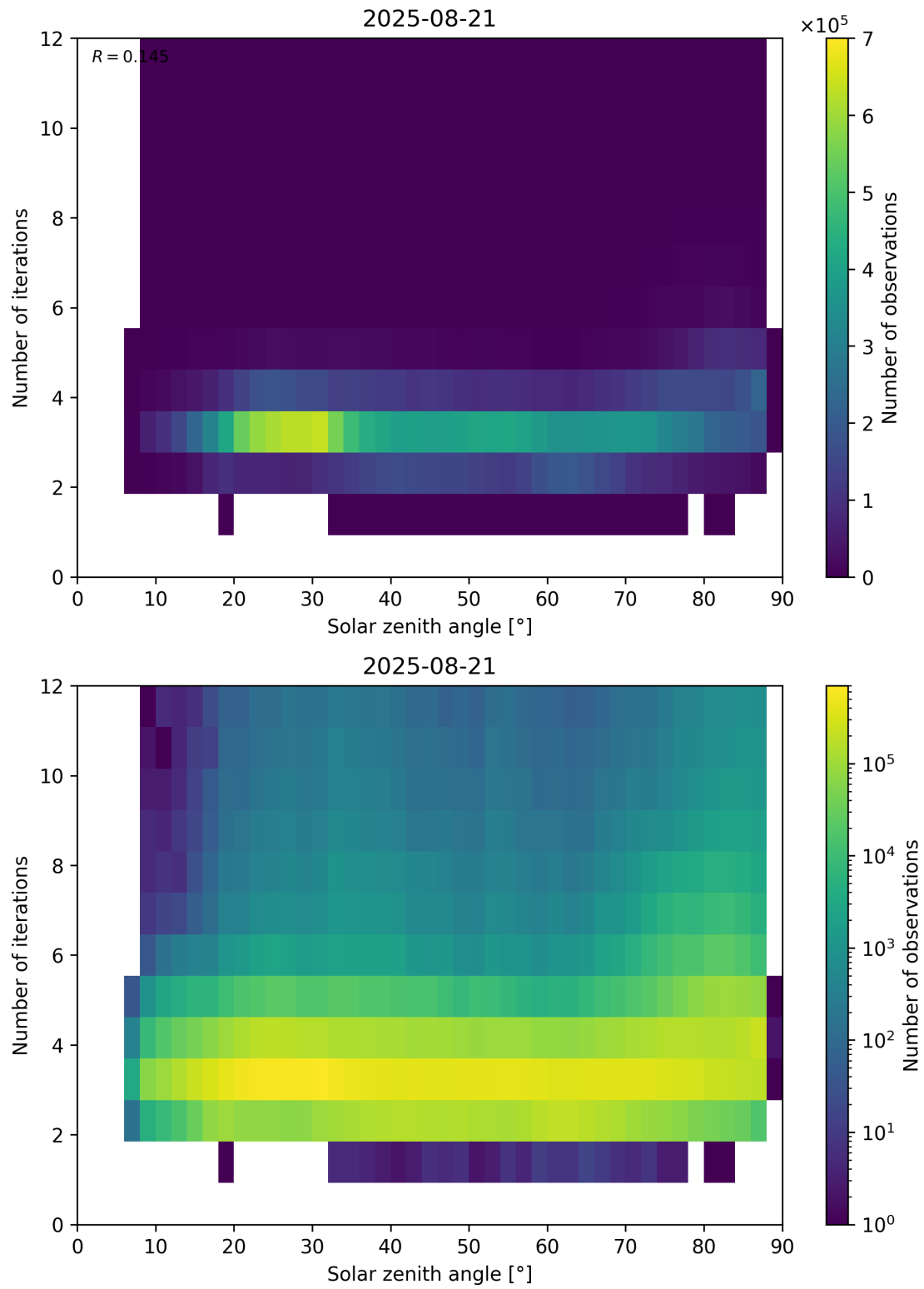
Figure 114: Scatter density plot of “Solar zenith angle” against “Number of iterations” for 2025-08-20 to 2025-08-22.
