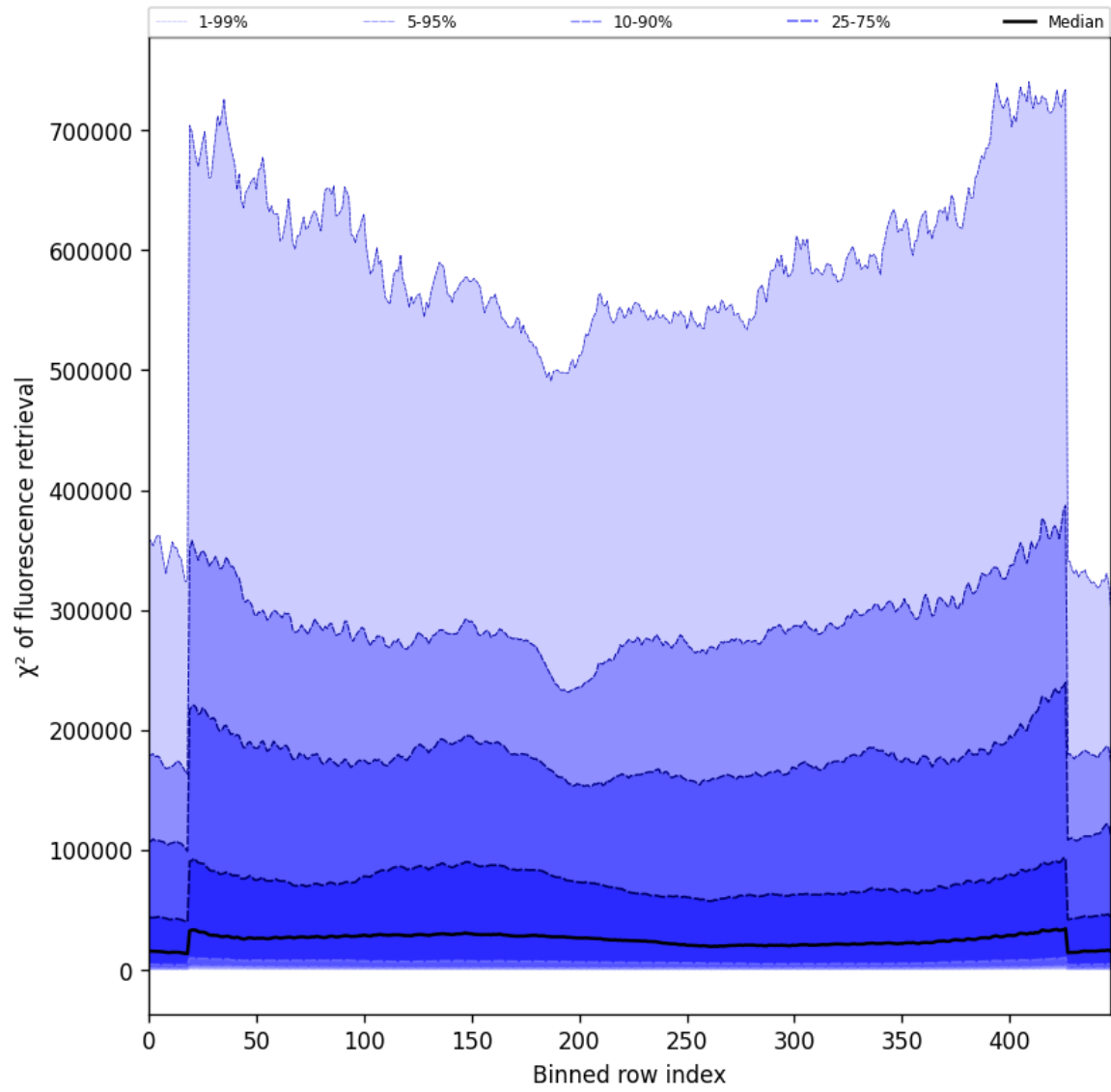
Figure 59: Along track statistics of “ \chi^2 of fluorescence retrieval” for 2025-08-20 to 2025-08-22
