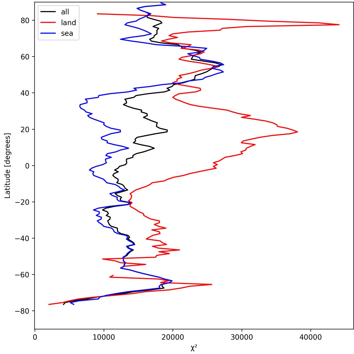
Figure 21: Zonal average of “ \chi^2 ” for 2025-08-20 to 2025-08-22.
