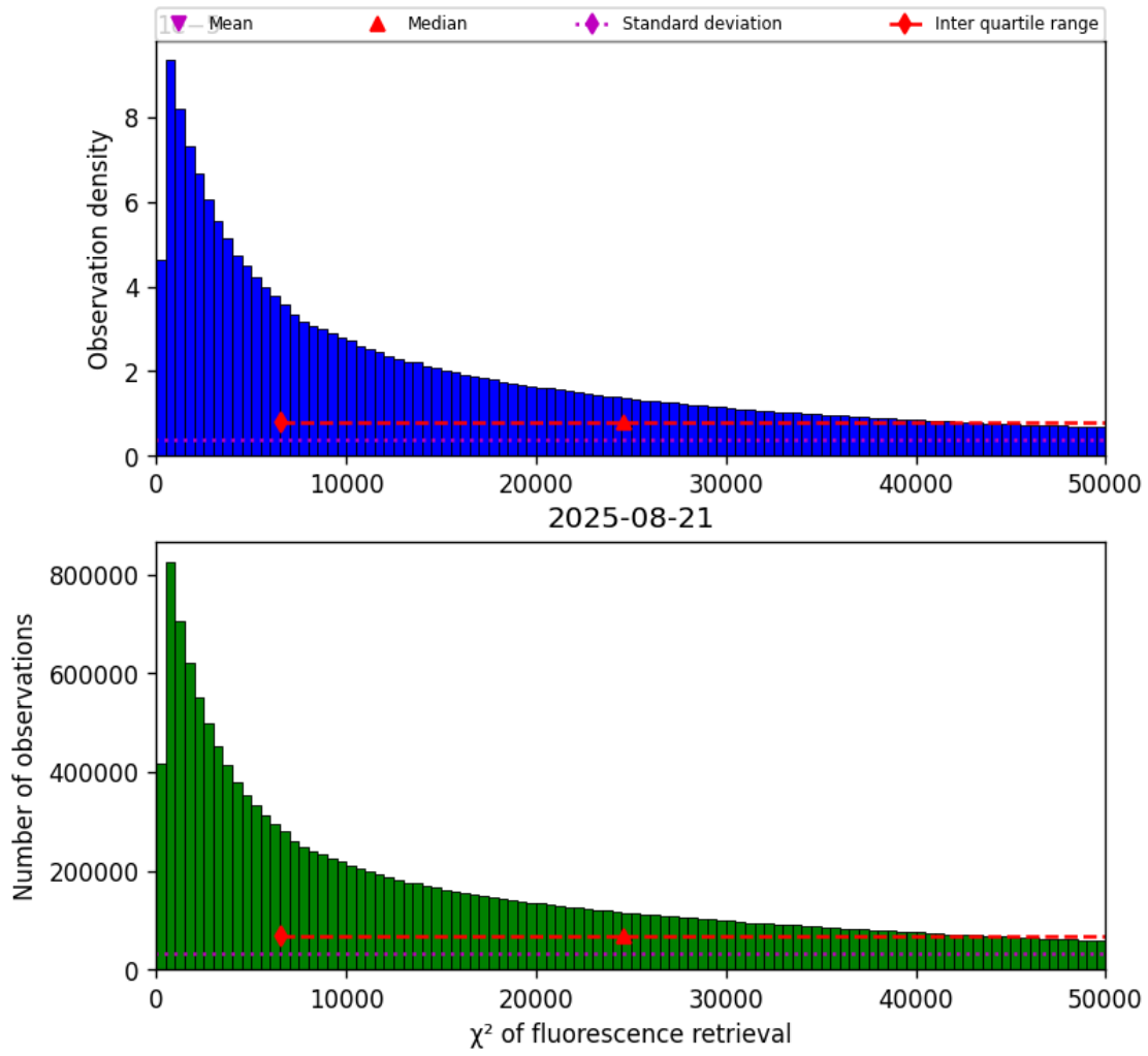
Figure 42: Histogram of “ \chi^2 of fluorescence retrieval” for 2025-08-20 to 2025-08-22
