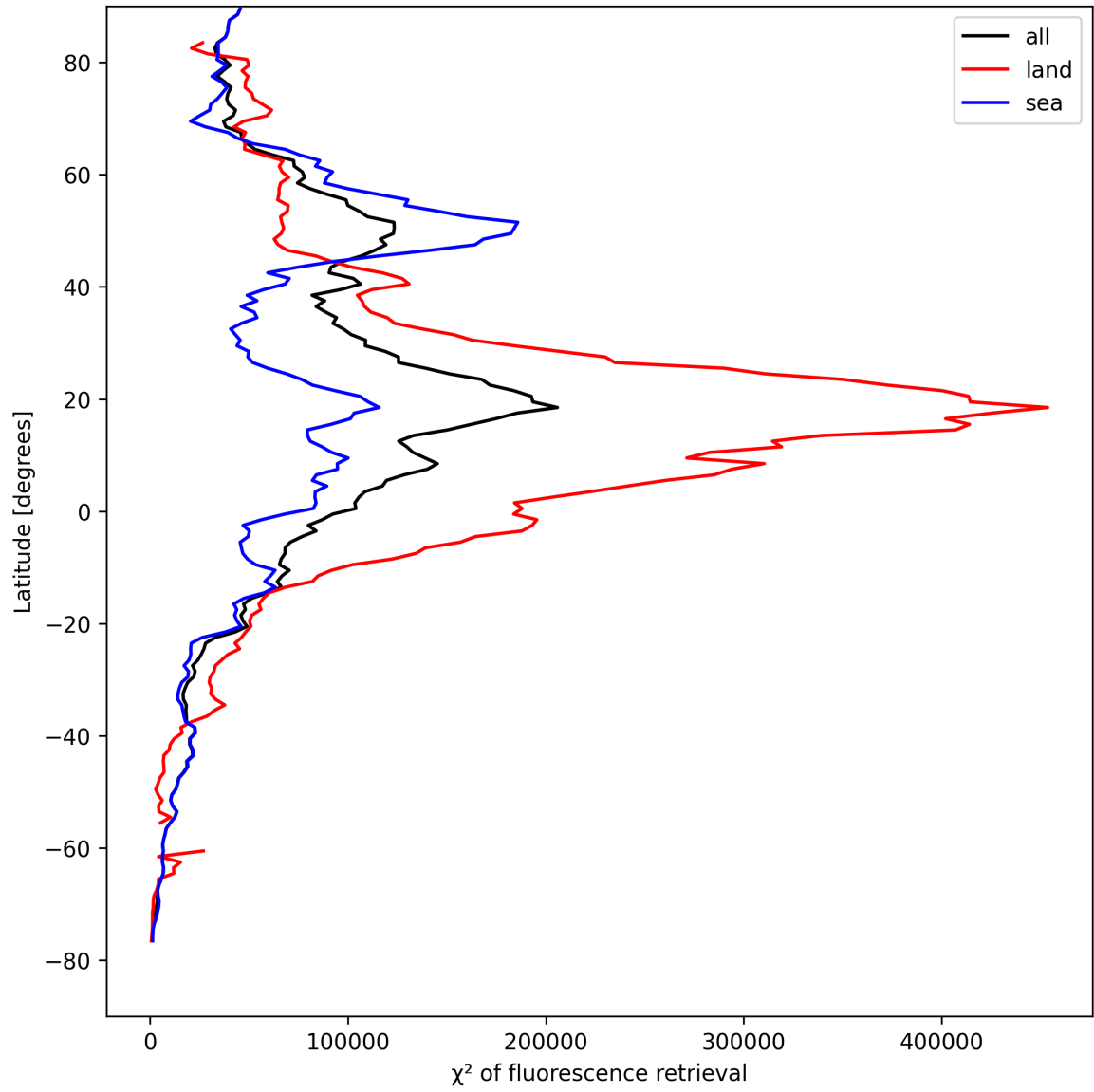
Figure 25: Zonal average of “ \chi^2 of fluorescence retrieval” for 2025-08-20 to 2025-08-22.
