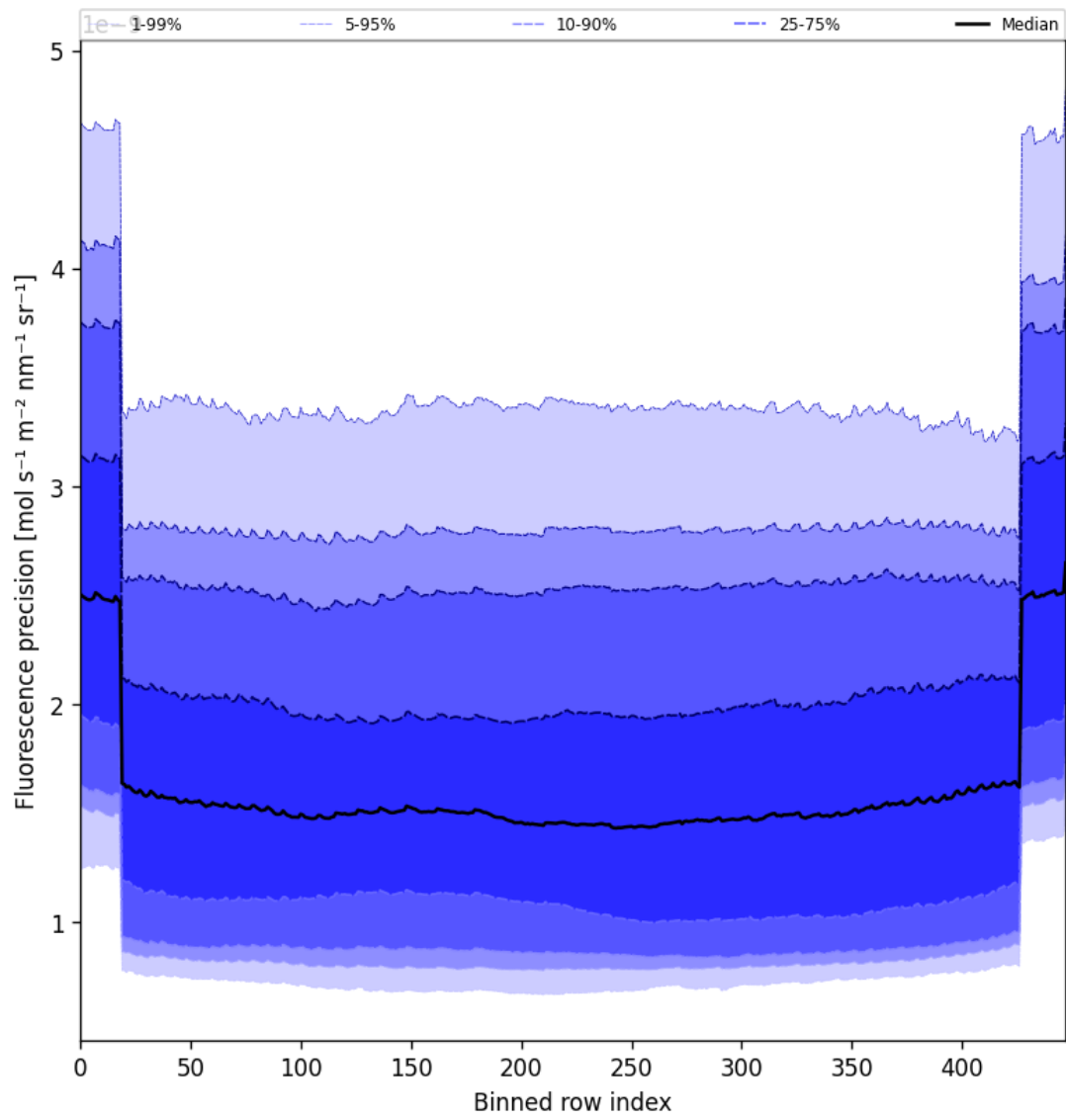
Figure 58: Along track statistics of “Fluorescence precision” for 2025-08-20 to 2025-08-22
