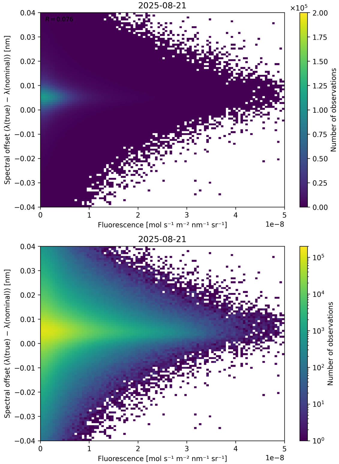
Figure 87: Scatter density plot of “Fluorescence” against “Spectral offset ( \lambda_{\text{true}} - \lambda_{\text{nominal}} )” for 2025-08-20 to 2025-08-22.
