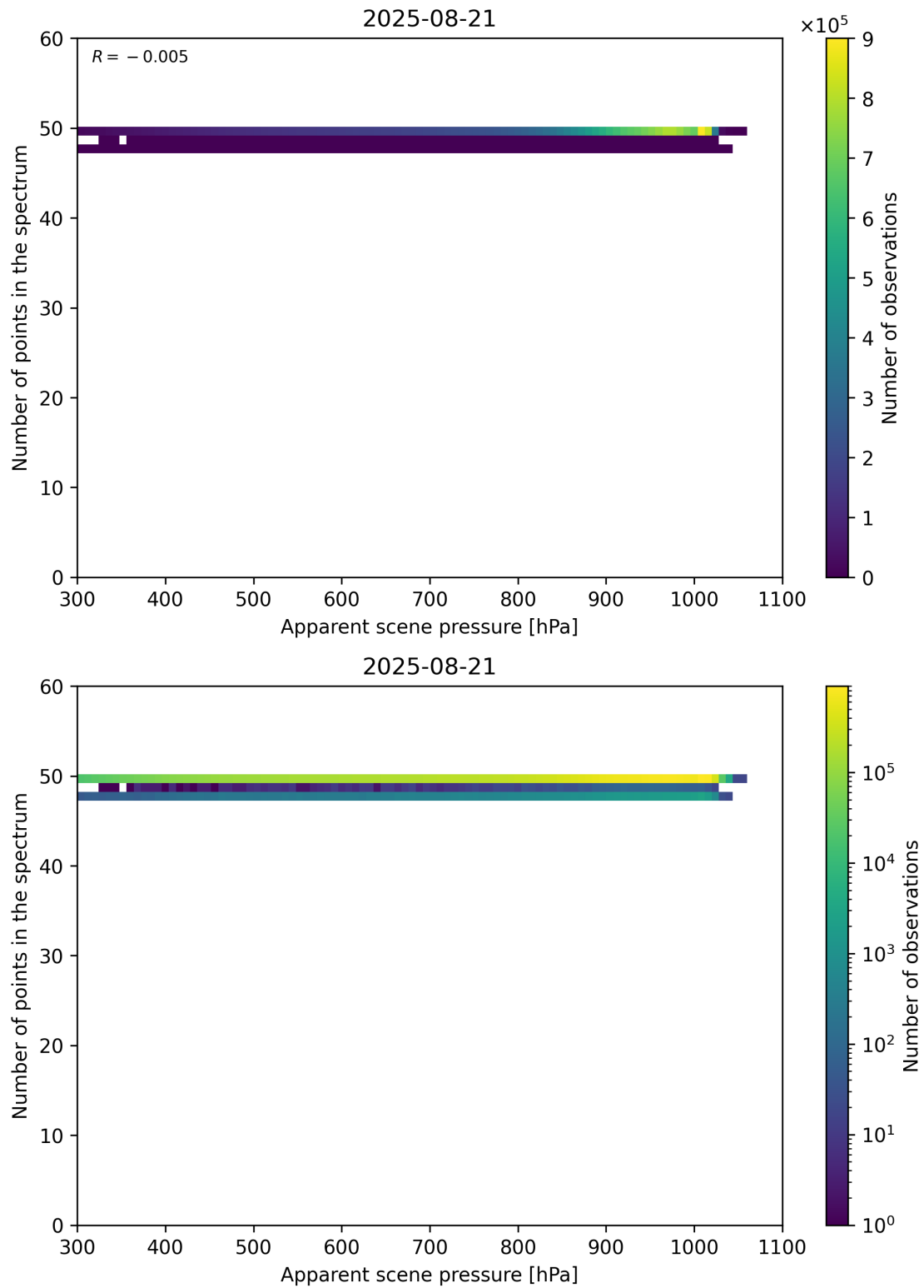
Figure 66: Scatter density plot of “Apparent scene pressure” against “Number of points in the spectrum” for 2025-08-20 to 2025-08-22.
