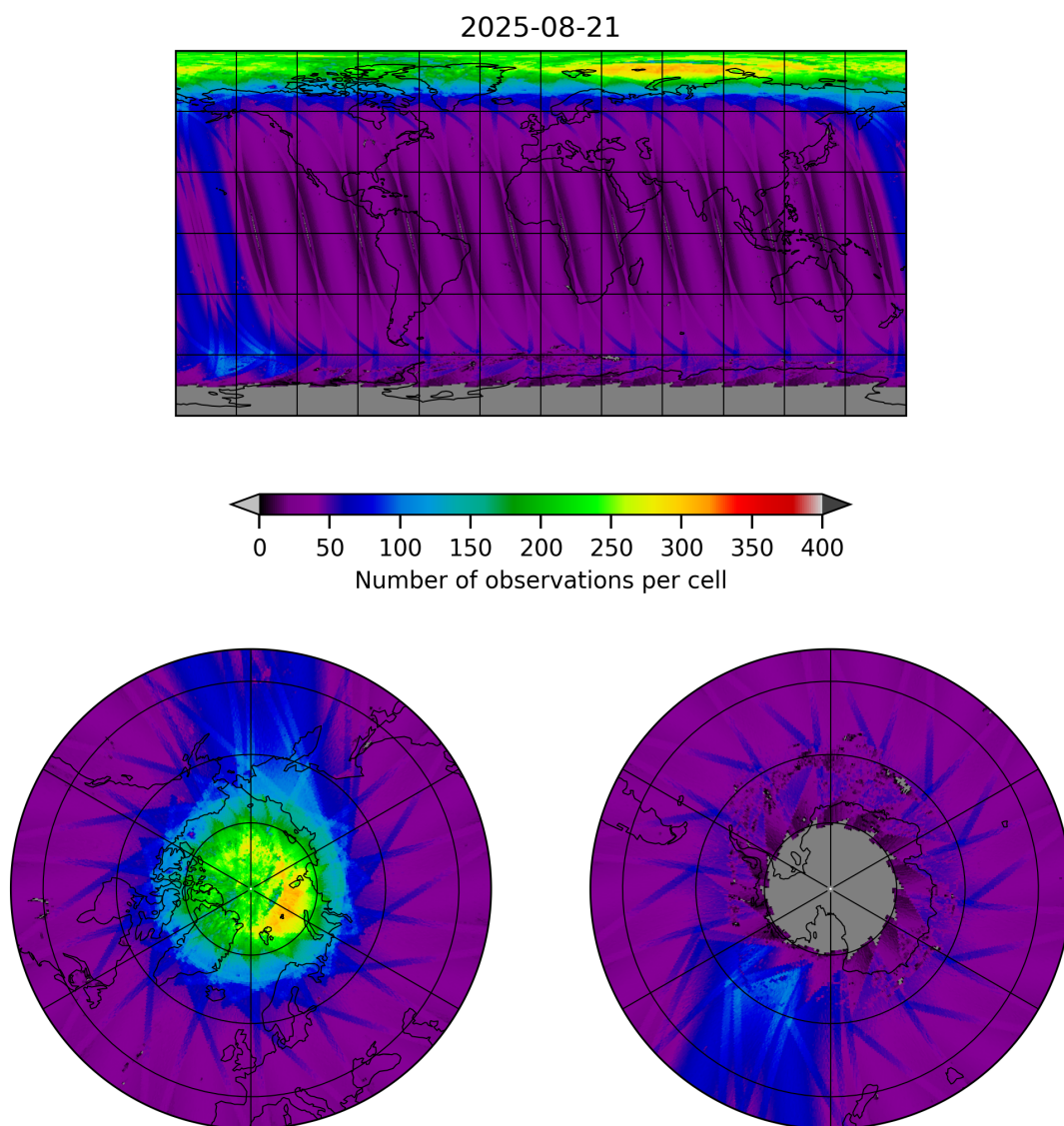
Figure 11: Map of the number of observations for 2025-08-20 to 2025-08-22
