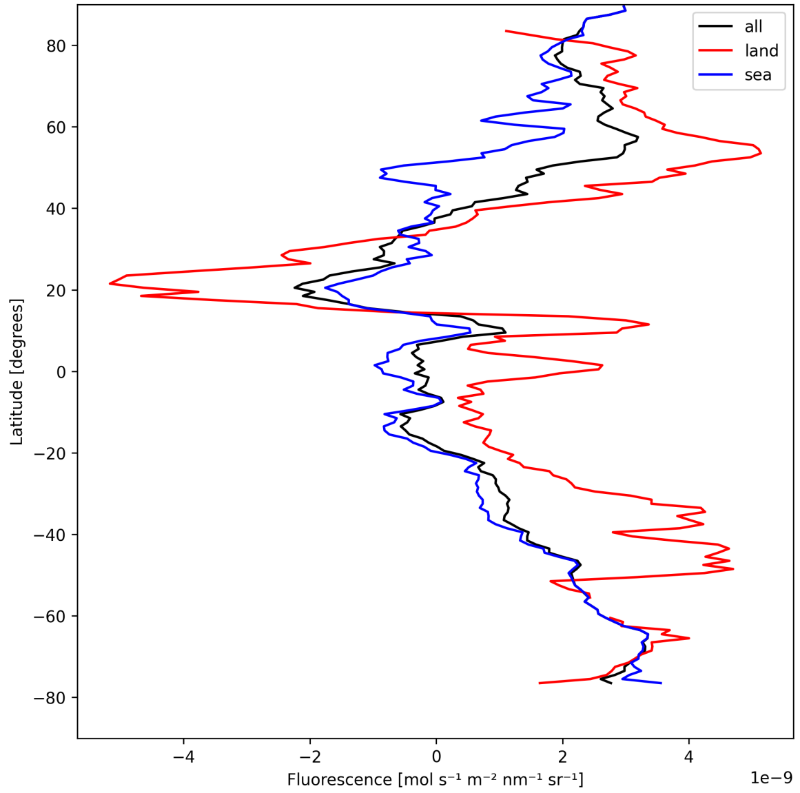
Figure 23: Zonal average of “Fluorescence” for 2025-08-20 to 2025-08-22.
