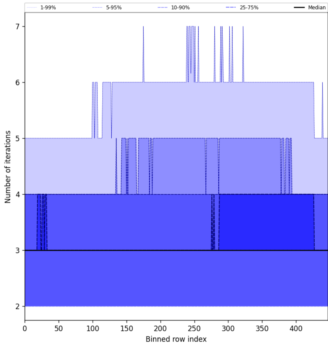
Figure 56: Along track statistics of “Number of iterations” for 2025-08-20 to 2025-08-22
