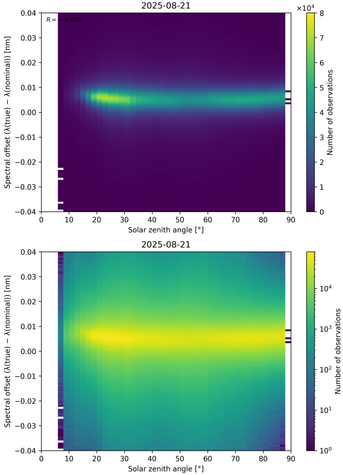
Figure 117: Scatter density plot of “Solar zenith angle” against “Spectral offset ( \lambda_{\text{true}} - \lambda_{\text{nominal}} )” for 2025-08-20 to 2025-08-22.
