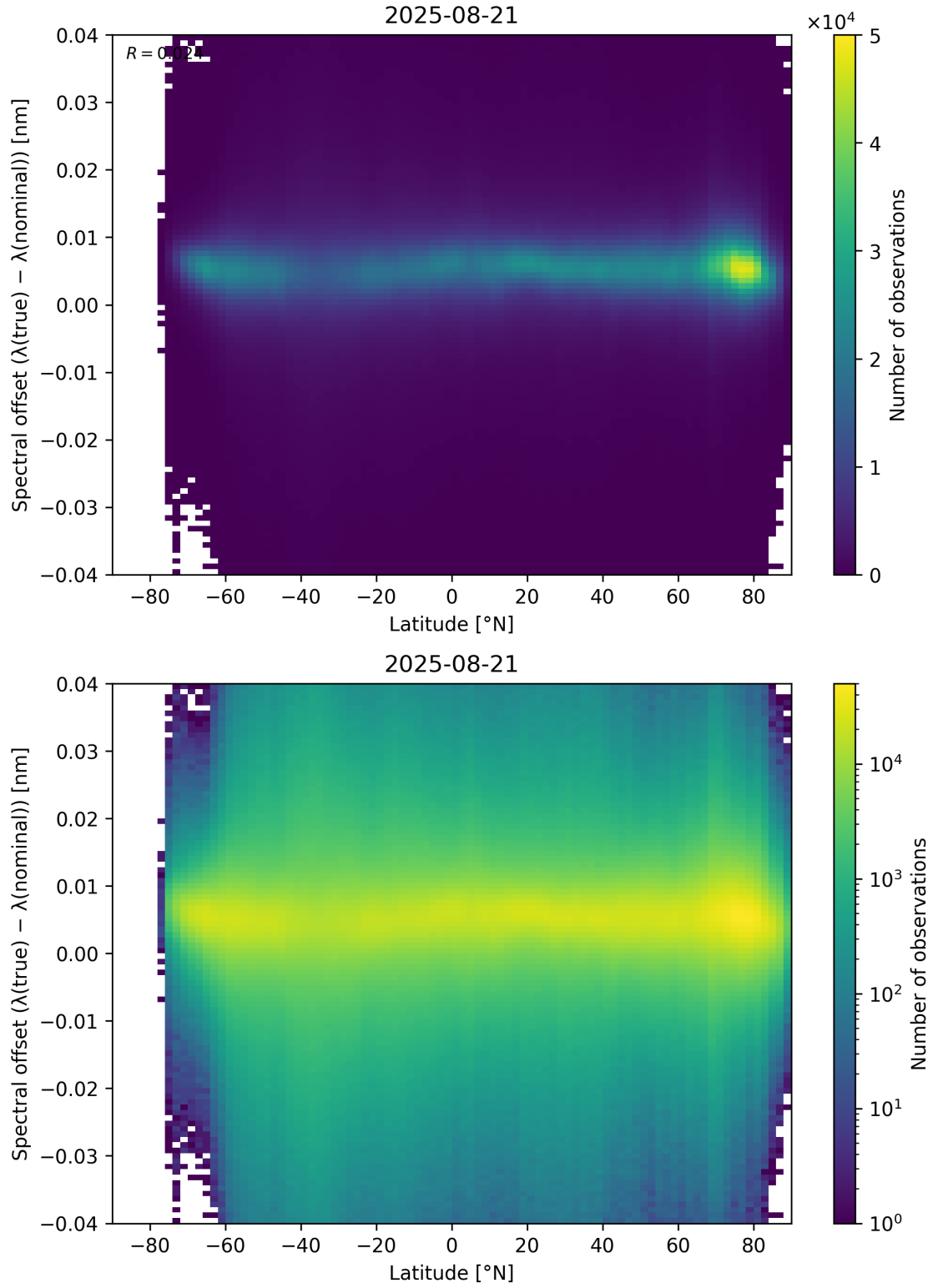
Figure 96: Scatter density plot of “Latitude” against “Spectral offset ( \lambda_{\text{true}} - \lambda_{\text{nominal}} )” for 2025-08-20 to 2025-08-22.
