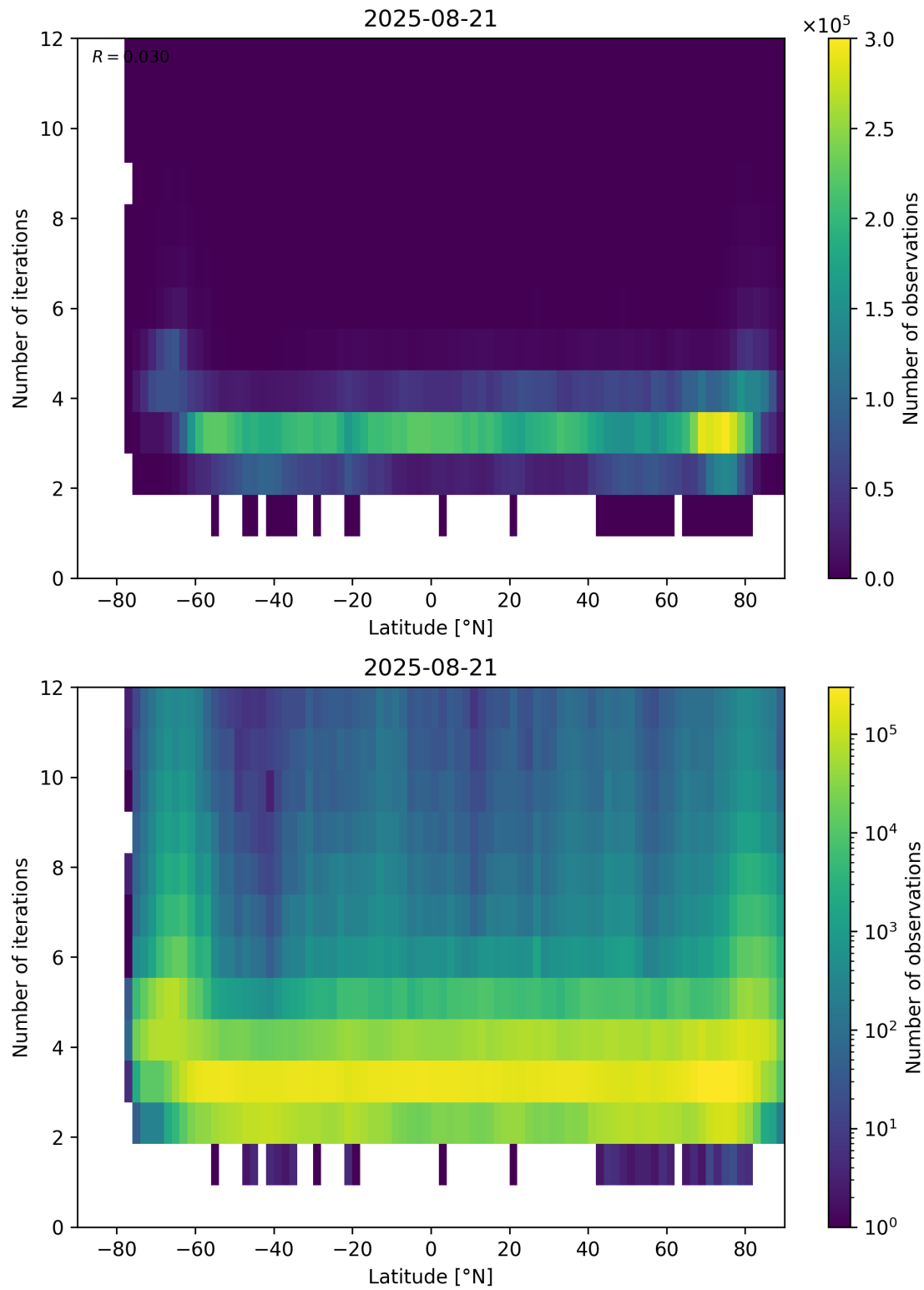
Figure 93: Scatter density plot of “Latitude” against “Number of iterations” for 2025-08-20 to 2025-08-22.
