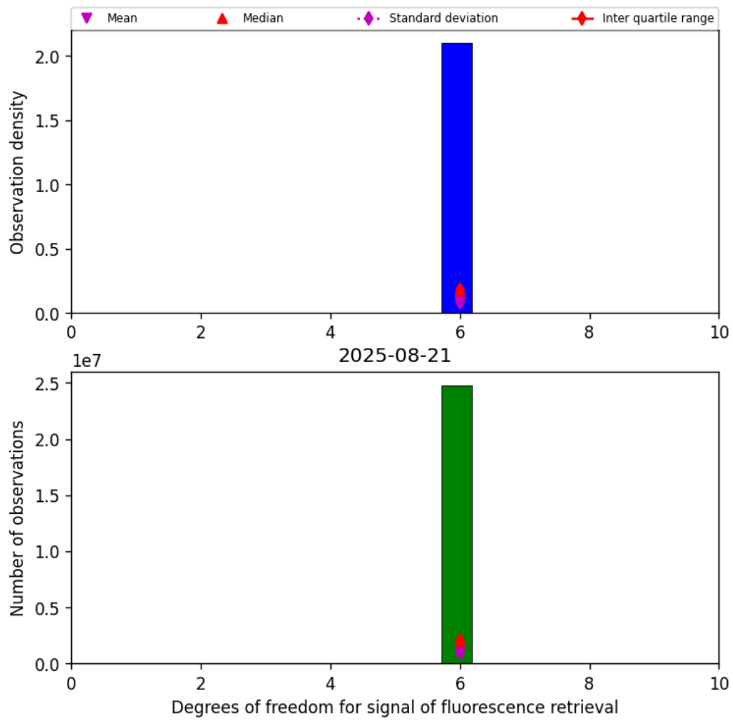
Figure 43: Histogram of "Degrees of freedom for signal of fluorescence retrieval" for 2025-08-20 to 2025-08-22
