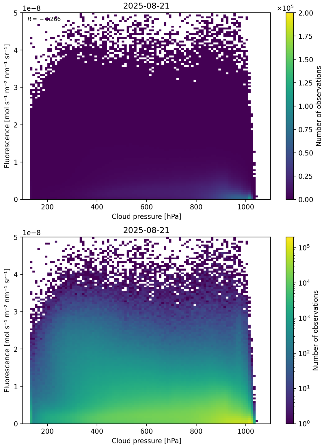
Figure 80: Scatter density plot of “Cloud pressure” against “Fluorescence” for 2025-08-20 to 2025-08-22.
