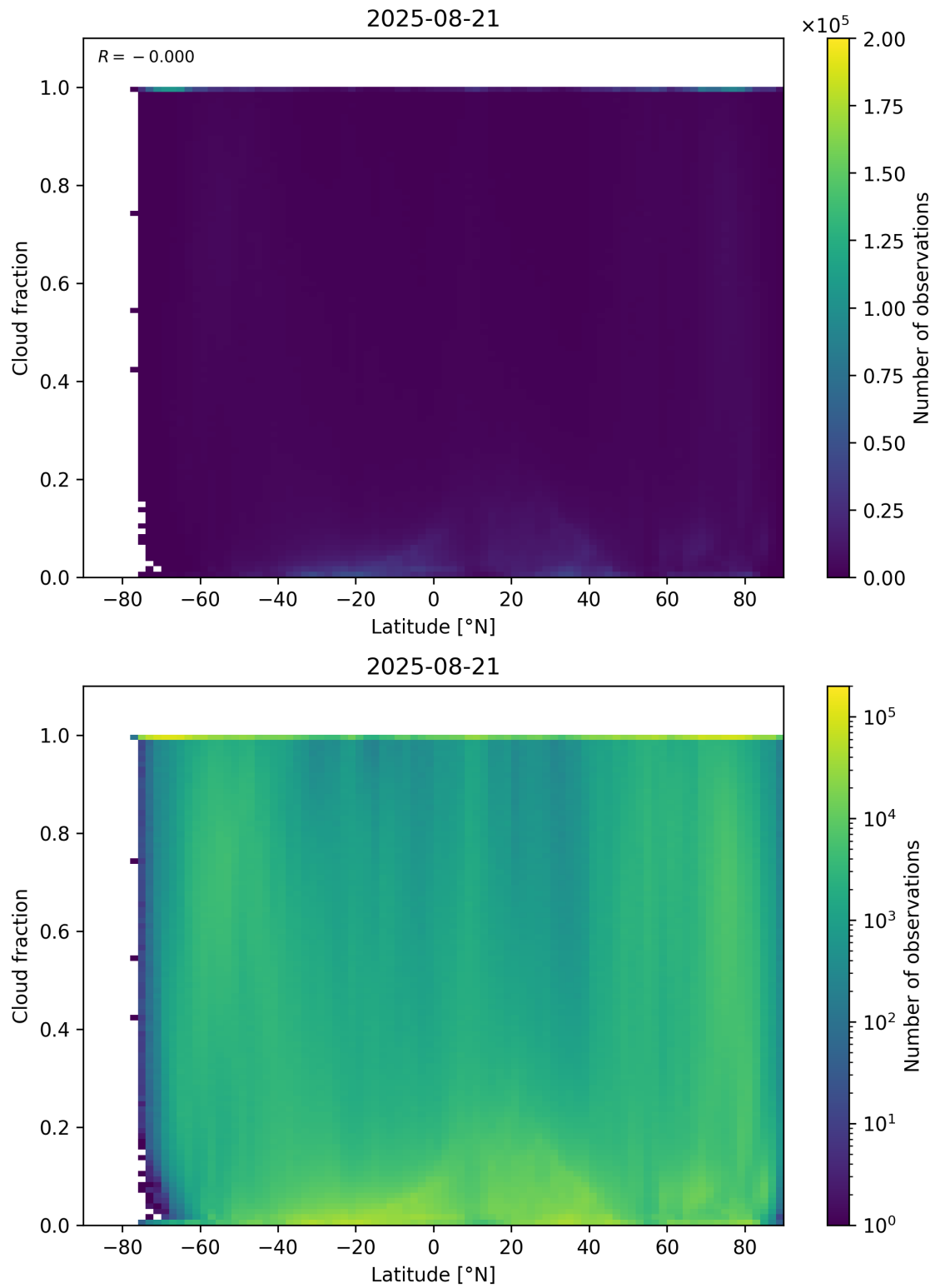
Figure 90: Scatter density plot of “Latitude” against “Cloud fraction” for 2025-08-20 to 2025-08-22.
