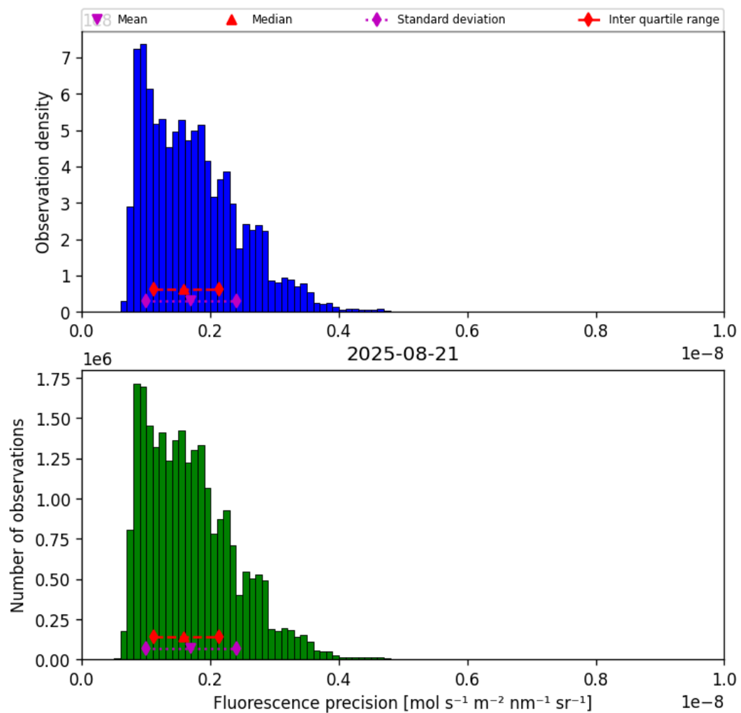
Figure 41: Histogram of “Fluorescence precision” for 2025-08-20 to 2025-08-22
