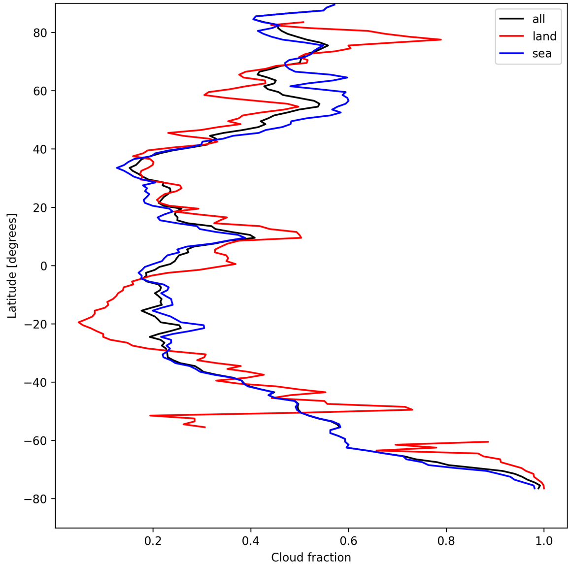
Figure 15: Zonal average of “Cloud fraction” for 2025-08-20 to 2025-08-22.
