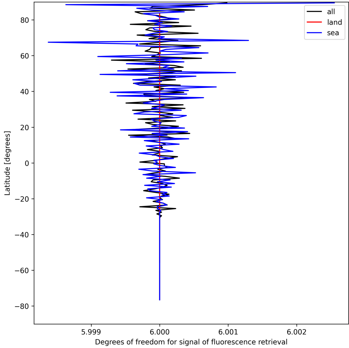
Figure 26: Zonal average of “Degrees of freedom for signal of fluorescence retrieval” for 2025-08-20 to 2025-08-22.
