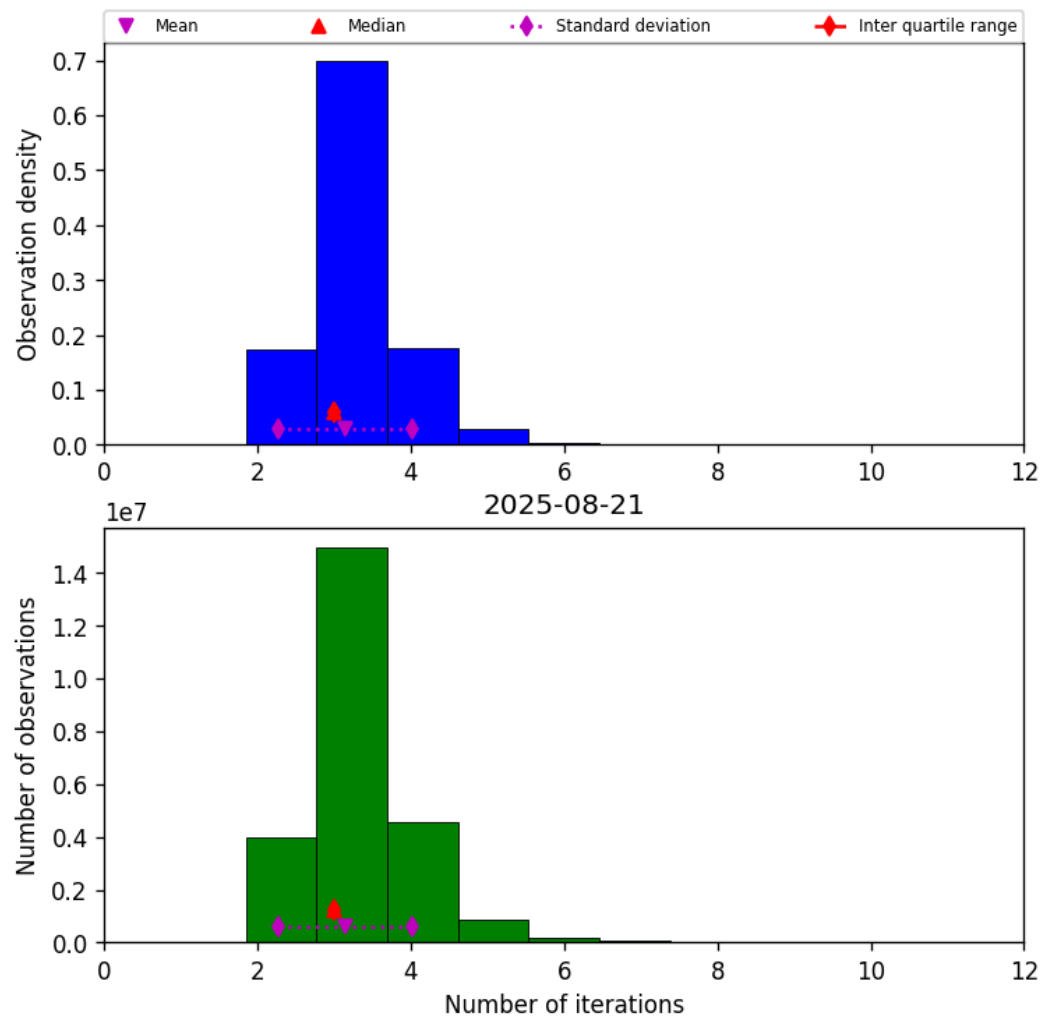
Figure 39: Histogram of “Number of iterations” for 2025-08-20 to 2025-08-22
