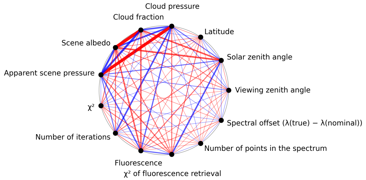
Figure 1: Map of correlation graph for 2025-08-20 to 2025-08-22.
