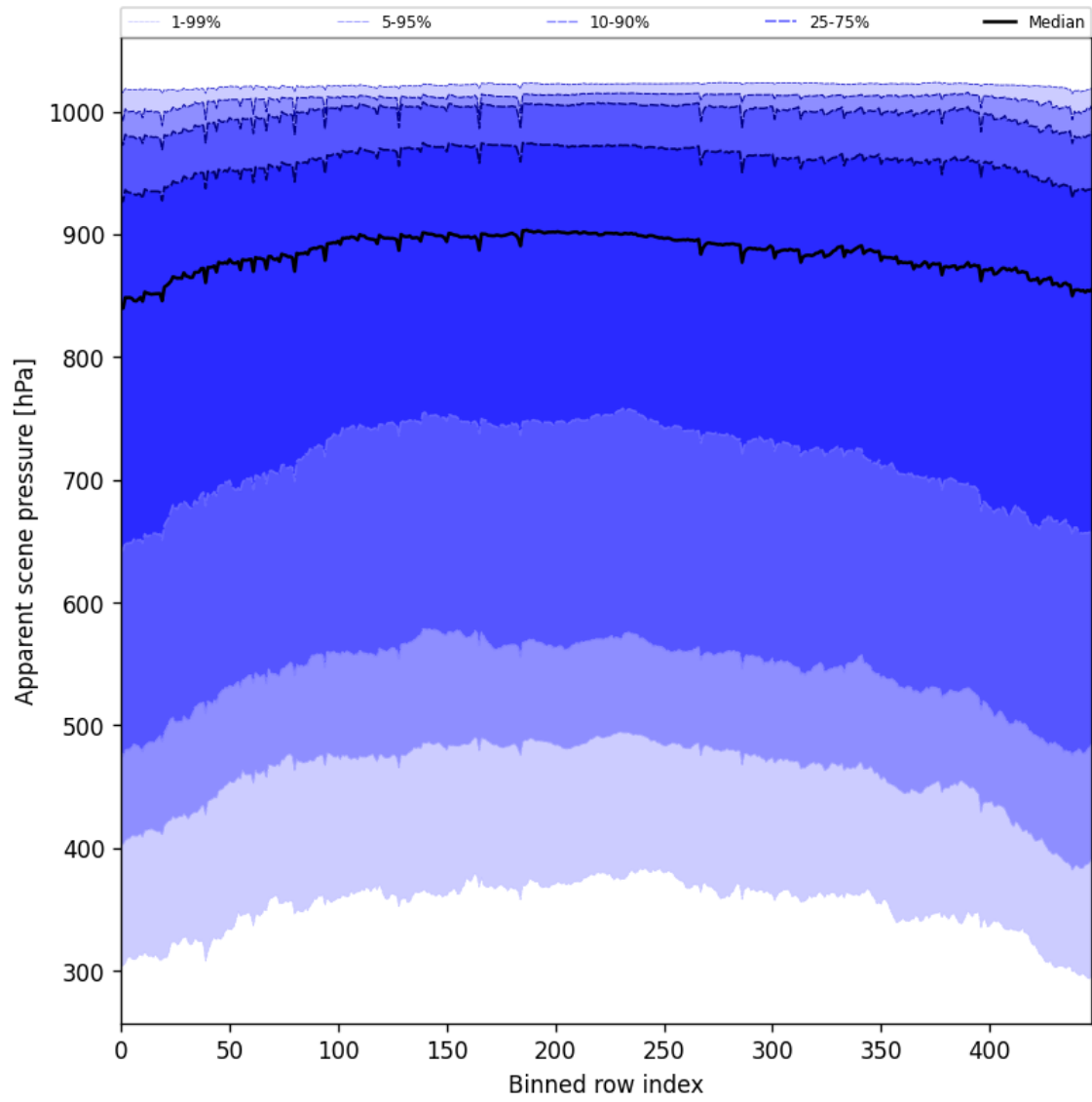
Figure 53: Along track statistics of “Apparent scene pressure” for 2025-08-20 to 2025-08-22
