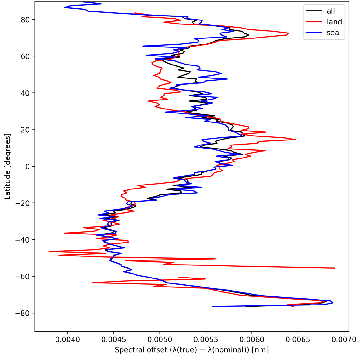
Figure 28: Zonal average of “Spectral offset ( \lambda_{\text{true}} - \lambda_{\text{nominal}} )” for 2025-08-20 to 2025-08-22.
