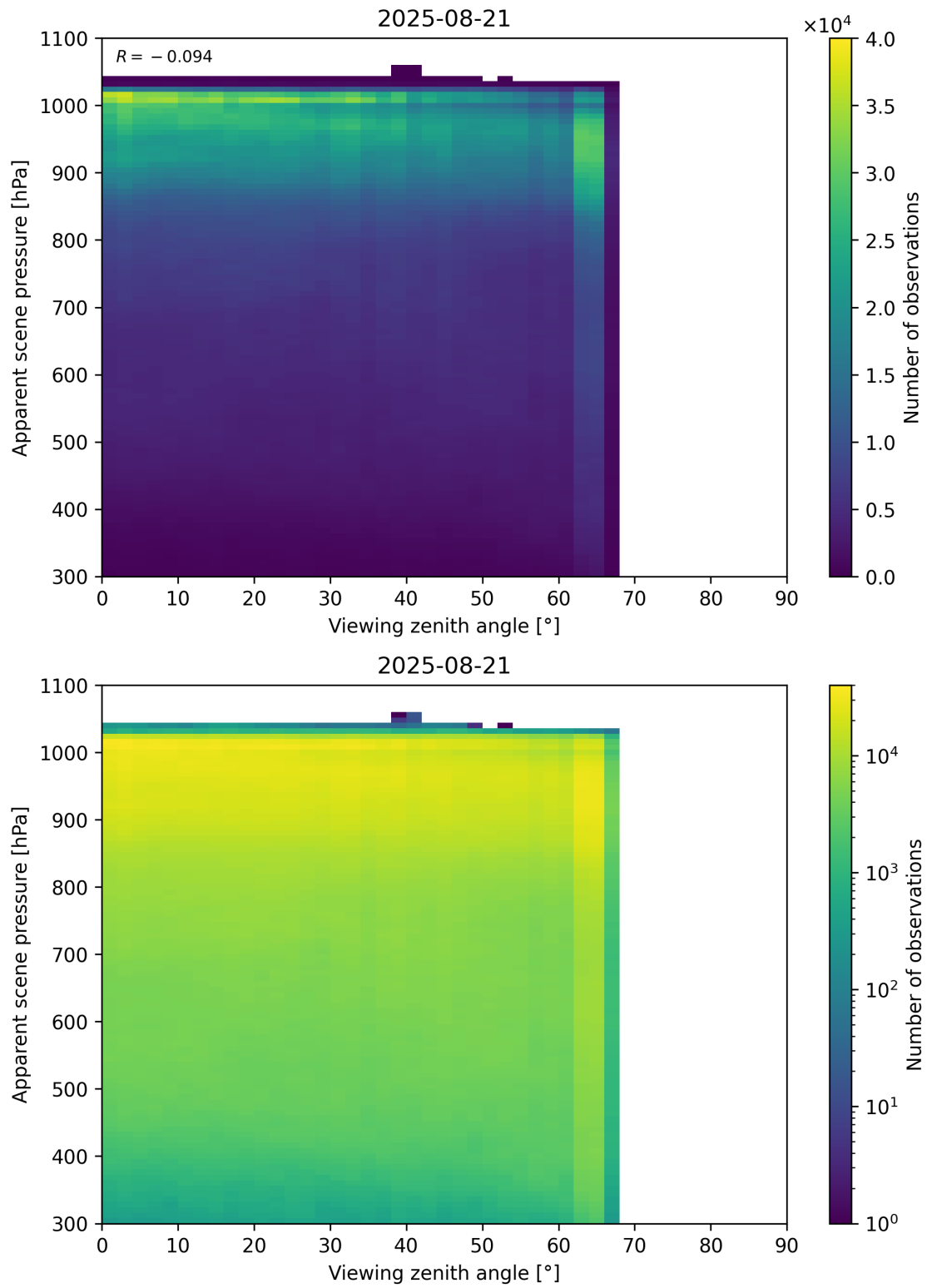
Figure 118: Scatter density plot of “Viewing zenith angle” against “Apparent scene pressure” for 2025-08-20 to 2025-08-22.
