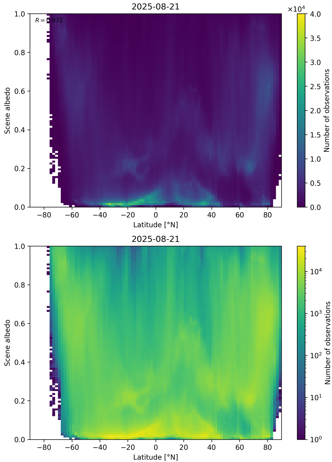
Figure 95: Scatter density plot of “Latitude” against “Scene albedo” for 2025-08-20 to 2025-08-22.
