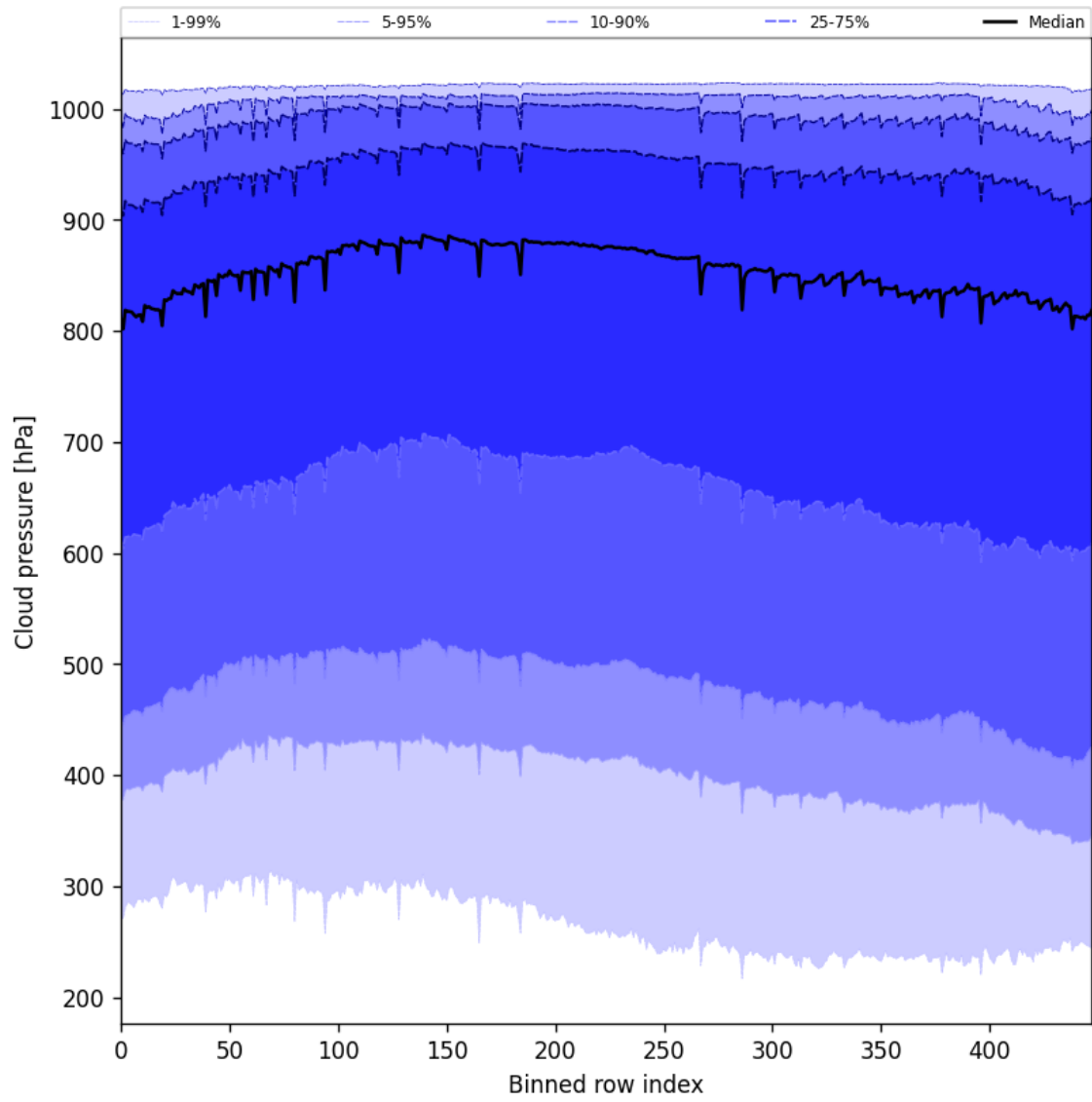
Figure 47: Along track statistics of “Cloud pressure” for 2025-08-20 to 2025-08-22
