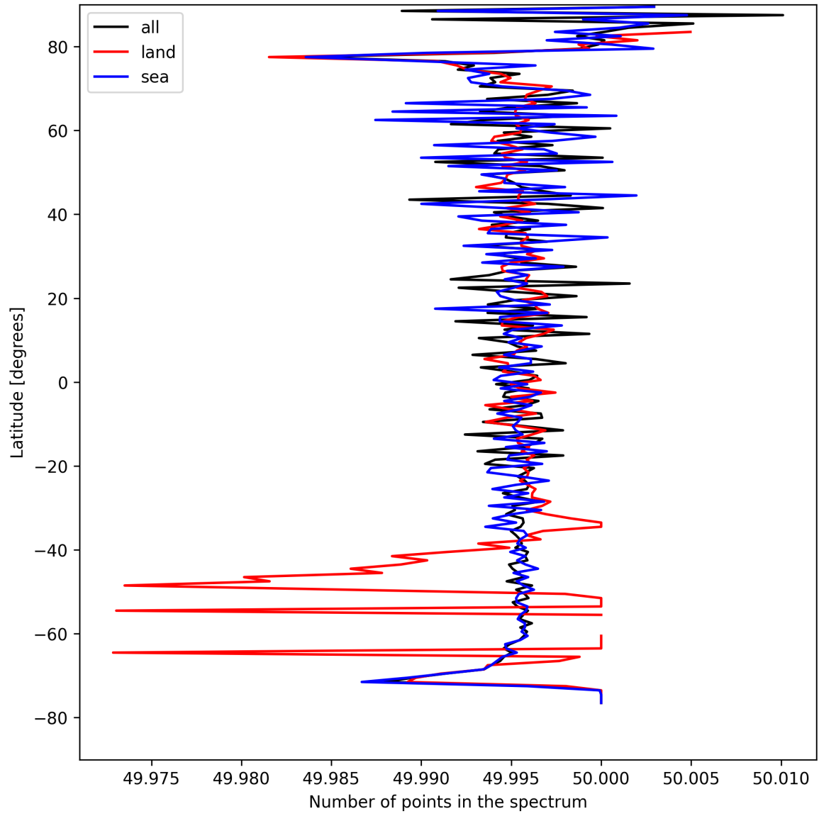
Figure 27: Zonal average of “Number of points in the spectrum” for 2025-08-20 to 2025-08-22.
