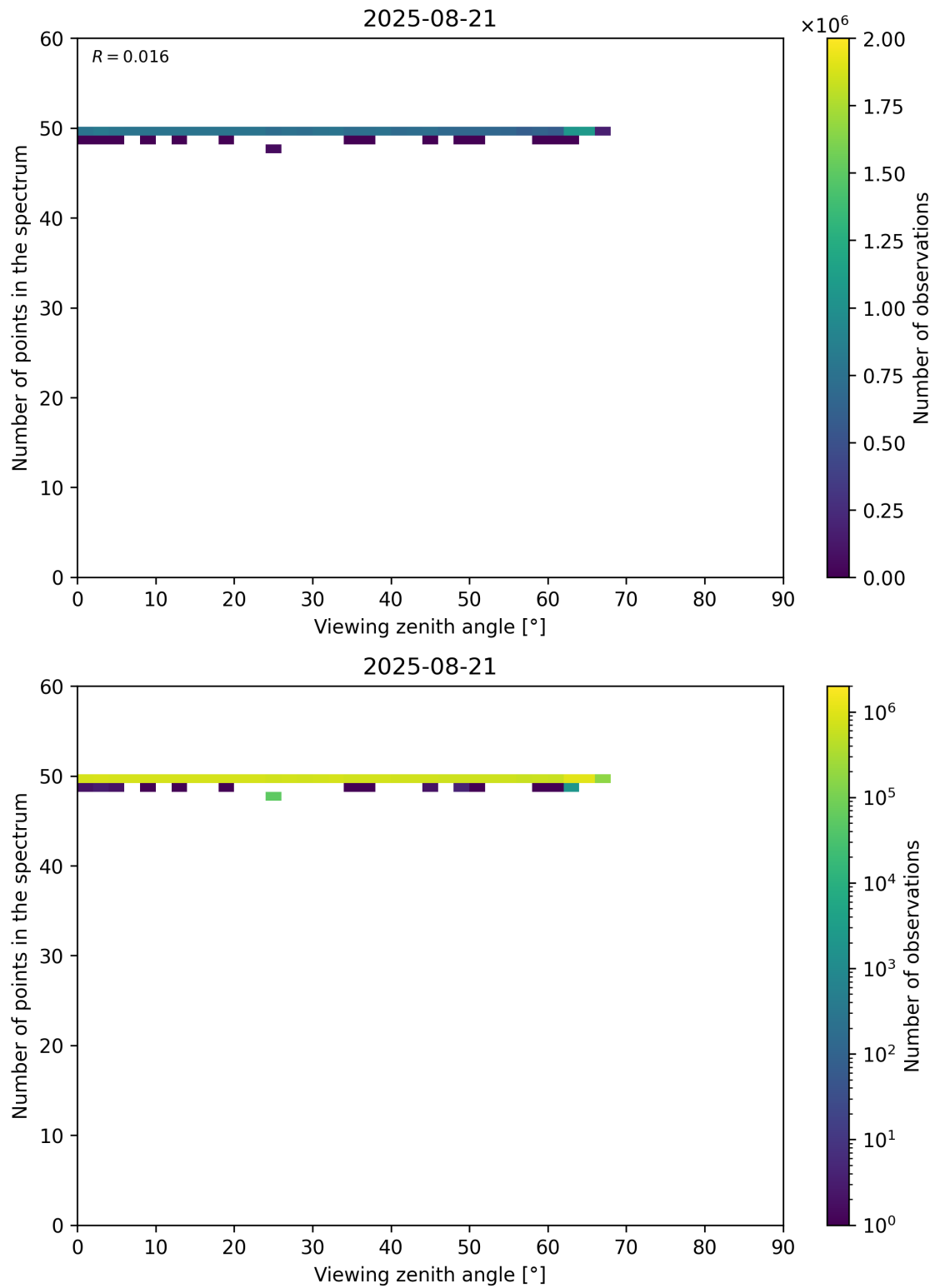
Figure 125: Scatter density plot of “Viewing zenith angle” against “Number of points in the spectrum” for 2025-08-20 to 2025-08-22.
