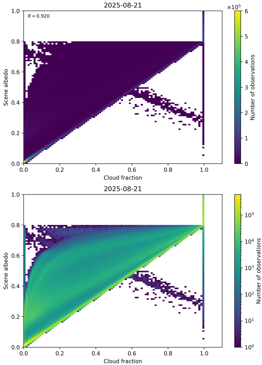
Figure 75: Scatter density plot of “Cloud fraction” against “Scene albedo” for 2025-08-20 to 2025-08-22.
