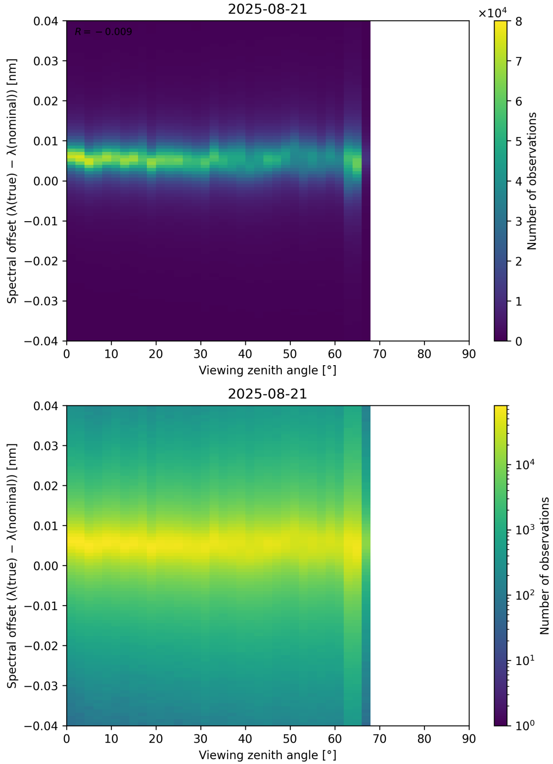
Figure 128: Scatter density plot of “Viewing zenith angle” against “Spectral offset ( \lambda_{\text{true}} - \lambda_{\text{nominal}} )” for 2025-08-20 to 2025-08-22.
