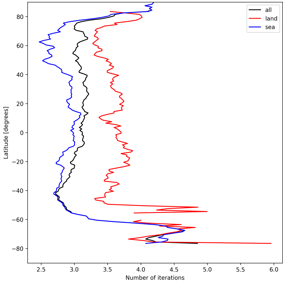
Figure 22: Zonal average of “Number of iterations” for 2025-08-20 to 2025-08-22.
