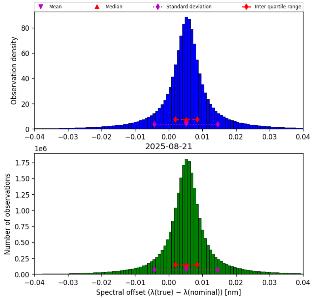
Figure 45: Histogram of “Spectral offset ( \lambda_{\text{true}} - \lambda_{\text{nominal}} )” for 2025-08-20 to 2025-08-22
