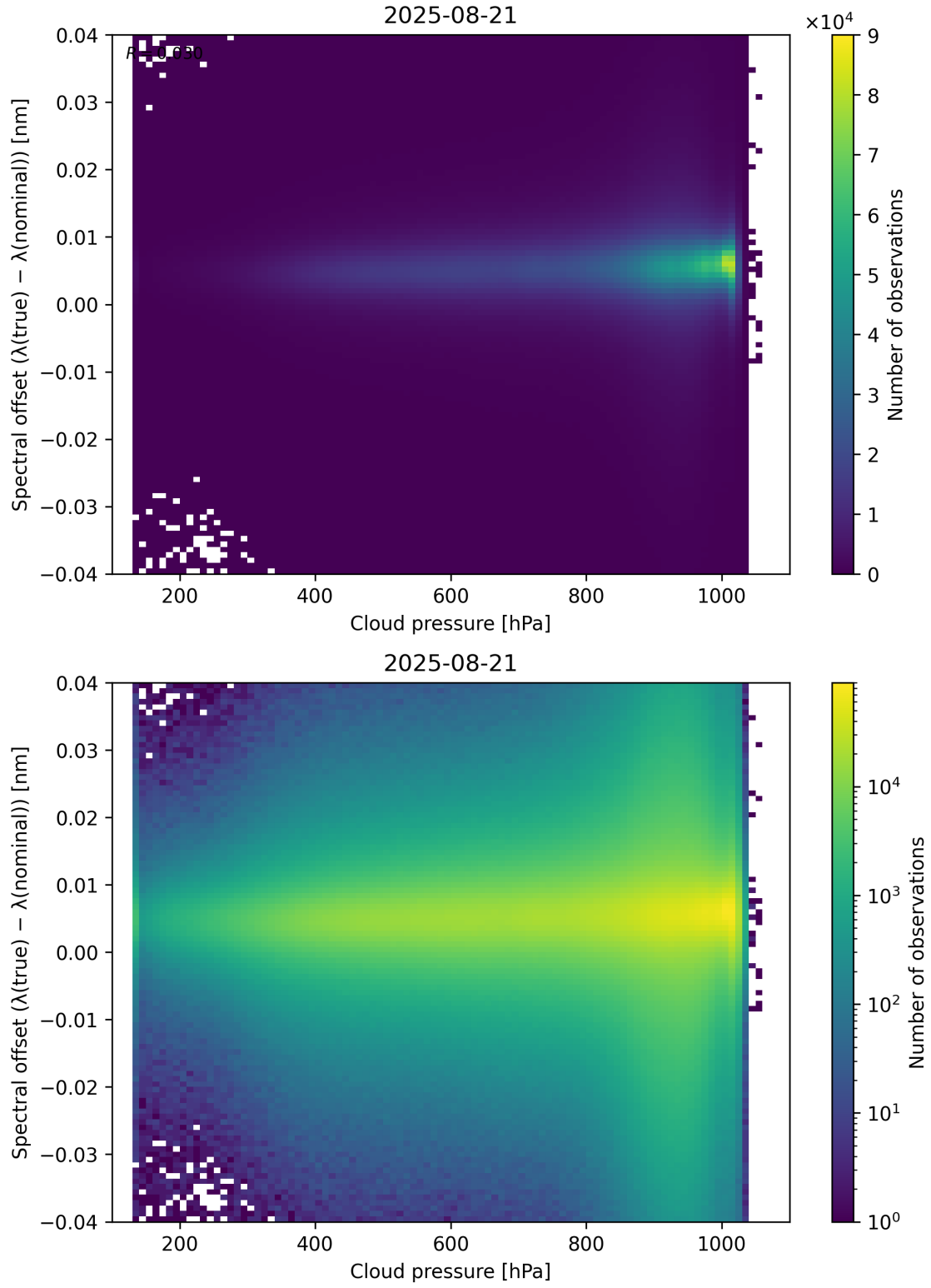
Figure 84: Scatter density plot of “Cloud pressure” against “Spectral offset ( \lambda_{\text{true}} - \lambda_{\text{nominal}} )” for 2025-08-20 to 2025-08-22.
