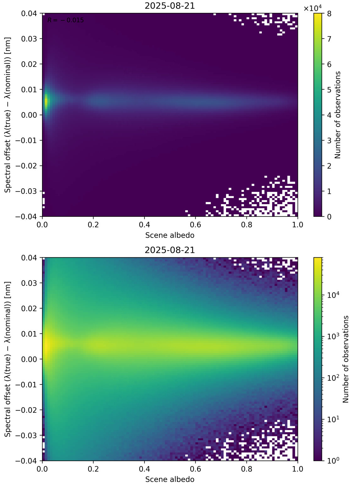
Figure 107: Scatter density plot of “Scene albedo” against “Spectral offset ( \lambda_{\text{true}} - \lambda_{\text{nominal}} )” for 2025-08-20 to 2025-08-22.
