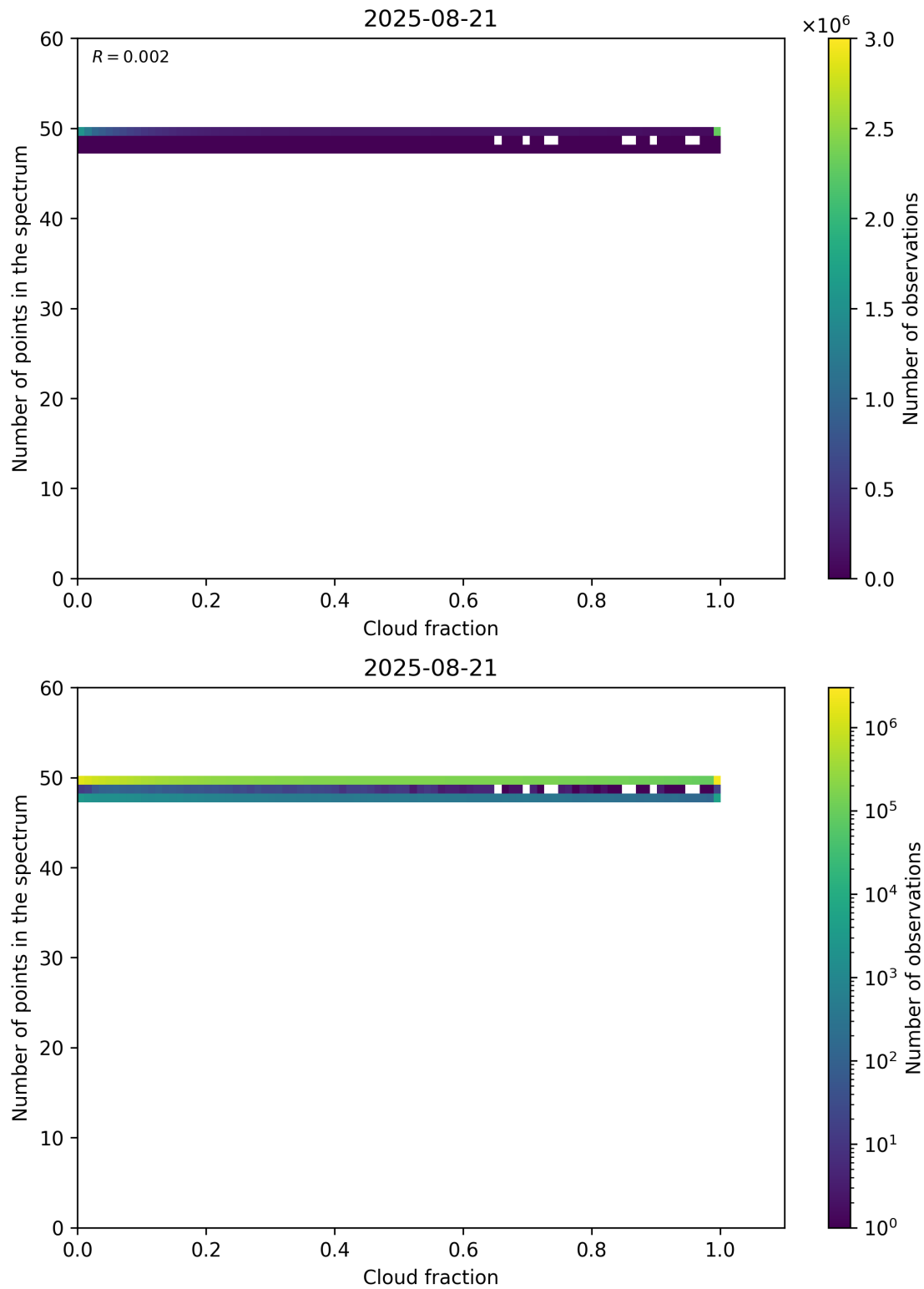
Figure 74: Scatter density plot of “Cloud fraction” against “Number of points in the spectrum” for 2025-08-20 to 2025-08-22.
