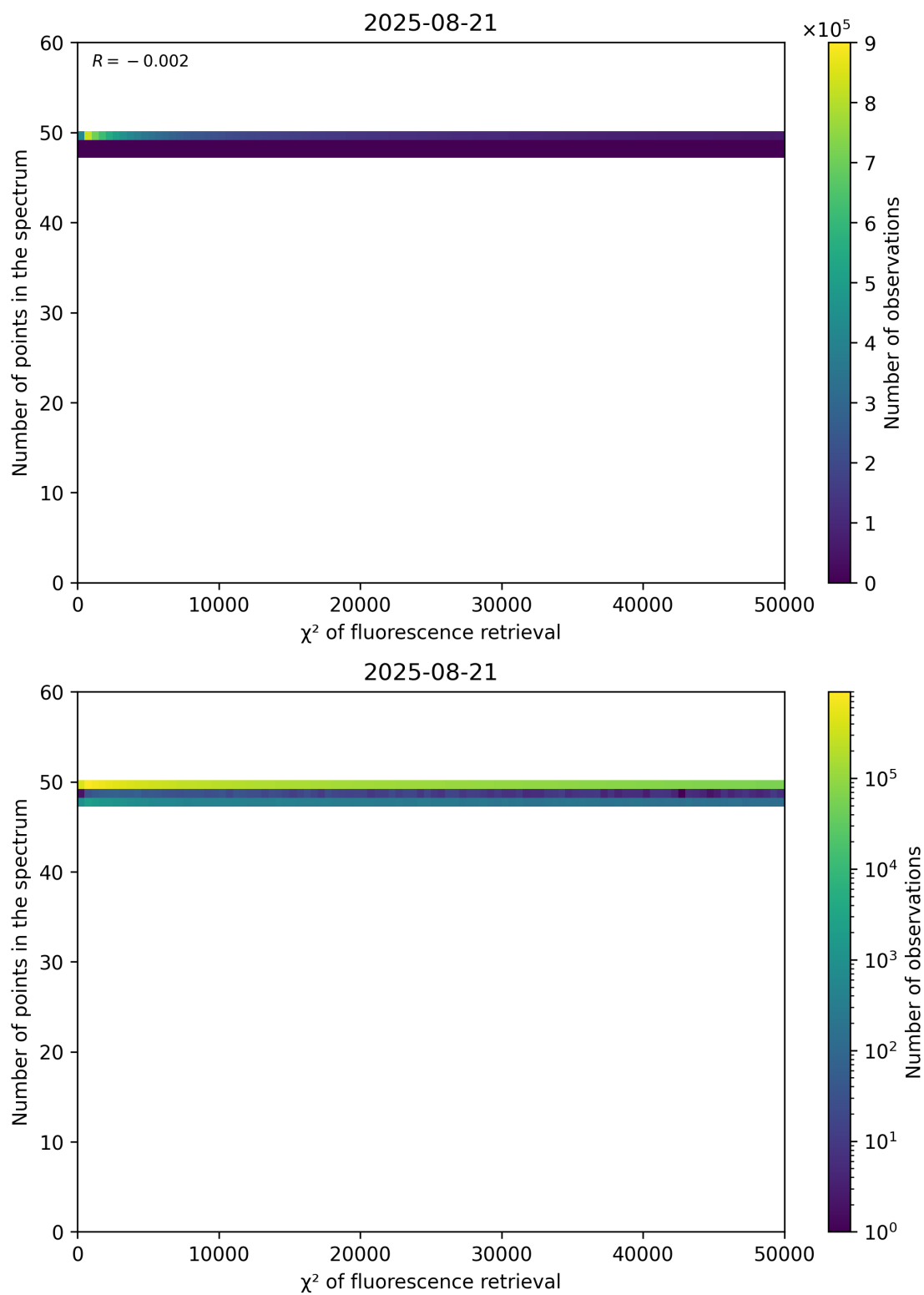
Figure 68: Scatter density plot of “ \chi^2 of fluorescence retrieval” against “Number of points in the spectrum” for 2025-08-20 to 2025-08-22.
