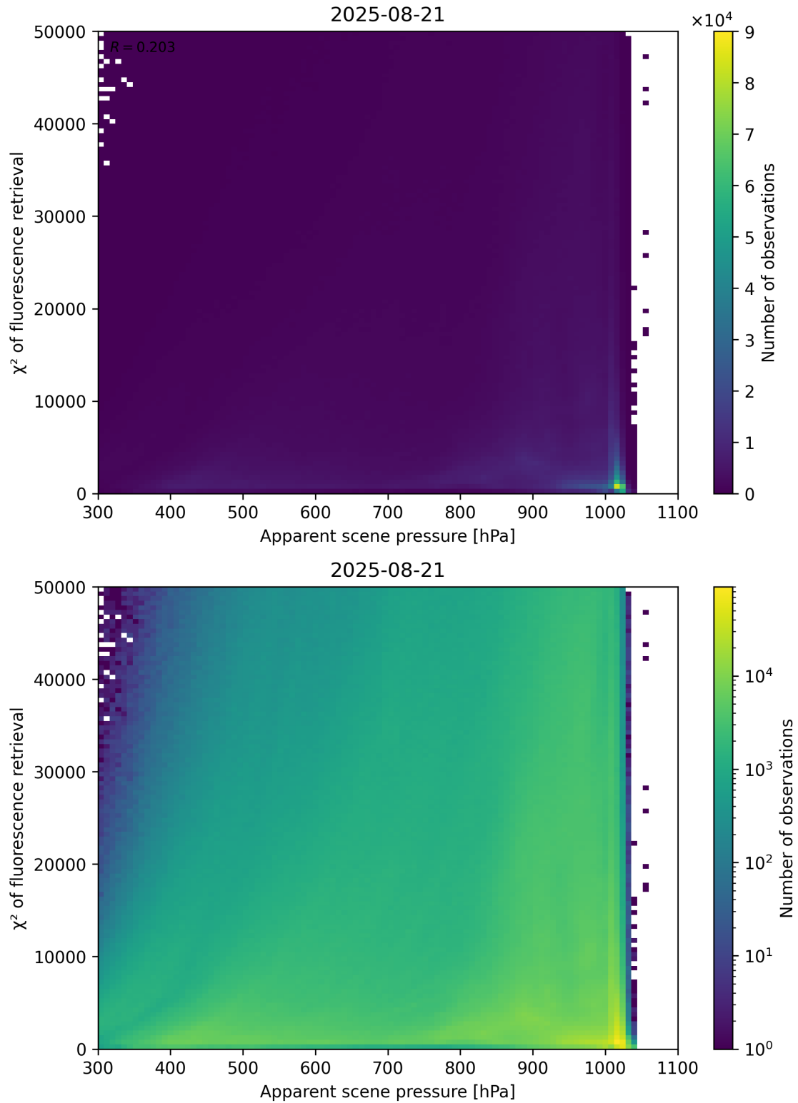
Figure 63: Scatter density plot of “Apparent scene pressure” against “ \chi^2 of fluorescence retrieval” for 2025-08-20 to 2025-08-22.
