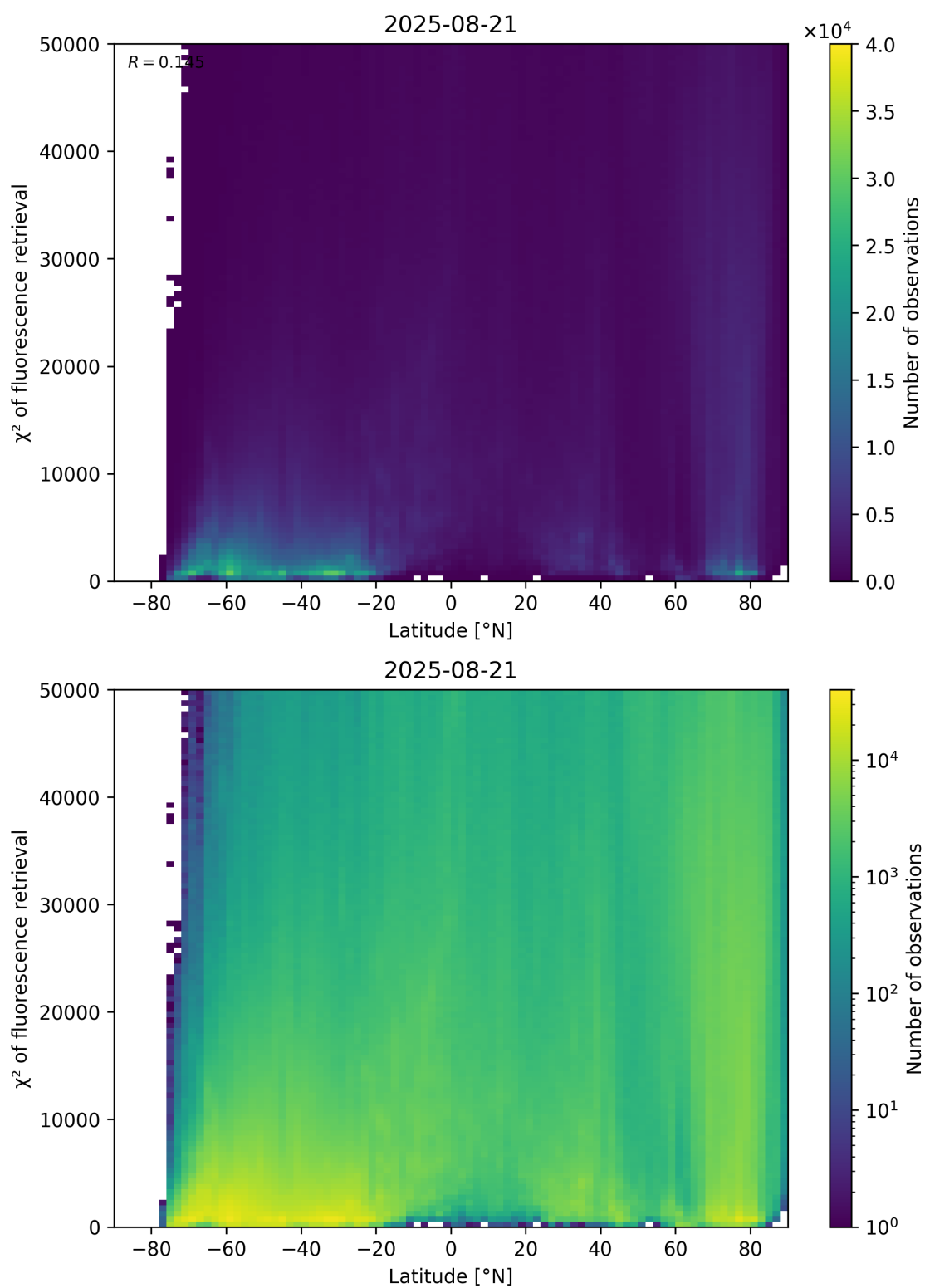
Figure 89: Scatter density plot of “Latitude” against “ \chi^2 of fluorescence retrieval” for 2025-08-20 to 2025-08-22.
