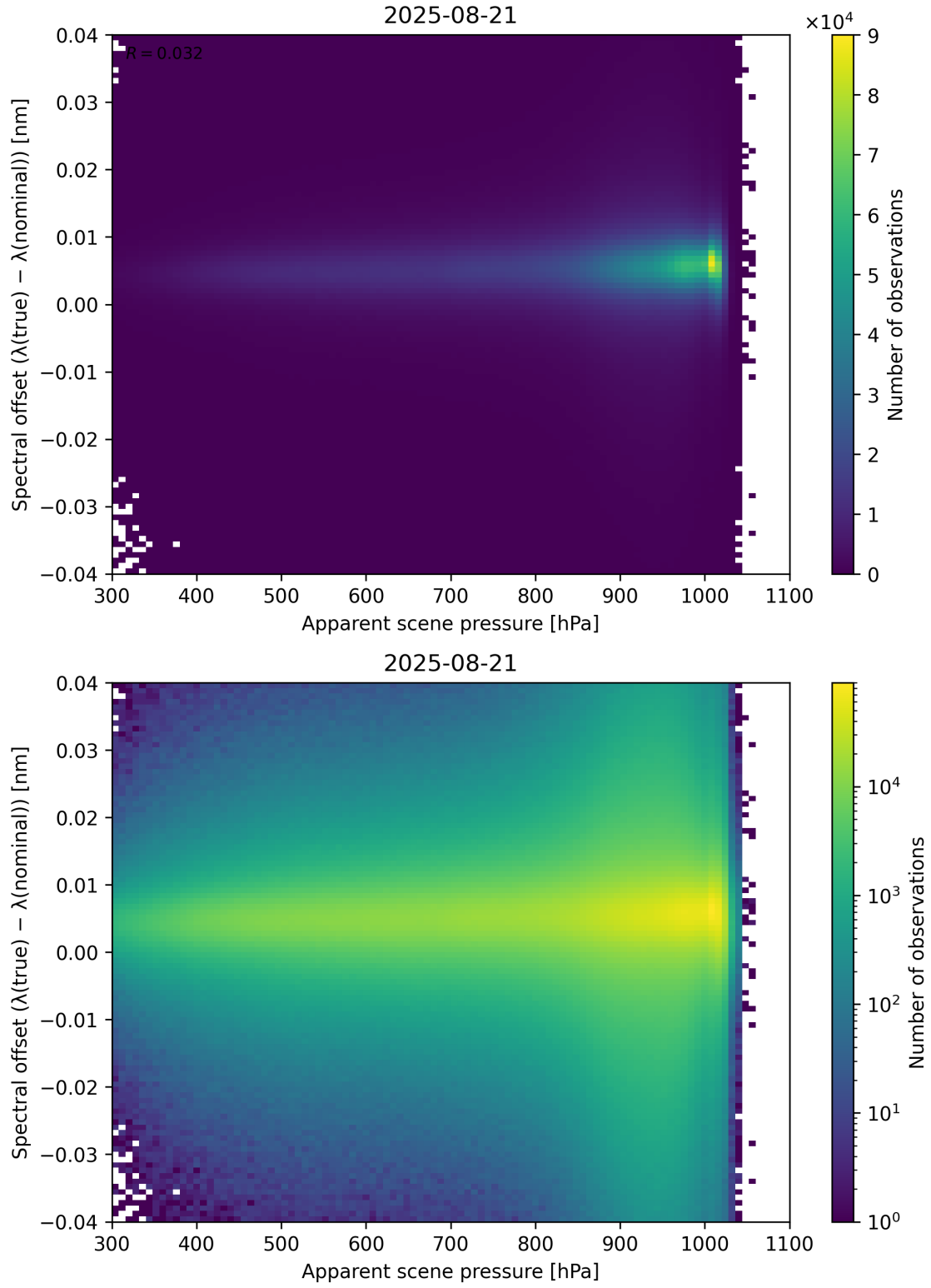
Figure 67: Scatter density plot of “Apparent scene pressure” against “Spectral offset ( \lambda_{\text{true}} - \lambda_{\text{nominal}} )” for 2025-08-20 to 2025-08-22.
