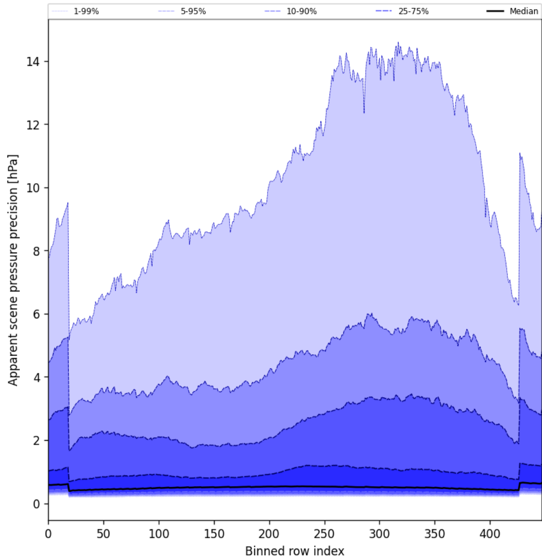
Figure 54: Along track statistics of “Apparent scene pressure precision” for 2025-08-20 to 2025-08-22
