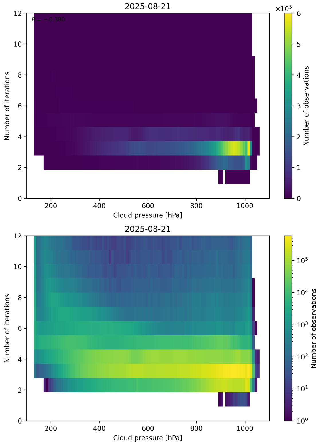
Figure 81: Scatter density plot of “Cloud pressure” against “Number of iterations” for 2025-08-20 to 2025-08-22.
