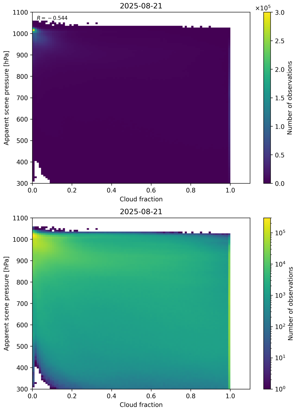
Figure 70: Scatter density plot of “Cloud fraction” against “Apparent scene pressure” for 2025-08-20 to 2025-08-22.
