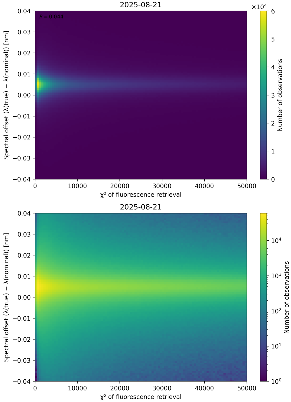
Figure 69: Scatter density plot of “ \chi^2 of fluorescence retrieval” against “Spectral offset ( \lambda_{\text{true}} - \lambda_{\text{nominal}} )” for 2025-08-20 to 2025-08-22.
