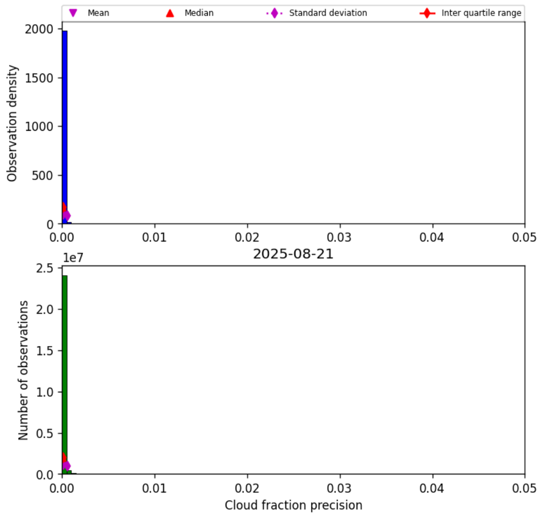
Figure 33: Histogram of “Cloud fraction precision” for 2025-08-20 to 2025-08-22
