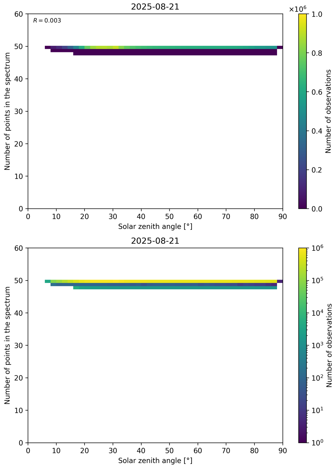
Figure 115: Scatter density plot of “Solar zenith angle” against “Number of points in the spectrum” for 2025-08-20 to 2025-08-22.
