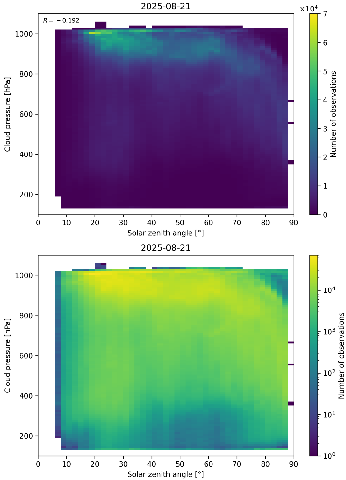
Figure 111: Scatter density plot of “Solar zenith angle” against “Cloud pressure” for 2025-08-20 to 2025-08-22.
