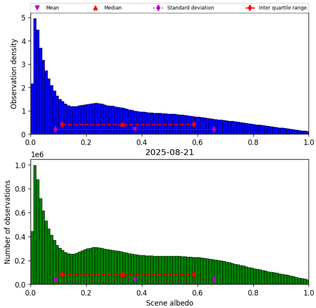
Figure 34: Histogram of “Scene albedo” for 2025-08-20 to 2025-08-22
