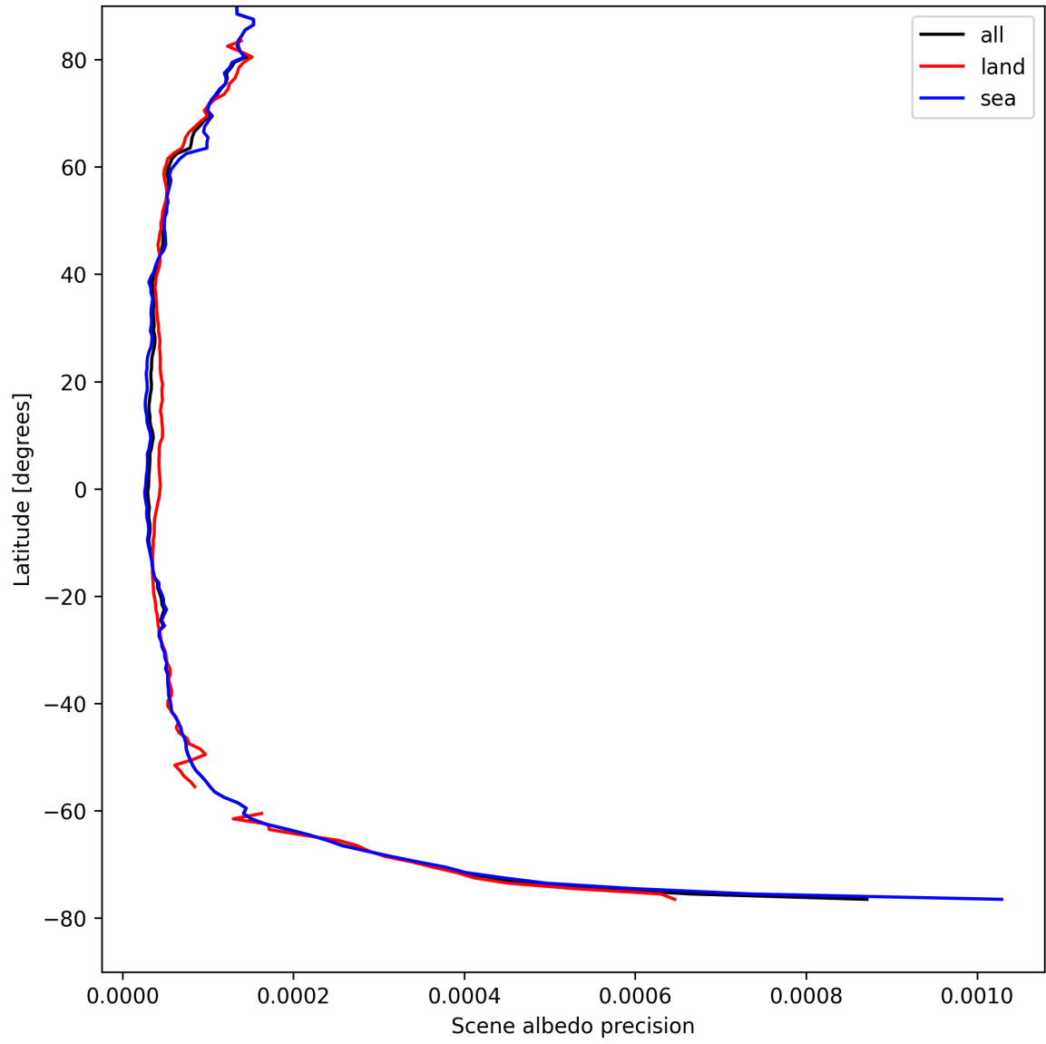
Figure 18: Zonal average of “Scene albedo precision” for 2025-08-20 to 2025-08-22.
