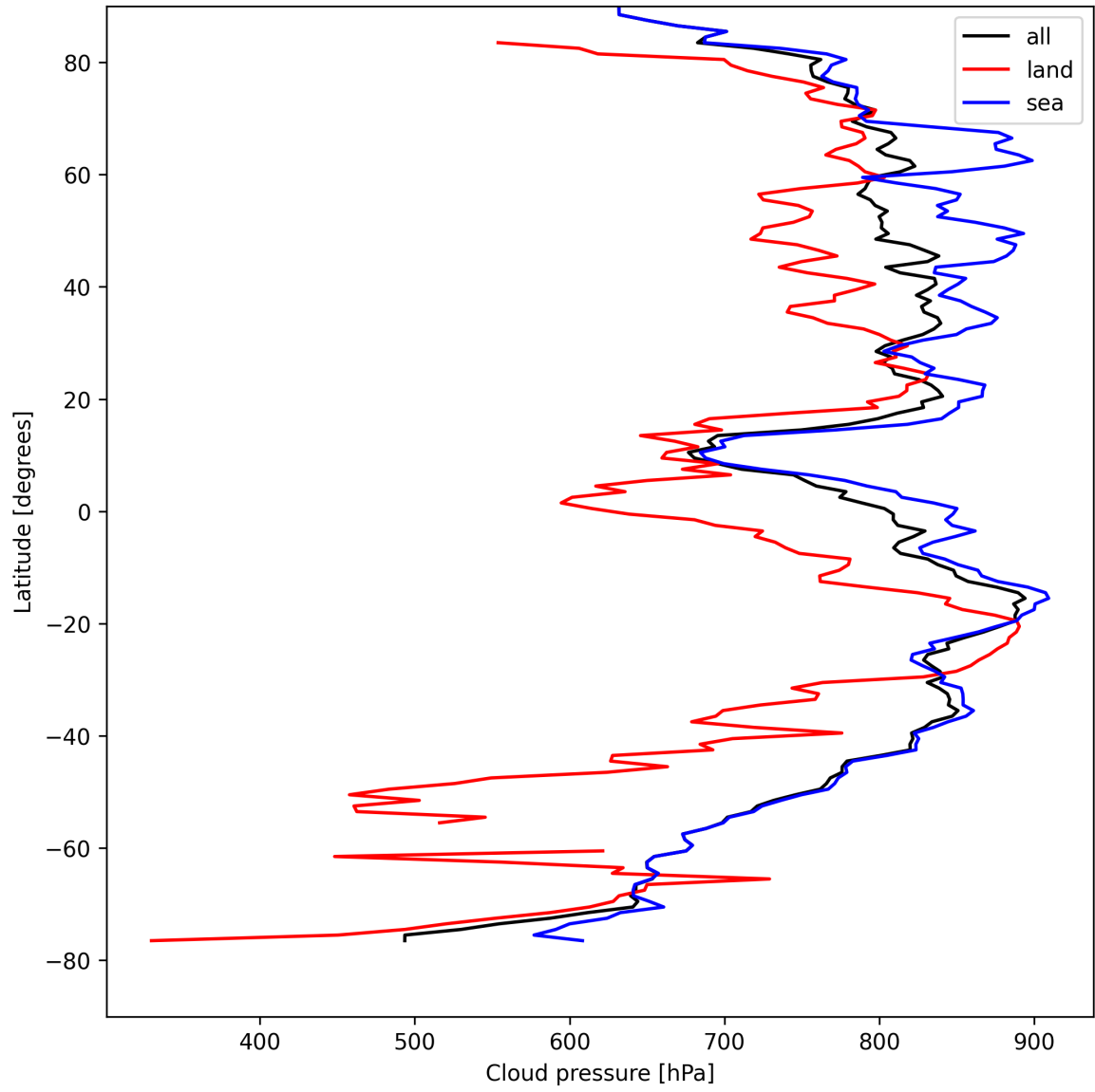
Figure 13: Zonal average of “Cloud pressure” for 2025-08-20 to 2025-08-22.
