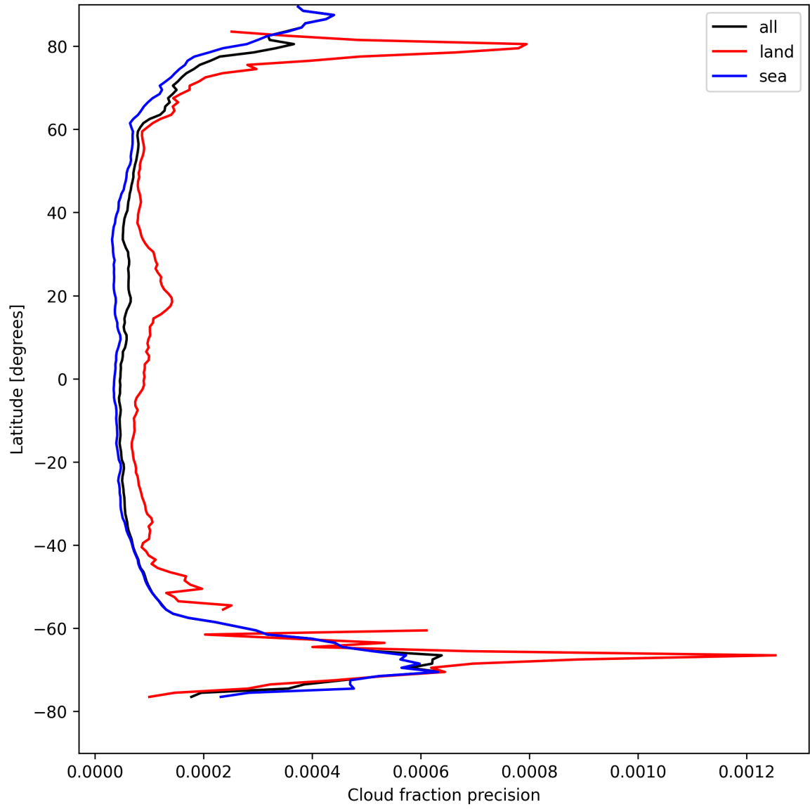
Figure 16: Zonal average of “Cloud fraction precision” for 2025-08-20 to 2025-08-22.
