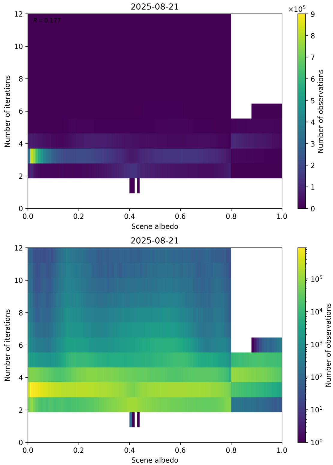
Figure 105: Scatter density plot of “Scene albedo” against “Number of iterations” for 2025-08-20 to 2025-08-22.
