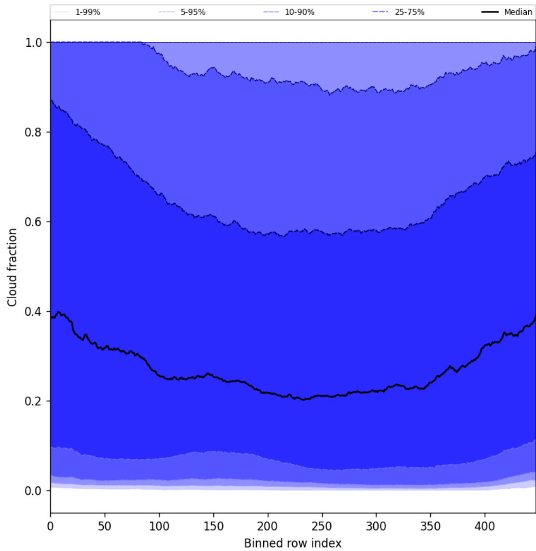
Figure 49: Along track statistics of “Cloud fraction” for 2025-08-20 to 2025-08-22
