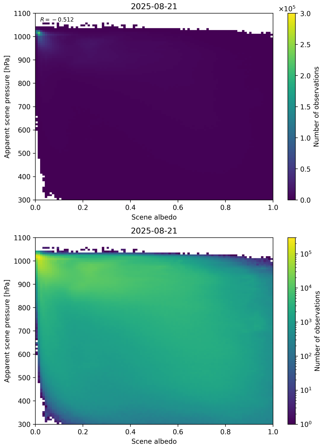
Figure 102: Scatter density plot of “Scene albedo” against “Apparent scene pressure” for 2025-08-20 to 2025-08-22.
