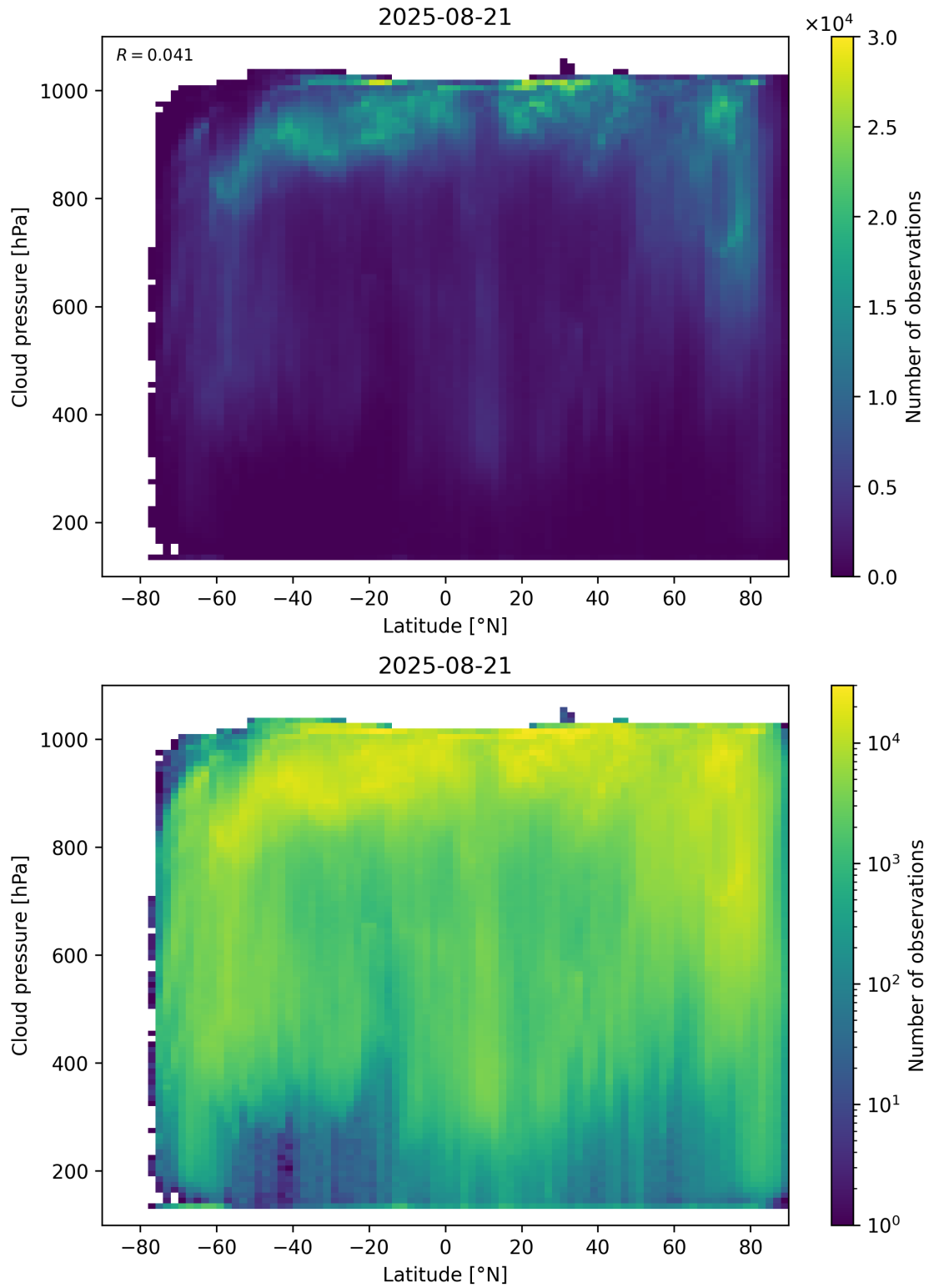
Figure 91: Scatter density plot of “Latitude” against “Cloud pressure” for 2025-08-20 to 2025-08-22.
