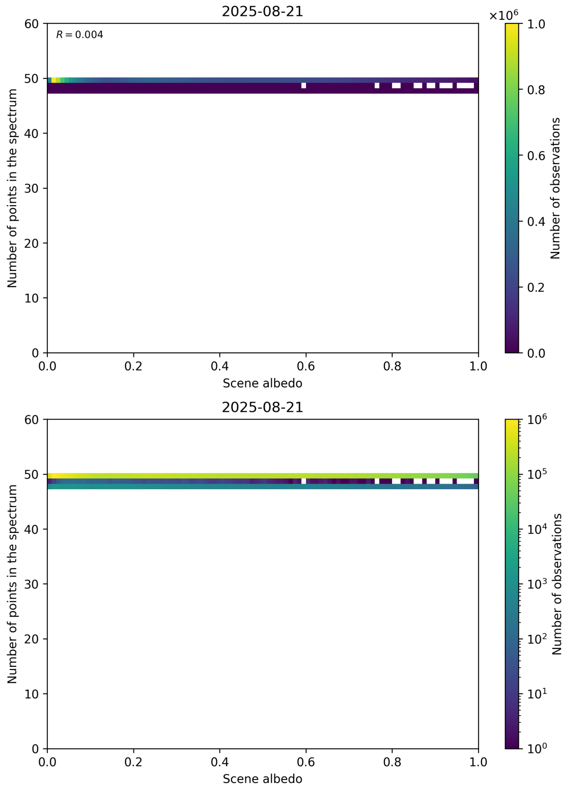
Figure 106: Scatter density plot of “Scene albedo” against “Number of points in the spectrum” for 2025-08-20 to 2025-08-22.
