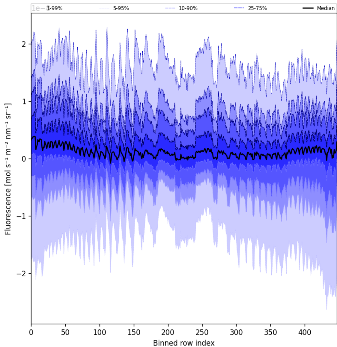
Figure 57: Along track statistics of “Fluorescence” for 2025-08-20 to 2025-08-22
