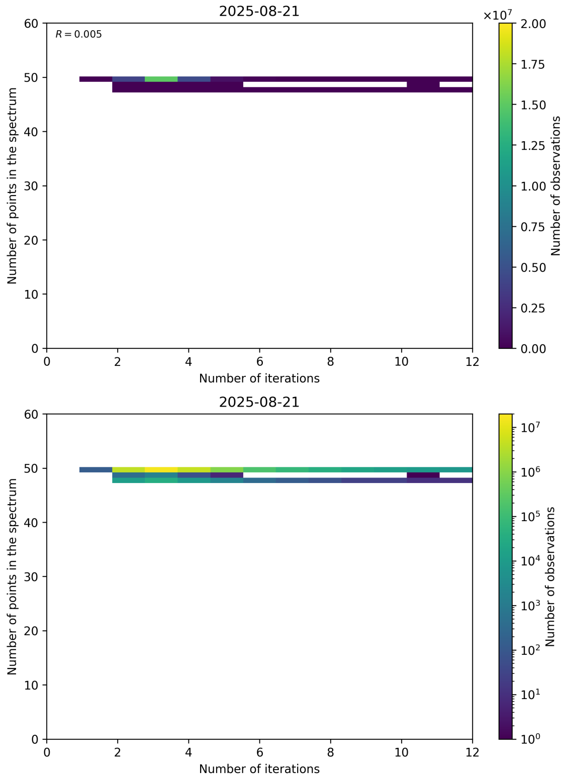
Figure 99: Scatter density plot of “Number of iterations” against “Number of points in the spectrum” for 2025-08-20 to 2025-08-22.
