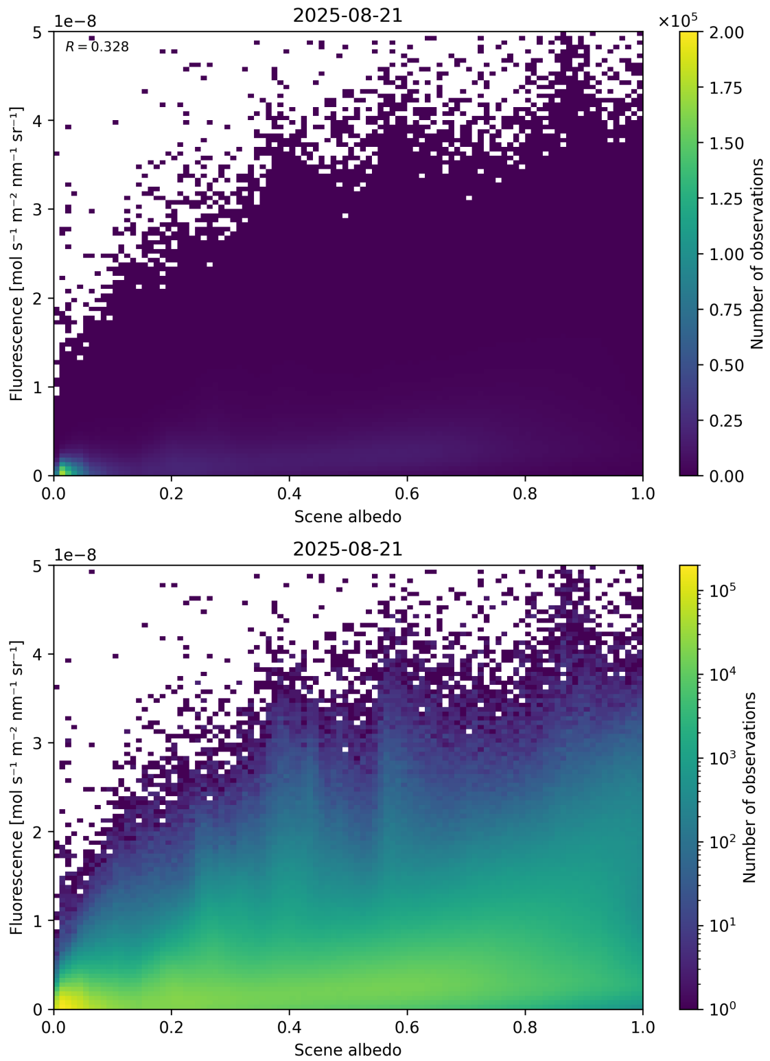
Figure 104: Scatter density plot of “Scene albedo” against “Fluorescence” for 2025-08-20 to 2025-08-22.
