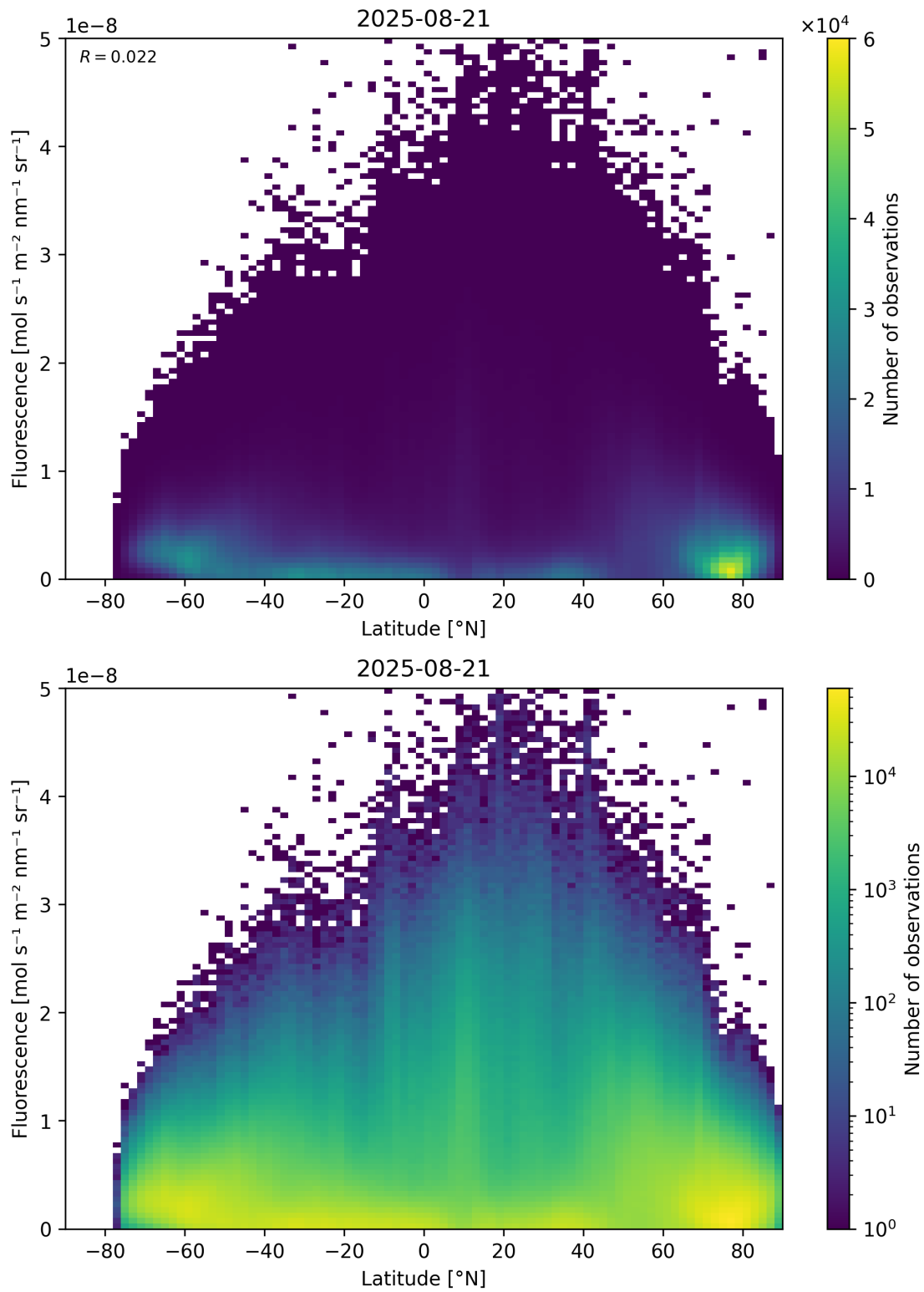
Figure 92: Scatter density plot of “Latitude” against “Fluorescence” for 2025-08-20 to 2025-08-22.
