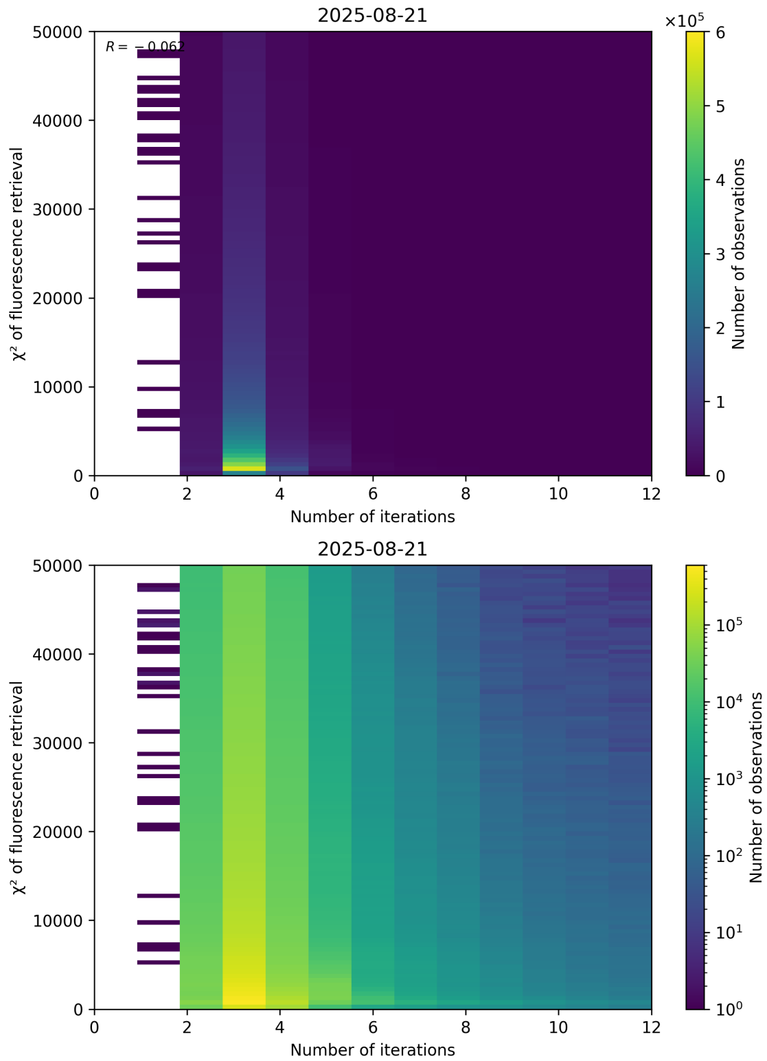
Figure 97: Scatter density plot of “Number of iterations” against “ \chi^2 of fluorescence retrieval” for 2025-08-20 to 2025-08-22.
