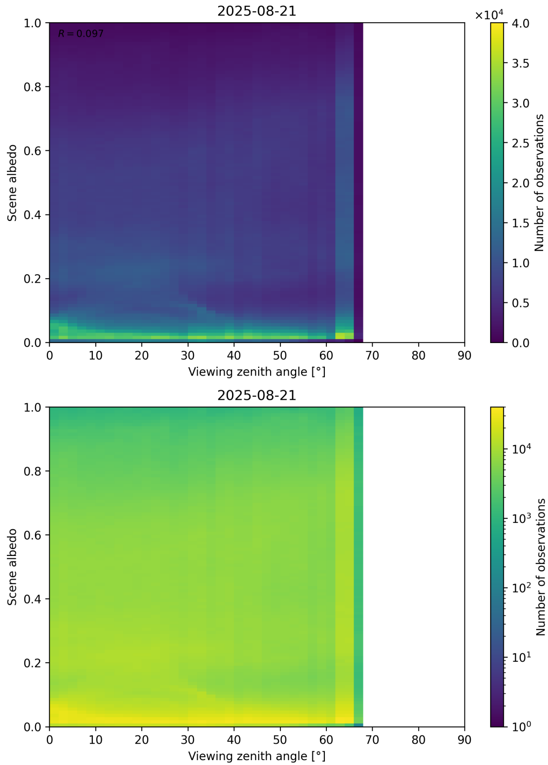
Figure 126: Scatter density plot of “Viewing zenith angle” against “Scene albedo” for 2025-08-20 to 2025-08-22.
