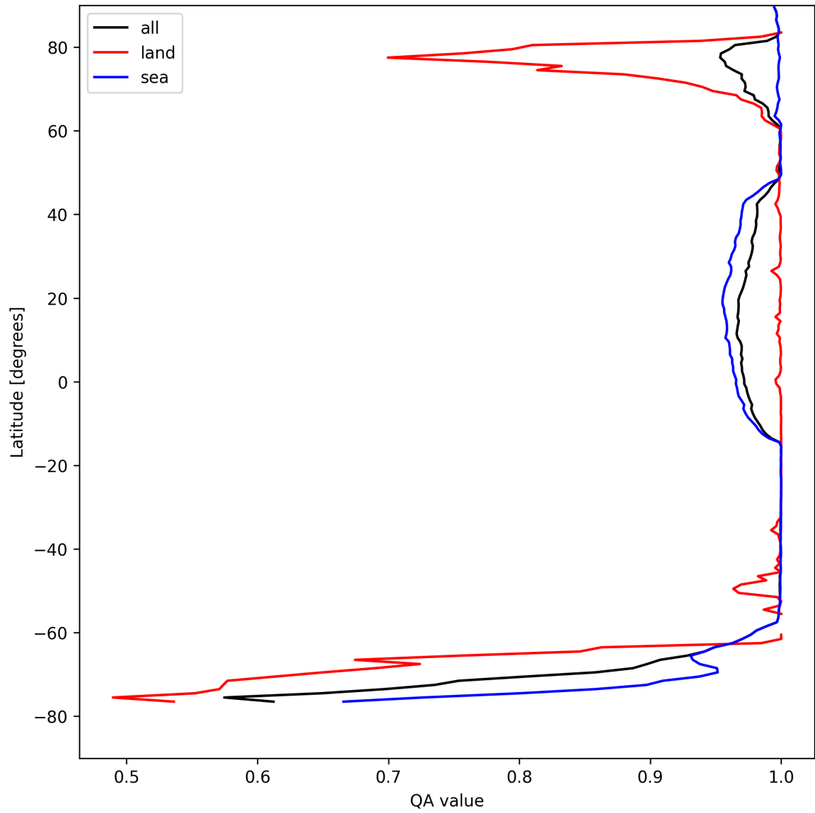
Figure 12: Zonal average of “QA value” for 2025-08-20 to 2025-08-22.
