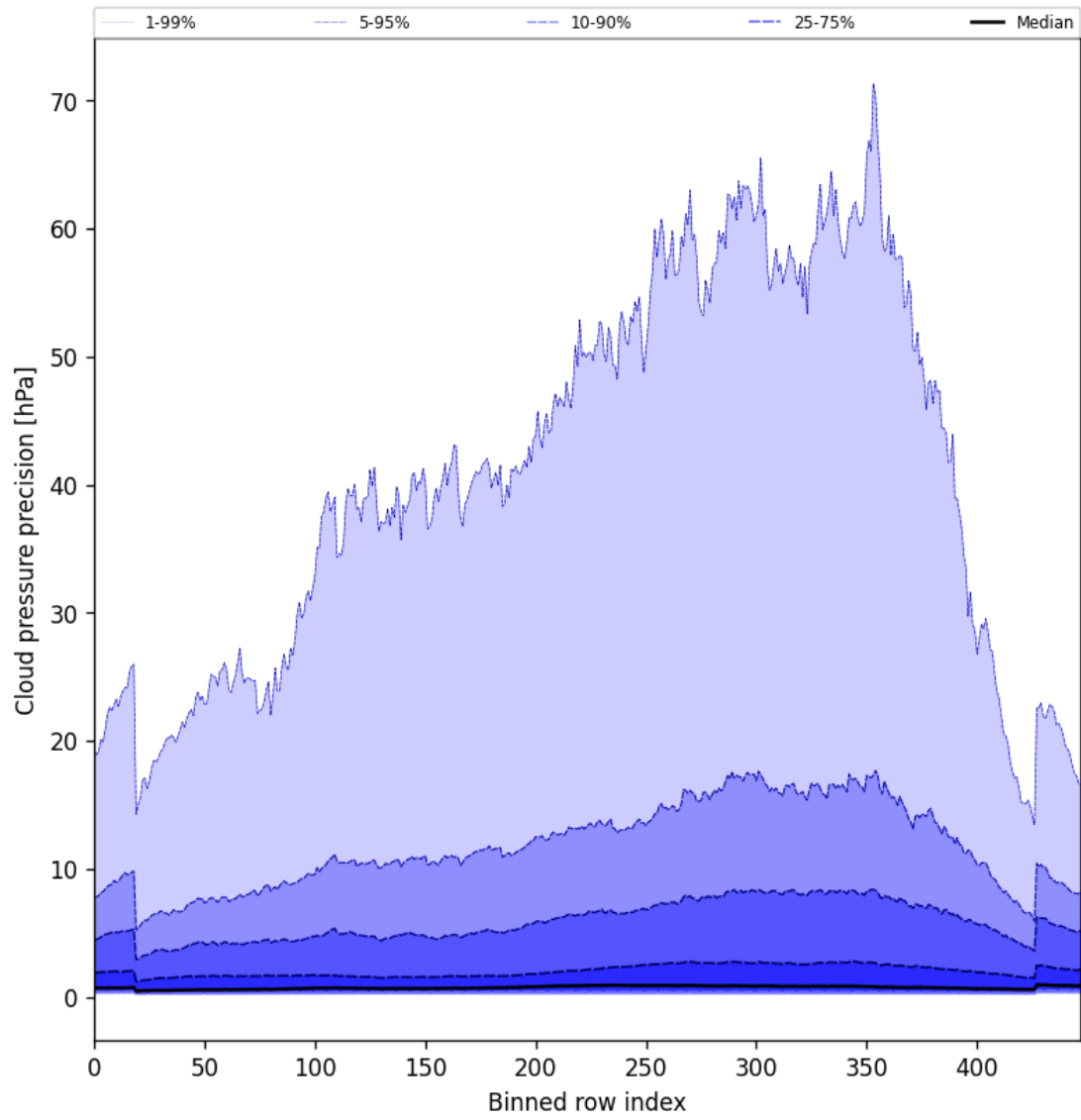
Figure 48: Along track statistics of “Cloud pressure precision” for 2025-08-20 to 2025-08-22
