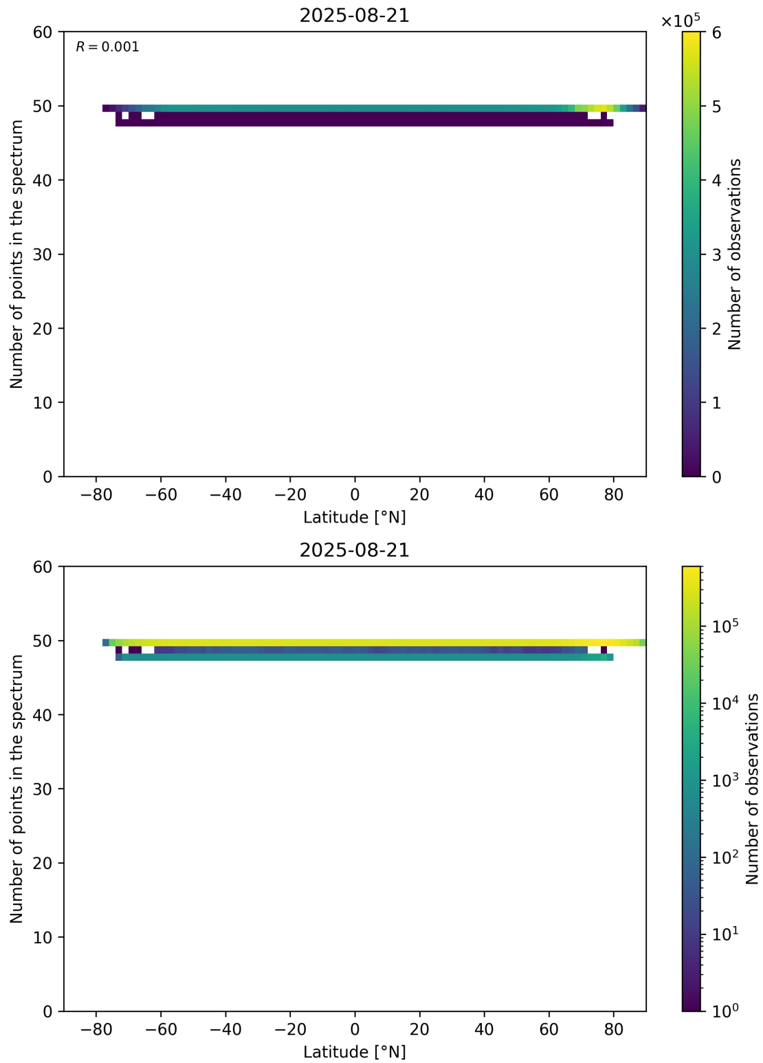
Figure 94: Scatter density plot of “Latitude” against “Number of points in the spectrum” for 2025-08-20 to 2025-08-22.
