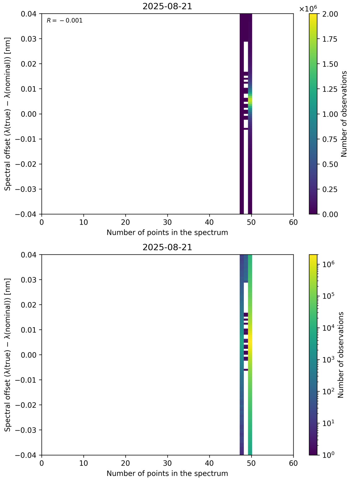
Figure 101: Scatter density plot of “Number of points in the spectrum” against “Spectral offset ( \lambda_{\text{true}} - \lambda_{\text{nominal}} )” for 2025-08-20 to 2025-08-22.
