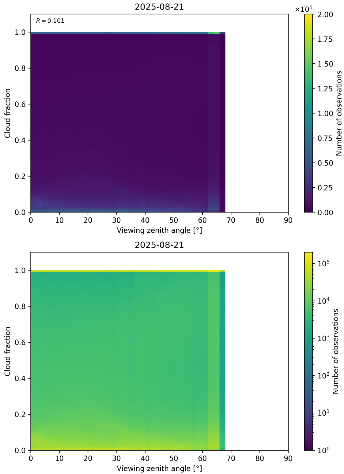
Figure 120: Scatter density plot of “Viewing zenith angle” against “Cloud fraction” for 2025-08-20 to 2025-08-22.
