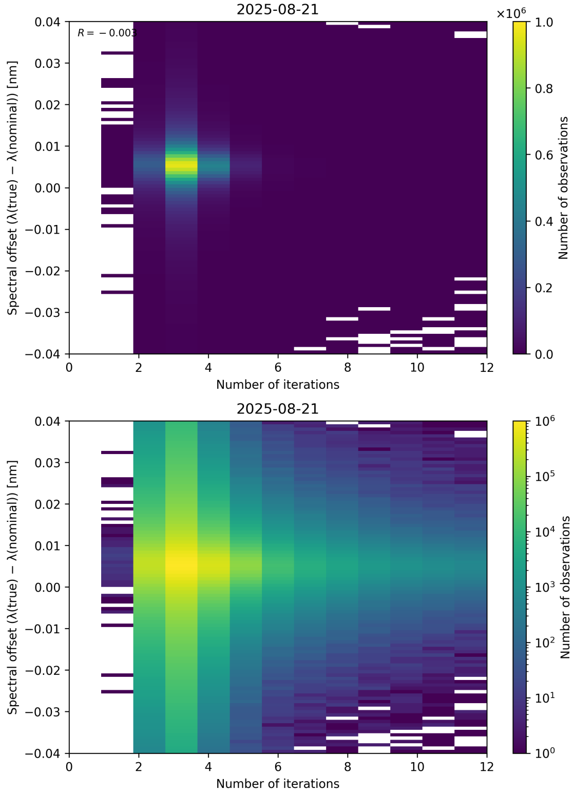
Figure 100: Scatter density plot of “Number of iterations” against “Spectral offset ( \lambda_{\text{true}} - \lambda_{\text{nominal}} )” for 2025-08-20 to 2025-08-22.
