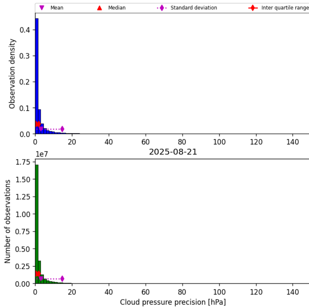
Figure 31: Histogram of “Cloud pressure precision” for 2025-08-20 to 2025-08-22
