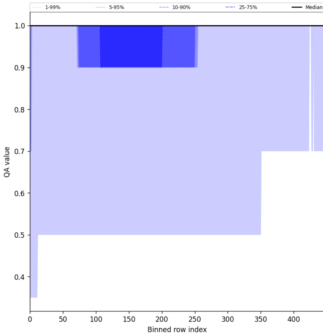
Figure 46: Along track statistics of “QA value” for 2025-08-20 to 2025-08-22
