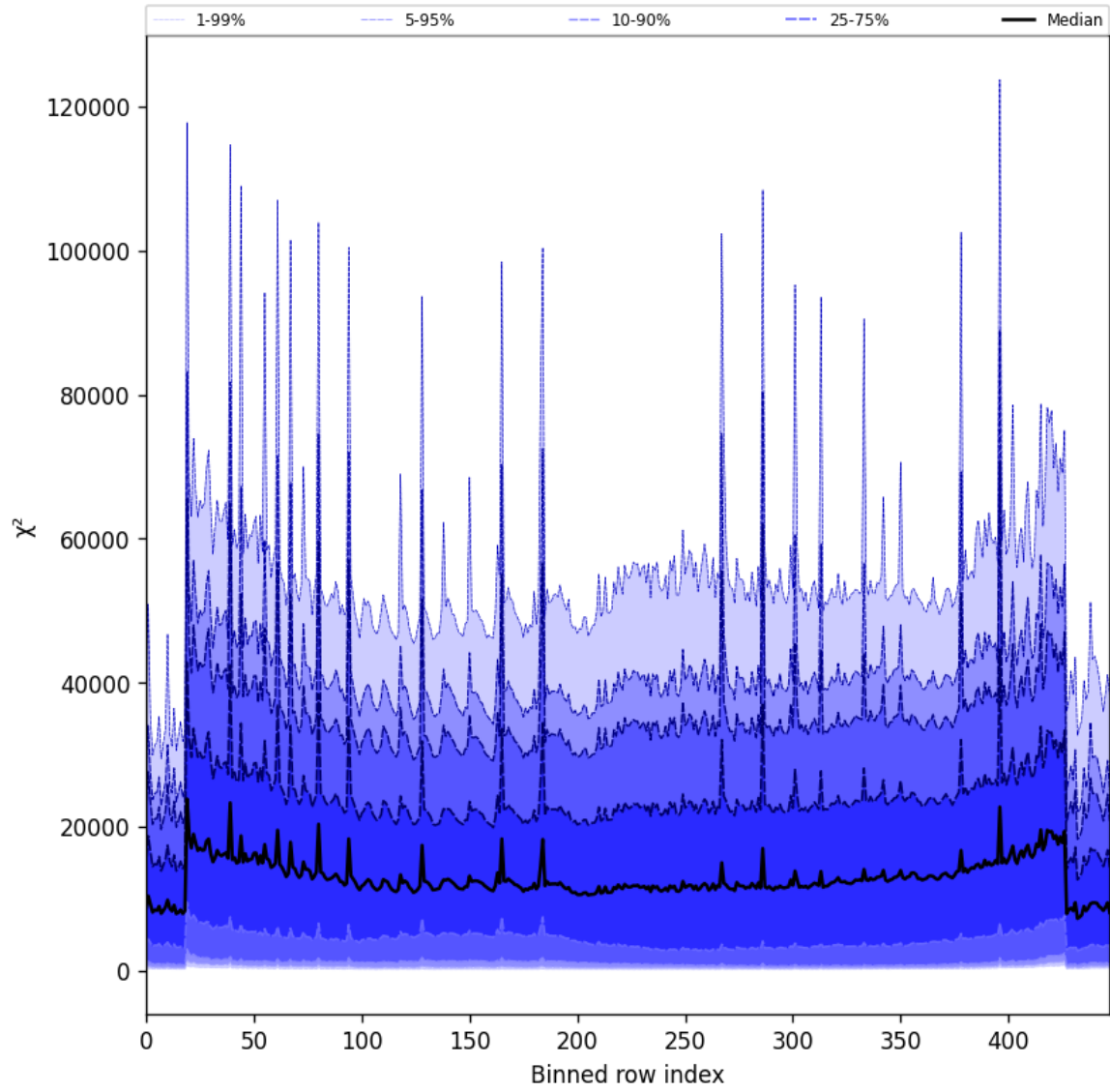
Figure 55: Along track statistics of “ \chi^2 ” for 2025-08-20 to 2025-08-22
