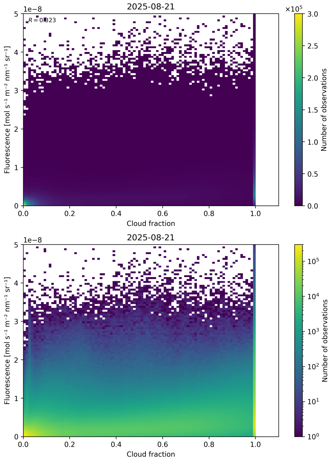
Figure 72: Scatter density plot of “Cloud fraction” against “Fluorescence” for 2025-08-20 to 2025-08-22.
