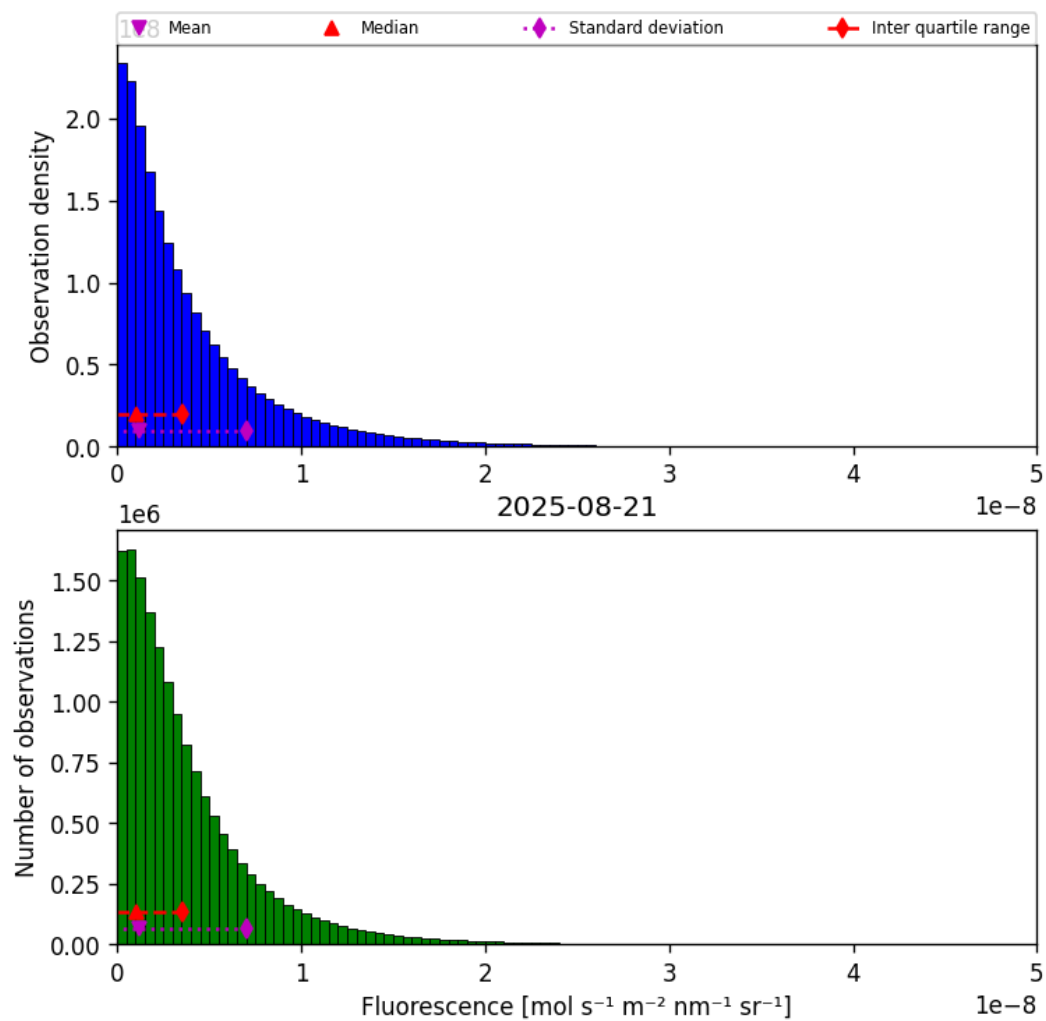
Figure 40: Histogram of “Fluorescence” for 2025-08-20 to 2025-08-22
