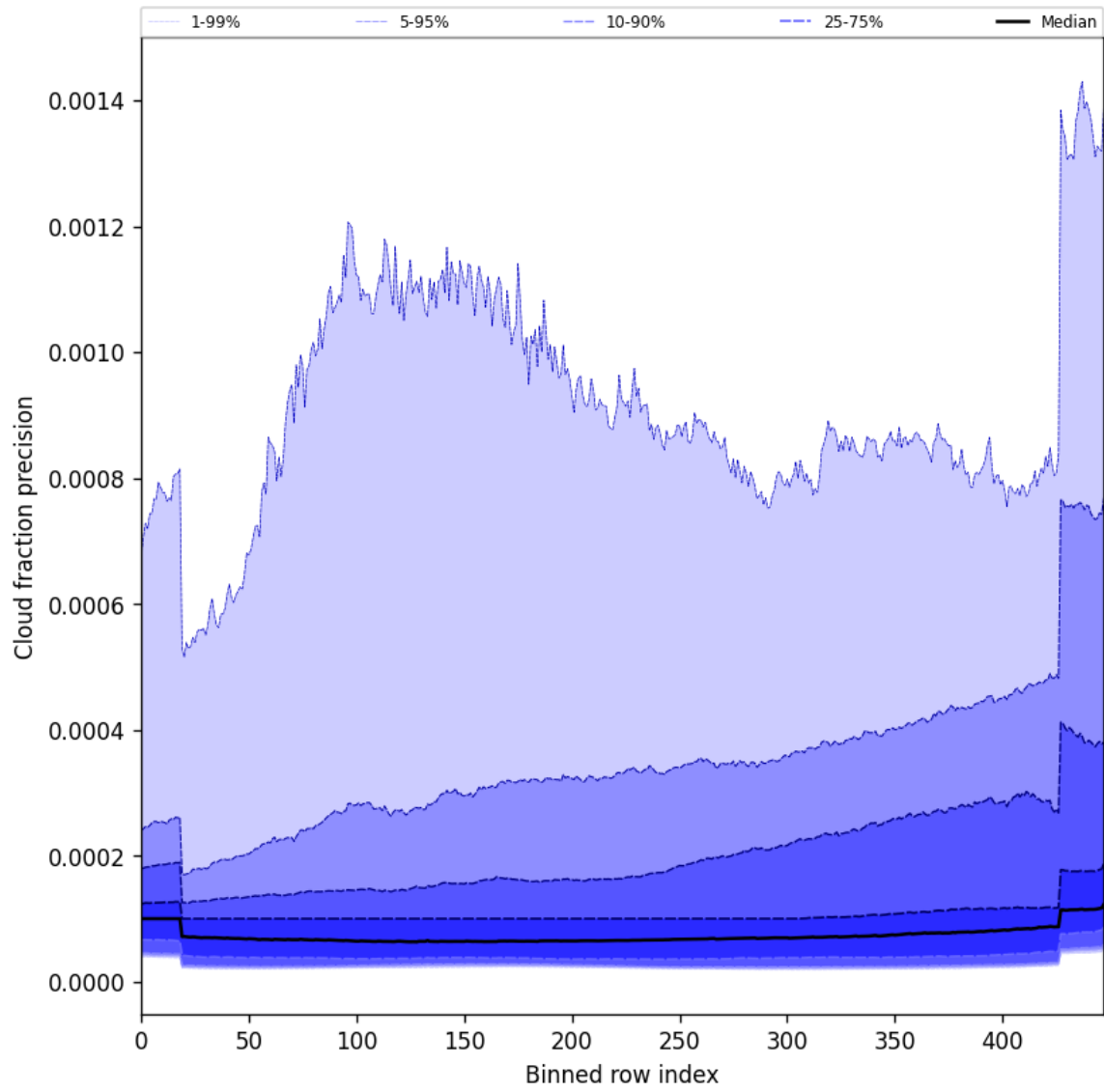
Figure 50: Along track statistics of “Cloud fraction precision” for 2025-08-20 to 2025-08-22
