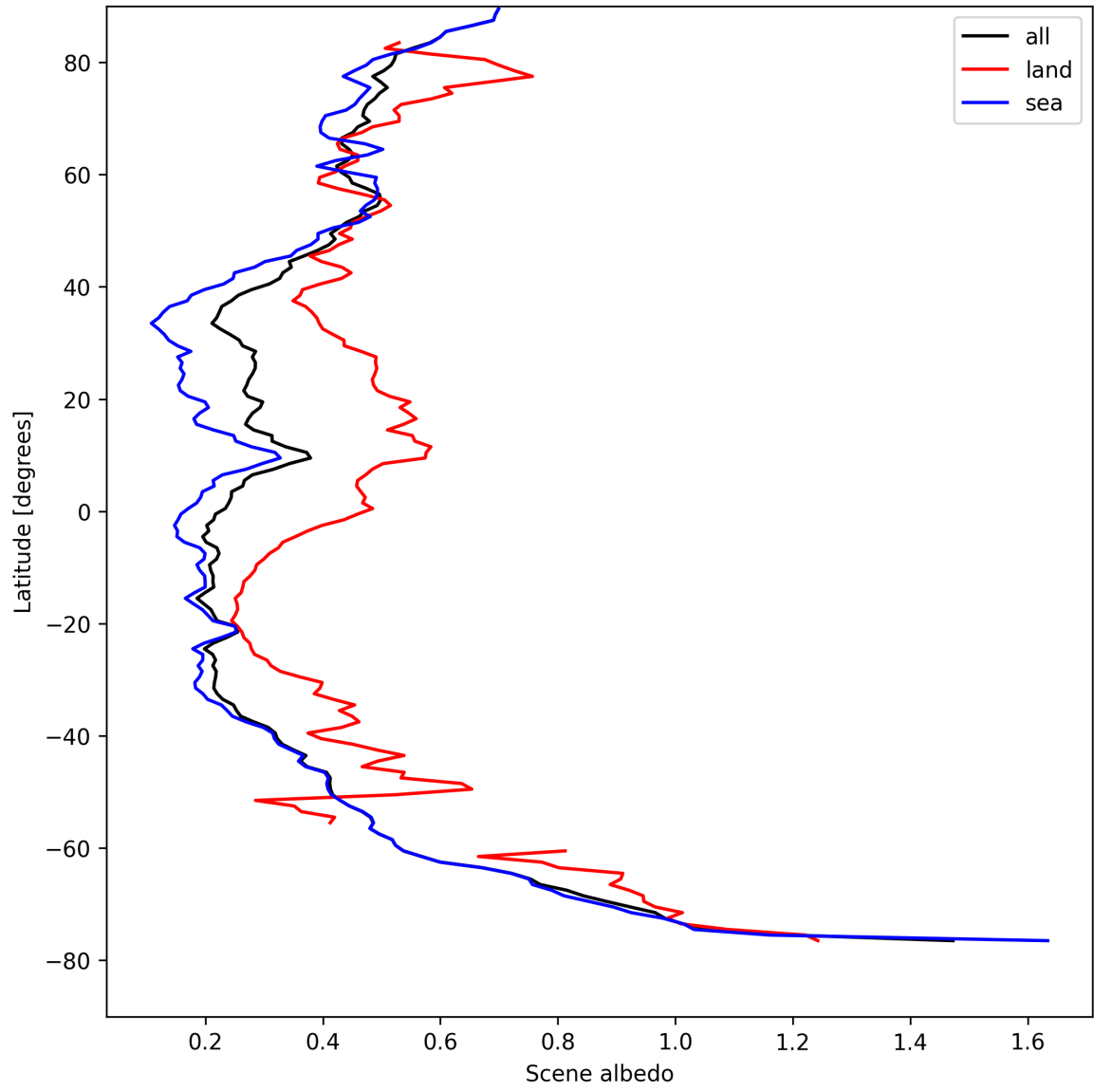
Figure 17: Zonal average of “Scene albedo” for 2025-08-20 to 2025-08-22.
