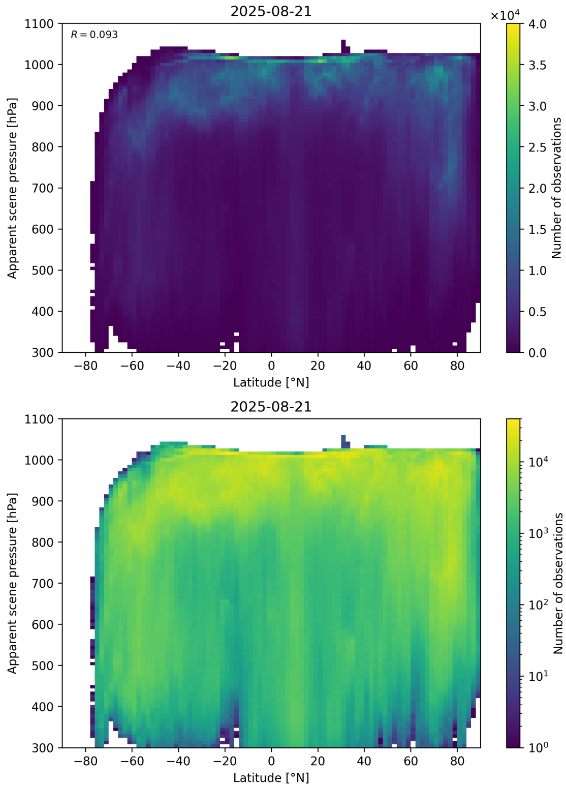
Figure 88: Scatter density plot of “Latitude” against “Apparent scene pressure” for 2025-08-20 to 2025-08-22.
