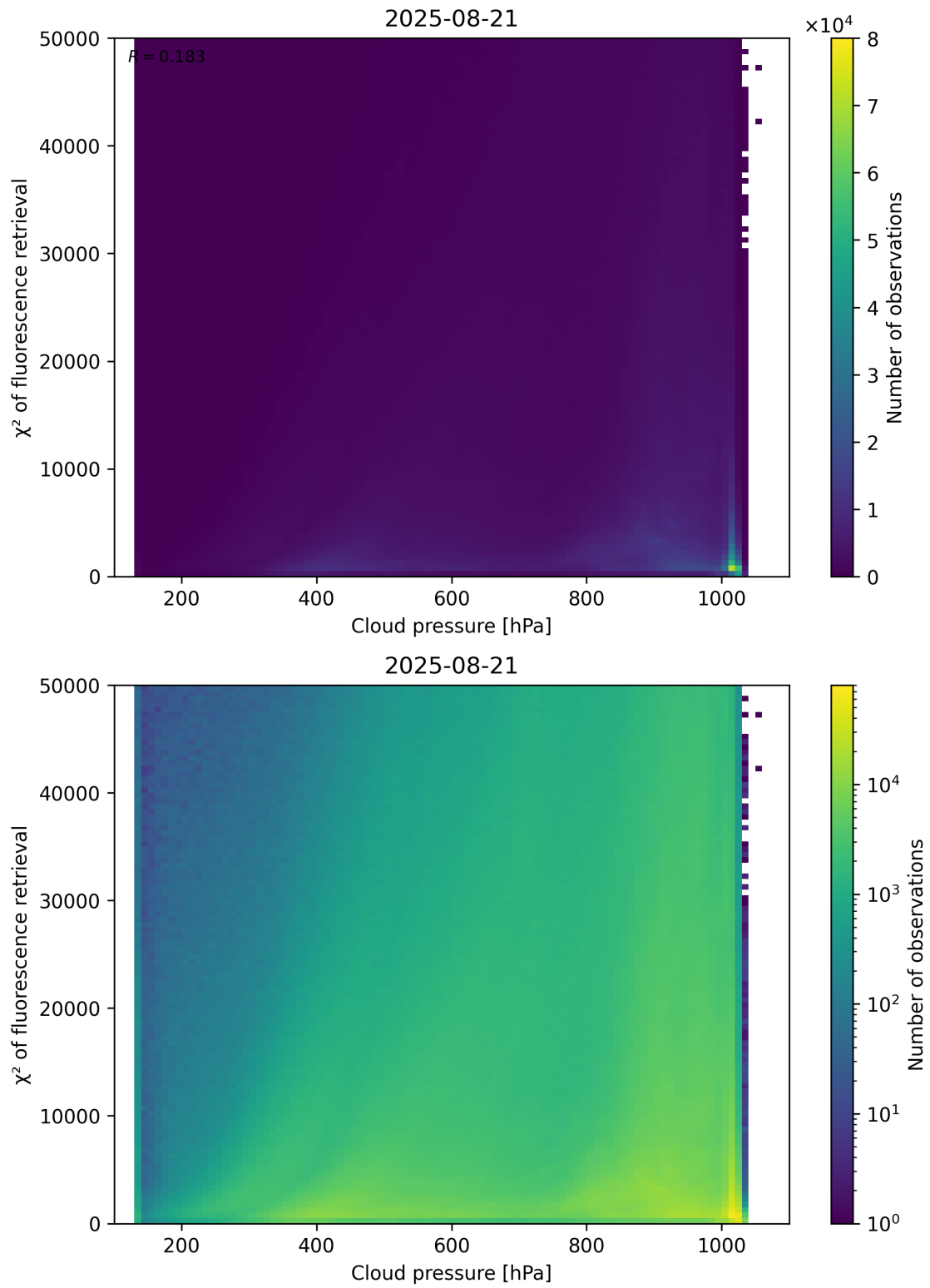
Figure 78: Scatter density plot of “Cloud pressure” against “ \chi^2 of fluorescence retrieval” for 2025-08-20 to 2025-08-22.
