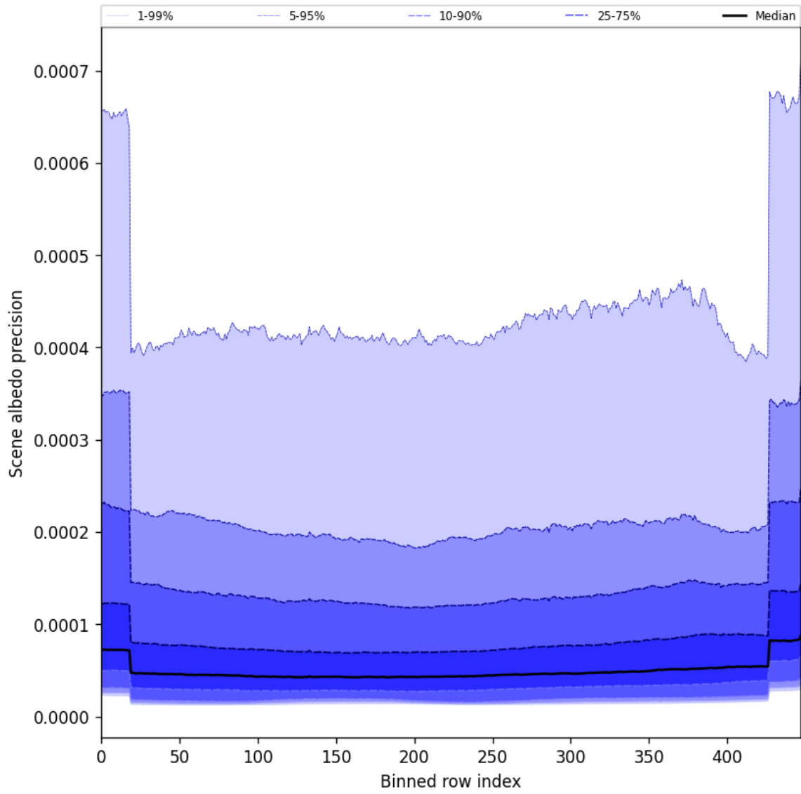
Figure 52: Along track statistics of “Scene albedo precision” for 2025-08-20 to 2025-08-22
