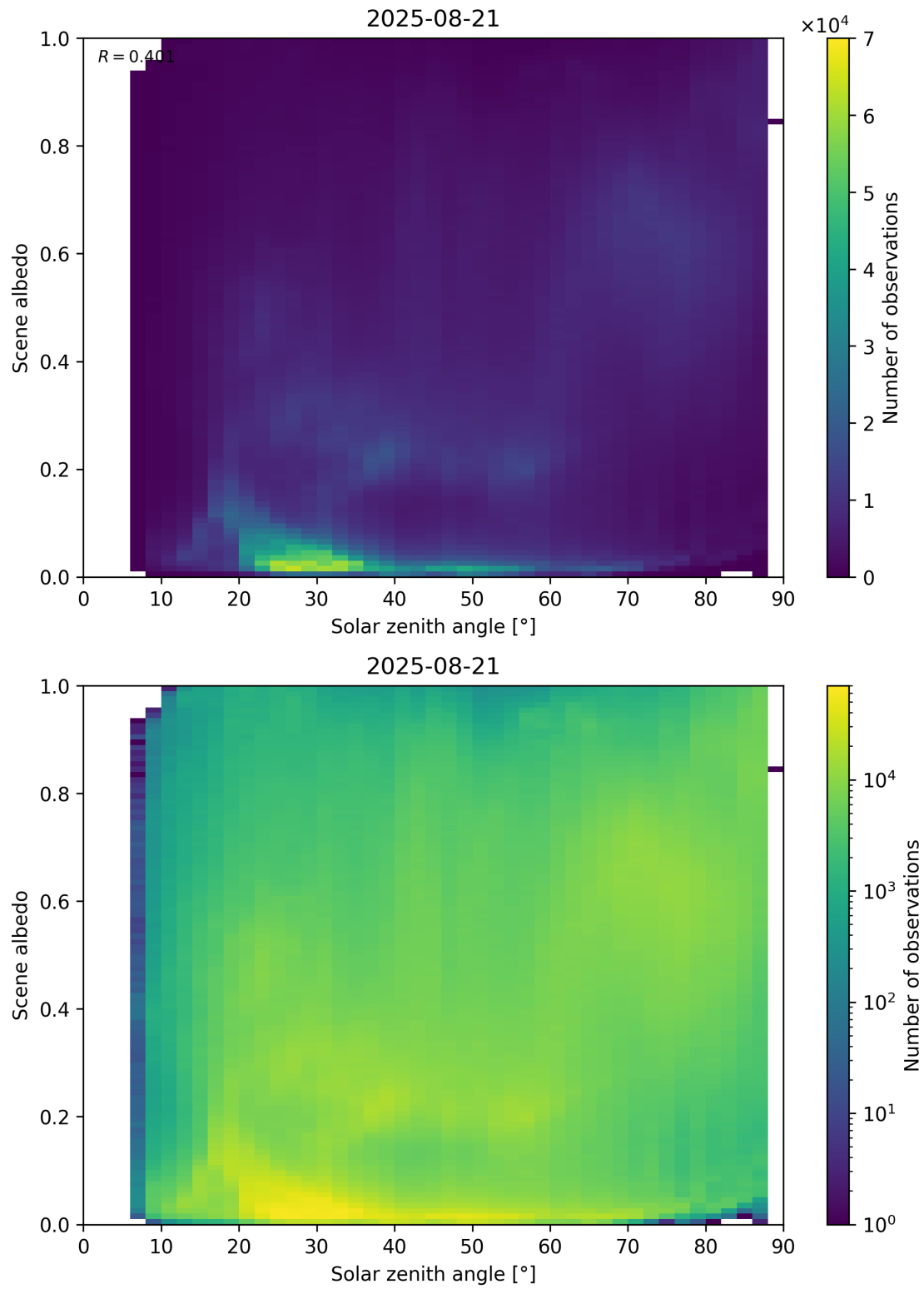
Figure 116: Scatter density plot of “Solar zenith angle” against “Scene albedo” for 2025-08-20 to 2025-08-22.
