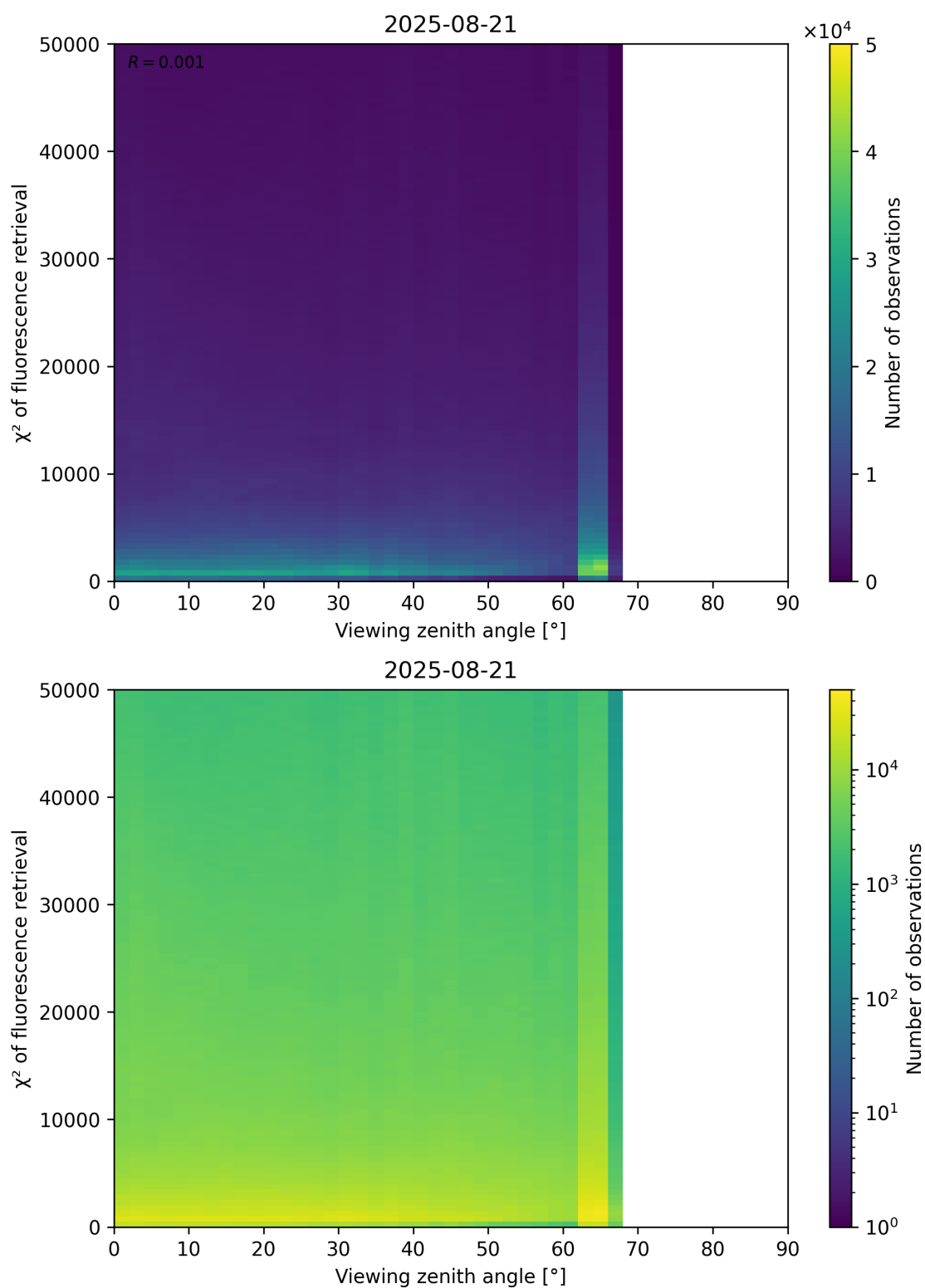
Figure 119: Scatter density plot of “Viewing zenith angle” against “ \chi^2 of fluorescence retrieval” for 2025-08-20 to 2025-08-22.
