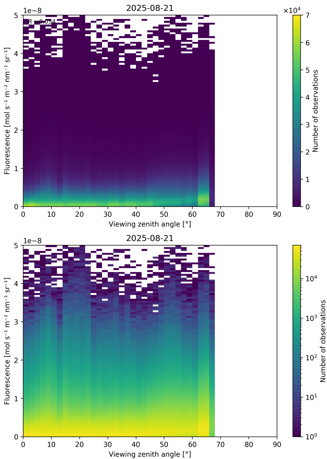
Figure 122: Scatter density plot of “Viewing zenith angle” against “Fluorescence” for 2025-08-20 to 2025-08-22.
