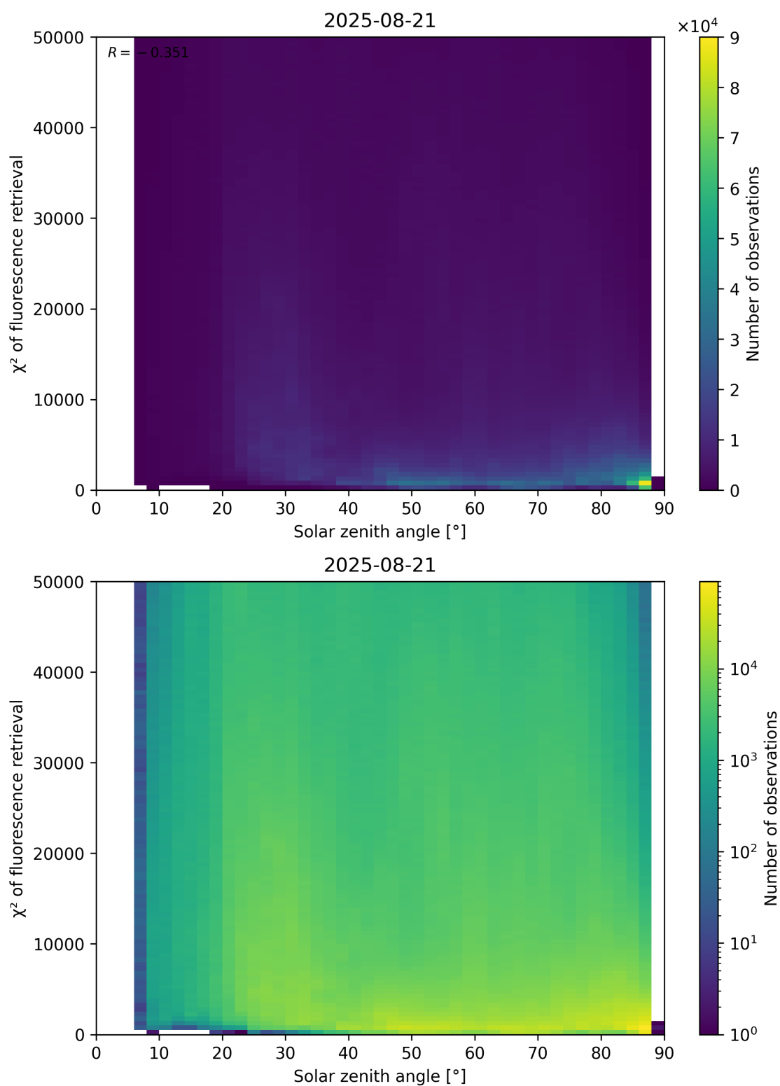
Figure 109: Scatter density plot of “Solar zenith angle” against “ \chi^2 of fluorescence retrieval” for 2025-08-20 to 2025-08-22.
