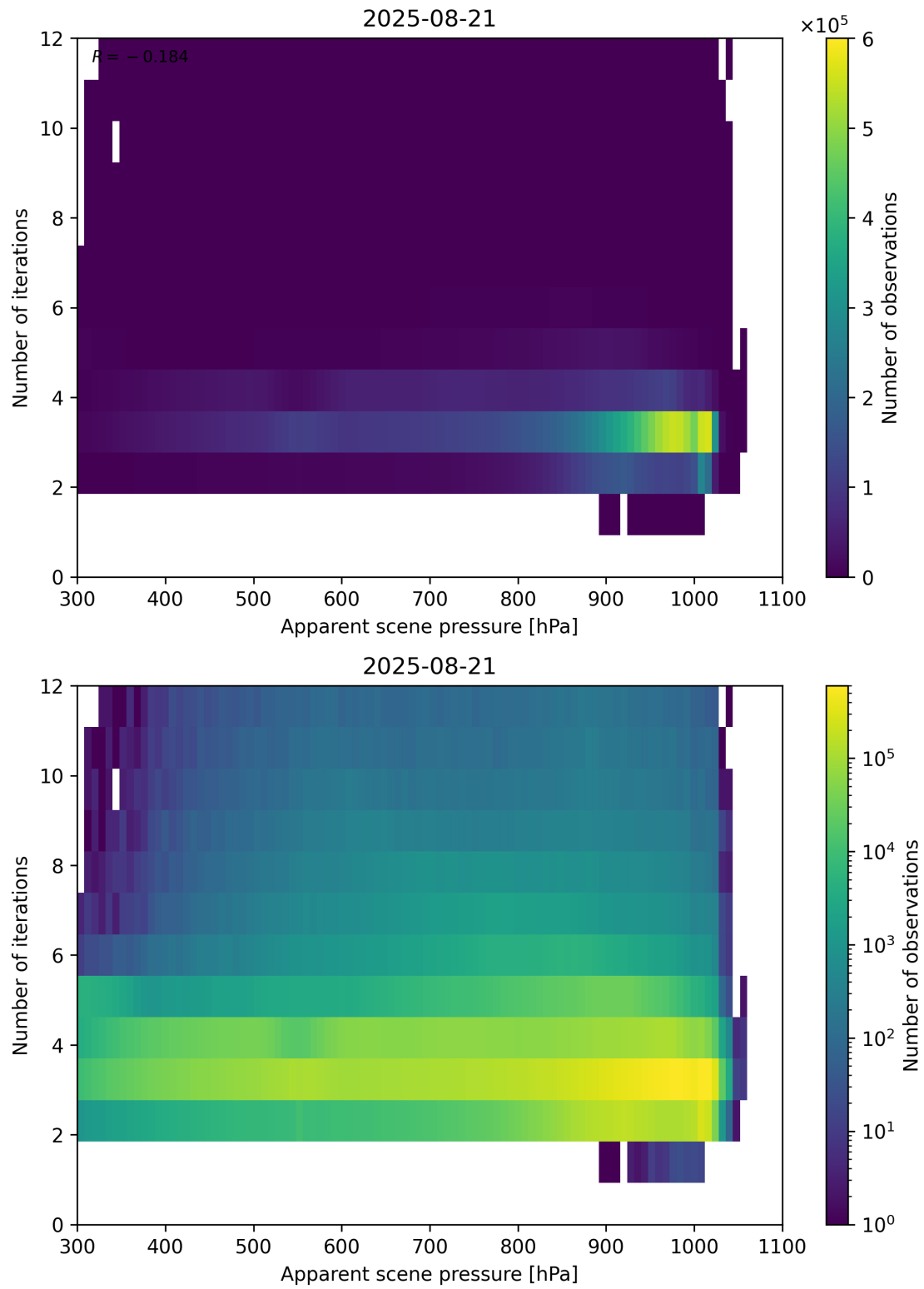
Figure 65: Scatter density plot of “Apparent scene pressure” against “Number of iterations” for 2025-08-20 to 2025-08-22.
