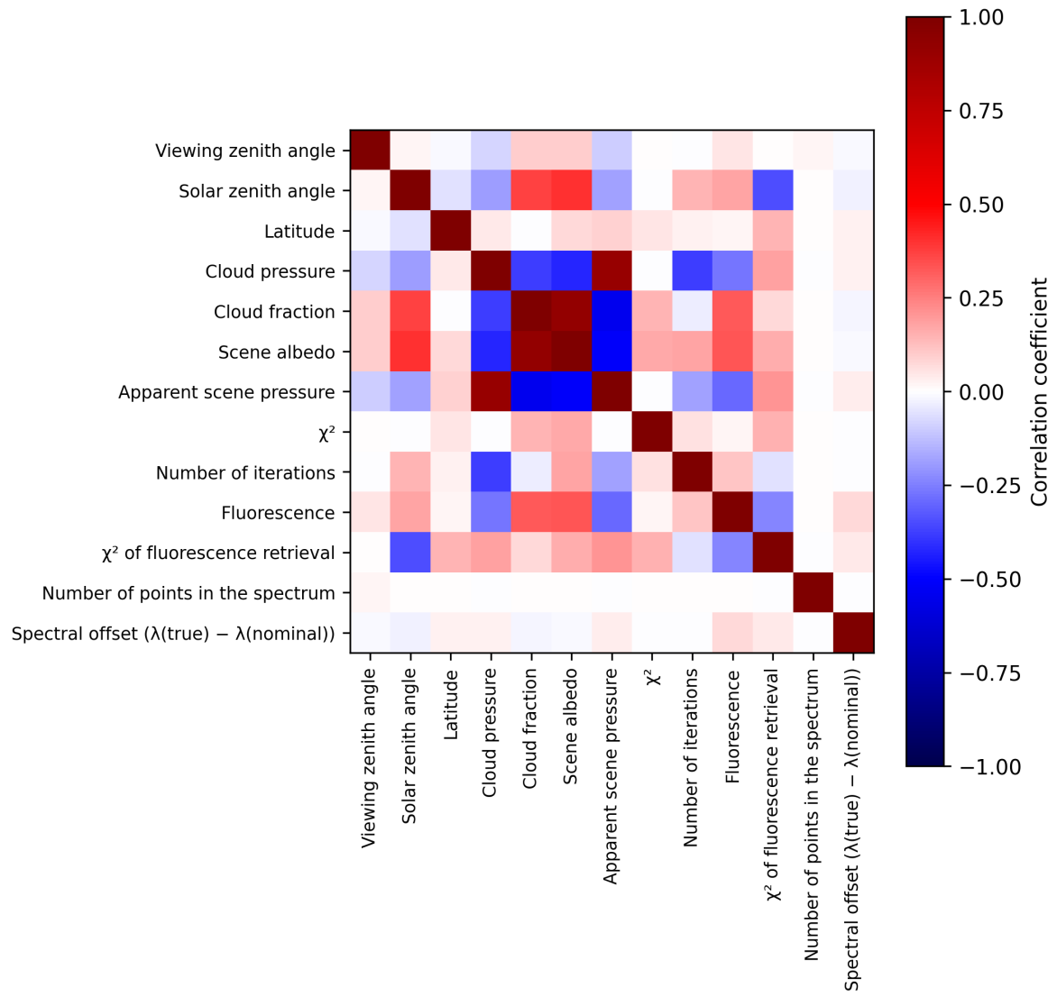
Figure 2: Map of correlation matrix for 2025-08-20 to 2025-08-22.
