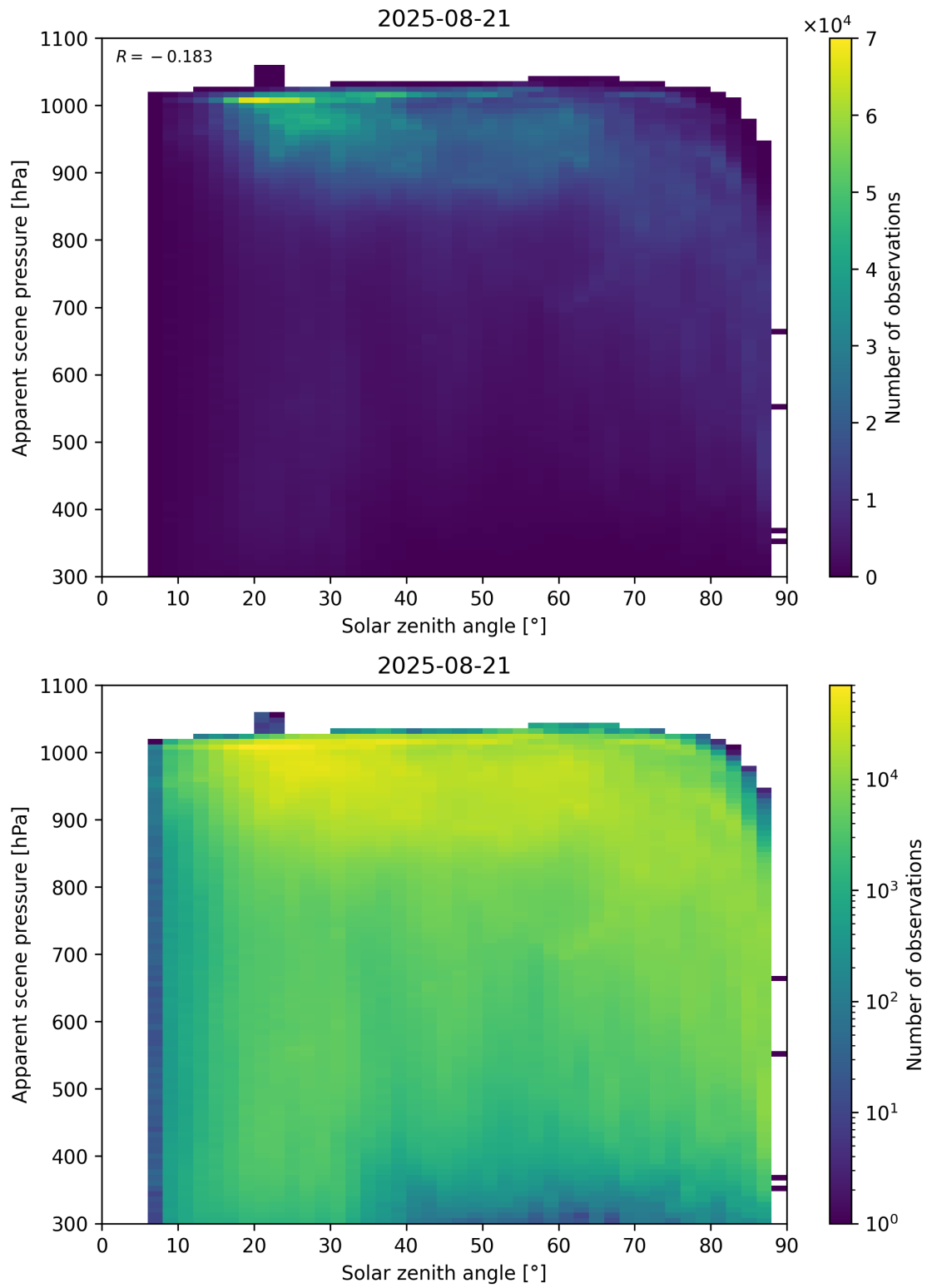
Figure 108: Scatter density plot of “Solar zenith angle” against “Apparent scene pressure” for 2025-08-20 to 2025-08-22.
