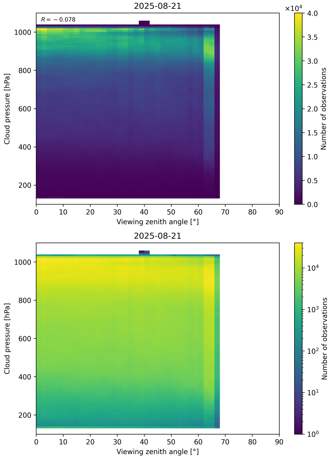
Figure 121: Scatter density plot of “Viewing zenith angle” against “Cloud pressure” for 2025-08-20 to 2025-08-22.
