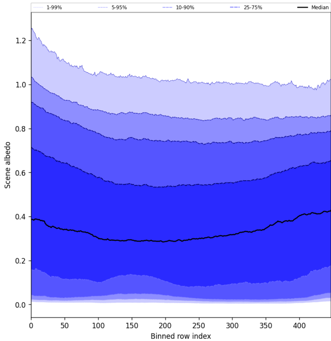
Figure 51: Along track statistics of “Scene albedo” for 2025-08-20 to 2025-08-22
