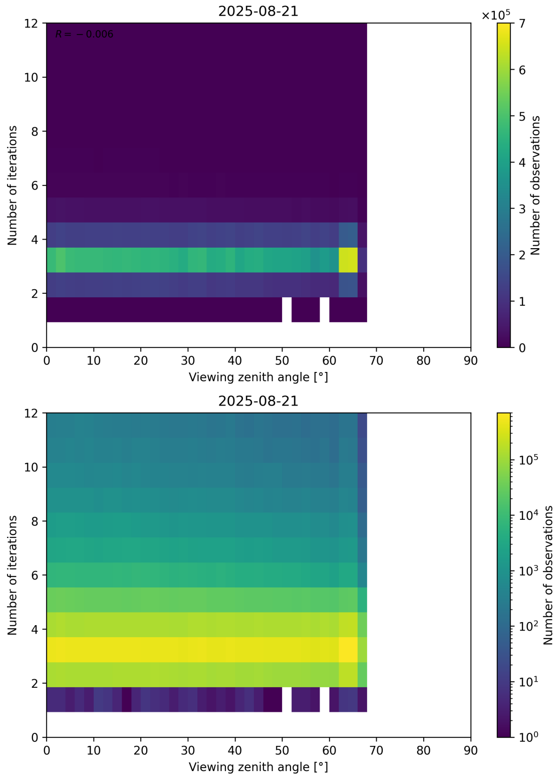
Figure 124: Scatter density plot of “Viewing zenith angle” against “Number of iterations” for 2025-08-20 to 2025-08-22.
