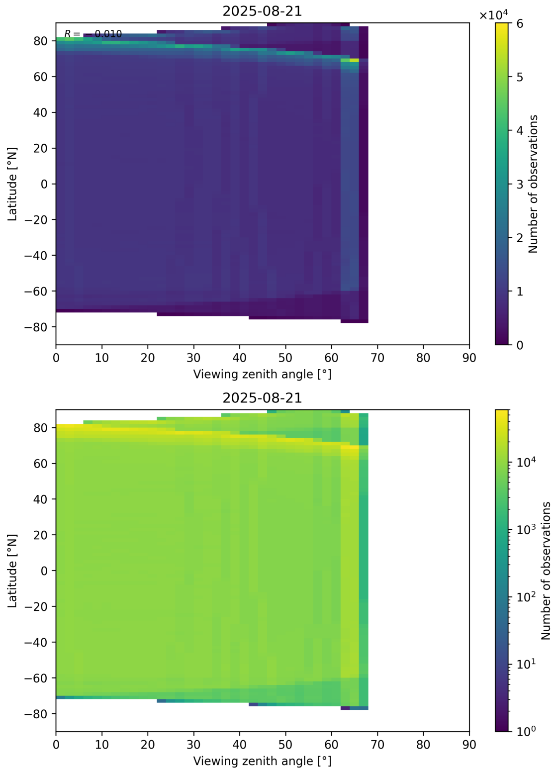
Figure 123: Scatter density plot of “Viewing zenith angle” against “Latitude” for 2025-08-20 to 2025-08-22.
