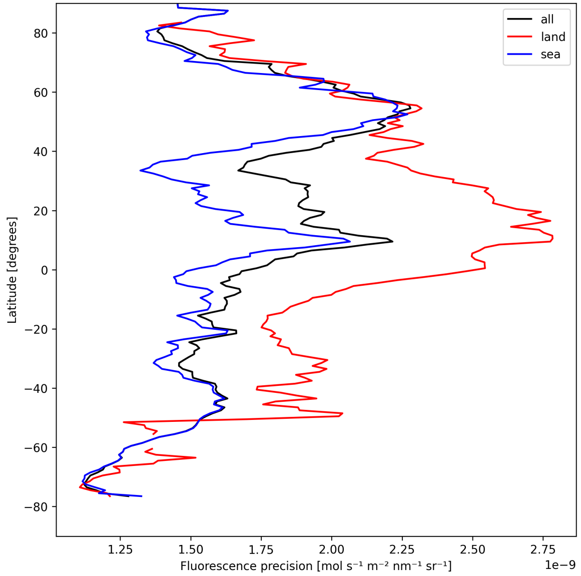
Figure 24: Zonal average of “Fluorescence precision” for 2025-08-20 to 2025-08-22.
