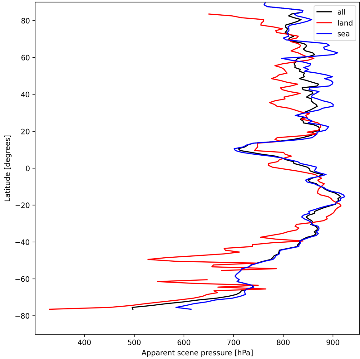
Figure 19: Zonal average of “Apparent scene pressure” for 2025-08-20 to 2025-08-22.
