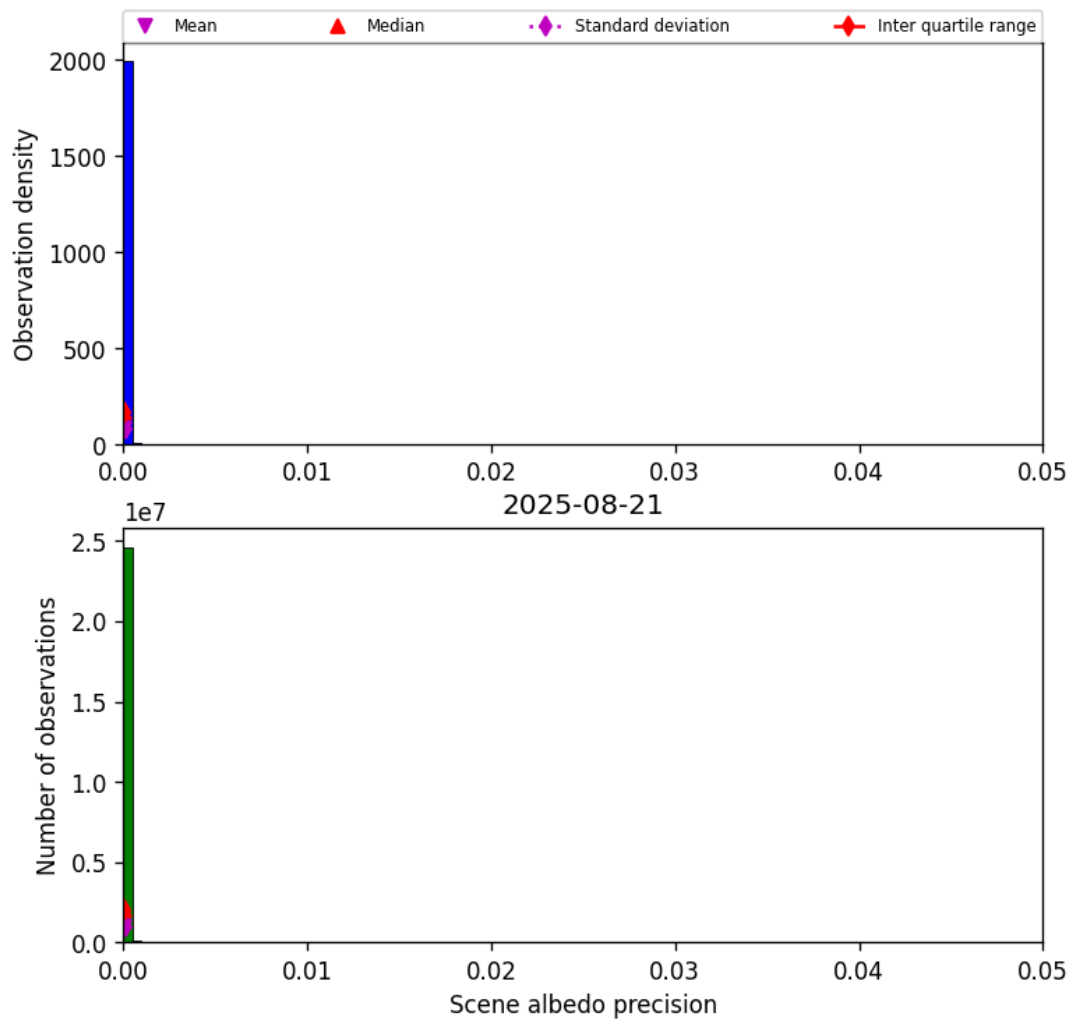
Figure 35: Histogram of “Scene albedo precision” for 2025-08-20 to 2025-08-22
