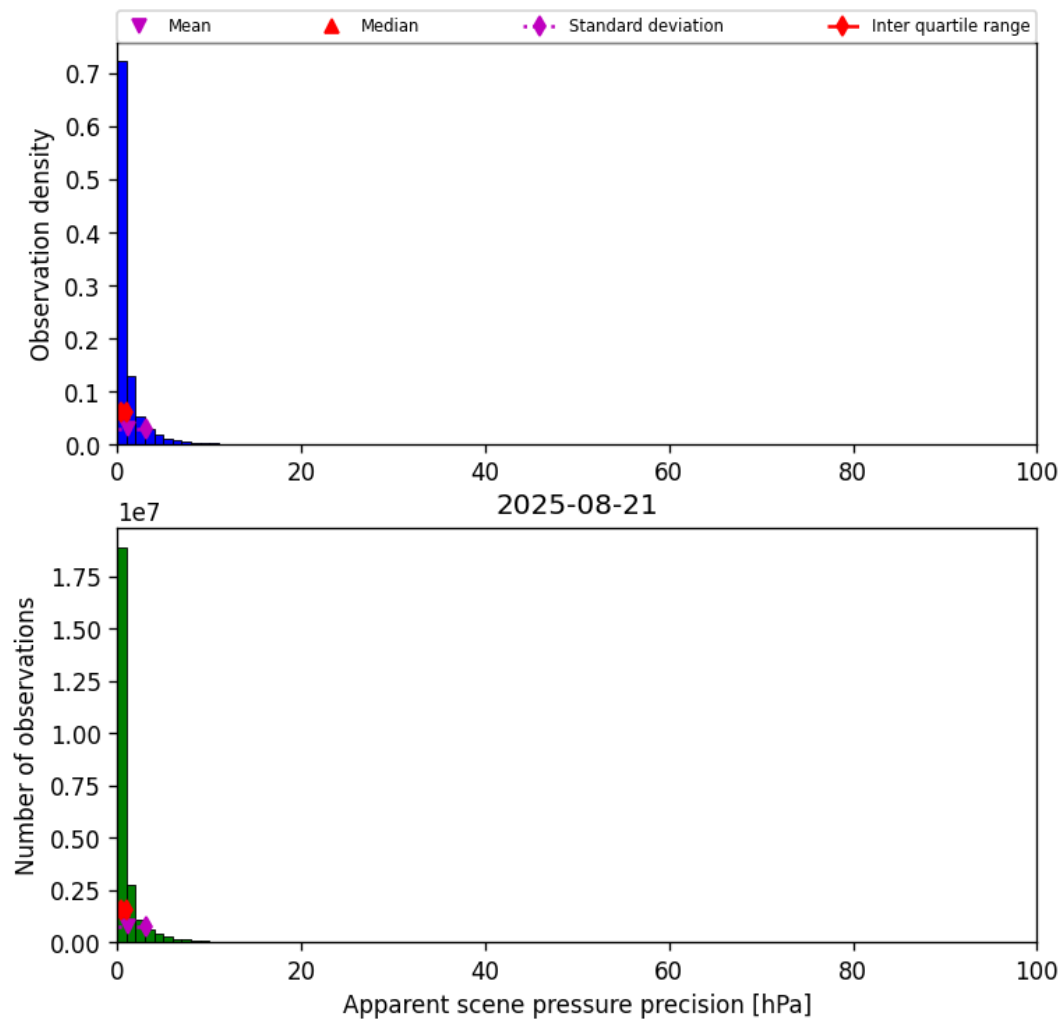
Figure 37: Histogram of “Apparent scene pressure precision” for 2025-08-20 to 2025-08-22
