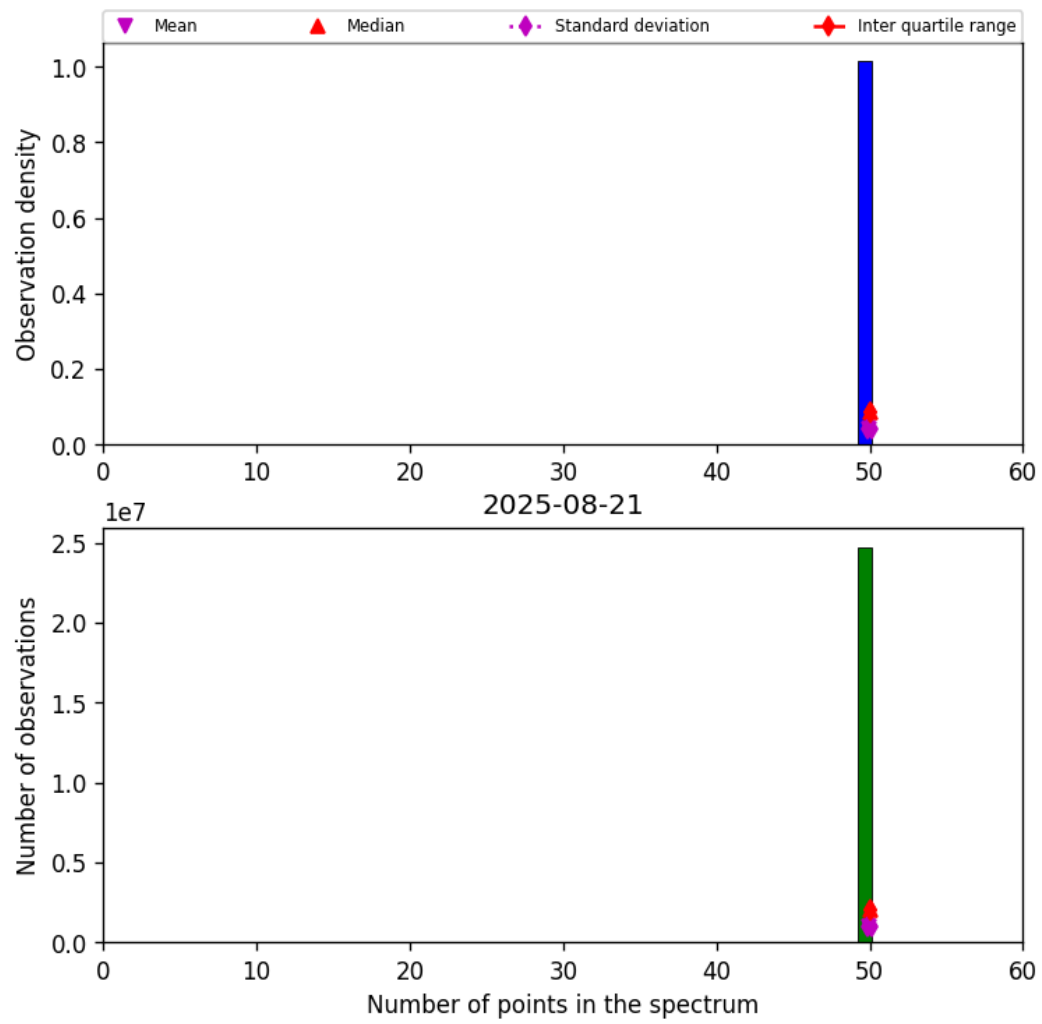
Figure 44: Histogram of “Number of points in the spectrum” for 2025-08-20 to 2025-08-22
