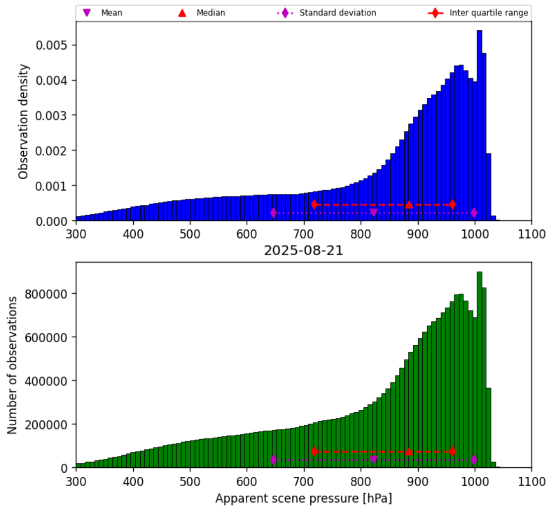
Figure 36: Histogram of “Apparent scene pressure” for 2025-08-20 to 2025-08-22
