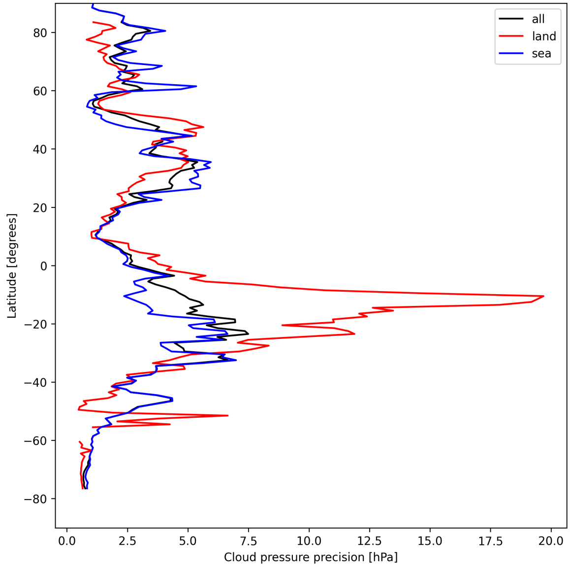
Figure 14: Zonal average of “Cloud pressure precision” for 2025-08-20 to 2025-08-22.
