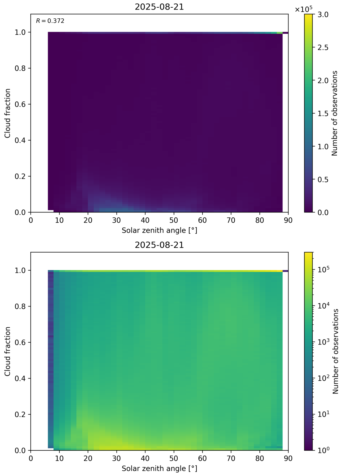
Figure 110: Scatter density plot of “Solar zenith angle” against “Cloud fraction” for 2025-08-20 to 2025-08-22.
