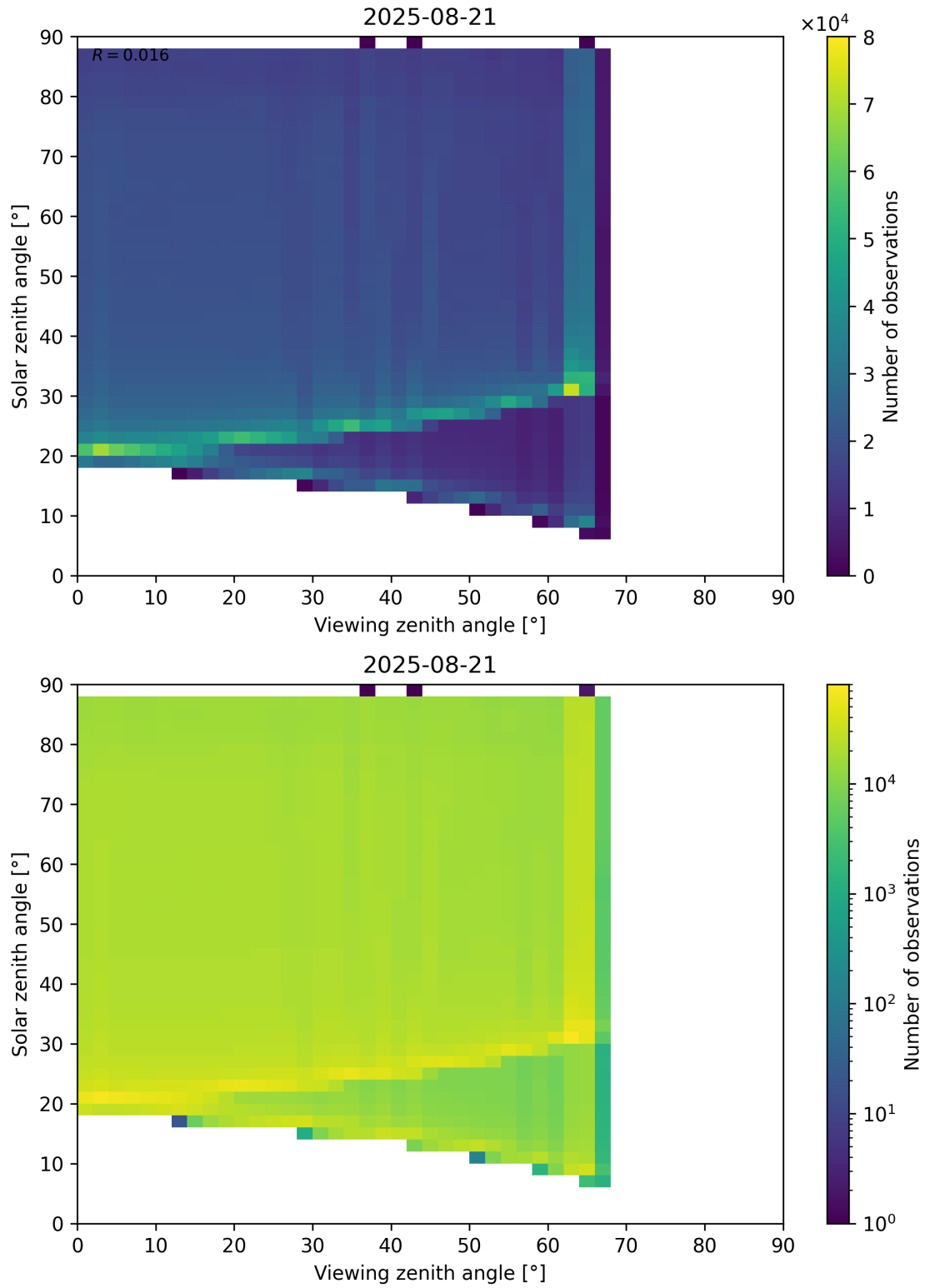
Figure 127: Scatter density plot of “Viewing zenith angle” against “Solar zenith angle” for 2025-08-20 to 2025-08-22.
