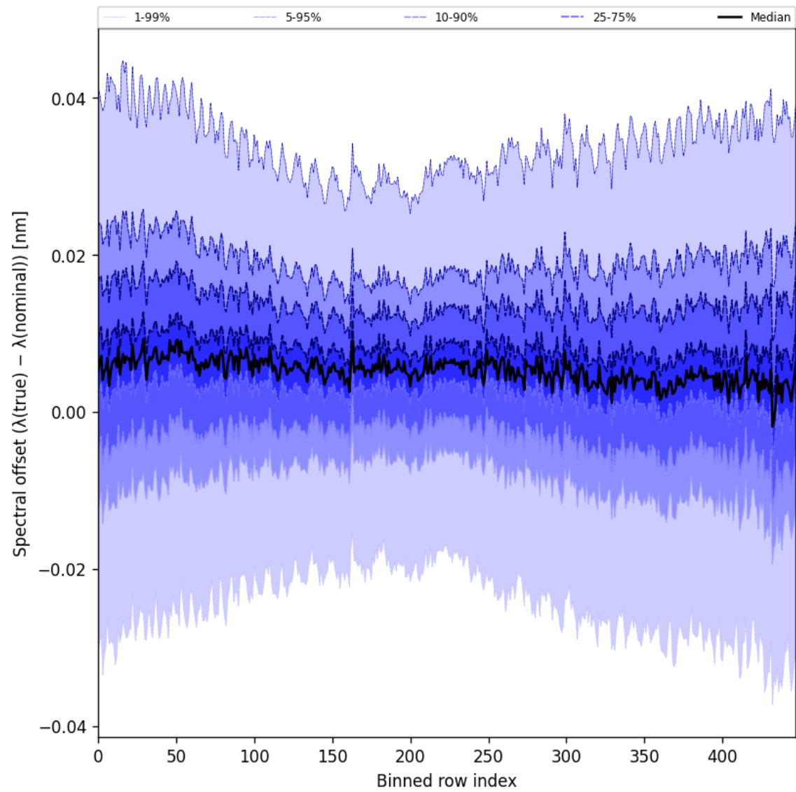
Figure 62: Along track statistics of “Spectral offset ( \lambda_{\text{true}} - \lambda_{\text{nominal}} )” for 2025-08-20 to 2025-08-22
