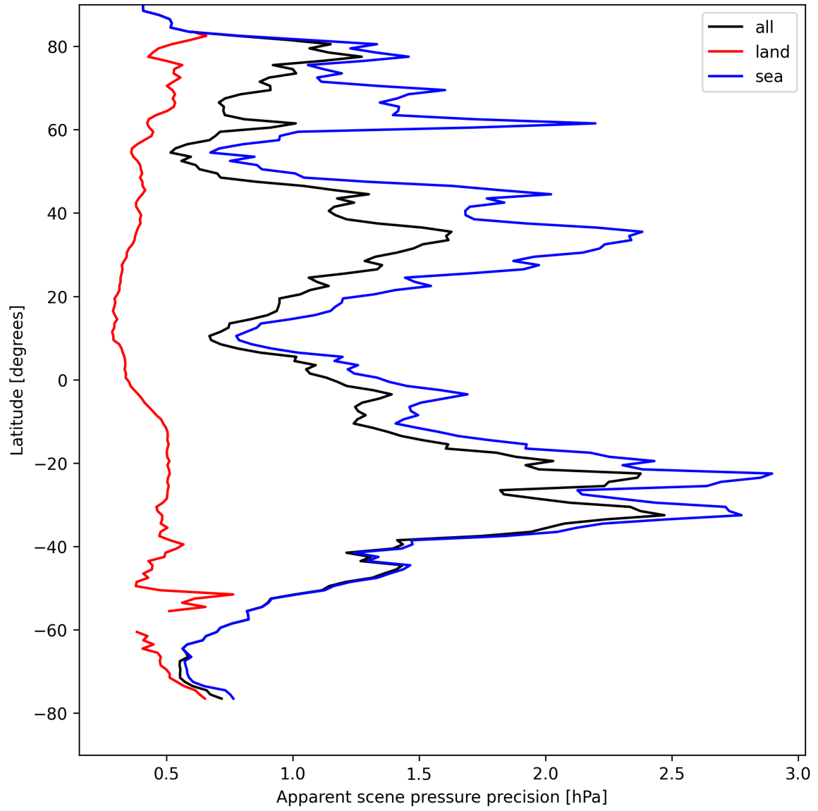
Figure 20: Zonal average of “Apparent scene pressure precision” for 2025-08-20 to 2025-08-22.
