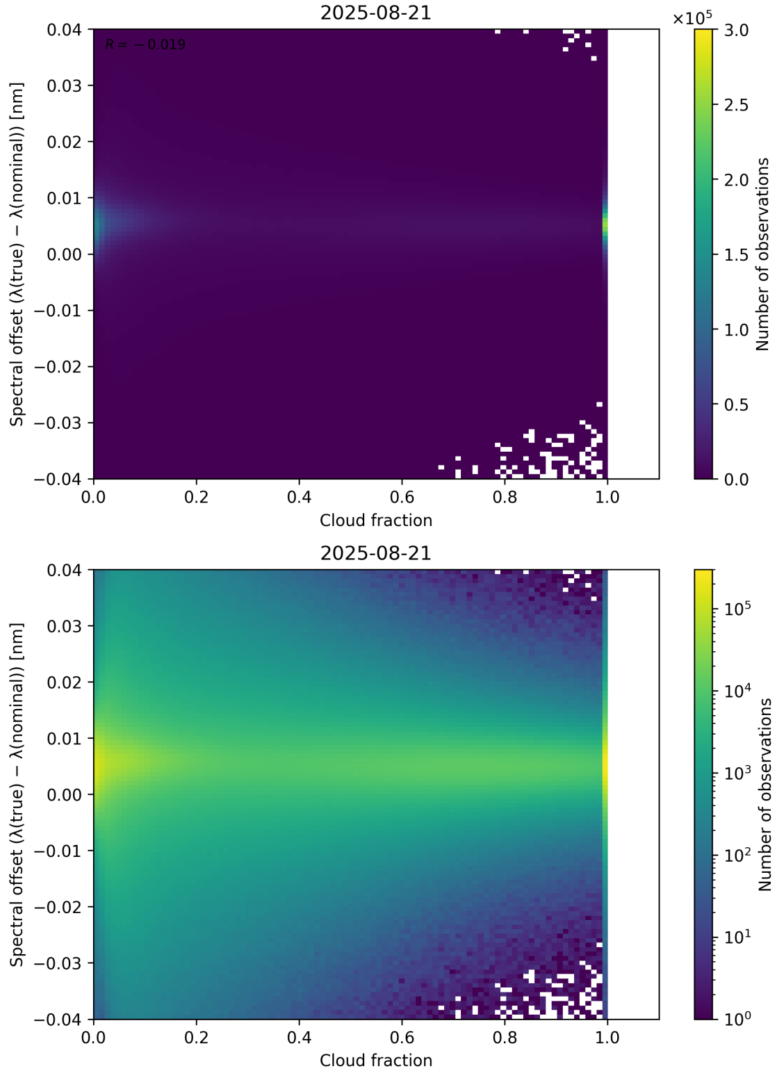
Figure 76: Scatter density plot of “Cloud fraction” against “Spectral offset ( \lambda_{\text{true}} - \lambda_{\text{nominal}} )” for 2025-08-20 to 2025-08-22.
