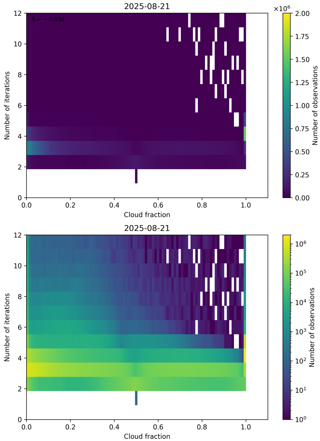
Figure 73: Scatter density plot of “Cloud fraction” against “Number of iterations” for 2025-08-20 to 2025-08-22.
