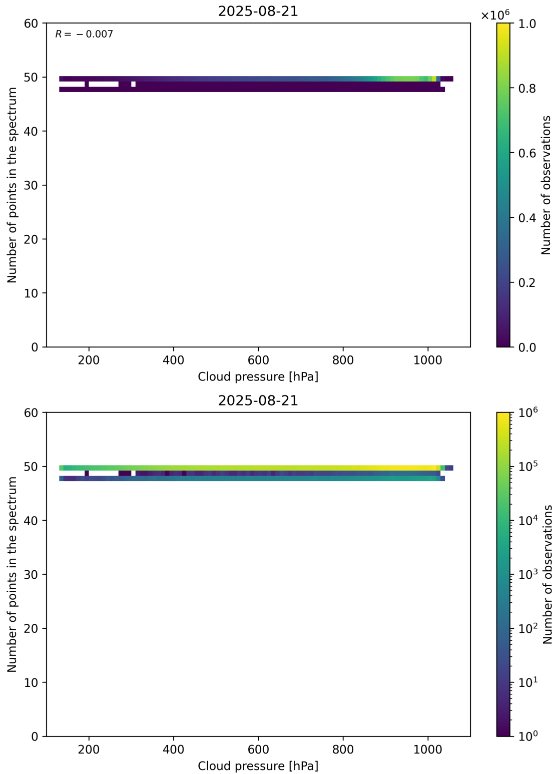
Figure 82: Scatter density plot of “Cloud pressure” against “Number of points in the spectrum” for 2025-08-20 to 2025-08-22.
