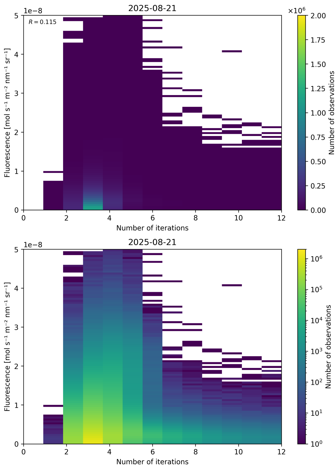
Figure 98: Scatter density plot of “Number of iterations” against “Fluorescence” for 2025-08-20 to 2025-08-22.
