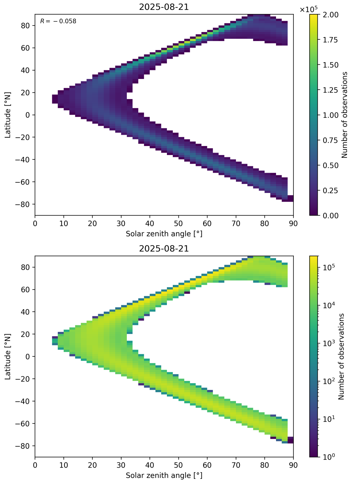
Figure 113: Scatter density plot of “Solar zenith angle” against “Latitude” for 2025-08-20 to 2025-08-22.
