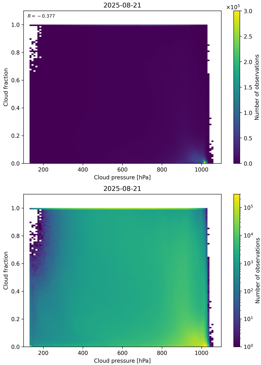
Figure 79: Scatter density plot of “Cloud pressure” against “Cloud fraction” for 2025-08-20 to 2025-08-22.
