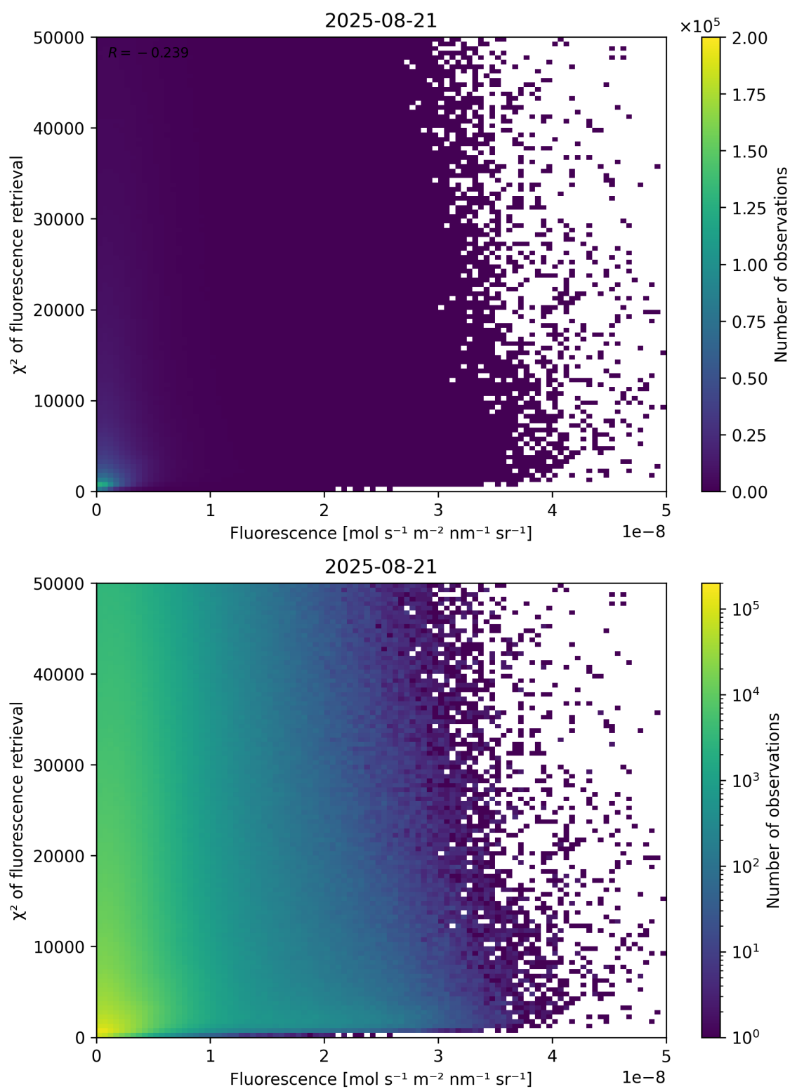
Figure 85: Scatter density plot of “Fluorescence” against “ \chi^2 of fluorescence retrieval” for 2025-08-20 to 2025-08-22.
