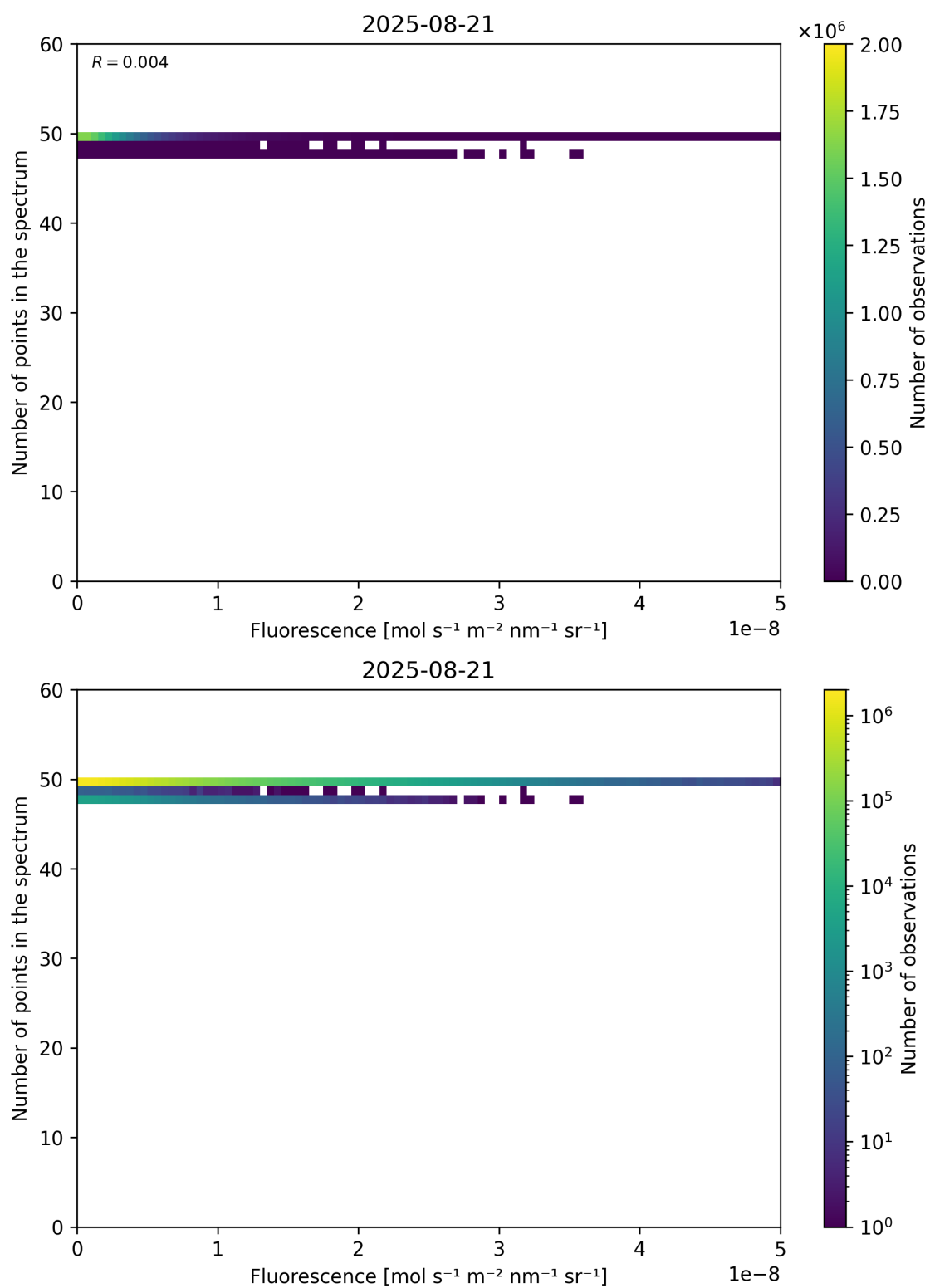
Figure 86: Scatter density plot of “Fluorescence” against “Number of points in the spectrum” for 2025-08-20 to 2025-08-22.
