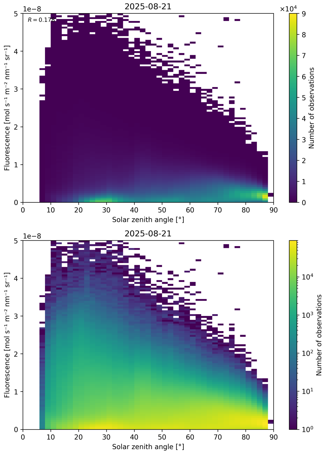
Figure 112: Scatter density plot of “Solar zenith angle” against “Fluorescence” for 2025-08-20 to 2025-08-22.
