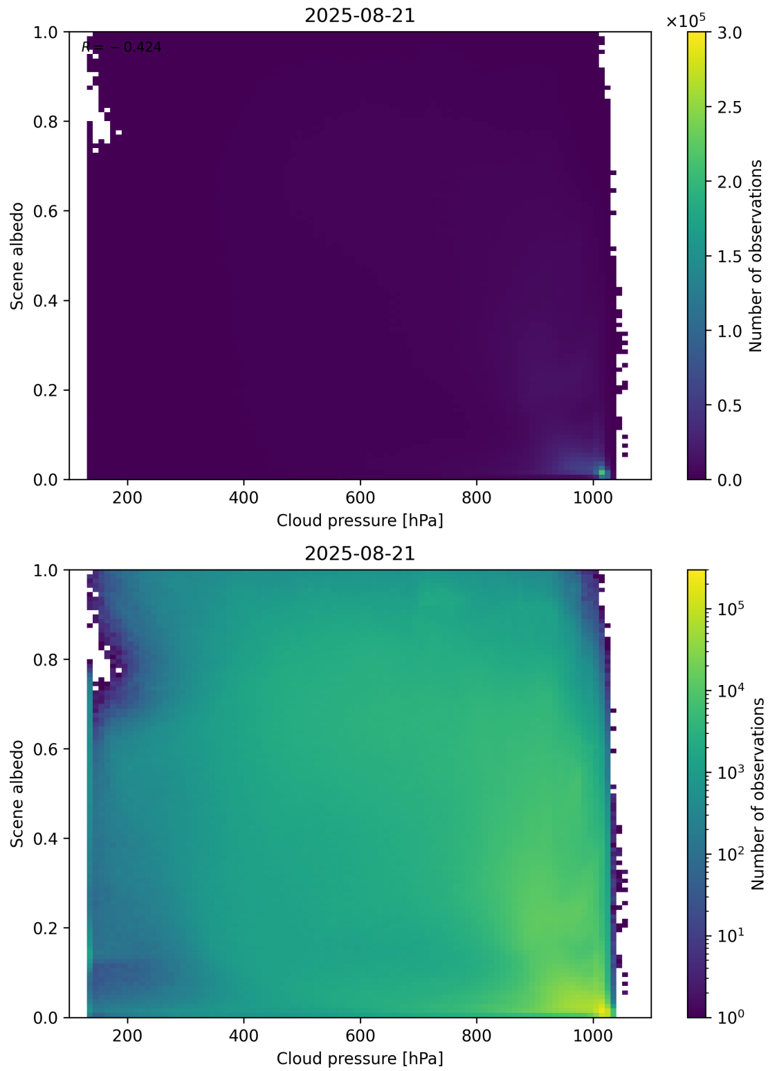
Figure 83: Scatter density plot of “Cloud pressure” against “Scene albedo” for 2025-08-20 to 2025-08-22.
