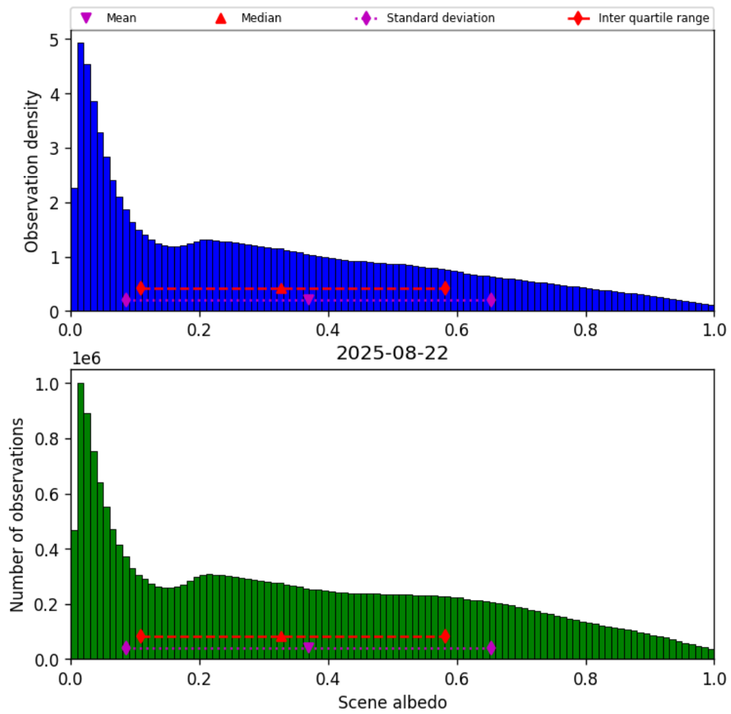
Figure 34: Histogram of “Scene albedo” for 2025-08-21 to 2025-08-23
