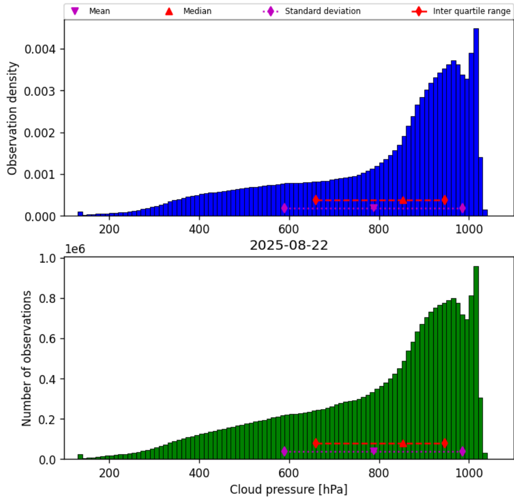
Figure 30: Histogram of “Cloud pressure” for 2025-08-21 to 2025-08-23
