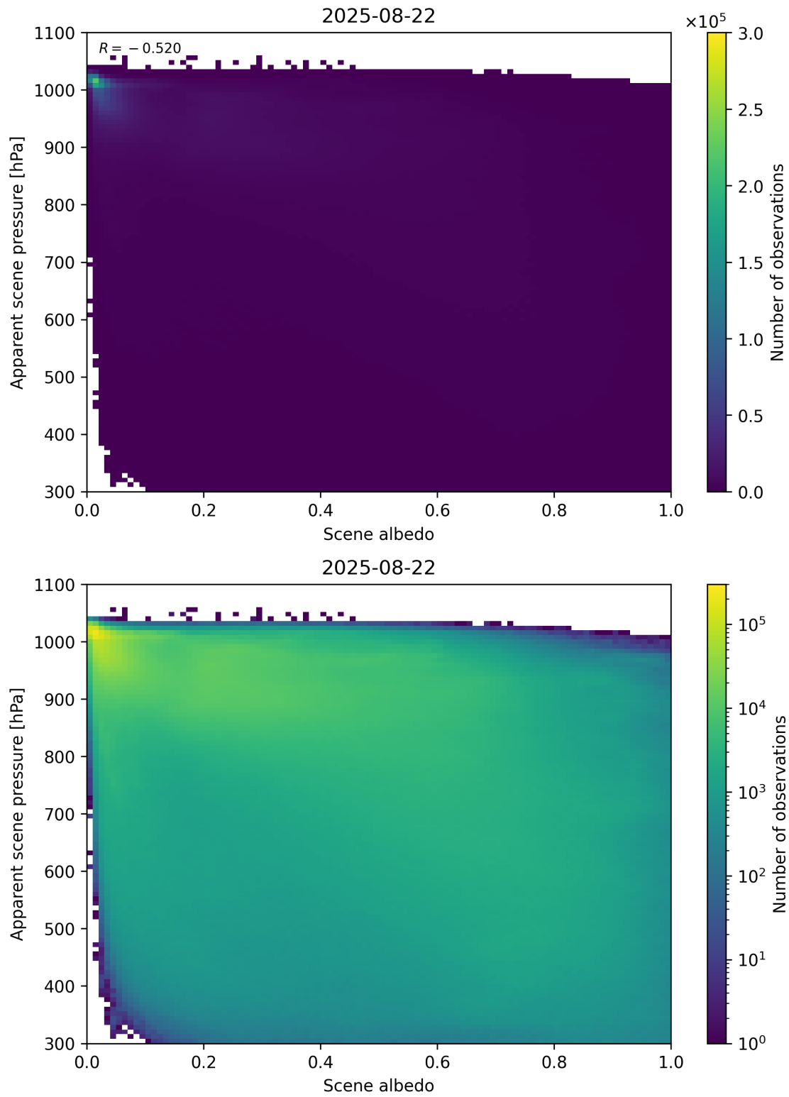
Figure 102: Scatter density plot of “Scene albedo” against “Apparent scene pressure” for 2025-08-21 to 2025-08-23.
