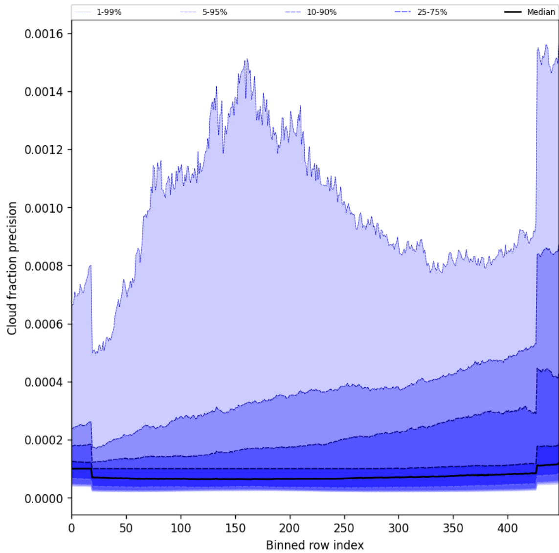
Figure 50: Along track statistics of “Cloud fraction precision” for 2025-08-21 to 2025-08-23
