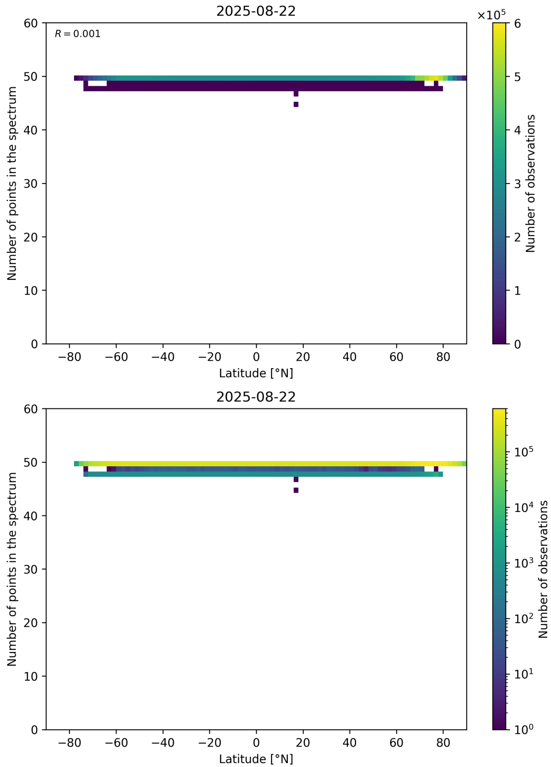
Figure 94: Scatter density plot of “Latitude” against “Number of points in the spectrum” for 2025-08-21 to 2025-08-23.
