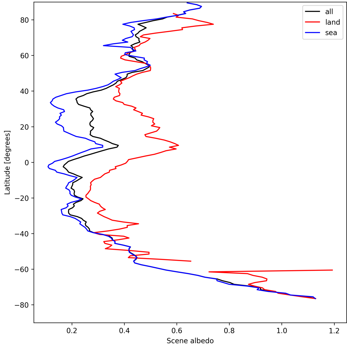
Figure 17: Zonal average of “Scene albedo” for 2025-08-21 to 2025-08-23.
