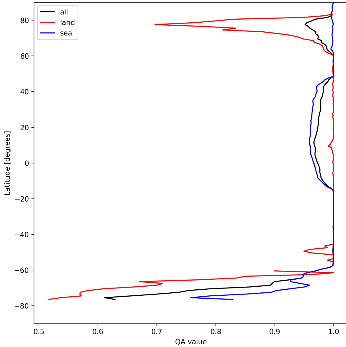
Figure 12: Zonal average of “QA value” for 2025-08-21 to 2025-08-23.
