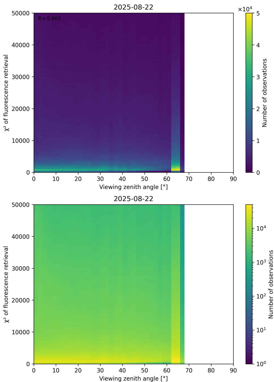
Figure 119: Scatter density plot of “Viewing zenith angle” against “ \chi^2 of fluorescence retrieval” for 2025-08-21 to 2025-08-23.
