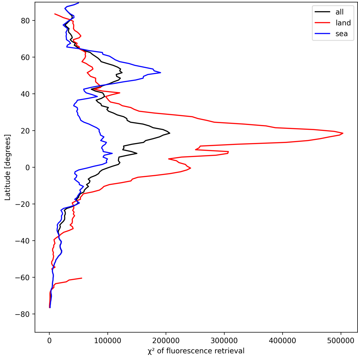
Figure 25: Zonal average of “ \chi^2 of fluorescence retrieval” for 2025-08-21 to 2025-08-23.
