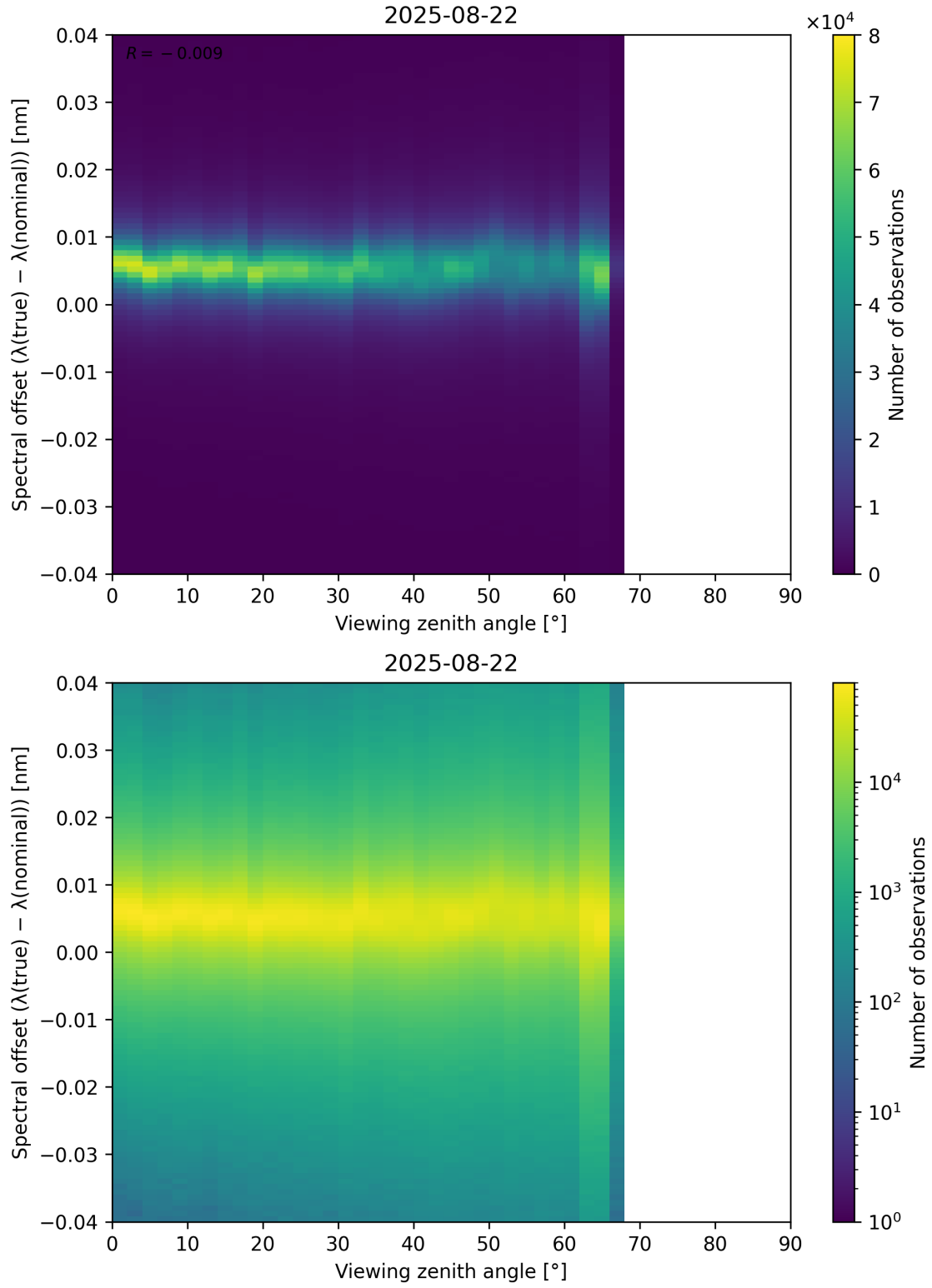
Figure 128: Scatter density plot of “Viewing zenith angle” against “Spectral offset ( \lambda_{\text{true}} - \lambda_{\text{nominal}} )” for 2025-08-21 to 2025-08-23.
