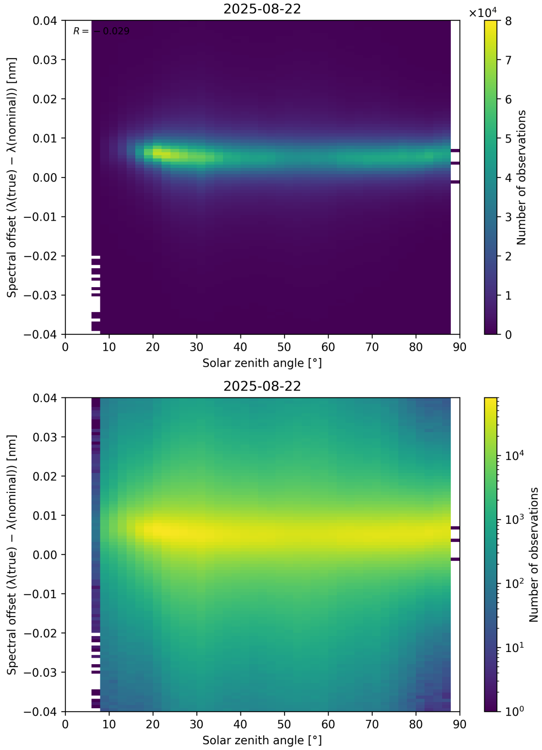
Figure 117: Scatter density plot of “Solar zenith angle” against “Spectral offset ( \lambda_{\text{true}} - \lambda_{\text{nominal}} )” for 2025-08-21 to 2025-08-23.
