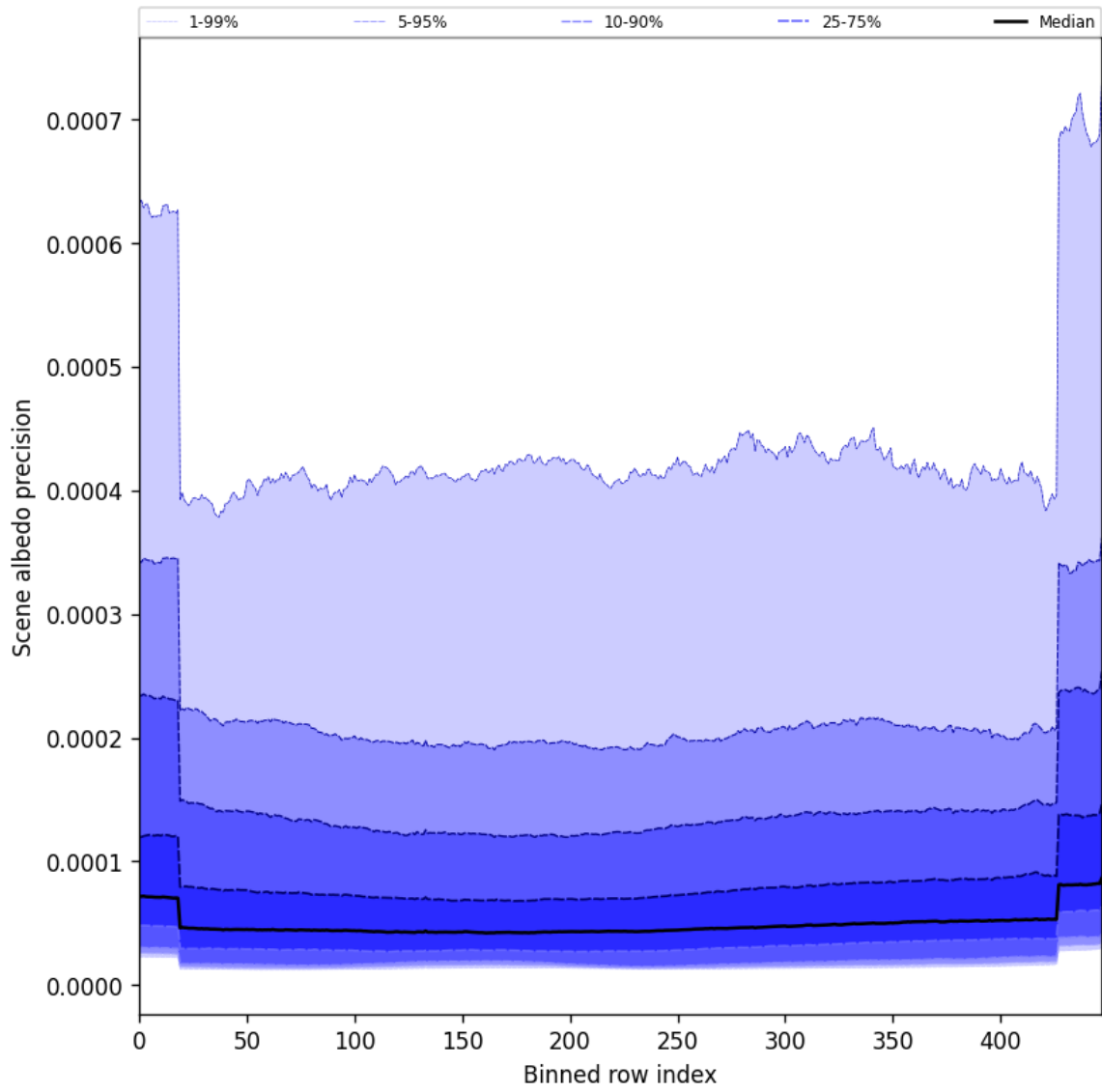
Figure 52: Along track statistics of “Scene albedo precision” for 2025-08-21 to 2025-08-23
