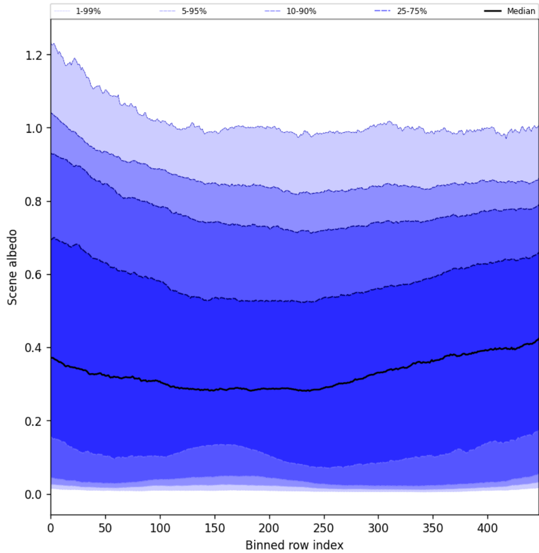
Figure 51: Along track statistics of “Scene albedo” for 2025-08-21 to 2025-08-23
