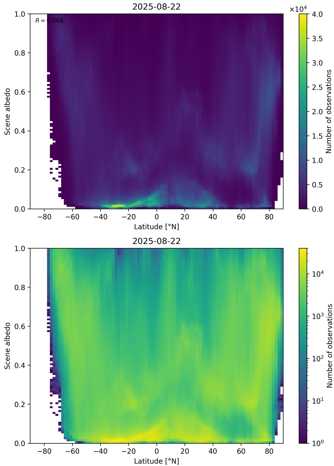
Figure 95: Scatter density plot of “Latitude” against “Scene albedo” for 2025-08-21 to 2025-08-23.
