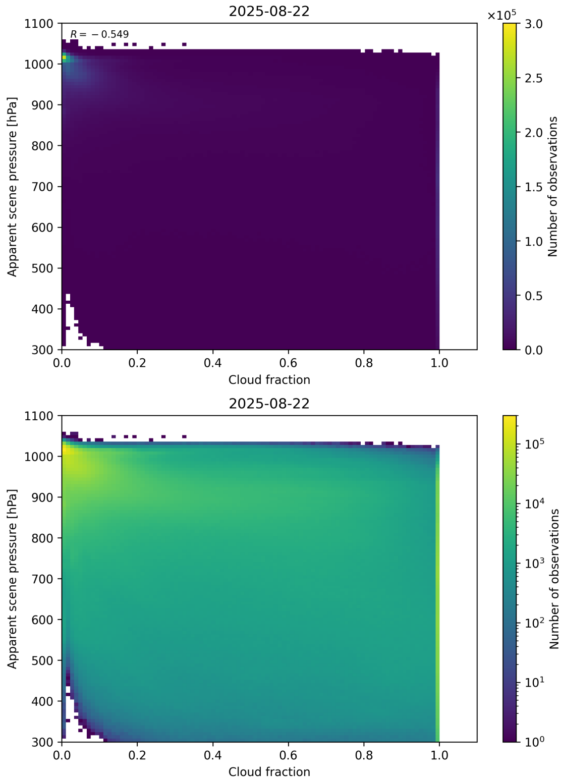
Figure 70: Scatter density plot of “Cloud fraction” against “Apparent scene pressure” for 2025-08-21 to 2025-08-23.
