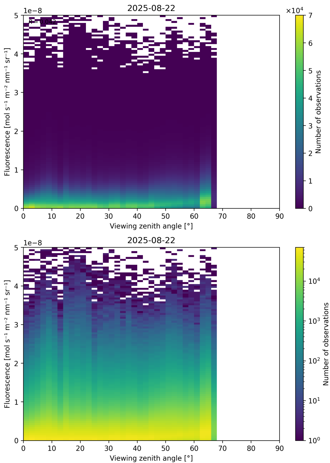
Figure 122: Scatter density plot of “Viewing zenith angle” against “Fluorescence” for 2025-08-21 to 2025-08-23.
