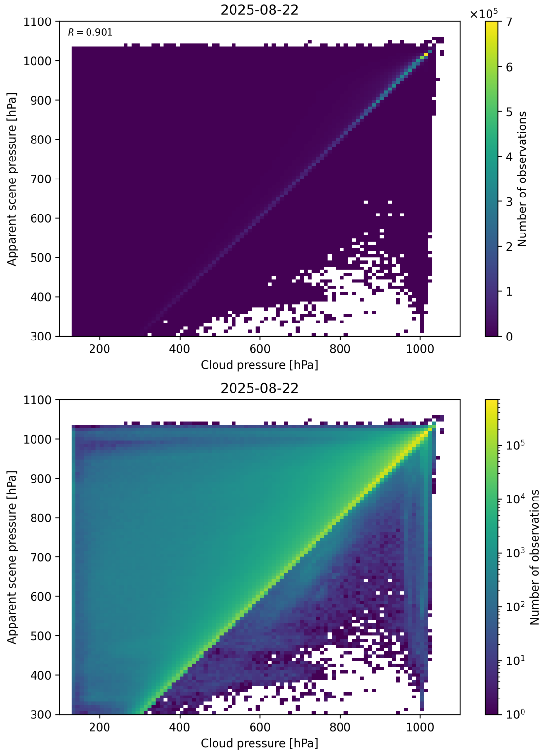
Figure 77: Scatter density plot of “Cloud pressure” against “Apparent scene pressure” for 2025-08-21 to 2025-08-23.
