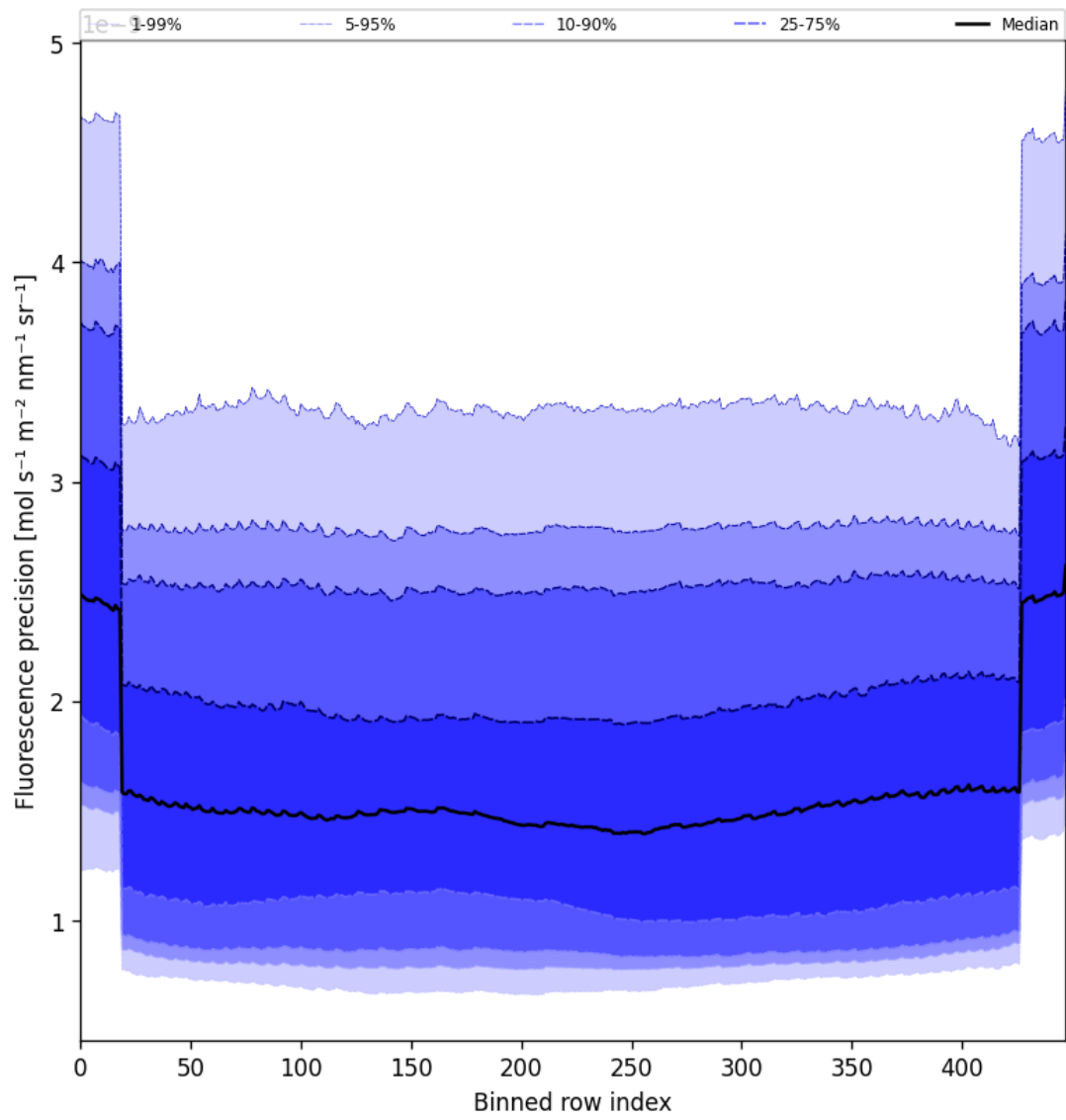
Figure 58: Along track statistics of “Fluorescence precision” for 2025-08-21 to 2025-08-23
