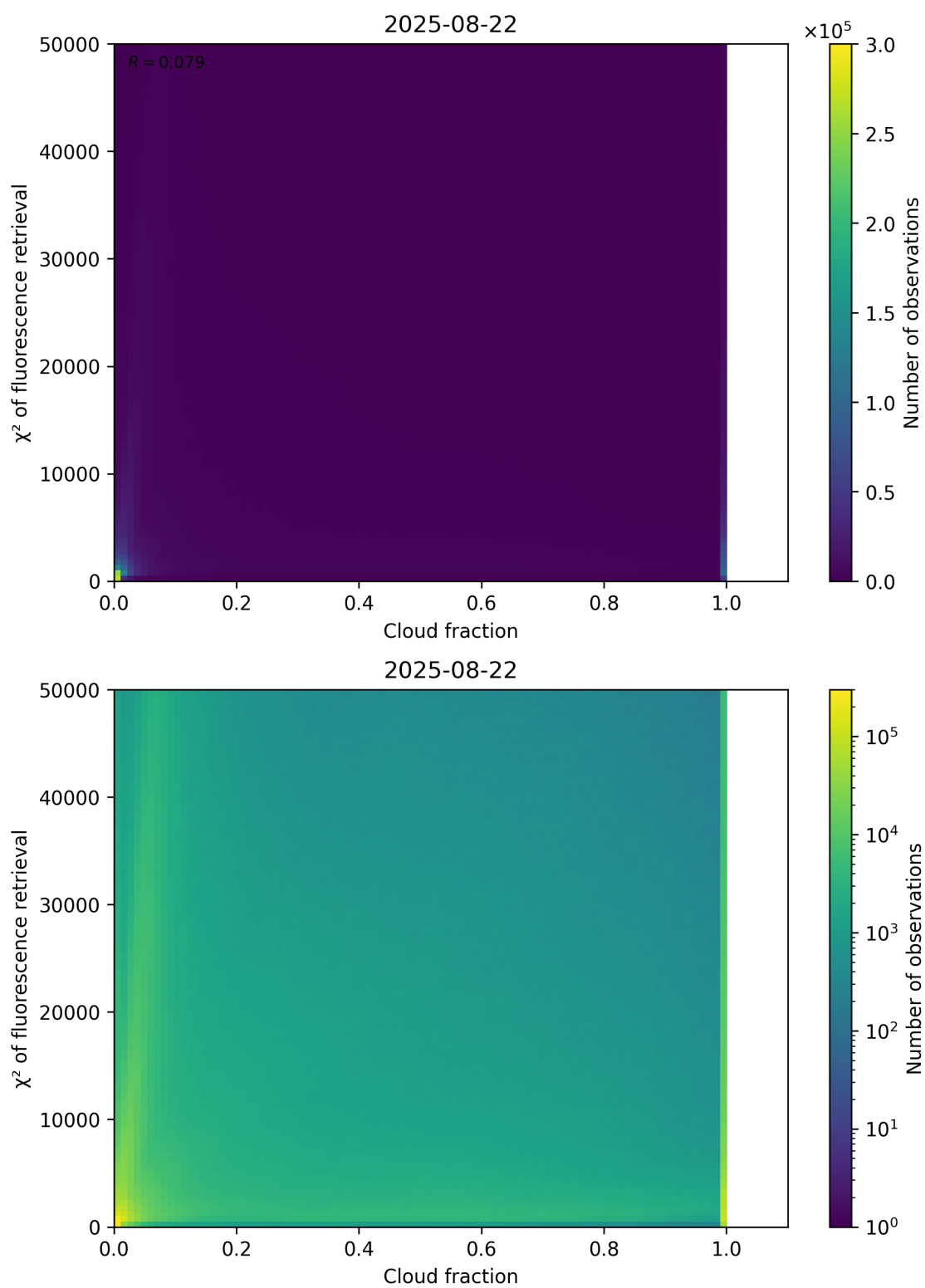
Figure 71: Scatter density plot of “Cloud fraction” against “ \chi^2 of fluorescence retrieval” for 2025-08-21 to 2025-08-23.
