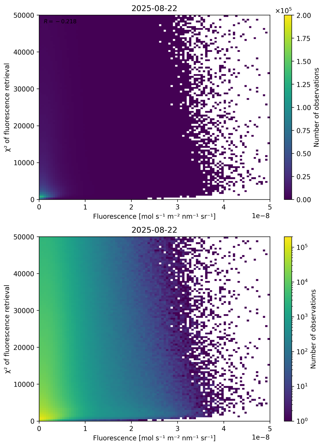
Figure 85: Scatter density plot of “Fluorescence” against “ \chi^2 of fluorescence retrieval” for 2025-08-21 to 2025-08-23.
