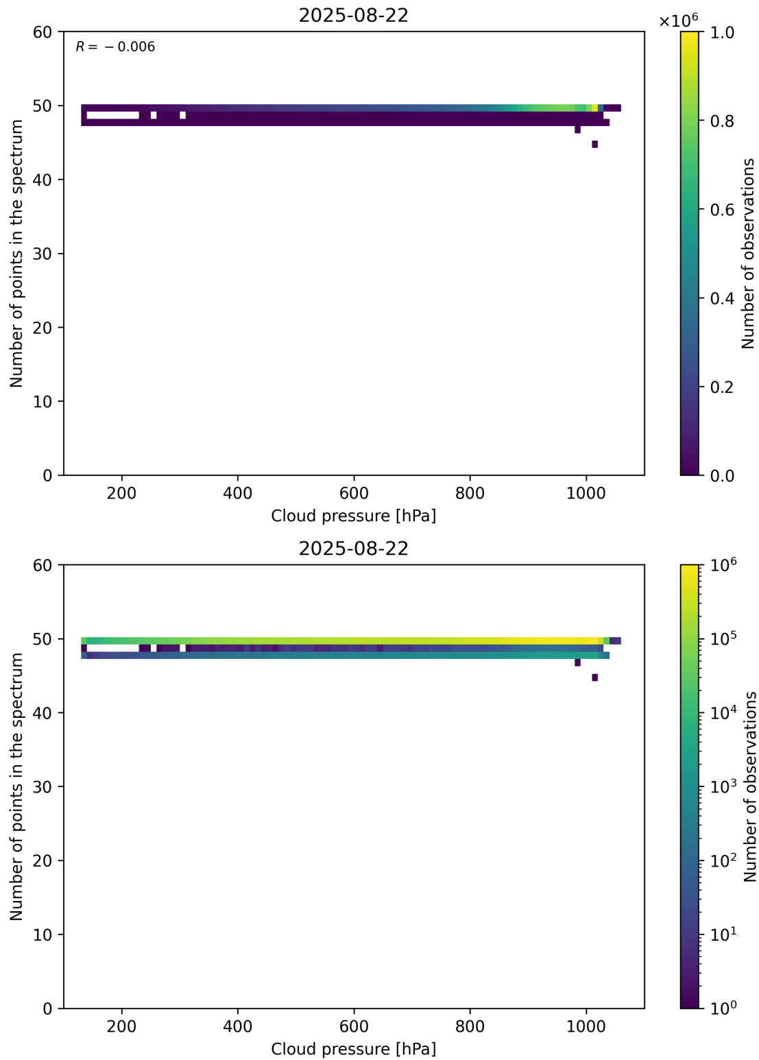
Figure 82: Scatter density plot of “Cloud pressure” against “Number of points in the spectrum” for 2025-08-21 to 2025-08-23.
