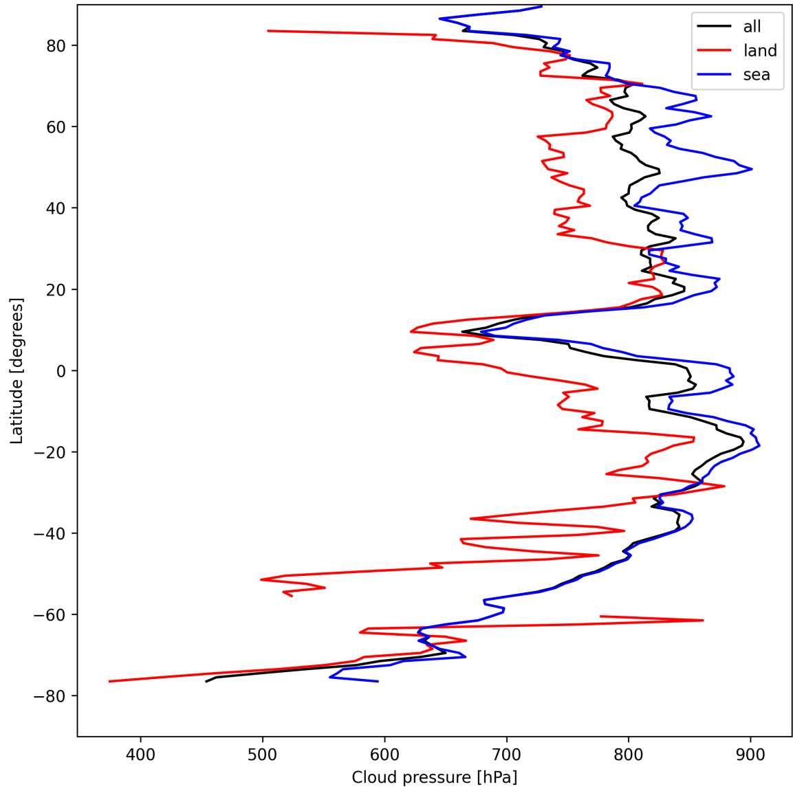
Figure 13: Zonal average of “Cloud pressure” for 2025-08-21 to 2025-08-23.
