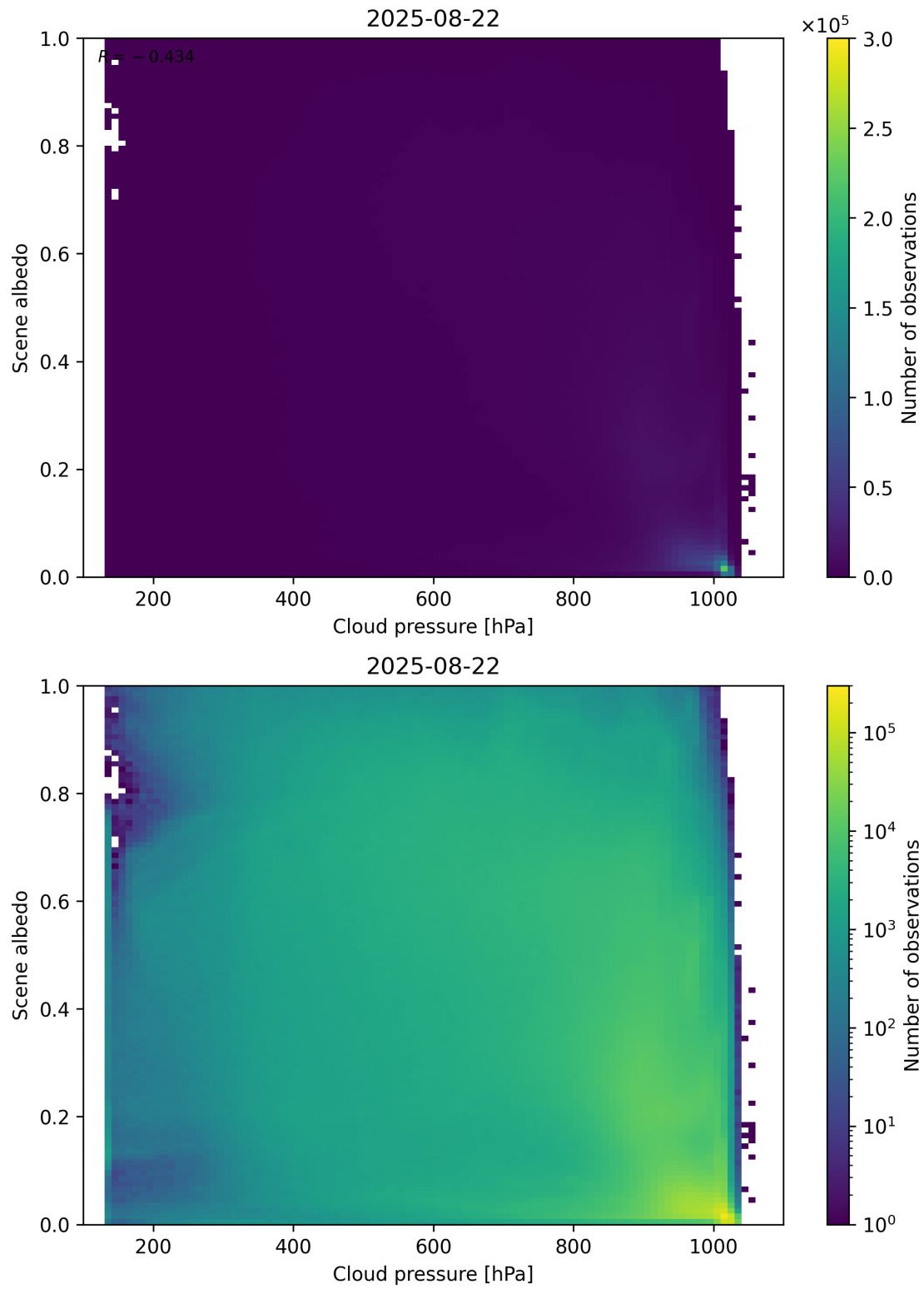
Figure 83: Scatter density plot of “Cloud pressure” against “Scene albedo” for 2025-08-21 to 2025-08-23.
