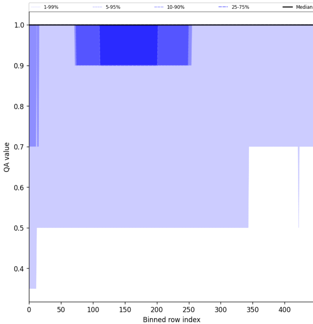
Figure 46: Along track statistics of “QA value” for 2025-08-21 to 2025-08-23
