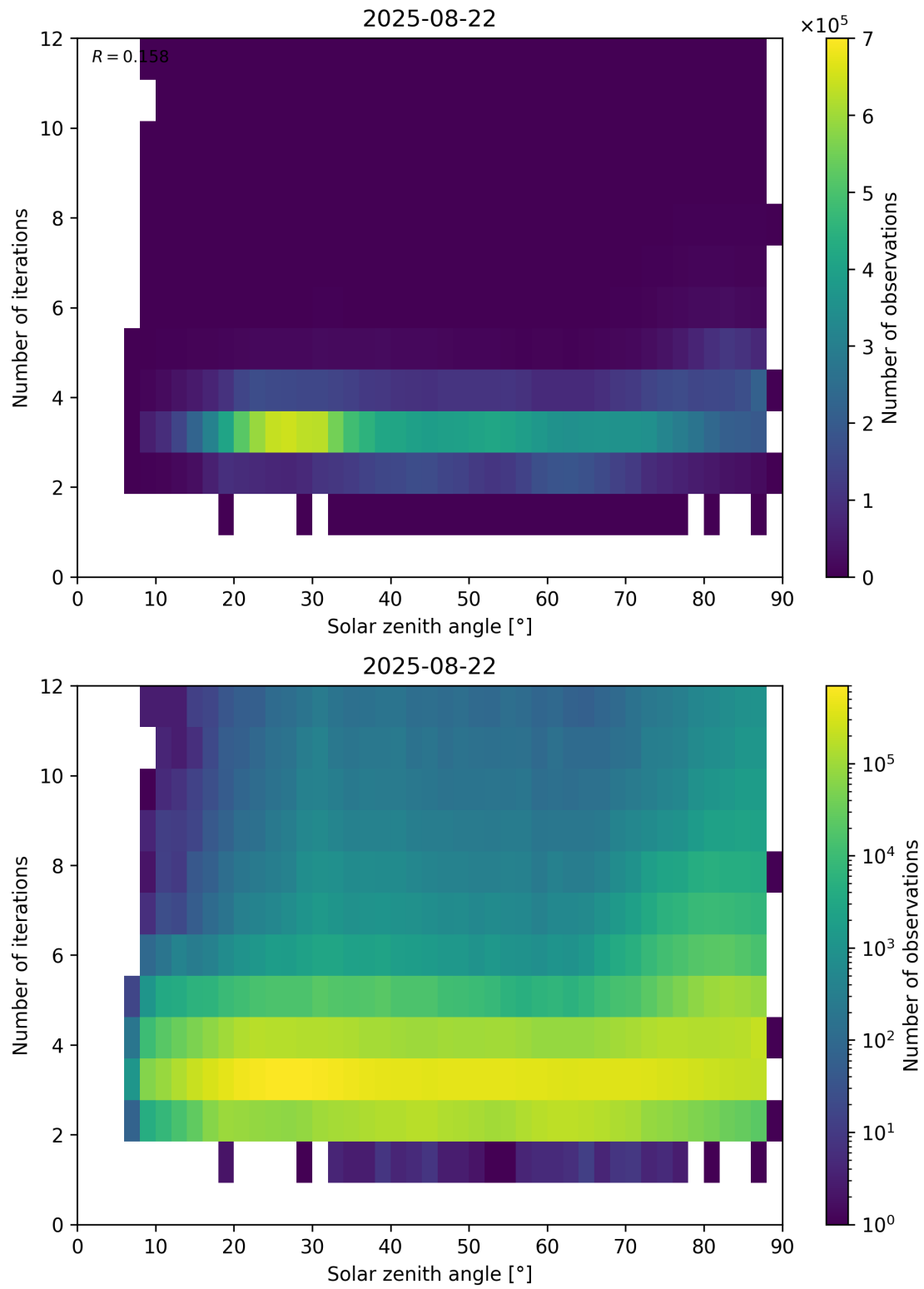
Figure 114: Scatter density plot of “Solar zenith angle” against “Number of iterations” for 2025-08-21 to 2025-08-23.
