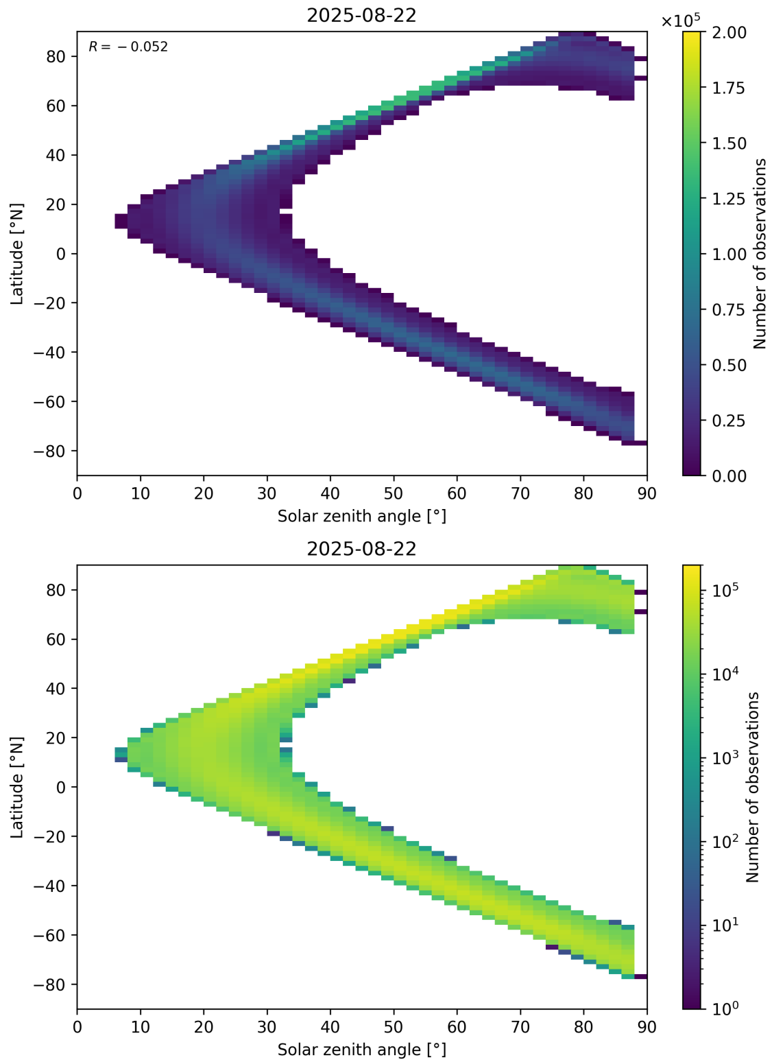
Figure 113: Scatter density plot of “Solar zenith angle” against “Latitude” for 2025-08-21 to 2025-08-23.
