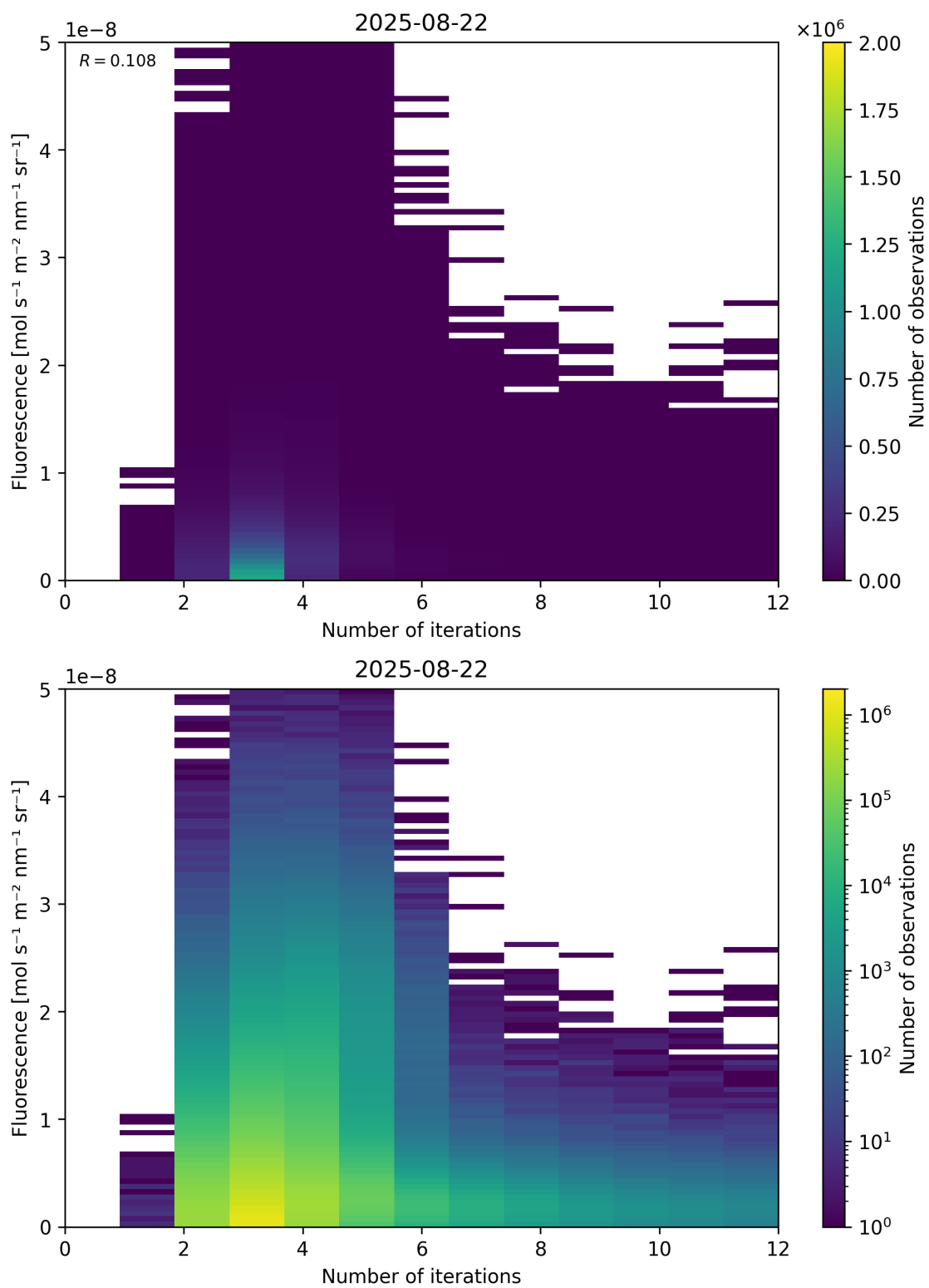
Figure 98: Scatter density plot of “Number of iterations” against “Fluorescence” for 2025-08-21 to 2025-08-23.
