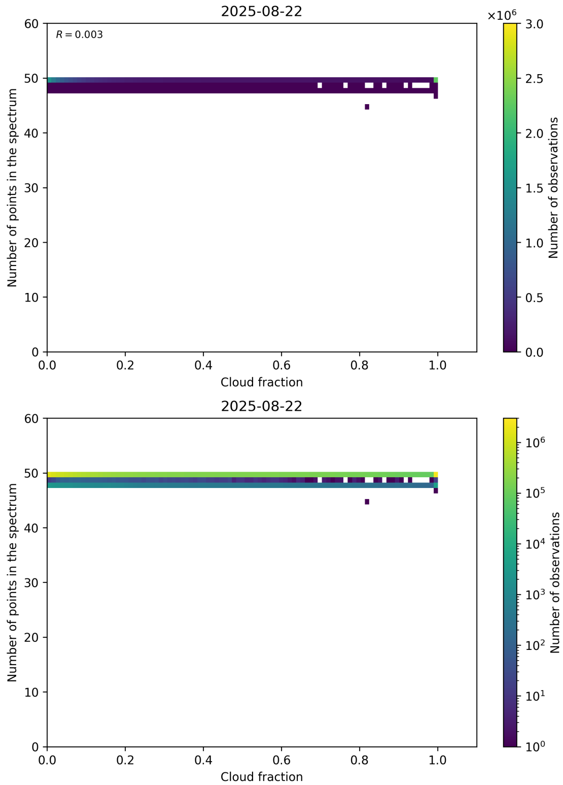
Figure 74: Scatter density plot of “Cloud fraction” against “Number of points in the spectrum” for 2025-08-21 to 2025-08-23.
