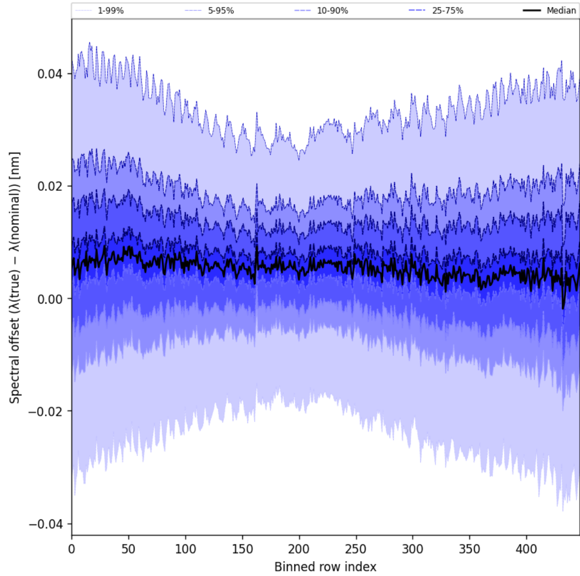
Figure 62: Along track statistics of “Spectral offset ( \lambda_{\text{true}} - \lambda_{\text{nominal}} )” for 2025-08-21 to 2025-08-23
