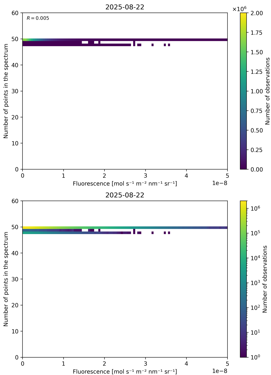
Figure 86: Scatter density plot of “Fluorescence” against “Number of points in the spectrum” for 2025-08-21 to 2025-08-23.
