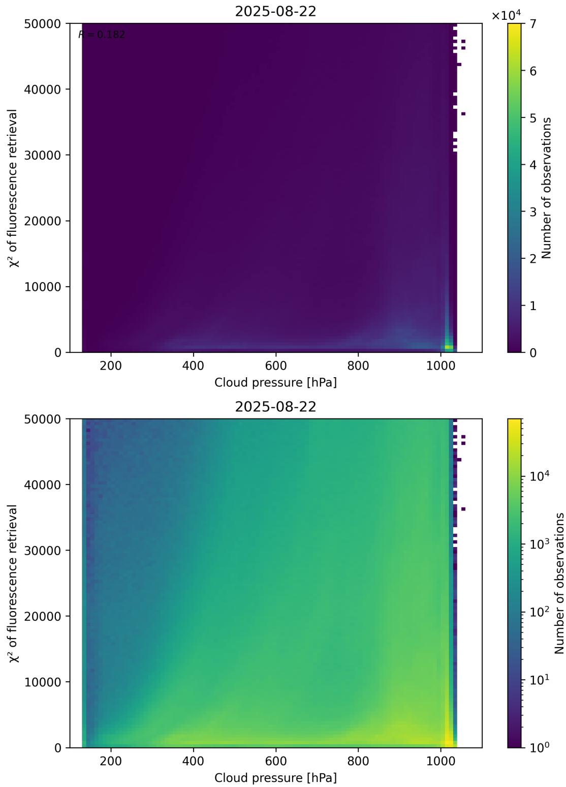
Figure 78: Scatter density plot of “Cloud pressure” against “ \chi^2 of fluorescence retrieval” for 2025-08-21 to 2025-08-23.
