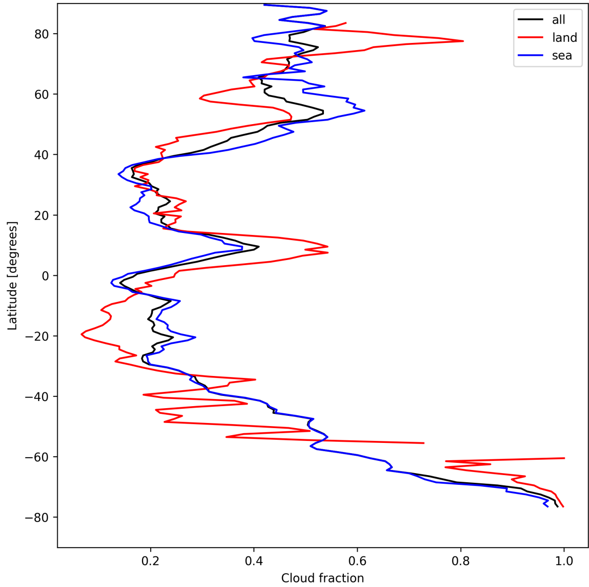
Figure 15: Zonal average of “Cloud fraction” for 2025-08-21 to 2025-08-23.
