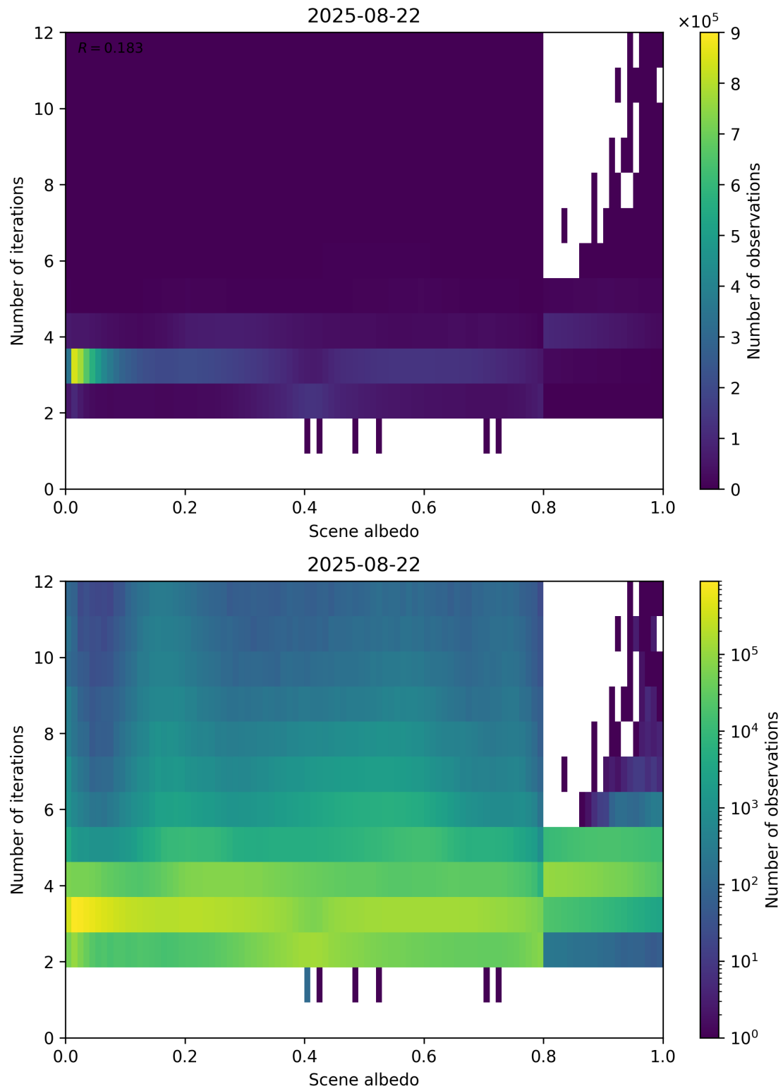
Figure 105: Scatter density plot of “Scene albedo” against “Number of iterations” for 2025-08-21 to 2025-08-23.
