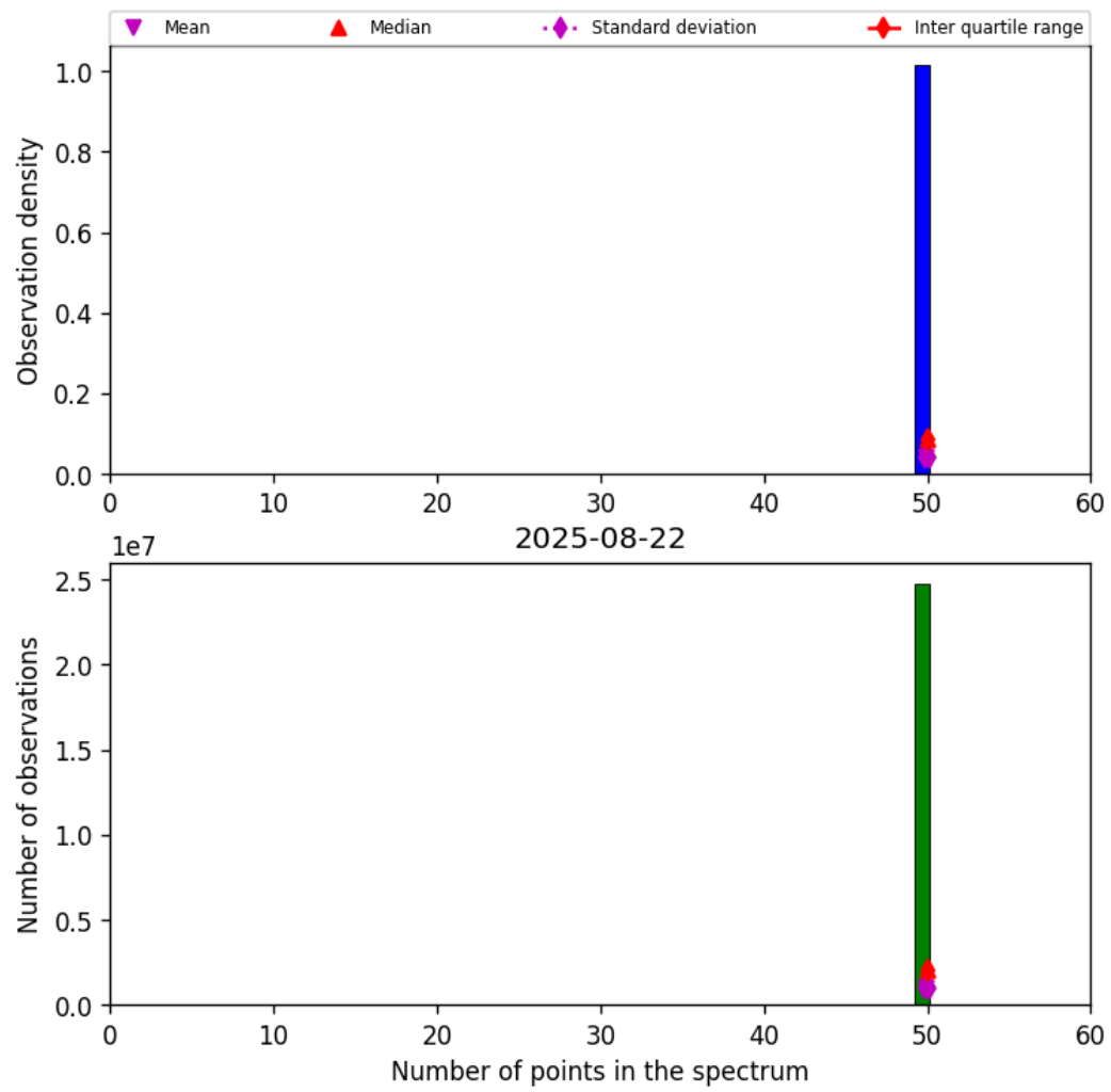
Figure 44: Histogram of “Number of points in the spectrum” for 2025-08-21 to 2025-08-23
