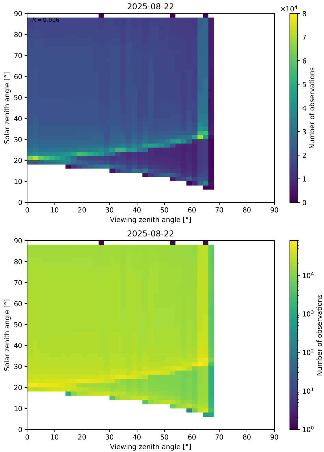
Figure 127: Scatter density plot of “Viewing zenith angle” against “Solar zenith angle” for 2025-08-21 to 2025-08-23.
