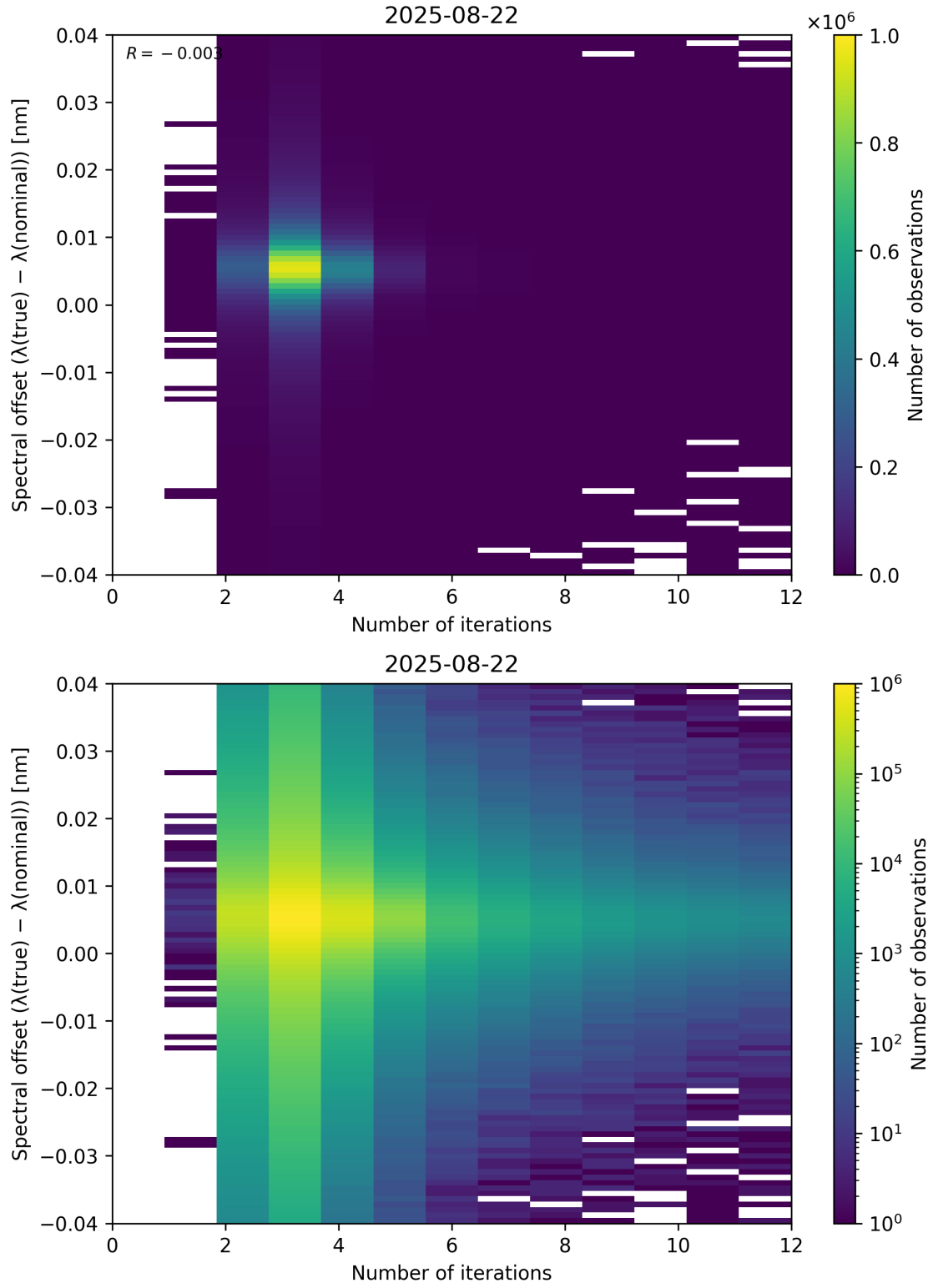
Figure 100: Scatter density plot of “Number of iterations” against “Spectral offset ( \lambda_{\text{true}} - \lambda_{\text{nominal}} )” for 2025-08-21 to 2025-08-23.
