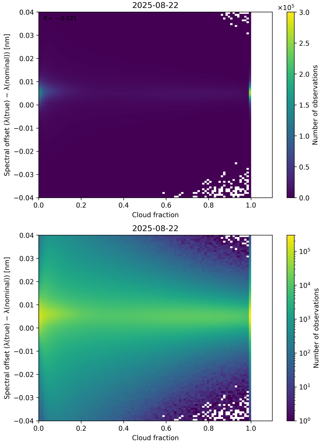
Figure 76: Scatter density plot of “Cloud fraction” against “Spectral offset ( \lambda_{\text{true}} - \lambda_{\text{nominal}} )” for 2025-08-21 to 2025-08-23.
