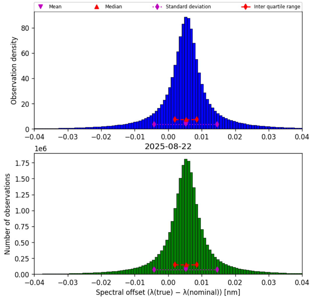
Figure 45: Histogram of “Spectral offset ( \lambda_{\text{true}} - \lambda_{\text{nominal}} )” for 2025-08-21 to 2025-08-23
