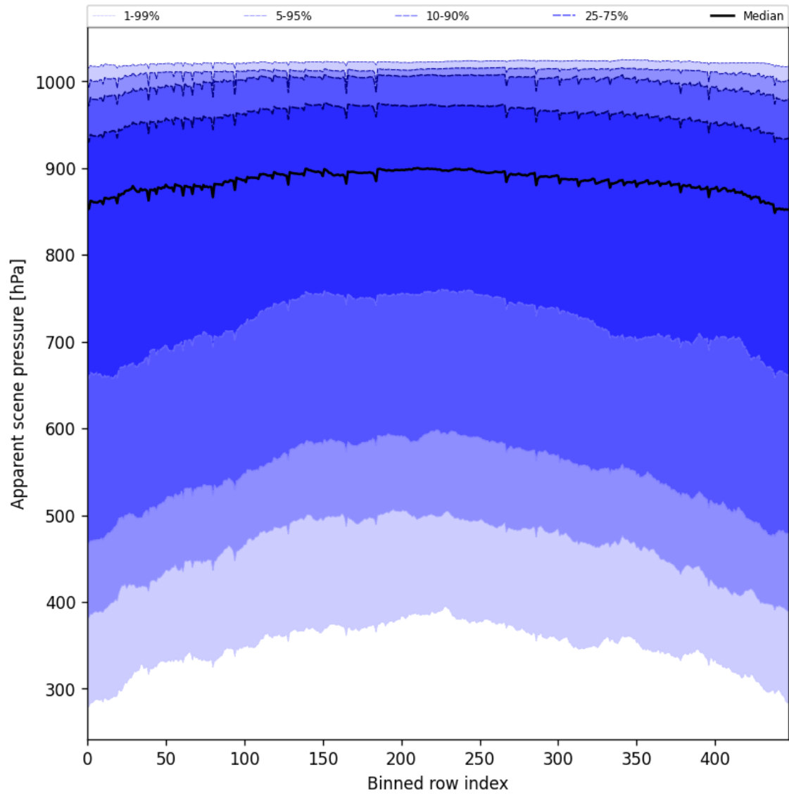
Figure 53: Along track statistics of “Apparent scene pressure” for 2025-08-21 to 2025-08-23
