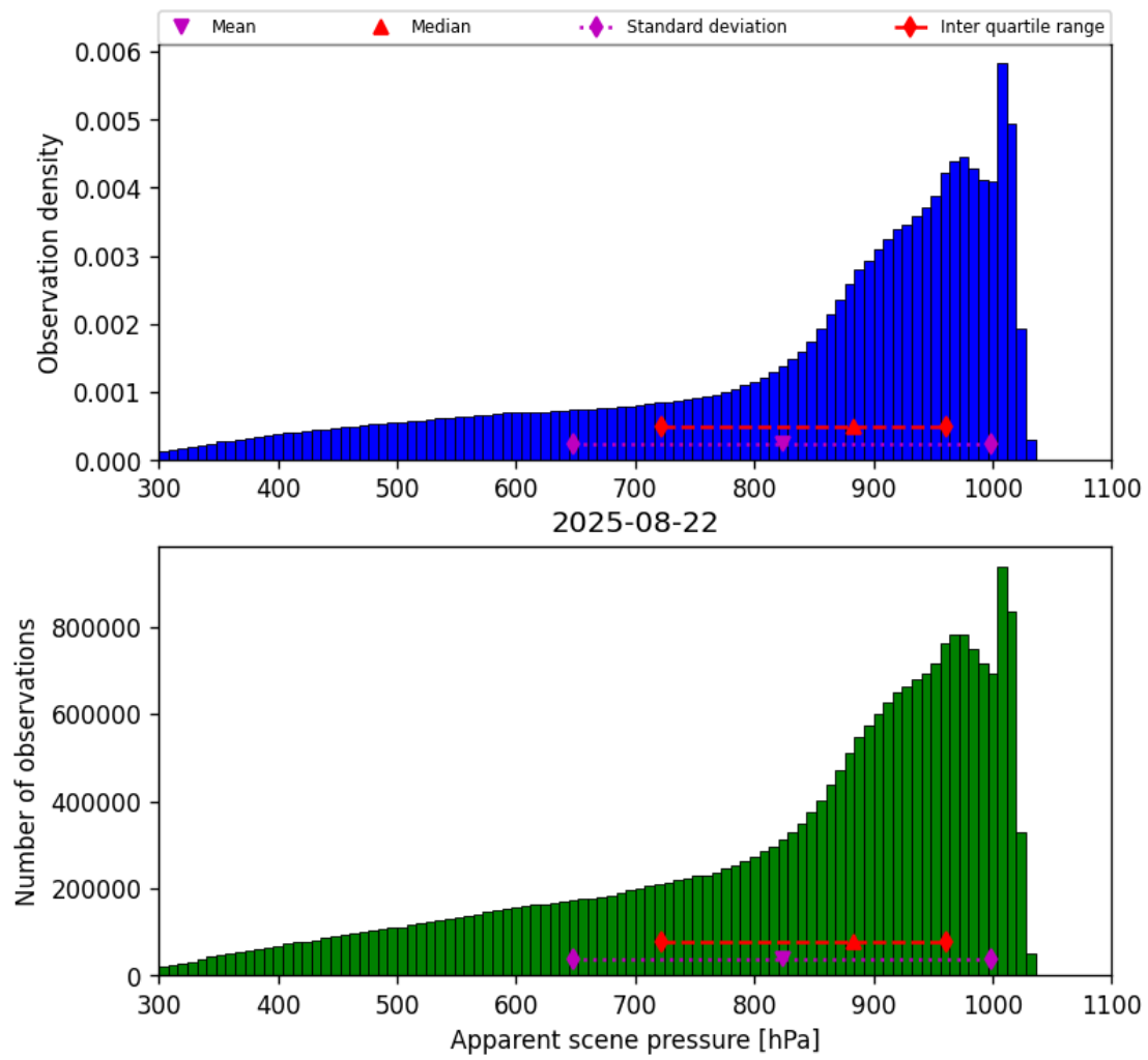
Figure 36: Histogram of “Apparent scene pressure” for 2025-08-21 to 2025-08-23
