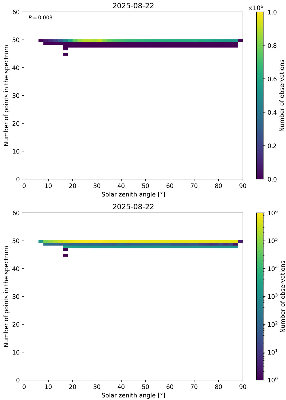
Figure 115: Scatter density plot of “Solar zenith angle” against “Number of points in the spectrum” for 2025-08-21 to 2025-08-23.
