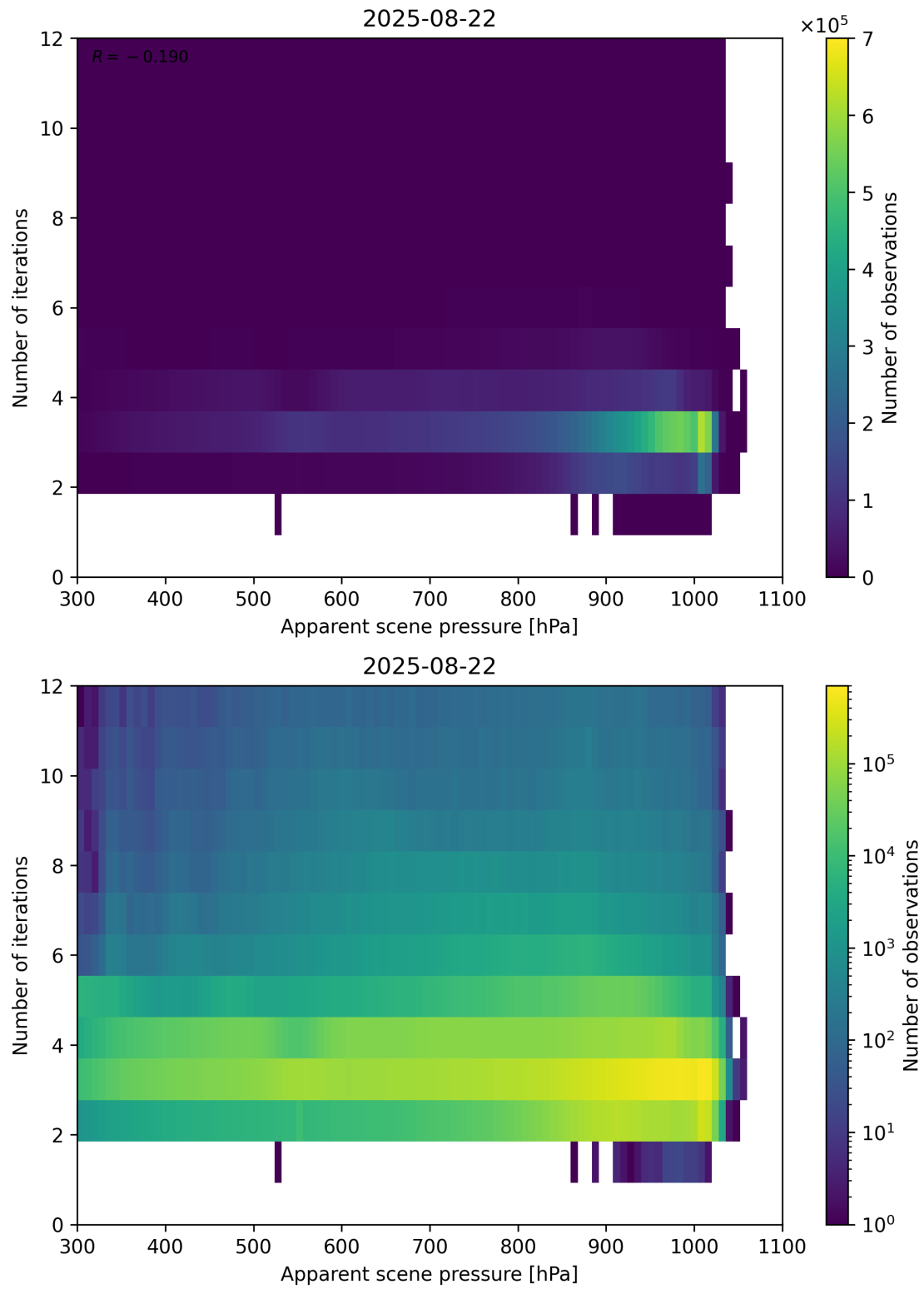
Figure 65: Scatter density plot of “Apparent scene pressure” against “Number of iterations” for 2025-08-21 to 2025-08-23.
