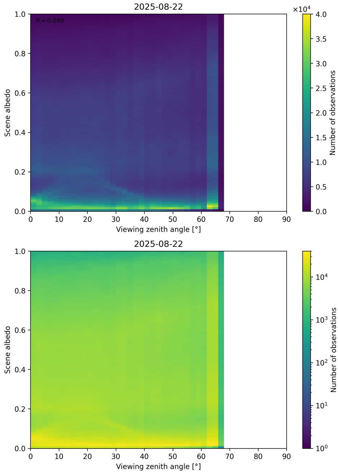
Figure 126: Scatter density plot of “Viewing zenith angle” against “Scene albedo” for 2025-08-21 to 2025-08-23.
