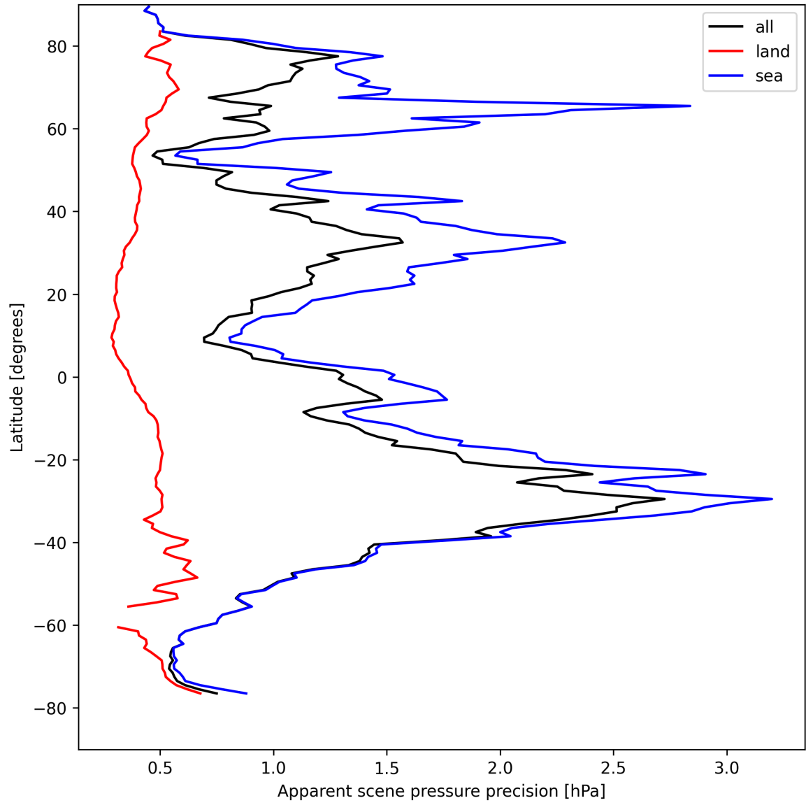
Figure 20: Zonal average of “Apparent scene pressure precision” for 2025-08-21 to 2025-08-23.
