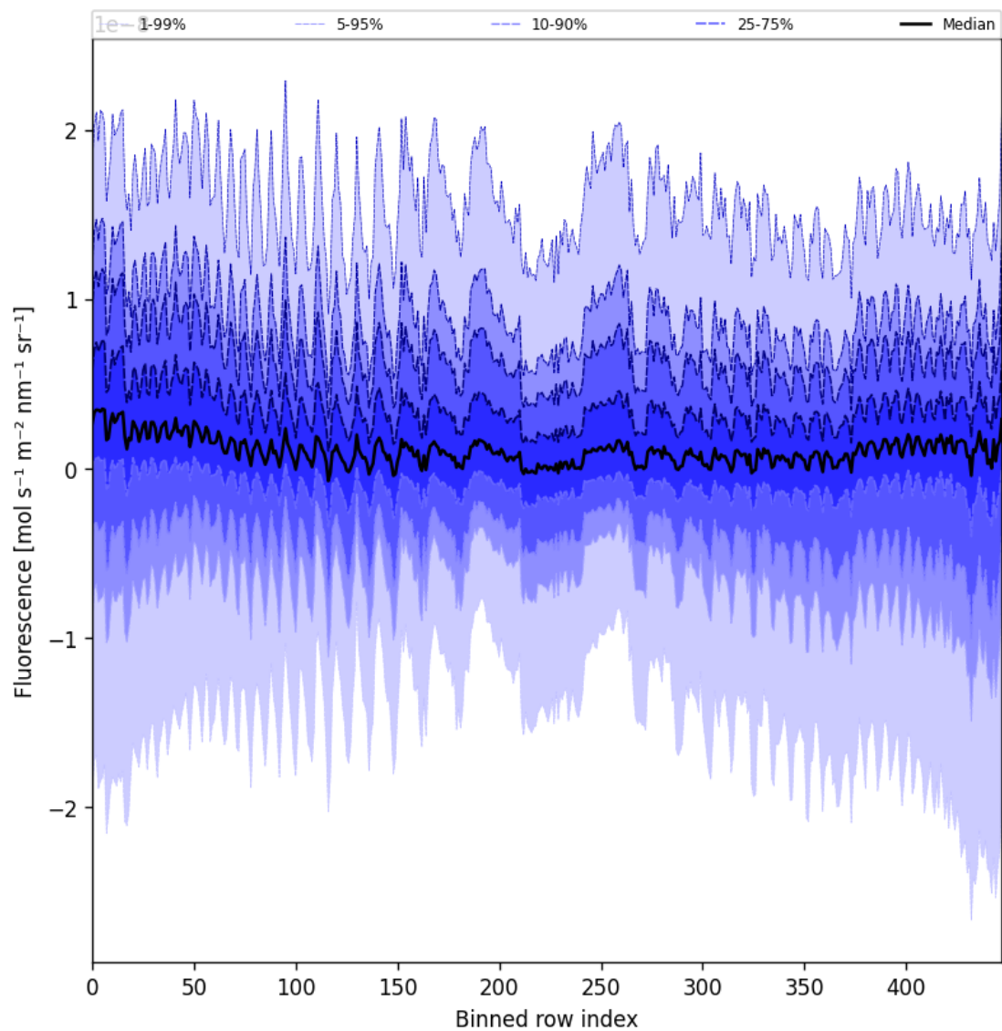
Figure 57: Along track statistics of “Fluorescence” for 2025-08-21 to 2025-08-23
