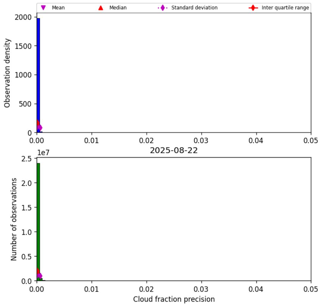
Figure 33: Histogram of “Cloud fraction precision” for 2025-08-21 to 2025-08-23
