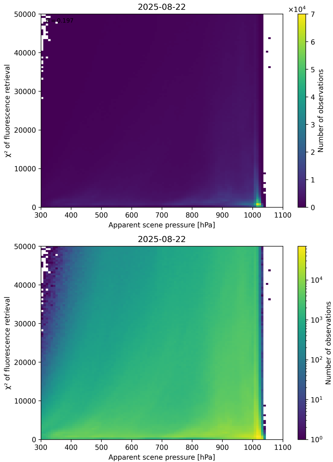
Figure 63: Scatter density plot of “Apparent scene pressure” against “ \chi^2 of fluorescence retrieval” for 2025-08-21 to 2025-08-23.
