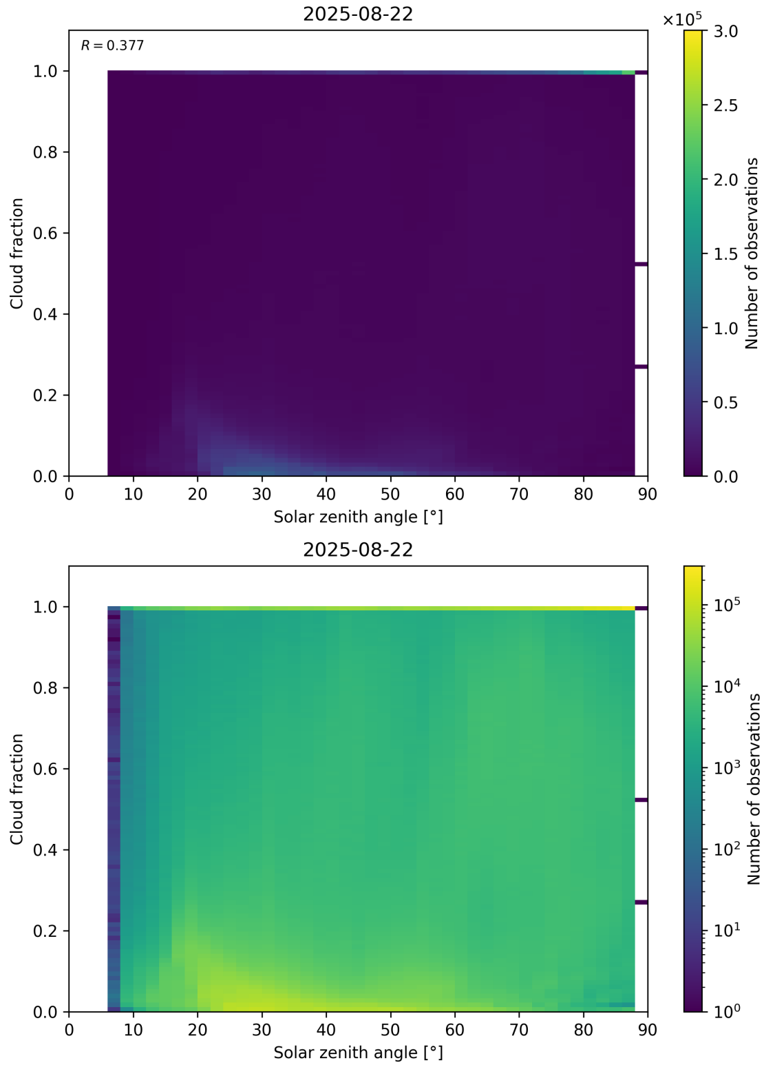
Figure 110: Scatter density plot of “Solar zenith angle” against “Cloud fraction” for 2025-08-21 to 2025-08-23.
