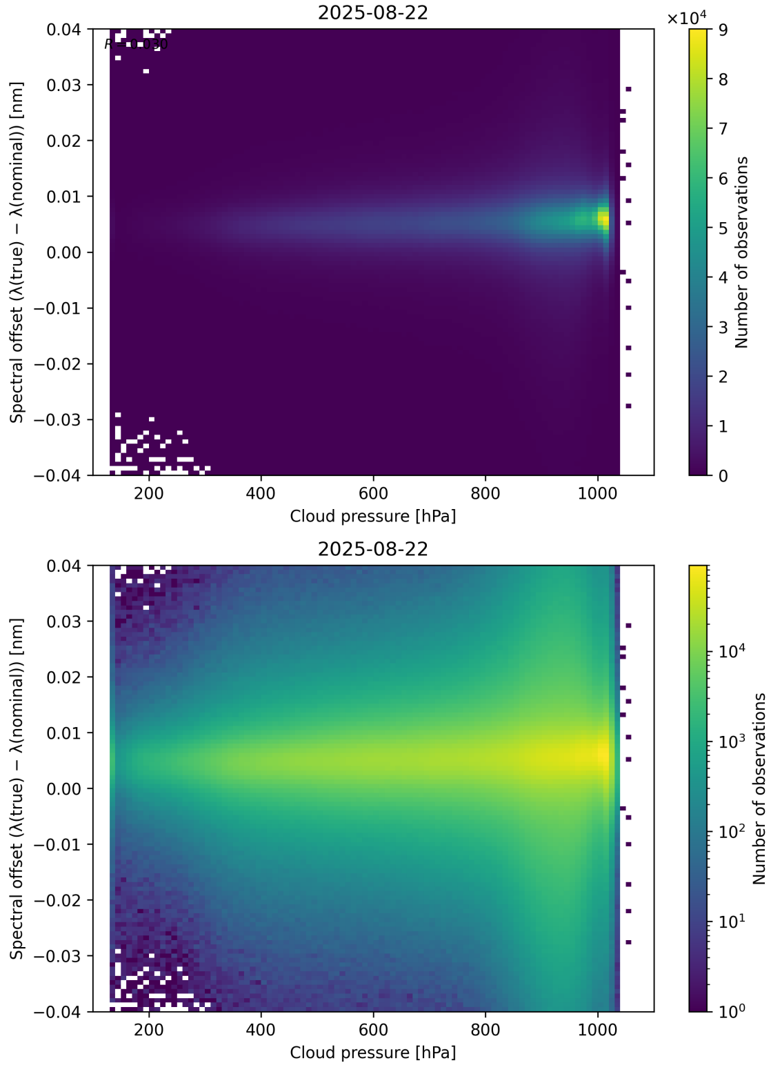
Figure 84: Scatter density plot of “Cloud pressure” against “Spectral offset ( \lambda_{\text{true}} - \lambda_{\text{nominal}} )” for 2025-08-21 to 2025-08-23.
