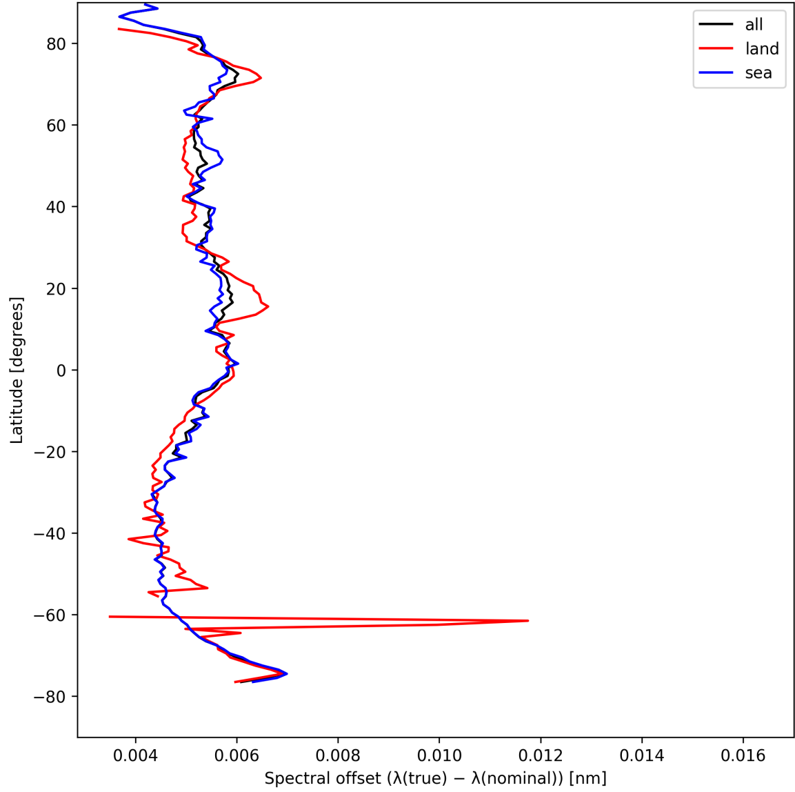
Figure 28: Zonal average of “Spectral offset ( \lambda_{\text{true}} - \lambda_{\text{nominal}} )” for 2025-08-21 to 2025-08-23.
