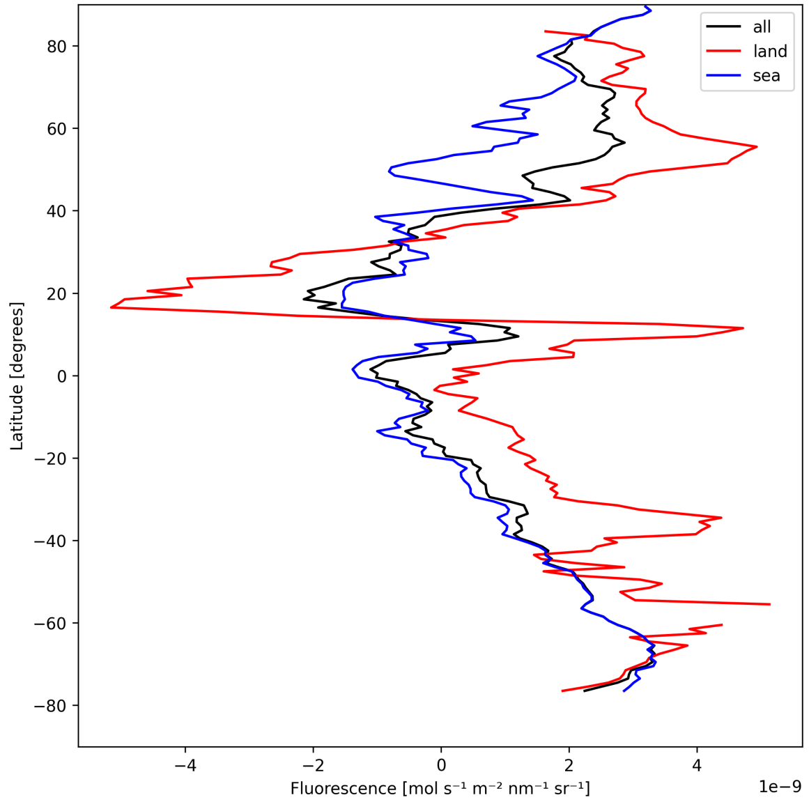
Figure 23: Zonal average of “Fluorescence” for 2025-08-21 to 2025-08-23.
