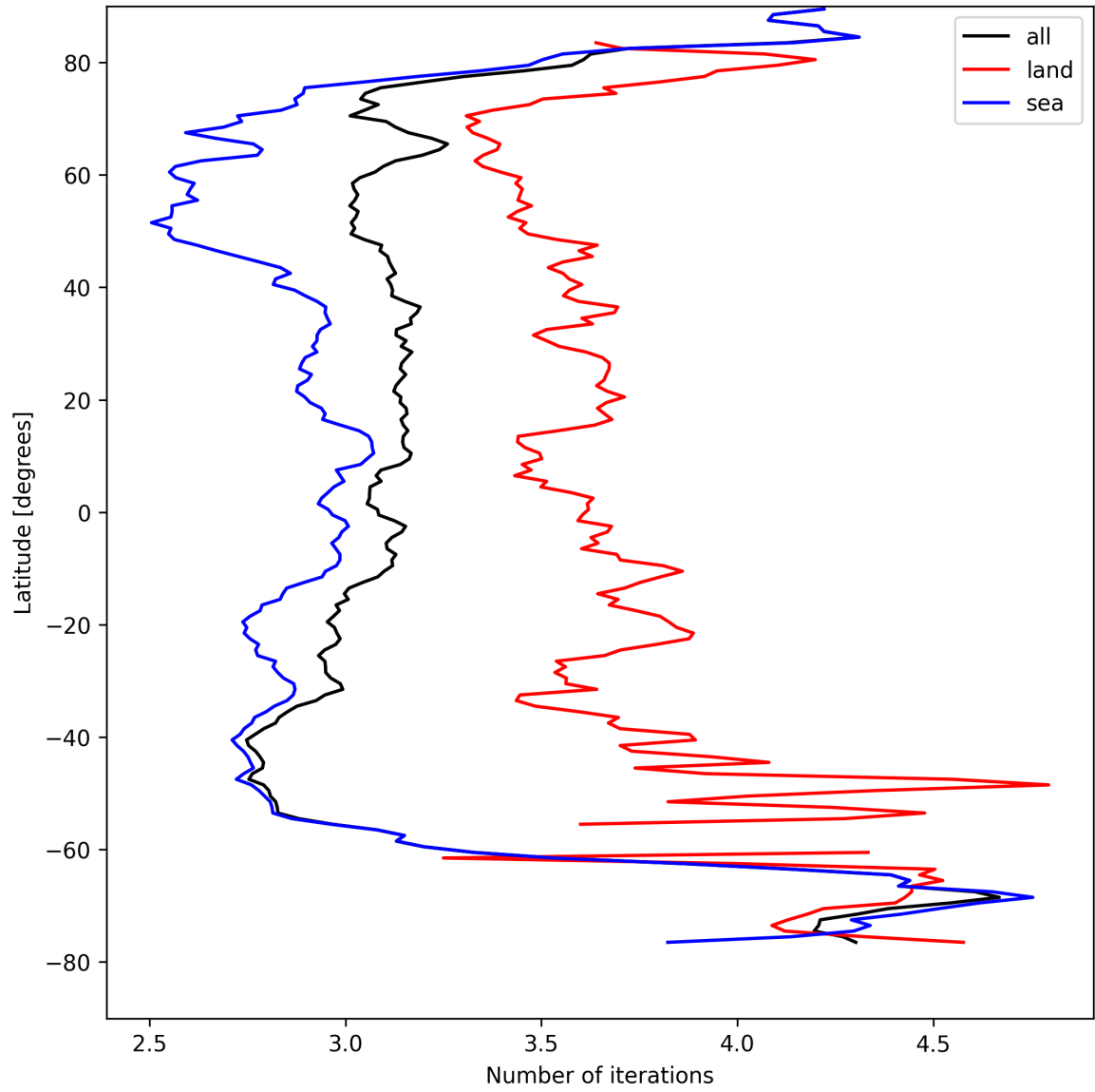
Figure 22: Zonal average of “Number of iterations” for 2025-08-21 to 2025-08-23.
