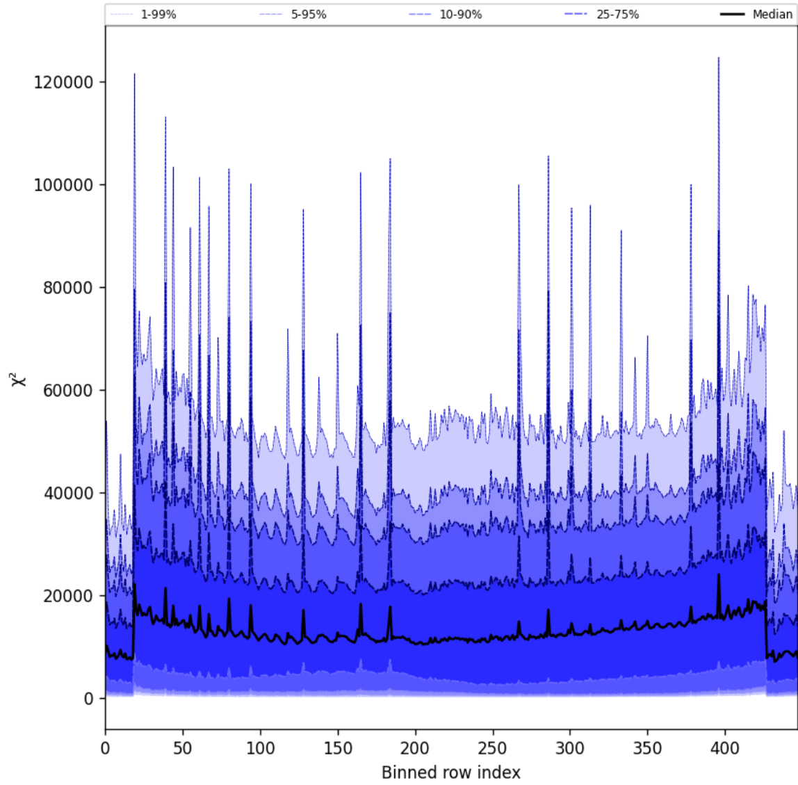
Figure 55: Along track statistics of “ \chi^2 ” for 2025-08-21 to 2025-08-23
