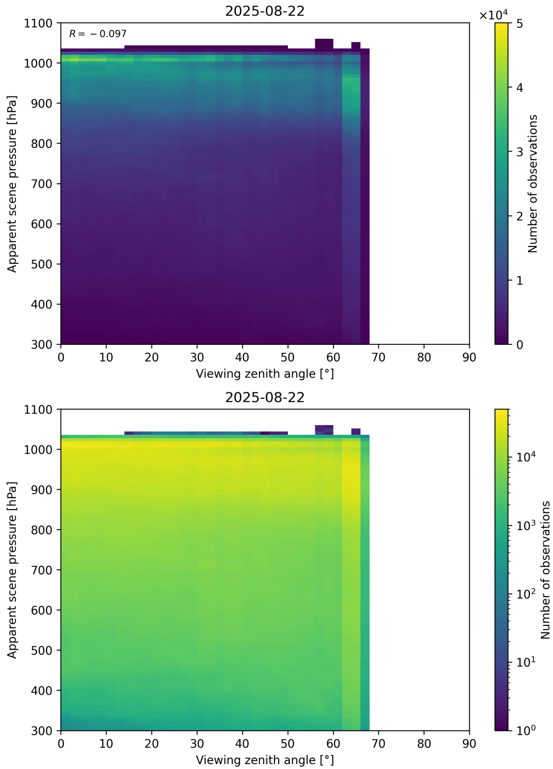
Figure 118: Scatter density plot of “Viewing zenith angle” against “Apparent scene pressure” for 2025-08-21 to 2025-08-23.
