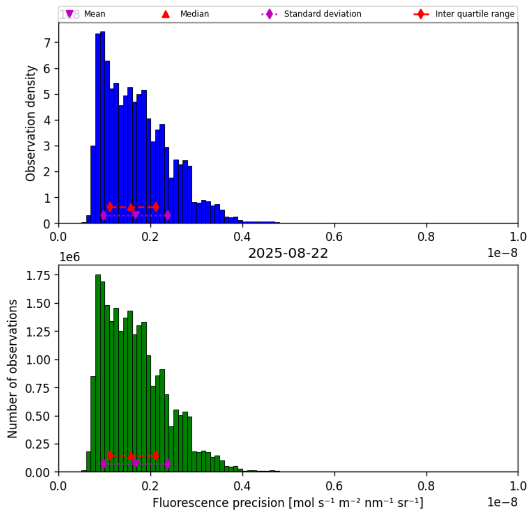
Figure 41: Histogram of “Fluorescence precision” for 2025-08-21 to 2025-08-23
