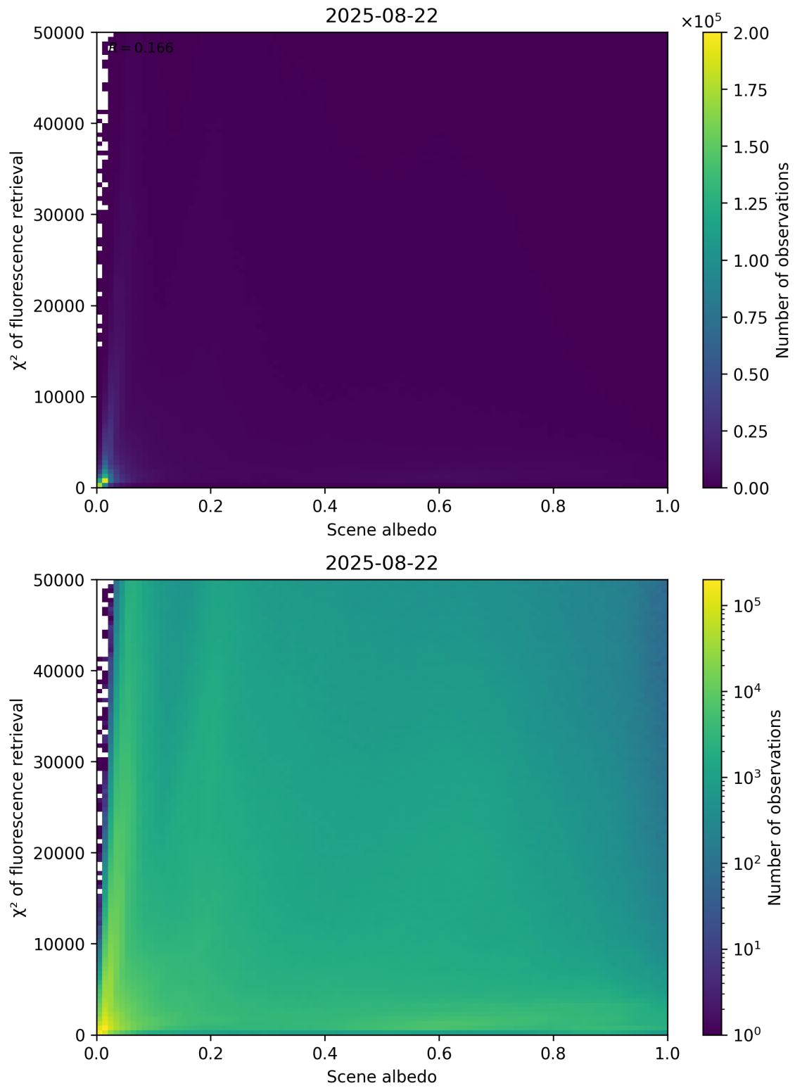
Figure 103: Scatter density plot of “Scene albedo” against “ \chi^2 of fluorescence retrieval” for 2025-08-21 to 2025-08-23.
