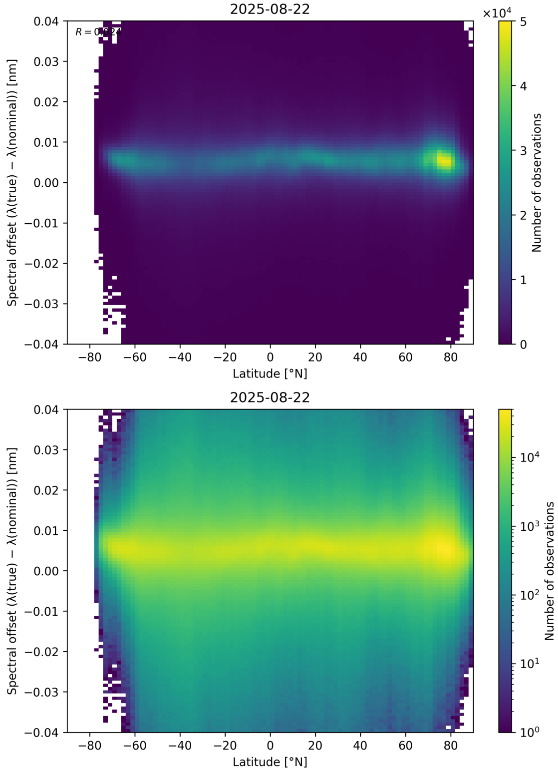
Figure 96: Scatter density plot of “Latitude” against “Spectral offset ( \lambda_{\text{true}} - \lambda_{\text{nominal}} )” for 2025-08-21 to 2025-08-23.
