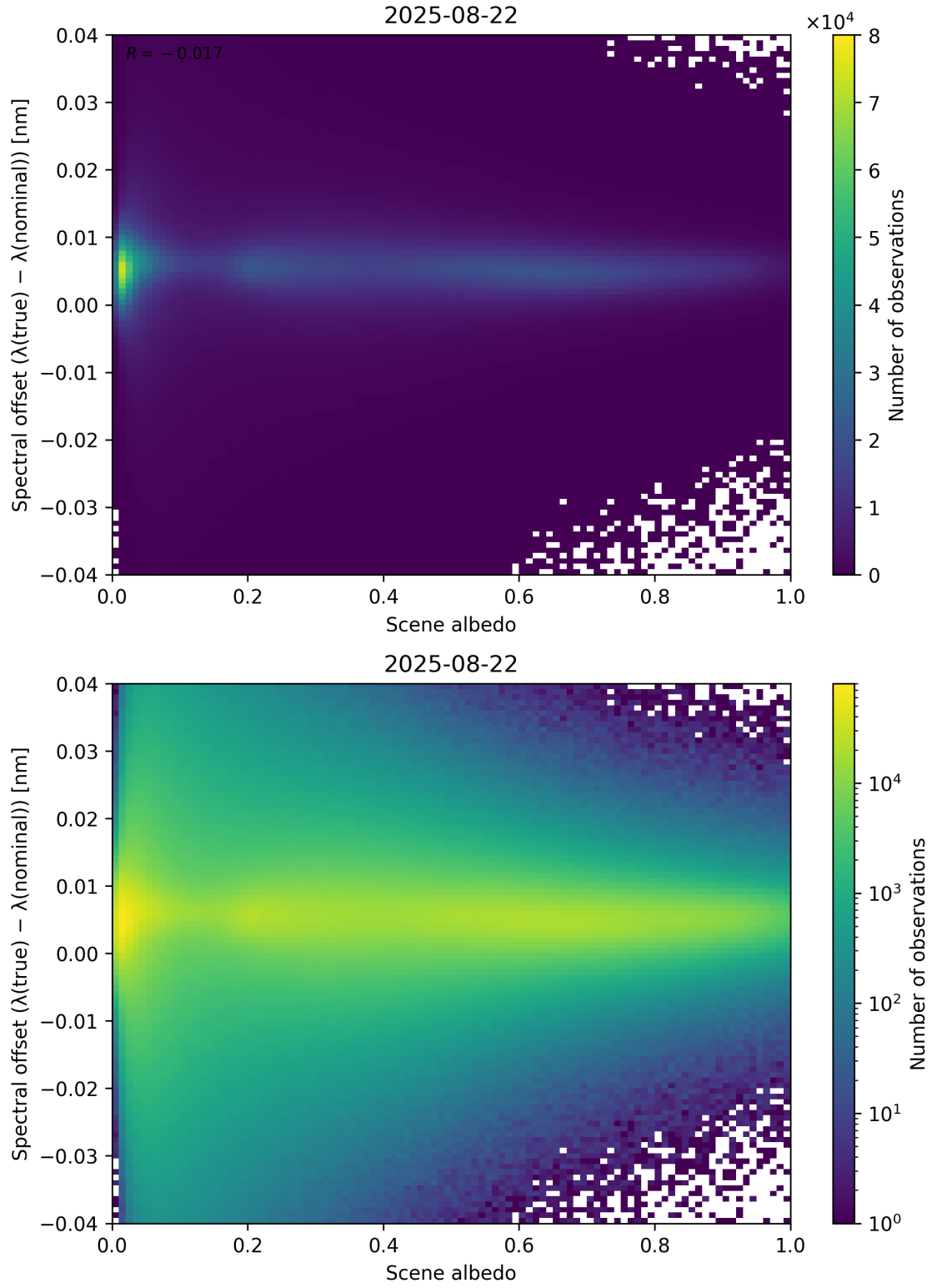
Figure 107: Scatter density plot of “Scene albedo” against “Spectral offset ( \lambda_{\text{true}} - \lambda_{\text{nominal}} )” for 2025-08-21 to 2025-08-23.
