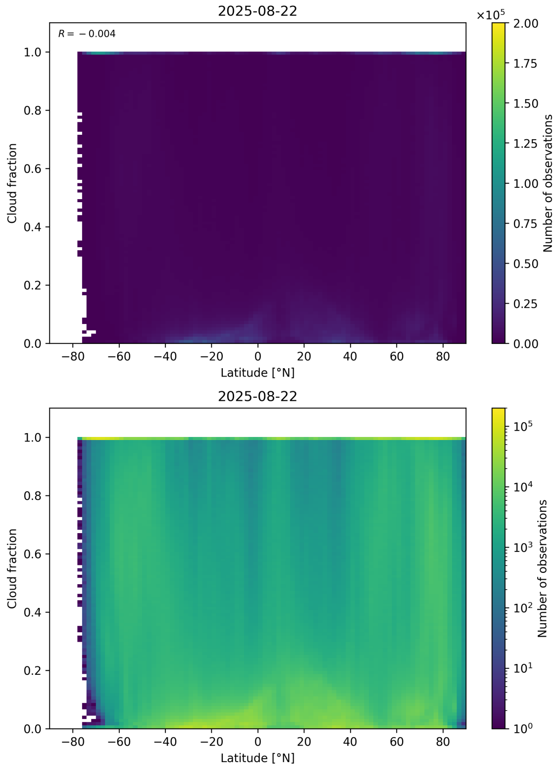
Figure 90: Scatter density plot of “Latitude” against “Cloud fraction” for 2025-08-21 to 2025-08-23.
