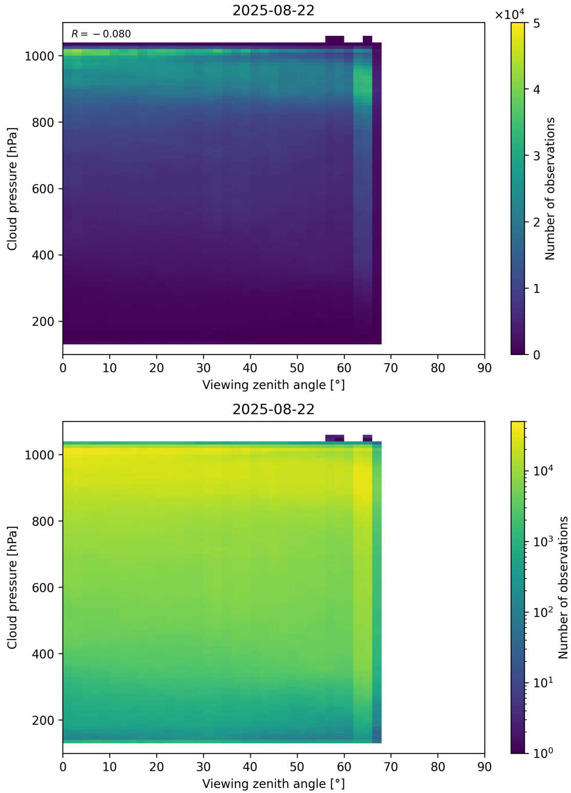
Figure 121: Scatter density plot of “Viewing zenith angle” against “Cloud pressure” for 2025-08-21 to 2025-08-23.
