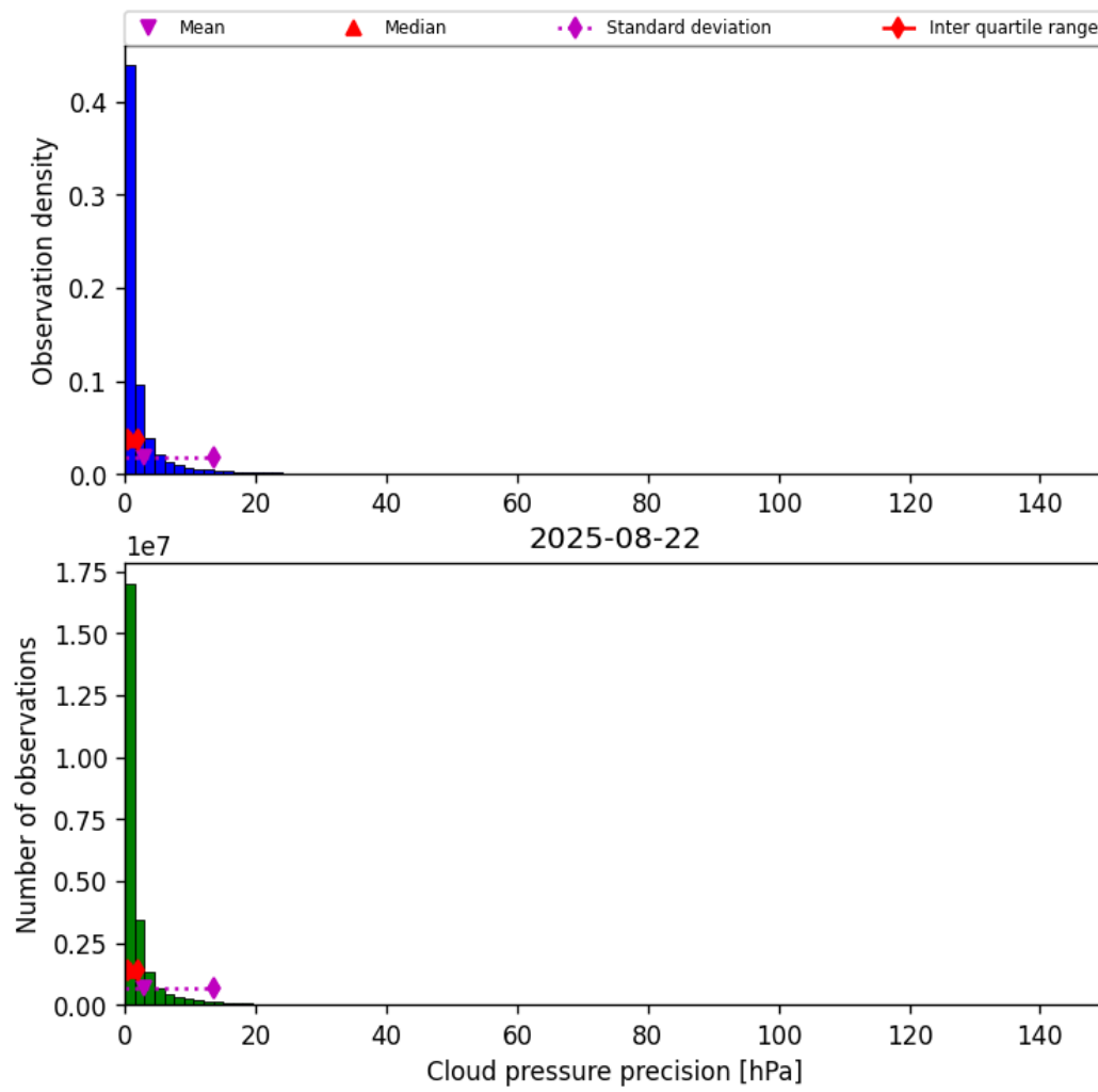
Figure 31: Histogram of “Cloud pressure precision” for 2025-08-21 to 2025-08-23
