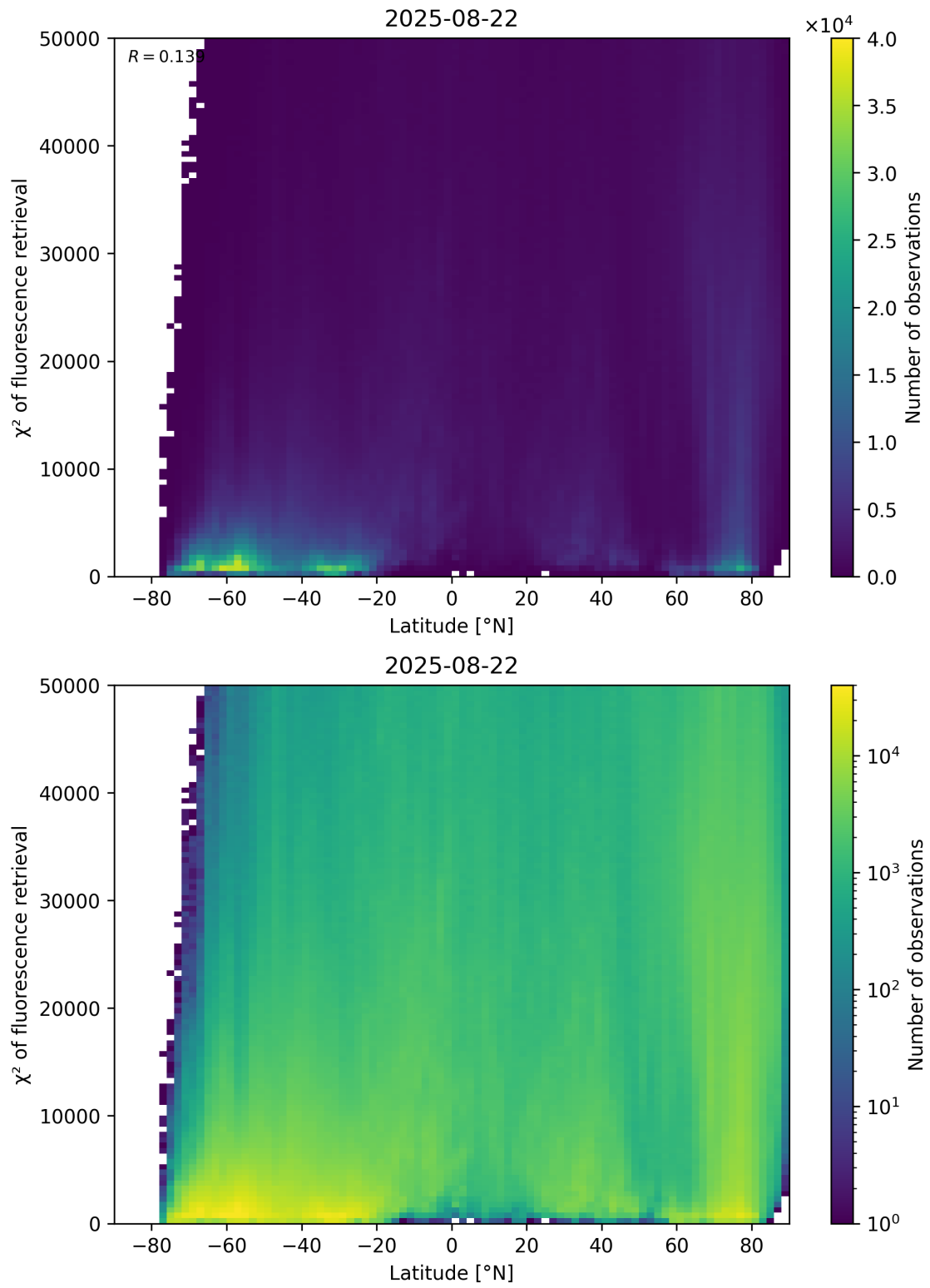
Figure 89: Scatter density plot of “Latitude” against “ \chi^2 of fluorescence retrieval” for 2025-08-21 to 2025-08-23.
