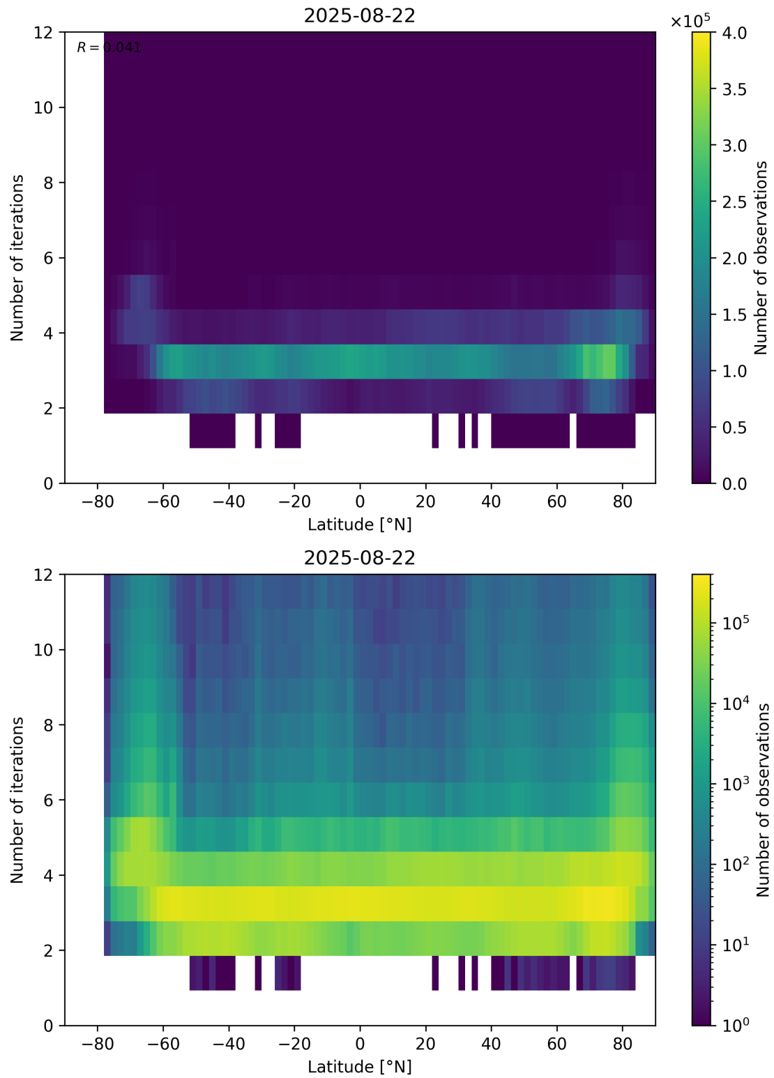
Figure 93: Scatter density plot of “Latitude” against “Number of iterations” for 2025-08-21 to 2025-08-23.
