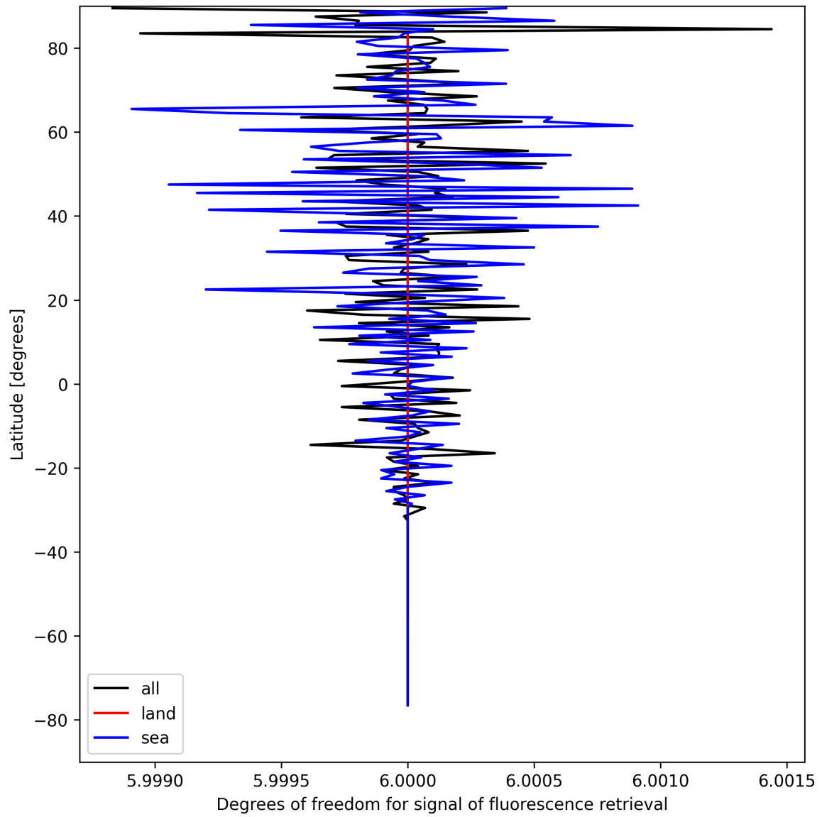
Figure 26: Zonal average of “Degrees of freedom for signal of fluorescence retrieval” for 2025-08-21 to 2025-08-23.
