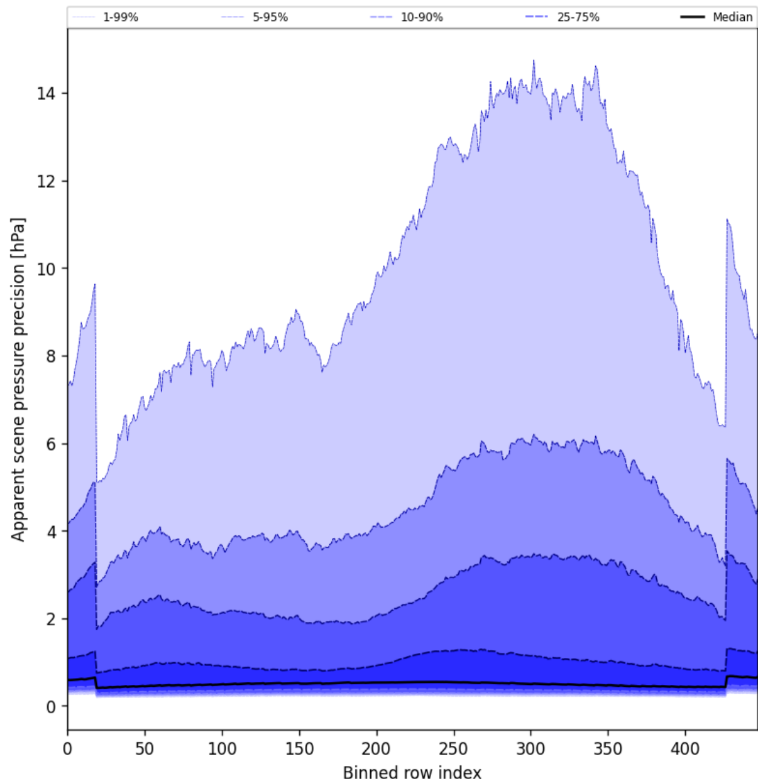
Figure 54: Along track statistics of “Apparent scene pressure precision” for 2025-08-21 to 2025-08-23
