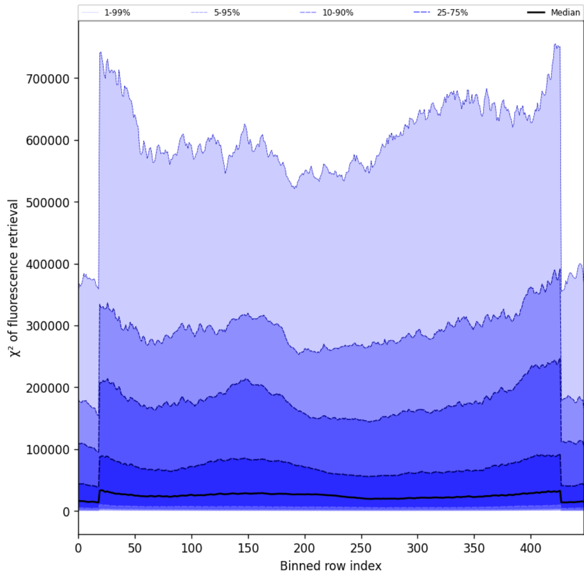
Figure 59: Along track statistics of “ \chi^2 of fluorescence retrieval” for 2025-08-21 to 2025-08-23
