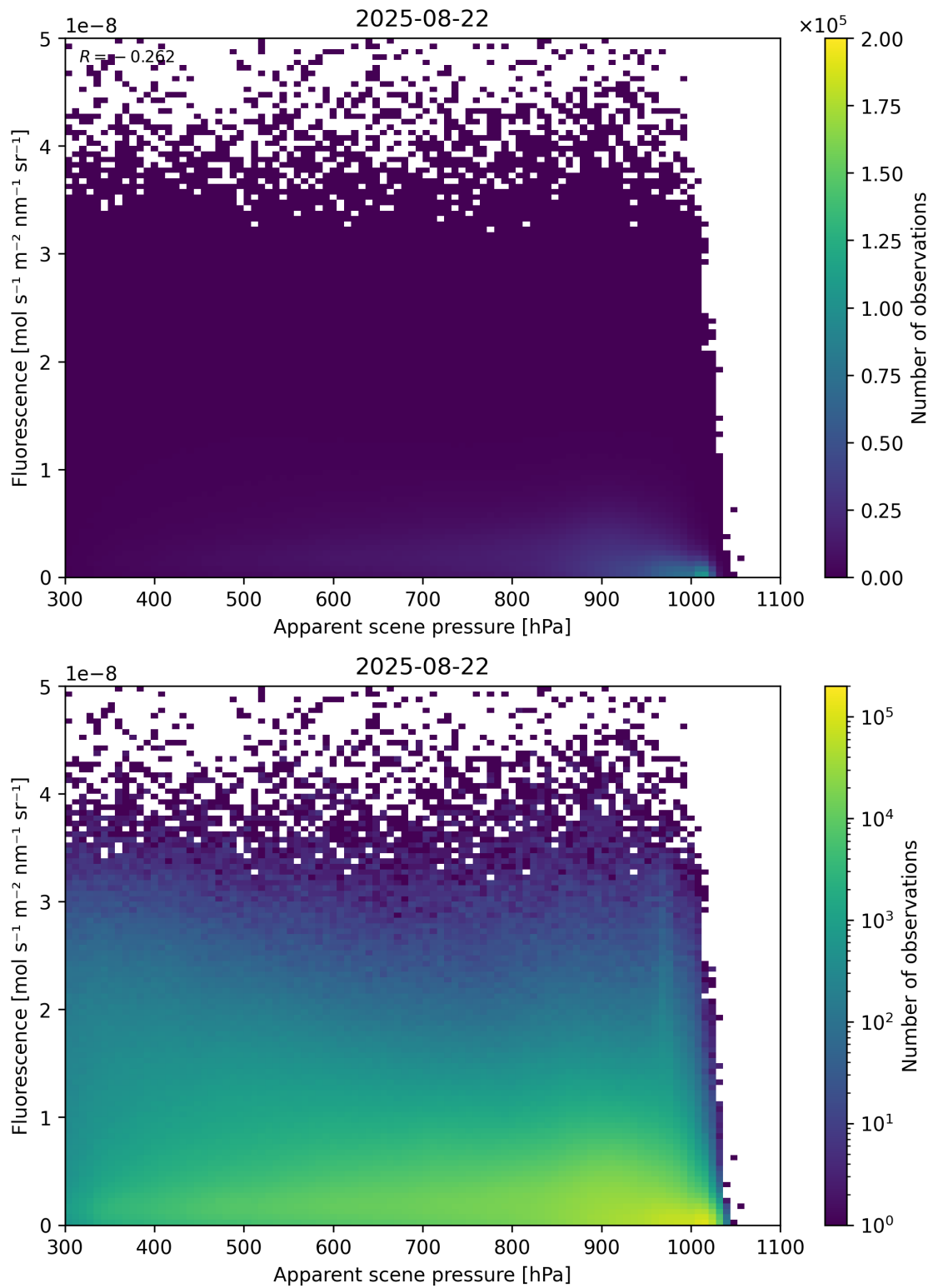
Figure 64: Scatter density plot of “Apparent scene pressure” against “Fluorescence” for 2025-08-21 to 2025-08-23.
