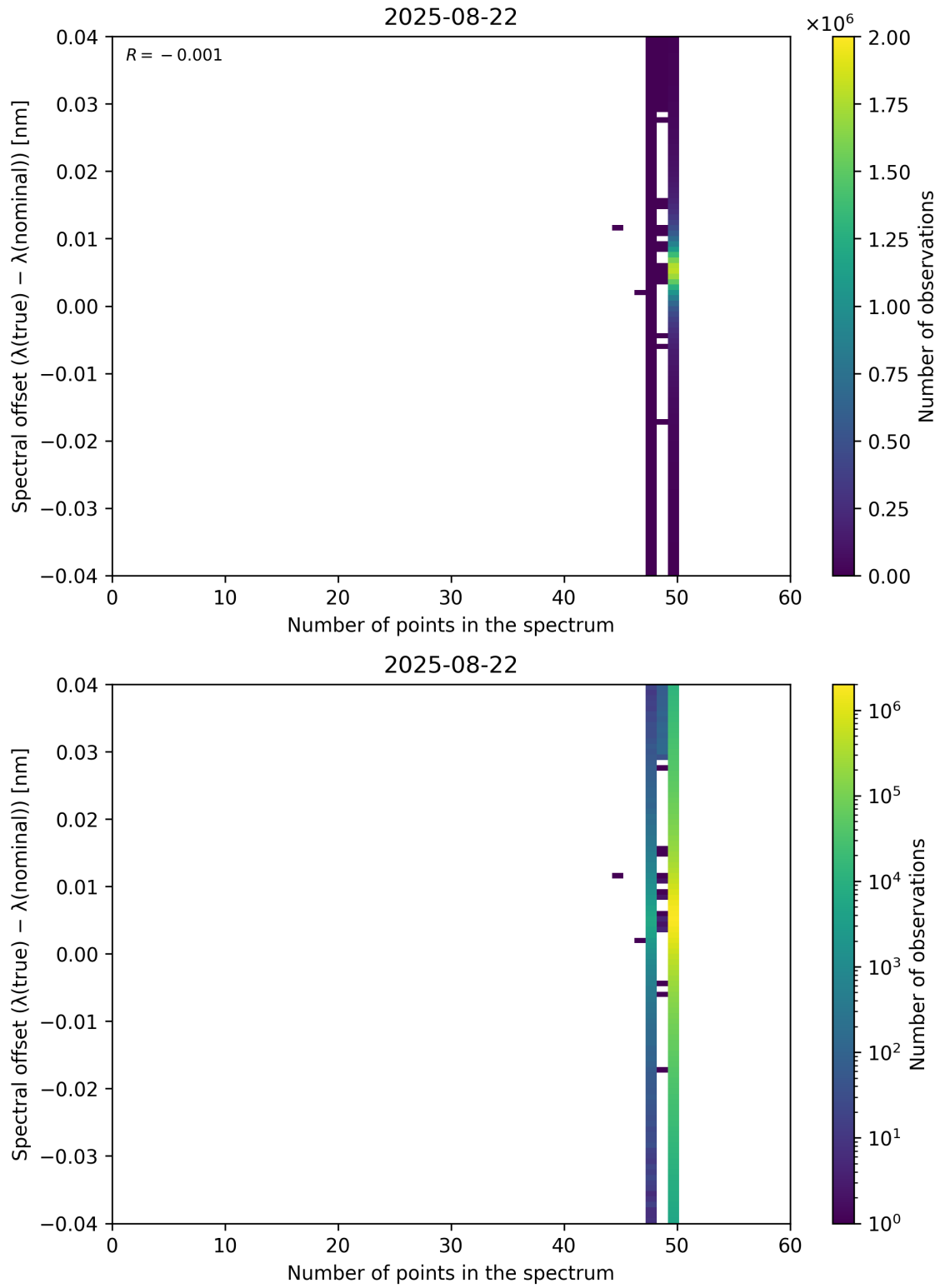
Figure 101: Scatter density plot of “Number of points in the spectrum” against “Spectral offset ( \lambda_{\text{true}} - \lambda_{\text{nominal}} )” for 2025-08-21 to 2025-08-23.
