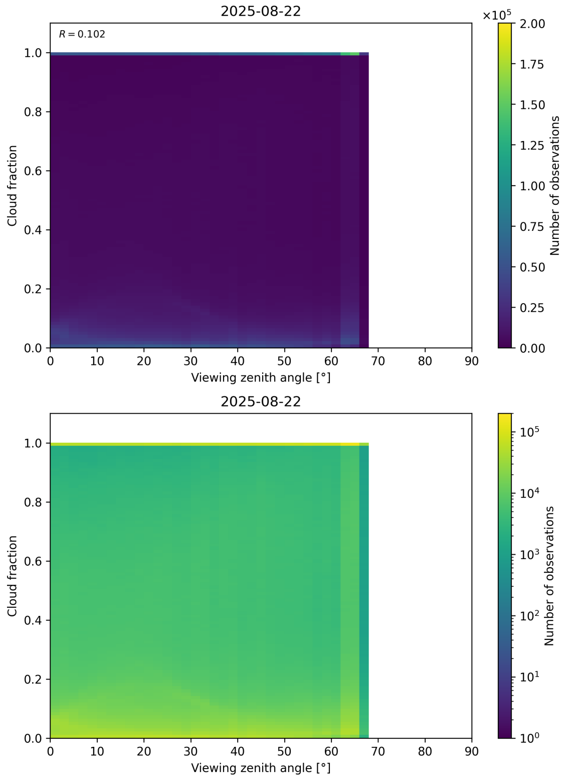
Figure 120: Scatter density plot of “Viewing zenith angle” against “Cloud fraction” for 2025-08-21 to 2025-08-23.
