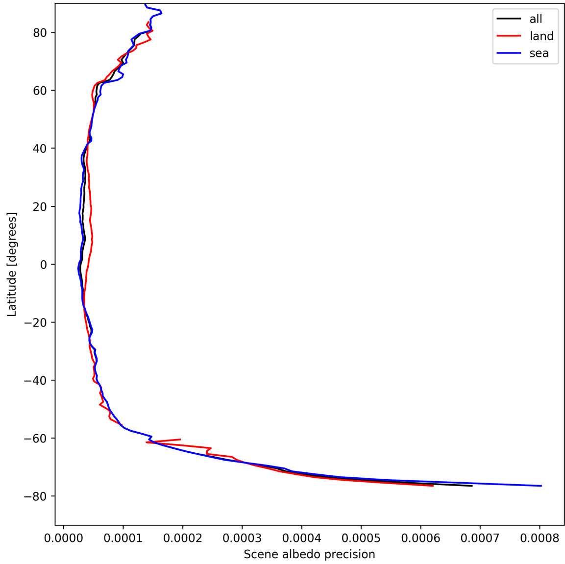
Figure 18: Zonal average of “Scene albedo precision” for 2025-08-21 to 2025-08-23.
