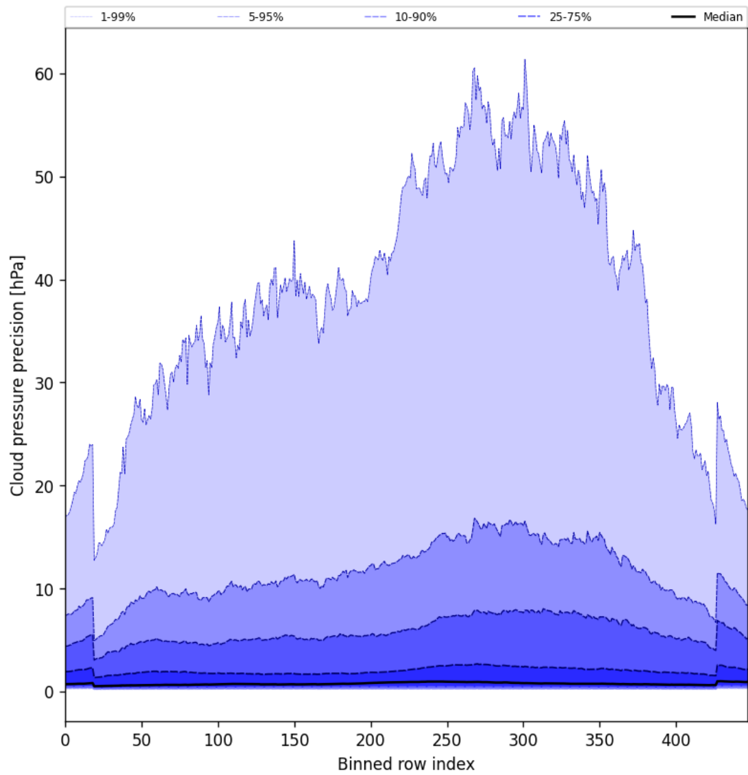
Figure 48: Along track statistics of “Cloud pressure precision” for 2025-08-21 to 2025-08-23
