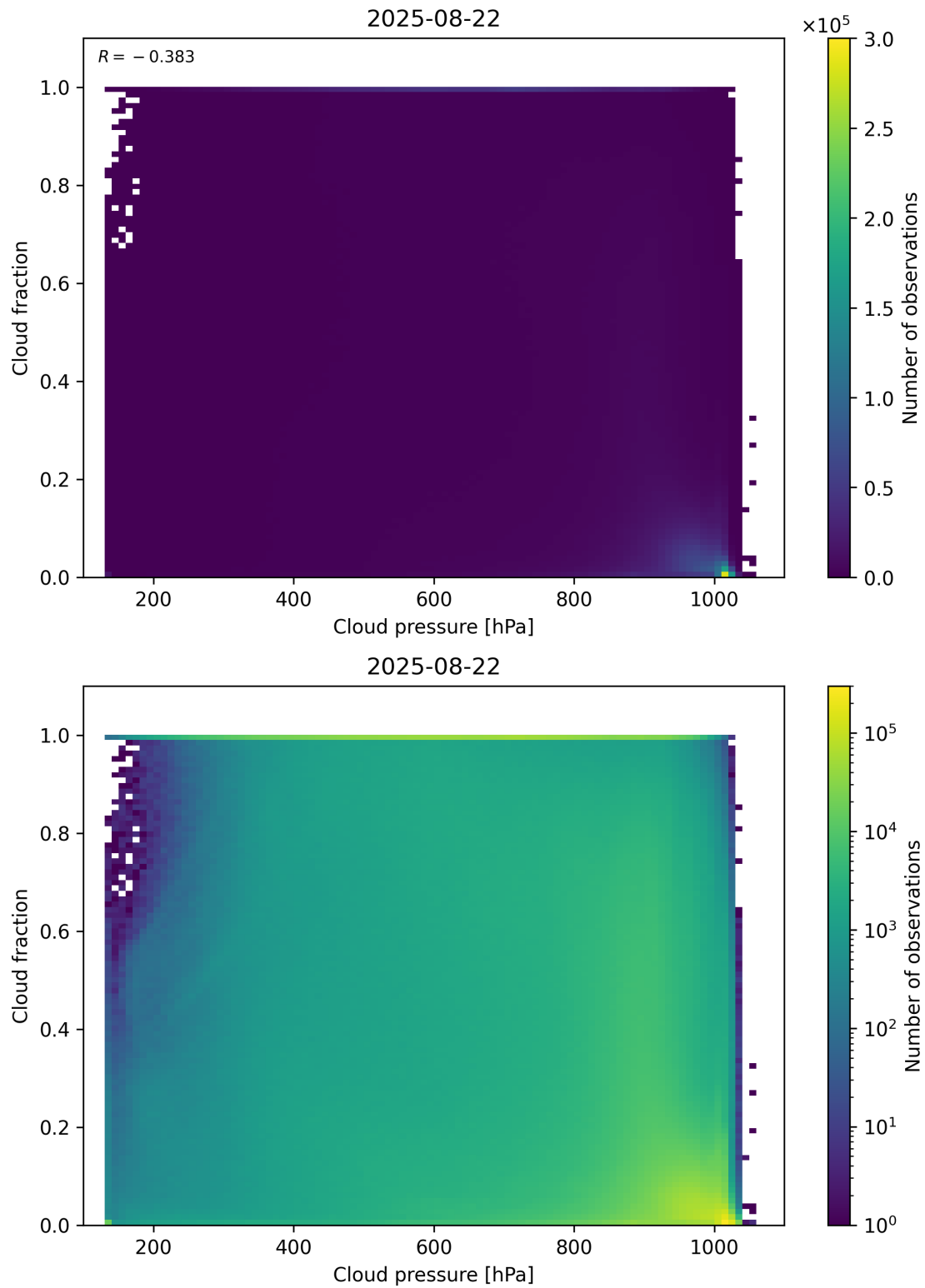
Figure 79: Scatter density plot of “Cloud pressure” against “Cloud fraction” for 2025-08-21 to 2025-08-23.
