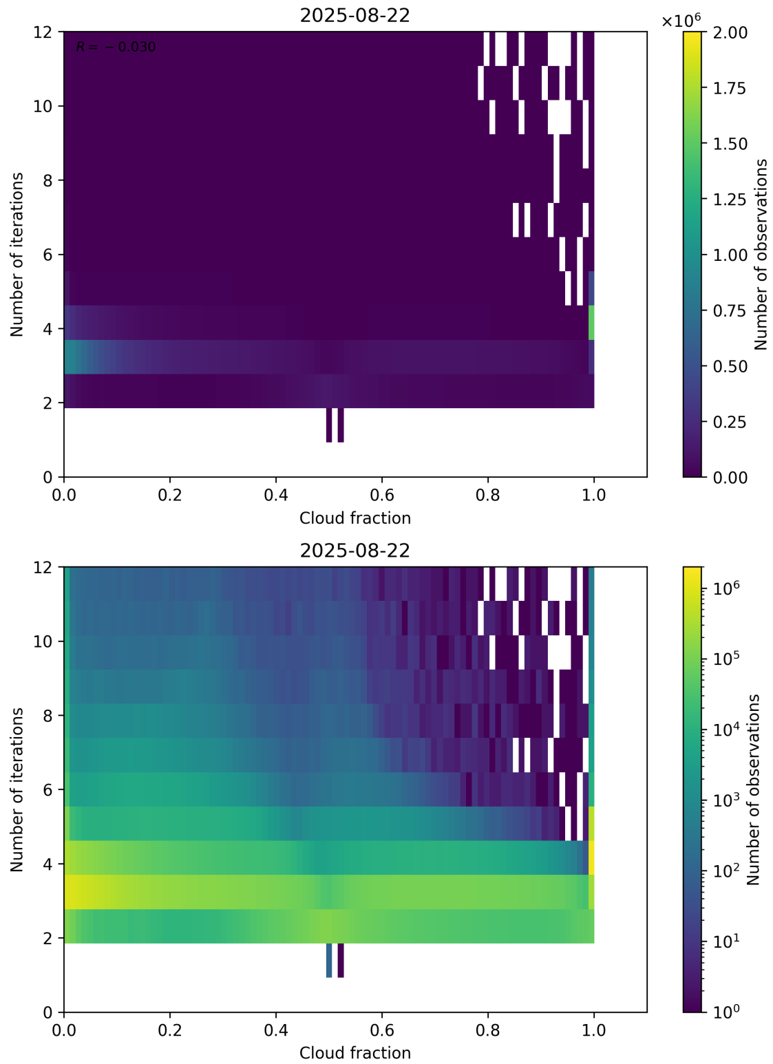
Figure 73: Scatter density plot of “Cloud fraction” against “Number of iterations” for 2025-08-21 to 2025-08-23.
