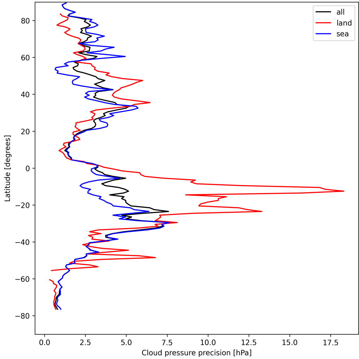
Figure 14: Zonal average of “Cloud pressure precision” for 2025-08-21 to 2025-08-23.
