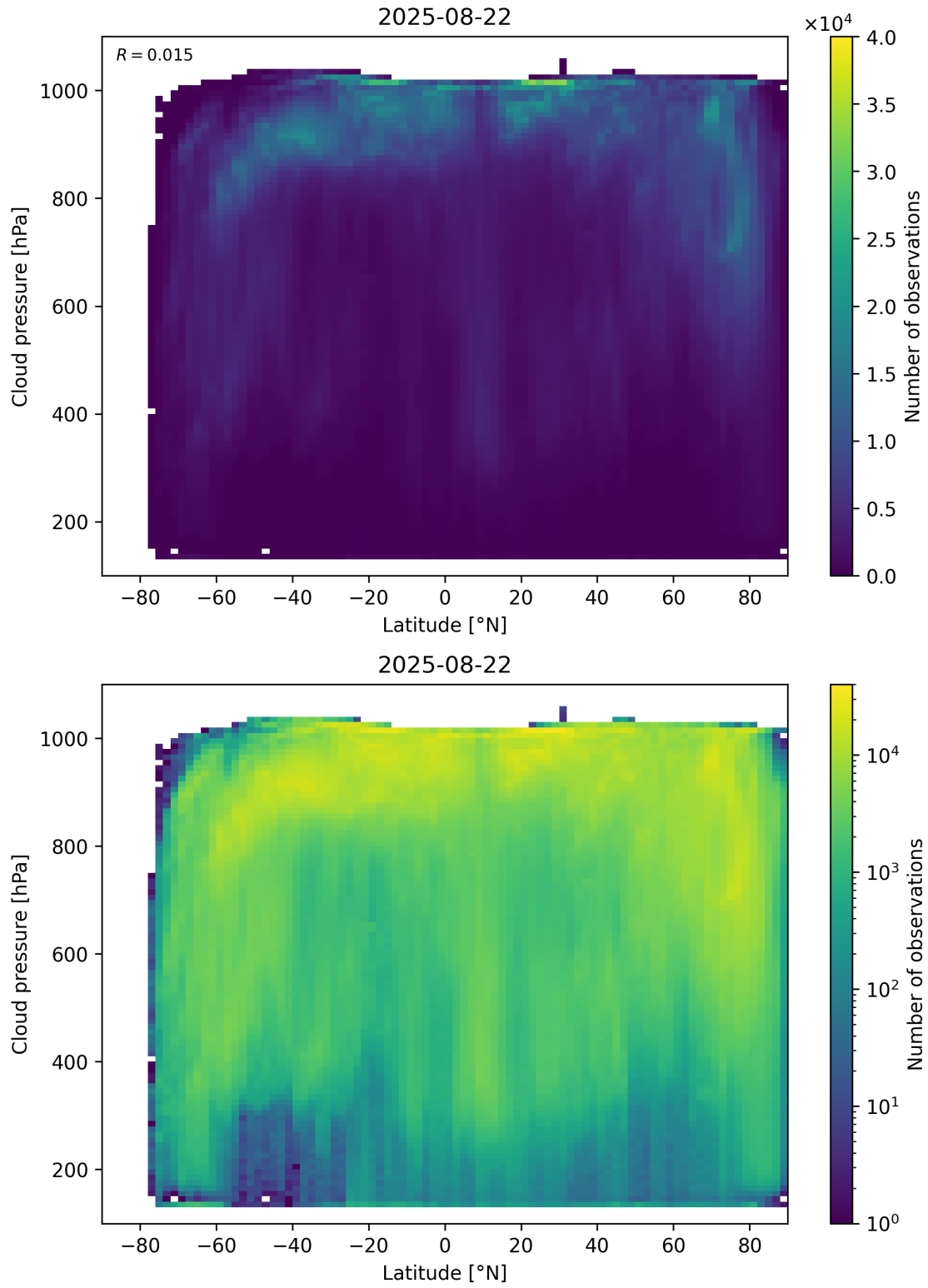
Figure 91: Scatter density plot of “Latitude” against “Cloud pressure” for 2025-08-21 to 2025-08-23.
