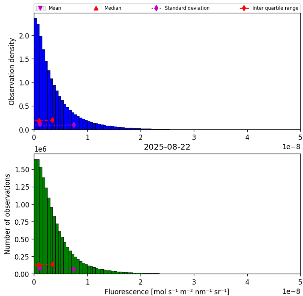
Figure 40: Histogram of “Fluorescence” for 2025-08-21 to 2025-08-23
