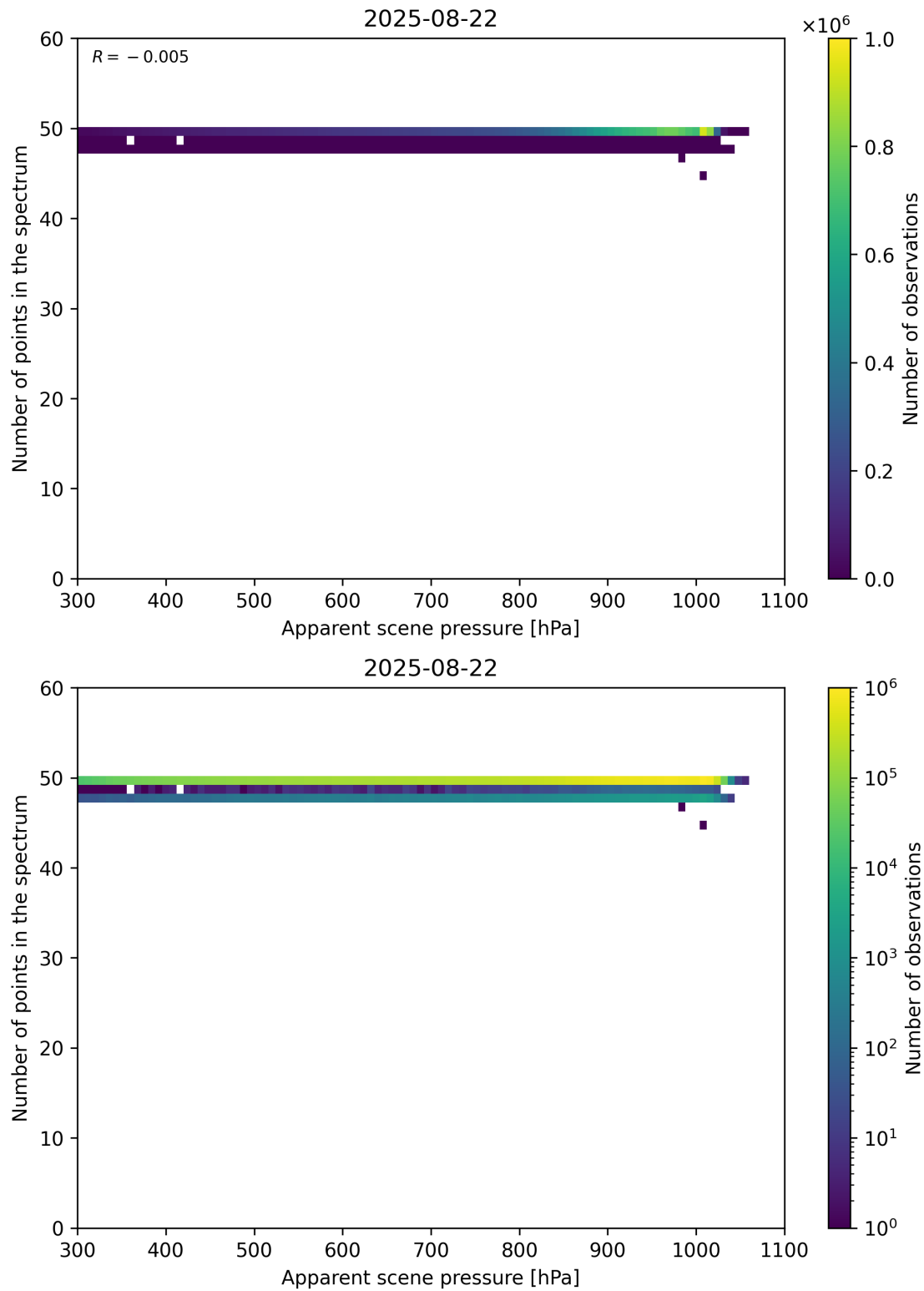
Figure 66: Scatter density plot of “Apparent scene pressure” against “Number of points in the spectrum” for 2025-08-21 to 2025-08-23.
