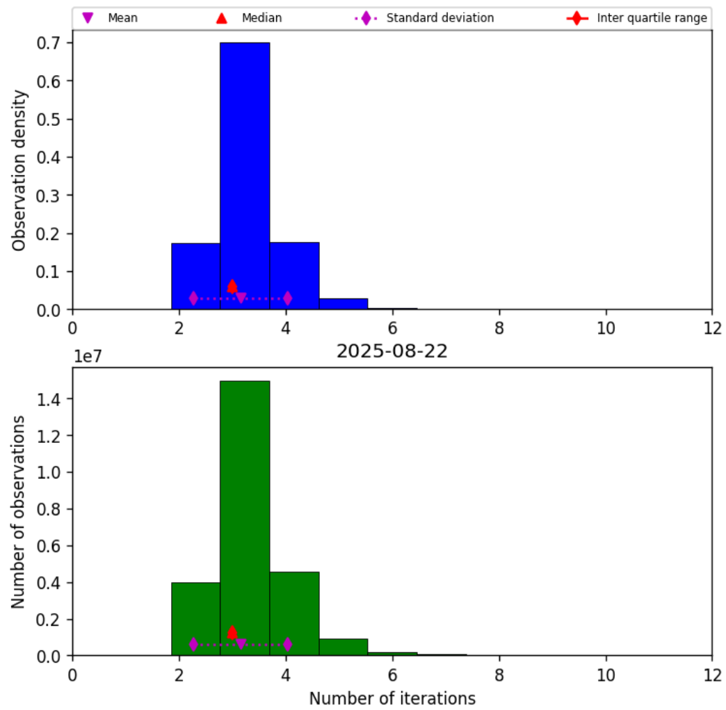
Figure 39: Histogram of “Number of iterations” for 2025-08-21 to 2025-08-23
