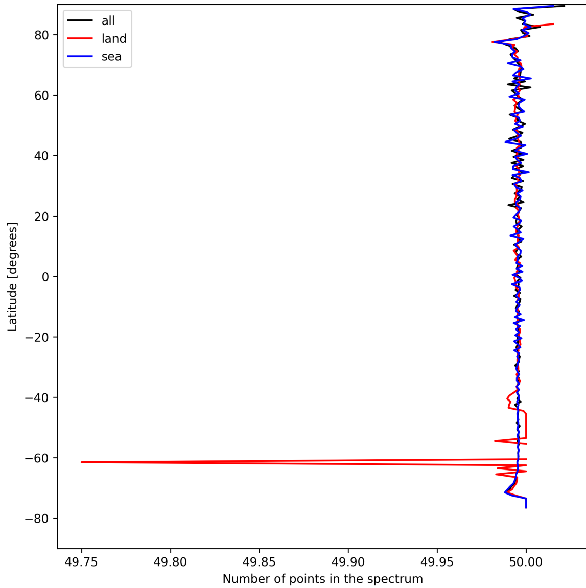
Figure 27: Zonal average of “Number of points in the spectrum” for 2025-08-21 to 2025-08-23.
