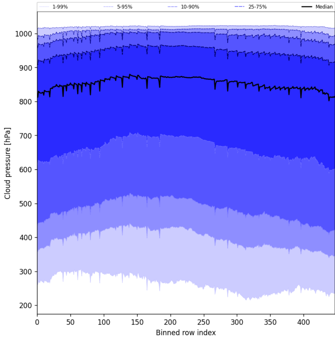
Figure 47: Along track statistics of “Cloud pressure” for 2025-08-21 to 2025-08-23
