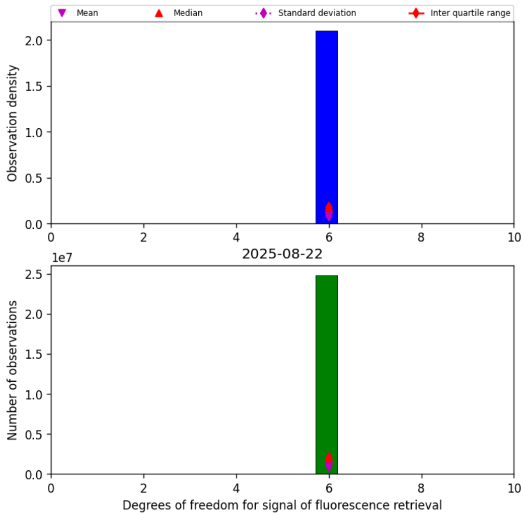
Figure 43: Histogram of "Degrees of freedom for signal of fluorescence retrieval" for 2025-08-21 to 2025-08-23
