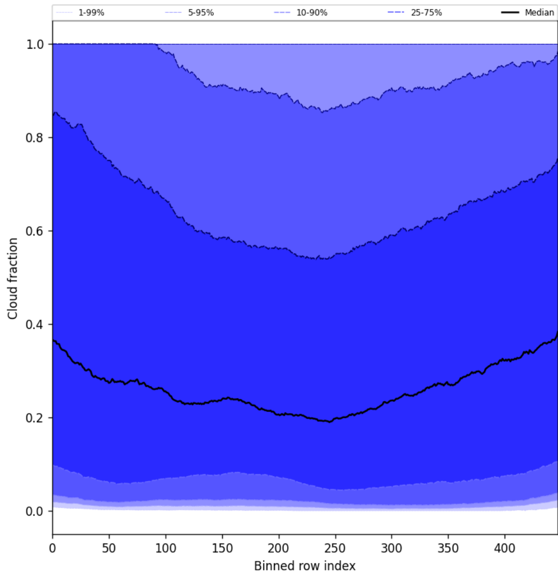
Figure 49: Along track statistics of “Cloud fraction” for 2025-08-21 to 2025-08-23
