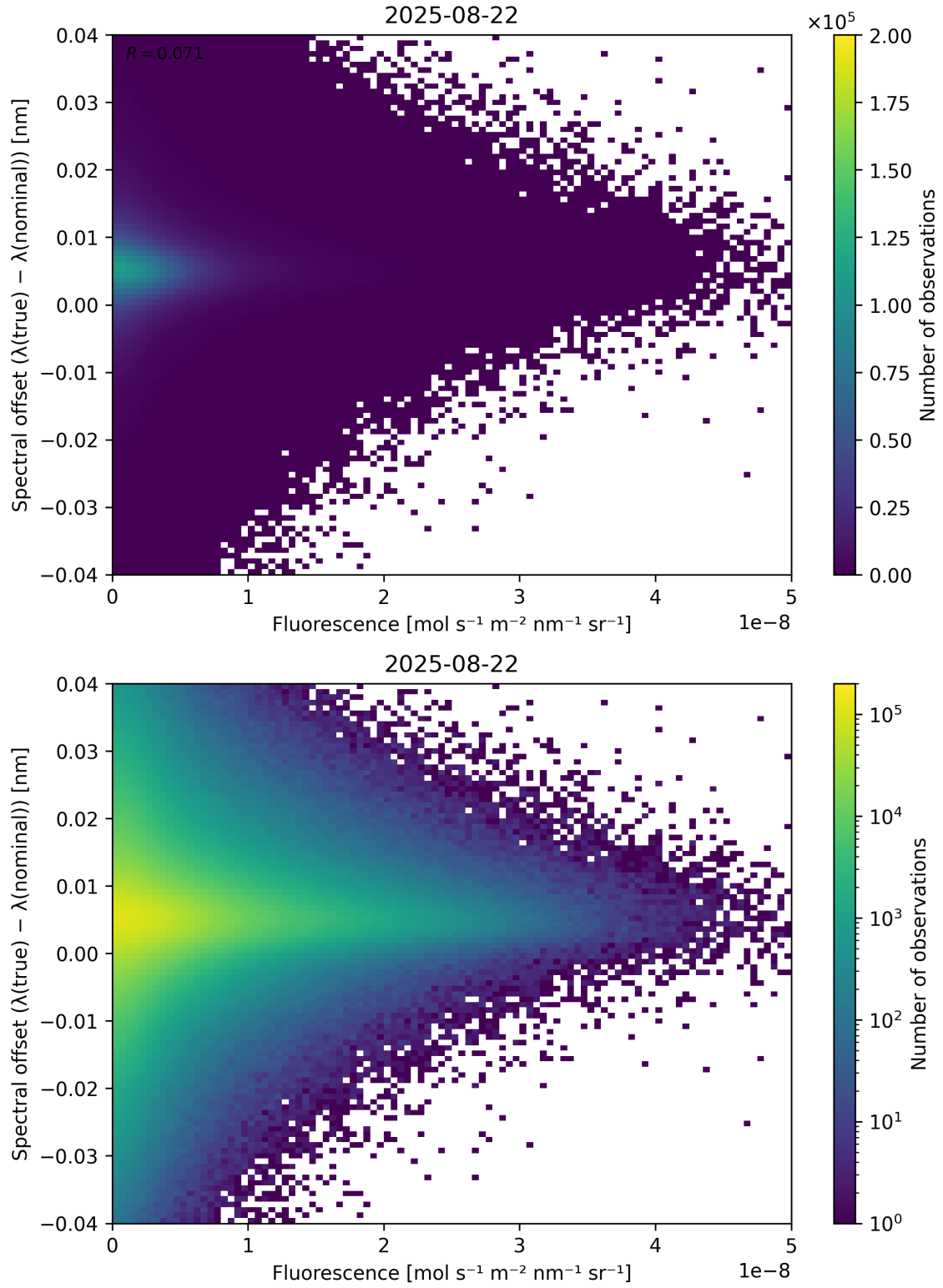
Figure 87: Scatter density plot of “Fluorescence” against “Spectral offset ( \lambda_{\text{true}} - \lambda_{\text{nominal}} )” for 2025-08-21 to 2025-08-23.
