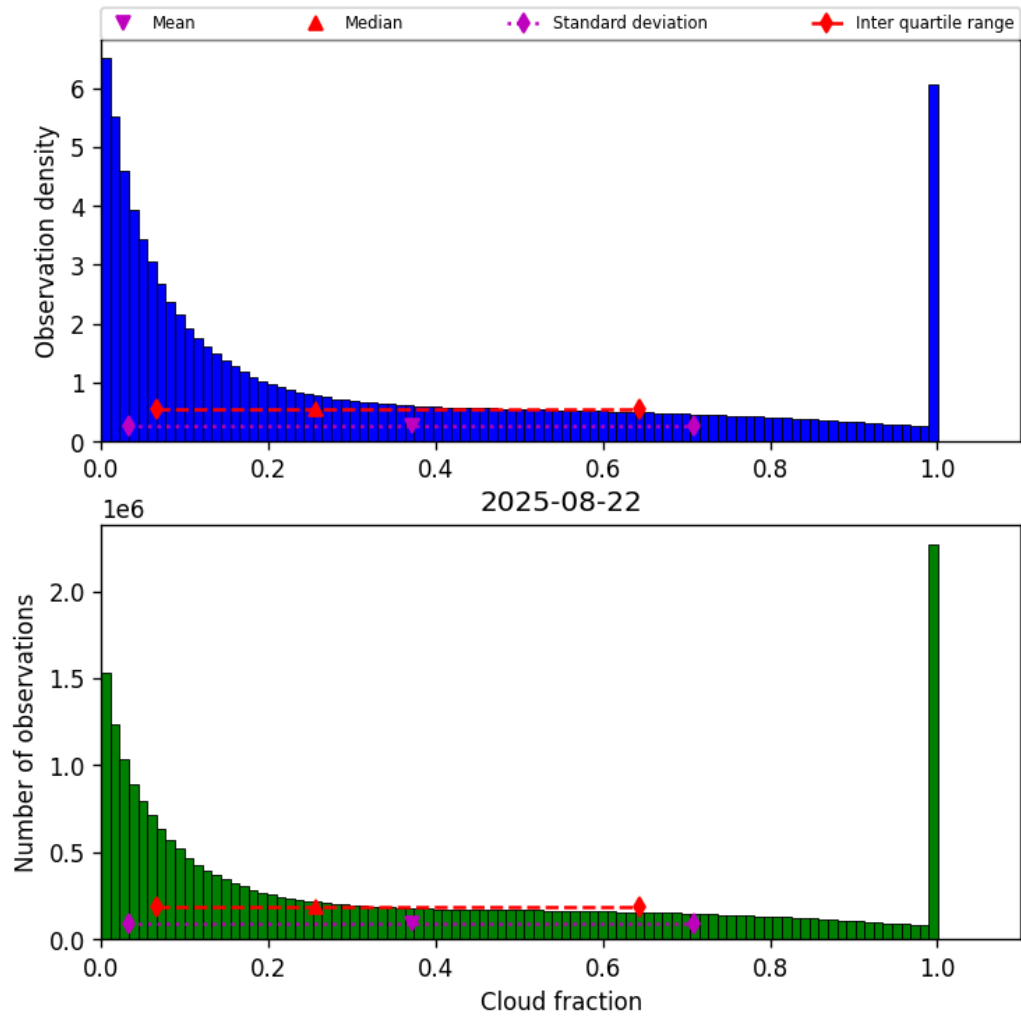
Figure 32: Histogram of “Cloud fraction” for 2025-08-21 to 2025-08-23
