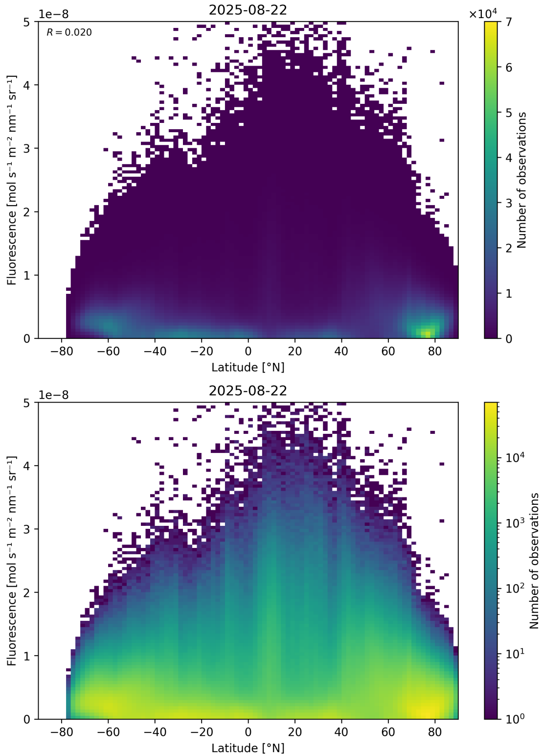
Figure 92: Scatter density plot of “Latitude” against “Fluorescence” for 2025-08-21 to 2025-08-23.
