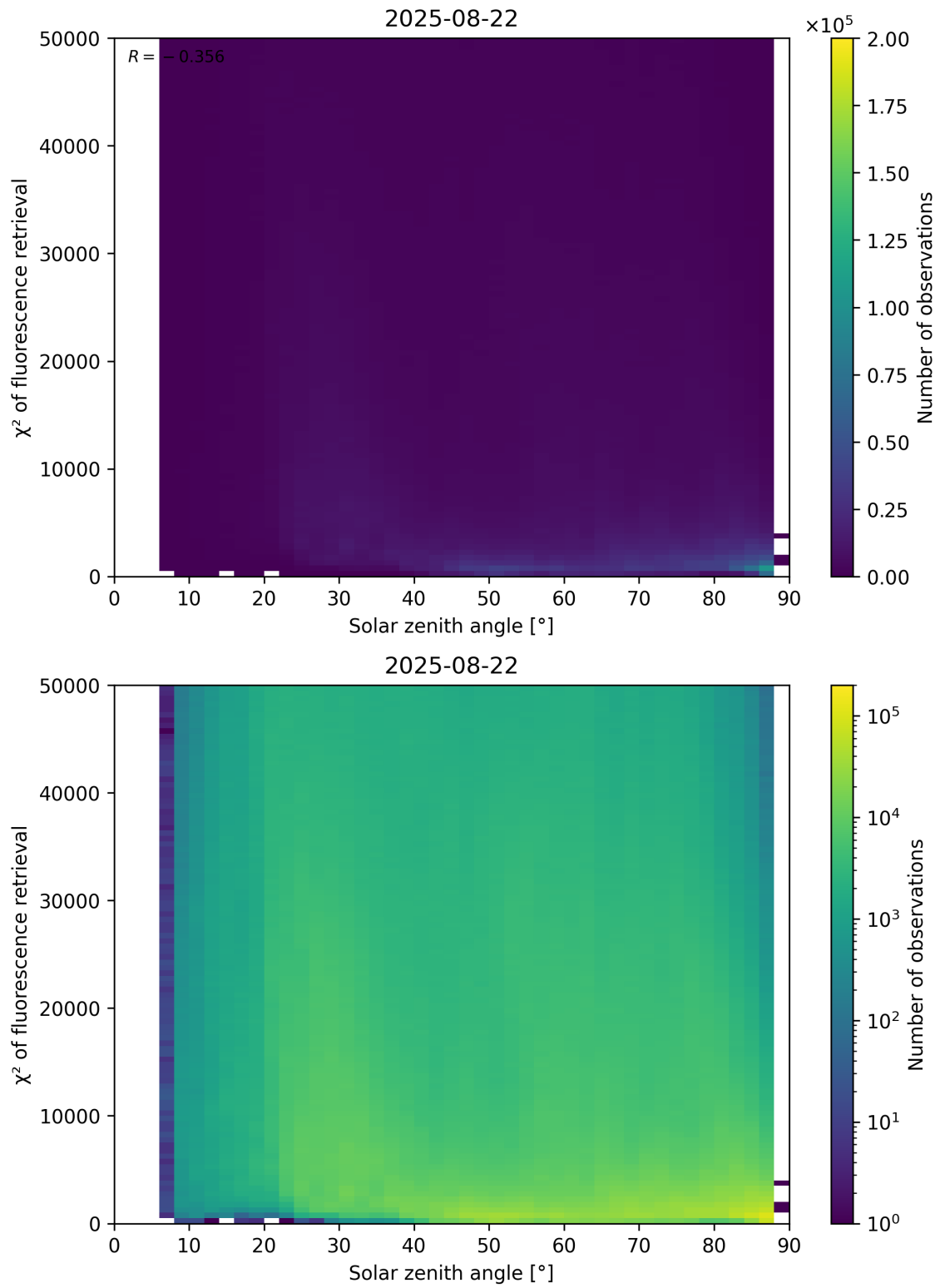
Figure 109: Scatter density plot of “Solar zenith angle” against “ \chi^2 of fluorescence retrieval” for 2025-08-21 to 2025-08-23.
