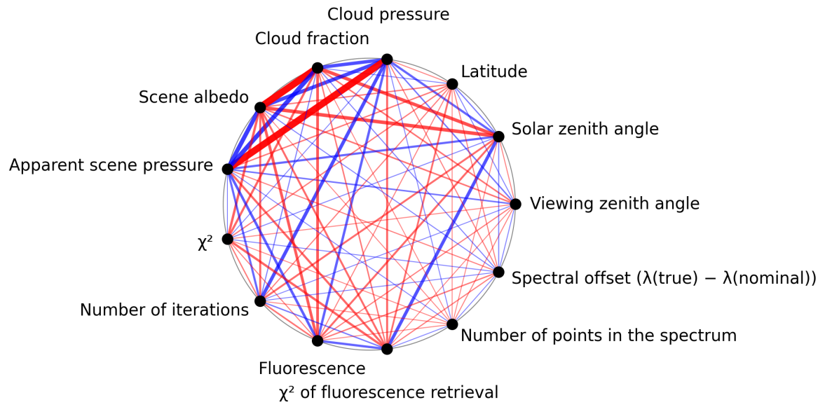
Figure 1: Map of correlation graph for 2025-08-21 to 2025-08-23.
