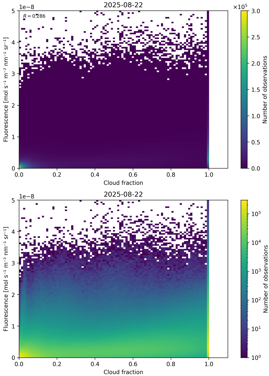
Figure 72: Scatter density plot of “Cloud fraction” against “Fluorescence” for 2025-08-21 to 2025-08-23.
