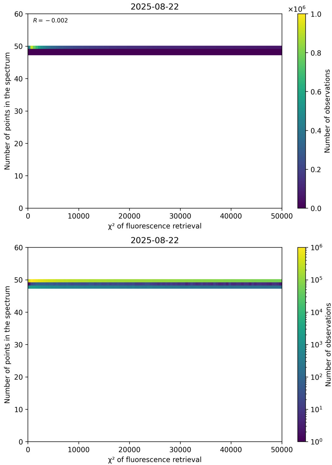
Figure 68: Scatter density plot of " \chi^2 of fluorescence retrieval" against "Number of points in the spectrum" for 2025-08-21 to 2025-08-23.
