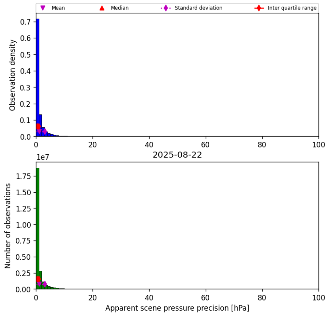
Figure 37: Histogram of “Apparent scene pressure precision” for 2025-08-21 to 2025-08-23
