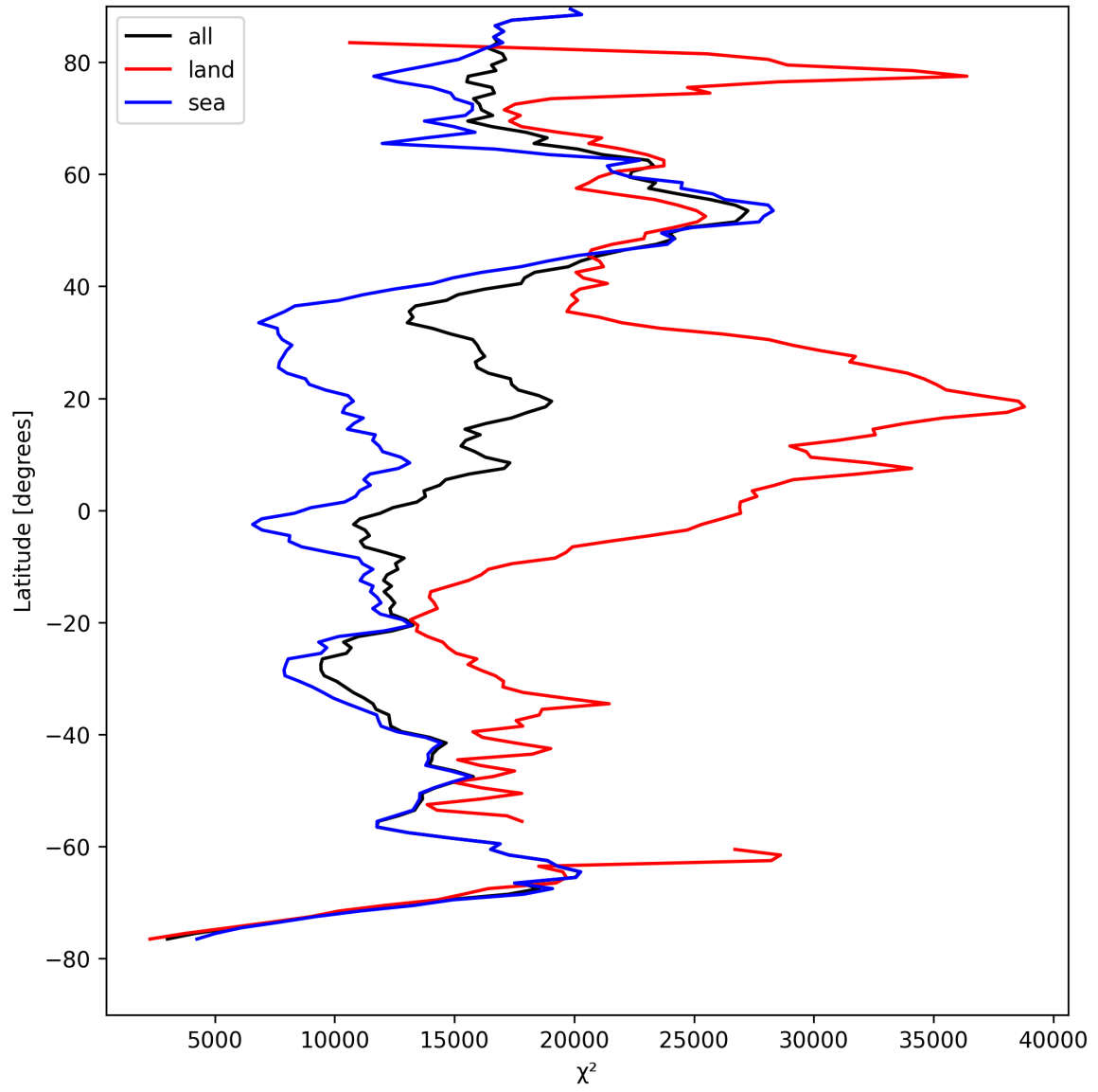
Figure 21: Zonal average of “ \chi^2 ” for 2025-08-21 to 2025-08-23.
