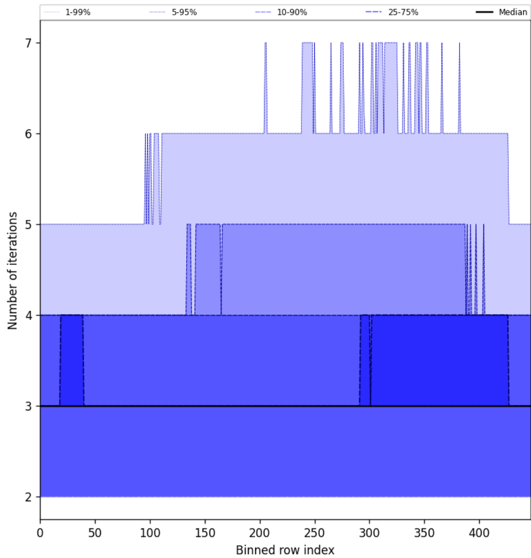
Figure 56: Along track statistics of “Number of iterations” for 2025-08-21 to 2025-08-23
