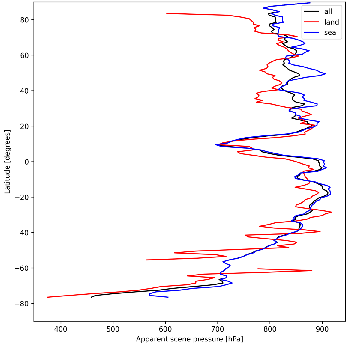
Figure 19: Zonal average of “Apparent scene pressure” for 2025-08-21 to 2025-08-23.
