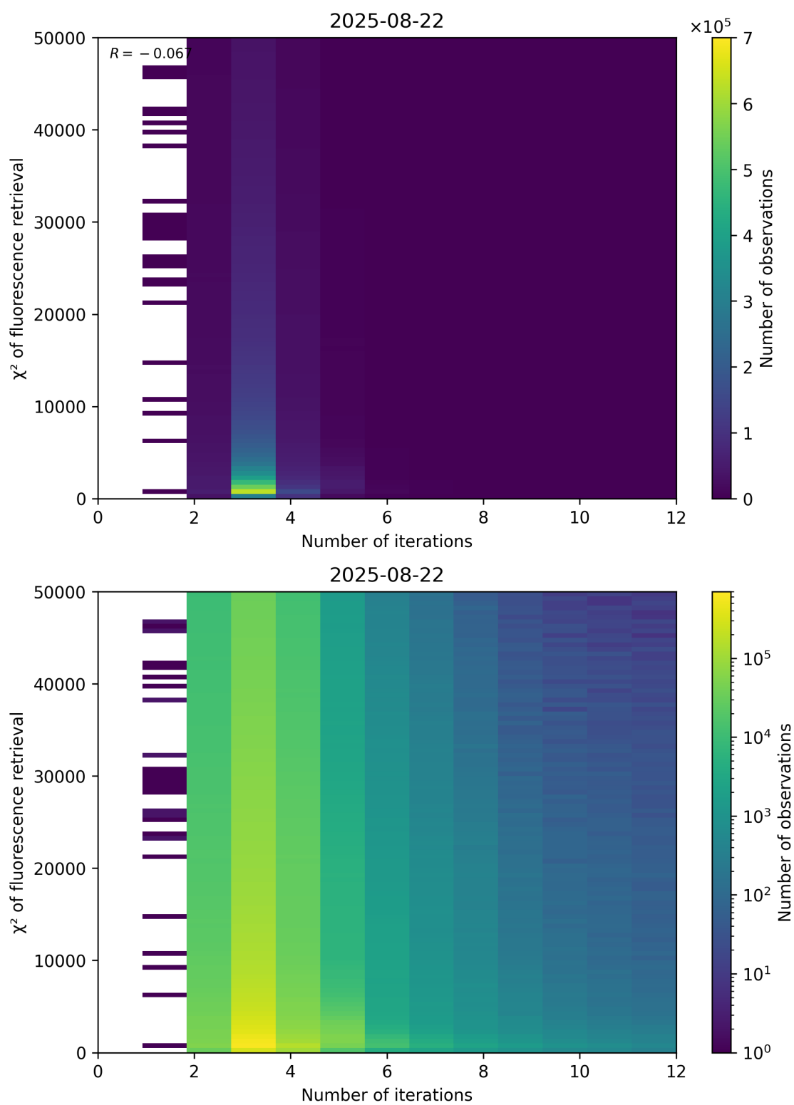
Figure 97: Scatter density plot of “Number of iterations” against “ \chi^2 of fluorescence retrieval” for 2025-08-21 to 2025-08-23.
