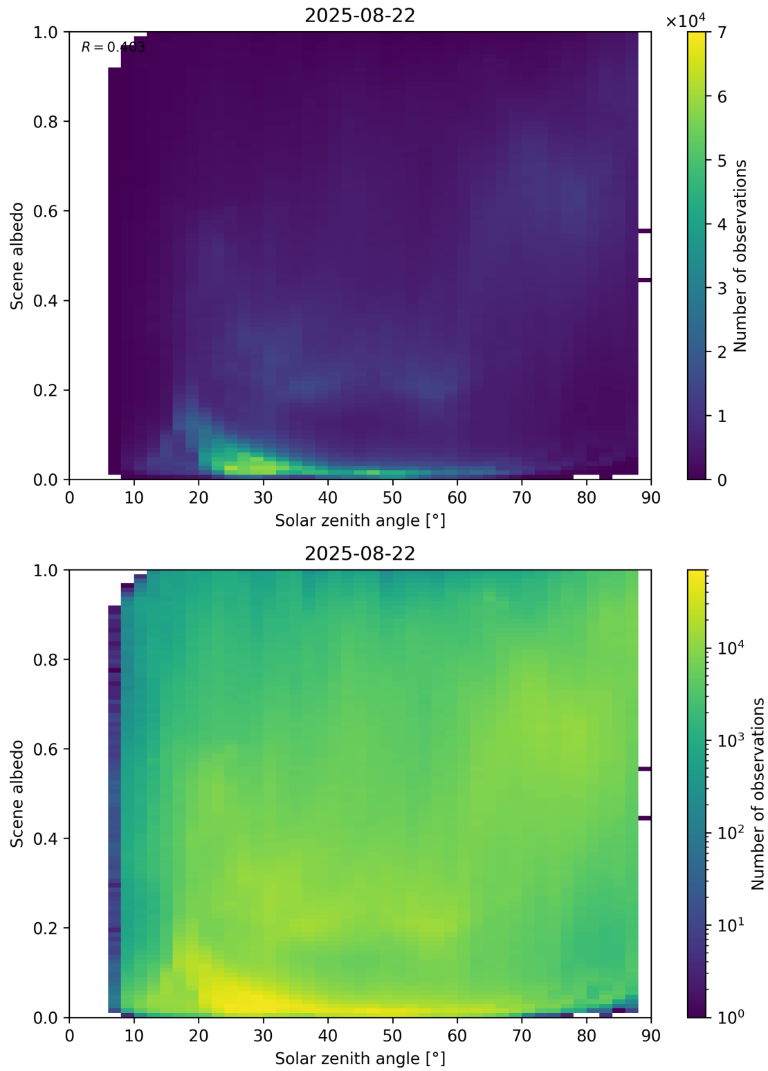
Figure 116: Scatter density plot of “Solar zenith angle” against “Scene albedo” for 2025-08-21 to 2025-08-23.
