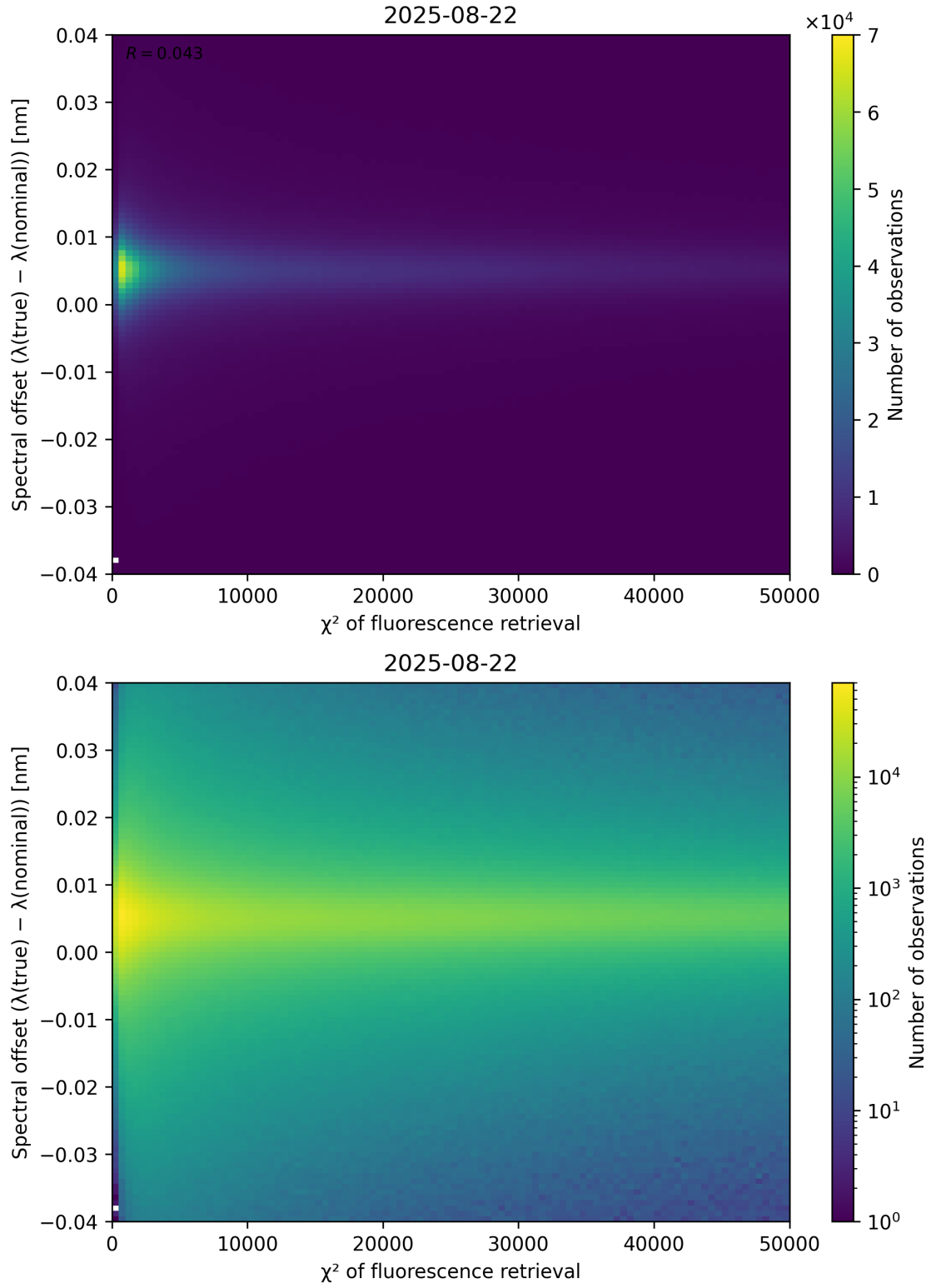
Figure 69: Scatter density plot of “ \chi^2 of fluorescence retrieval” against “Spectral offset ( \lambda_{\text{true}} - \lambda_{\text{nominal}} )” for 2025-08-21 to 2025-08-23.
