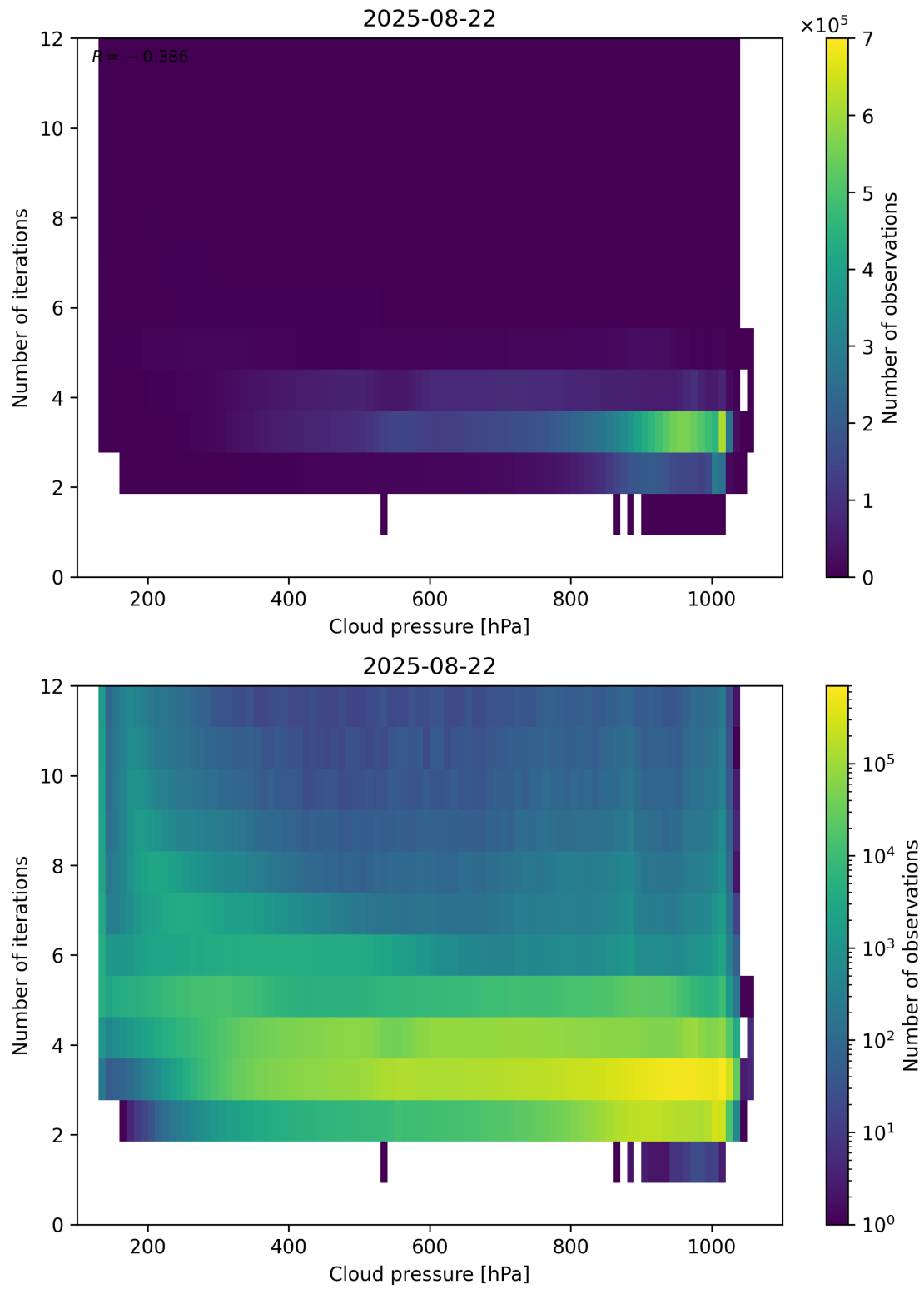
Figure 81: Scatter density plot of “Cloud pressure” against “Number of iterations” for 2025-08-21 to 2025-08-23.
