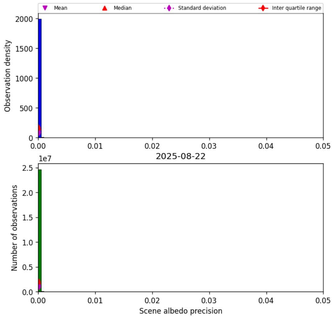
Figure 35: Histogram of “Scene albedo precision” for 2025-08-21 to 2025-08-23
