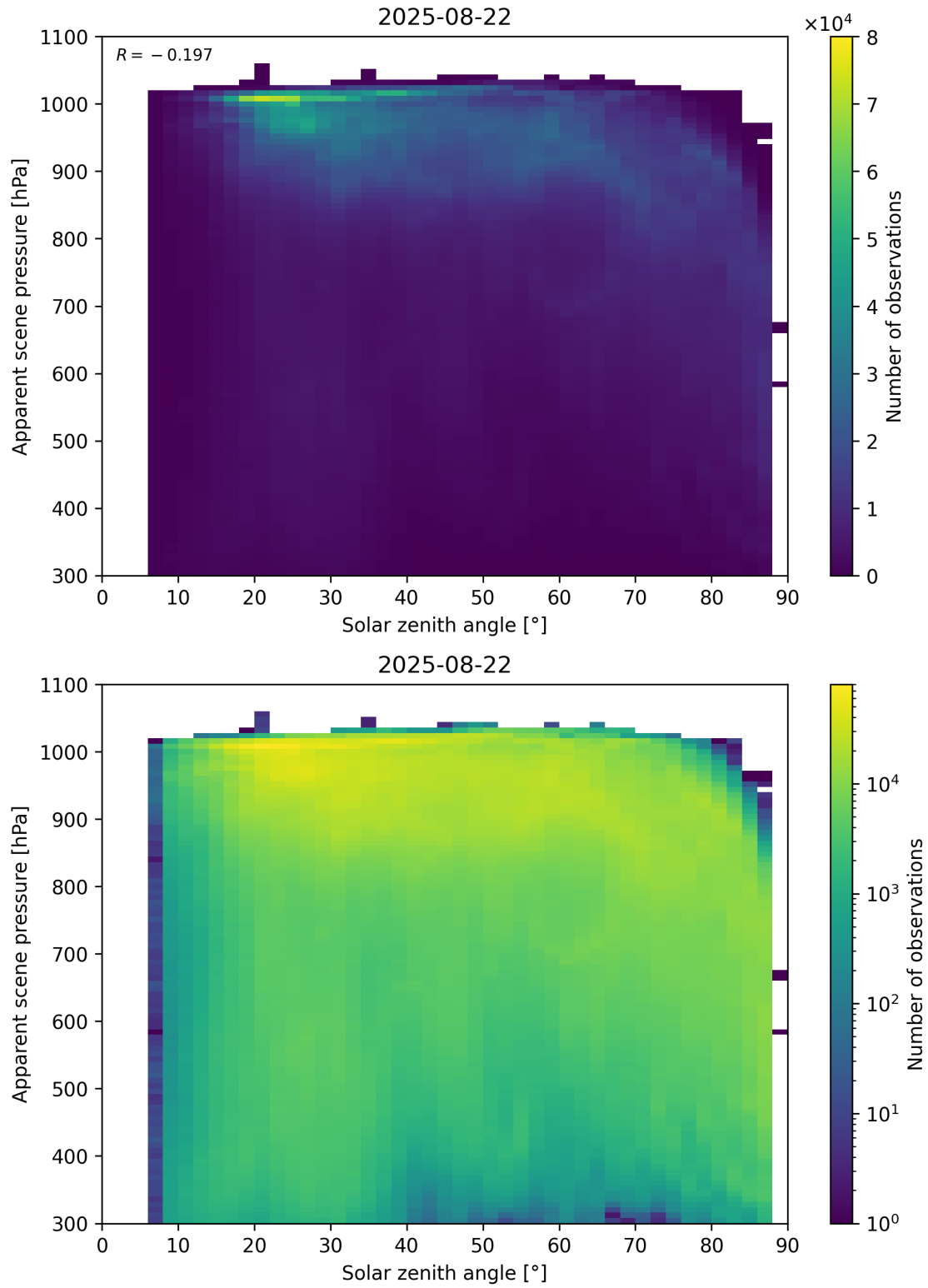
Figure 108: Scatter density plot of “Solar zenith angle” against “Apparent scene pressure” for 2025-08-21 to 2025-08-23.
