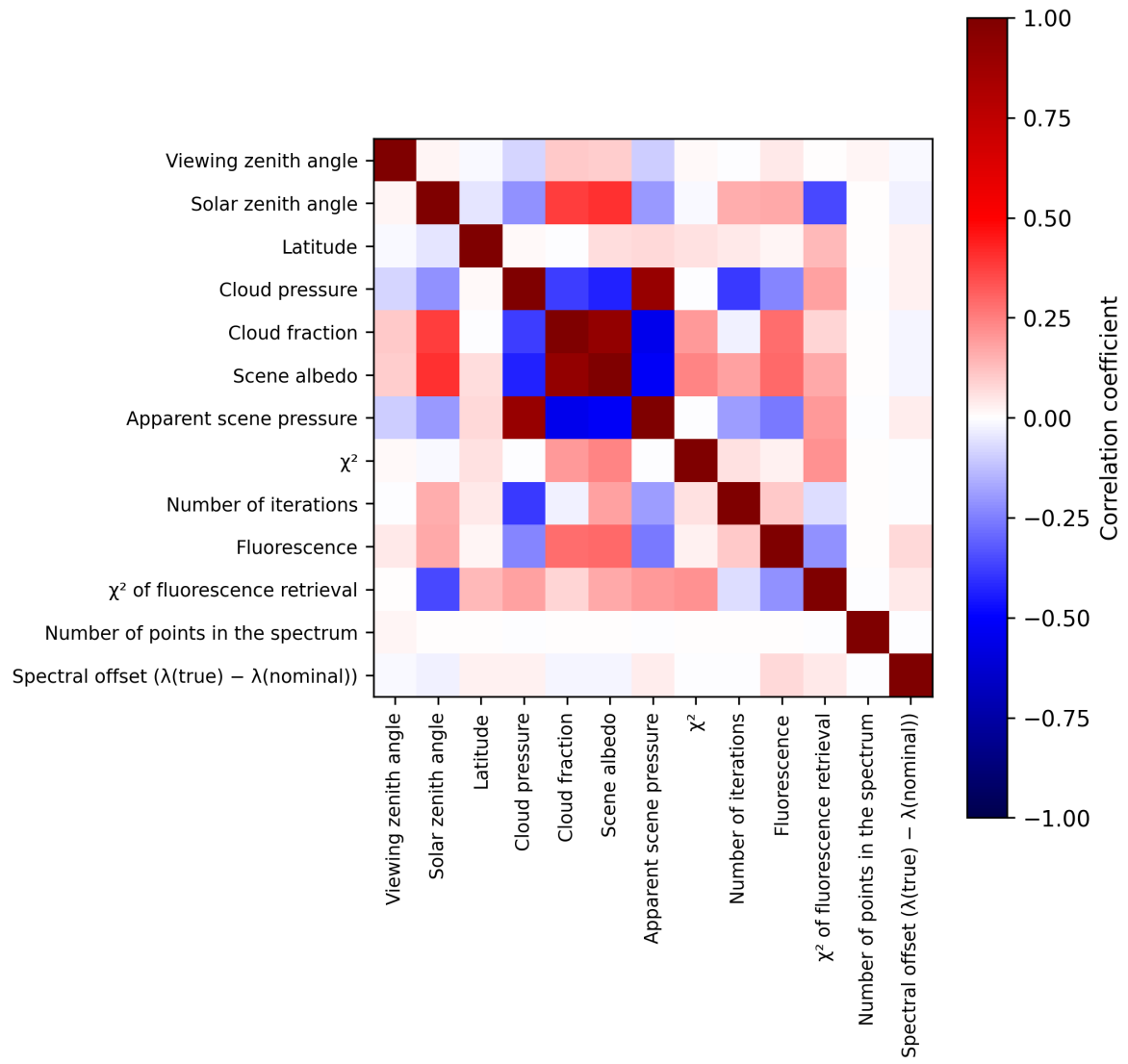
Figure 2: Map of correlation matrix for 2025-08-21 to 2025-08-23.
