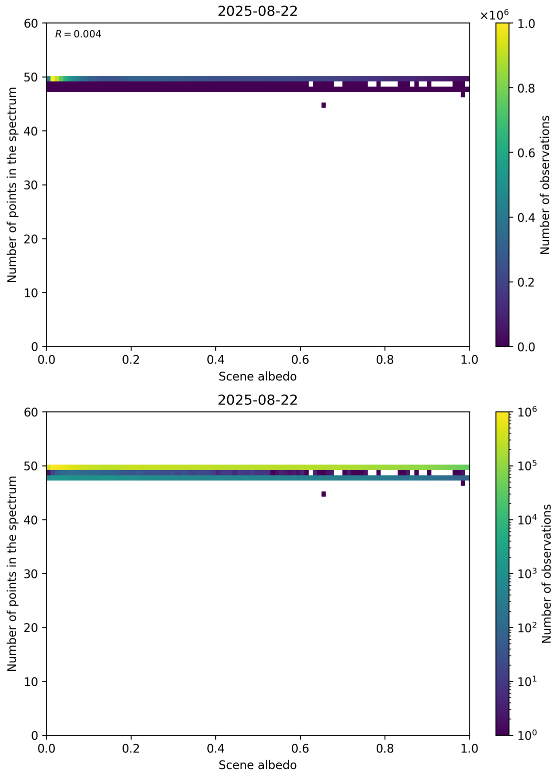
Figure 106: Scatter density plot of “Scene albedo” against “Number of points in the spectrum” for 2025-08-21 to 2025-08-23.
