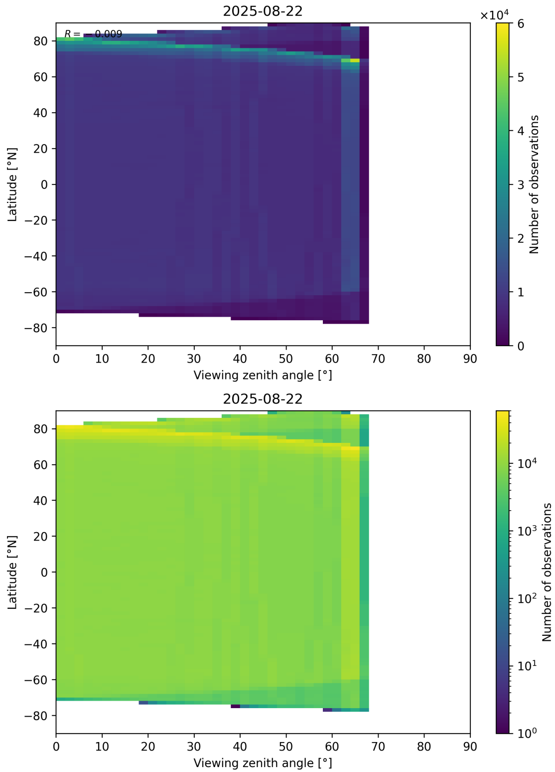
Figure 123: Scatter density plot of “Viewing zenith angle” against “Latitude” for 2025-08-21 to 2025-08-23.
