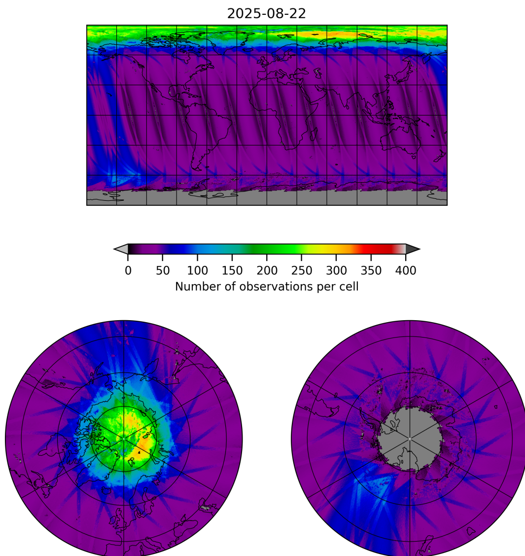
Figure 11: Map of the number of observations for 2025-08-21 to 2025-08-23
