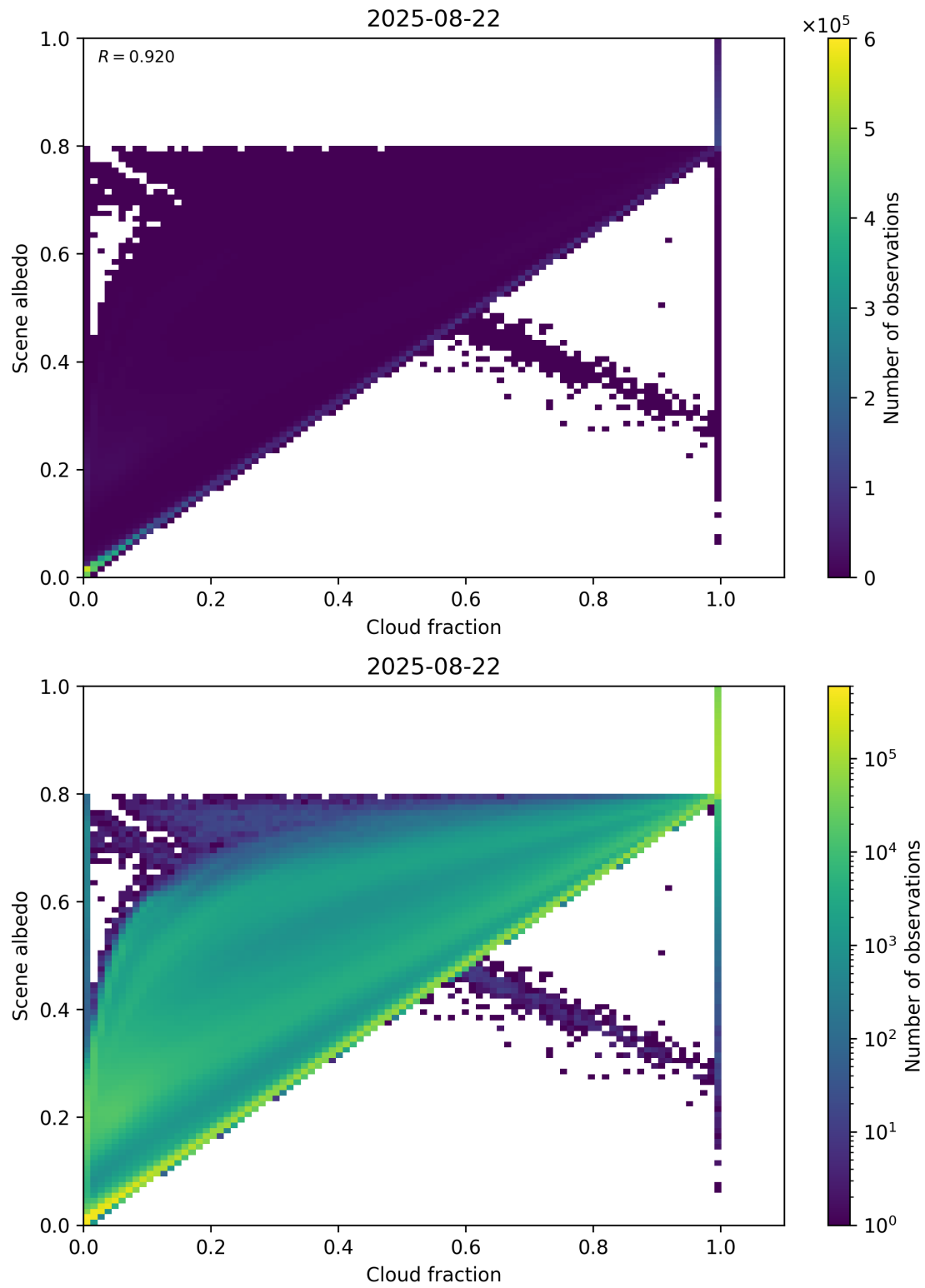
Figure 75: Scatter density plot of “Cloud fraction” against “Scene albedo” for 2025-08-21 to 2025-08-23.
