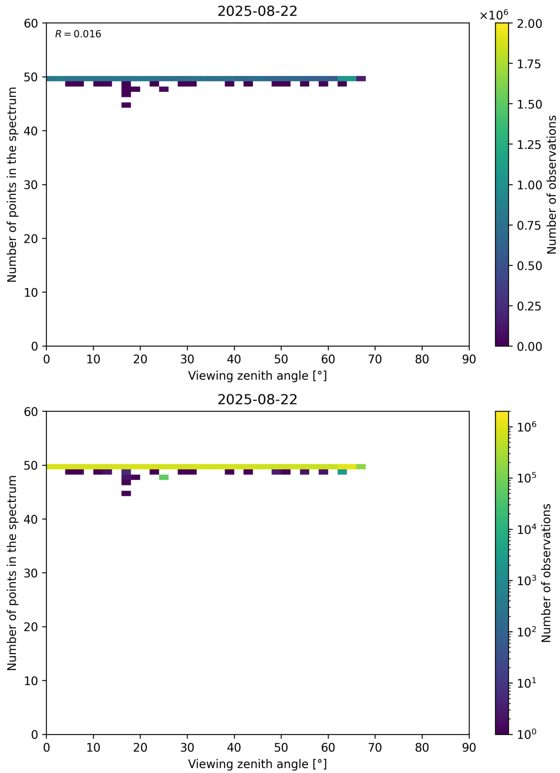
Figure 125: Scatter density plot of “Viewing zenith angle” against “Number of points in the spectrum” for 2025-08-21 to 2025-08-23.
