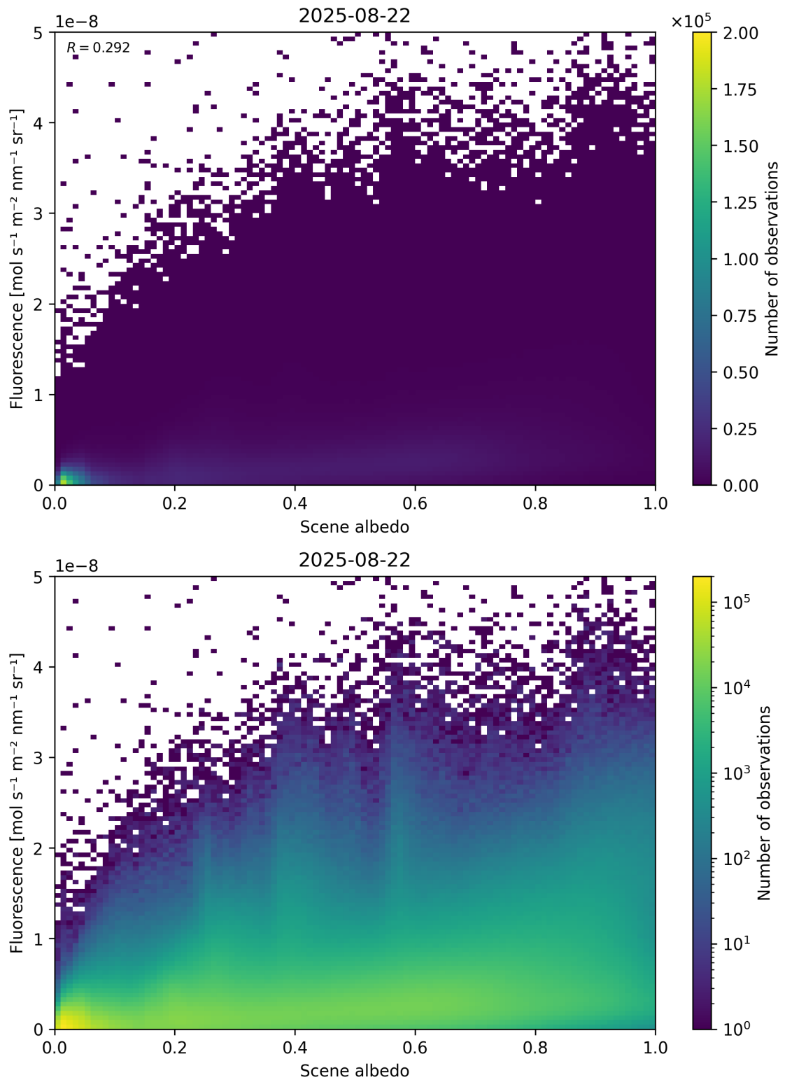
Figure 104: Scatter density plot of “Scene albedo” against “Fluorescence” for 2025-08-21 to 2025-08-23.
