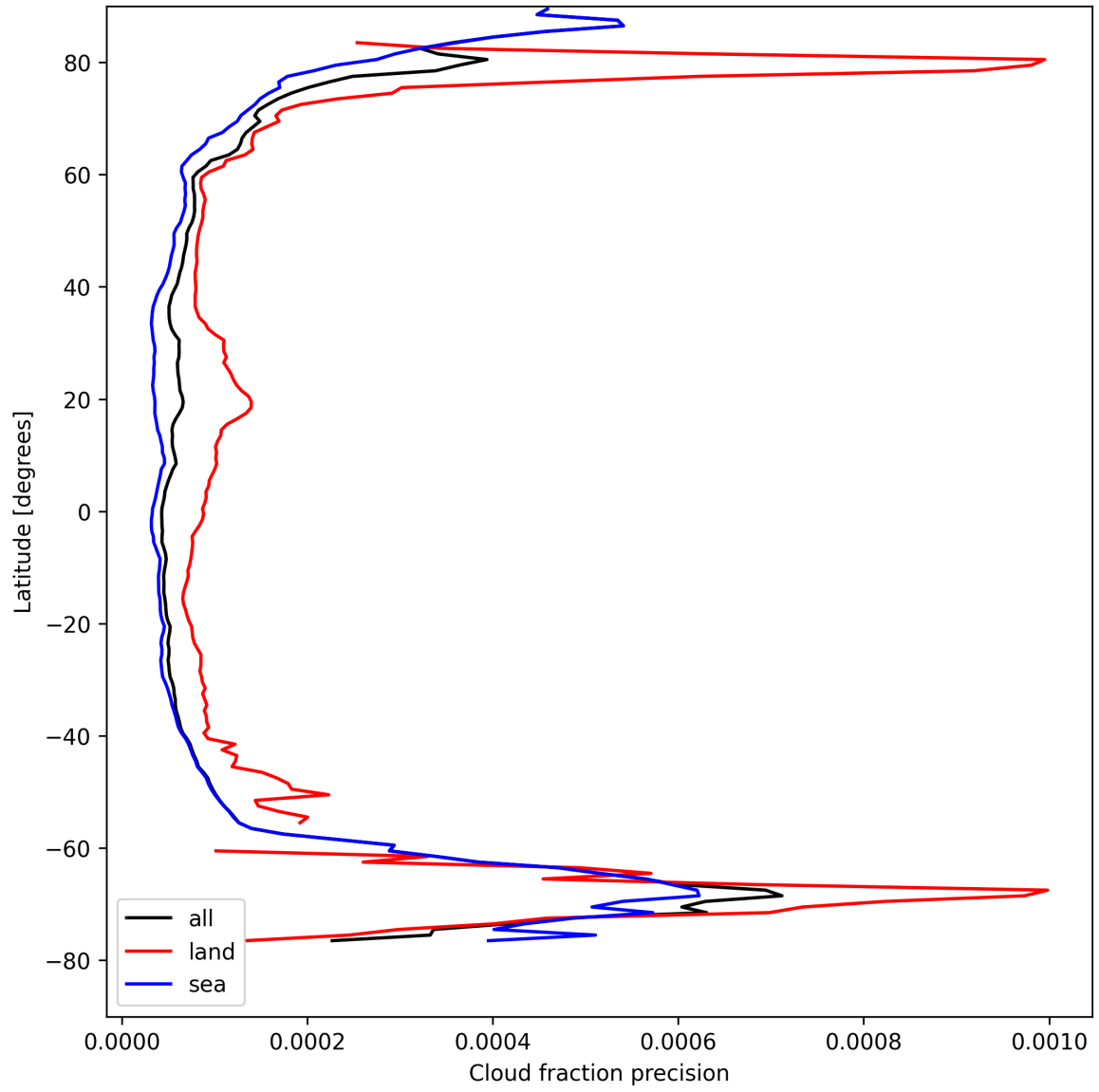
Figure 16: Zonal average of “Cloud fraction precision” for 2025-08-21 to 2025-08-23.
