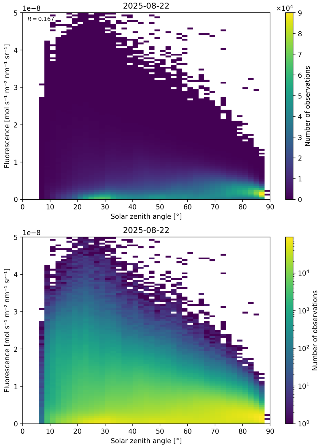
Figure 112: Scatter density plot of “Solar zenith angle” against “Fluorescence” for 2025-08-21 to 2025-08-23.
