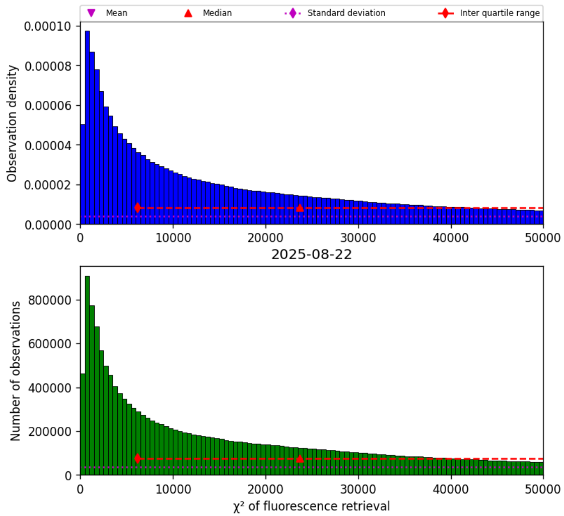
Figure 42: Histogram of “ \chi^2 of fluorescence retrieval” for 2025-08-21 to 2025-08-23
