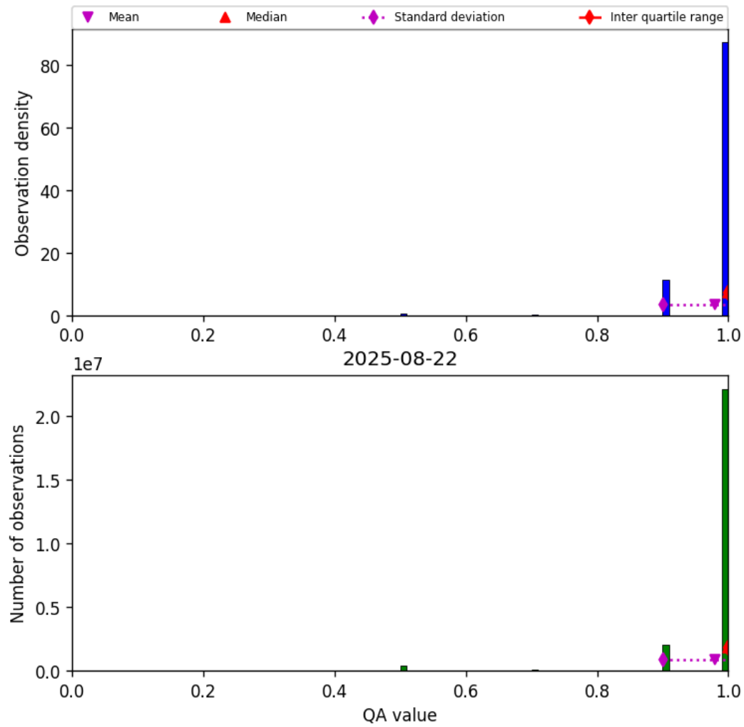
Figure 29: Histogram of “QA value” for 2025-08-21 to 2025-08-23
