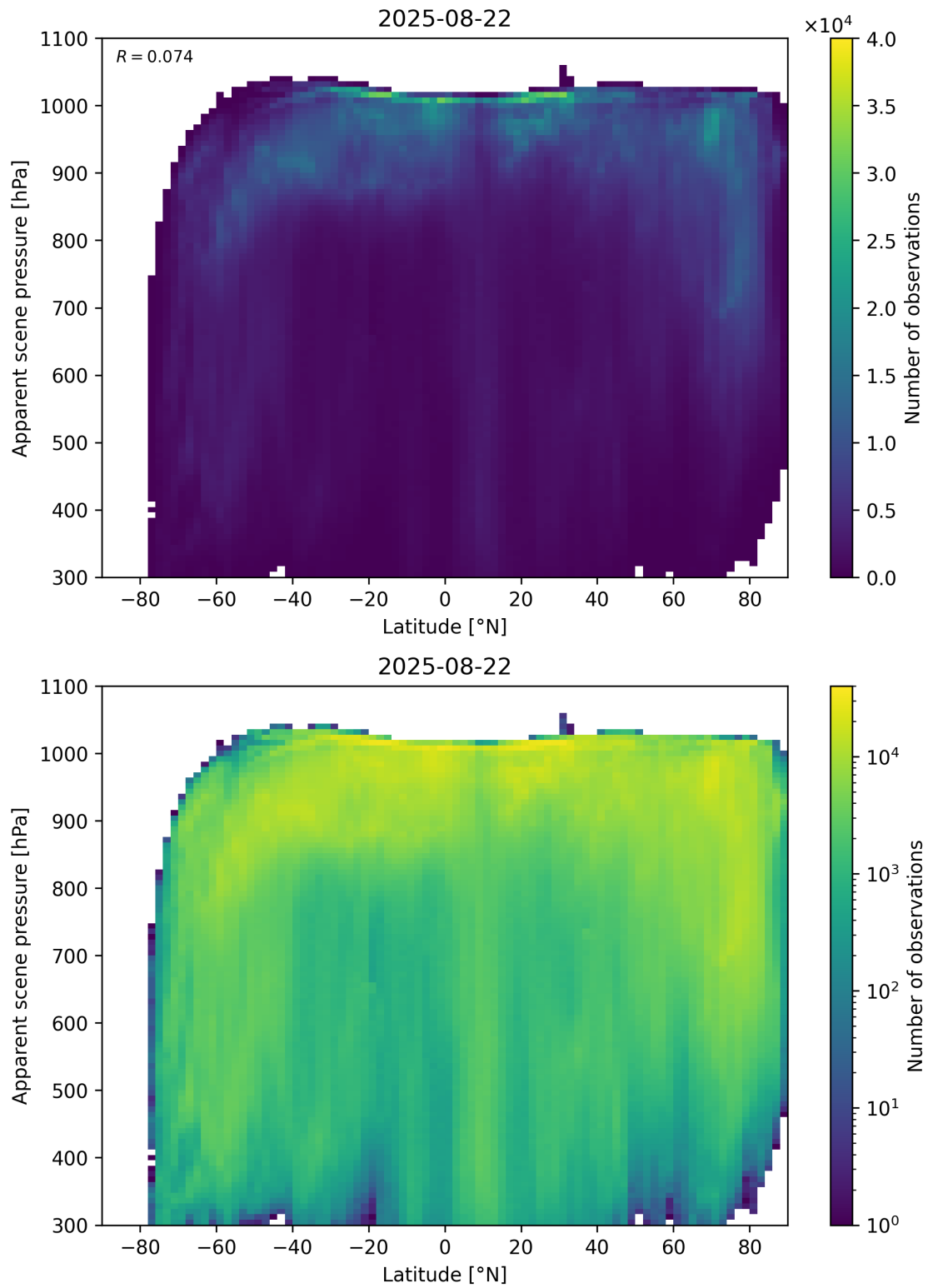
Figure 88: Scatter density plot of “Latitude” against “Apparent scene pressure” for 2025-08-21 to 2025-08-23.
