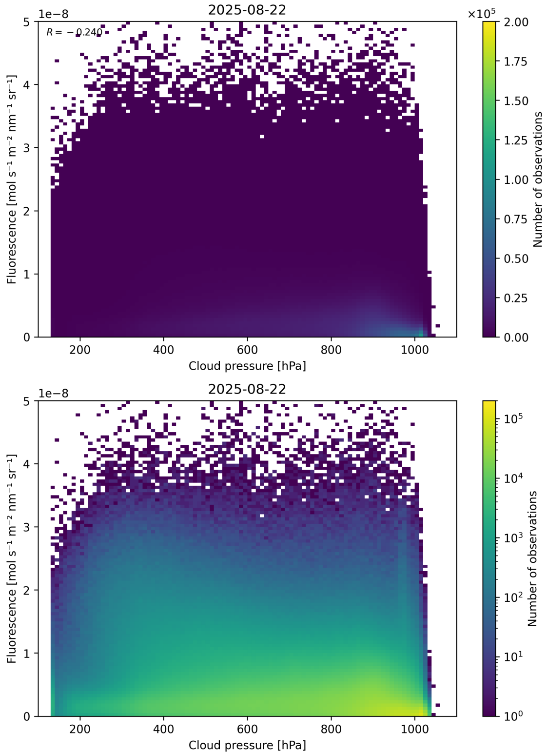
Figure 80: Scatter density plot of “Cloud pressure” against “Fluorescence” for 2025-08-21 to 2025-08-23.
