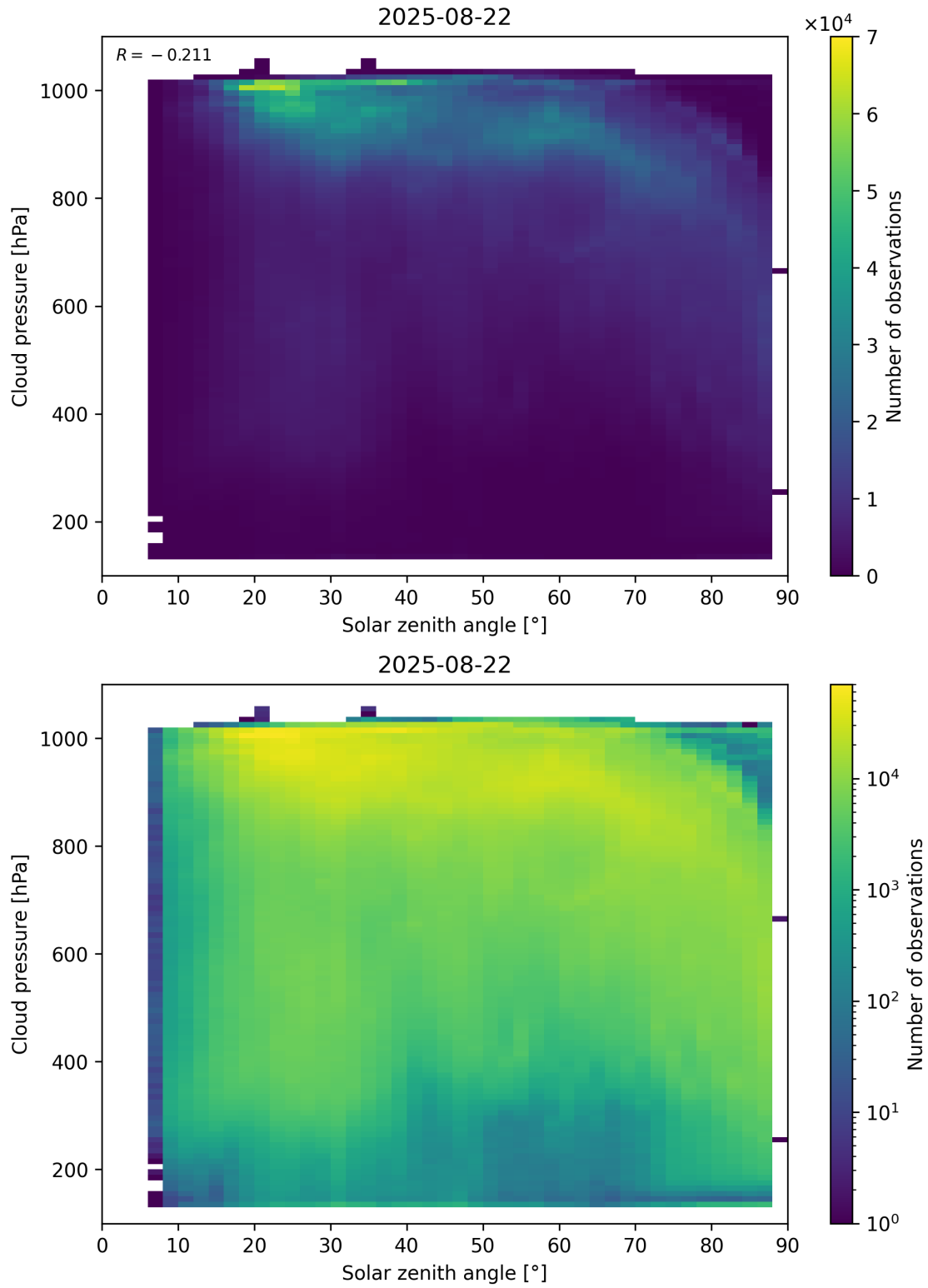
Figure 111: Scatter density plot of “Solar zenith angle” against “Cloud pressure” for 2025-08-21 to 2025-08-23.
