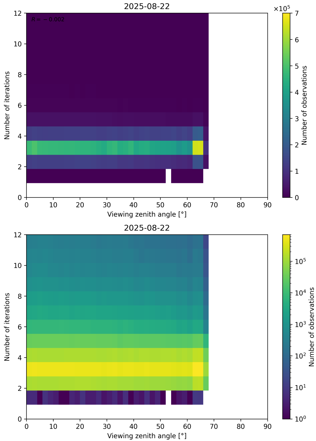
Figure 124: Scatter density plot of “Viewing zenith angle” against “Number of iterations” for 2025-08-21 to 2025-08-23.
