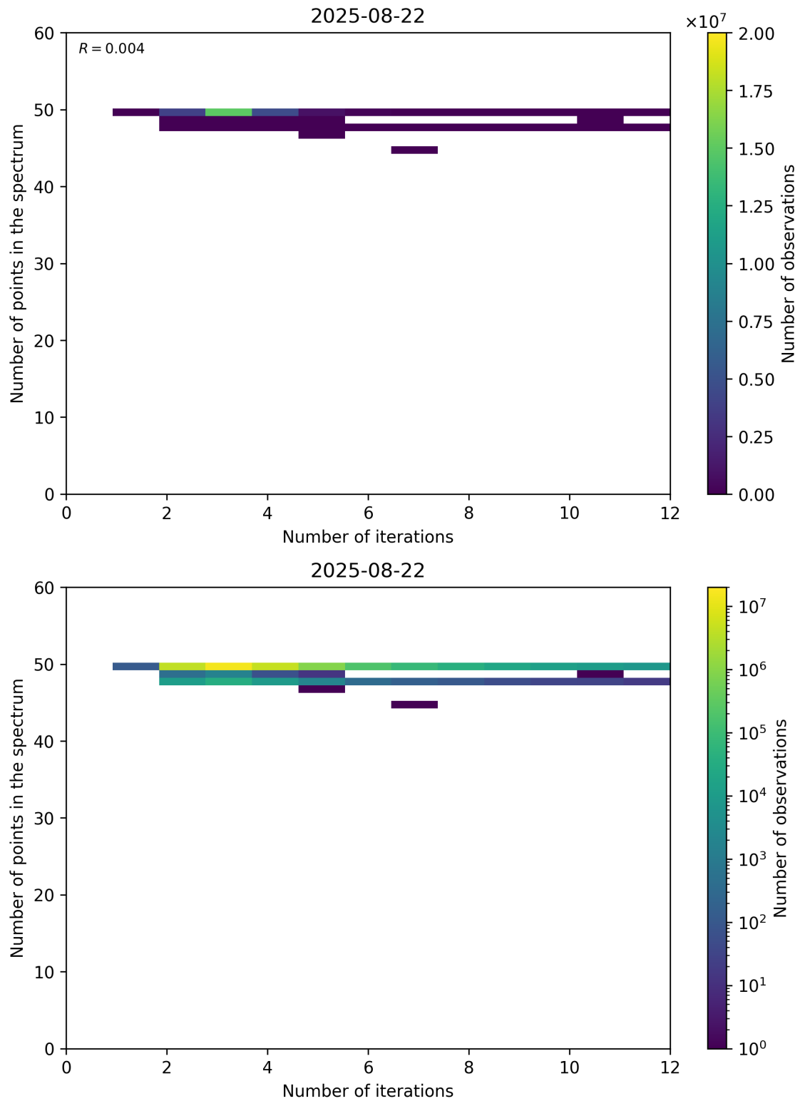
Figure 99: Scatter density plot of “Number of iterations” against “Number of points in the spectrum” for 2025-08-21 to 2025-08-23.
