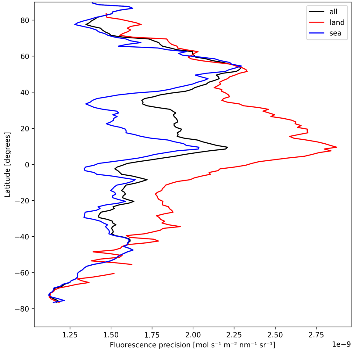
Figure 24: Zonal average of “Fluorescence precision” for 2025-08-21 to 2025-08-23.
