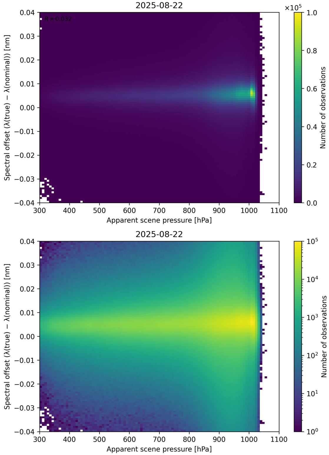
Figure 67: Scatter density plot of “Apparent scene pressure” against “Spectral offset ( \lambda_{\text{true}} - \lambda_{\text{nominal}} )” for 2025-08-21 to 2025-08-23.
