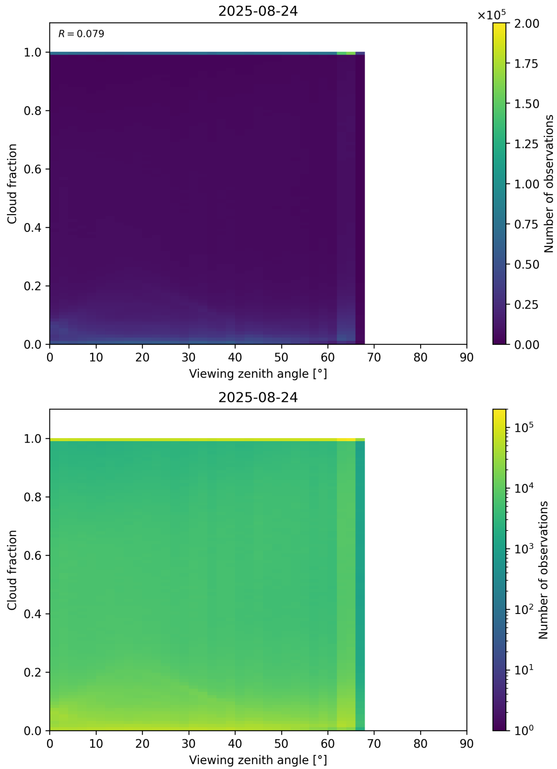
Figure 120: Scatter density plot of “Viewing zenith angle” against “Cloud fraction” for 2025-08-23 to 2025-08-25.
