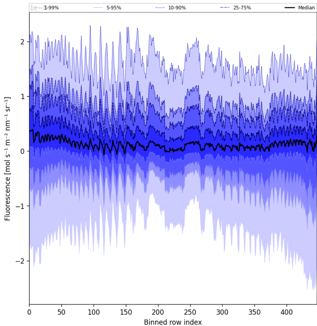
Figure 57: Along track statistics of “Fluorescence” for 2025-08-23 to 2025-08-25
