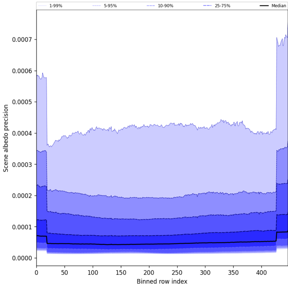
Figure 52: Along track statistics of “Scene albedo precision” for 2025-08-23 to 2025-08-25
