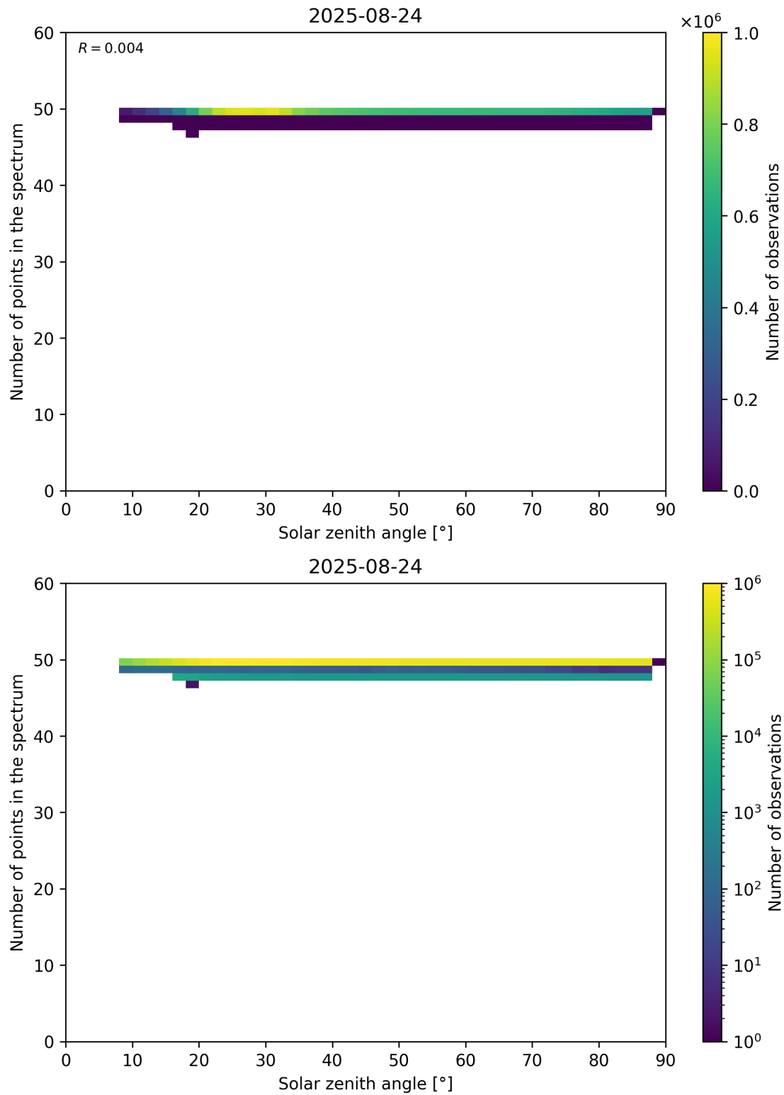
Figure 115: Scatter density plot of “Solar zenith angle” against “Number of points in the spectrum” for 2025-08-23 to 2025-08-25.
