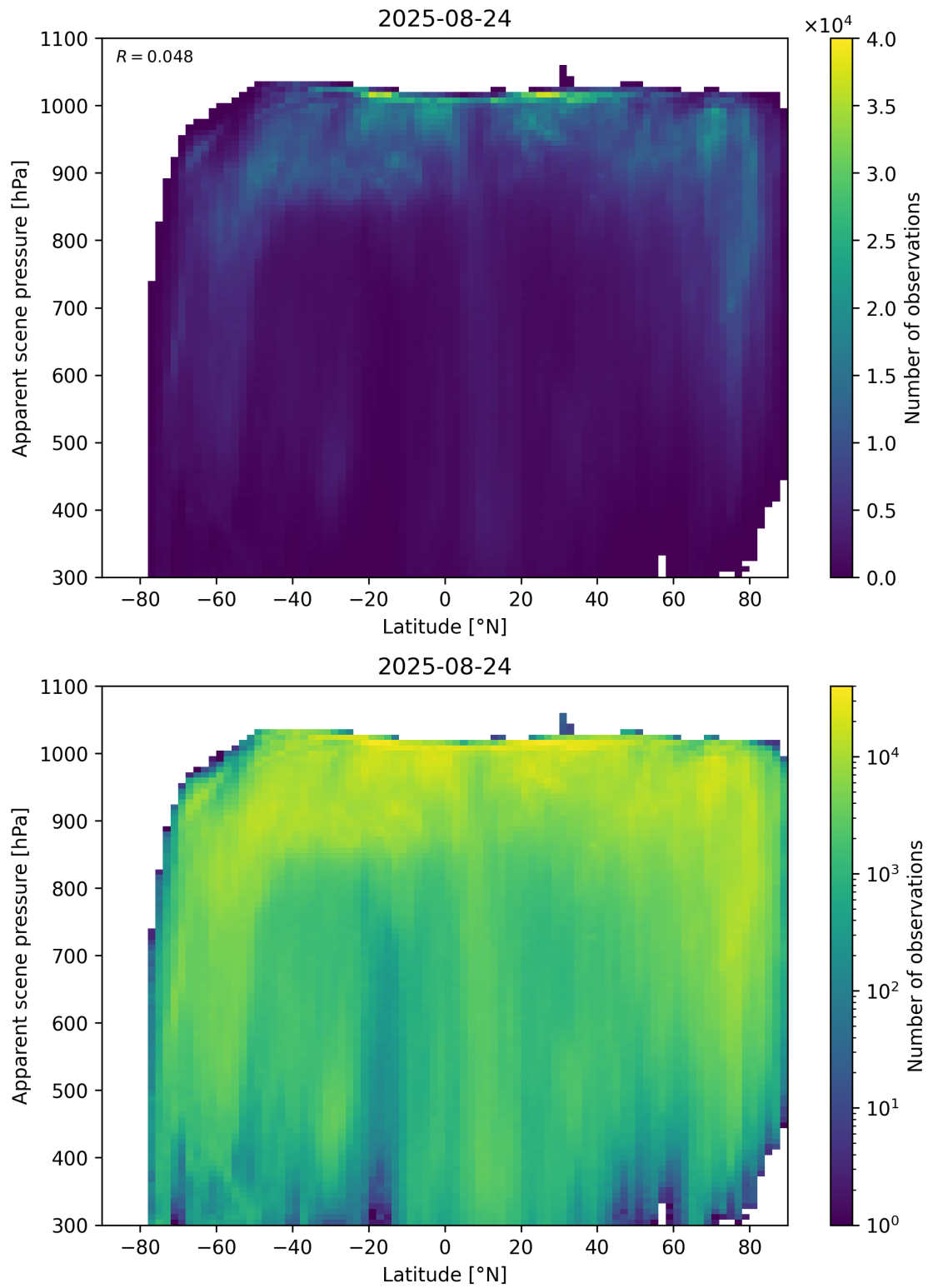
Figure 88: Scatter density plot of “Latitude” against “Apparent scene pressure” for 2025-08-23 to 2025-08-25.
