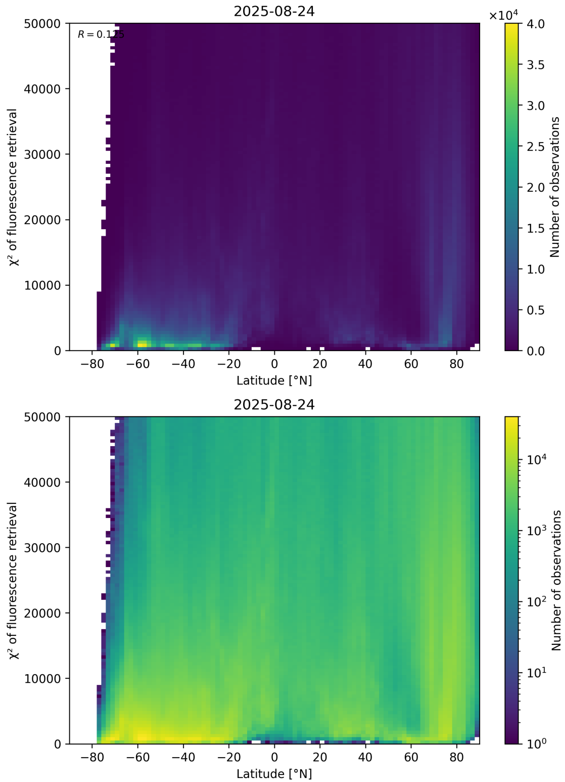
Figure 89: Scatter density plot of “Latitude” against “ \chi^2 of fluorescence retrieval” for 2025-08-23 to 2025-08-25.
