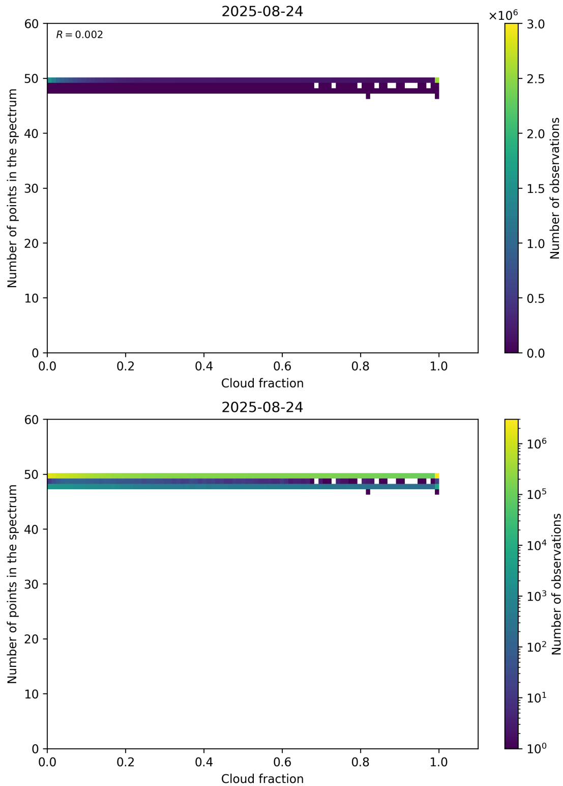
Figure 74: Scatter density plot of “Cloud fraction” against “Number of points in the spectrum” for 2025-08-23 to 2025-08-25.
