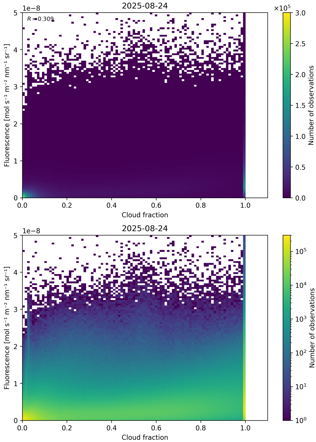
Figure 72: Scatter density plot of “Cloud fraction” against “Fluorescence” for 2025-08-23 to 2025-08-25.
