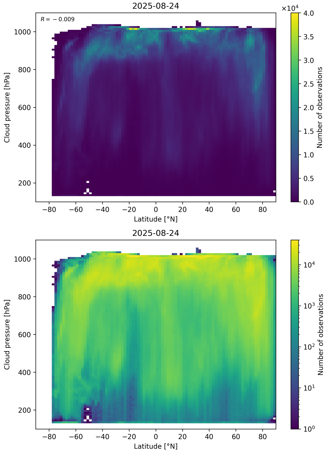
Figure 91: Scatter density plot of “Latitude” against “Cloud pressure” for 2025-08-23 to 2025-08-25.
