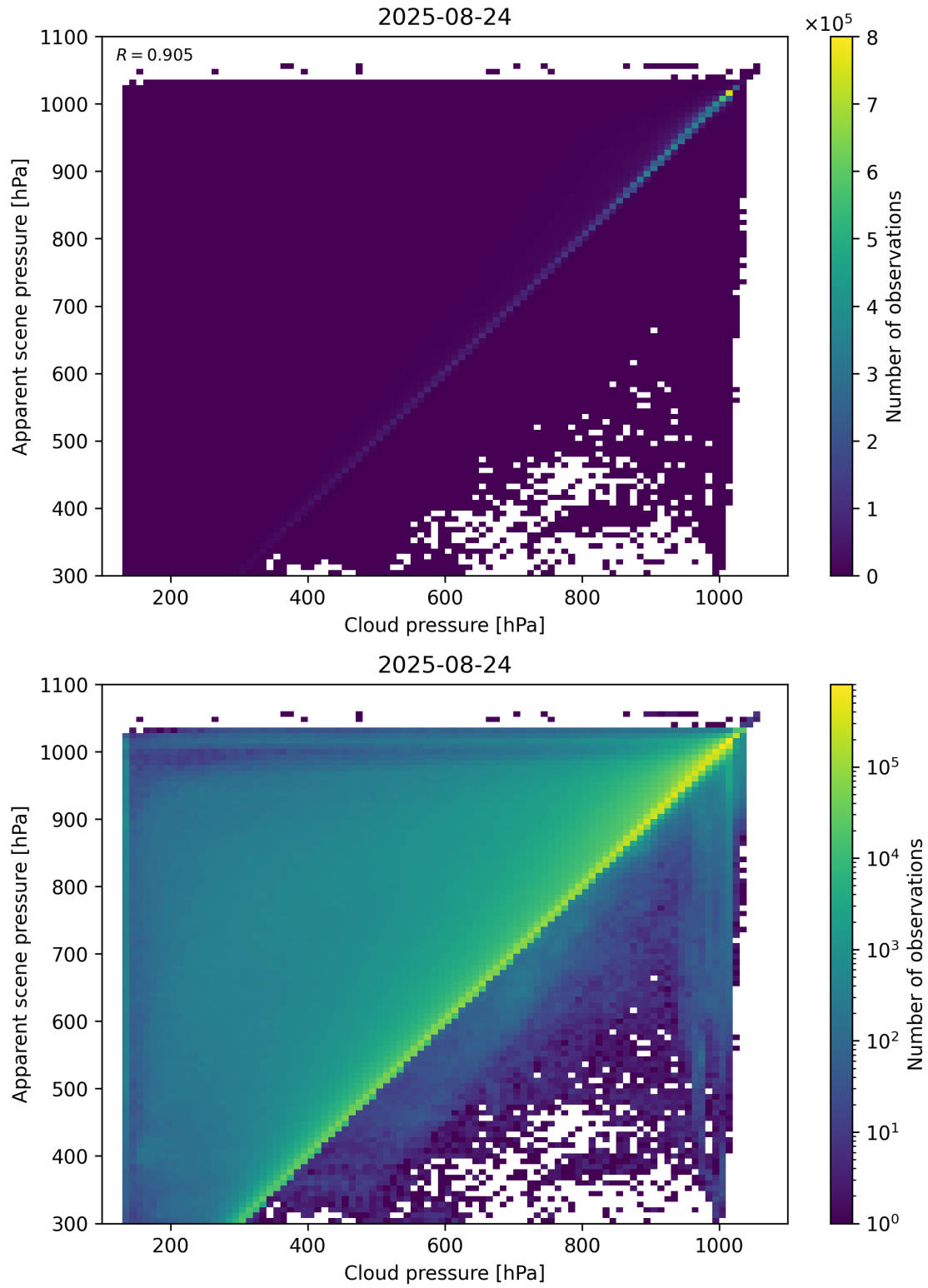
Figure 77: Scatter density plot of “Cloud pressure” against “Apparent scene pressure” for 2025-08-23 to 2025-08-25.
