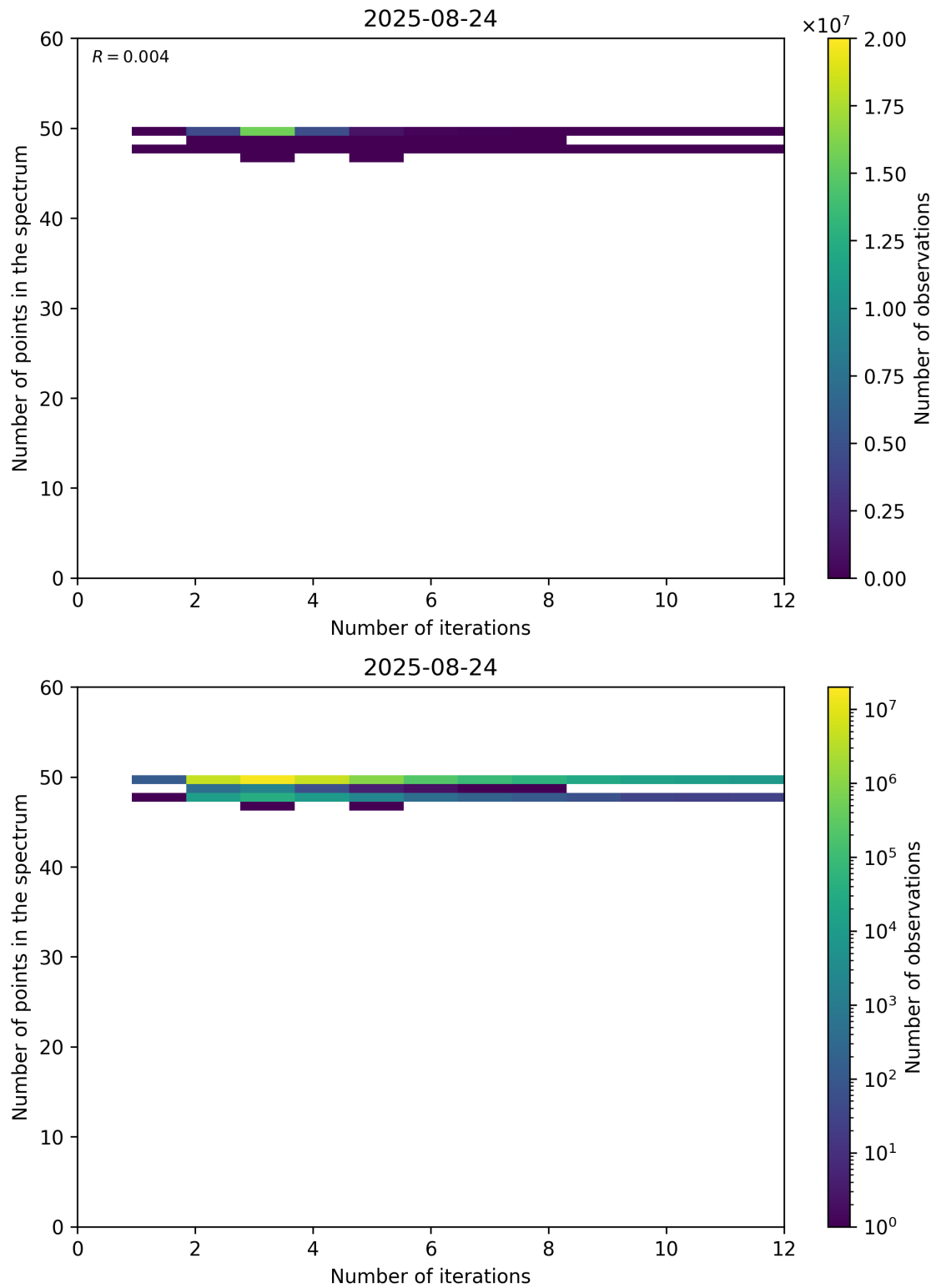
Figure 99: Scatter density plot of “Number of iterations” against “Number of points in the spectrum” for 2025-08-23 to 2025-08-25.
