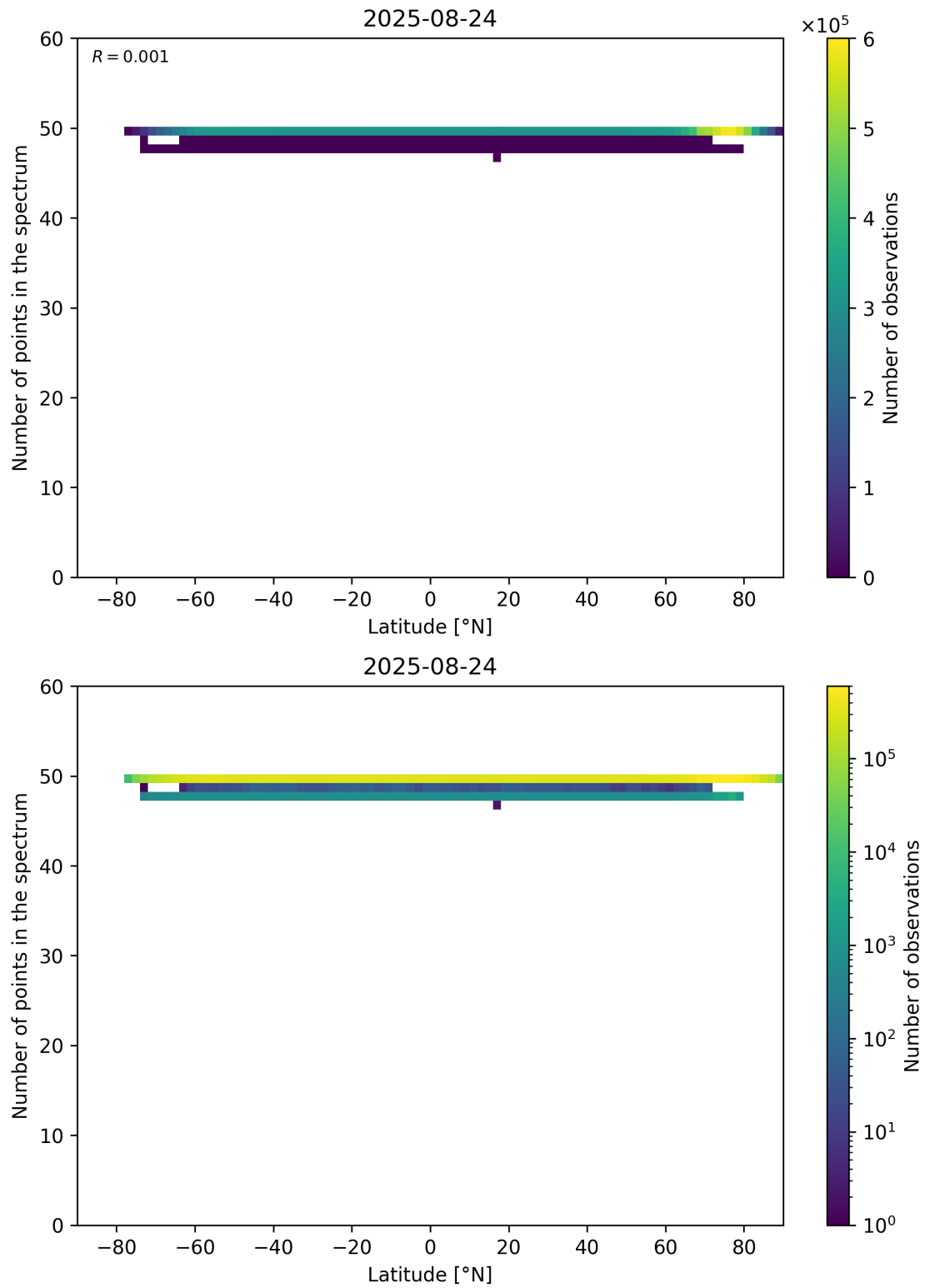
Figure 94: Scatter density plot of “Latitude” against “Number of points in the spectrum” for 2025-08-23 to 2025-08-25.
