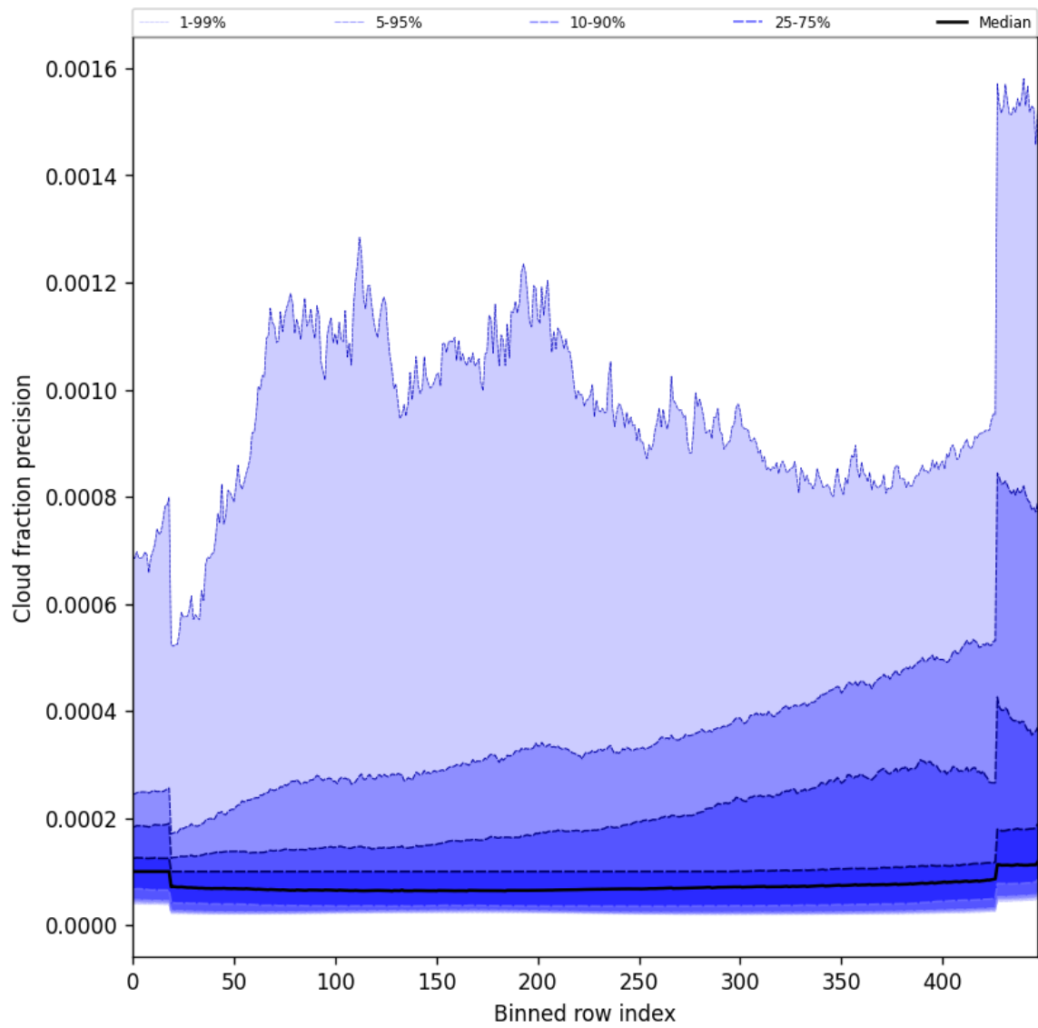
Figure 50: Along track statistics of “Cloud fraction precision” for 2025-08-23 to 2025-08-25
