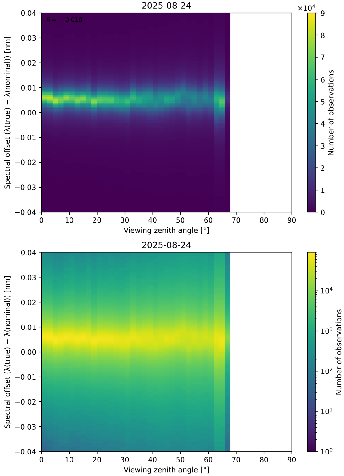
Figure 128: Scatter density plot of “Viewing zenith angle” against “Spectral offset ( \lambda_{\text{true}} - \lambda_{\text{nominal}} )” for 2025-08-23 to 2025-08-25.
