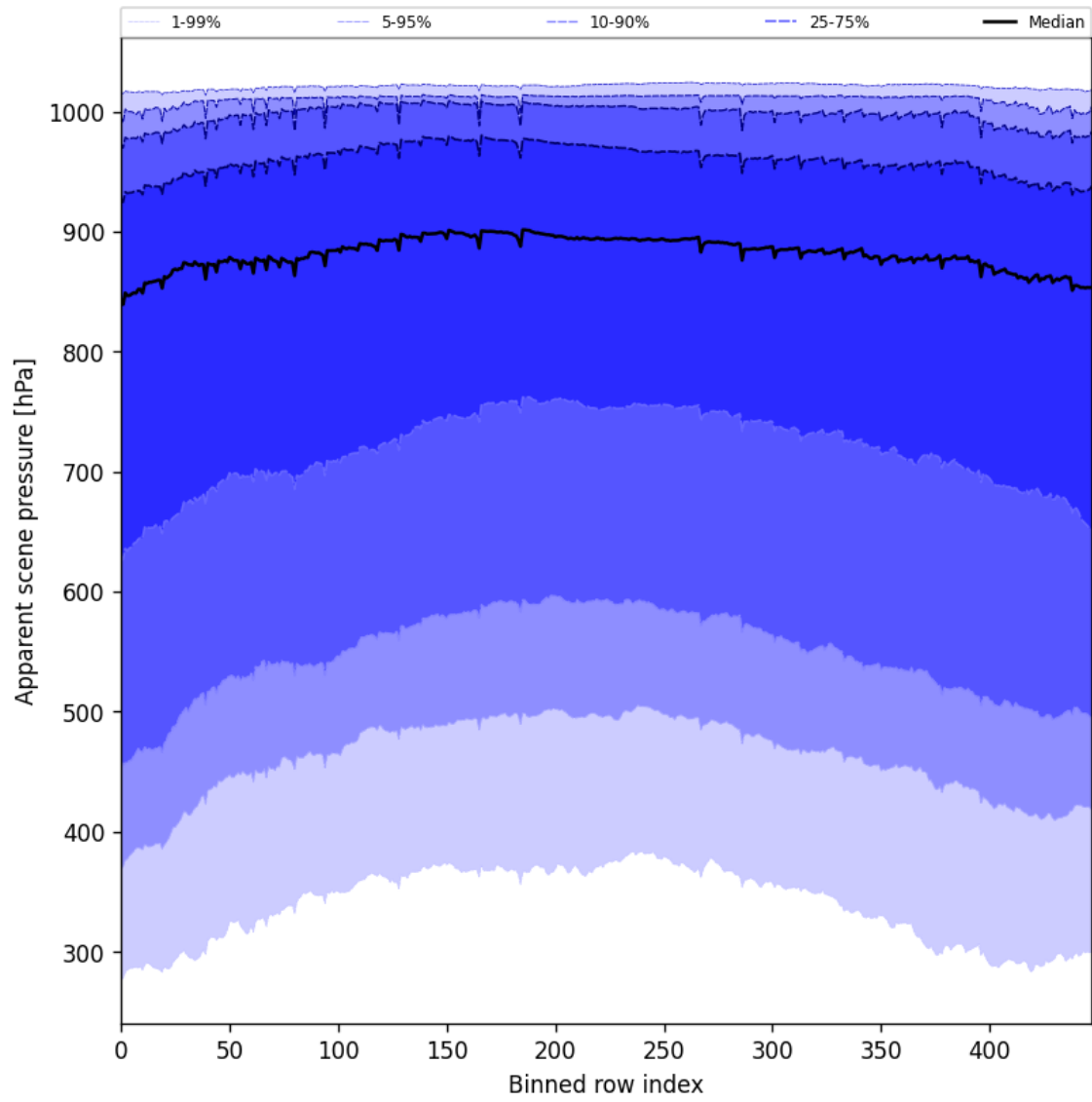
Figure 53: Along track statistics of “Apparent scene pressure” for 2025-08-23 to 2025-08-25
