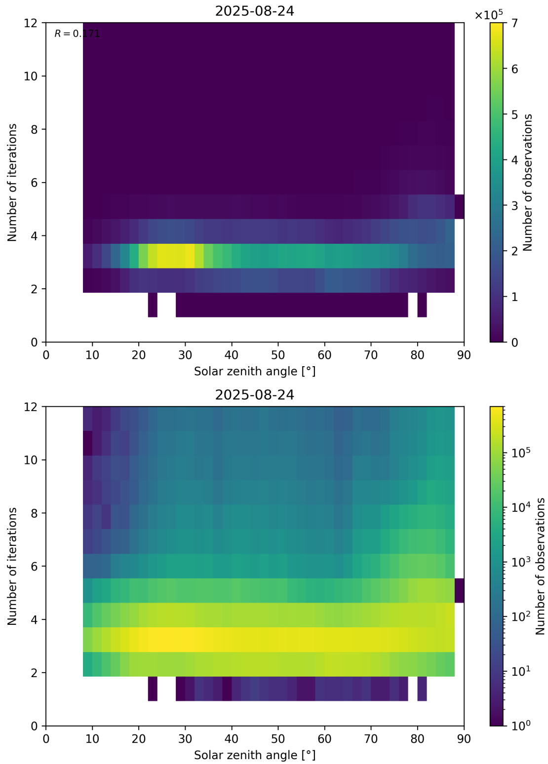
Figure 114: Scatter density plot of “Solar zenith angle” against “Number of iterations” for 2025-08-23 to 2025-08-25.
