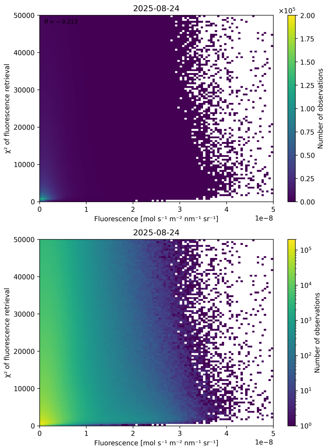
Figure 85: Scatter density plot of “Fluorescence” against “ \chi^2 of fluorescence retrieval” for 2025-08-23 to 2025-08-25.
