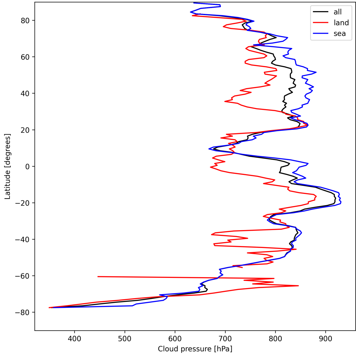
Figure 13: Zonal average of “Cloud pressure” for 2025-08-23 to 2025-08-25.
