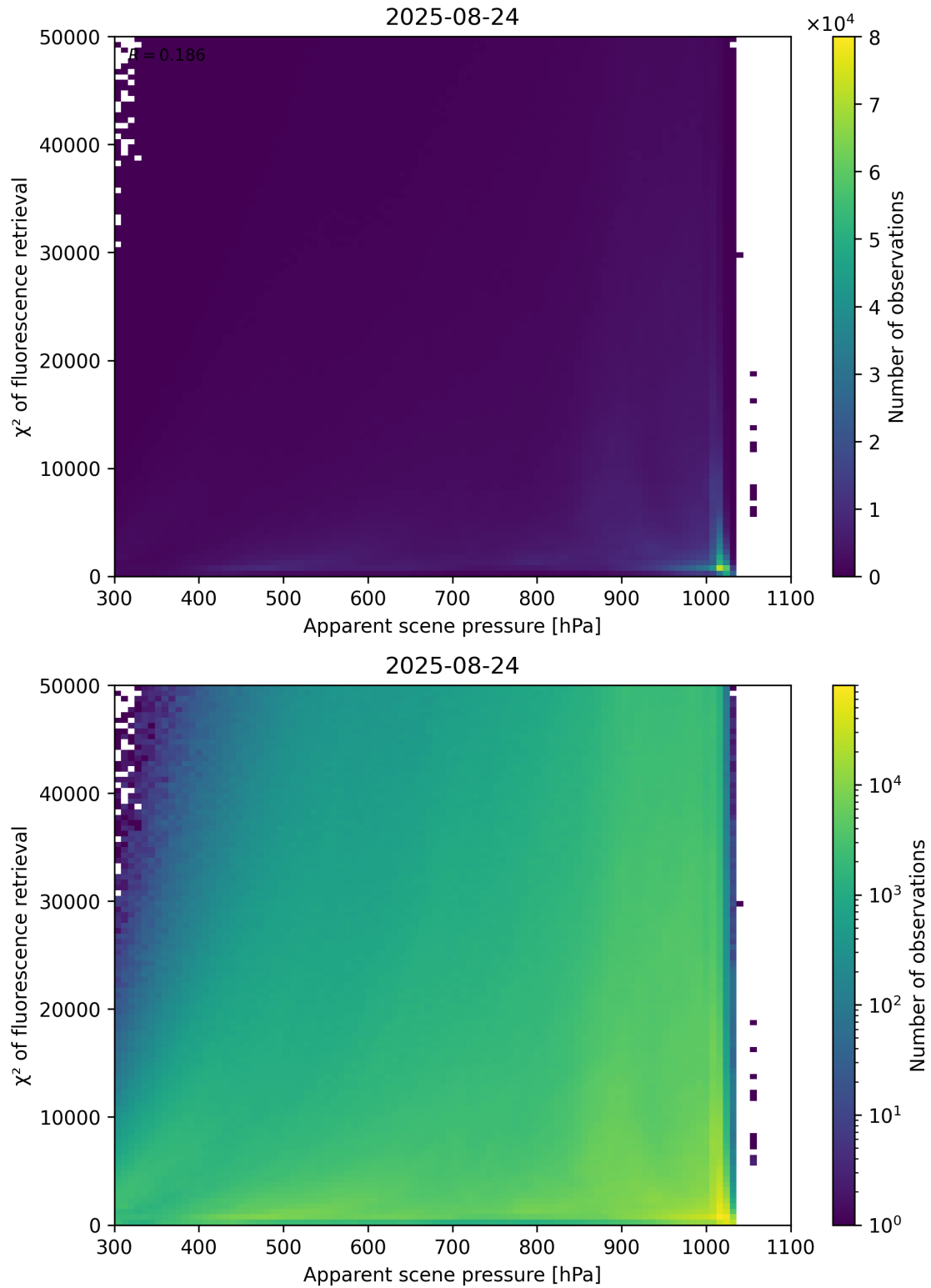
Figure 63: Scatter density plot of “Apparent scene pressure” against “ \chi^2 of fluorescence retrieval” for 2025-08-23 to 2025-08-25.
