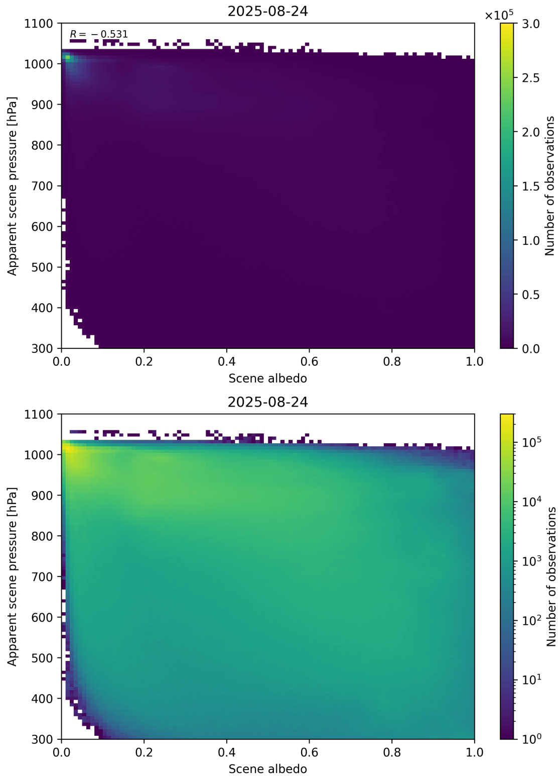
Figure 102: Scatter density plot of “Scene albedo” against “Apparent scene pressure” for 2025-08-23 to 2025-08-25.
