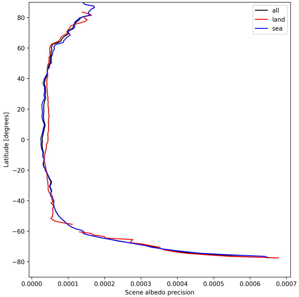
Figure 18: Zonal average of “Scene albedo precision” for 2025-08-23 to 2025-08-25.
