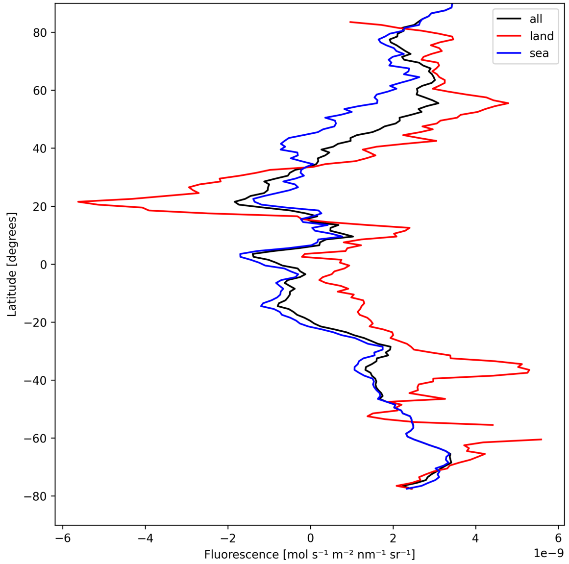
Figure 23: Zonal average of “Fluorescence” for 2025-08-23 to 2025-08-25.
