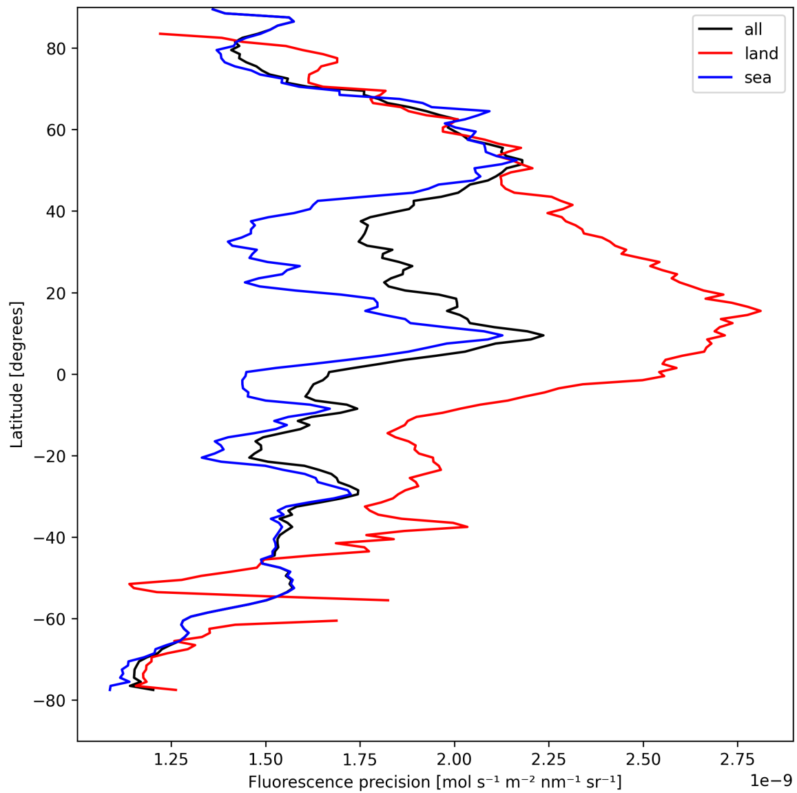
Figure 24: Zonal average of “Fluorescence precision” for 2025-08-23 to 2025-08-25.
