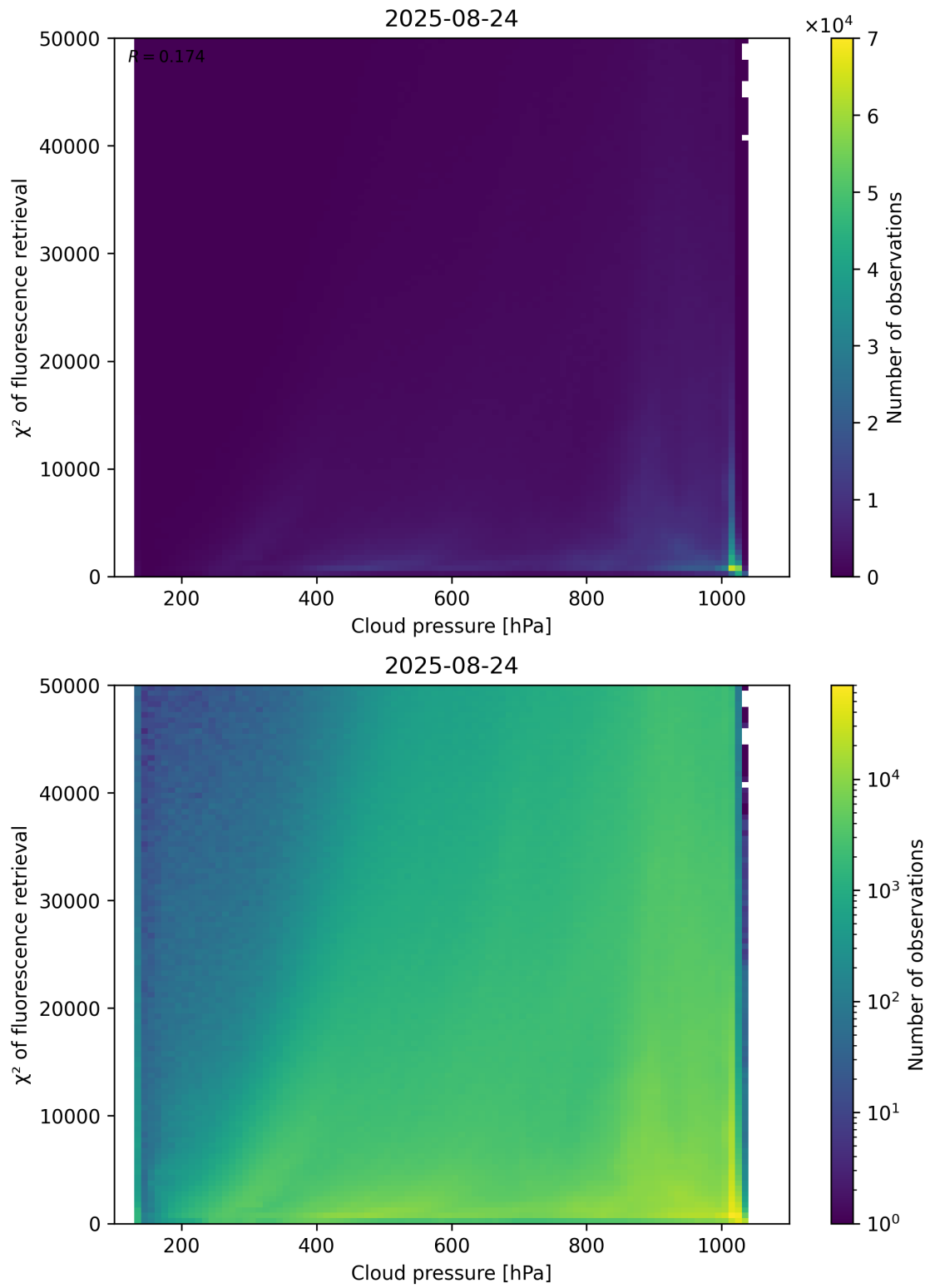
Figure 78: Scatter density plot of “Cloud pressure” against “ \chi^2 of fluorescence retrieval” for 2025-08-23 to 2025-08-25.
