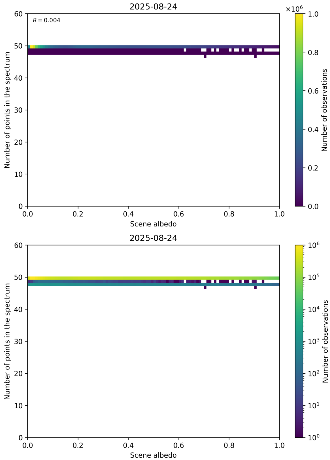
Figure 106: Scatter density plot of “Scene albedo” against “Number of points in the spectrum” for 2025-08-23 to 2025-08-25.
