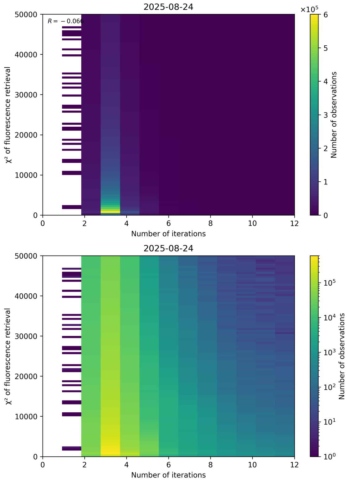
Figure 97: Scatter density plot of “Number of iterations” against “ \chi^2 of fluorescence retrieval” for 2025-08-23 to 2025-08-25.
