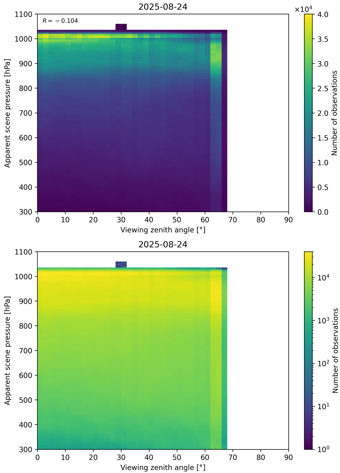
Figure 118: Scatter density plot of “Viewing zenith angle” against “Apparent scene pressure” for 2025-08-23 to 2025-08-25.
