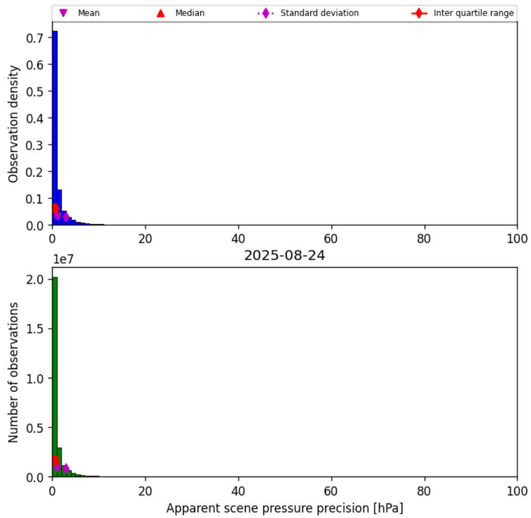
Figure 37: Histogram of “Apparent scene pressure precision” for 2025-08-23 to 2025-08-25
