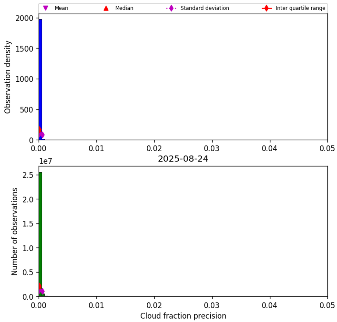
Figure 33: Histogram of “Cloud fraction precision” for 2025-08-23 to 2025-08-25
