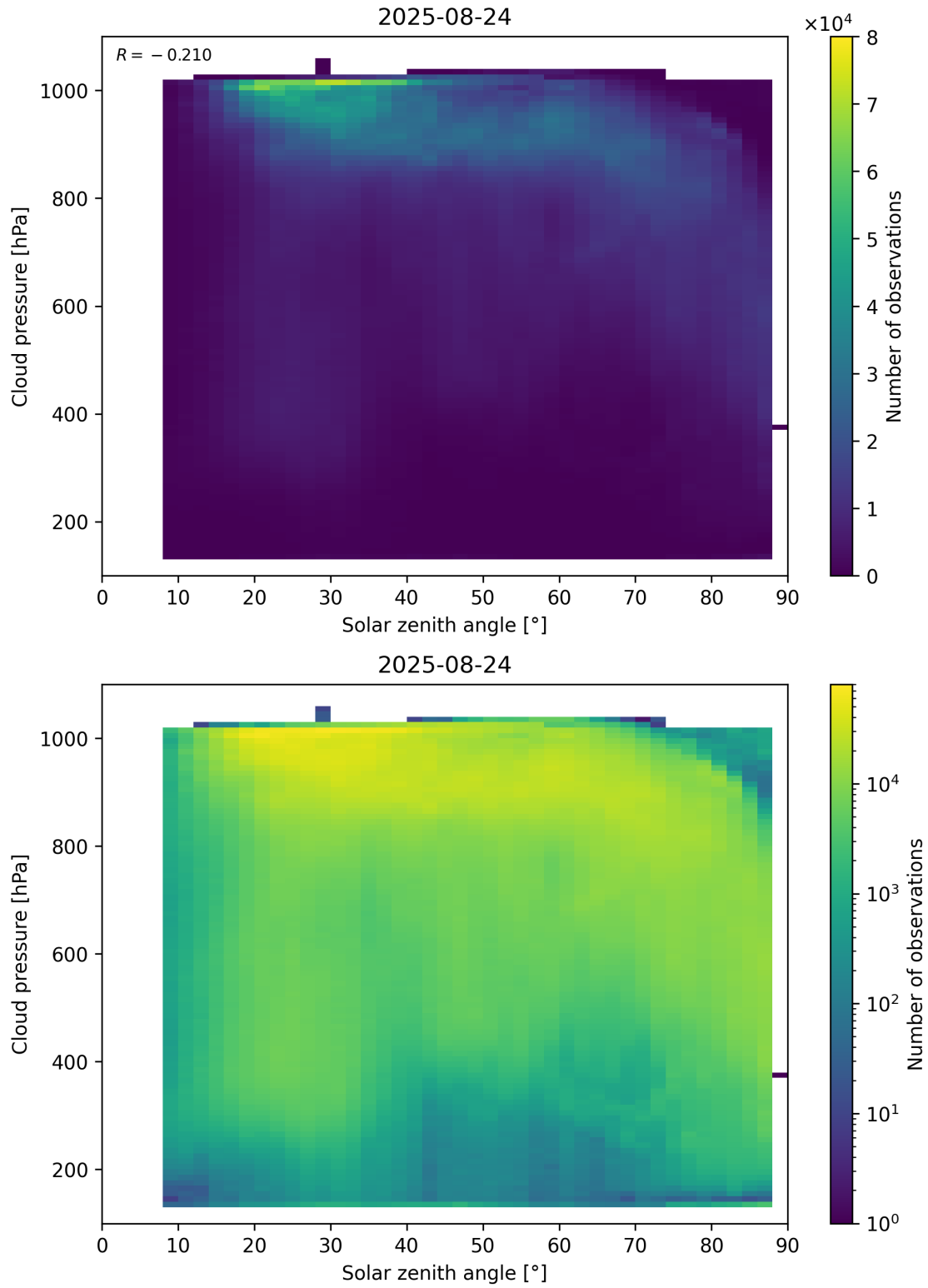
Figure 111: Scatter density plot of “Solar zenith angle” against “Cloud pressure” for 2025-08-23 to 2025-08-25.
