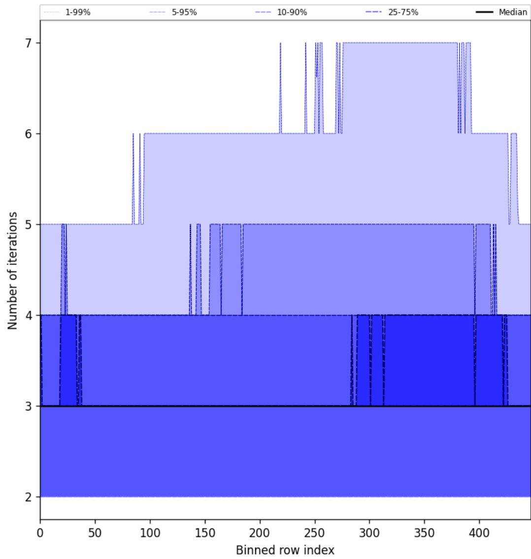
Figure 56: Along track statistics of “Number of iterations” for 2025-08-23 to 2025-08-25
