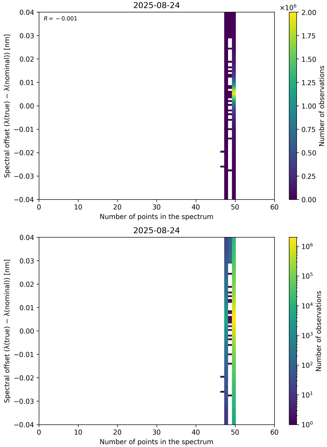
Figure 101: Scatter density plot of “Number of points in the spectrum” against “Spectral offset ( \lambda_{\text{true}} - \lambda_{\text{nominal}} )” for 2025-08-23 to 2025-08-25.
