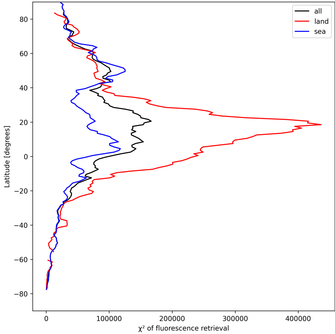
Figure 25: Zonal average of “ \chi^2 of fluorescence retrieval” for 2025-08-23 to 2025-08-25.
