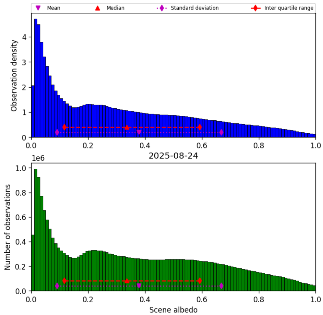
Figure 34: Histogram of “Scene albedo” for 2025-08-23 to 2025-08-25
