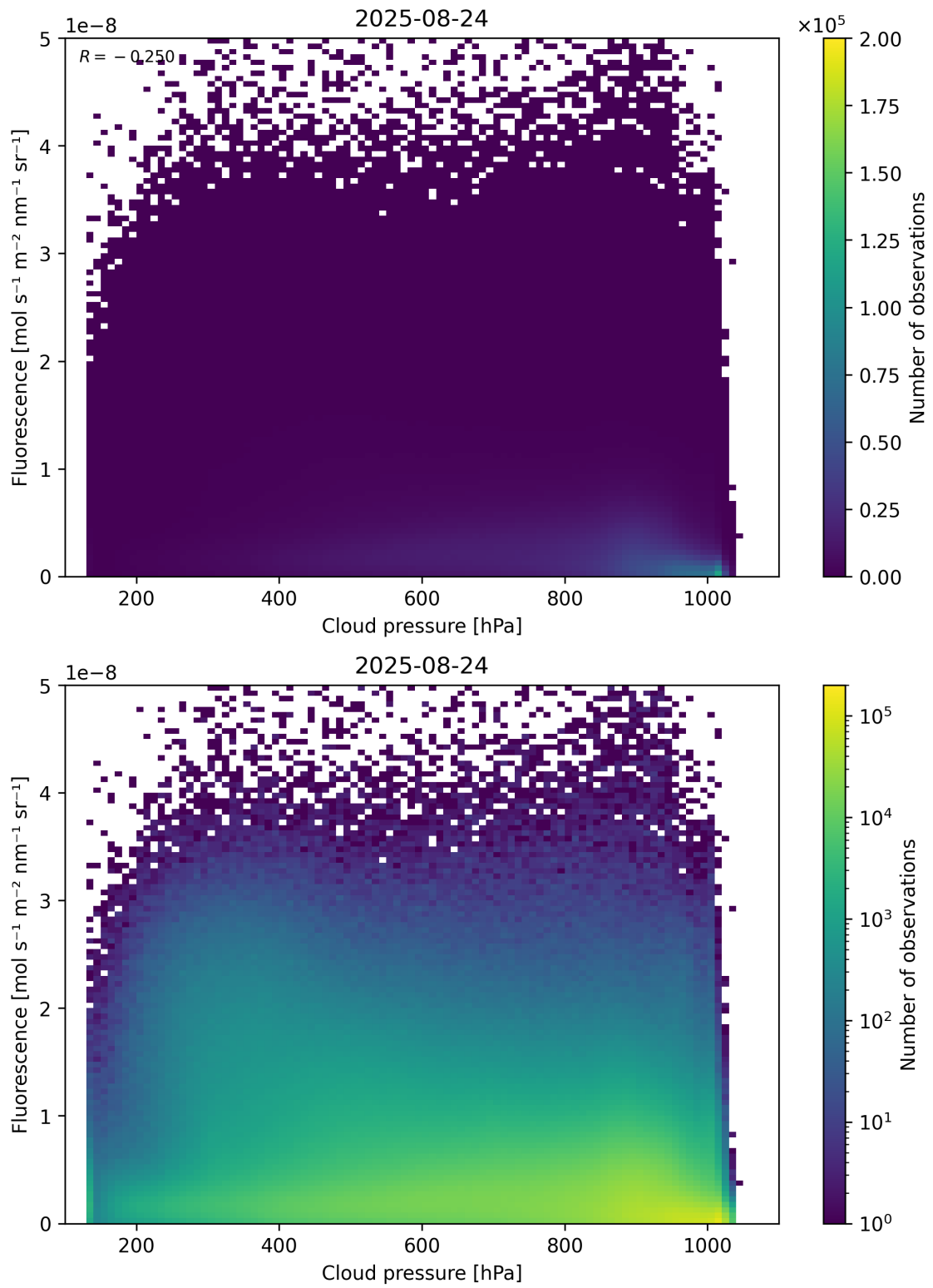
Figure 80: Scatter density plot of “Cloud pressure” against “Fluorescence” for 2025-08-23 to 2025-08-25.
