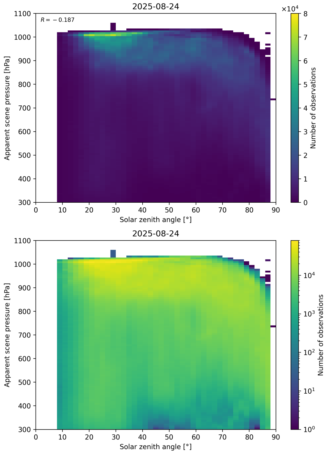
Figure 108: Scatter density plot of “Solar zenith angle” against “Apparent scene pressure” for 2025-08-23 to 2025-08-25.
