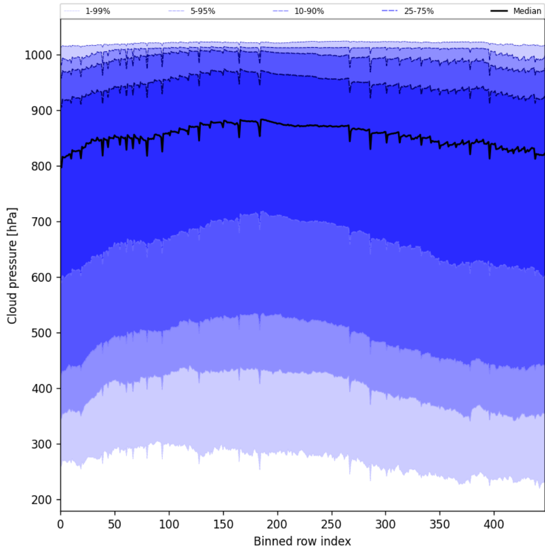
Figure 47: Along track statistics of “Cloud pressure” for 2025-08-23 to 2025-08-25
