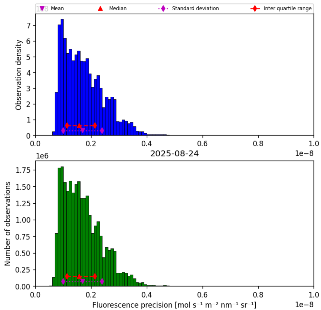
Figure 41: Histogram of “Fluorescence precision” for 2025-08-23 to 2025-08-25
