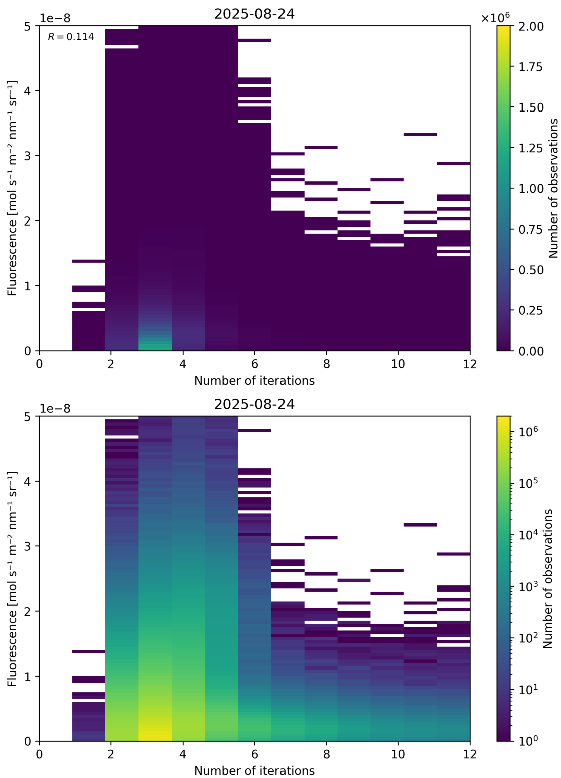
Figure 98: Scatter density plot of “Number of iterations” against “Fluorescence” for 2025-08-23 to 2025-08-25.
