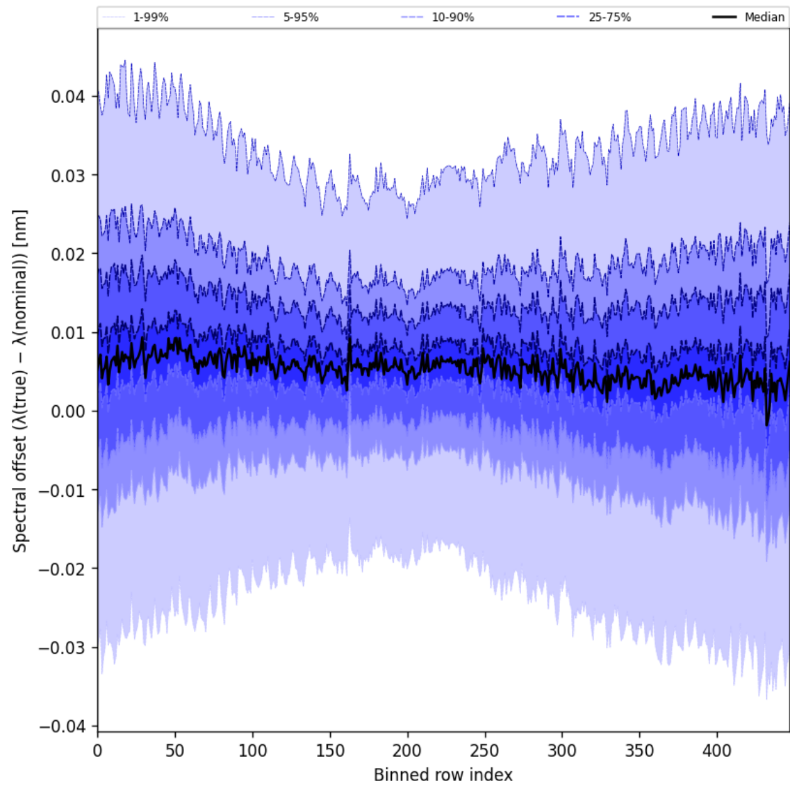
Figure 62: Along track statistics of “Spectral offset ( \lambda_{\text{true}} - \lambda_{\text{nominal}} )” for 2025-08-23 to 2025-08-25
