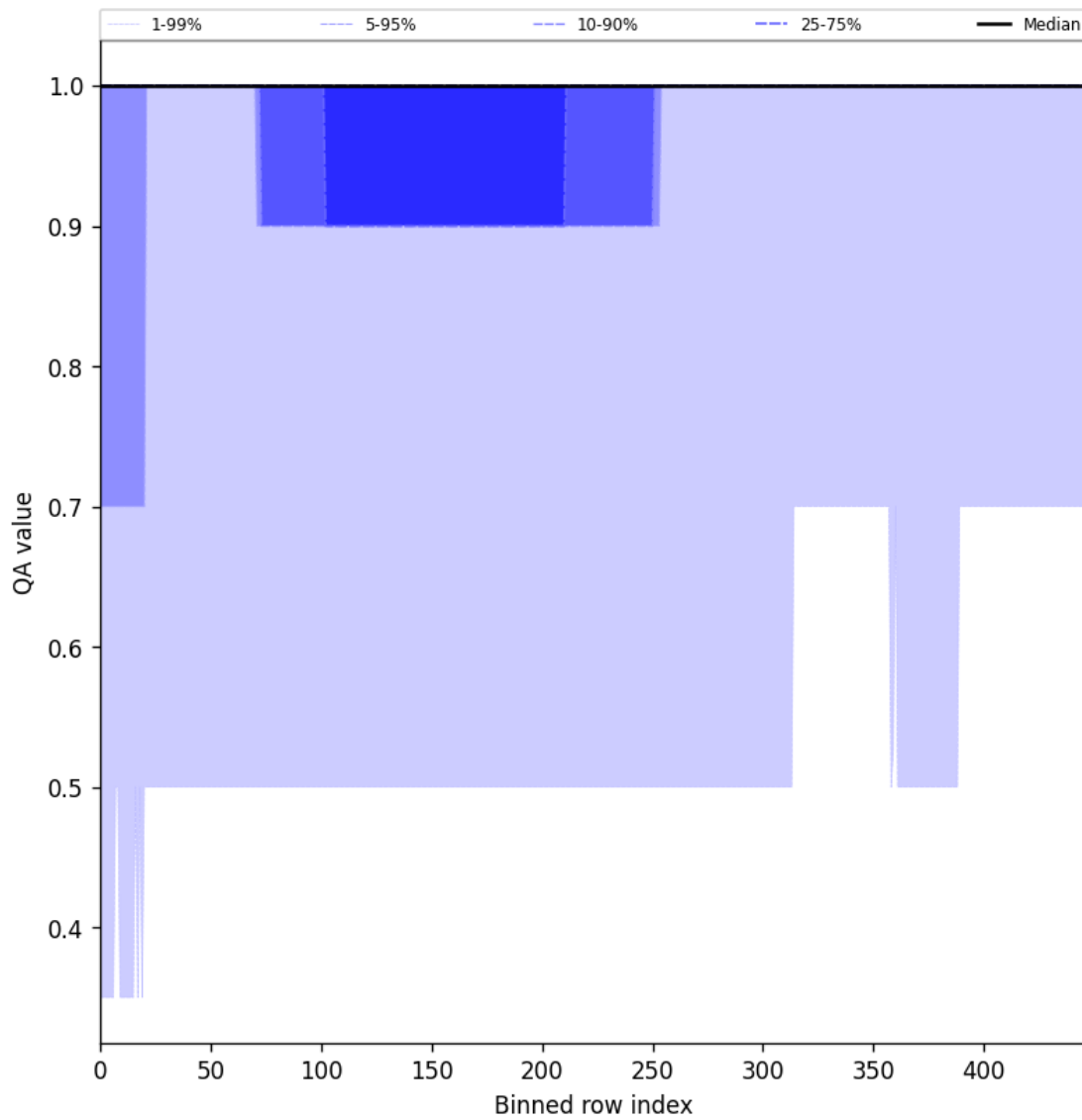
Figure 46: Along track statistics of “QA value” for 2025-08-23 to 2025-08-25
