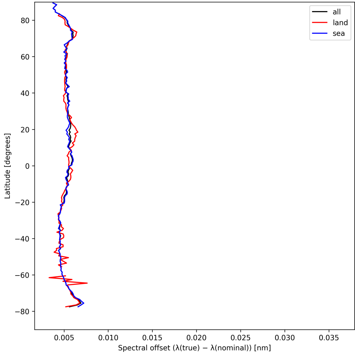
Figure 28: Zonal average of “Spectral offset ( \lambda_{\text{true}} - \lambda_{\text{nominal}} )” for 2025-08-23 to 2025-08-25.
