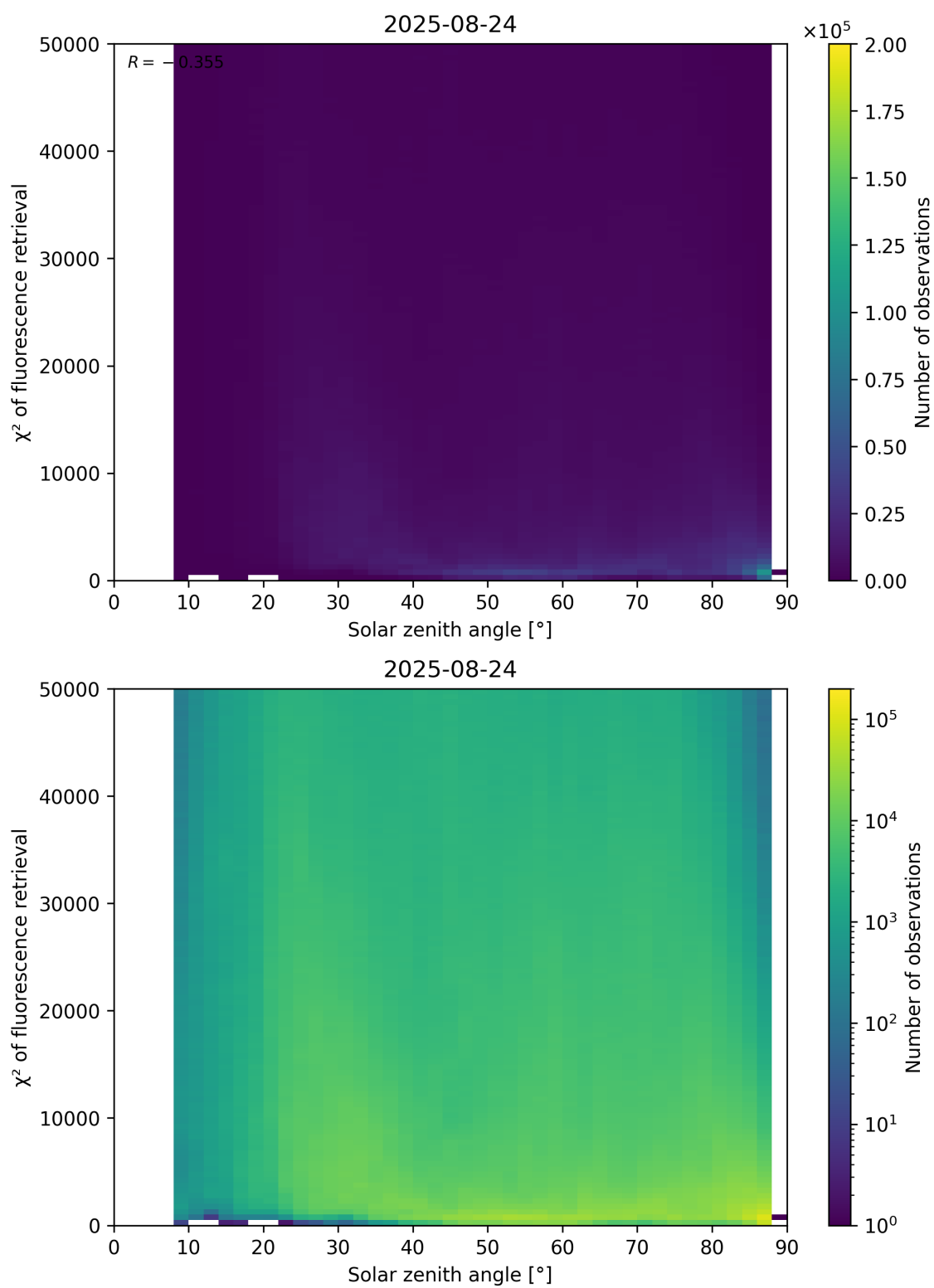
Figure 109: Scatter density plot of “Solar zenith angle” against “ \chi^2 of fluorescence retrieval” for 2025-08-23 to 2025-08-25.
