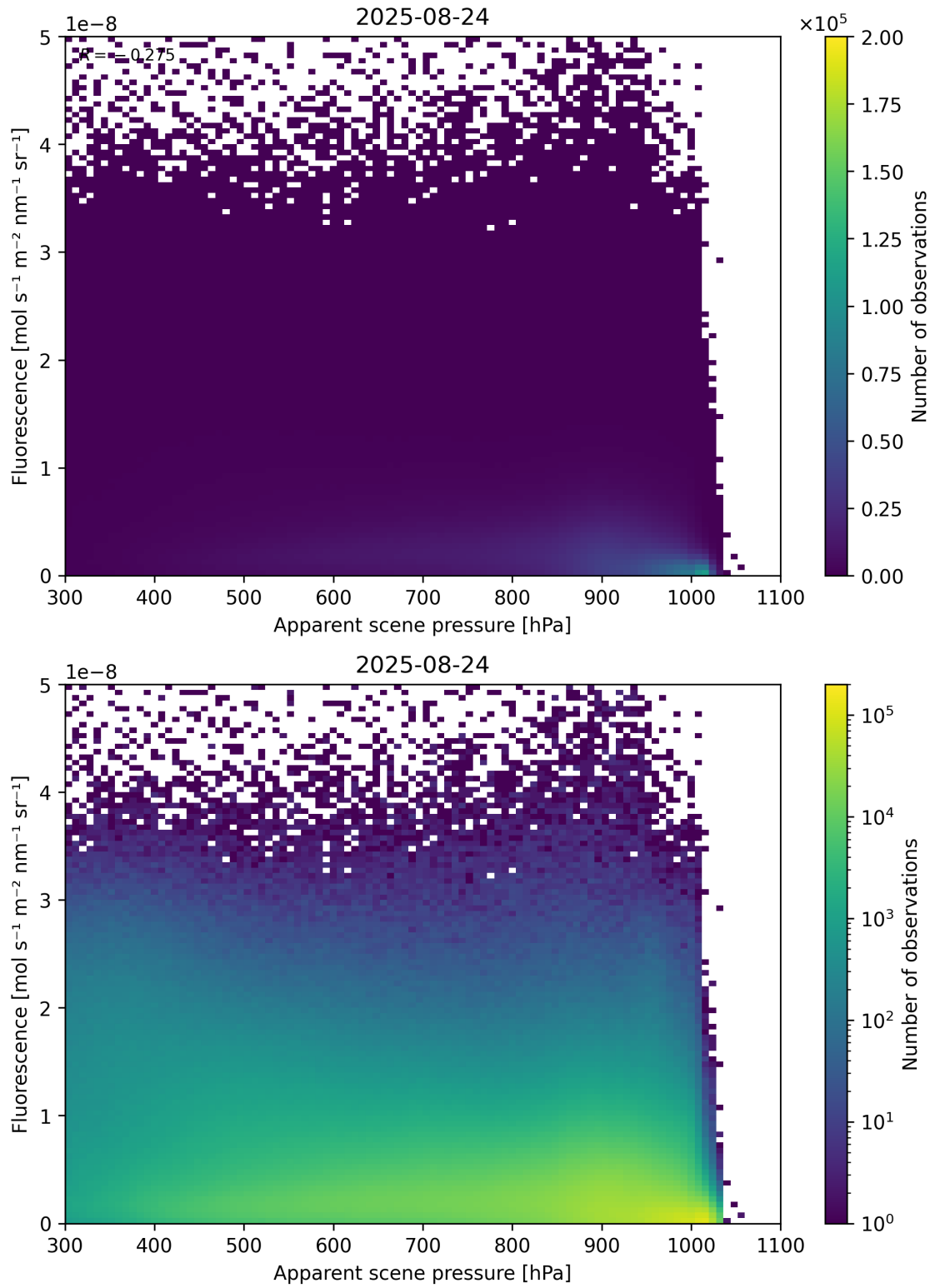
Figure 64: Scatter density plot of “Apparent scene pressure” against “Fluorescence” for 2025-08-23 to 2025-08-25.
