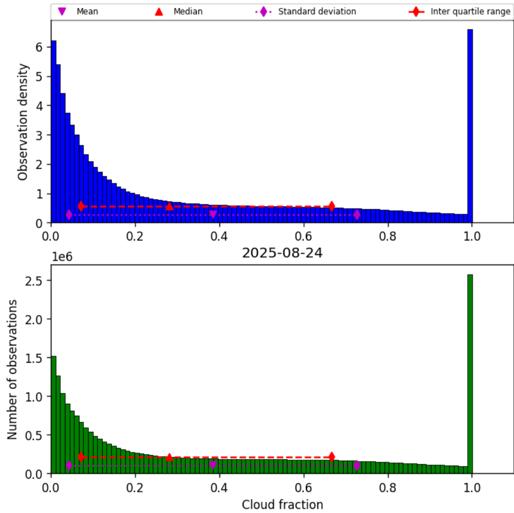
Figure 32: Histogram of “Cloud fraction” for 2025-08-23 to 2025-08-25
