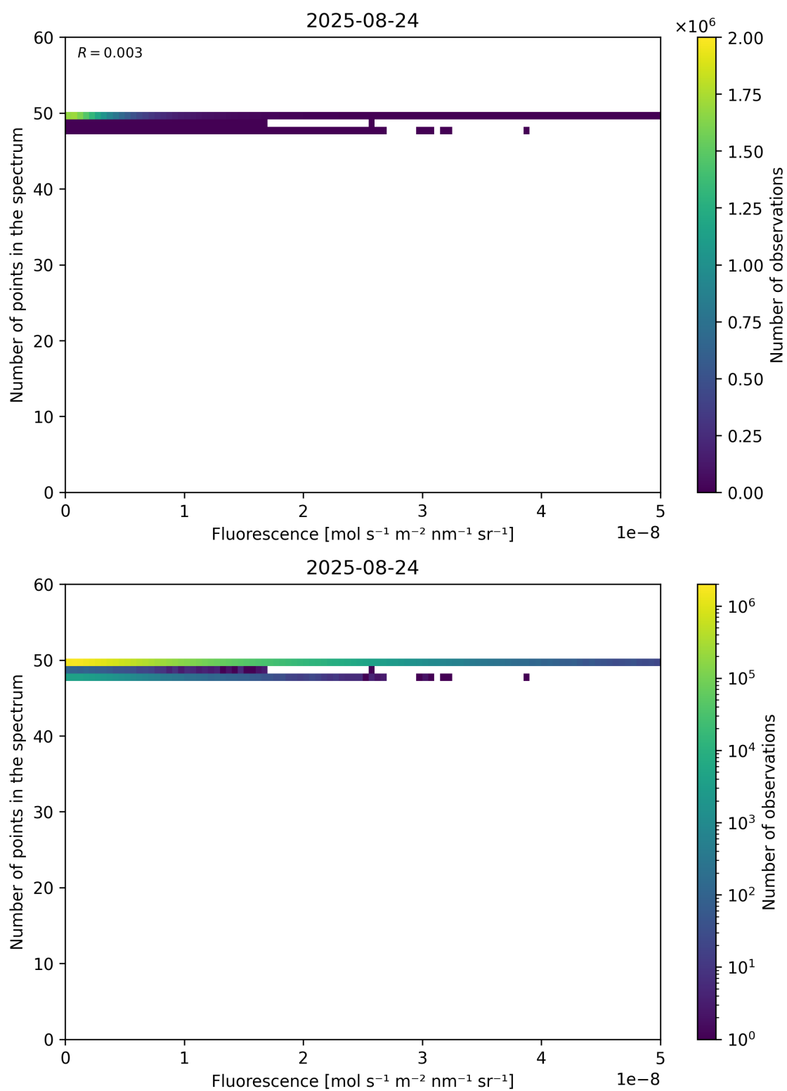
Figure 86: Scatter density plot of “Fluorescence” against “Number of points in the spectrum” for 2025-08-23 to 2025-08-25.
