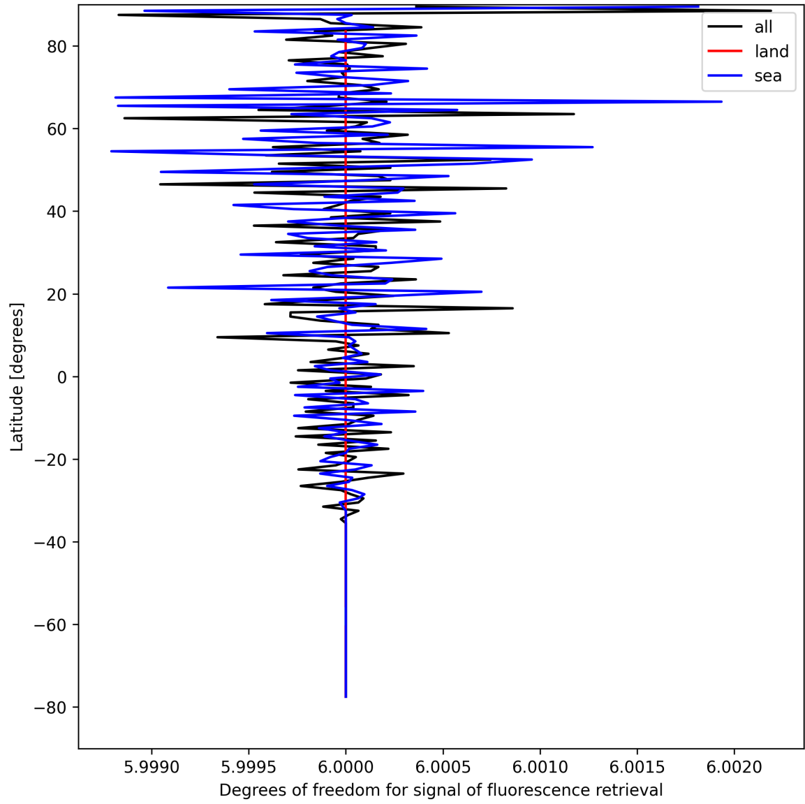
Figure 26: Zonal average of “Degrees of freedom for signal of fluorescence retrieval” for 2025-08-23 to 2025-08-25.
