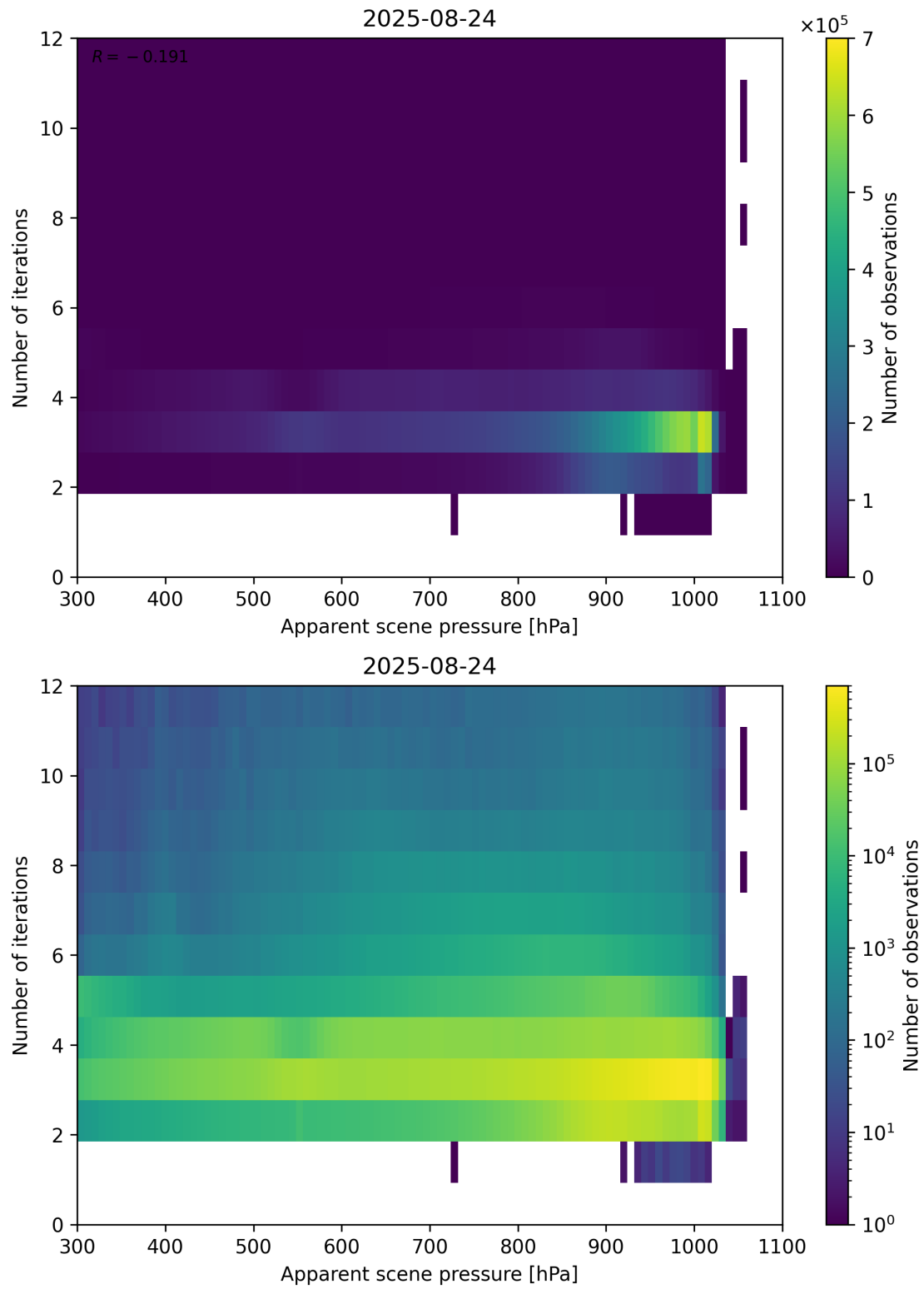
Figure 65: Scatter density plot of “Apparent scene pressure” against “Number of iterations” for 2025-08-23 to 2025-08-25.
