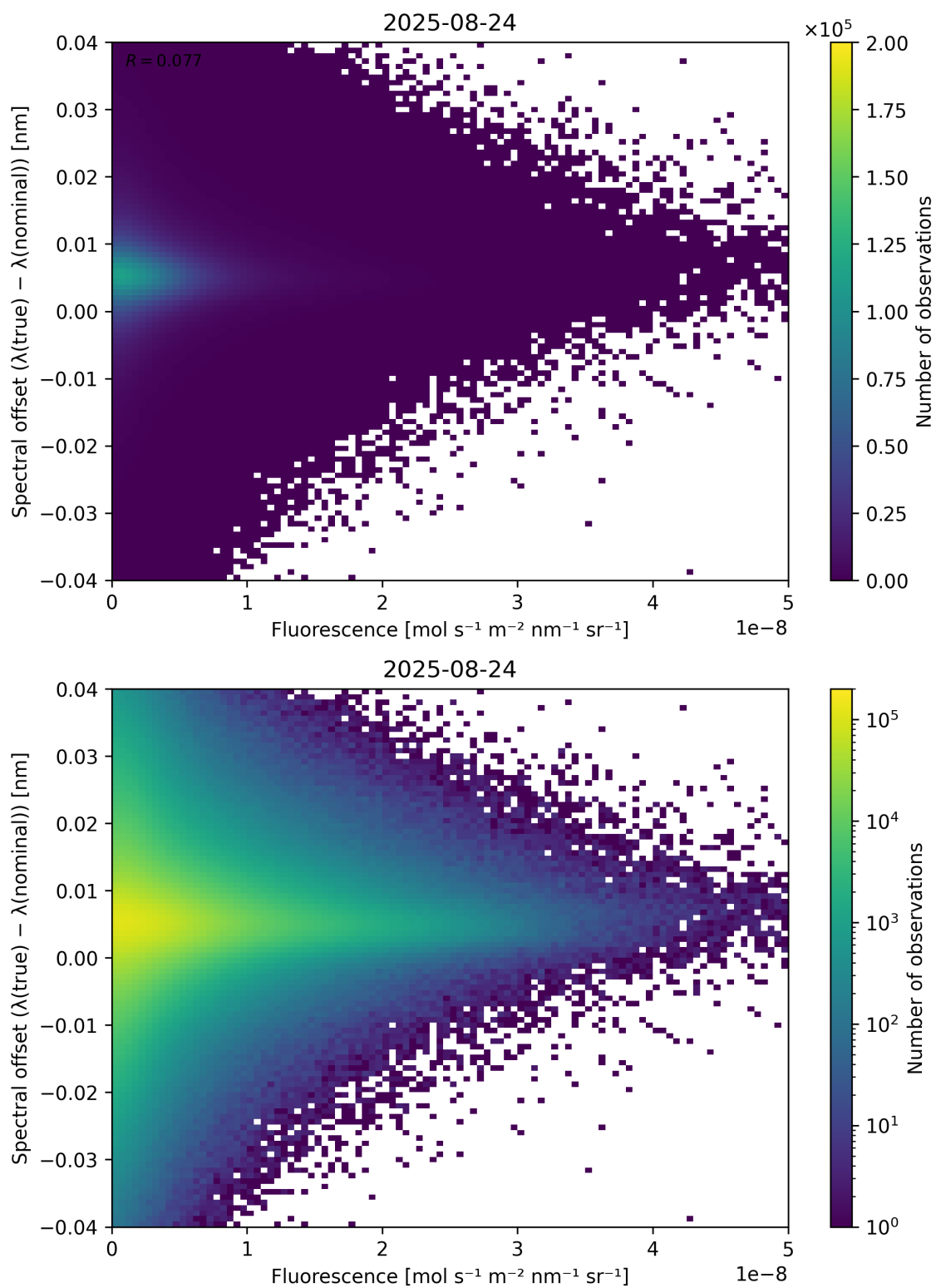
Figure 87: Scatter density plot of “Fluorescence” against “Spectral offset ( \lambda_{\text{true}} - \lambda_{\text{nominal}} )” for 2025-08-23 to 2025-08-25.
