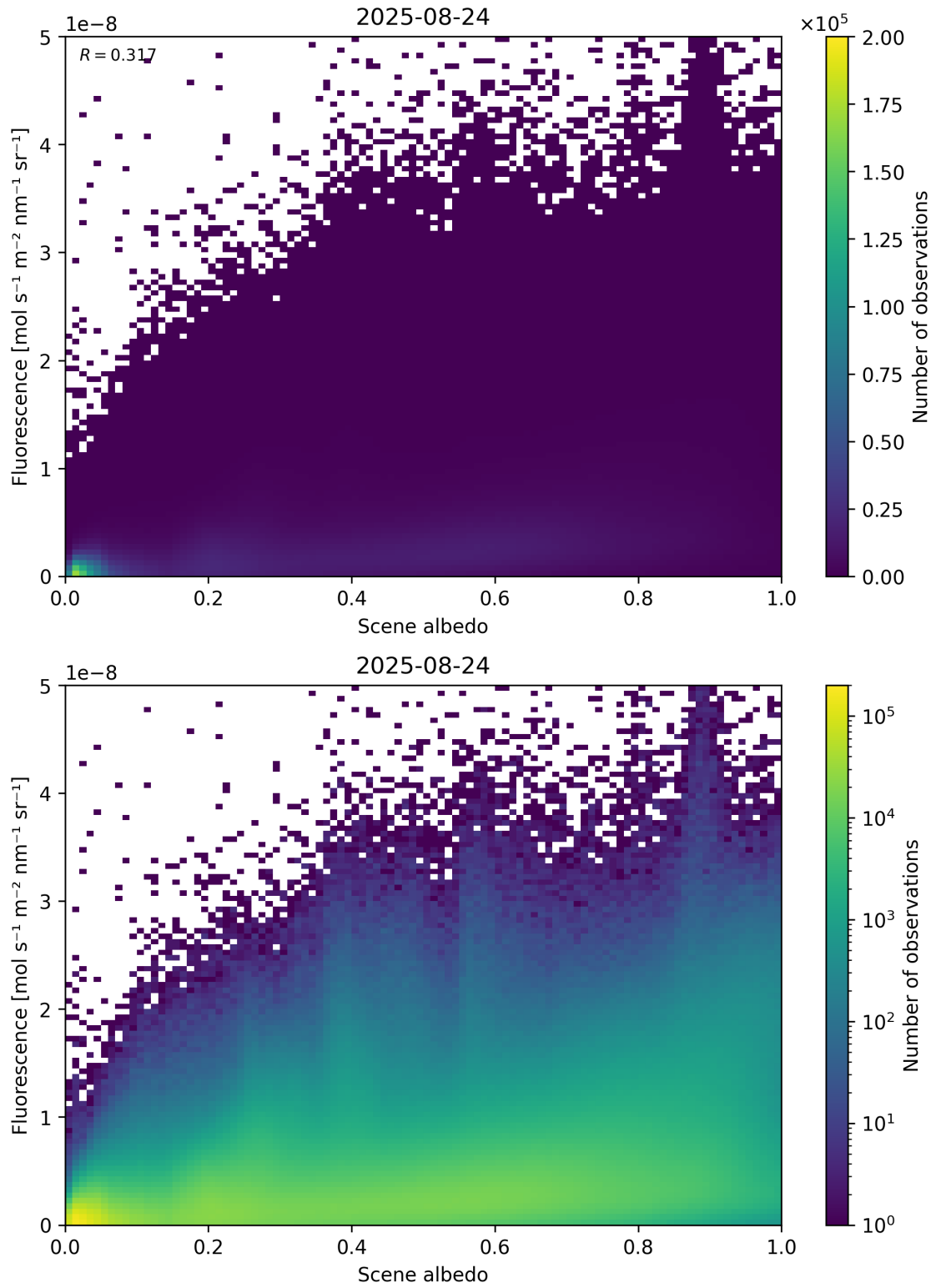
Figure 104: Scatter density plot of “Scene albedo” against “Fluorescence” for 2025-08-23 to 2025-08-25.
