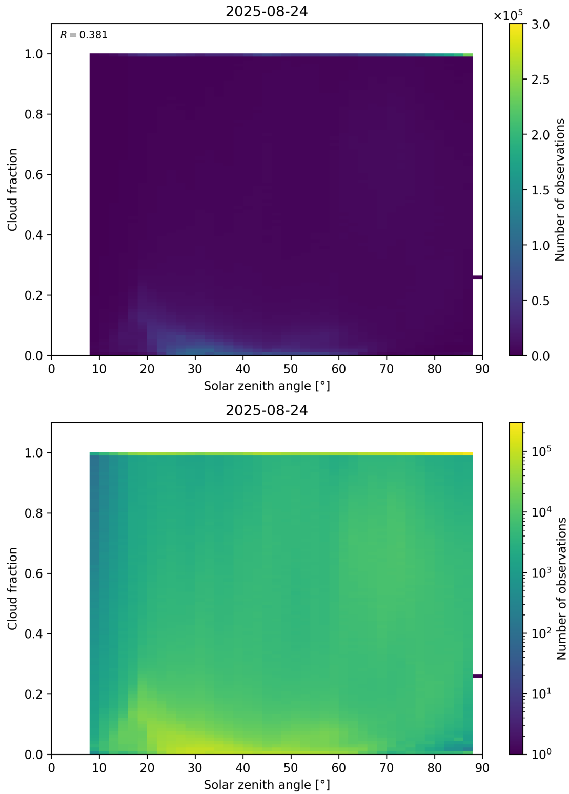
Figure 110: Scatter density plot of “Solar zenith angle” against “Cloud fraction” for 2025-08-23 to 2025-08-25.
