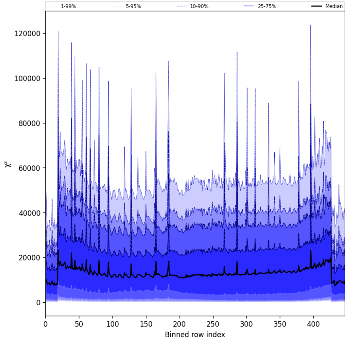
Figure 55: Along track statistics of “ \chi^2 ” for 2025-08-23 to 2025-08-25
