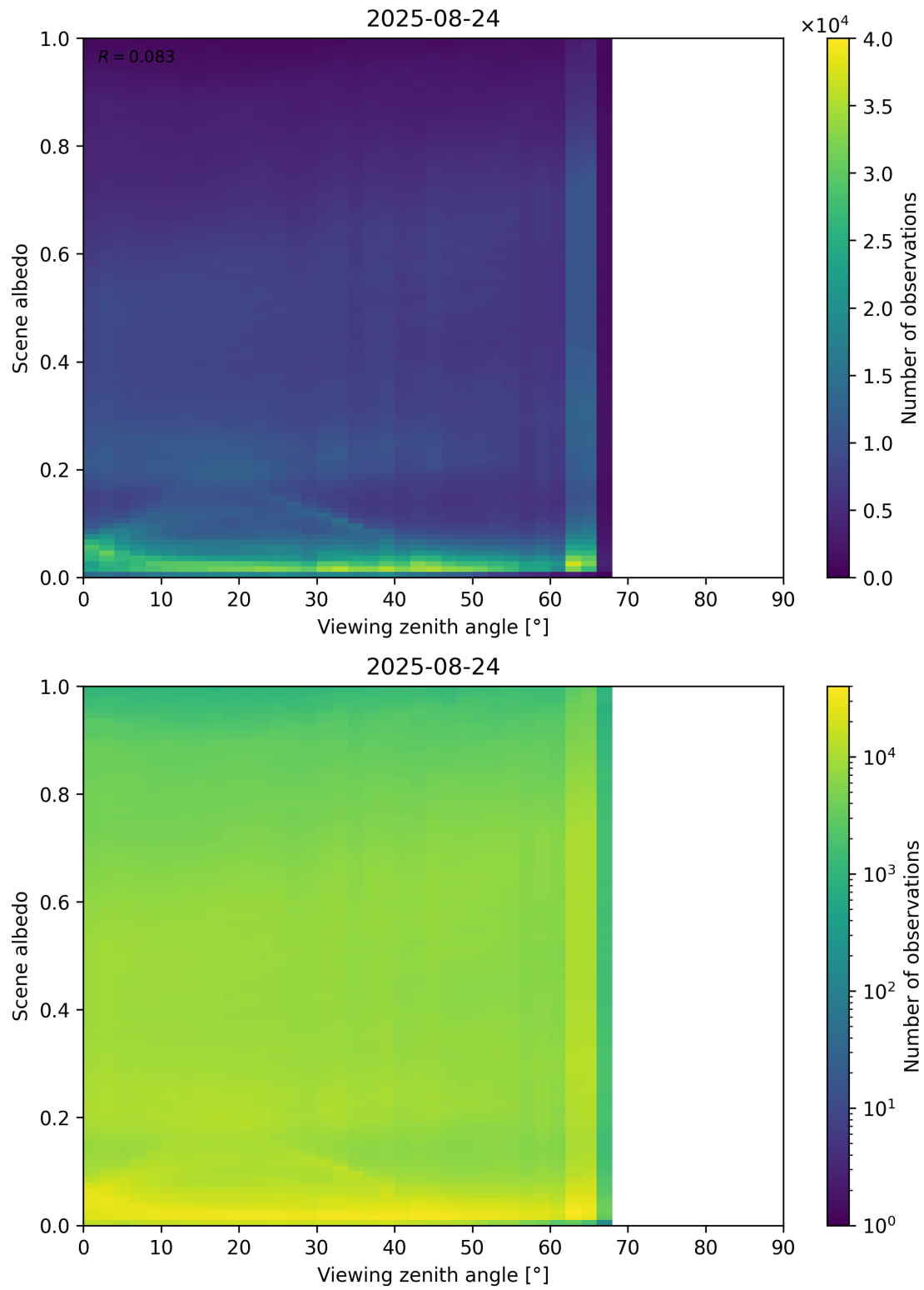
Figure 126: Scatter density plot of “Viewing zenith angle” against “Scene albedo” for 2025-08-23 to 2025-08-25.
