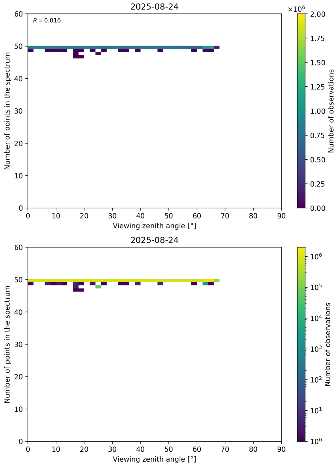
Figure 125: Scatter density plot of “Viewing zenith angle” against “Number of points in the spectrum” for 2025-08-23 to 2025-08-25.
