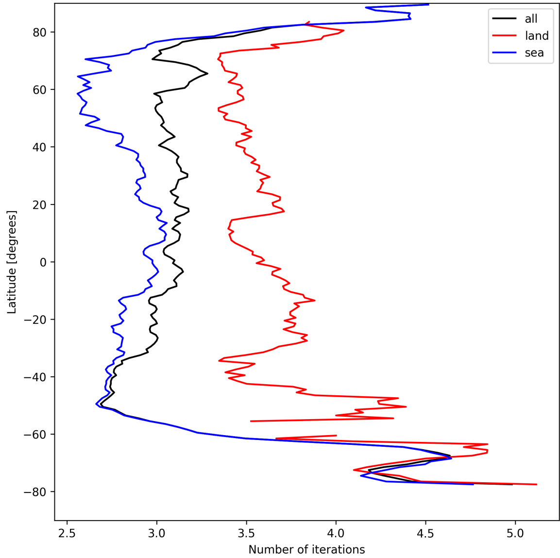
Figure 22: Zonal average of “Number of iterations” for 2025-08-23 to 2025-08-25.
