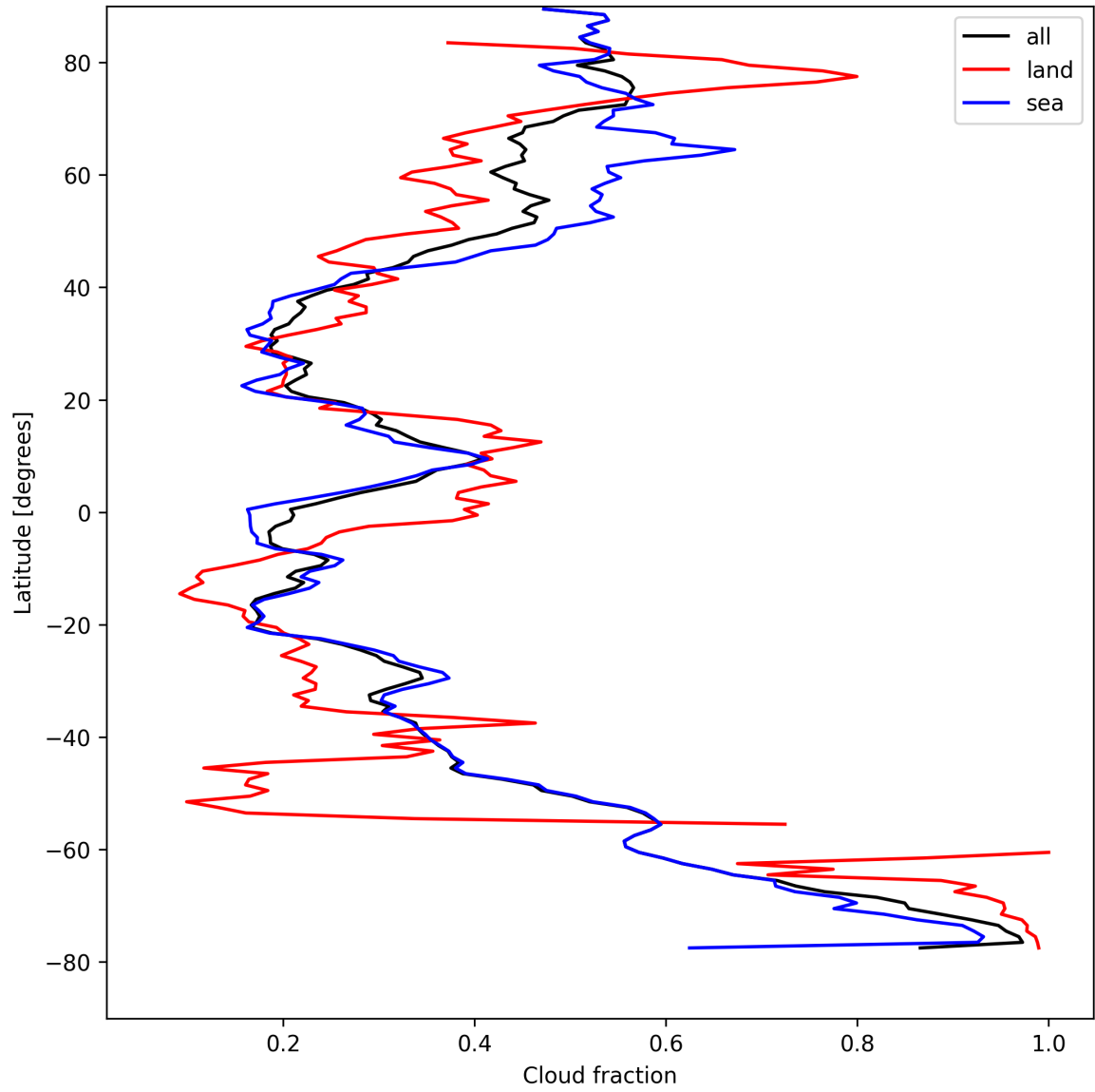
Figure 15: Zonal average of “Cloud fraction” for 2025-08-23 to 2025-08-25.
