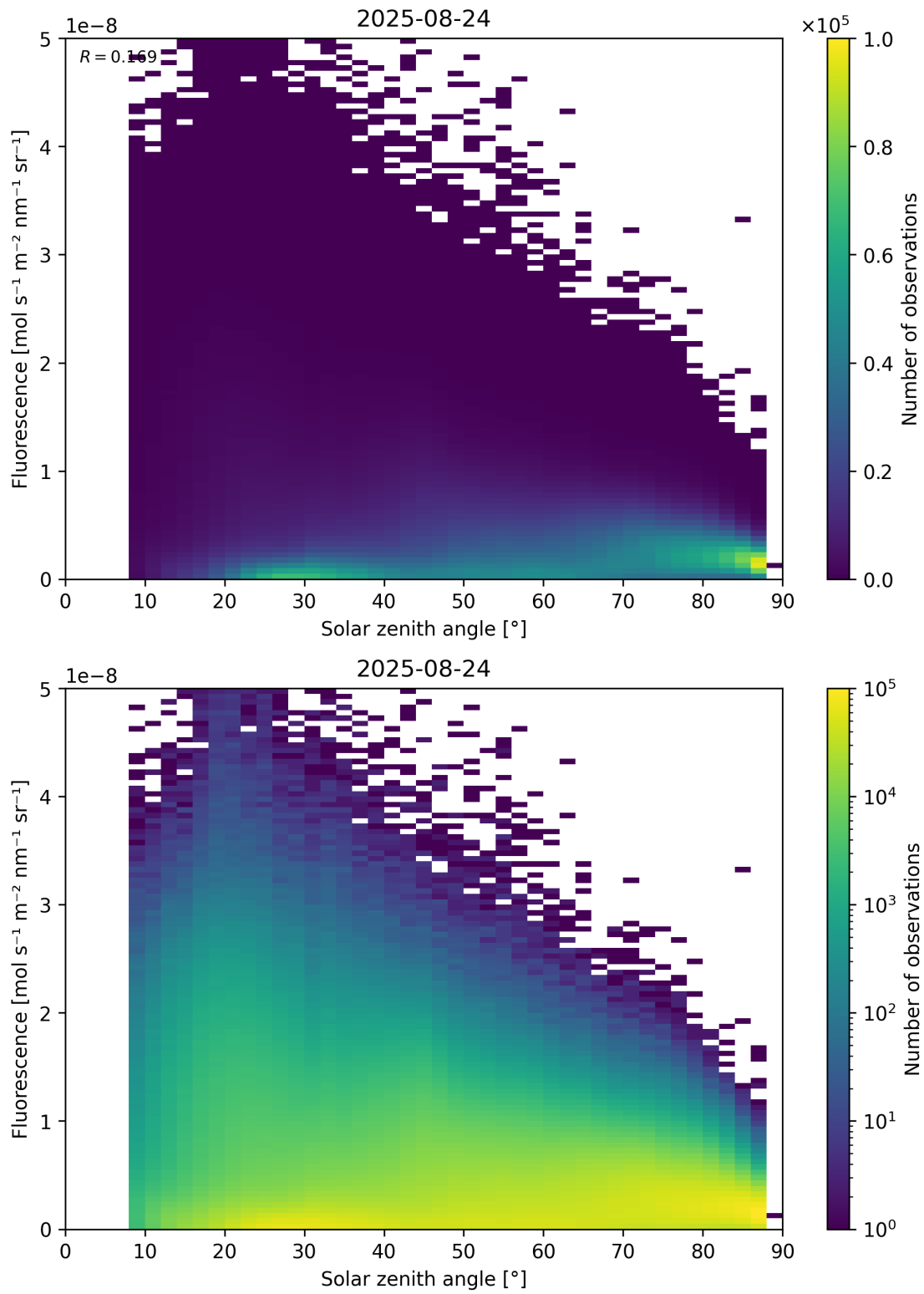
Figure 112: Scatter density plot of “Solar zenith angle” against “Fluorescence” for 2025-08-23 to 2025-08-25.
