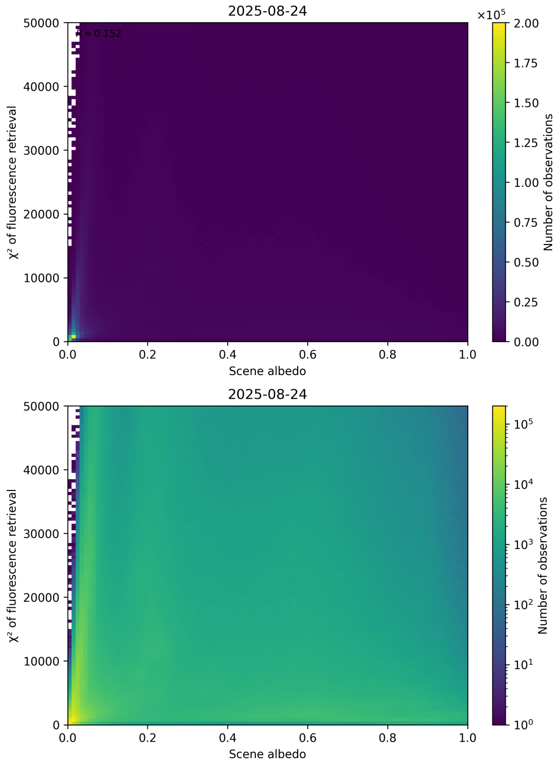
Figure 103: Scatter density plot of “Scene albedo” against “ \chi^2 of fluorescence retrieval” for 2025-08-23 to 2025-08-25.
