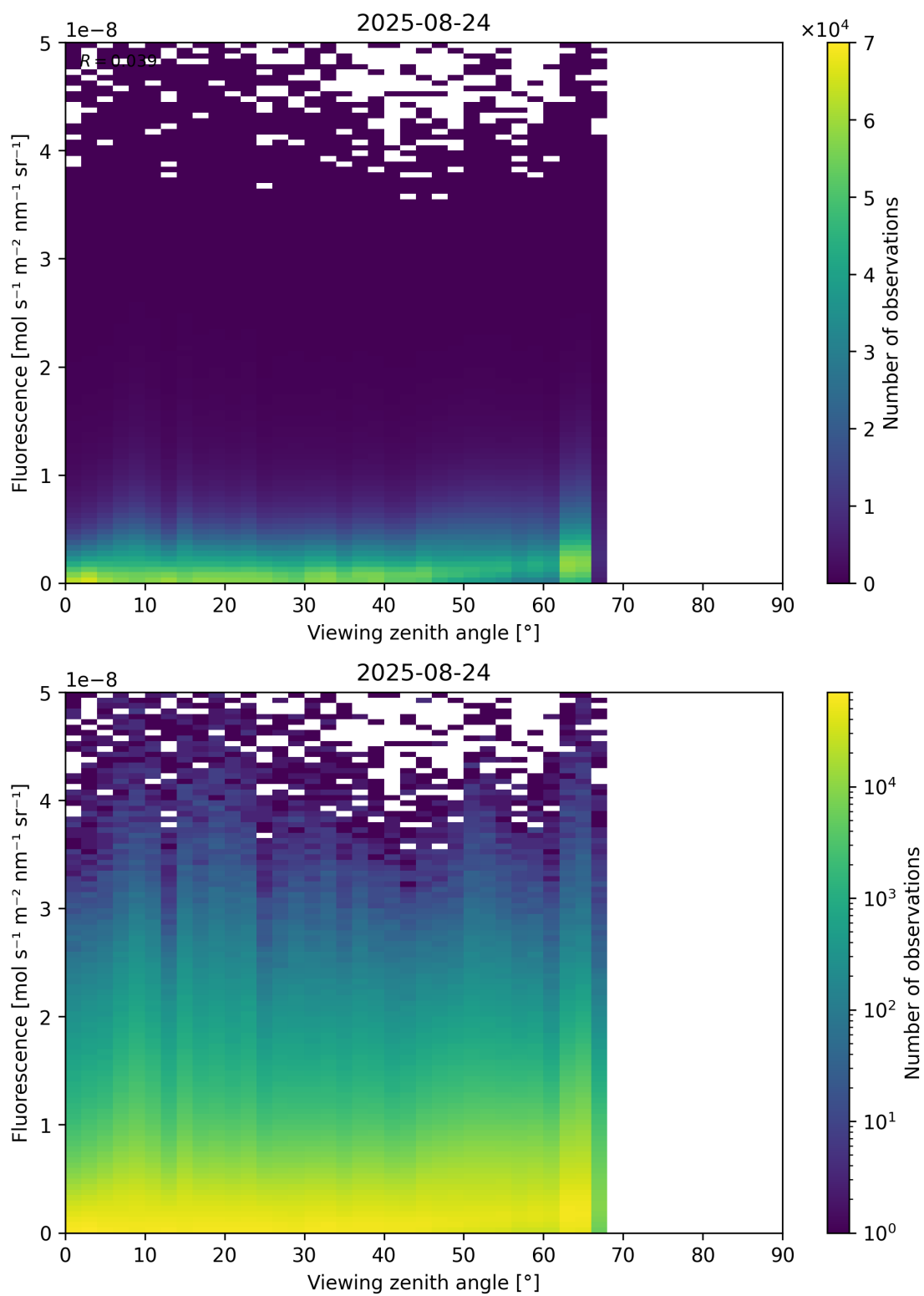
Figure 122: Scatter density plot of “Viewing zenith angle” against “Fluorescence” for 2025-08-23 to 2025-08-25.
