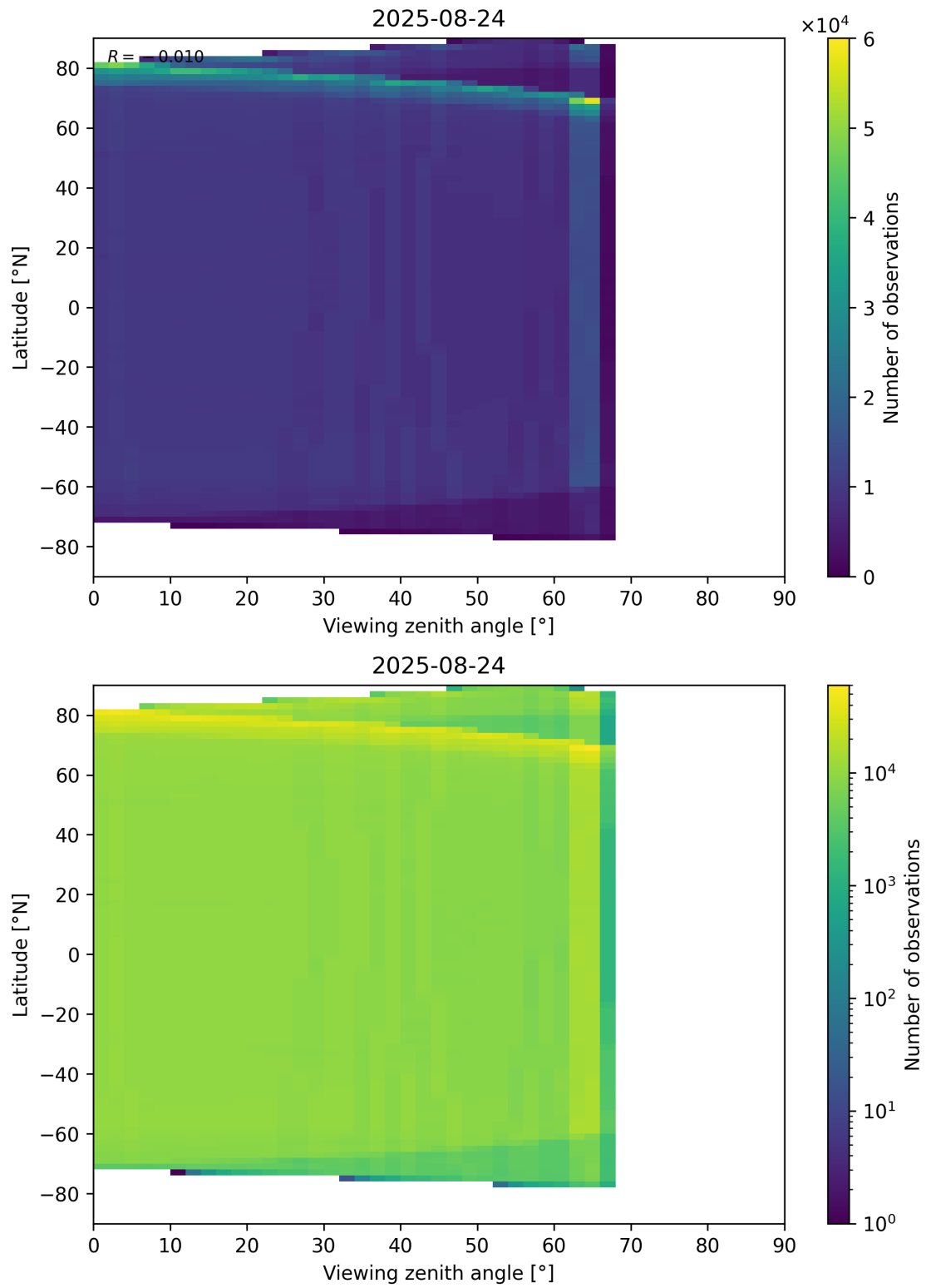
Figure 123: Scatter density plot of “Viewing zenith angle” against “Latitude” for 2025-08-23 to 2025-08-25.
