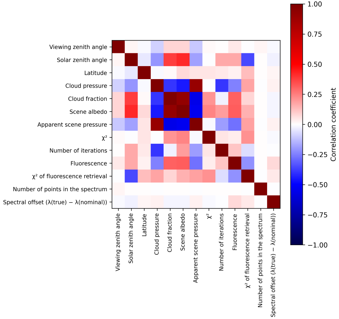
Figure 2: Map of correlation matrix for 2025-08-23 to 2025-08-25.
