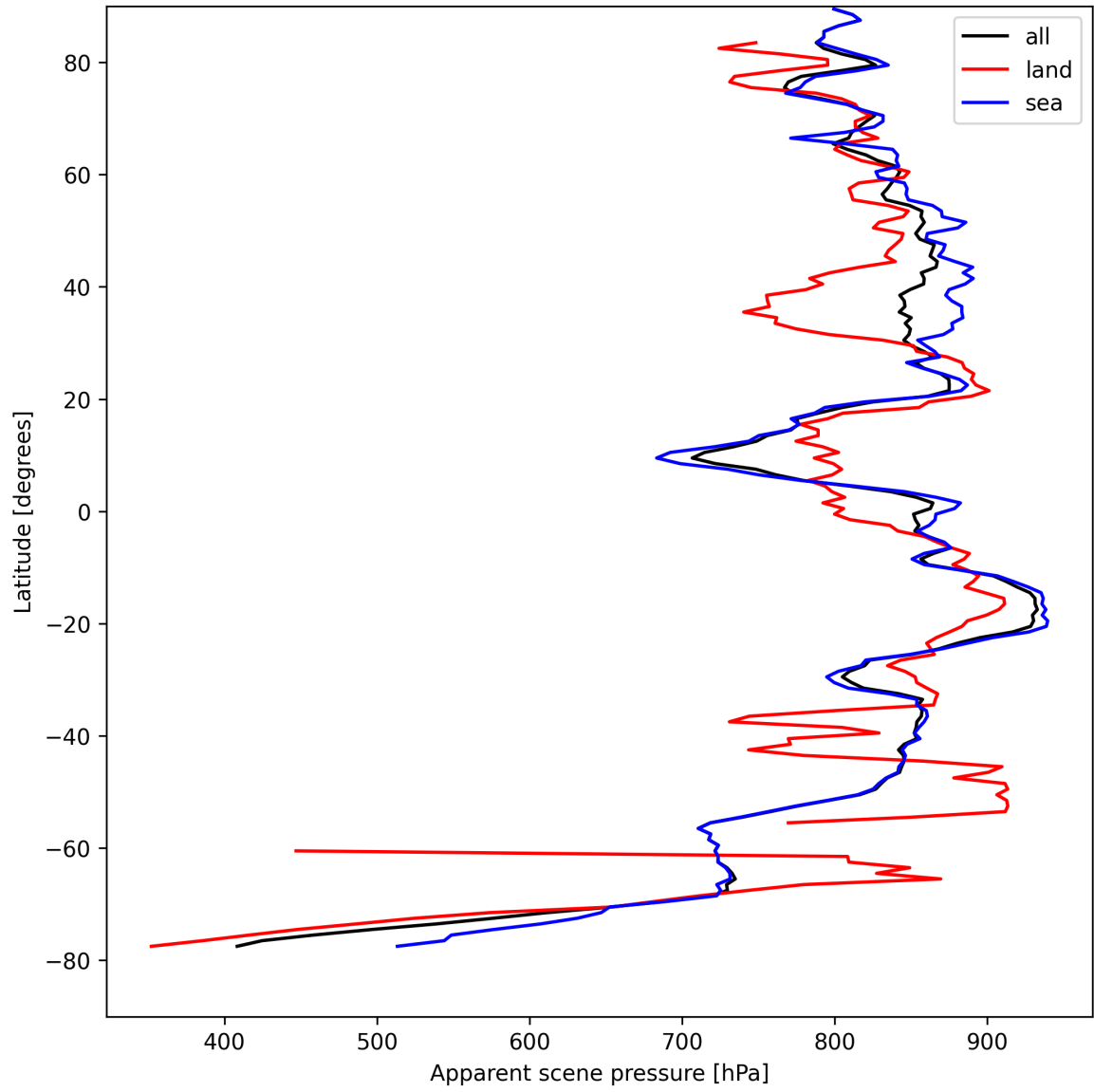
Figure 19: Zonal average of “Apparent scene pressure” for 2025-08-23 to 2025-08-25.
