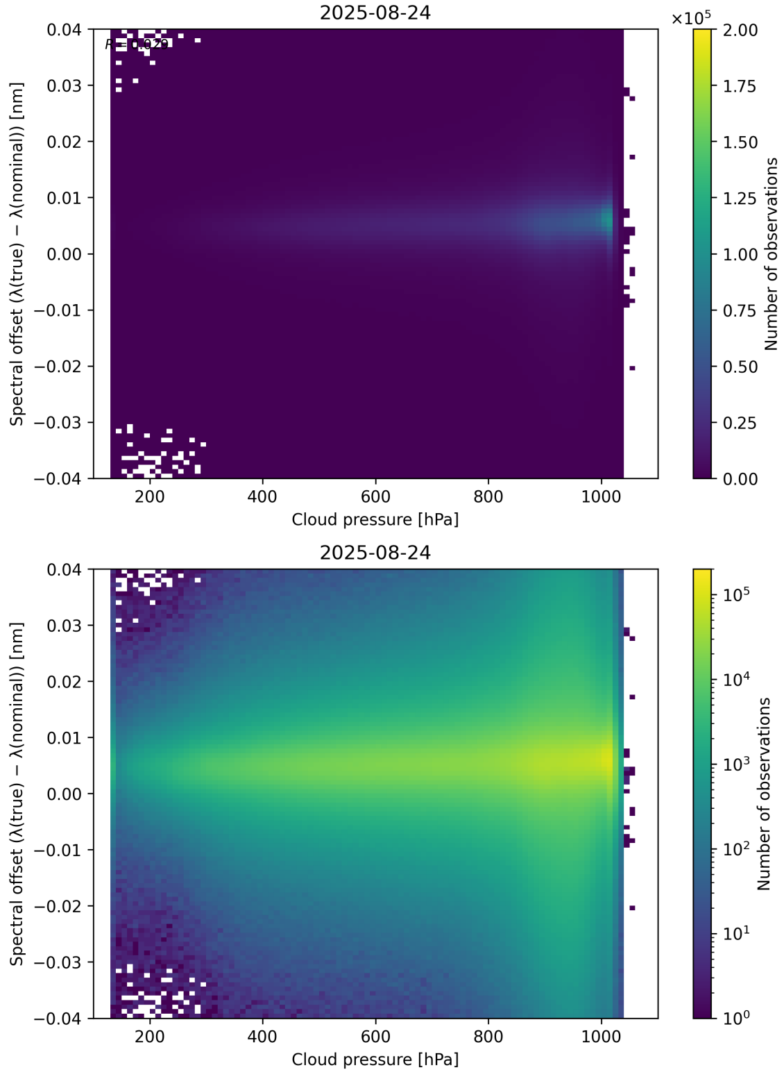
Figure 84: Scatter density plot of “Cloud pressure” against “Spectral offset ( \lambda_{\text{true}} - \lambda_{\text{nominal}} )” for 2025-08-23 to 2025-08-25.
