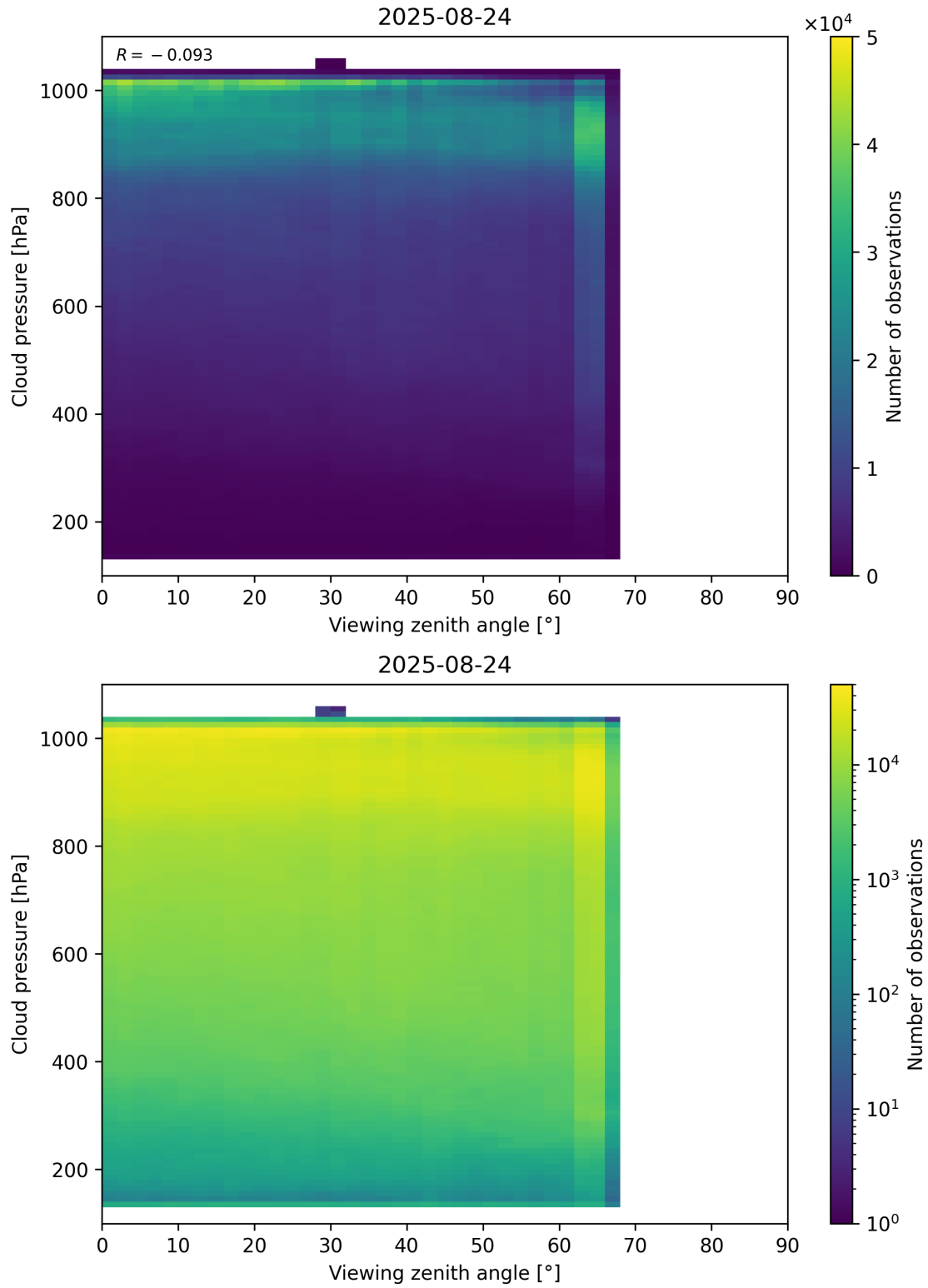
Figure 121: Scatter density plot of “Viewing zenith angle” against “Cloud pressure” for 2025-08-23 to 2025-08-25.
