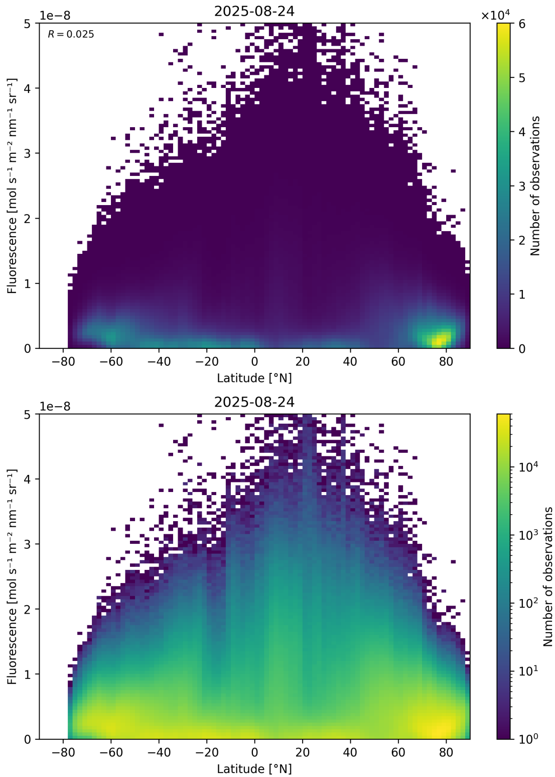
Figure 92: Scatter density plot of “Latitude” against “Fluorescence” for 2025-08-23 to 2025-08-25.
