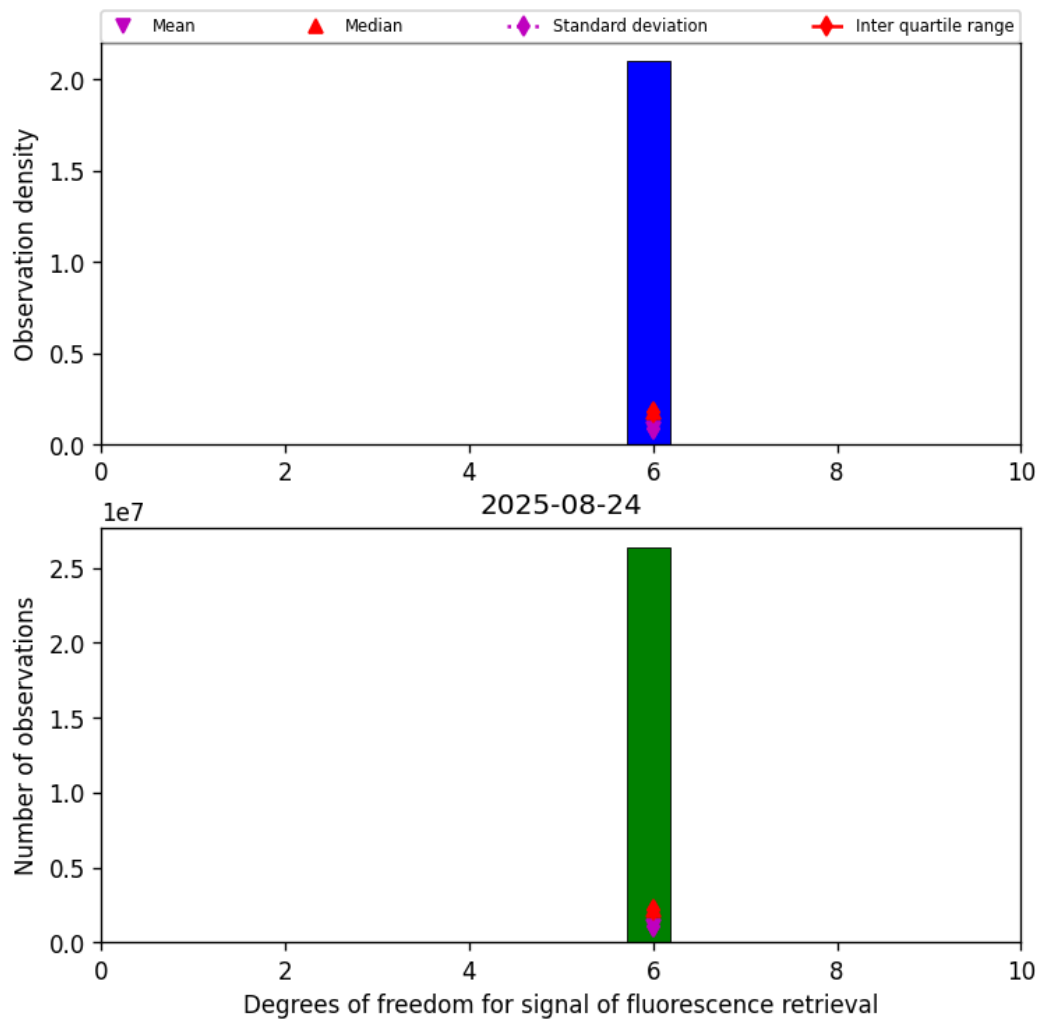
Figure 43: Histogram of "Degrees of freedom for signal of fluorescence retrieval" for 2025-08-23 to 2025-08-25
