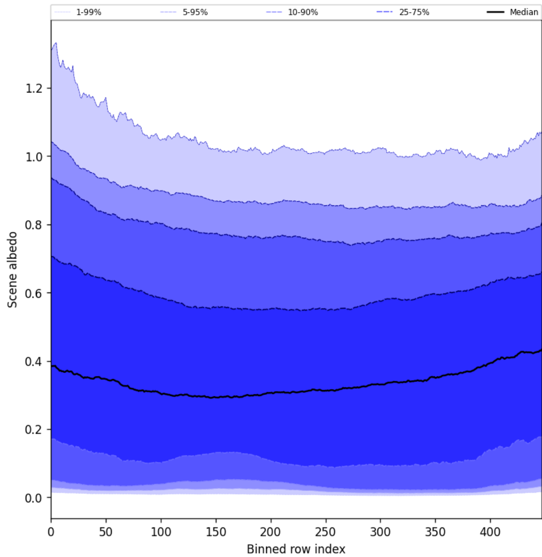
Figure 51: Along track statistics of “Scene albedo” for 2025-08-23 to 2025-08-25
