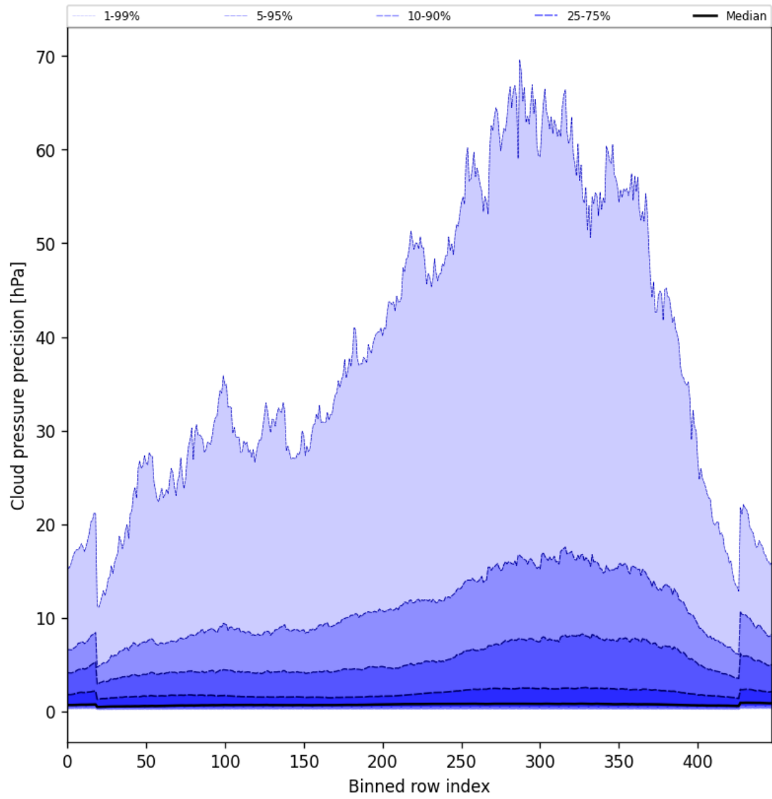
Figure 48: Along track statistics of “Cloud pressure precision” for 2025-08-23 to 2025-08-25
