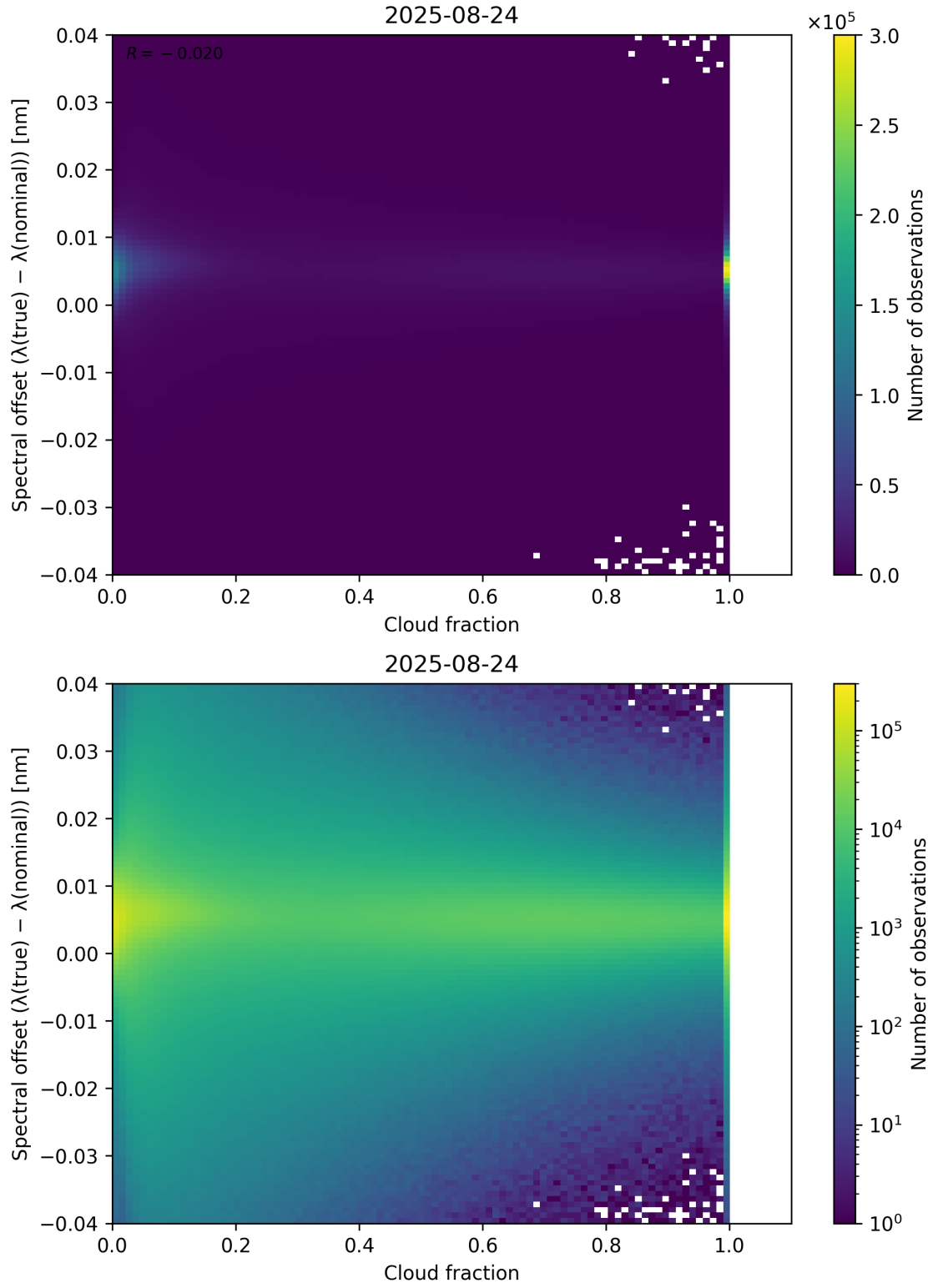
Figure 76: Scatter density plot of “Cloud fraction” against “Spectral offset ( \lambda_{\text{true}} - \lambda_{\text{nominal}} )” for 2025-08-23 to 2025-08-25.
