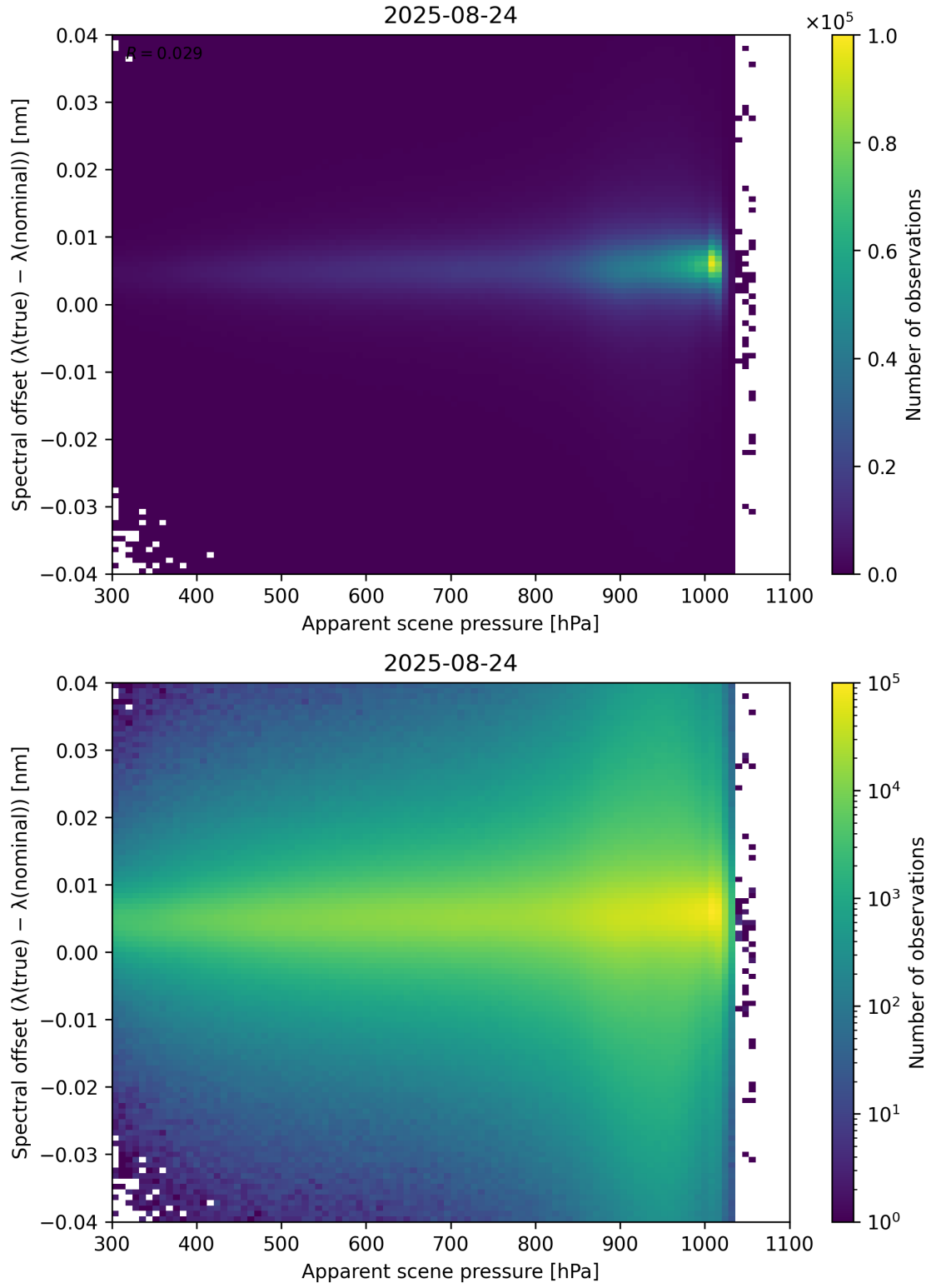
Figure 67: Scatter density plot of “Apparent scene pressure” against “Spectral offset ( \lambda_{\text{true}} - \lambda_{\text{nominal}} )” for 2025-08-23 to 2025-08-25.
