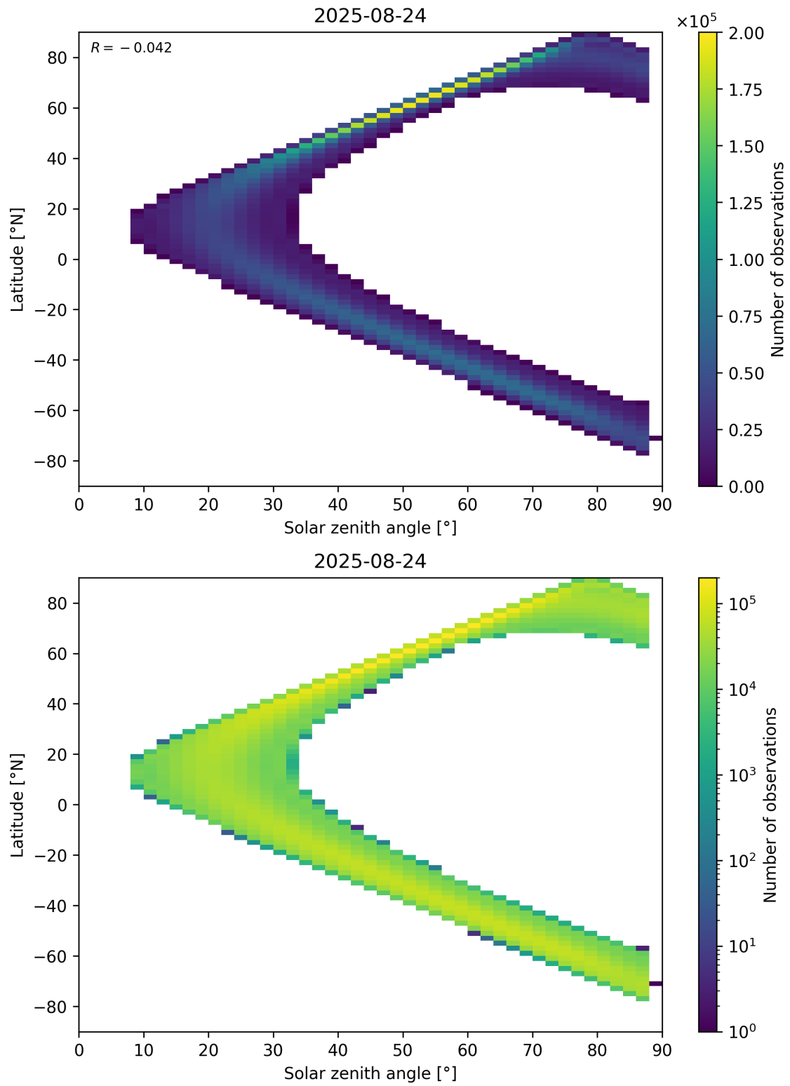
Figure 113: Scatter density plot of “Solar zenith angle” against “Latitude” for 2025-08-23 to 2025-08-25.
