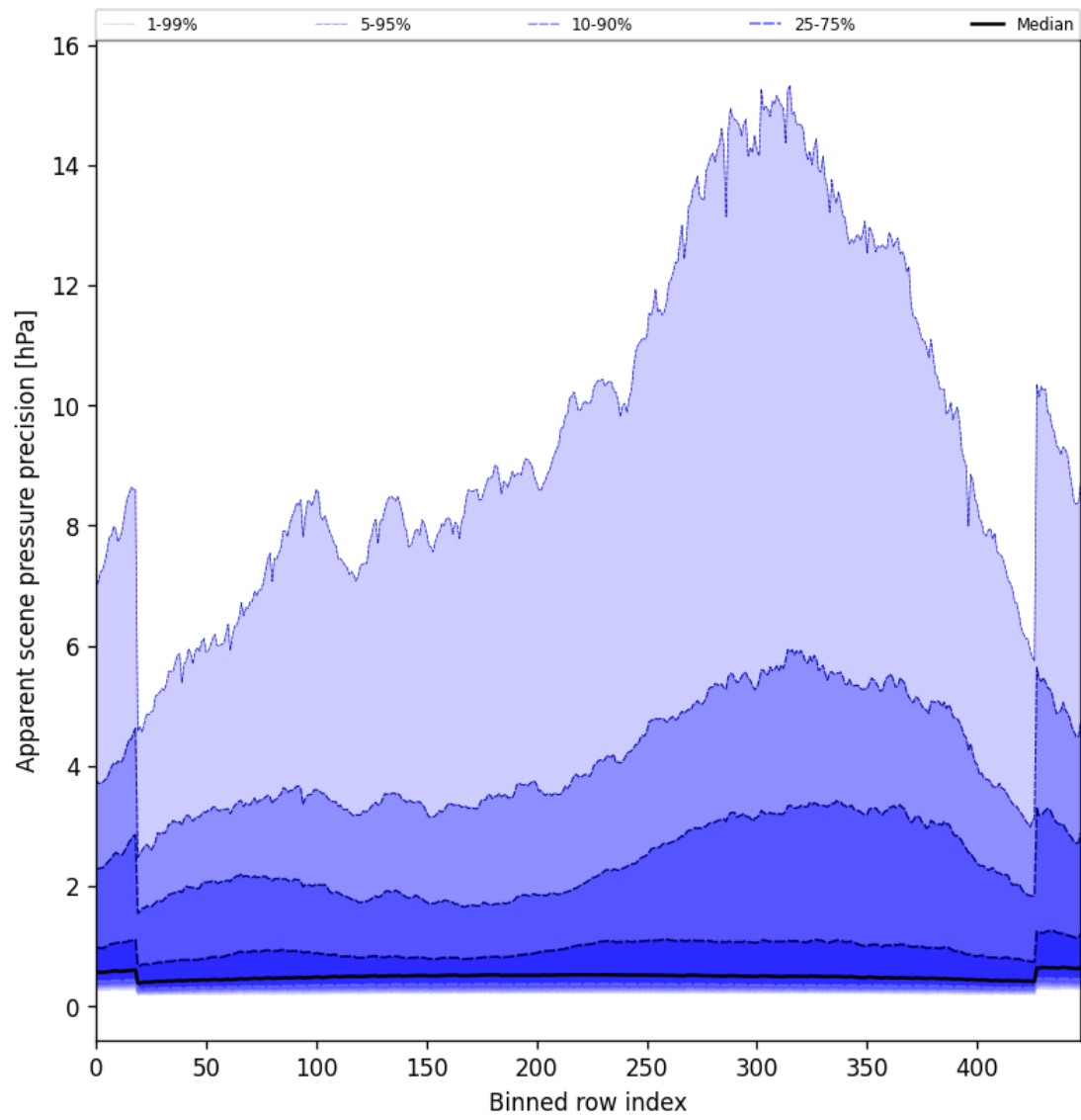
Figure 54: Along track statistics of “Apparent scene pressure precision” for 2025-08-23 to 2025-08-25
