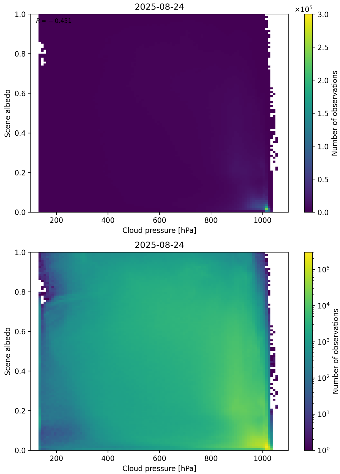
Figure 83: Scatter density plot of “Cloud pressure” against “Scene albedo” for 2025-08-23 to 2025-08-25.
