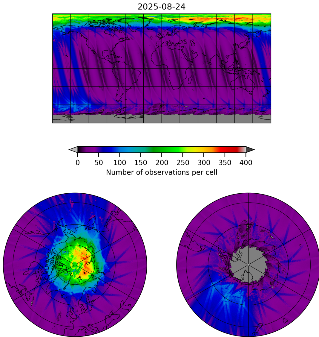
Figure 11: Map of the number of observations for 2025-08-23 to 2025-08-25
