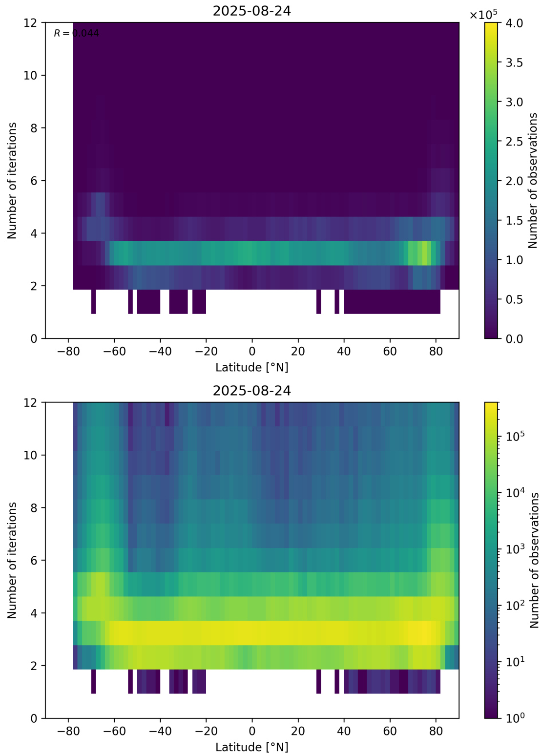
Figure 93: Scatter density plot of “Latitude” against “Number of iterations” for 2025-08-23 to 2025-08-25.
