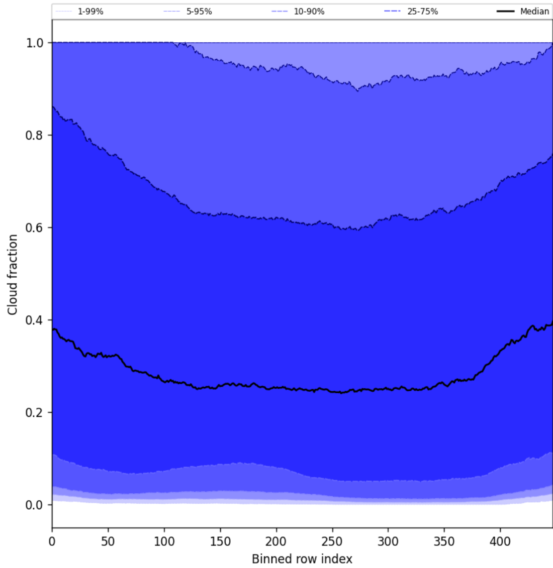
Figure 49: Along track statistics of “Cloud fraction” for 2025-08-23 to 2025-08-25
