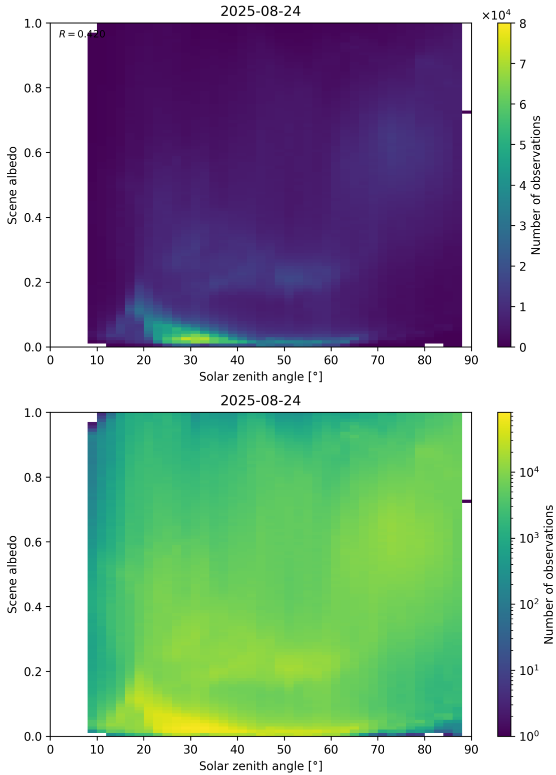
Figure 116: Scatter density plot of “Solar zenith angle” against “Scene albedo” for 2025-08-23 to 2025-08-25.
