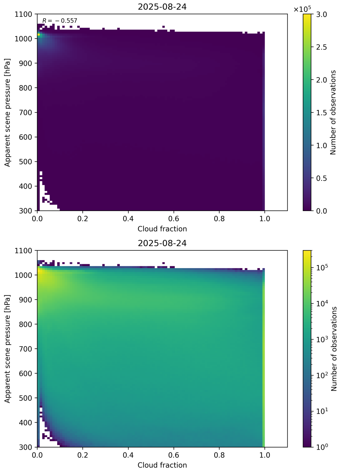
Figure 70: Scatter density plot of “Cloud fraction” against “Apparent scene pressure” for 2025-08-23 to 2025-08-25.
