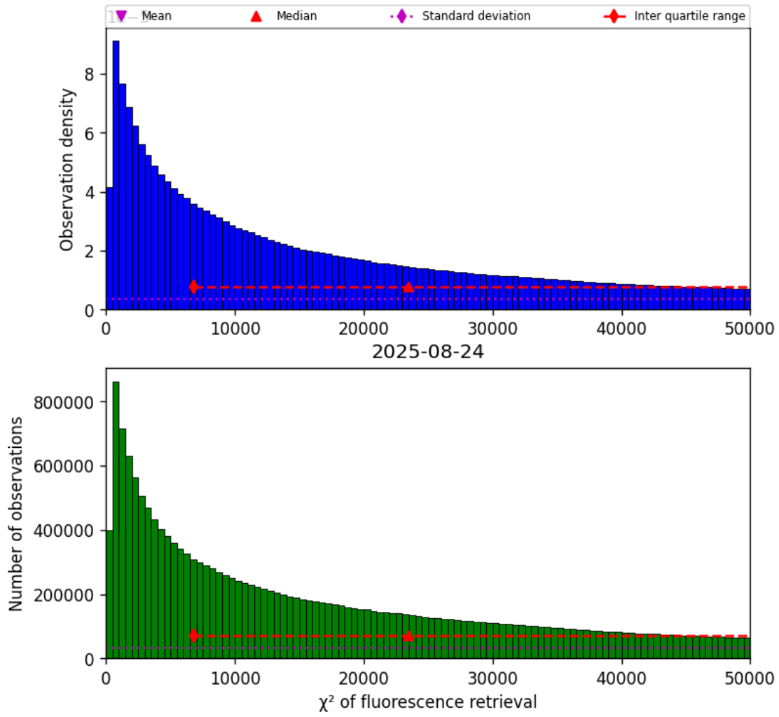
Figure 42: Histogram of “ \chi^2 of fluorescence retrieval” for 2025-08-23 to 2025-08-25
