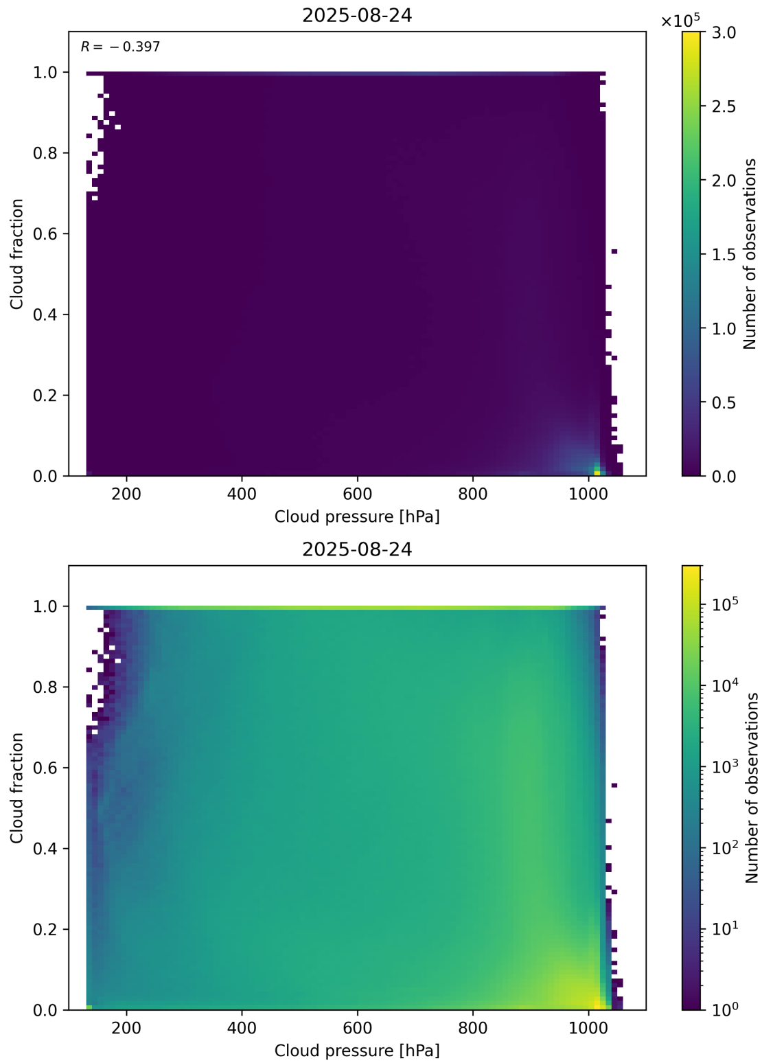
Figure 79: Scatter density plot of “Cloud pressure” against “Cloud fraction” for 2025-08-23 to 2025-08-25.
