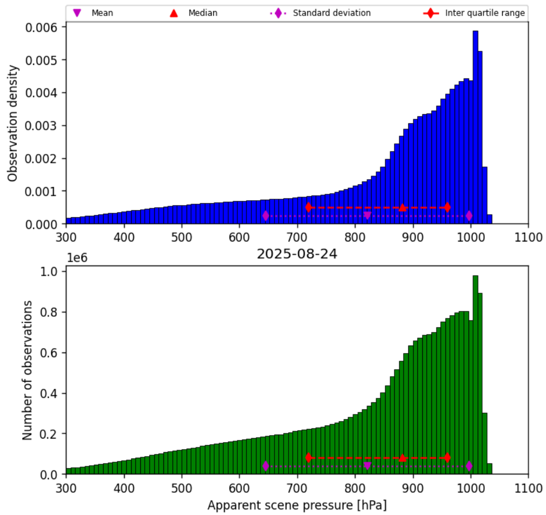
Figure 36: Histogram of “Apparent scene pressure” for 2025-08-23 to 2025-08-25
