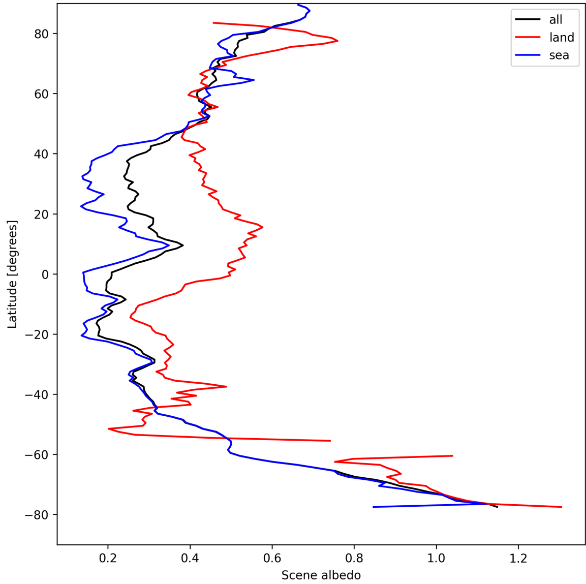
Figure 17: Zonal average of “Scene albedo” for 2025-08-23 to 2025-08-25.
