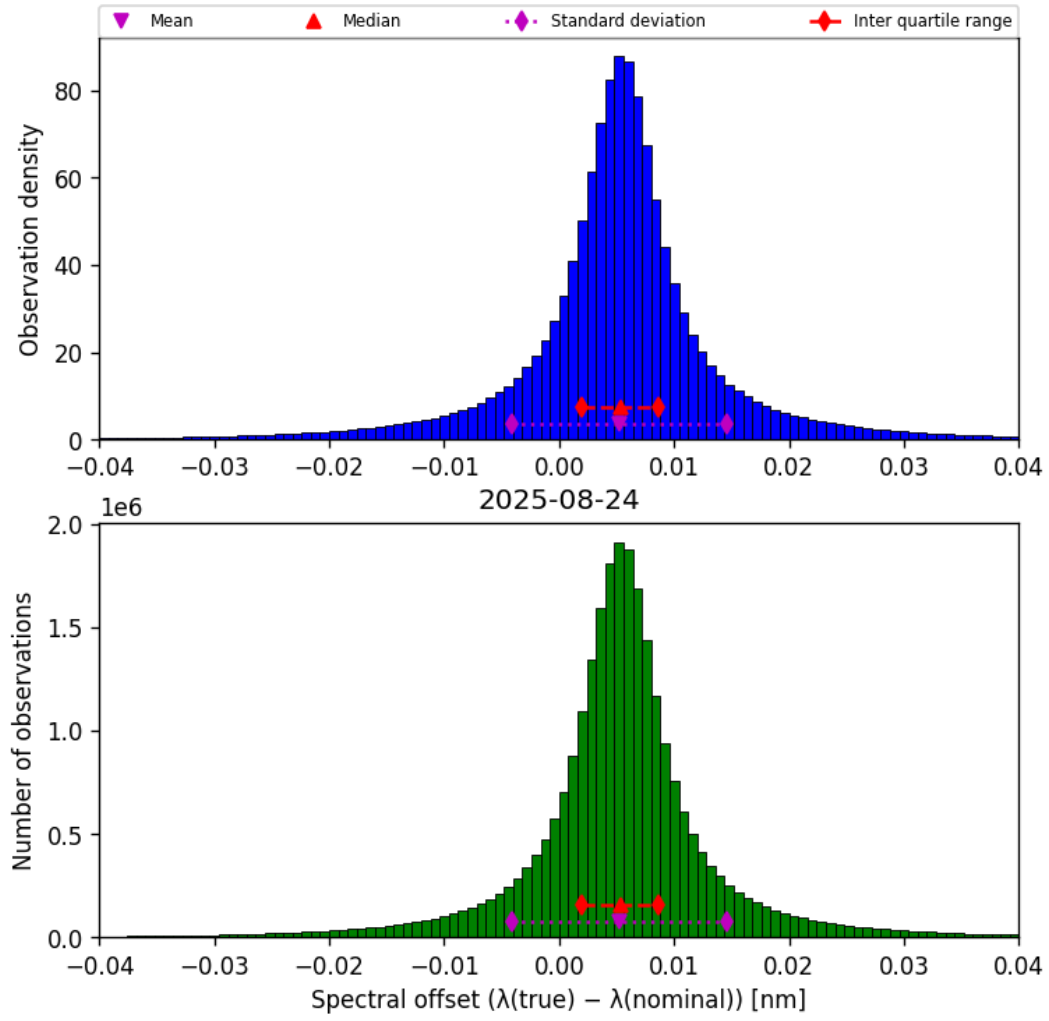
Figure 45: Histogram of “Spectral offset ( \lambda_{\text{true}} - \lambda_{\text{nominal}} )” for 2025-08-23 to 2025-08-25
