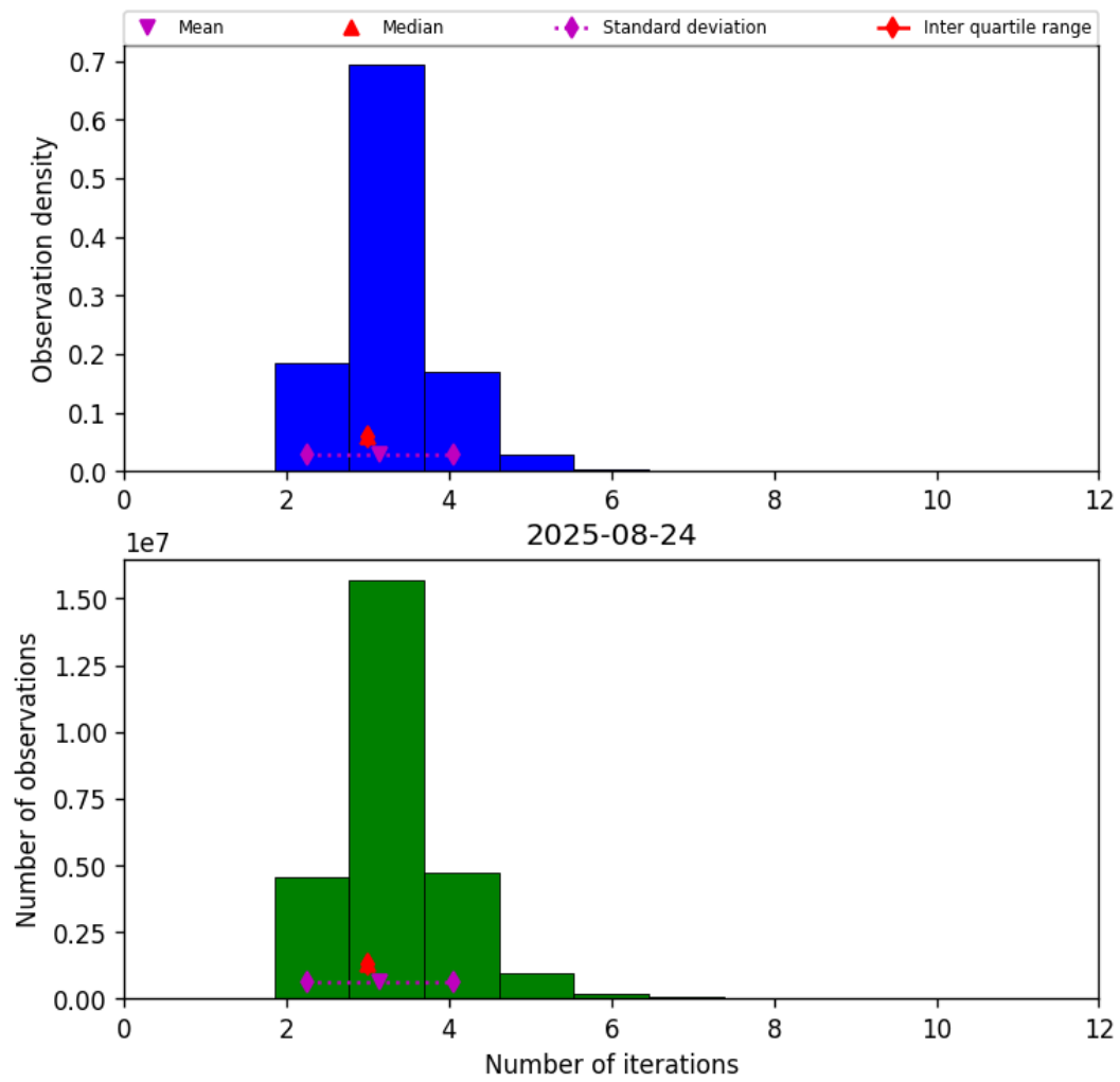
Figure 39: Histogram of “Number of iterations” for 2025-08-23 to 2025-08-25
