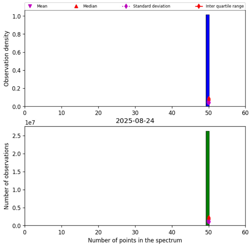
Figure 44: Histogram of “Number of points in the spectrum” for 2025-08-23 to 2025-08-25
