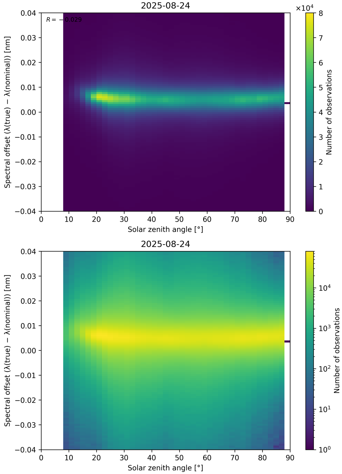
Figure 117: Scatter density plot of “Solar zenith angle” against “Spectral offset ( \lambda_{\text{true}} - \lambda_{\text{nominal}} )” for 2025-08-23 to 2025-08-25.
