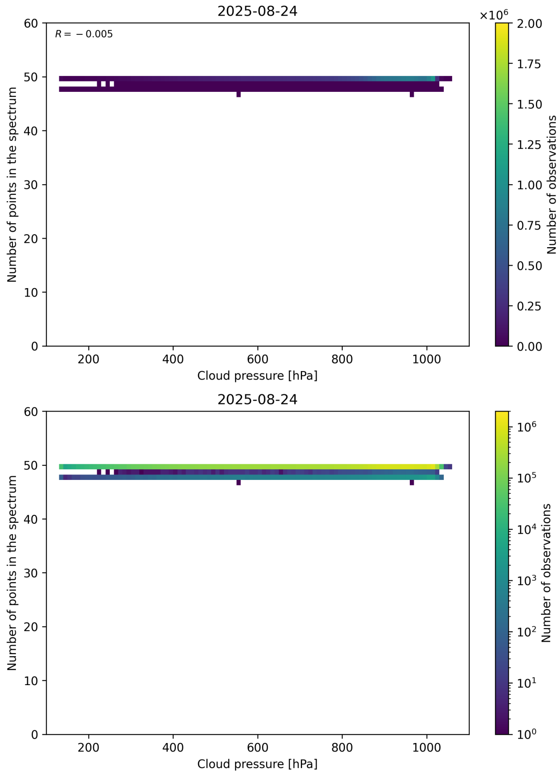
Figure 82: Scatter density plot of “Cloud pressure” against “Number of points in the spectrum” for 2025-08-23 to 2025-08-25.
