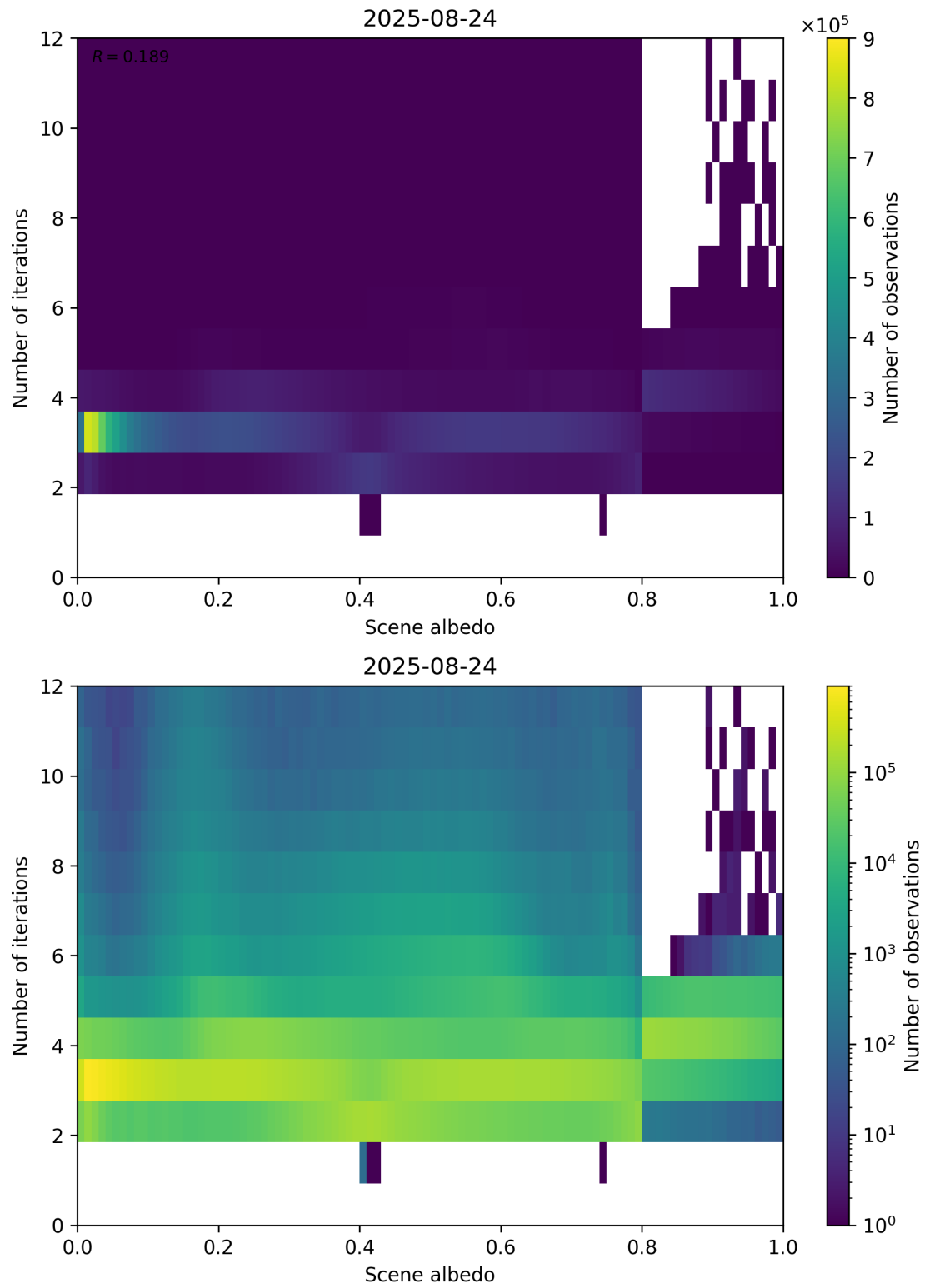
Figure 105: Scatter density plot of “Scene albedo” against “Number of iterations” for 2025-08-23 to 2025-08-25.
