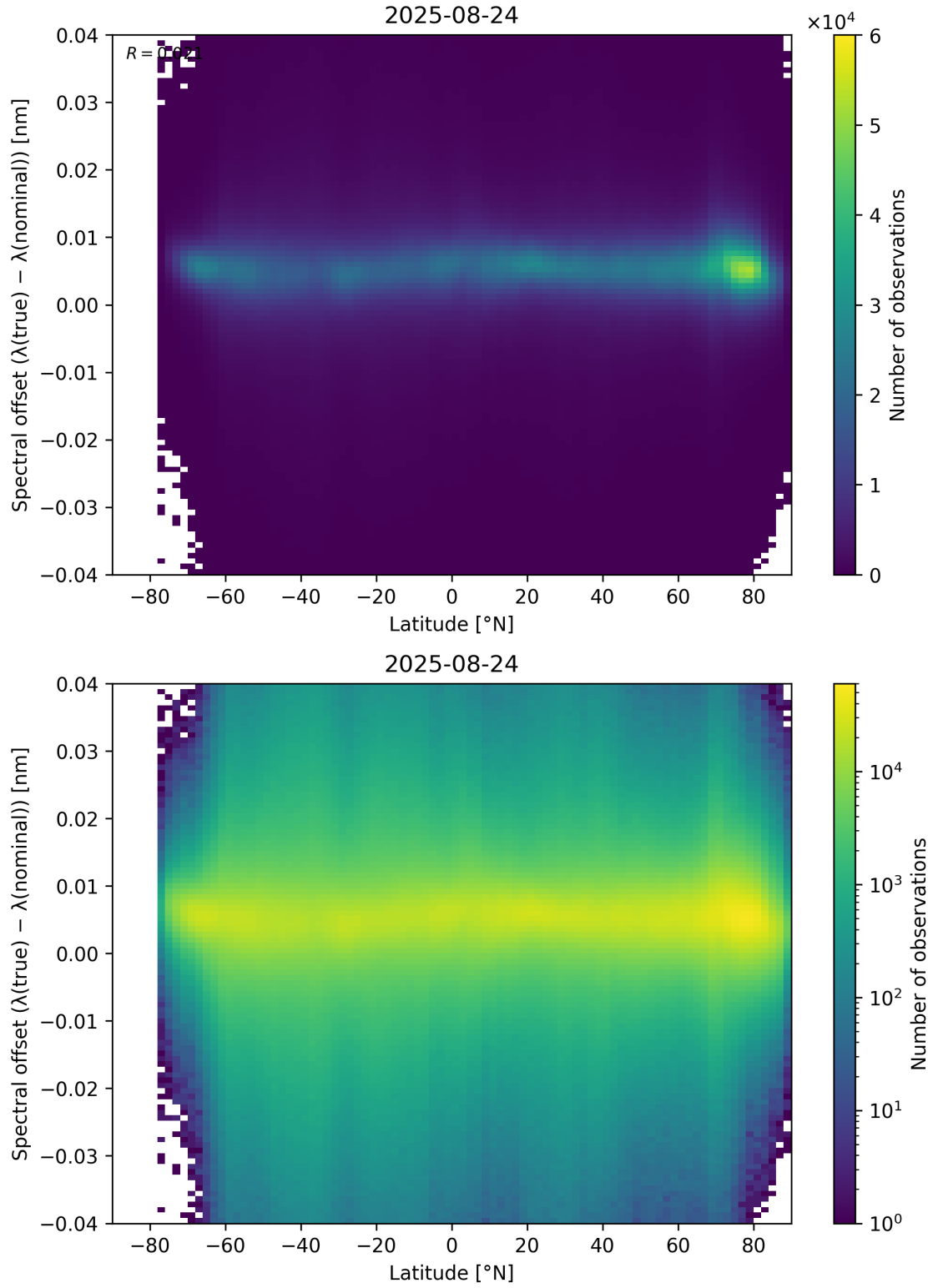
Figure 96: Scatter density plot of “Latitude” against “Spectral offset ( \lambda_{\text{true}} - \lambda_{\text{nominal}} )” for 2025-08-23 to 2025-08-25.
