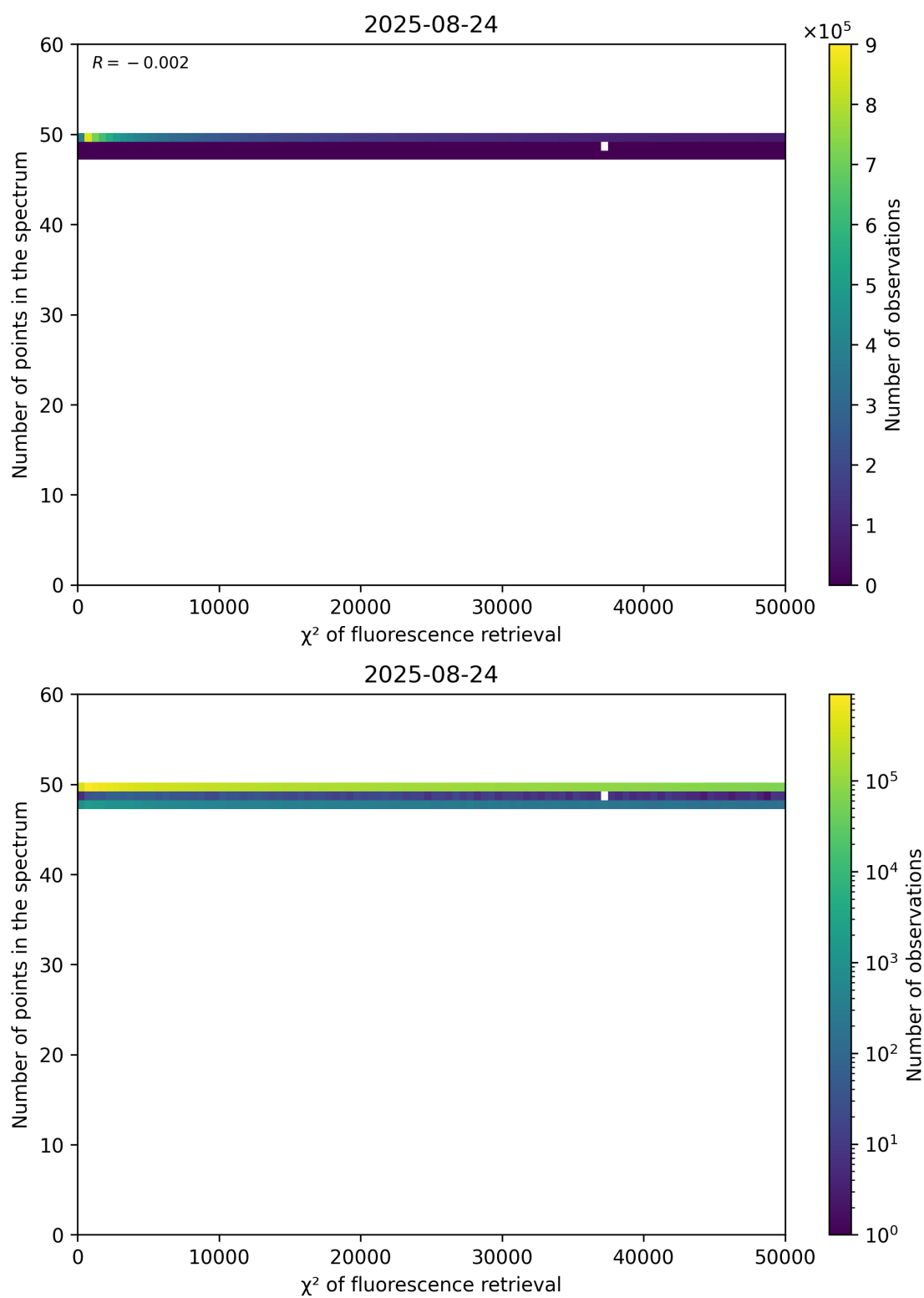
Figure 68: Scatter density plot of “ \chi^2 of fluorescence retrieval” against “Number of points in the spectrum” for 2025-08-23 to 2025-08-25.
