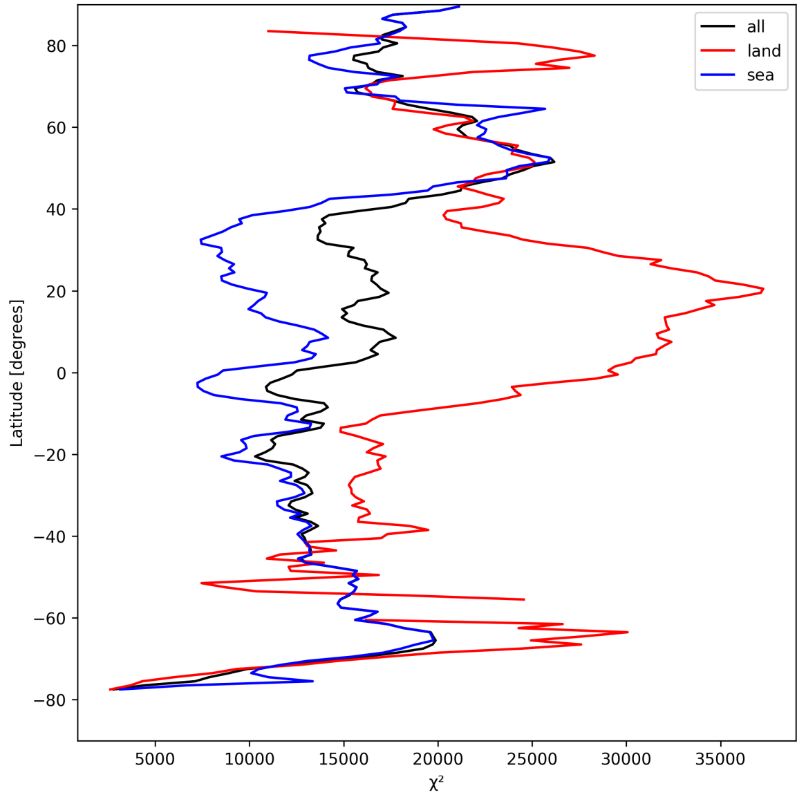
Figure 21: Zonal average of “ \chi^2 ” for 2025-08-23 to 2025-08-25.
