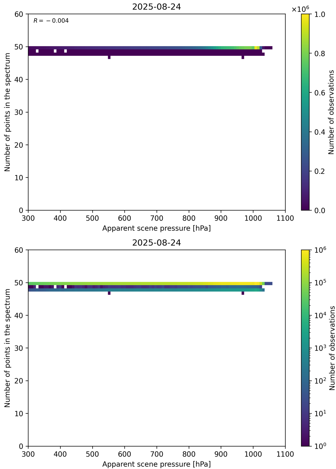
Figure 66: Scatter density plot of “Apparent scene pressure” against “Number of points in the spectrum” for 2025-08-23 to 2025-08-25.
