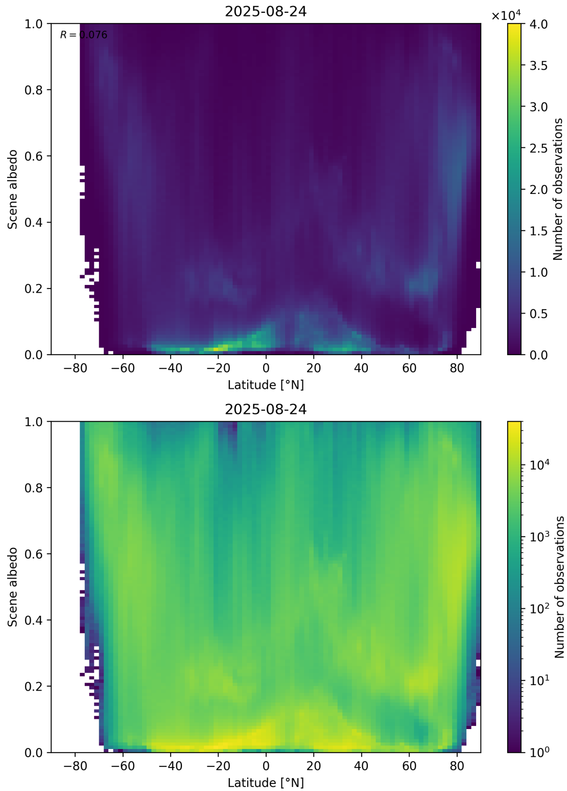
Figure 95: Scatter density plot of “Latitude” against “Scene albedo” for 2025-08-23 to 2025-08-25.
