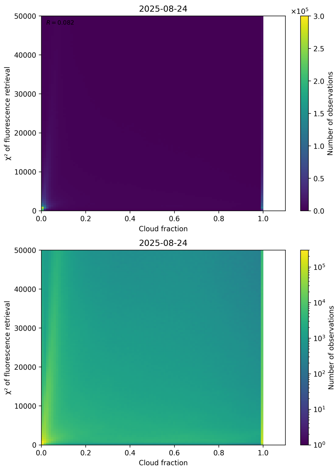
Figure 71: Scatter density plot of “Cloud fraction” against “ \chi^2 of fluorescence retrieval” for 2025-08-23 to 2025-08-25.
