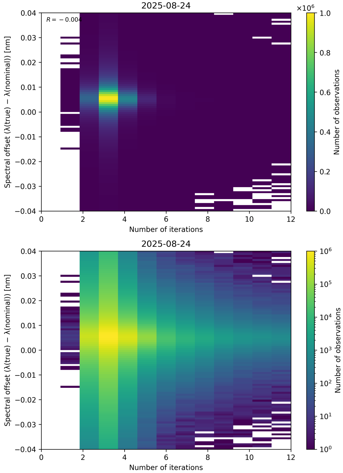
Figure 100: Scatter density plot of “Number of iterations” against “Spectral offset ( \lambda_{\text{true}} - \lambda_{\text{nominal}} )” for 2025-08-23 to 2025-08-25.
