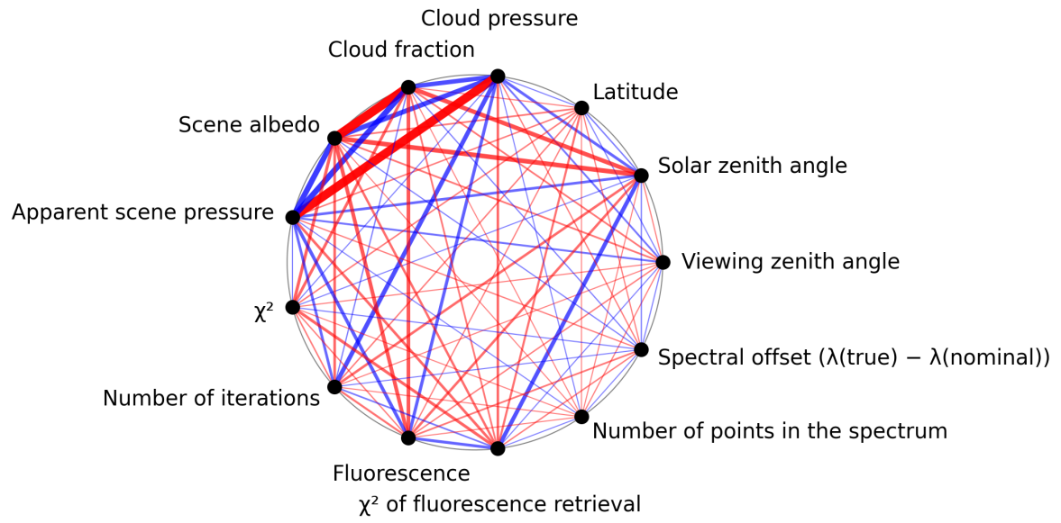
Figure 1: Map of correlation graph for 2025-08-23 to 2025-08-25.
