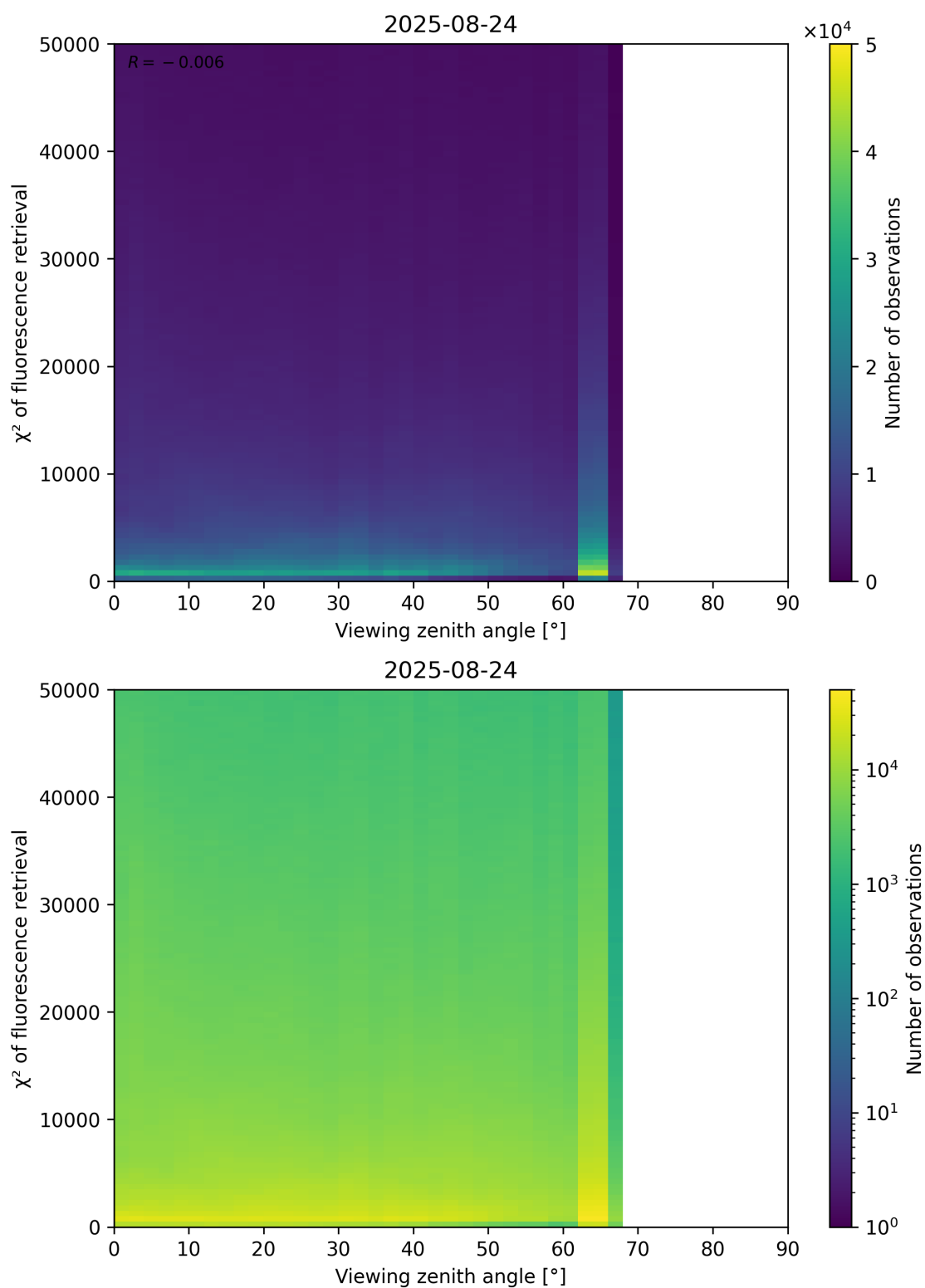
Figure 119: Scatter density plot of “Viewing zenith angle” against “ \chi^2 of fluorescence retrieval” for 2025-08-23 to 2025-08-25.
