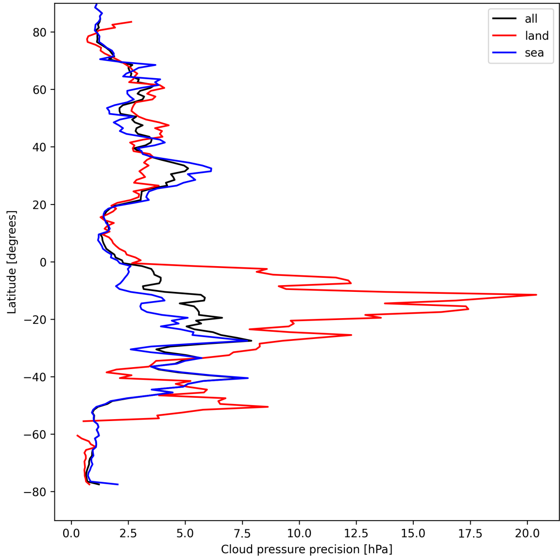
Figure 14: Zonal average of "Cloud pressure precision" for 2025-08-23 to 2025-08-25.
