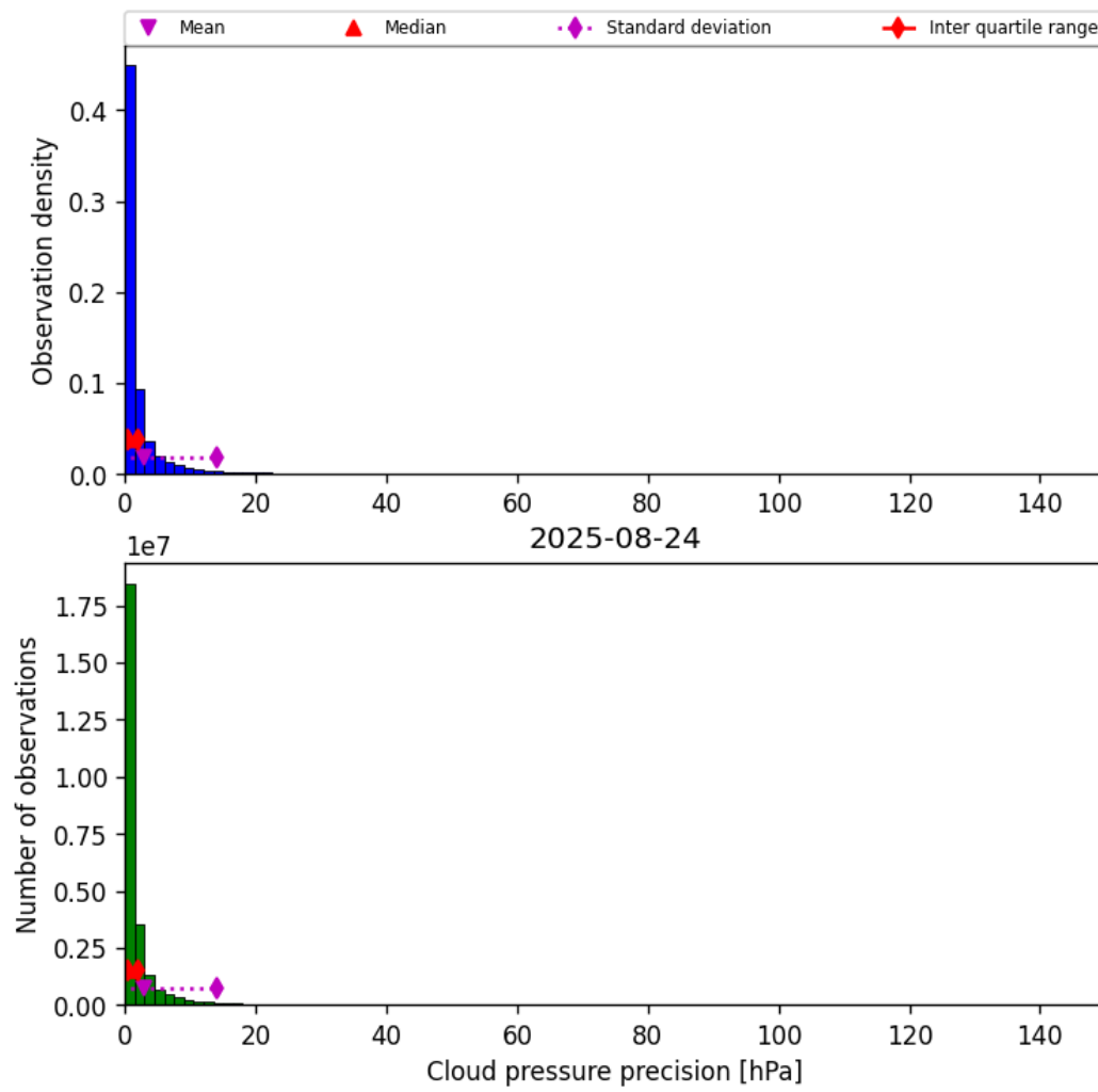
Figure 31: Histogram of “Cloud pressure precision” for 2025-08-23 to 2025-08-25
