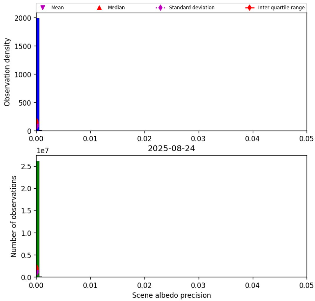
Figure 35: Histogram of “Scene albedo precision” for 2025-08-23 to 2025-08-25
