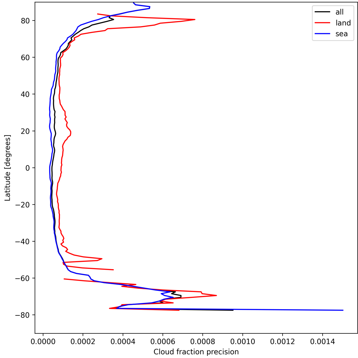
Figure 16: Zonal average of “Cloud fraction precision” for 2025-08-23 to 2025-08-25.
