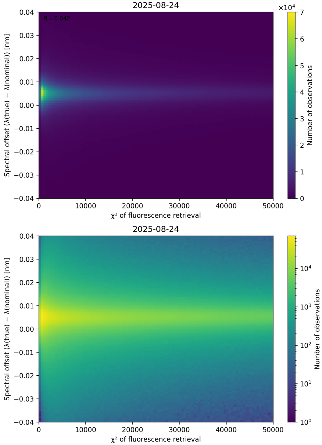
Figure 69: Scatter density plot of “ \chi^2 of fluorescence retrieval” against “Spectral offset ( \lambda_{\text{true}} - \lambda_{\text{nominal}} )” for 2025-08-23 to 2025-08-25.
