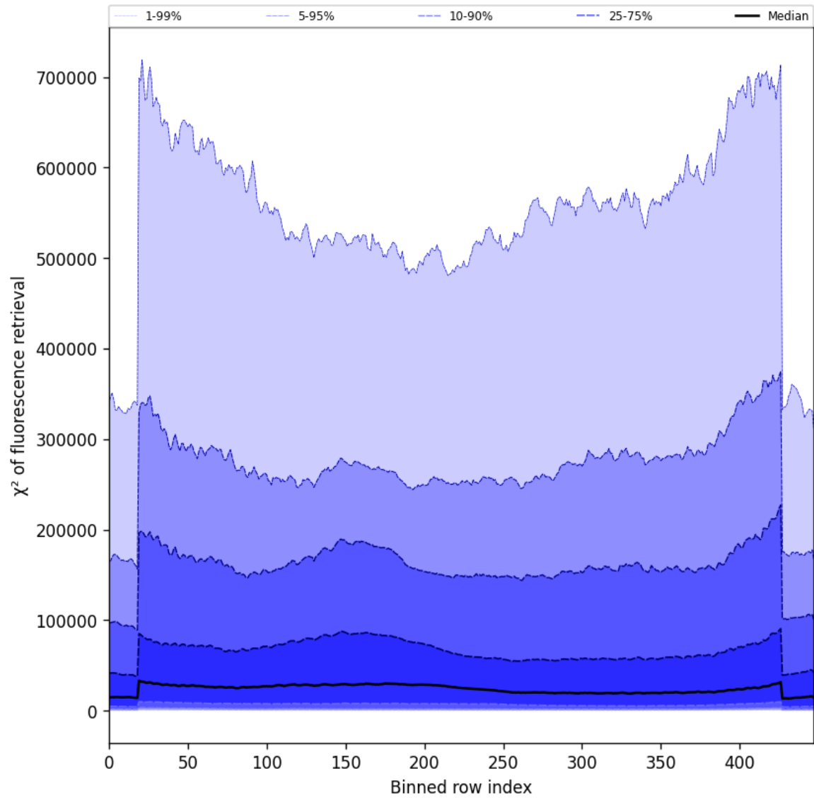
Figure 59: Along track statistics of “ \chi^2 of fluorescence retrieval” for 2025-08-23 to 2025-08-25
