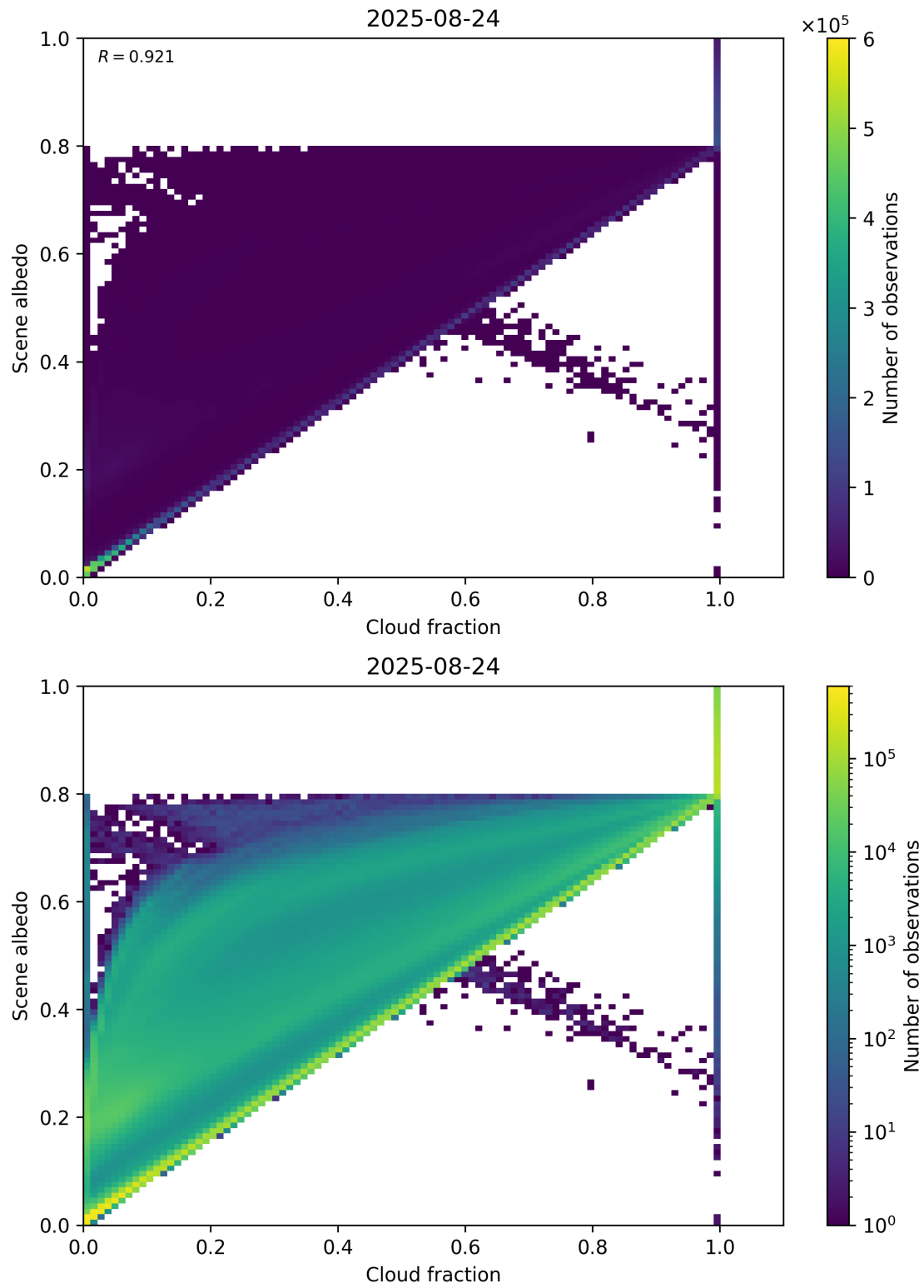
Figure 75: Scatter density plot of “Cloud fraction” against “Scene albedo” for 2025-08-23 to 2025-08-25.
