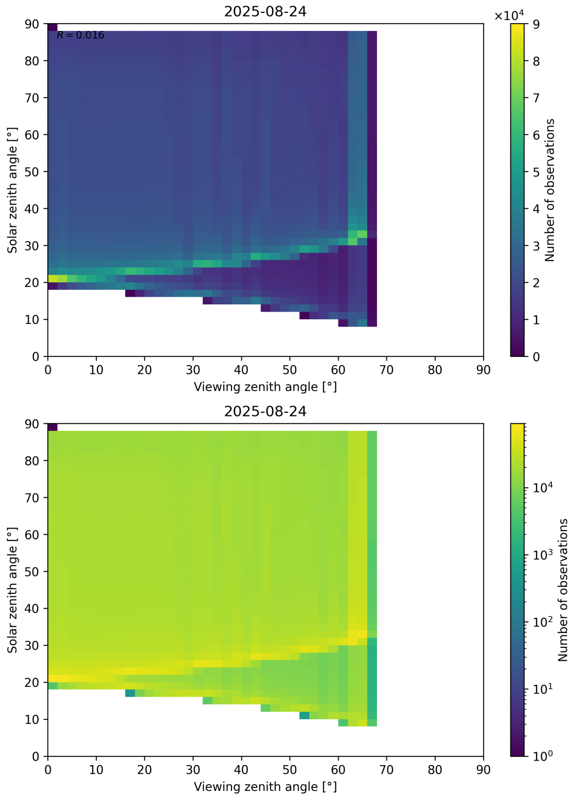
Figure 127: Scatter density plot of “Viewing zenith angle” against “Solar zenith angle” for 2025-08-23 to 2025-08-25.
