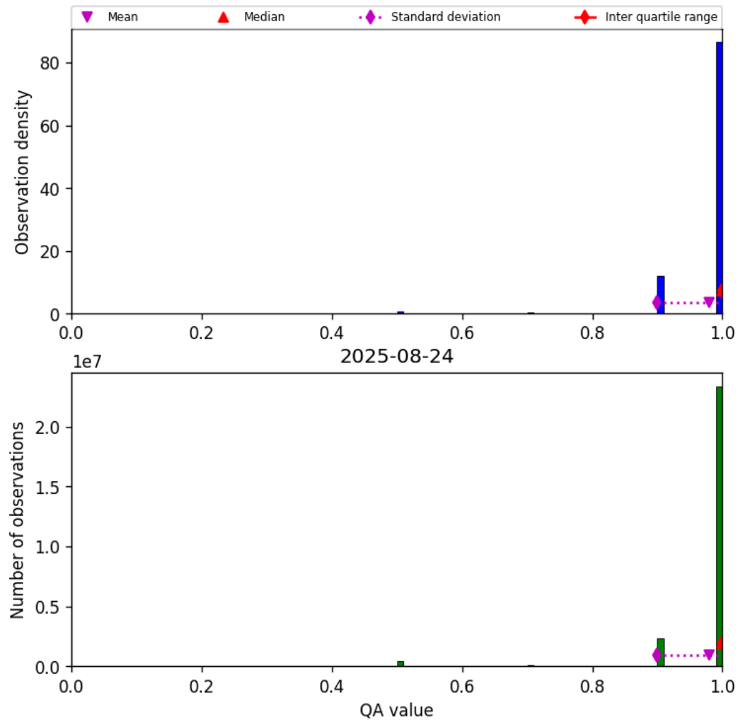
Figure 29: Histogram of “QA value” for 2025-08-23 to 2025-08-25
