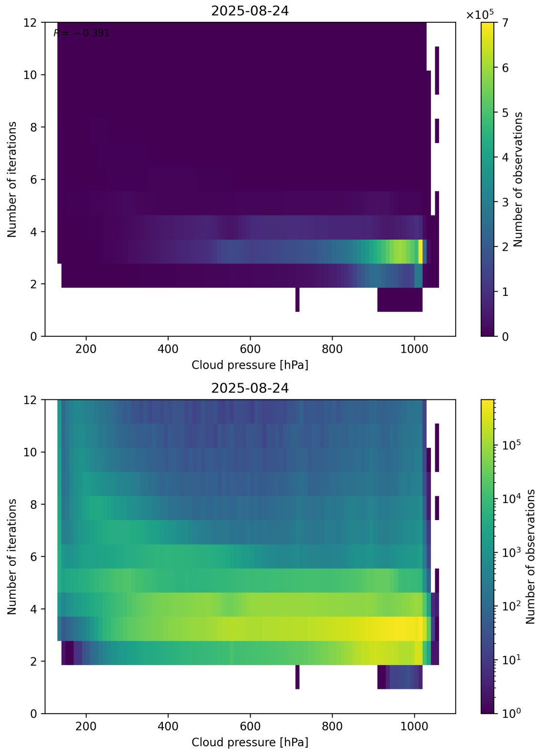
Figure 81: Scatter density plot of “Cloud pressure” against “Number of iterations” for 2025-08-23 to 2025-08-25.
