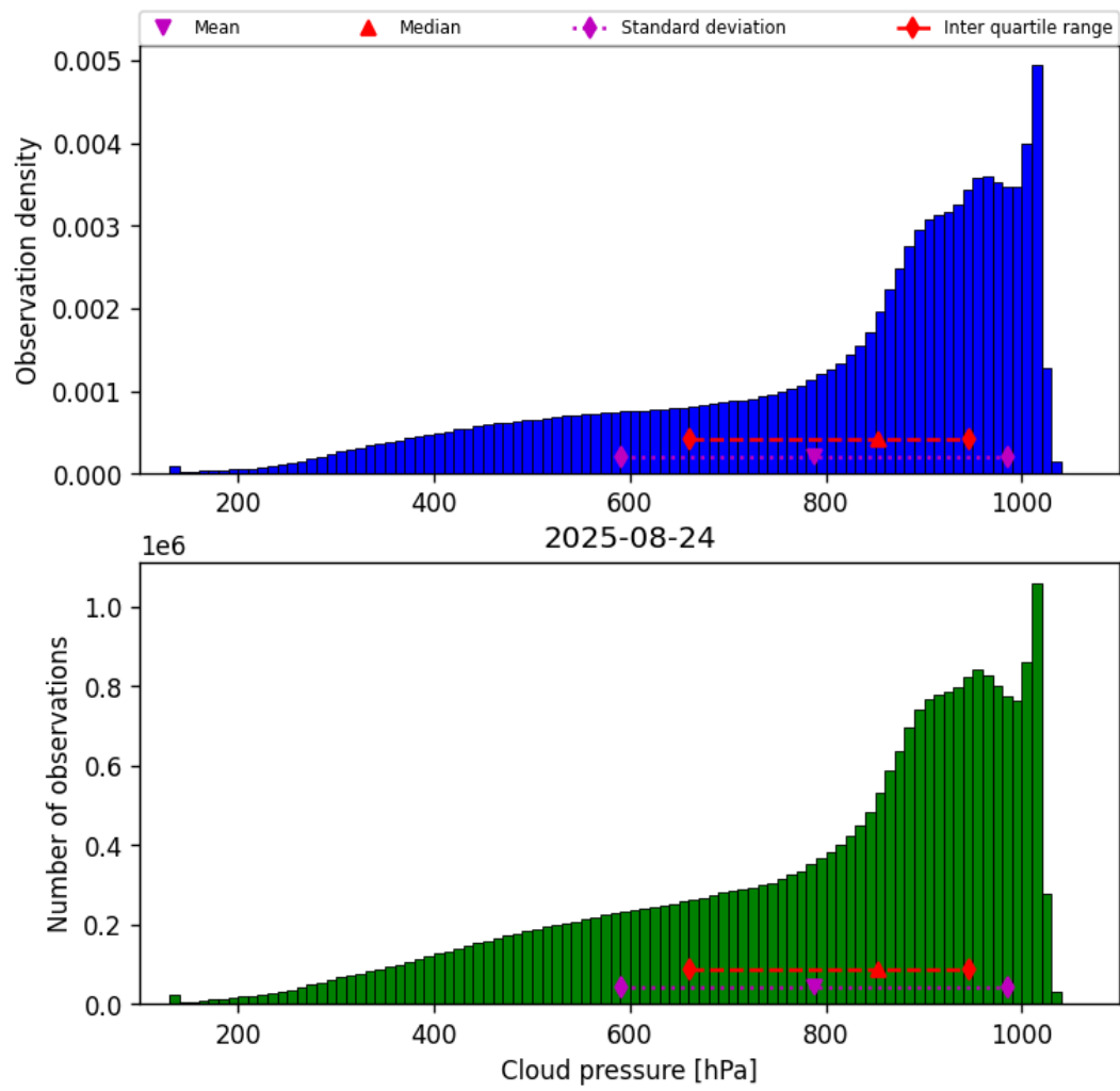
Figure 30: Histogram of “Cloud pressure” for 2025-08-23 to 2025-08-25
