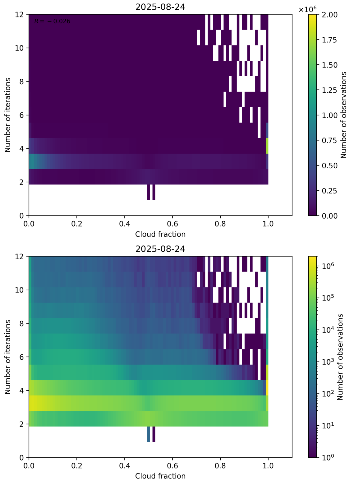
Figure 73: Scatter density plot of “Cloud fraction” against “Number of iterations” for 2025-08-23 to 2025-08-25.
