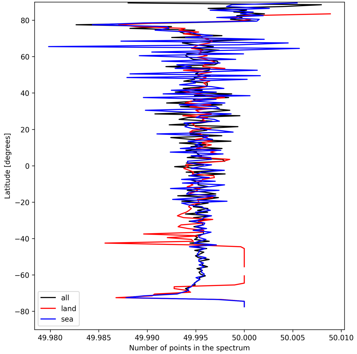
Figure 27: Zonal average of “Number of points in the spectrum” for 2025-08-23 to 2025-08-25.
