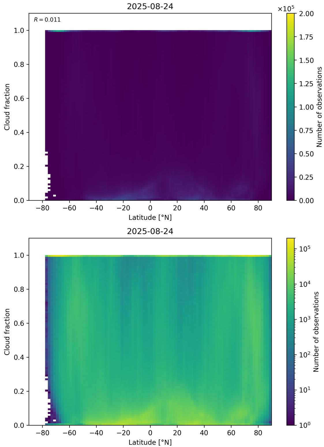
Figure 90: Scatter density plot of “Latitude” against “Cloud fraction” for 2025-08-23 to 2025-08-25.
