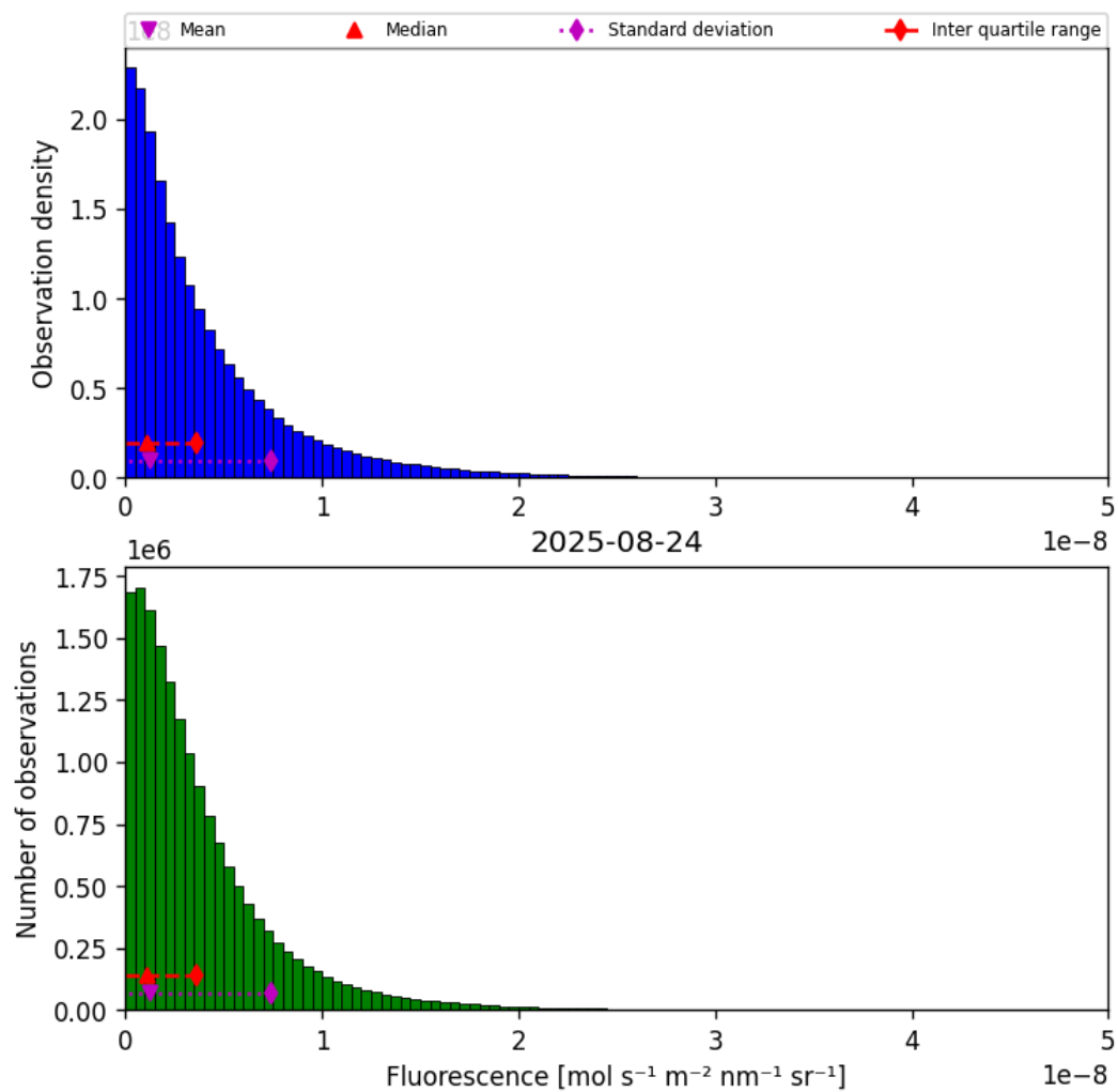
Figure 40: Histogram of “Fluorescence” for 2025-08-23 to 2025-08-25
