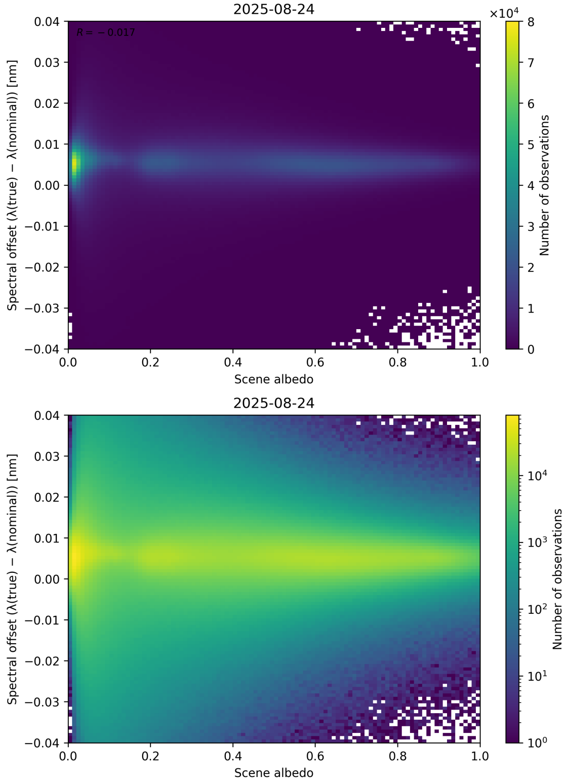
Figure 107: Scatter density plot of “Scene albedo” against “Spectral offset ( \lambda_{\text{true}} - \lambda_{\text{nominal}} )” for 2025-08-23 to 2025-08-25.
