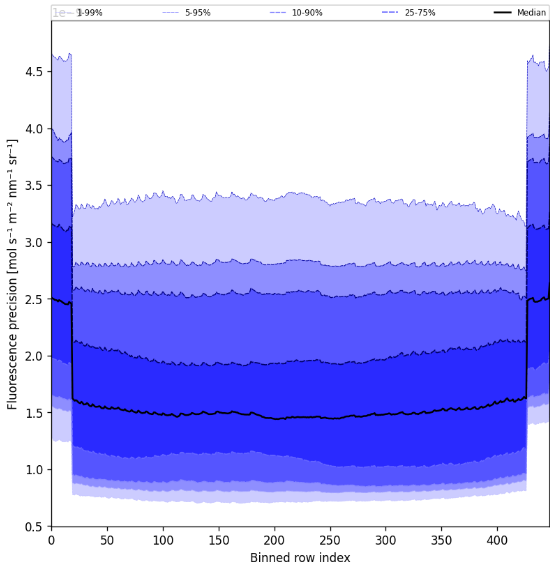
Figure 58: Along track statistics of “Fluorescence precision” for 2025-08-23 to 2025-08-25
