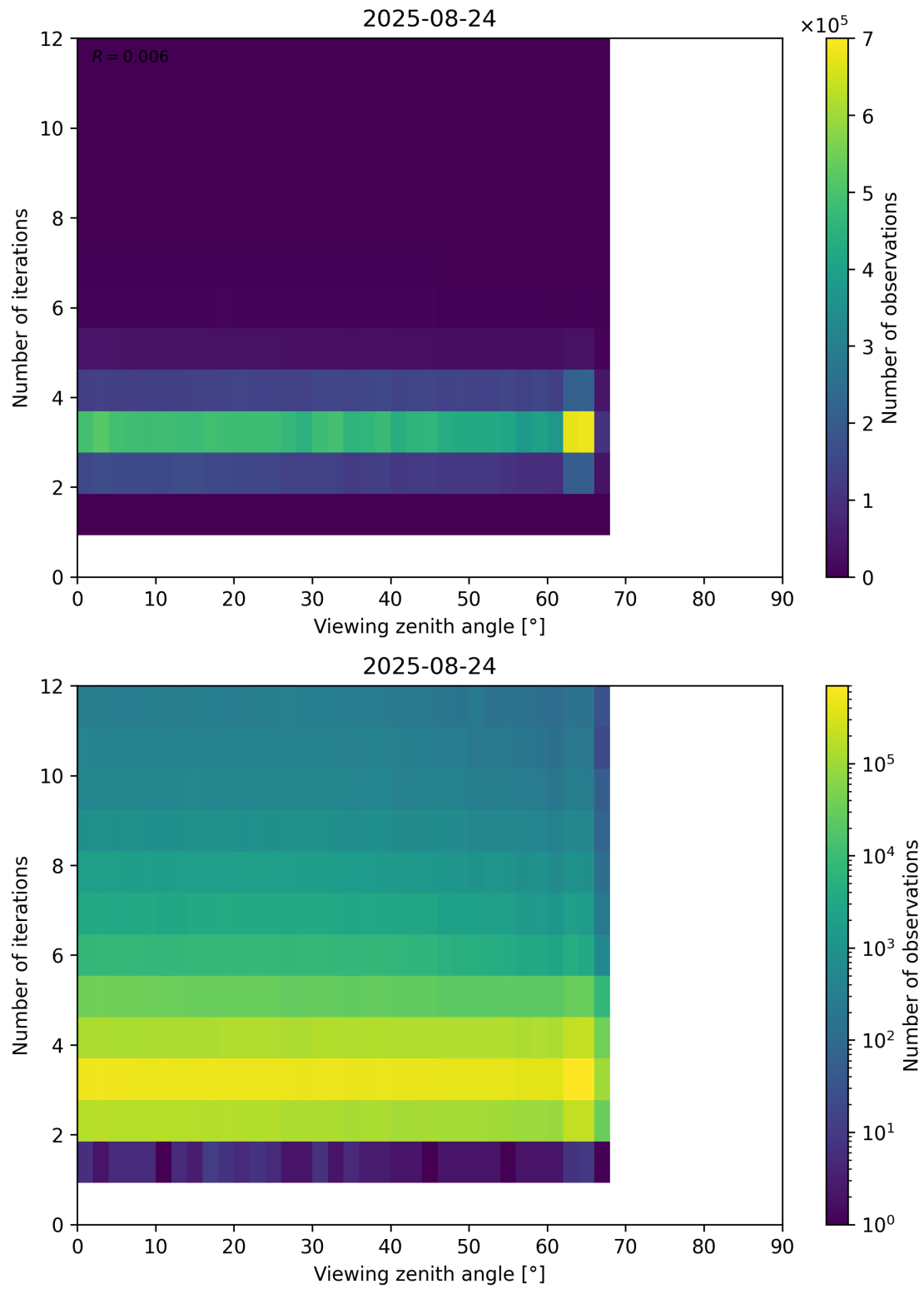
Figure 124: Scatter density plot of “Viewing zenith angle” against “Number of iterations” for 2025-08-23 to 2025-08-25.
