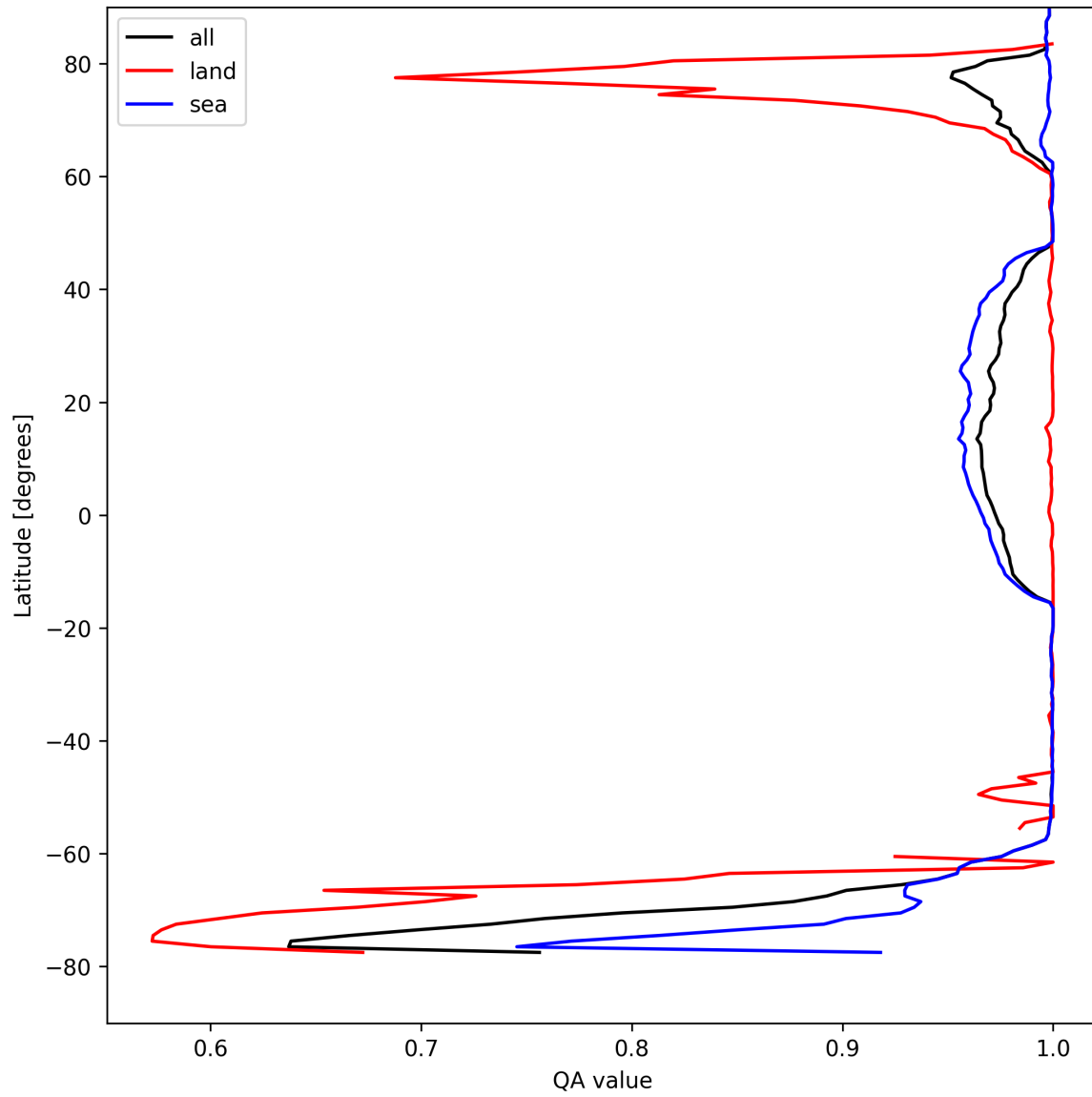
Figure 12: Zonal average of "QA value" for 2025-08-23 to 2025-08-25.
