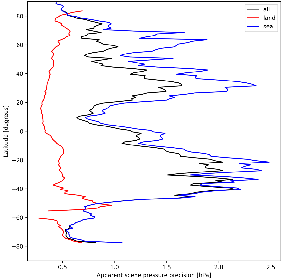
Figure 20: Zonal average of “Apparent scene pressure precision” for 2025-08-23 to 2025-08-25.
