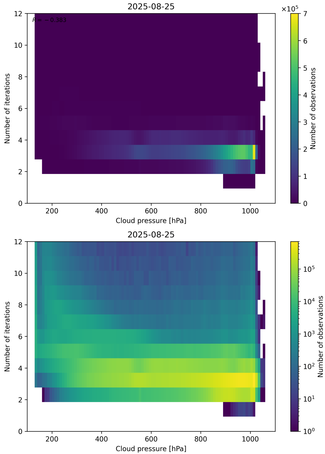
Figure 81: Scatter density plot of “Cloud pressure” against “Number of iterations” for 2025-08-25 to 2025-08-26.
