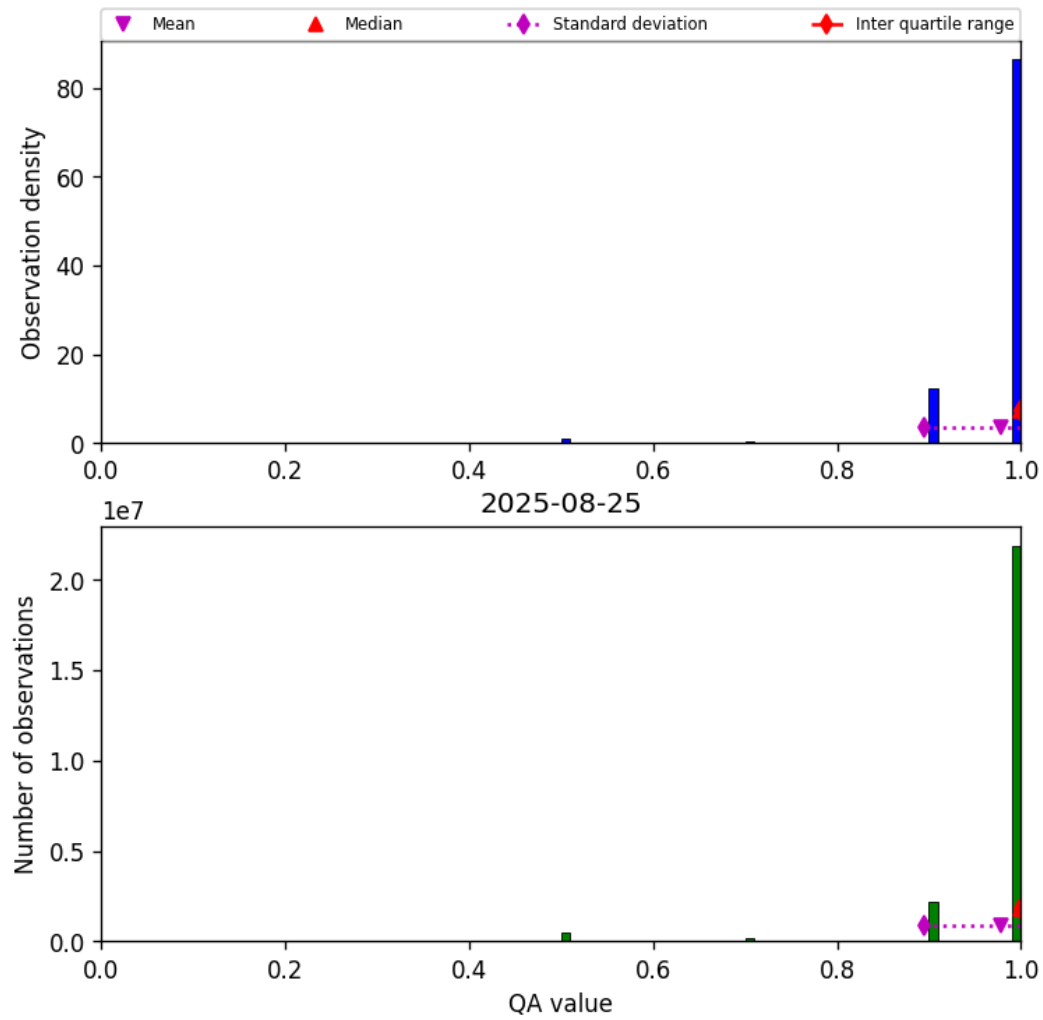
Figure 29: Histogram of “QA value” for 2025-08-25 to 2025-08-26
