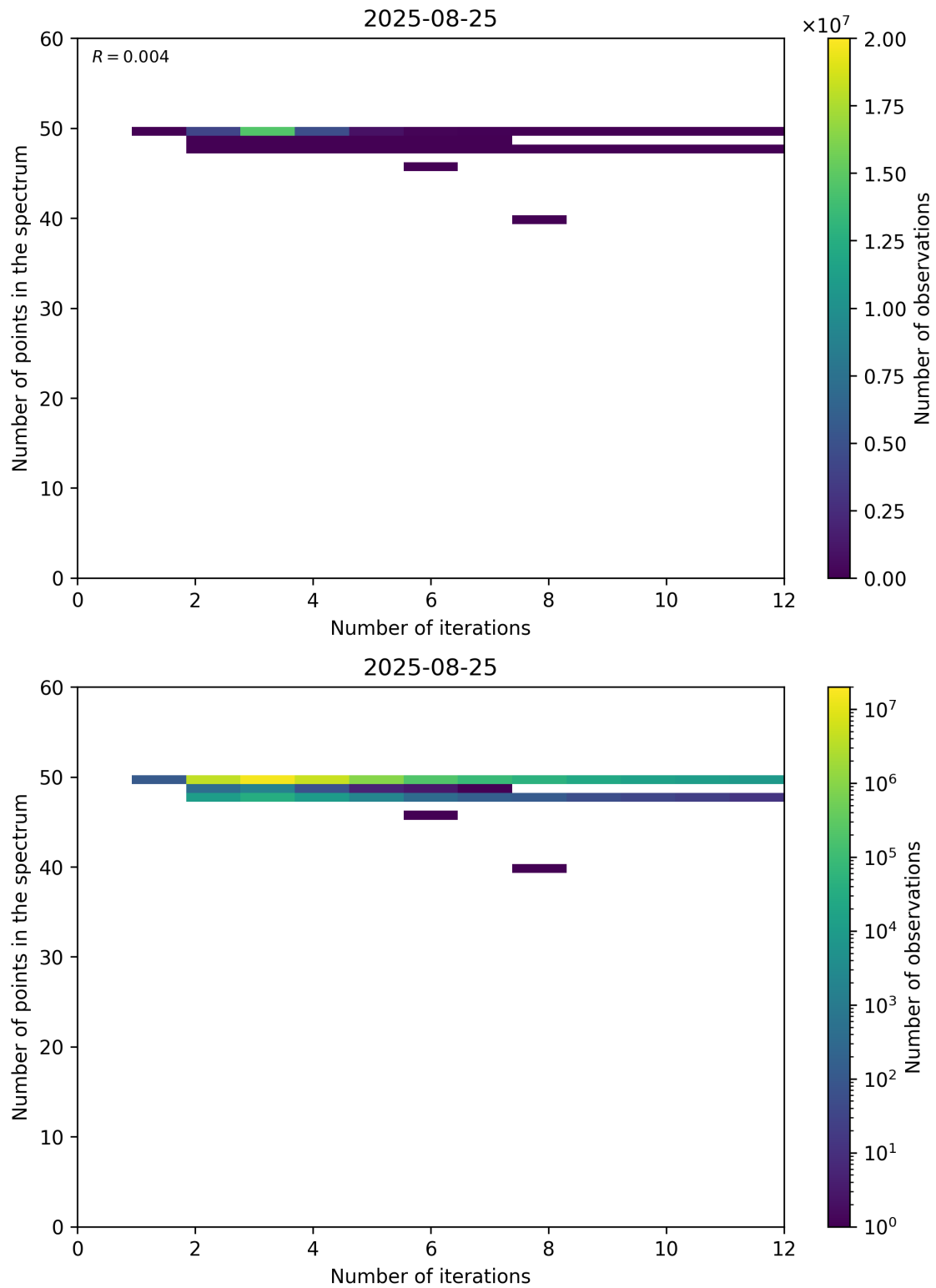
Figure 99: Scatter density plot of “Number of iterations” against “Number of points in the spectrum” for 2025-08-25 to 2025-08-26.
