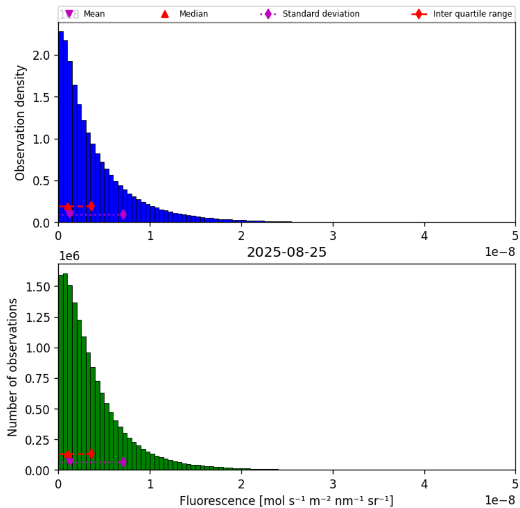
Figure 40: Histogram of “Fluorescence” for 2025-08-25 to 2025-08-26
