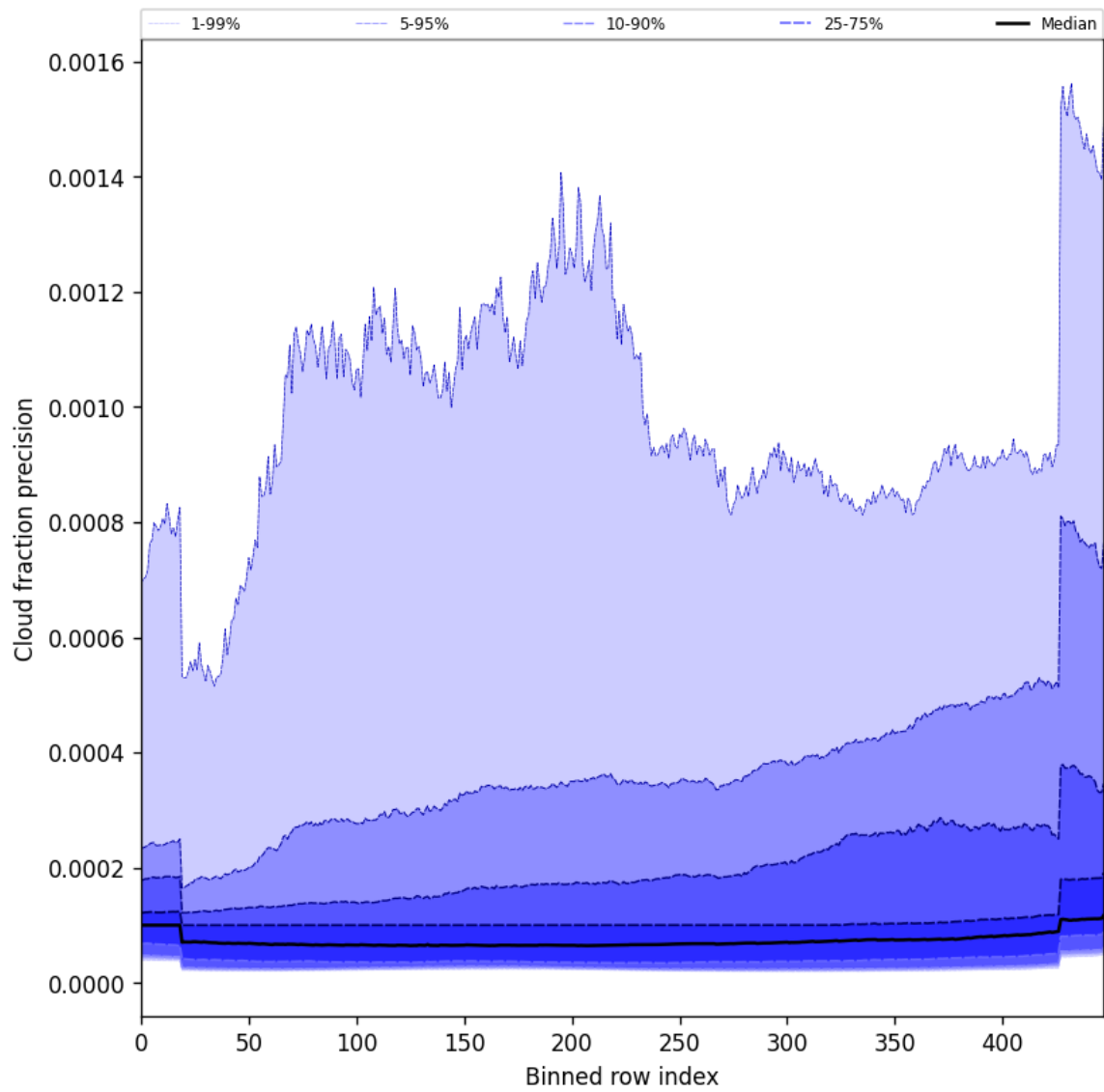
Figure 50: Along track statistics of “Cloud fraction precision” for 2025-08-25 to 2025-08-26
