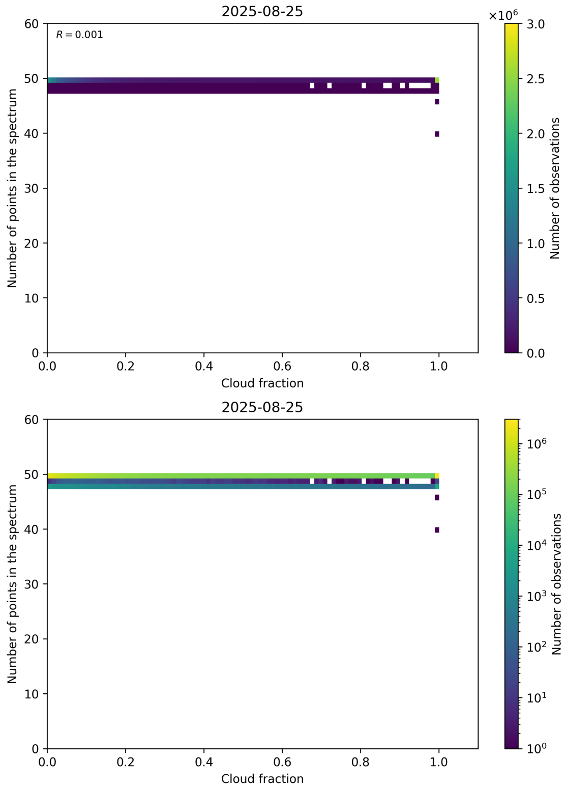
Figure 74: Scatter density plot of “Cloud fraction” against “Number of points in the spectrum” for 2025-08-25 to 2025-08-26.
