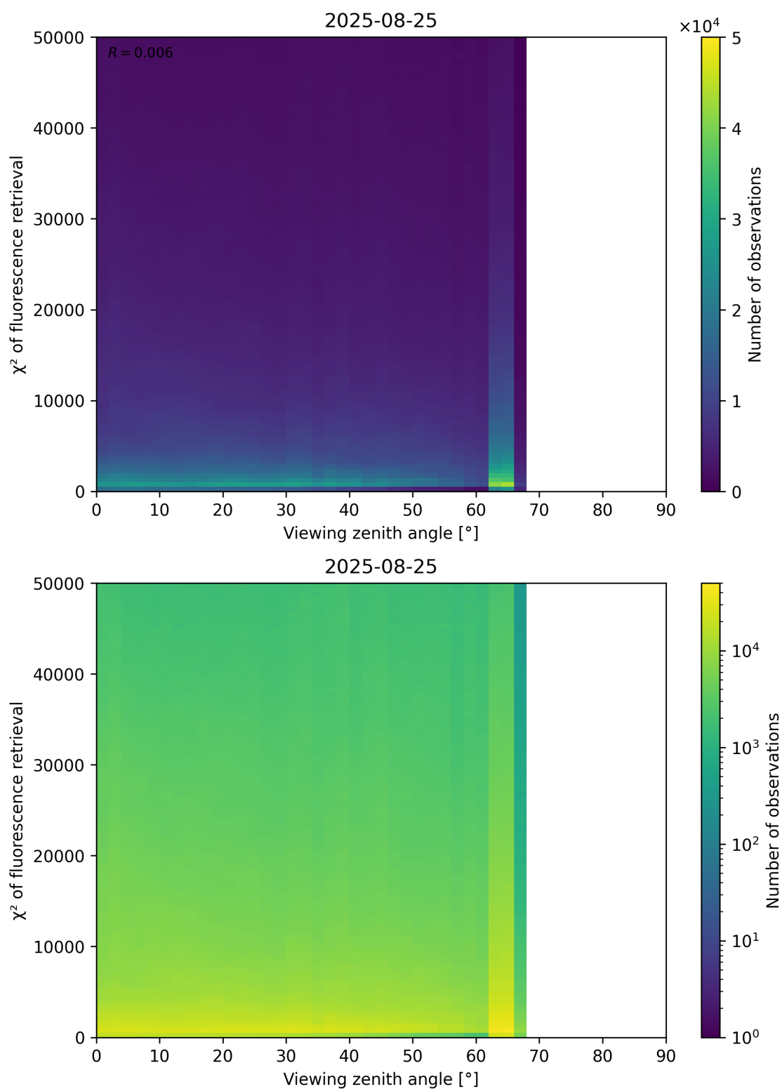
Figure 119: Scatter density plot of “Viewing zenith angle” against “ \chi^2 of fluorescence retrieval” for 2025-08-25 to 2025-08-26.
