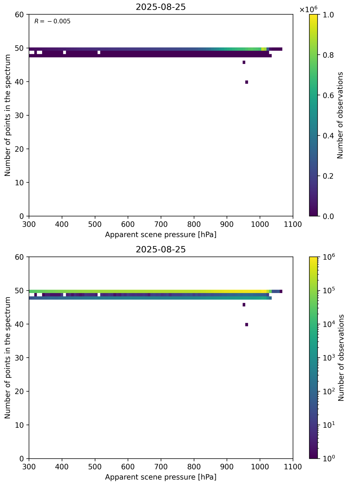
Figure 66: Scatter density plot of “Apparent scene pressure” against “Number of points in the spectrum” for 2025-08-25 to 2025-08-26.
