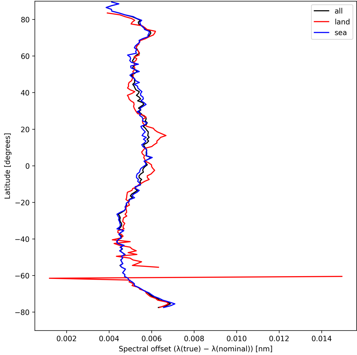
Figure 28: Zonal average of “Spectral offset ( \lambda_{\text{true}} - \lambda_{\text{nominal}} )” for 2025-08-25 to 2025-08-26.
