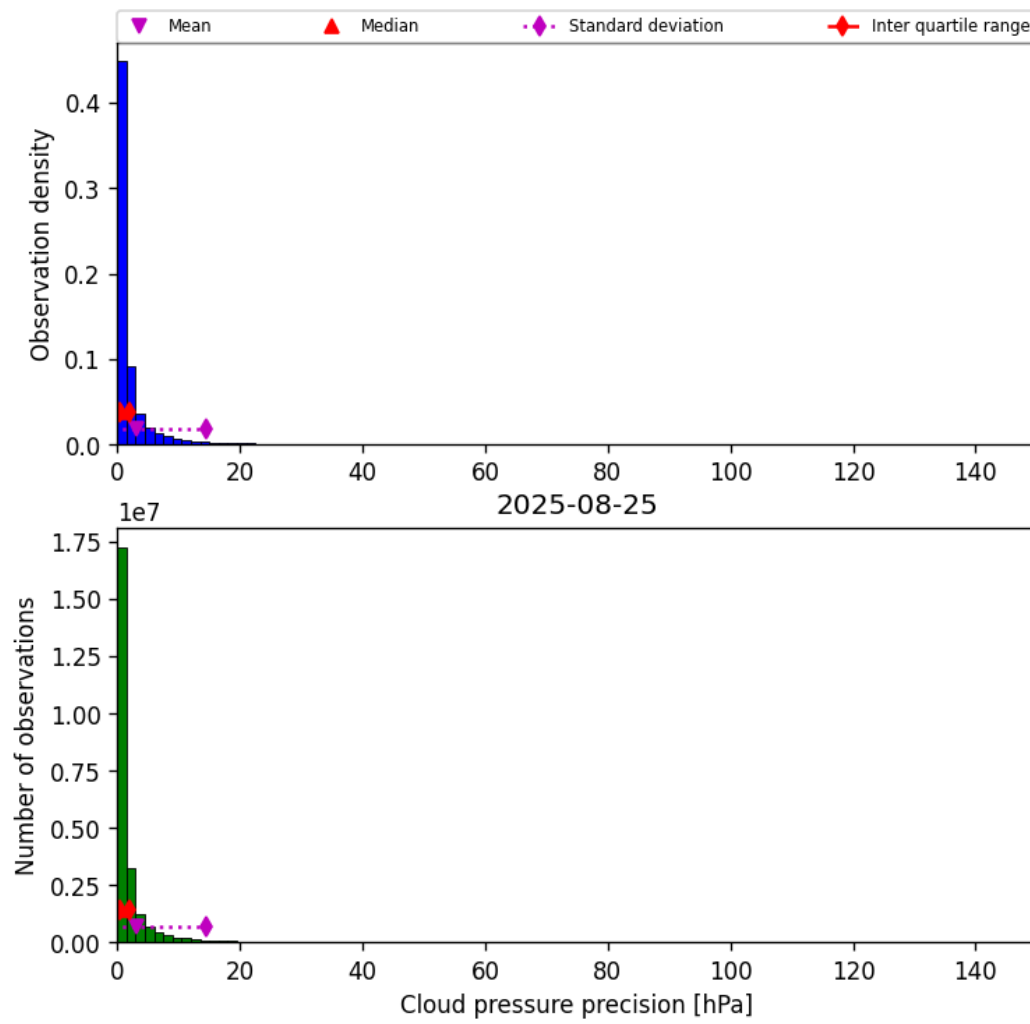
Figure 31: Histogram of “Cloud pressure precision” for 2025-08-25 to 2025-08-26
