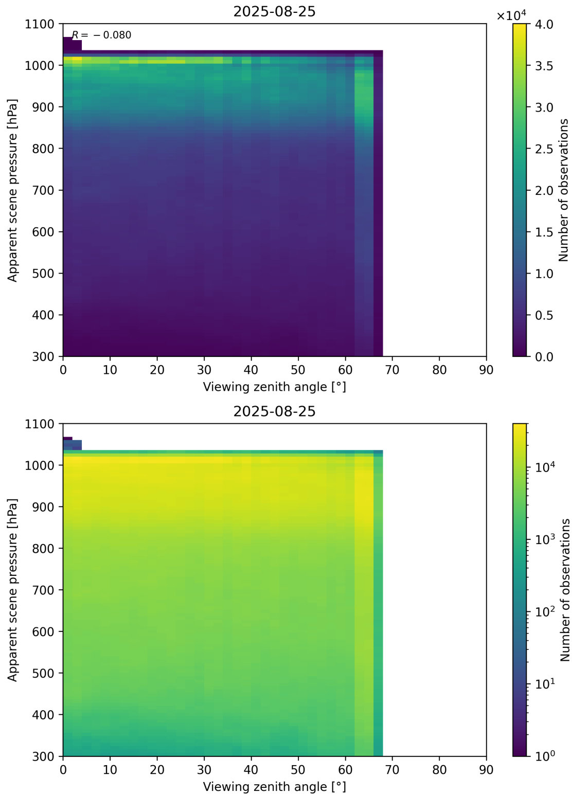
Figure 118: Scatter density plot of “Viewing zenith angle” against “Apparent scene pressure” for 2025-08-25 to 2025-08-26.
