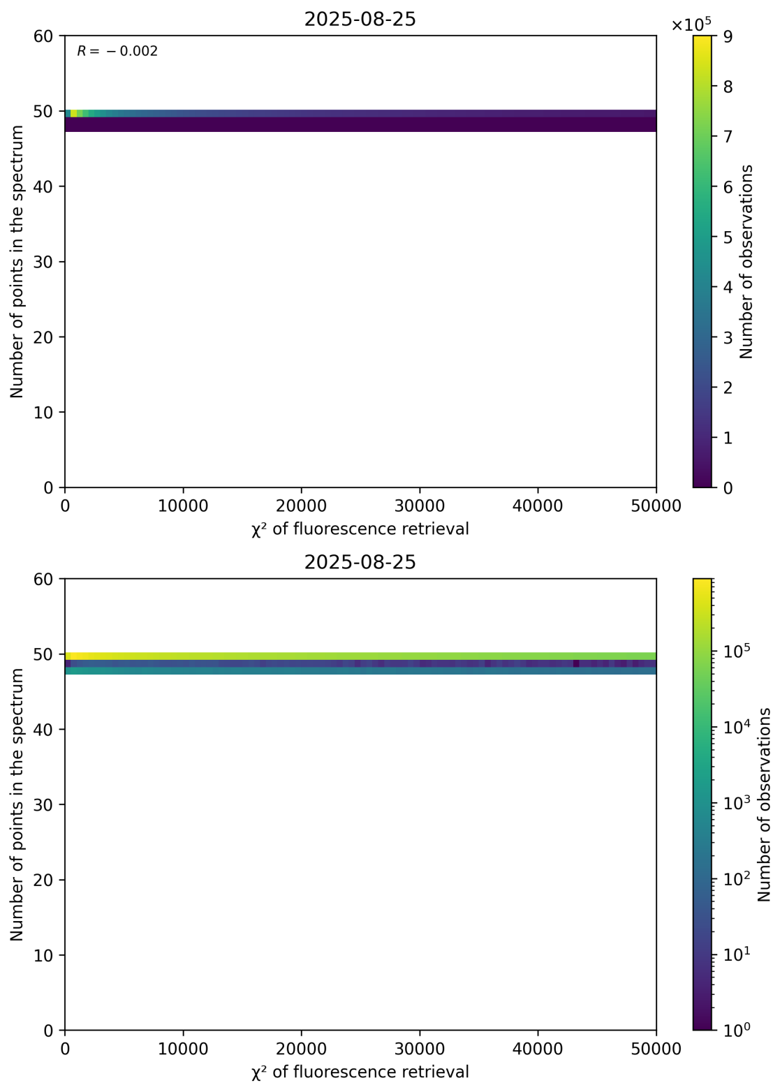
Figure 68: Scatter density plot of “ \chi^2 of fluorescence retrieval” against “Number of points in the spectrum” for 2025-08-25 to 2025-08-26.
