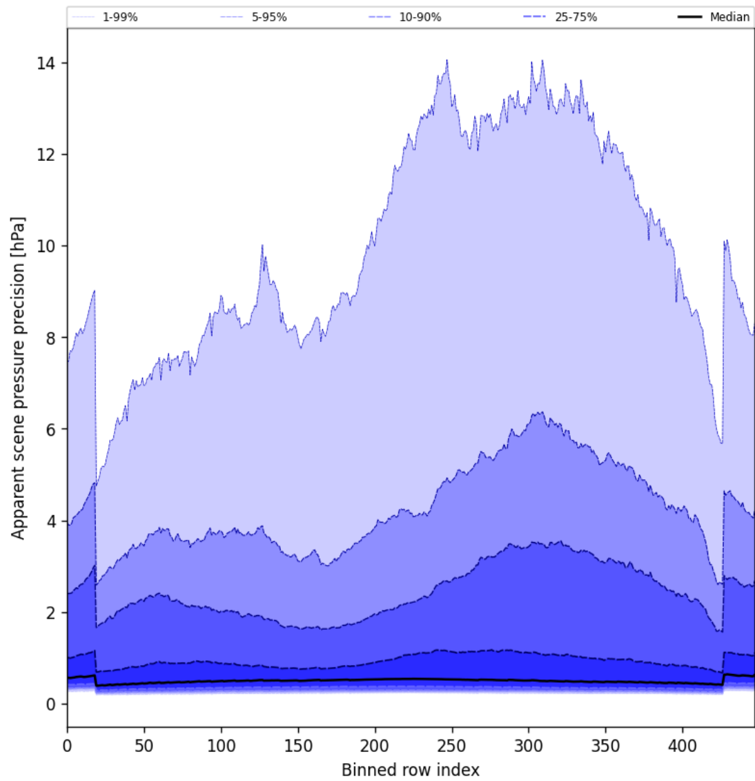
Figure 54: Along track statistics of “Apparent scene pressure precision” for 2025-08-25 to 2025-08-26
