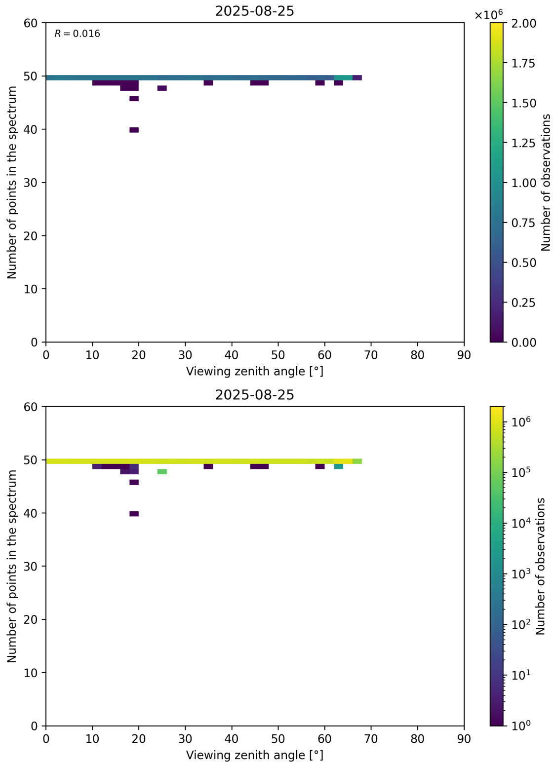
Figure 125: Scatter density plot of “Viewing zenith angle” against “Number of points in the spectrum” for 2025-08-25 to 2025-08-26.
