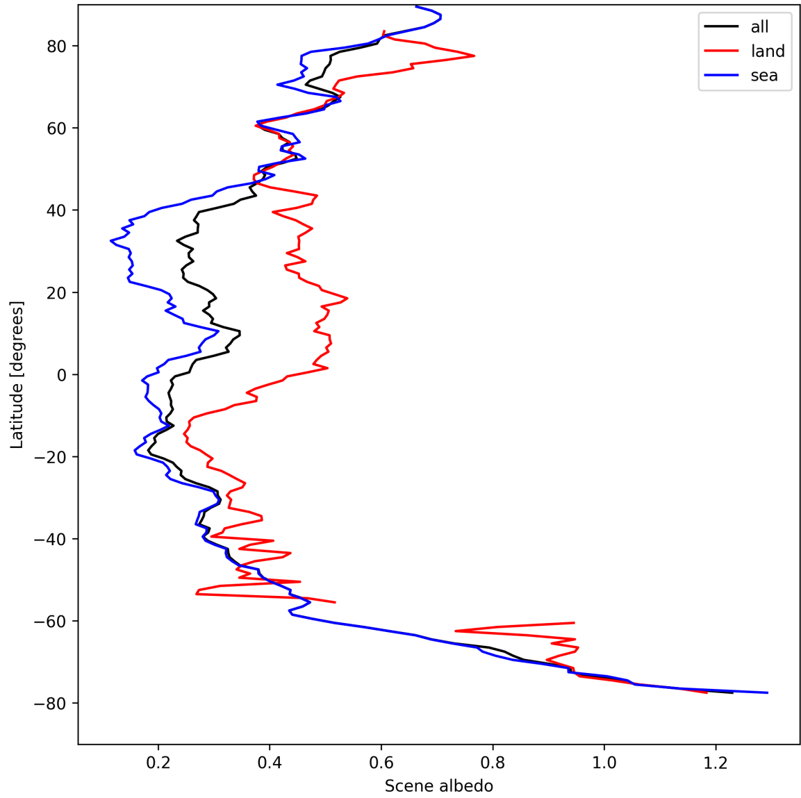
Figure 17: Zonal average of “Scene albedo” for 2025-08-25 to 2025-08-26.
