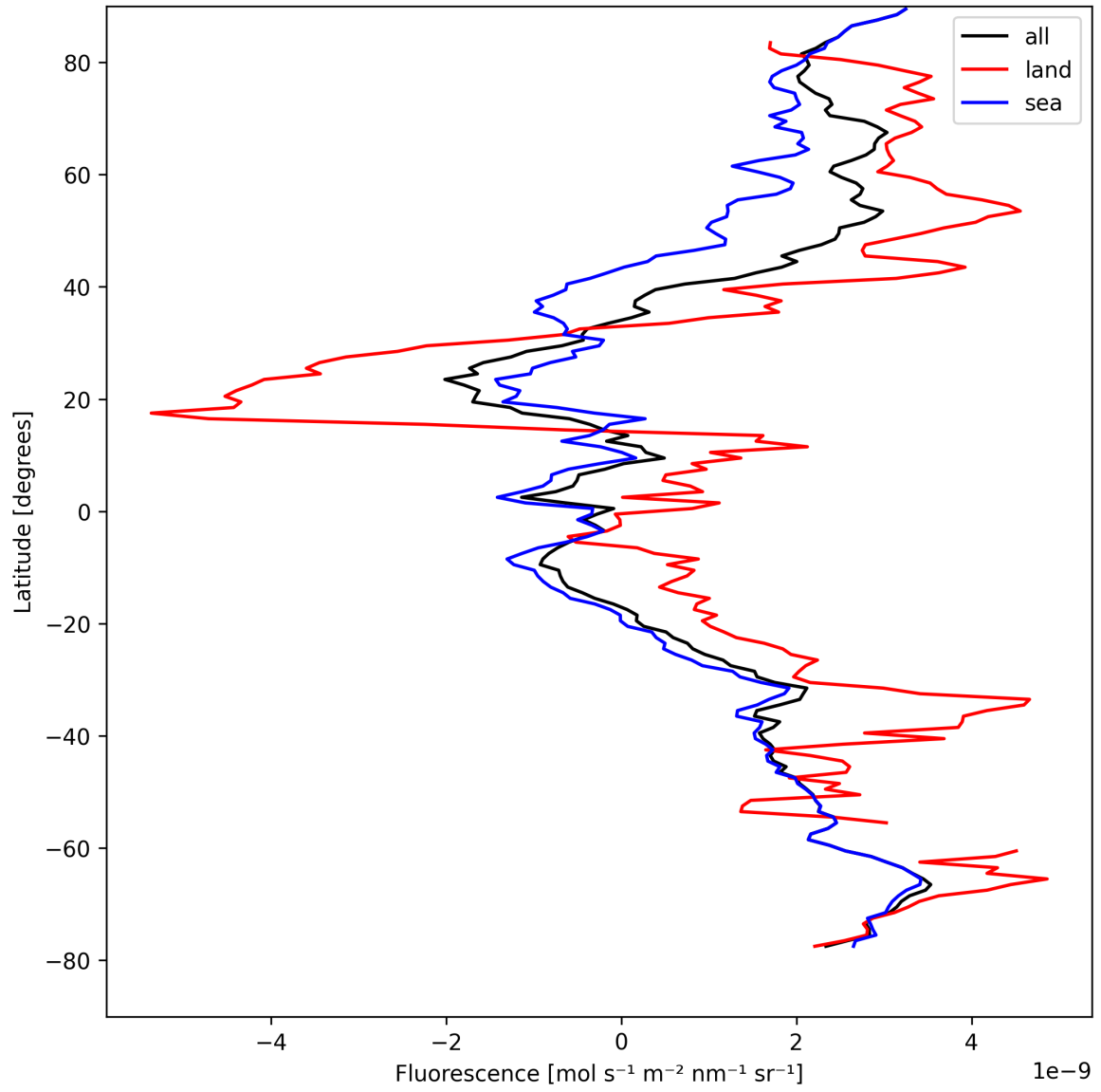
Figure 23: Zonal average of “Fluorescence” for 2025-08-25 to 2025-08-26.
