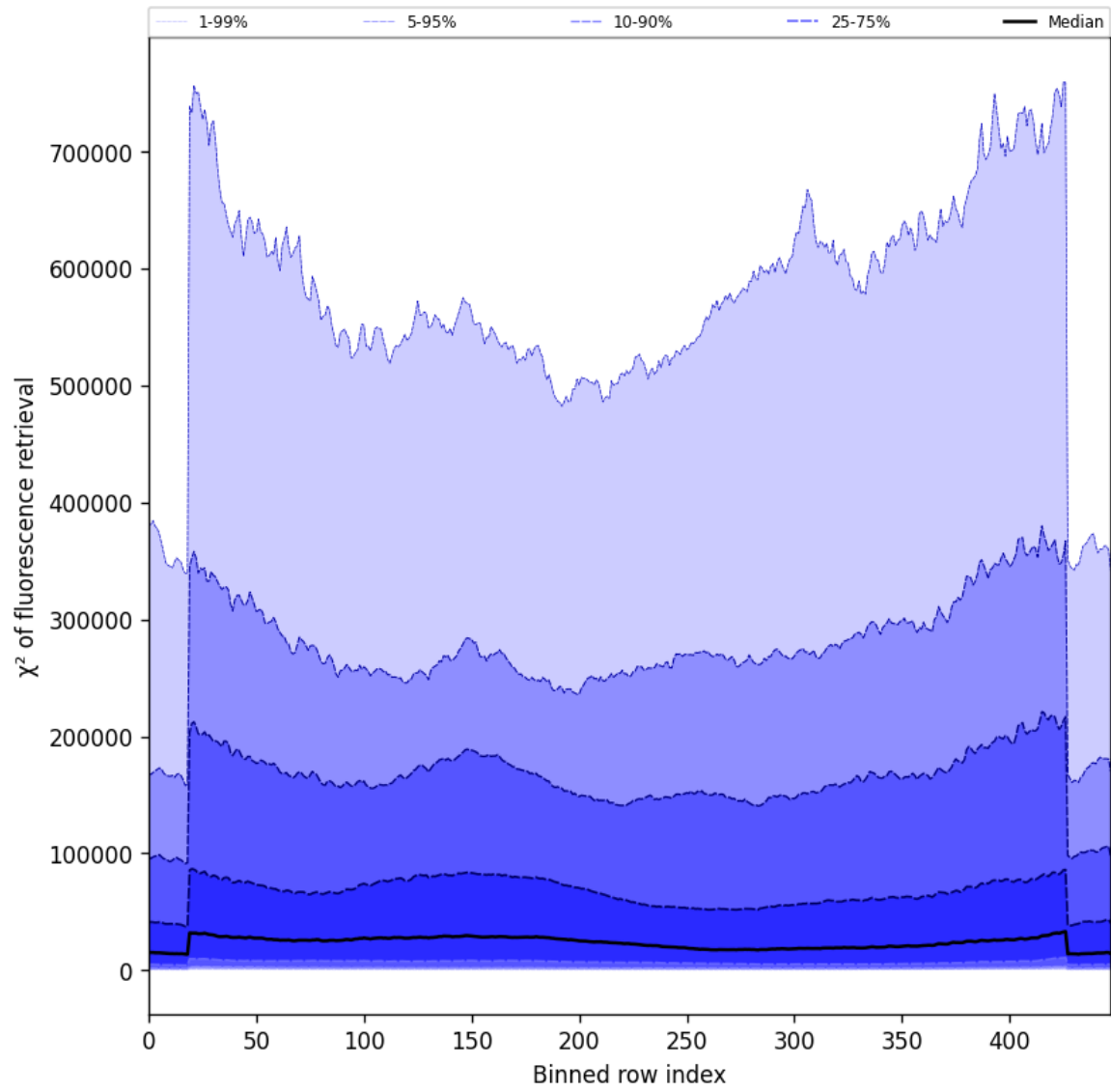
Figure 59: Along track statistics of “ \chi^2 of fluorescence retrieval” for 2025-08-25 to 2025-08-26
