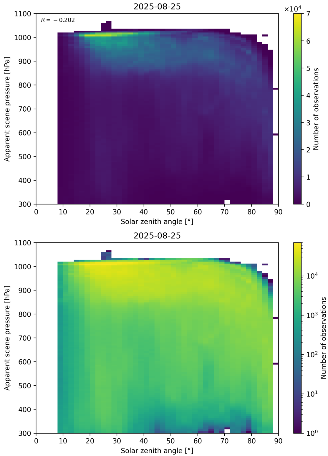
Figure 108: Scatter density plot of “Solar zenith angle” against “Apparent scene pressure” for 2025-08-25 to 2025-08-26.
