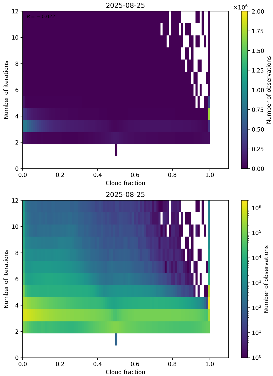
Figure 73: Scatter density plot of “Cloud fraction” against “Number of iterations” for 2025-08-25 to 2025-08-26.
