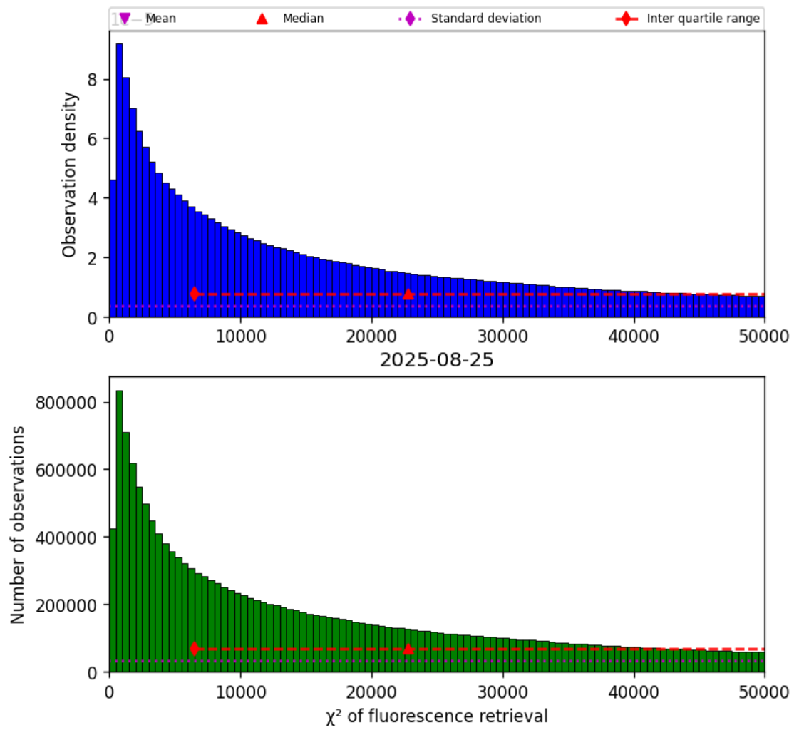
Figure 42: Histogram of “ \chi^2 of fluorescence retrieval” for 2025-08-25 to 2025-08-26
