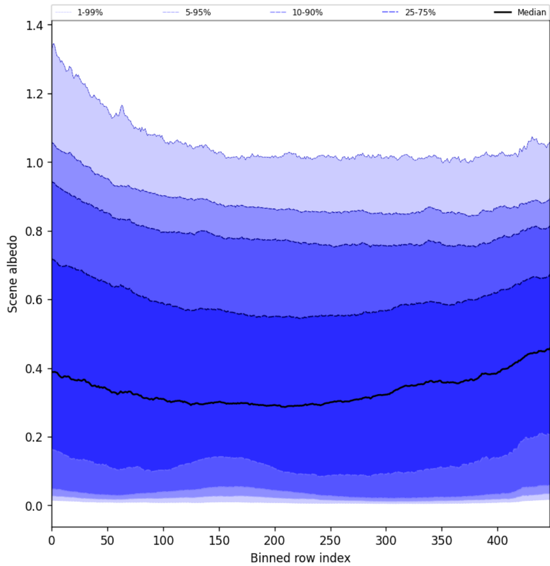
Figure 51: Along track statistics of “Scene albedo” for 2025-08-25 to 2025-08-26
