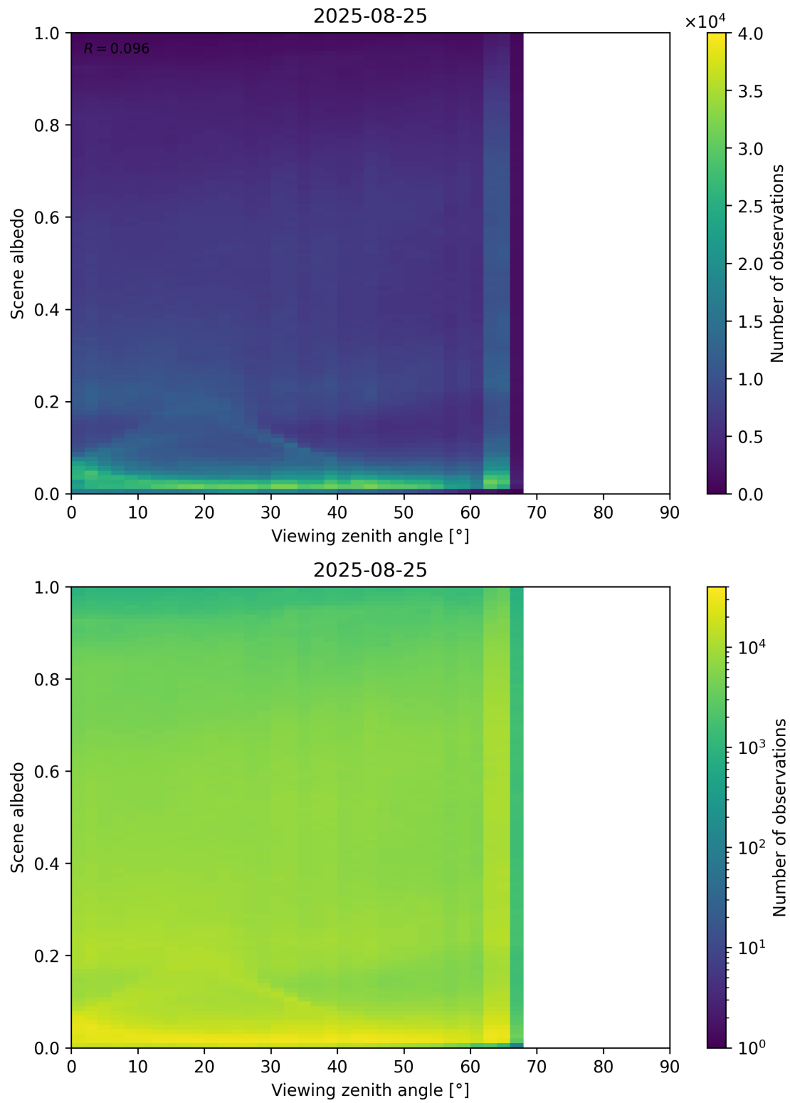
Figure 126: Scatter density plot of “Viewing zenith angle” against “Scene albedo” for 2025-08-25 to 2025-08-26.
