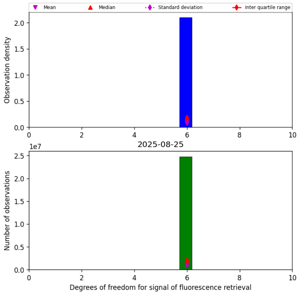
Figure 43: Histogram of “Degrees of freedom for signal of fluorescence retrieval” for 2025-08-25 to 2025-08-26
