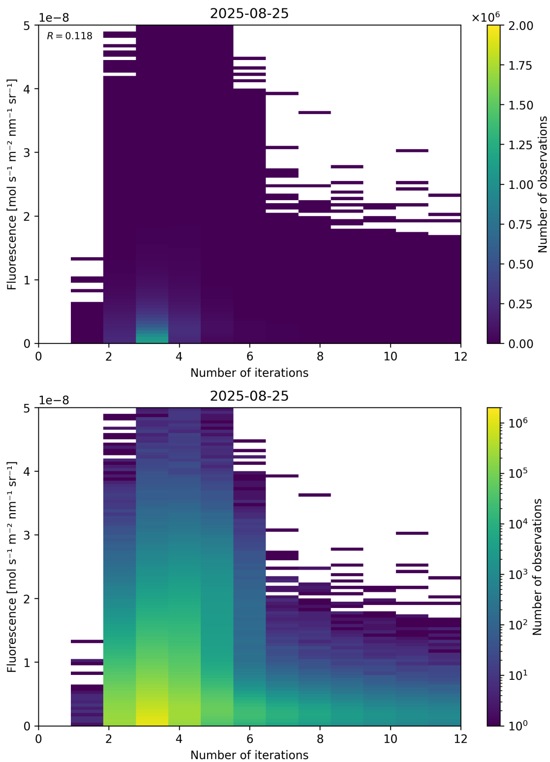
Figure 98: Scatter density plot of “Number of iterations” against “Fluorescence” for 2025-08-25 to 2025-08-26.
