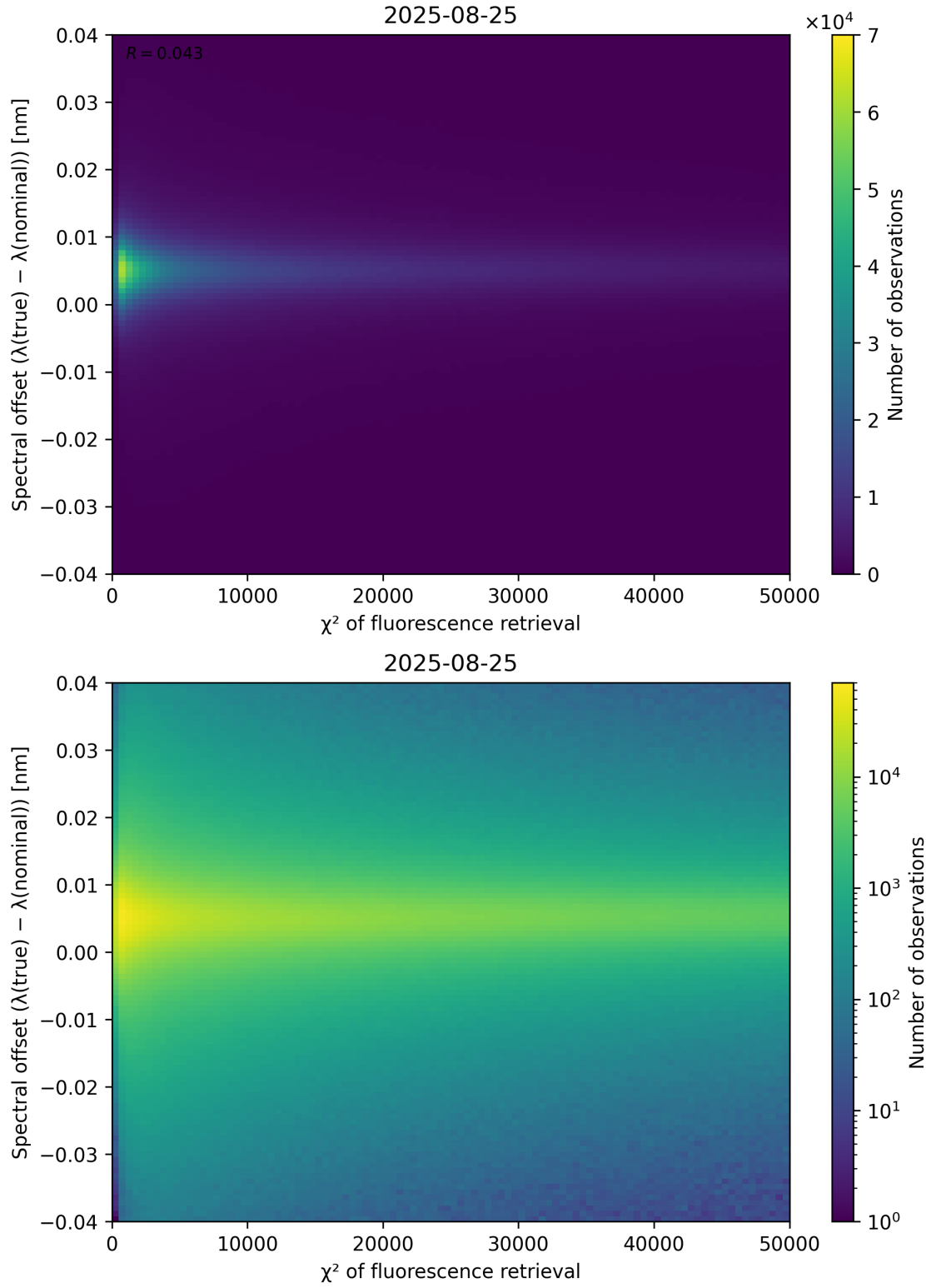
Figure 69: Scatter density plot of “ \chi^2 of fluorescence retrieval” against “Spectral offset ( \lambda_{\text{true}} - \lambda_{\text{nominal}} )” for 2025-08-25 to 2025-08-26.
