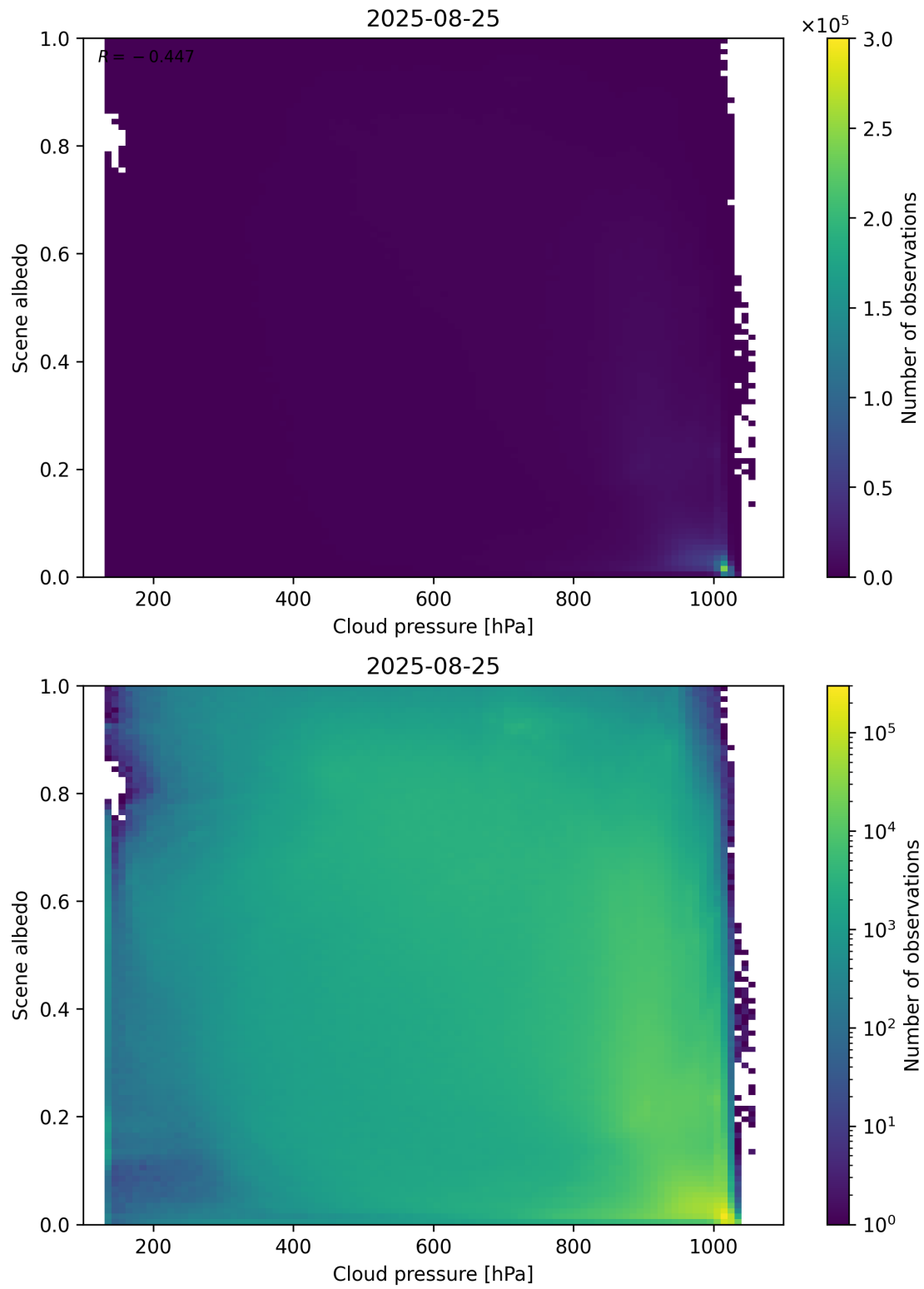
Figure 83: Scatter density plot of “Cloud pressure” against “Scene albedo” for 2025-08-25 to 2025-08-26.
