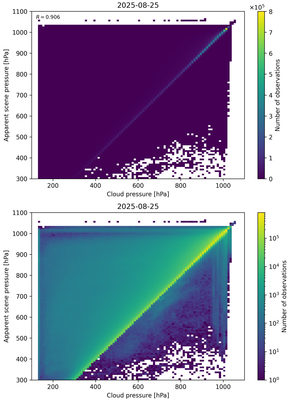
Figure 77: Scatter density plot of “Cloud pressure” against “Apparent scene pressure” for 2025-08-25 to 2025-08-26.
