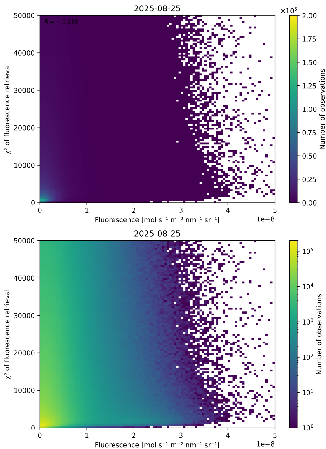
Figure 85: Scatter density plot of “Fluorescence” against “ \chi^2 of fluorescence retrieval” for 2025-08-25 to 2025-08-26.
