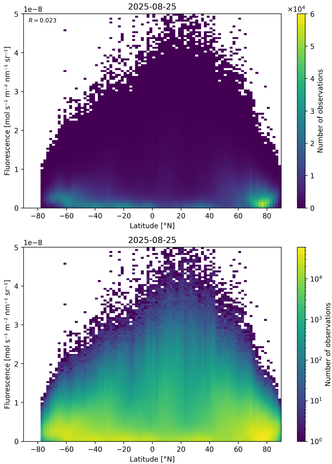
Figure 92: Scatter density plot of “Latitude” against “Fluorescence” for 2025-08-25 to 2025-08-26.
