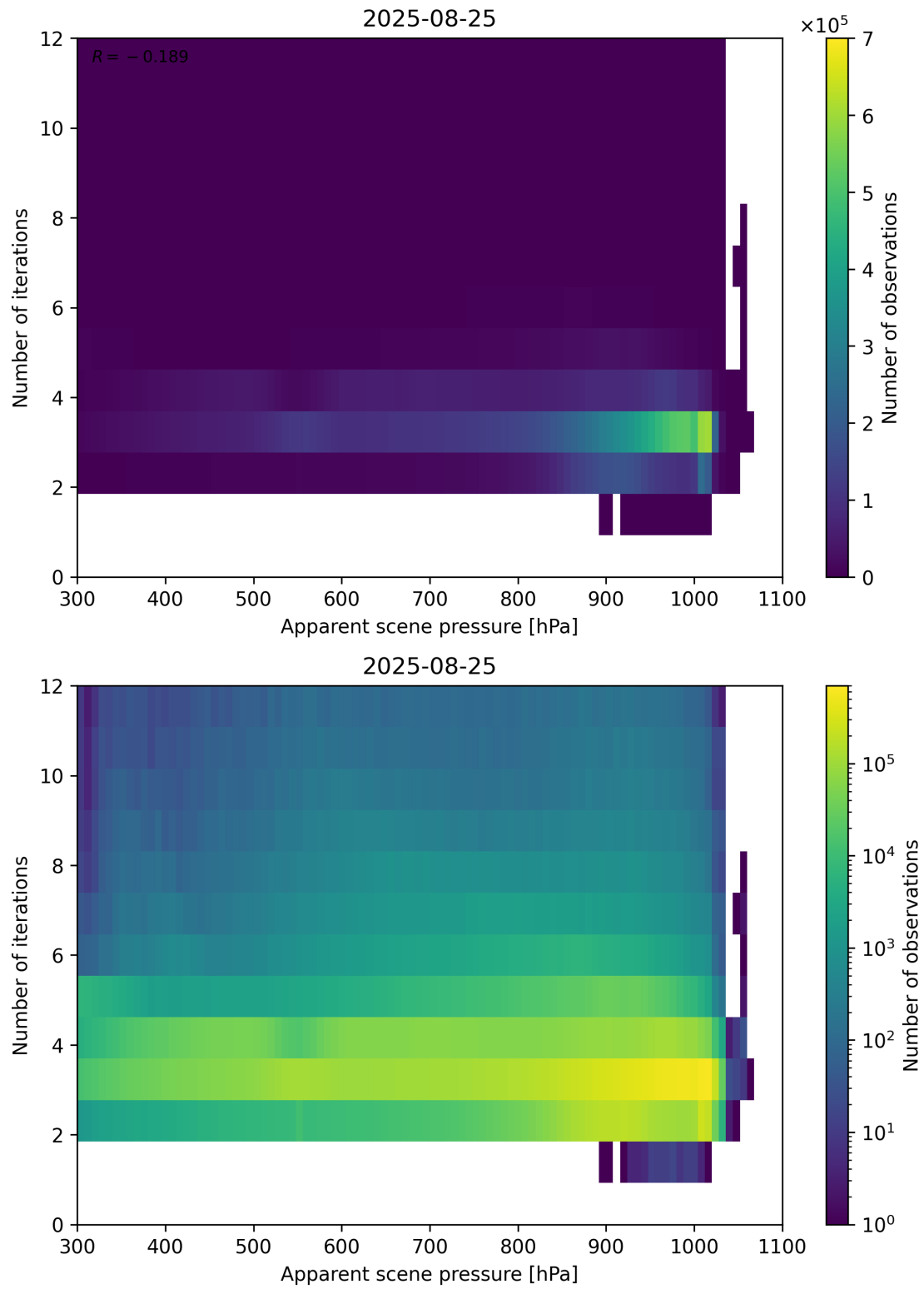
Figure 65: Scatter density plot of “Apparent scene pressure” against “Number of iterations” for 2025-08-25 to 2025-08-26.
