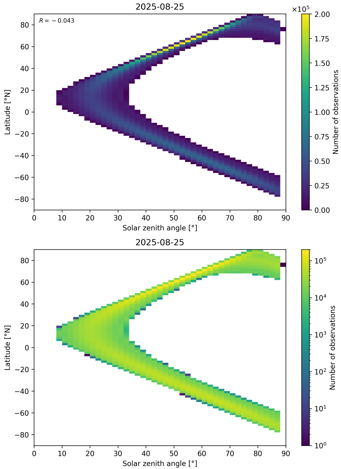
Figure 113: Scatter density plot of “Solar zenith angle” against “Latitude” for 2025-08-25 to 2025-08-26.
