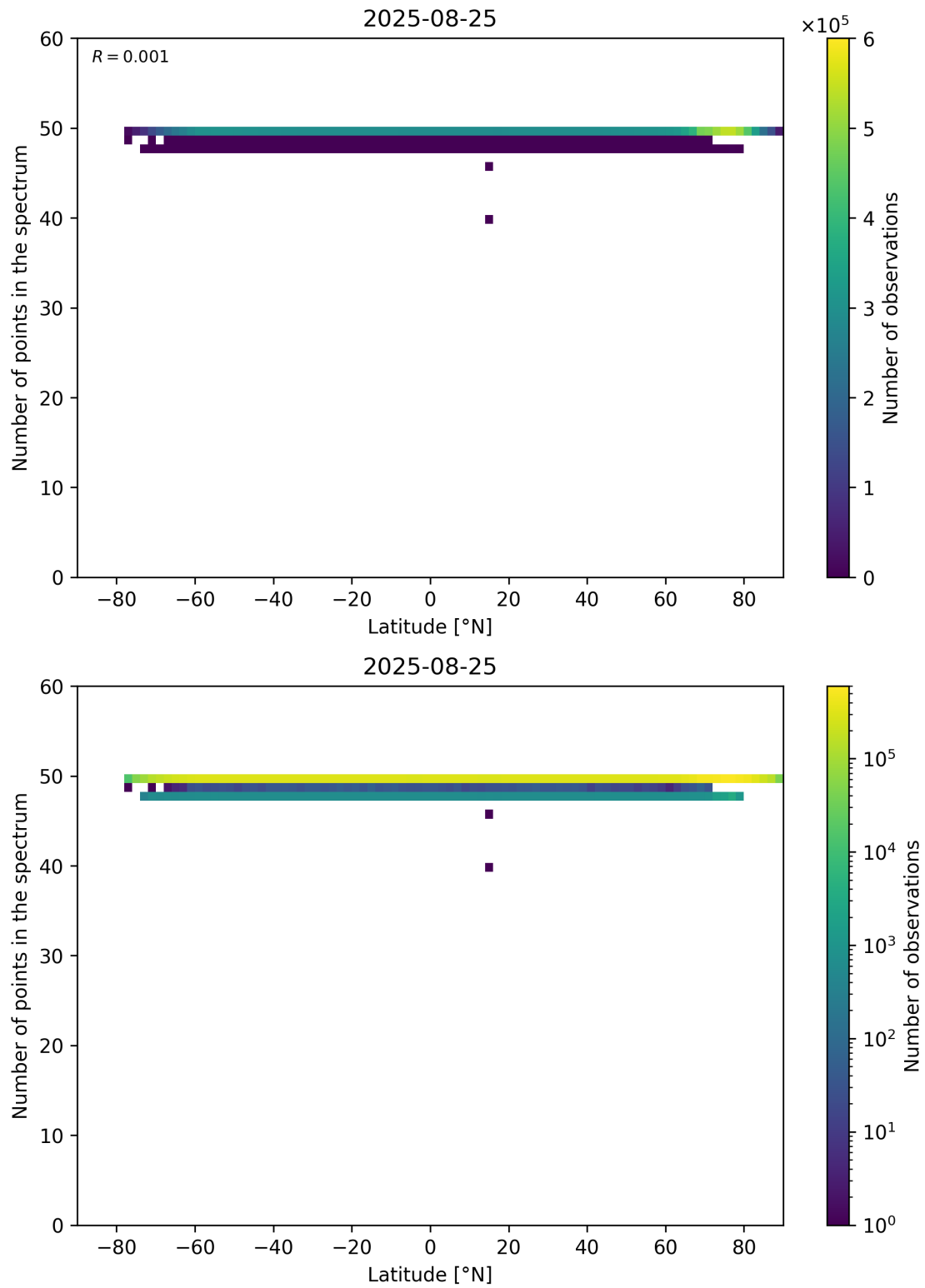
Figure 94: Scatter density plot of “Latitude” against “Number of points in the spectrum” for 2025-08-25 to 2025-08-26.
