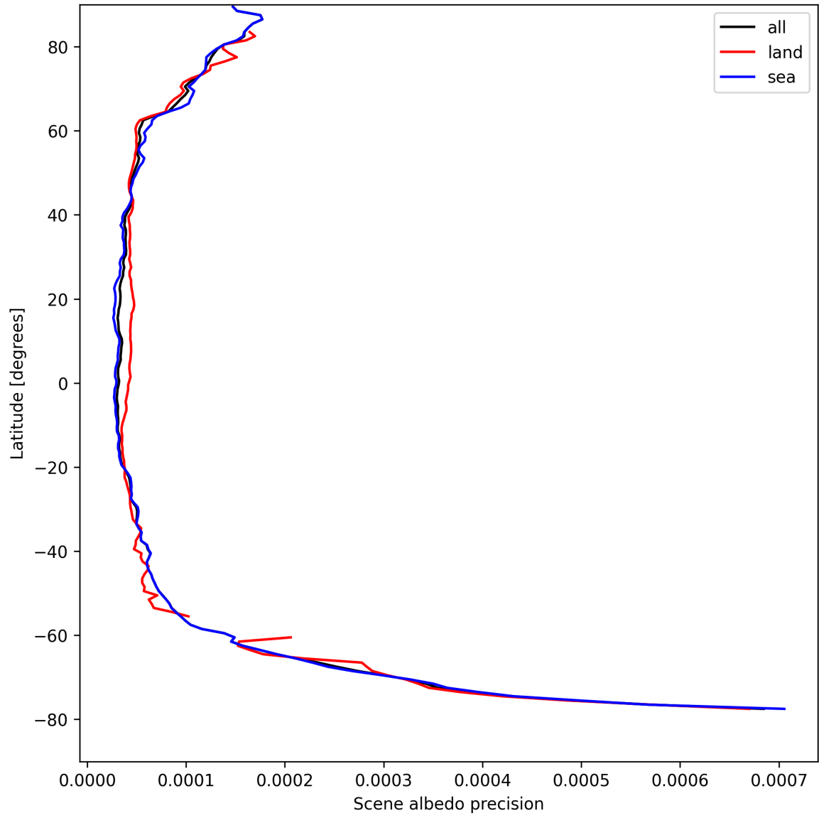
Figure 18: Zonal average of “Scene albedo precision” for 2025-08-25 to 2025-08-26.
