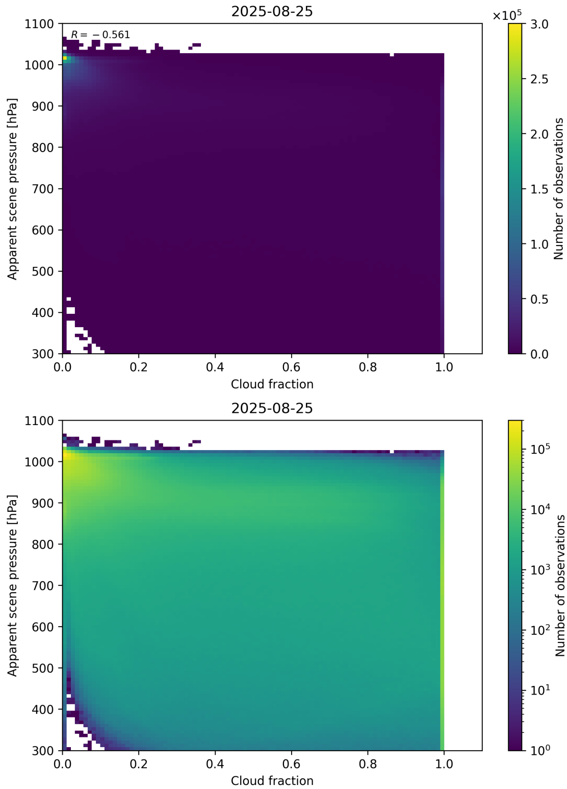
Figure 70: Scatter density plot of “Cloud fraction” against “Apparent scene pressure” for 2025-08-25 to 2025-08-26.
