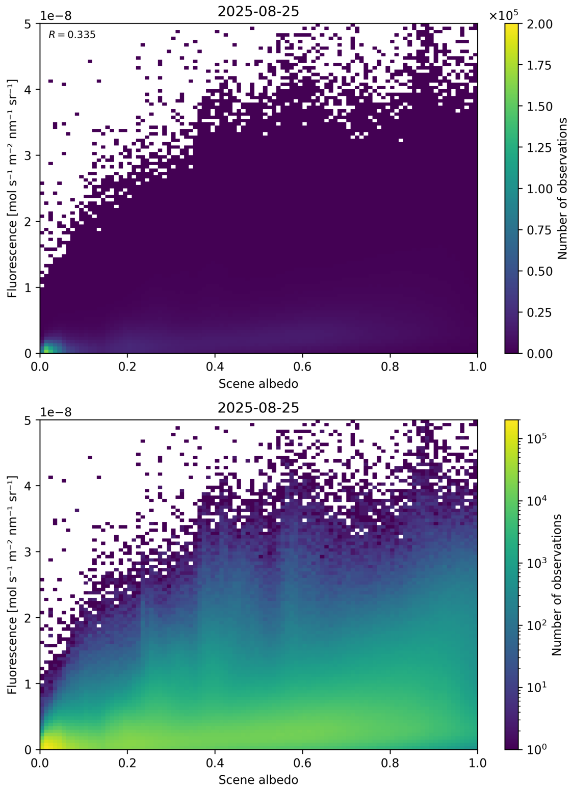
Figure 104: Scatter density plot of “Scene albedo” against “Fluorescence” for 2025-08-25 to 2025-08-26.
