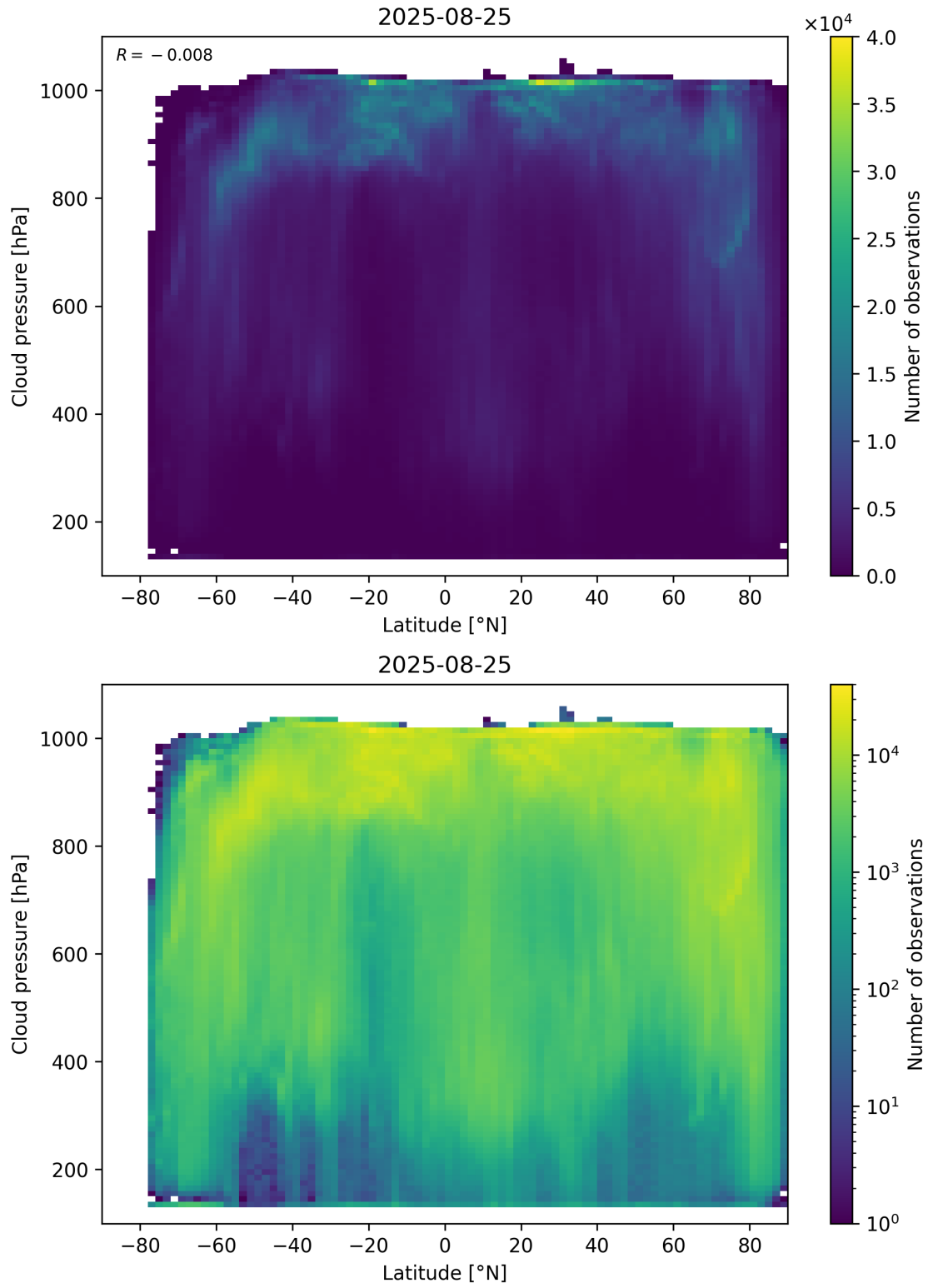
Figure 91: Scatter density plot of “Latitude” against “Cloud pressure” for 2025-08-25 to 2025-08-26.
