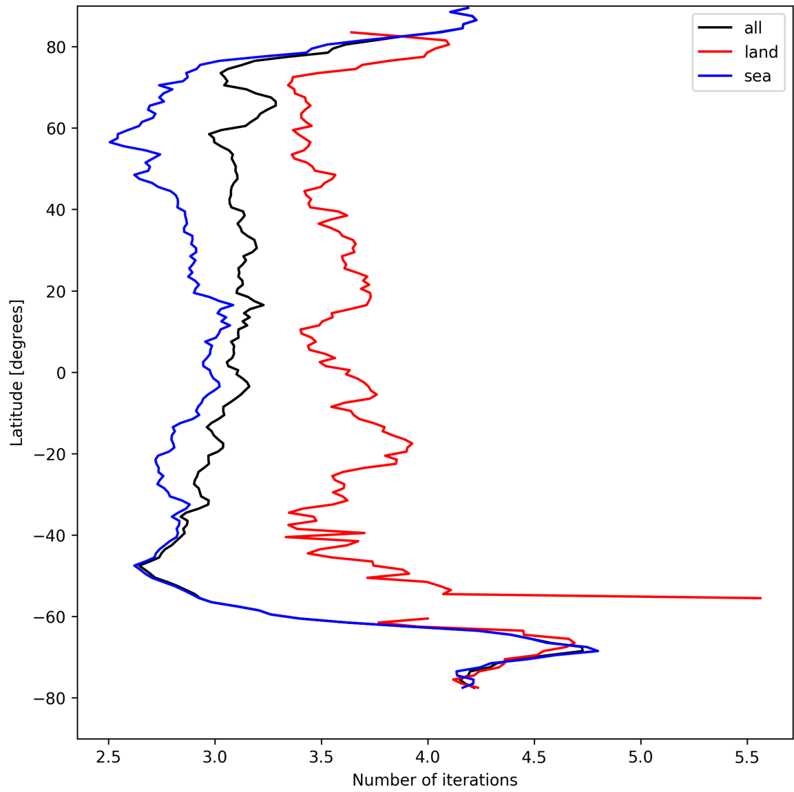
Figure 22: Zonal average of “Number of iterations” for 2025-08-25 to 2025-08-26.
