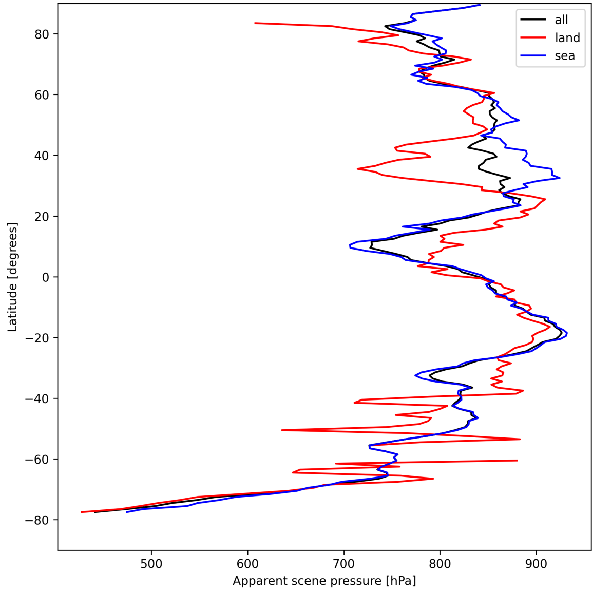
Figure 19: Zonal average of “Apparent scene pressure” for 2025-08-25 to 2025-08-26.
