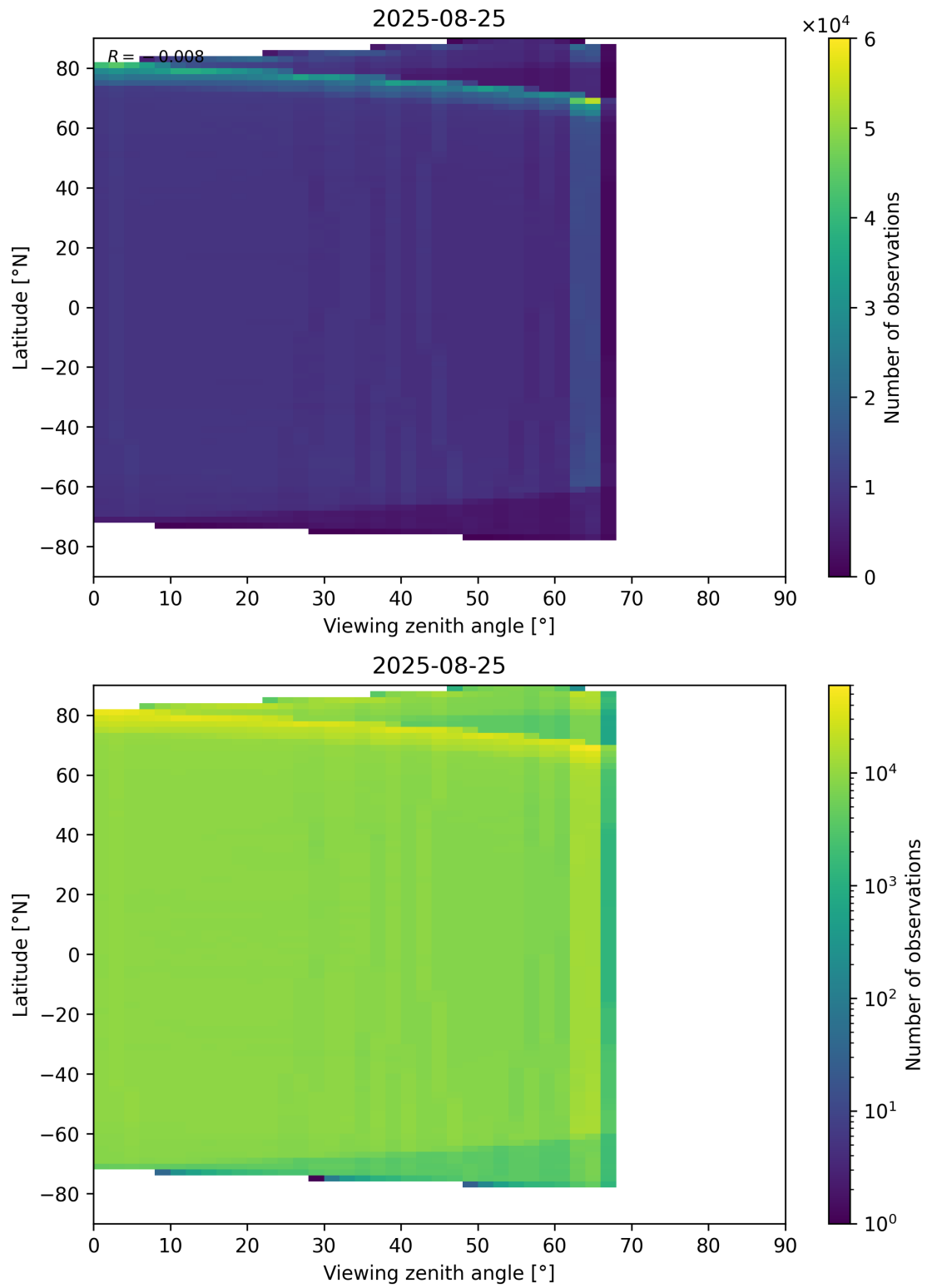
Figure 123: Scatter density plot of “Viewing zenith angle” against “Latitude” for 2025-08-25 to 2025-08-26.
