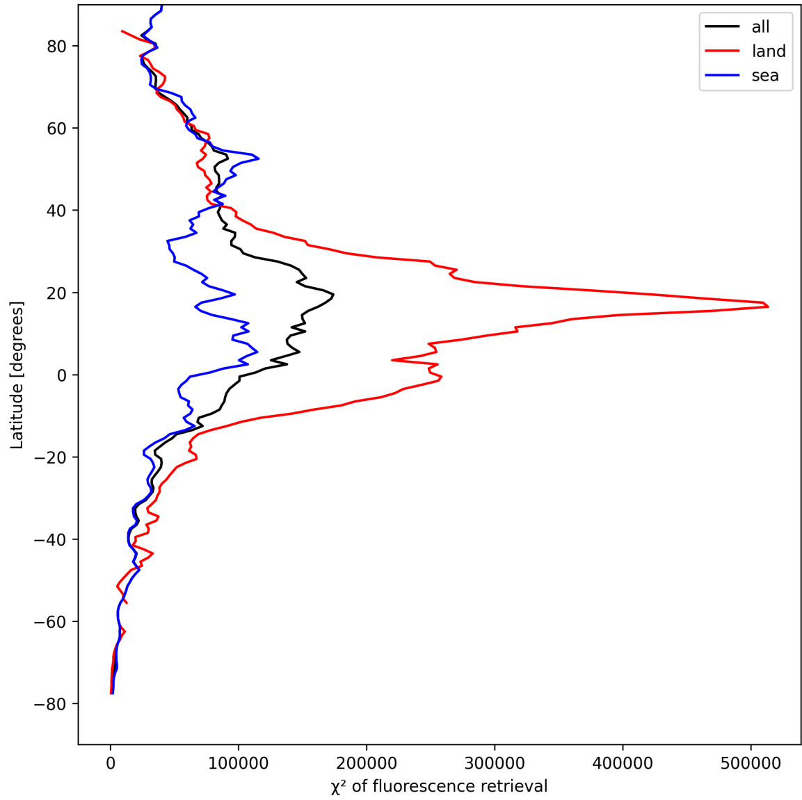
Figure 25: Zonal average of “ \chi^2 of fluorescence retrieval” for 2025-08-25 to 2025-08-26.
