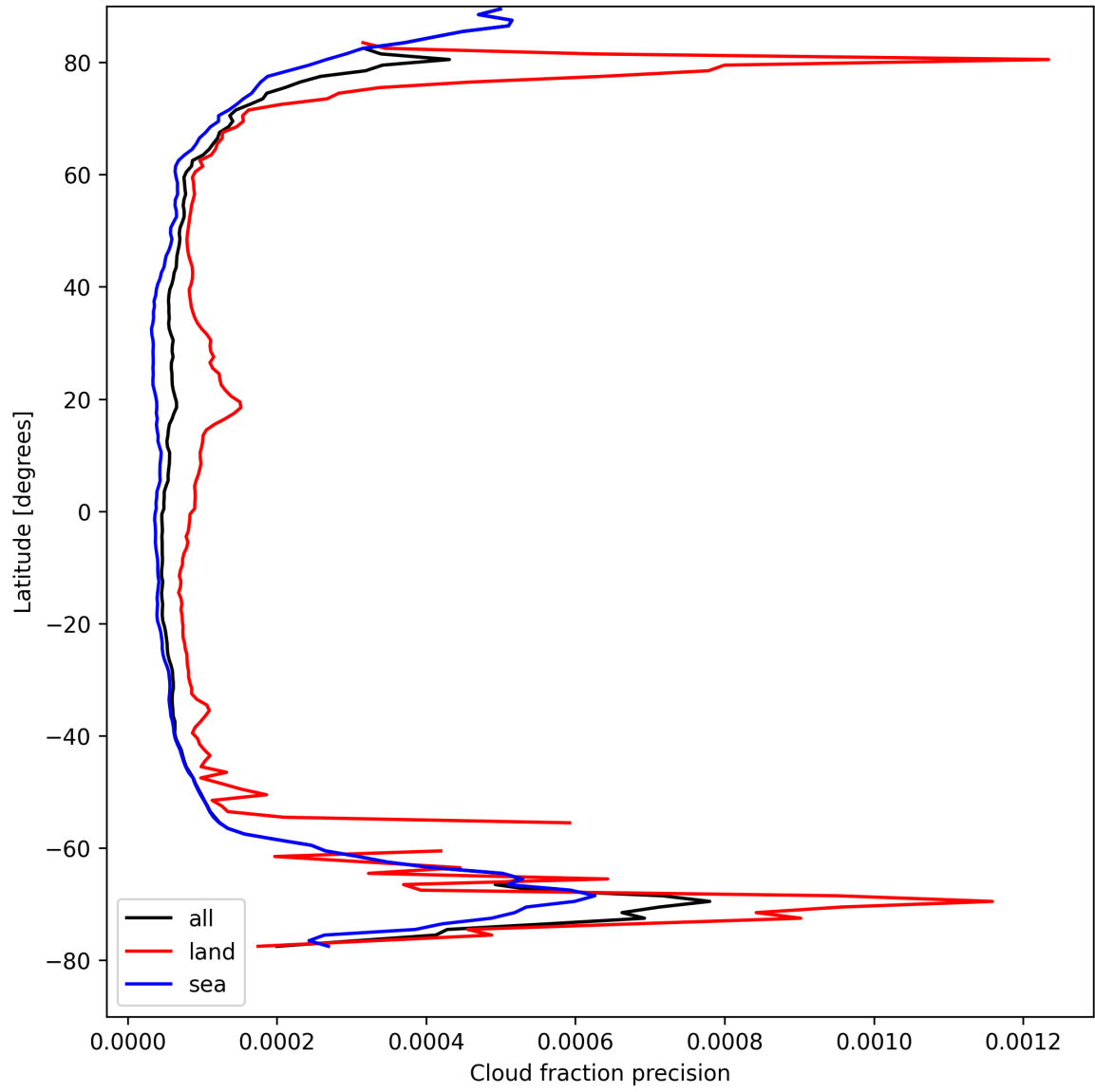
Figure 16: Zonal average of “Cloud fraction precision” for 2025-08-25 to 2025-08-26.
