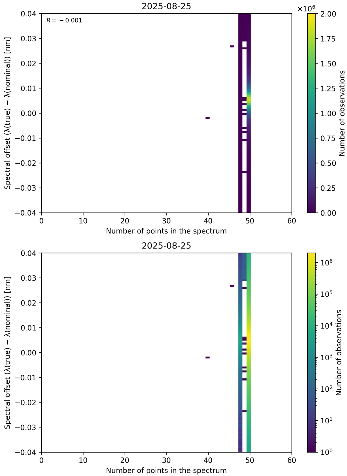
Figure 101: Scatter density plot of “Number of points in the spectrum” against “Spectral offset ( \lambda_{\text{true}} - \lambda_{\text{nominal}} )” for 2025-08-25 to 2025-08-26.
