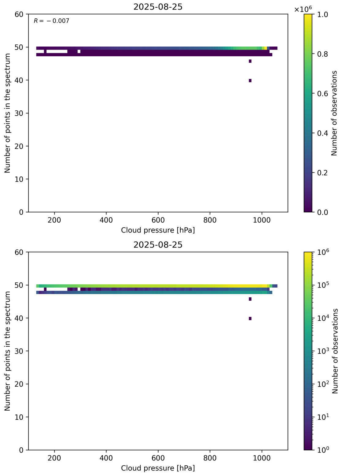
Figure 82: Scatter density plot of “Cloud pressure” against “Number of points in the spectrum” for 2025-08-25 to 2025-08-26.
