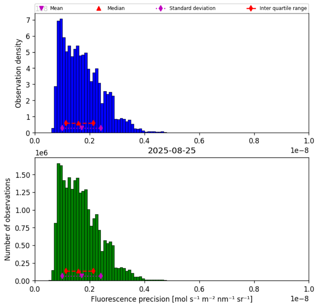
Figure 41: Histogram of “Fluorescence precision” for 2025-08-25 to 2025-08-26
