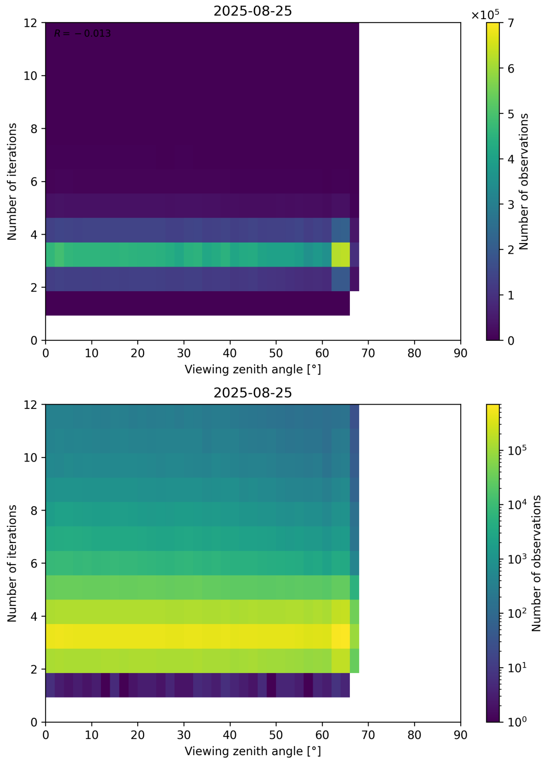
Figure 124: Scatter density plot of “Viewing zenith angle” against “Number of iterations” for 2025-08-25 to 2025-08-26.
