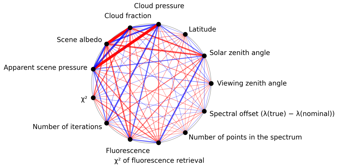
Figure 1: Map of correlation graph for 2025-08-25 to 2025-08-26.
