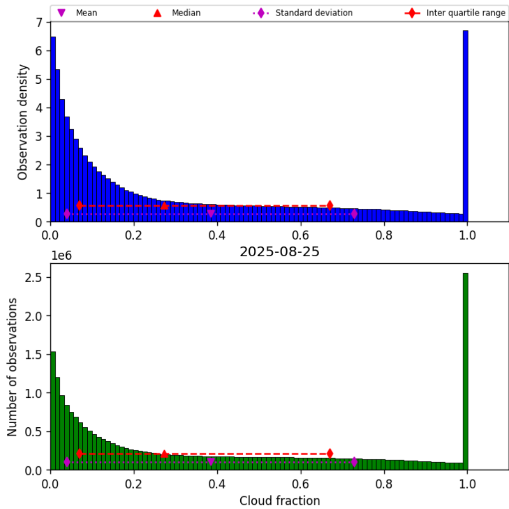
Figure 32: Histogram of “Cloud fraction” for 2025-08-25 to 2025-08-26
