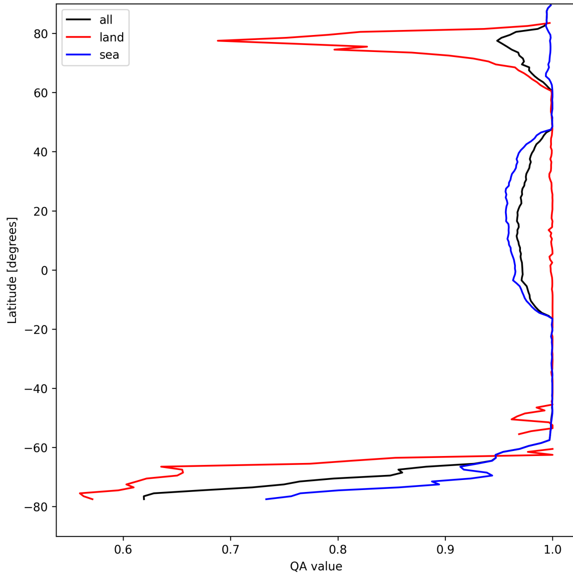
Figure 12: Zonal average of “QA value” for 2025-08-25 to 2025-08-26.
