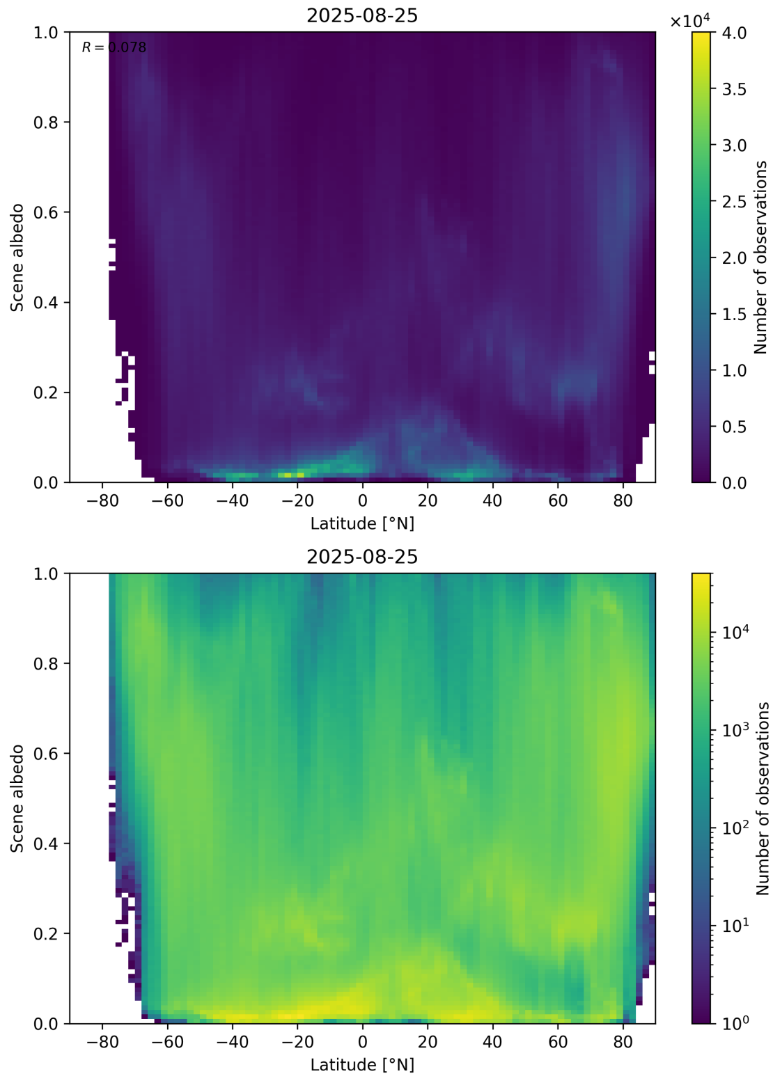
Figure 95: Scatter density plot of “Latitude” against “Scene albedo” for 2025-08-25 to 2025-08-26.
