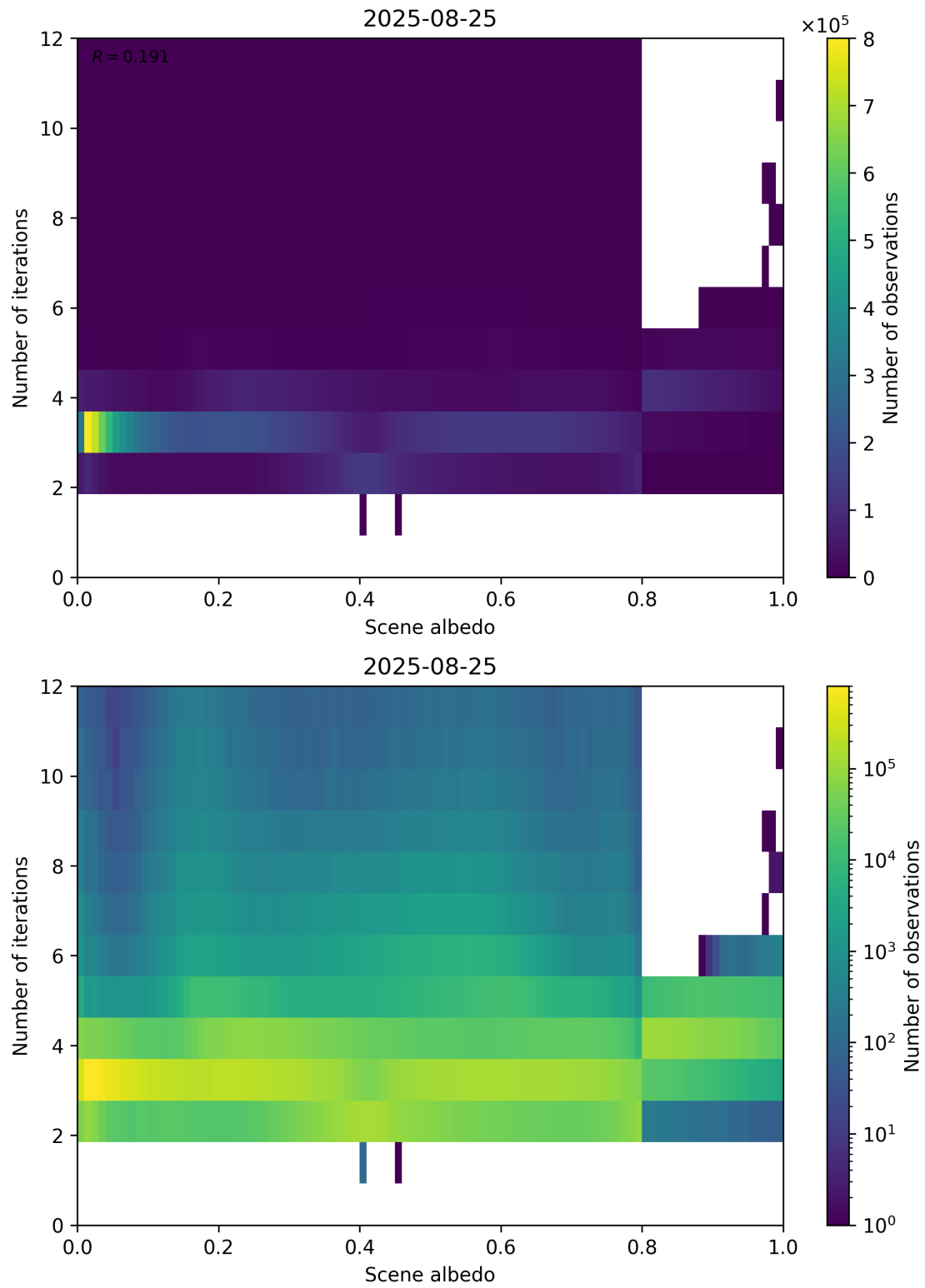
Figure 105: Scatter density plot of “Scene albedo” against “Number of iterations” for 2025-08-25 to 2025-08-26.
