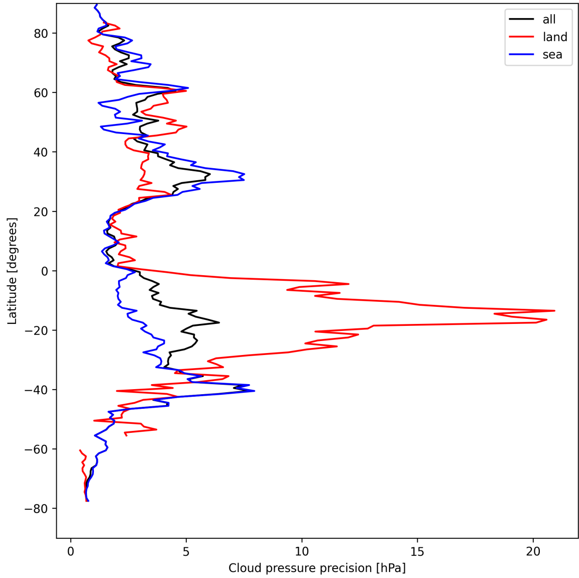
Figure 14: Zonal average of “Cloud pressure precision” for 2025-08-25 to 2025-08-26.
