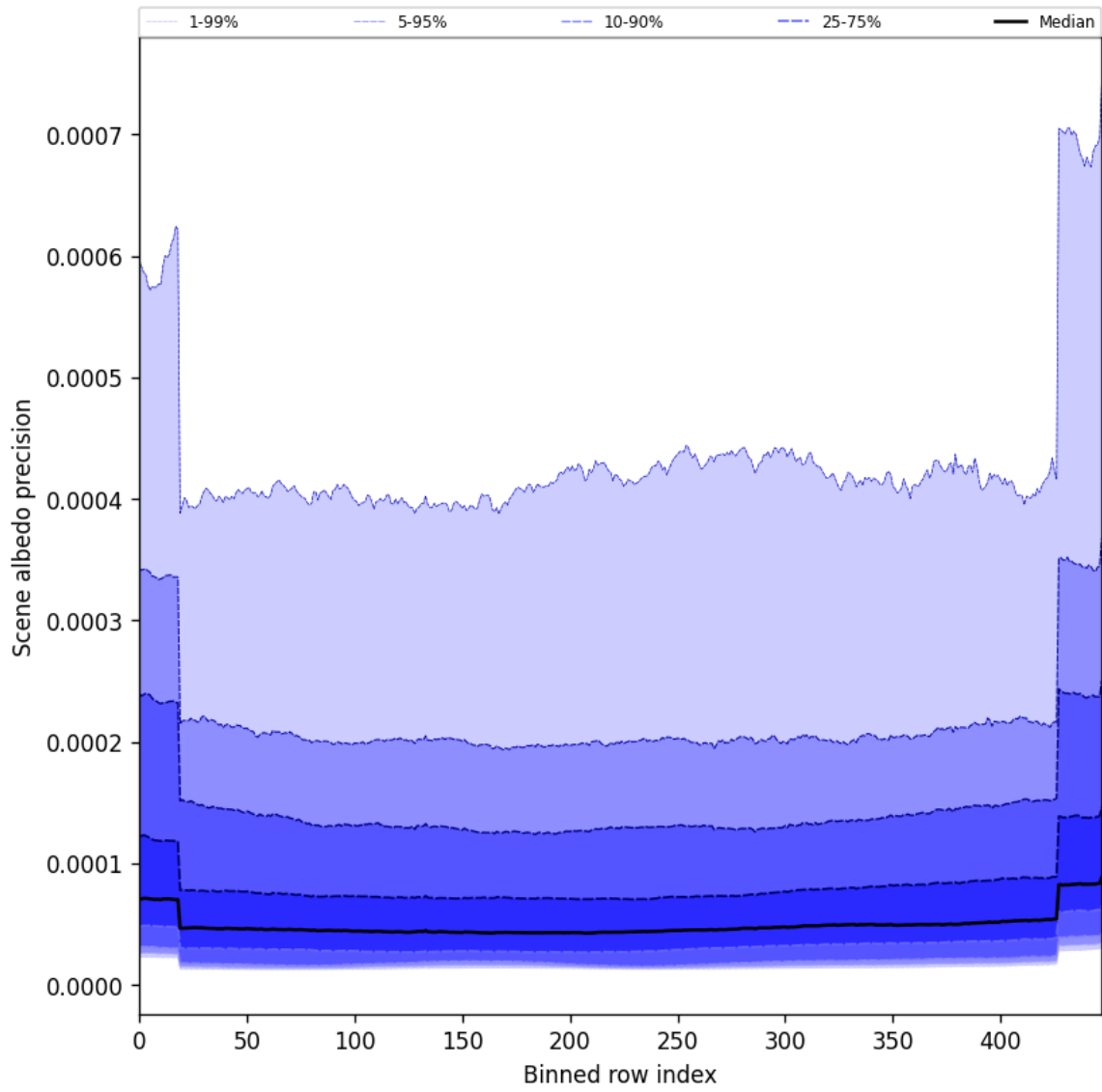
Figure 52: Along track statistics of “Scene albedo precision” for 2025-08-25 to 2025-08-26
