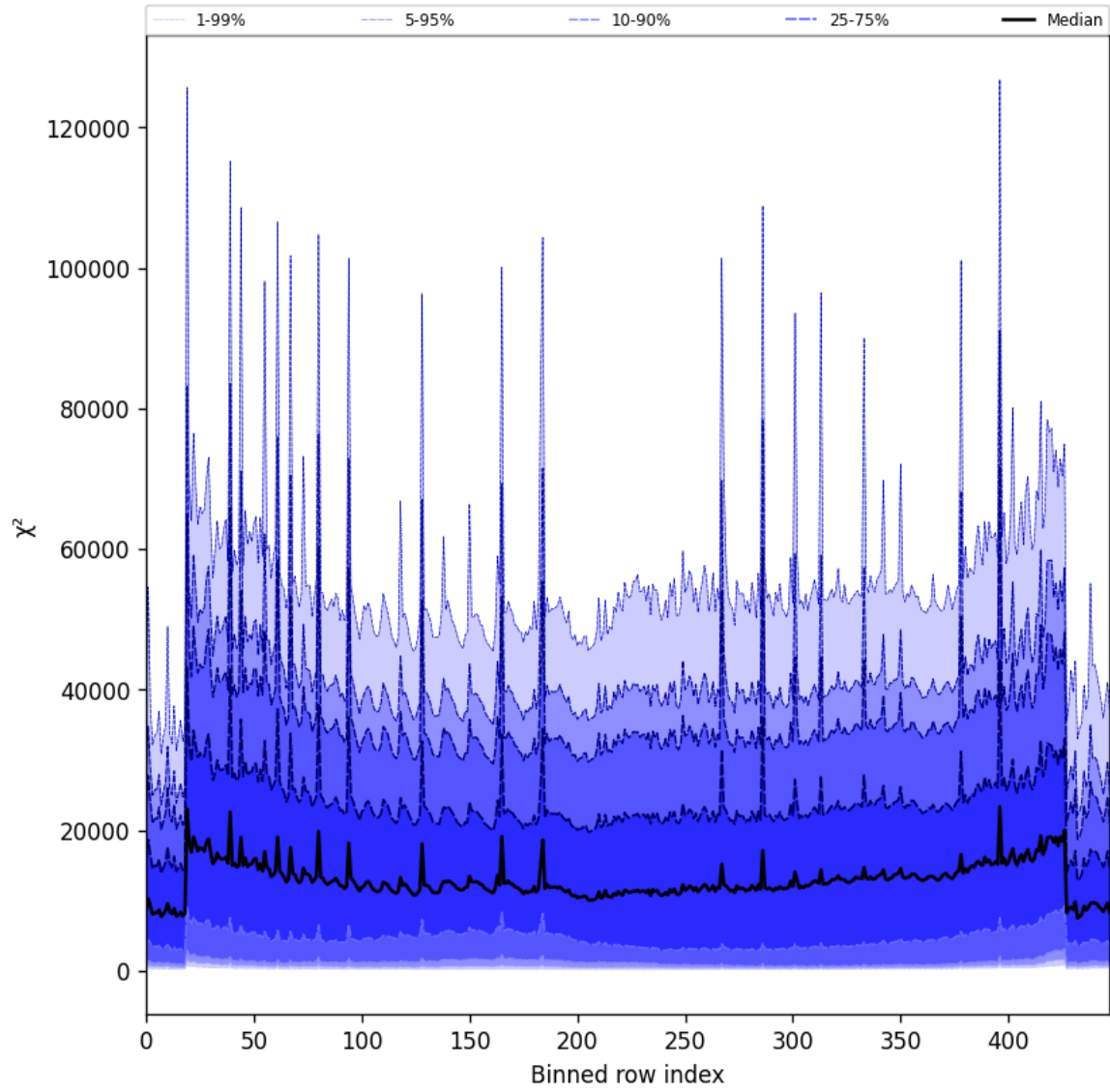
Figure 55: Along track statistics of “ \chi^2 ” for 2025-08-25 to 2025-08-26
