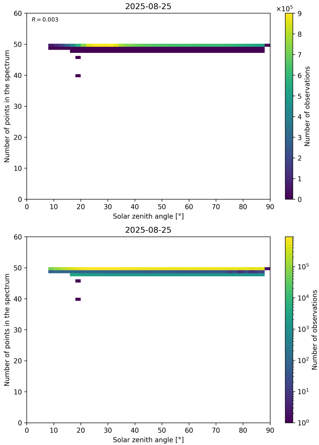
Figure 115: Scatter density plot of “Solar zenith angle” against “Number of points in the spectrum” for 2025-08-25 to 2025-08-26.
