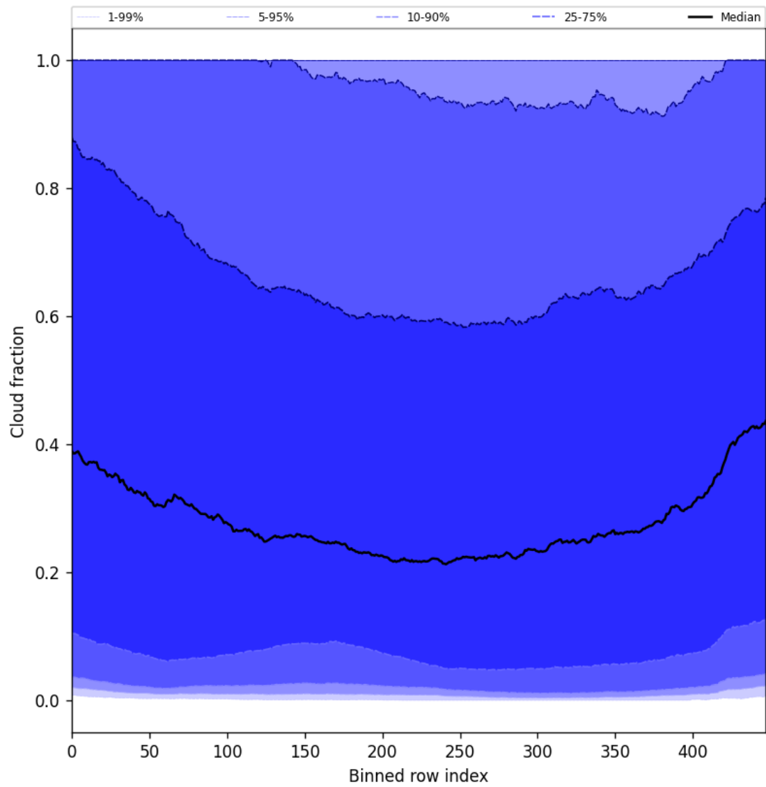
Figure 49: Along track statistics of “Cloud fraction” for 2025-08-25 to 2025-08-26
