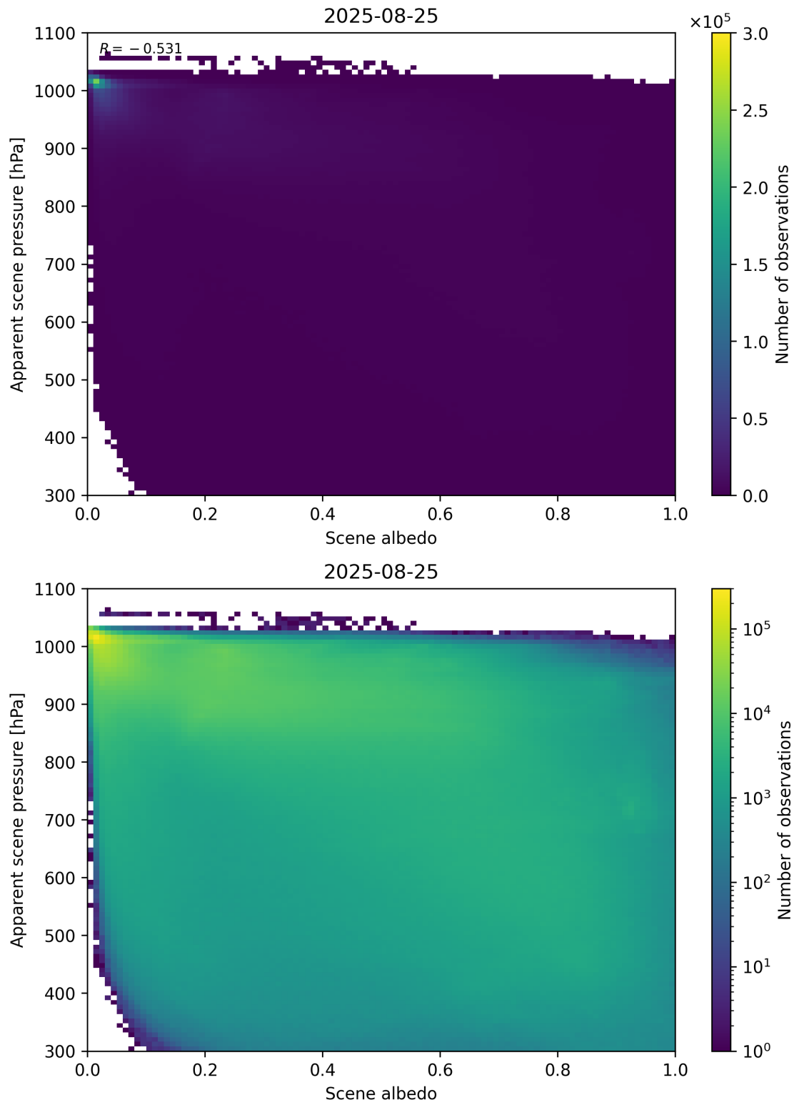
Figure 102: Scatter density plot of “Scene albedo” against “Apparent scene pressure” for 2025-08-25 to 2025-08-26.
