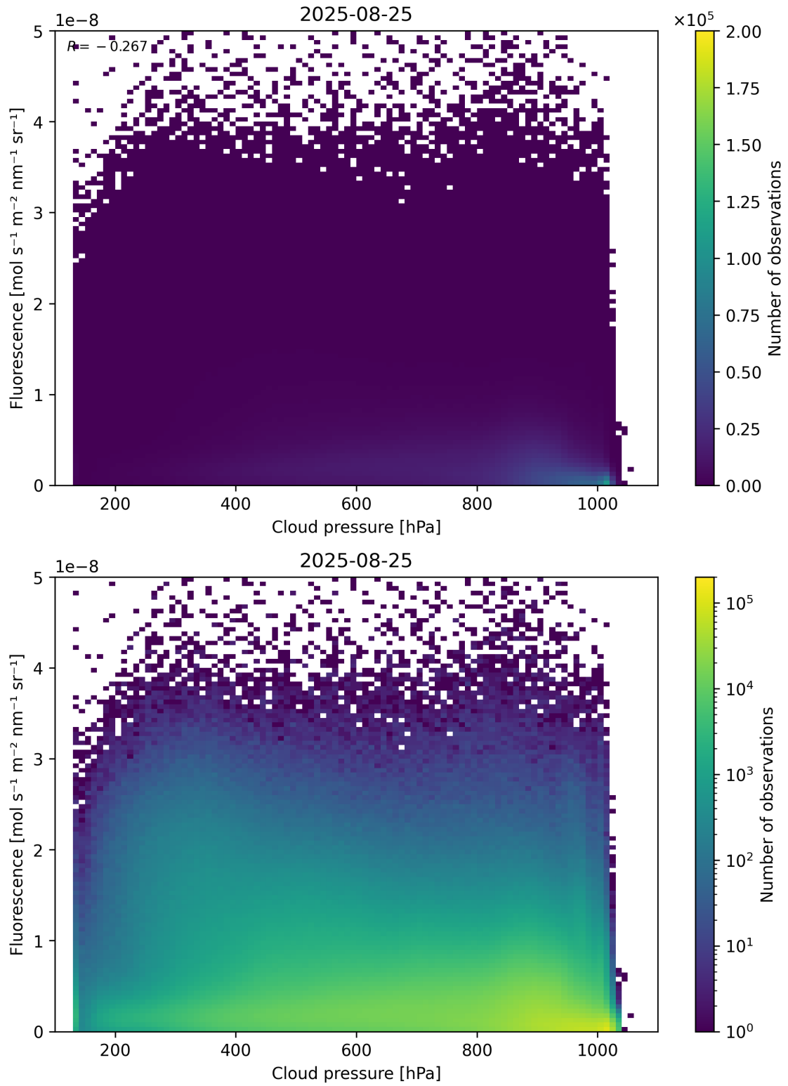
Figure 80: Scatter density plot of “Cloud pressure” against “Fluorescence” for 2025-08-25 to 2025-08-26.
