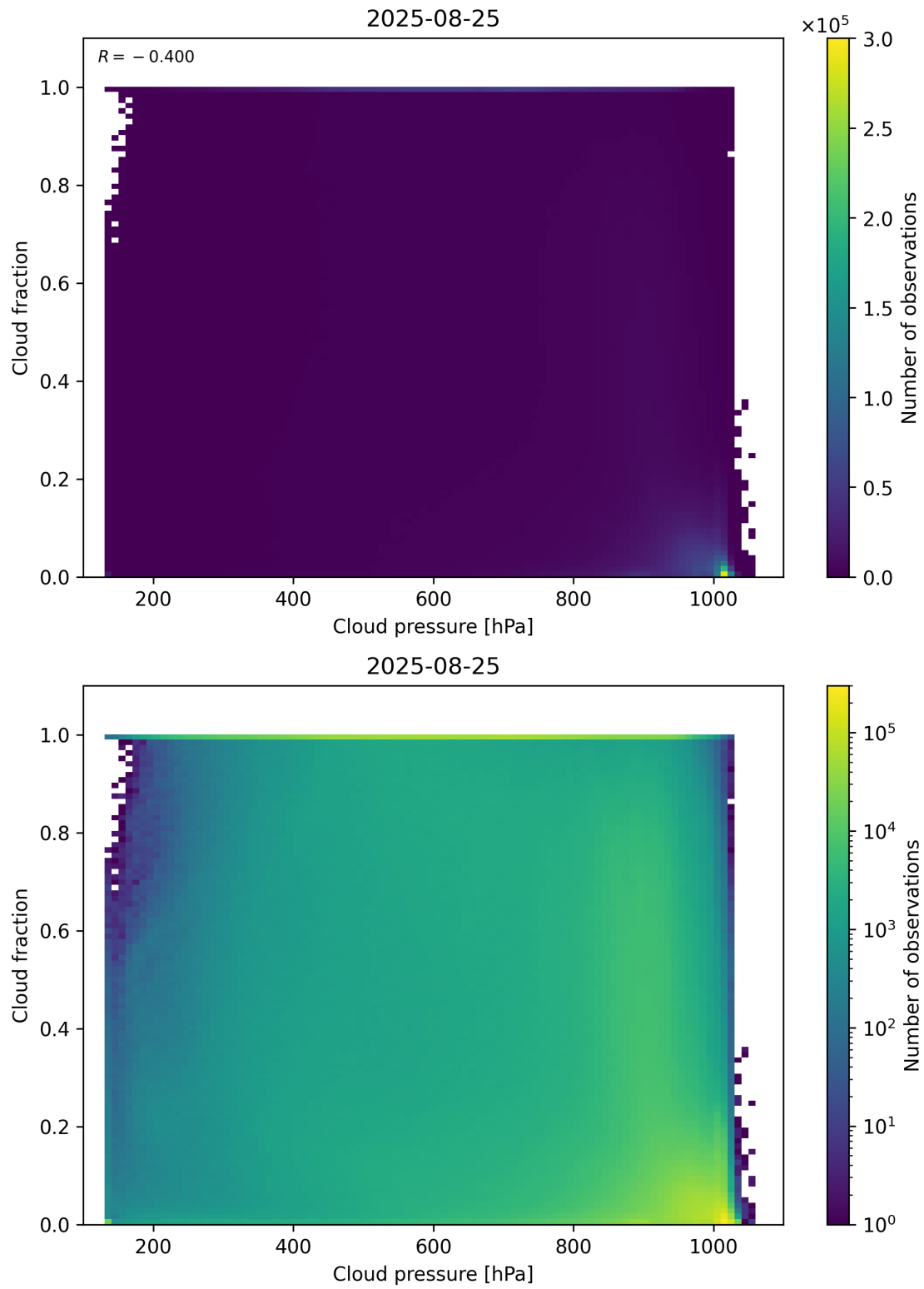
Figure 79: Scatter density plot of “Cloud pressure” against “Cloud fraction” for 2025-08-25 to 2025-08-26.
