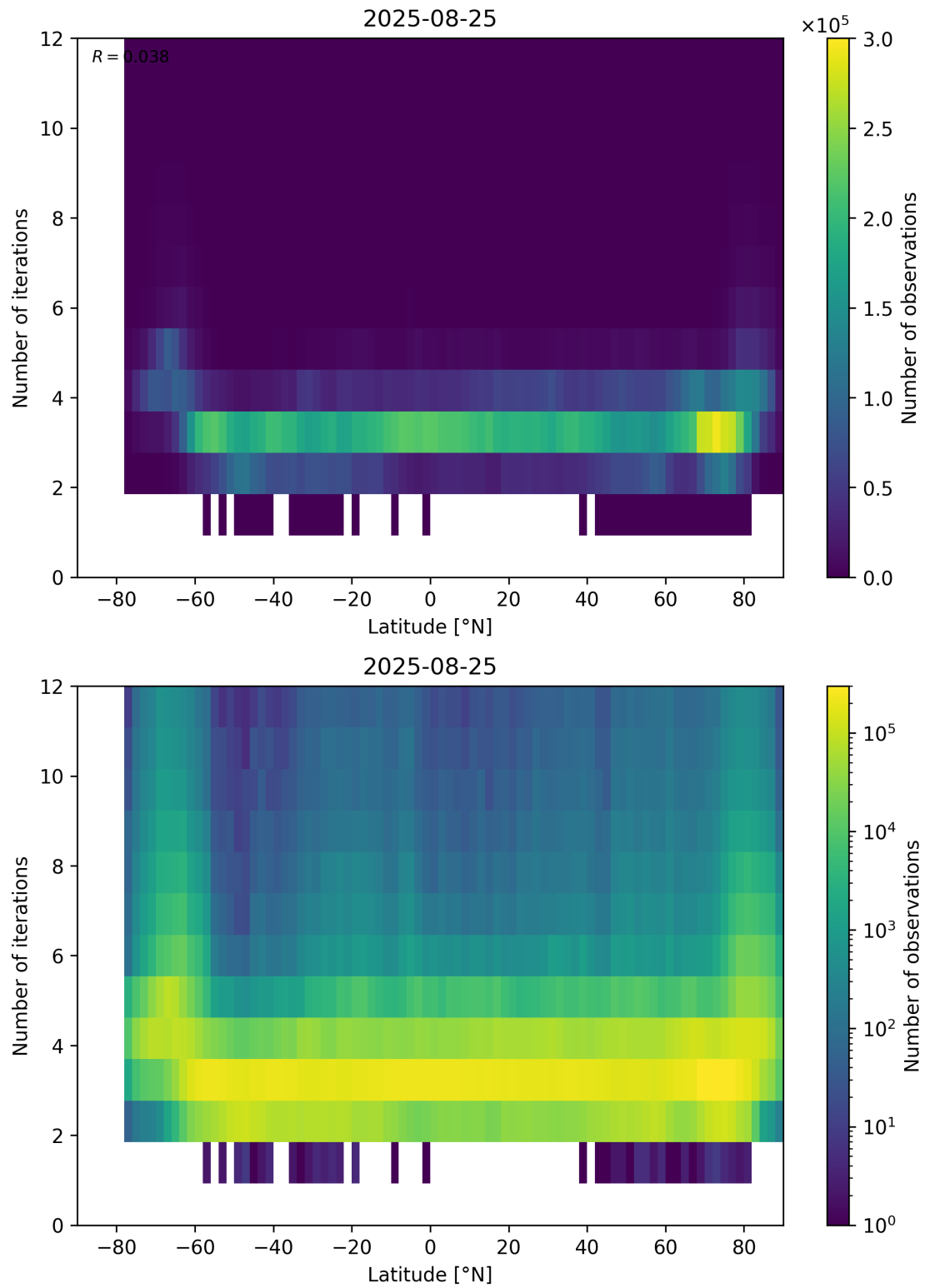
Figure 93: Scatter density plot of “Latitude” against “Number of iterations” for 2025-08-25 to 2025-08-26.
