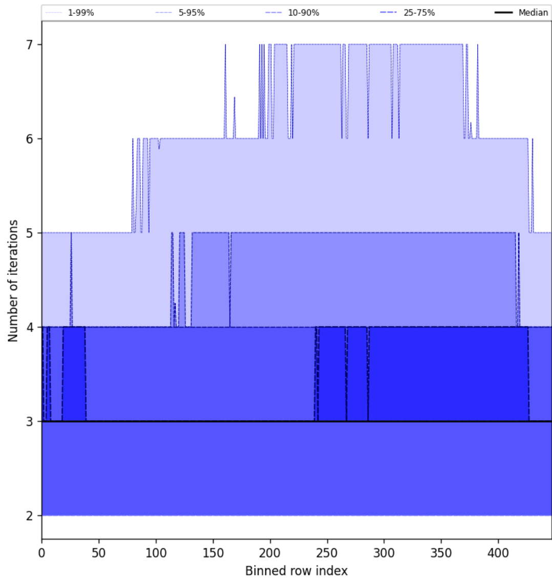
Figure 56: Along track statistics of “Number of iterations” for 2025-08-25 to 2025-08-26
