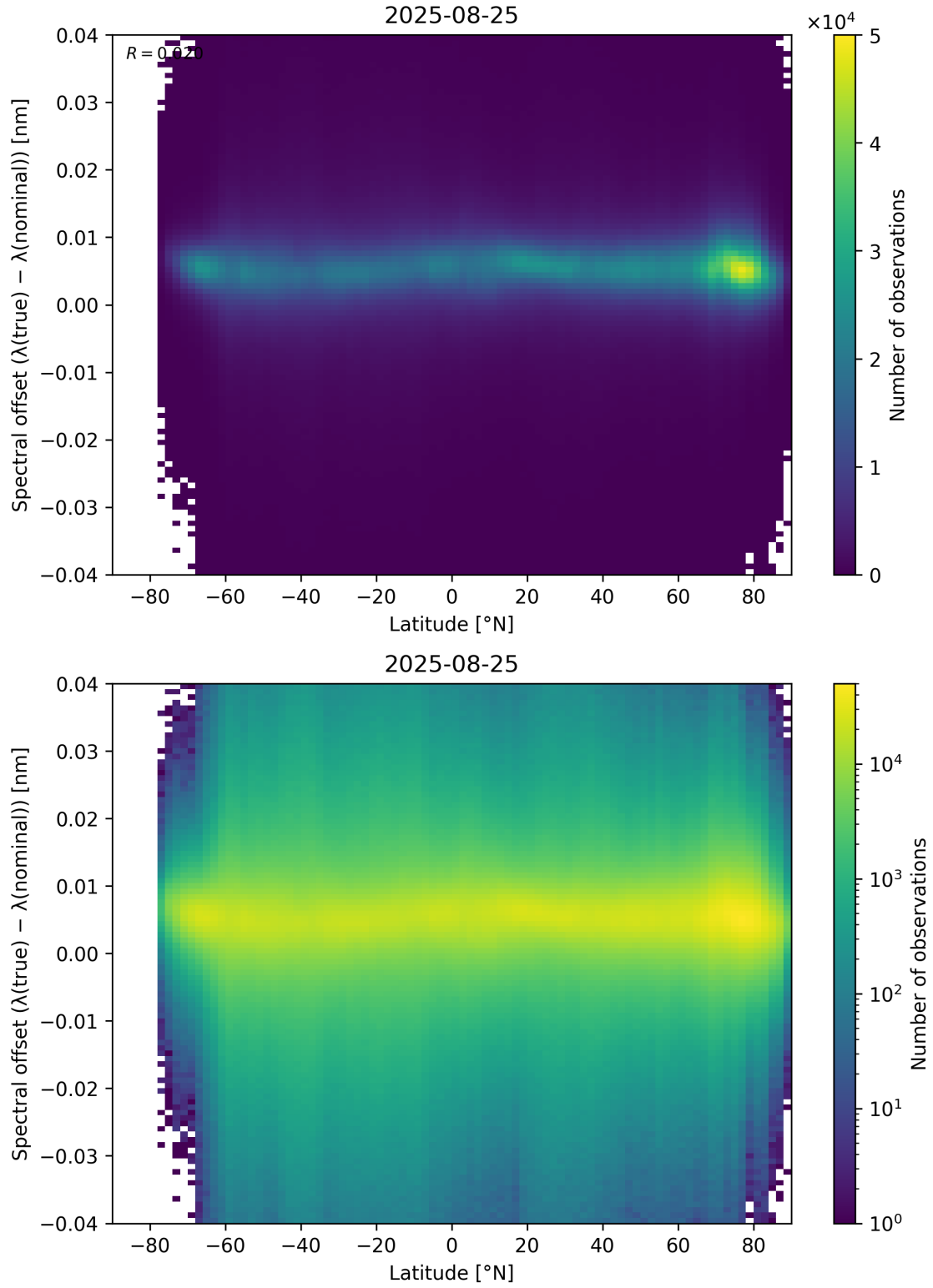
Figure 96: Scatter density plot of “Latitude” against “Spectral offset ( \lambda_{\text{true}} - \lambda_{\text{nominal}} )” for 2025-08-25 to 2025-08-26.
