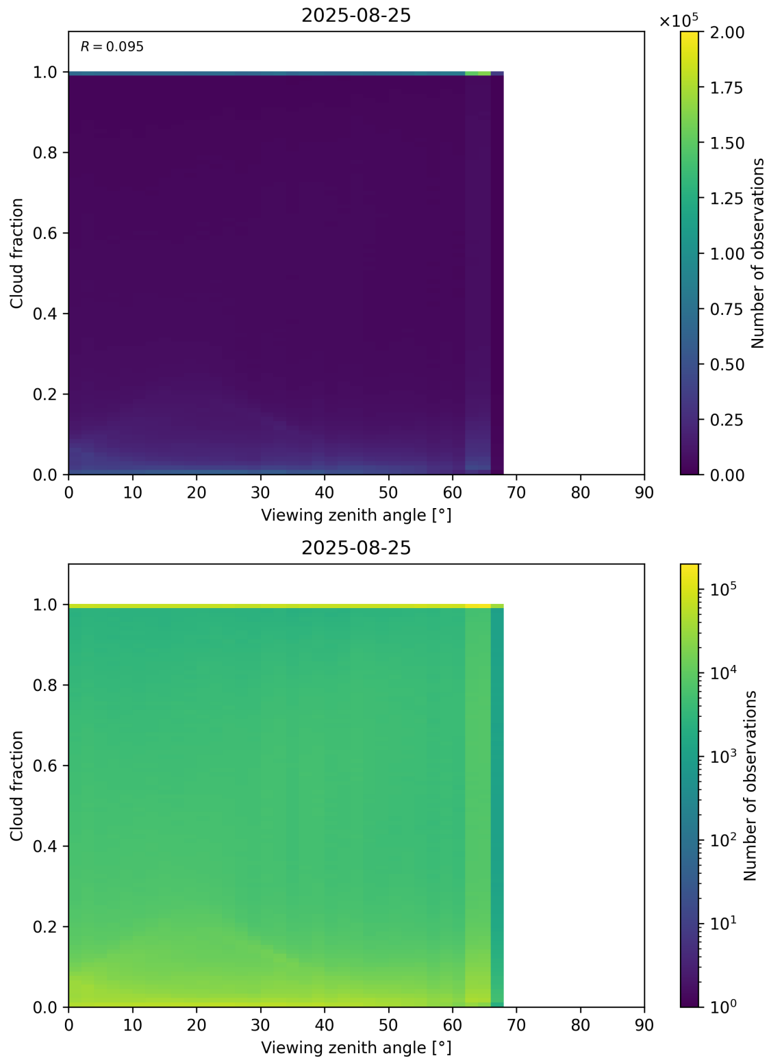
Figure 120: Scatter density plot of “Viewing zenith angle” against “Cloud fraction” for 2025-08-25 to 2025-08-26.
