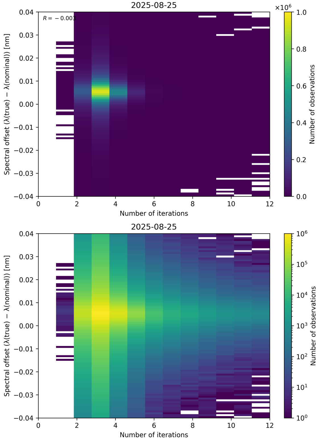
Figure 100: Scatter density plot of “Number of iterations” against “Spectral offset ( \lambda_{\text{true}} - \lambda_{\text{nominal}} )” for 2025-08-25 to 2025-08-26.
