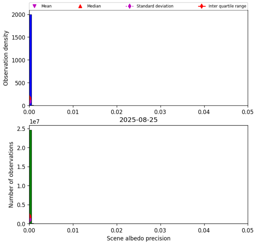
Figure 35: Histogram of “Scene albedo precision” for 2025-08-25 to 2025-08-26
