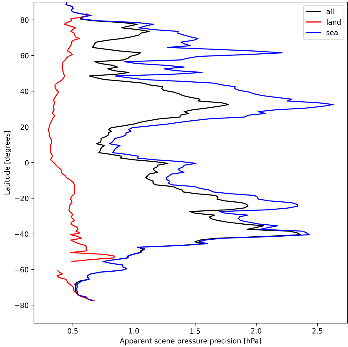
Figure 20: Zonal average of “Apparent scene pressure precision” for 2025-08-25 to 2025-08-26.
