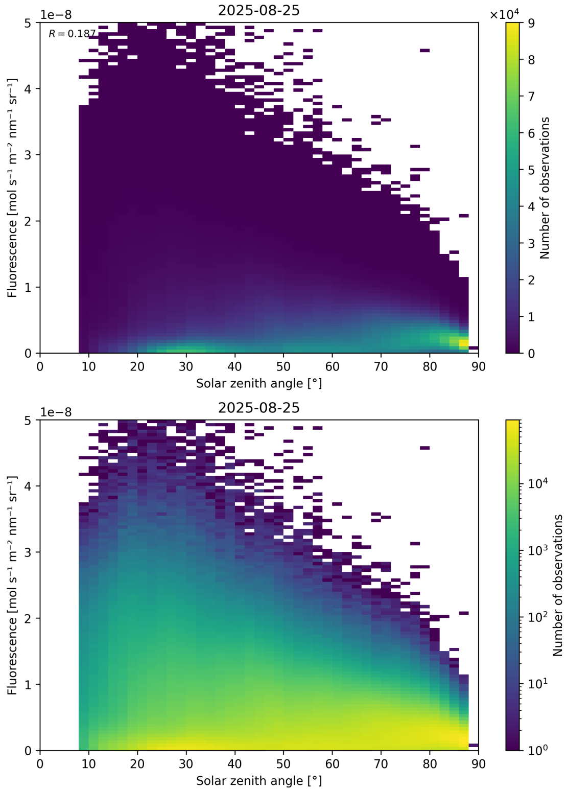
Figure 112: Scatter density plot of “Solar zenith angle” against “Fluorescence” for 2025-08-25 to 2025-08-26.
