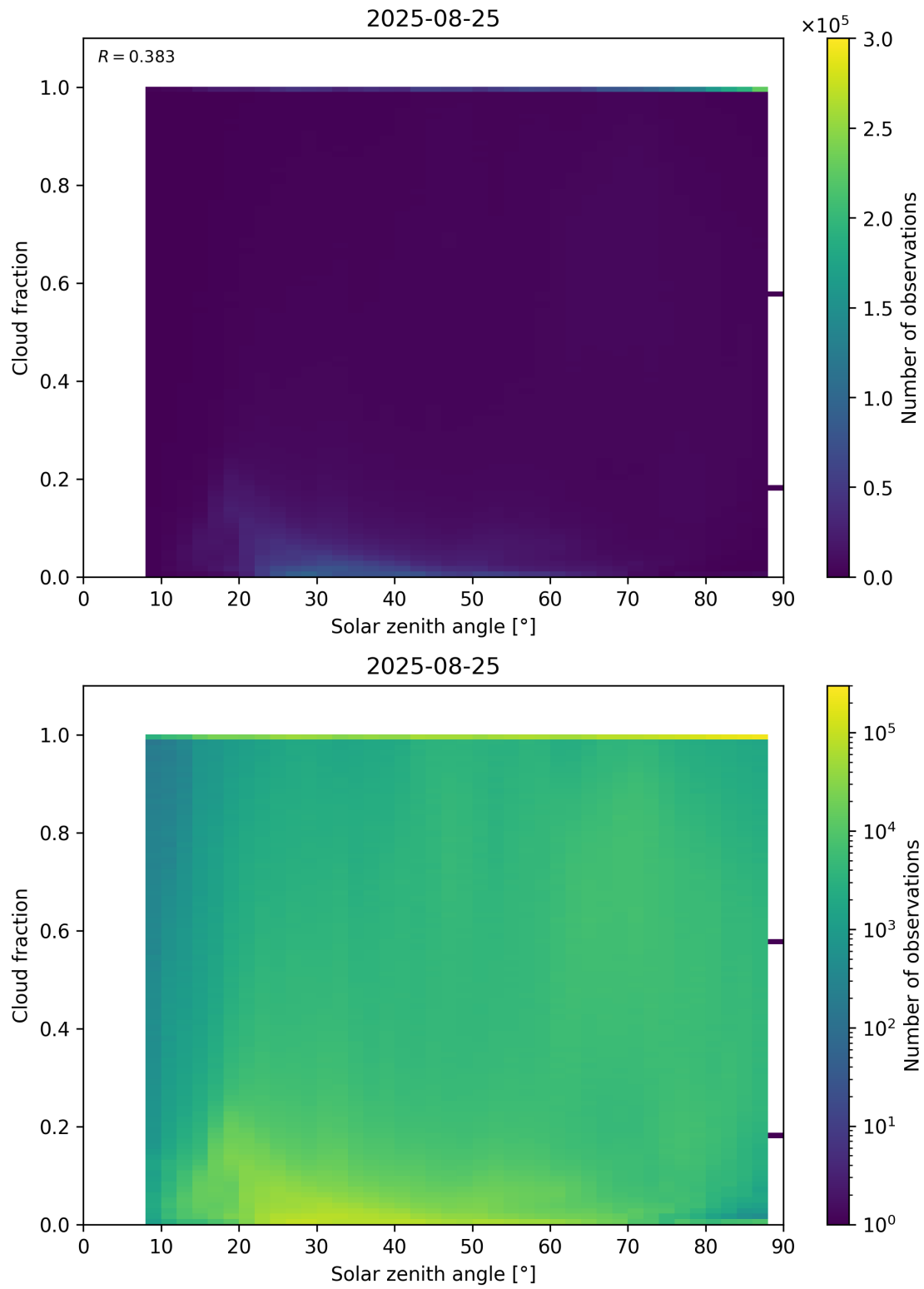
Figure 110: Scatter density plot of “Solar zenith angle” against “Cloud fraction” for 2025-08-25 to 2025-08-26.
