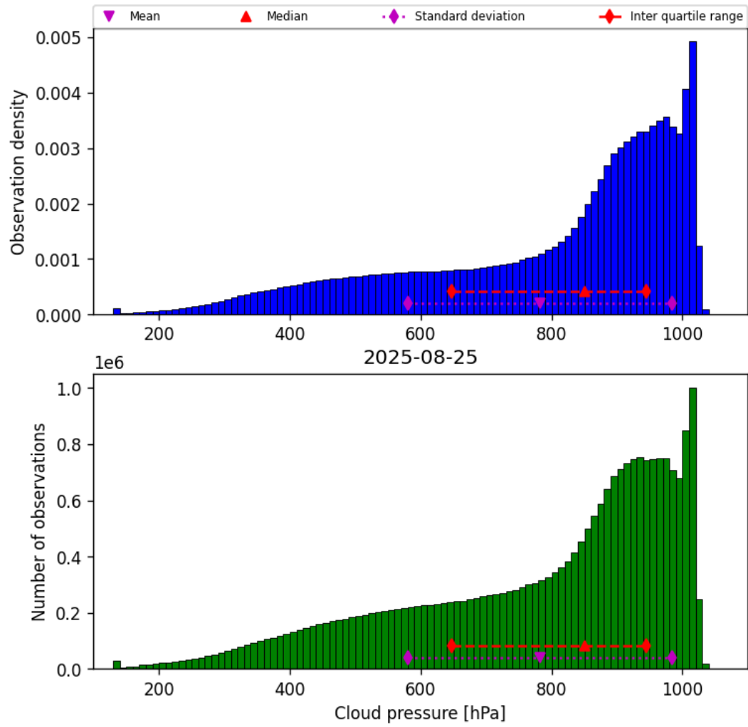
Figure 30: Histogram of “Cloud pressure” for 2025-08-25 to 2025-08-26
