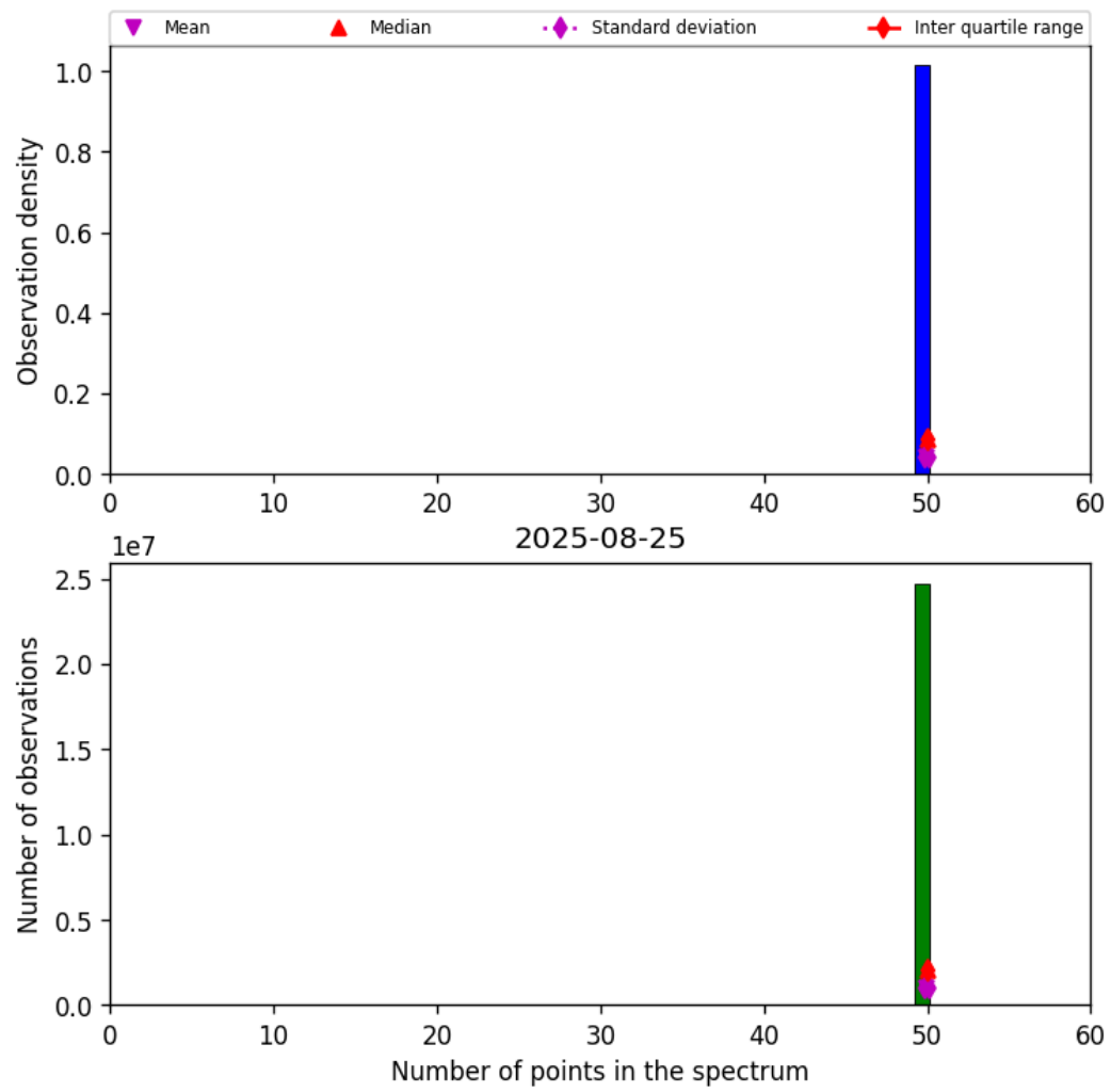
Figure 44: Histogram of “Number of points in the spectrum” for 2025-08-25 to 2025-08-26
