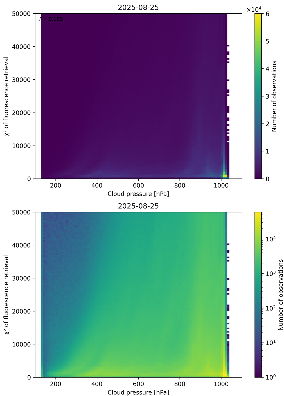
Figure 78: Scatter density plot of “Cloud pressure” against “ \chi^2 of fluorescence retrieval” for 2025-08-25 to 2025-08-26.
