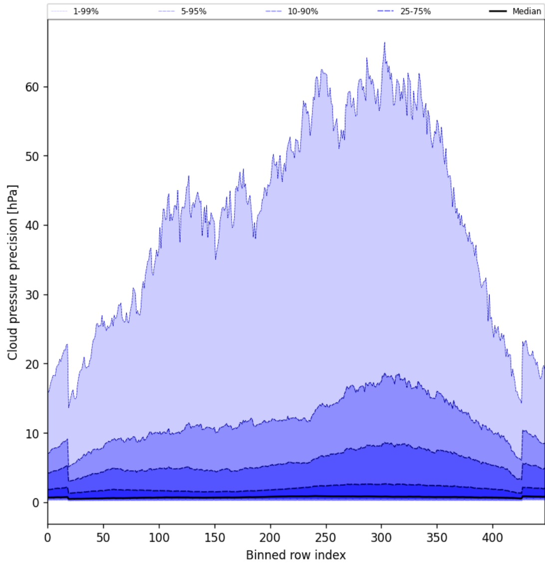
Figure 48: Along track statistics of “Cloud pressure precision” for 2025-08-25 to 2025-08-26
