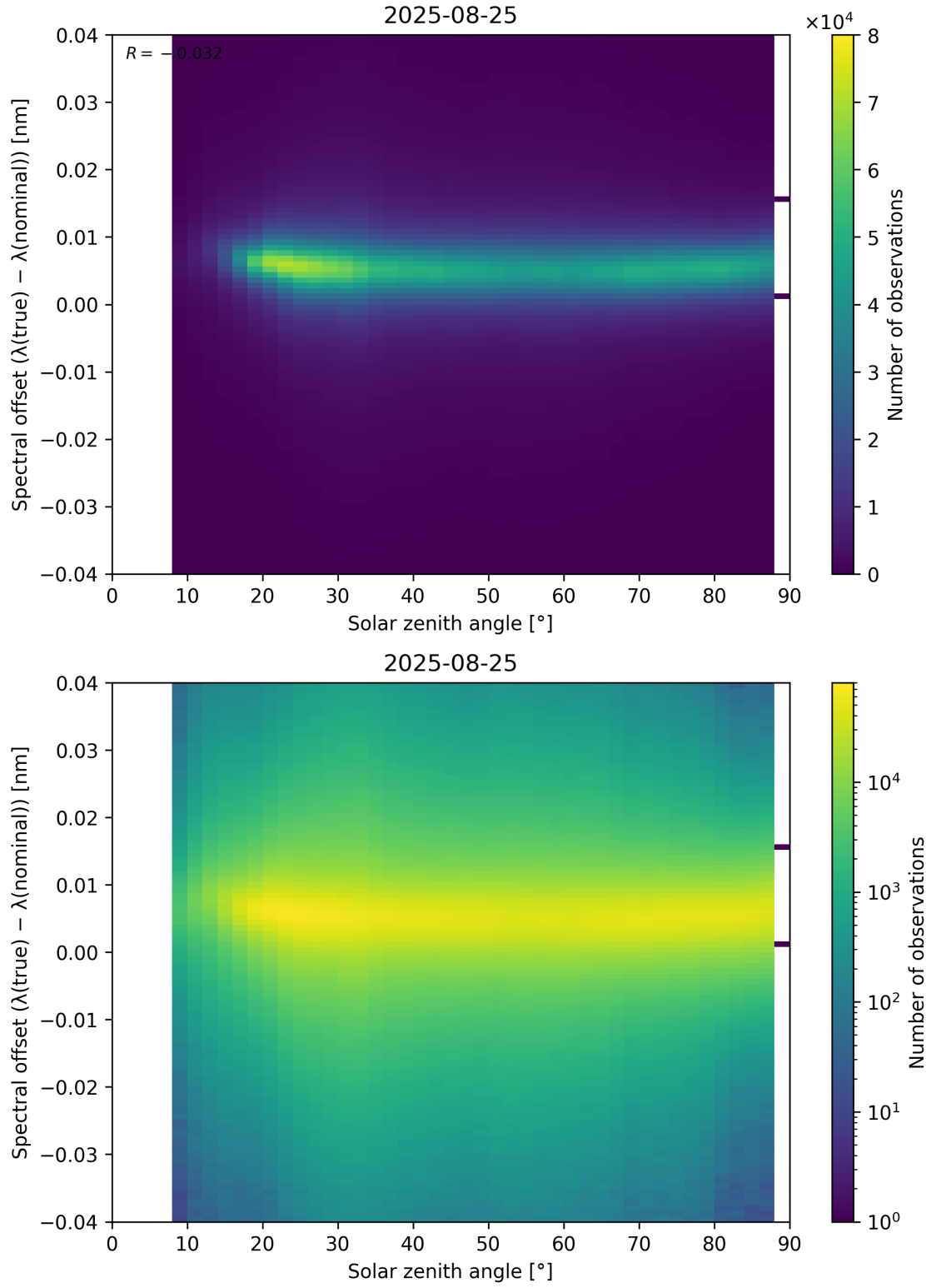
Figure 117: Scatter density plot of “Solar zenith angle” against “Spectral offset ( \lambda_{\text{true}} - \lambda_{\text{nominal}} )” for 2025-08-25 to 2025-08-26.
