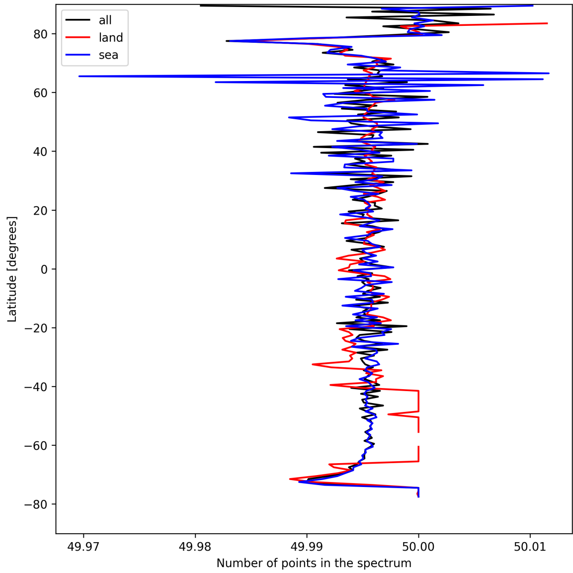
Figure 27: Zonal average of “Number of points in the spectrum” for 2025-08-25 to 2025-08-26.
