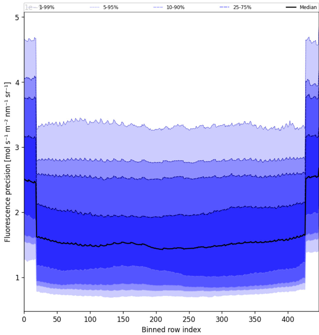
Figure 58: Along track statistics of “Fluorescence precision” for 2025-08-25 to 2025-08-26
