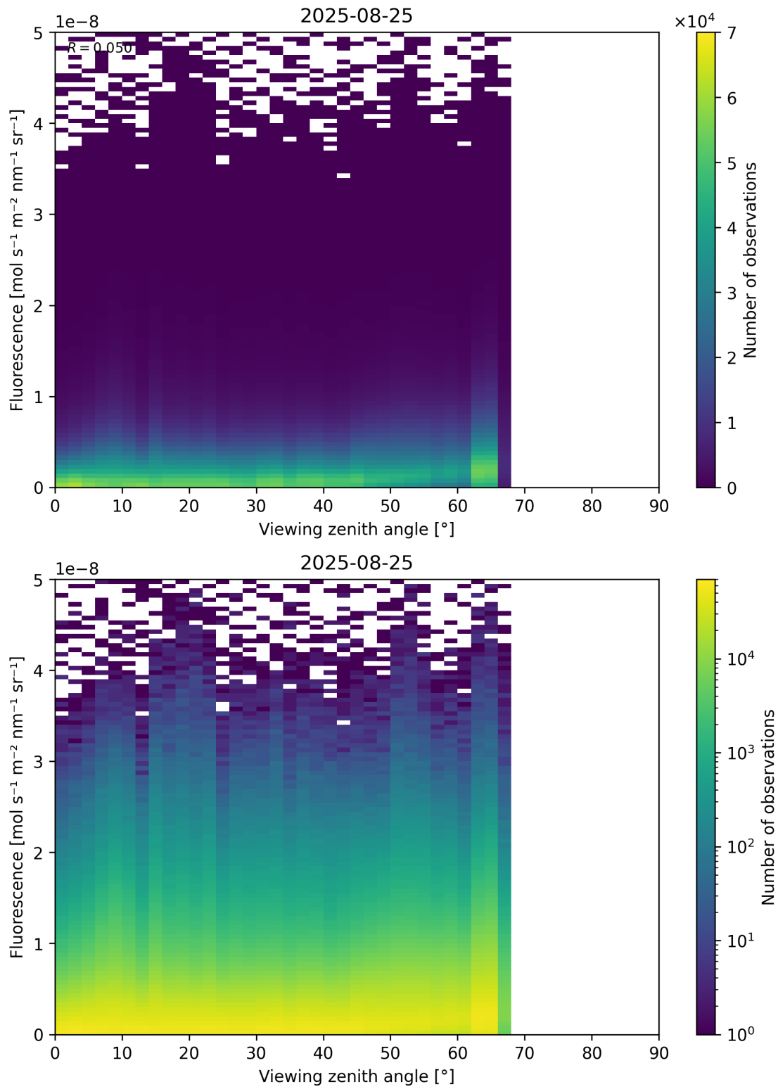
Figure 122: Scatter density plot of “Viewing zenith angle” against “Fluorescence” for 2025-08-25 to 2025-08-26.
