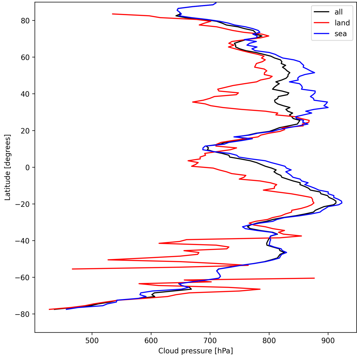
Figure 13: Zonal average of “Cloud pressure” for 2025-08-25 to 2025-08-26.
