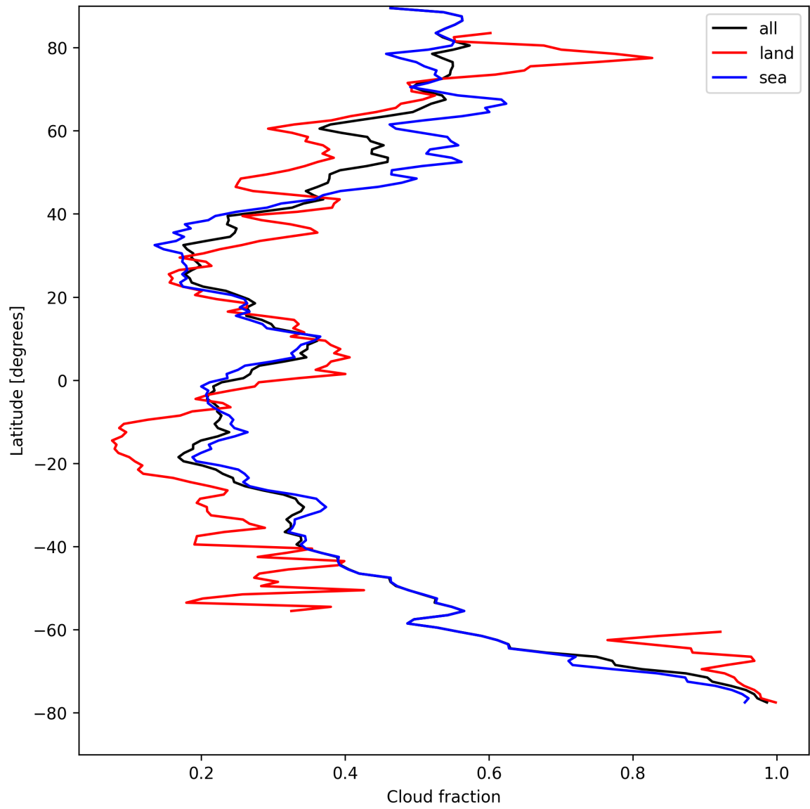
Figure 15: Zonal average of “Cloud fraction” for 2025-08-25 to 2025-08-26.
