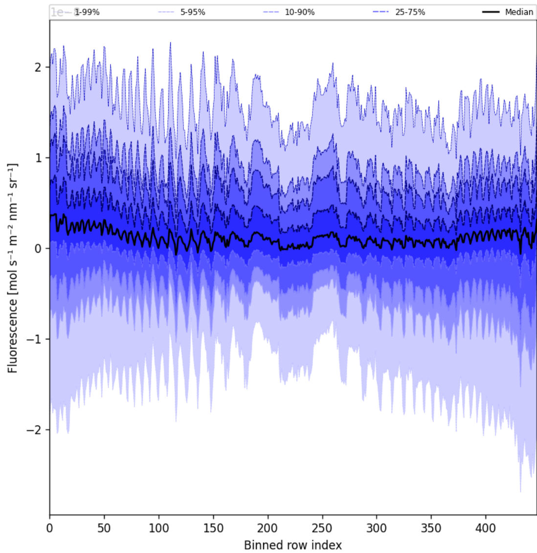
Figure 57: Along track statistics of “Fluorescence” for 2025-08-25 to 2025-08-26
