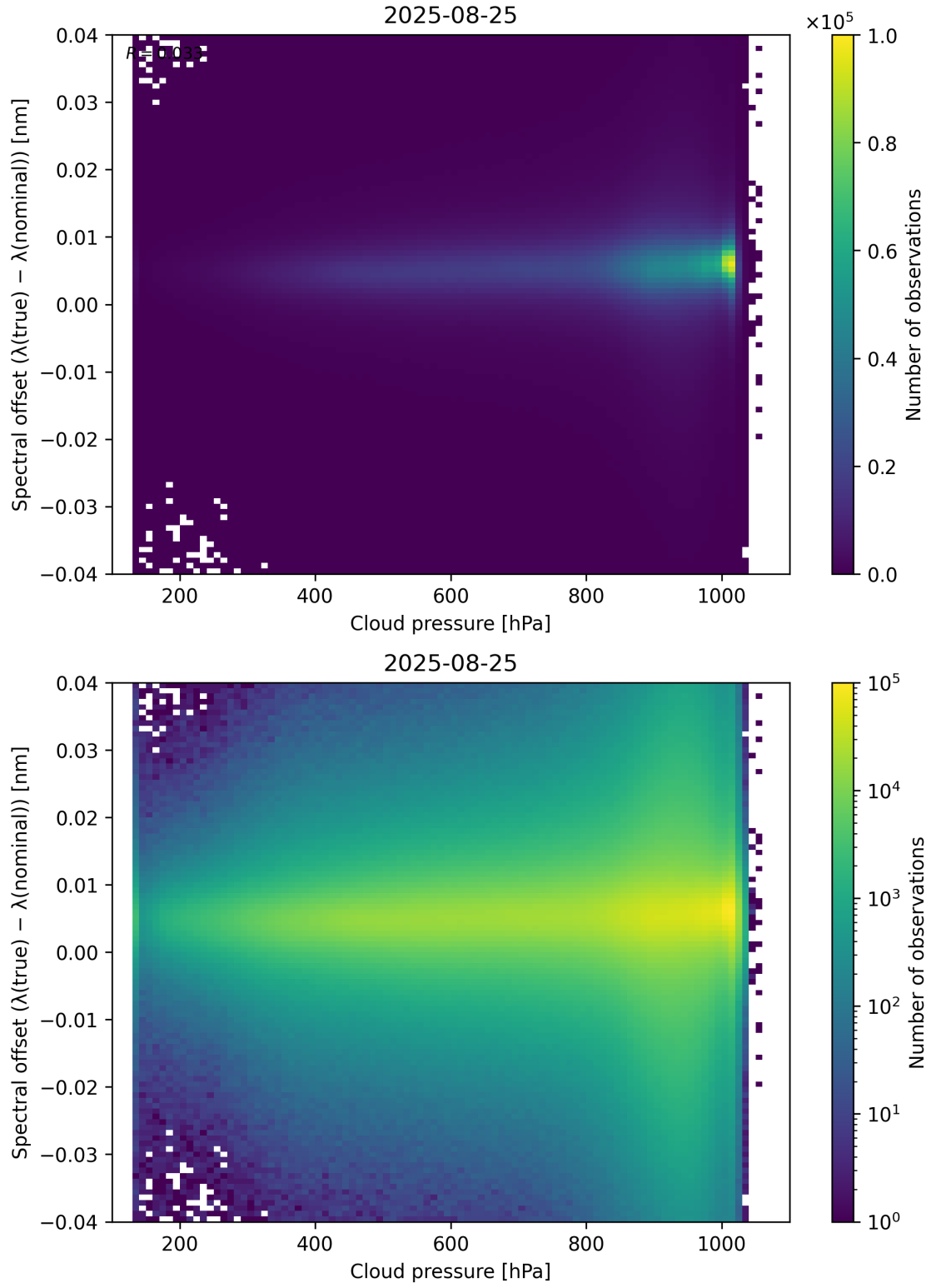
Figure 84: Scatter density plot of “Cloud pressure” against “Spectral offset ( \lambda_{\text{true}} - \lambda_{\text{nominal}} )” for 2025-08-25 to 2025-08-26.
