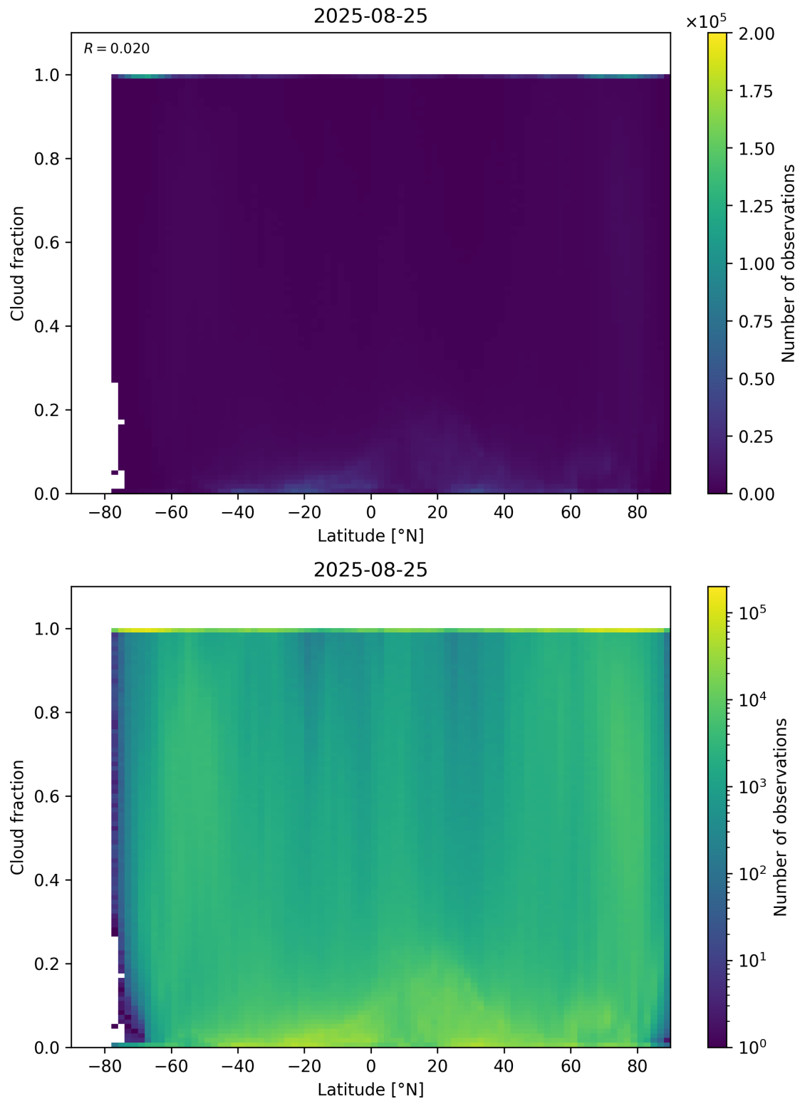
Figure 90: Scatter density plot of “Latitude” against “Cloud fraction” for 2025-08-25 to 2025-08-26.
