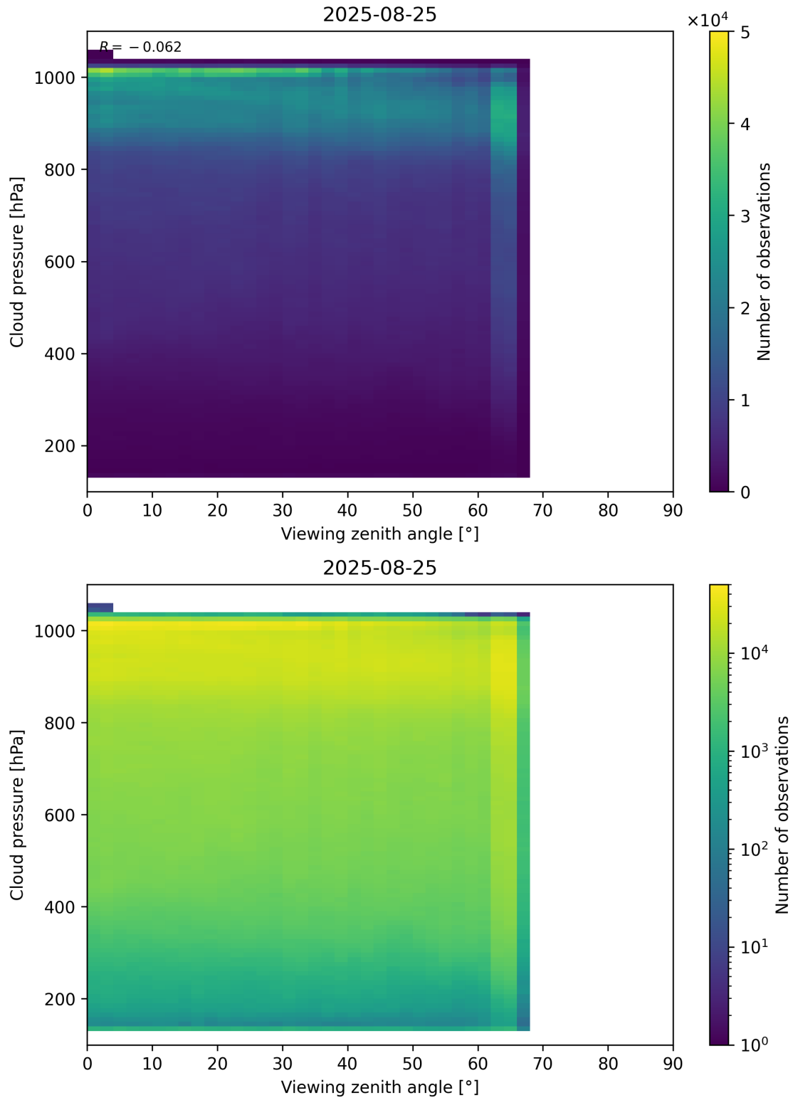
Figure 121: Scatter density plot of “Viewing zenith angle” against “Cloud pressure” for 2025-08-25 to 2025-08-26.
