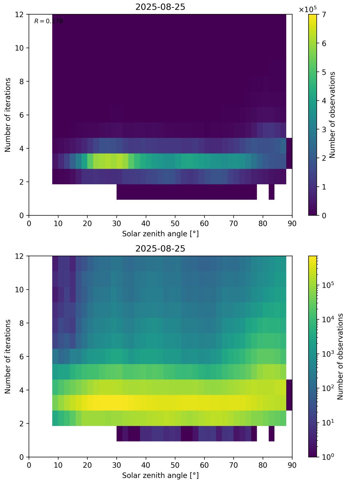
Figure 114: Scatter density plot of “Solar zenith angle” against “Number of iterations” for 2025-08-25 to 2025-08-26.
