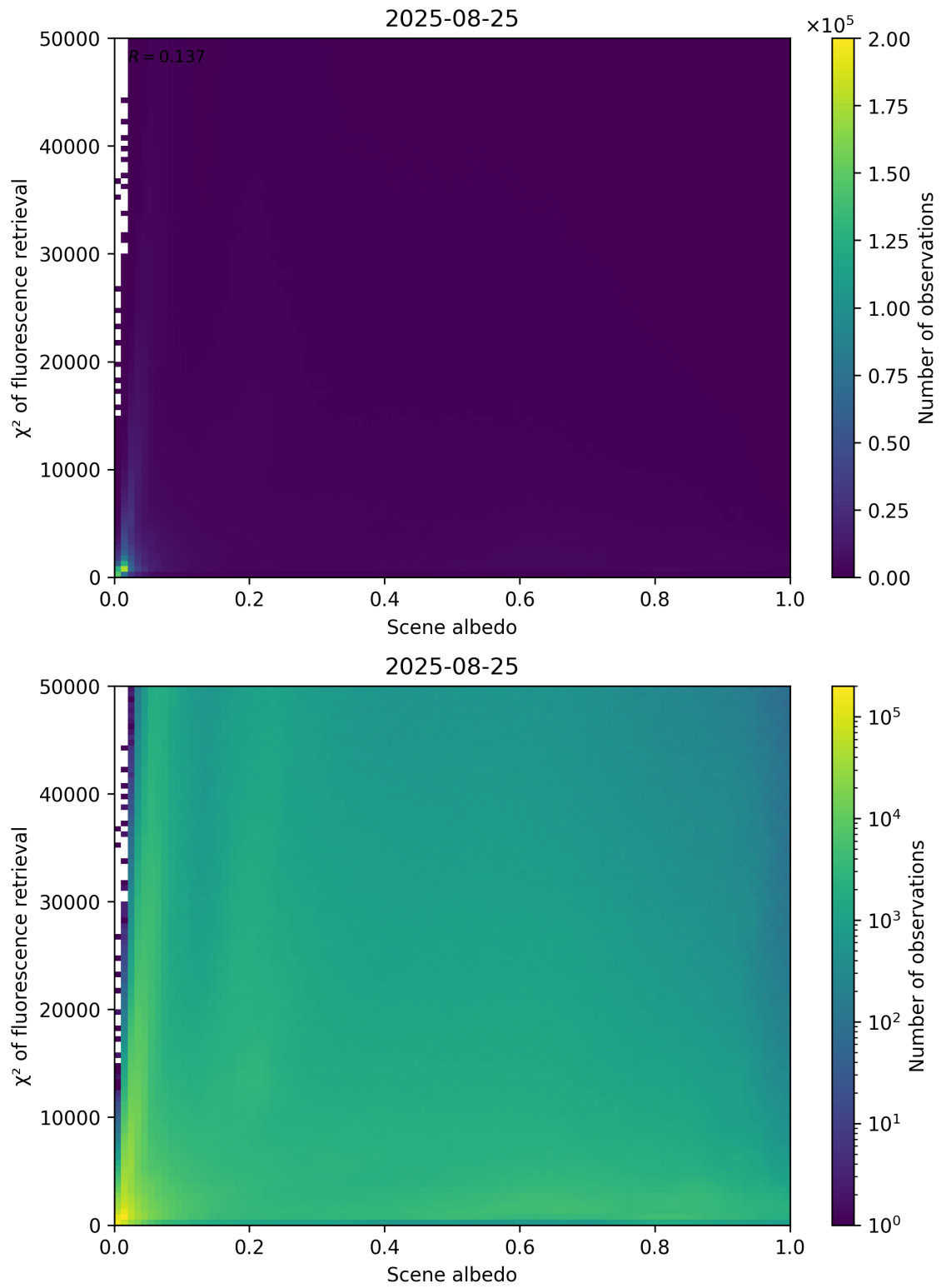
Figure 103: Scatter density plot of “Scene albedo” against “ \chi^2 of fluorescence retrieval” for 2025-08-25 to 2025-08-26.
