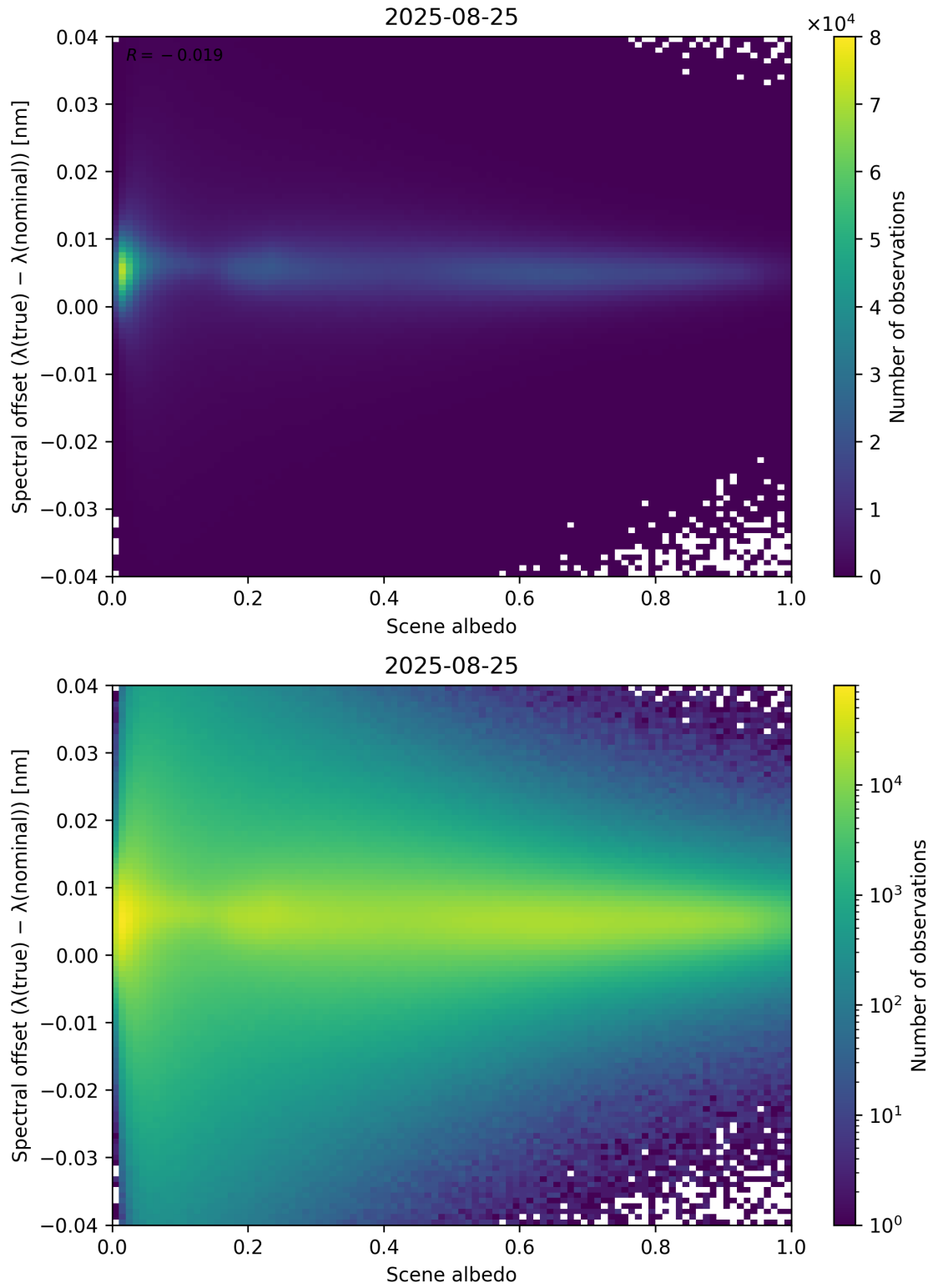
Figure 107: Scatter density plot of “Scene albedo” against “Spectral offset ( \lambda_{\text{true}} - \lambda_{\text{nominal}} )” for 2025-08-25 to 2025-08-26.
