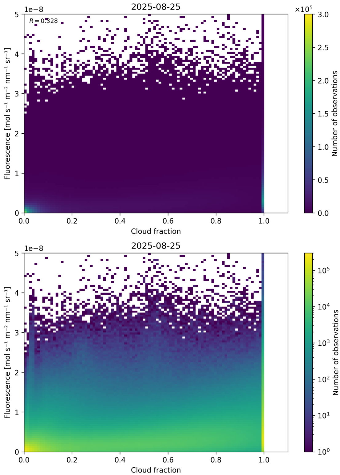
Figure 72: Scatter density plot of “Cloud fraction” against “Fluorescence” for 2025-08-25 to 2025-08-26.
