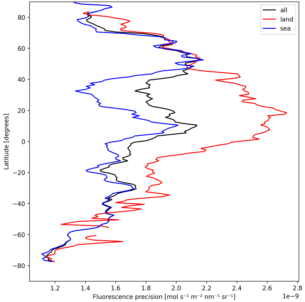
Figure 24: Zonal average of “Fluorescence precision” for 2025-08-25 to 2025-08-26.
