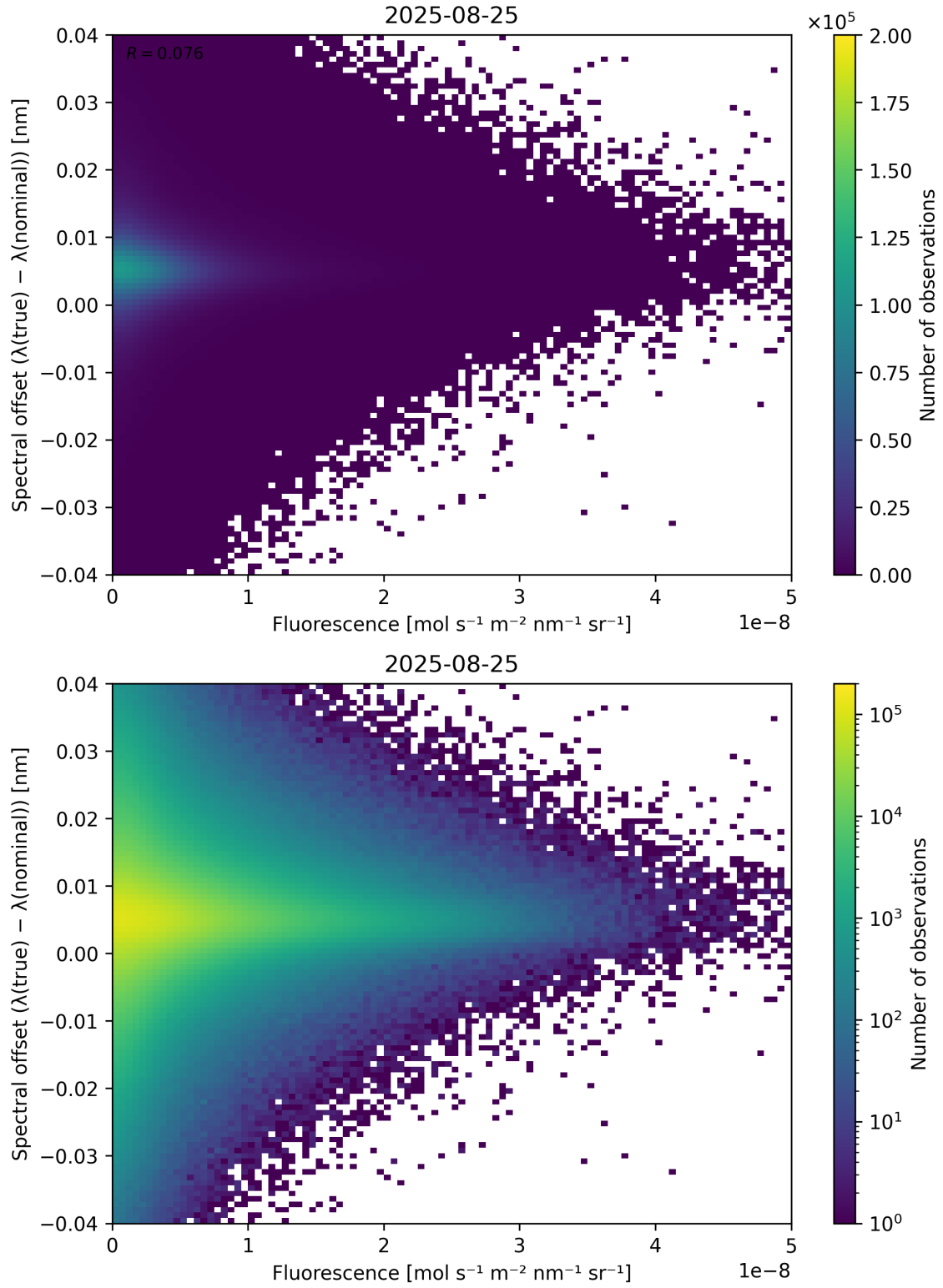
Figure 87: Scatter density plot of “Fluorescence” against “Spectral offset ( \lambda_{\text{true}} - \lambda_{\text{nominal}} )” for 2025-08-25 to 2025-08-26.
