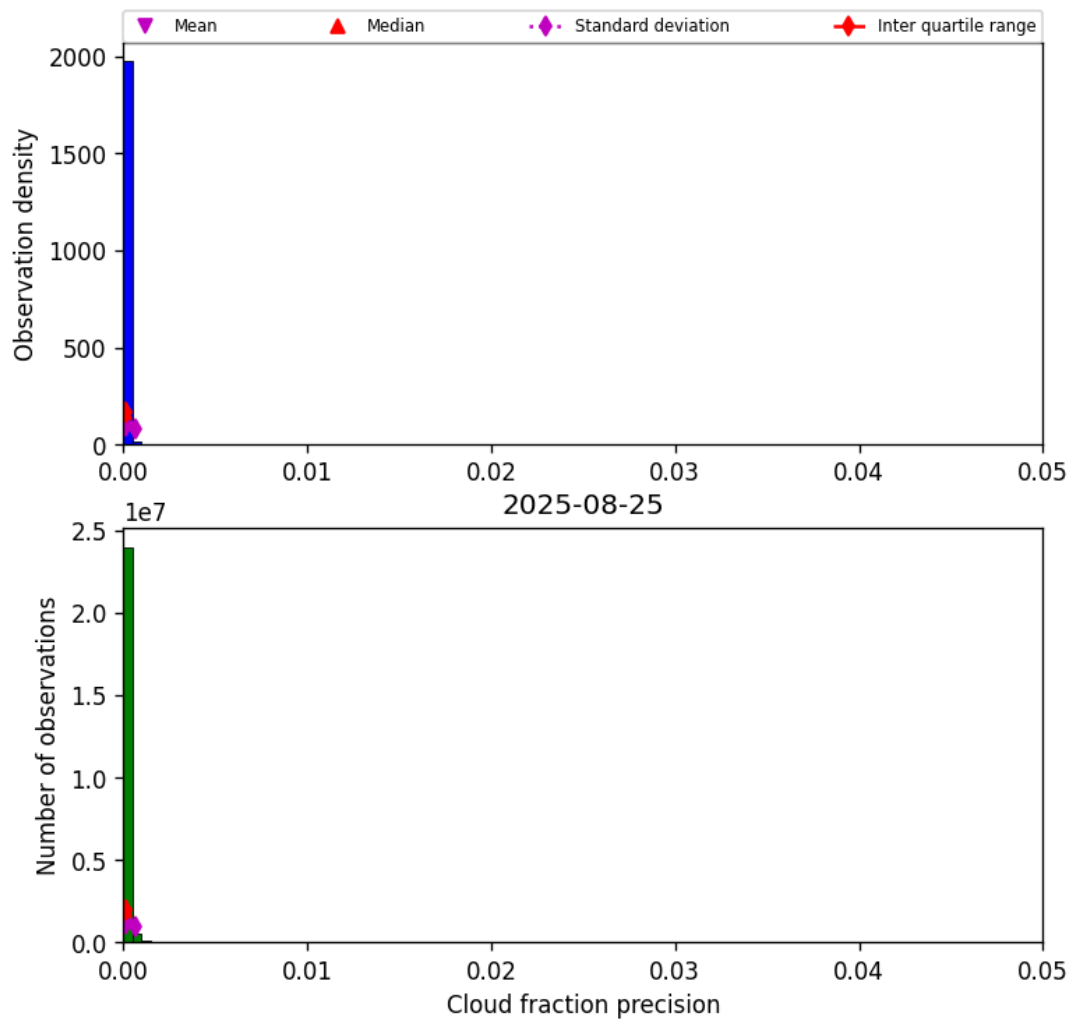
Figure 33: Histogram of “Cloud fraction precision” for 2025-08-25 to 2025-08-26
