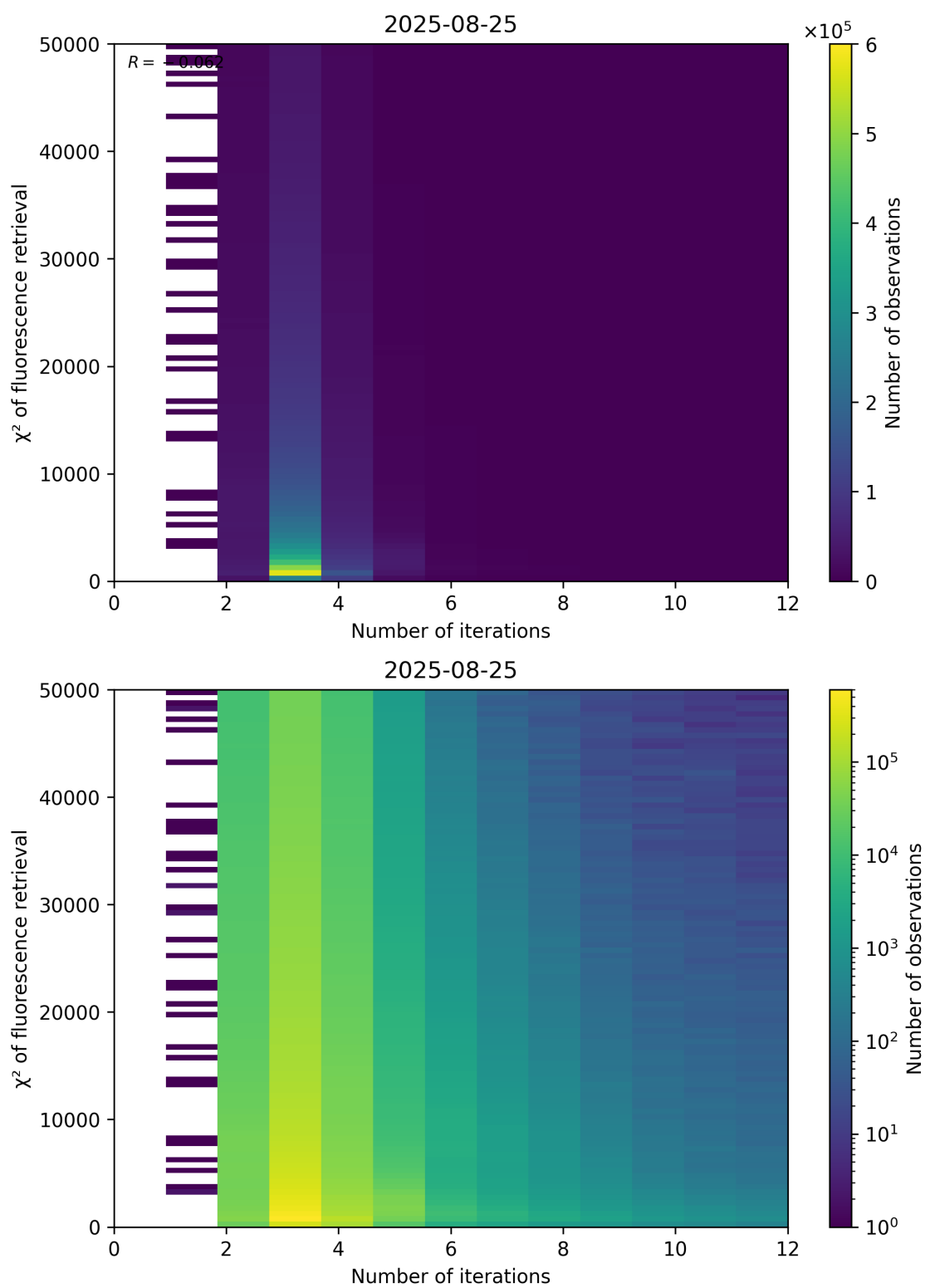
Figure 97: Scatter density plot of “Number of iterations” against “ \chi^2 of fluorescence retrieval” for 2025-08-25 to 2025-08-26.
