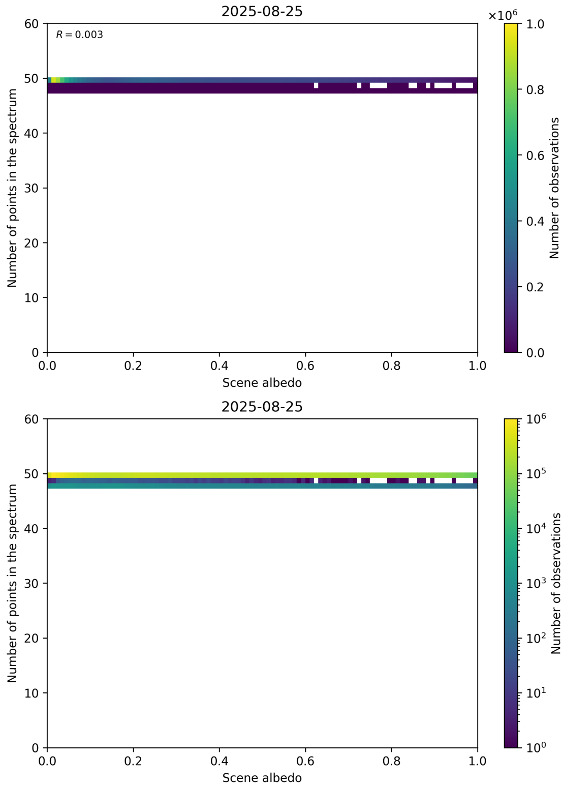
Figure 106: Scatter density plot of “Scene albedo” against “Number of points in the spectrum” for 2025-08-25 to 2025-08-26.
