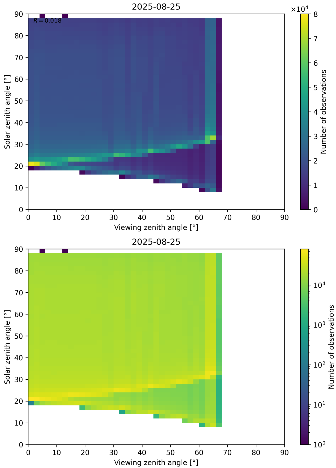
Figure 127: Scatter density plot of “Viewing zenith angle” against “Solar zenith angle” for 2025-08-25 to 2025-08-26.
