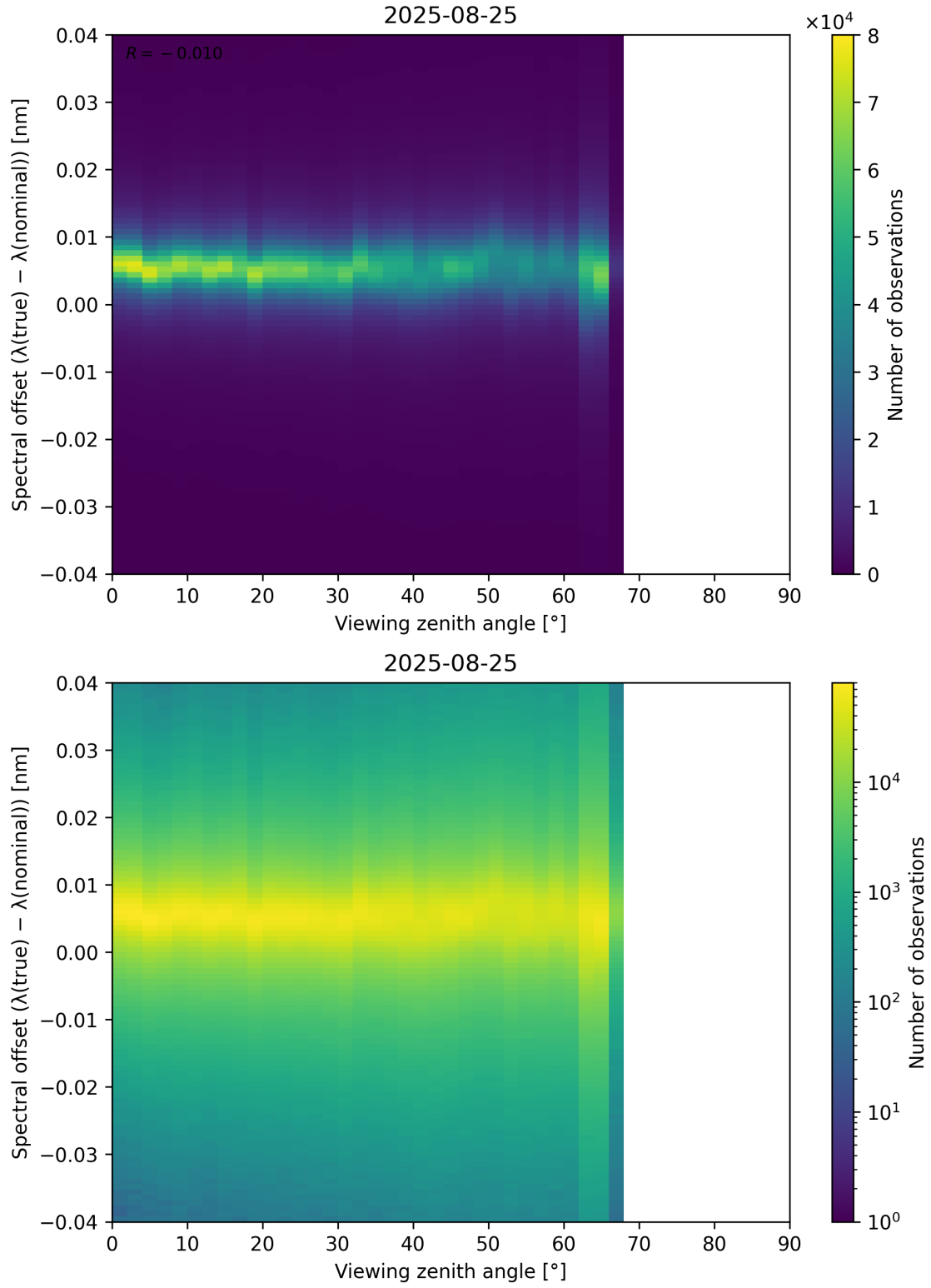
Figure 128: Scatter density plot of “Viewing zenith angle” against “Spectral offset ( \lambda_{\text{true}} - \lambda_{\text{nominal}} )” for 2025-08-25 to 2025-08-26.
