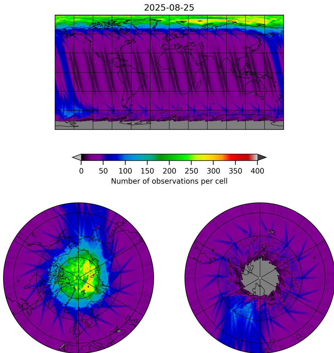
Figure 11: Map of the number of observations for 2025-08-25 to 2025-08-26
