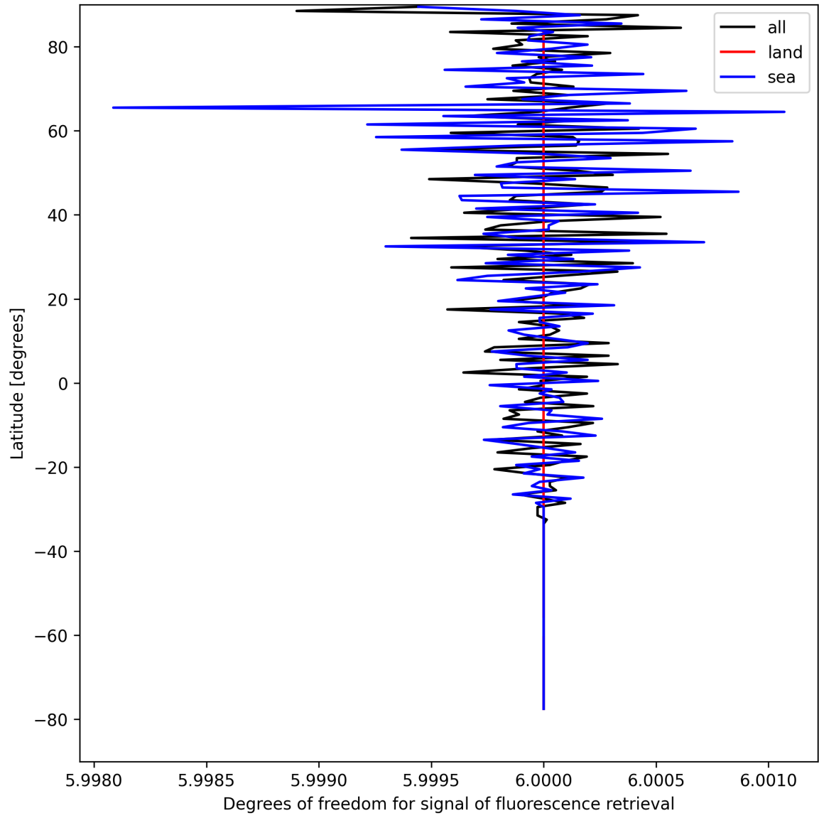
Figure 26: Zonal average of “Degrees of freedom for signal of fluorescence retrieval” for 2025-08-25 to 2025-08-26.
