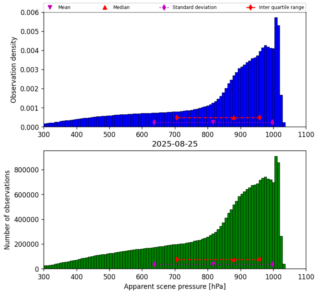
Figure 36: Histogram of “Apparent scene pressure” for 2025-08-25 to 2025-08-26
