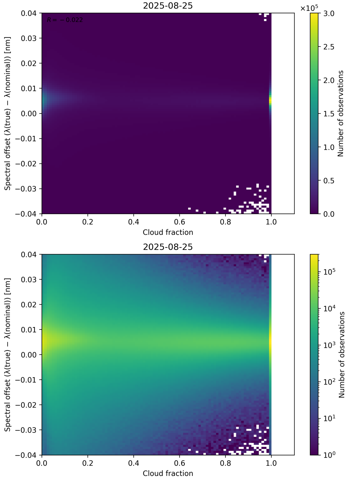
Figure 76: Scatter density plot of “Cloud fraction” against “Spectral offset ( \lambda_{\text{true}} - \lambda_{\text{nominal}} )” for 2025-08-25 to 2025-08-26.
