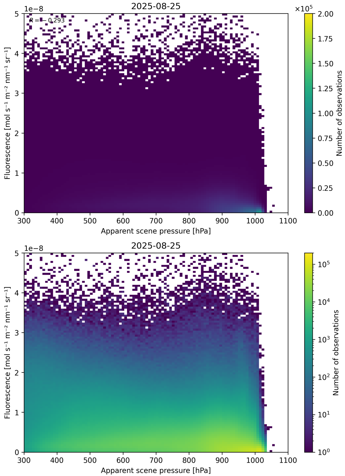
Figure 64: Scatter density plot of “Apparent scene pressure” against “Fluorescence” for 2025-08-25 to 2025-08-26.
