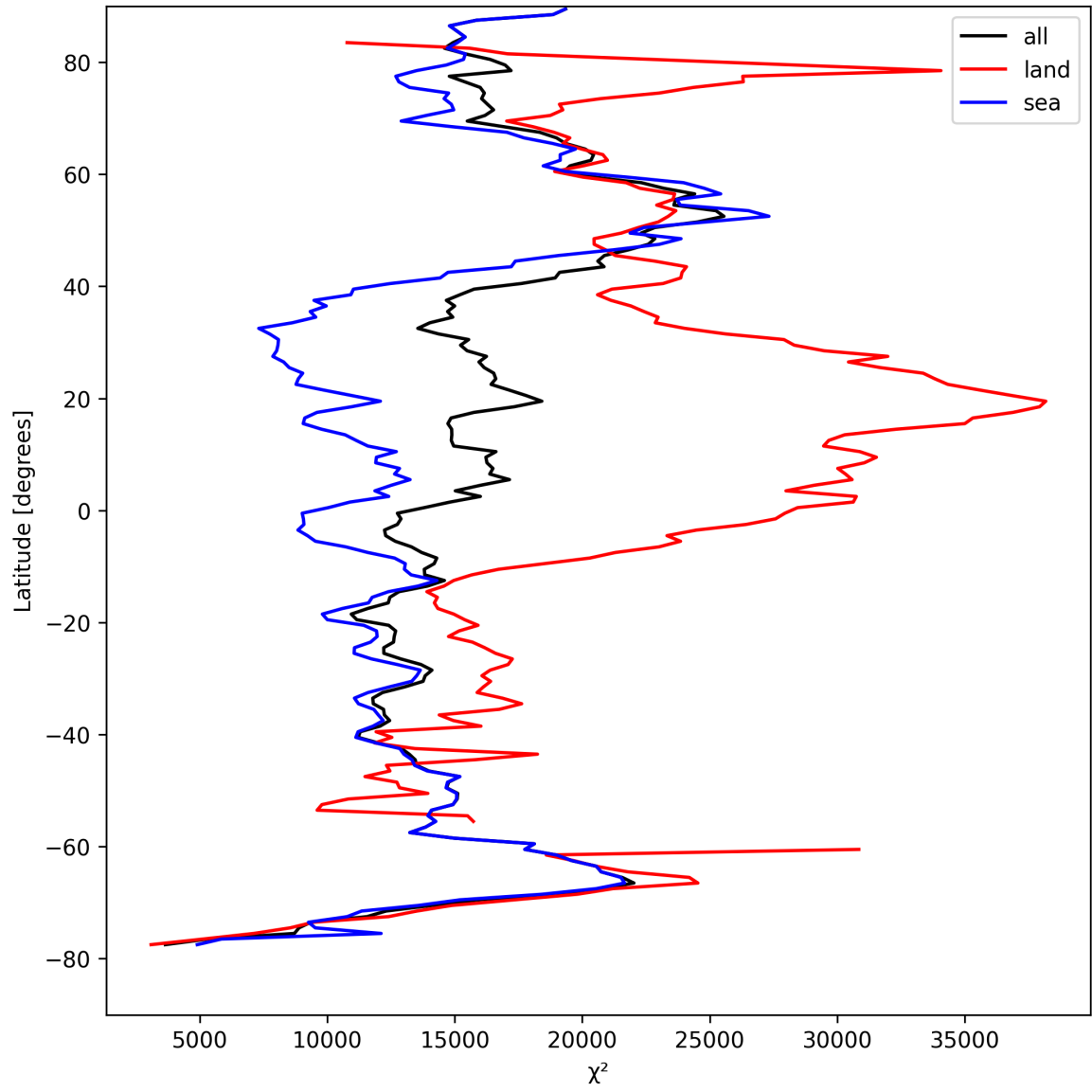
Figure 21: Zonal average of “ \chi^2 ” for 2025-08-25 to 2025-08-26.
