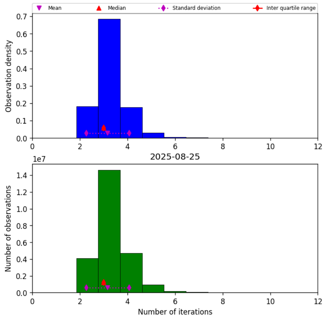
Figure 39: Histogram of “Number of iterations” for 2025-08-25 to 2025-08-26
