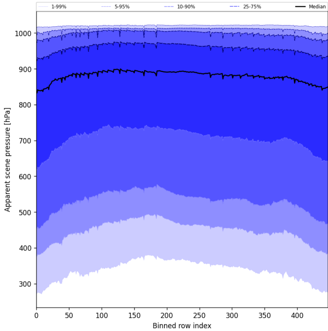
Figure 53: Along track statistics of “Apparent scene pressure” for 2025-08-25 to 2025-08-26
