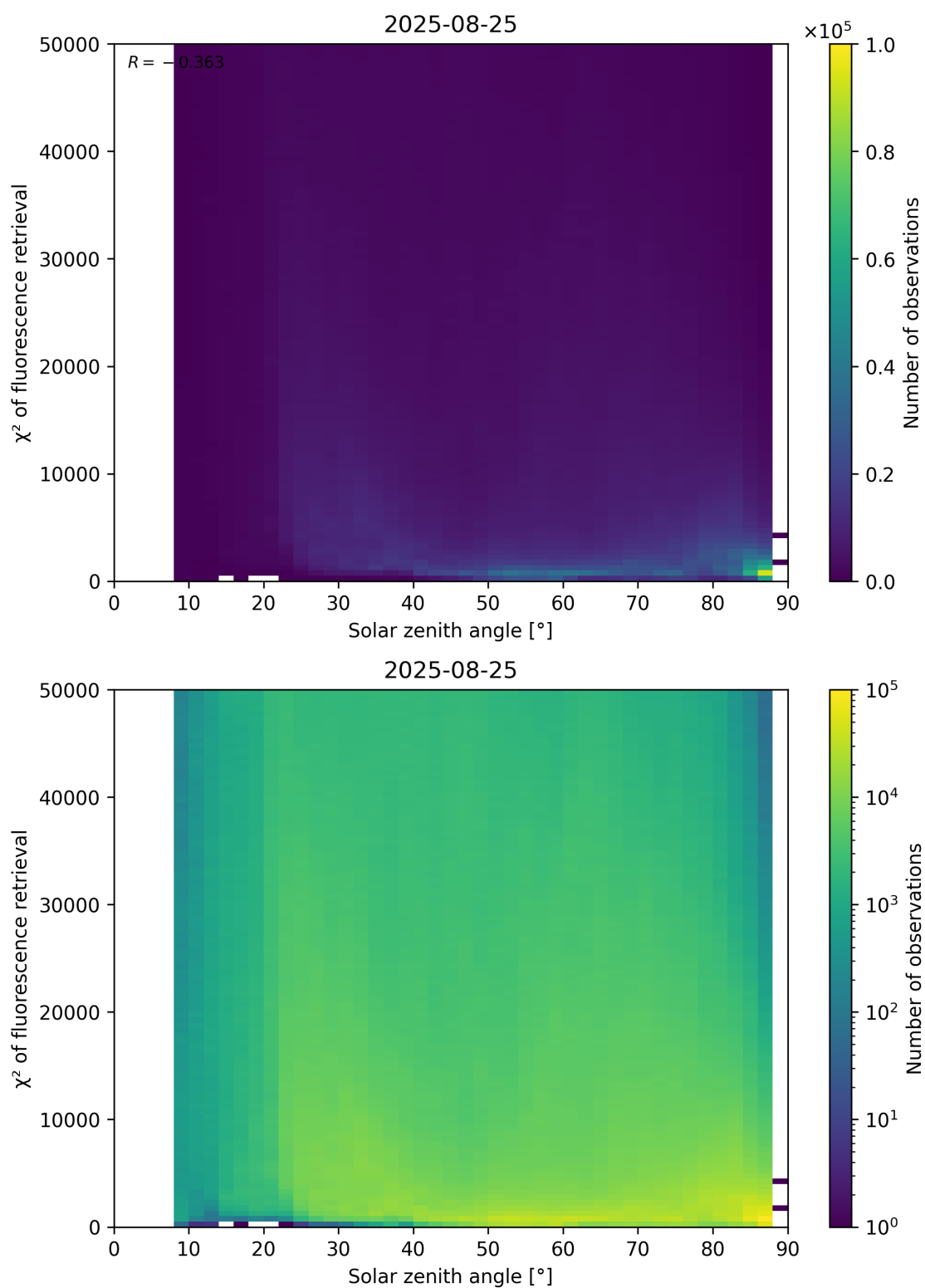
Figure 109: Scatter density plot of “Solar zenith angle” against “ \chi^2 of fluorescence retrieval” for 2025-08-25 to 2025-08-26.
