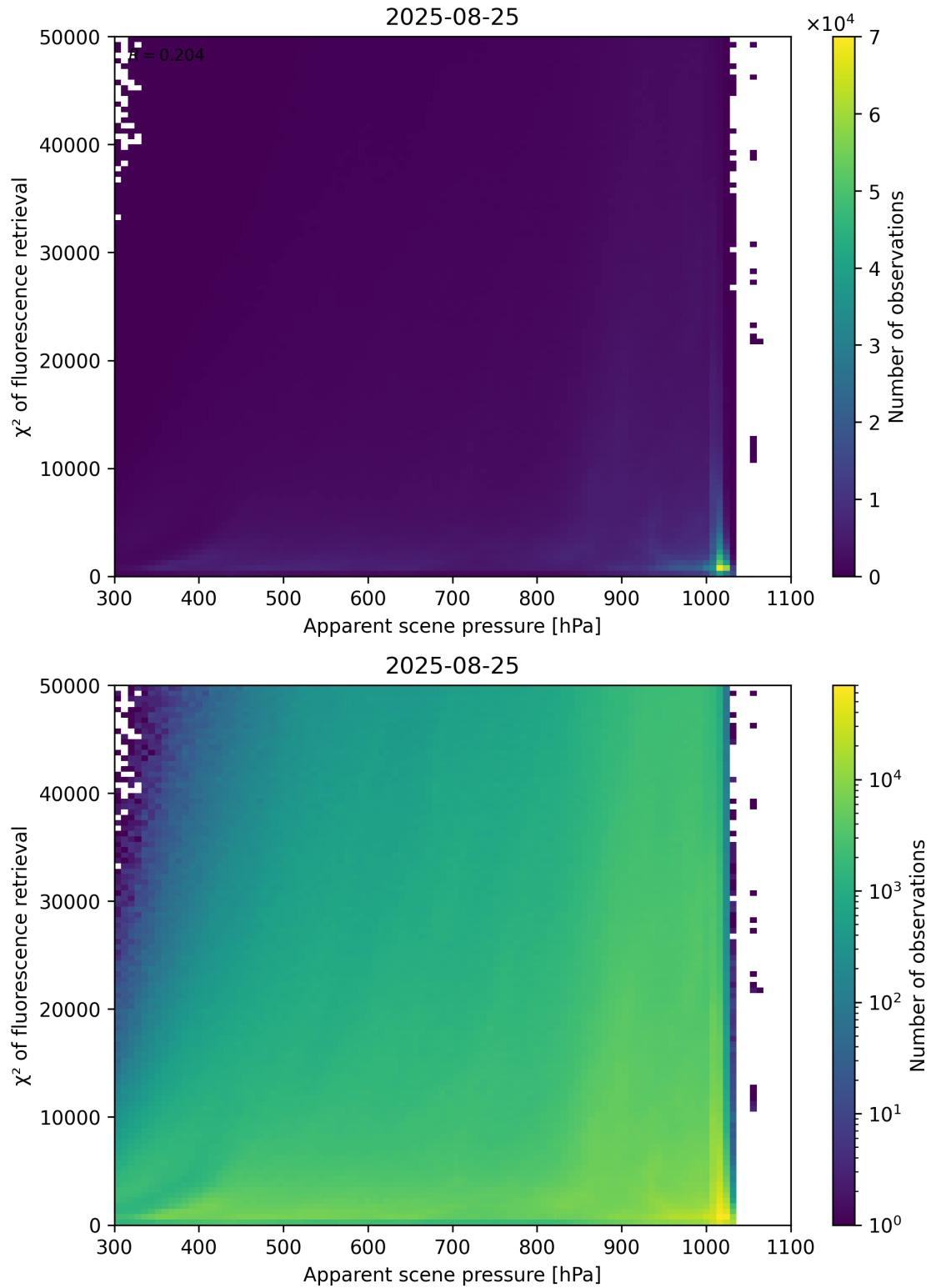
Figure 63: Scatter density plot of “Apparent scene pressure” against “ \chi^2 of fluorescence retrieval” for 2025-08-25 to 2025-08-26.
