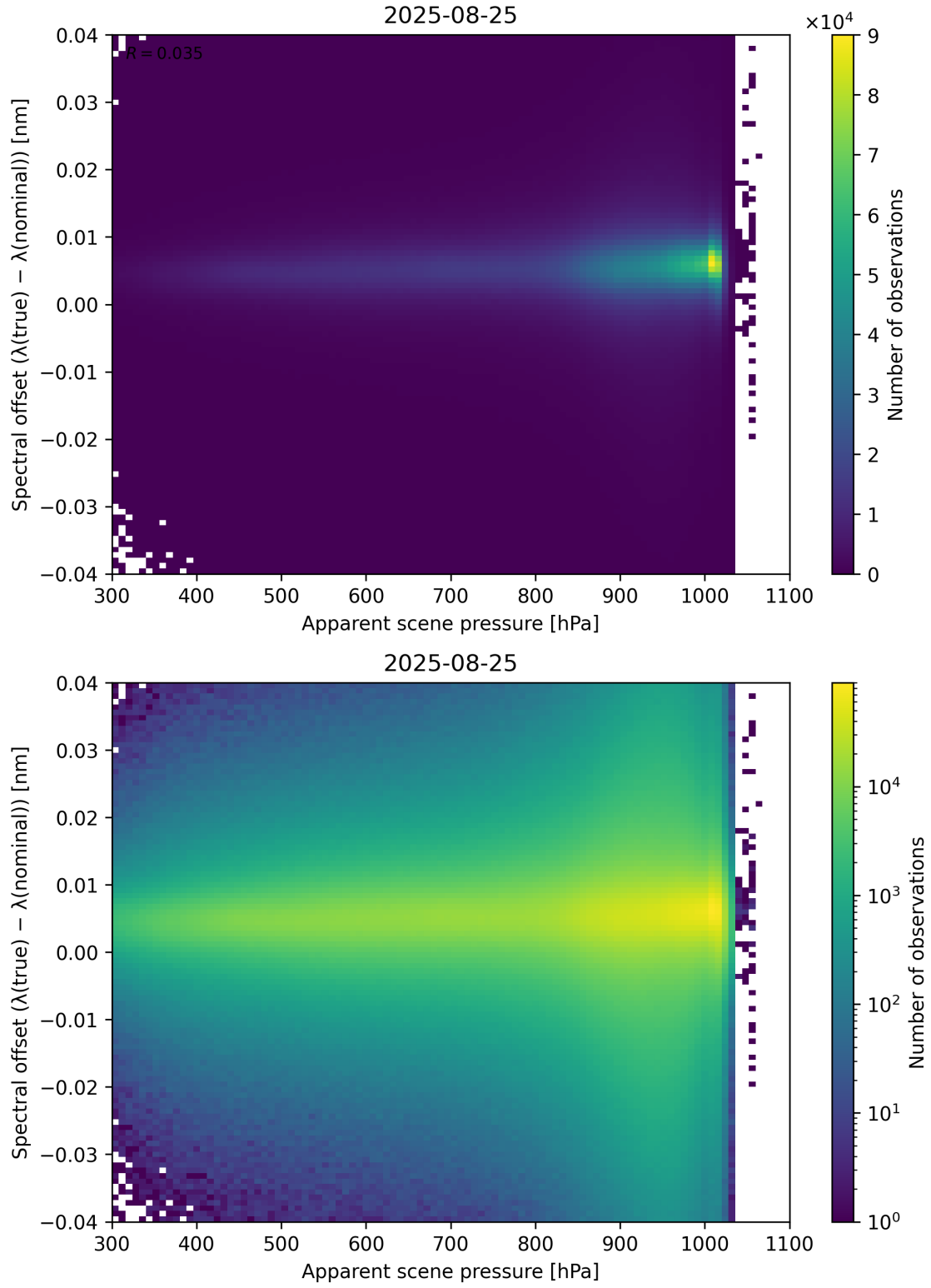
Figure 67: Scatter density plot of “Apparent scene pressure” against “Spectral offset ( \lambda_{\text{true}} - \lambda_{\text{nominal}} )” for 2025-08-25 to 2025-08-26.
