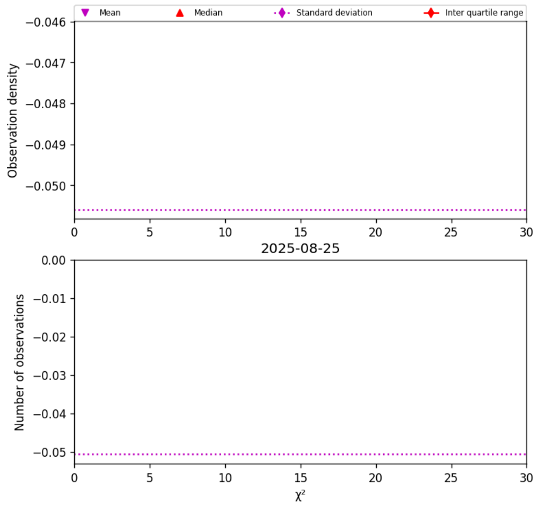
Figure 38: Histogram of " \chi^2 " for 2025-08-25 to 2025-08-26
