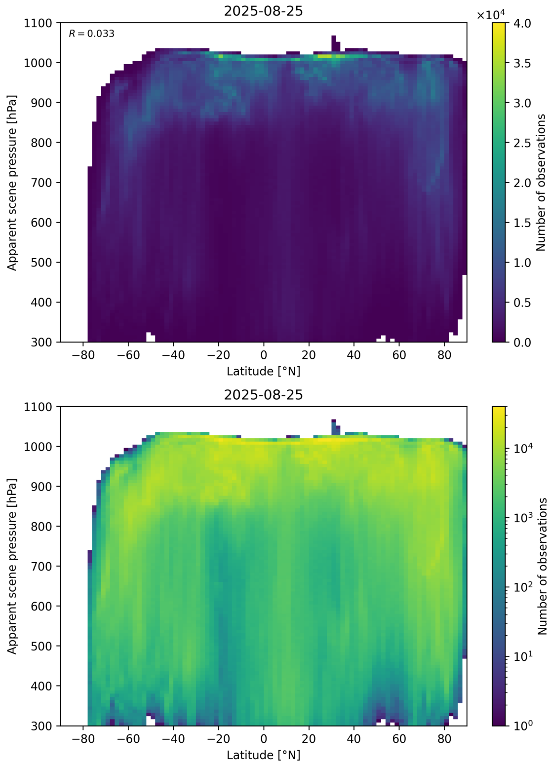
Figure 88: Scatter density plot of “Latitude” against “Apparent scene pressure” for 2025-08-25 to 2025-08-26.
