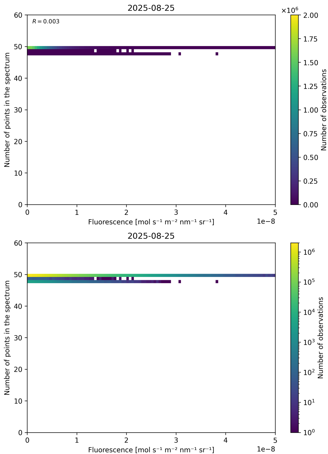
Figure 86: Scatter density plot of “Fluorescence” against “Number of points in the spectrum” for 2025-08-25 to 2025-08-26.
