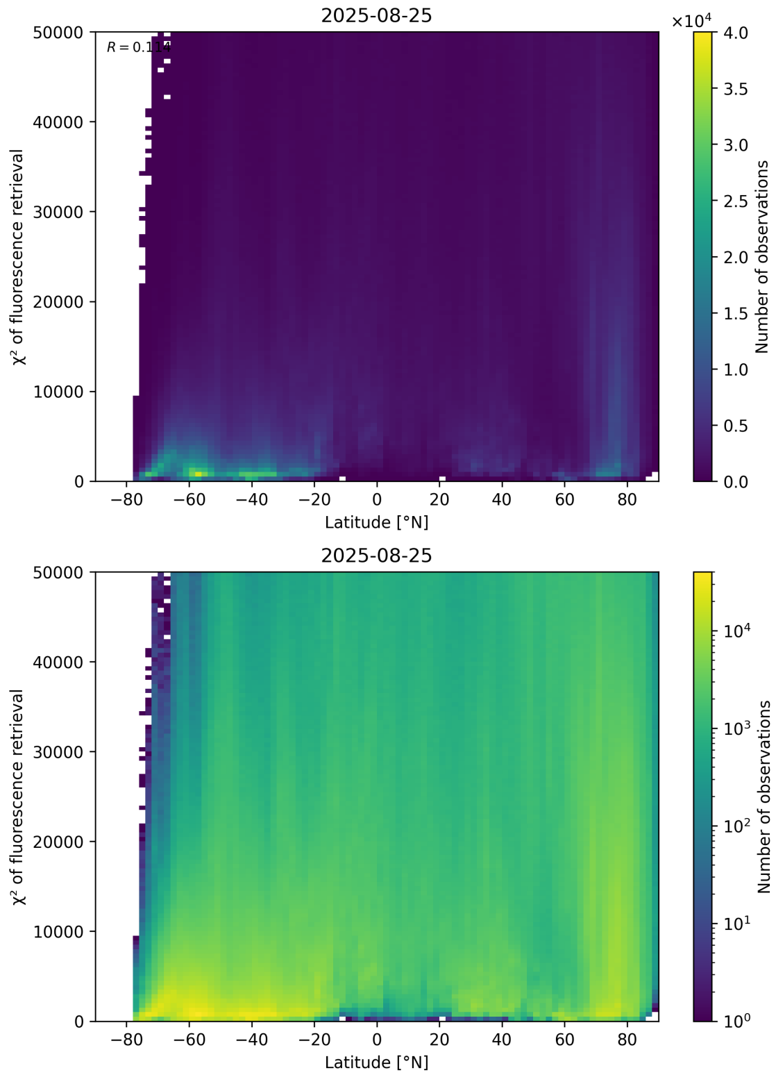
Figure 89: Scatter density plot of “Latitude” against “ \chi^2 of fluorescence retrieval” for 2025-08-25 to 2025-08-26.
