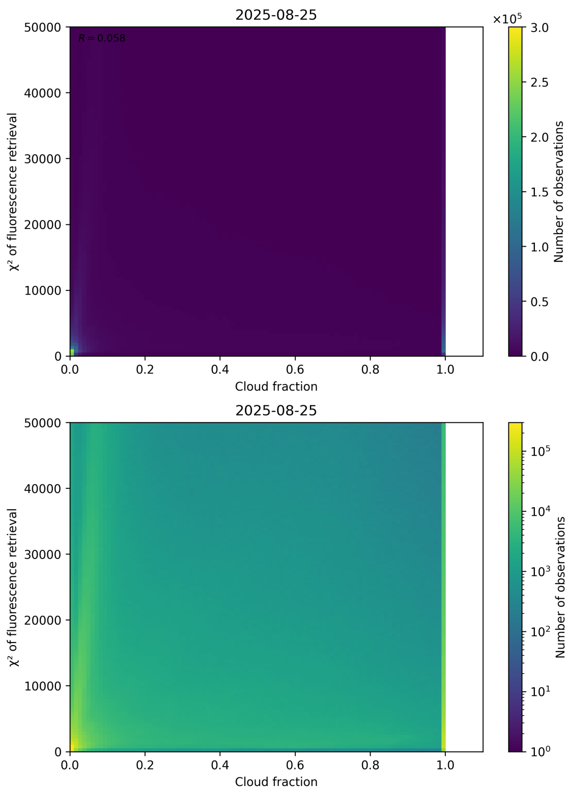
Figure 71: Scatter density plot of “Cloud fraction” against “ \chi^2 of fluorescence retrieval” for 2025-08-25 to 2025-08-26.
