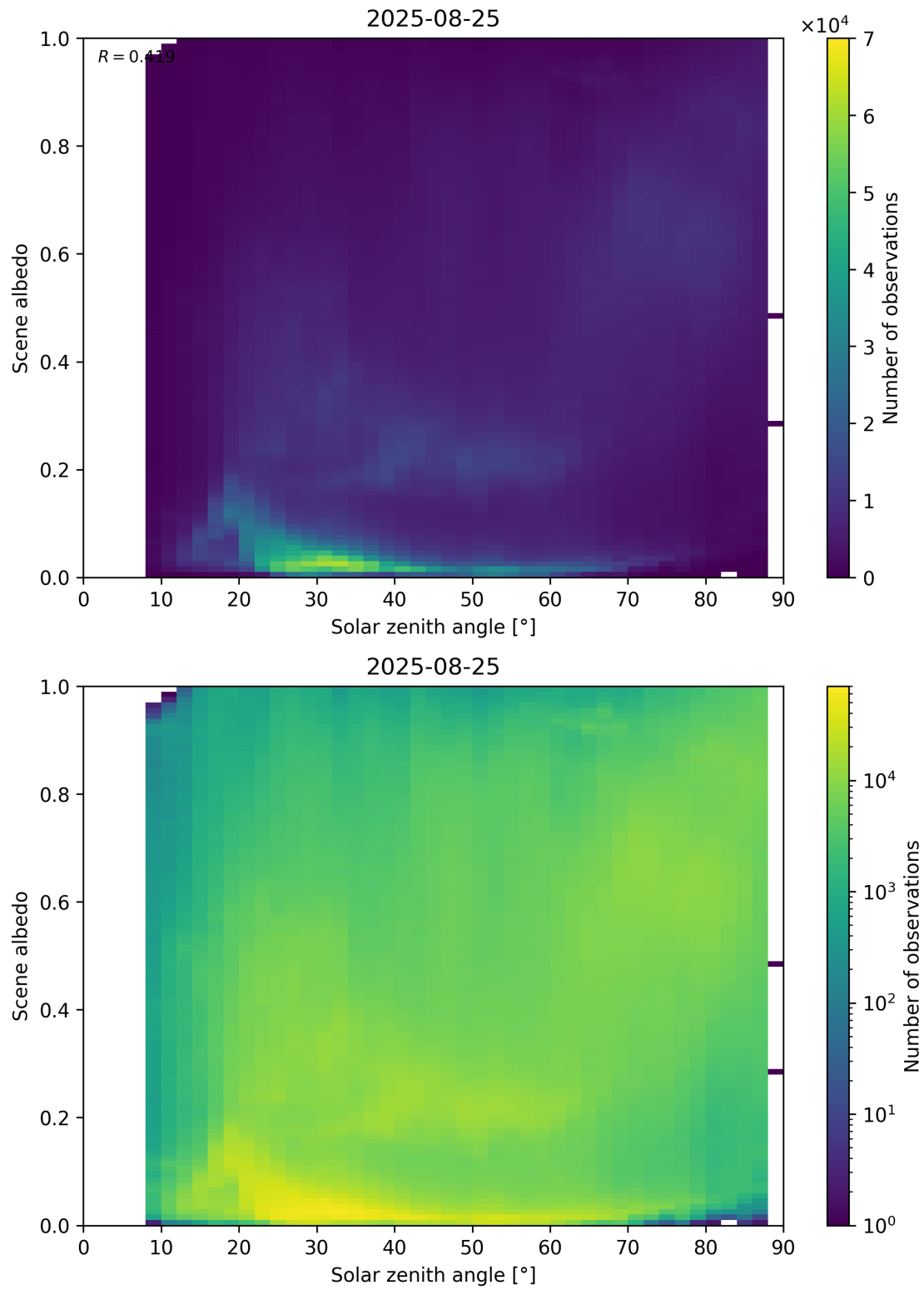
Figure 116: Scatter density plot of “Solar zenith angle” against “Scene albedo” for 2025-08-25 to 2025-08-26.
