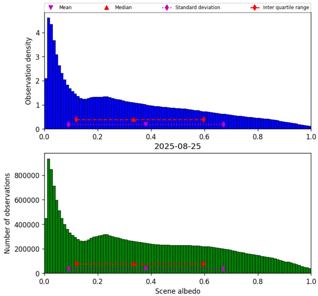
Figure 34: Histogram of “Scene albedo” for 2025-08-25 to 2025-08-26
