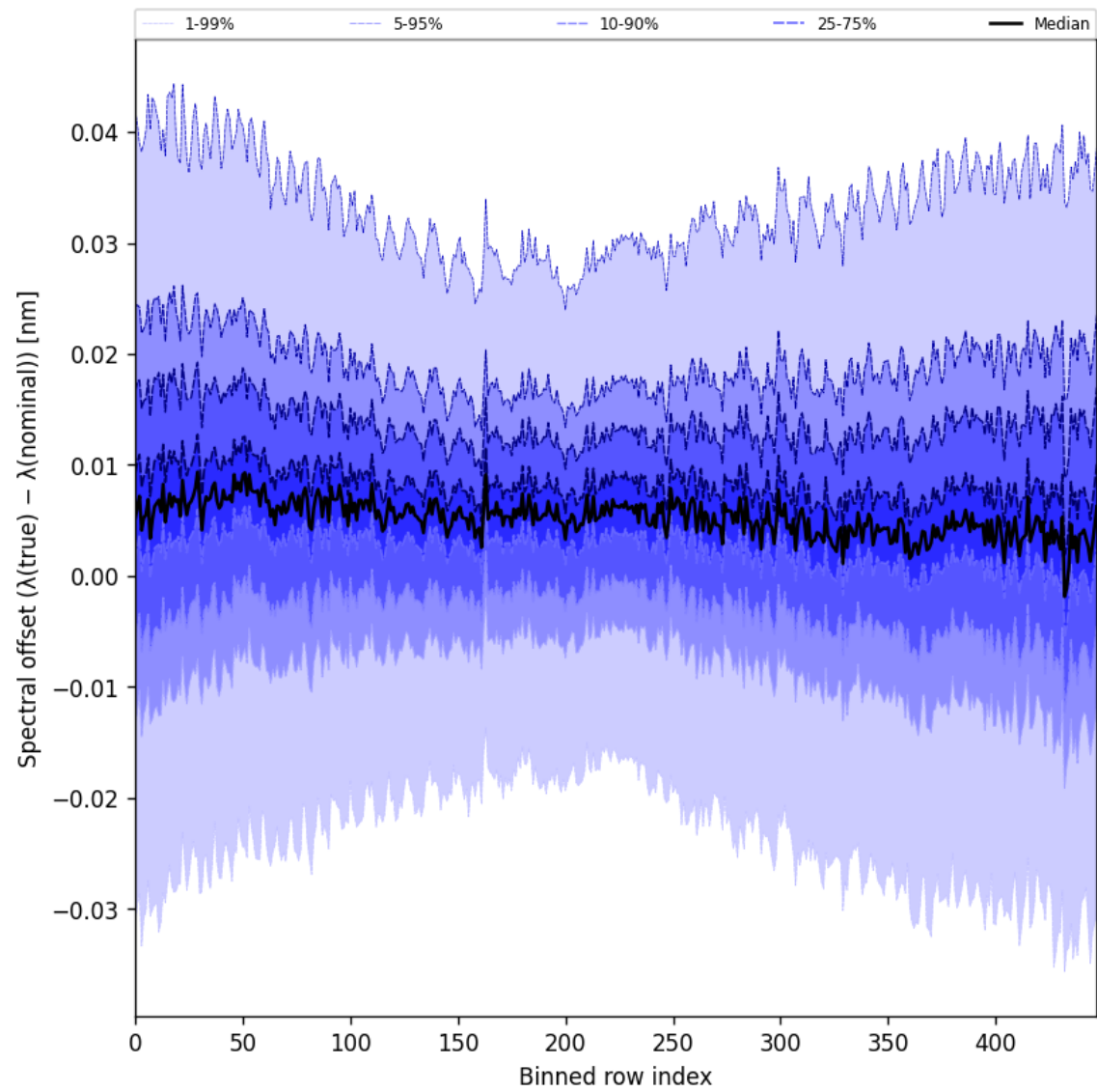
Figure 62: Along track statistics of “Spectral offset ( \lambda_{\text{true}} - \lambda_{\text{nominal}} )” for 2025-08-25 to 2025-08-26
