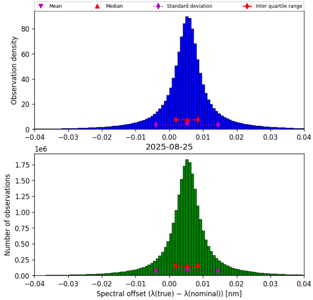
Figure 45: Histogram of “Spectral offset ( \lambda_{\text{true}} - \lambda_{\text{nominal}} )” for 2025-08-25 to 2025-08-26
