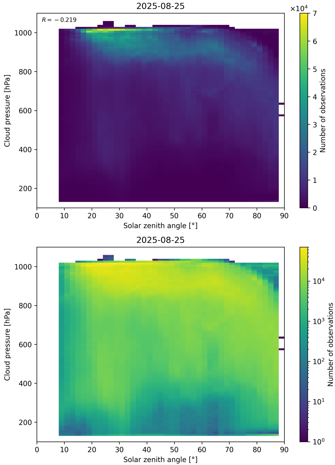
Figure 111: Scatter density plot of “Solar zenith angle” against “Cloud pressure” for 2025-08-25 to 2025-08-26.
