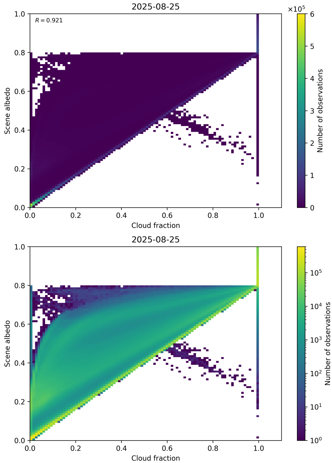
Figure 75: Scatter density plot of “Cloud fraction” against “Scene albedo” for 2025-08-25 to 2025-08-26.
