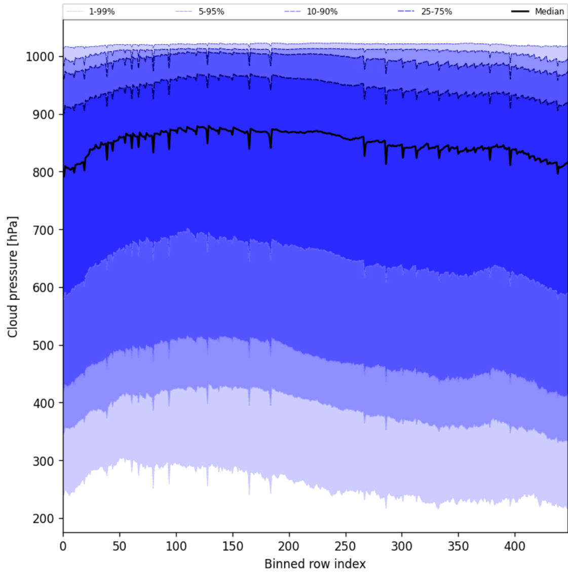
Figure 47: Along track statistics of “Cloud pressure” for 2025-08-25 to 2025-08-26
