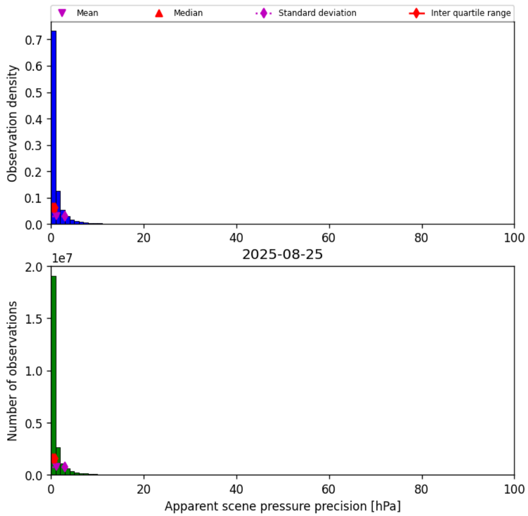
Figure 37: Histogram of “Apparent scene pressure precision” for 2025-08-25 to 2025-08-26
