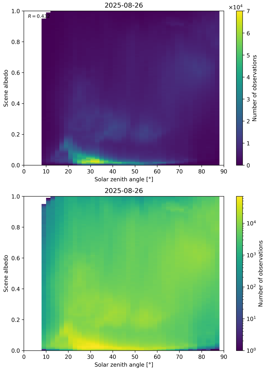
Figure 116: Scatter density plot of “Solar zenith angle” against “Scene albedo” for 2025-08-25 to 2025-08-27.
