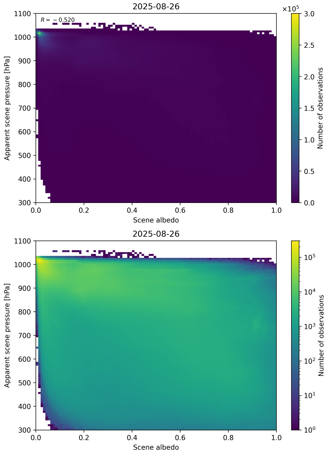
Figure 102: Scatter density plot of “Scene albedo” against “Apparent scene pressure” for 2025-08-25 to 2025-08-27.
