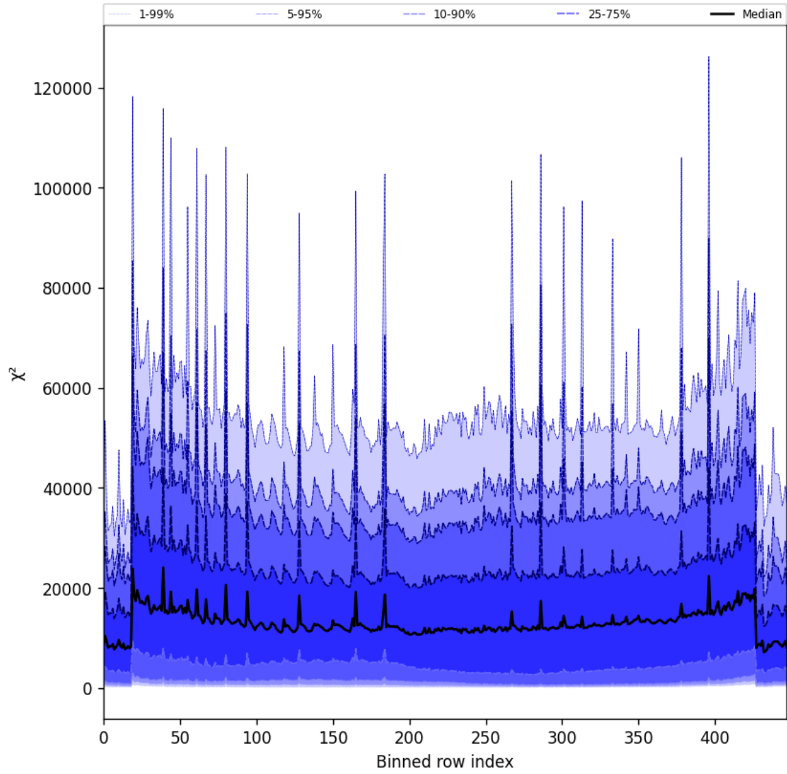
Figure 55: Along track statistics of “ \chi^2 ” for 2025-08-25 to 2025-08-27
