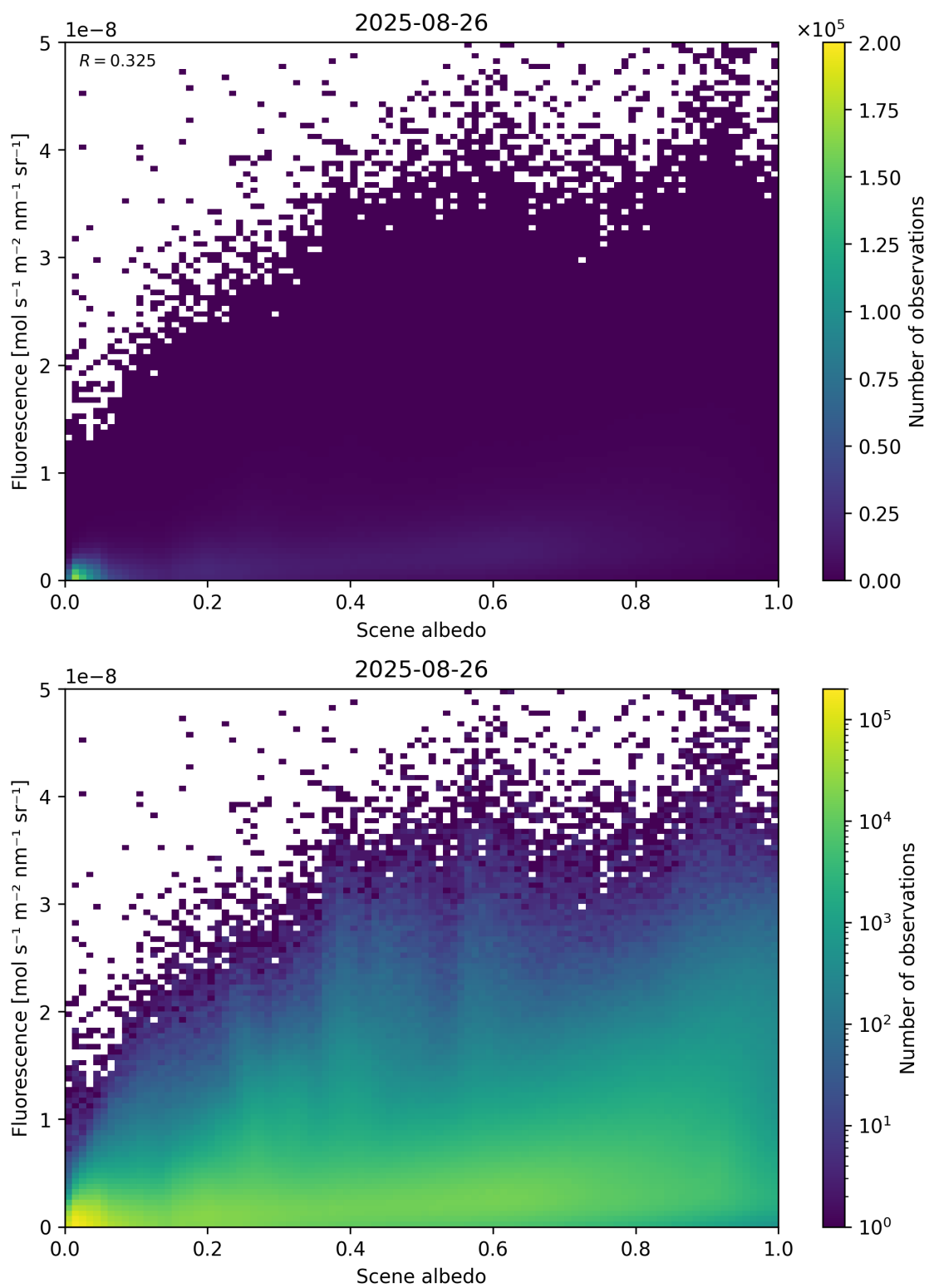
Figure 104: Scatter density plot of “Scene albedo” against “Fluorescence” for 2025-08-25 to 2025-08-27.
