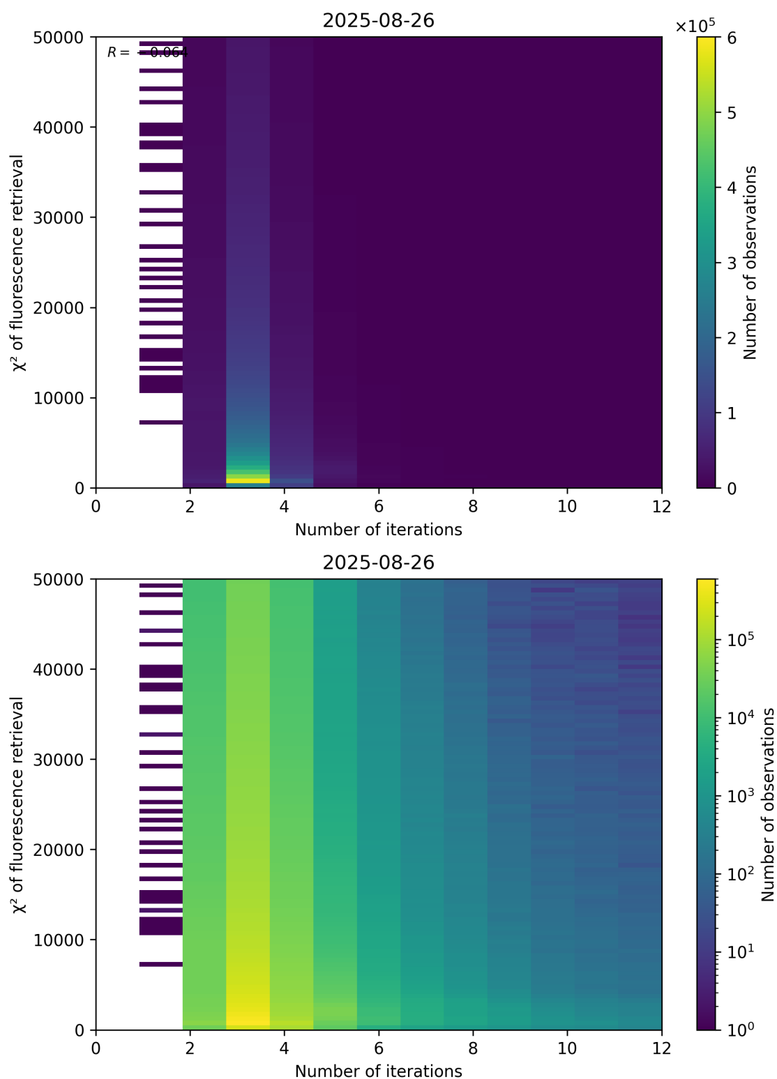
Figure 97: Scatter density plot of “Number of iterations” against “ \chi^2 of fluorescence retrieval” for 2025-08-25 to 2025-08-27.
