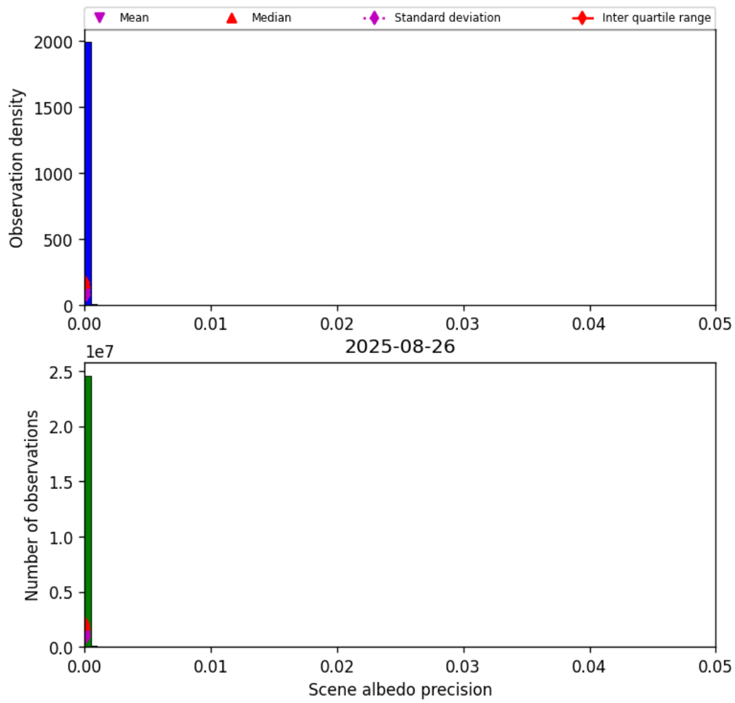
Figure 35: Histogram of “Scene albedo precision” for 2025-08-25 to 2025-08-27
