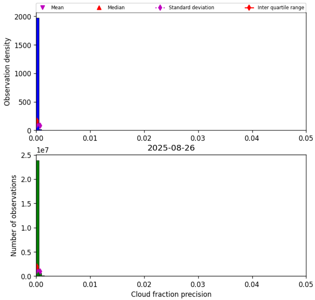
Figure 33: Histogram of “Cloud fraction precision” for 2025-08-25 to 2025-08-27
