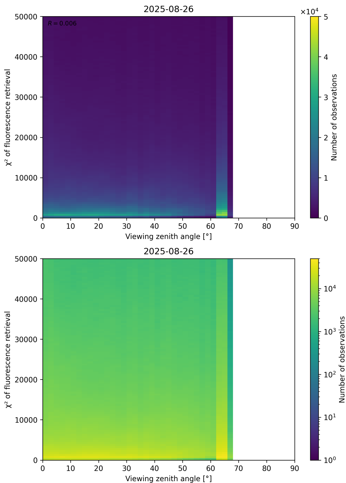
Figure 119: Scatter density plot of “Viewing zenith angle” against “ \chi^2 of fluorescence retrieval” for 2025-08-25 to 2025-08-27.
