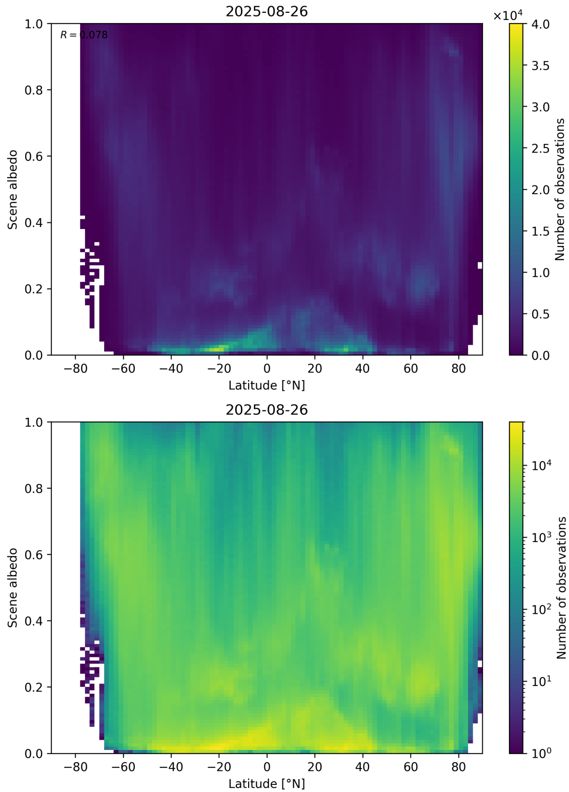
Figure 95: Scatter density plot of “Latitude” against “Scene albedo” for 2025-08-25 to 2025-08-27.
