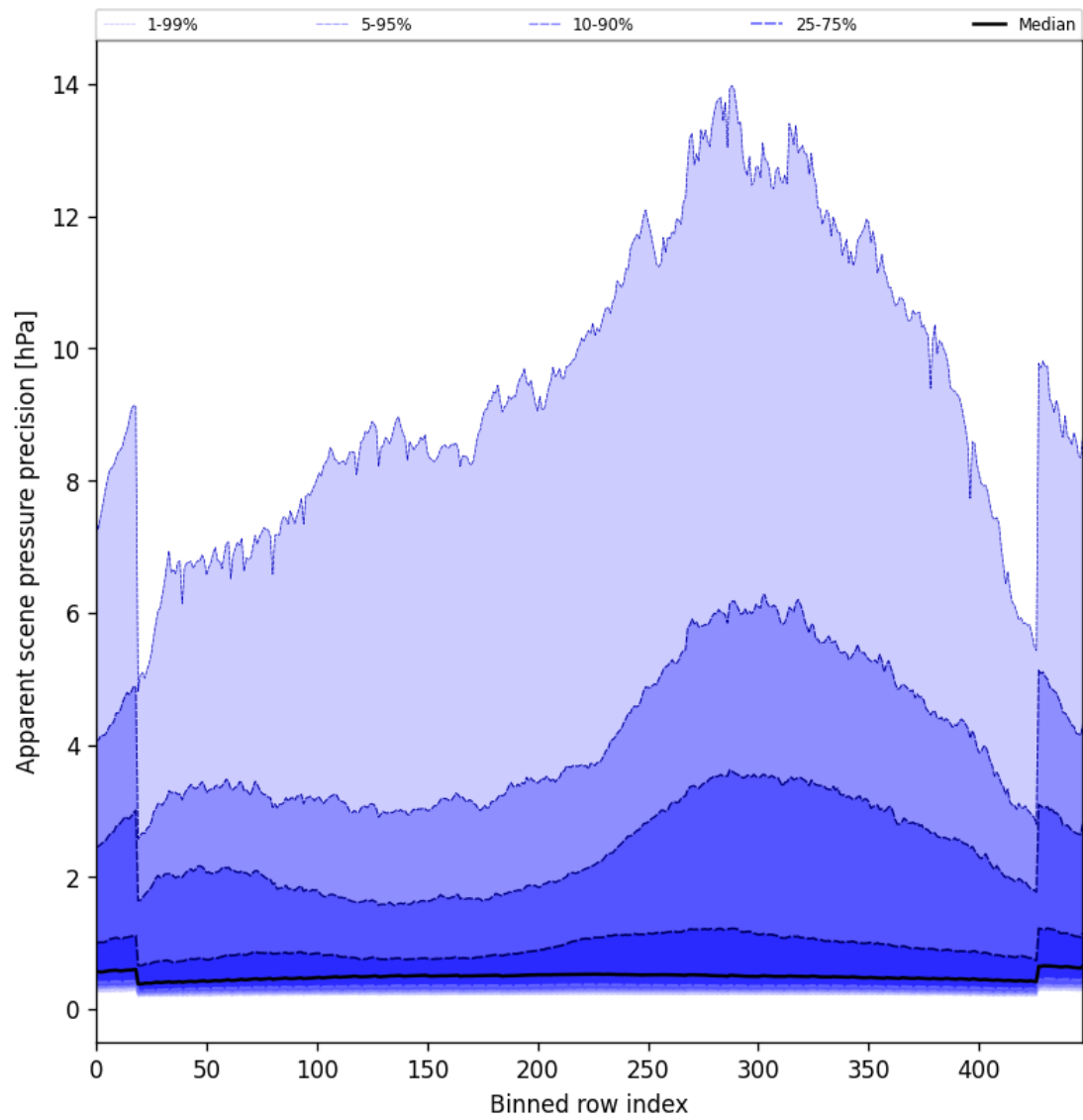
Figure 54: Along track statistics of “Apparent scene pressure precision” for 2025-08-25 to 2025-08-27
