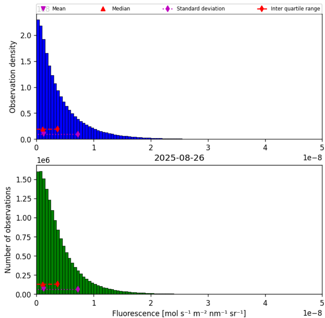
Figure 40: Histogram of “Fluorescence” for 2025-08-25 to 2025-08-27
