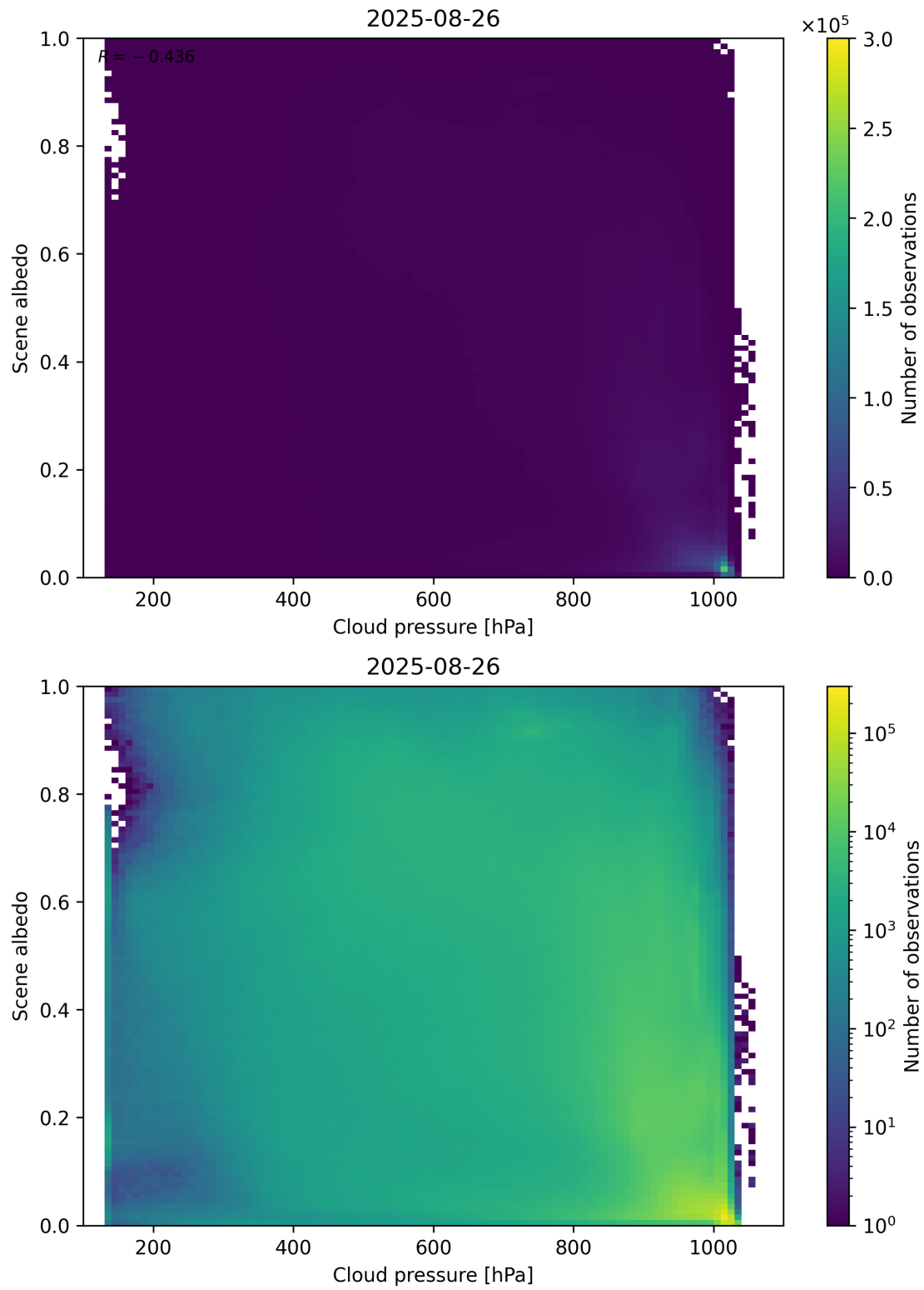
Figure 83: Scatter density plot of “Cloud pressure” against “Scene albedo” for 2025-08-25 to 2025-08-27.
