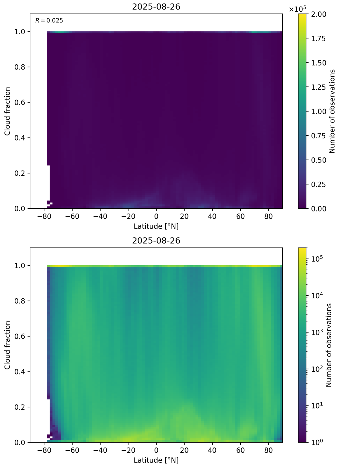
Figure 90: Scatter density plot of “Latitude” against “Cloud fraction” for 2025-08-25 to 2025-08-27.
