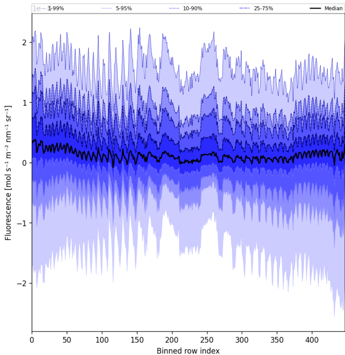
Figure 57: Along track statistics of “Fluorescence” for 2025-08-25 to 2025-08-27
