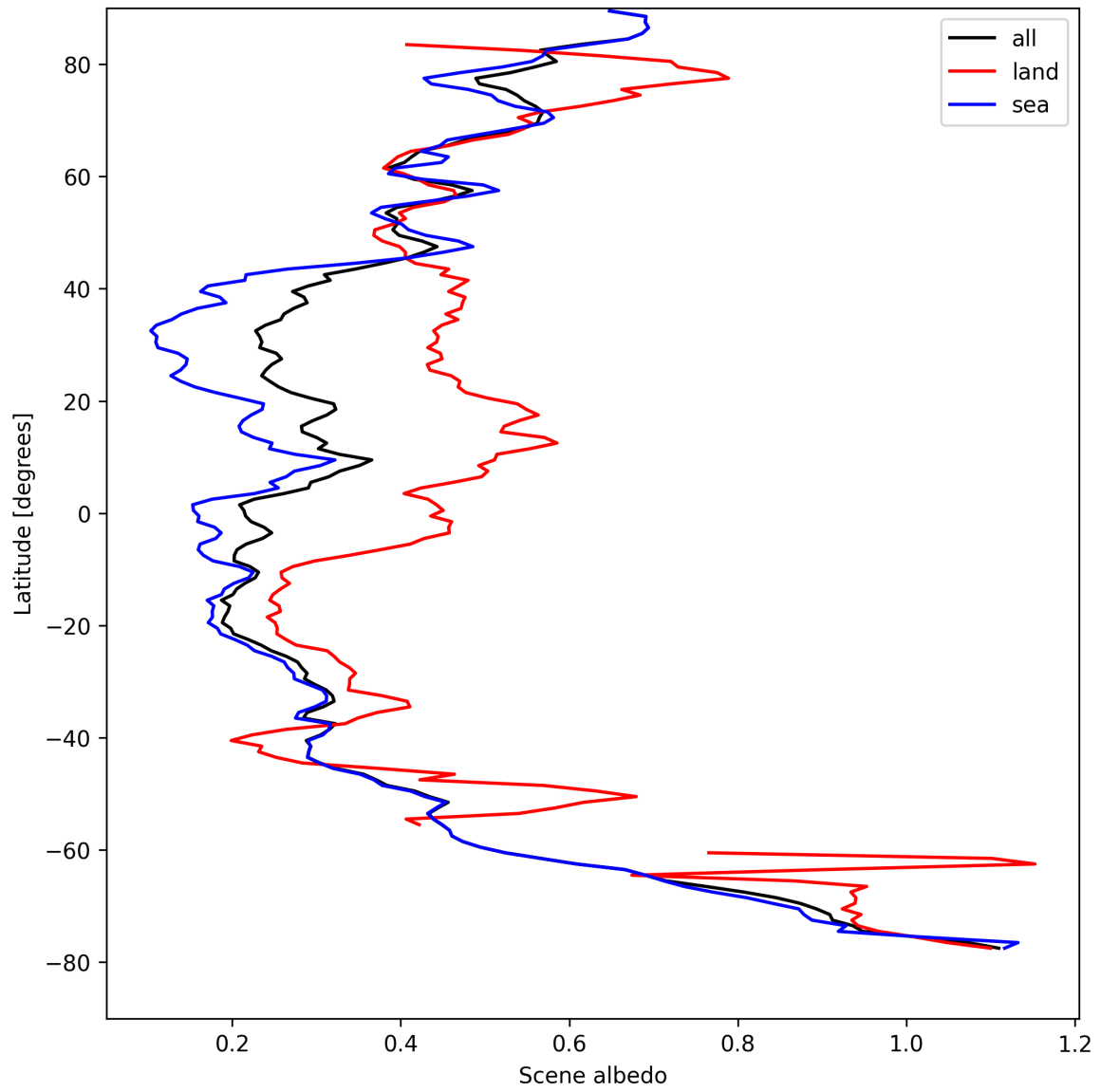
Figure 17: Zonal average of “Scene albedo” for 2025-08-25 to 2025-08-27.
