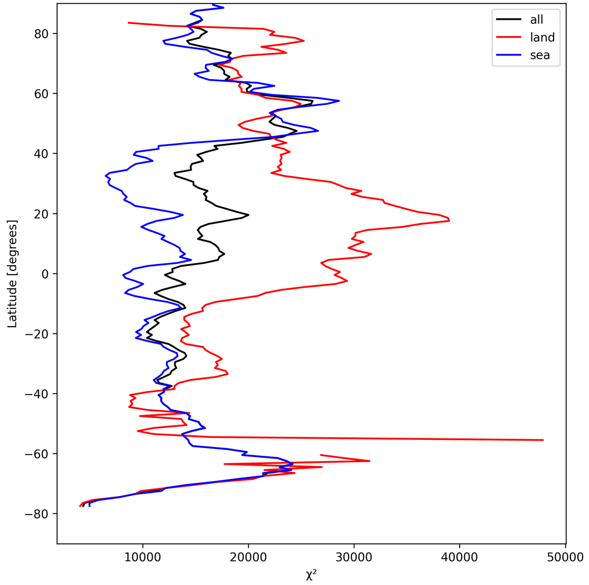
Figure 21: Zonal average of “ \chi^2 ” for 2025-08-25 to 2025-08-27.
