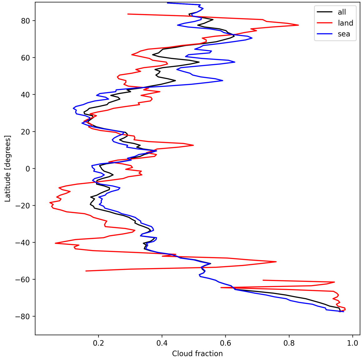
Figure 15: Zonal average of “Cloud fraction” for 2025-08-25 to 2025-08-27.
