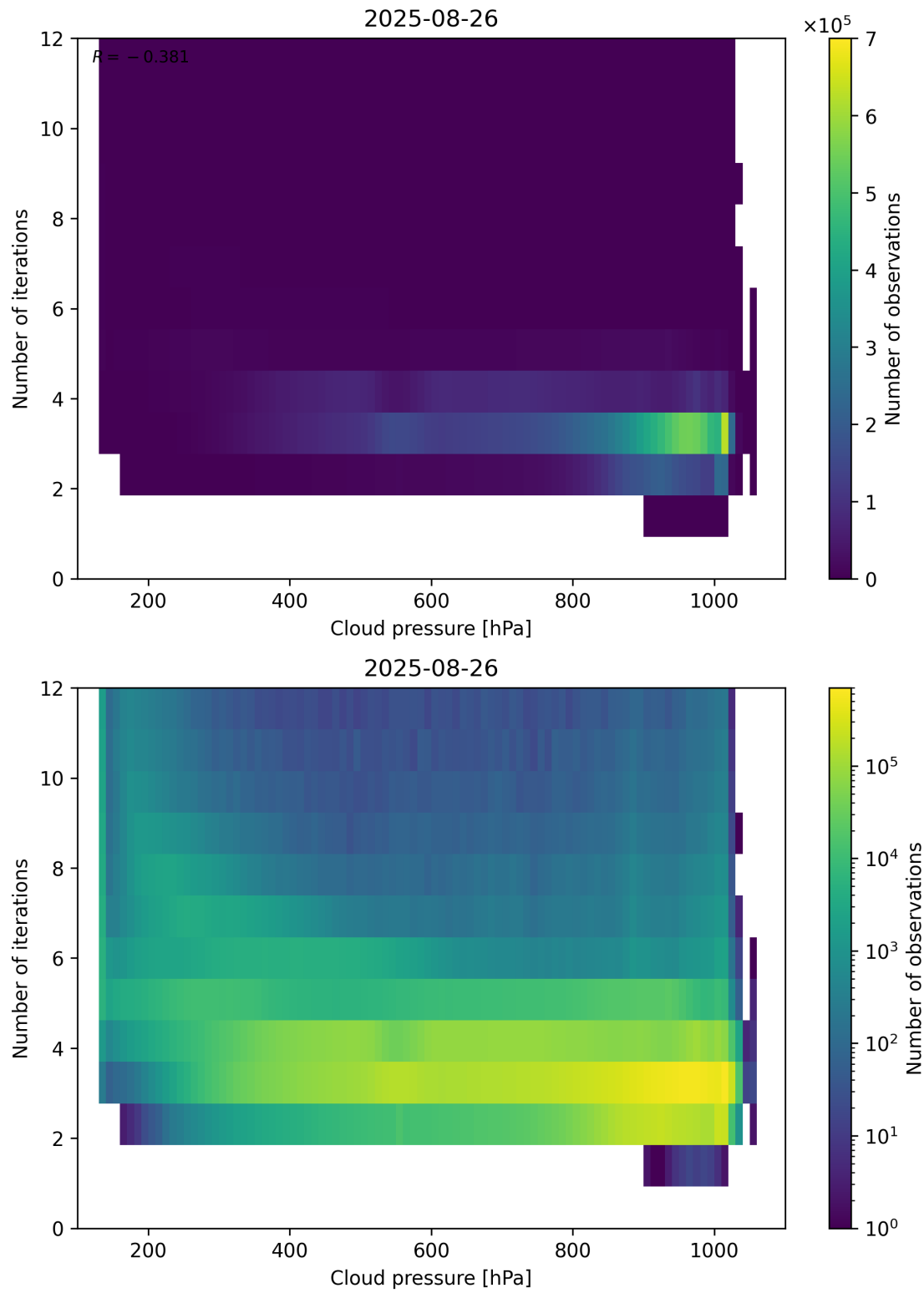
Figure 81: Scatter density plot of “Cloud pressure” against “Number of iterations” for 2025-08-25 to 2025-08-27.
