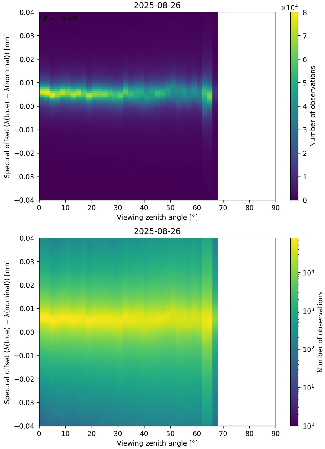
Figure 128: Scatter density plot of “Viewing zenith angle” against “Spectral offset ( \lambda_{\text{true}} - \lambda_{\text{nominal}} )” for 2025-08-25 to 2025-08-27.
