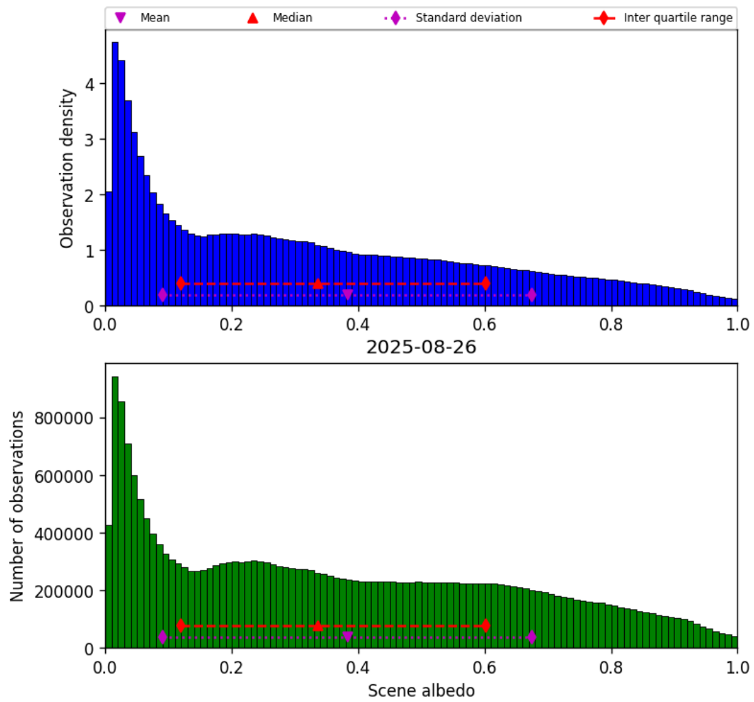
Figure 34: Histogram of “Scene albedo” for 2025-08-25 to 2025-08-27
