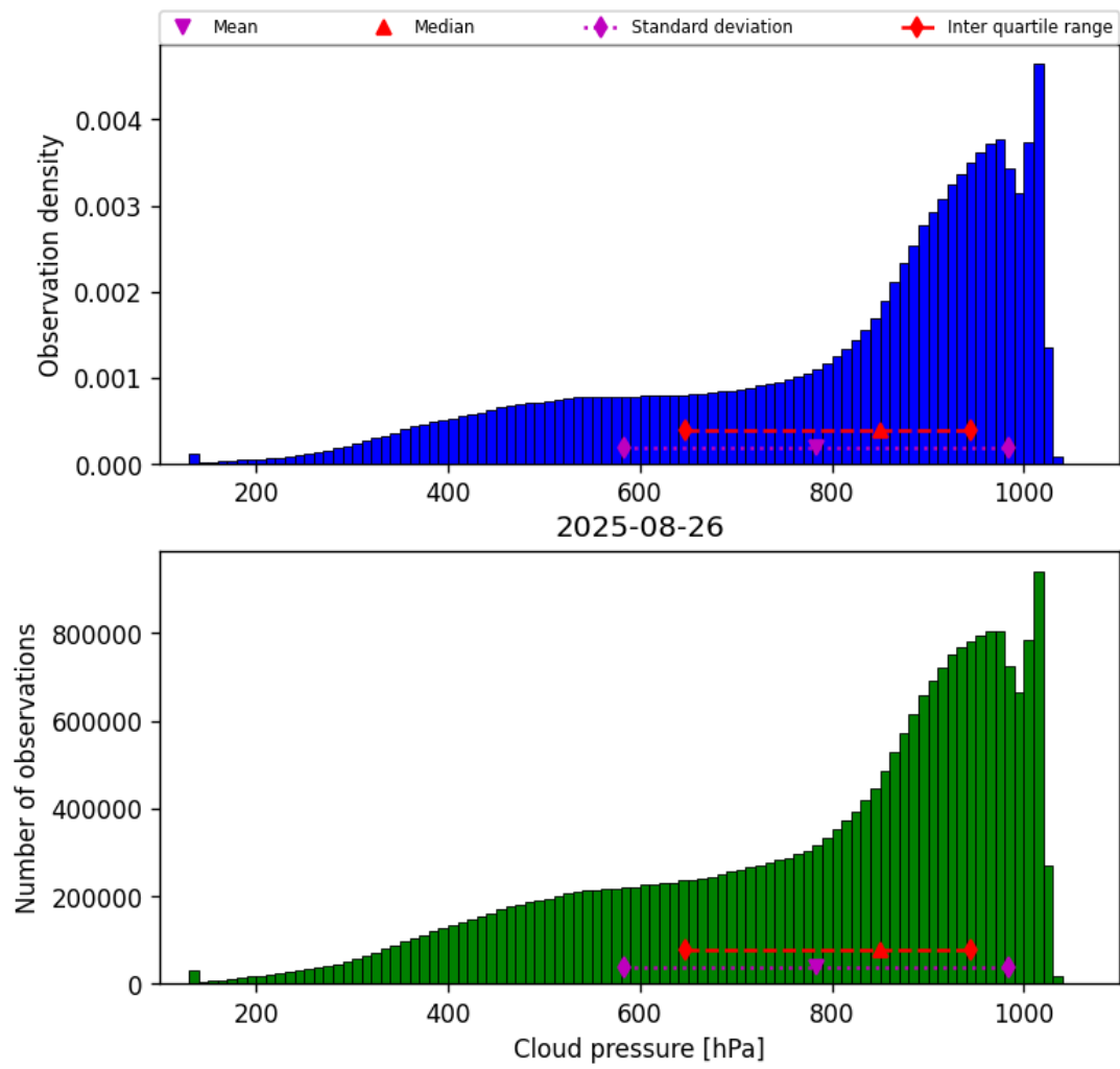
Figure 30: Histogram of “Cloud pressure” for 2025-08-25 to 2025-08-27
