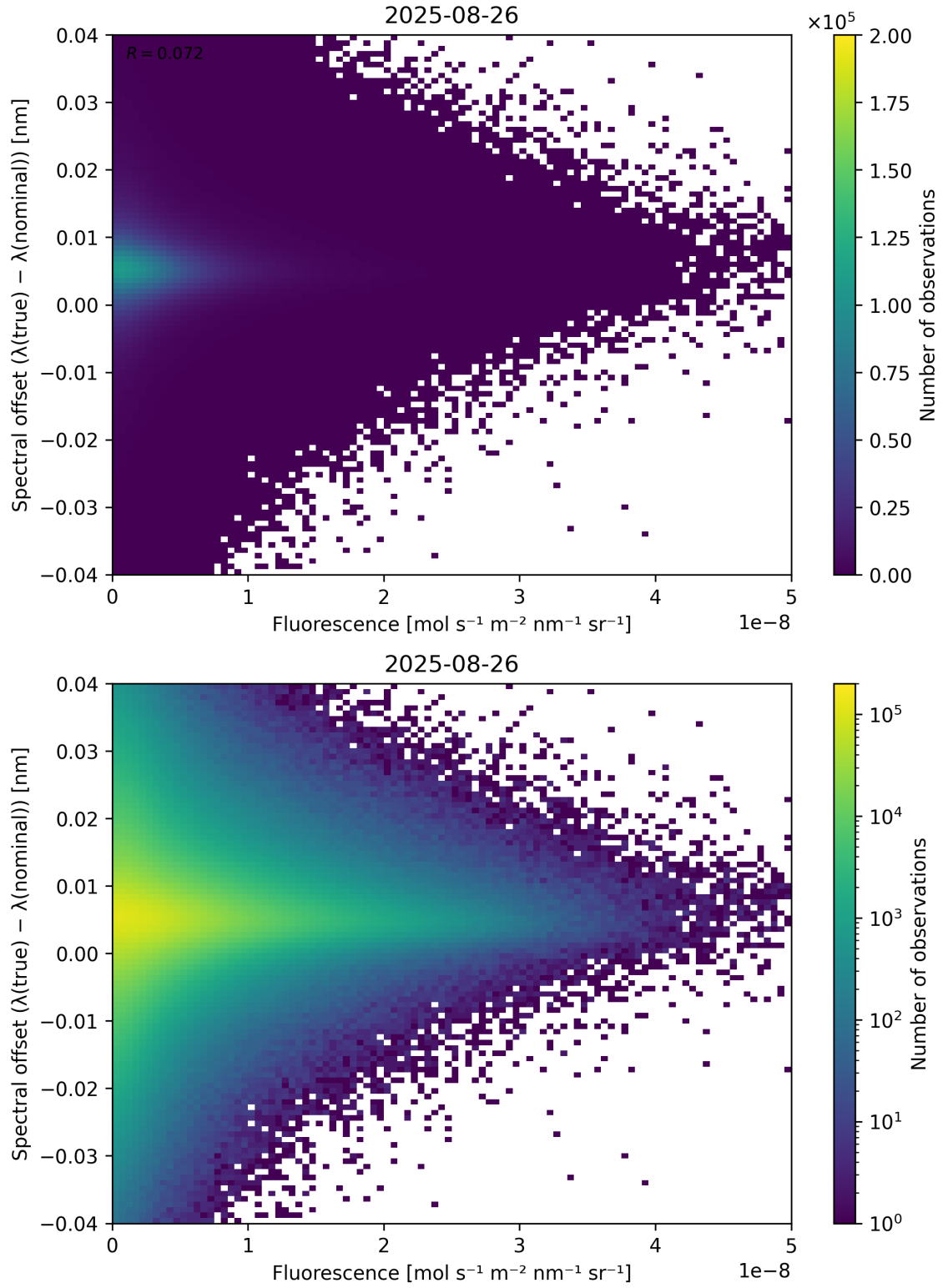
Figure 87: Scatter density plot of “Fluorescence” against “Spectral offset ( \lambda_{\text{true}} - \lambda_{\text{nominal}} )” for 2025-08-25 to 2025-08-27.
