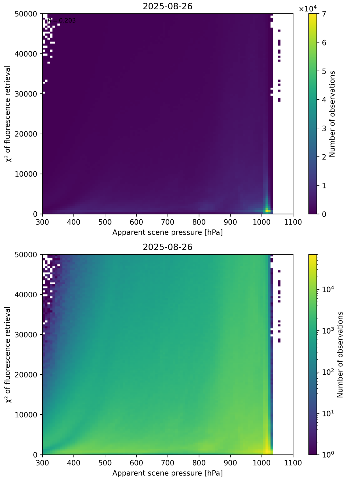
Figure 63: Scatter density plot of “Apparent scene pressure” against “ \chi^2 of fluorescence retrieval” for 2025-08-25 to 2025-08-27.
