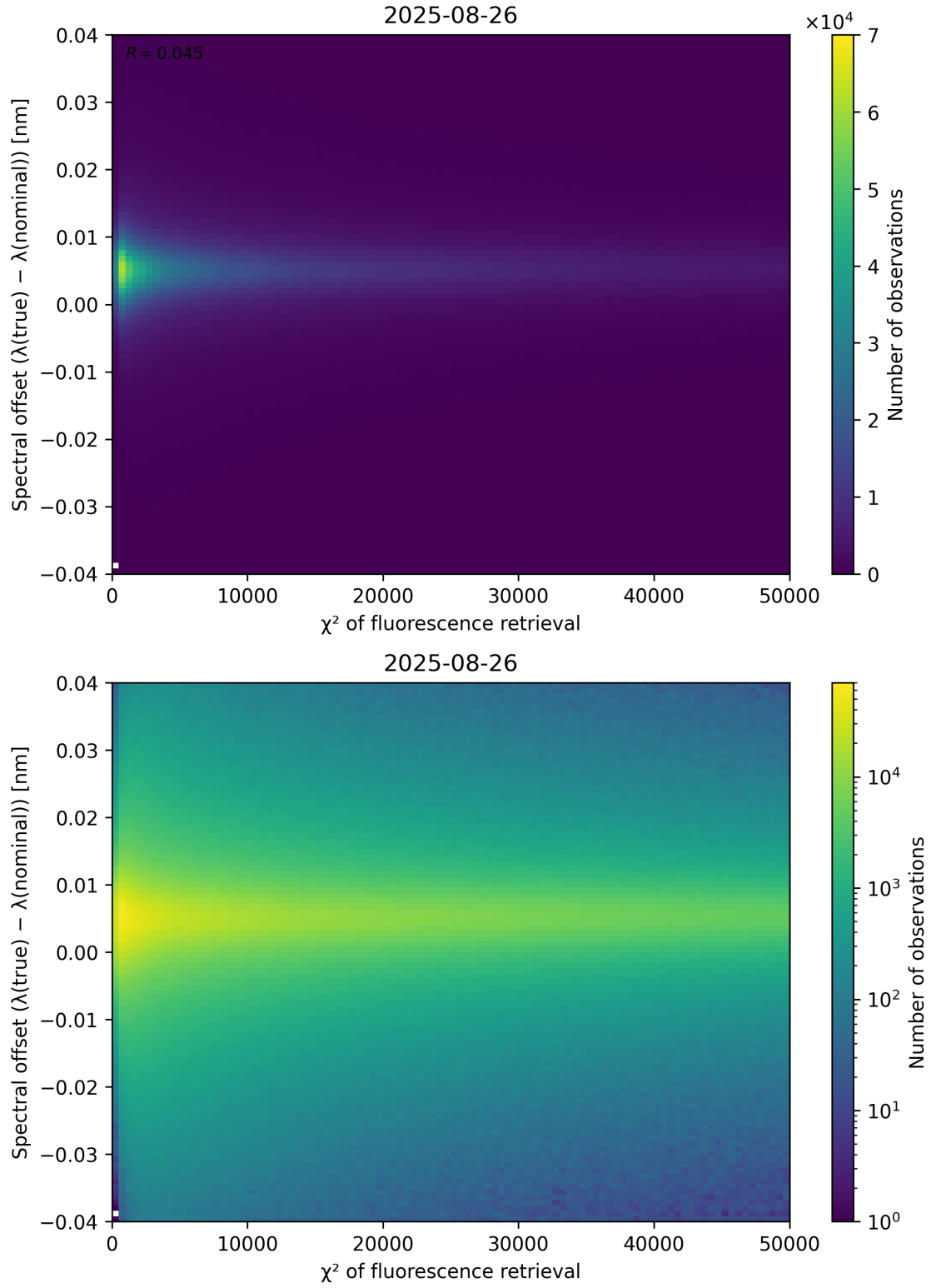
Figure 69: Scatter density plot of “ \chi^2 of fluorescence retrieval” against “Spectral offset ( \lambda_{\text{true}} - \lambda_{\text{nominal}} )” for 2025-08-25 to 2025-08-27.
