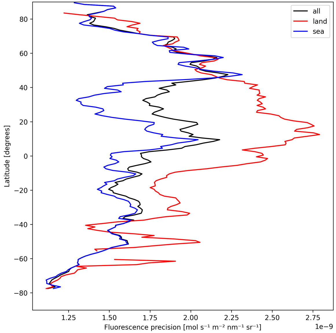
Figure 24: Zonal average of “Fluorescence precision” for 2025-08-25 to 2025-08-27.
