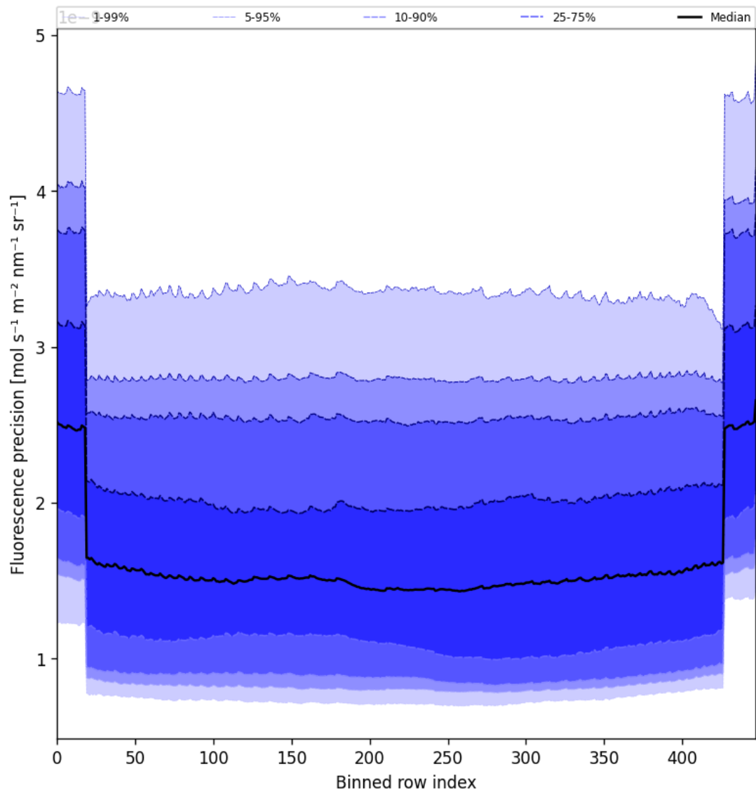
Figure 58: Along track statistics of “Fluorescence precision” for 2025-08-25 to 2025-08-27
