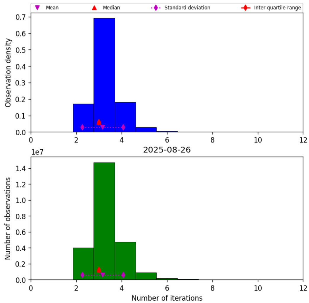
Figure 39: Histogram of “Number of iterations” for 2025-08-25 to 2025-08-27
