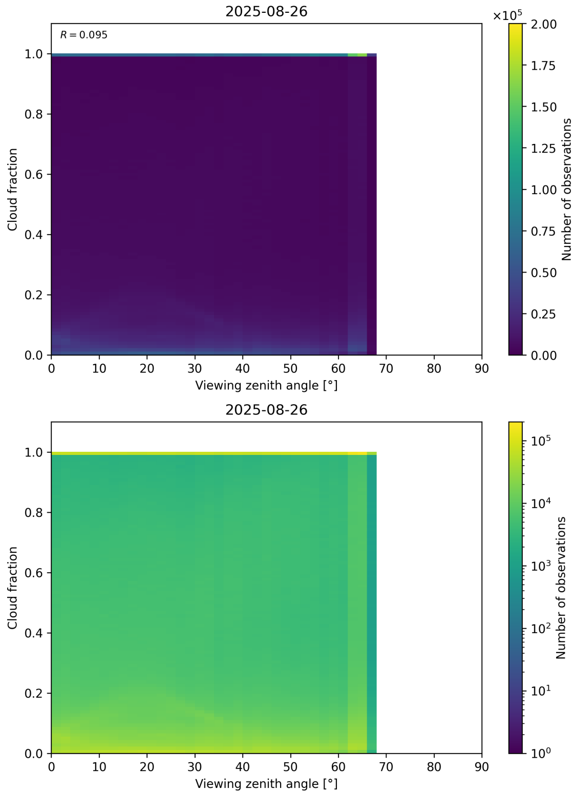
Figure 120: Scatter density plot of “Viewing zenith angle” against “Cloud fraction” for 2025-08-25 to 2025-08-27.
