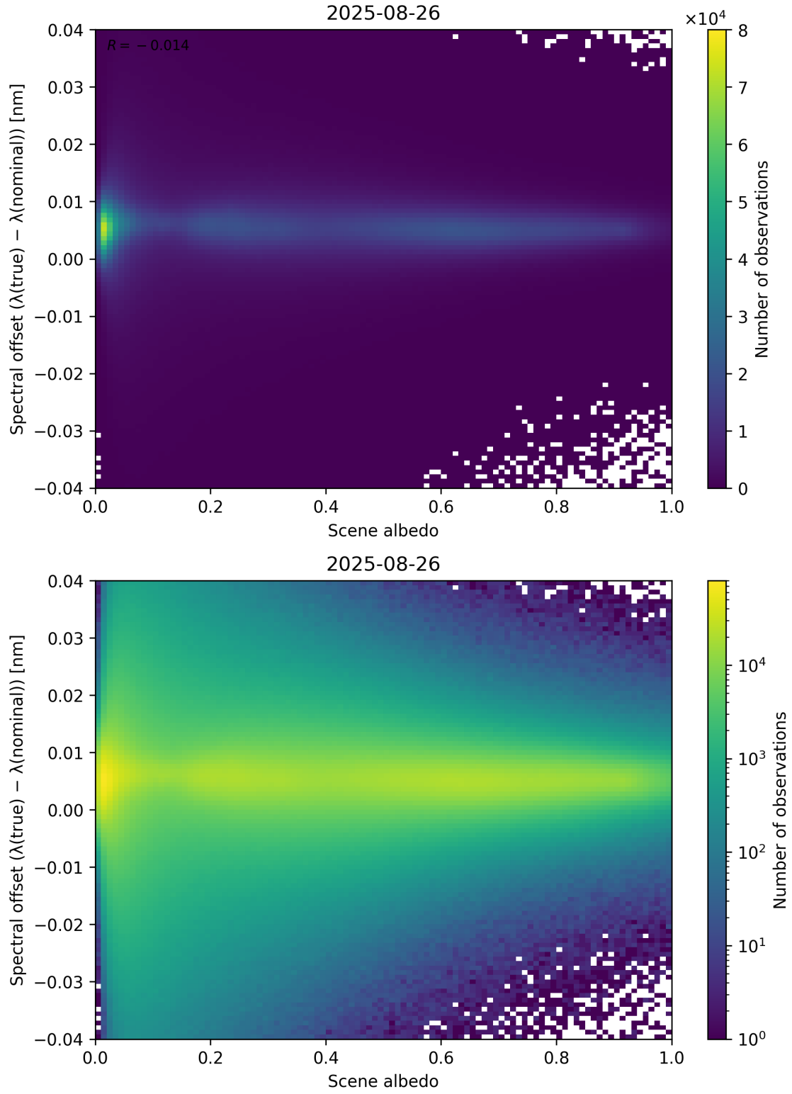
Figure 107: Scatter density plot of “Scene albedo” against “Spectral offset ( \lambda_{\text{true}} - \lambda_{\text{nominal}} )” for 2025-08-25 to 2025-08-27.
