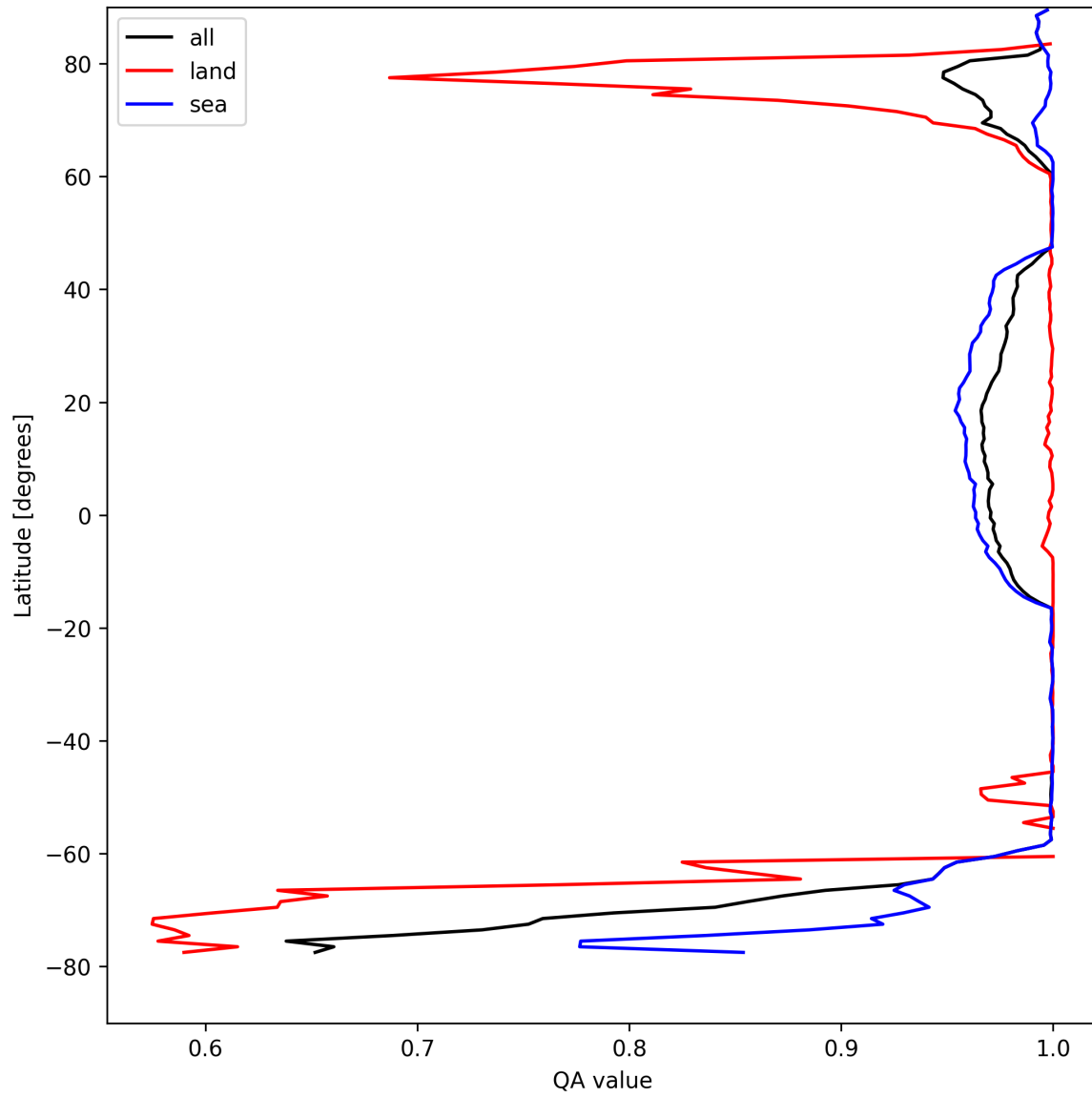
Figure 12: Zonal average of “QA value” for 2025-08-25 to 2025-08-27.
