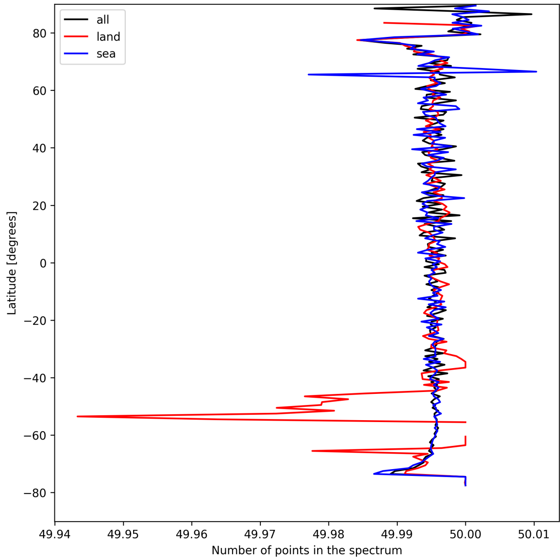
Figure 27: Zonal average of “Number of points in the spectrum” for 2025-08-25 to 2025-08-27.
