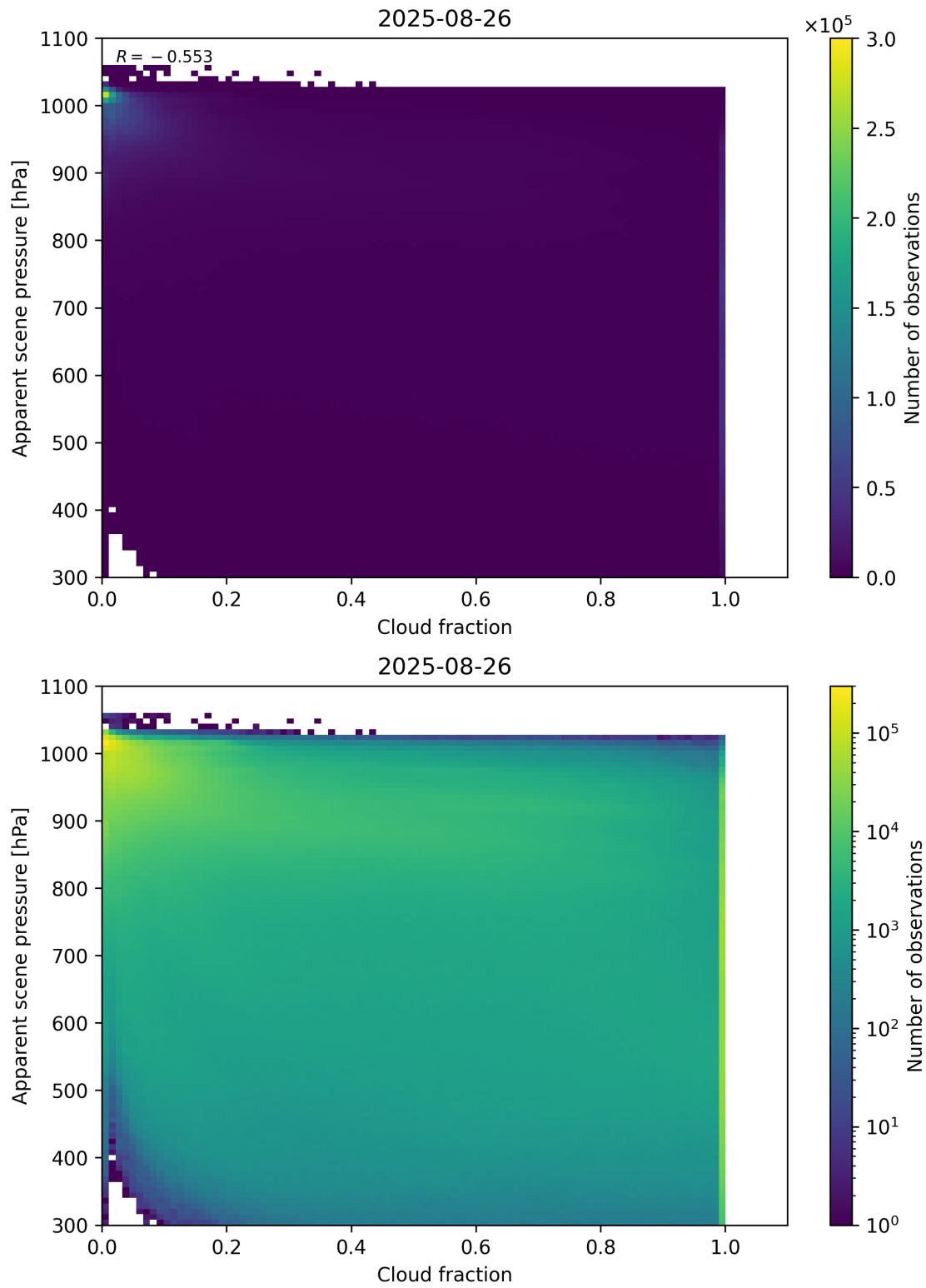
Figure 70: Scatter density plot of “Cloud fraction” against “Apparent scene pressure” for 2025-08-25 to 2025-08-27.
