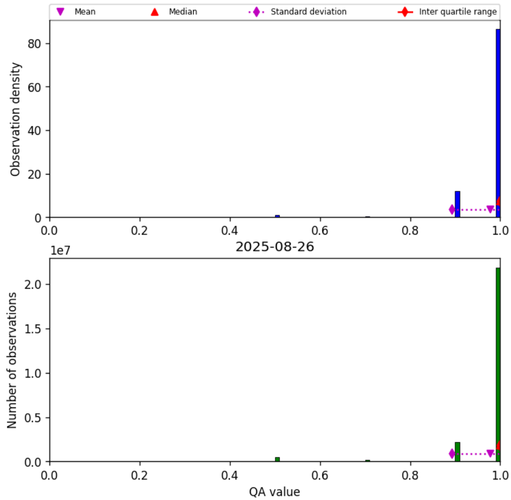
Figure 29: Histogram of “QA value” for 2025-08-25 to 2025-08-27
