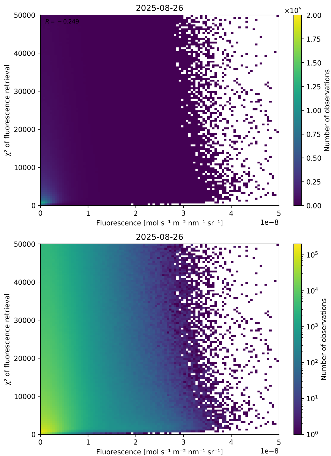
Figure 85: Scatter density plot of “Fluorescence” against “ \chi^2 of fluorescence retrieval” for 2025-08-25 to 2025-08-27.
