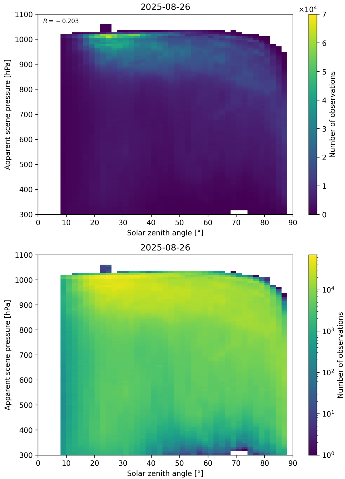
Figure 108: Scatter density plot of “Solar zenith angle” against “Apparent scene pressure” for 2025-08-25 to 2025-08-27.
