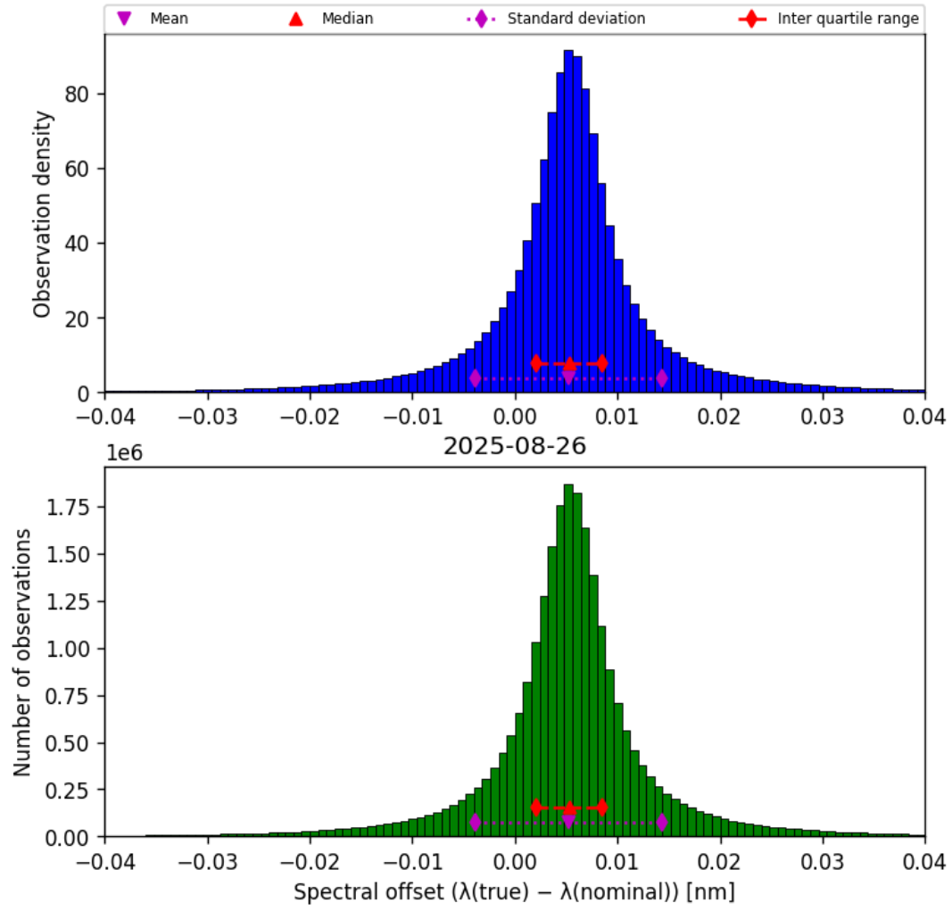
Figure 45: Histogram of “Spectral offset ( \lambda_{\text{true}} - \lambda_{\text{nominal}} )” for 2025-08-25 to 2025-08-27
