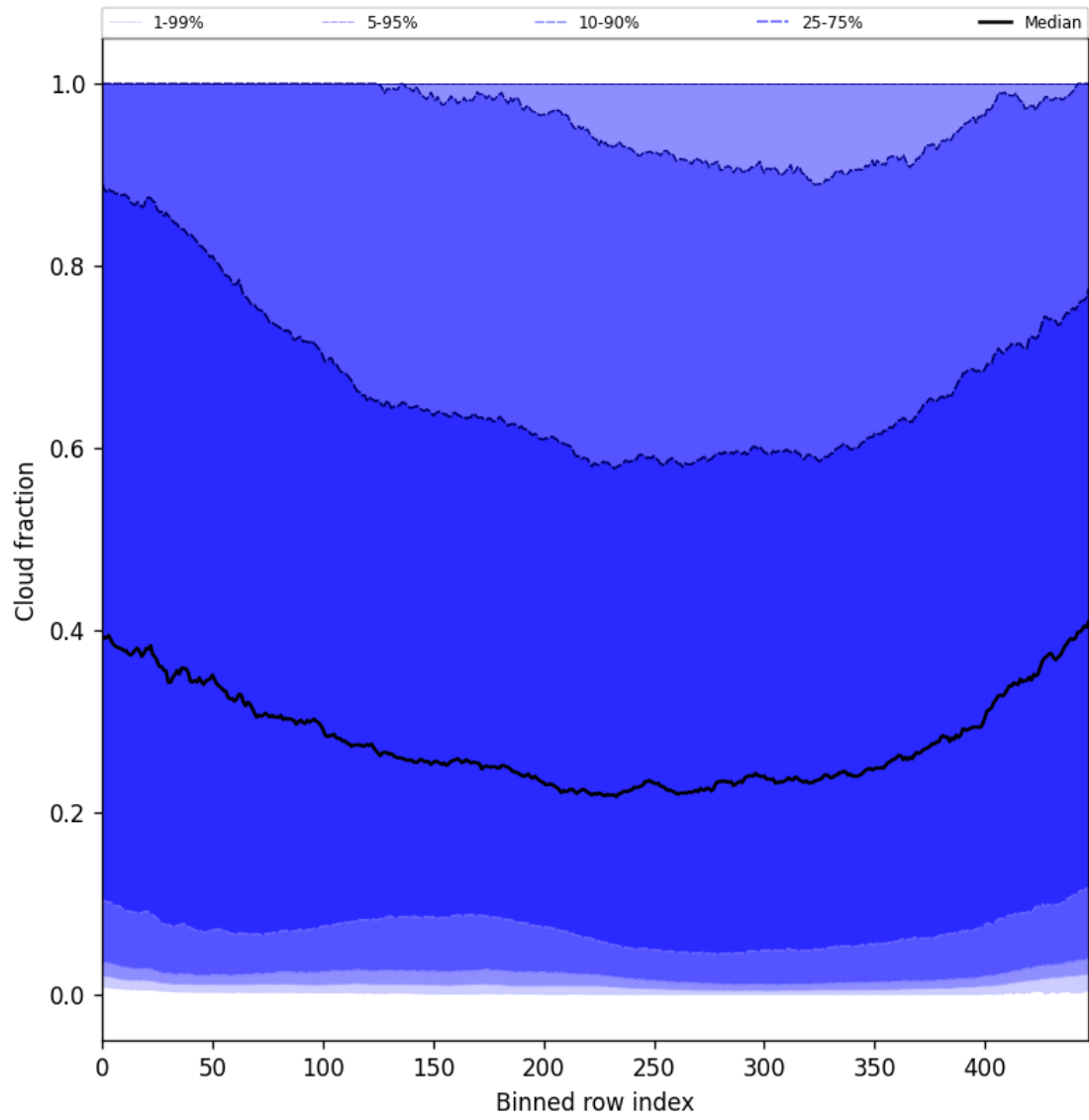
Figure 49: Along track statistics of “Cloud fraction” for 2025-08-25 to 2025-08-27
