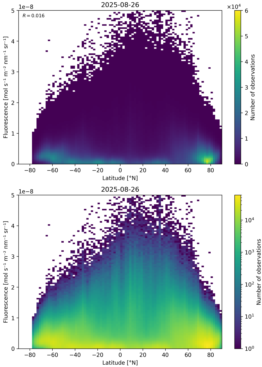
Figure 92: Scatter density plot of “Latitude” against “Fluorescence” for 2025-08-25 to 2025-08-27.
