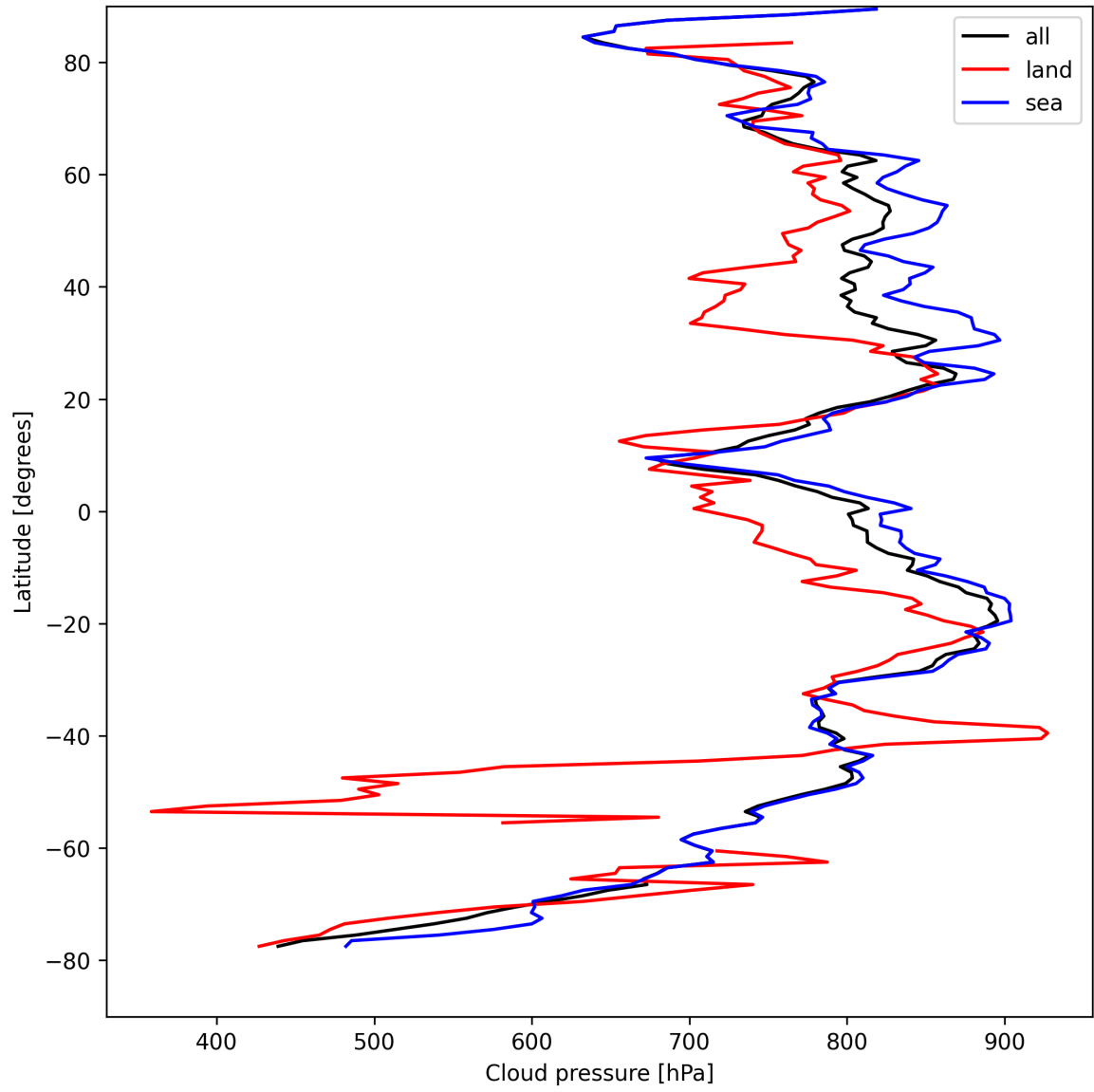
Figure 13: Zonal average of “Cloud pressure” for 2025-08-25 to 2025-08-27.
