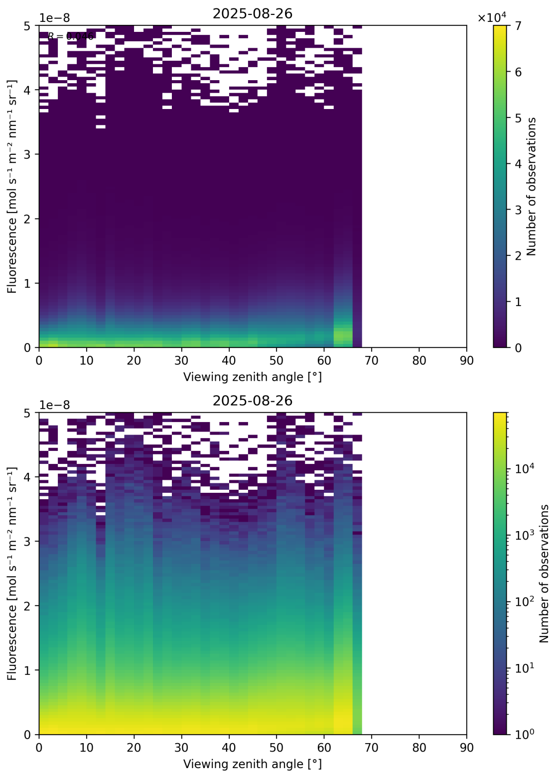
Figure 122: Scatter density plot of “Viewing zenith angle” against “Fluorescence” for 2025-08-25 to 2025-08-27.
