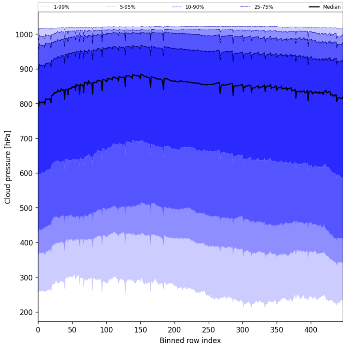
Figure 47: Along track statistics of “Cloud pressure” for 2025-08-25 to 2025-08-27
