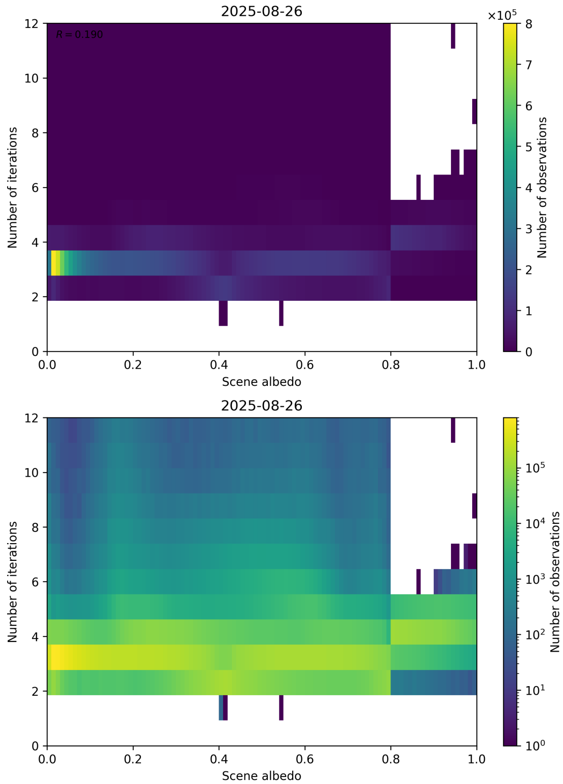
Figure 105: Scatter density plot of “Scene albedo” against “Number of iterations” for 2025-08-25 to 2025-08-27.
