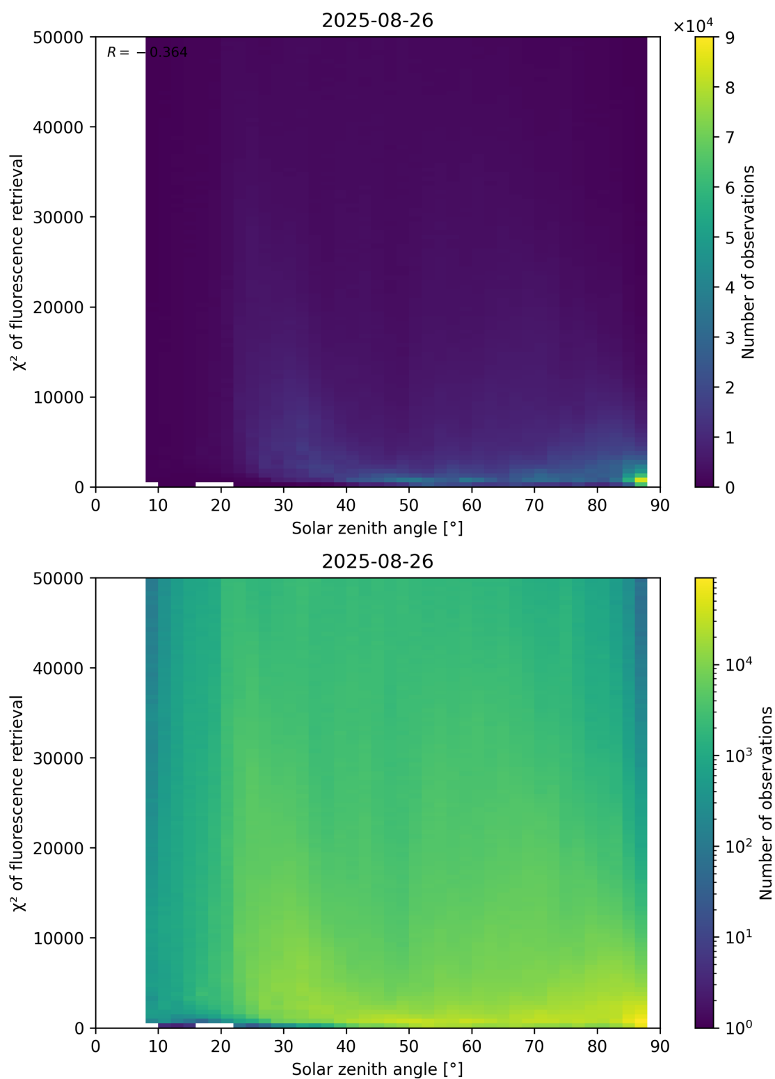
Figure 109: Scatter density plot of “Solar zenith angle” against “ \chi^2 of fluorescence retrieval” for 2025-08-25 to 2025-08-27.
