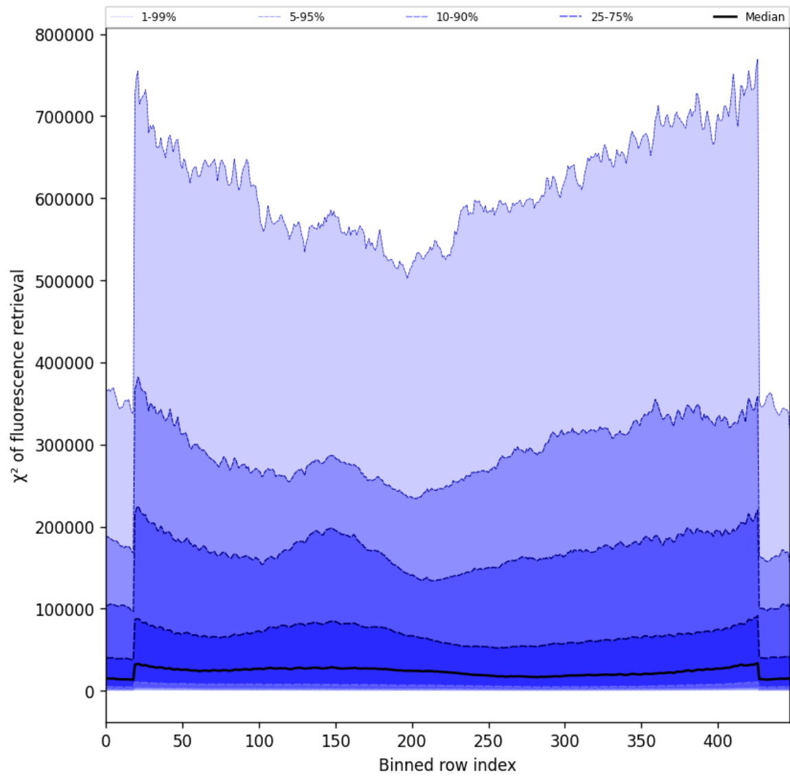
Figure 59: Along track statistics of “ \chi^2 of fluorescence retrieval” for 2025-08-25 to 2025-08-27
