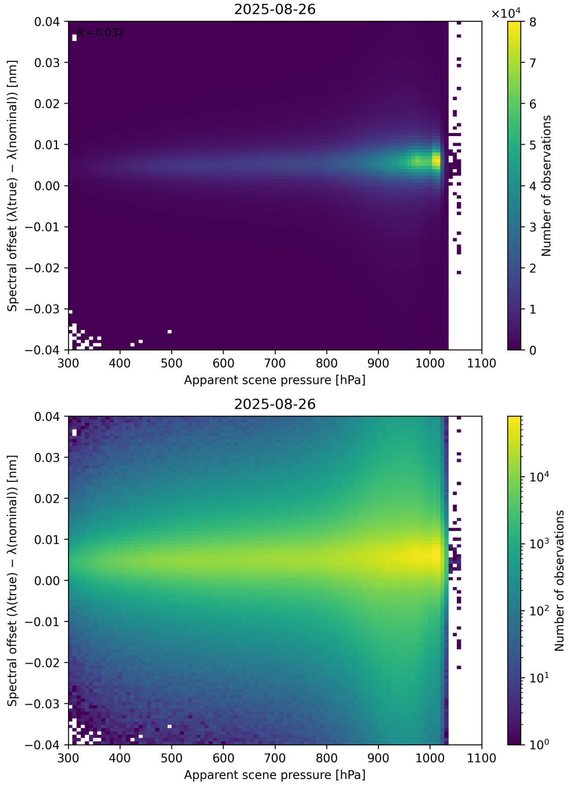
Figure 67: Scatter density plot of “Apparent scene pressure” against “Spectral offset ( \lambda_{\text{true}} - \lambda_{\text{nominal}} )” for 2025-08-25 to 2025-08-27.
