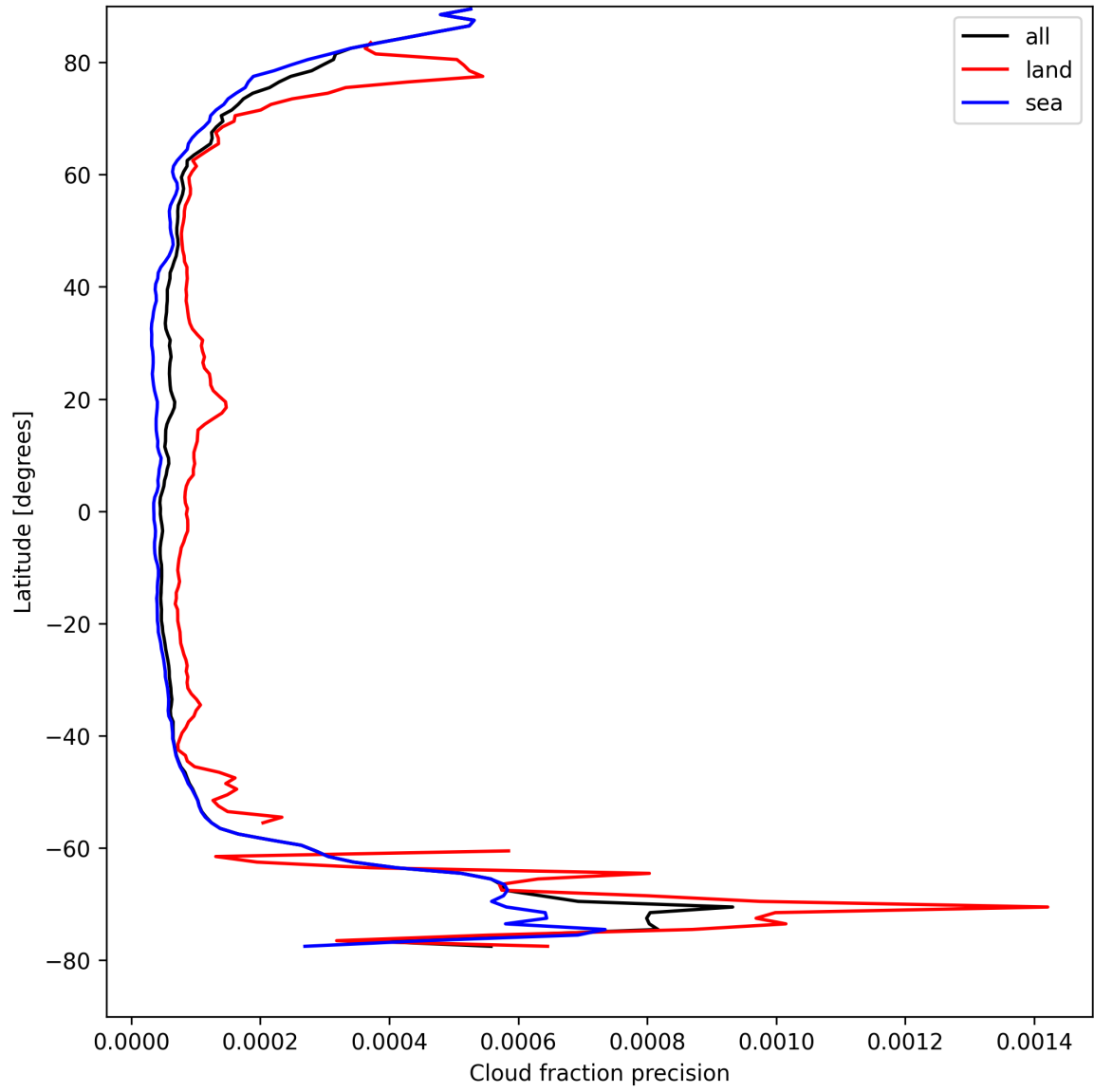
Figure 16: Zonal average of “Cloud fraction precision” for 2025-08-25 to 2025-08-27.
