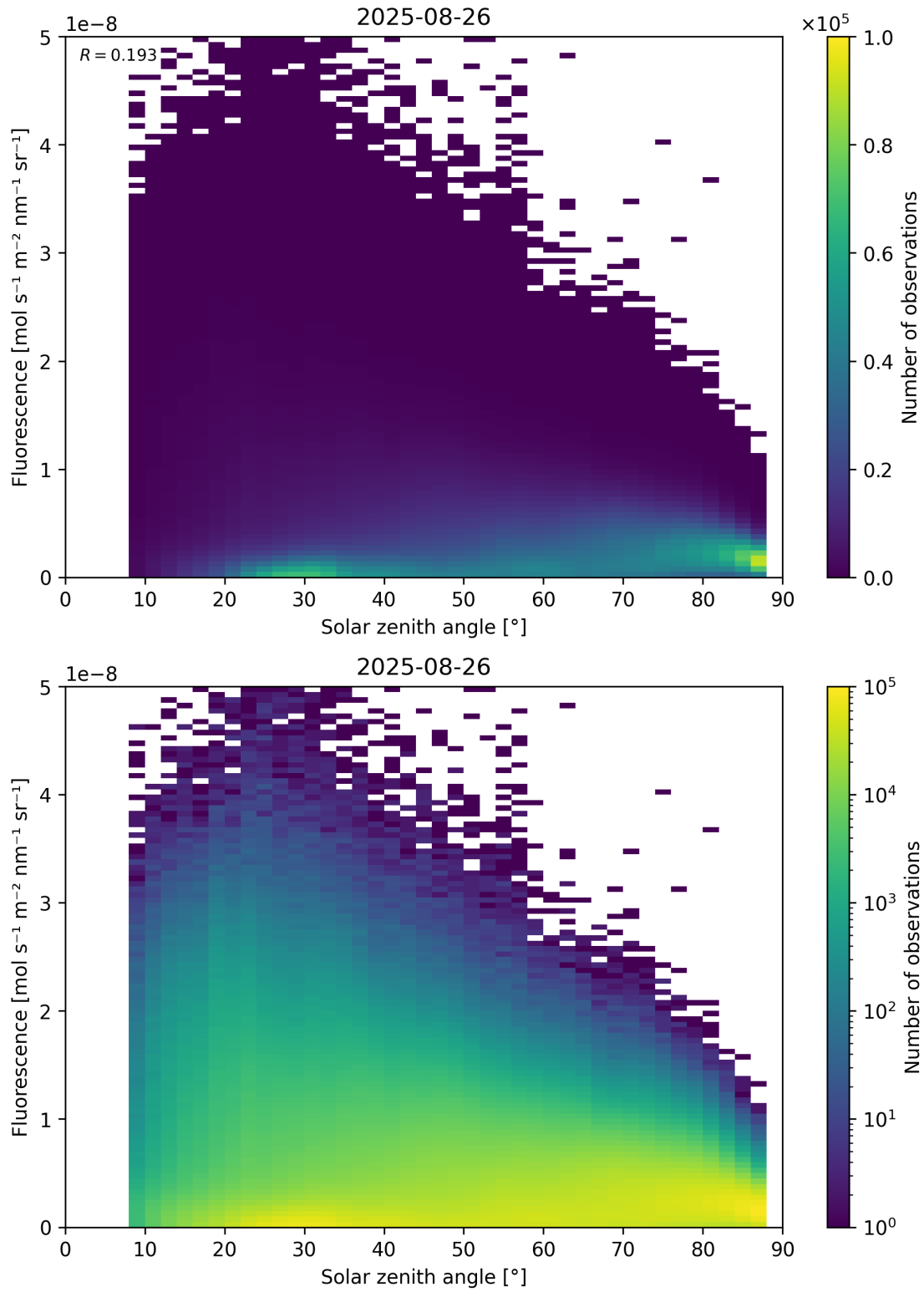
Figure 112: Scatter density plot of “Solar zenith angle” against “Fluorescence” for 2025-08-25 to 2025-08-27.
