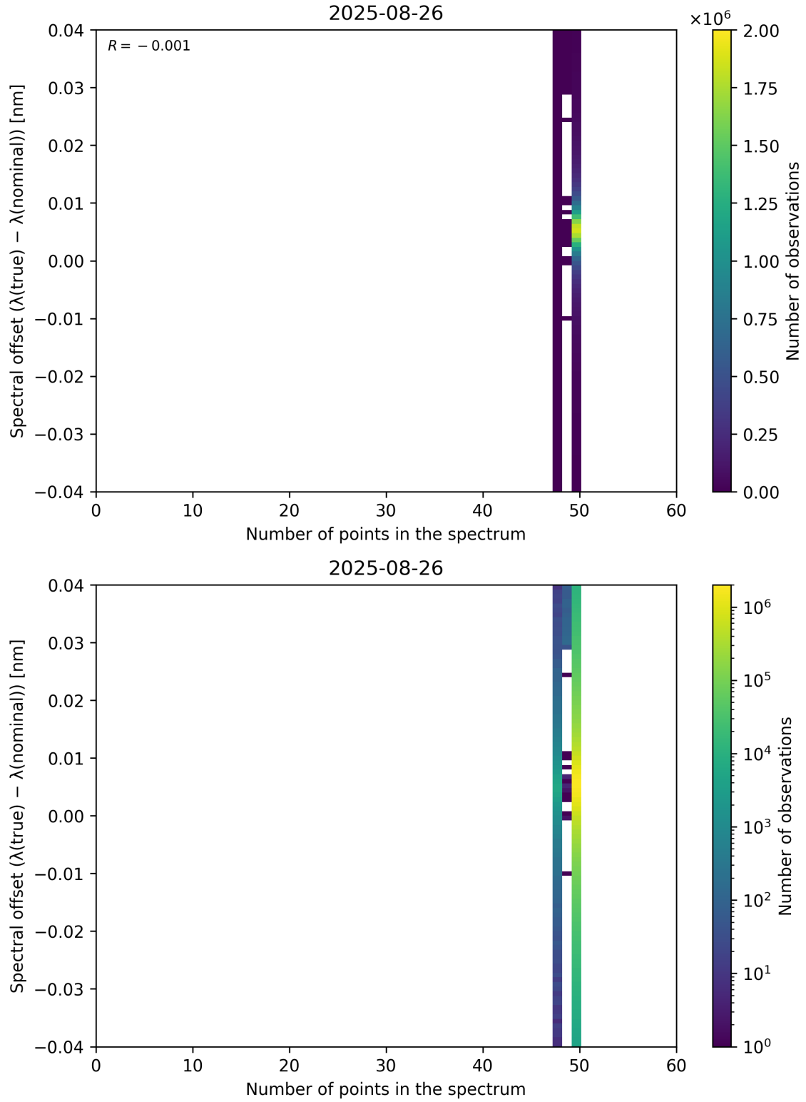
Figure 101: Scatter density plot of “Number of points in the spectrum” against “Spectral offset ( \lambda_{\text{true}} - \lambda_{\text{nominal}} )” for 2025-08-25 to 2025-08-27.
