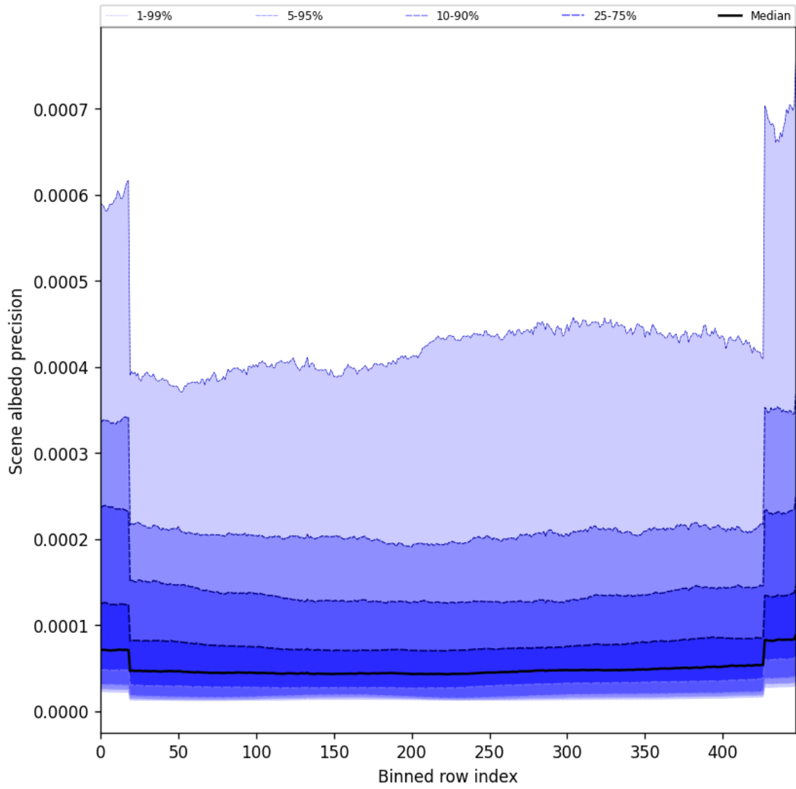
Figure 52: Along track statistics of “Scene albedo precision” for 2025-08-25 to 2025-08-27
