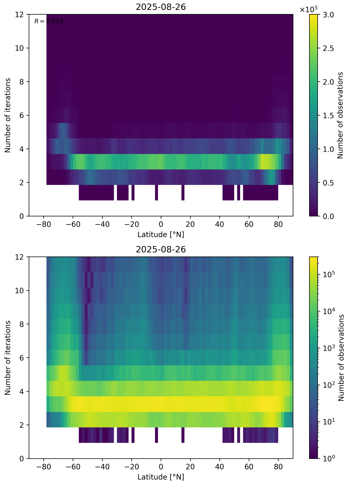
Figure 93: Scatter density plot of “Latitude” against “Number of iterations” for 2025-08-25 to 2025-08-27.
