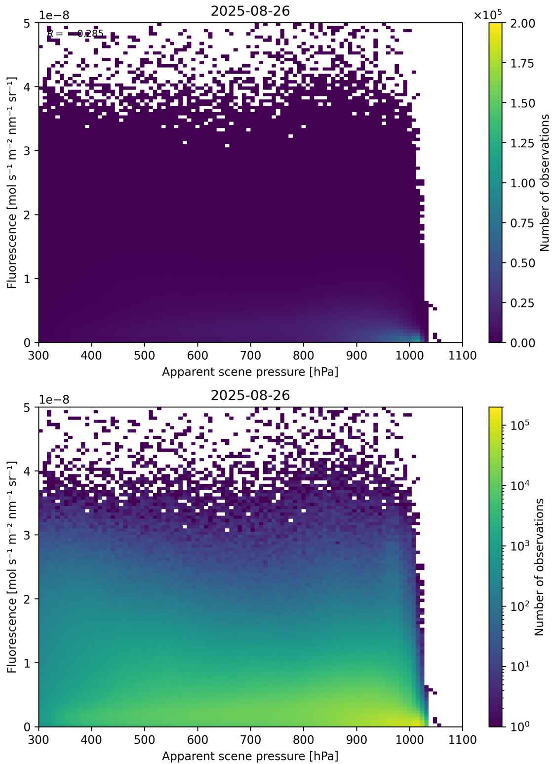
Figure 64: Scatter density plot of “Apparent scene pressure” against “Fluorescence” for 2025-08-25 to 2025-08-27.
