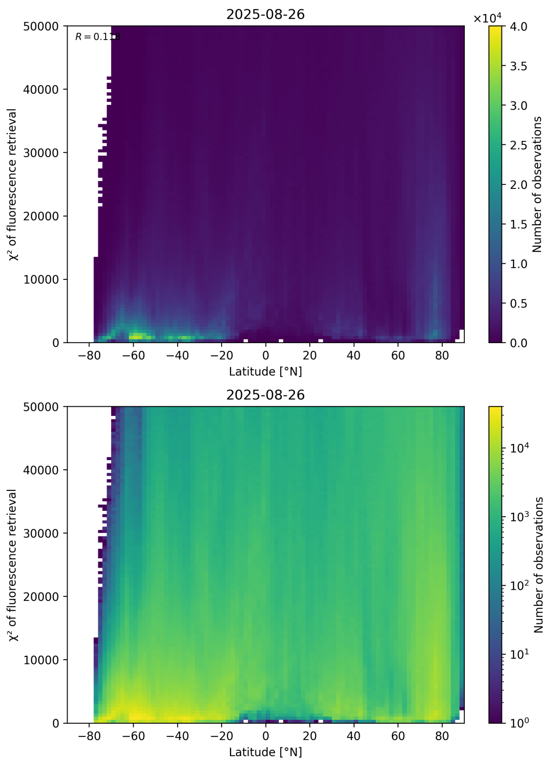
Figure 89: Scatter density plot of “Latitude” against “ \chi^2 of fluorescence retrieval” for 2025-08-25 to 2025-08-27.
