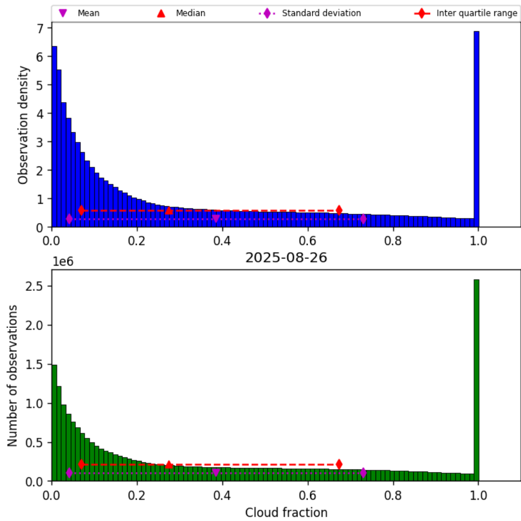
Figure 32: Histogram of “Cloud fraction” for 2025-08-25 to 2025-08-27
