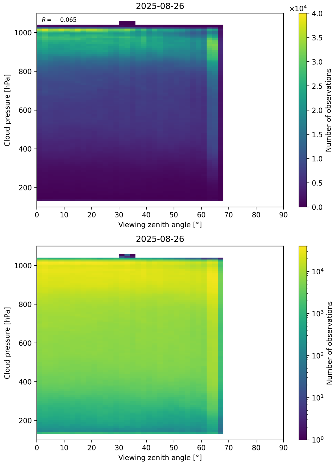
Figure 121: Scatter density plot of “Viewing zenith angle” against “Cloud pressure” for 2025-08-25 to 2025-08-27.
