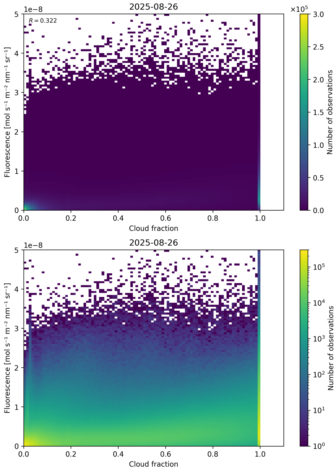
Figure 72: Scatter density plot of “Cloud fraction” against “Fluorescence” for 2025-08-25 to 2025-08-27.
