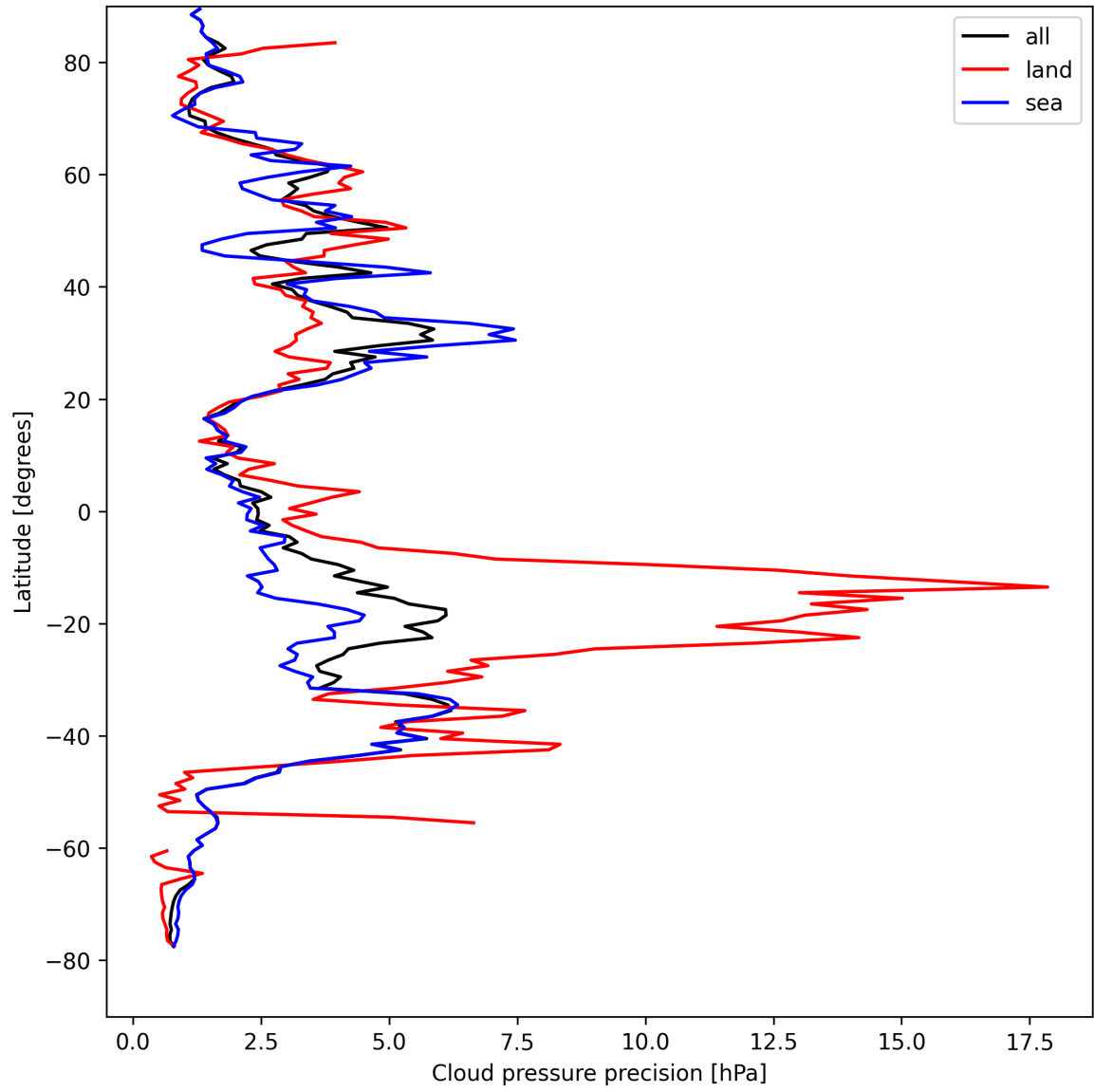
Figure 14: Zonal average of “Cloud pressure precision” for 2025-08-25 to 2025-08-27.
