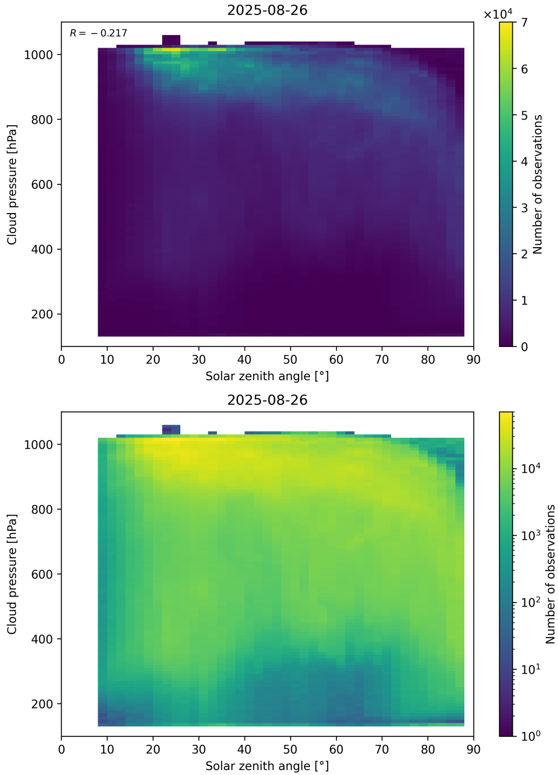
Figure 111: Scatter density plot of “Solar zenith angle” against “Cloud pressure” for 2025-08-25 to 2025-08-27.
