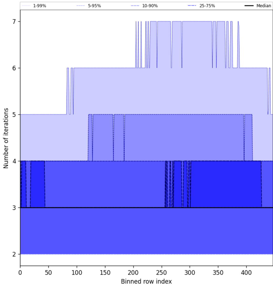
Figure 56: Along track statistics of “Number of iterations” for 2025-08-25 to 2025-08-27
