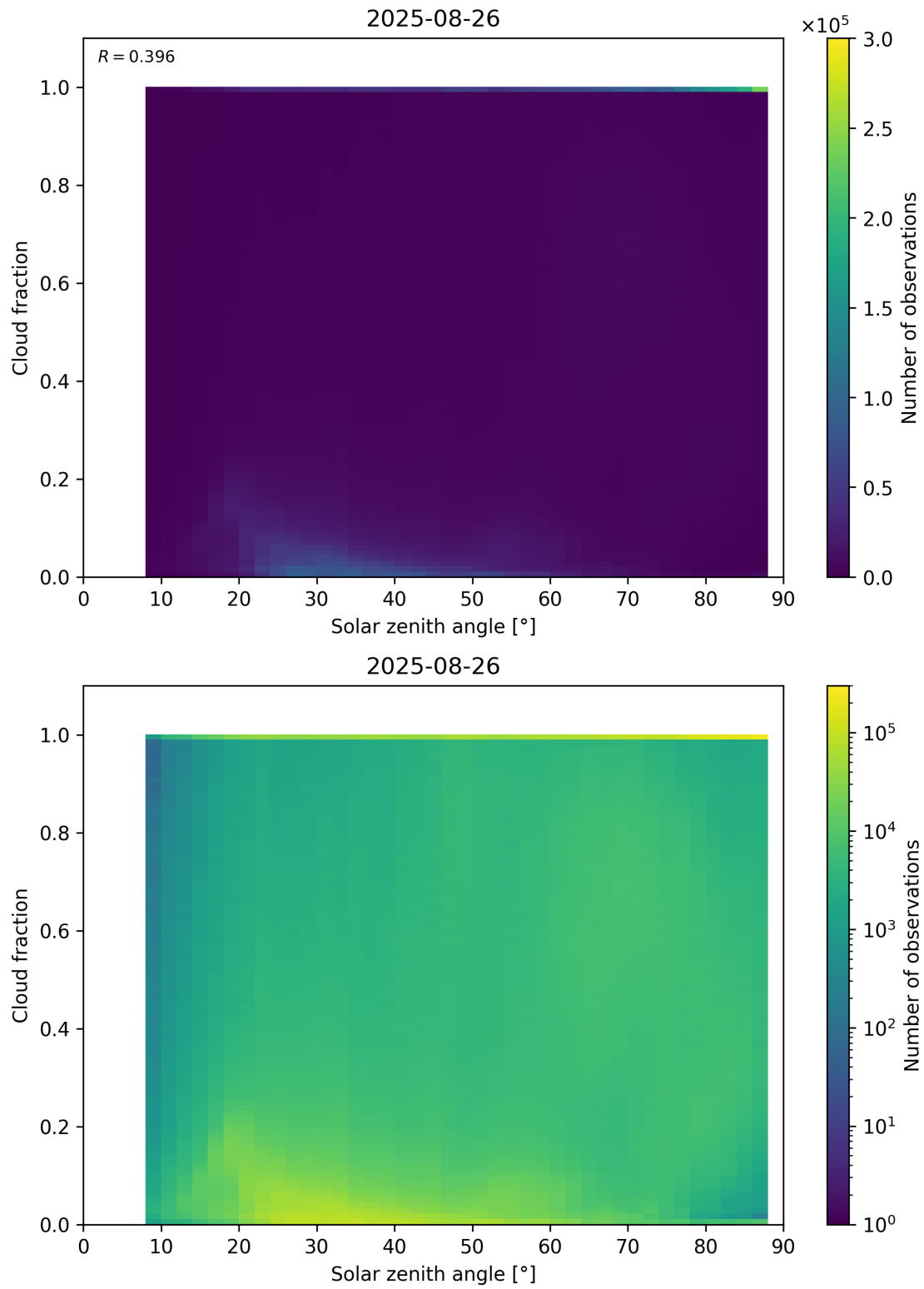
Figure 110: Scatter density plot of “Solar zenith angle” against “Cloud fraction” for 2025-08-25 to 2025-08-27.
