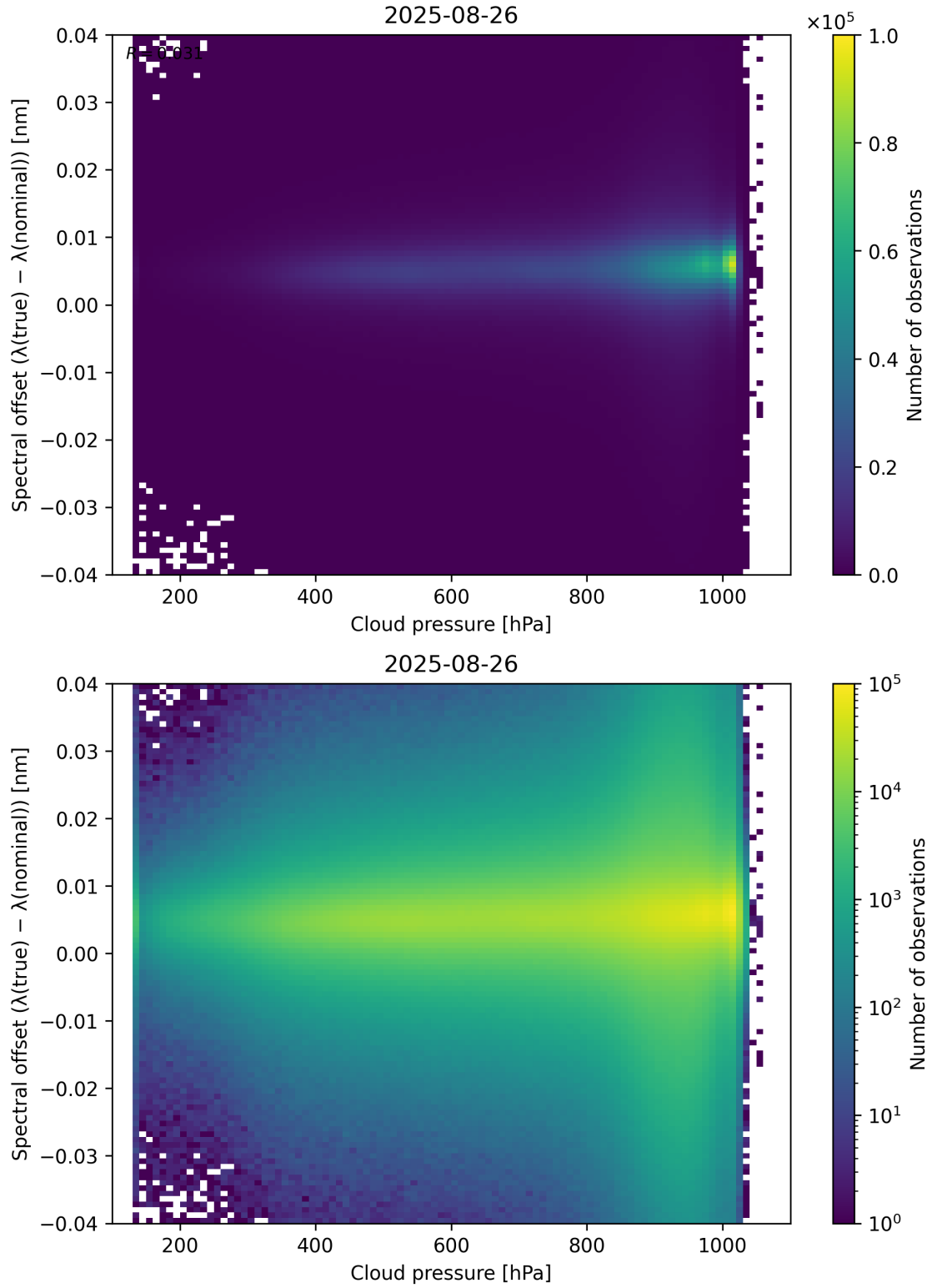
Figure 84: Scatter density plot of “Cloud pressure” against “Spectral offset ( \lambda_{\text{true}} - \lambda_{\text{nominal}} )” for 2025-08-25 to 2025-08-27.
