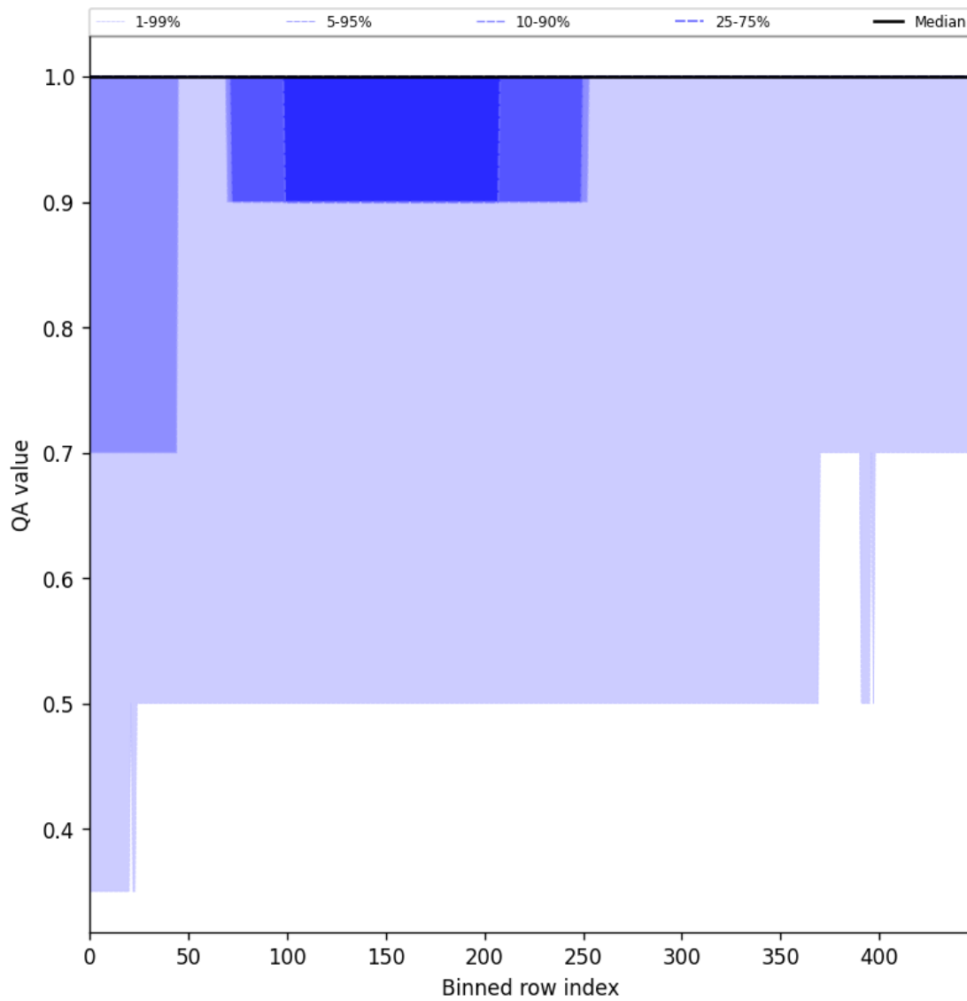
Figure 46: Along track statistics of “QA value” for 2025-08-25 to 2025-08-27
