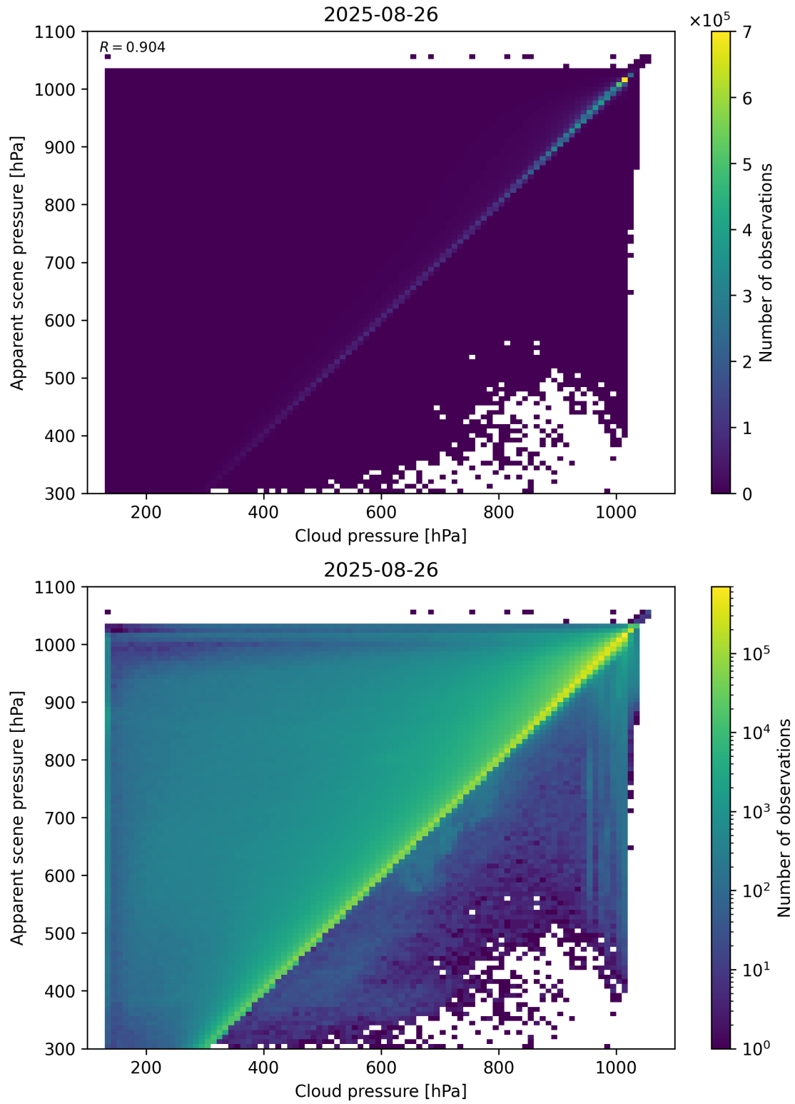
Figure 77: Scatter density plot of “Cloud pressure” against “Apparent scene pressure” for 2025-08-25 to 2025-08-27.
