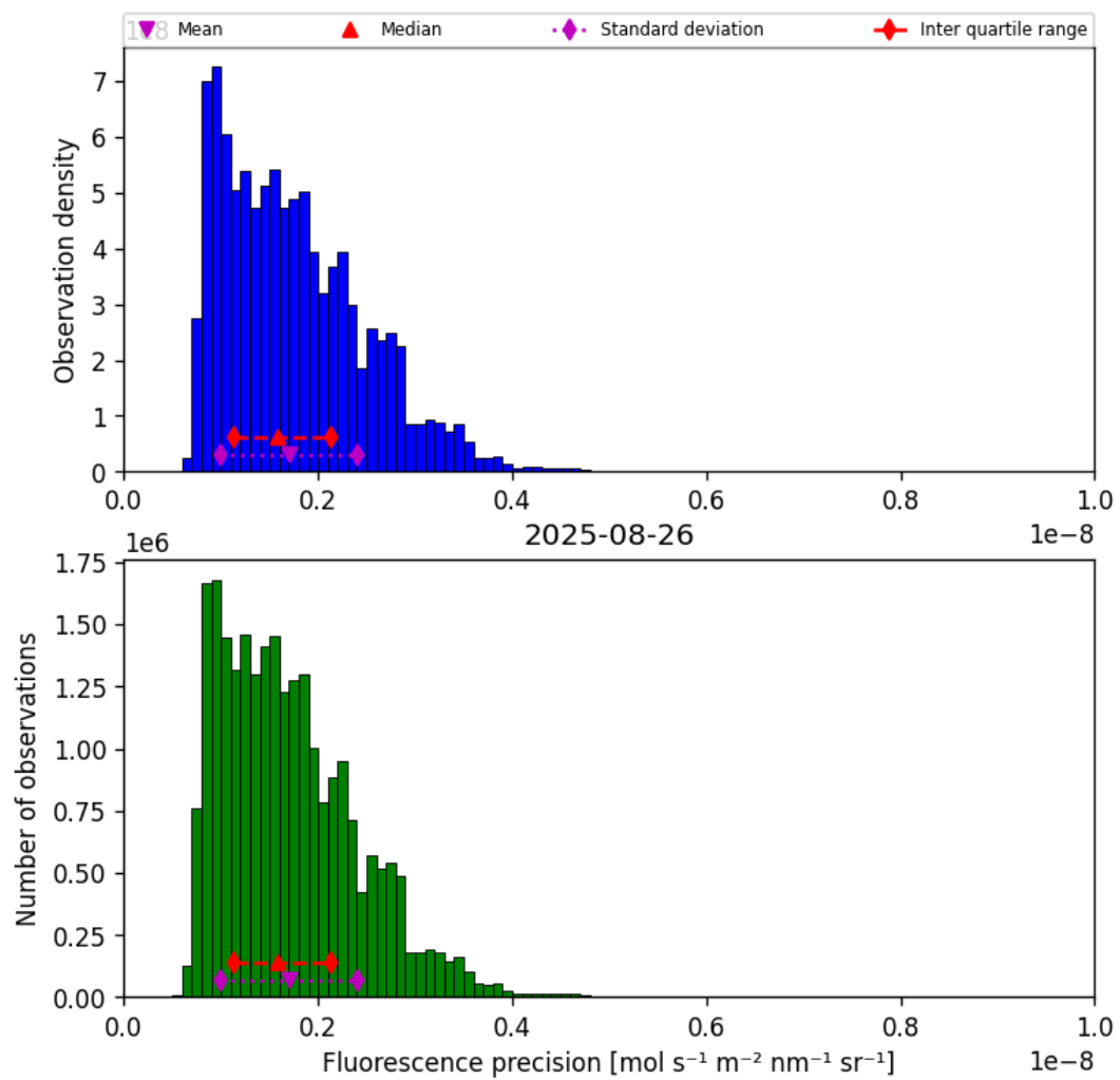
Figure 41: Histogram of “Fluorescence precision” for 2025-08-25 to 2025-08-27
