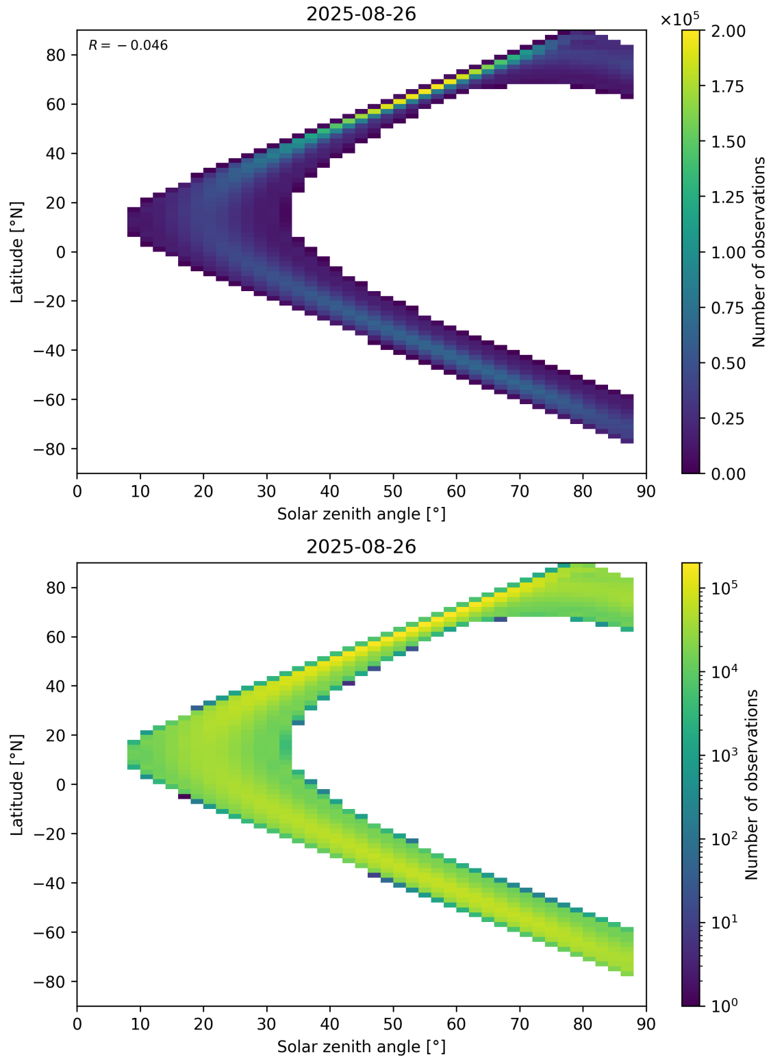
Figure 113: Scatter density plot of “Solar zenith angle” against “Latitude” for 2025-08-25 to 2025-08-27.
