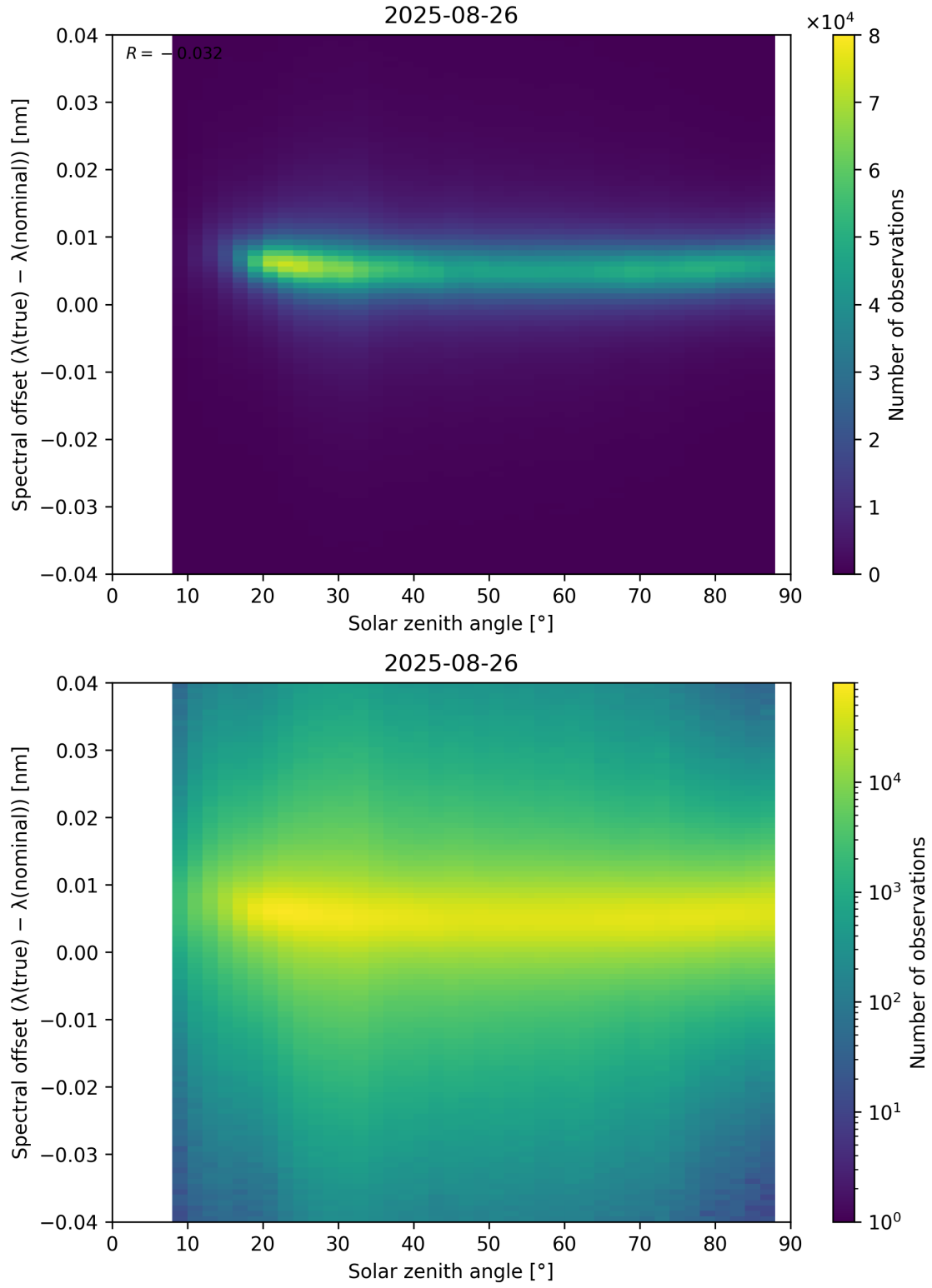
Figure 117: Scatter density plot of “Solar zenith angle” against “Spectral offset ( \lambda_{\text{true}} - \lambda_{\text{nominal}} )” for 2025-08-25 to 2025-08-27.
