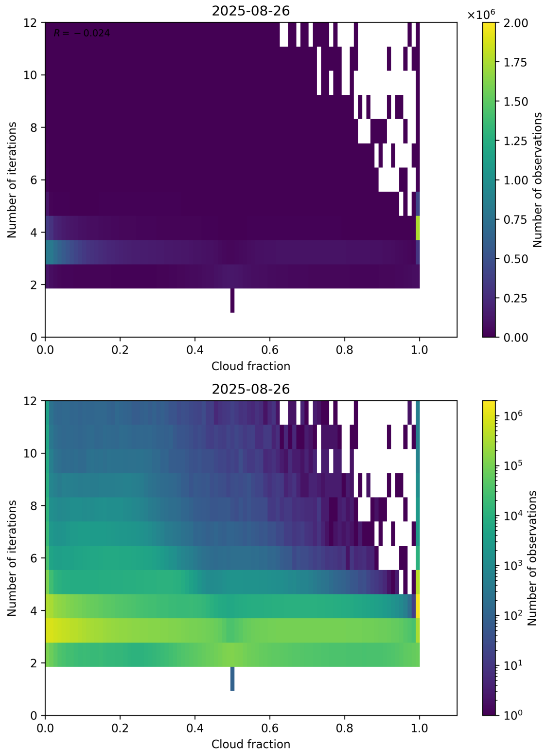
Figure 73: Scatter density plot of “Cloud fraction” against “Number of iterations” for 2025-08-25 to 2025-08-27.
