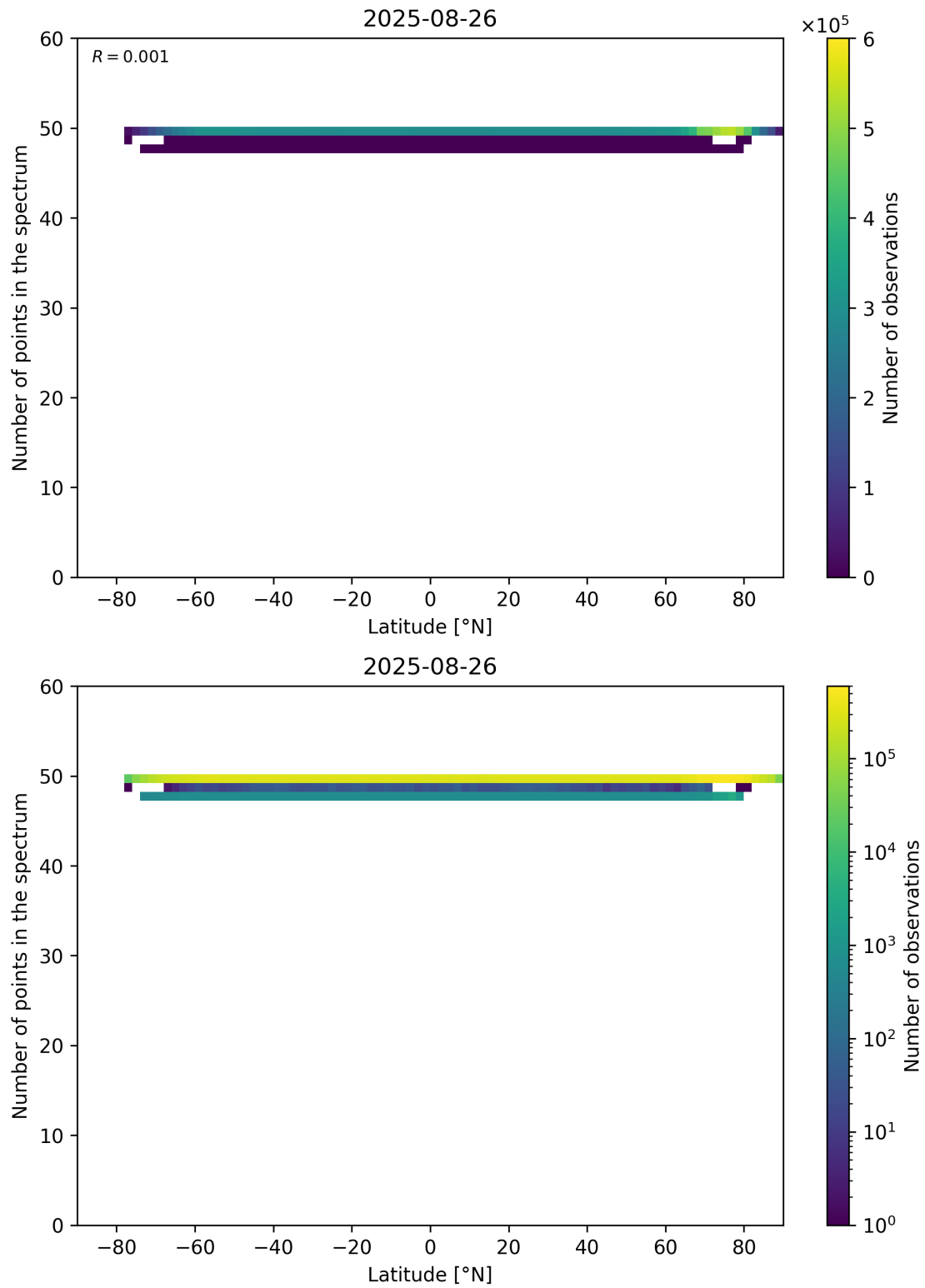
Figure 94: Scatter density plot of “Latitude” against “Number of points in the spectrum” for 2025-08-25 to 2025-08-27.
