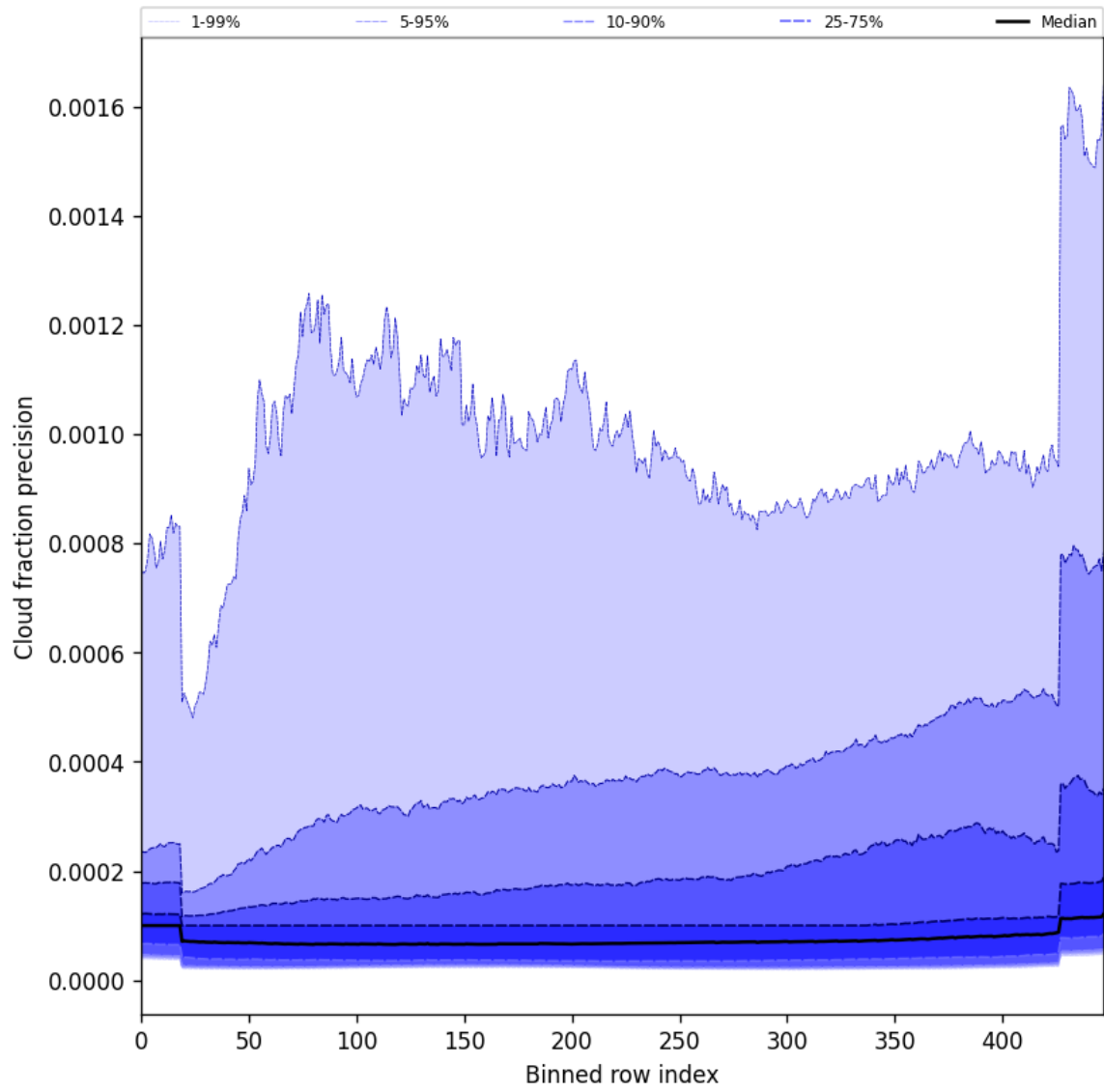
Figure 50: Along track statistics of “Cloud fraction precision” for 2025-08-25 to 2025-08-27
