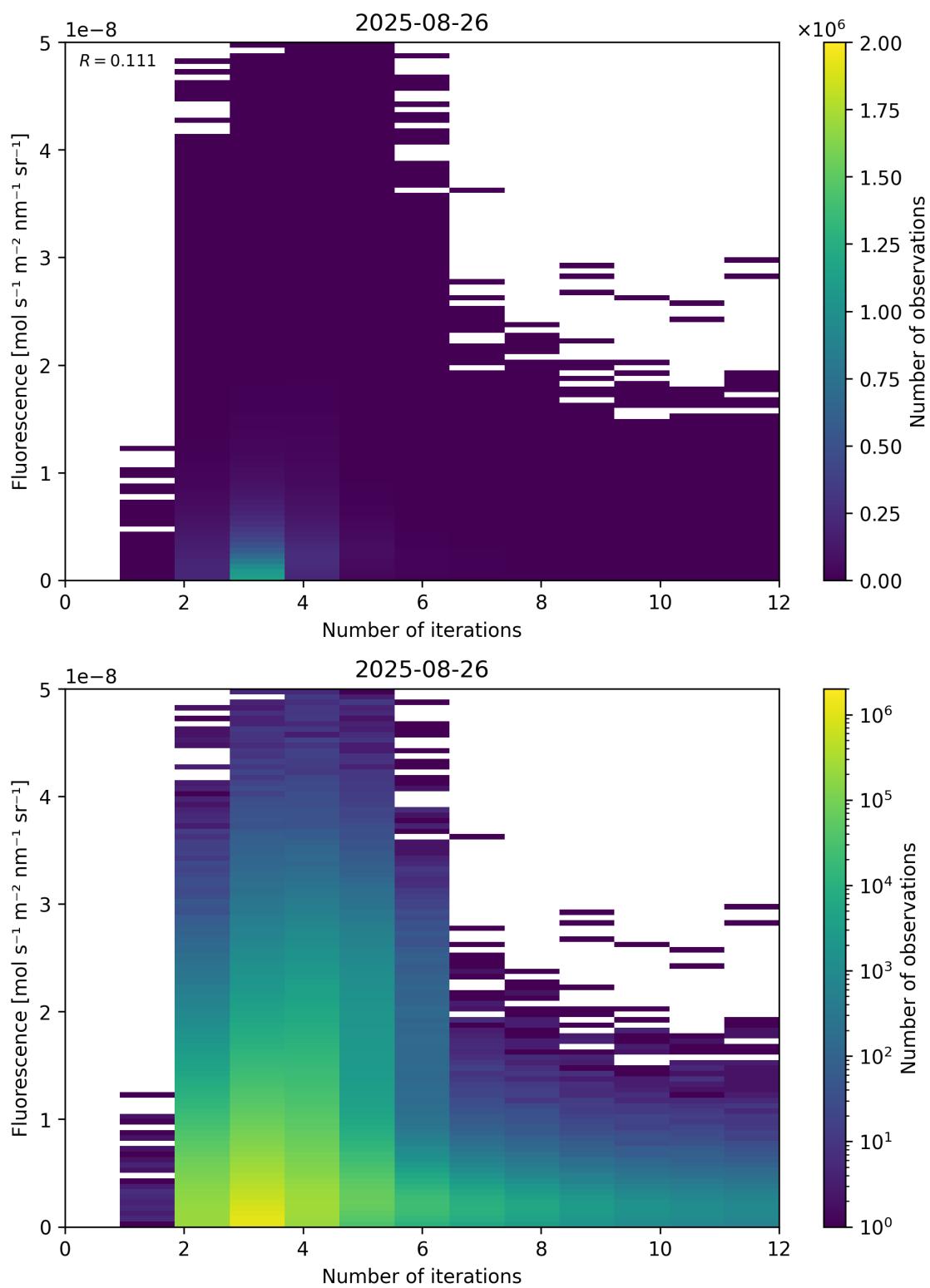
Figure 98: Scatter density plot of “Number of iterations” against “Fluorescence” for 2025-08-25 to 2025-08-27.
