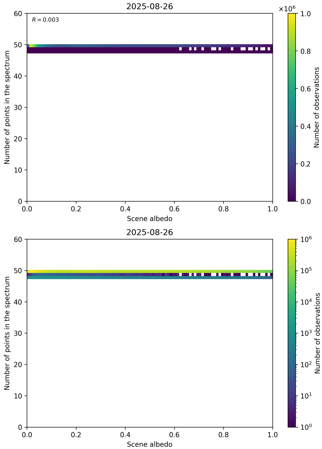
Figure 106: Scatter density plot of “Scene albedo” against “Number of points in the spectrum” for 2025-08-25 to 2025-08-27.
