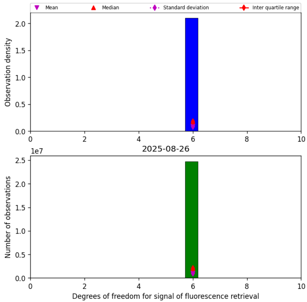
Figure 43: Histogram of "Degrees of freedom for signal of fluorescence retrieval" for 2025-08-25 to 2025-08-27
