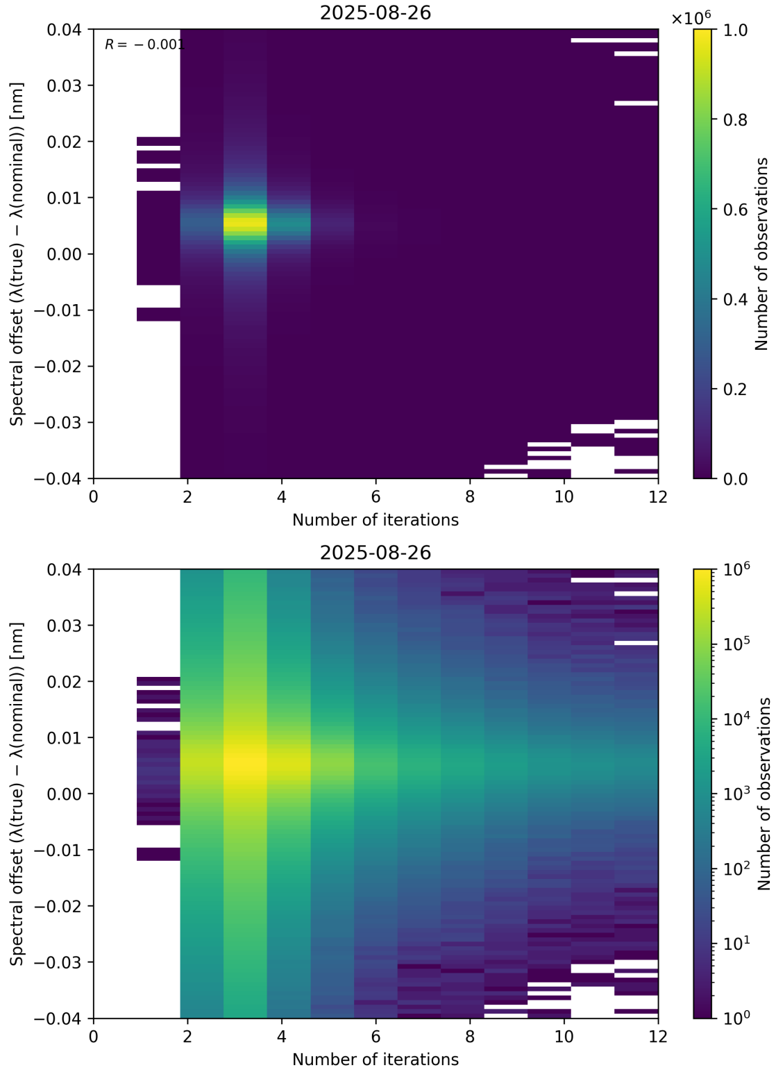
Figure 100: Scatter density plot of “Number of iterations” against “Spectral offset ( \lambda_{\text{true}} - \lambda_{\text{nominal}} )” for 2025-08-25 to 2025-08-27.
