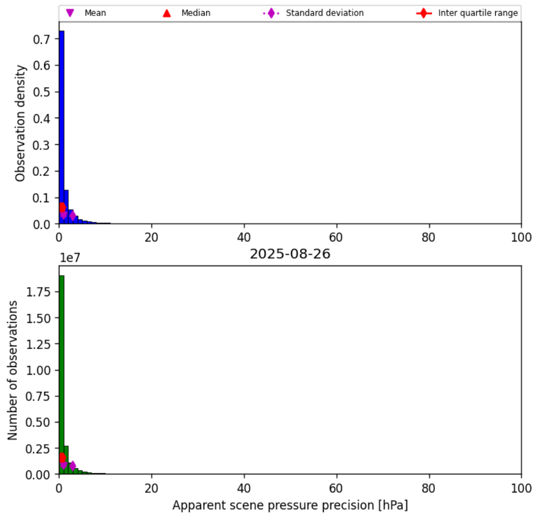
Figure 37: Histogram of “Apparent scene pressure precision” for 2025-08-25 to 2025-08-27
