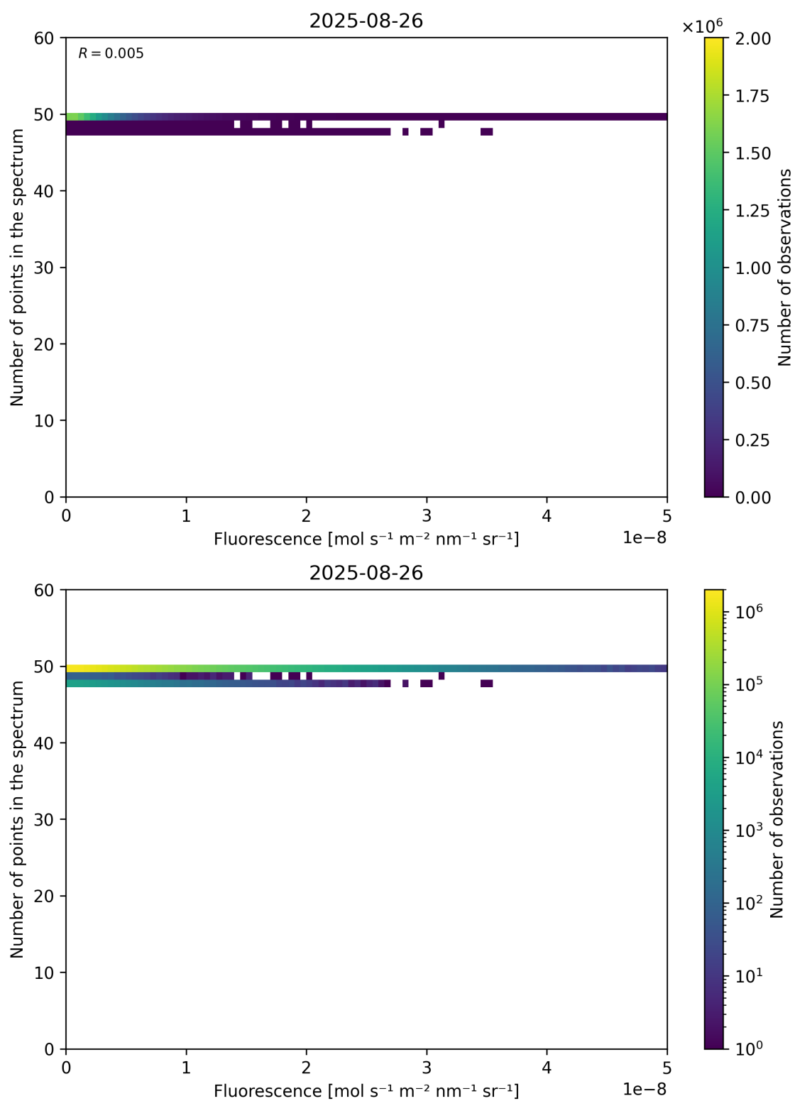
Figure 86: Scatter density plot of “Fluorescence” against “Number of points in the spectrum” for 2025-08-25 to 2025-08-27.
