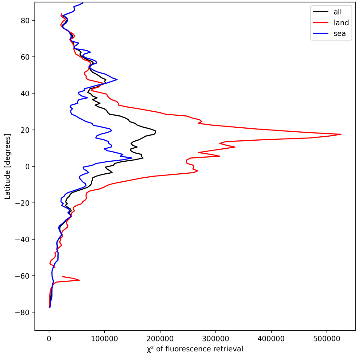
Figure 25: Zonal average of “ \chi^2 of fluorescence retrieval” for 2025-08-25 to 2025-08-27.
