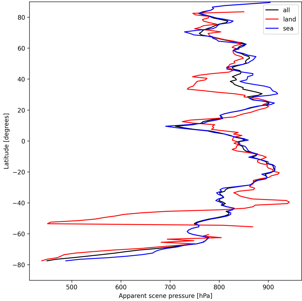
Figure 19: Zonal average of “Apparent scene pressure” for 2025-08-25 to 2025-08-27.
