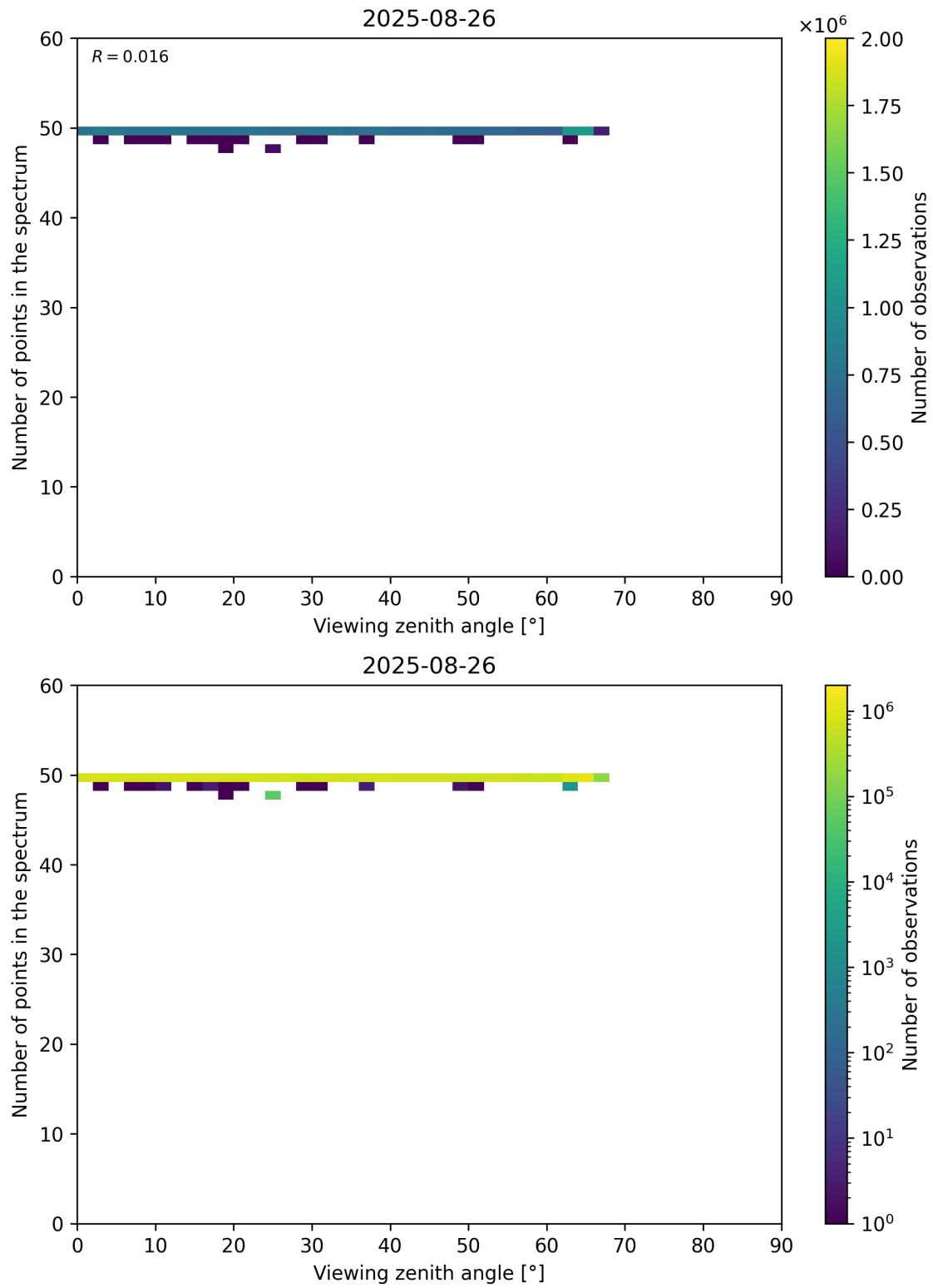
Figure 125: Scatter density plot of “Viewing zenith angle” against “Number of points in the spectrum” for 2025-08-25 to 2025-08-27.
