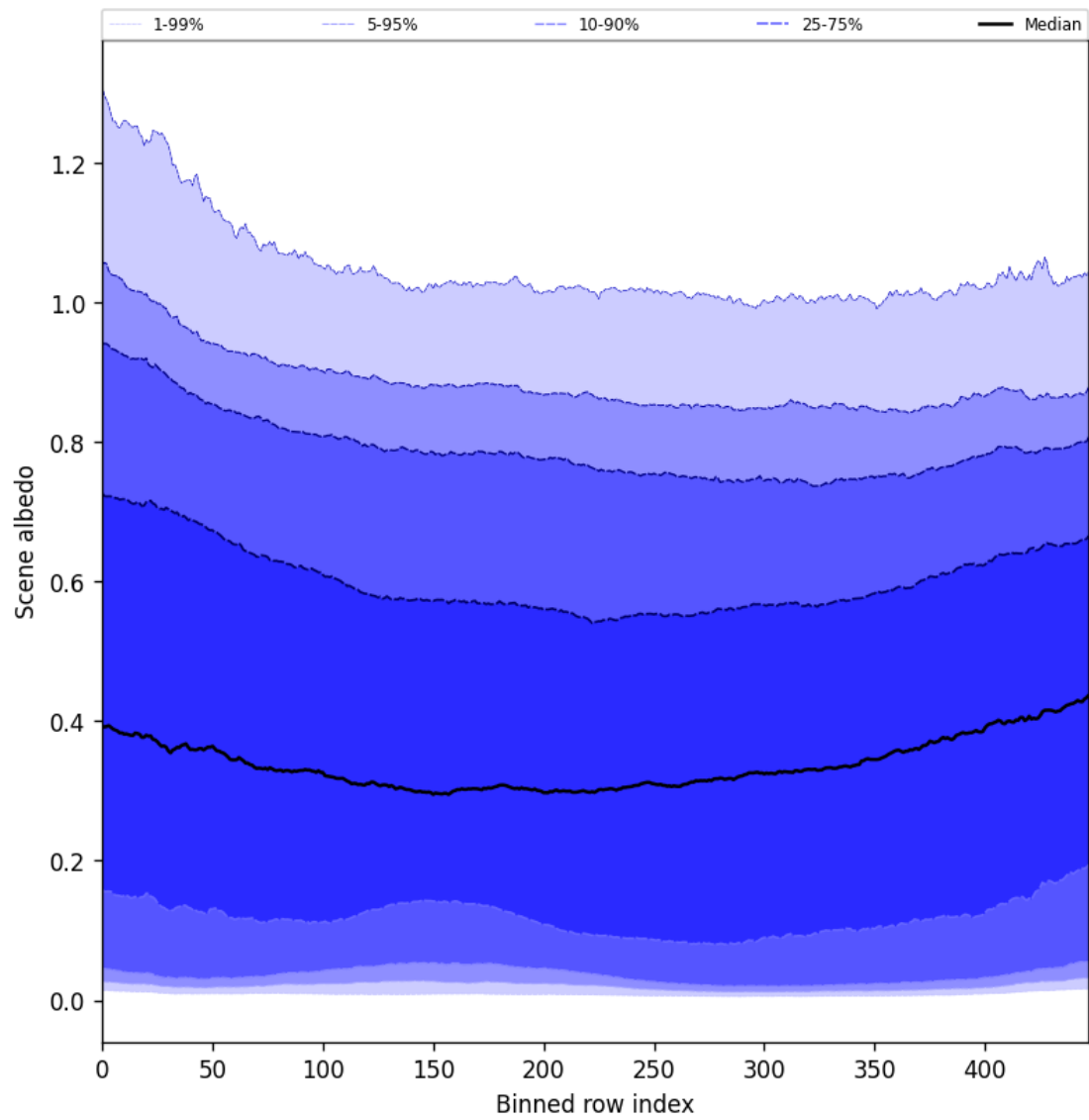
Figure 51: Along track statistics of “Scene albedo” for 2025-08-25 to 2025-08-27
