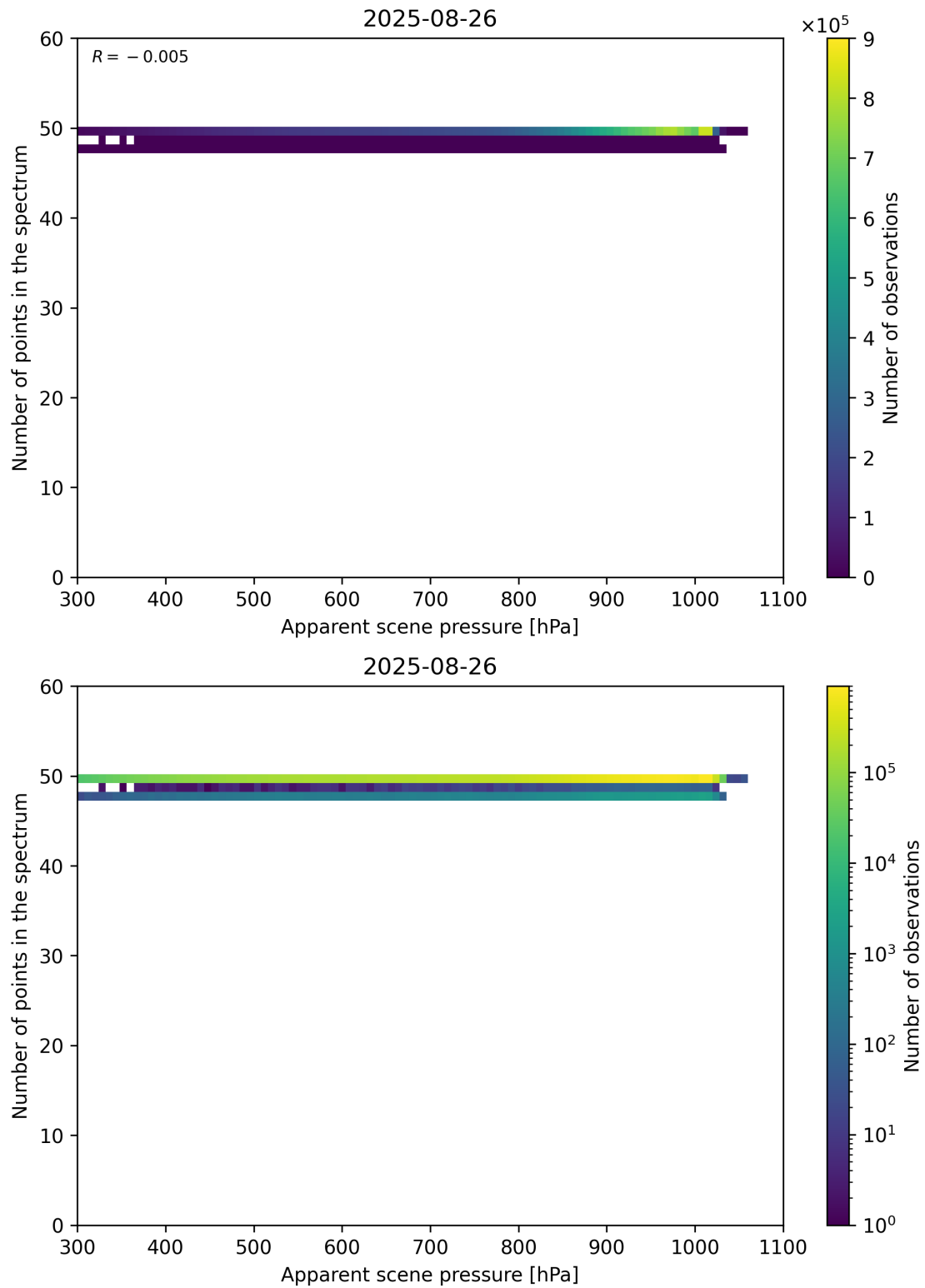
Figure 66: Scatter density plot of “Apparent scene pressure” against “Number of points in the spectrum” for 2025-08-25 to 2025-08-27.
