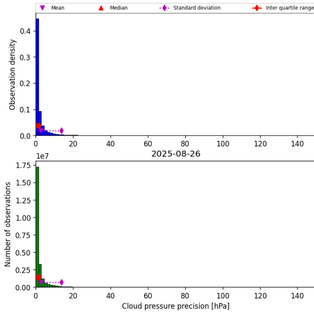
Figure 31: Histogram of “Cloud pressure precision” for 2025-08-25 to 2025-08-27
