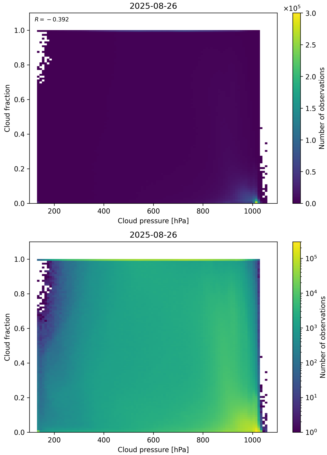
Figure 79: Scatter density plot of “Cloud pressure” against “Cloud fraction” for 2025-08-25 to 2025-08-27.
