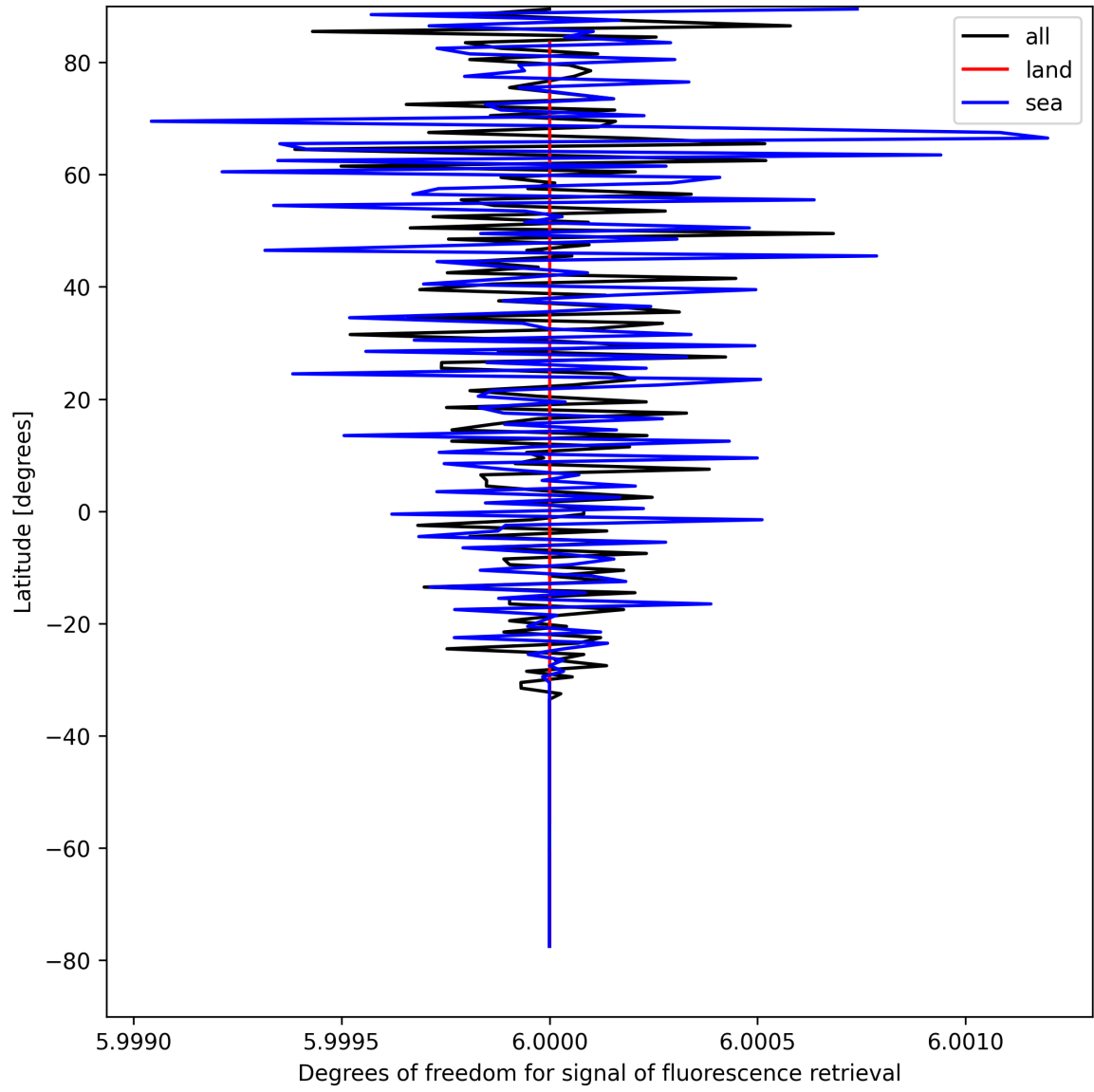
Figure 26: Zonal average of “Degrees of freedom for signal of fluorescence retrieval” for 2025-08-25 to 2025-08-27.
