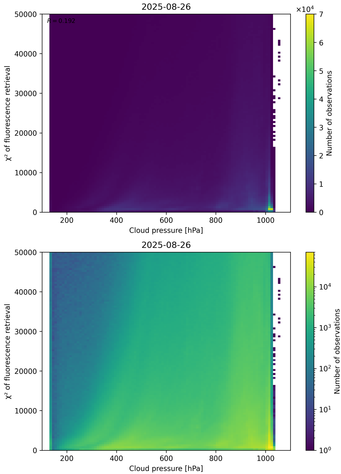
Figure 78: Scatter density plot of “Cloud pressure” against “ \chi^2 of fluorescence retrieval” for 2025-08-25 to 2025-08-27.
