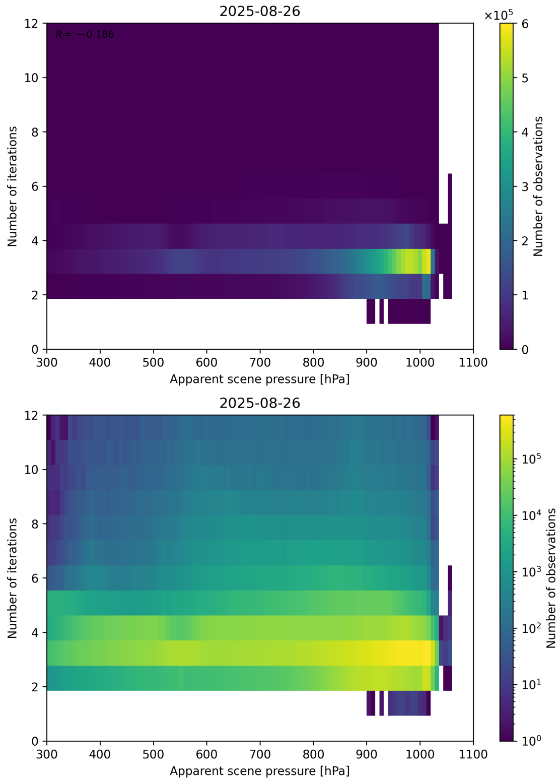
Figure 65: Scatter density plot of “Apparent scene pressure” against “Number of iterations” for 2025-08-25 to 2025-08-27.
