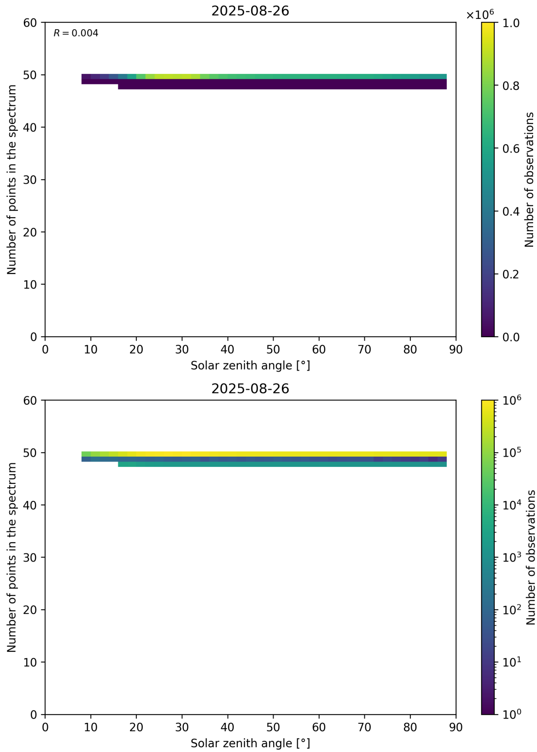
Figure 115: Scatter density plot of “Solar zenith angle” against “Number of points in the spectrum” for 2025-08-25 to 2025-08-27.
