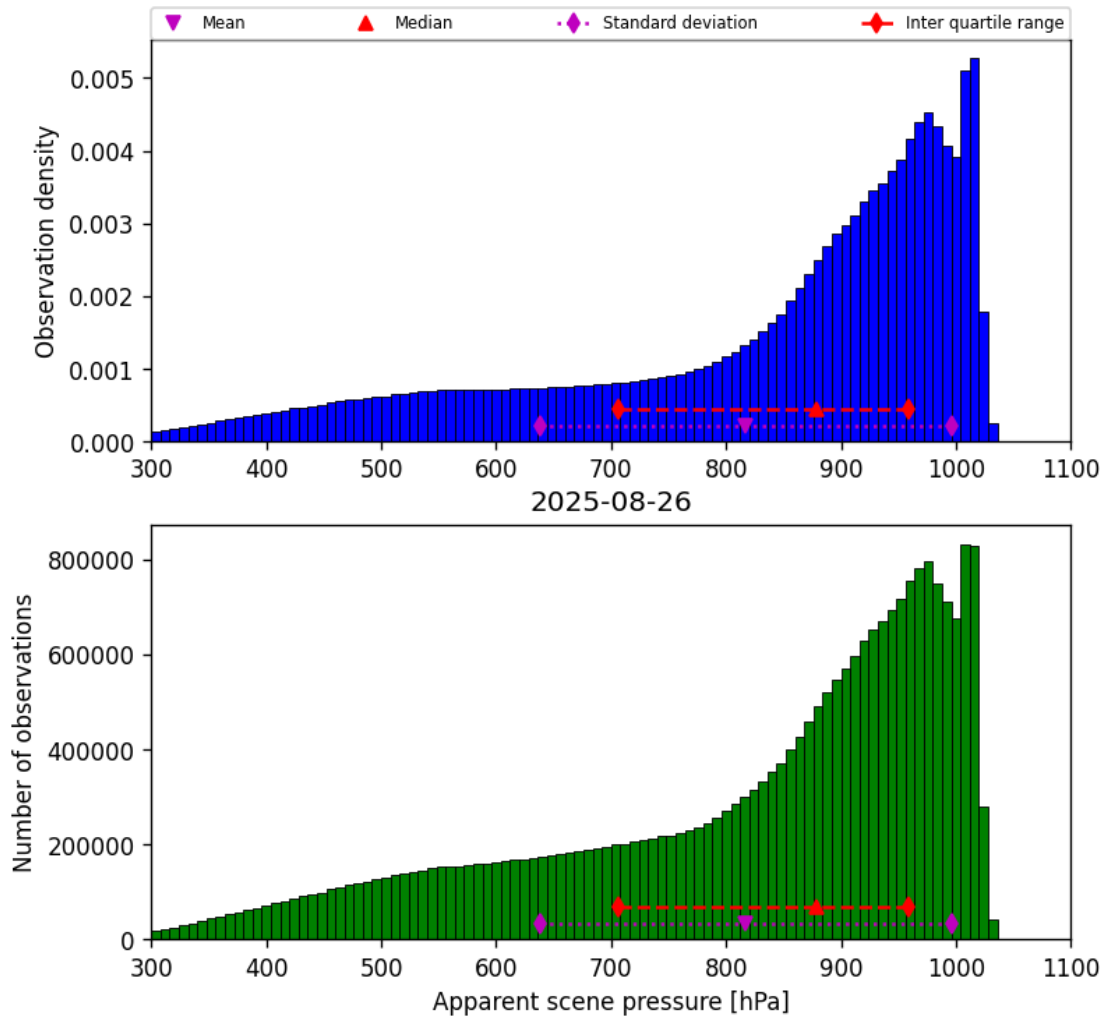
Figure 36: Histogram of “Apparent scene pressure” for 2025-08-25 to 2025-08-27
