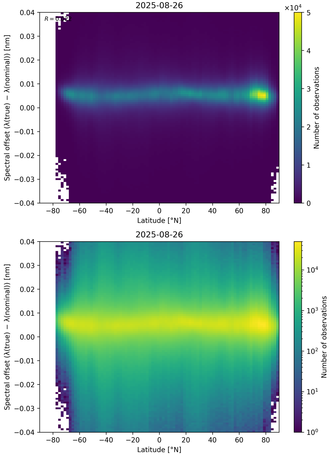
Figure 96: Scatter density plot of “Latitude” against “Spectral offset ( \lambda_{\text{true}} - \lambda_{\text{nominal}} )” for 2025-08-25 to 2025-08-27.
