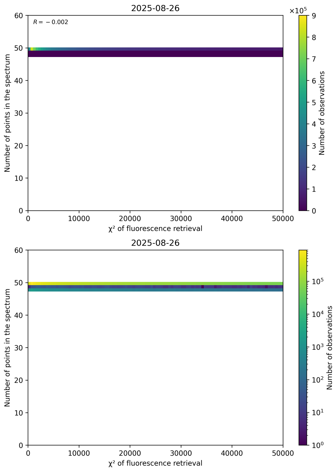
Figure 68: Scatter density plot of " \chi^2 of fluorescence retrieval" against "Number of points in the spectrum" for 2025-08-25 to 2025-08-27.
