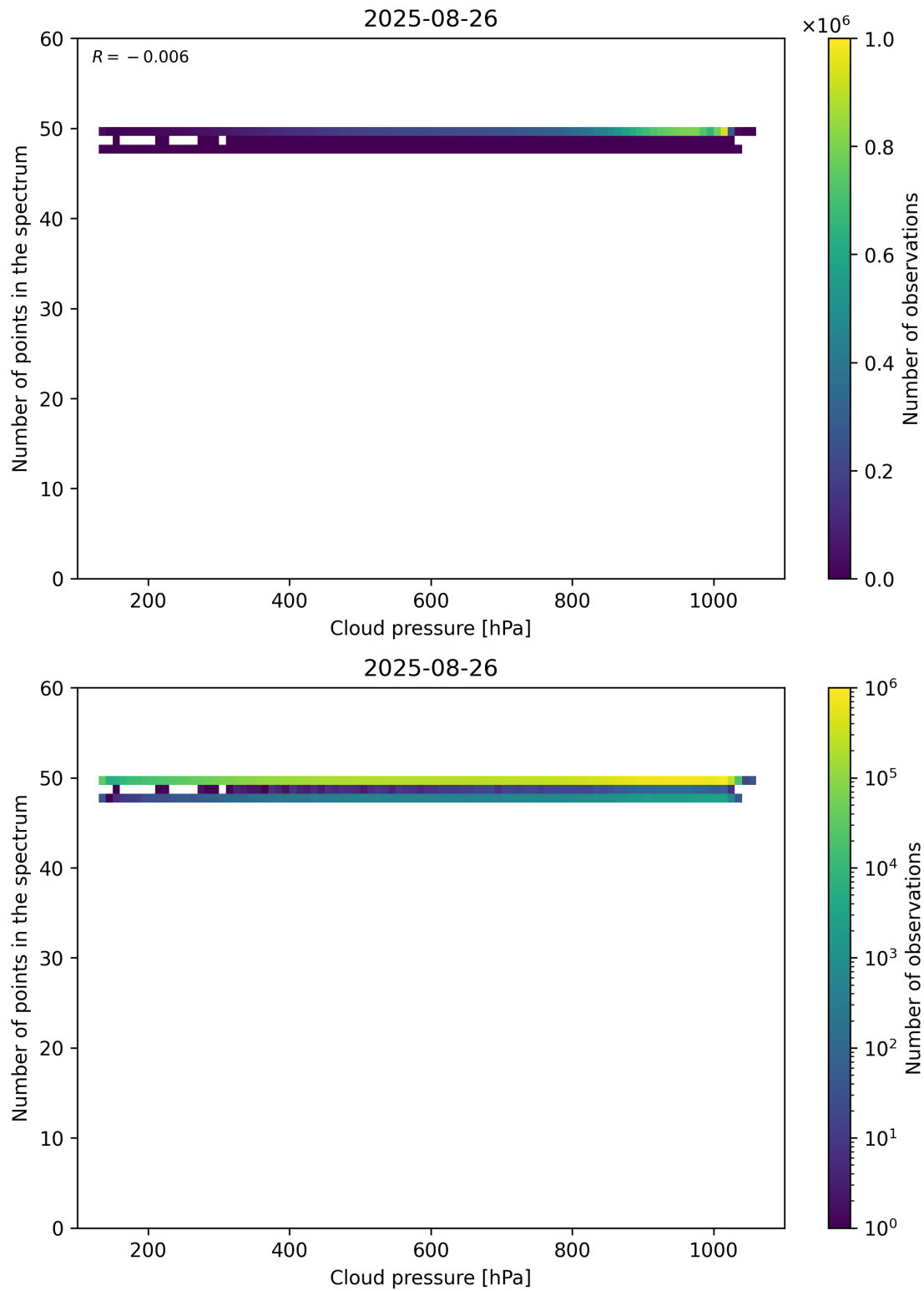
Figure 82: Scatter density plot of “Cloud pressure” against “Number of points in the spectrum” for 2025-08-25 to 2025-08-27.
