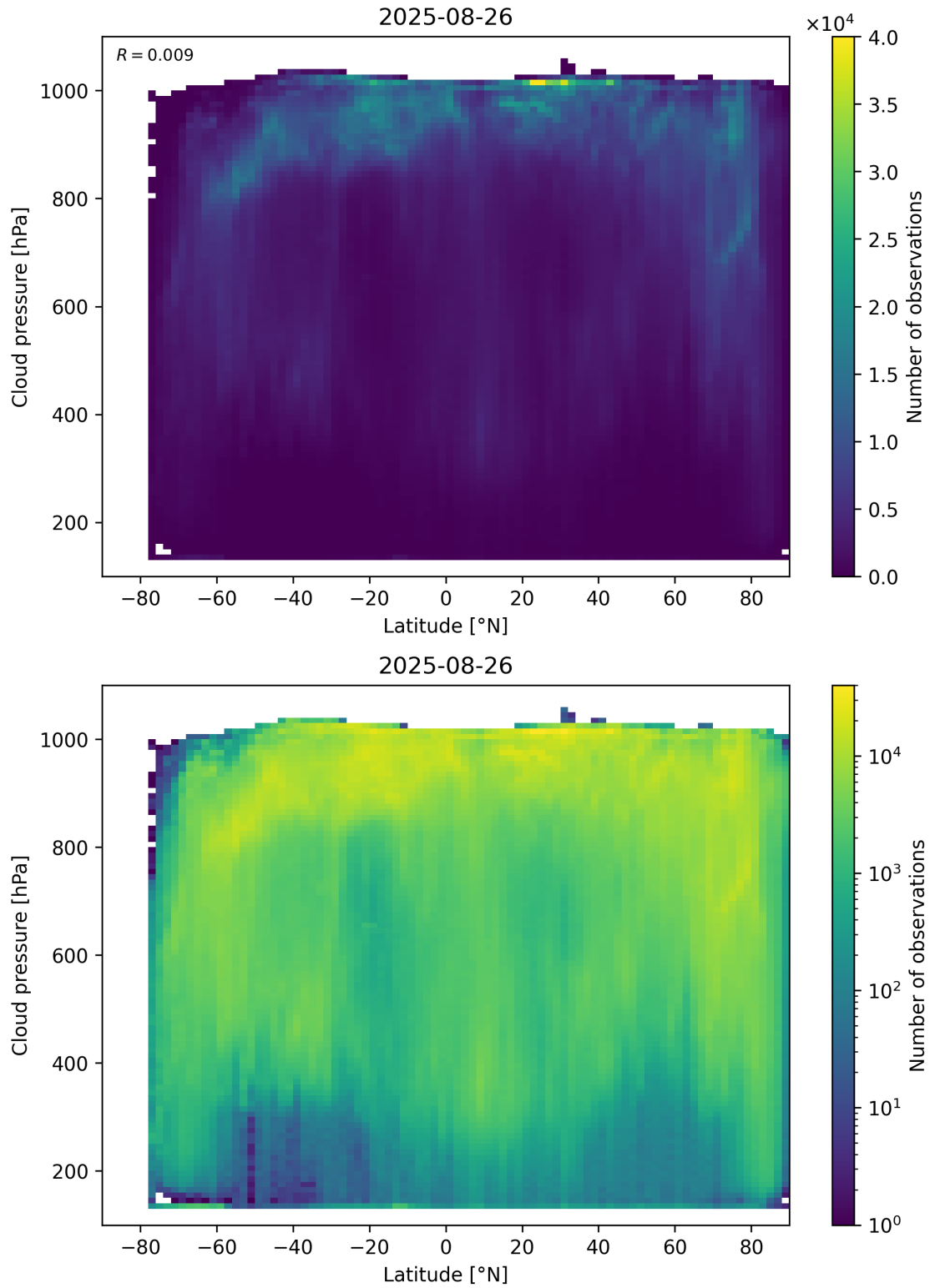
Figure 91: Scatter density plot of “Latitude” against “Cloud pressure” for 2025-08-25 to 2025-08-27.
