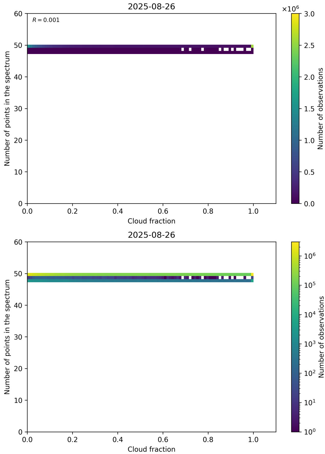
Figure 74: Scatter density plot of “Cloud fraction” against “Number of points in the spectrum” for 2025-08-25 to 2025-08-27.
