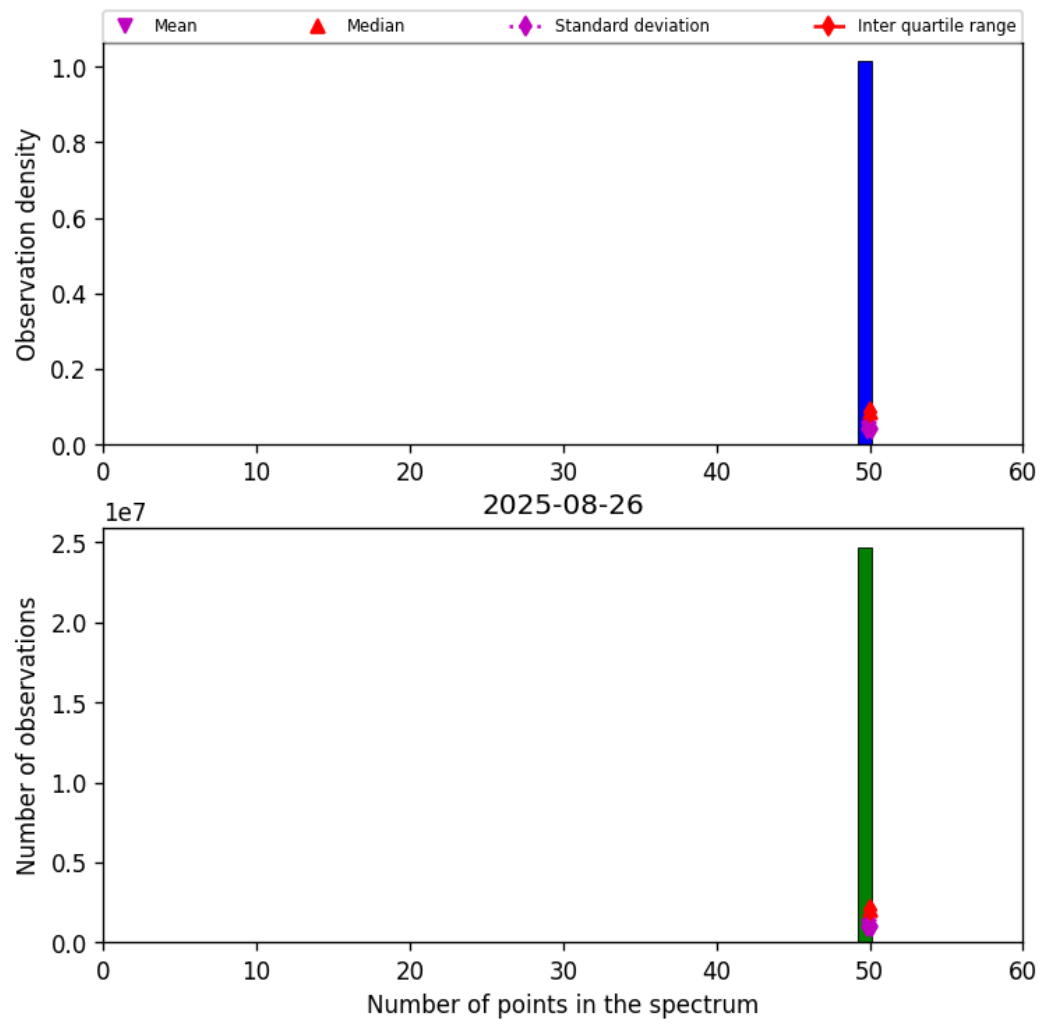
Figure 44: Histogram of “Number of points in the spectrum” for 2025-08-25 to 2025-08-27
