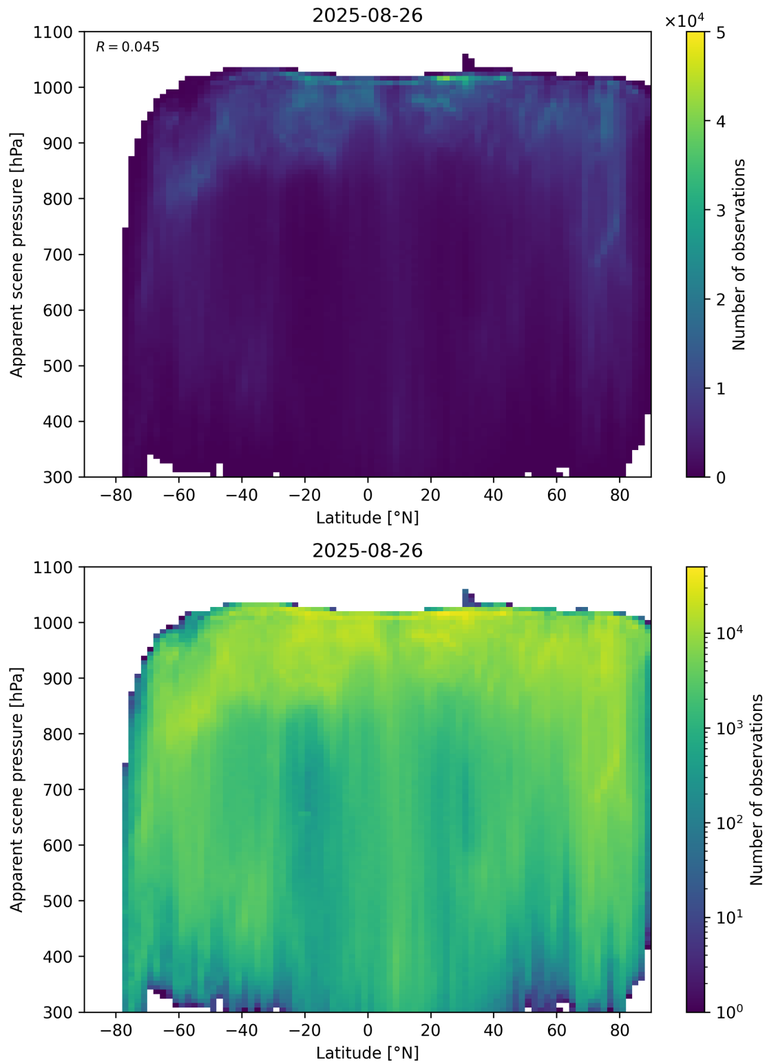
Figure 88: Scatter density plot of “Latitude” against “Apparent scene pressure” for 2025-08-25 to 2025-08-27.
