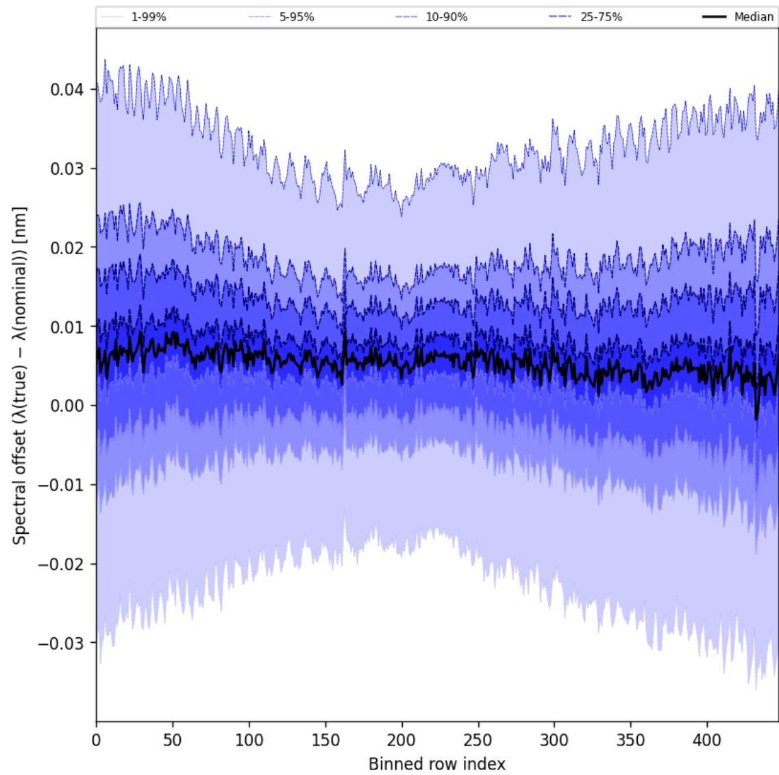
Figure 62: Along track statistics of “Spectral offset ( \lambda_{\text{true}} - \lambda_{\text{nominal}} )” for 2025-08-25 to 2025-08-27
