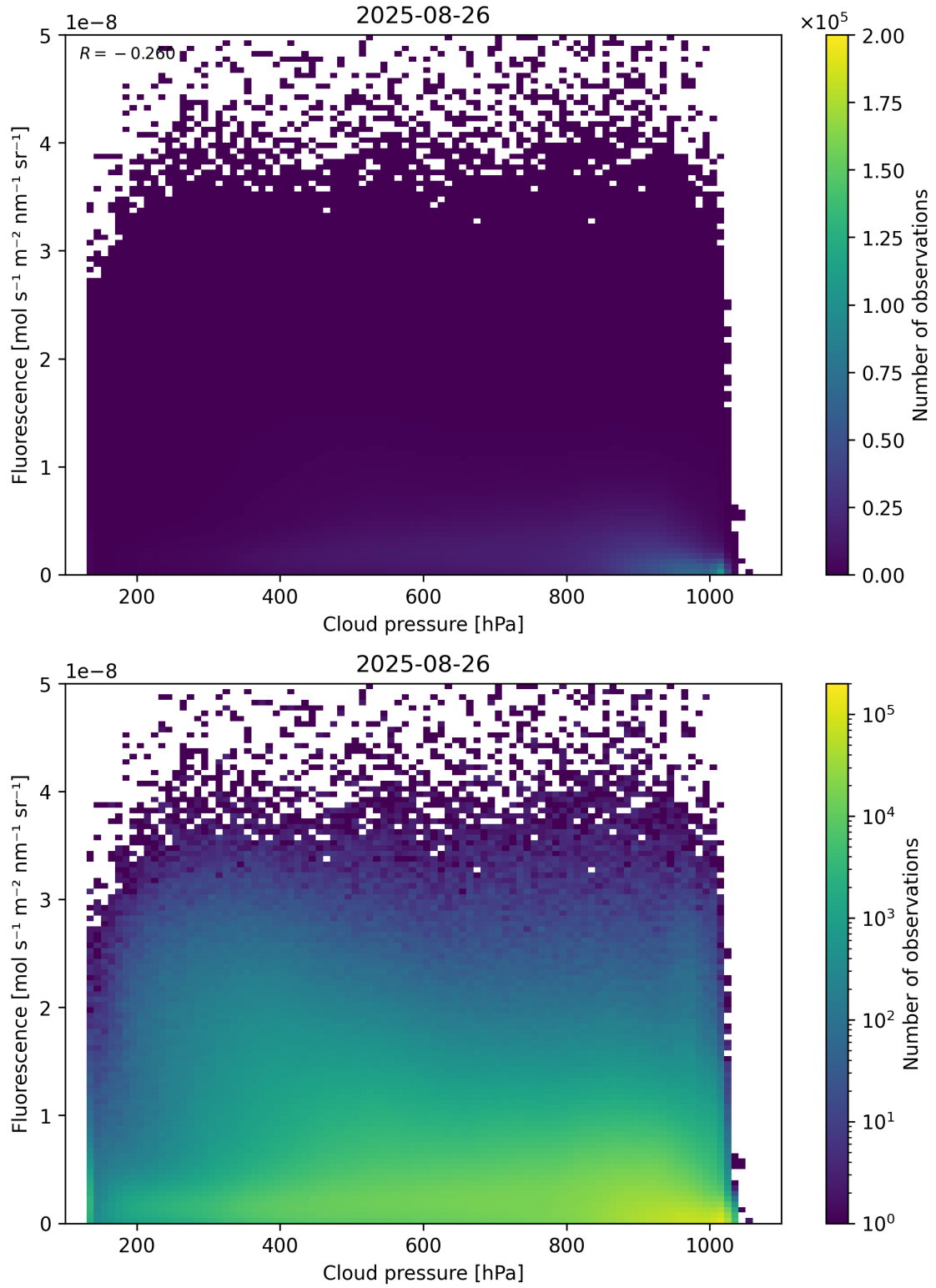
Figure 80: Scatter density plot of “Cloud pressure” against “Fluorescence” for 2025-08-25 to 2025-08-27.
