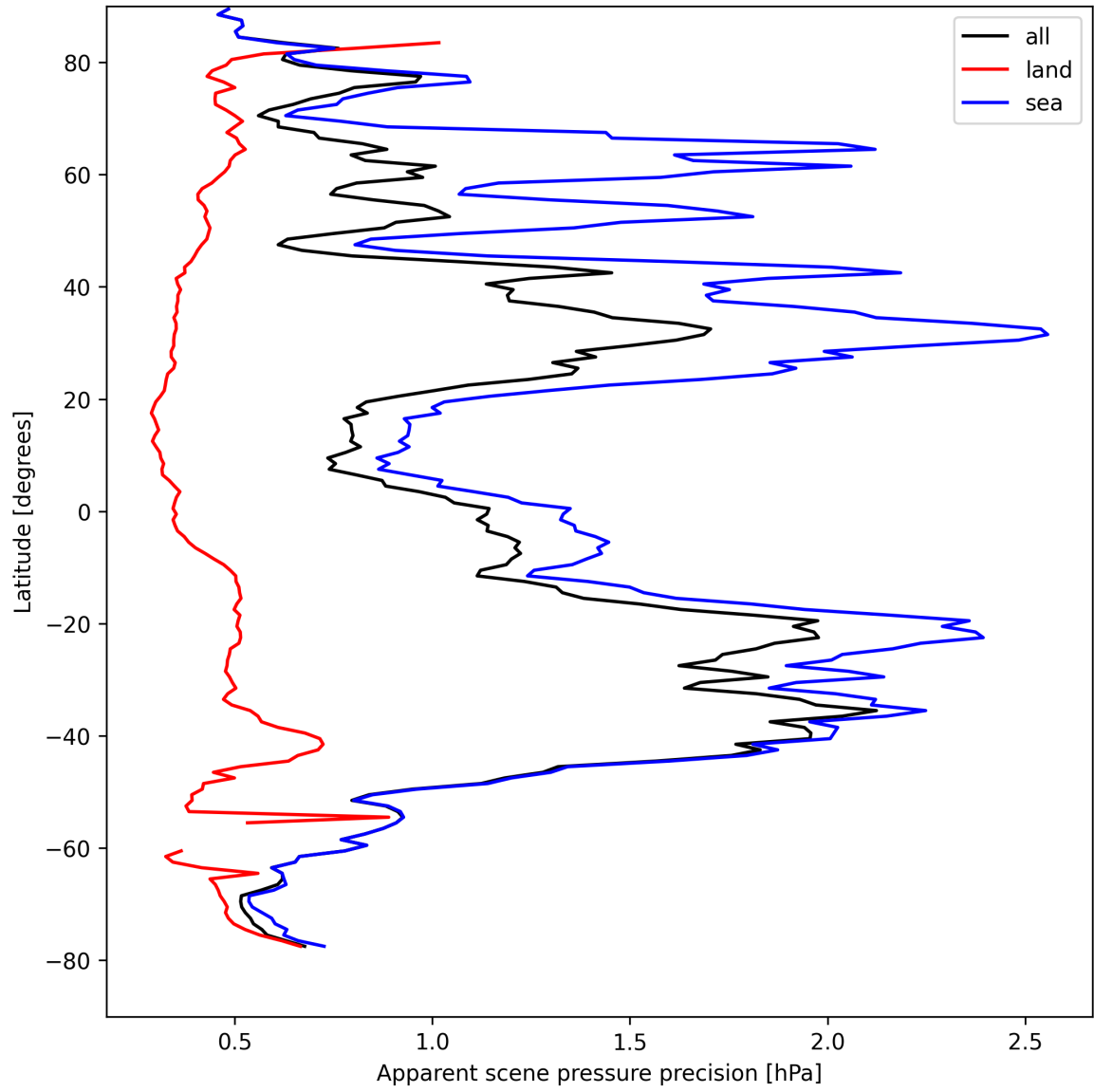
Figure 20: Zonal average of “Apparent scene pressure precision” for 2025-08-25 to 2025-08-27.
