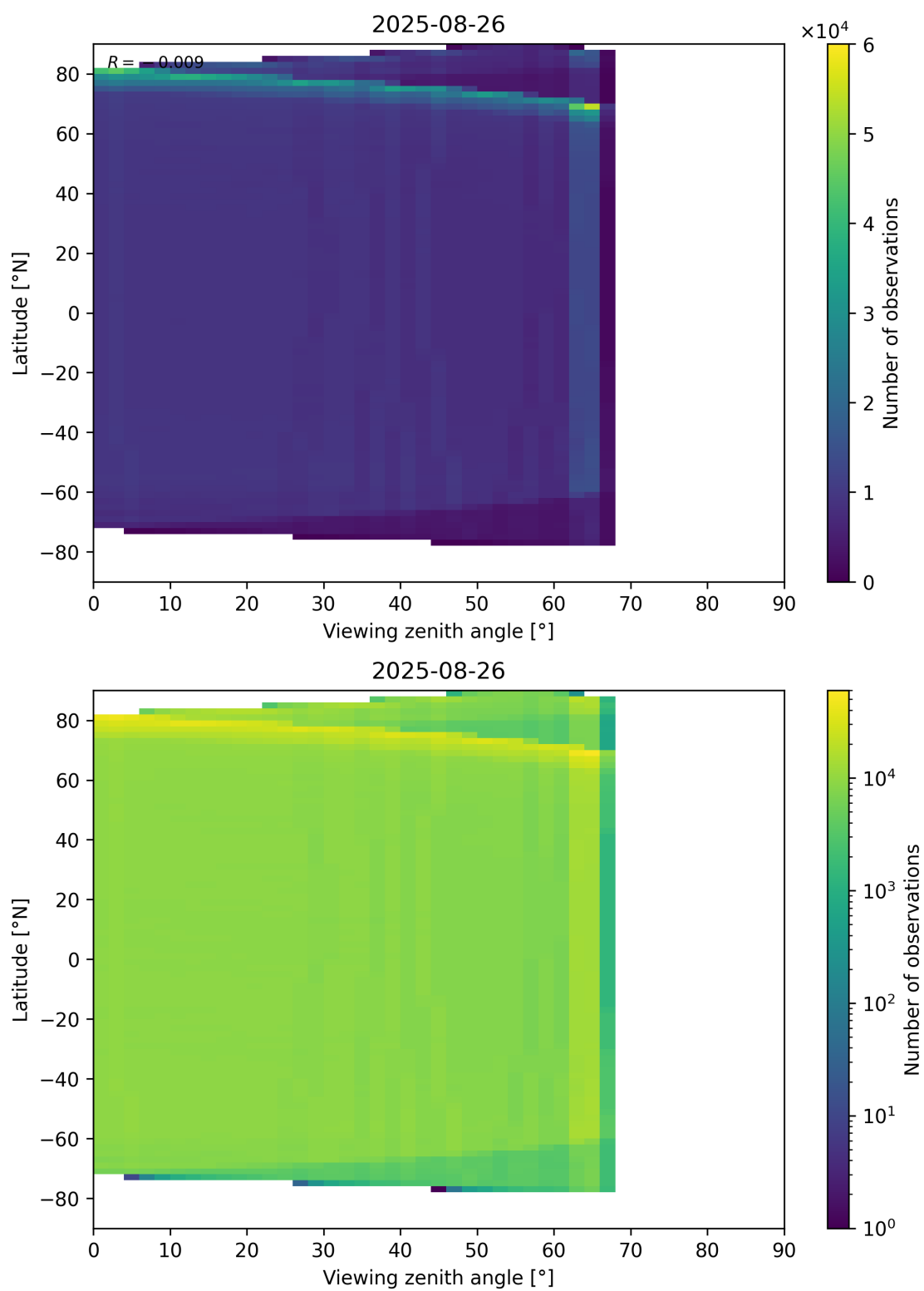
Figure 123: Scatter density plot of “Viewing zenith angle” against “Latitude” for 2025-08-25 to 2025-08-27.
