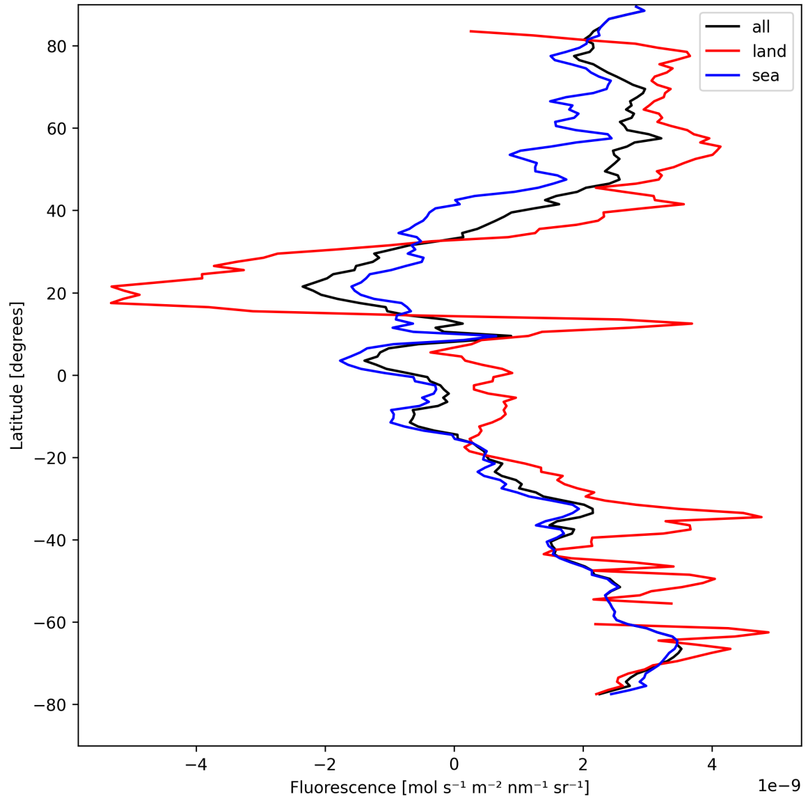
Figure 23: Zonal average of “Fluorescence” for 2025-08-25 to 2025-08-27.
