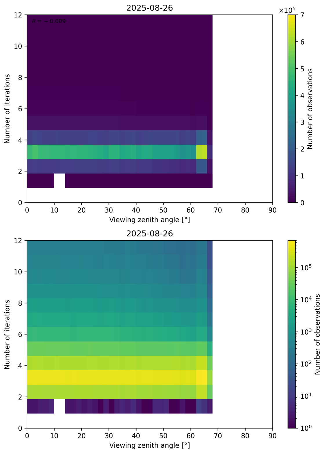
Figure 124: Scatter density plot of “Viewing zenith angle” against “Number of iterations” for 2025-08-25 to 2025-08-27.
