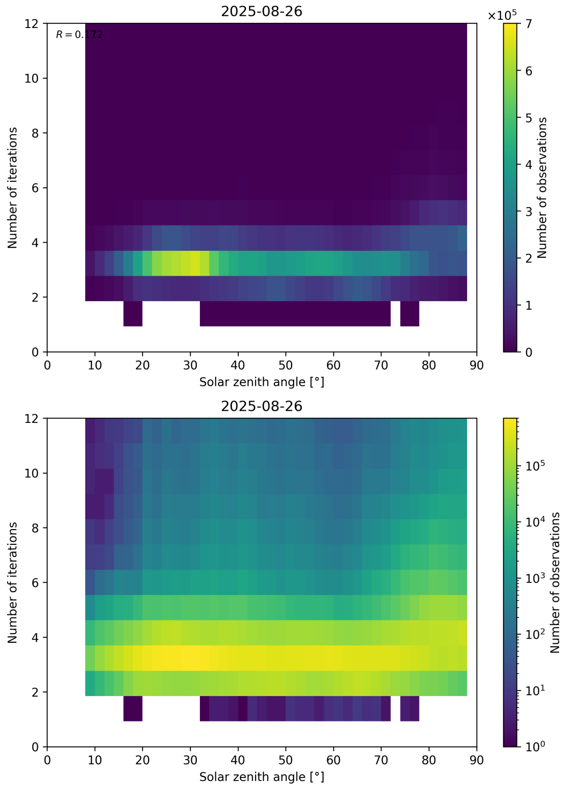
Figure 114: Scatter density plot of “Solar zenith angle” against “Number of iterations” for 2025-08-25 to 2025-08-27.
