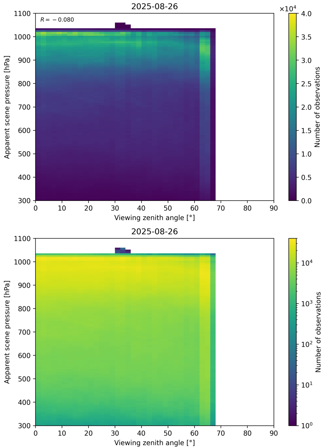
Figure 118: Scatter density plot of “Viewing zenith angle” against “Apparent scene pressure” for 2025-08-25 to 2025-08-27.
