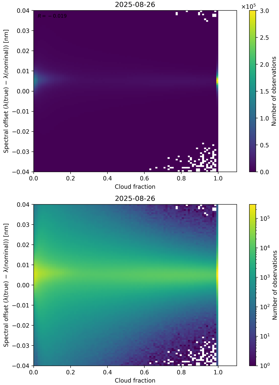
Figure 76: Scatter density plot of “Cloud fraction” against “Spectral offset ( \lambda_{\text{true}} - \lambda_{\text{nominal}} )” for 2025-08-25 to 2025-08-27.
