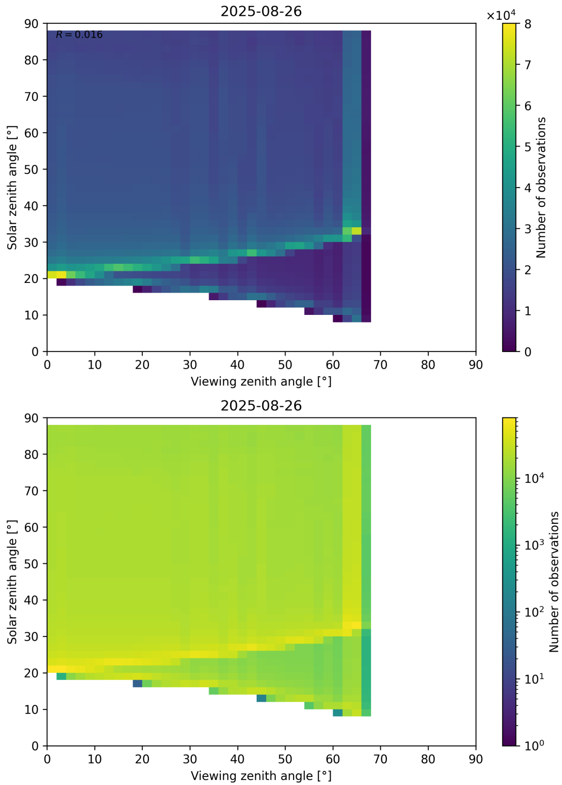
Figure 127: Scatter density plot of “Viewing zenith angle” against “Solar zenith angle” for 2025-08-25 to 2025-08-27.
