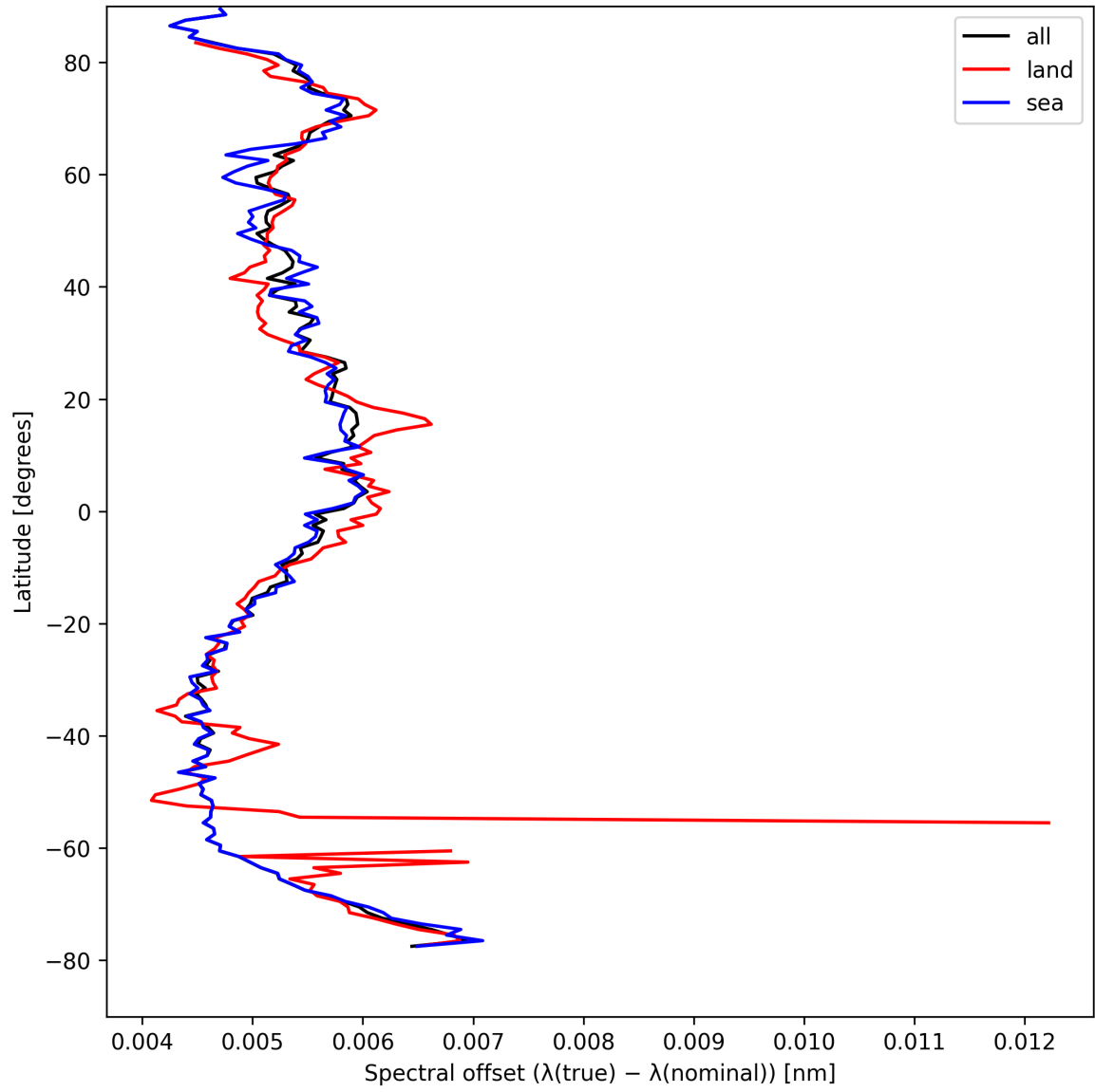
Figure 28: Zonal average of “Spectral offset ( \lambda_{\text{true}} - \lambda_{\text{nominal}} )” for 2025-08-25 to 2025-08-27.
