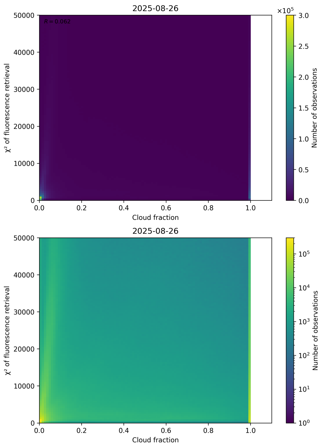
Figure 71: Scatter density plot of “Cloud fraction” against “ \chi^2 of fluorescence retrieval” for 2025-08-25 to 2025-08-27.
