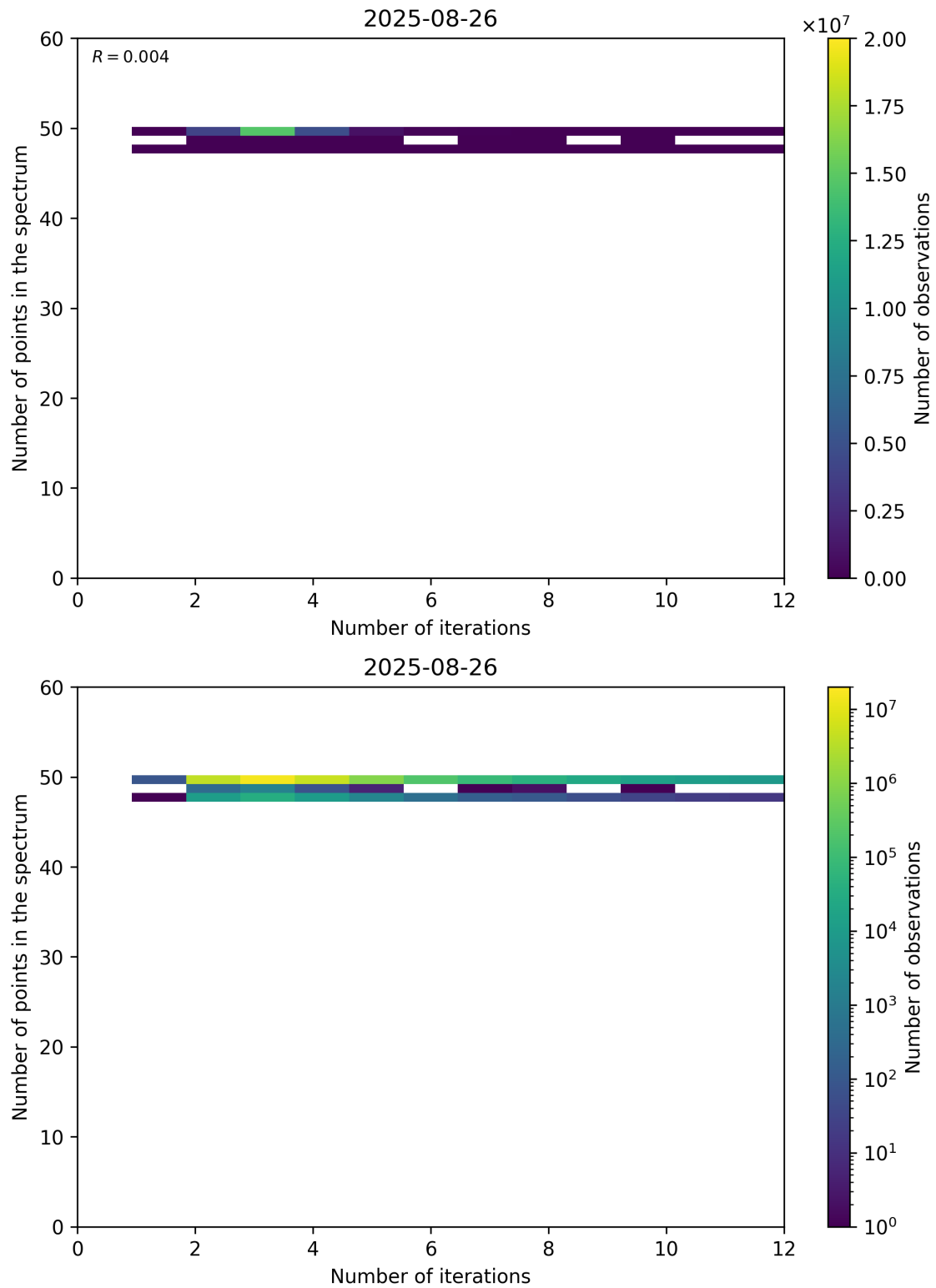
Figure 99: Scatter density plot of “Number of iterations” against “Number of points in the spectrum” for 2025-08-25 to 2025-08-27.
