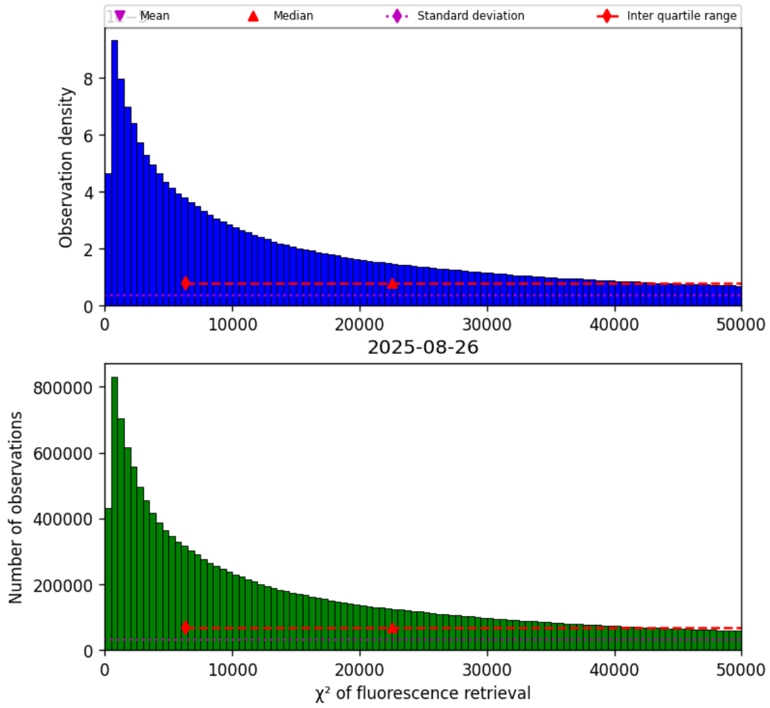
Figure 42: Histogram of “ \chi^2 of fluorescence retrieval” for 2025-08-25 to 2025-08-27
