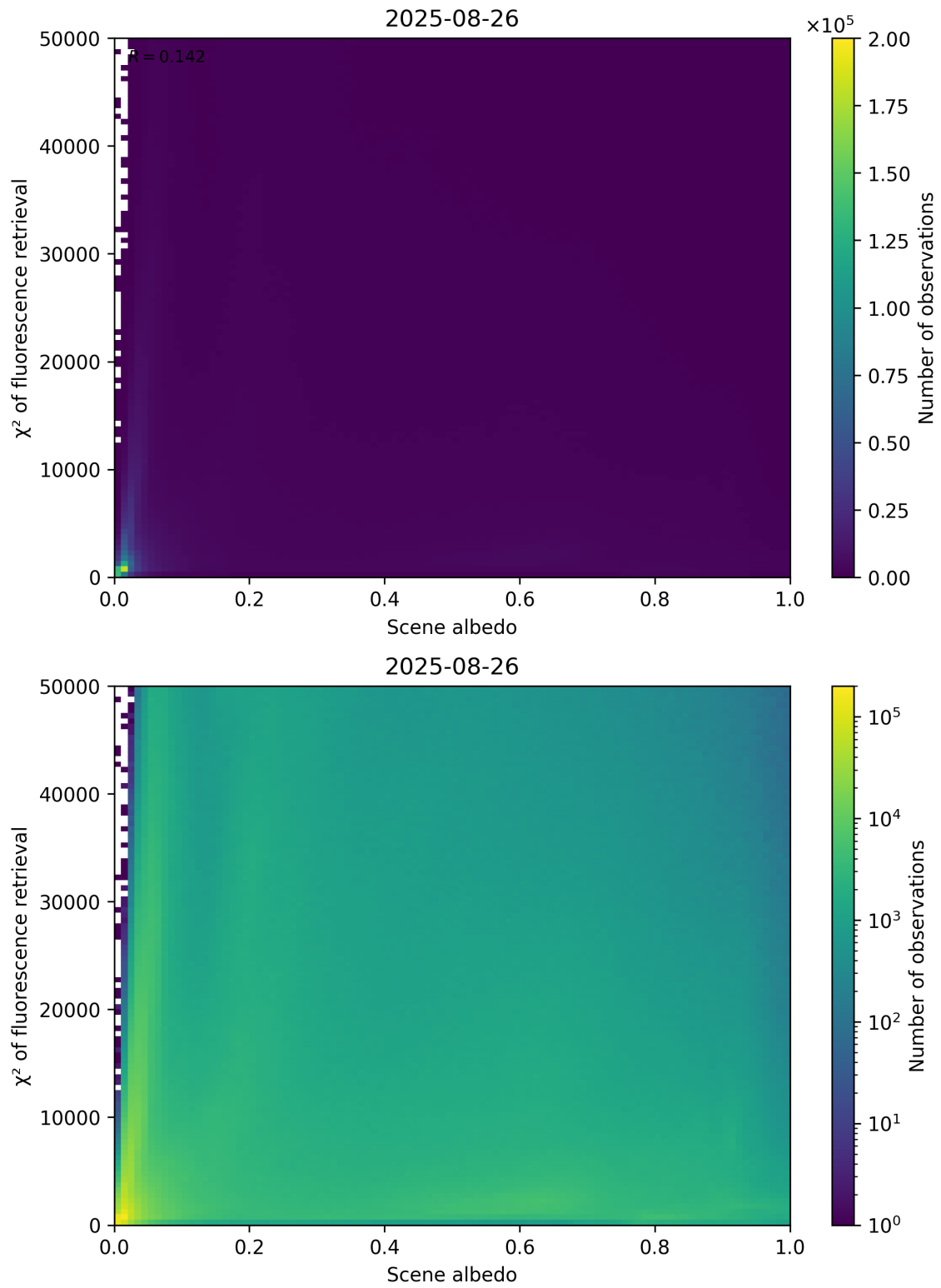
Figure 103: Scatter density plot of “Scene albedo” against “ \chi^2 of fluorescence retrieval” for 2025-08-25 to 2025-08-27.
