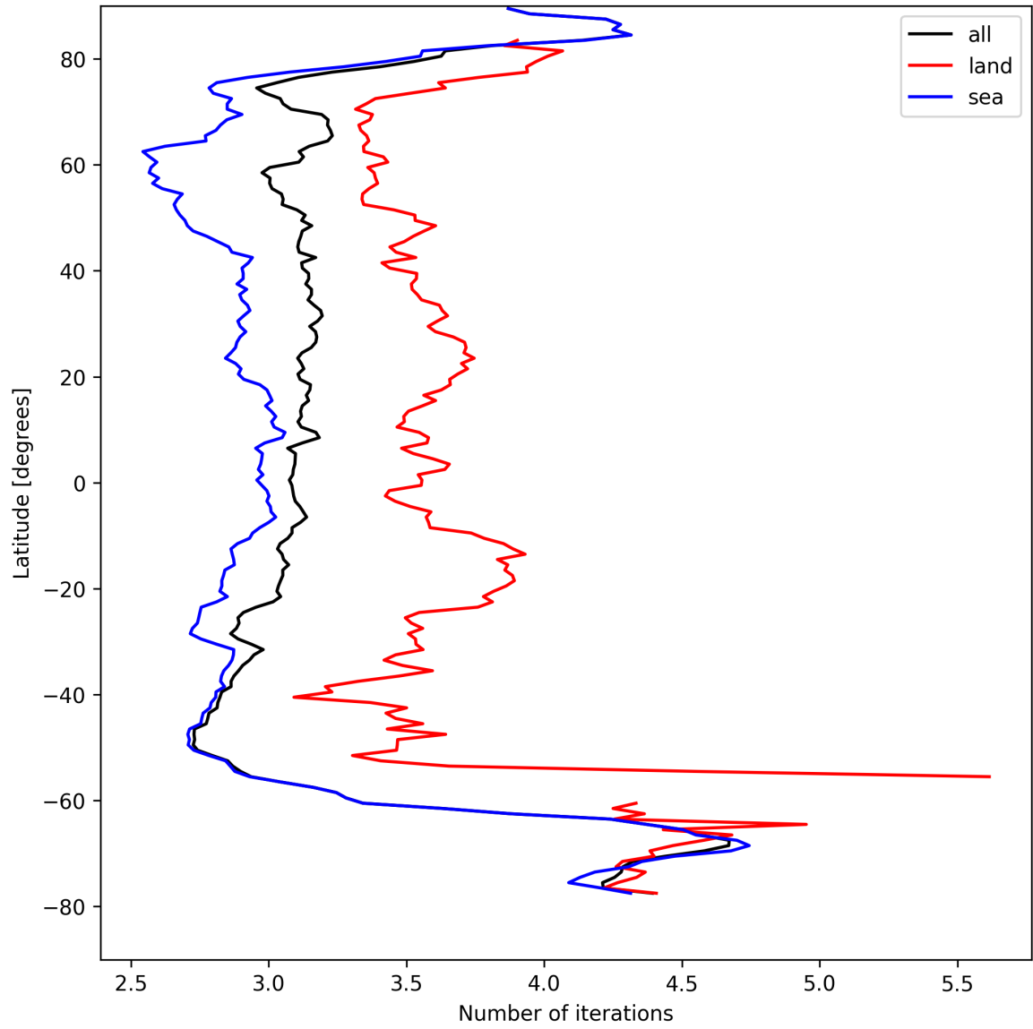
Figure 22: Zonal average of “Number of iterations” for 2025-08-25 to 2025-08-27.
