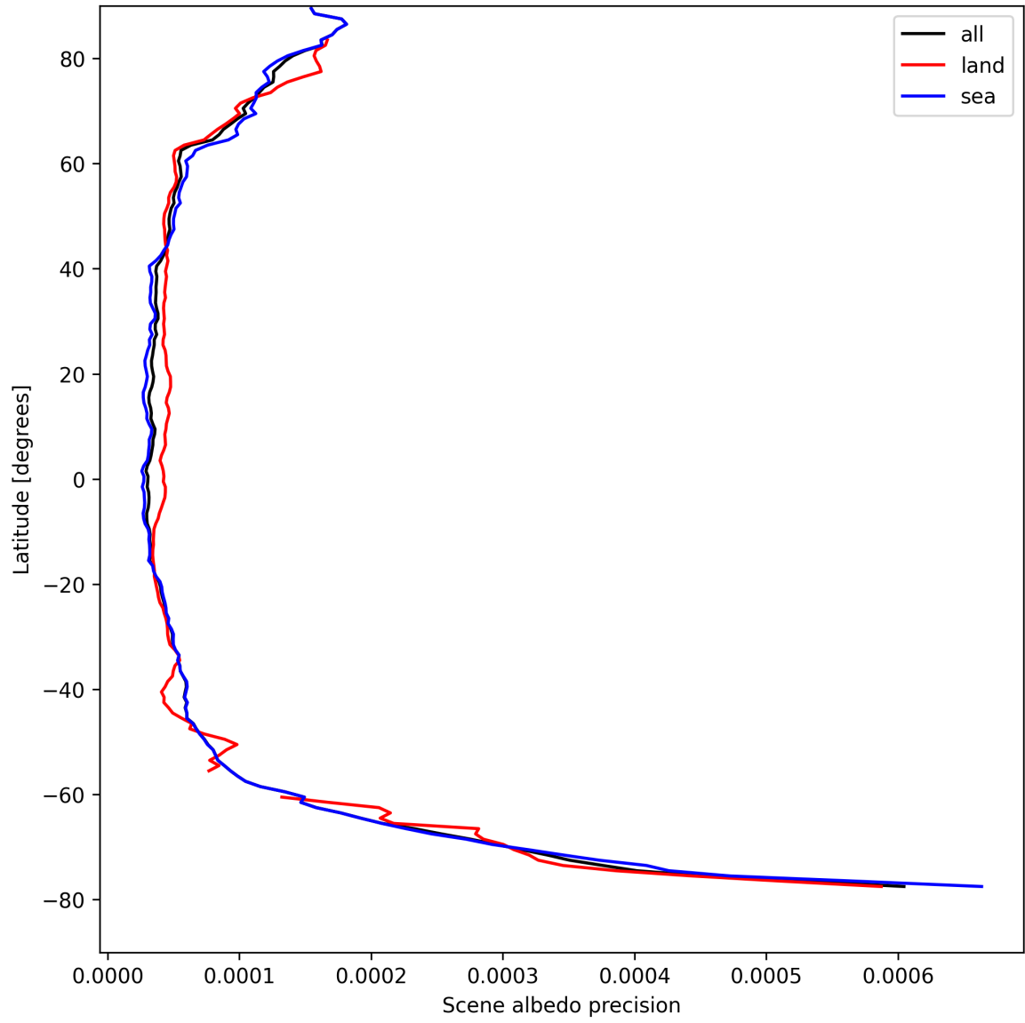
Figure 18: Zonal average of “Scene albedo precision” for 2025-08-25 to 2025-08-27.
