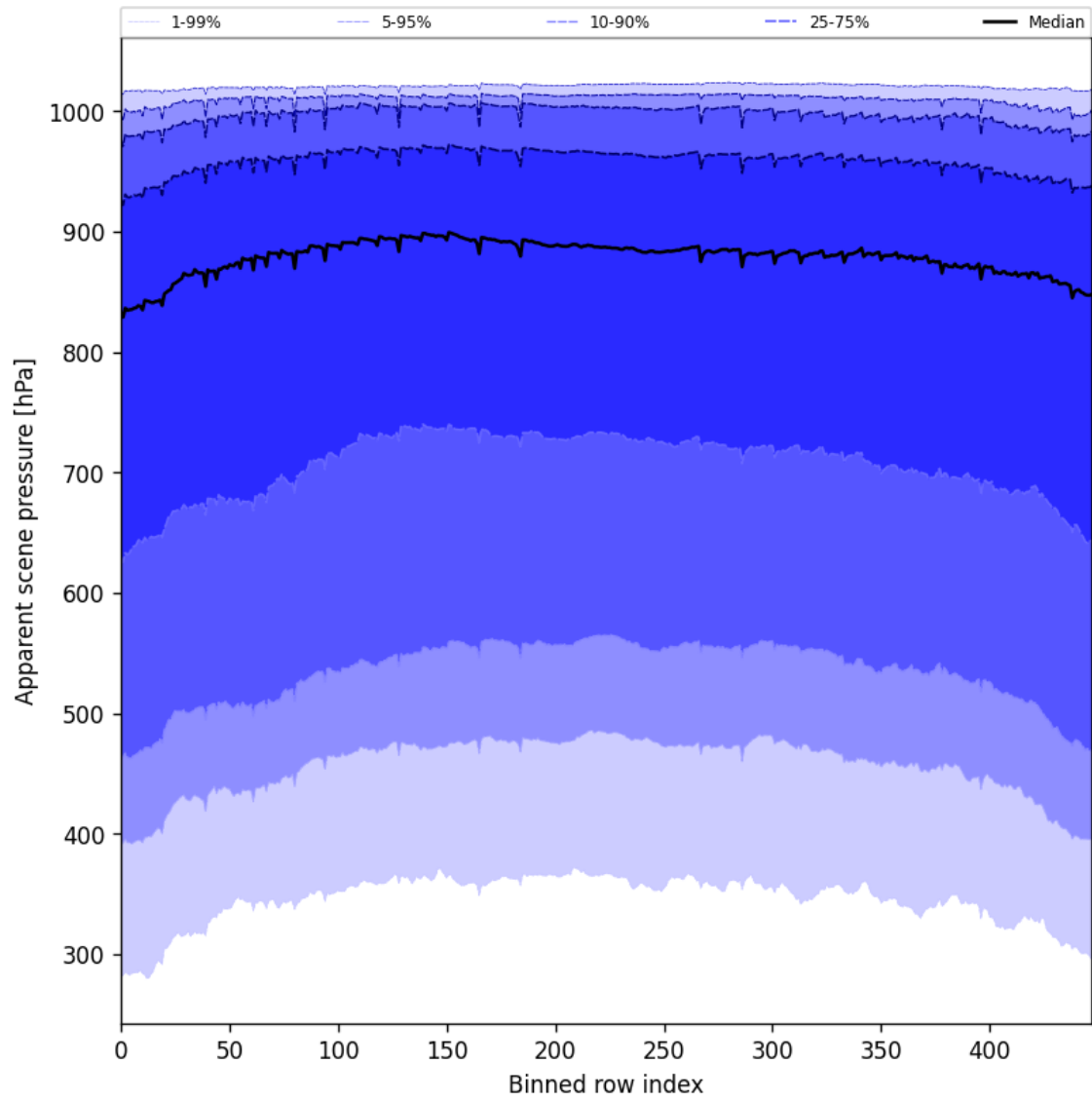
Figure 53: Along track statistics of “Apparent scene pressure” for 2025-08-25 to 2025-08-27
