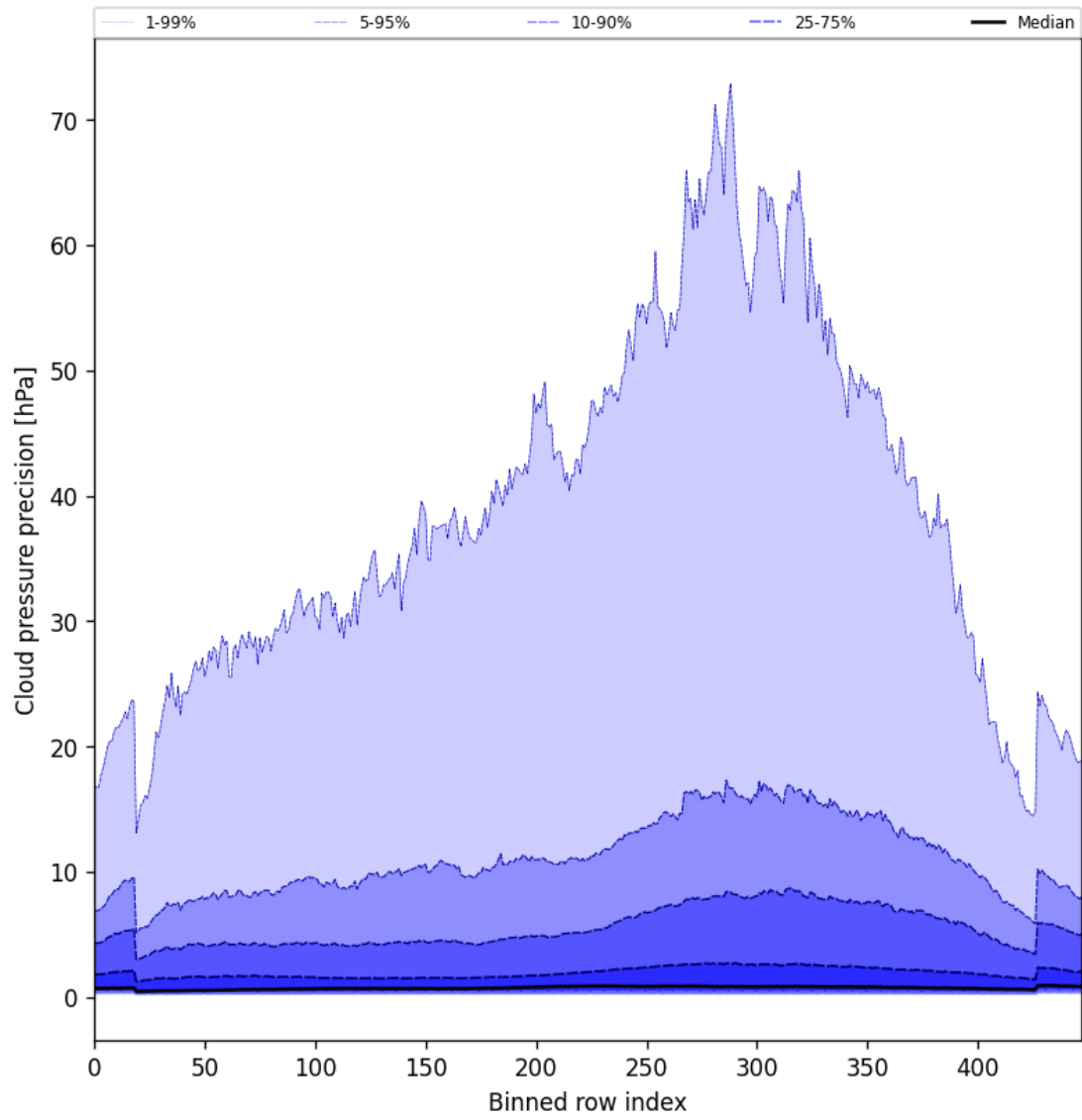
Figure 48: Along track statistics of “Cloud pressure precision” for 2025-08-25 to 2025-08-27
