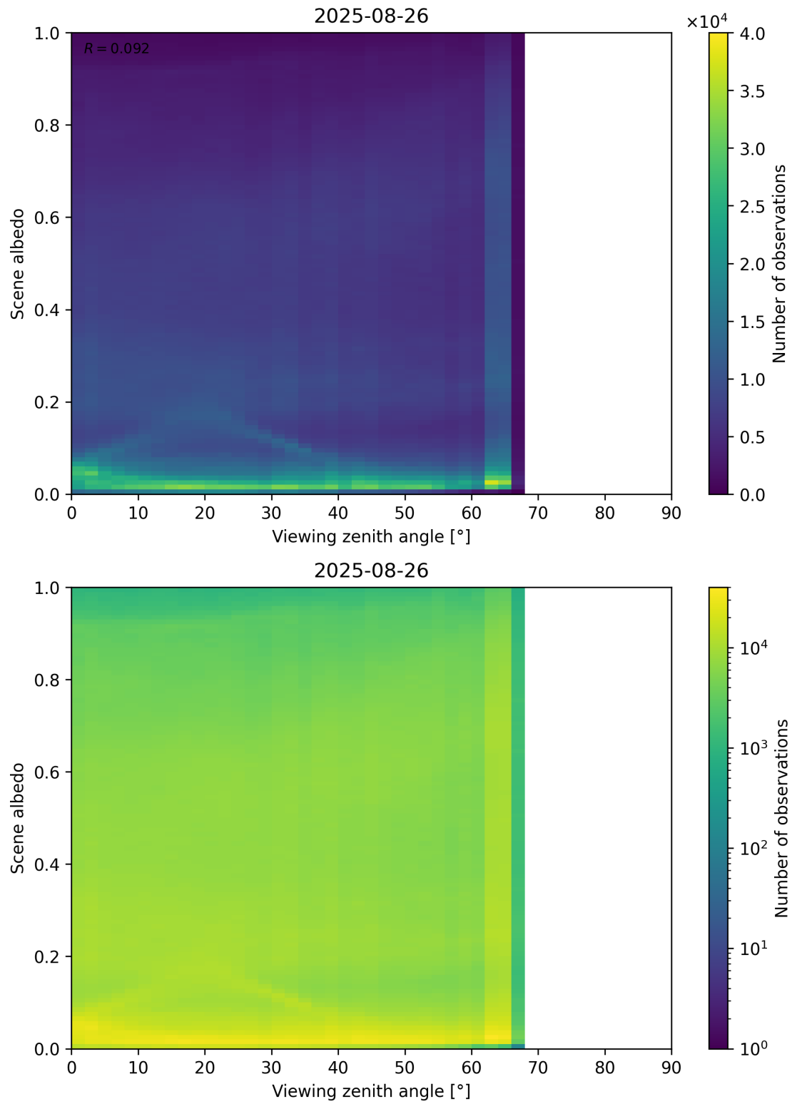
Figure 126: Scatter density plot of “Viewing zenith angle” against “Scene albedo” for 2025-08-25 to 2025-08-27.
