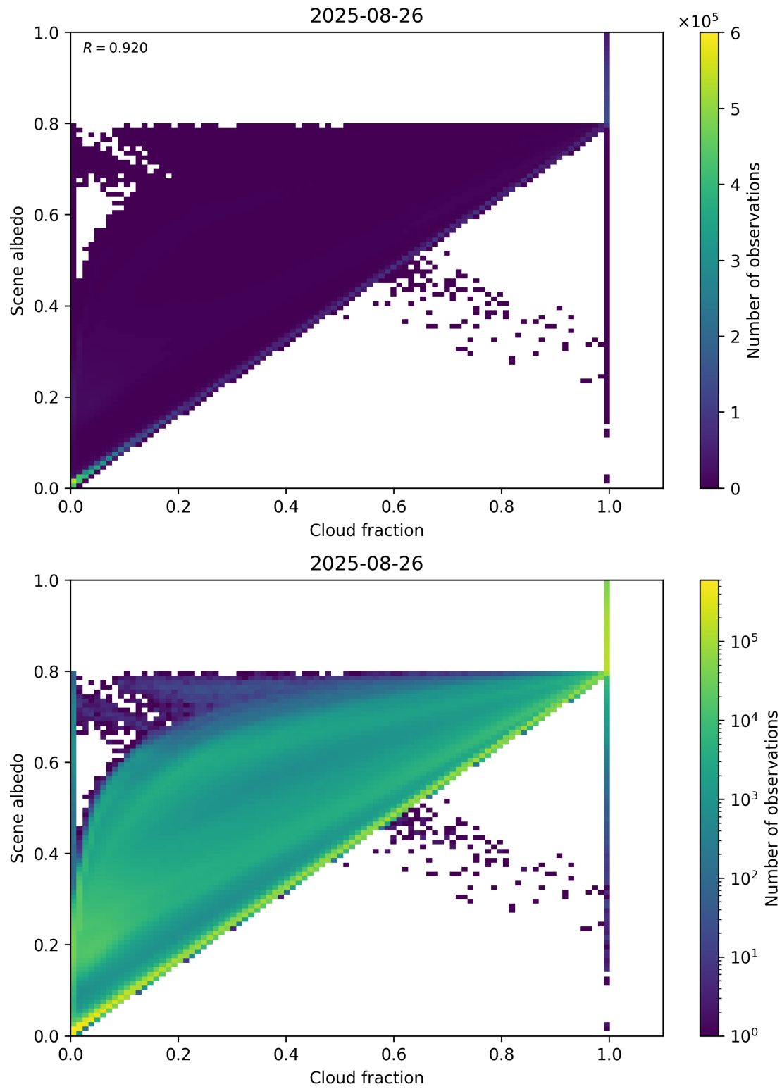
Figure 75: Scatter density plot of “Cloud fraction” against “Scene albedo” for 2025-08-25 to 2025-08-27.
