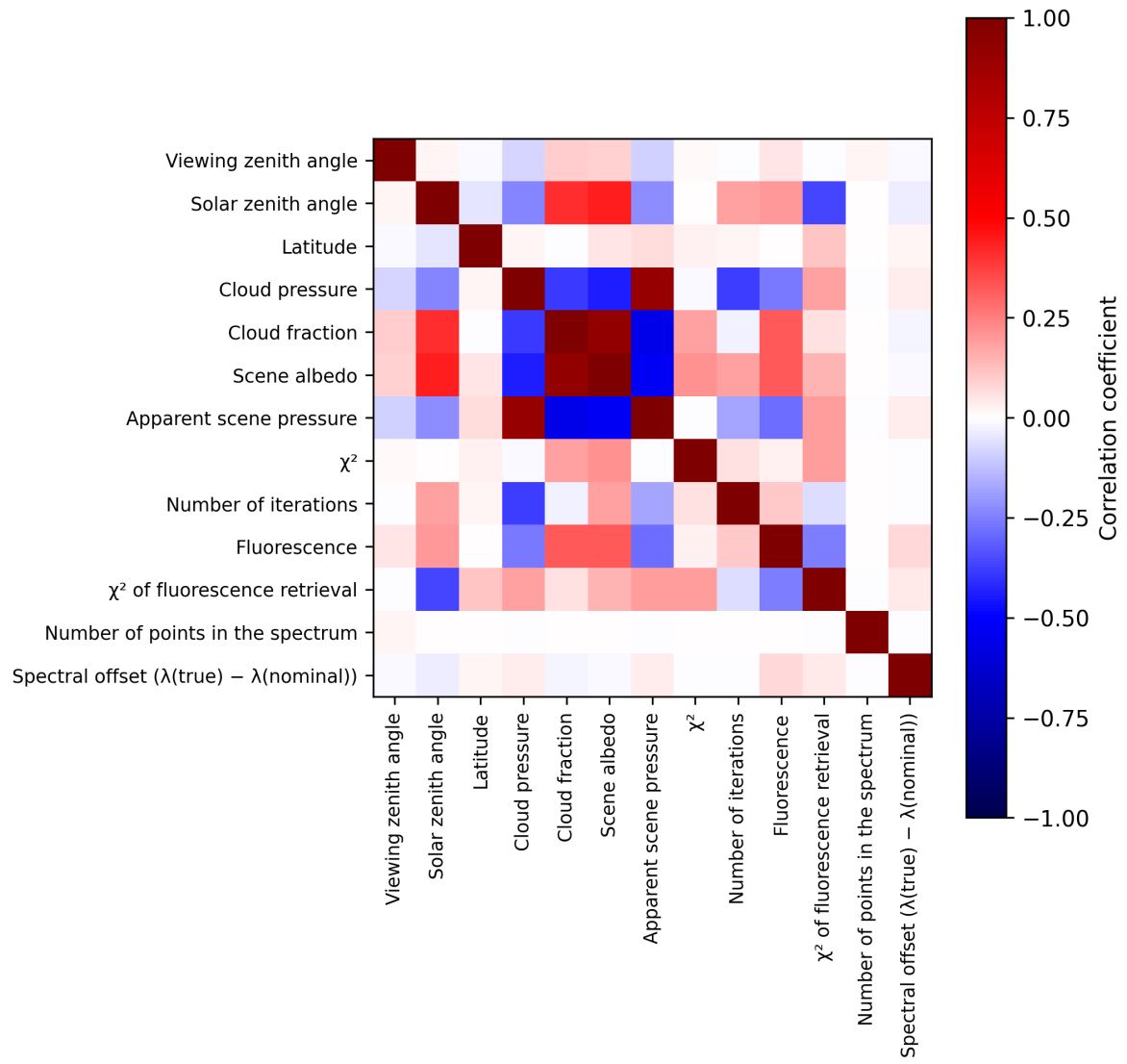
Figure 2: Map of correlation matrix for 2025-08-26 to 2025-08-28.
