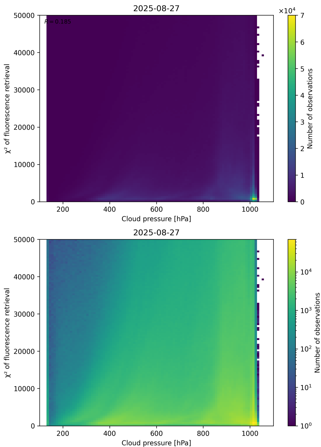
Figure 78: Scatter density plot of “Cloud pressure” against “ \chi^2 of fluorescence retrieval” for 2025-08-26 to 2025-08-28.
