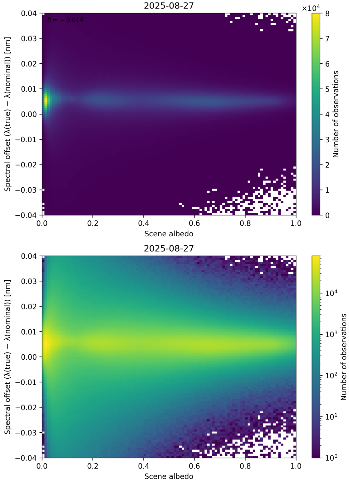
Figure 107: Scatter density plot of “Scene albedo” against “Spectral offset ( \lambda_{\text{true}} - \lambda_{\text{nominal}} )” for 2025-08-26 to 2025-08-28.
