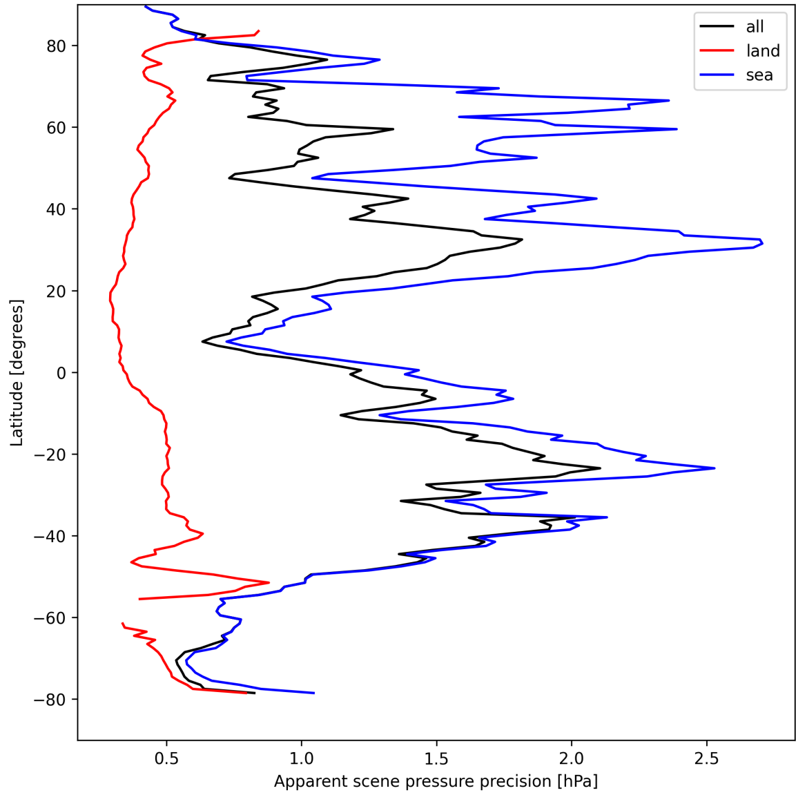
Figure 20: Zonal average of “Apparent scene pressure precision” for 2025-08-26 to 2025-08-28.
