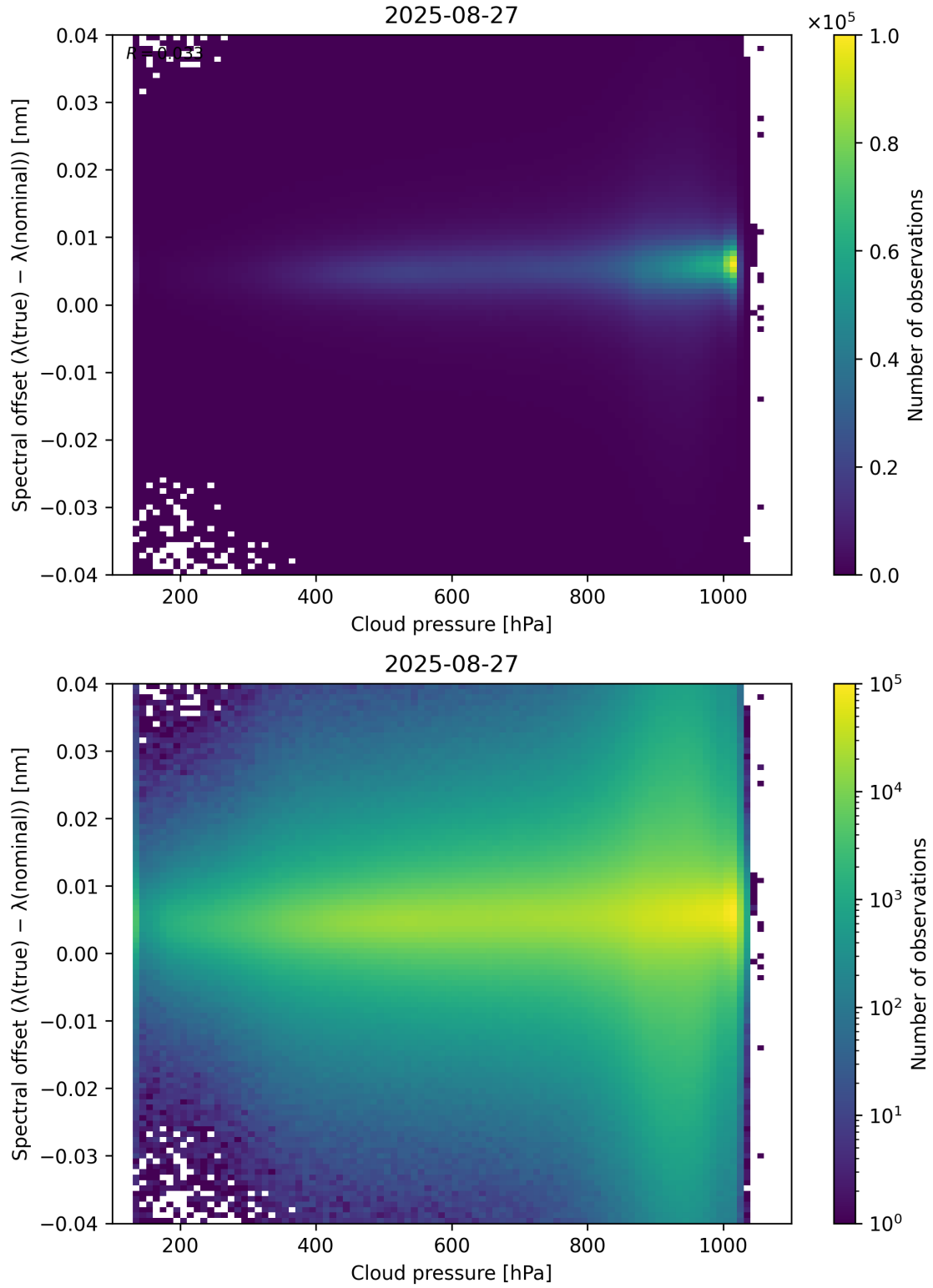
Figure 84: Scatter density plot of “Cloud pressure” against “Spectral offset ( \lambda_{\text{true}} - \lambda_{\text{nominal}} )” for 2025-08-26 to 2025-08-28.
