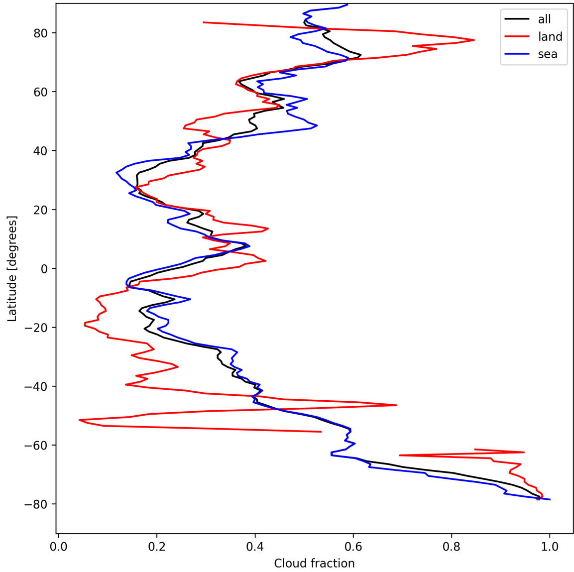
Figure 15: Zonal average of “Cloud fraction” for 2025-08-26 to 2025-08-28.
