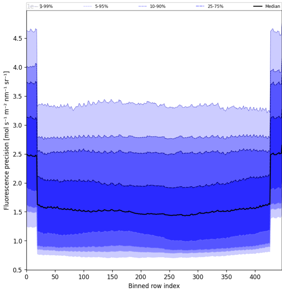
Figure 58: Along track statistics of “Fluorescence precision” for 2025-08-26 to 2025-08-28
