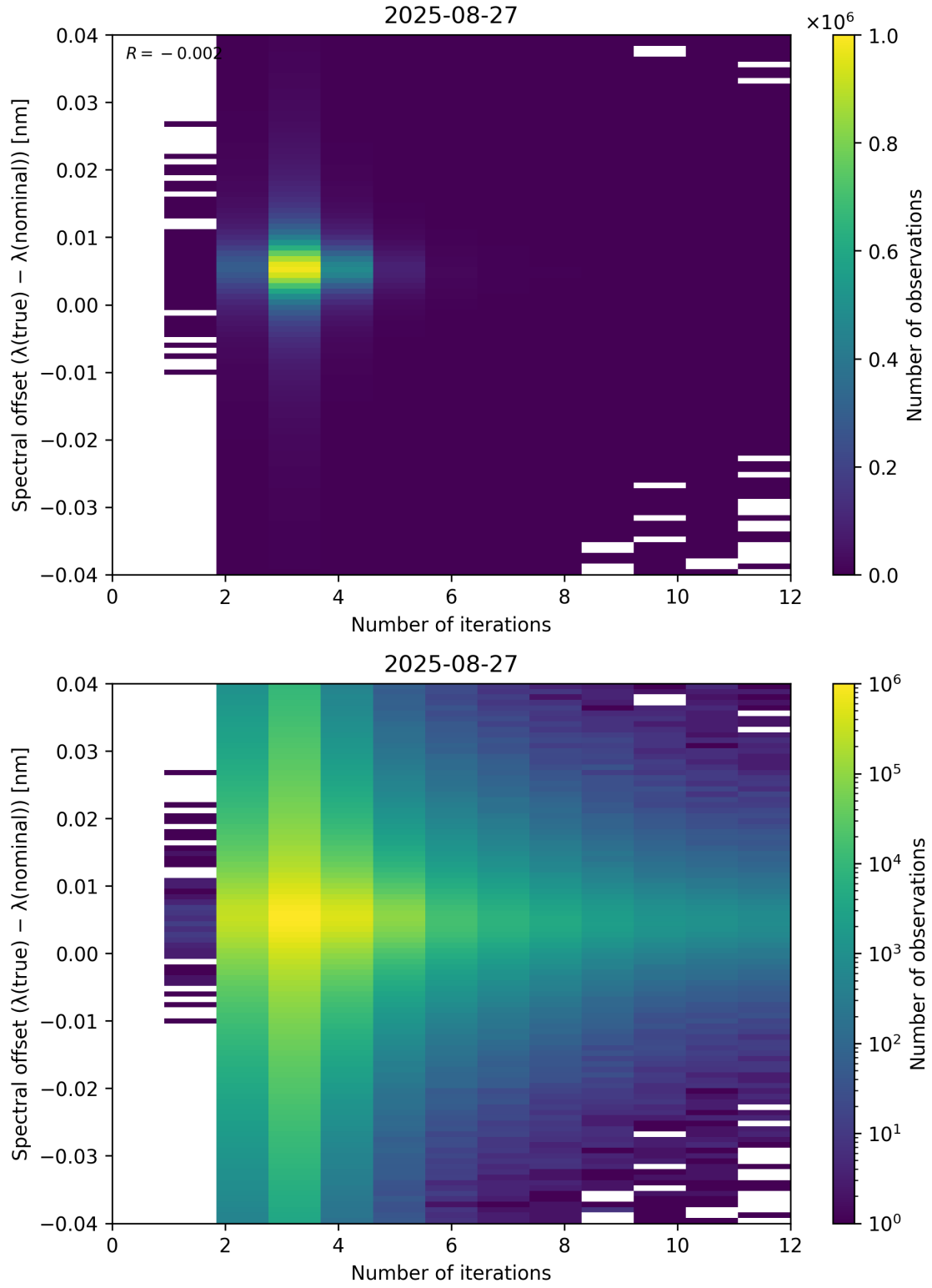
Figure 100: Scatter density plot of “Number of iterations” against “Spectral offset ( \lambda_{\text{true}} - \lambda_{\text{nominal}} )” for 2025-08-26 to 2025-08-28.
