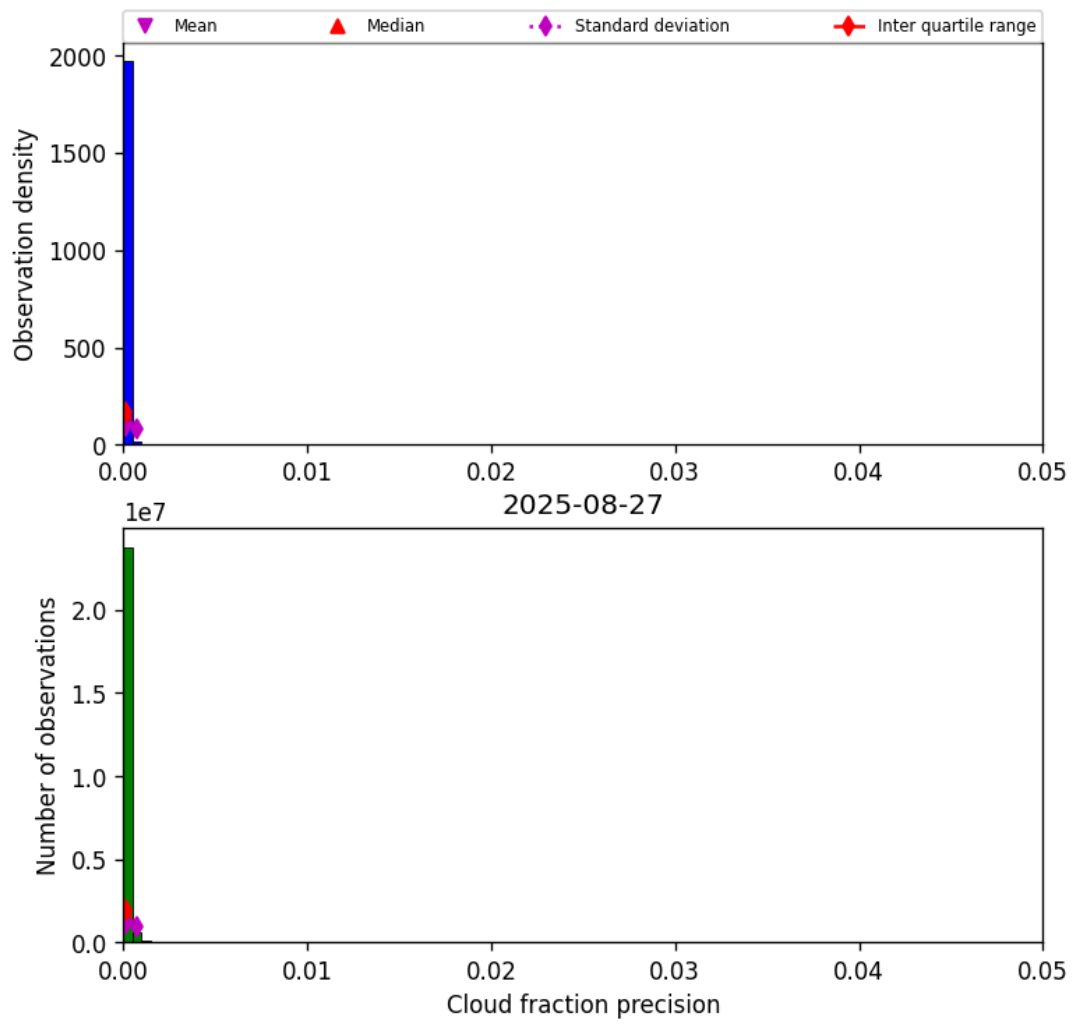
Figure 33: Histogram of “Cloud fraction precision” for 2025-08-26 to 2025-08-28
