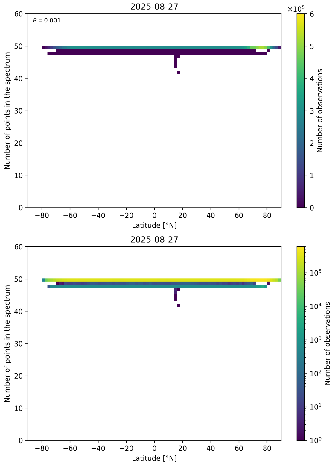
Figure 94: Scatter density plot of “Latitude” against “Number of points in the spectrum” for 2025-08-26 to 2025-08-28.
