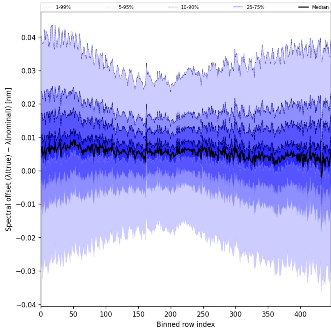
Figure 62: Along track statistics of “Spectral offset ( \lambda_{\text{true}} - \lambda_{\text{nominal}} )” for 2025-08-26 to 2025-08-28
