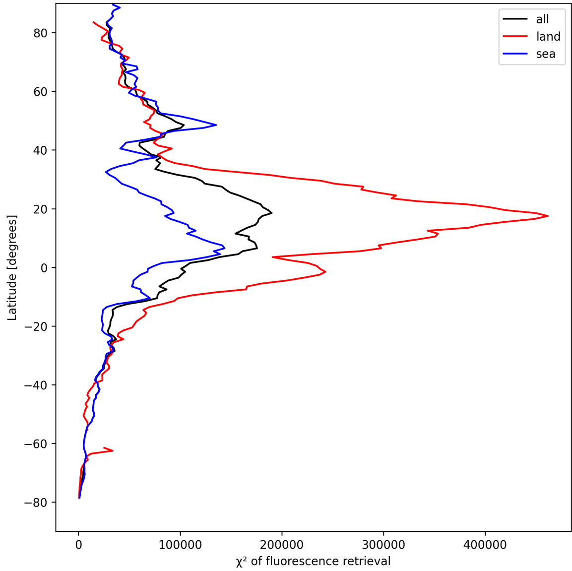
Figure 25: Zonal average of “ \chi^2 of fluorescence retrieval” for 2025-08-26 to 2025-08-28.
