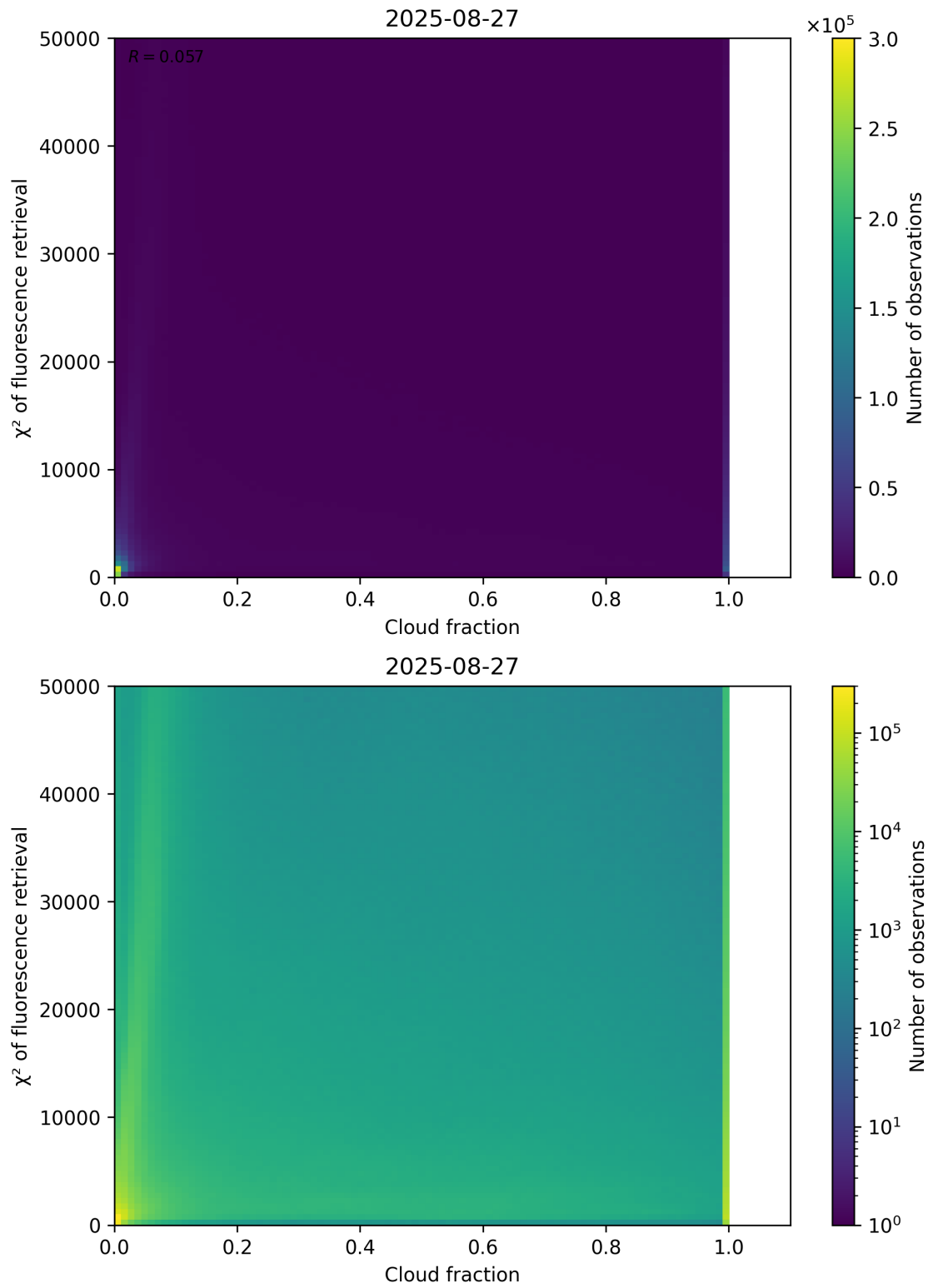
Figure 71: Scatter density plot of “Cloud fraction” against “ \chi^2 of fluorescence retrieval” for 2025-08-26 to 2025-08-28.
