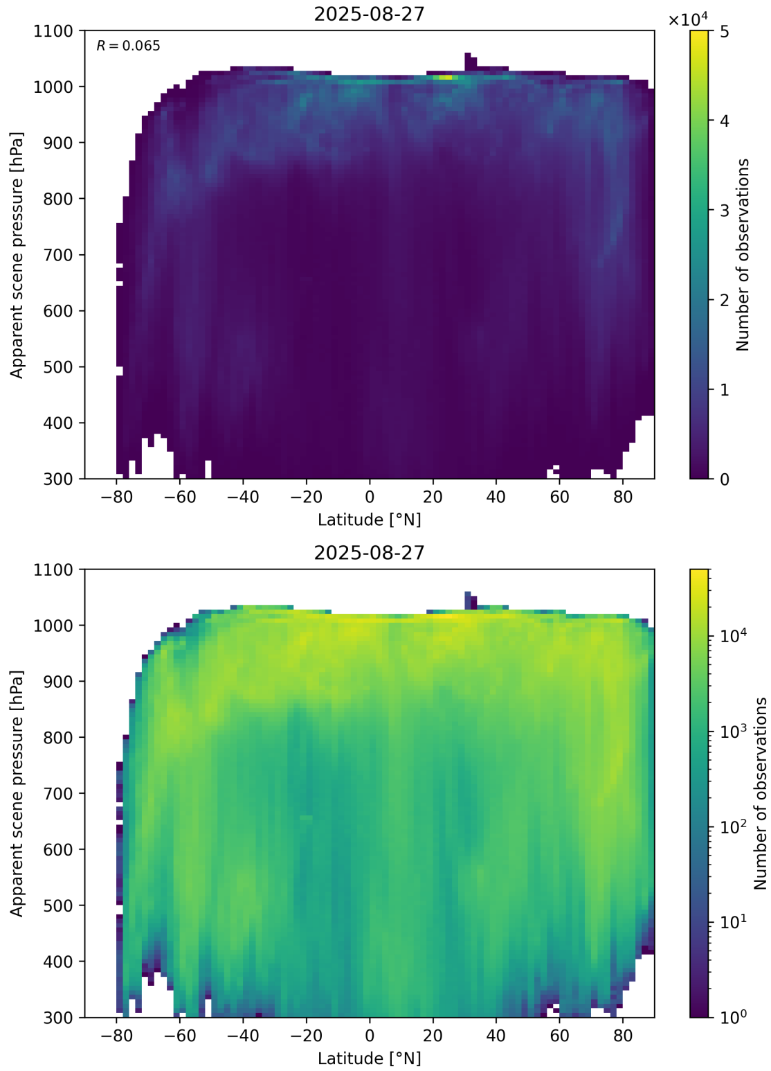
Figure 88: Scatter density plot of “Latitude” against “Apparent scene pressure” for 2025-08-26 to 2025-08-28.
