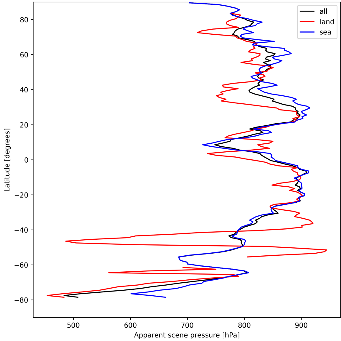
Figure 19: Zonal average of “Apparent scene pressure” for 2025-08-26 to 2025-08-28.
