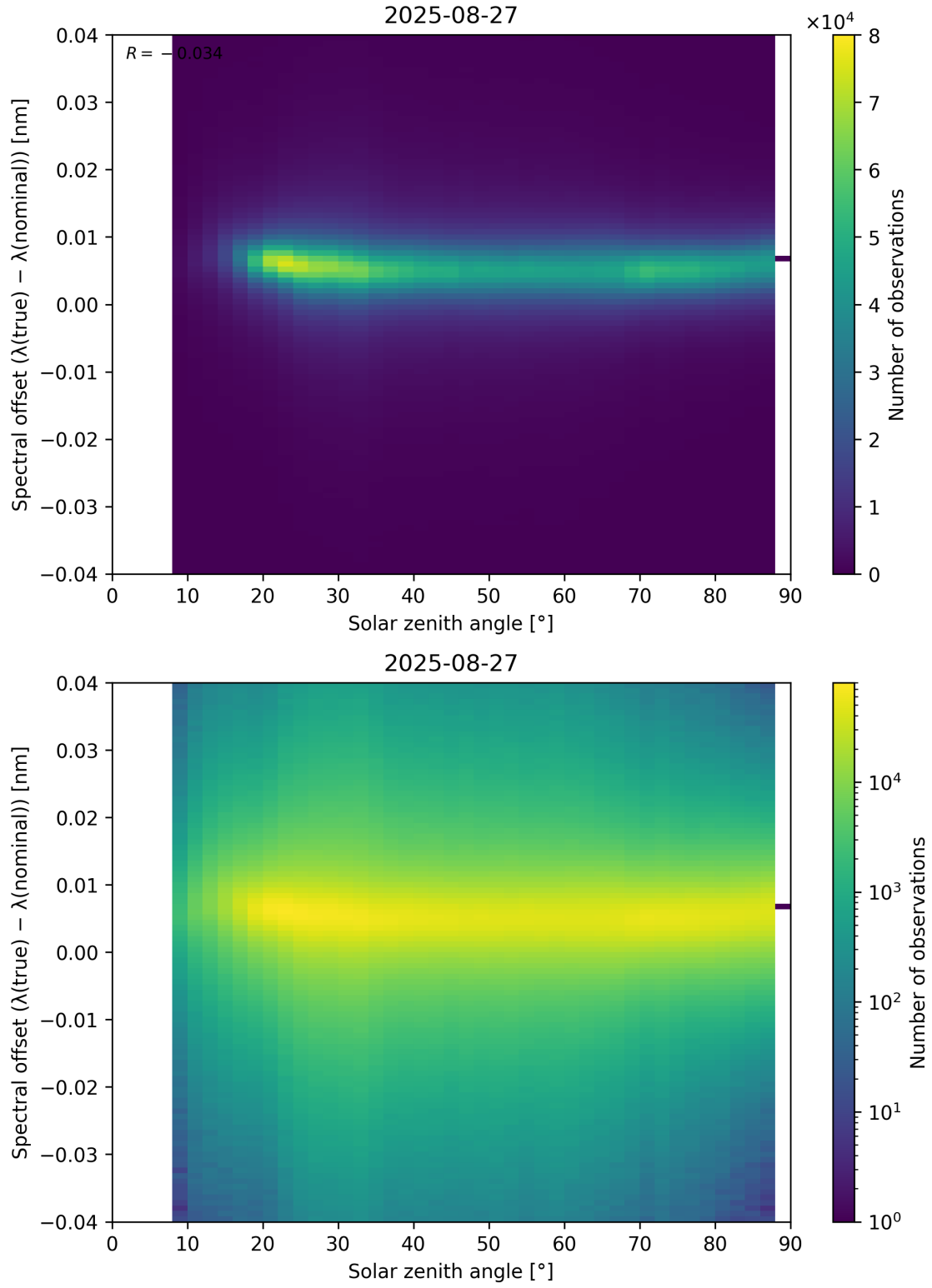
Figure 117: Scatter density plot of “Solar zenith angle” against “Spectral offset ( \lambda_{\text{true}} - \lambda_{\text{nominal}} )” for 2025-08-26 to 2025-08-28.
