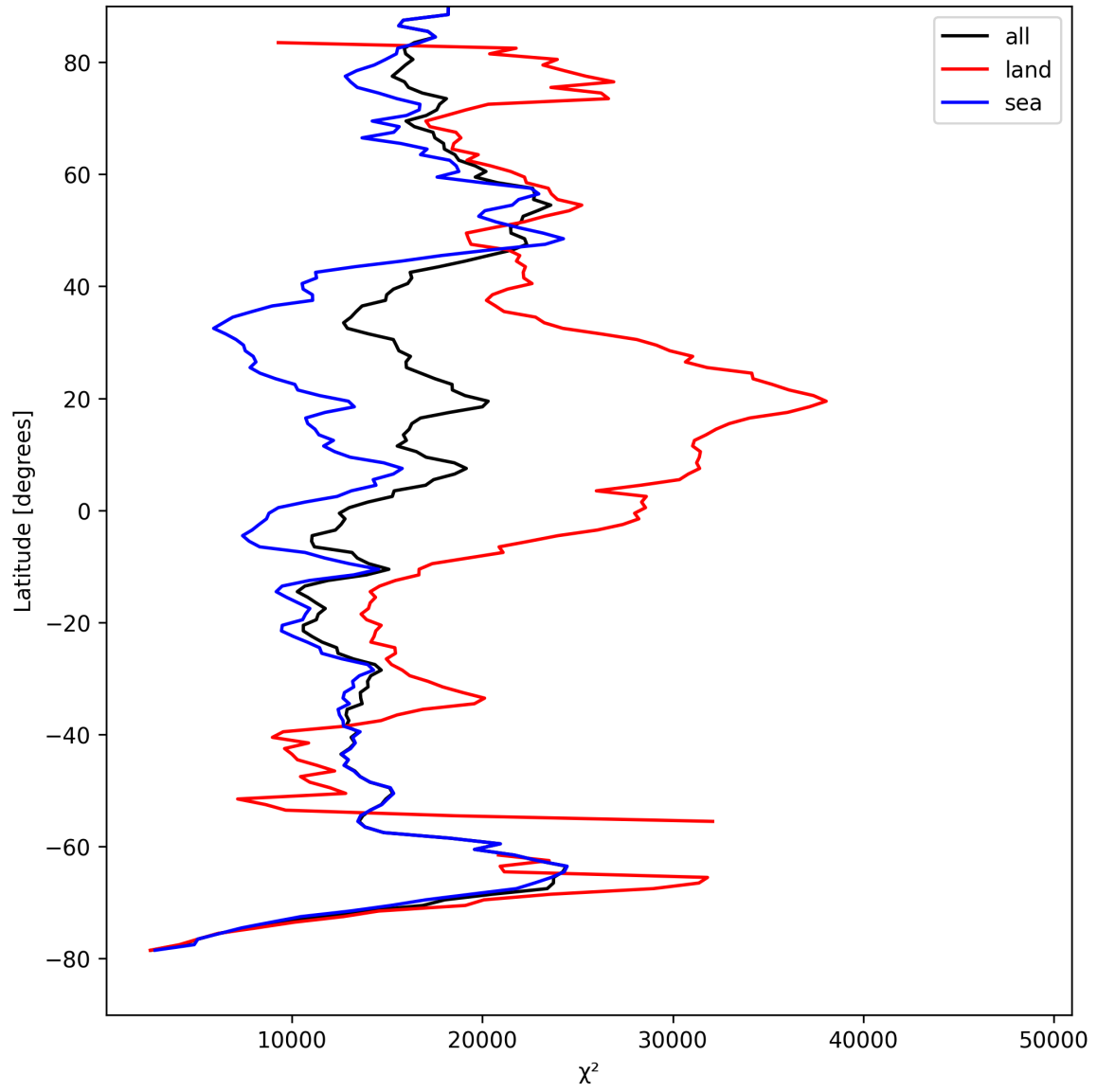
Figure 21: Zonal average of “ \chi^2 ” for 2025-08-26 to 2025-08-28.
