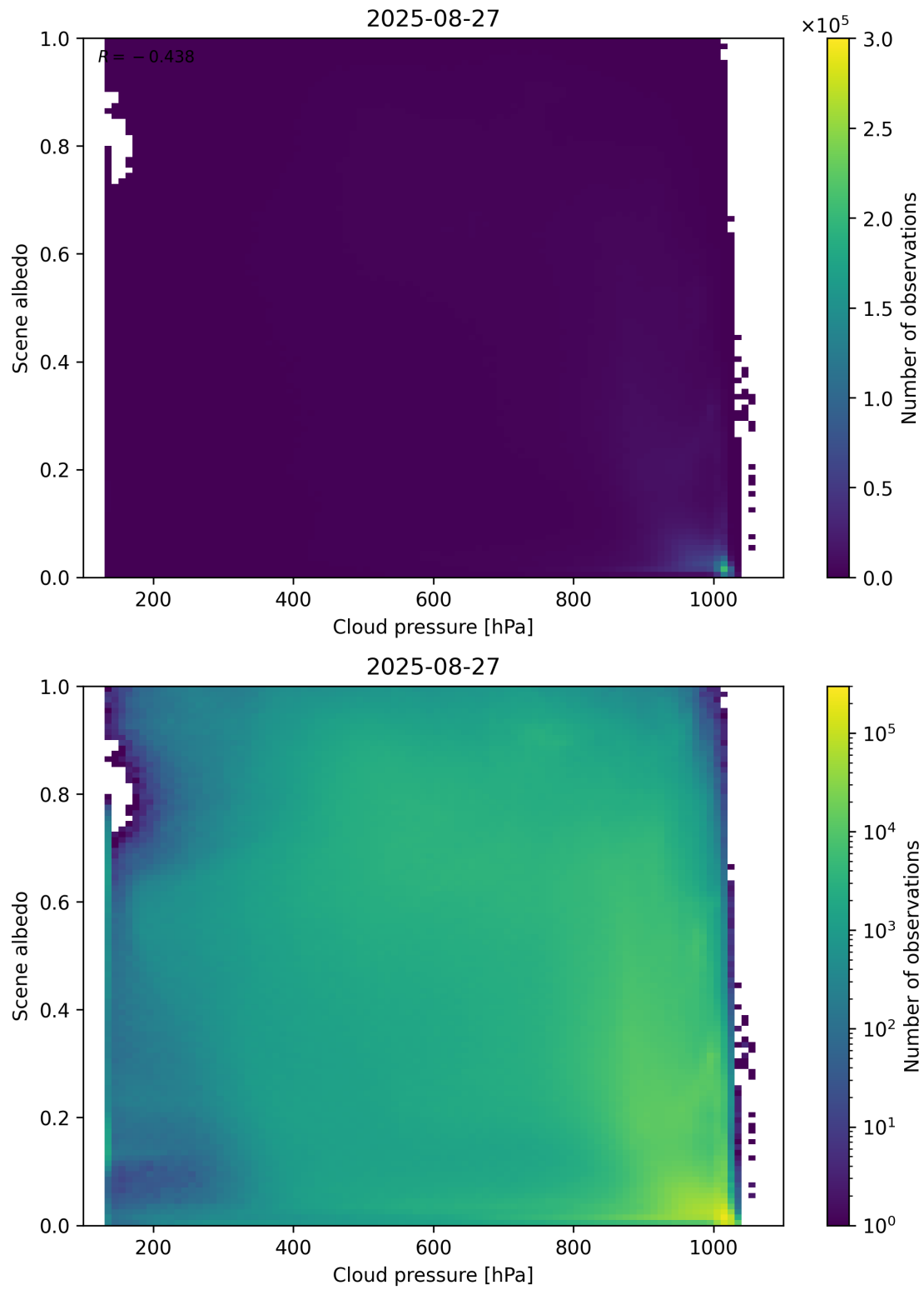
Figure 83: Scatter density plot of “Cloud pressure” against “Scene albedo” for 2025-08-26 to 2025-08-28.
