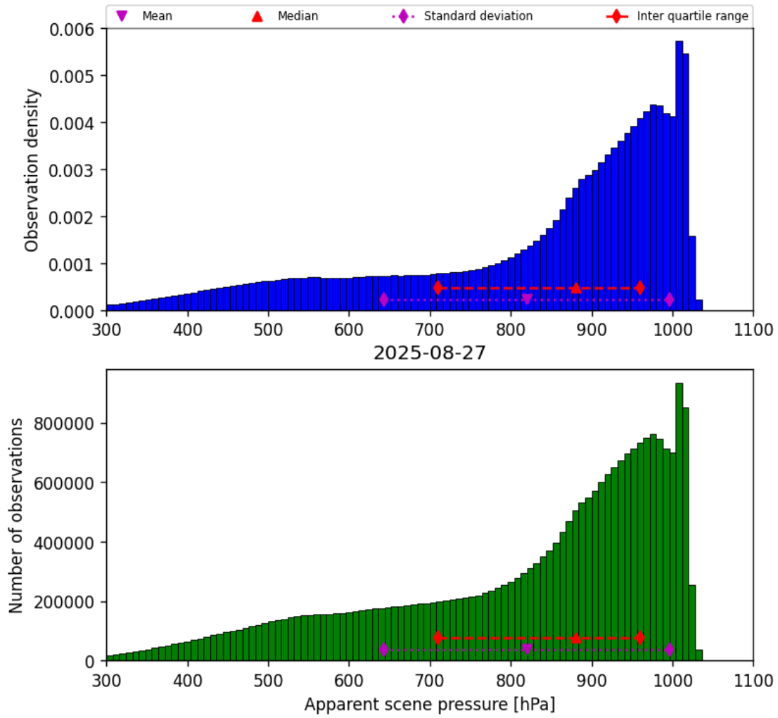
Figure 36: Histogram of “Apparent scene pressure” for 2025-08-26 to 2025-08-28
