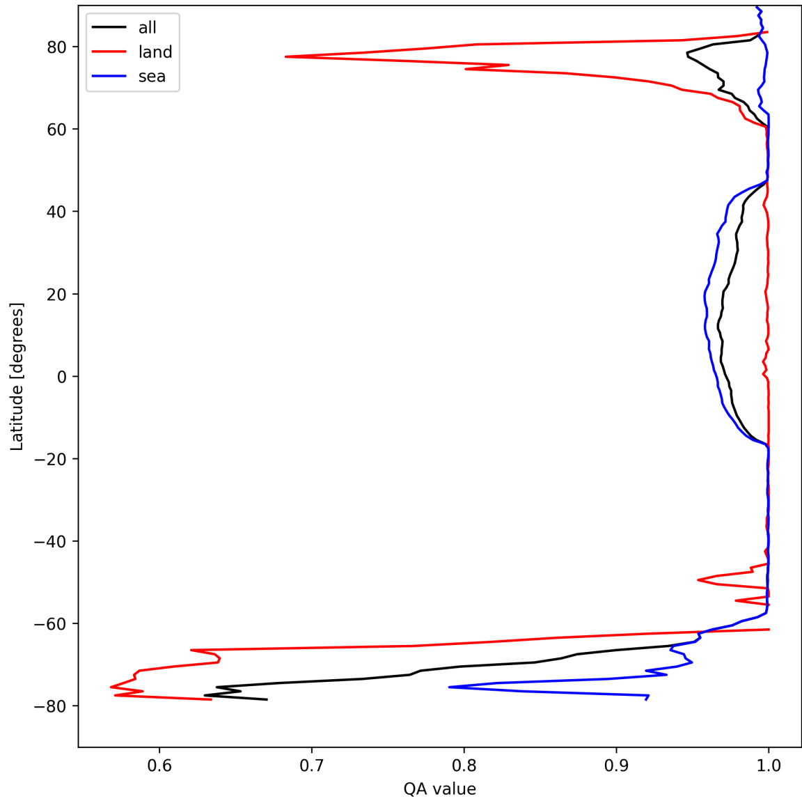
Figure 12: Zonal average of “QA value” for 2025-08-26 to 2025-08-28.
