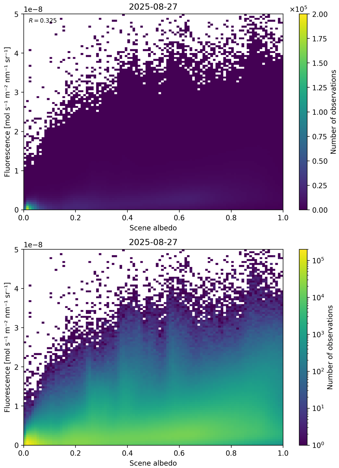
Figure 104: Scatter density plot of “Scene albedo” against “Fluorescence” for 2025-08-26 to 2025-08-28.
