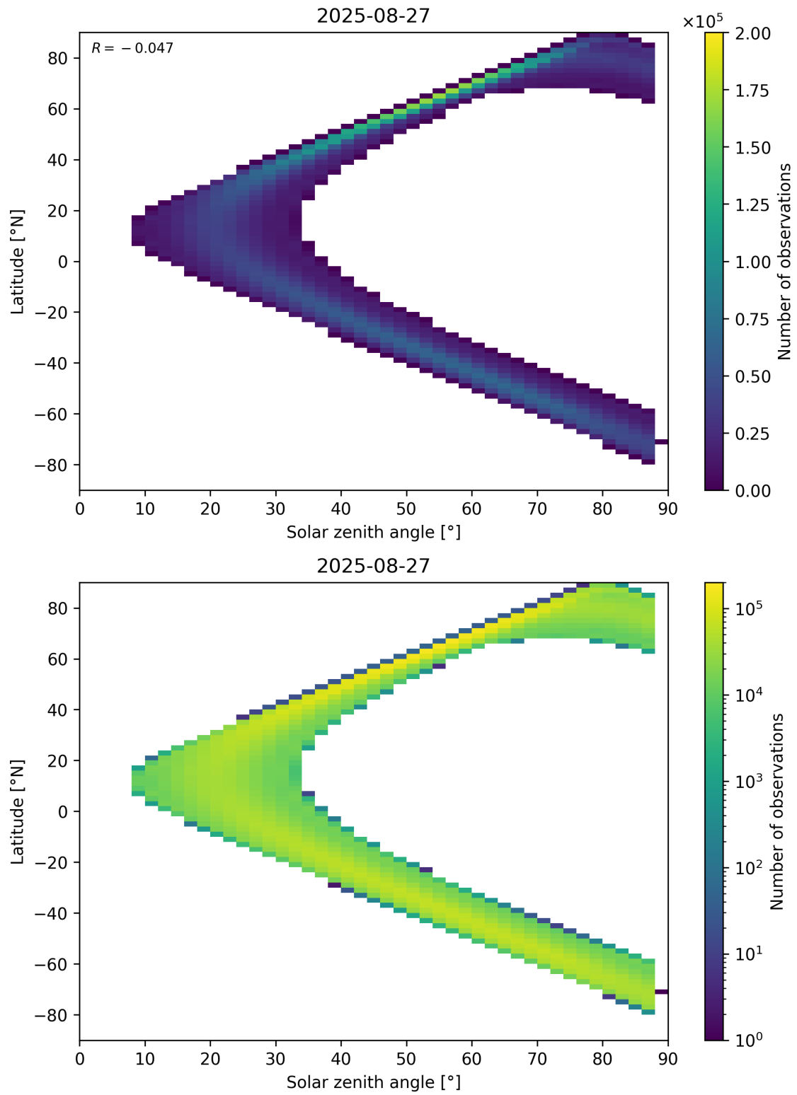
Figure 113: Scatter density plot of “Solar zenith angle” against “Latitude” for 2025-08-26 to 2025-08-28.
