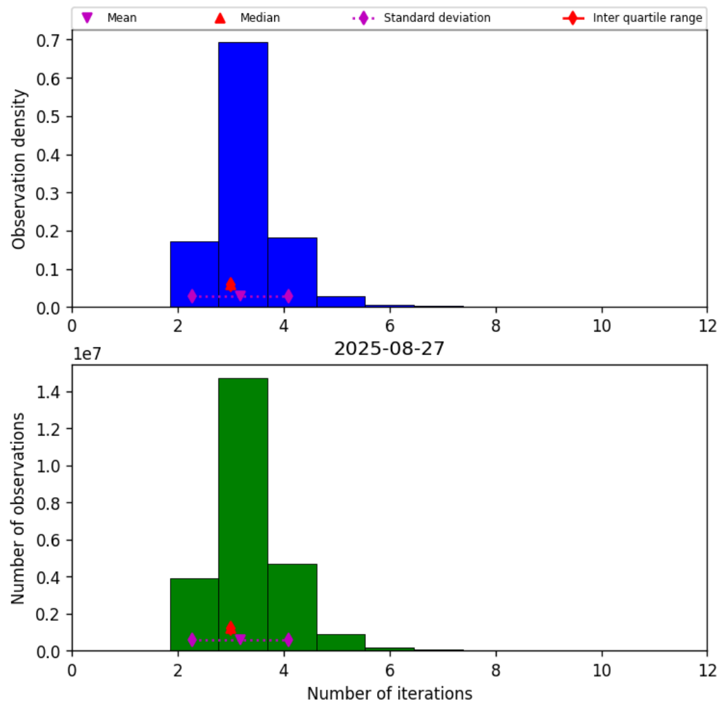
Figure 39: Histogram of “Number of iterations” for 2025-08-26 to 2025-08-28
