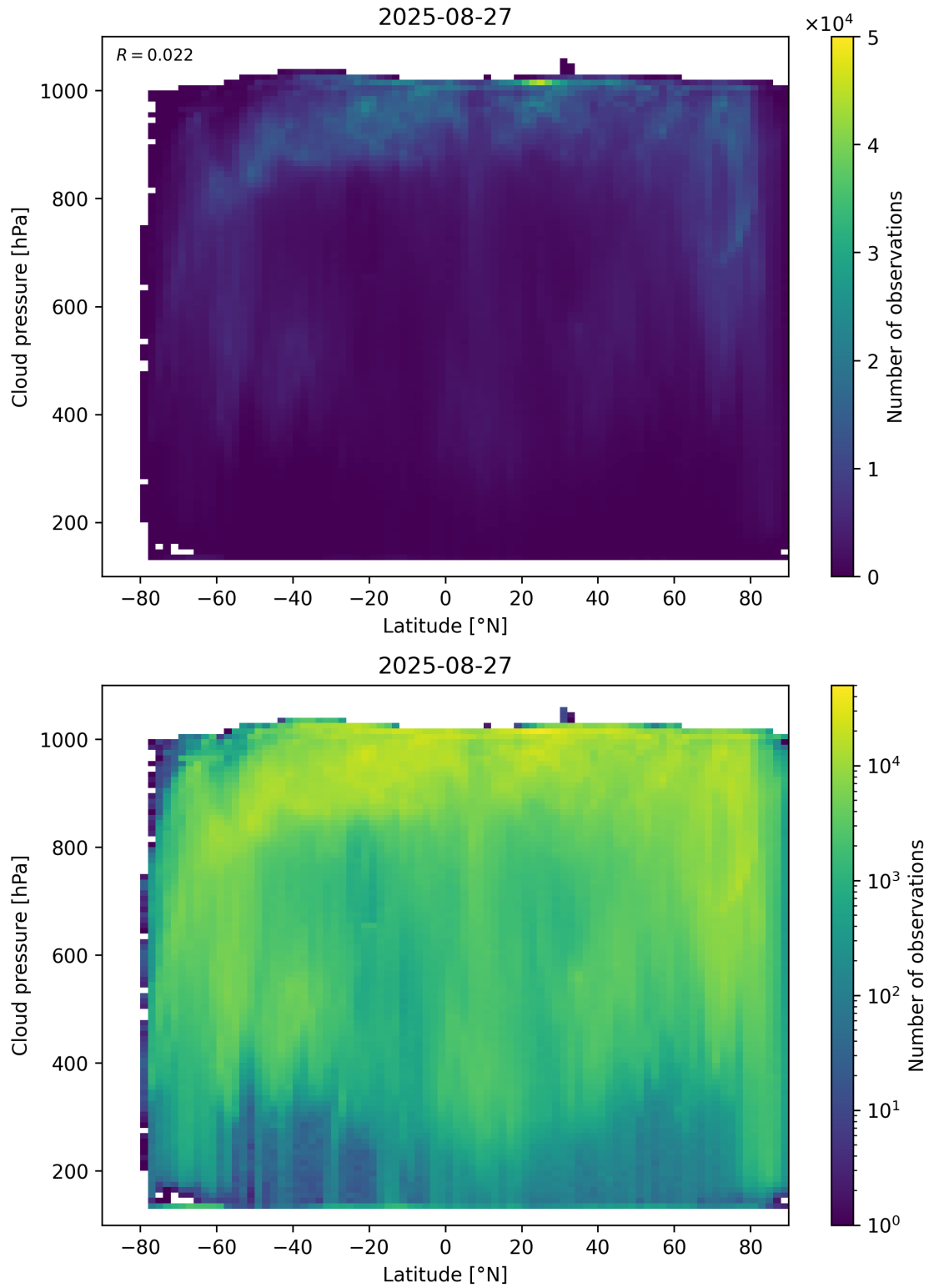
Figure 91: Scatter density plot of “Latitude” against “Cloud pressure” for 2025-08-26 to 2025-08-28.
