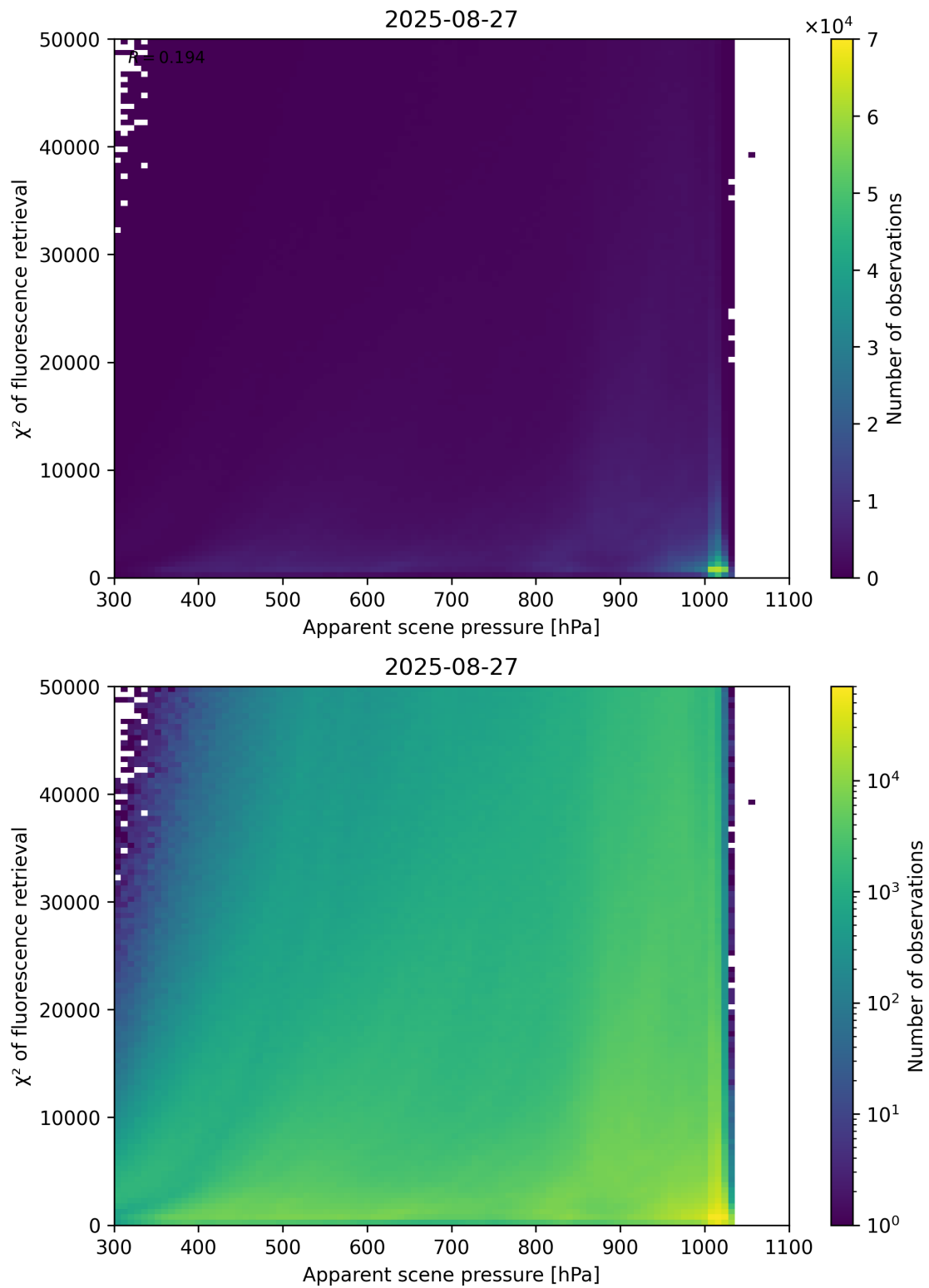
Figure 63: Scatter density plot of “Apparent scene pressure” against “ \chi^2 of fluorescence retrieval” for 2025-08-26 to 2025-08-28.
