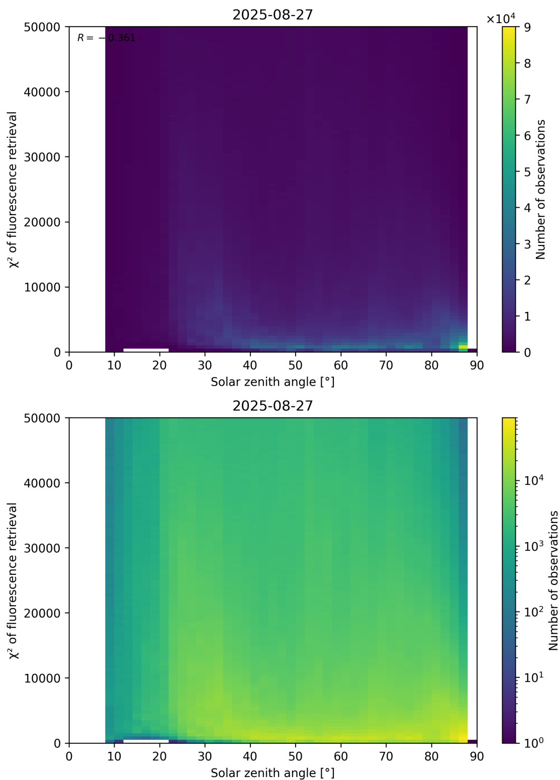
Figure 109: Scatter density plot of “Solar zenith angle” against “ \chi^2 of fluorescence retrieval” for 2025-08-26 to 2025-08-28.
