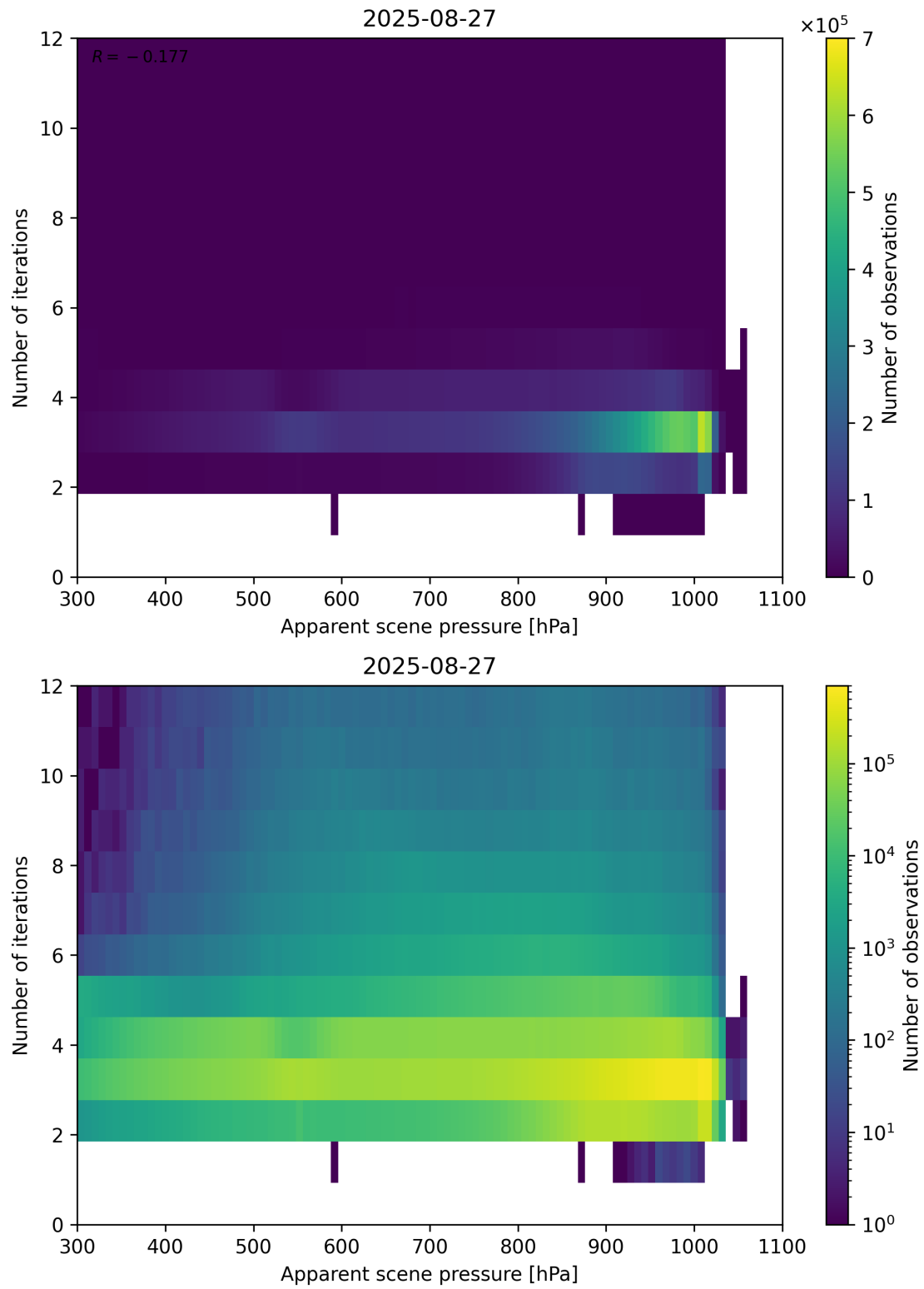
Figure 65: Scatter density plot of “Apparent scene pressure” against “Number of iterations” for 2025-08-26 to 2025-08-28.
