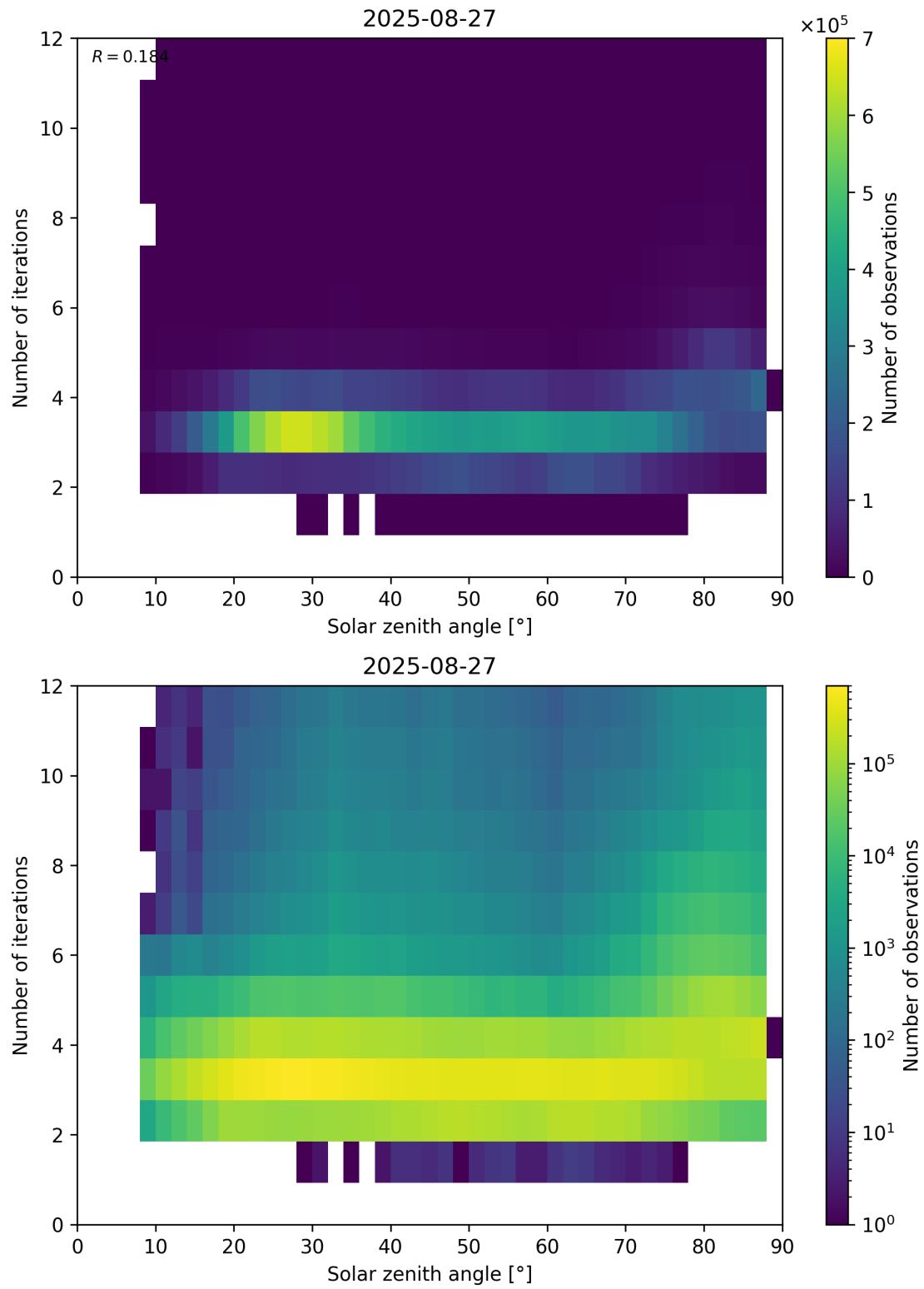
Figure 114: Scatter density plot of “Solar zenith angle” against “Number of iterations” for 2025-08-26 to 2025-08-28.
