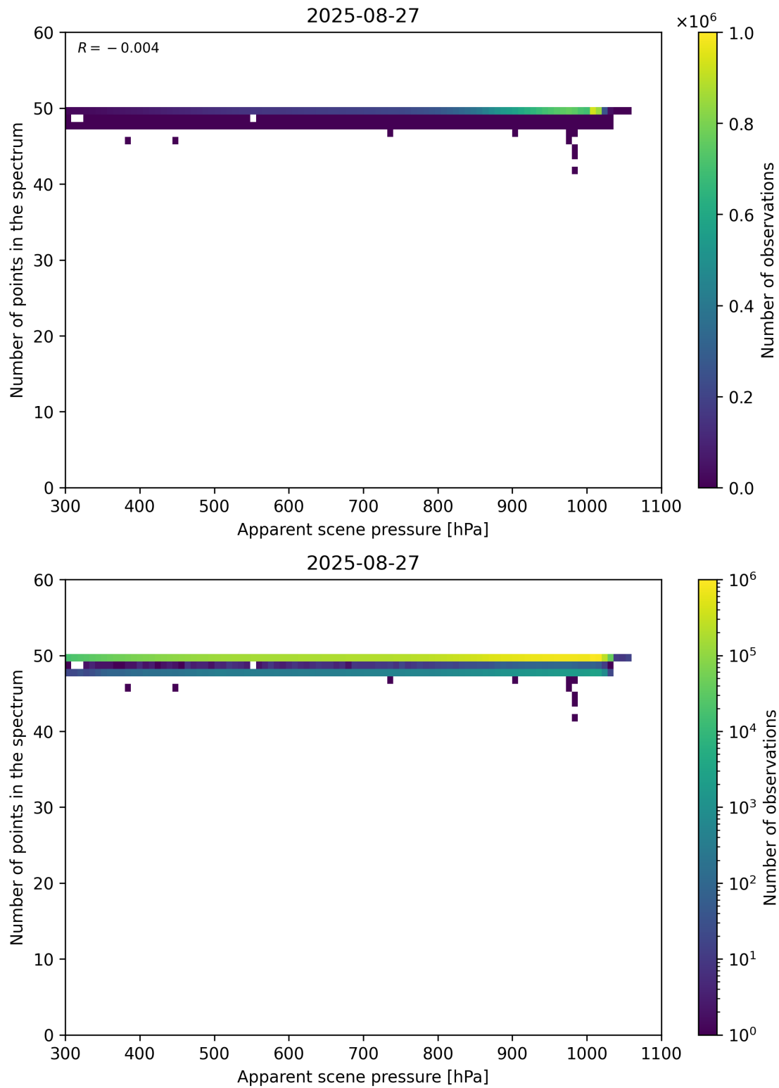
Figure 66: Scatter density plot of “Apparent scene pressure” against “Number of points in the spectrum” for 2025-08-26 to 2025-08-28.
