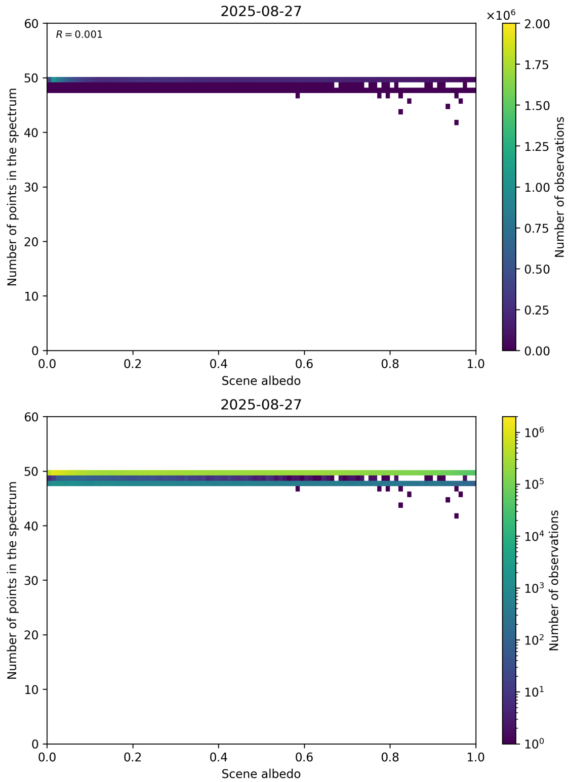
Figure 106: Scatter density plot of “Scene albedo” against “Number of points in the spectrum” for 2025-08-26 to 2025-08-28.
