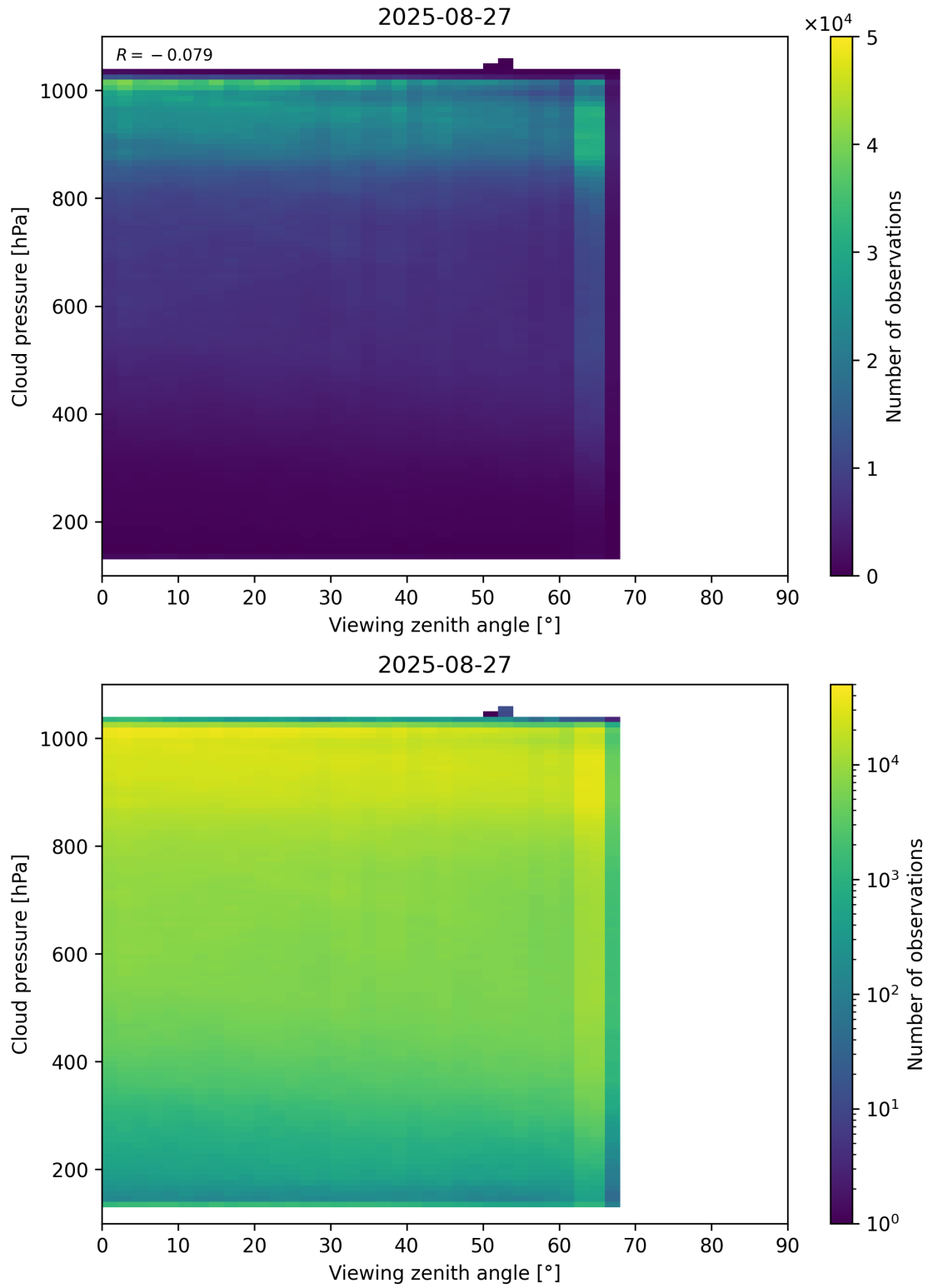
Figure 121: Scatter density plot of “Viewing zenith angle” against “Cloud pressure” for 2025-08-26 to 2025-08-28.
