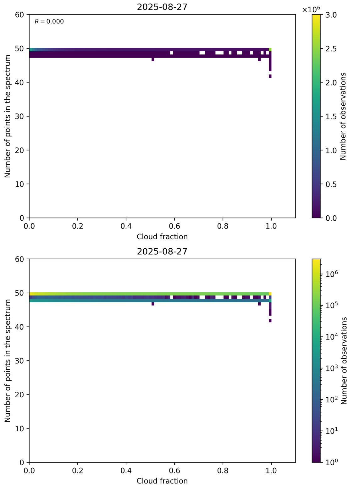
Figure 74: Scatter density plot of “Cloud fraction” against “Number of points in the spectrum” for 2025-08-26 to 2025-08-28.
