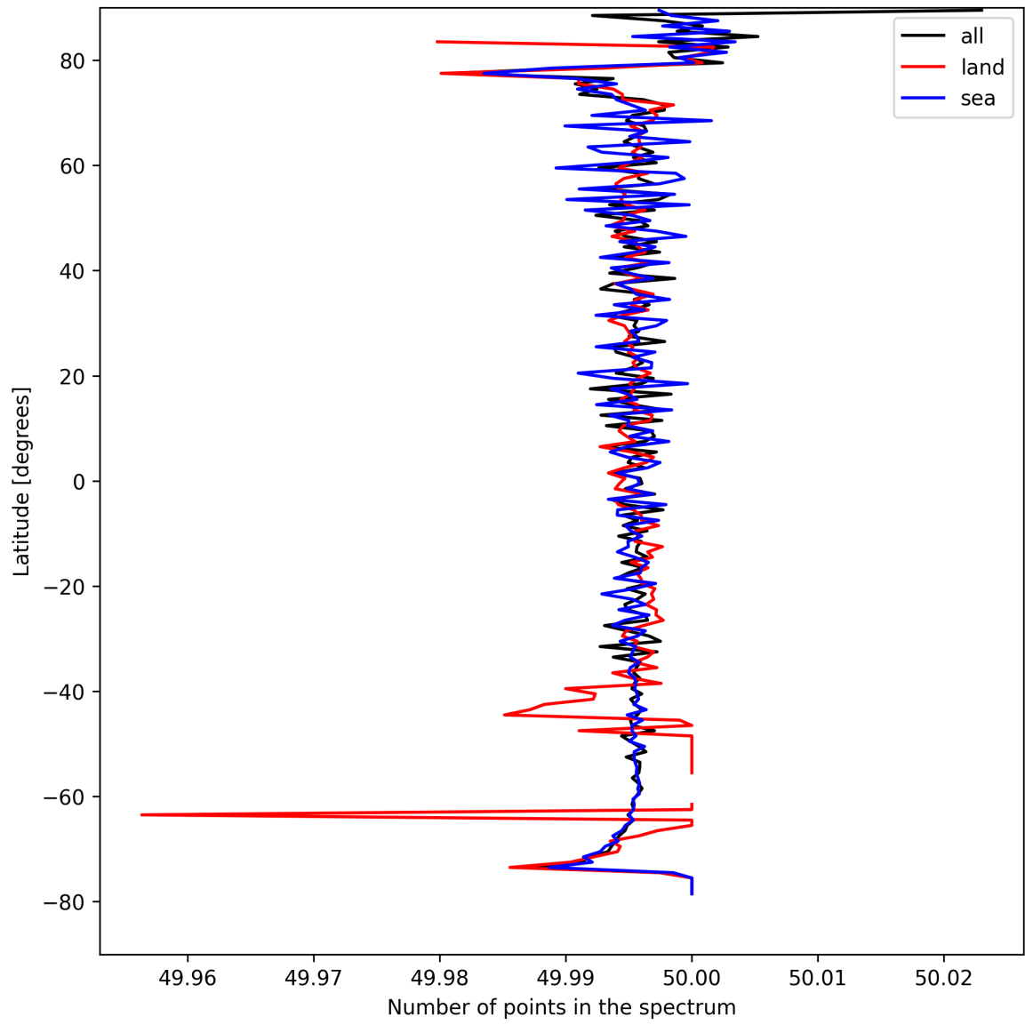
Figure 27: Zonal average of “Number of points in the spectrum” for 2025-08-26 to 2025-08-28.
