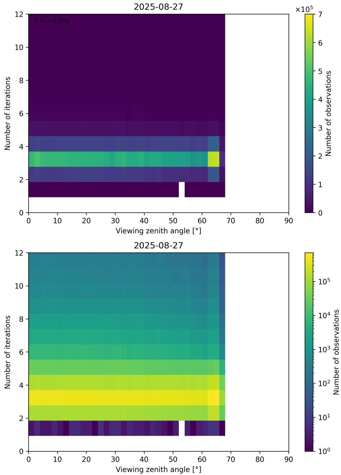
Figure 124: Scatter density plot of “Viewing zenith angle” against “Number of iterations” for 2025-08-26 to 2025-08-28.
