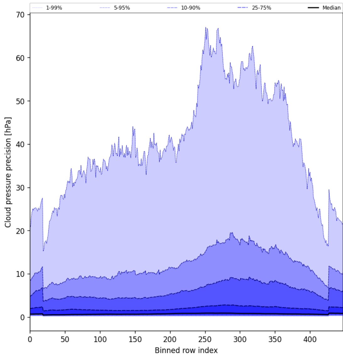
Figure 48: Along track statistics of “Cloud pressure precision” for 2025-08-26 to 2025-08-28
