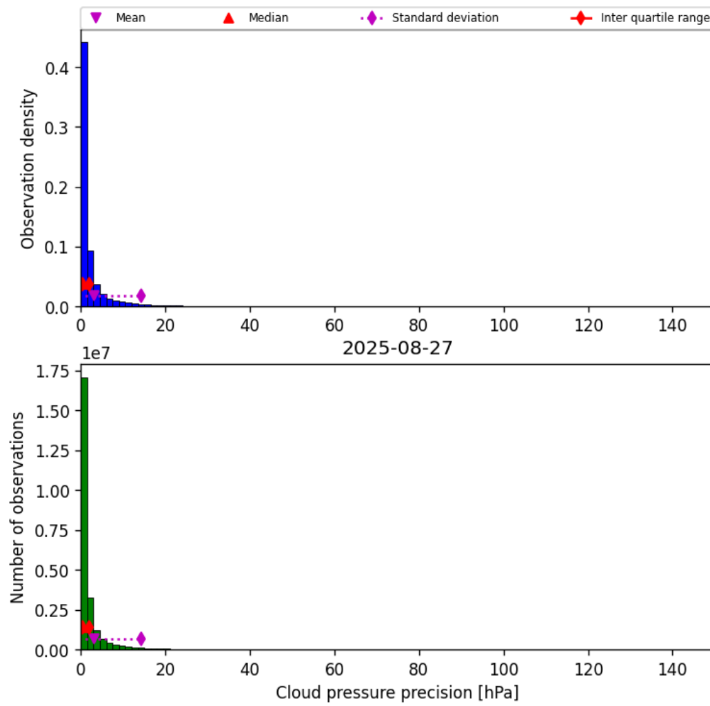
Figure 31: Histogram of “Cloud pressure precision” for 2025-08-26 to 2025-08-28
