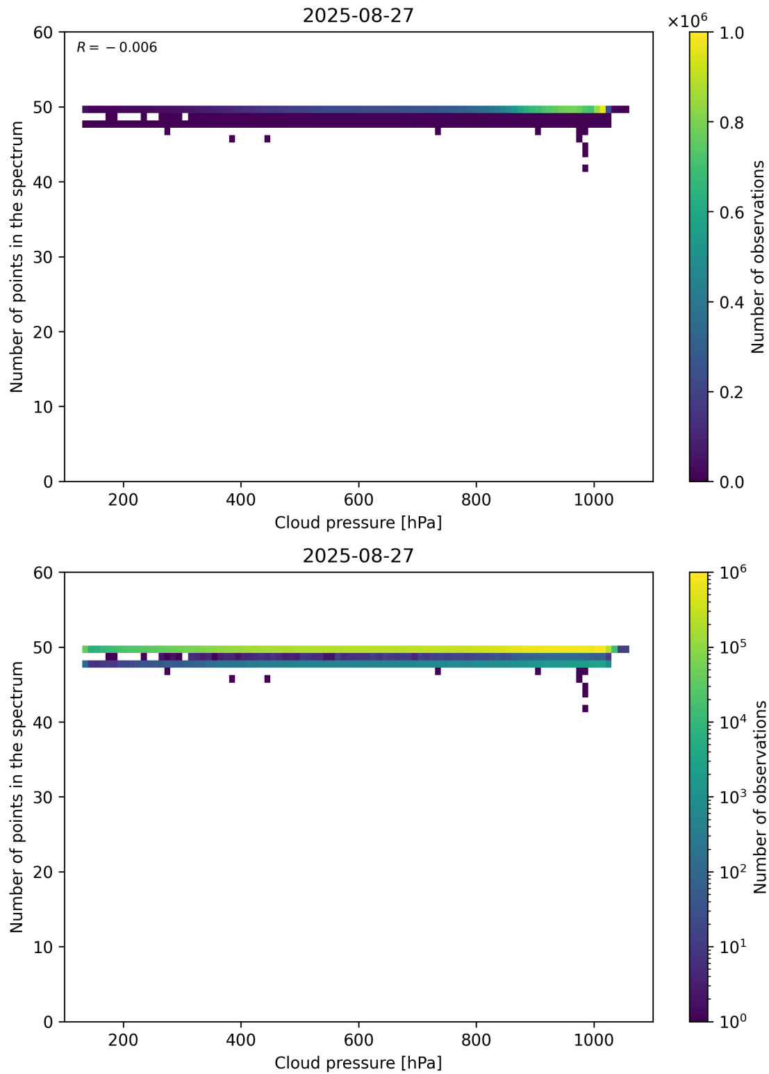
Figure 82: Scatter density plot of “Cloud pressure” against “Number of points in the spectrum” for 2025-08-26 to 2025-08-28.
