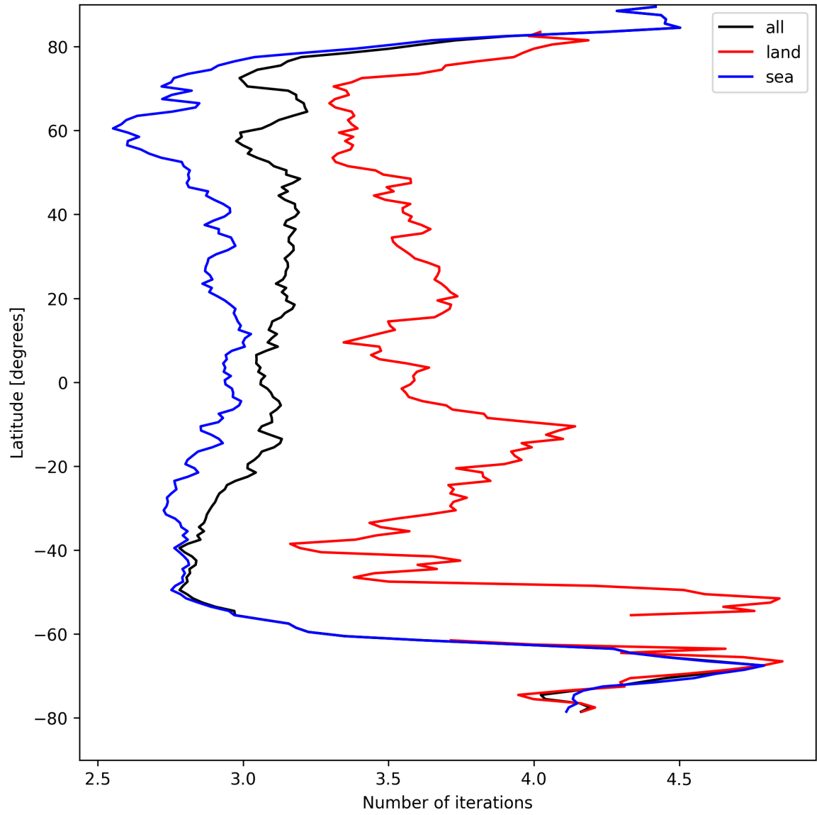
Figure 22: Zonal average of “Number of iterations” for 2025-08-26 to 2025-08-28.
