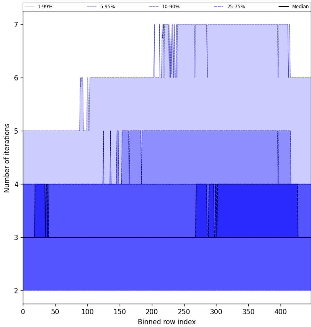
Figure 56: Along track statistics of “Number of iterations” for 2025-08-26 to 2025-08-28
