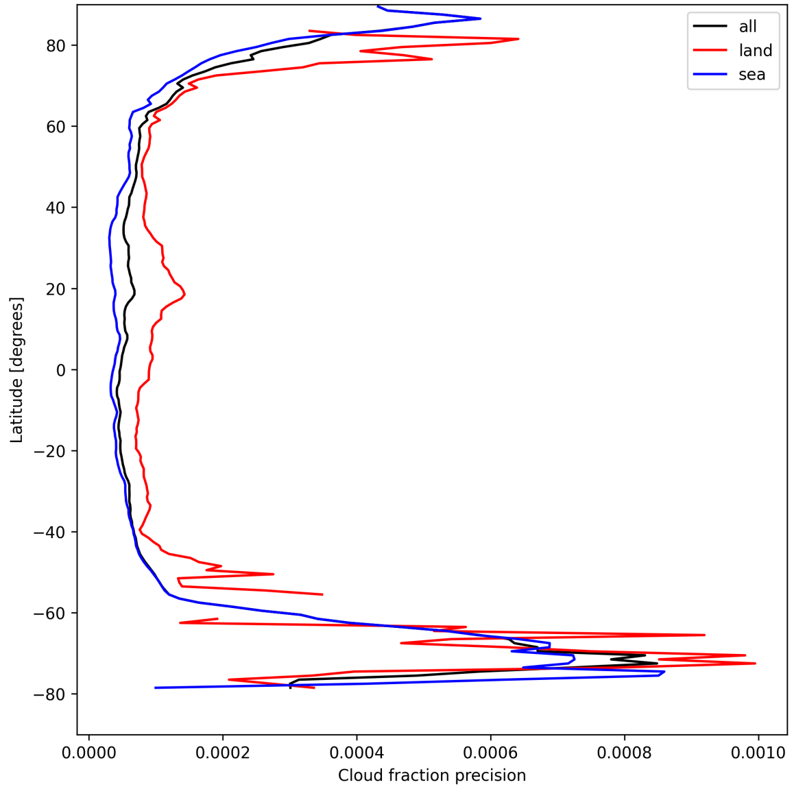
Figure 16: Zonal average of “Cloud fraction precision” for 2025-08-26 to 2025-08-28.
