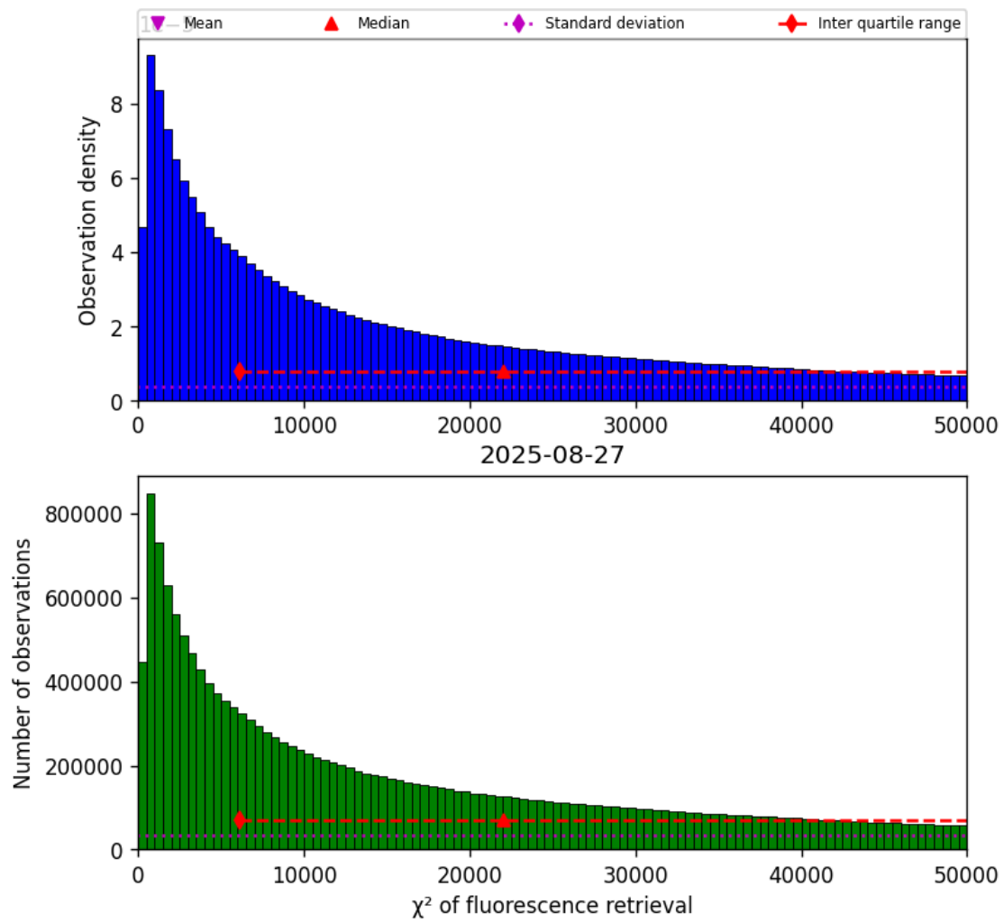
Figure 42: Histogram of “ \chi^2 of fluorescence retrieval” for 2025-08-26 to 2025-08-28
