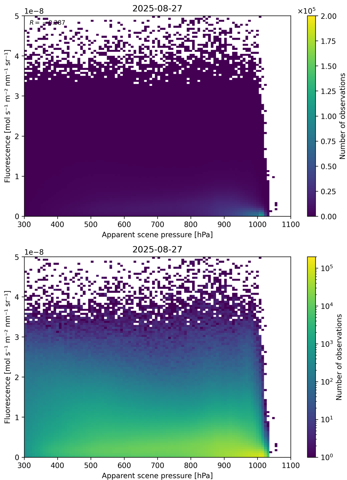
Figure 64: Scatter density plot of “Apparent scene pressure” against “Fluorescence” for 2025-08-26 to 2025-08-28.
