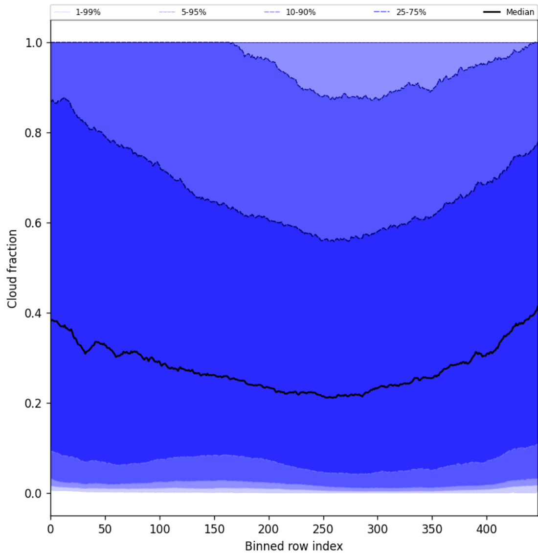
Figure 49: Along track statistics of “Cloud fraction” for 2025-08-26 to 2025-08-28
