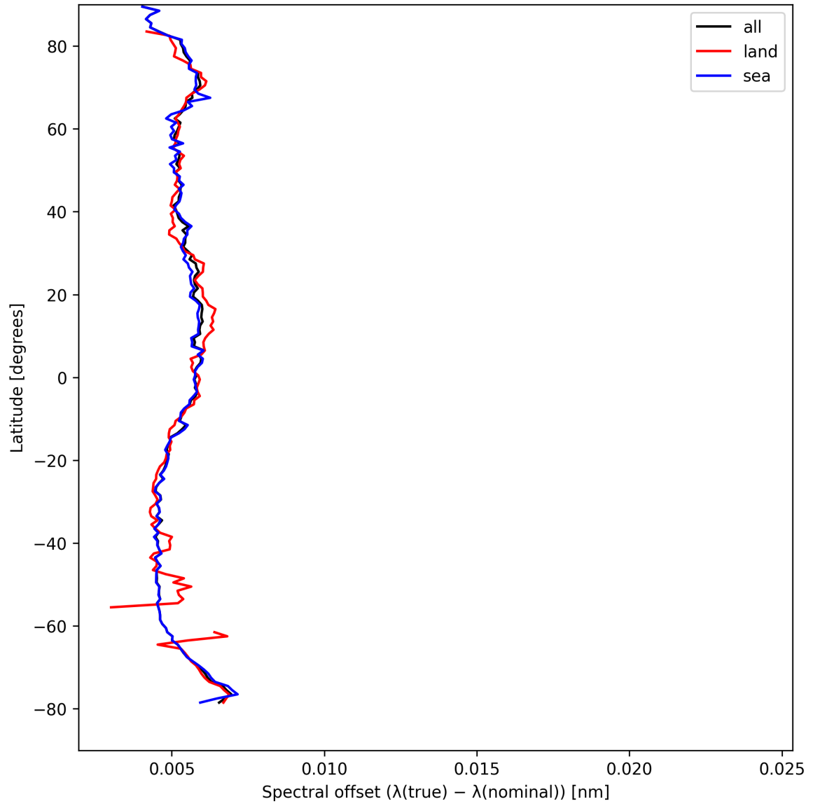
Figure 28: Zonal average of “Spectral offset ( \lambda_{\text{true}} - \lambda_{\text{nominal}} )” for 2025-08-26 to 2025-08-28.
