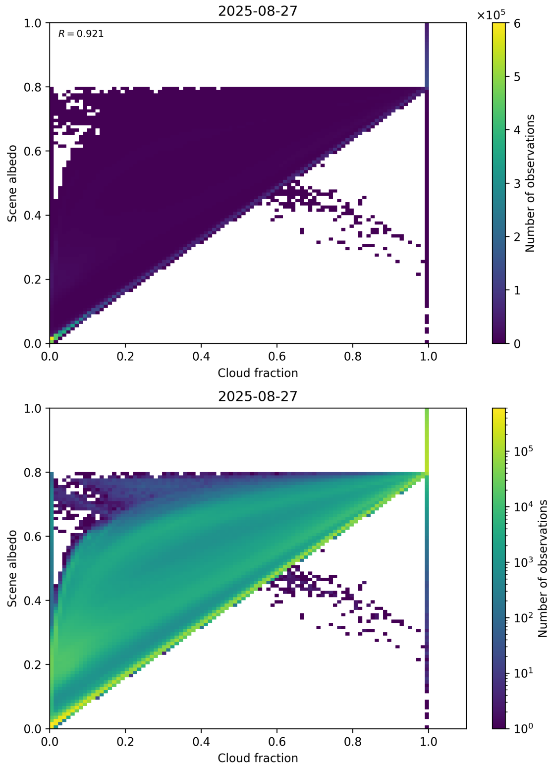
Figure 75: Scatter density plot of “Cloud fraction” against “Scene albedo” for 2025-08-26 to 2025-08-28.
