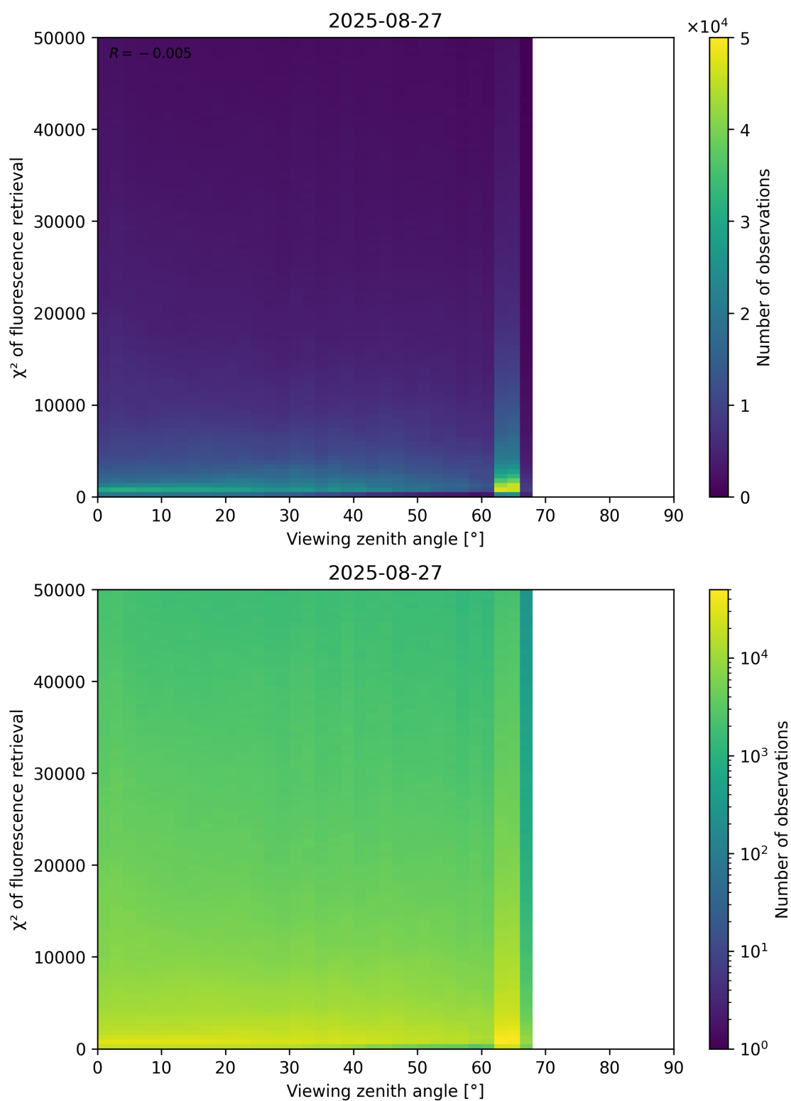
Figure 119: Scatter density plot of “Viewing zenith angle” against “ \chi^2 of fluorescence retrieval” for 2025-08-26 to 2025-08-28.
