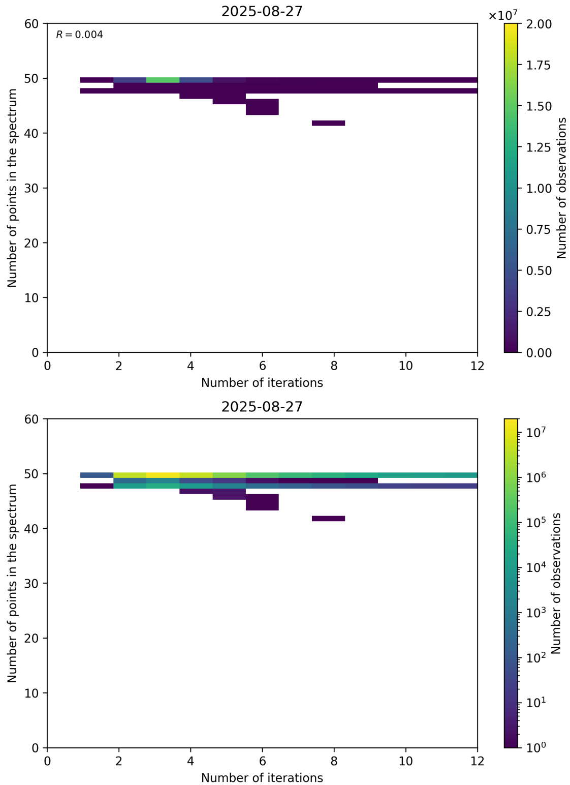
Figure 99: Scatter density plot of “Number of iterations” against “Number of points in the spectrum” for 2025-08-26 to 2025-08-28.
