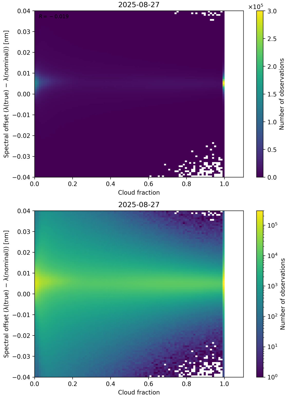
Figure 76: Scatter density plot of “Cloud fraction” against “Spectral offset ( \lambda_{\text{true}} - \lambda_{\text{nominal}} )” for 2025-08-26 to 2025-08-28.
