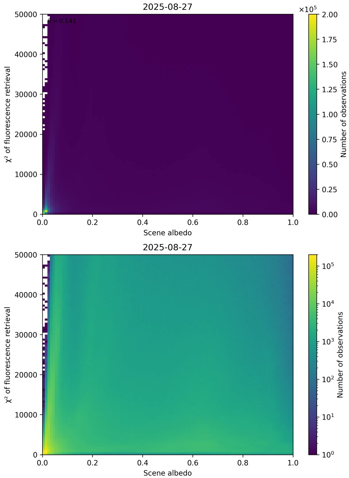
Figure 103: Scatter density plot of “Scene albedo” against “ \chi^2 of fluorescence retrieval” for 2025-08-26 to 2025-08-28.
