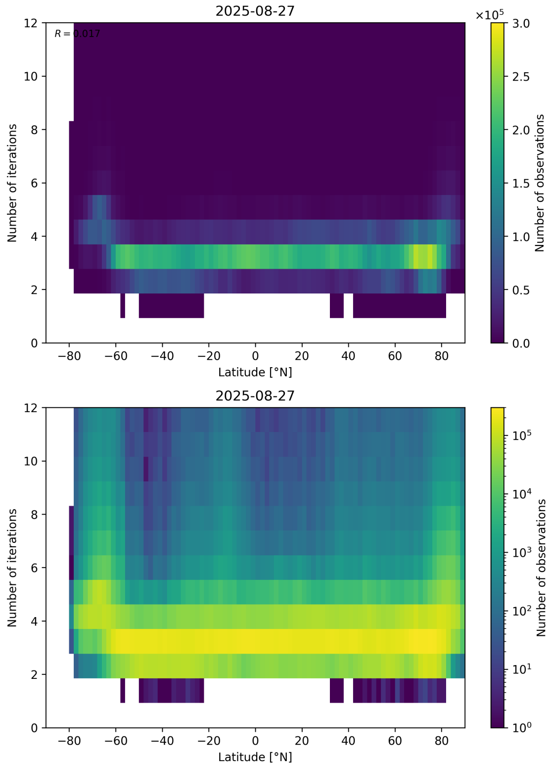
Figure 93: Scatter density plot of “Latitude” against “Number of iterations” for 2025-08-26 to 2025-08-28.
