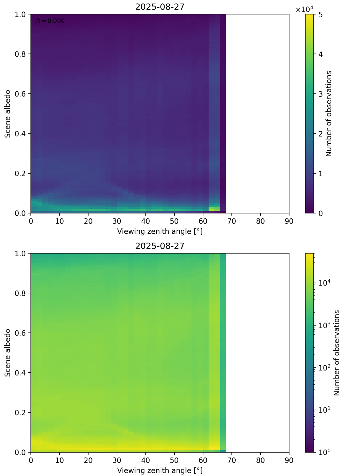
Figure 126: Scatter density plot of “Viewing zenith angle” against “Scene albedo” for 2025-08-26 to 2025-08-28.
