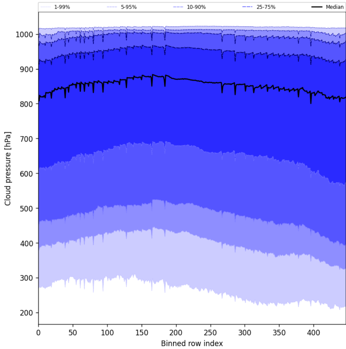
Figure 47: Along track statistics of “Cloud pressure” for 2025-08-26 to 2025-08-28
