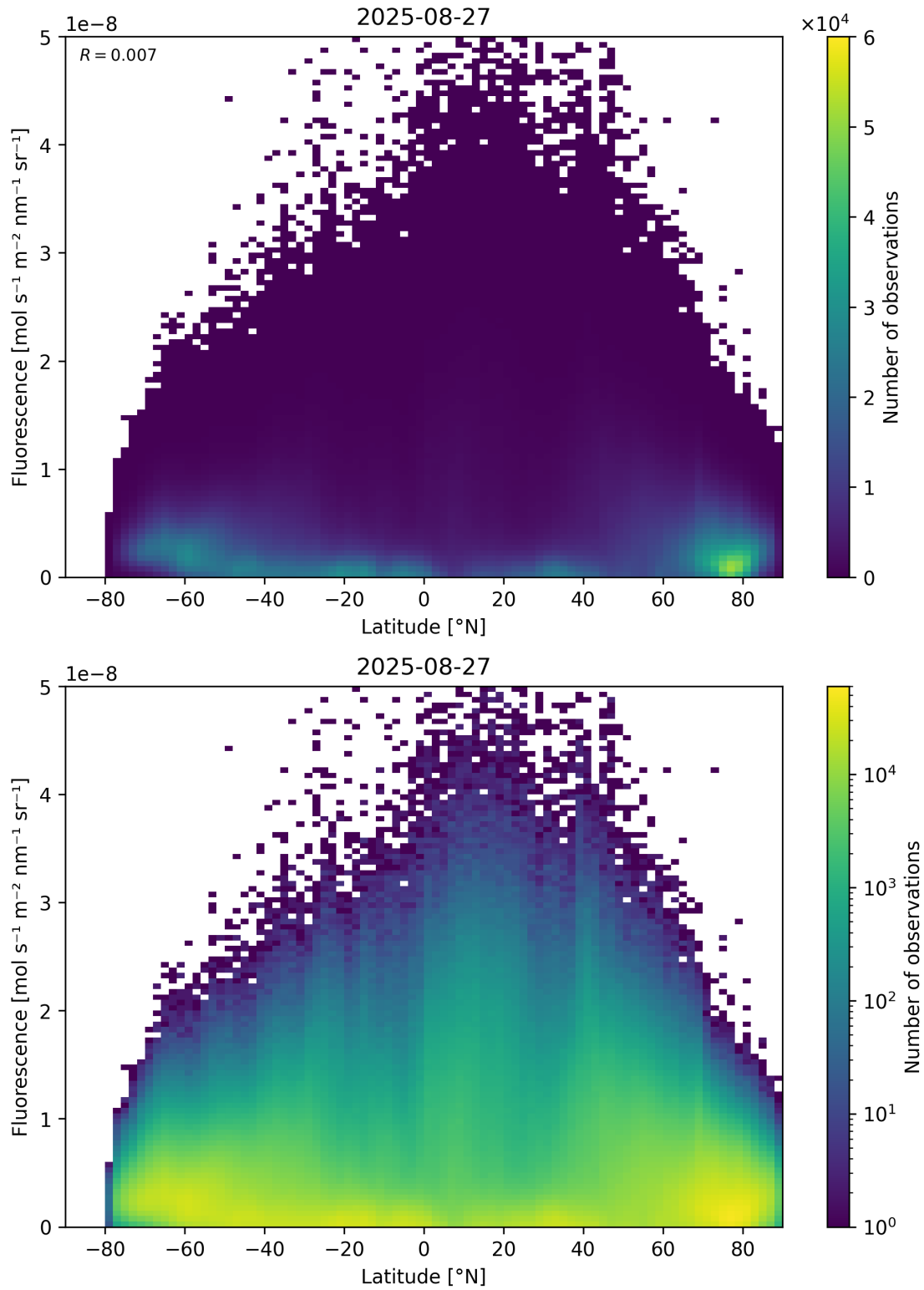
Figure 92: Scatter density plot of “Latitude” against “Fluorescence” for 2025-08-26 to 2025-08-28.
