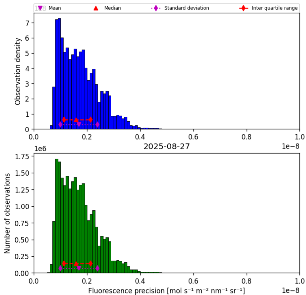
Figure 41: Histogram of “Fluorescence precision” for 2025-08-26 to 2025-08-28
