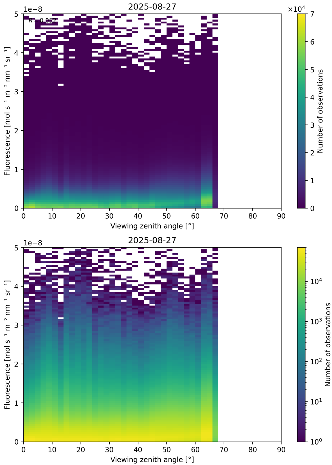
Figure 122: Scatter density plot of “Viewing zenith angle” against “Fluorescence” for 2025-08-26 to 2025-08-28.
