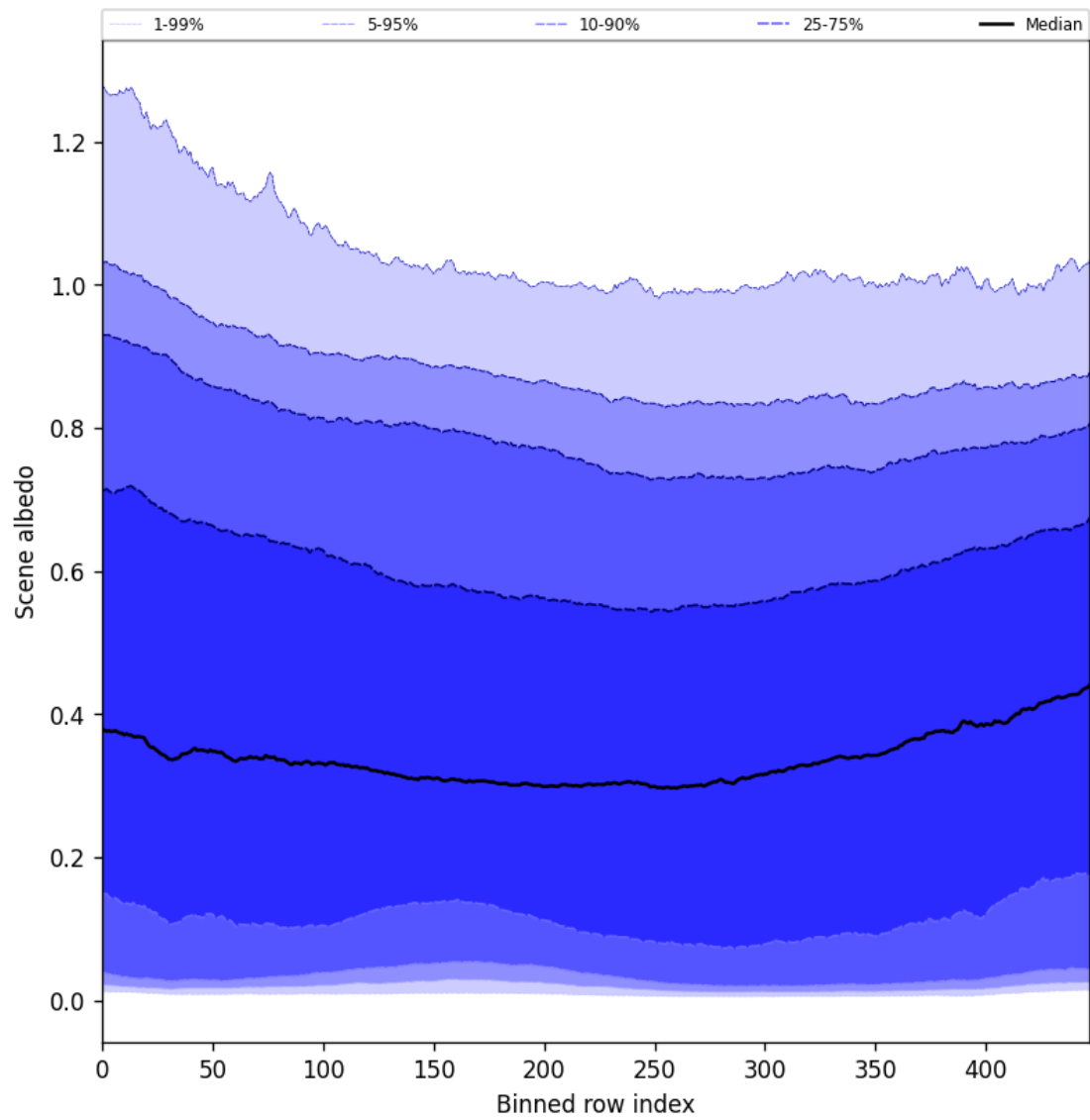
Figure 51: Along track statistics of “Scene albedo” for 2025-08-26 to 2025-08-28
