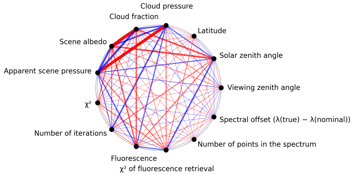
Figure 1: Map of correlation graph for 2025-08-26 to 2025-08-28.
