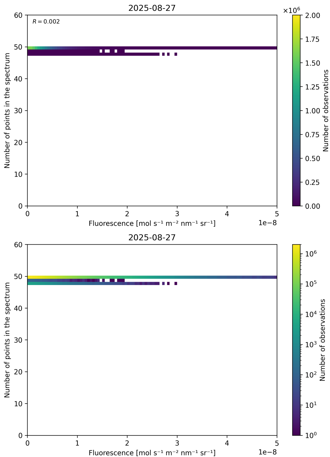
Figure 86: Scatter density plot of “Fluorescence” against “Number of points in the spectrum” for 2025-08-26 to 2025-08-28.
