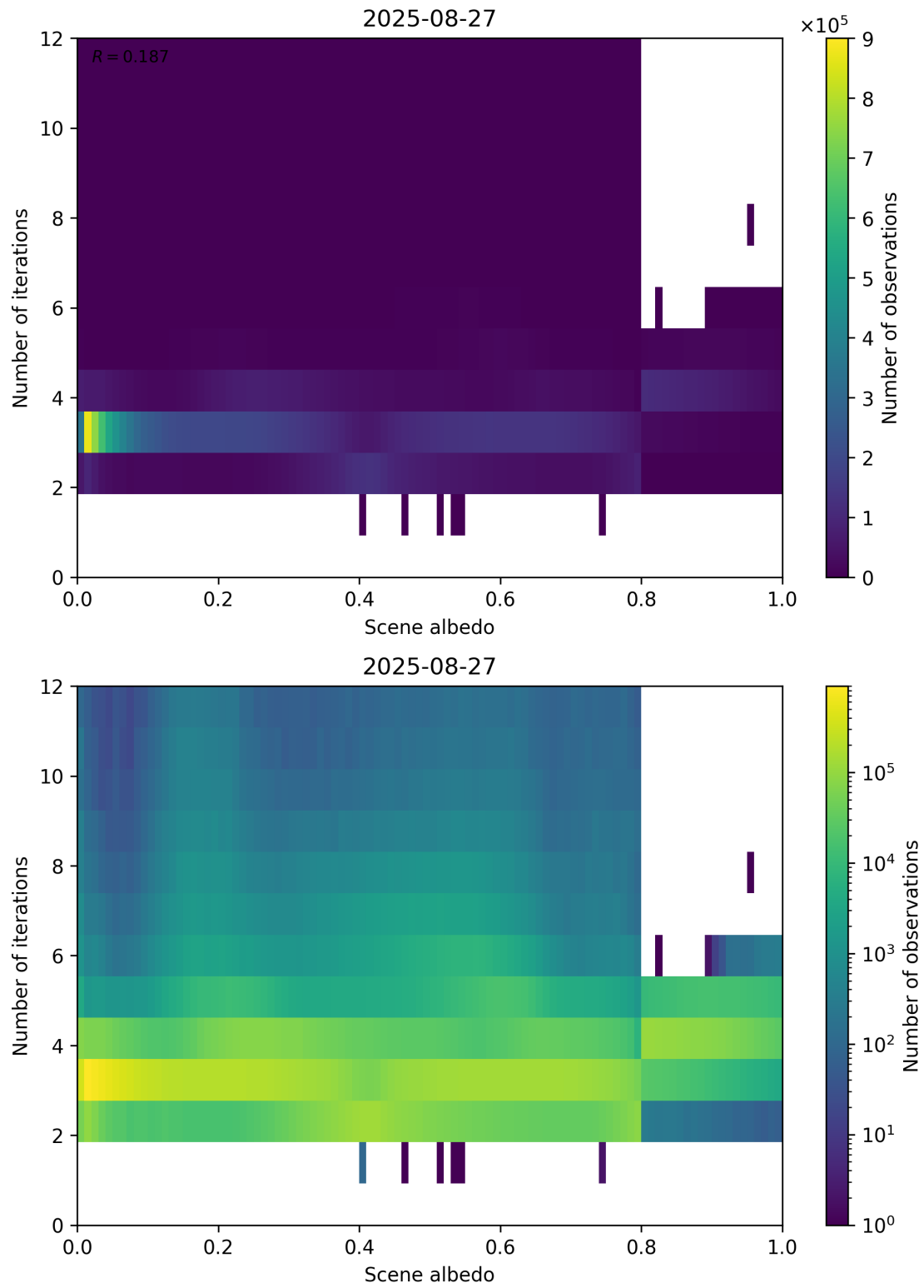
Figure 105: Scatter density plot of “Scene albedo” against “Number of iterations” for 2025-08-26 to 2025-08-28.
