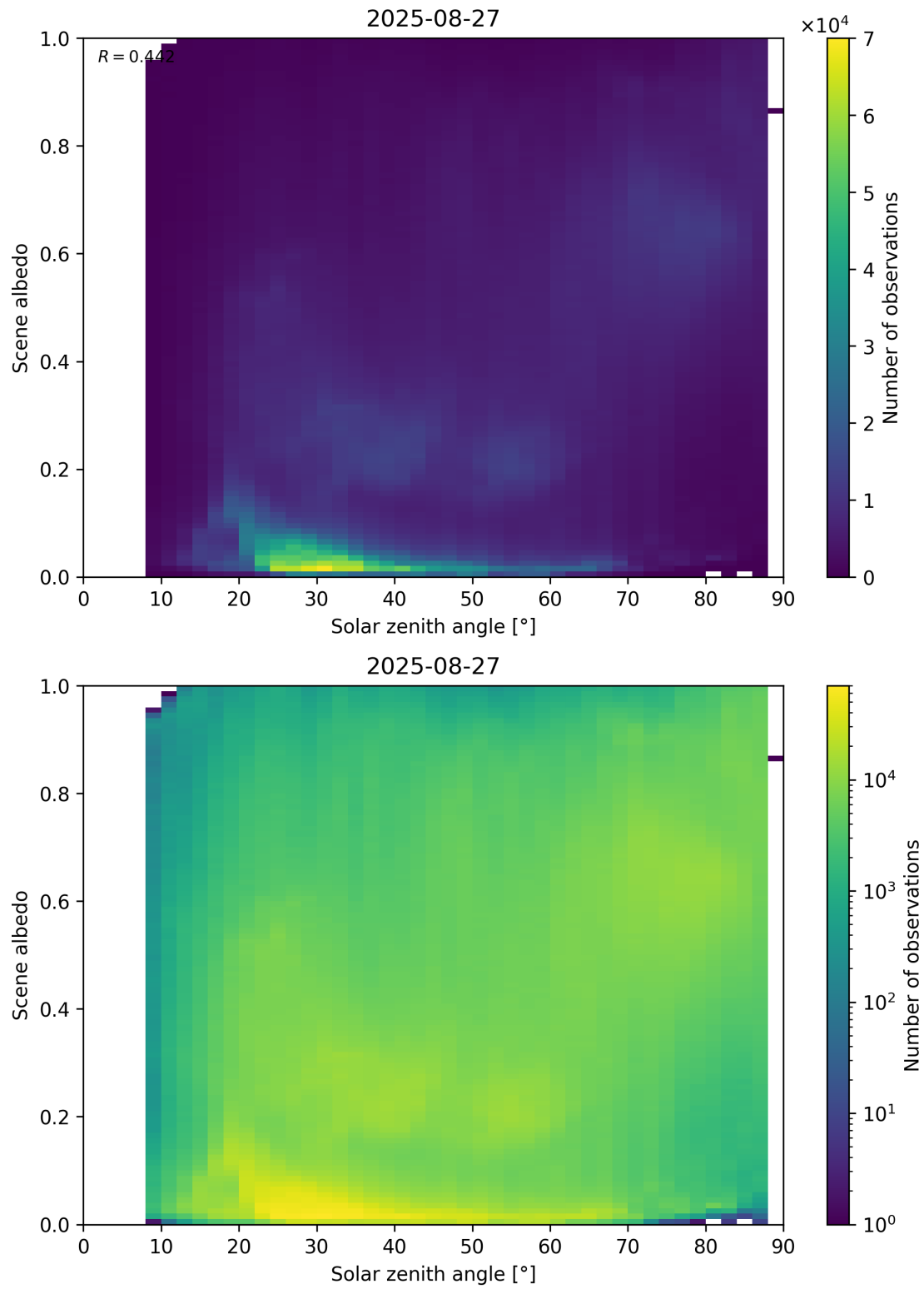
Figure 116: Scatter density plot of “Solar zenith angle” against “Scene albedo” for 2025-08-26 to 2025-08-28.
