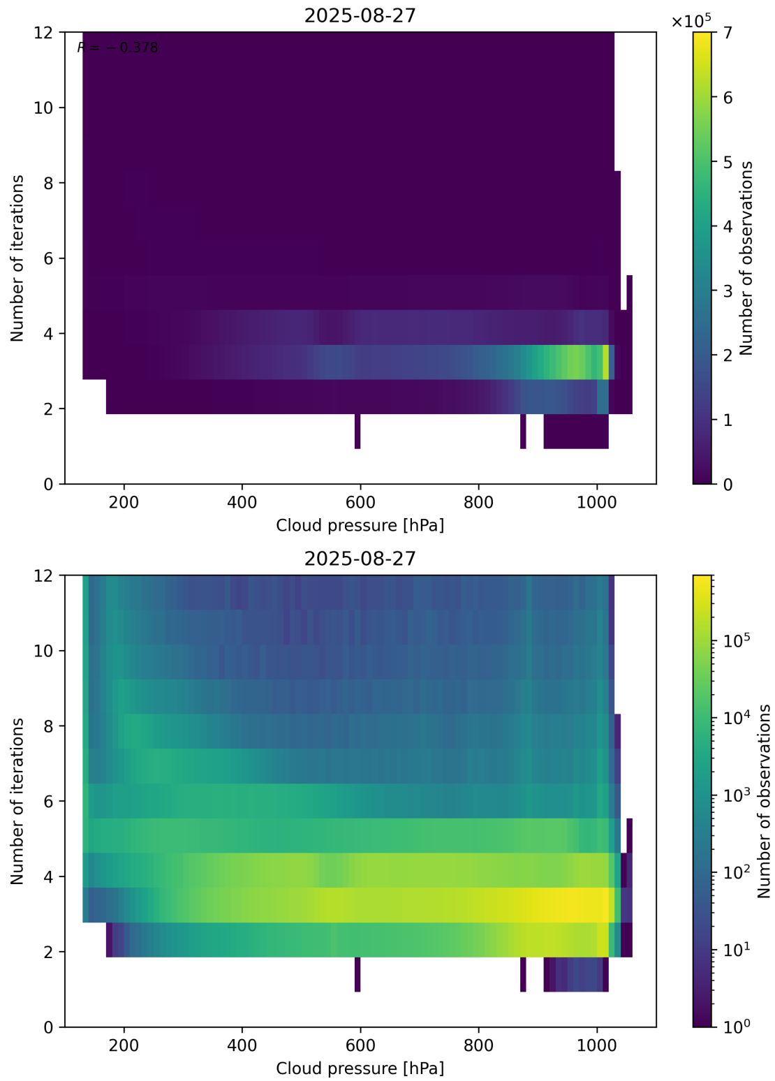
Figure 81: Scatter density plot of “Cloud pressure” against “Number of iterations” for 2025-08-26 to 2025-08-28.
