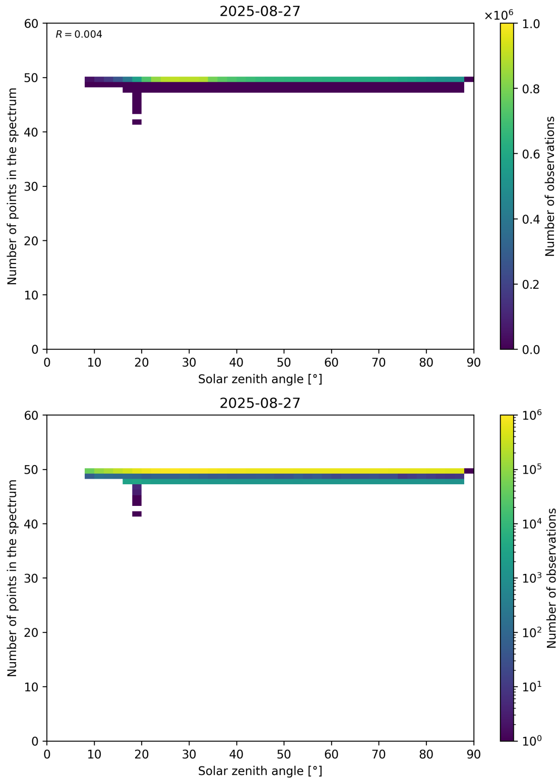
Figure 115: Scatter density plot of “Solar zenith angle” against “Number of points in the spectrum” for 2025-08-26 to 2025-08-28.
