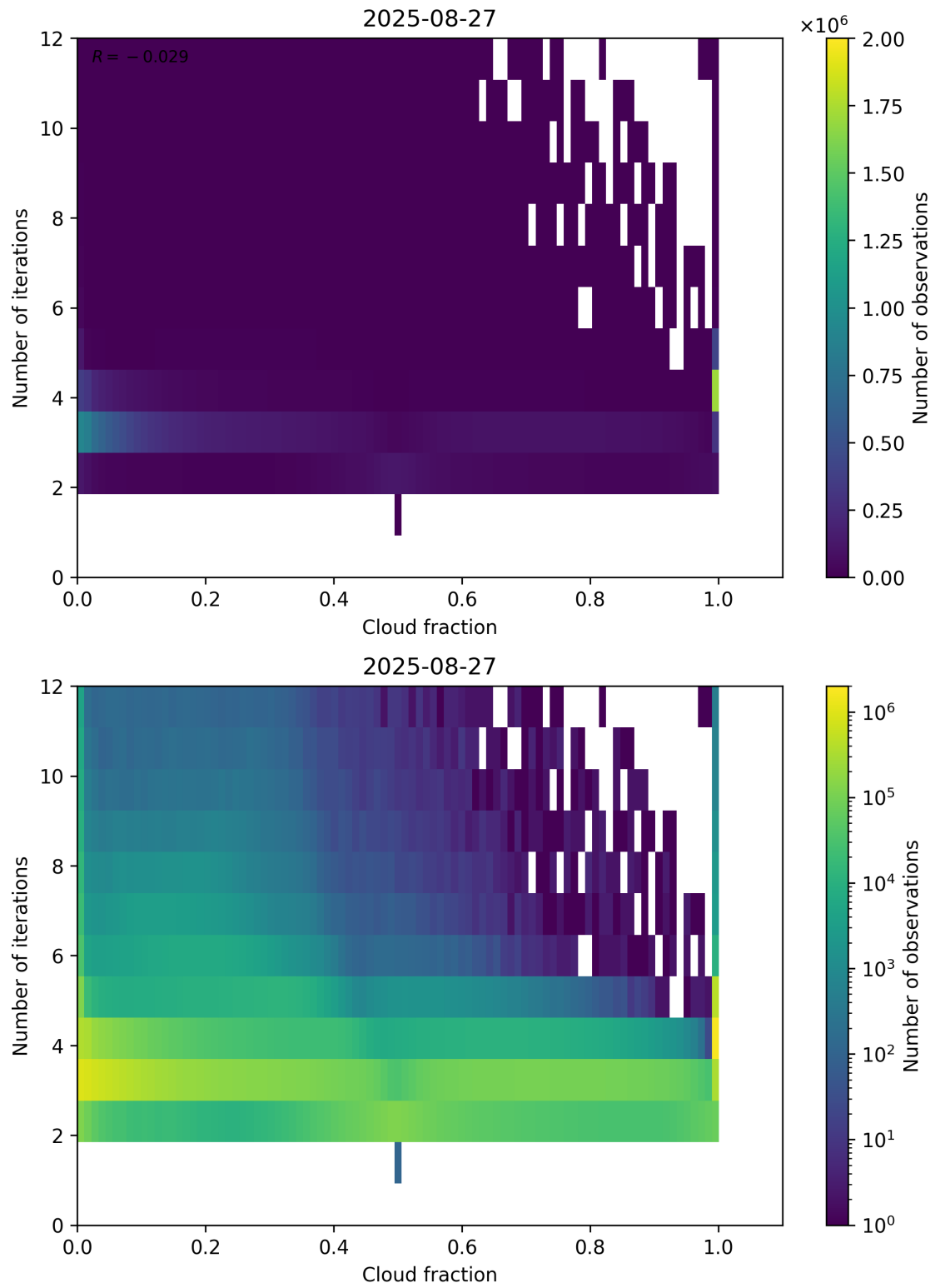
Figure 73: Scatter density plot of “Cloud fraction” against “Number of iterations” for 2025-08-26 to 2025-08-28.
