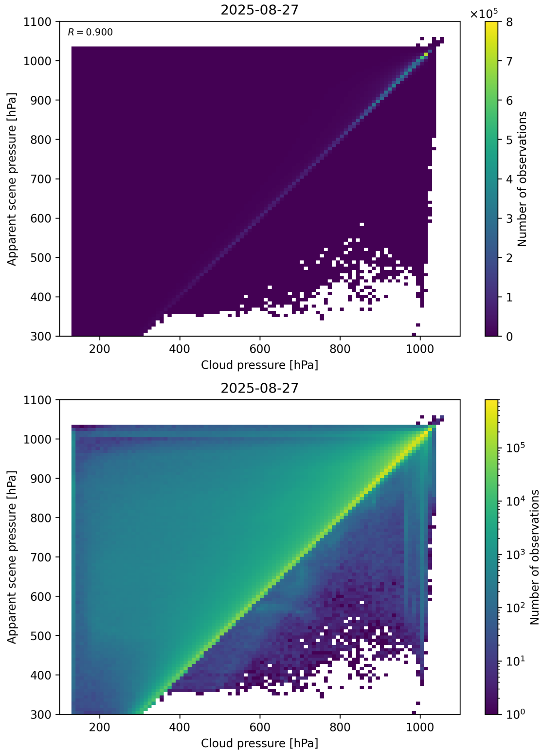
Figure 77: Scatter density plot of “Cloud pressure” against “Apparent scene pressure” for 2025-08-26 to 2025-08-28.
