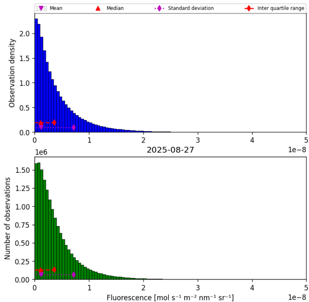
Figure 40: Histogram of “Fluorescence” for 2025-08-26 to 2025-08-28
