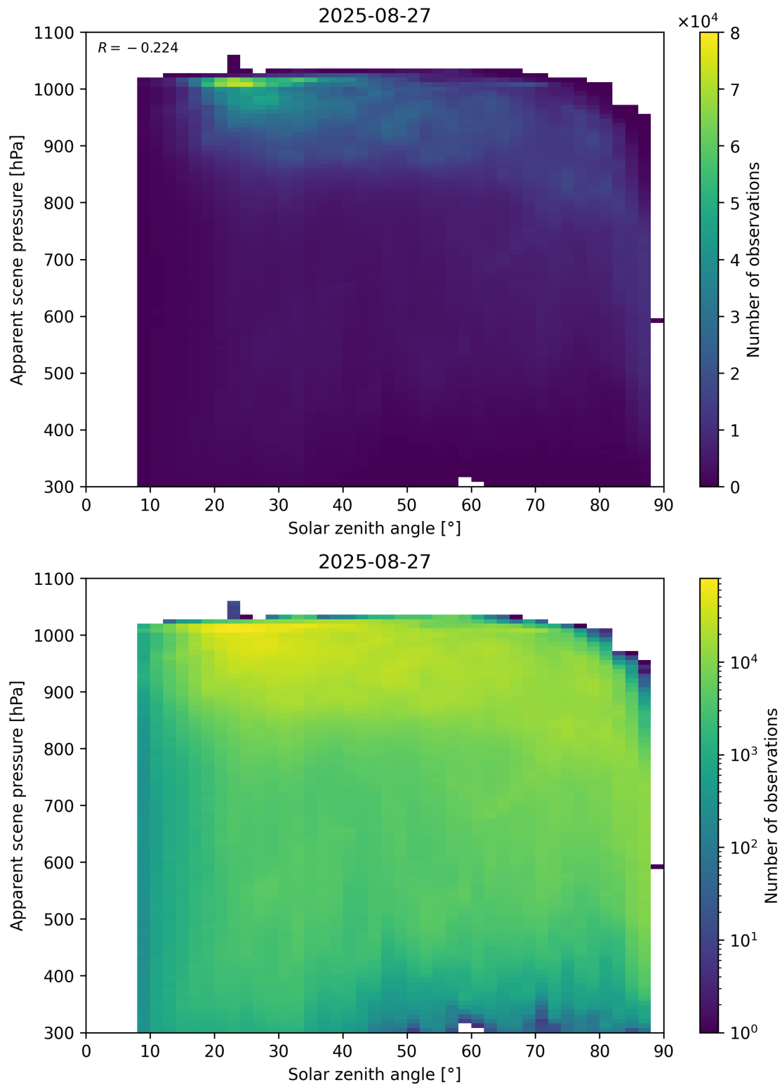
Figure 108: Scatter density plot of “Solar zenith angle” against “Apparent scene pressure” for 2025-08-26 to 2025-08-28.
