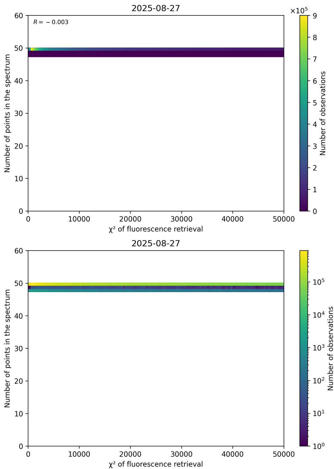
Figure 68: Scatter density plot of “ \chi^2 of fluorescence retrieval” against “Number of points in the spectrum” for 2025-08-26 to 2025-08-28.
