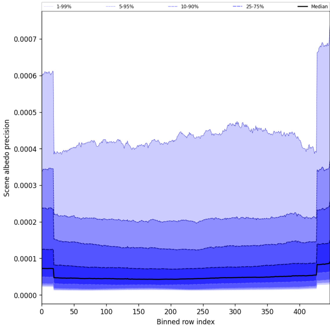
Figure 52: Along track statistics of “Scene albedo precision” for 2025-08-26 to 2025-08-28
