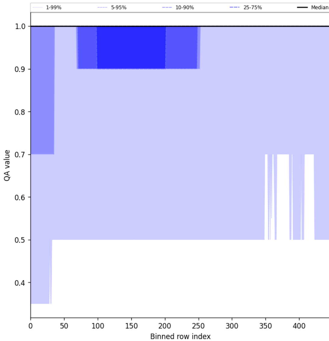
Figure 46: Along track statistics of “QA value” for 2025-08-26 to 2025-08-28
