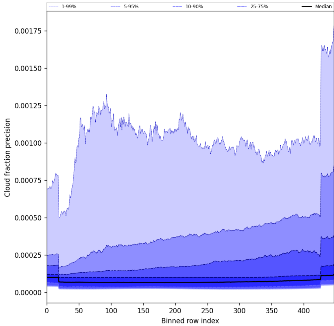
Figure 50: Along track statistics of “Cloud fraction precision” for 2025-08-26 to 2025-08-28
