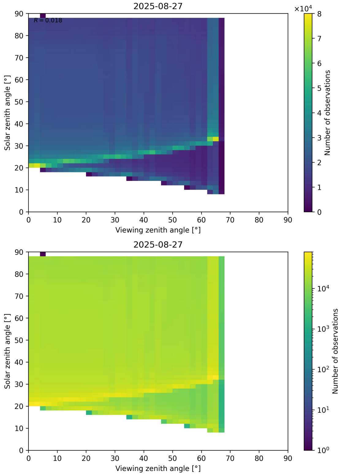
Figure 127: Scatter density plot of “Viewing zenith angle” against “Solar zenith angle” for 2025-08-26 to 2025-08-28.
