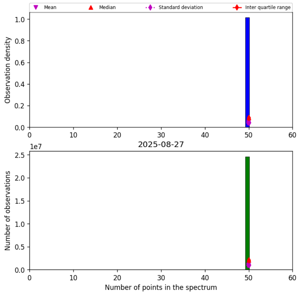
Figure 44: Histogram of “Number of points in the spectrum” for 2025-08-26 to 2025-08-28
