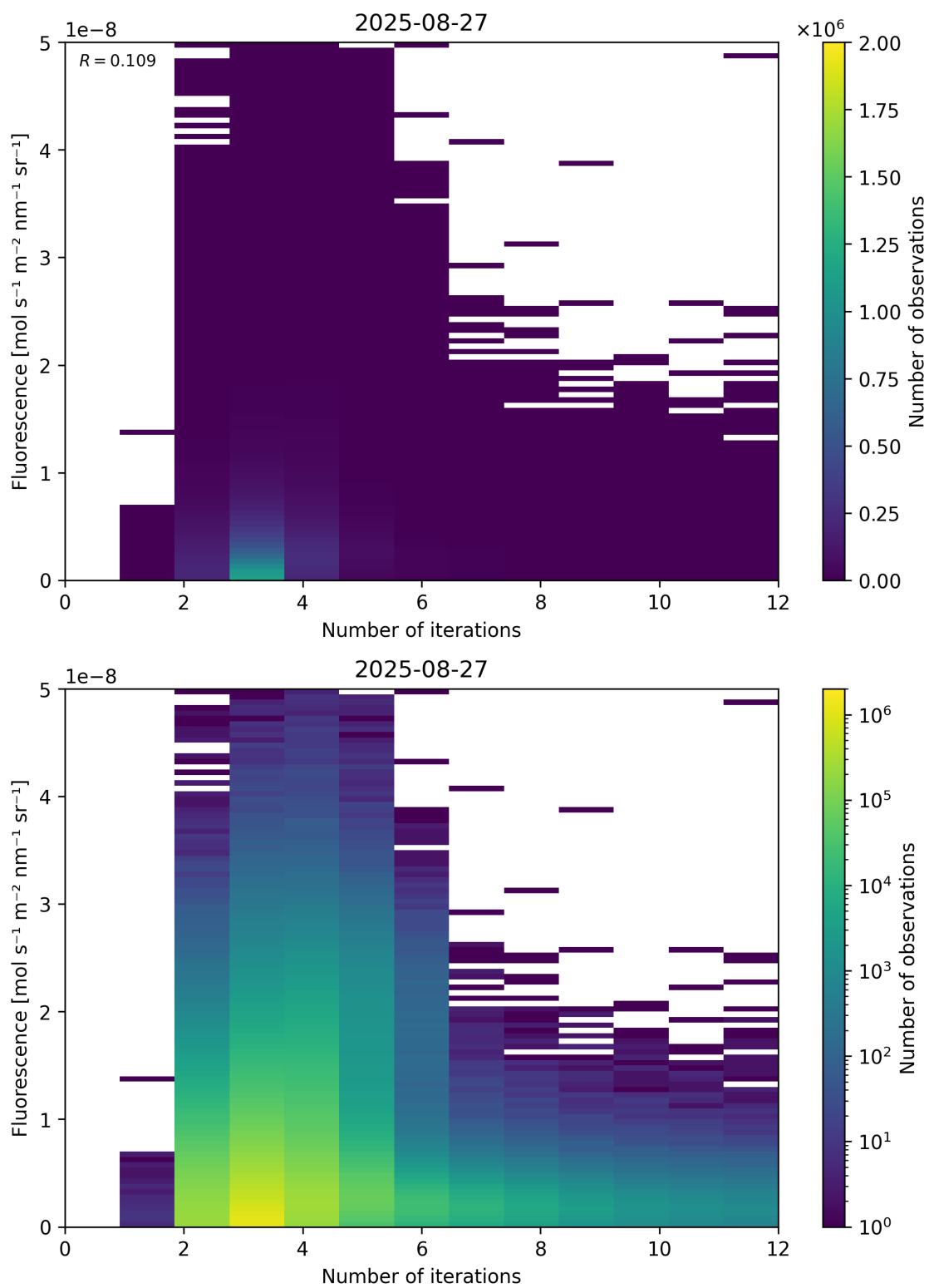
Figure 98: Scatter density plot of “Number of iterations” against “Fluorescence” for 2025-08-26 to 2025-08-28.
