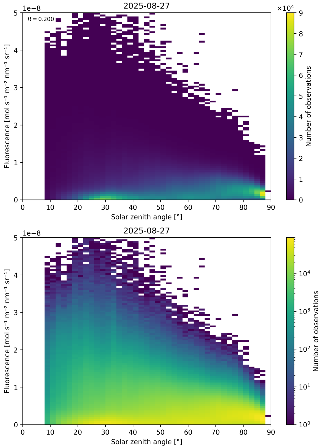
Figure 112: Scatter density plot of “Solar zenith angle” against “Fluorescence” for 2025-08-26 to 2025-08-28.
