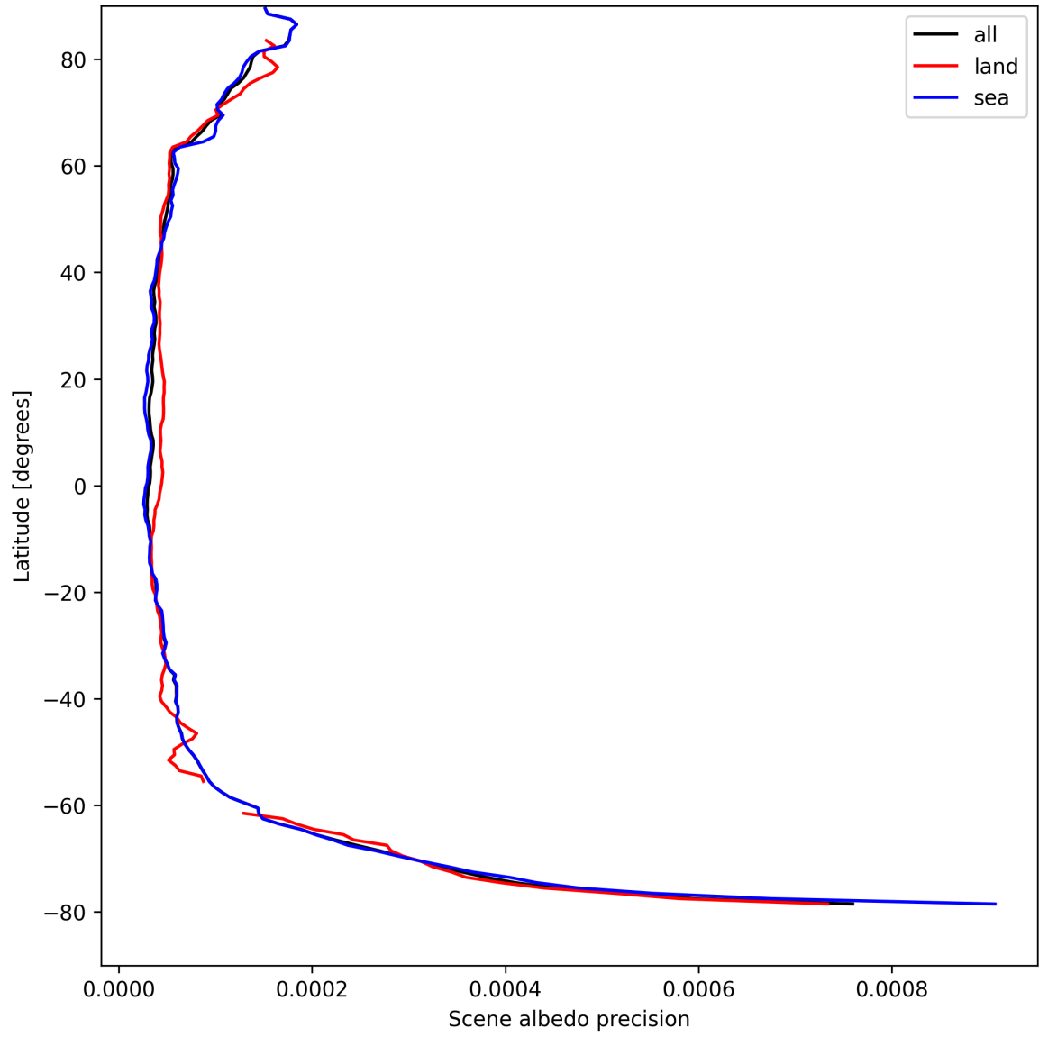
Figure 18: Zonal average of “Scene albedo precision” for 2025-08-26 to 2025-08-28.
