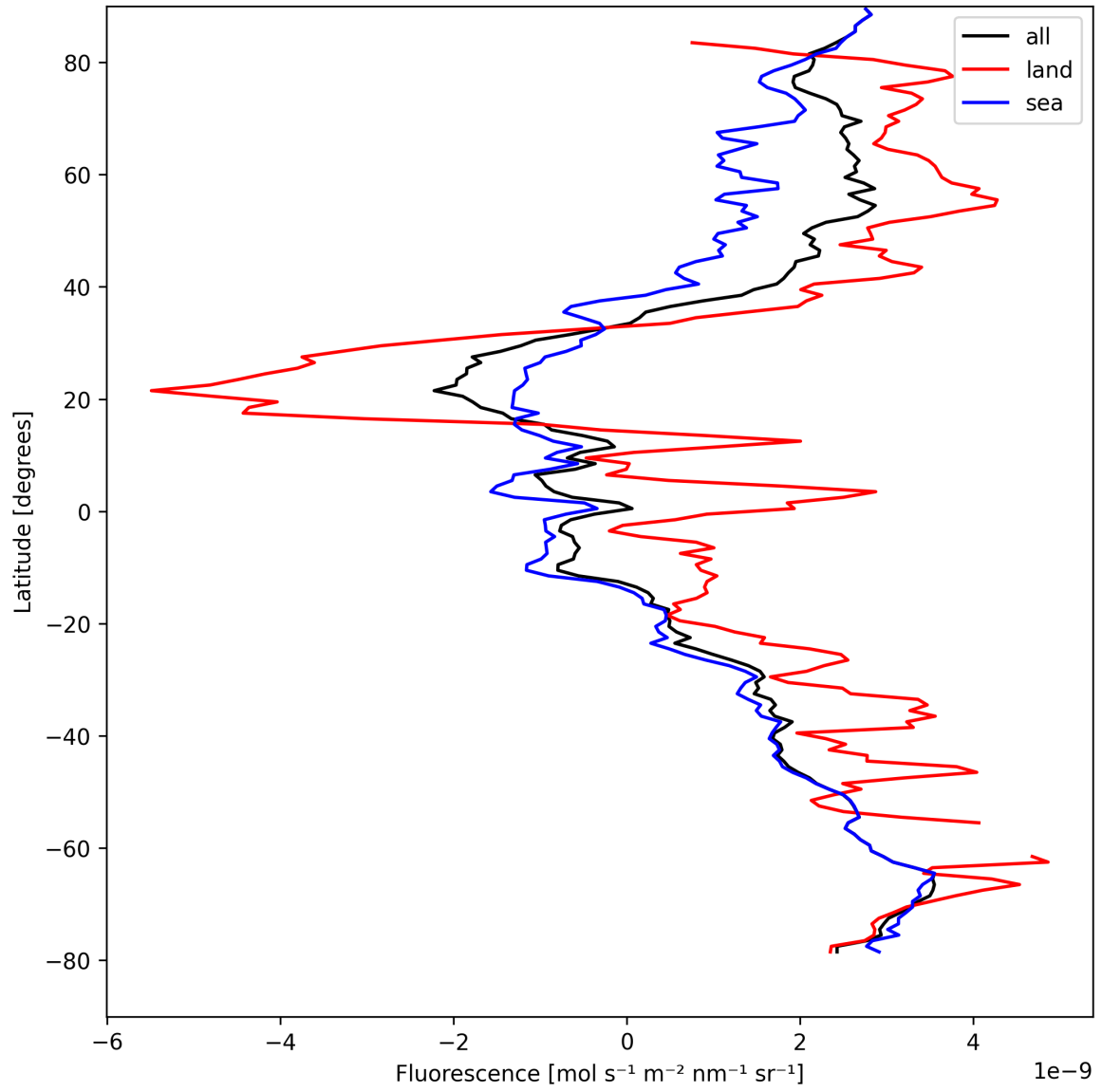
Figure 23: Zonal average of “Fluorescence” for 2025-08-26 to 2025-08-28.
