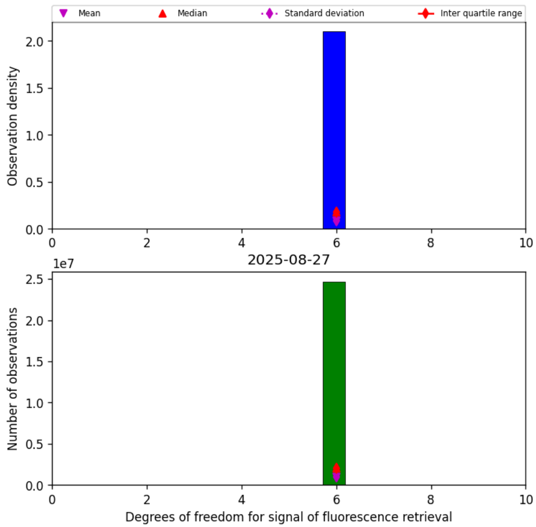
Figure 43: Histogram of “Degrees of freedom for signal of fluorescence retrieval” for 2025-08-26 to 2025-08-28
