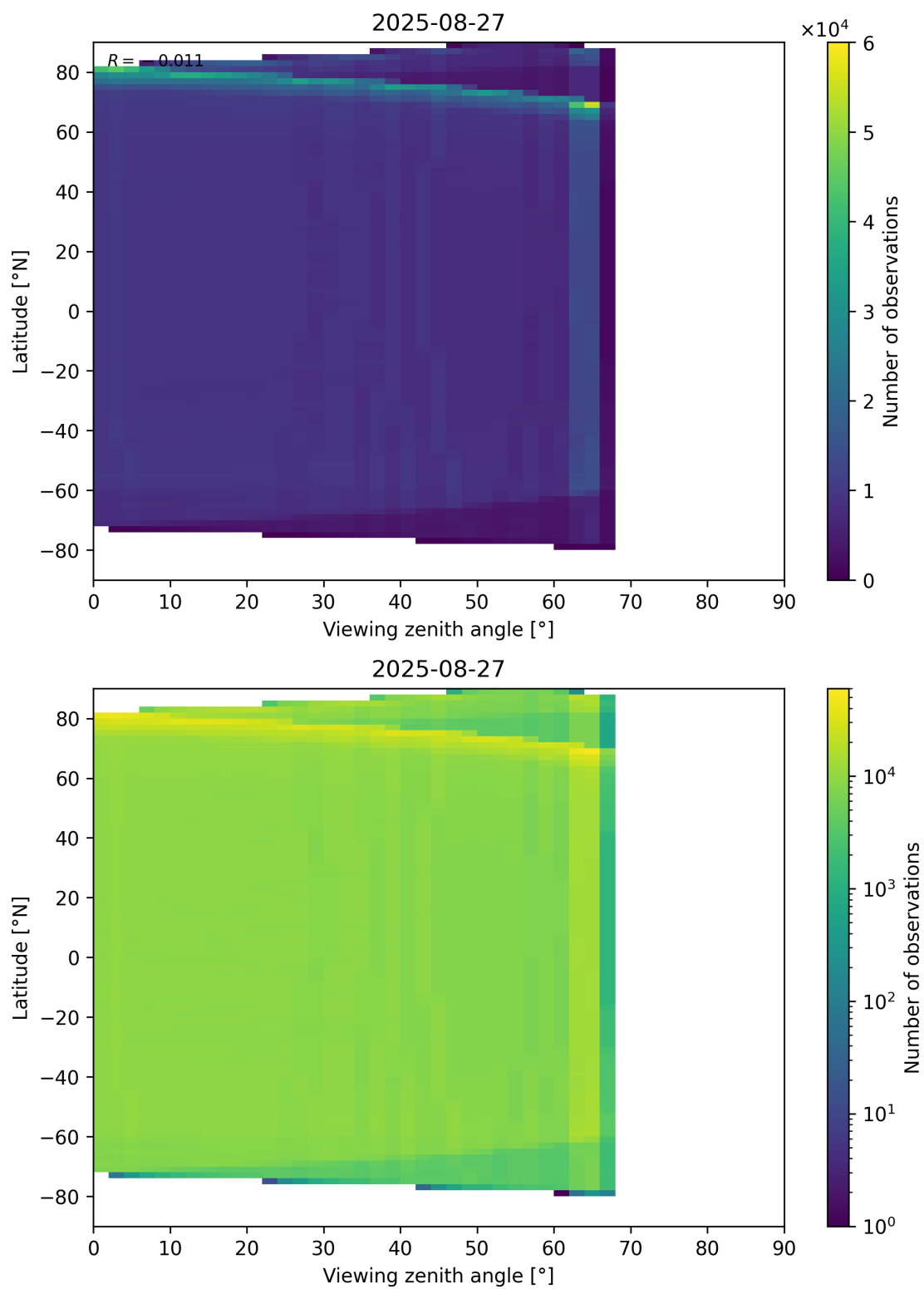
Figure 123: Scatter density plot of “Viewing zenith angle” against “Latitude” for 2025-08-26 to 2025-08-28.
