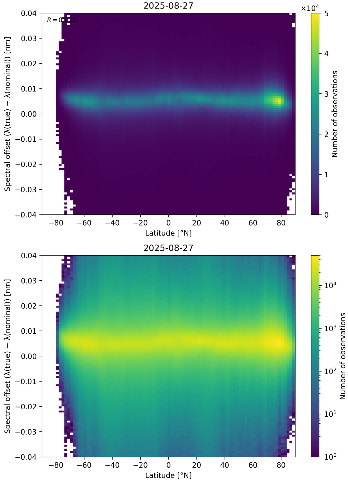
Figure 96: Scatter density plot of “Latitude” against “Spectral offset ( \lambda_{\text{true}} - \lambda_{\text{nominal}} )” for 2025-08-26 to 2025-08-28.
