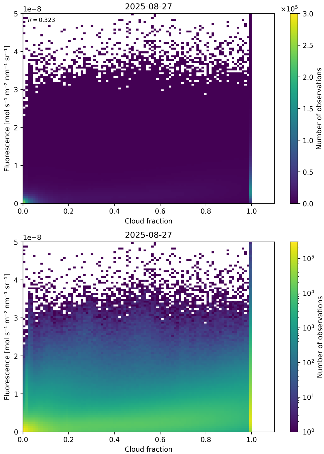
Figure 72: Scatter density plot of “Cloud fraction” against “Fluorescence” for 2025-08-26 to 2025-08-28.
