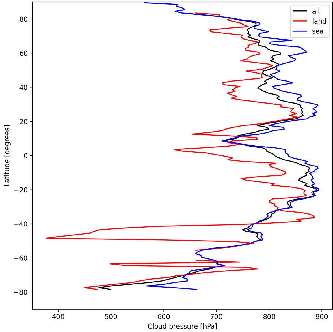
Figure 13: Zonal average of “Cloud pressure” for 2025-08-26 to 2025-08-28.
