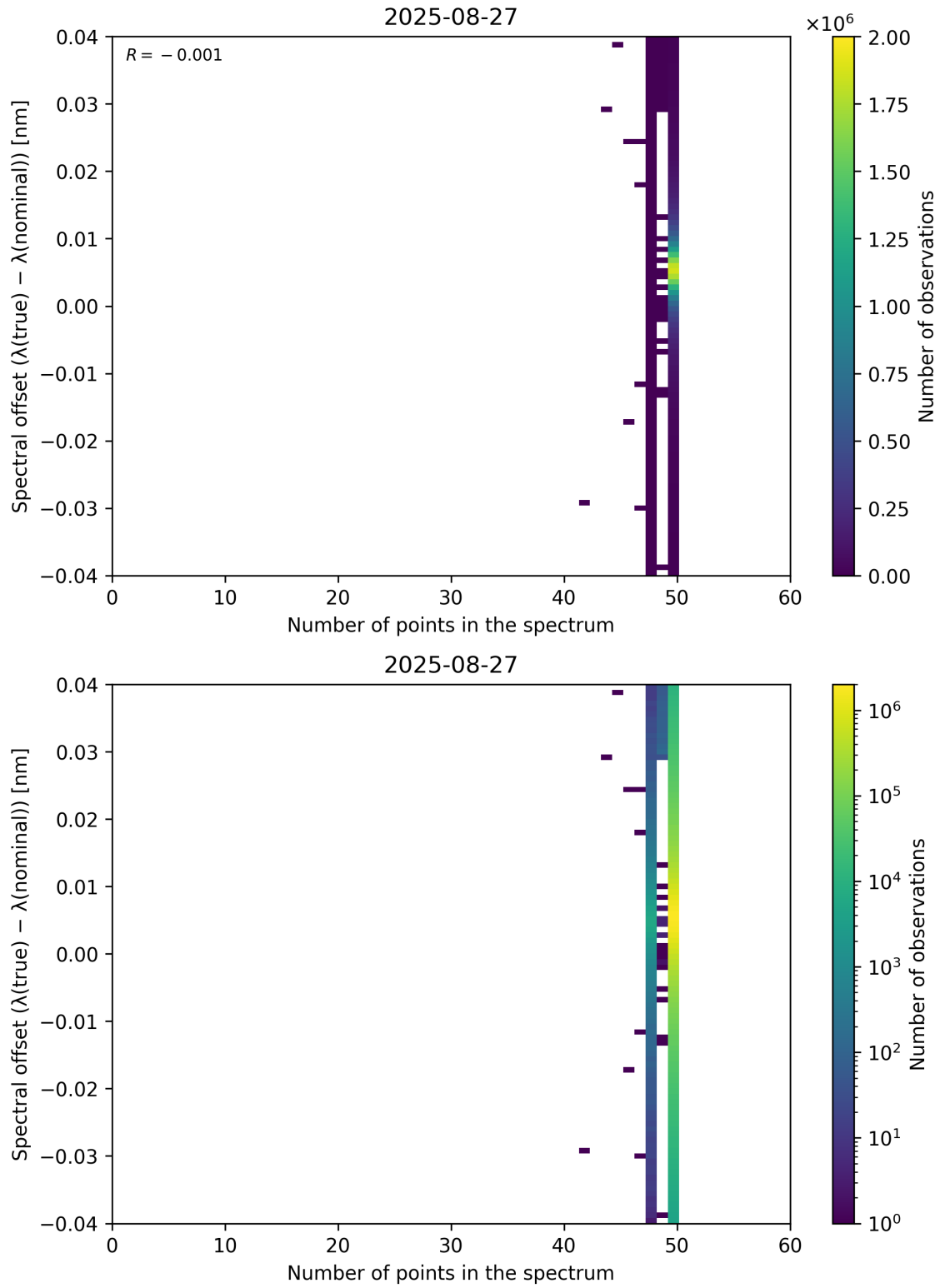
Figure 101: Scatter density plot of “Number of points in the spectrum” against “Spectral offset ( \lambda_{\text{true}} - \lambda_{\text{nominal}} )” for 2025-08-26 to 2025-08-28.
