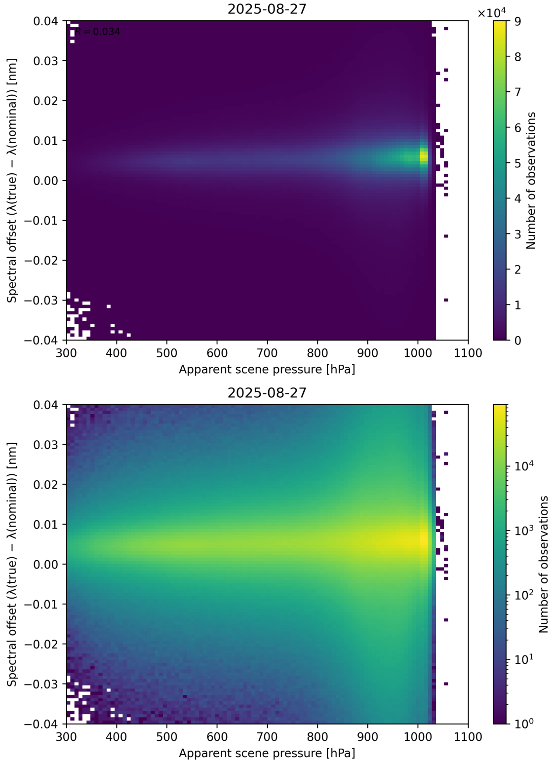
Figure 67: Scatter density plot of “Apparent scene pressure” against “Spectral offset ( \lambda_{\text{true}} - \lambda_{\text{nominal}} )” for 2025-08-26 to 2025-08-28.
