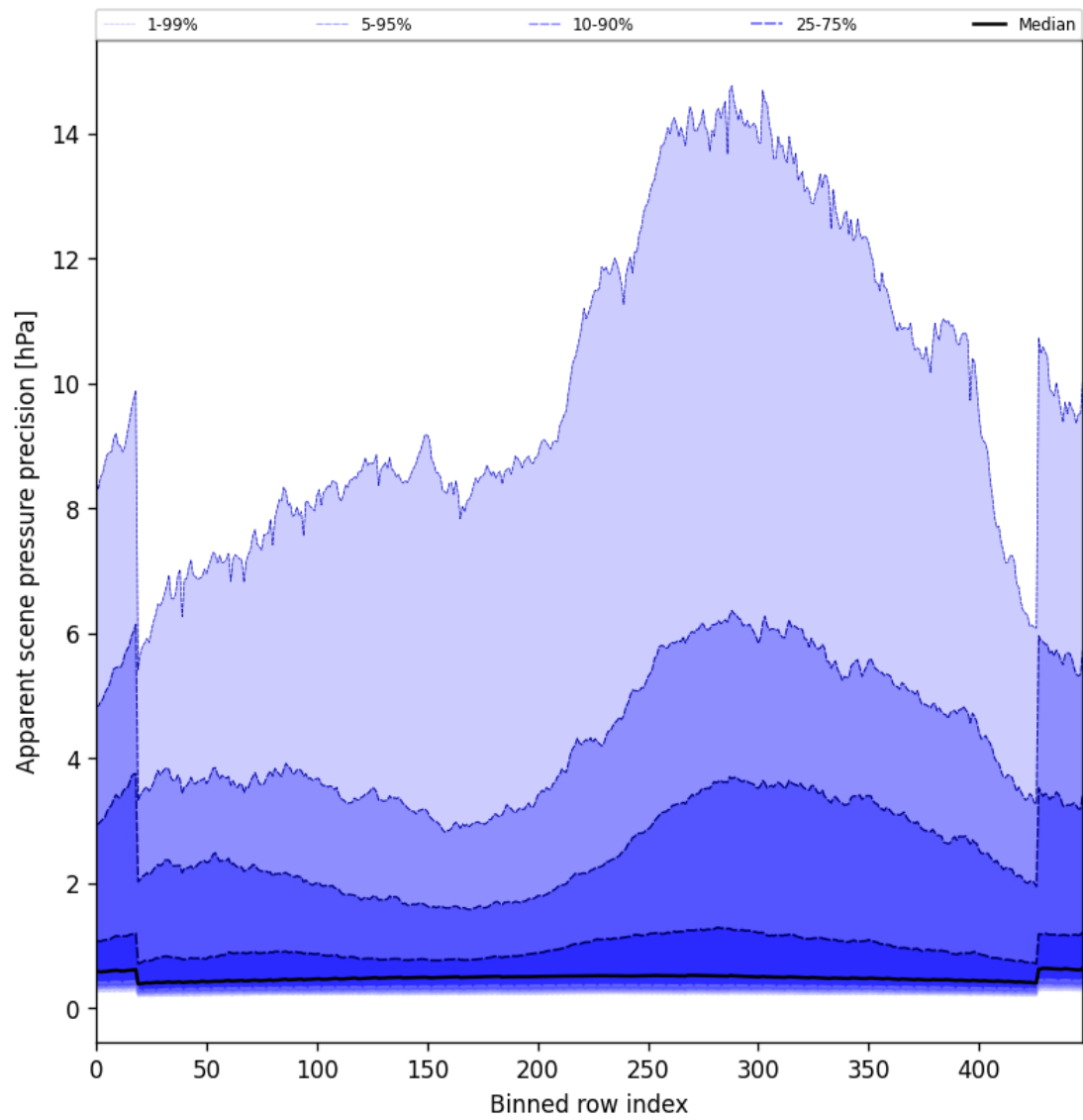
Figure 54: Along track statistics of “Apparent scene pressure precision” for 2025-08-26 to 2025-08-28
