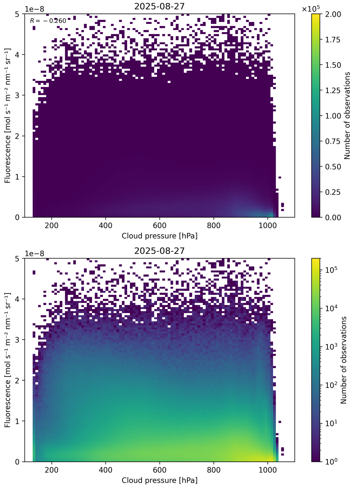
Figure 80: Scatter density plot of “Cloud pressure” against “Fluorescence” for 2025-08-26 to 2025-08-28.
