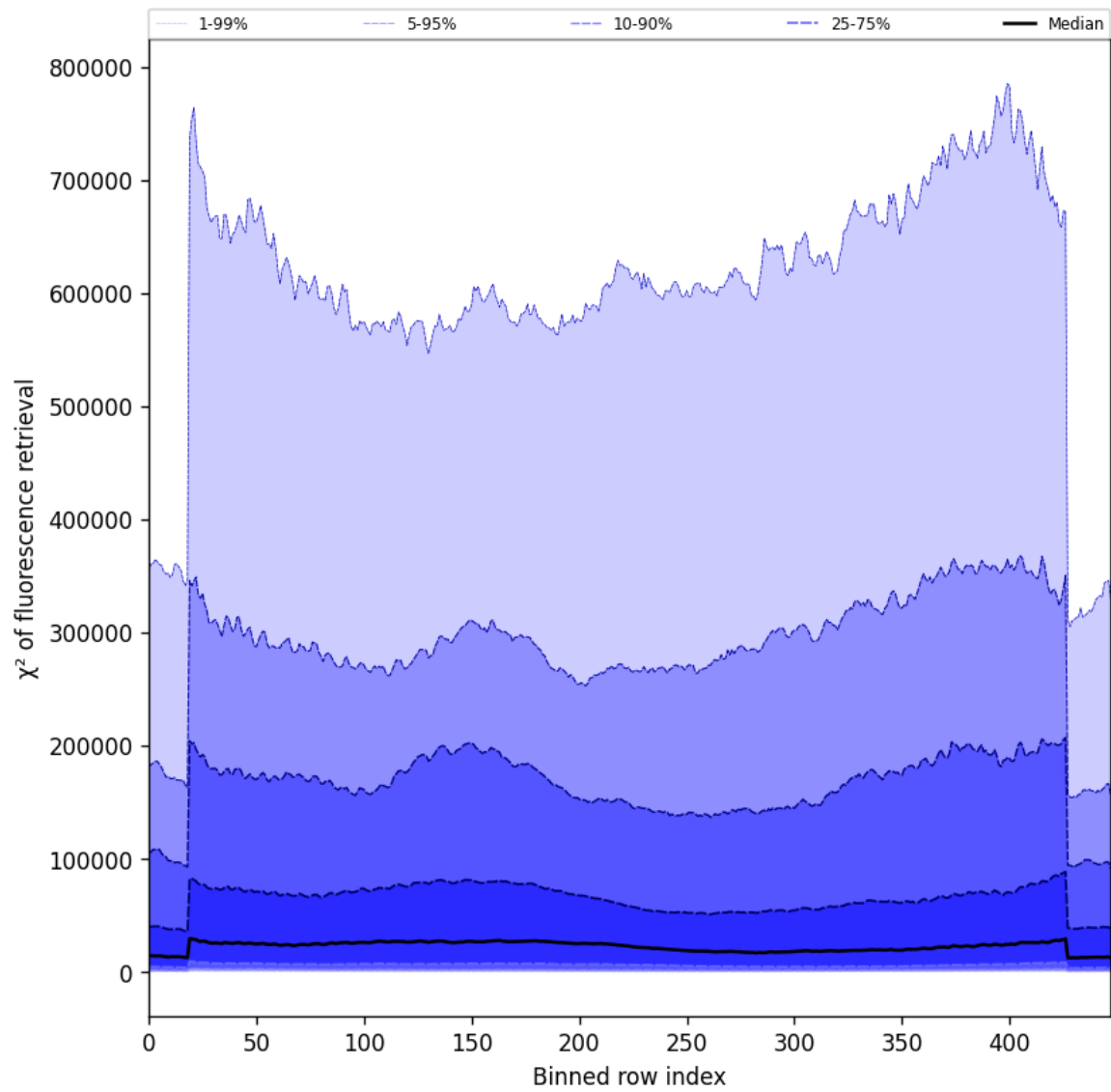
Figure 59: Along track statistics of " \chi^2 of fluorescence retrieval" for 2025-08-26 to 2025-08-28
