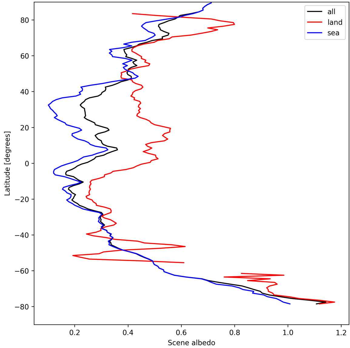
Figure 17: Zonal average of “Scene albedo” for 2025-08-26 to 2025-08-28.
