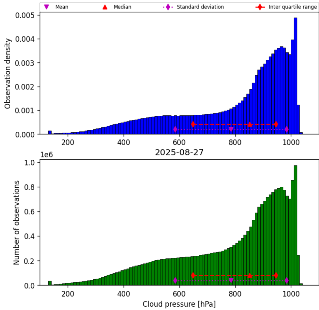
Figure 30: Histogram of “Cloud pressure” for 2025-08-26 to 2025-08-28
