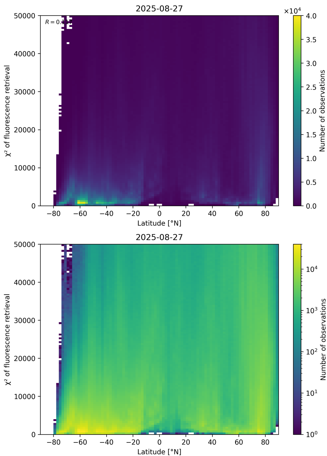
Figure 89: Scatter density plot of “Latitude” against “ \chi^2 of fluorescence retrieval” for 2025-08-26 to 2025-08-28.
