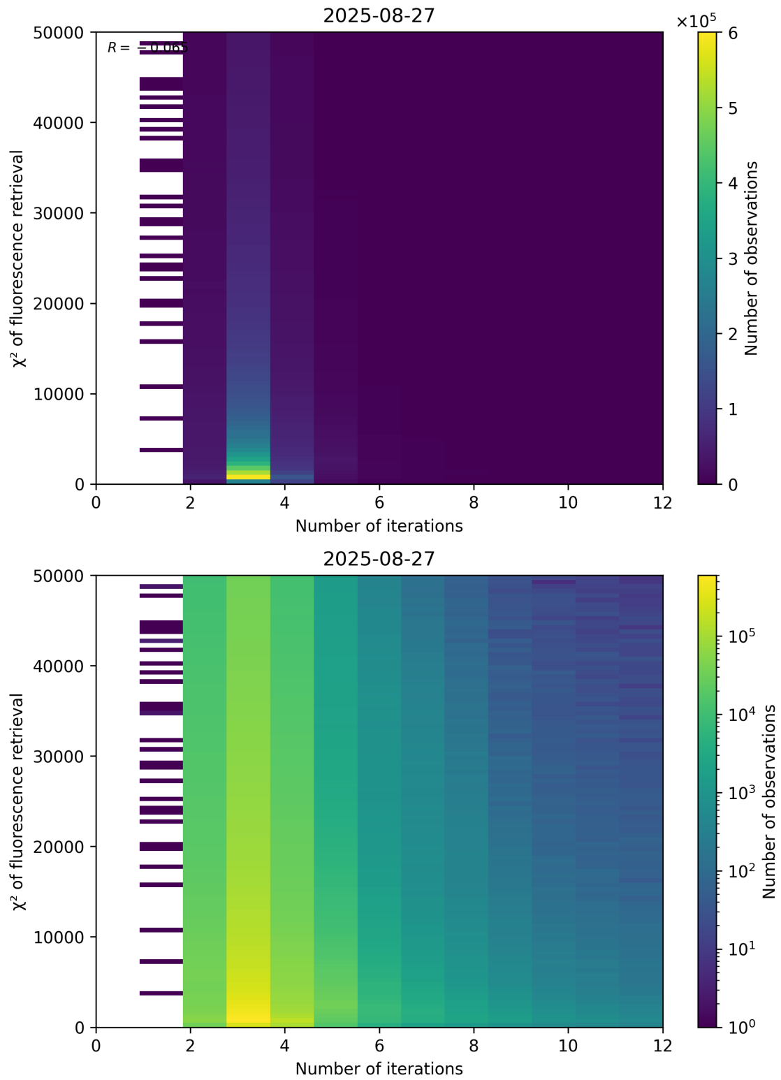
Figure 97: Scatter density plot of “Number of iterations” against “ \chi^2 of fluorescence retrieval” for 2025-08-26 to 2025-08-28.
