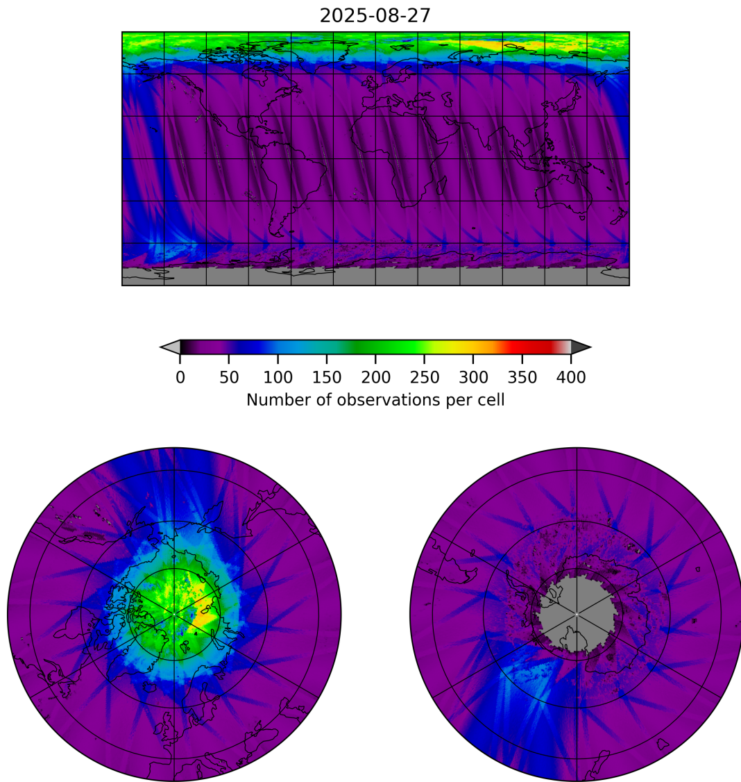
Figure 11: Map of the number of observations for 2025-08-26 to 2025-08-28
