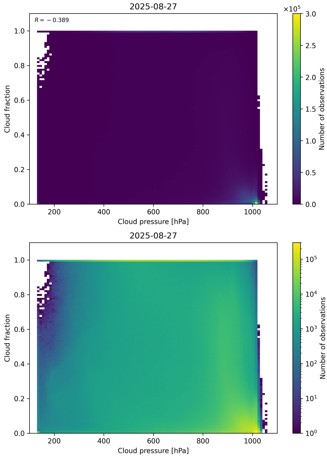
Figure 79: Scatter density plot of “Cloud pressure” against “Cloud fraction” for 2025-08-26 to 2025-08-28.
