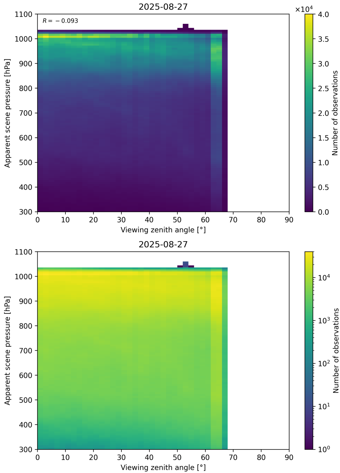
Figure 118: Scatter density plot of “Viewing zenith angle” against “Apparent scene pressure” for 2025-08-26 to 2025-08-28.
