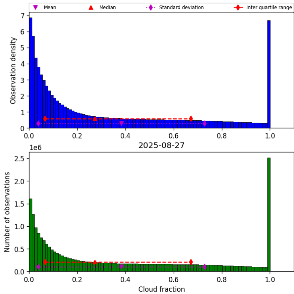
Figure 32: Histogram of “Cloud fraction” for 2025-08-26 to 2025-08-28
