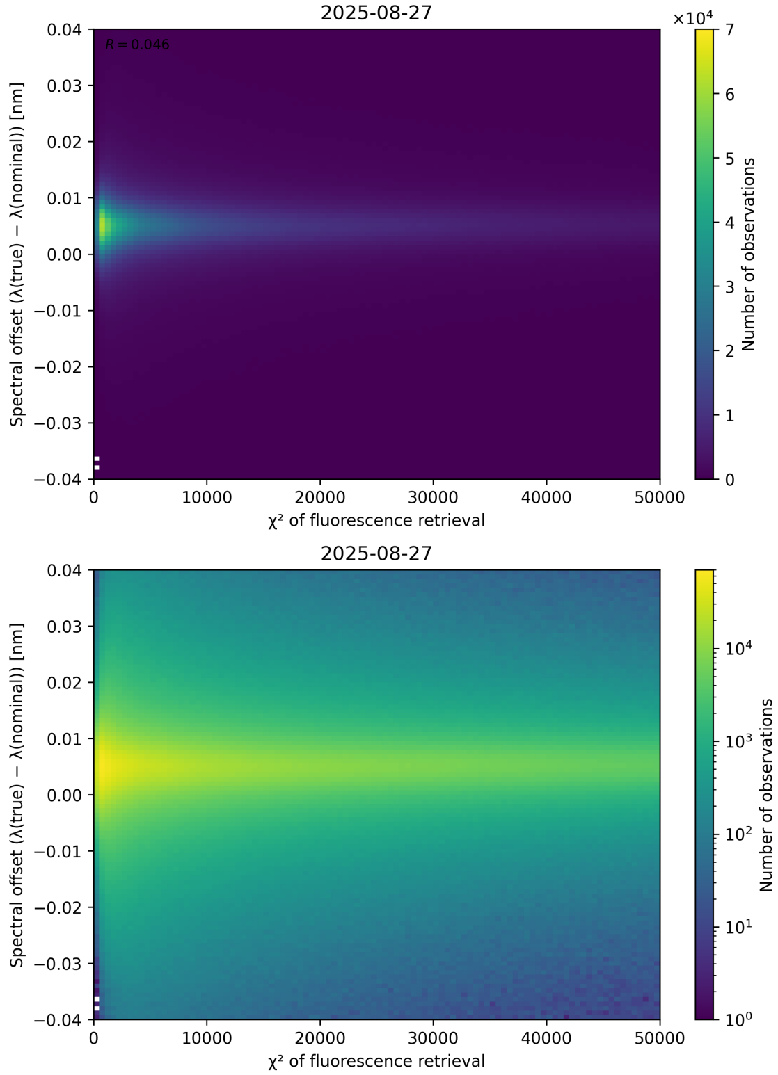
Figure 69: Scatter density plot of “ \chi^2 of fluorescence retrieval” against “Spectral offset ( \lambda_{\text{true}} - \lambda_{\text{nominal}} )” for 2025-08-26 to 2025-08-28.
