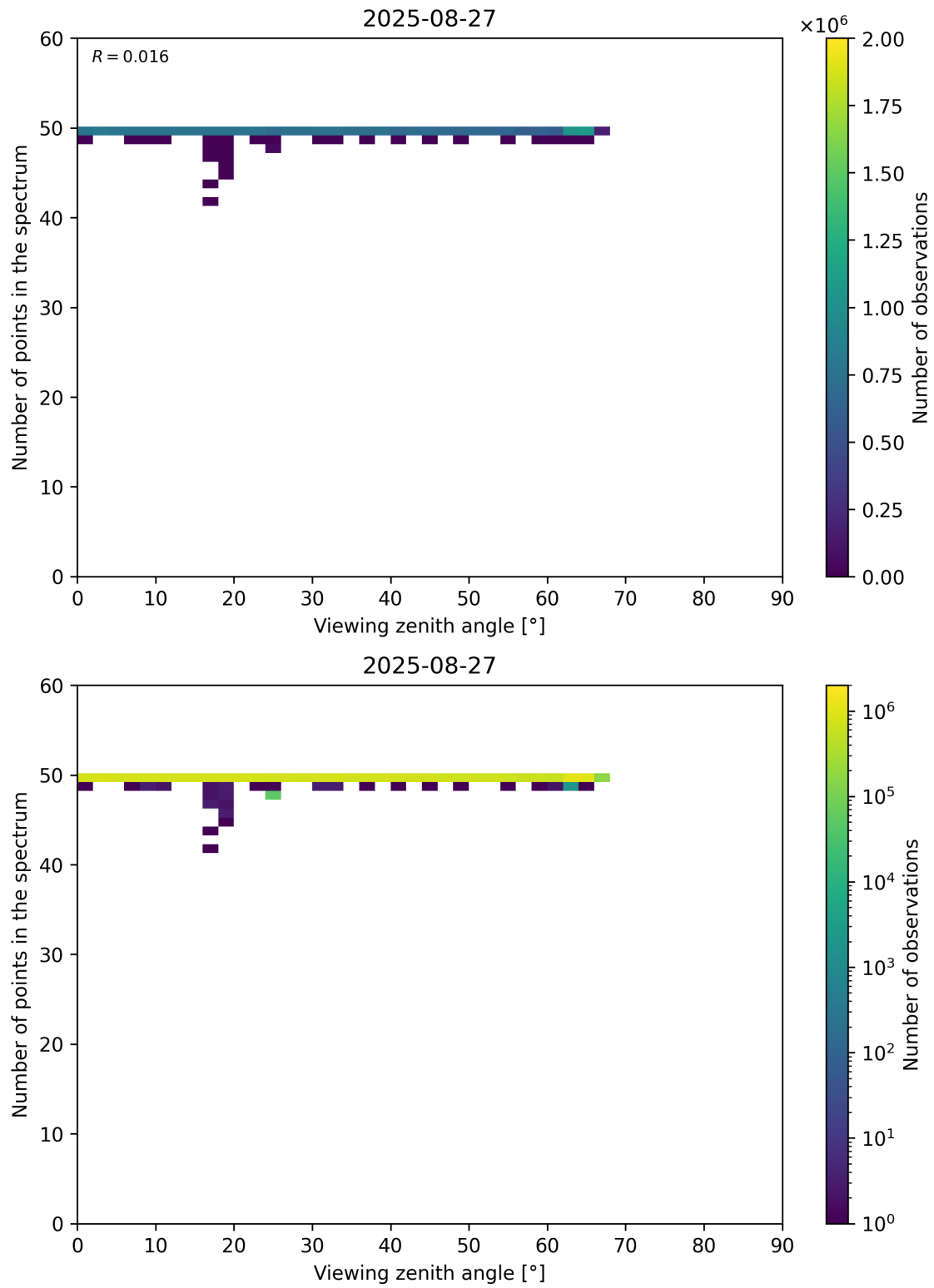
Figure 125: Scatter density plot of “Viewing zenith angle” against “Number of points in the spectrum” for 2025-08-26 to 2025-08-28.
