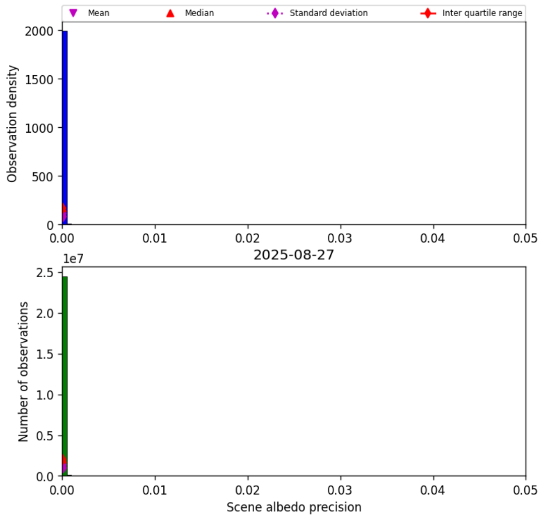
Figure 35: Histogram of “Scene albedo precision” for 2025-08-26 to 2025-08-28
