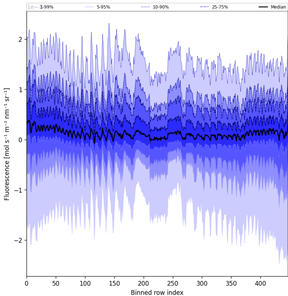
Figure 57: Along track statistics of “Fluorescence” for 2025-08-26 to 2025-08-28
