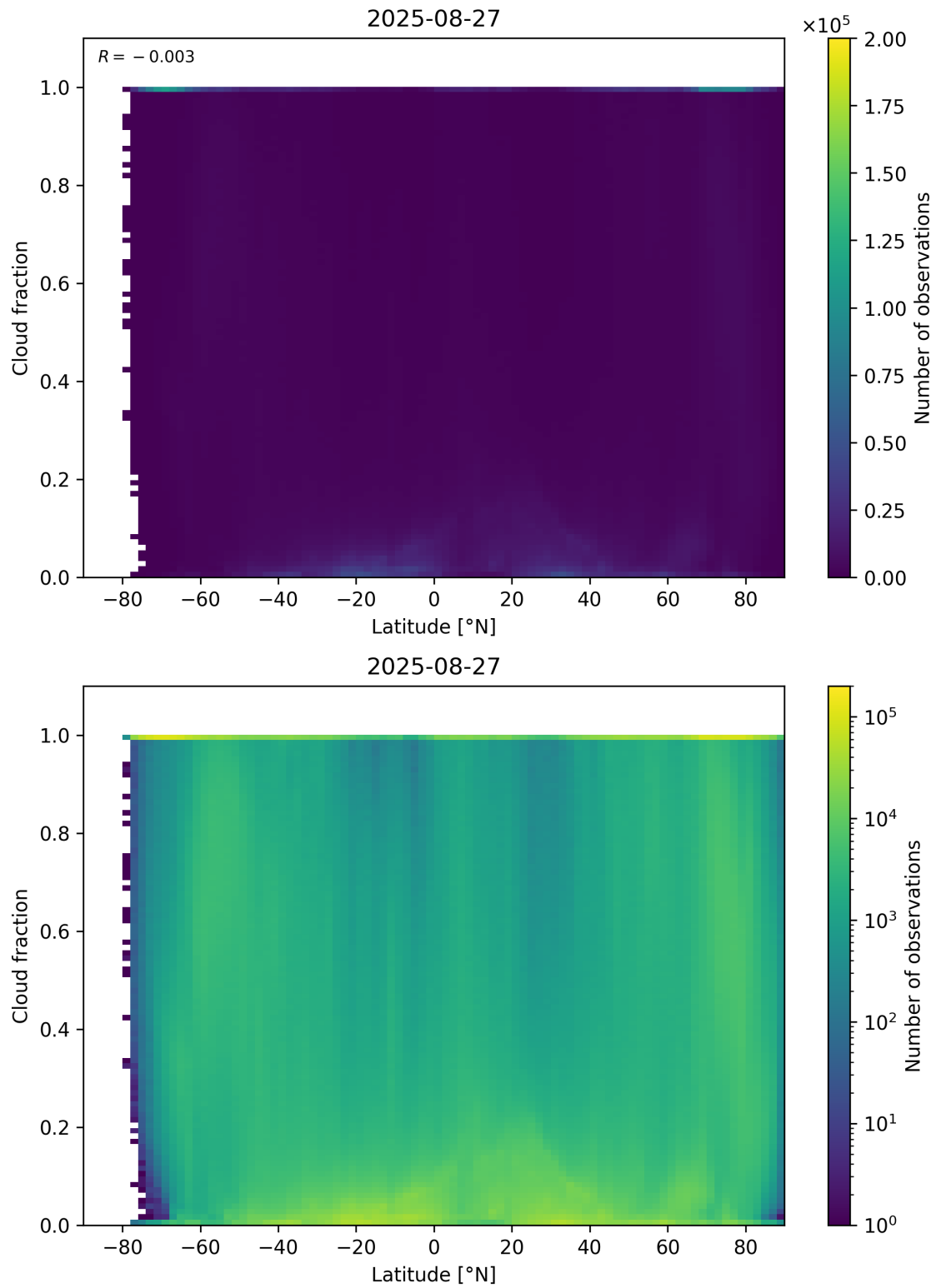
Figure 90: Scatter density plot of “Latitude” against “Cloud fraction” for 2025-08-26 to 2025-08-28.
