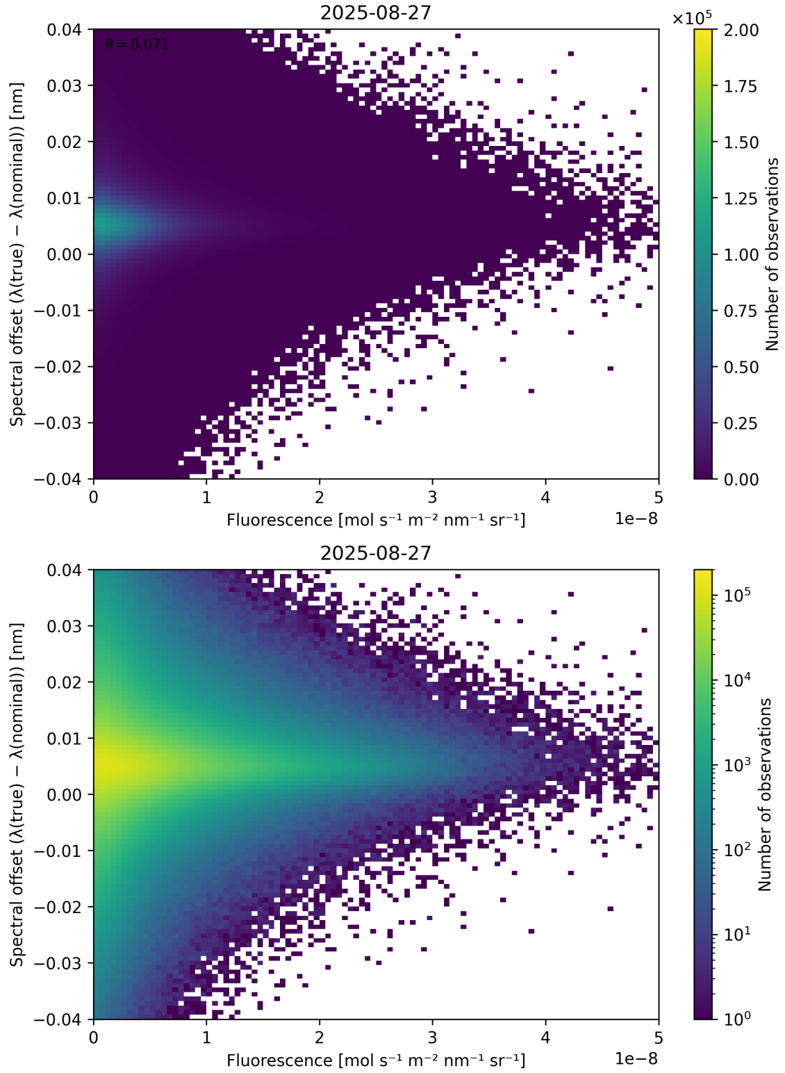
Figure 87: Scatter density plot of “Fluorescence” against “Spectral offset ( \lambda_{\text{true}} - \lambda_{\text{nominal}} )” for 2025-08-26 to 2025-08-28.
