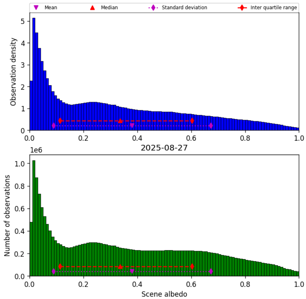
Figure 34: Histogram of “Scene albedo” for 2025-08-26 to 2025-08-28
