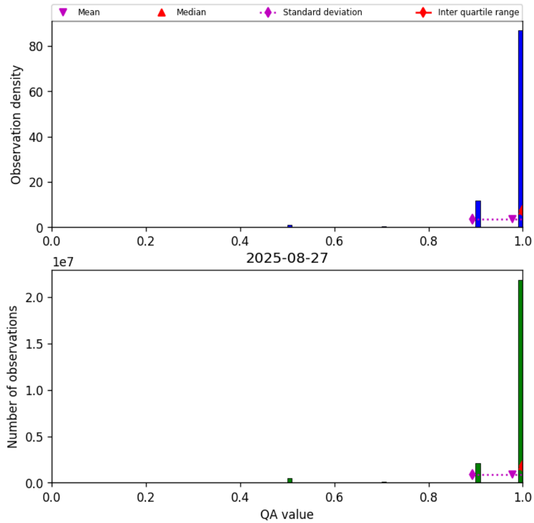
Figure 29: Histogram of “QA value” for 2025-08-26 to 2025-08-28
