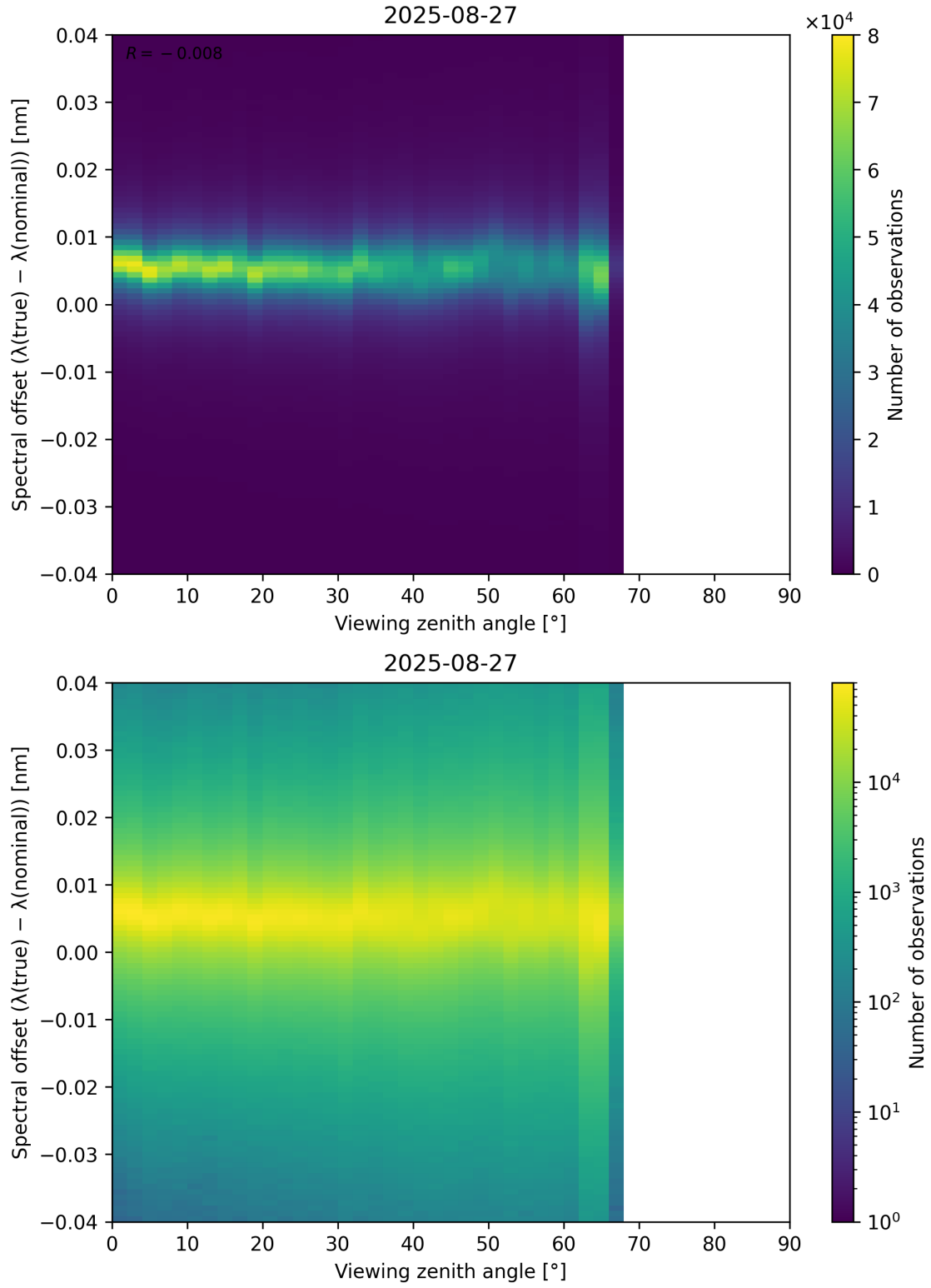
Figure 128: Scatter density plot of “Viewing zenith angle” against “Spectral offset ( \lambda_{\text{true}} - \lambda_{\text{nominal}} )” for 2025-08-26 to 2025-08-28.
