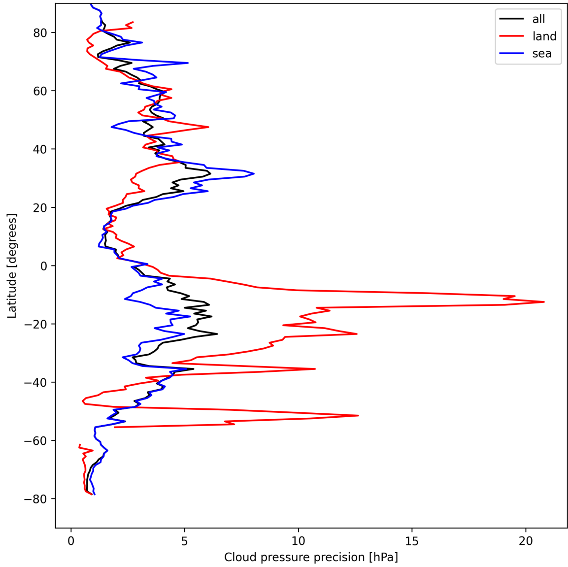
Figure 14: Zonal average of “Cloud pressure precision” for 2025-08-26 to 2025-08-28.
