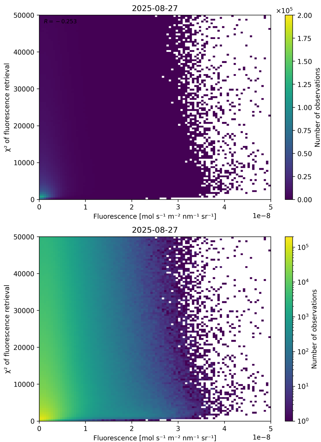
Figure 85: Scatter density plot of “Fluorescence” against “ \chi^2 of fluorescence retrieval” for 2025-08-26 to 2025-08-28.
