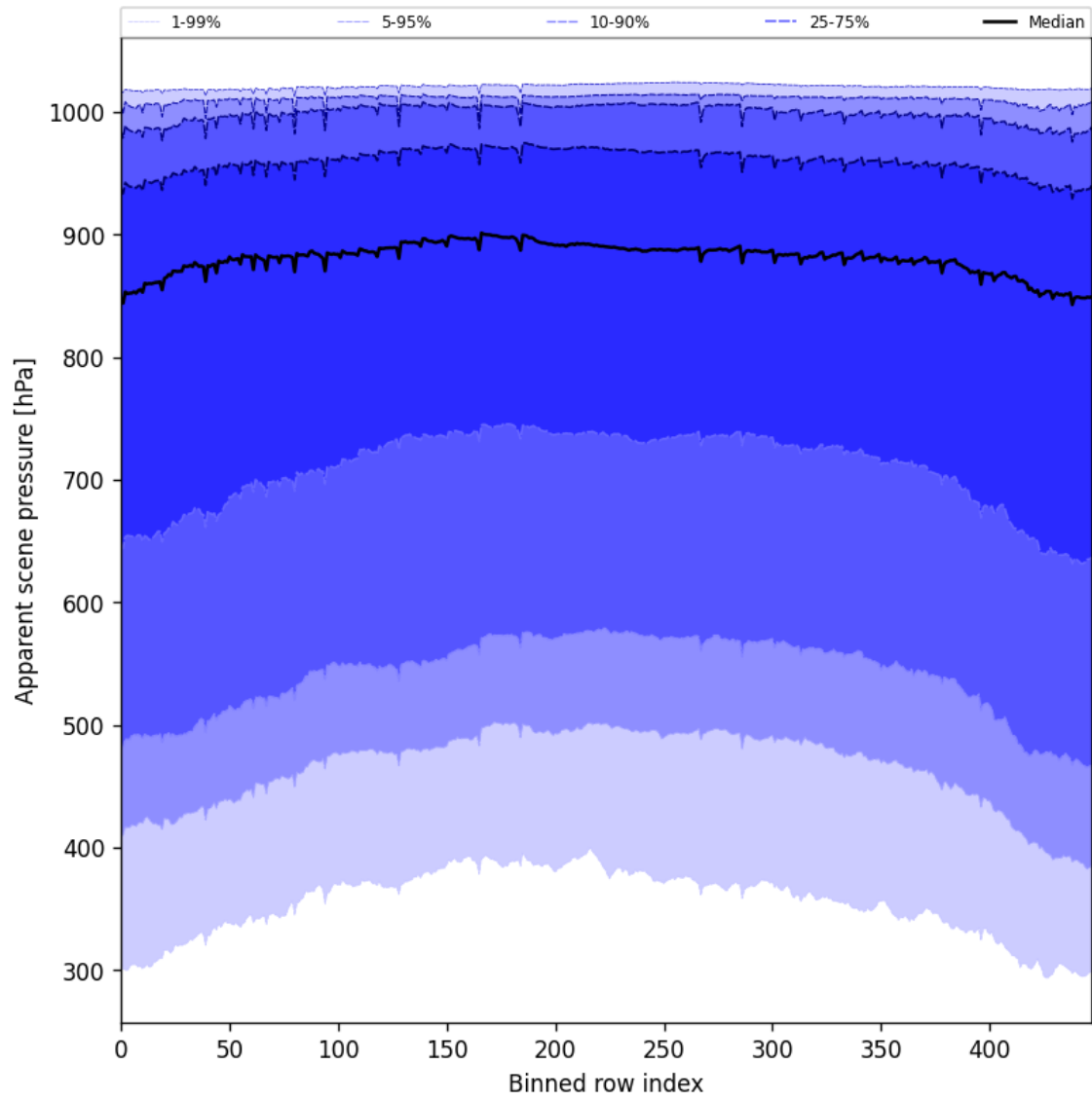
Figure 53: Along track statistics of “Apparent scene pressure” for 2025-08-26 to 2025-08-28
