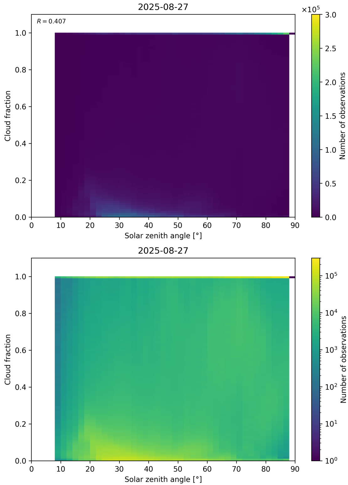
Figure 110: Scatter density plot of “Solar zenith angle” against “Cloud fraction” for 2025-08-26 to 2025-08-28.
