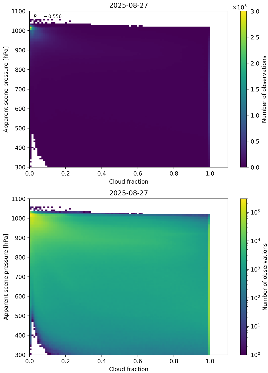
Figure 70: Scatter density plot of “Cloud fraction” against “Apparent scene pressure” for 2025-08-26 to 2025-08-28.
