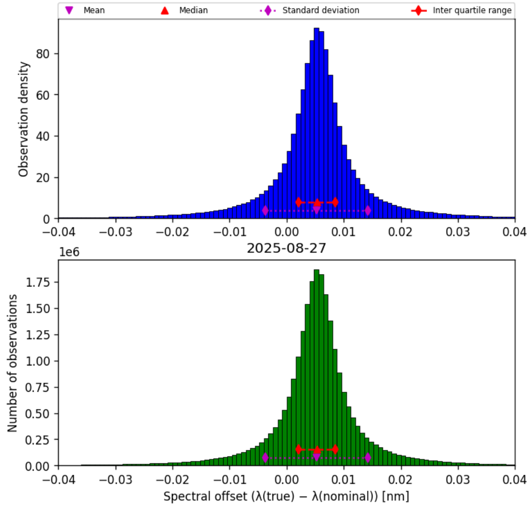
Figure 45: Histogram of “Spectral offset ( \lambda_{\text{true}} - \lambda_{\text{nominal}} )” for 2025-08-26 to 2025-08-28
