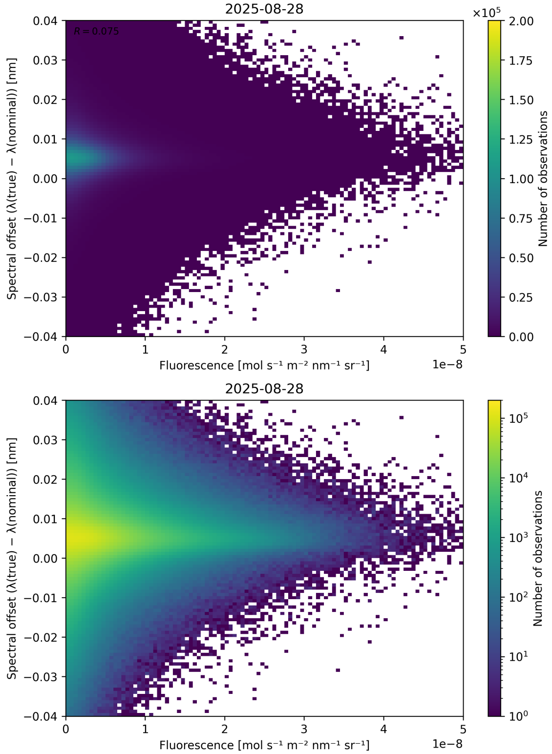
Figure 87: Scatter density plot of “Fluorescence” against “Spectral offset ( \lambda_{\text{true}} - \lambda_{\text{nominal}} )” for 2025-08-27 to 2025-08-29.
