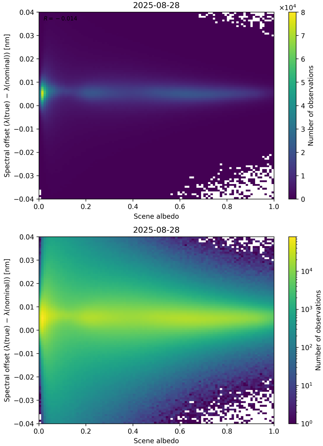
Figure 107: Scatter density plot of “Scene albedo” against “Spectral offset ( \lambda_{\text{true}} - \lambda_{\text{nominal}} )” for 2025-08-27 to 2025-08-29.
