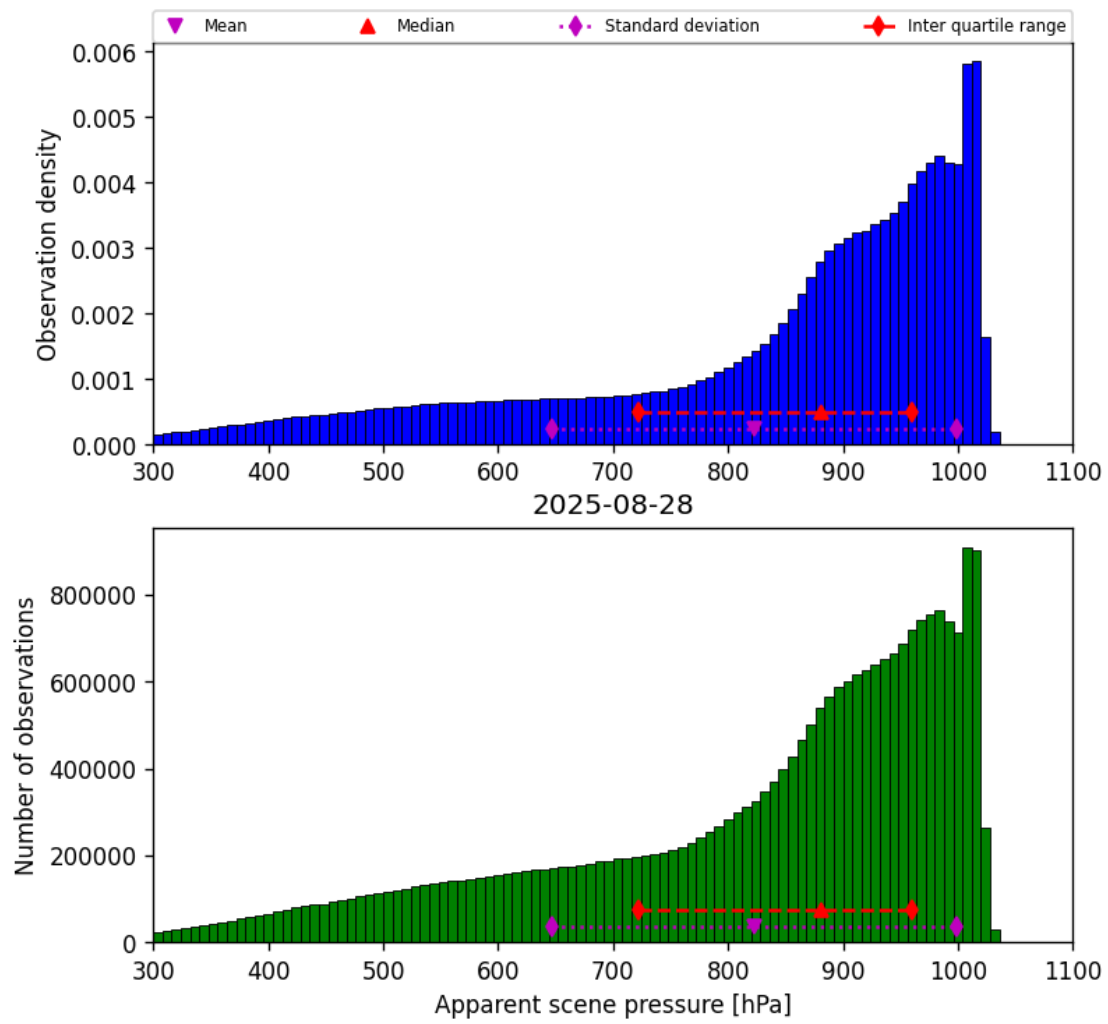
Figure 36: Histogram of “Apparent scene pressure” for 2025-08-27 to 2025-08-29
