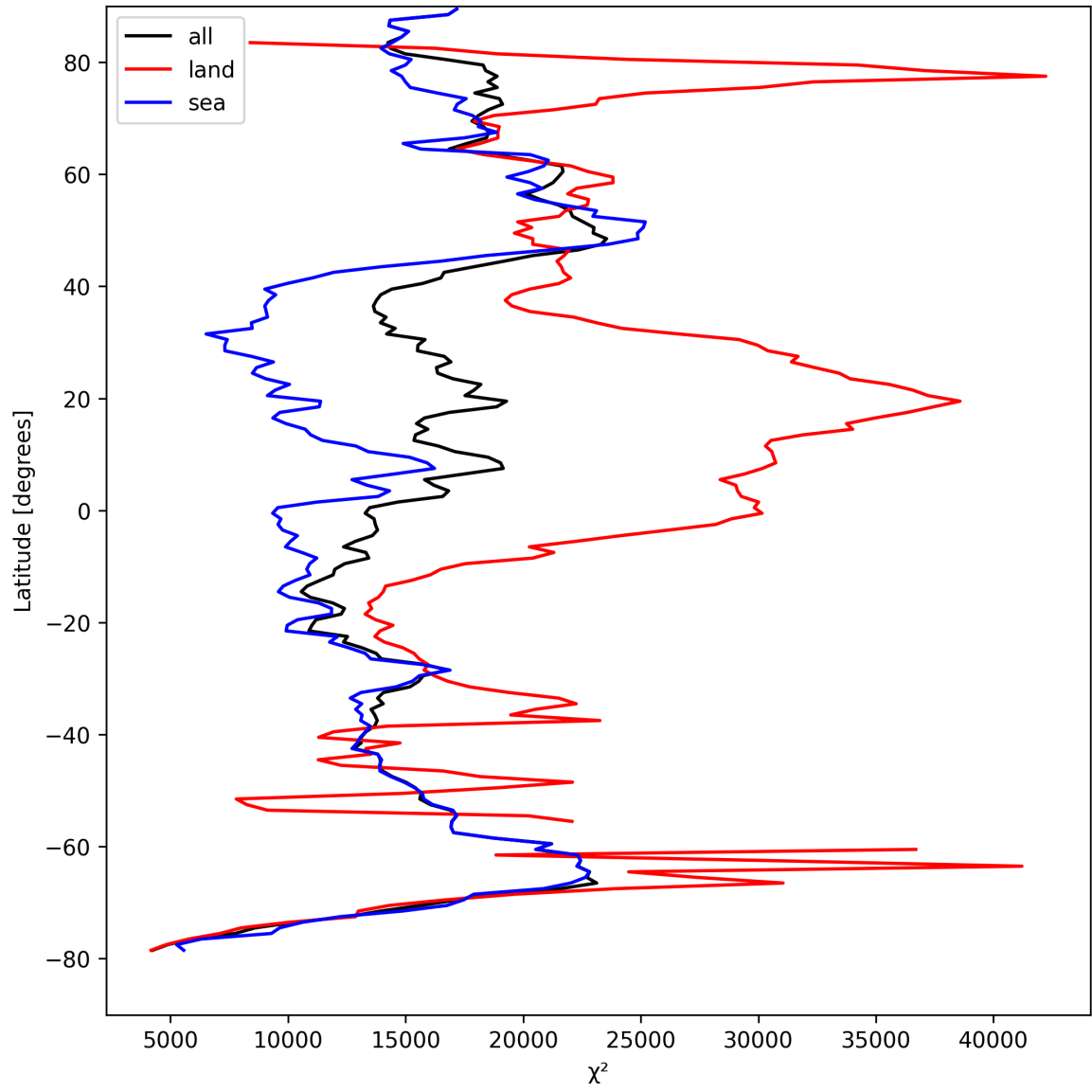
Figure 21: Zonal average of “ \chi^2 ” for 2025-08-27 to 2025-08-29.
