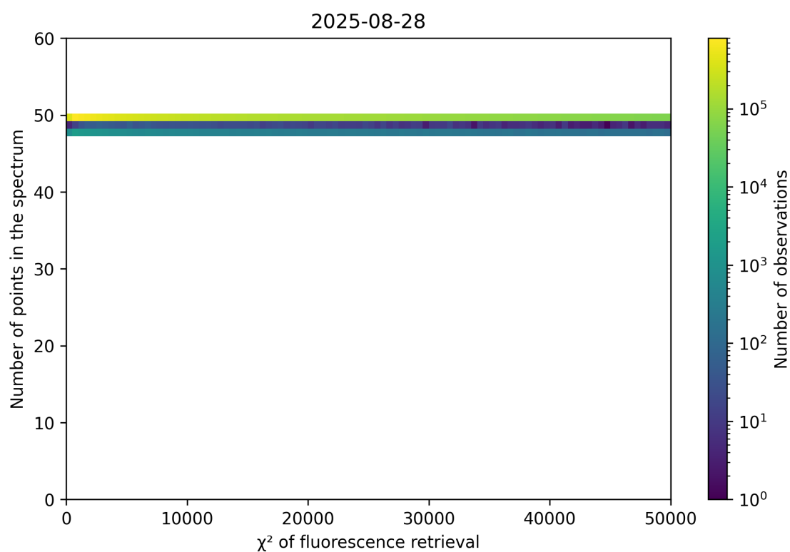
Figure 68: Scatter density plot of “ \chi^2 of fluorescence retrieval” against “Number of points in the spectrum” for 2025-08-27 to 2025-08-29.
