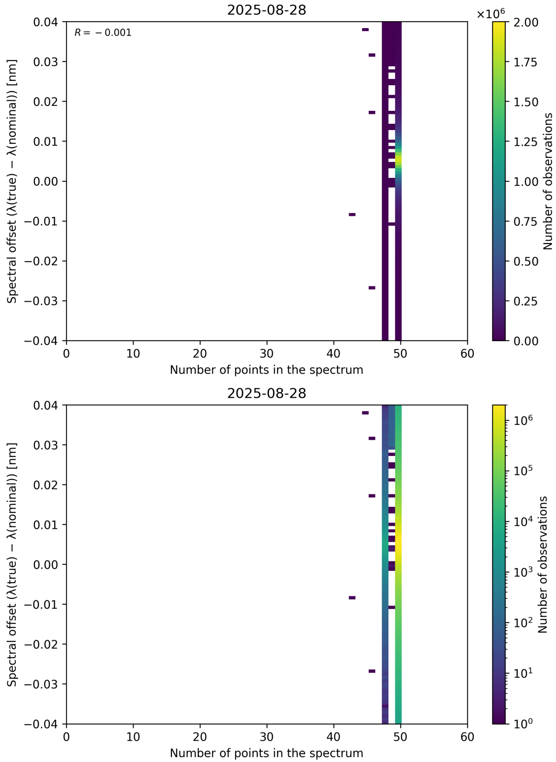
Figure 101: Scatter density plot of “Number of points in the spectrum” against “Spectral offset ( \lambda_{\text{true}} - \lambda_{\text{nominal}} )” for 2025-08-27 to 2025-08-29.
