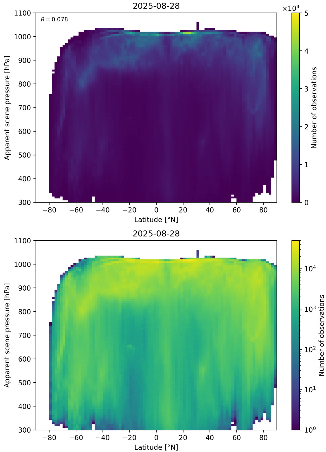
Figure 88: Scatter density plot of “Latitude” against “Apparent scene pressure” for 2025-08-27 to 2025-08-29.
