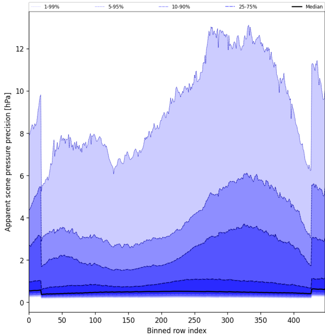
Figure 54: Along track statistics of “Apparent scene pressure precision” for 2025-08-27 to 2025-08-29
