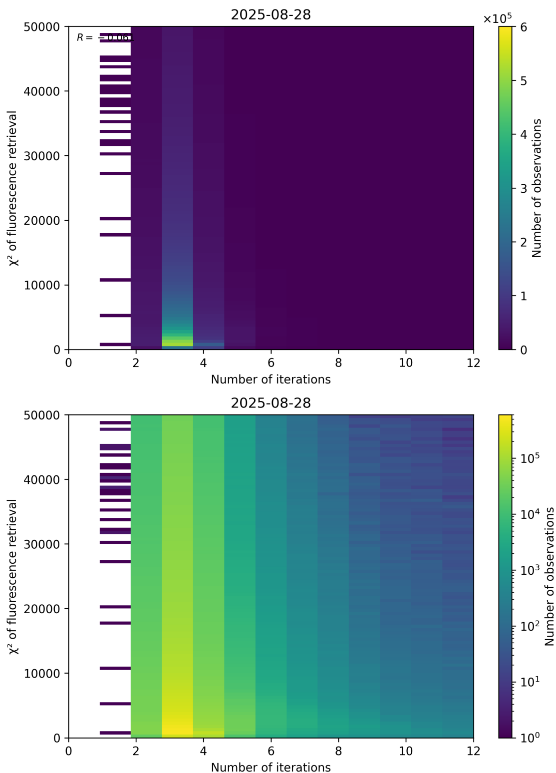
Figure 97: Scatter density plot of “Number of iterations” against “ \chi^2 of fluorescence retrieval” for 2025-08-27 to 2025-08-29.
