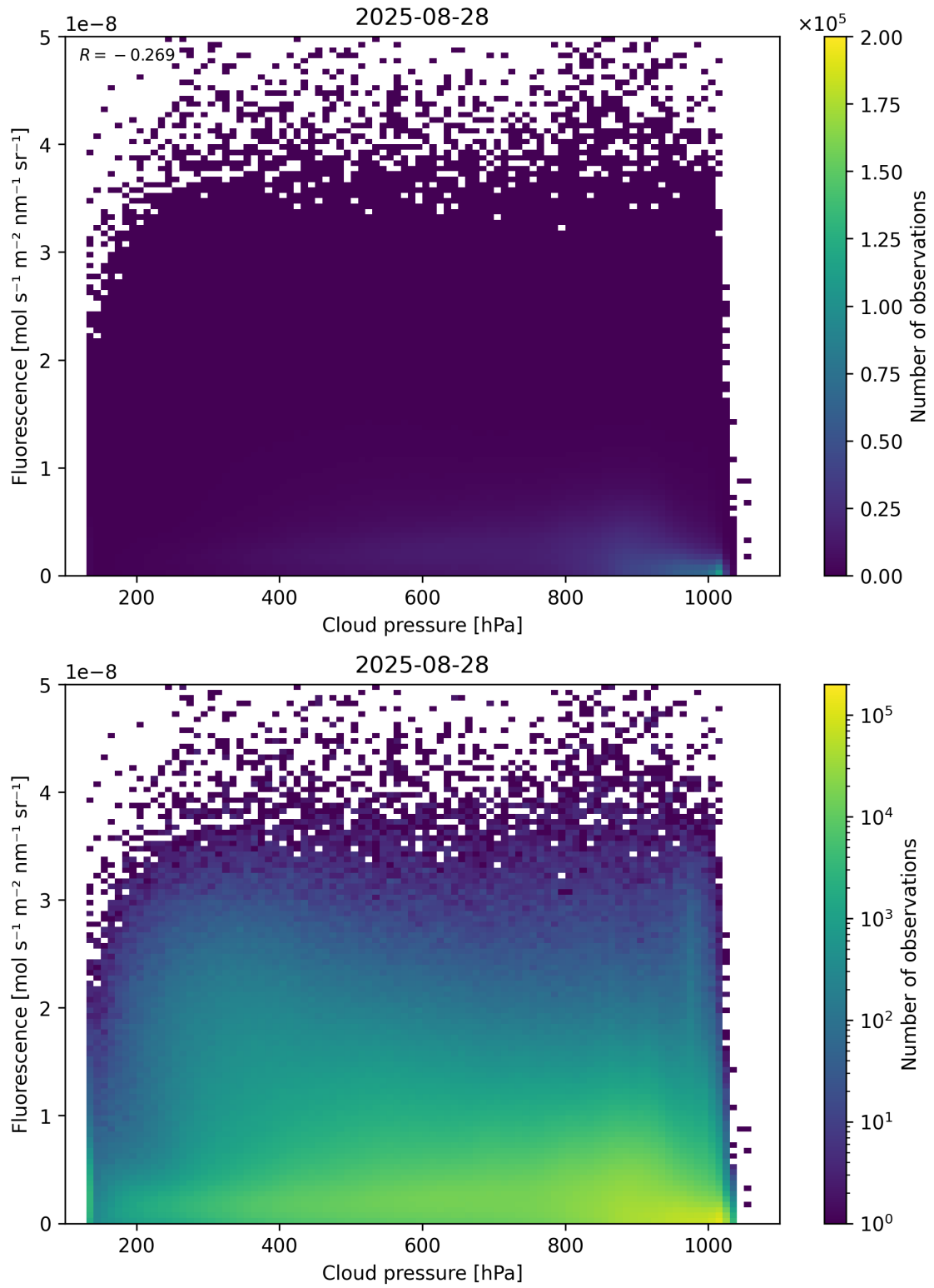
Figure 80: Scatter density plot of “Cloud pressure” against “Fluorescence” for 2025-08-27 to 2025-08-29.
