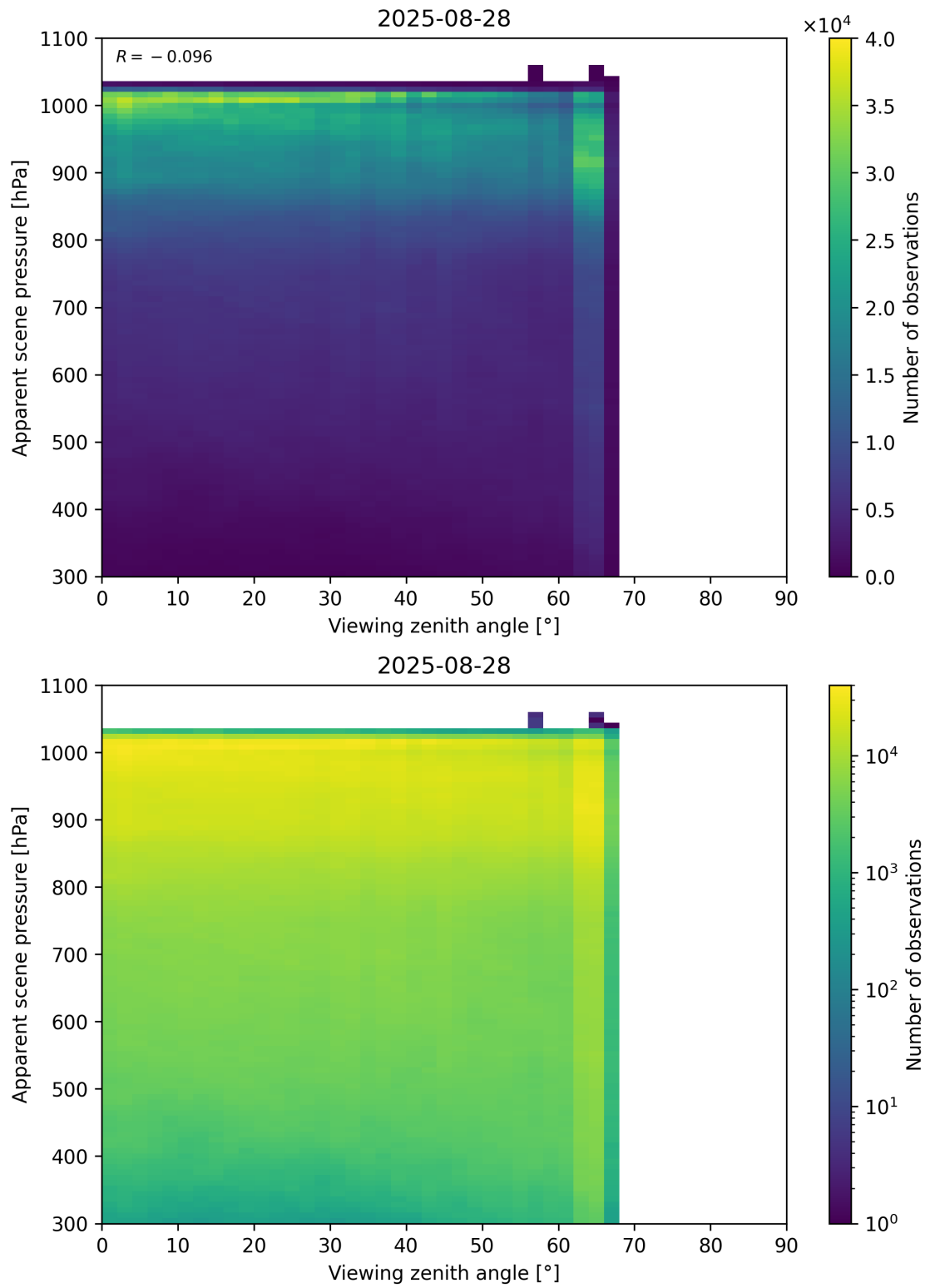
Figure 118: Scatter density plot of “Viewing zenith angle” against “Apparent scene pressure” for 2025-08-27 to 2025-08-29.
