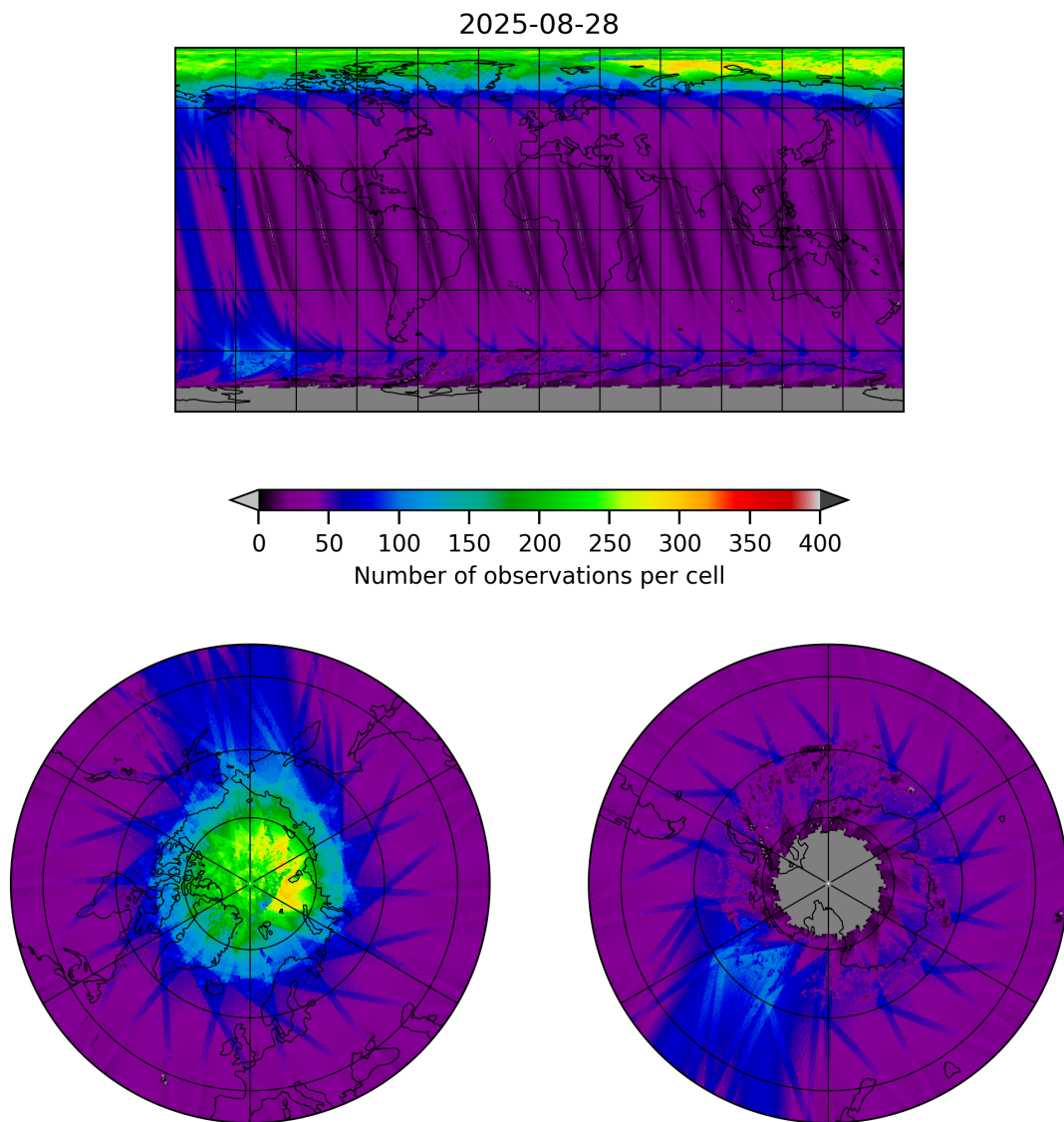
Figure 11: Map of the number of observations for 2025-08-27 to 2025-08-29
