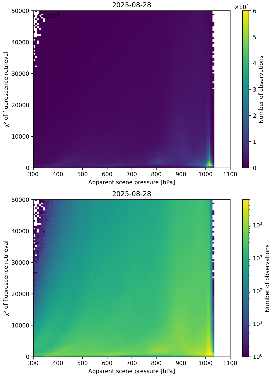
Figure 63: Scatter density plot of “Apparent scene pressure” against “ \chi^2 of fluorescence retrieval” for 2025-08-27 to 2025-08-29.
