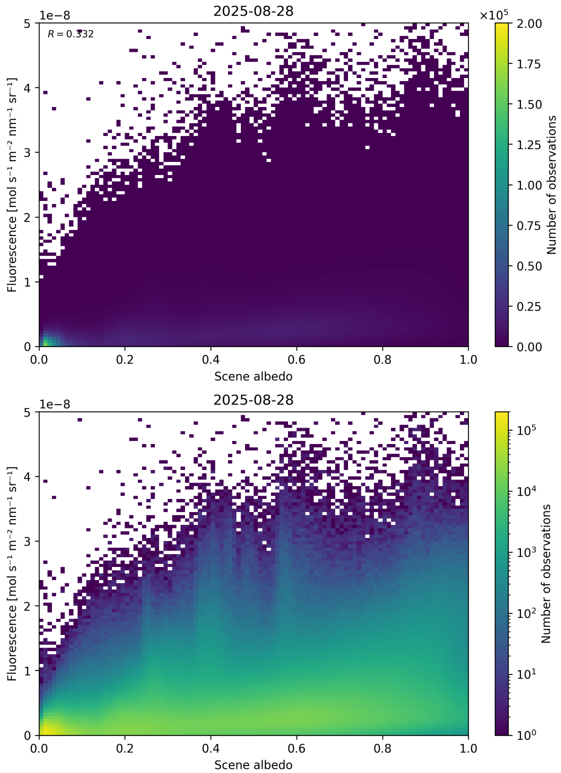
Figure 104: Scatter density plot of “Scene albedo” against “Fluorescence” for 2025-08-27 to 2025-08-29.
