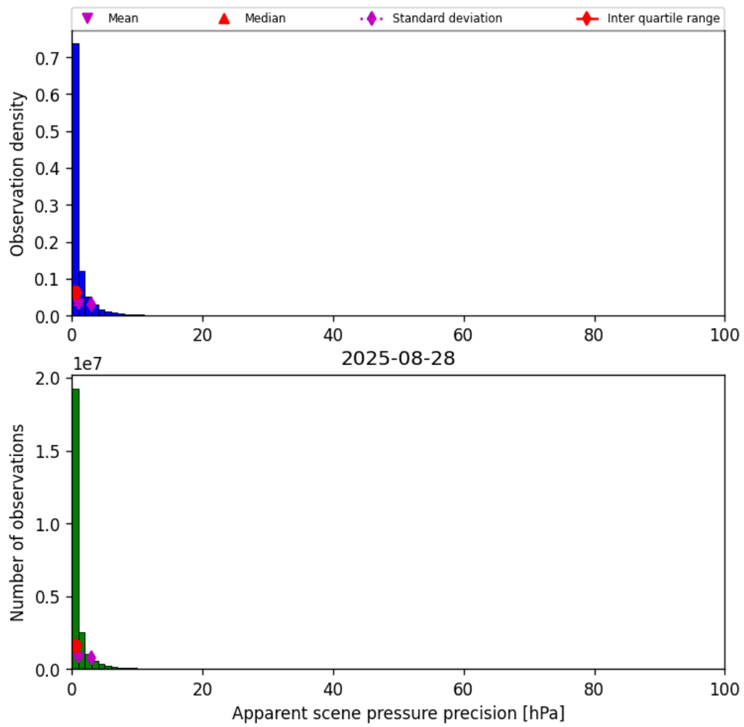
Figure 37: Histogram of “Apparent scene pressure precision” for 2025-08-27 to 2025-08-29
