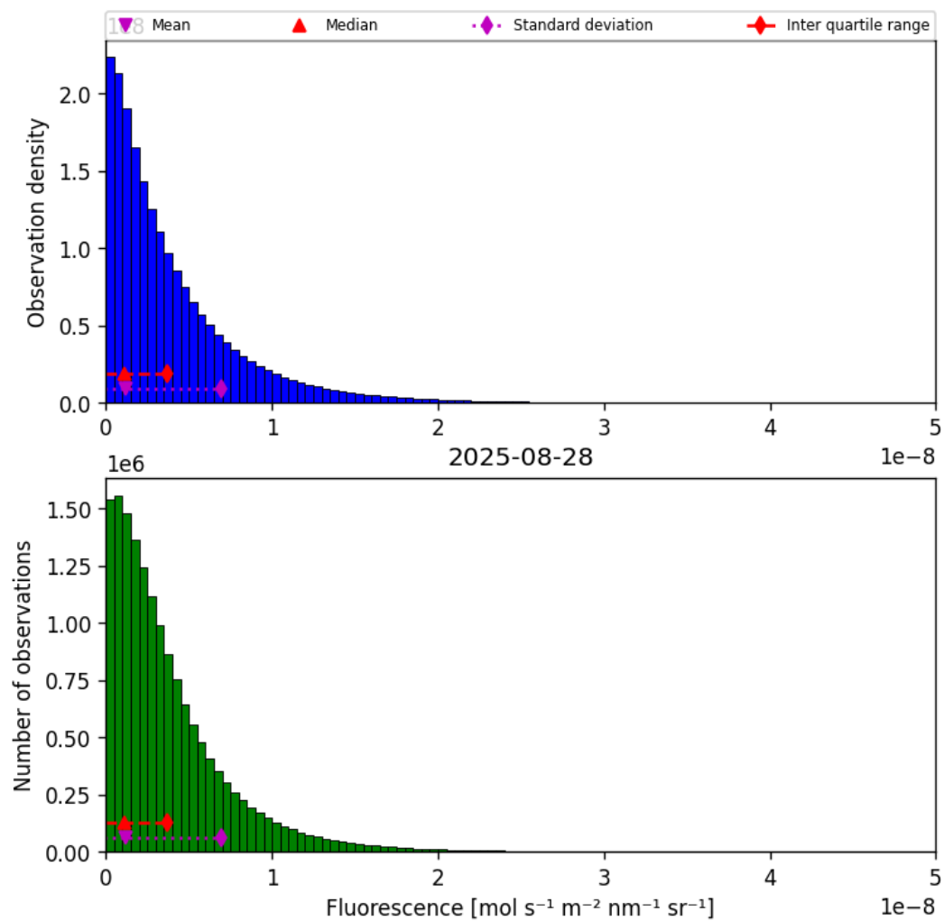
Figure 40: Histogram of “Fluorescence” for 2025-08-27 to 2025-08-29
