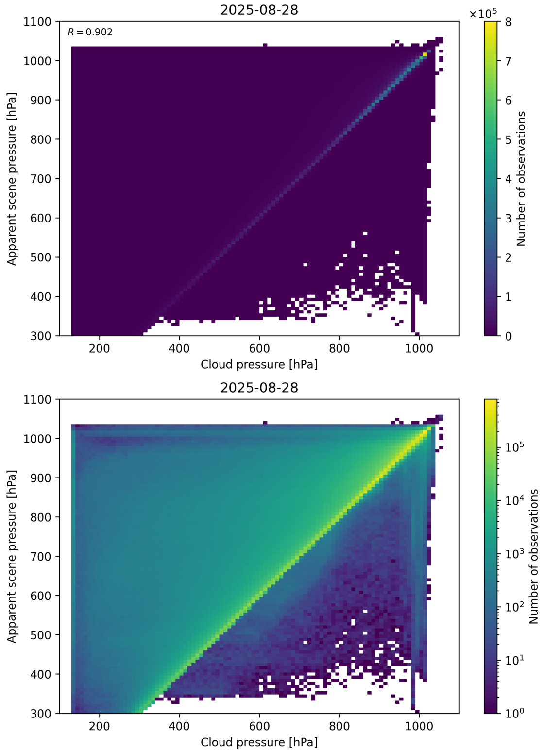
Figure 77: Scatter density plot of “Cloud pressure” against “Apparent scene pressure” for 2025-08-27 to 2025-08-29.
