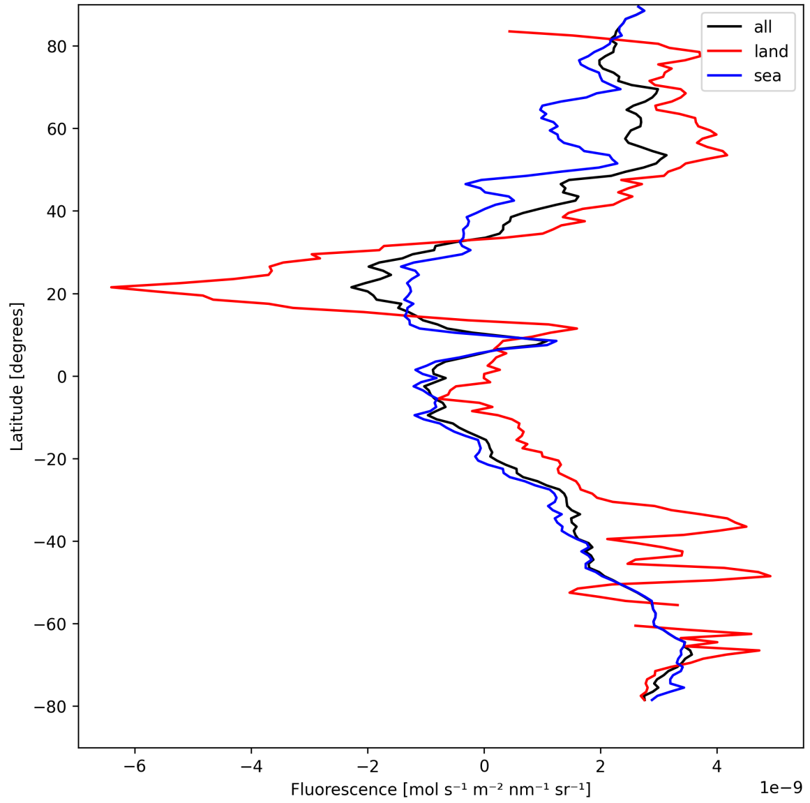
Figure 23: Zonal average of “Fluorescence” for 2025-08-27 to 2025-08-29.
