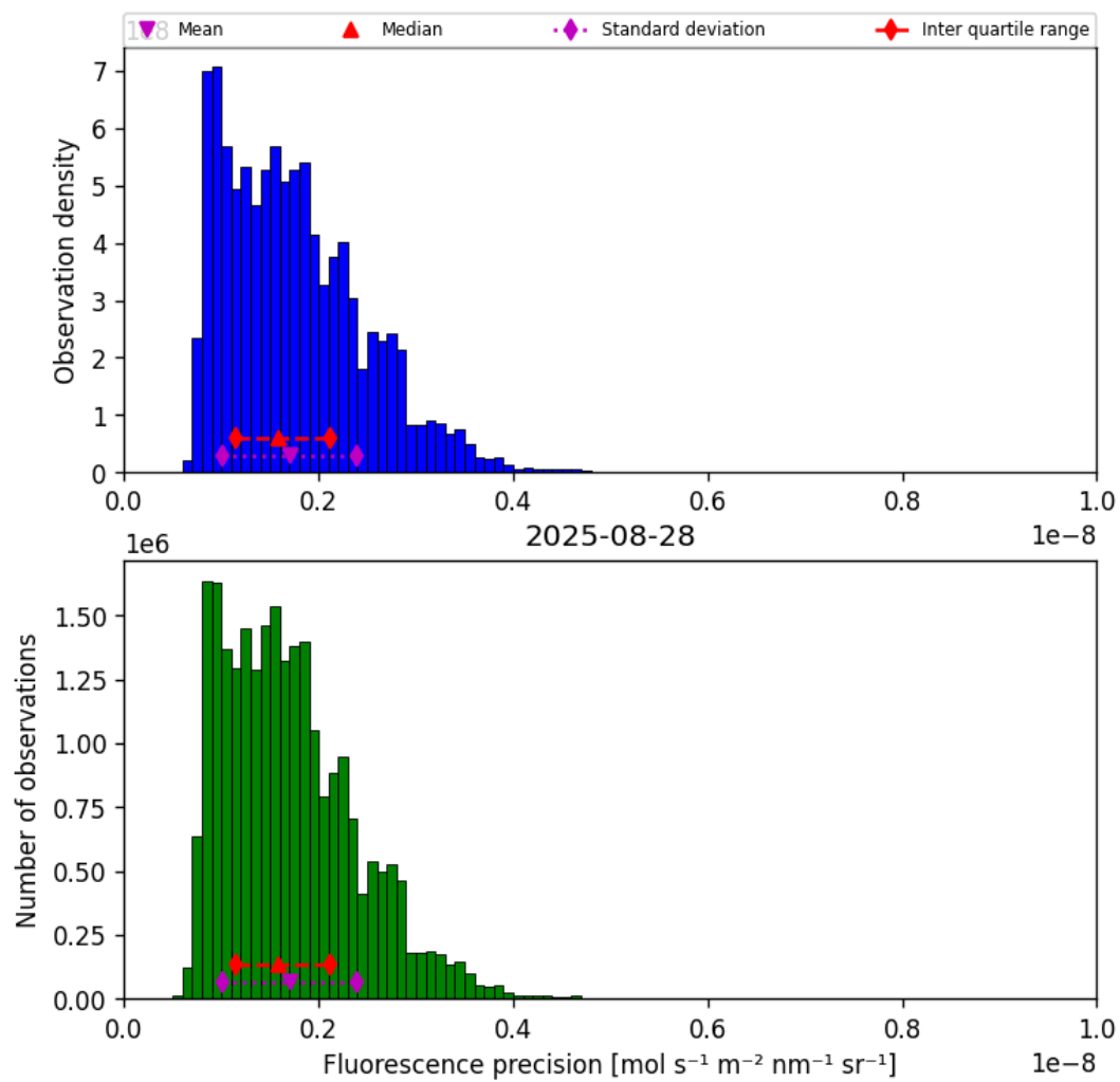
Figure 41: Histogram of “Fluorescence precision” for 2025-08-27 to 2025-08-29
