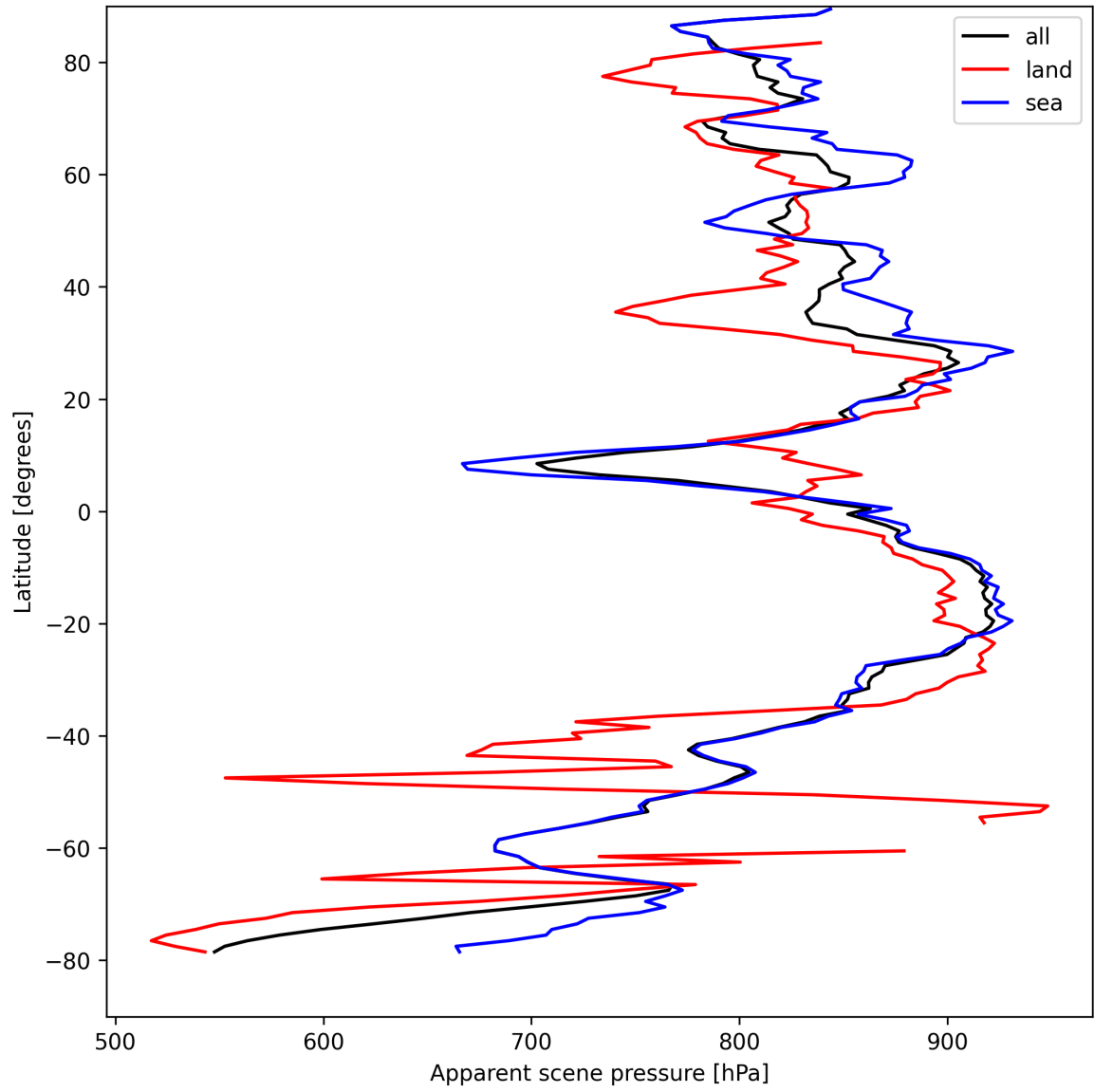
Figure 19: Zonal average of “Apparent scene pressure” for 2025-08-27 to 2025-08-29.
