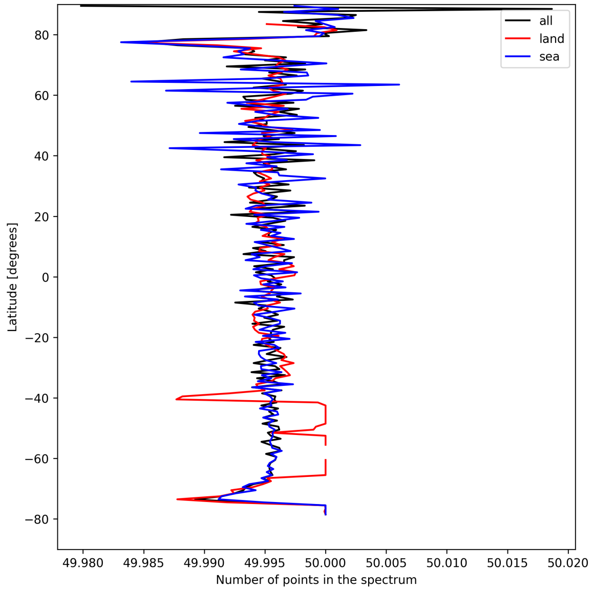
Figure 27: Zonal average of “Number of points in the spectrum” for 2025-08-27 to 2025-08-29.
