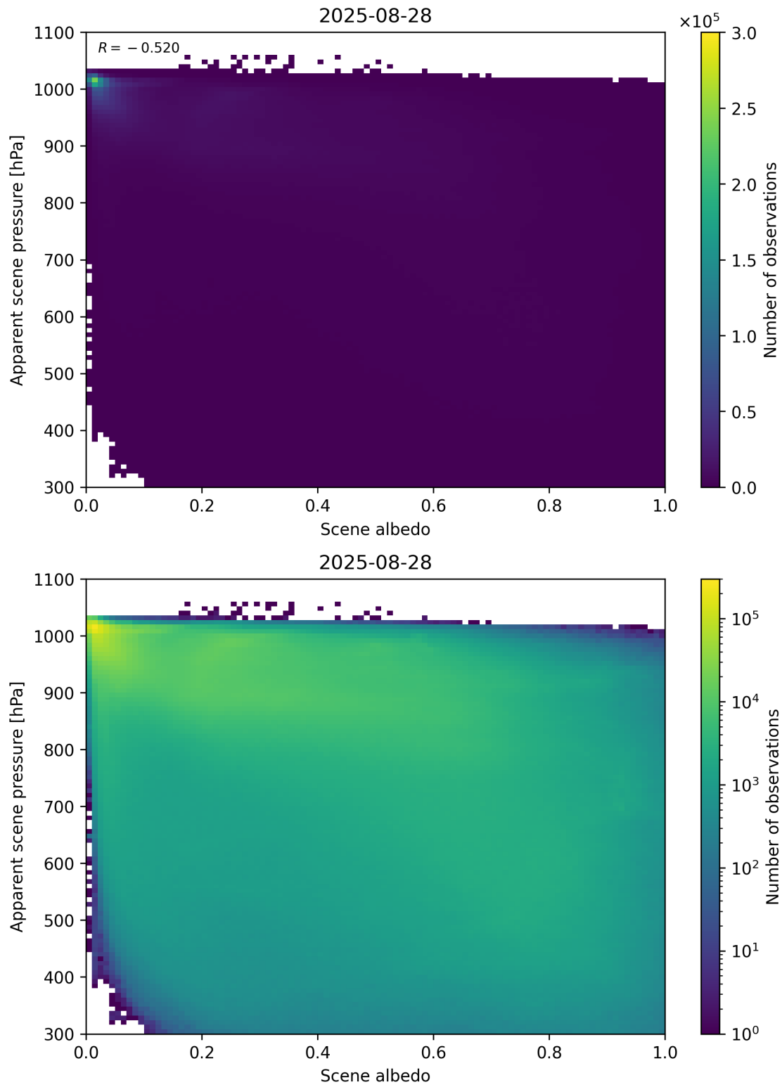
Figure 102: Scatter density plot of “Scene albedo” against “Apparent scene pressure” for 2025-08-27 to 2025-08-29.
