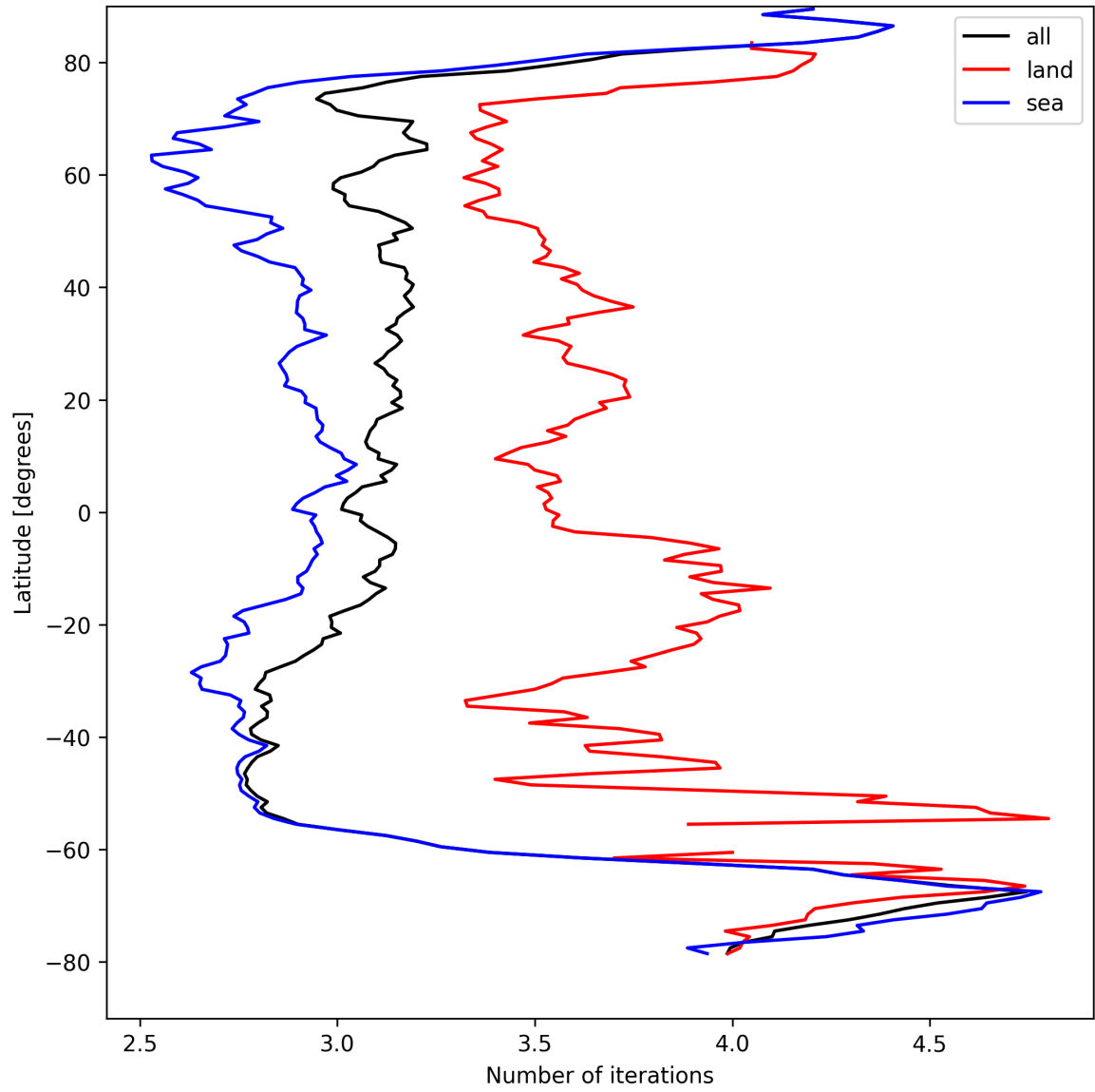
Figure 22: Zonal average of “Number of iterations” for 2025-08-27 to 2025-08-29.
