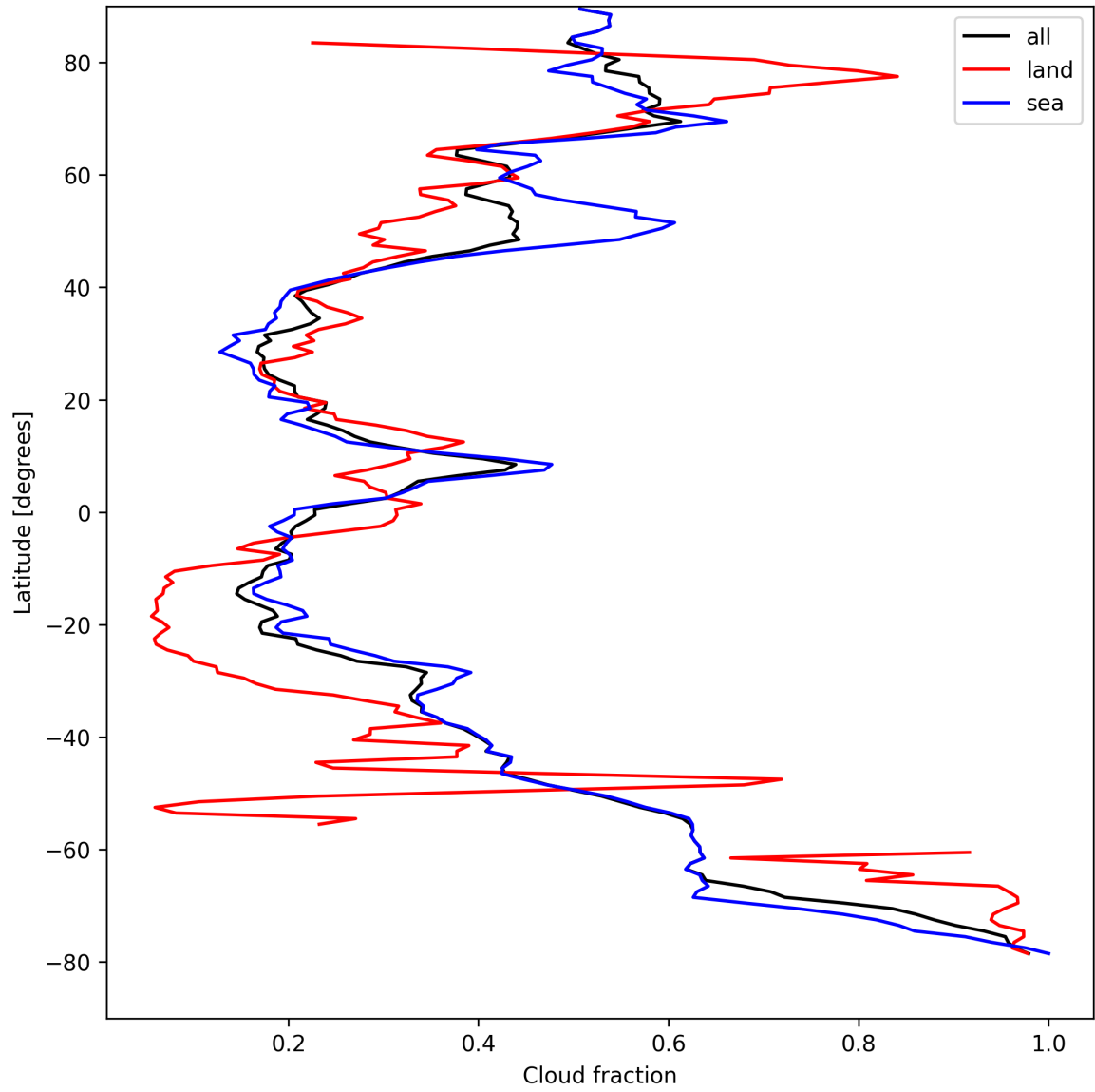
Figure 15: Zonal average of “Cloud fraction” for 2025-08-27 to 2025-08-29.
