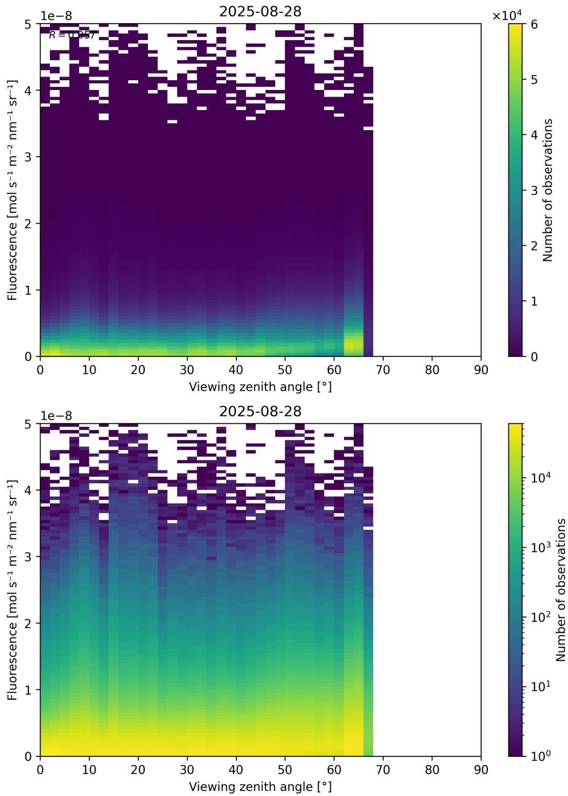
Figure 122: Scatter density plot of “Viewing zenith angle” against “Fluorescence” for 2025-08-27 to 2025-08-29.
