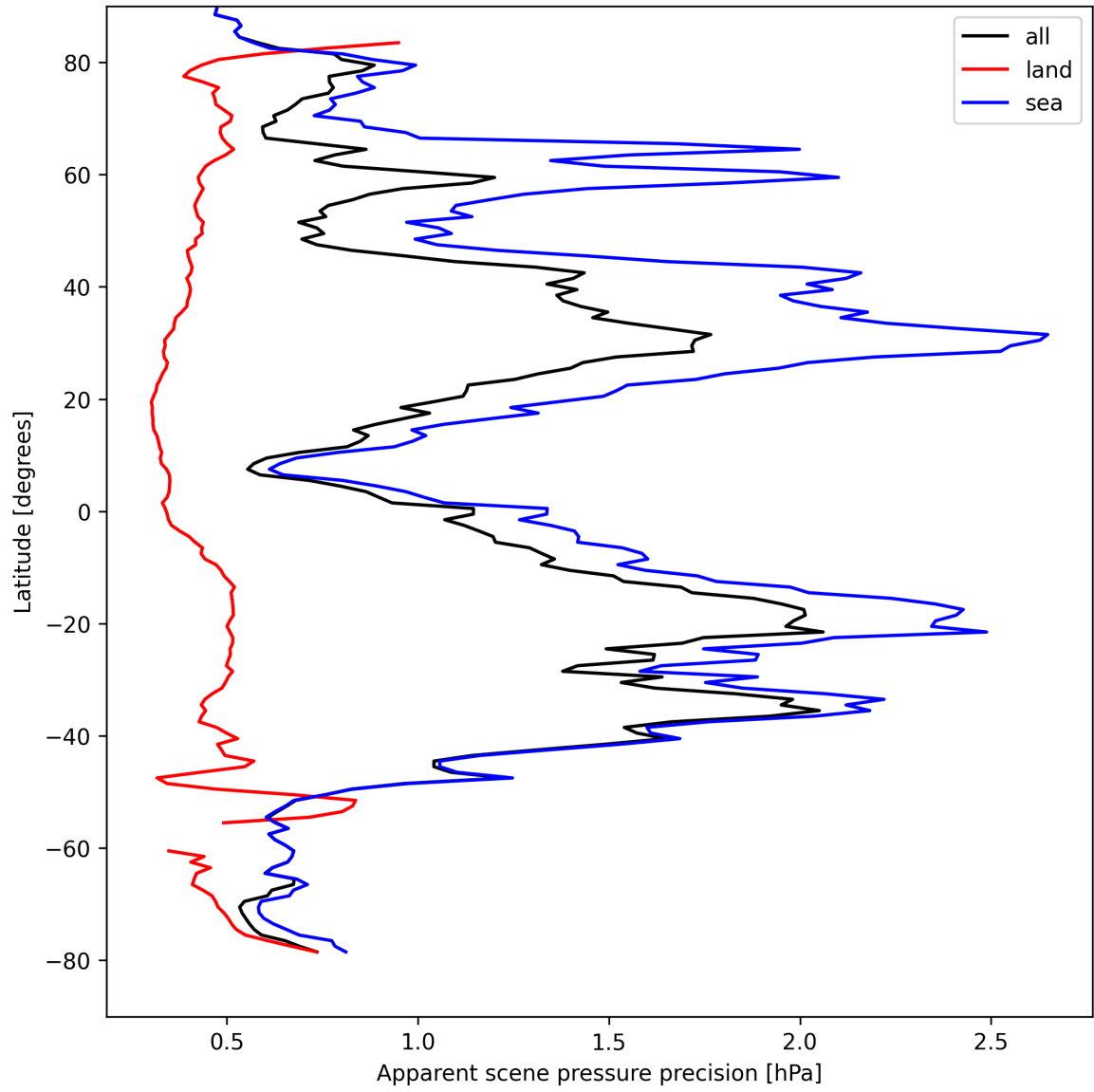
Figure 20: Zonal average of “Apparent scene pressure precision” for 2025-08-27 to 2025-08-29.
