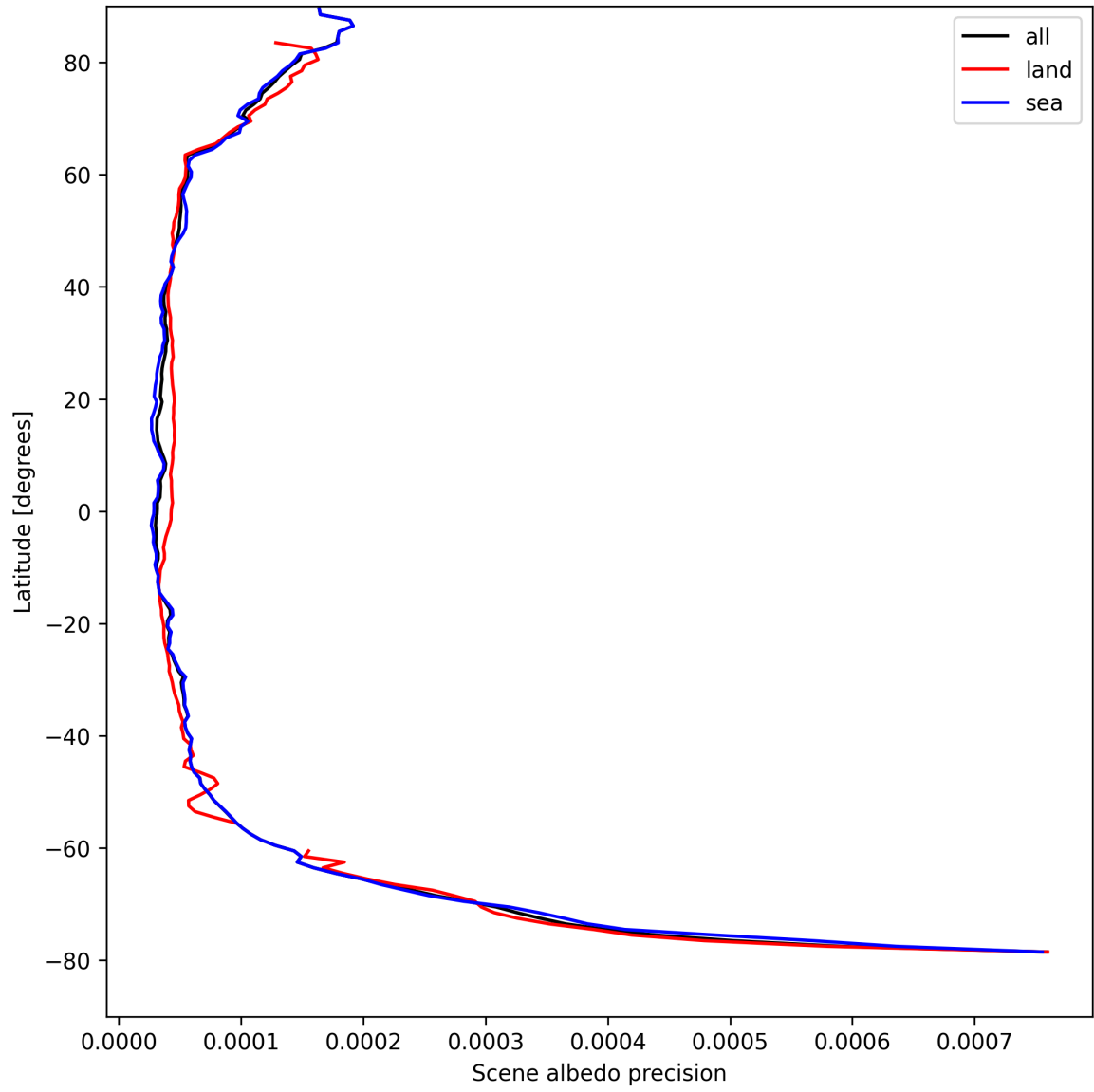
Figure 18: Zonal average of “Scene albedo precision” for 2025-08-27 to 2025-08-29.
