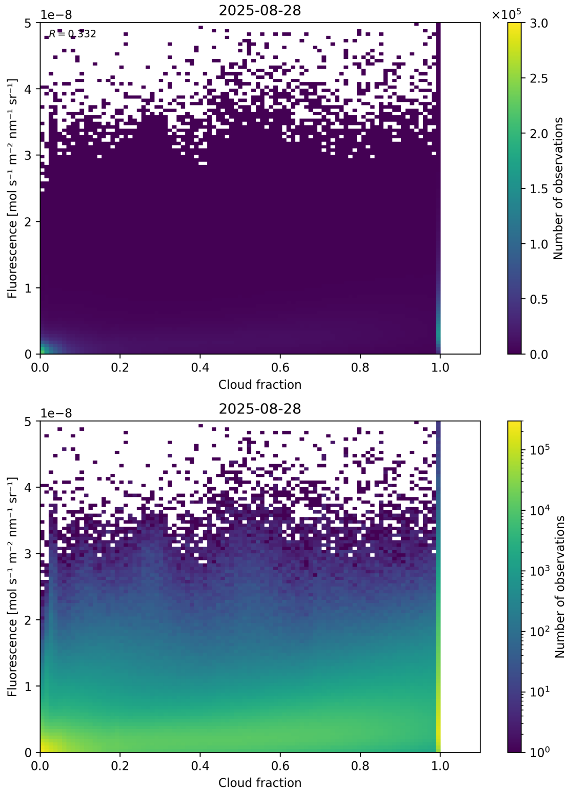
Figure 72: Scatter density plot of “Cloud fraction” against “Fluorescence” for 2025-08-27 to 2025-08-29.
