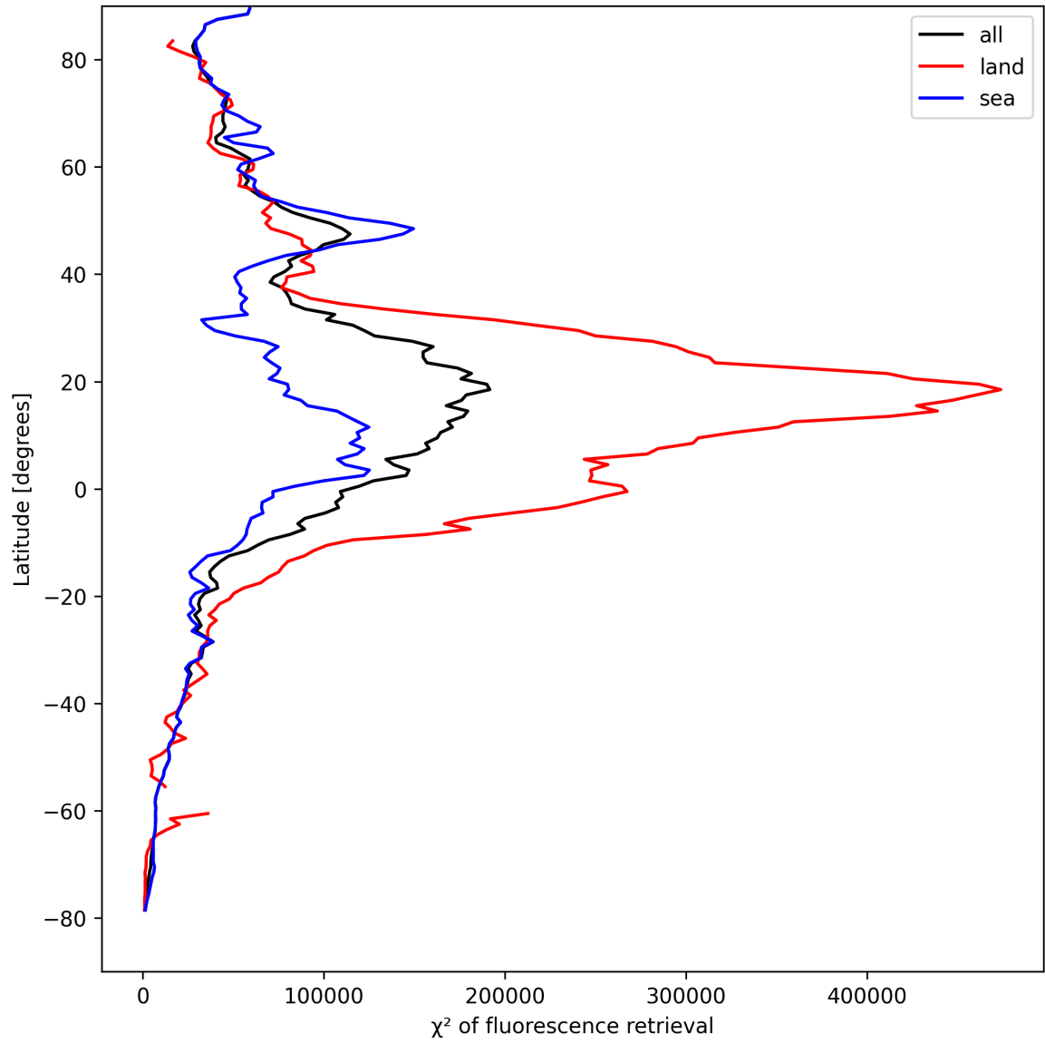
Figure 25: Zonal average of “ \chi^2 of fluorescence retrieval” for 2025-08-27 to 2025-08-29.
