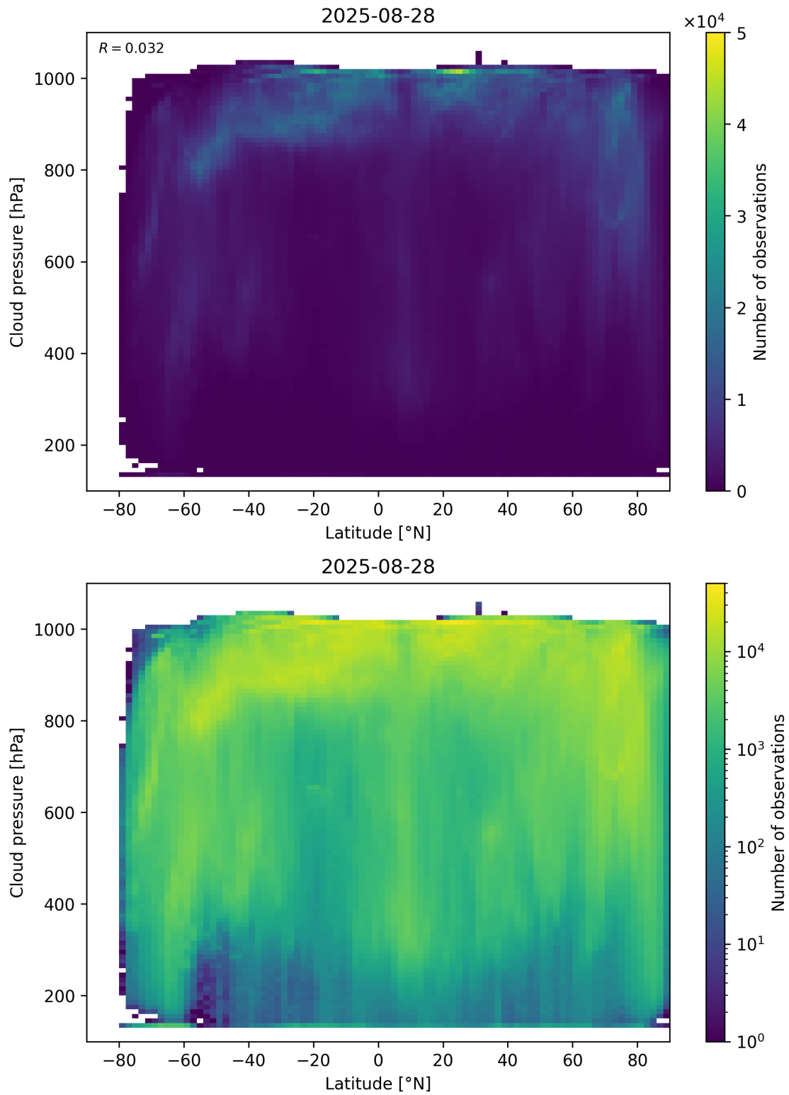
Figure 91: Scatter density plot of “Latitude” against “Cloud pressure” for 2025-08-27 to 2025-08-29.
