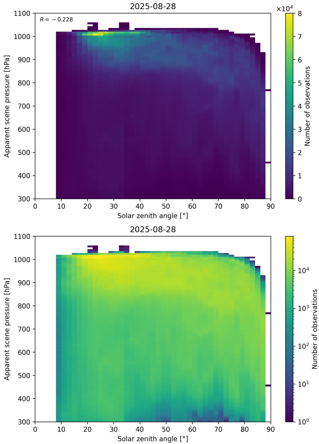
Figure 108: Scatter density plot of “Solar zenith angle” against “Apparent scene pressure” for 2025-08-27 to 2025-08-29.
