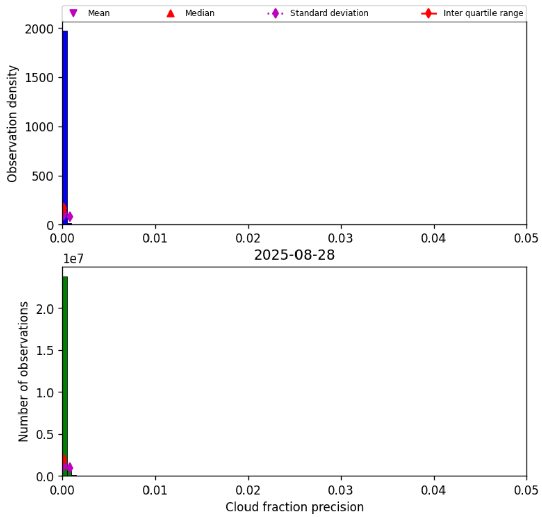
Figure 33: Histogram of “Cloud fraction precision” for 2025-08-27 to 2025-08-29
