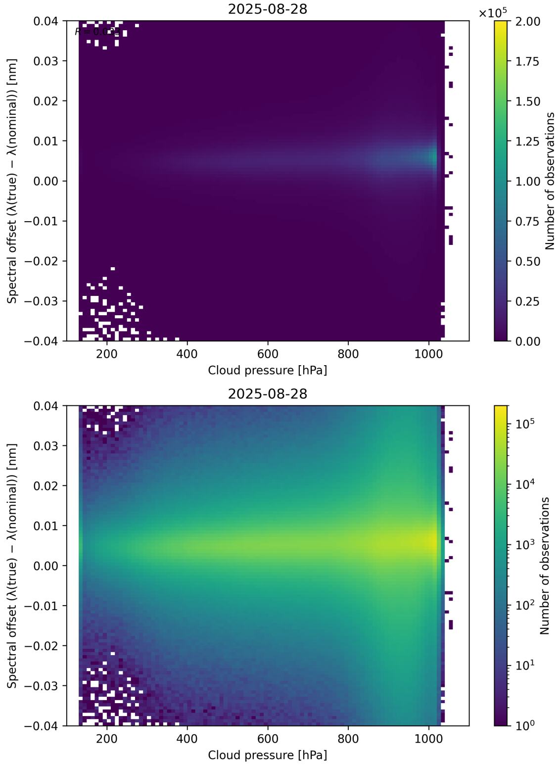
Figure 84: Scatter density plot of “Cloud pressure” against “Spectral offset ( \lambda_{\text{true}} - \lambda_{\text{nominal}} )” for 2025-08-27 to 2025-08-29.
