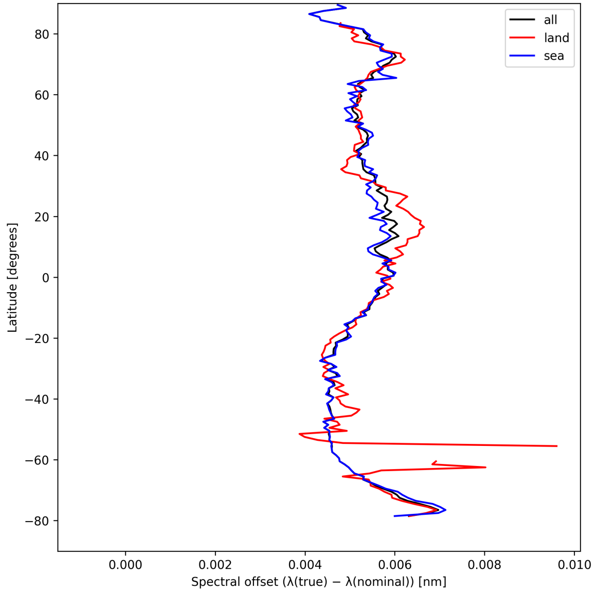
Figure 28: Zonal average of “Spectral offset ( \lambda_{\text{true}} - \lambda_{\text{nominal}} )” for 2025-08-27 to 2025-08-29.
