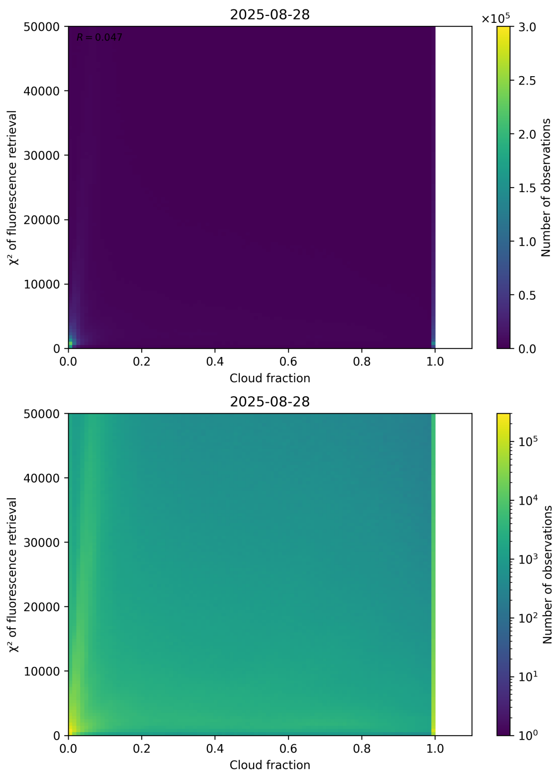
Figure 71: Scatter density plot of “Cloud fraction” against “ \chi^2 of fluorescence retrieval” for 2025-08-27 to 2025-08-29.
