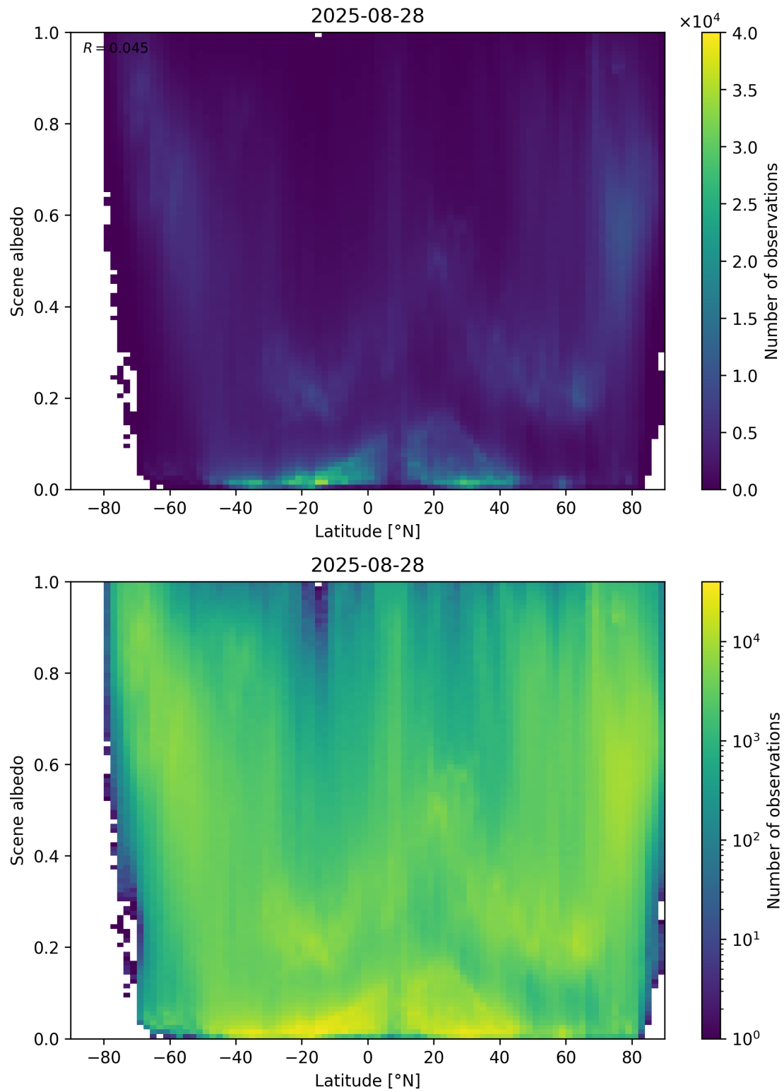
Figure 95: Scatter density plot of “Latitude” against “Scene albedo” for 2025-08-27 to 2025-08-29.
