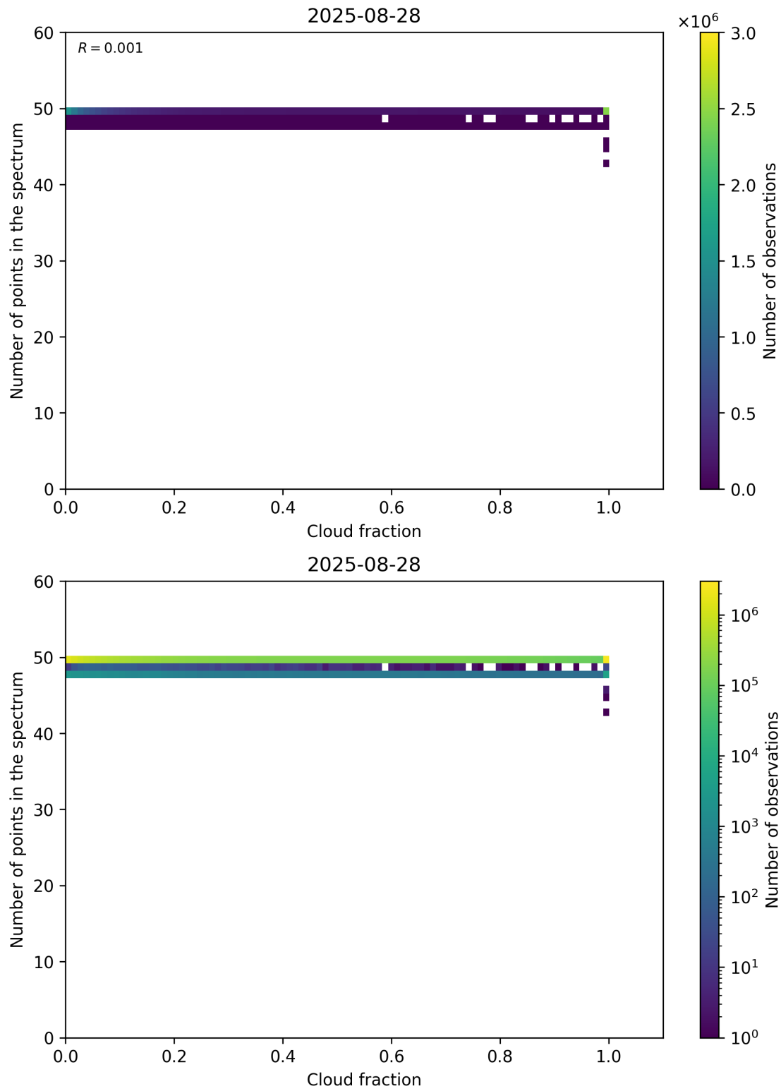
Figure 74: Scatter density plot of “Cloud fraction” against “Number of points in the spectrum” for 2025-08-27 to 2025-08-29.
