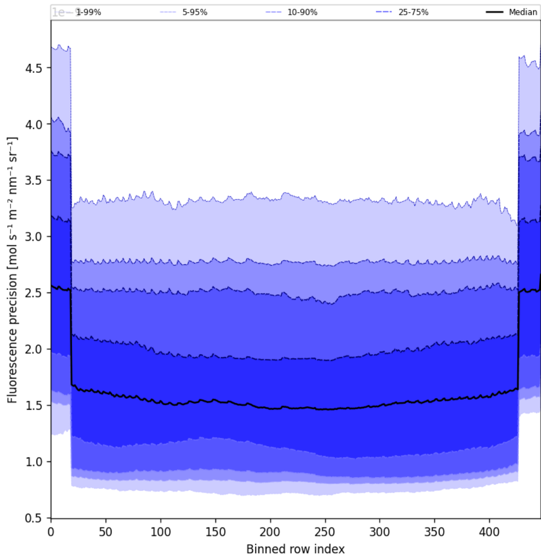
Figure 58: Along track statistics of “Fluorescence precision” for 2025-08-27 to 2025-08-29
