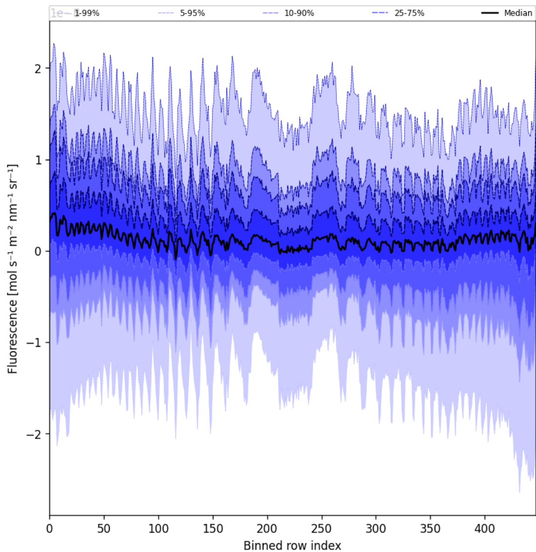
Figure 57: Along track statistics of “Fluorescence” for 2025-08-27 to 2025-08-29
