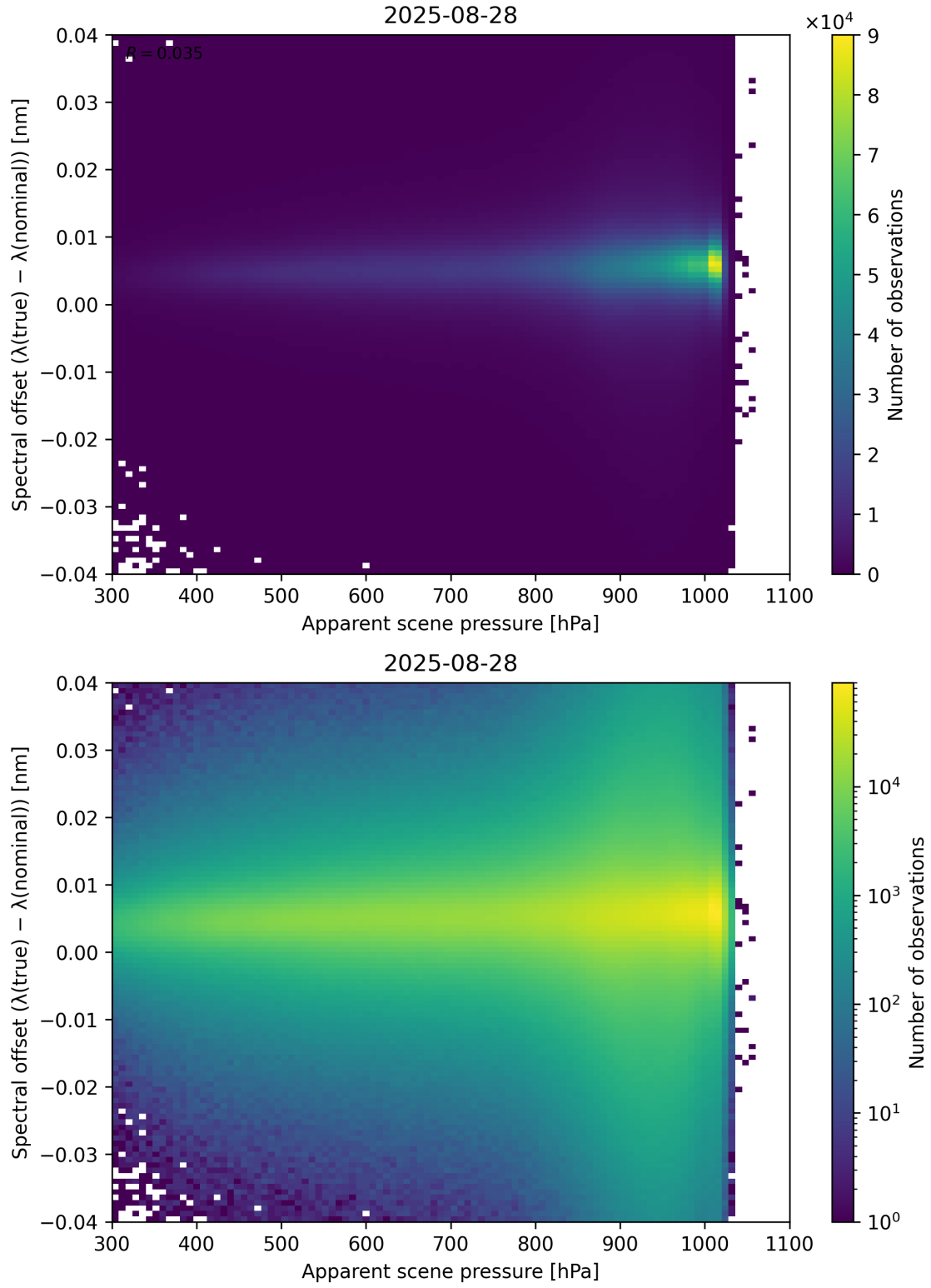
Figure 67: Scatter density plot of “Apparent scene pressure” against “Spectral offset ( \lambda_{\text{true}} - \lambda_{\text{nominal}} )” for 2025-08-27 to 2025-08-29.
