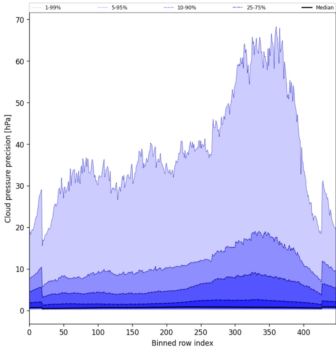
Figure 48: Along track statistics of “Cloud pressure precision” for 2025-08-27 to 2025-08-29
