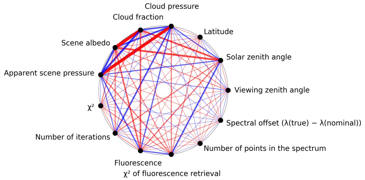
Figure 1: Map of correlation graph for 2025-08-27 to 2025-08-29.
