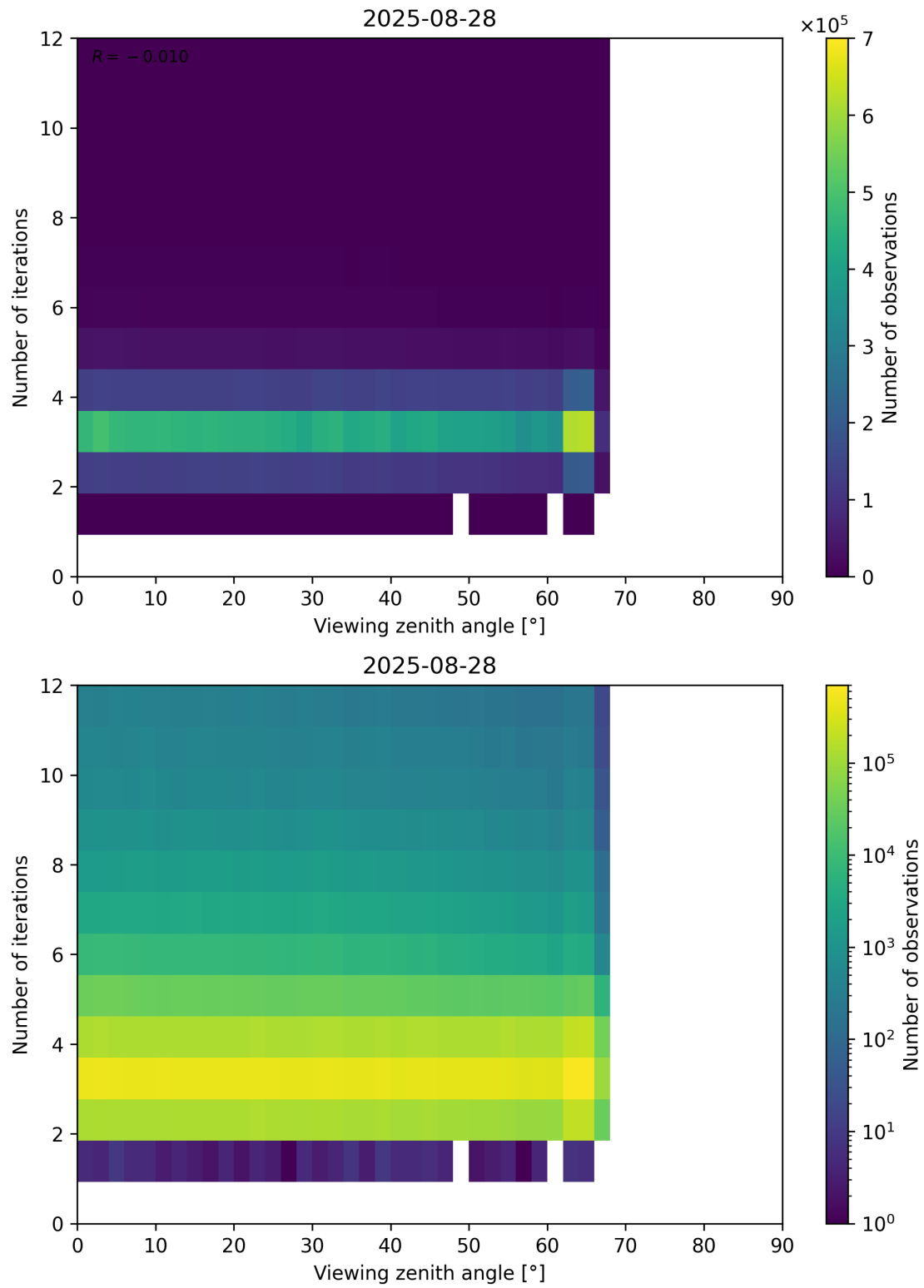
Figure 124: Scatter density plot of “Viewing zenith angle” against “Number of iterations” for 2025-08-27 to 2025-08-29.
