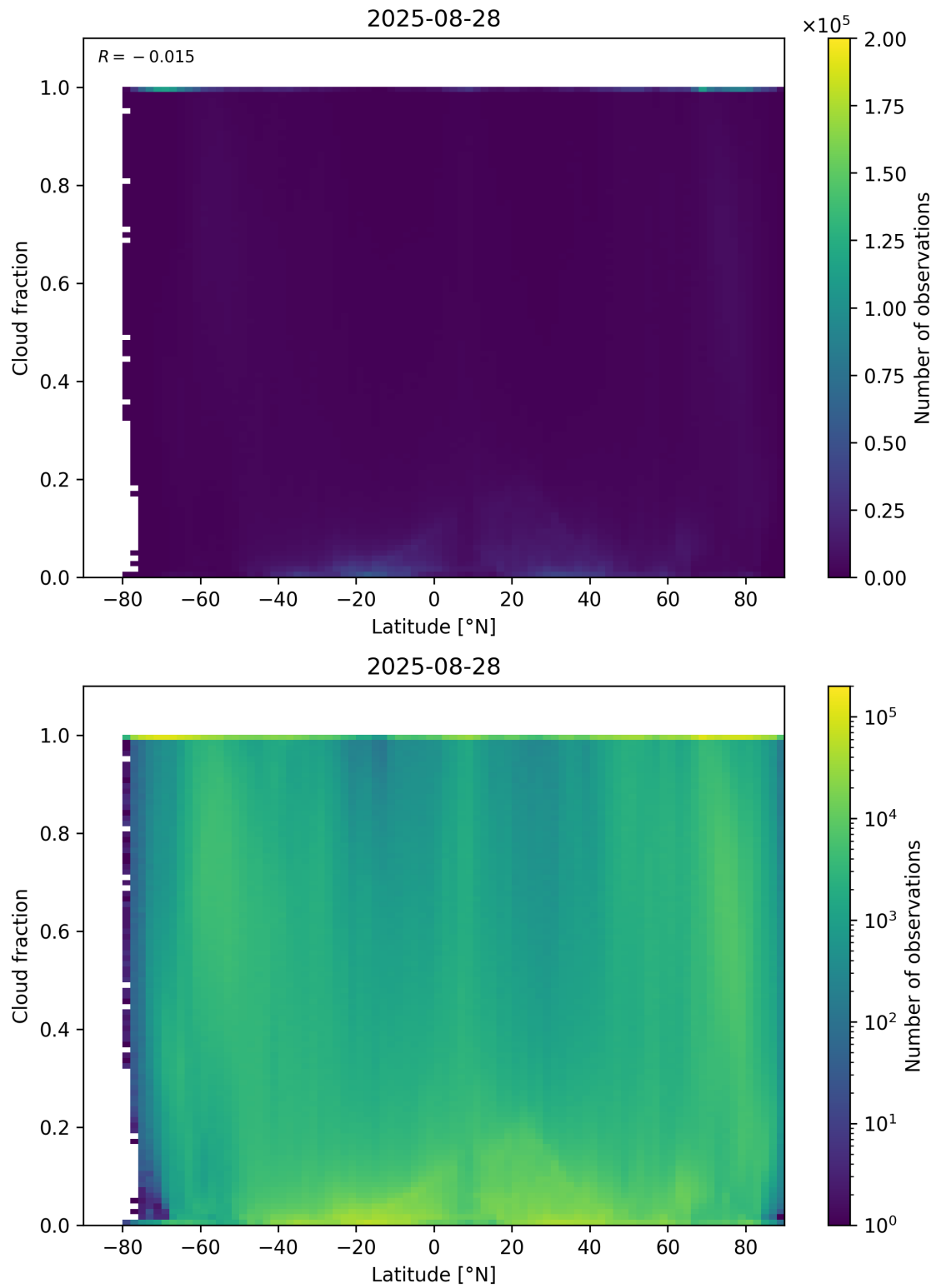
Figure 90: Scatter density plot of “Latitude” against “Cloud fraction” for 2025-08-27 to 2025-08-29.
