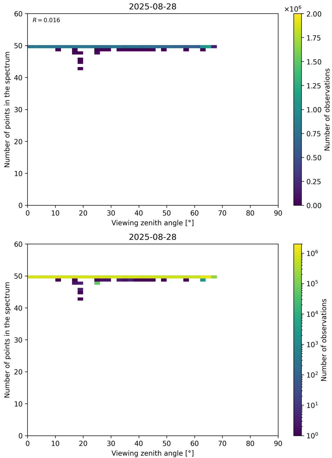
Figure 125: Scatter density plot of “Viewing zenith angle” against “Number of points in the spectrum” for 2025-08-27 to 2025-08-29.
