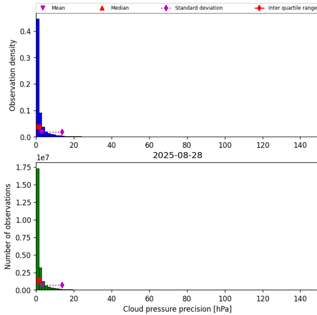
Figure 31: Histogram of “Cloud pressure precision” for 2025-08-27 to 2025-08-29
