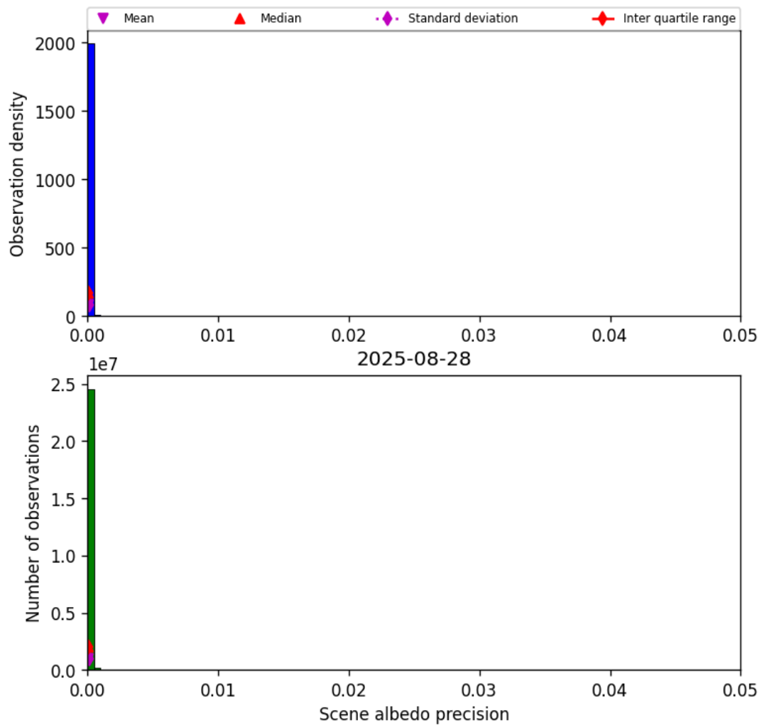
Figure 35: Histogram of “Scene albedo precision” for 2025-08-27 to 2025-08-29
