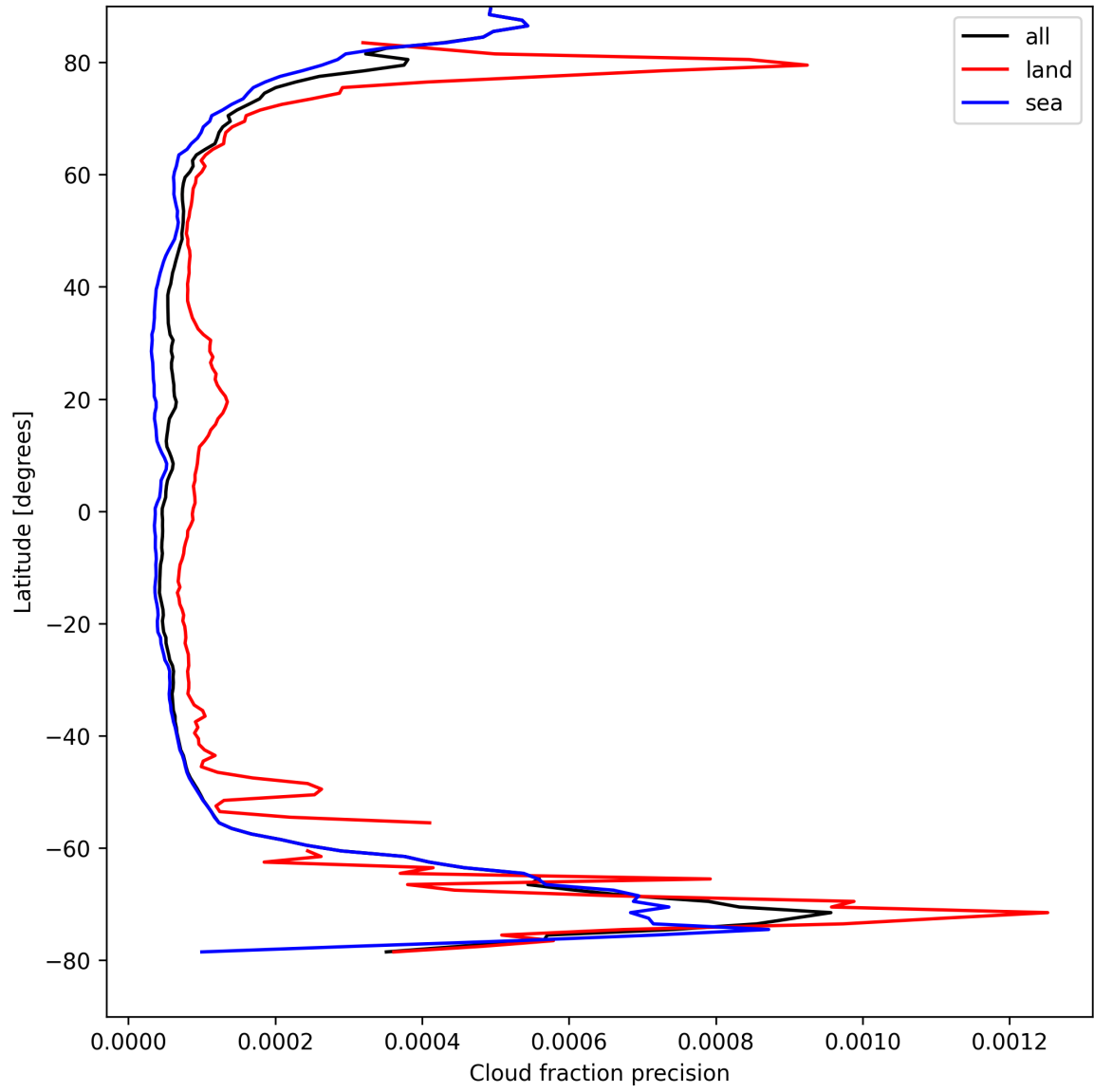
Figure 16: Zonal average of “Cloud fraction precision” for 2025-08-27 to 2025-08-29.
