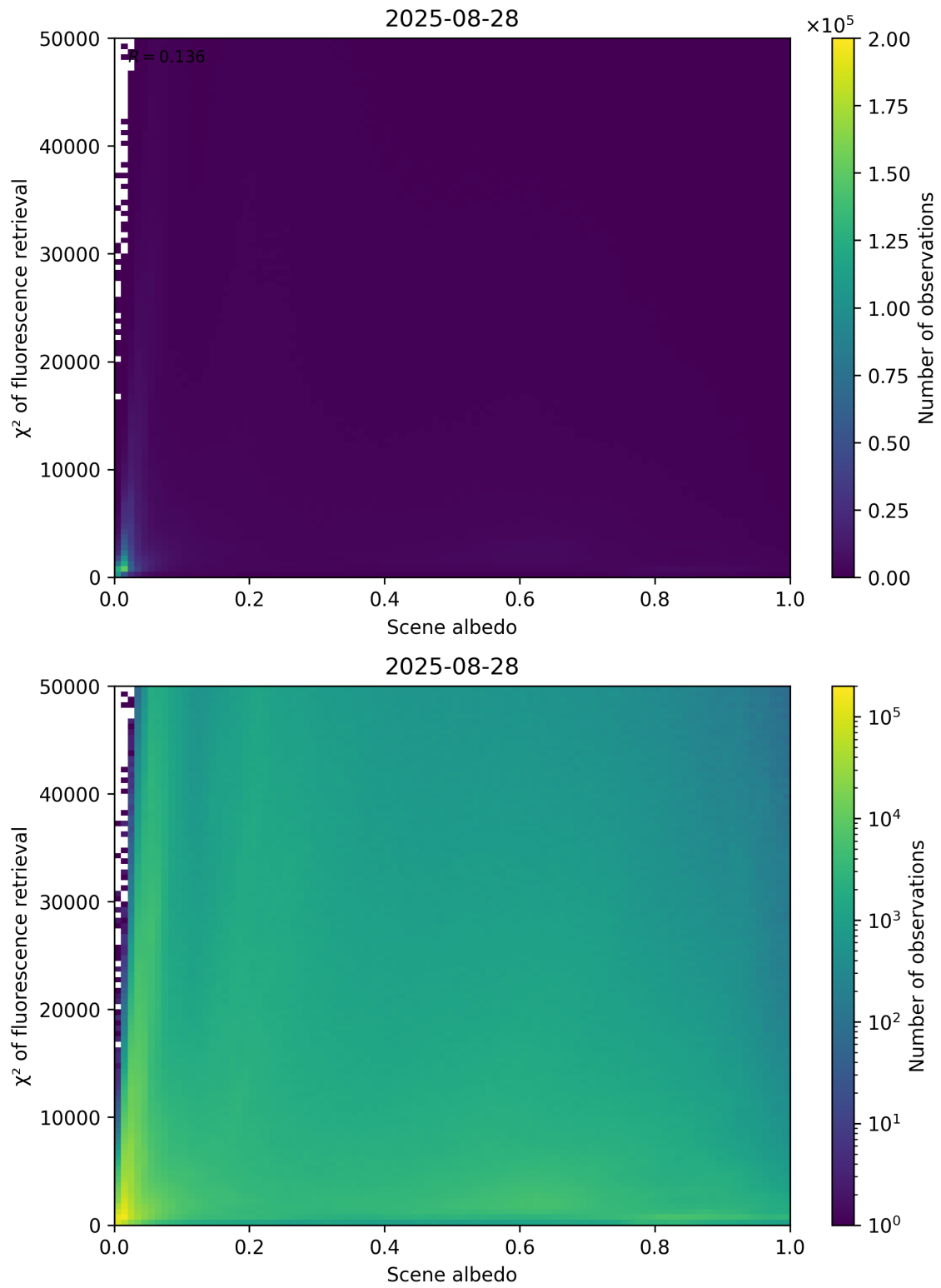
Figure 103: Scatter density plot of “Scene albedo” against “ \chi^2 of fluorescence retrieval” for 2025-08-27 to 2025-08-29.
