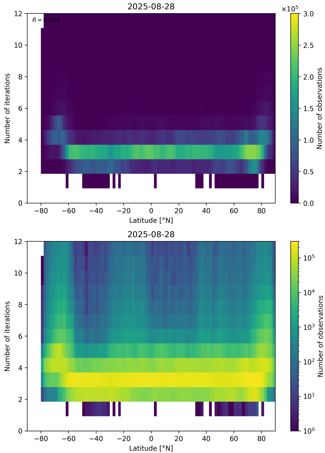
Figure 93: Scatter density plot of “Latitude” against “Number of iterations” for 2025-08-27 to 2025-08-29.
