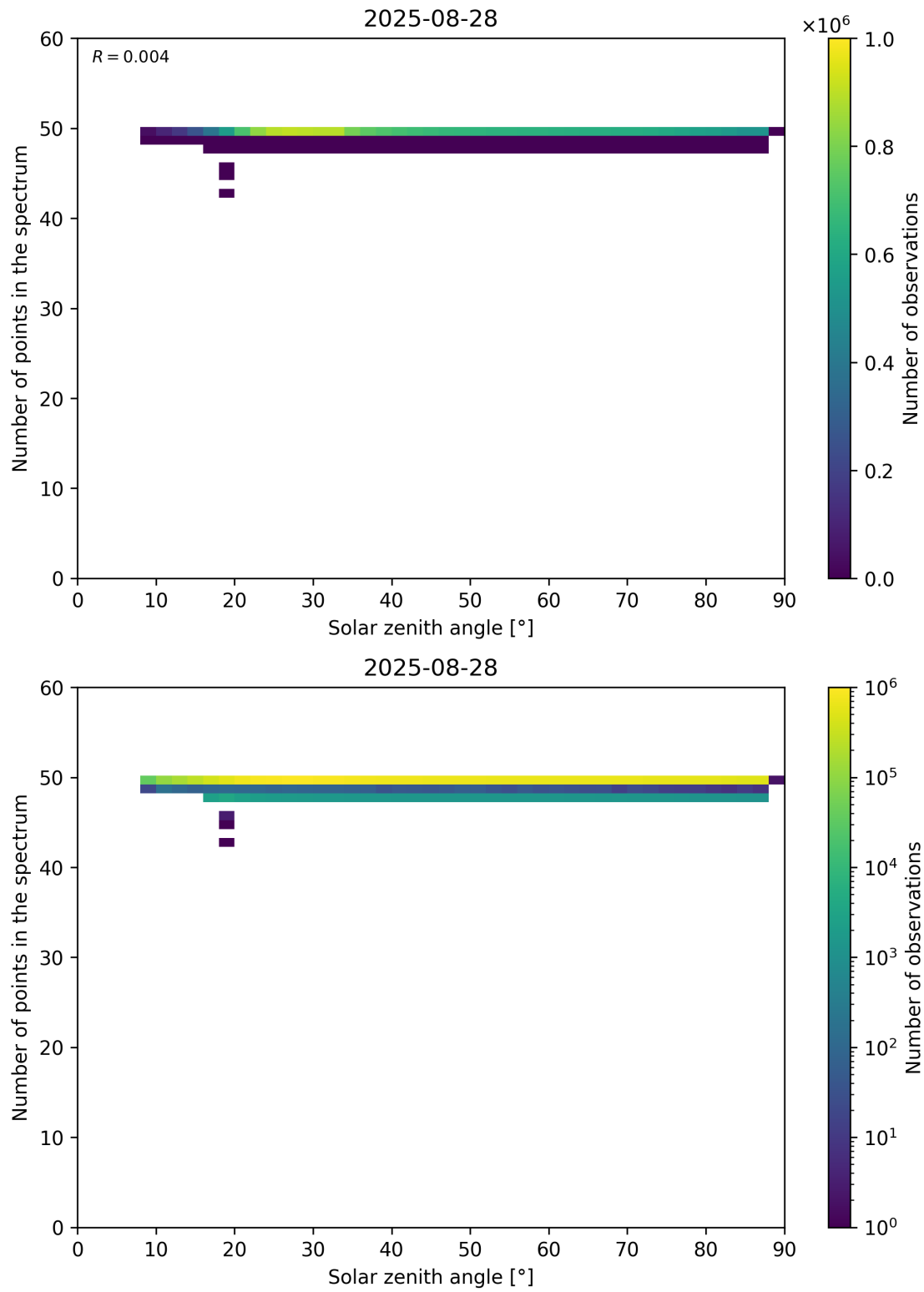
Figure 115: Scatter density plot of “Solar zenith angle” against “Number of points in the spectrum” for 2025-08-27 to 2025-08-29.
