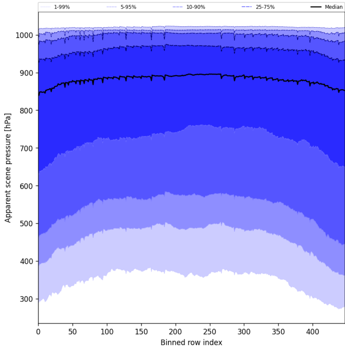
Figure 53: Along track statistics of “Apparent scene pressure” for 2025-08-27 to 2025-08-29
