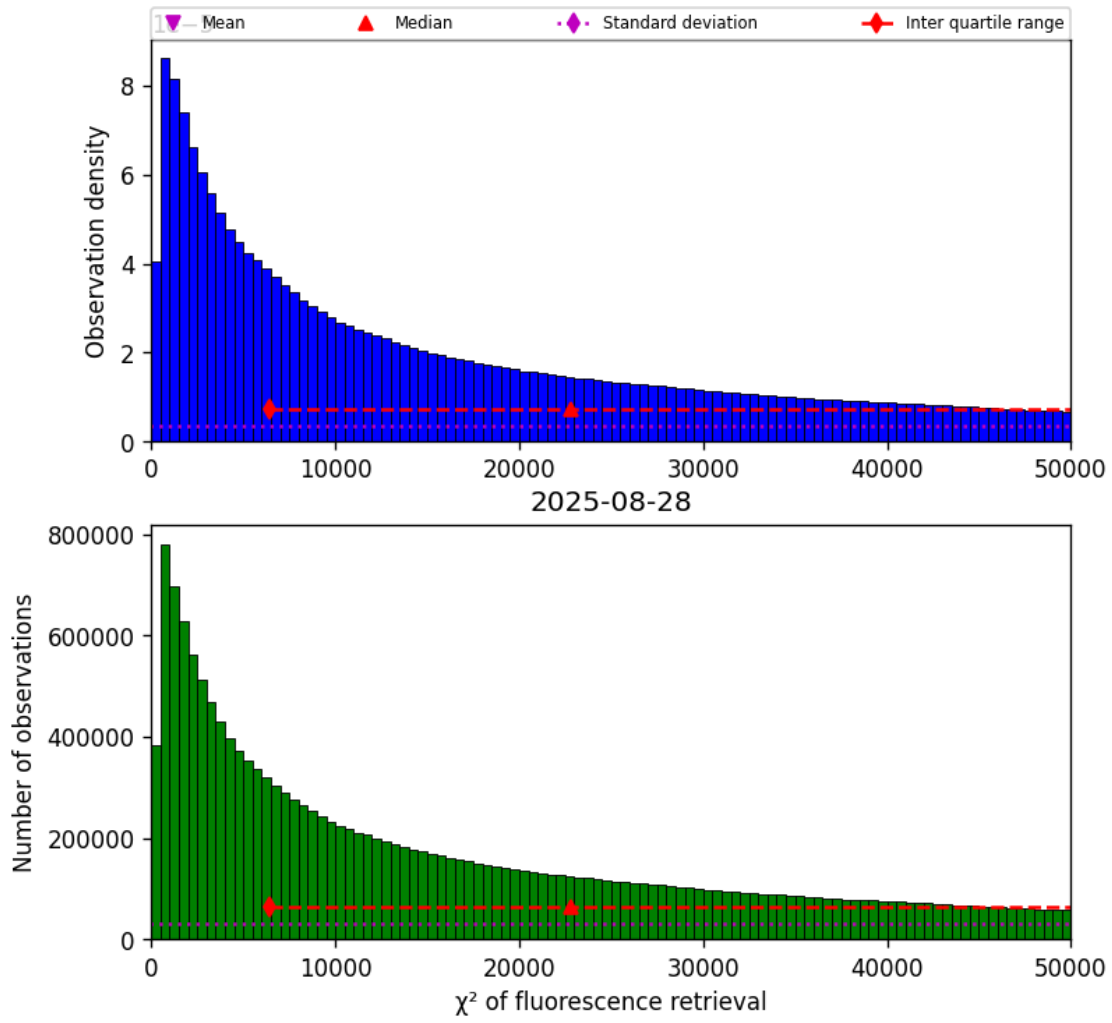
Figure 42: Histogram of “ \chi^2 of fluorescence retrieval” for 2025-08-27 to 2025-08-29
