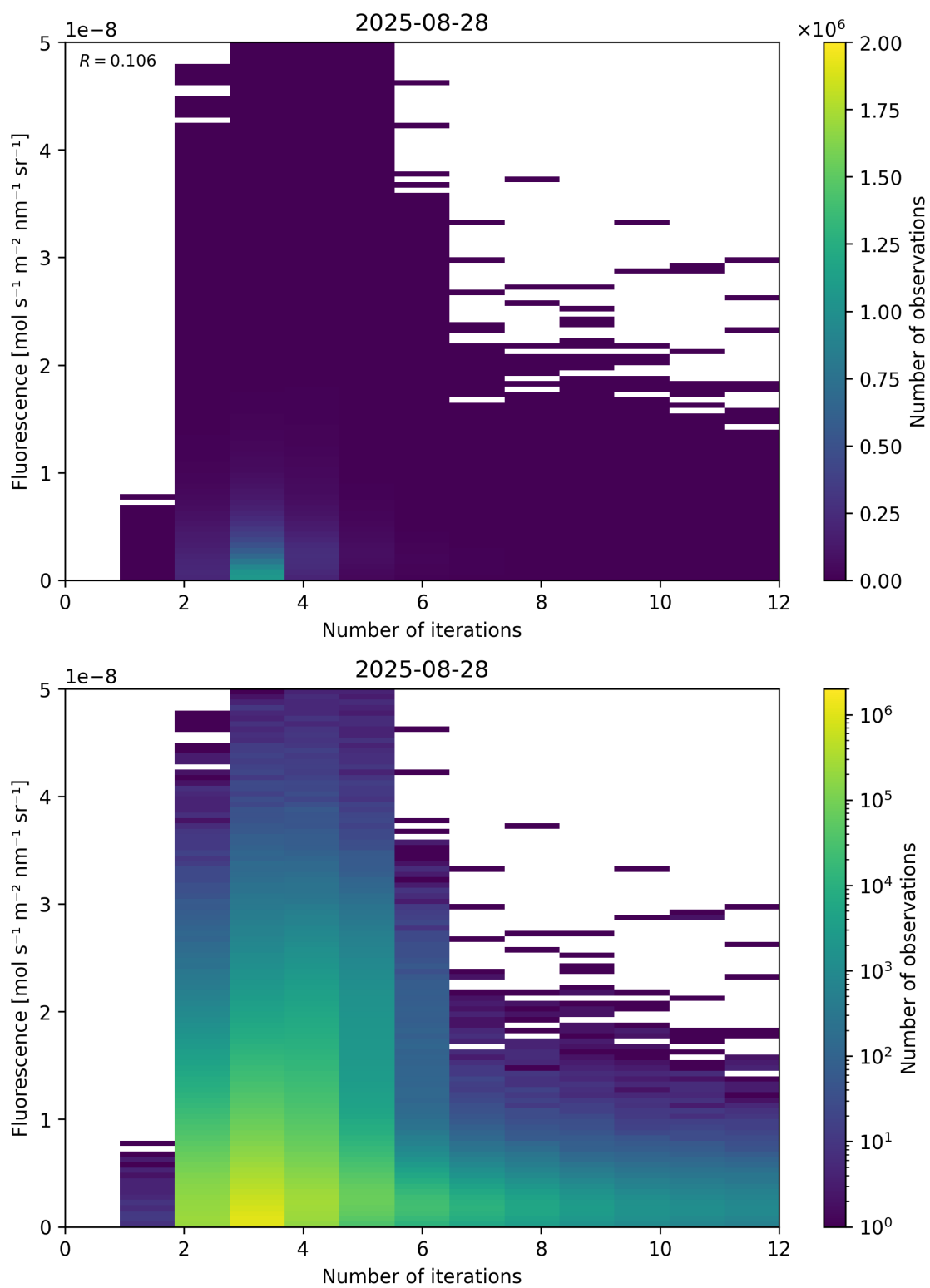
Figure 98: Scatter density plot of “Number of iterations” against “Fluorescence” for 2025-08-27 to 2025-08-29.
