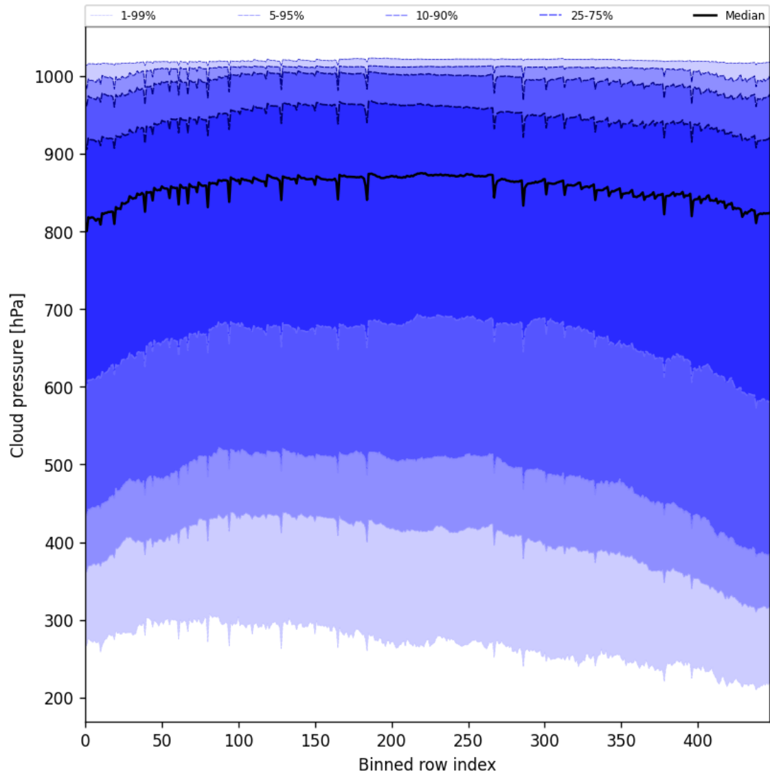
Figure 47: Along track statistics of “Cloud pressure” for 2025-08-27 to 2025-08-29
