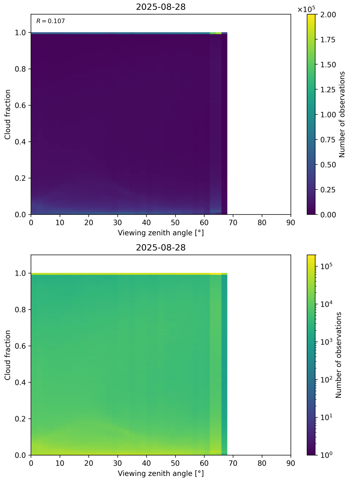
Figure 120: Scatter density plot of “Viewing zenith angle” against “Cloud fraction” for 2025-08-27 to 2025-08-29.
