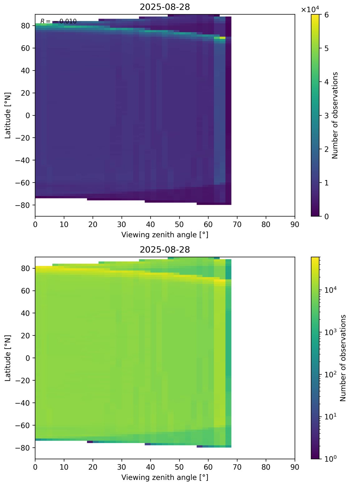
Figure 123: Scatter density plot of “Viewing zenith angle” against “Latitude” for 2025-08-27 to 2025-08-29.
