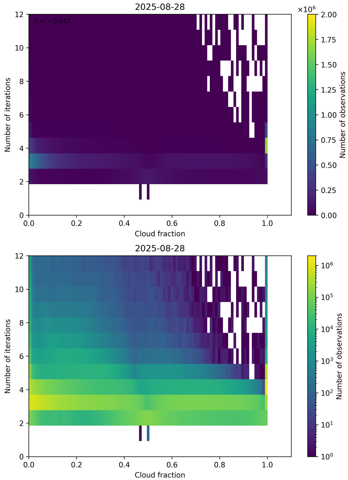
Figure 73: Scatter density plot of “Cloud fraction” against “Number of iterations” for 2025-08-27 to 2025-08-29.
