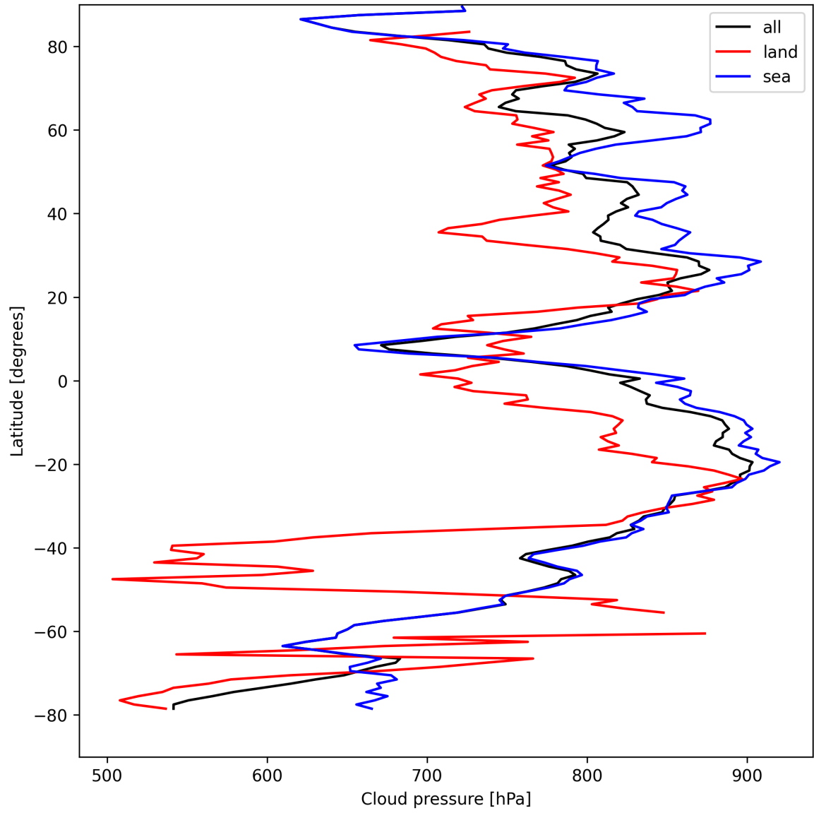
Figure 13: Zonal average of “Cloud pressure” for 2025-08-27 to 2025-08-29.
