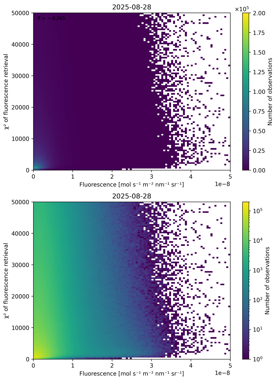
Figure 85: Scatter density plot of “Fluorescence” against “ \chi^2 of fluorescence retrieval” for 2025-08-27 to 2025-08-29.
