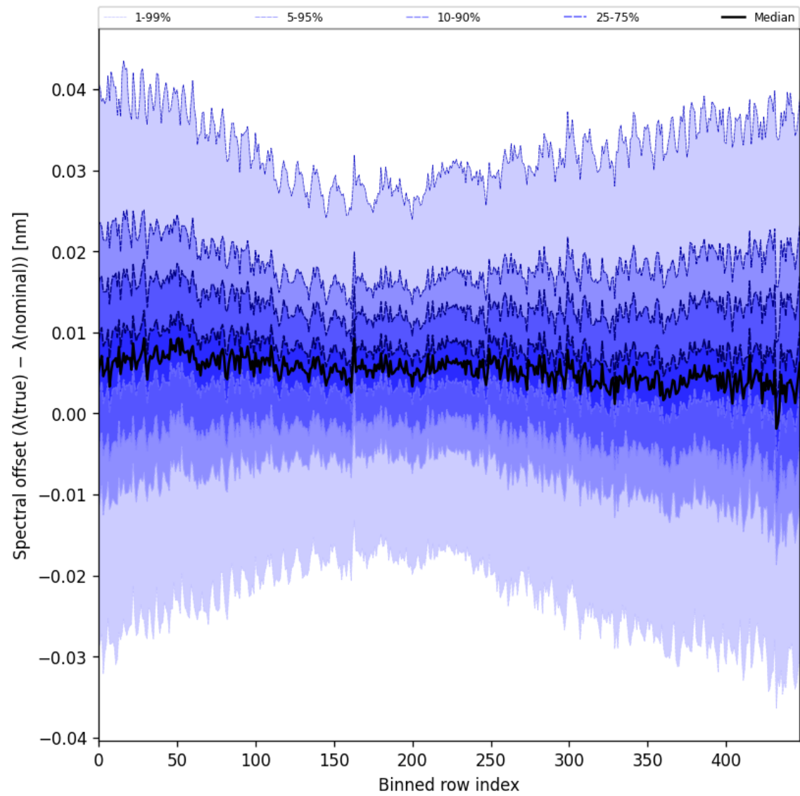
Figure 62: Along track statistics of “Spectral offset ( \lambda_{\text{true}} - \lambda_{\text{nominal}} )” for 2025-08-27 to 2025-08-29
