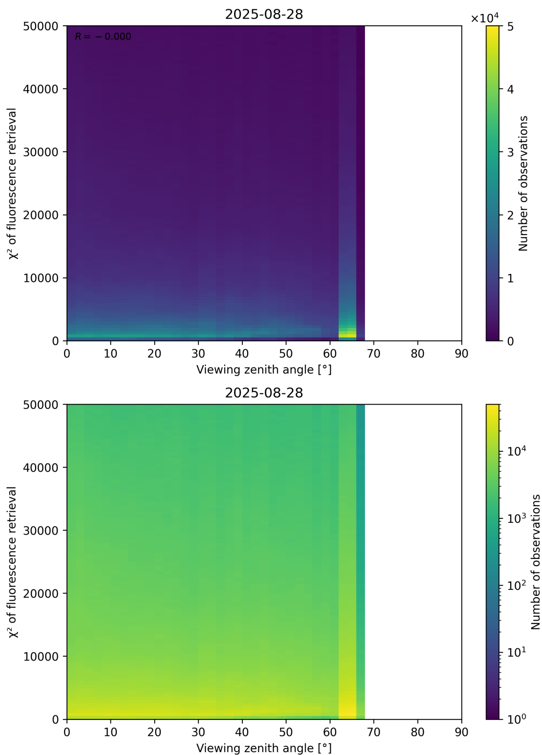
Figure 119: Scatter density plot of “Viewing zenith angle” against “ \chi^2 of fluorescence retrieval” for 2025-08-27 to 2025-08-29.
