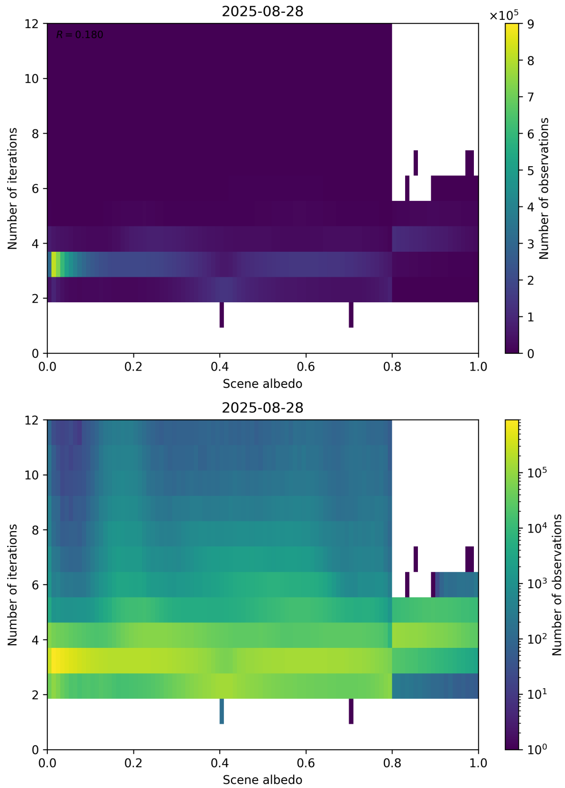
Figure 105: Scatter density plot of “Scene albedo” against “Number of iterations” for 2025-08-27 to 2025-08-29.
