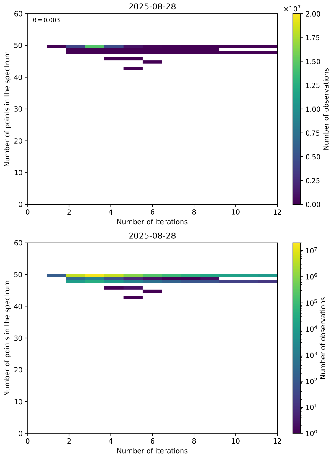
Figure 99: Scatter density plot of “Number of iterations” against “Number of points in the spectrum” for 2025-08-27 to 2025-08-29.
