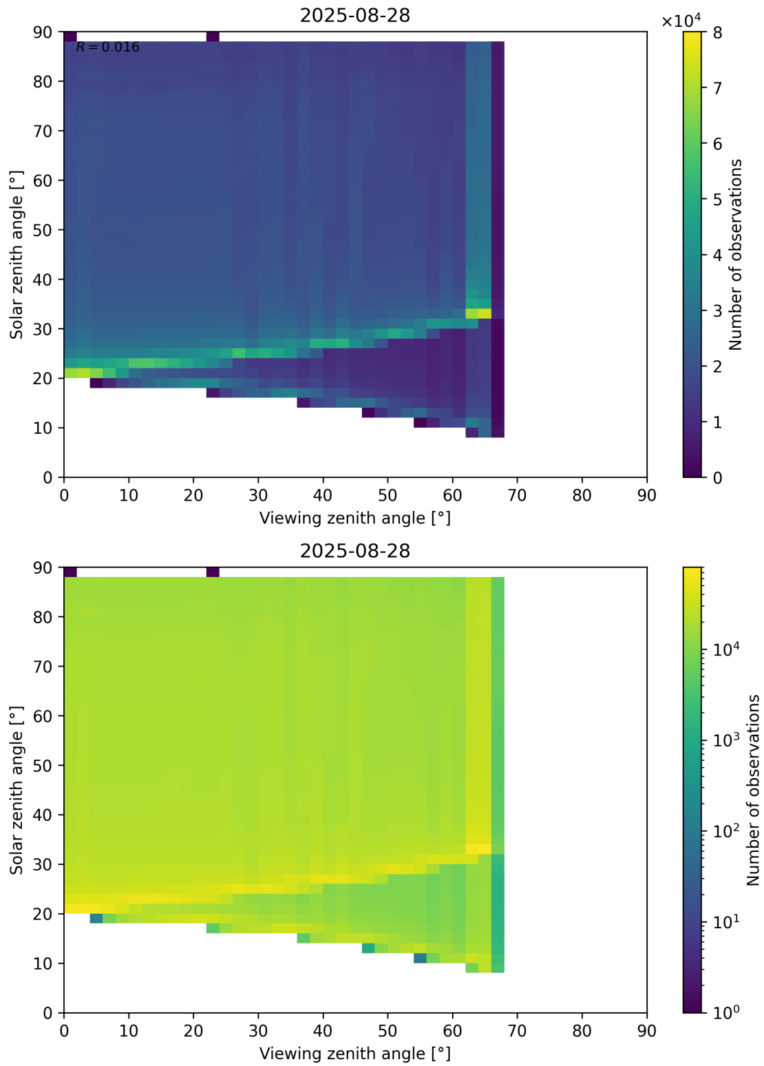
Figure 127: Scatter density plot of “Viewing zenith angle” against “Solar zenith angle” for 2025-08-27 to 2025-08-29.
