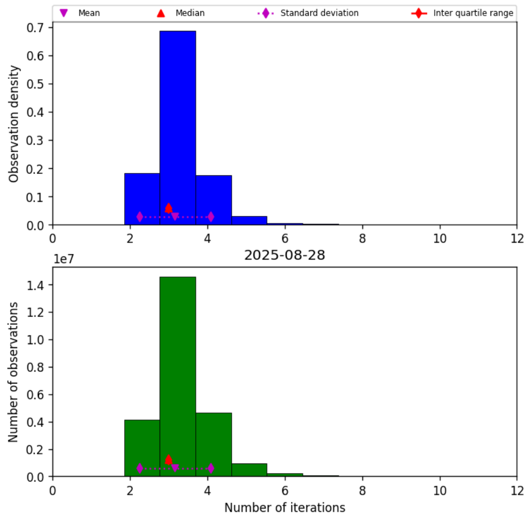
Figure 39: Histogram of “Number of iterations” for 2025-08-27 to 2025-08-29
