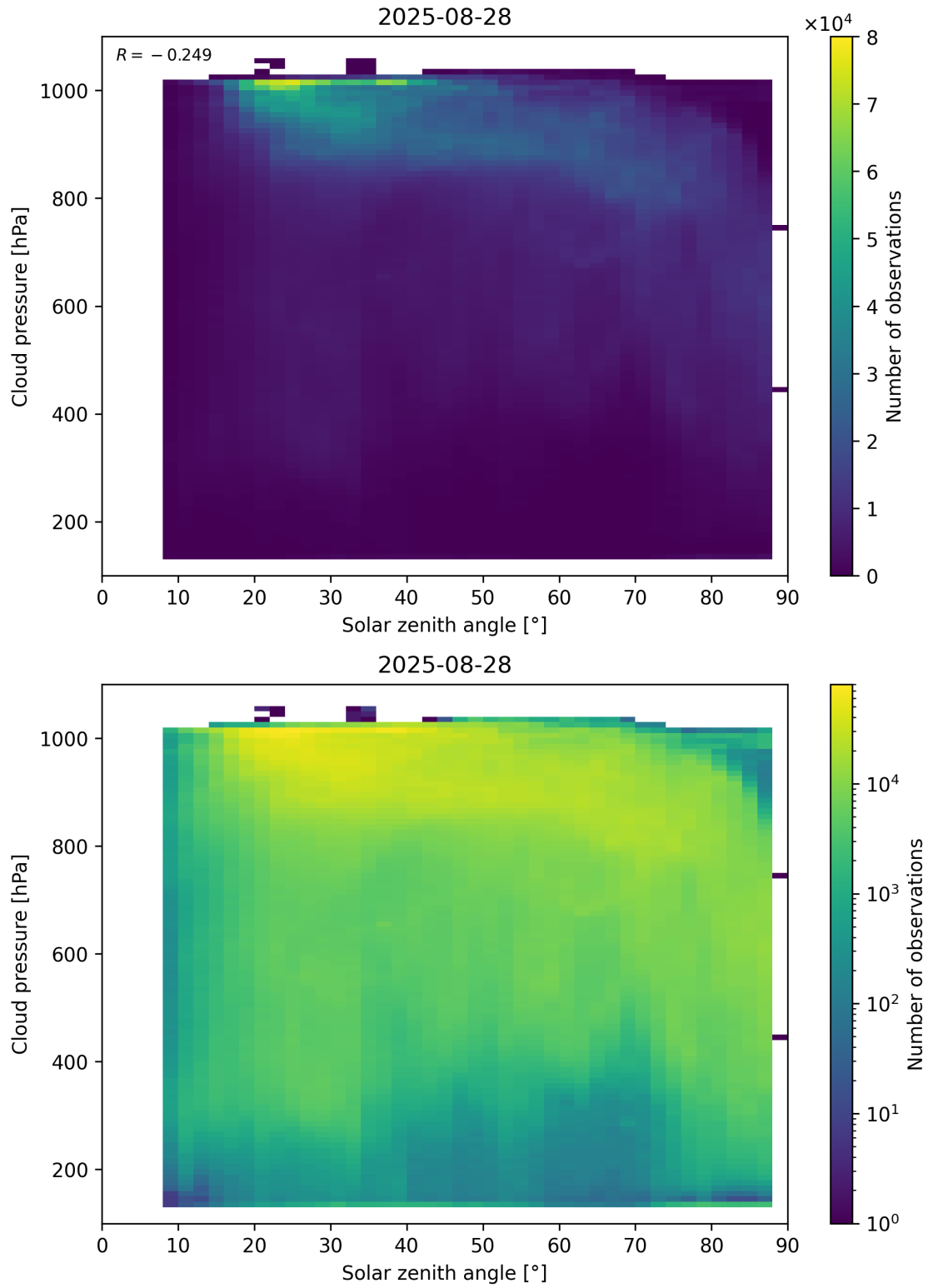
Figure 111: Scatter density plot of “Solar zenith angle” against “Cloud pressure” for 2025-08-27 to 2025-08-29.
