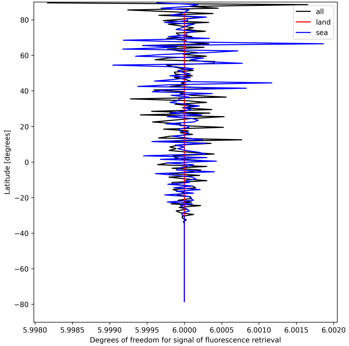
Figure 26: Zonal average of “Degrees of freedom for signal of fluorescence retrieval” for 2025-08-27 to 2025-08-29.
