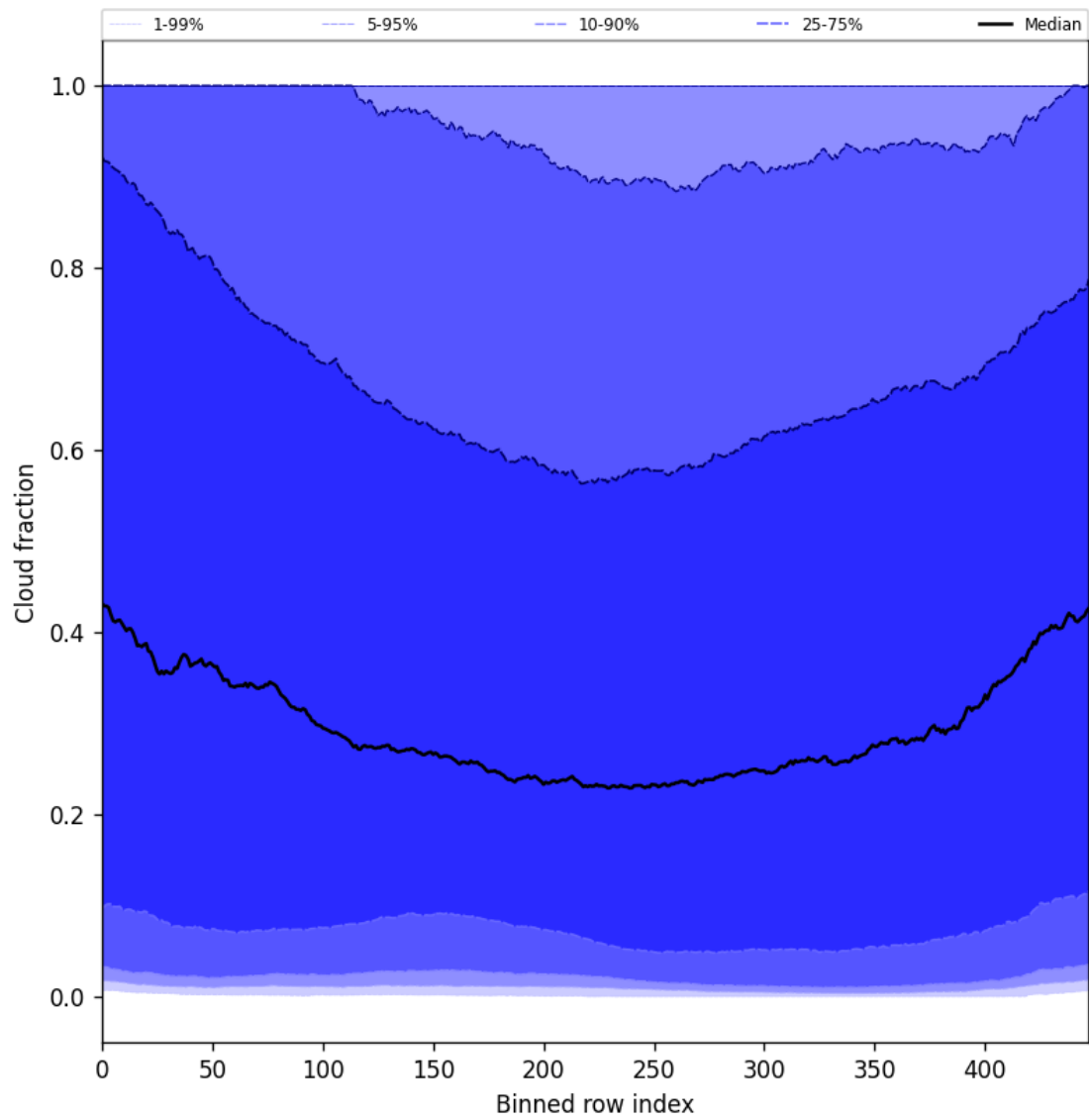
Figure 49: Along track statistics of “Cloud fraction” for 2025-08-27 to 2025-08-29
