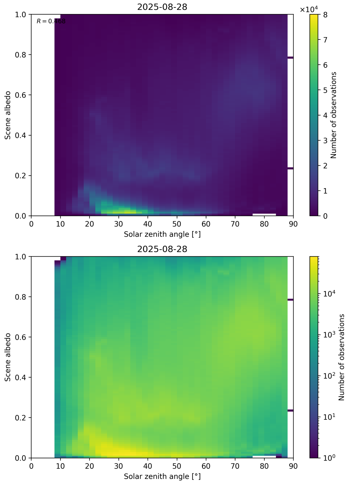
Figure 116: Scatter density plot of “Solar zenith angle” against “Scene albedo” for 2025-08-27 to 2025-08-29.
