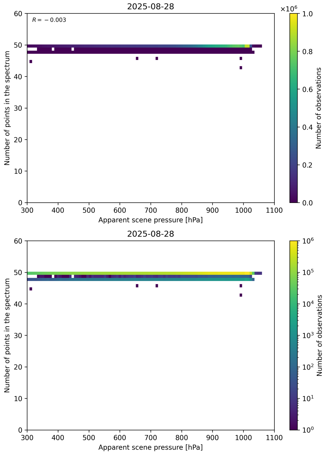
Figure 66: Scatter density plot of “Apparent scene pressure” against “Number of points in the spectrum” for 2025-08-27 to 2025-08-29.
