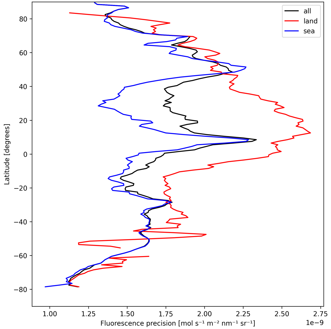
Figure 24: Zonal average of “Fluorescence precision” for 2025-08-27 to 2025-08-29.
