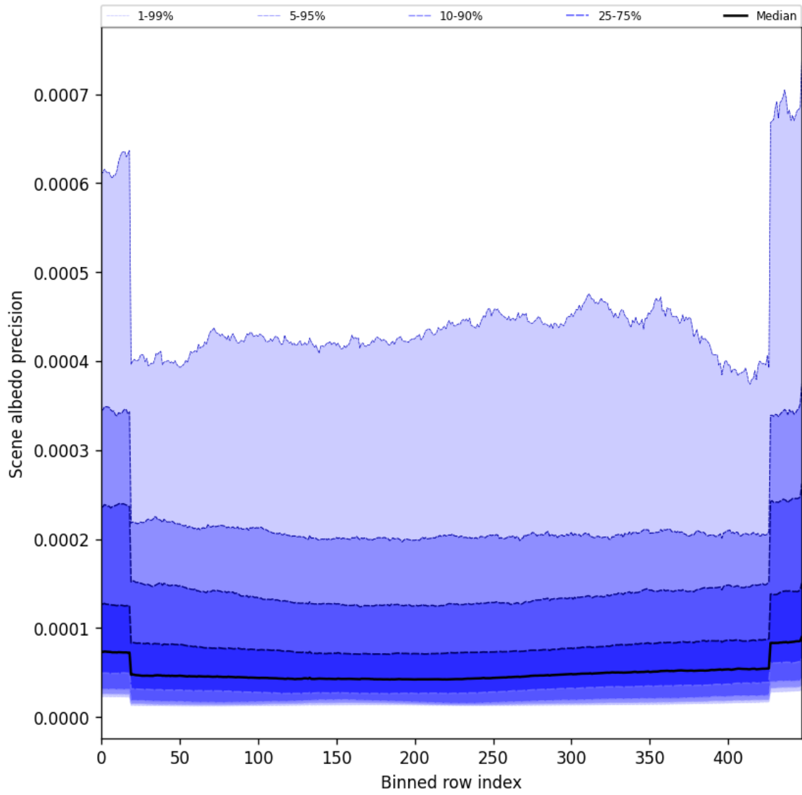
Figure 52: Along track statistics of “Scene albedo precision” for 2025-08-27 to 2025-08-29
