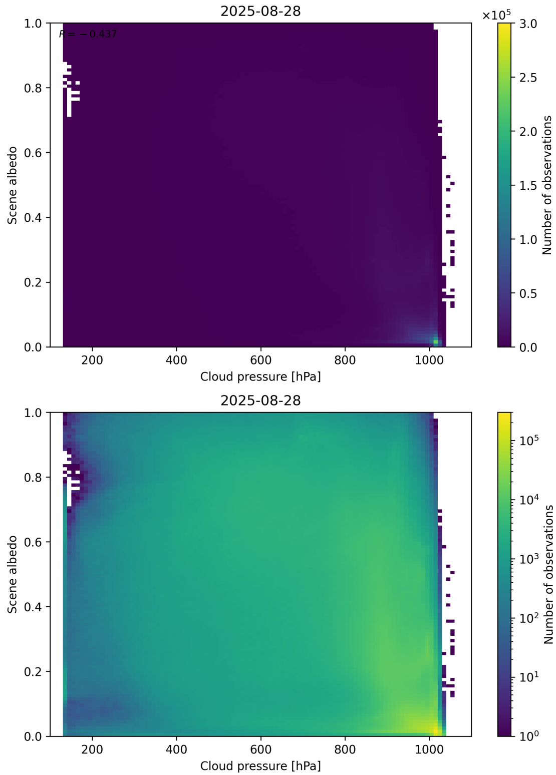
Figure 83: Scatter density plot of “Cloud pressure” against “Scene albedo” for 2025-08-27 to 2025-08-29.
