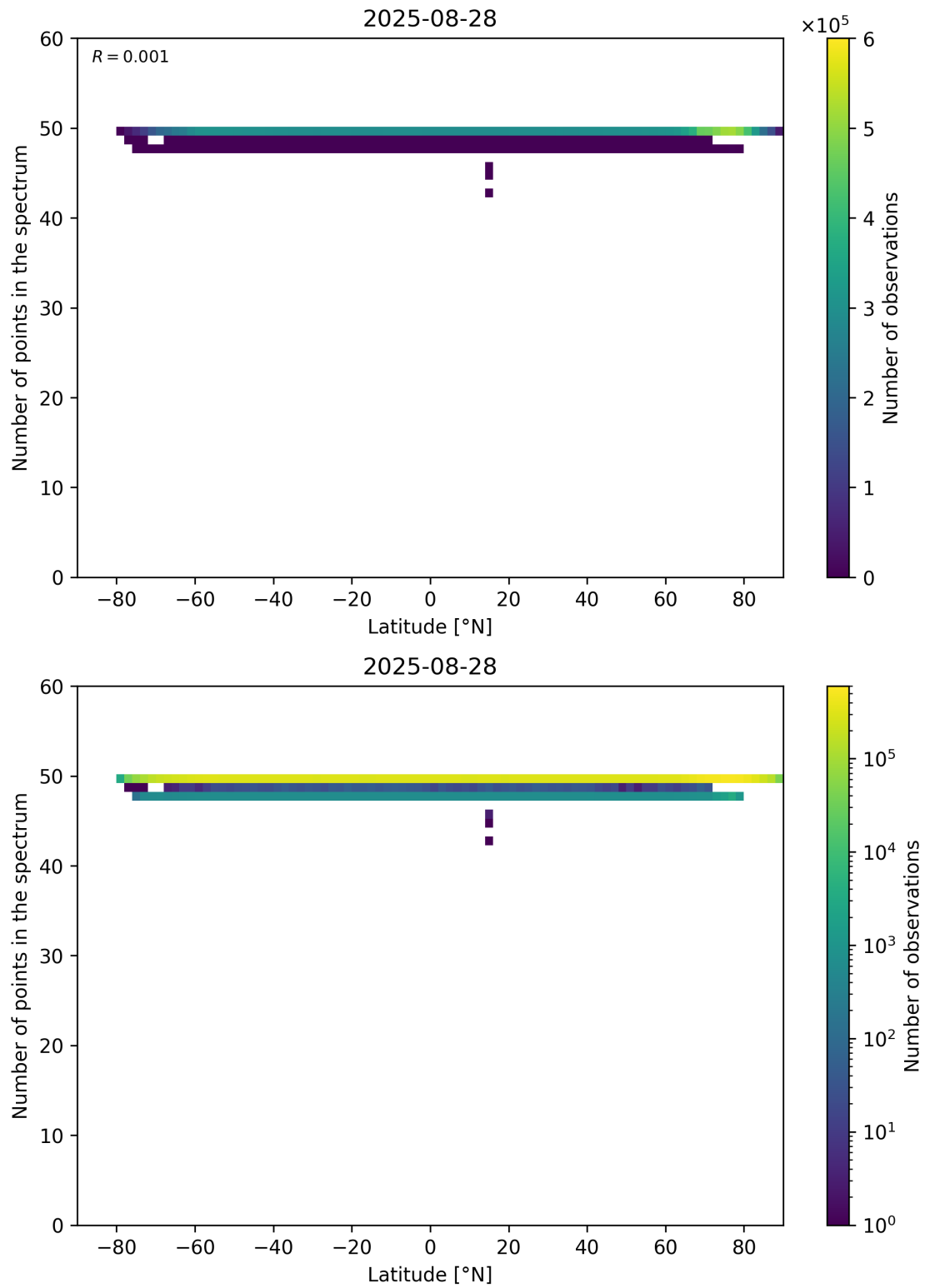
Figure 94: Scatter density plot of “Latitude” against “Number of points in the spectrum” for 2025-08-27 to 2025-08-29.
