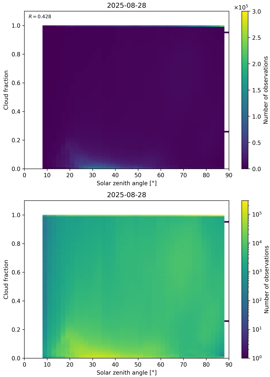
Figure 110: Scatter density plot of “Solar zenith angle” against “Cloud fraction” for 2025-08-27 to 2025-08-29.
