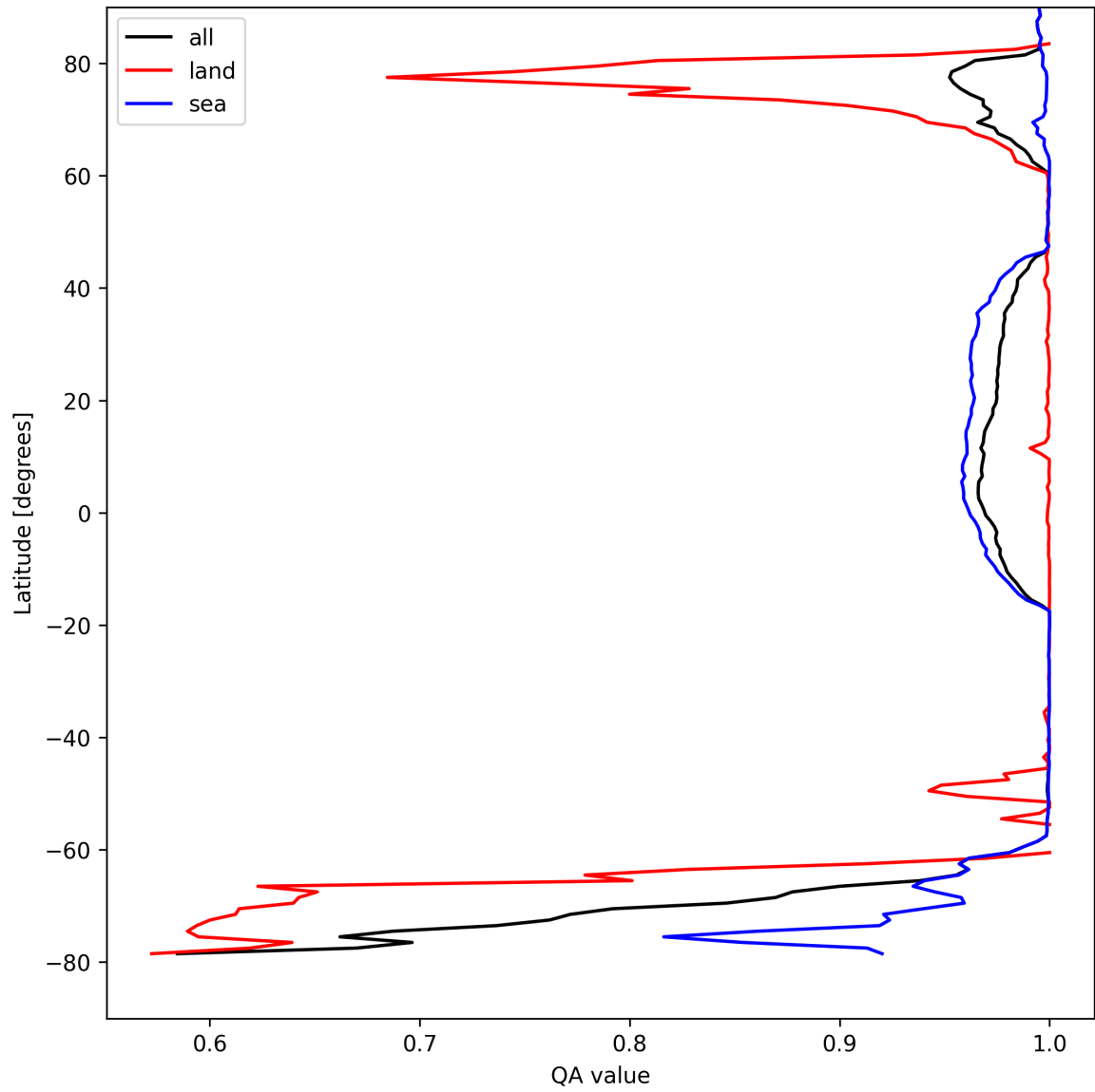
Figure 12: Zonal average of "QA value" for 2025-08-27 to 2025-08-29.
