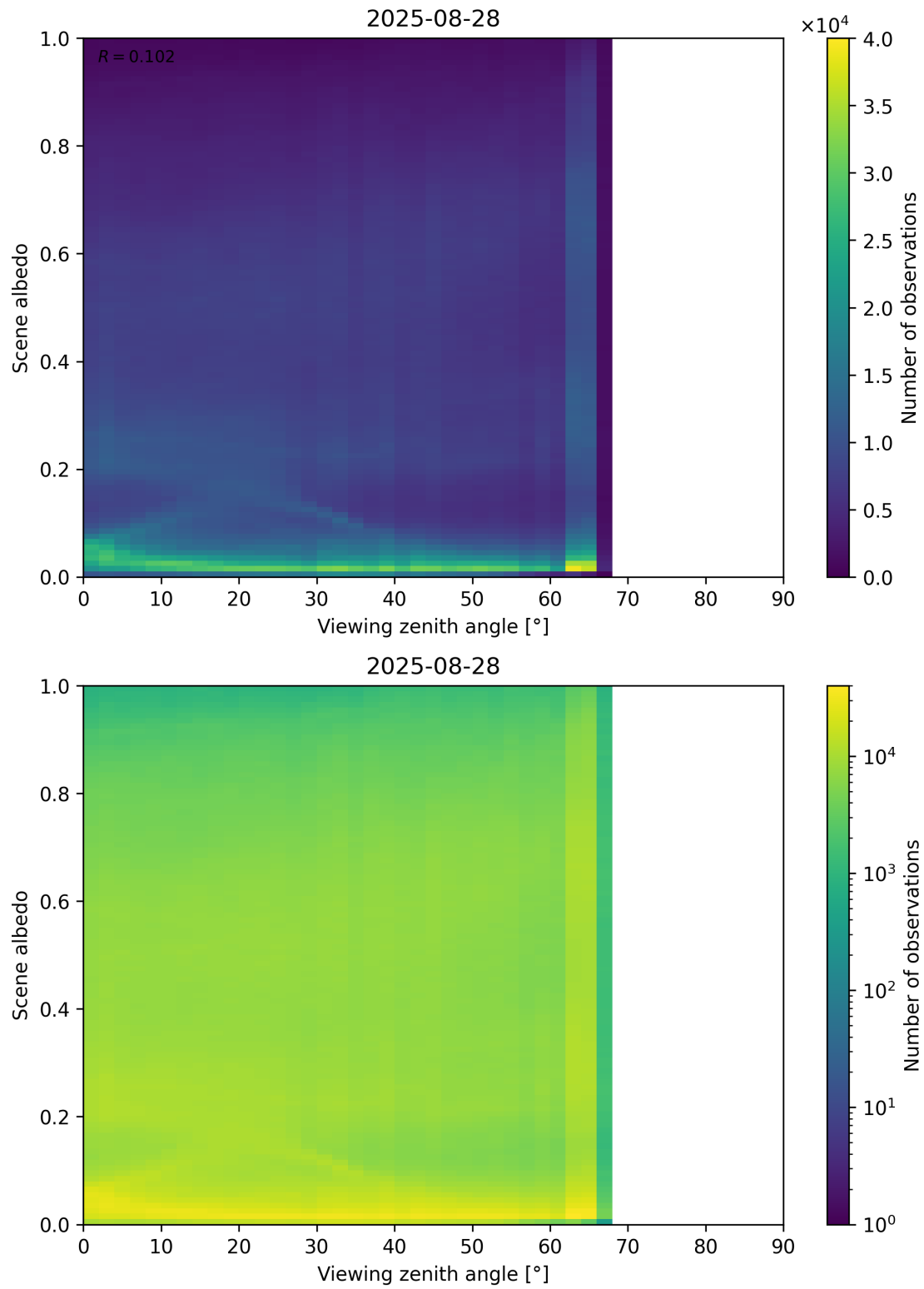
Figure 126: Scatter density plot of “Viewing zenith angle” against “Scene albedo” for 2025-08-27 to 2025-08-29.
