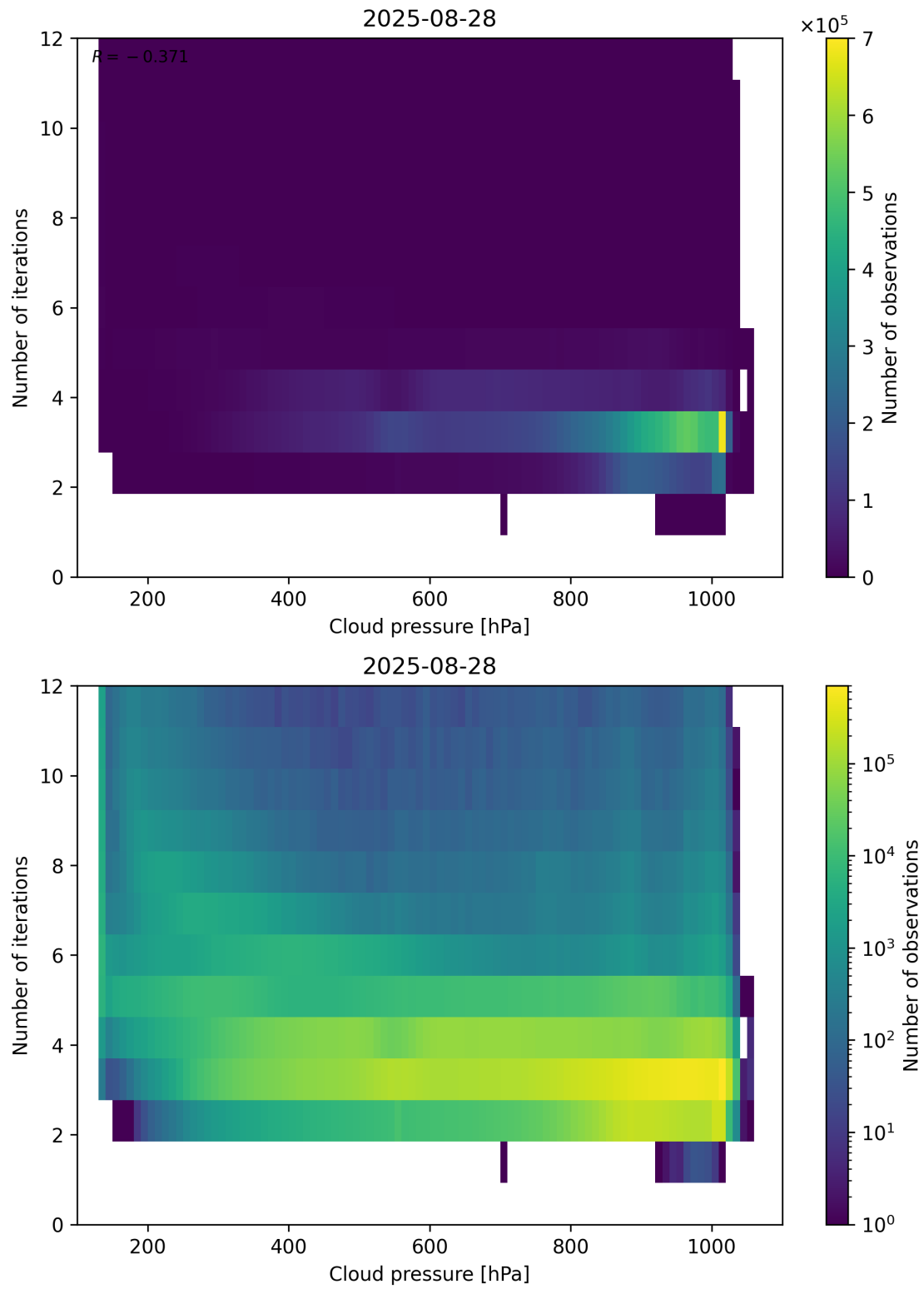
Figure 81: Scatter density plot of “Cloud pressure” against “Number of iterations” for 2025-08-27 to 2025-08-29.
