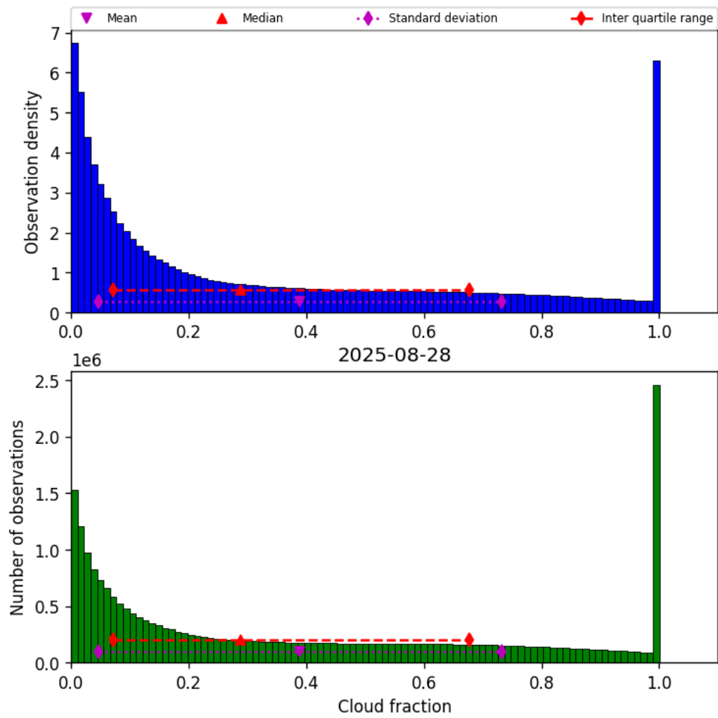
Figure 32: Histogram of “Cloud fraction” for 2025-08-27 to 2025-08-29
