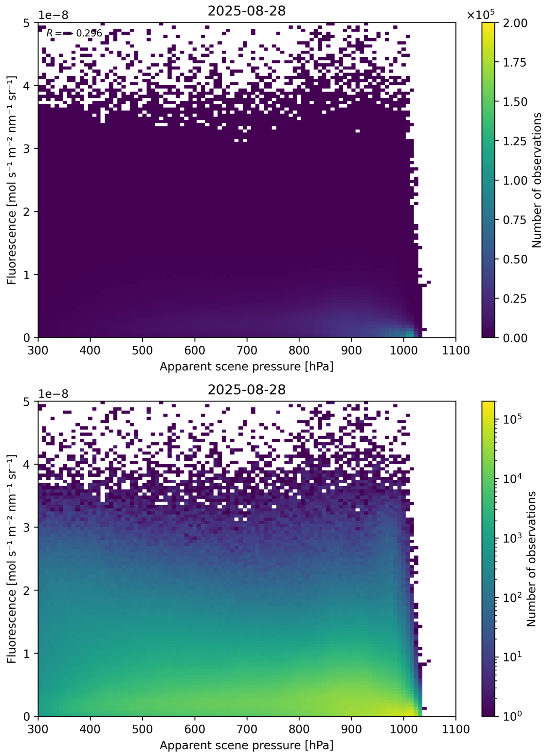
Figure 64: Scatter density plot of “Apparent scene pressure” against “Fluorescence” for 2025-08-27 to 2025-08-29.
