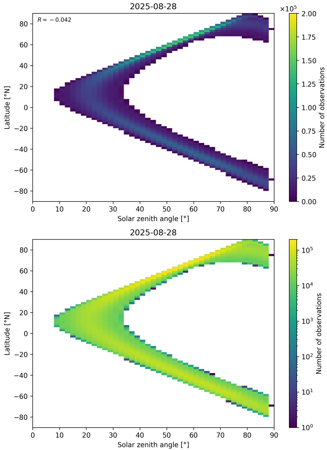
Figure 113: Scatter density plot of “Solar zenith angle” against “Latitude” for 2025-08-27 to 2025-08-29.
