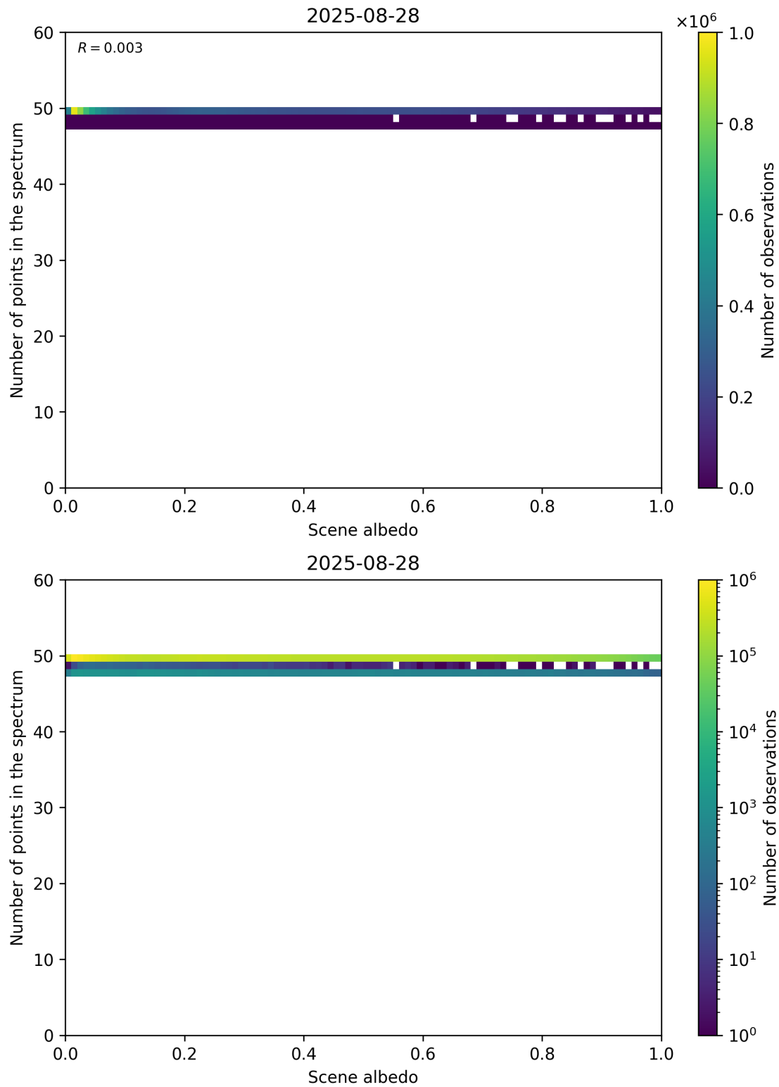
Figure 106: Scatter density plot of “Scene albedo” against “Number of points in the spectrum” for 2025-08-27 to 2025-08-29.
