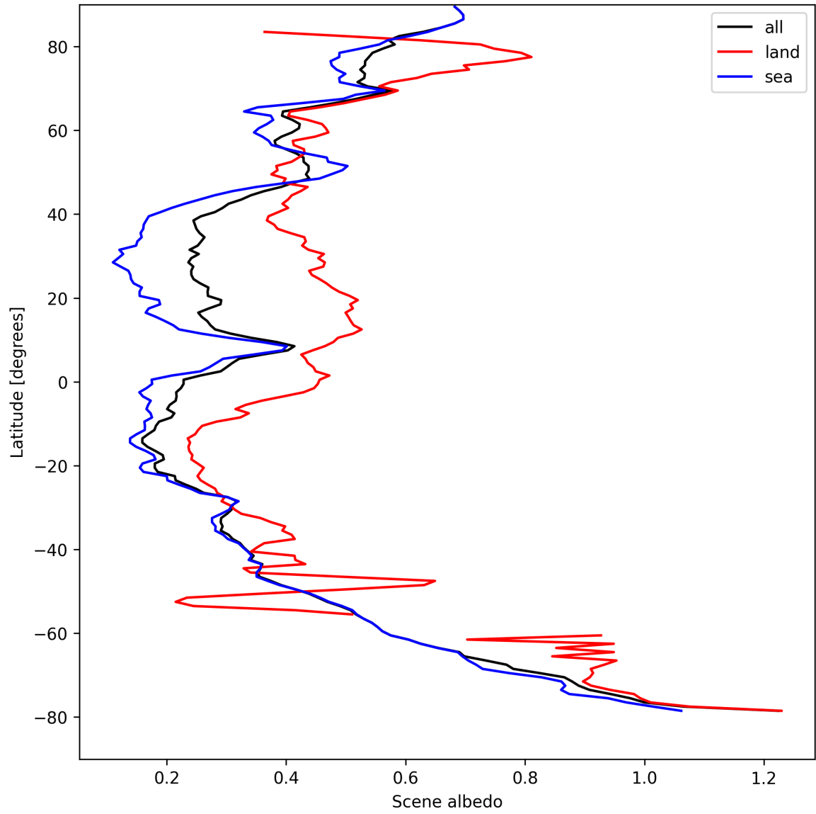
Figure 17: Zonal average of "Scene albedo" for 2025-08-27 to 2025-08-29.
