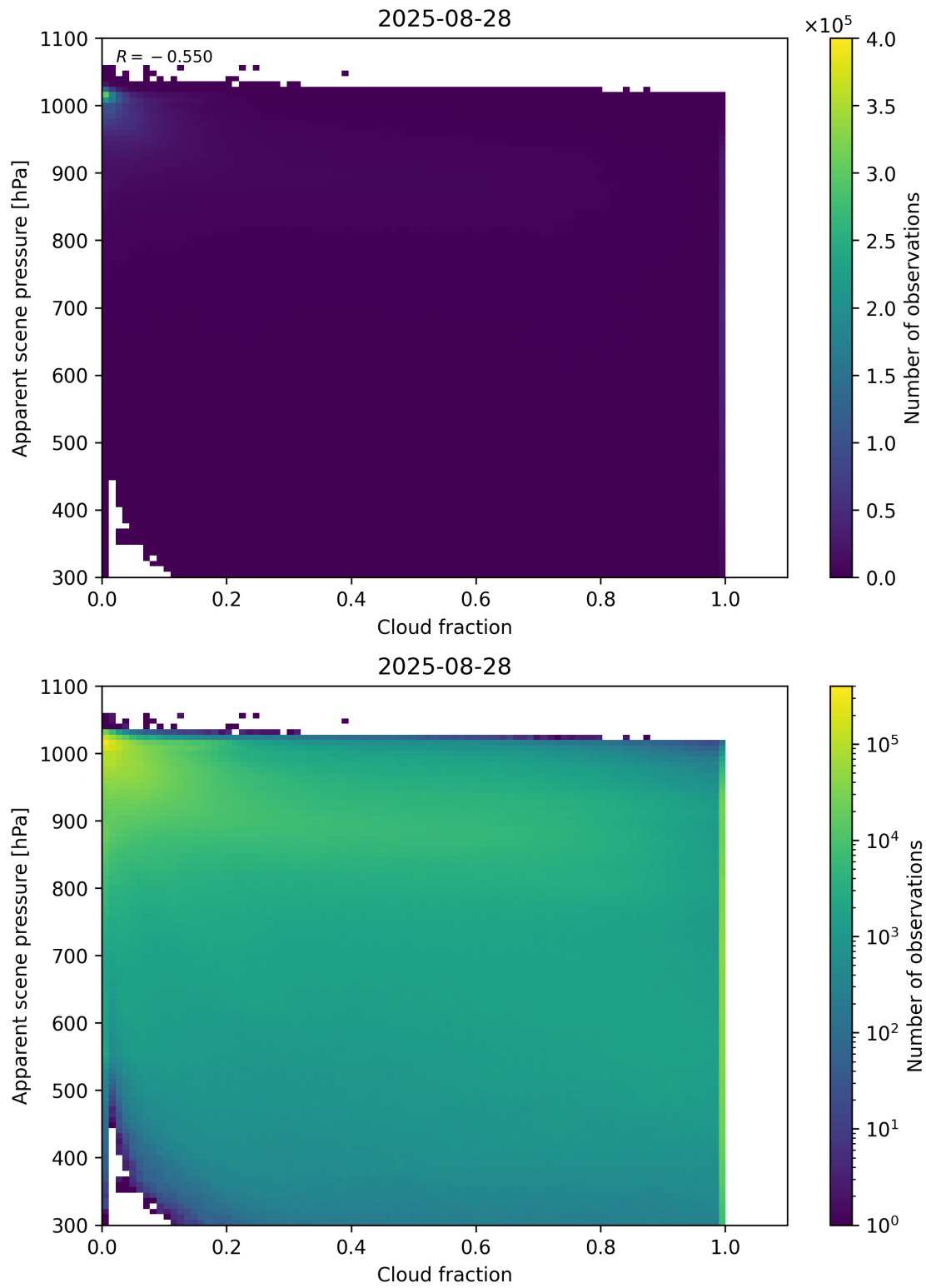
Figure 70: Scatter density plot of “Cloud fraction” against “Apparent scene pressure” for 2025-08-27 to 2025-08-29.
