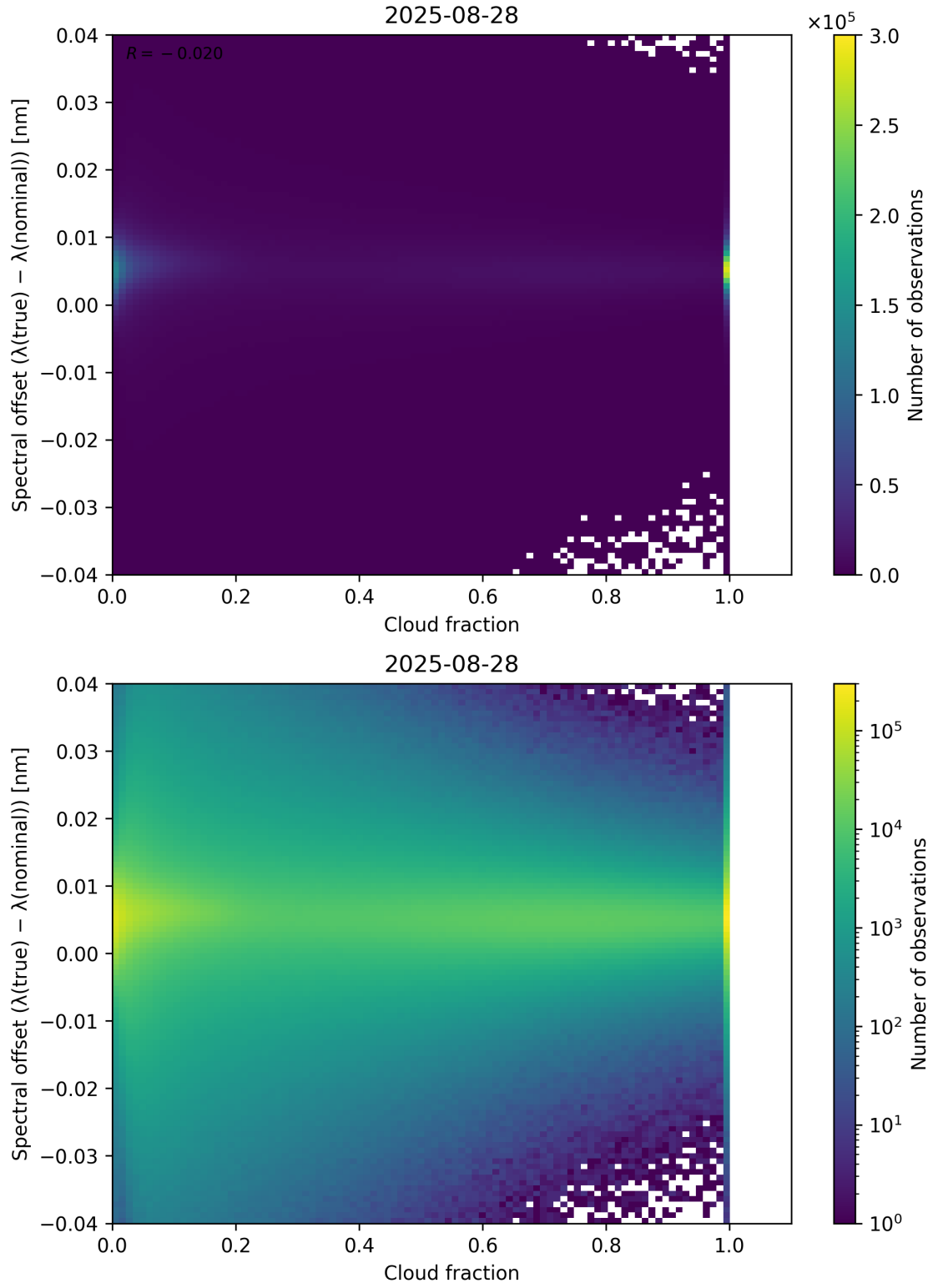
Figure 76: Scatter density plot of “Cloud fraction” against “Spectral offset ( \lambda_{\text{true}} - \lambda_{\text{nominal}} )” for 2025-08-27 to 2025-08-29.
