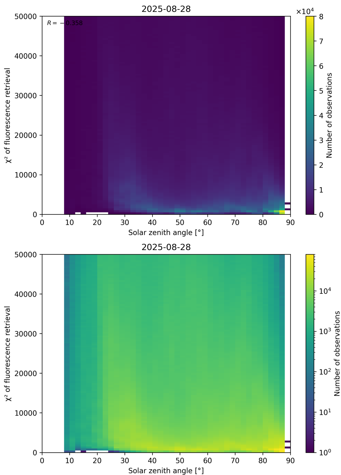
Figure 109: Scatter density plot of “Solar zenith angle” against “ \chi^2 of fluorescence retrieval” for 2025-08-27 to 2025-08-29.
