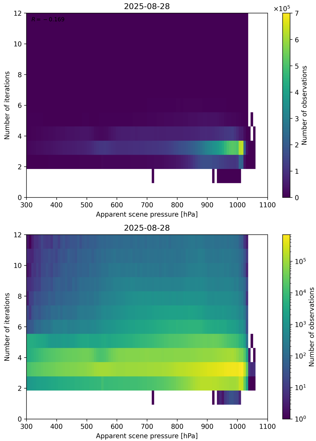
Figure 65: Scatter density plot of “Apparent scene pressure” against “Number of iterations” for 2025-08-27 to 2025-08-29.
