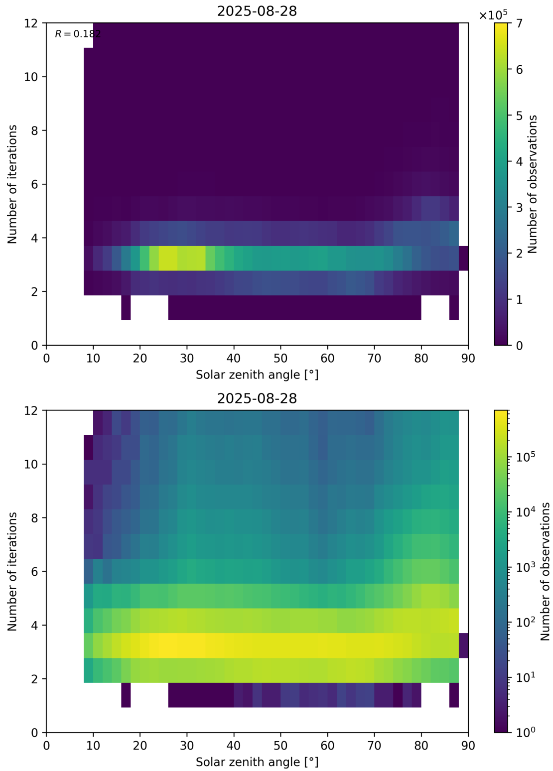
Figure 114: Scatter density plot of “Solar zenith angle” against “Number of iterations” for 2025-08-27 to 2025-08-29.
