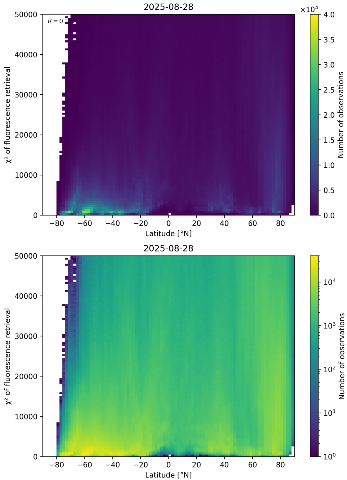
Figure 89: Scatter density plot of “Latitude” against “ \chi^2 of fluorescence retrieval” for 2025-08-27 to 2025-08-29.
