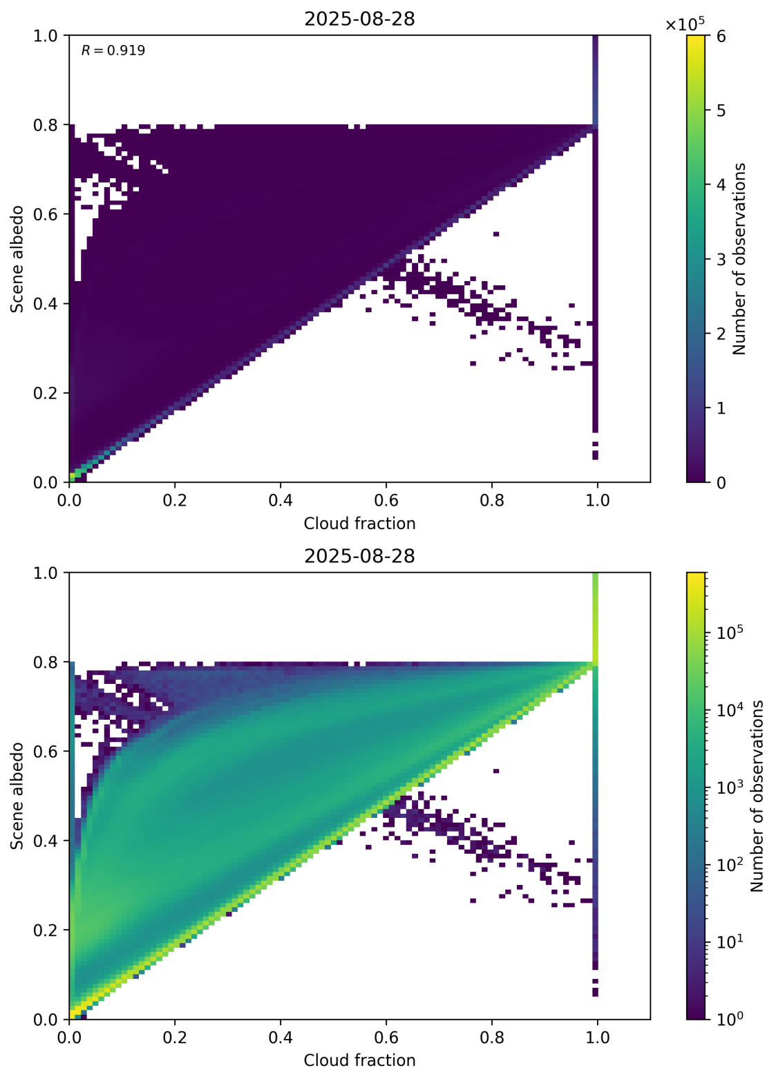
Figure 75: Scatter density plot of “Cloud fraction” against “Scene albedo” for 2025-08-27 to 2025-08-29.
