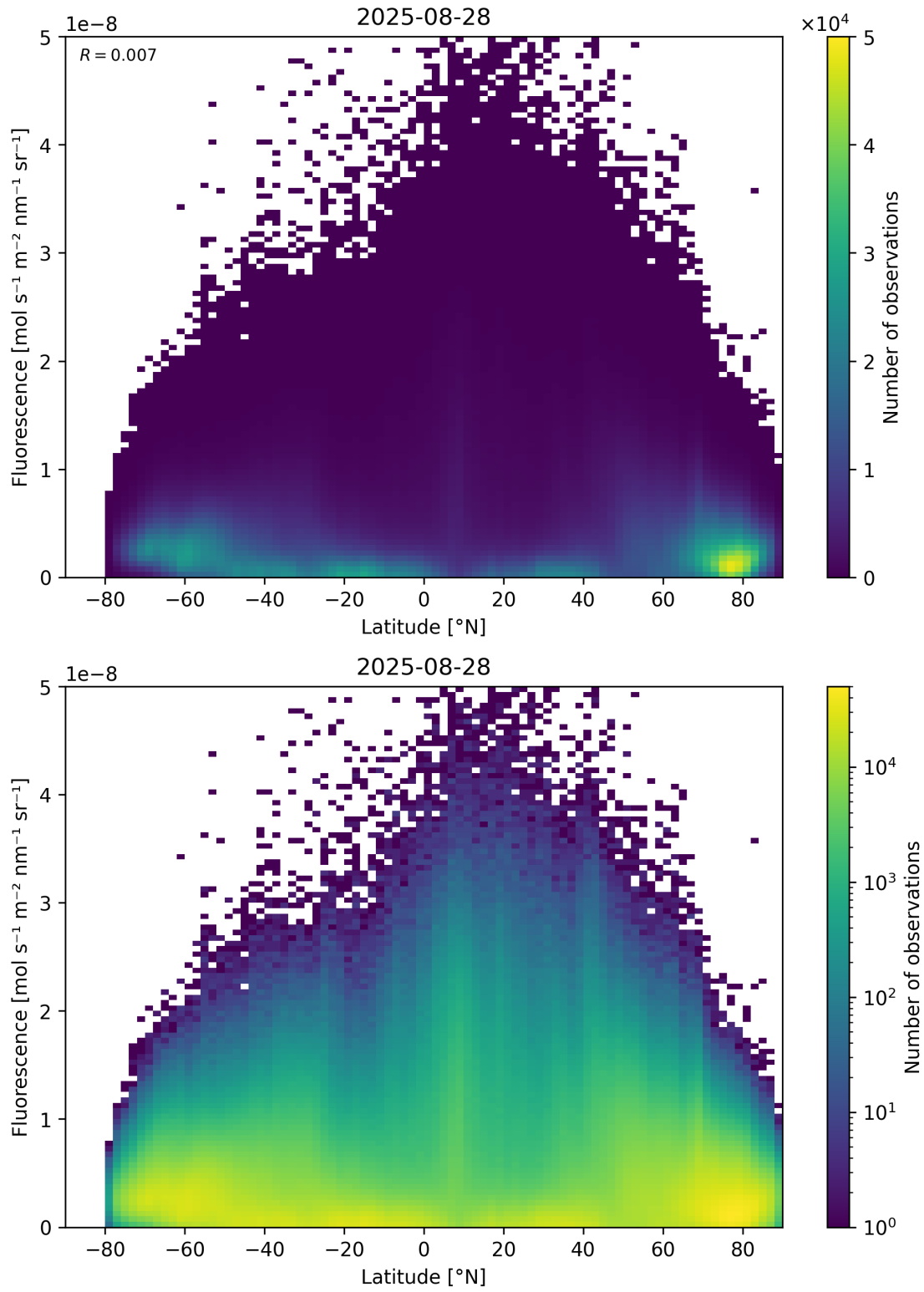
Figure 92: Scatter density plot of “Latitude” against “Fluorescence” for 2025-08-27 to 2025-08-29.
