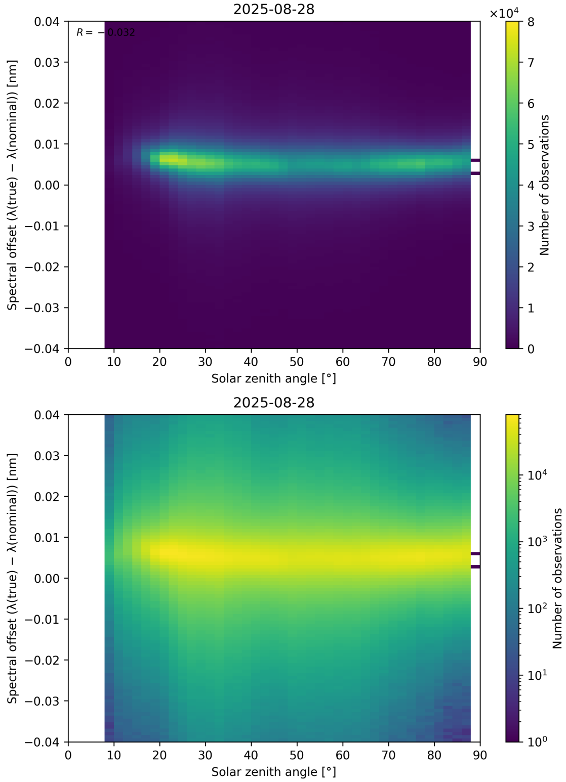
Figure 117: Scatter density plot of “Solar zenith angle” against “Spectral offset ( \lambda_{\text{true}} - \lambda_{\text{nominal}} )” for 2025-08-27 to 2025-08-29.
