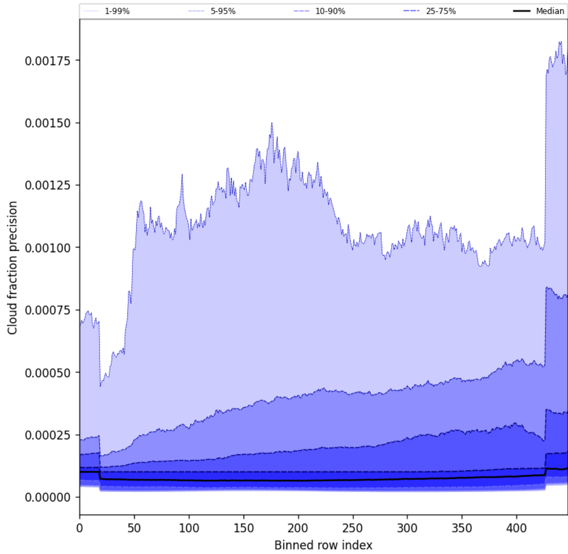
Figure 50: Along track statistics of “Cloud fraction precision” for 2025-08-27 to 2025-08-29
