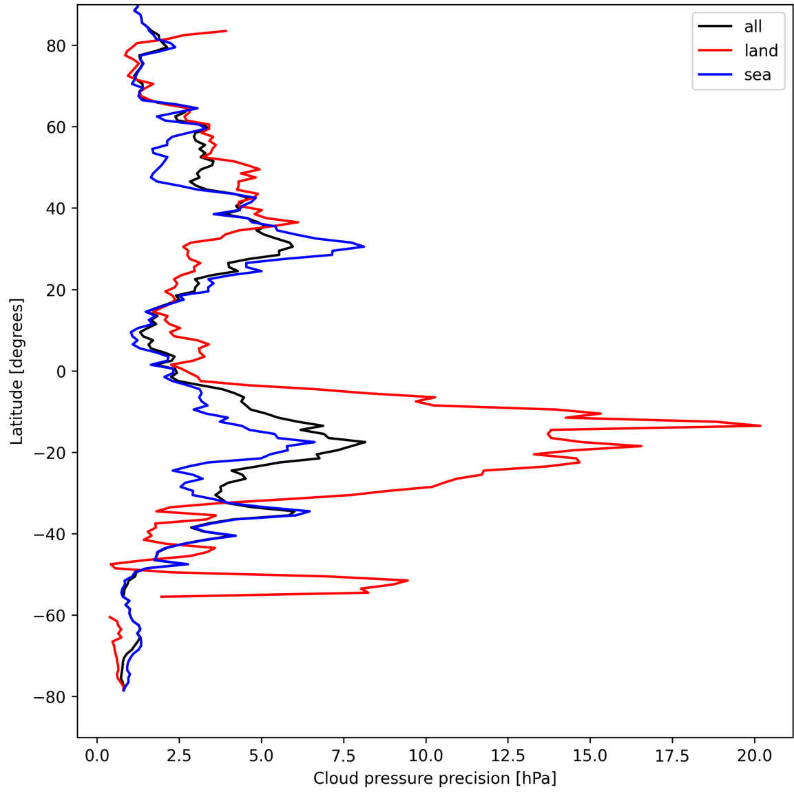
Figure 14: Zonal average of "Cloud pressure precision" for 2025-08-27 to 2025-08-29.
