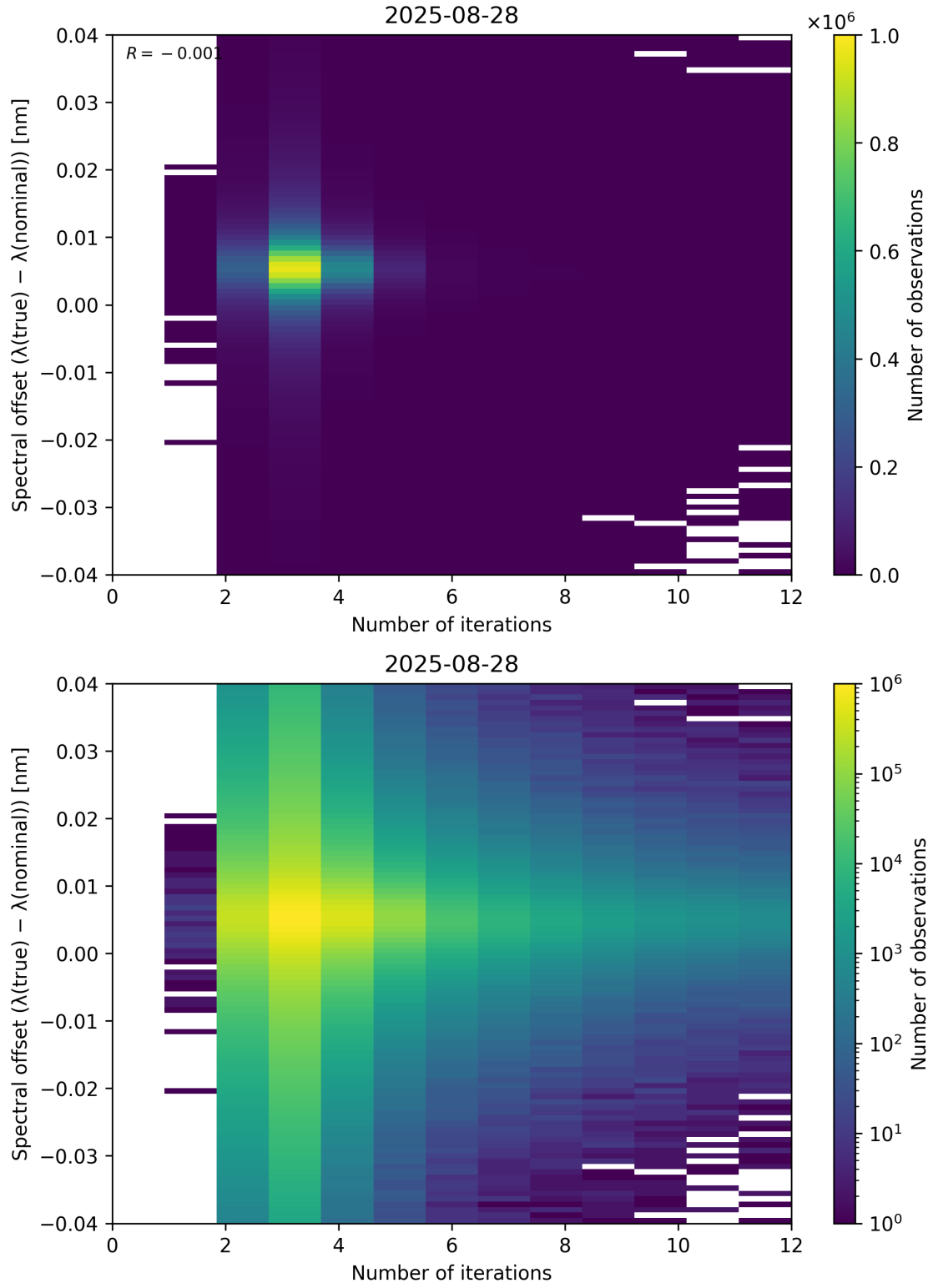
Figure 100: Scatter density plot of “Number of iterations” against “Spectral offset ( \lambda_{\text{true}} - \lambda_{\text{nominal}} )” for 2025-08-27 to 2025-08-29.
