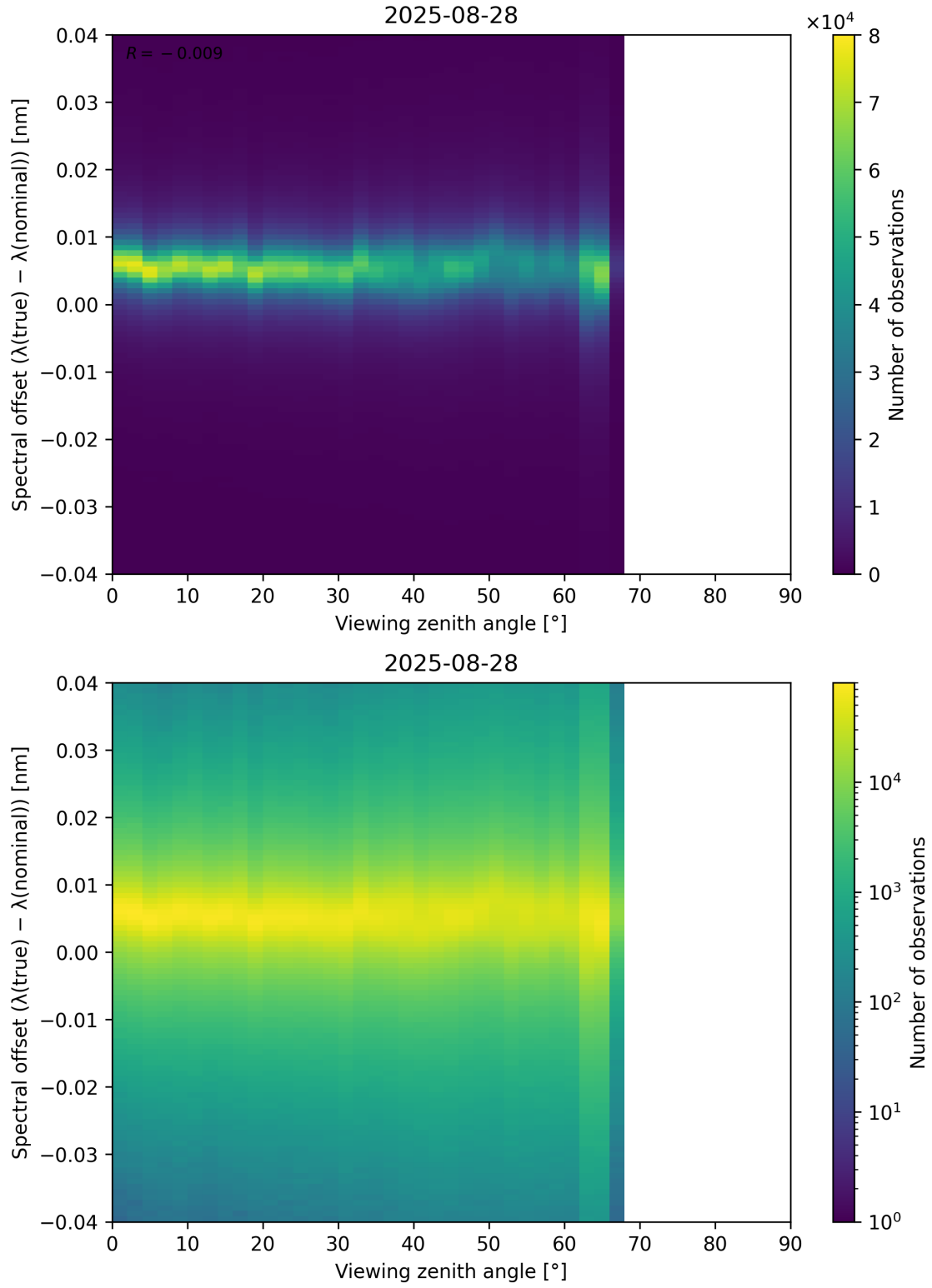
Figure 128: Scatter density plot of “Viewing zenith angle” against “Spectral offset ( \lambda_{\text{true}} - \lambda_{\text{nominal}} )” for 2025-08-27 to 2025-08-29.
