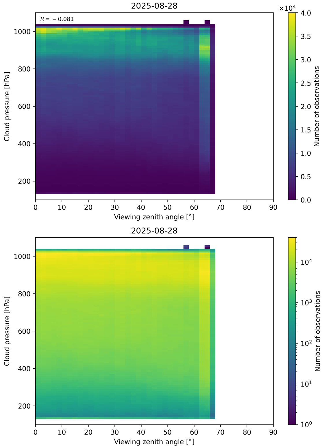
Figure 121: Scatter density plot of “Viewing zenith angle” against “Cloud pressure” for 2025-08-27 to 2025-08-29.
