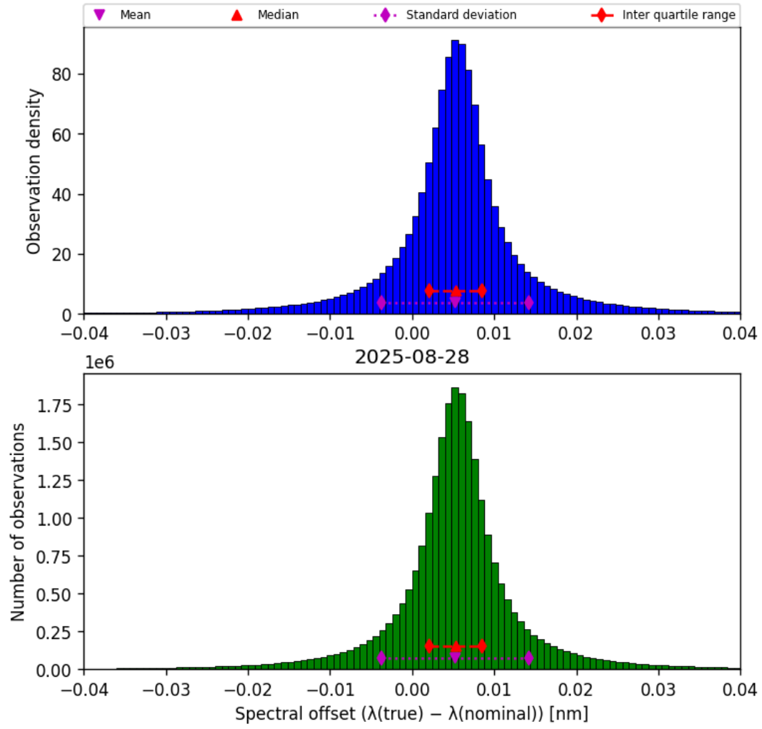
Figure 45: Histogram of “Spectral offset ( \lambda_{\text{true}} - \lambda_{\text{nominal}} )” for 2025-08-27 to 2025-08-29
