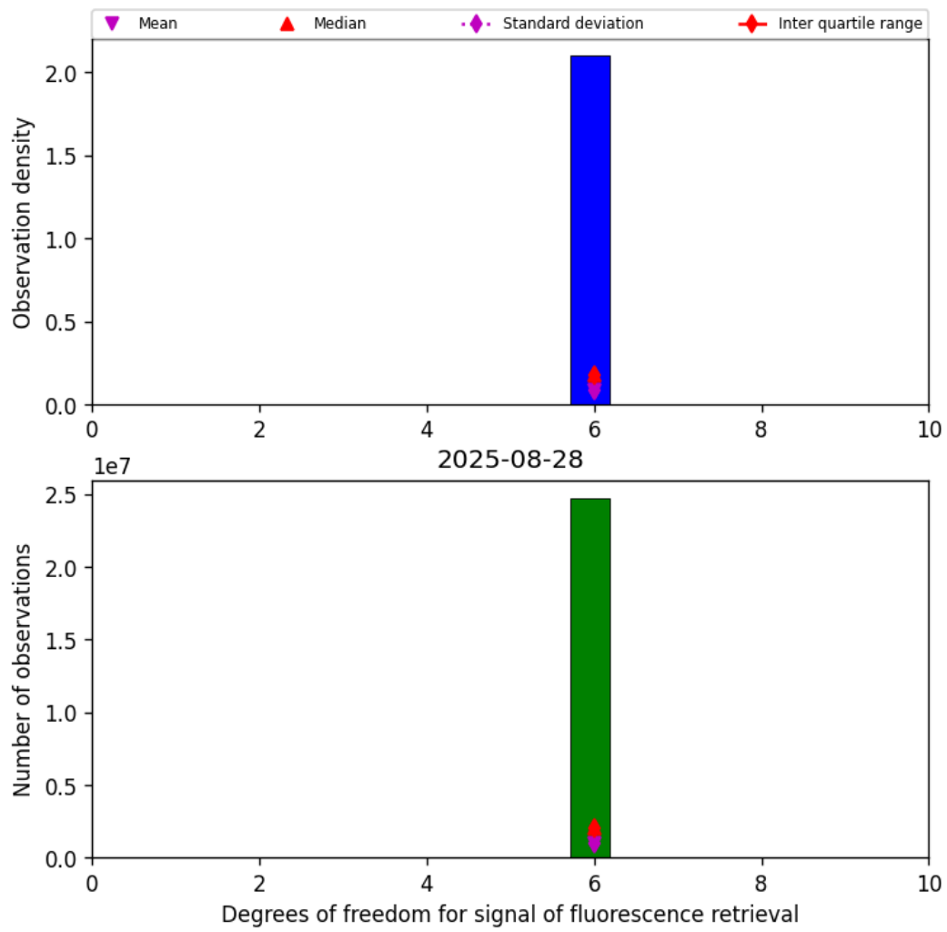
Figure 43: Histogram of "Degrees of freedom for signal of fluorescence retrieval" for 2025-08-27 to 2025-08-29
