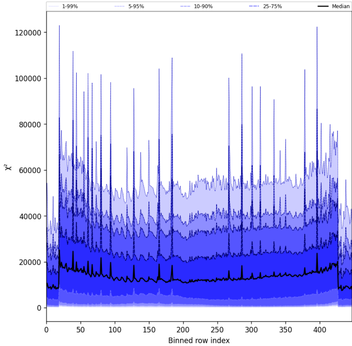
Figure 55: Along track statistics of “ \chi^2 ” for 2025-08-27 to 2025-08-29
