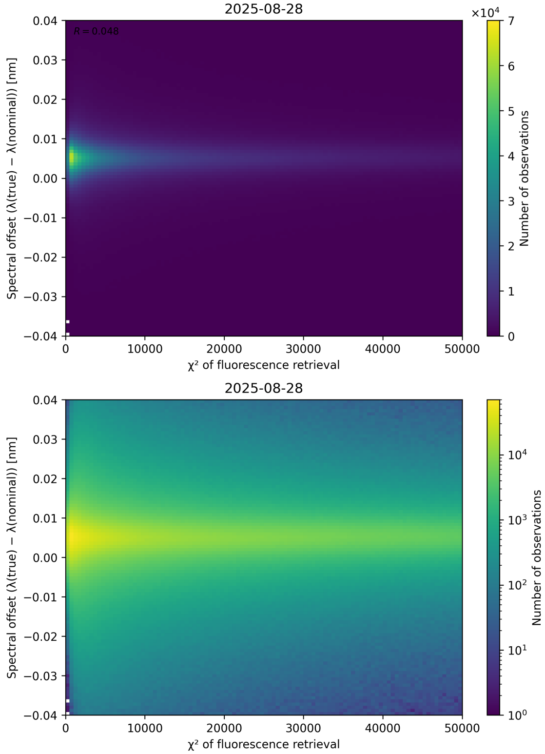
Figure 69: Scatter density plot of “ \chi^2 of fluorescence retrieval” against “Spectral offset ( \lambda_{\text{true}} - \lambda_{\text{nominal}} )” for 2025-08-27 to 2025-08-29.
