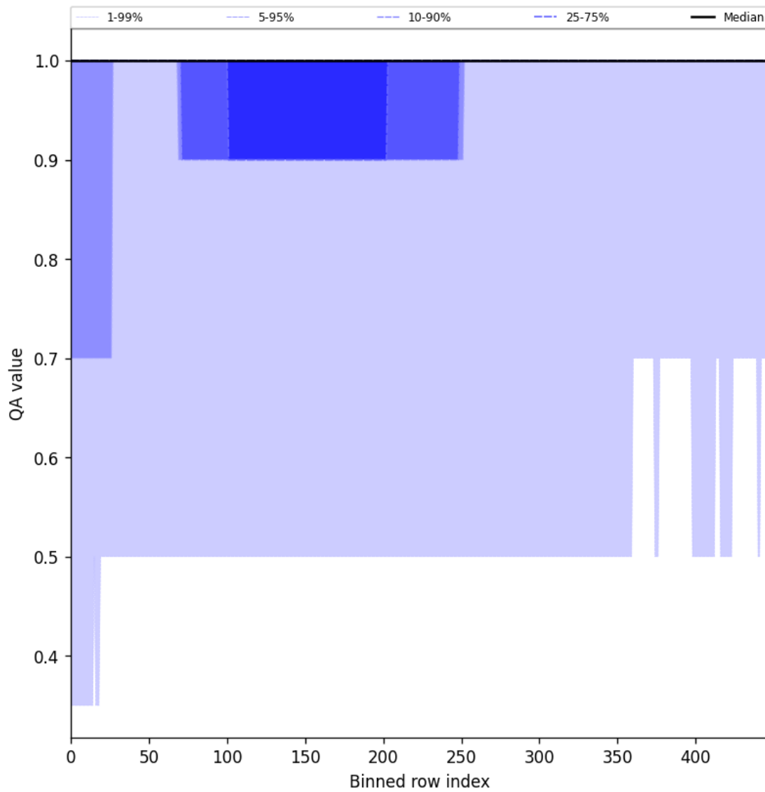
Figure 46: Along track statistics of “QA value” for 2025-08-27 to 2025-08-29
