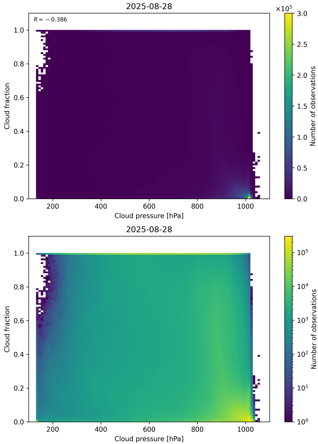
Figure 79: Scatter density plot of “Cloud pressure” against “Cloud fraction” for 2025-08-27 to 2025-08-29.
