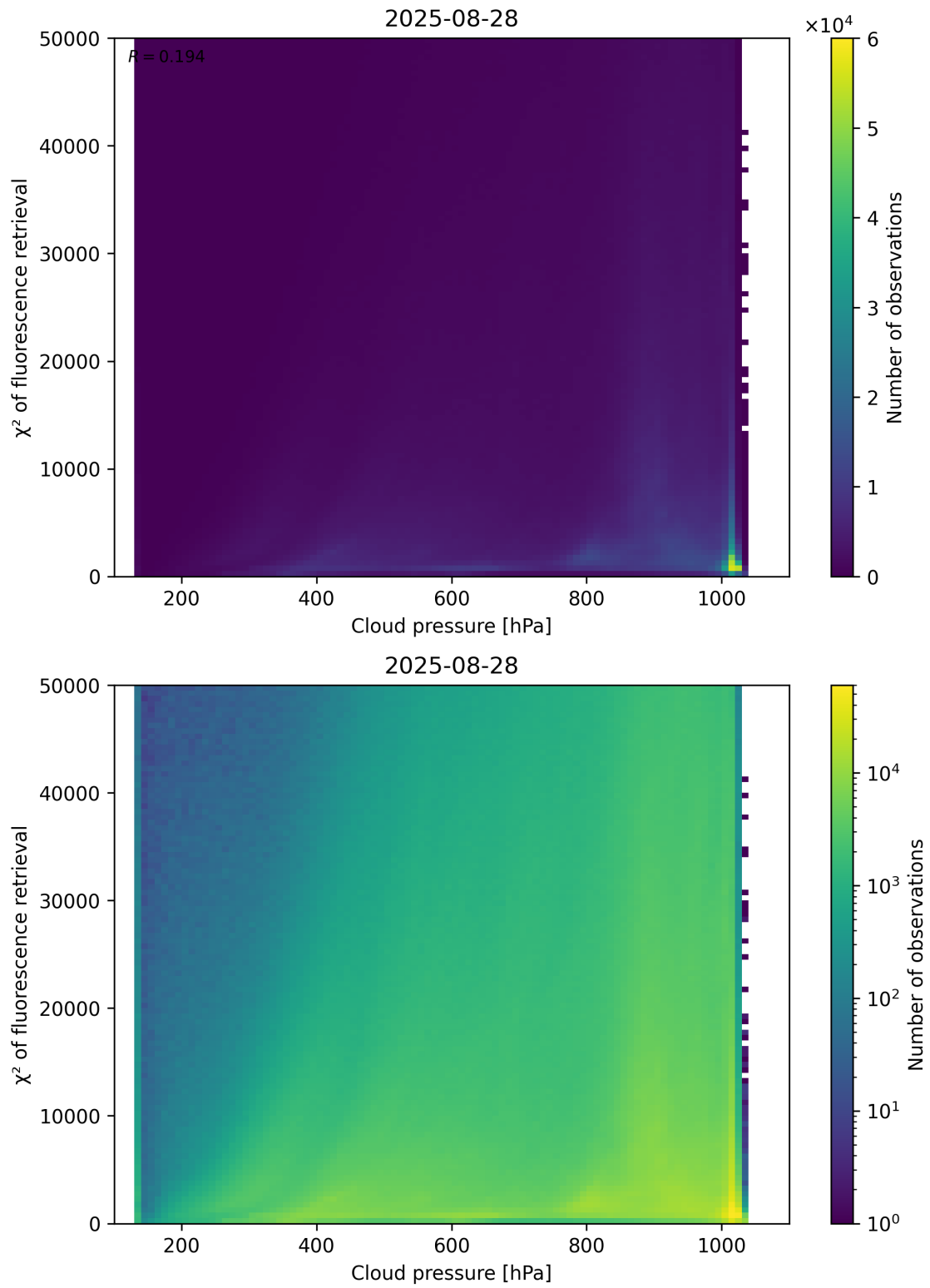
Figure 78: Scatter density plot of “Cloud pressure” against “ \chi^2 of fluorescence retrieval” for 2025-08-27 to 2025-08-29.
