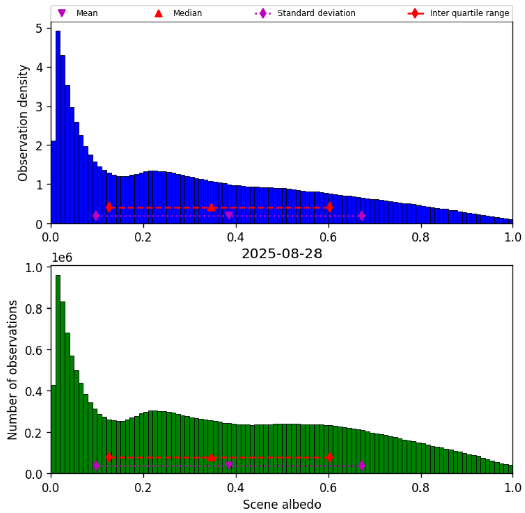
Figure 34: Histogram of “Scene albedo” for 2025-08-27 to 2025-08-29
