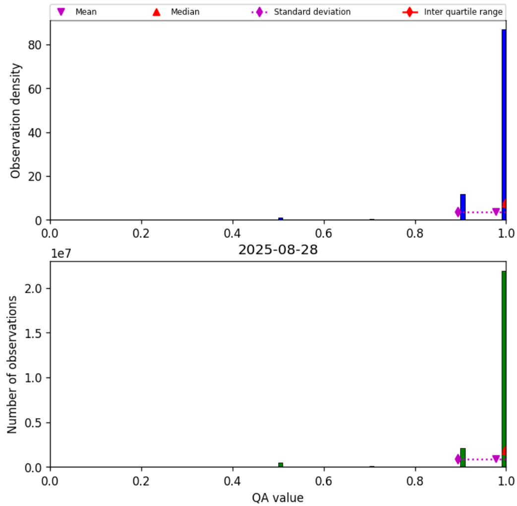
Figure 29: Histogram of “QA value” for 2025-08-27 to 2025-08-29
