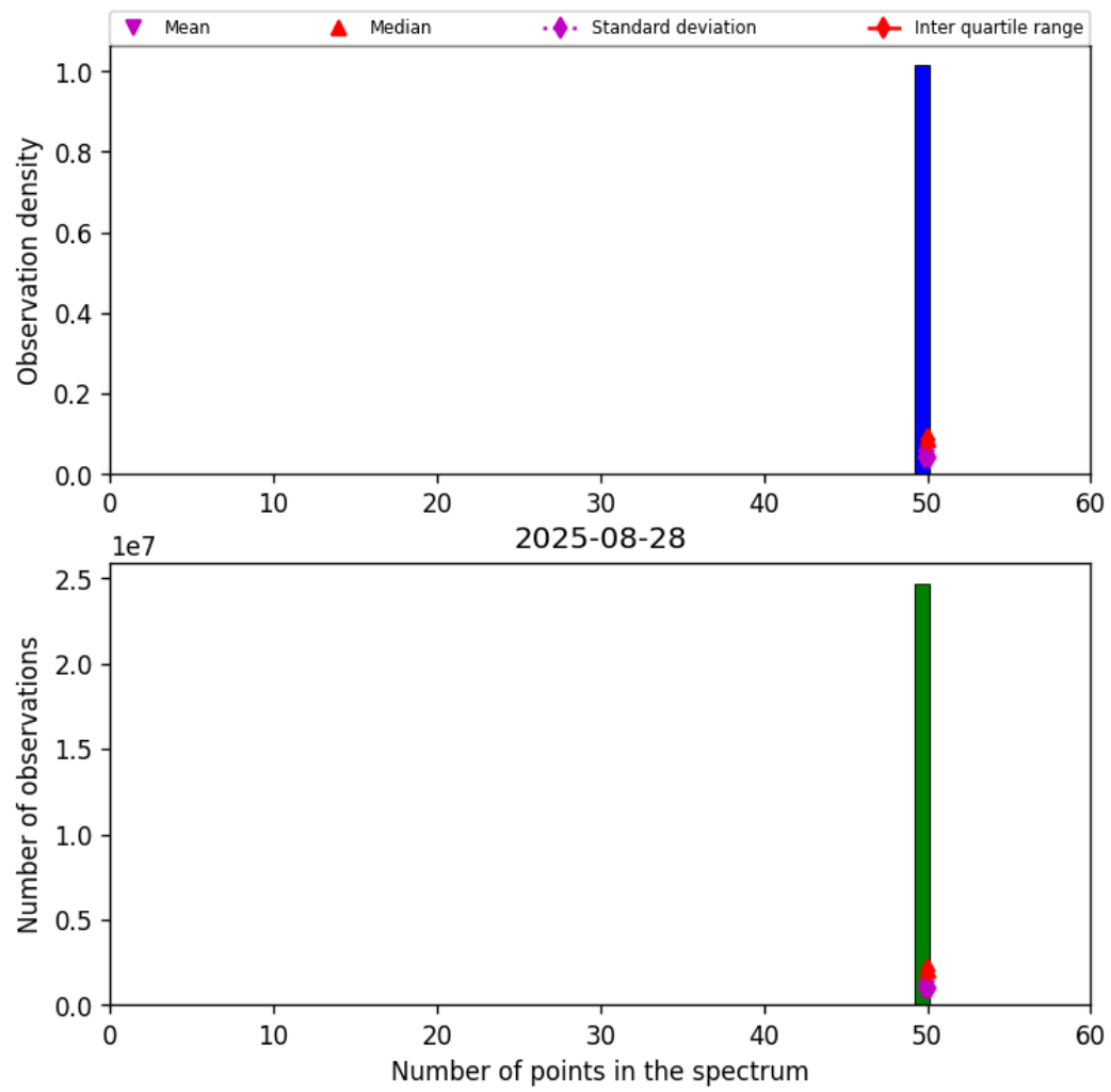
Figure 44: Histogram of “Number of points in the spectrum” for 2025-08-27 to 2025-08-29
