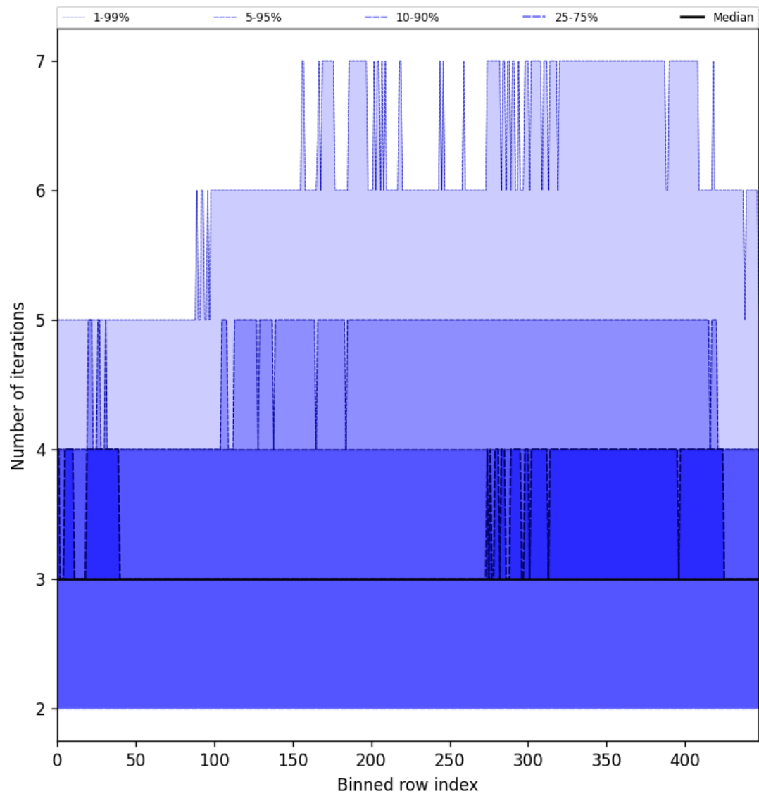
Figure 56: Along track statistics of “Number of iterations” for 2025-08-27 to 2025-08-29
