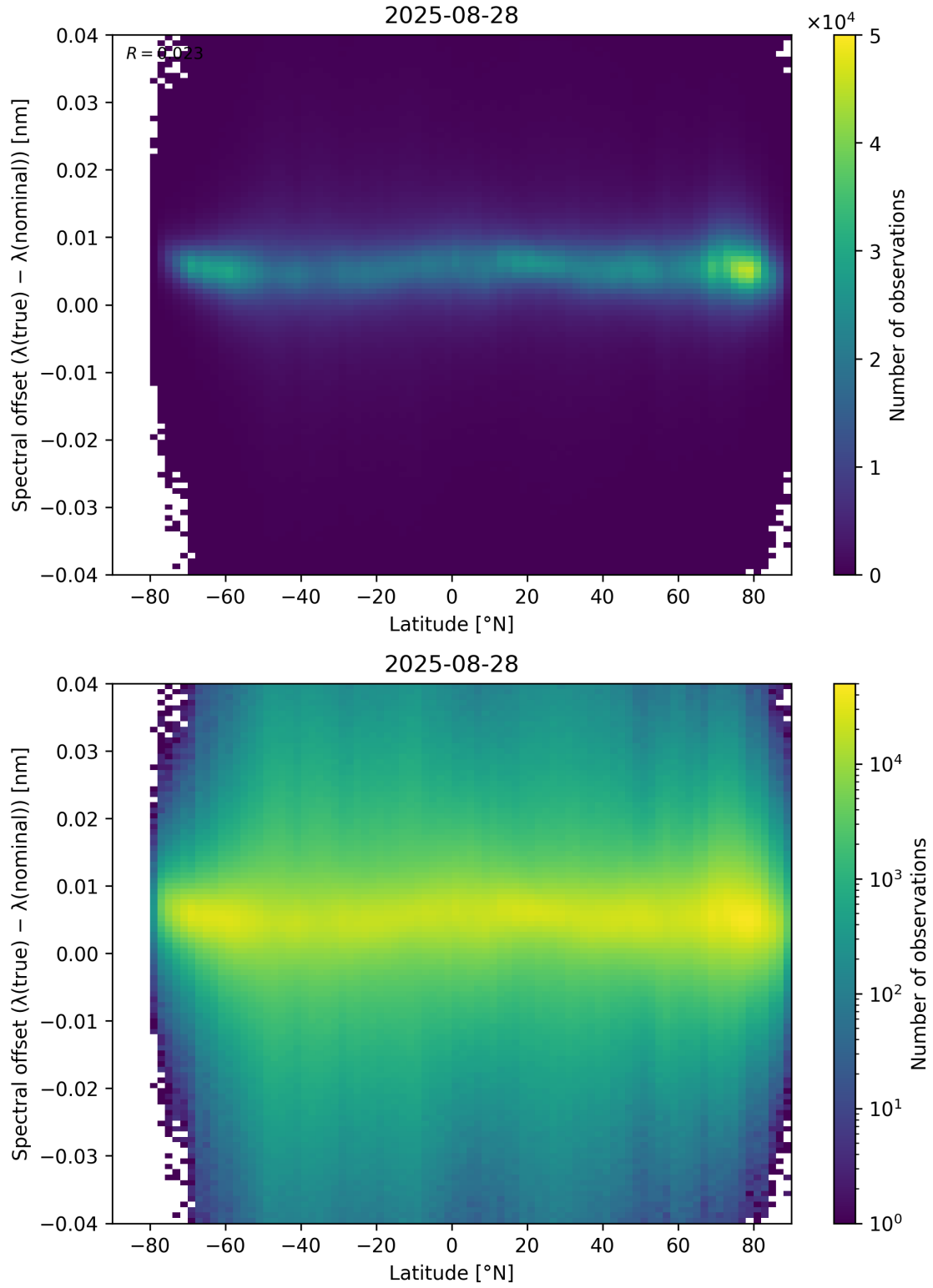
Figure 96: Scatter density plot of “Latitude” against “Spectral offset ( \lambda_{\text{true}} - \lambda_{\text{nominal}} )” for 2025-08-27 to 2025-08-29.
