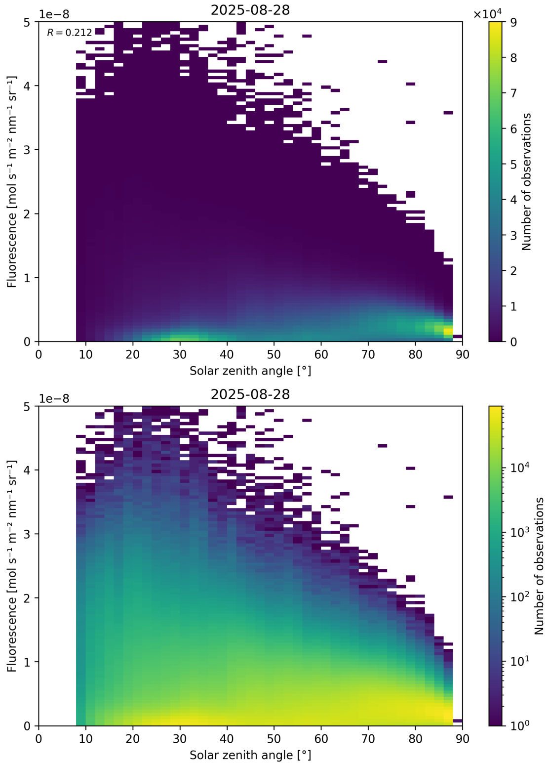
Figure 112: Scatter density plot of “Solar zenith angle” against “Fluorescence” for 2025-08-27 to 2025-08-29.
