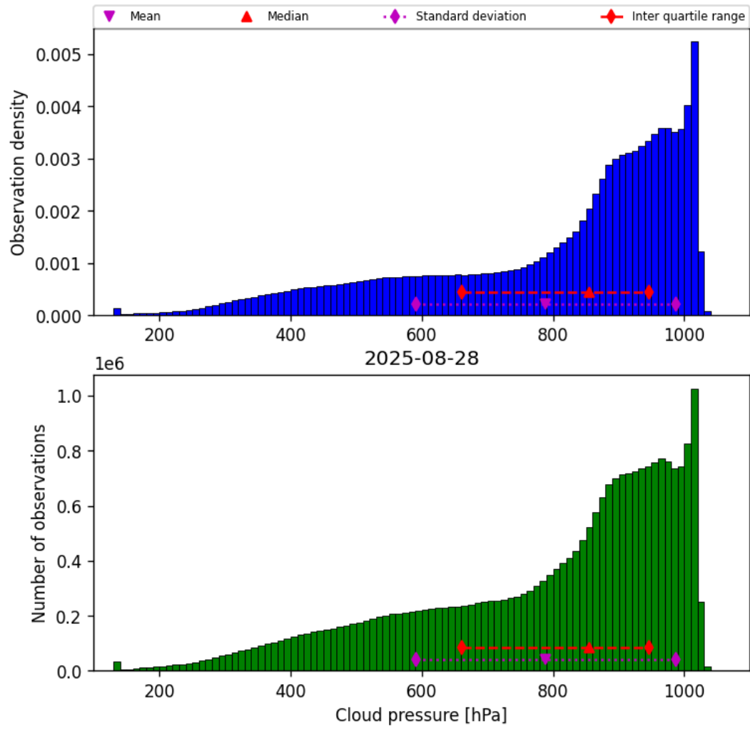
Figure 30: Histogram of “Cloud pressure” for 2025-08-27 to 2025-08-29
