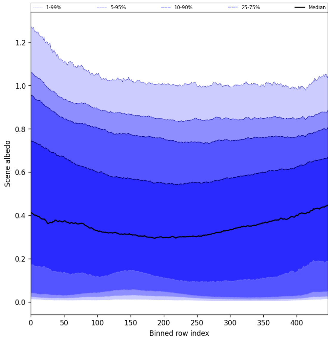
Figure 51: Along track statistics of “Scene albedo” for 2025-08-27 to 2025-08-29
