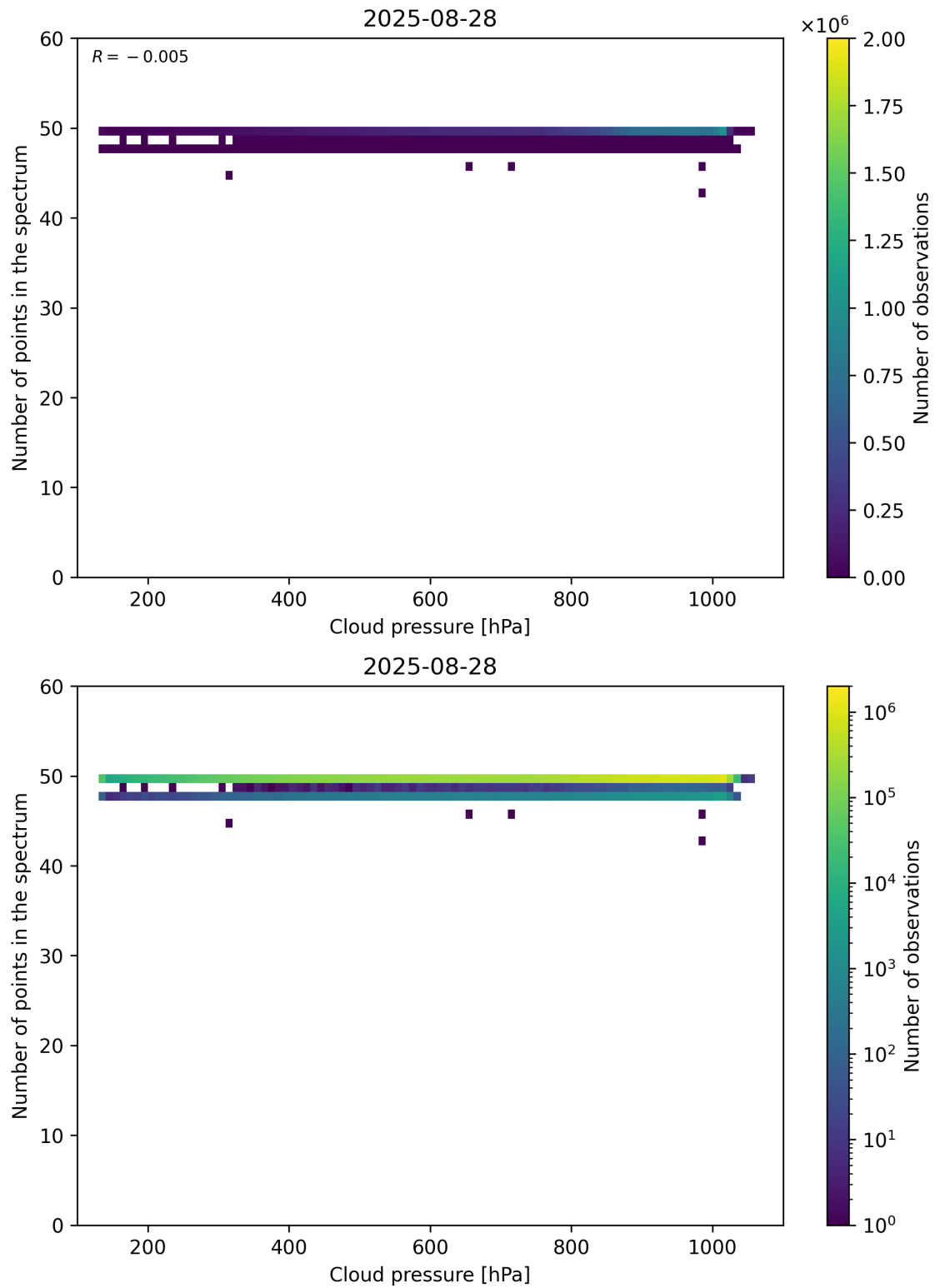
Figure 82: Scatter density plot of “Cloud pressure” against “Number of points in the spectrum” for 2025-08-27 to 2025-08-29.
