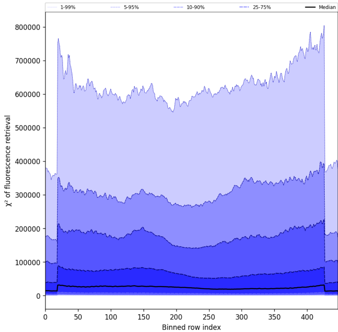
Figure 59: Along track statistics of “ \chi^2 of fluorescence retrieval” for 2025-08-27 to 2025-08-29
