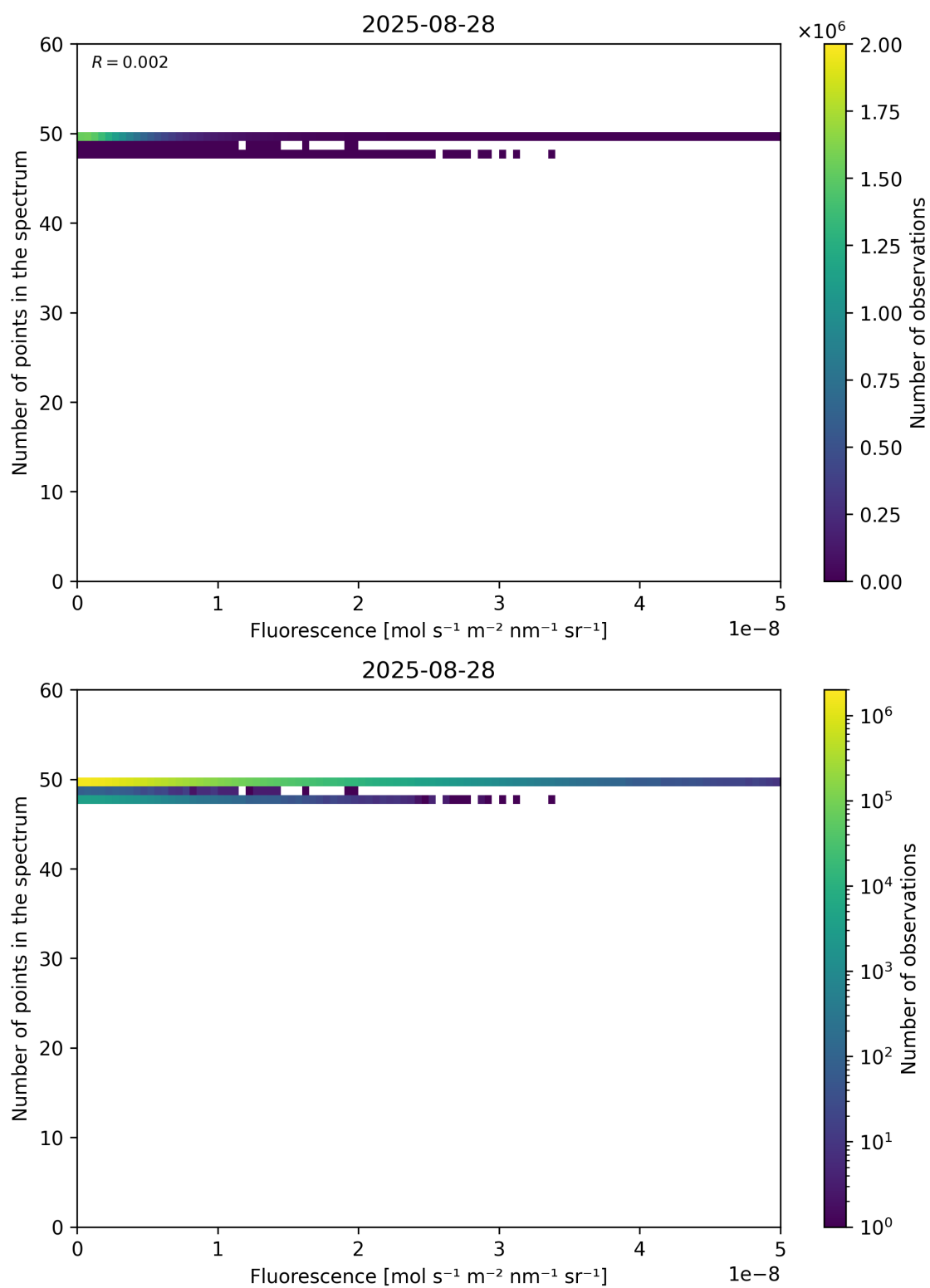
Figure 86: Scatter density plot of “Fluorescence” against “Number of points in the spectrum” for 2025-08-27 to 2025-08-29.
