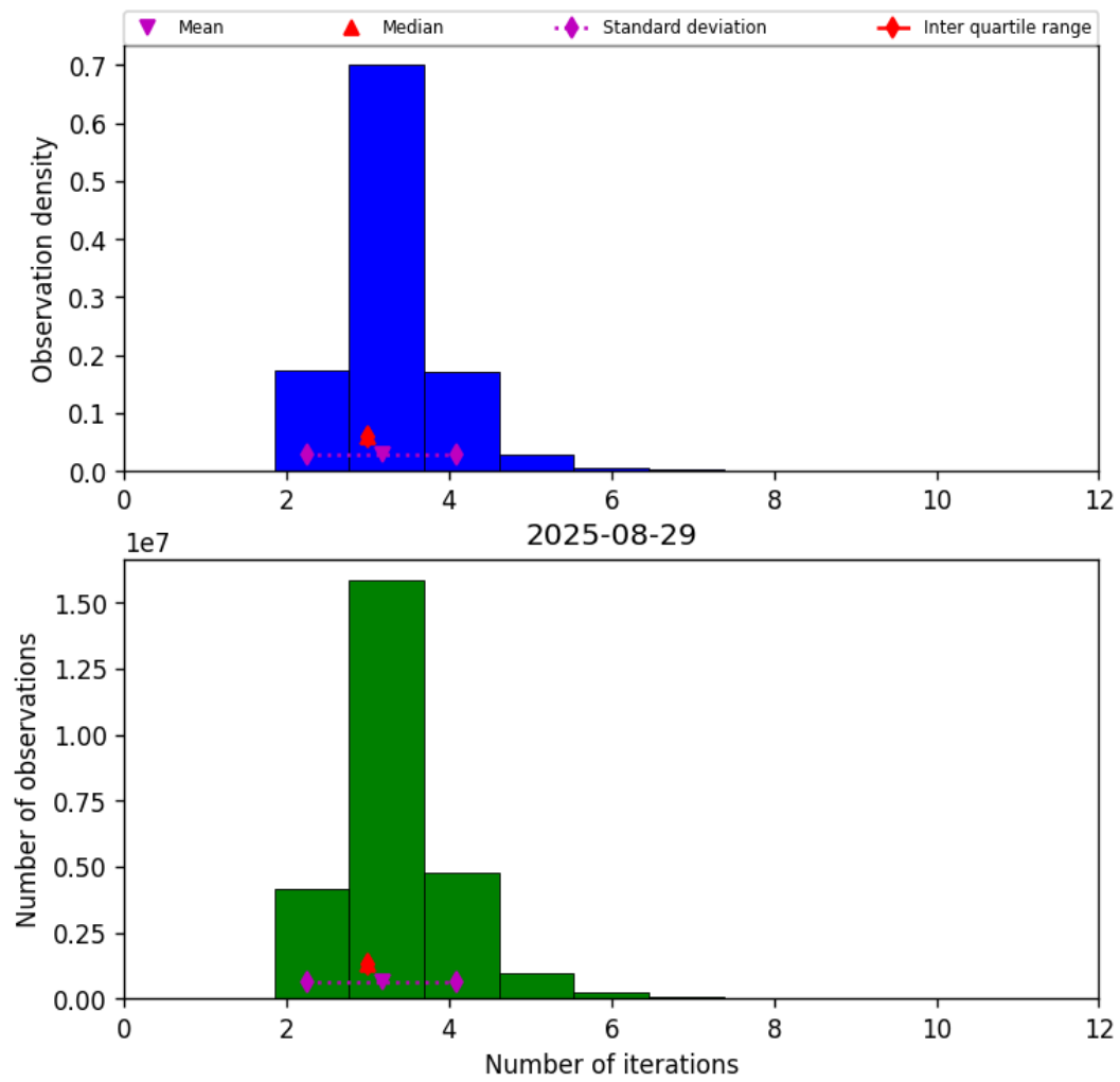
Figure 39: Histogram of “Number of iterations” for 2025-08-28 to 2025-08-30
