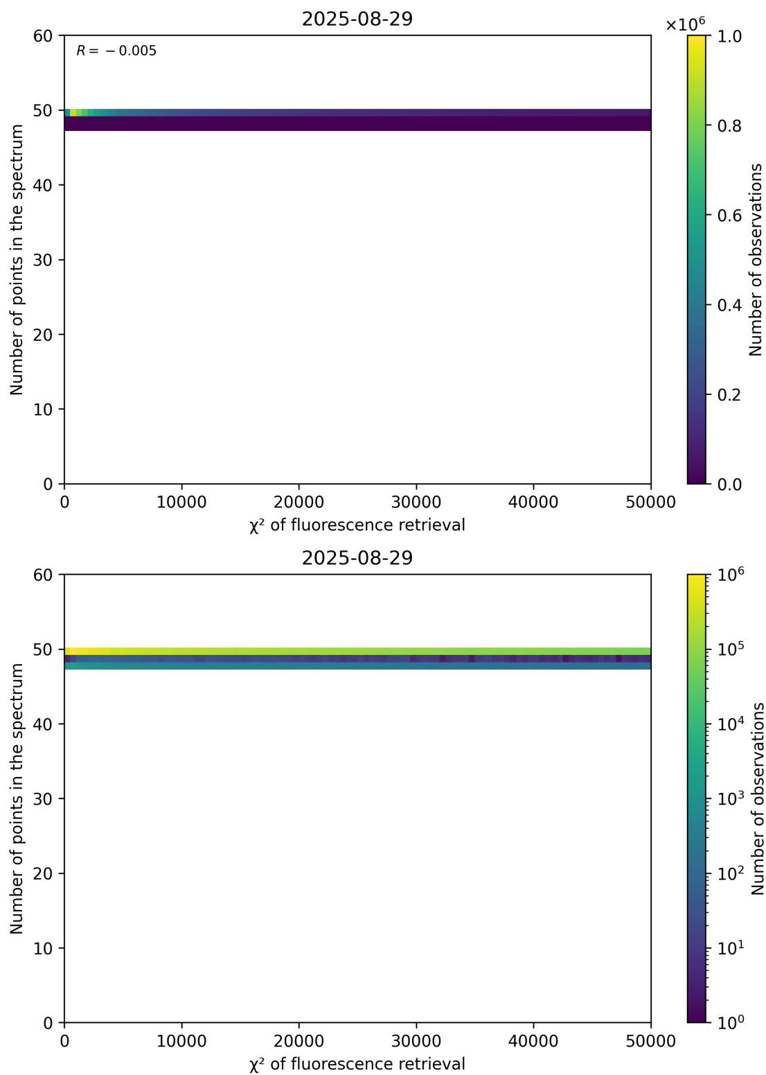
Figure 68: Scatter density plot of " \chi^2 of fluorescence retrieval" against "Number of points in the spectrum" for 2025-08-28 to 2025-08-30.
