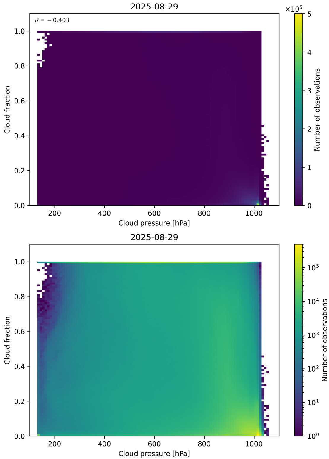
Figure 79: Scatter density plot of “Cloud pressure” against “Cloud fraction” for 2025-08-28 to 2025-08-30.
