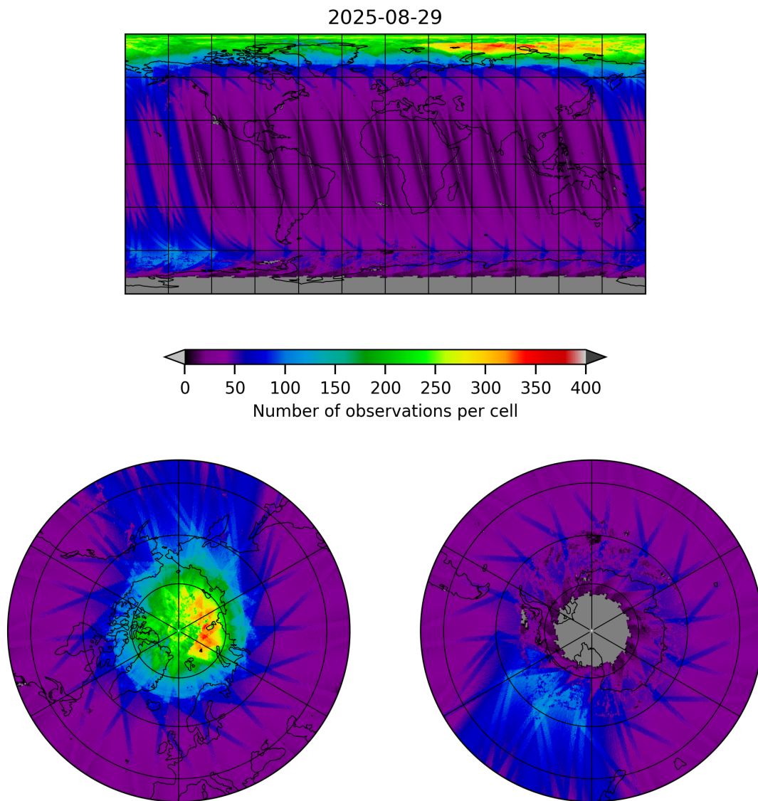
Figure 11: Map of the number of observations for 2025-08-28 to 2025-08-30
