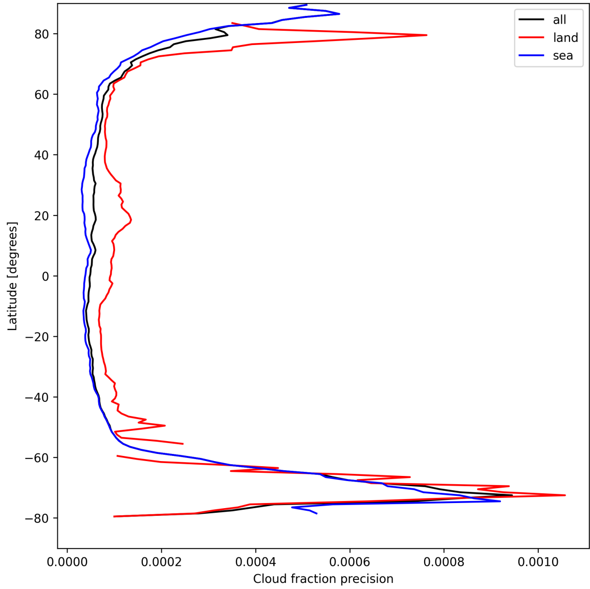
Figure 16: Zonal average of “Cloud fraction precision” for 2025-08-28 to 2025-08-30.
