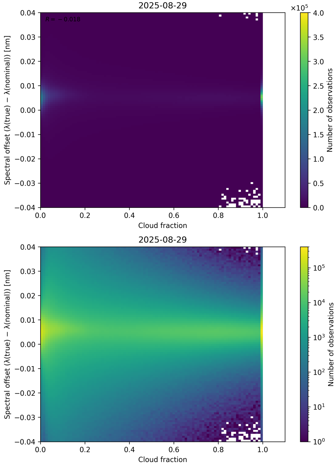
Figure 76: Scatter density plot of “Cloud fraction” against “Spectral offset ( \lambda_{\text{true}} - \lambda_{\text{nominal}} )” for 2025-08-28 to 2025-08-30.
