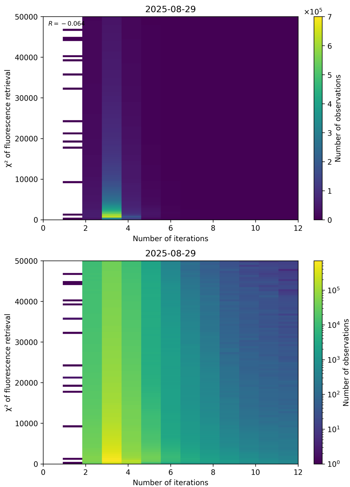
Figure 97: Scatter density plot of “Number of iterations” against “ \chi^2 of fluorescence retrieval” for 2025-08-28 to 2025-08-30.
