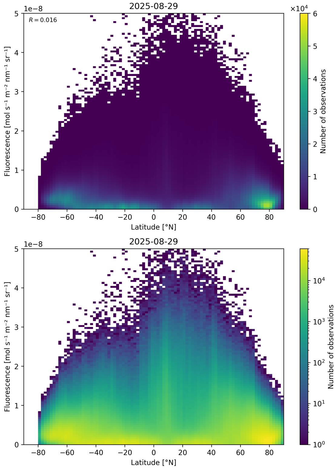
Figure 92: Scatter density plot of “Latitude” against “Fluorescence” for 2025-08-28 to 2025-08-30.
