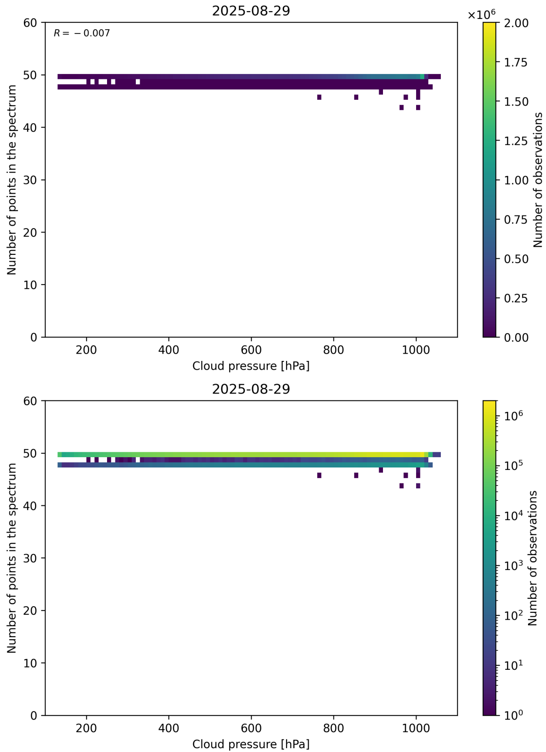
Figure 82: Scatter density plot of “Cloud pressure” against “Number of points in the spectrum” for 2025-08-28 to 2025-08-30.
