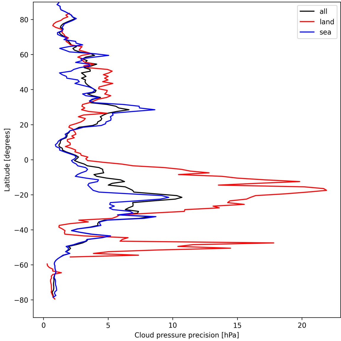
Figure 14: Zonal average of “Cloud pressure precision” for 2025-08-28 to 2025-08-30.
