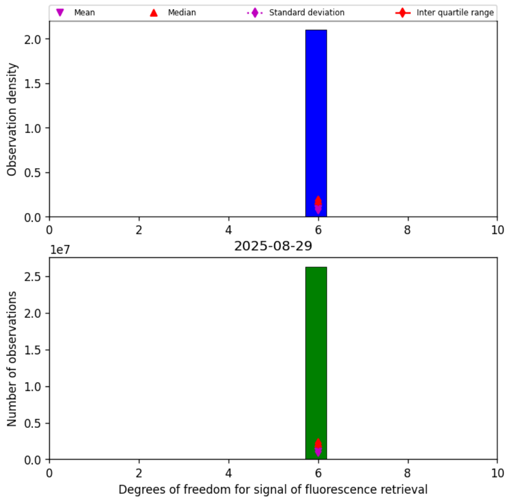
Figure 43: Histogram of "Degrees of freedom for signal of fluorescence retrieval" for 2025-08-28 to 2025-08-30
