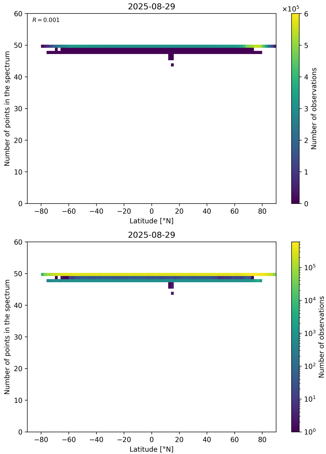
Figure 94: Scatter density plot of “Latitude” against “Number of points in the spectrum” for 2025-08-28 to 2025-08-30.
