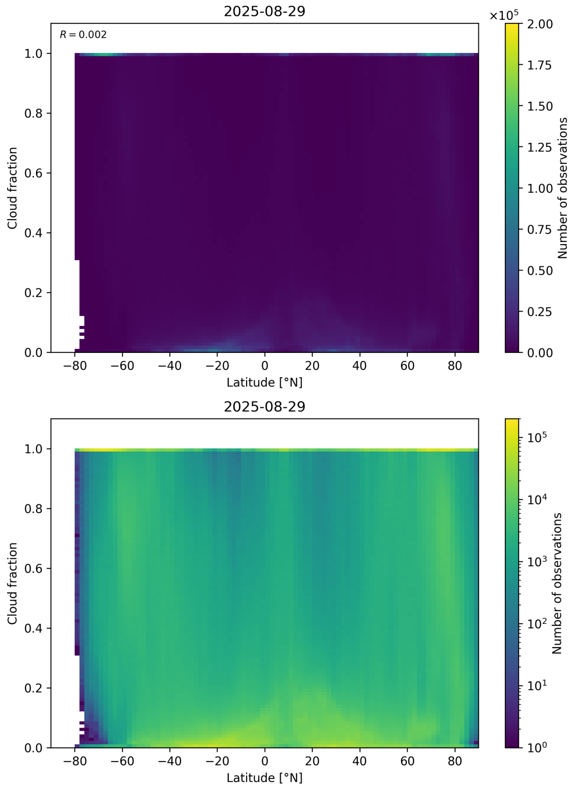
Figure 90: Scatter density plot of “Latitude” against “Cloud fraction” for 2025-08-28 to 2025-08-30.
