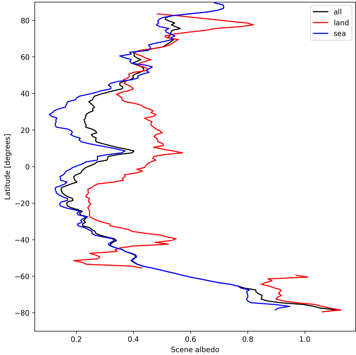
Figure 17: Zonal average of “Scene albedo” for 2025-08-28 to 2025-08-30.
