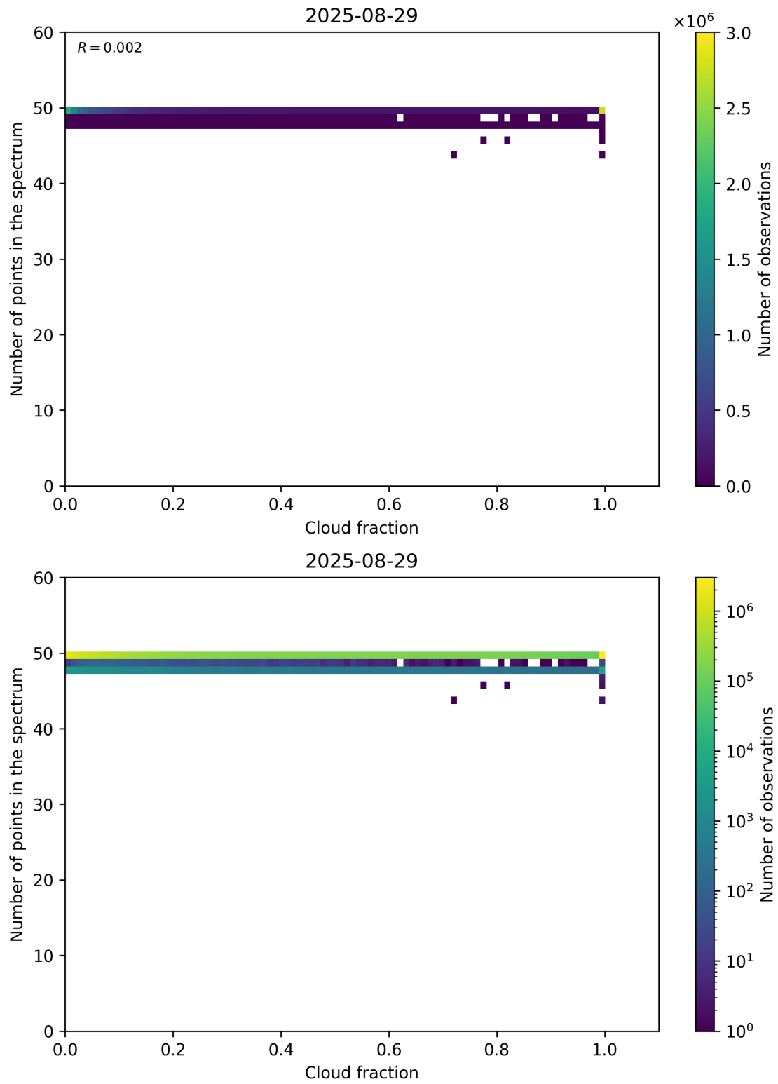
Figure 74: Scatter density plot of “Cloud fraction” against “Number of points in the spectrum” for 2025-08-28 to 2025-08-30.
