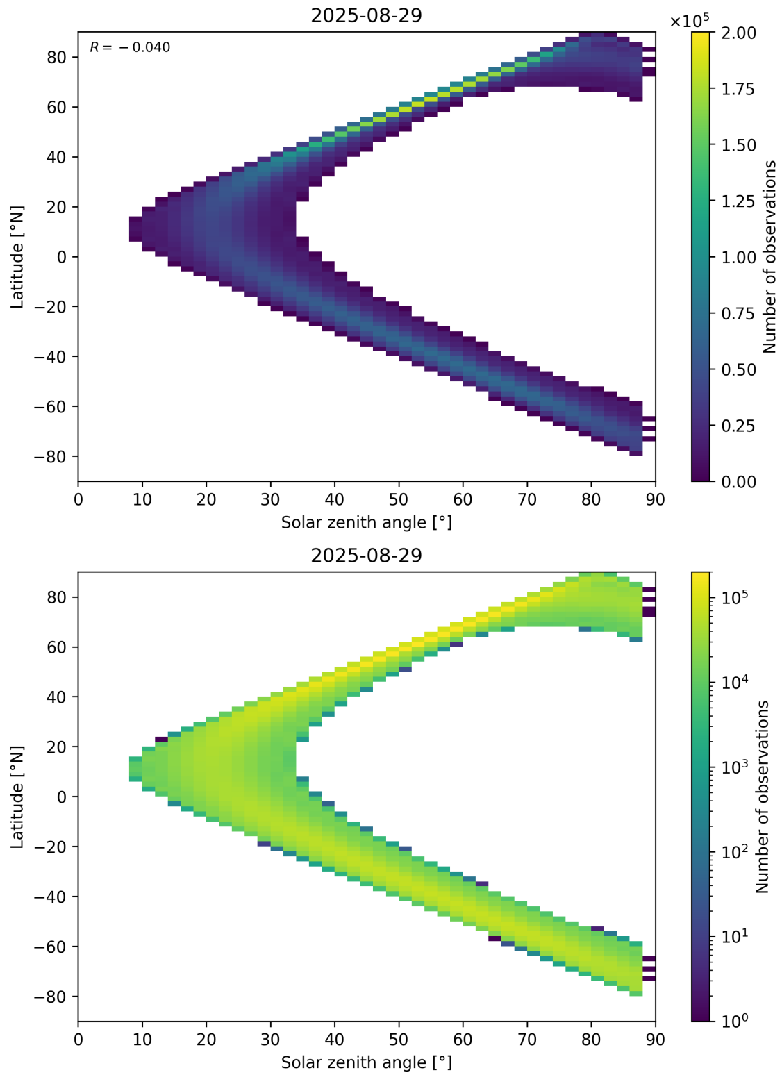
Figure 113: Scatter density plot of “Solar zenith angle” against “Latitude” for 2025-08-28 to 2025-08-30.
