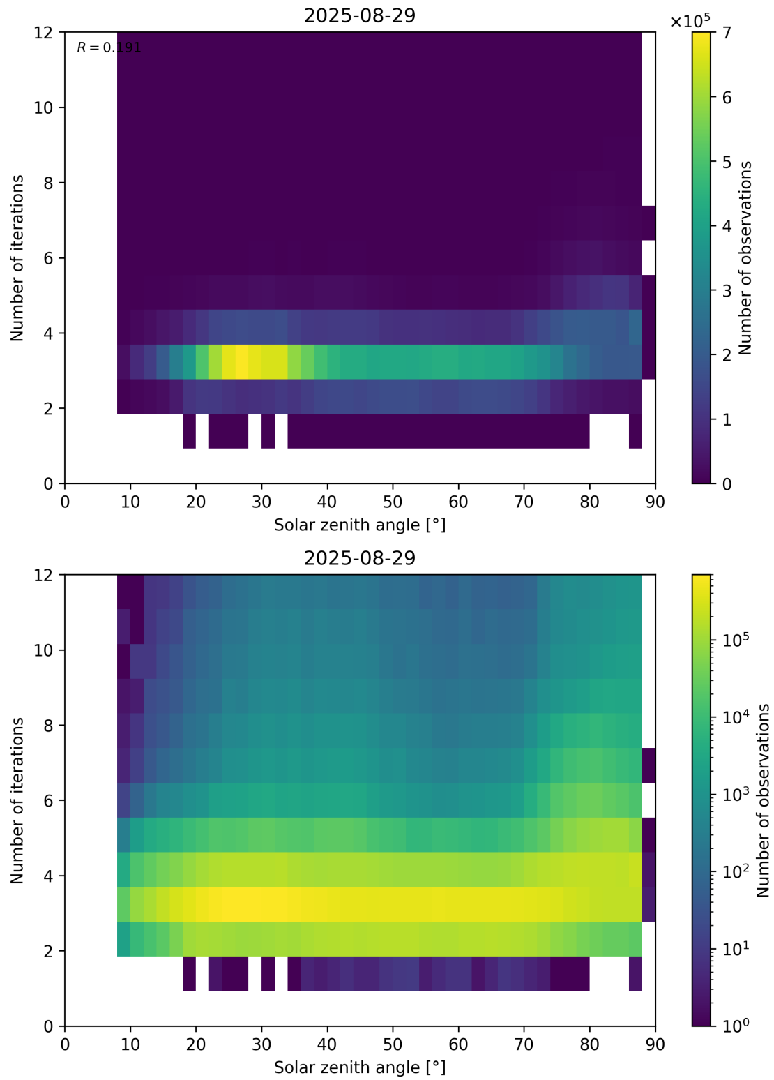
Figure 114: Scatter density plot of “Solar zenith angle” against “Number of iterations” for 2025-08-28 to 2025-08-30.
