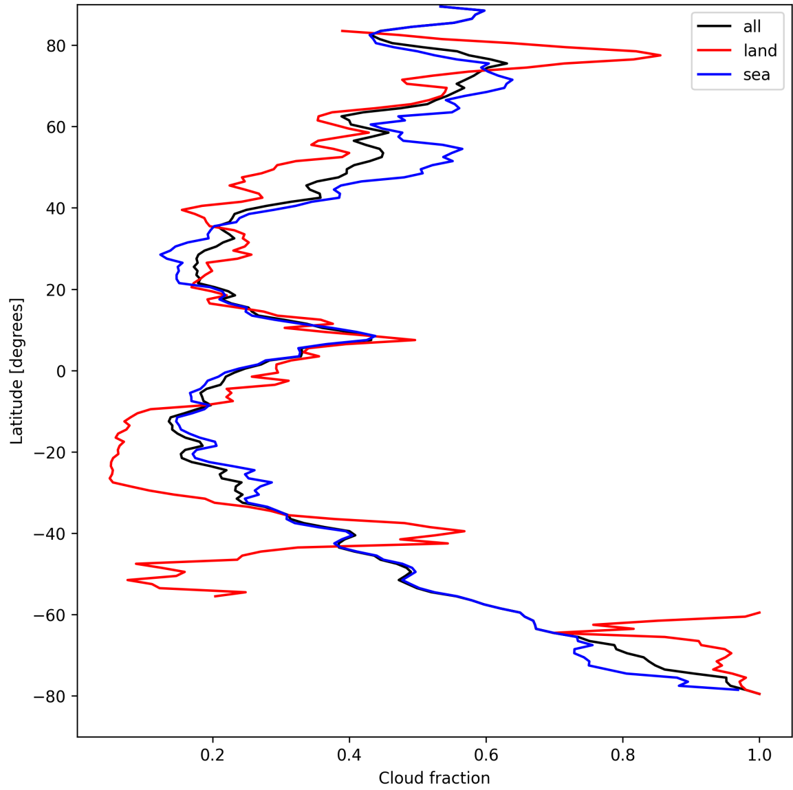
Figure 15: Zonal average of “Cloud fraction” for 2025-08-28 to 2025-08-30.
