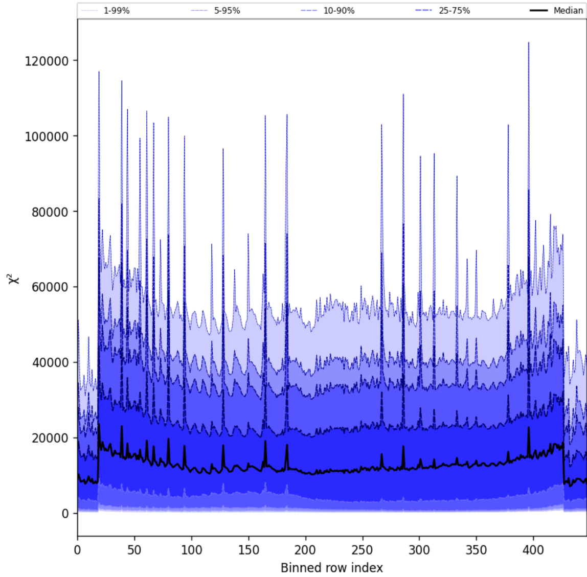
Figure 55: Along track statistics of “ \chi^2 ” for 2025-08-28 to 2025-08-30
