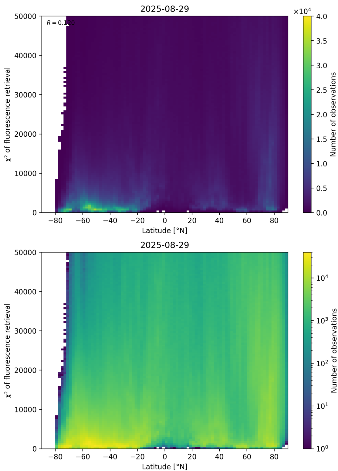
Figure 89: Scatter density plot of “Latitude” against “ \chi^2 of fluorescence retrieval” for 2025-08-28 to 2025-08-30.
