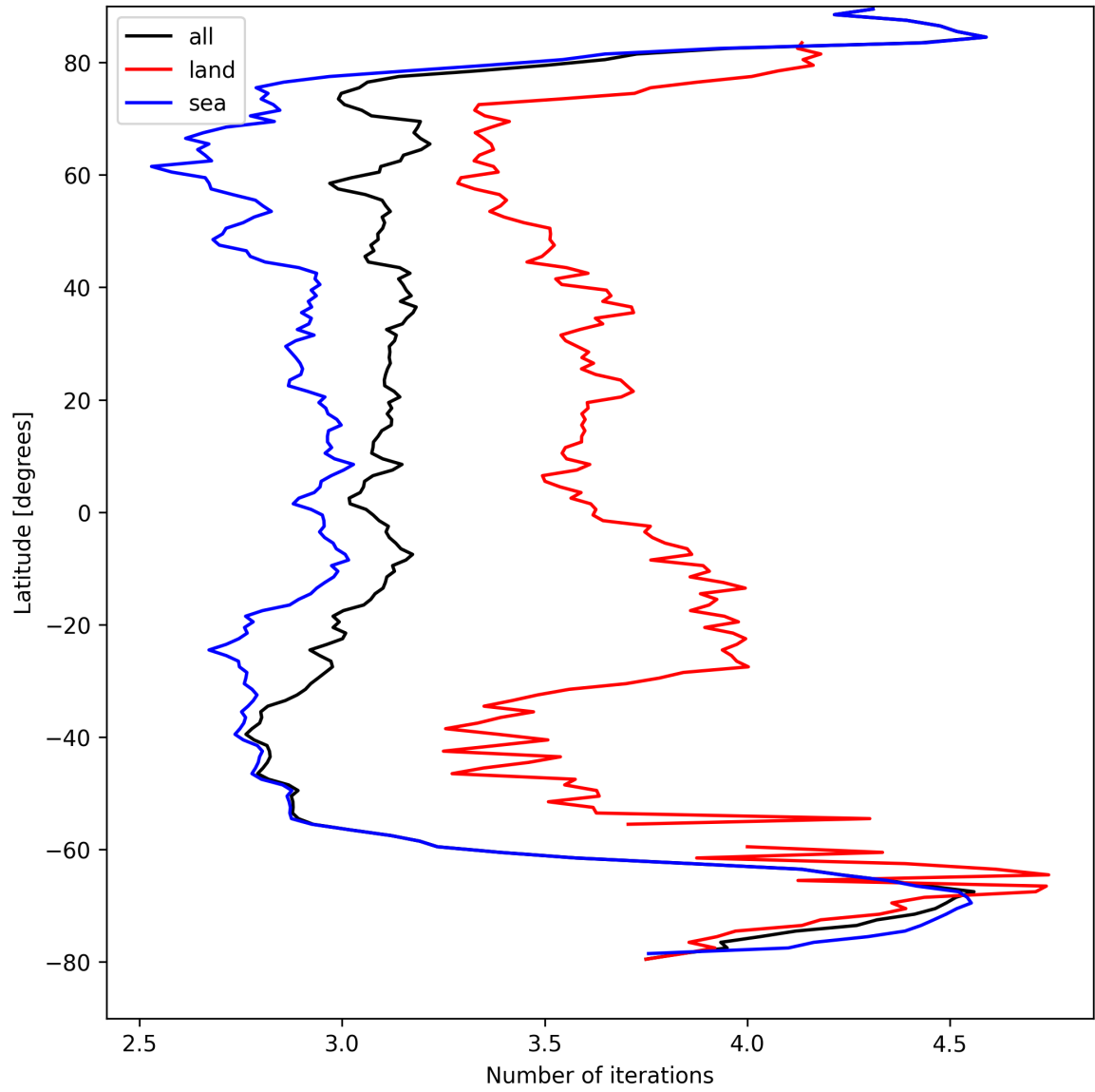
Figure 22: Zonal average of “Number of iterations” for 2025-08-28 to 2025-08-30.
