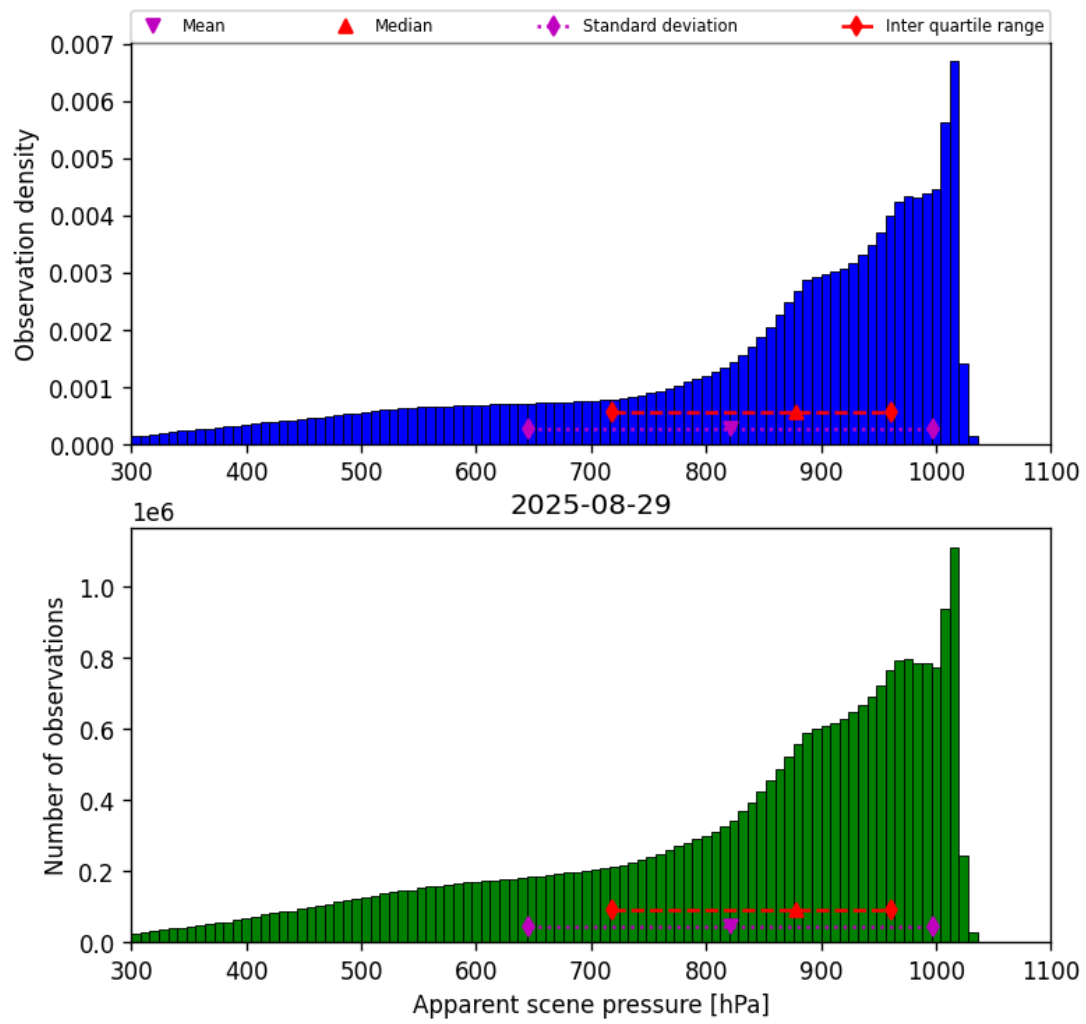
Figure 36: Histogram of “Apparent scene pressure” for 2025-08-28 to 2025-08-30
