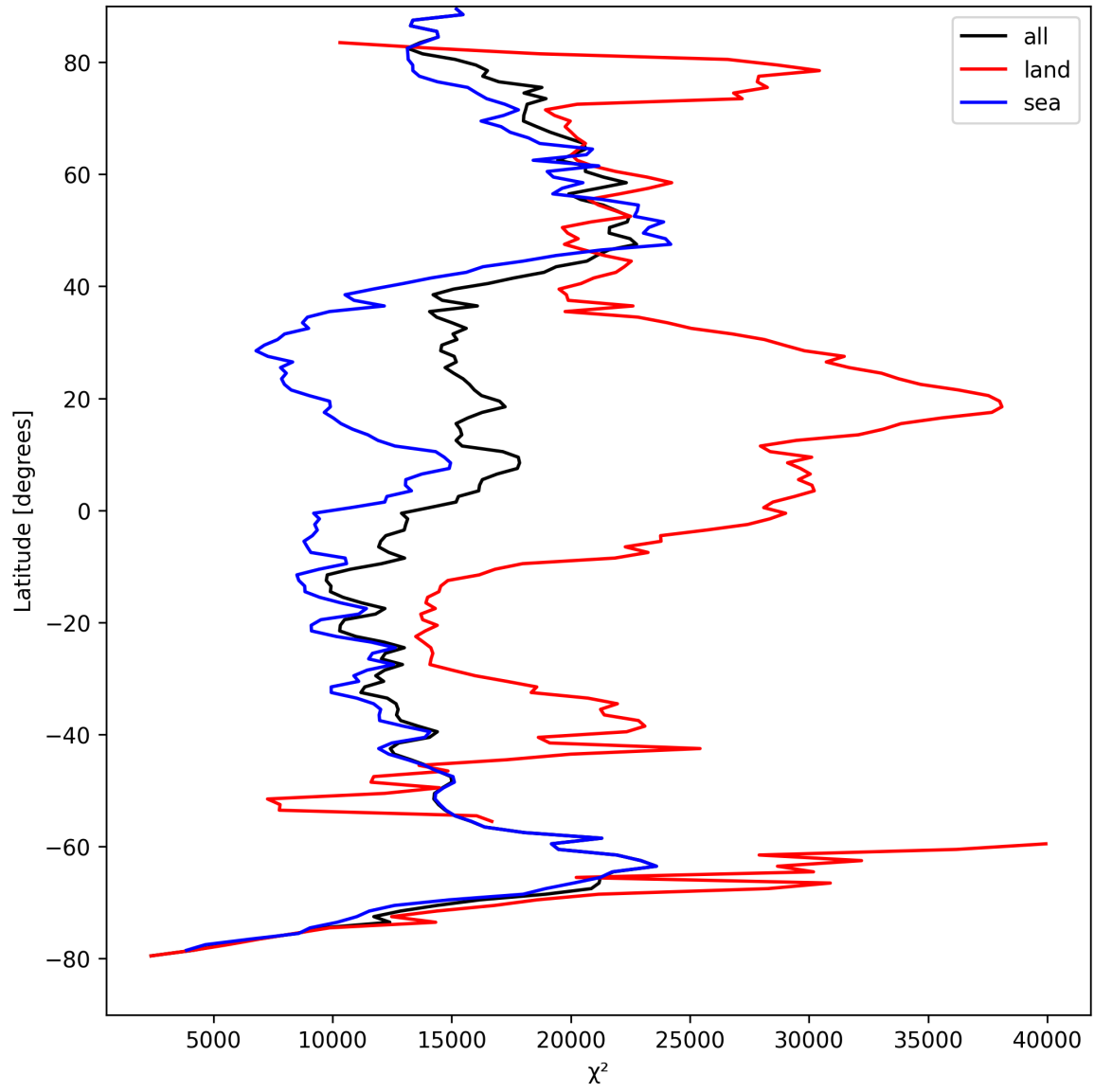
Figure 21: Zonal average of “ \chi^2 ” for 2025-08-28 to 2025-08-30.
