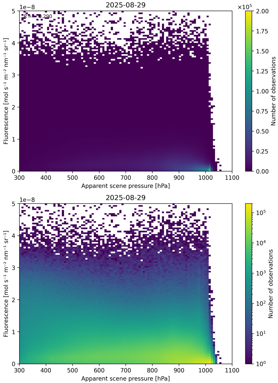
Figure 64: Scatter density plot of “Apparent scene pressure” against “Fluorescence” for 2025-08-28 to 2025-08-30.
