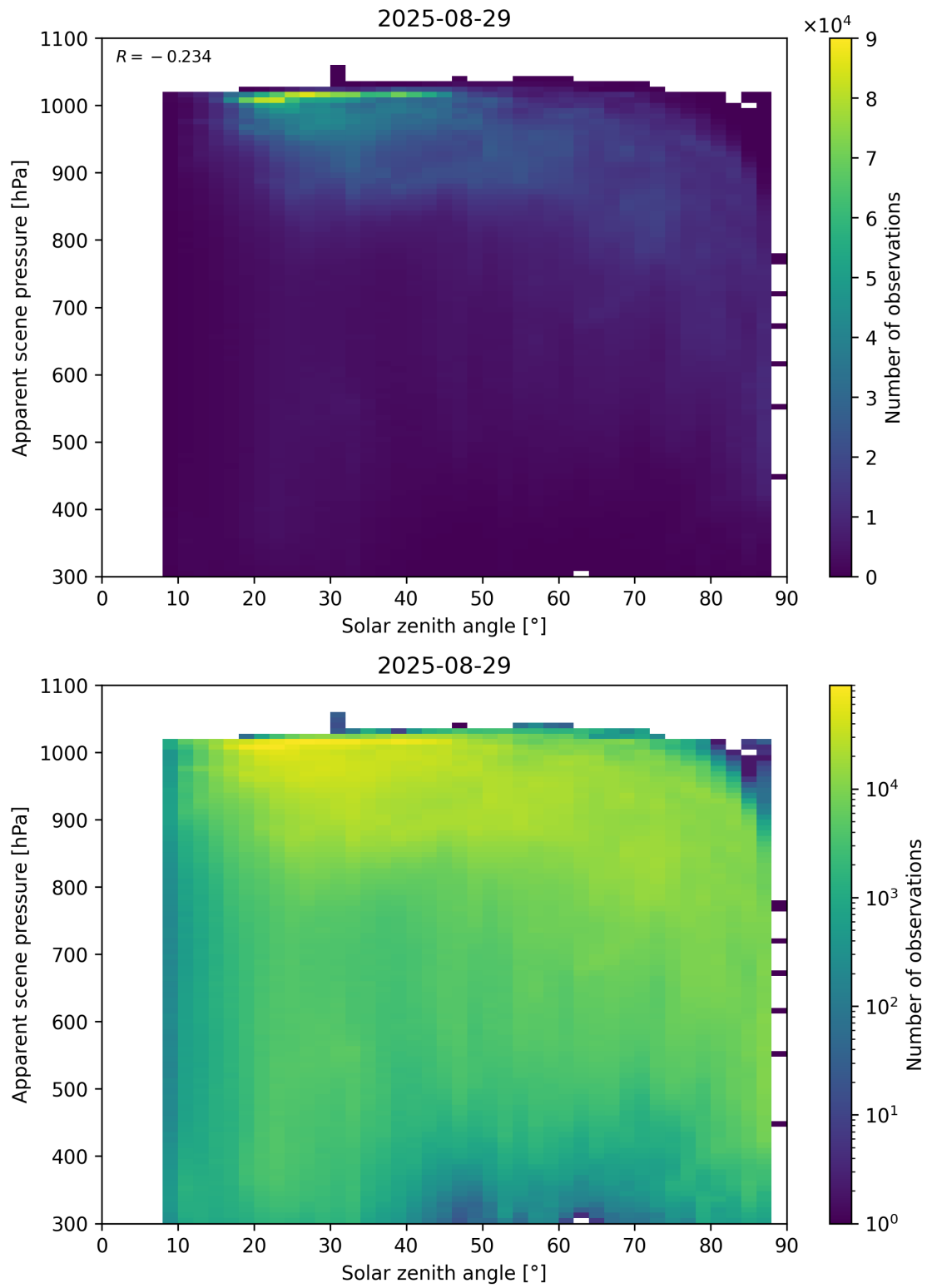
Figure 108: Scatter density plot of “Solar zenith angle” against “Apparent scene pressure” for 2025-08-28 to 2025-08-30.
