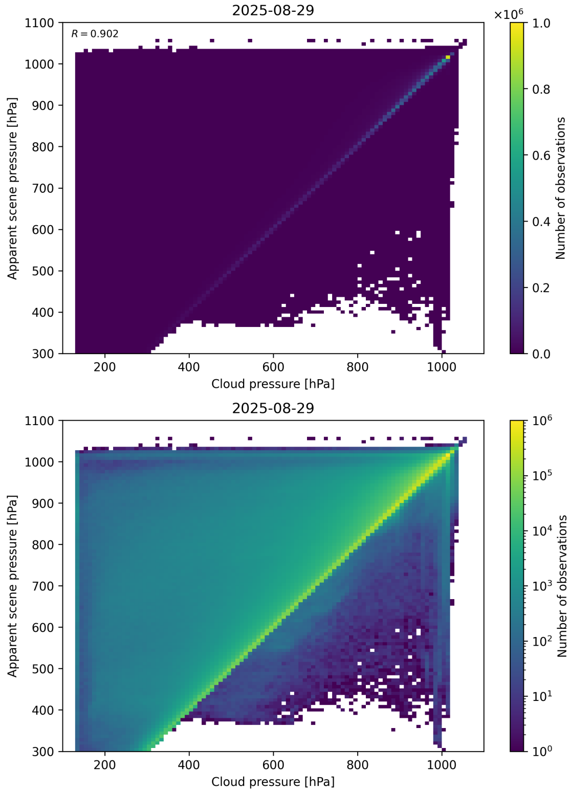
Figure 77: Scatter density plot of “Cloud pressure” against “Apparent scene pressure” for 2025-08-28 to 2025-08-30.
