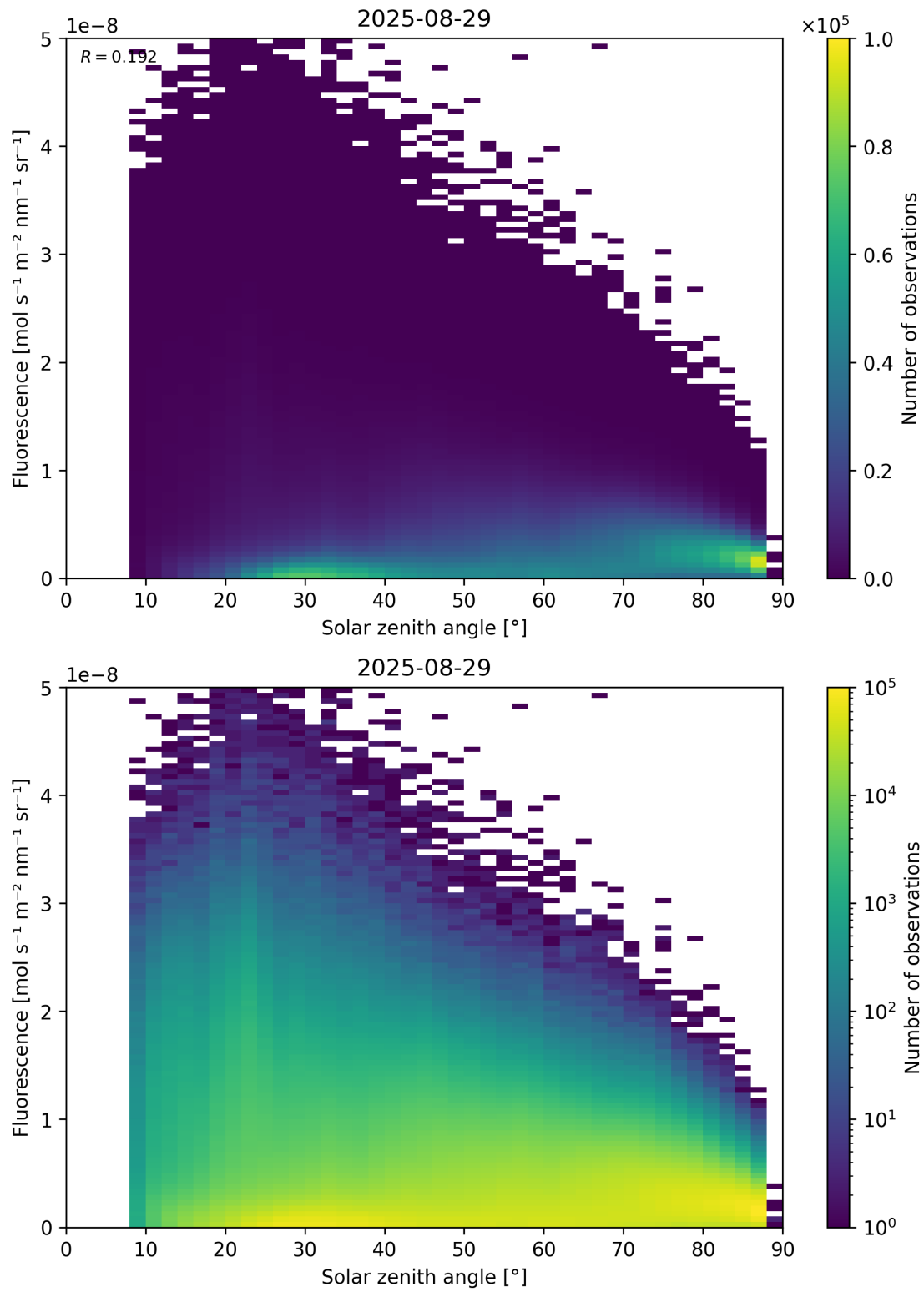
Figure 112: Scatter density plot of “Solar zenith angle” against “Fluorescence” for 2025-08-28 to 2025-08-30.
