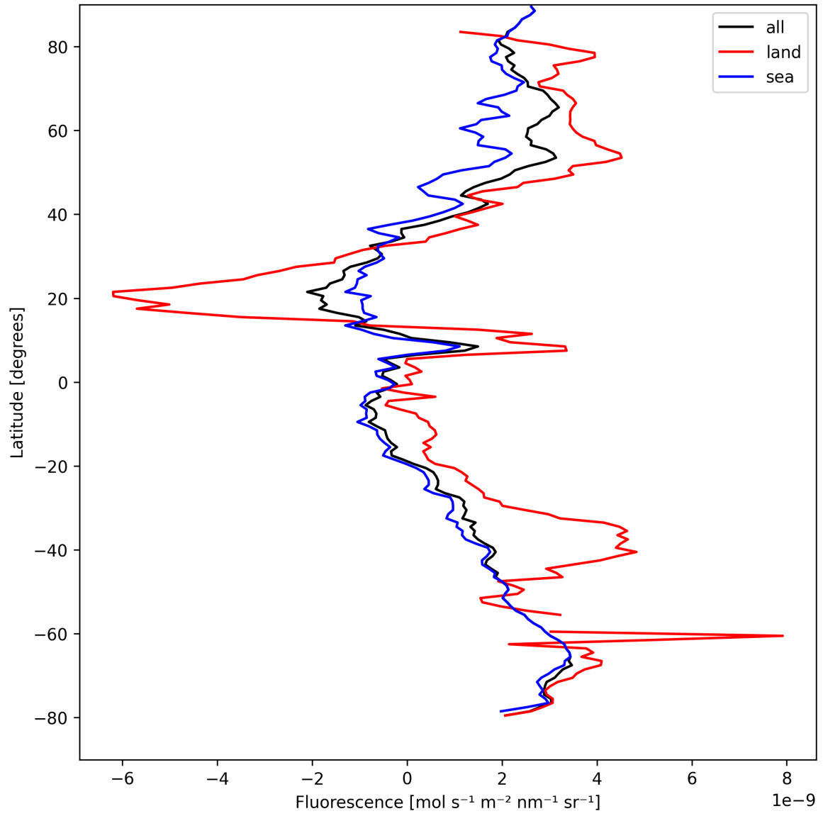
Figure 23: Zonal average of “Fluorescence” for 2025-08-28 to 2025-08-30.
