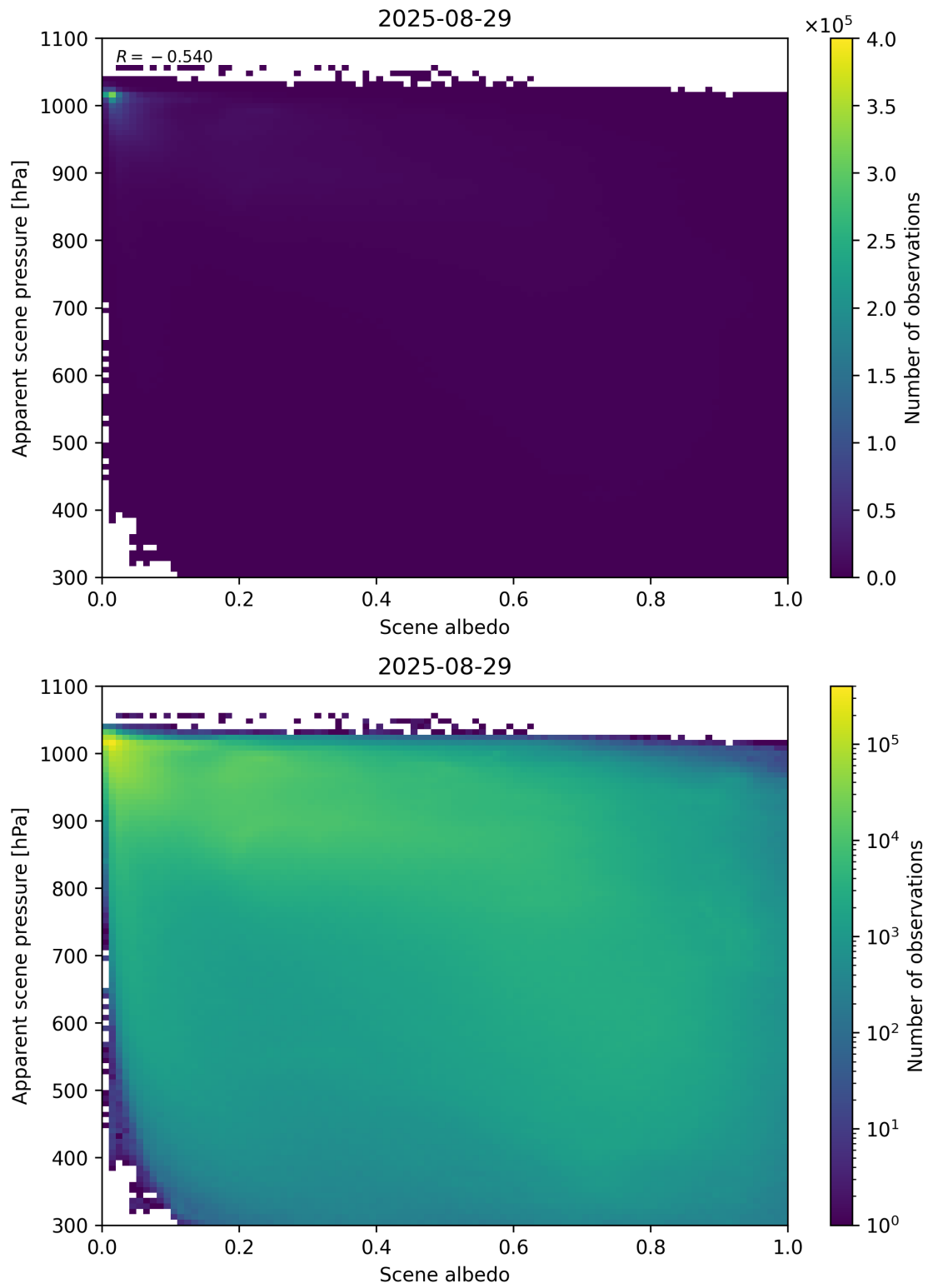
Figure 102: Scatter density plot of “Scene albedo” against “Apparent scene pressure” for 2025-08-28 to 2025-08-30.
