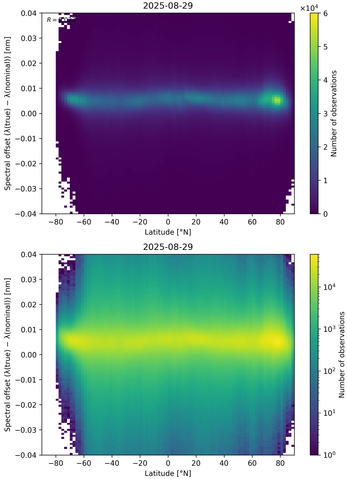
Figure 96: Scatter density plot of “Latitude” against “Spectral offset ( \lambda_{\text{true}} - \lambda_{\text{nominal}} )” for 2025-08-28 to 2025-08-30.
