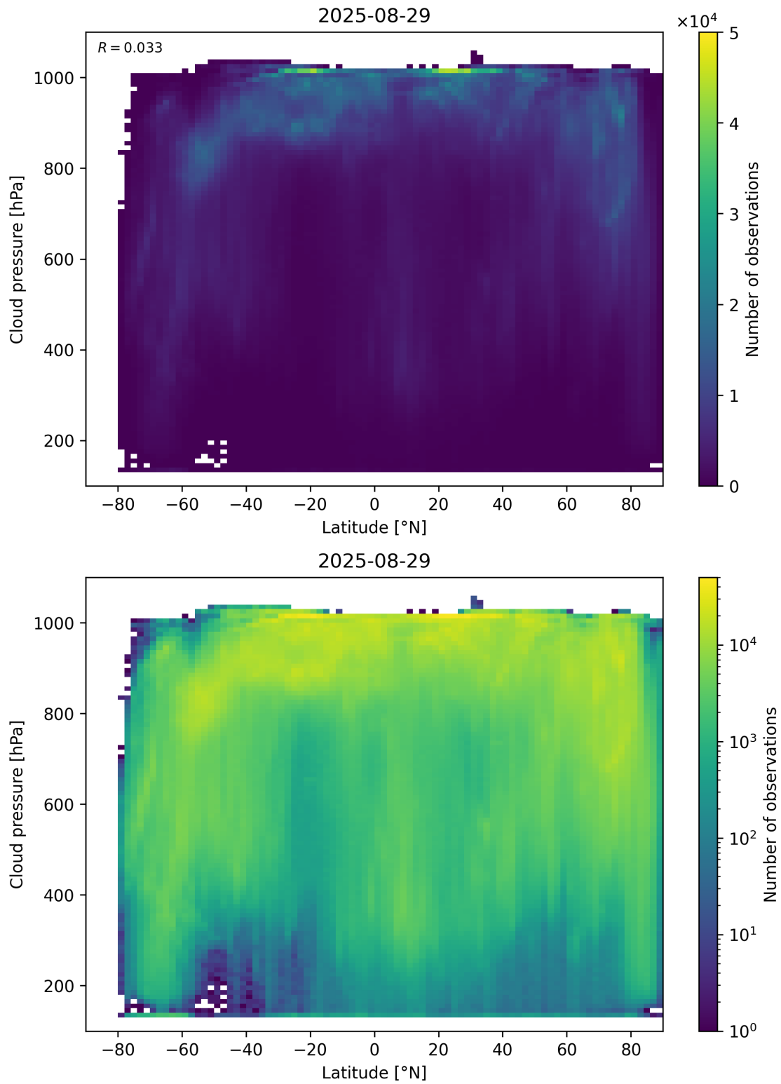
Figure 91: Scatter density plot of “Latitude” against “Cloud pressure” for 2025-08-28 to 2025-08-30.
