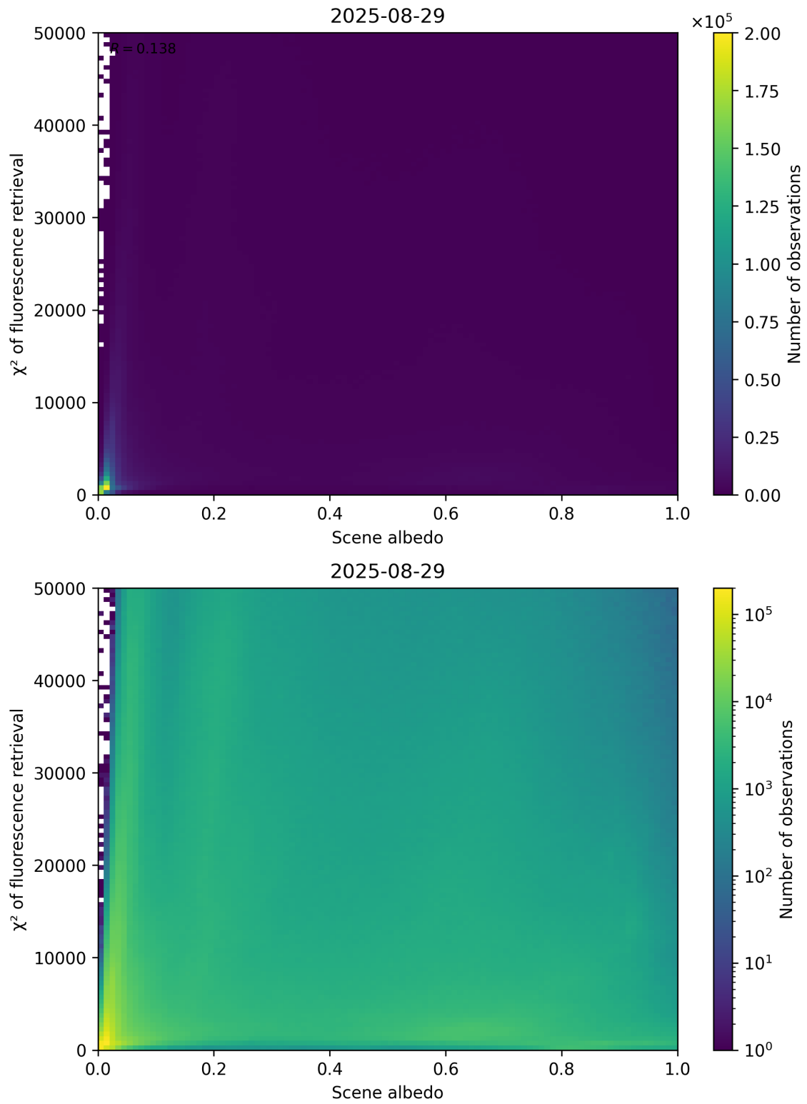
Figure 103: Scatter density plot of “Scene albedo” against “ \chi^2 of fluorescence retrieval” for 2025-08-28 to 2025-08-30.
