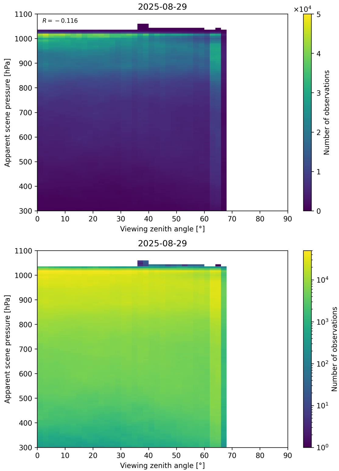
Figure 118: Scatter density plot of “Viewing zenith angle” against “Apparent scene pressure” for 2025-08-28 to 2025-08-30.
