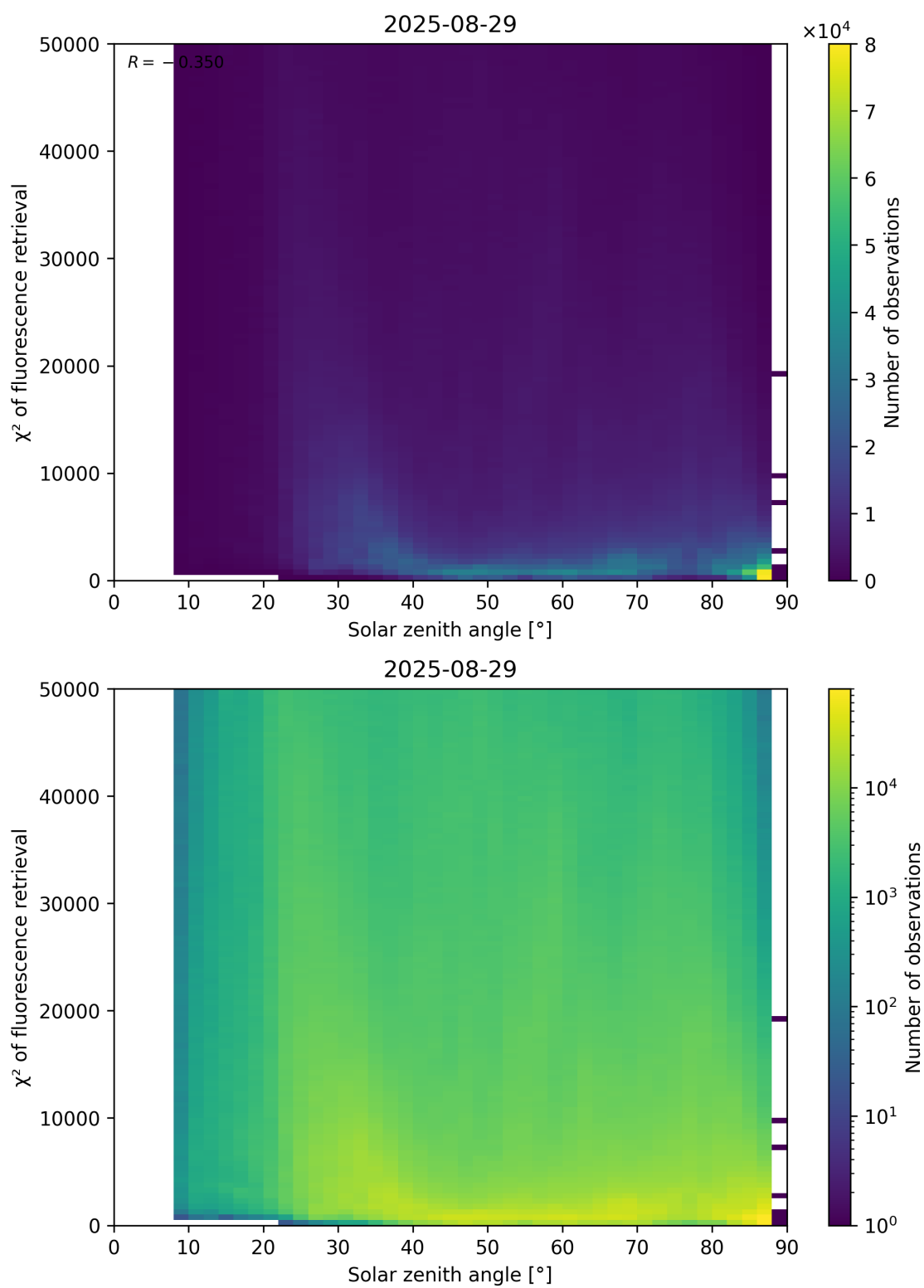
Figure 109: Scatter density plot of “Solar zenith angle” against “ \chi^2 of fluorescence retrieval” for 2025-08-28 to 2025-08-30.
