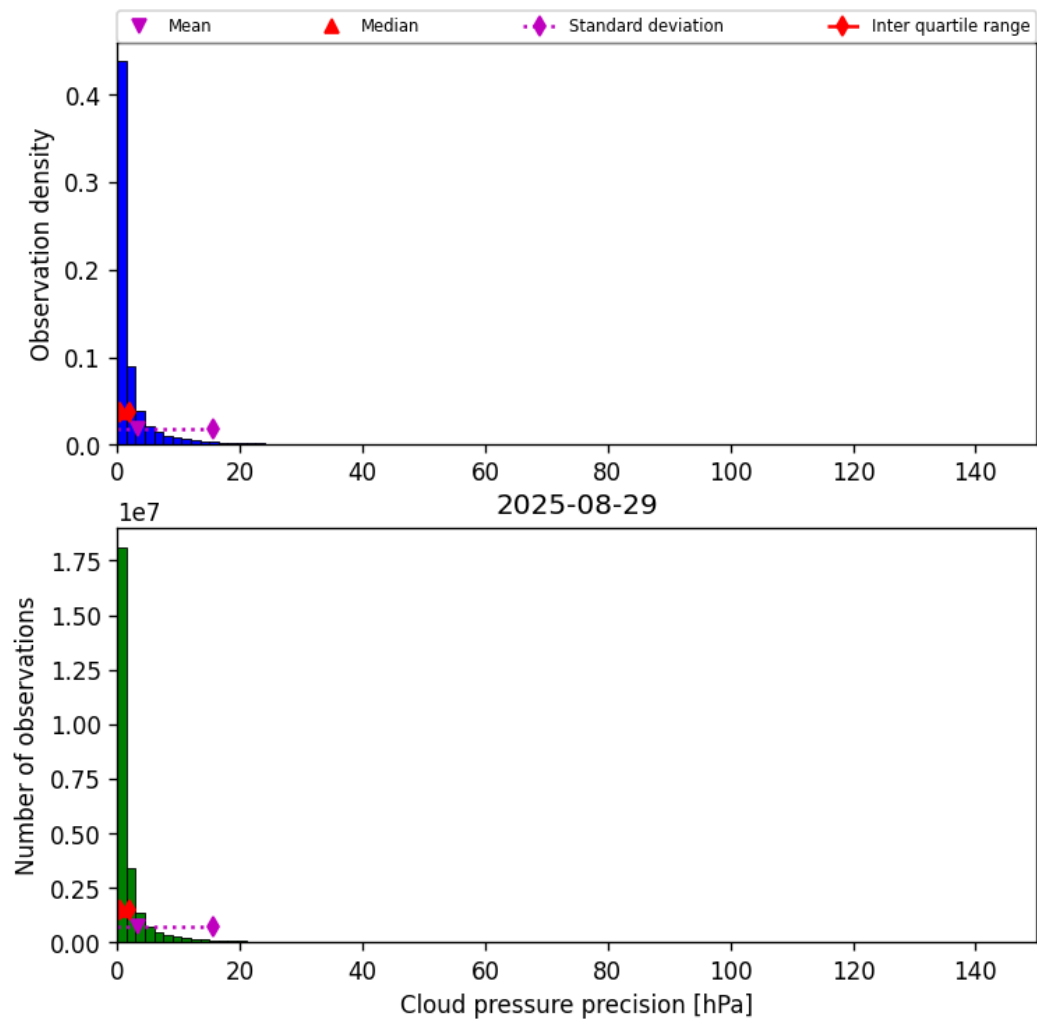
Figure 31: Histogram of “Cloud pressure precision” for 2025-08-28 to 2025-08-30
