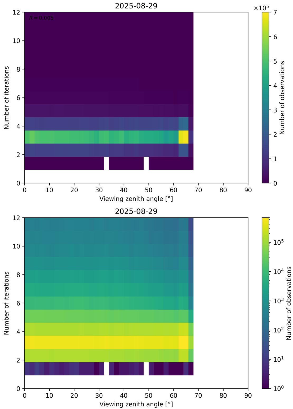
Figure 124: Scatter density plot of “Viewing zenith angle” against “Number of iterations” for 2025-08-28 to 2025-08-30.
