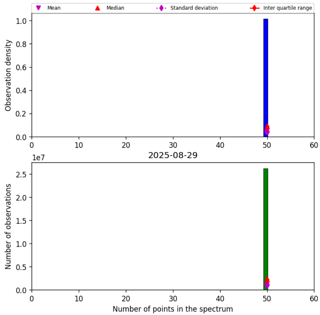
Figure 44: Histogram of "Number of points in the spectrum" for 2025-08-28 to 2025-08-30
