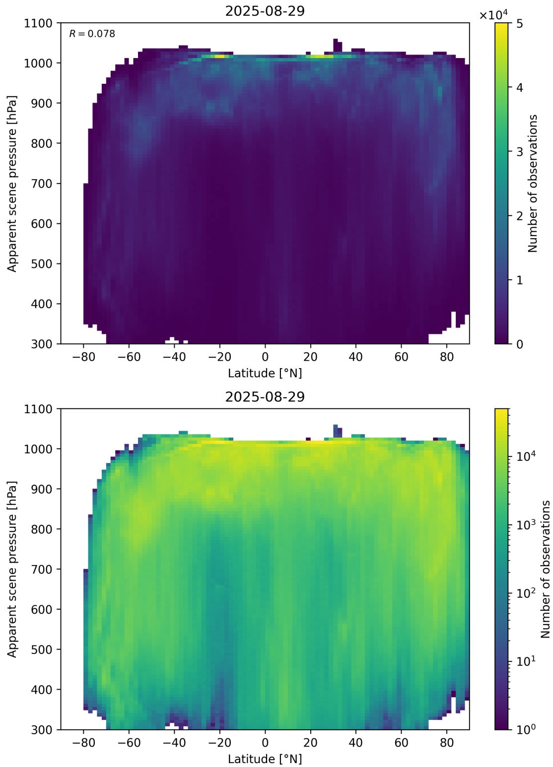
Figure 88: Scatter density plot of “Latitude” against “Apparent scene pressure” for 2025-08-28 to 2025-08-30.
