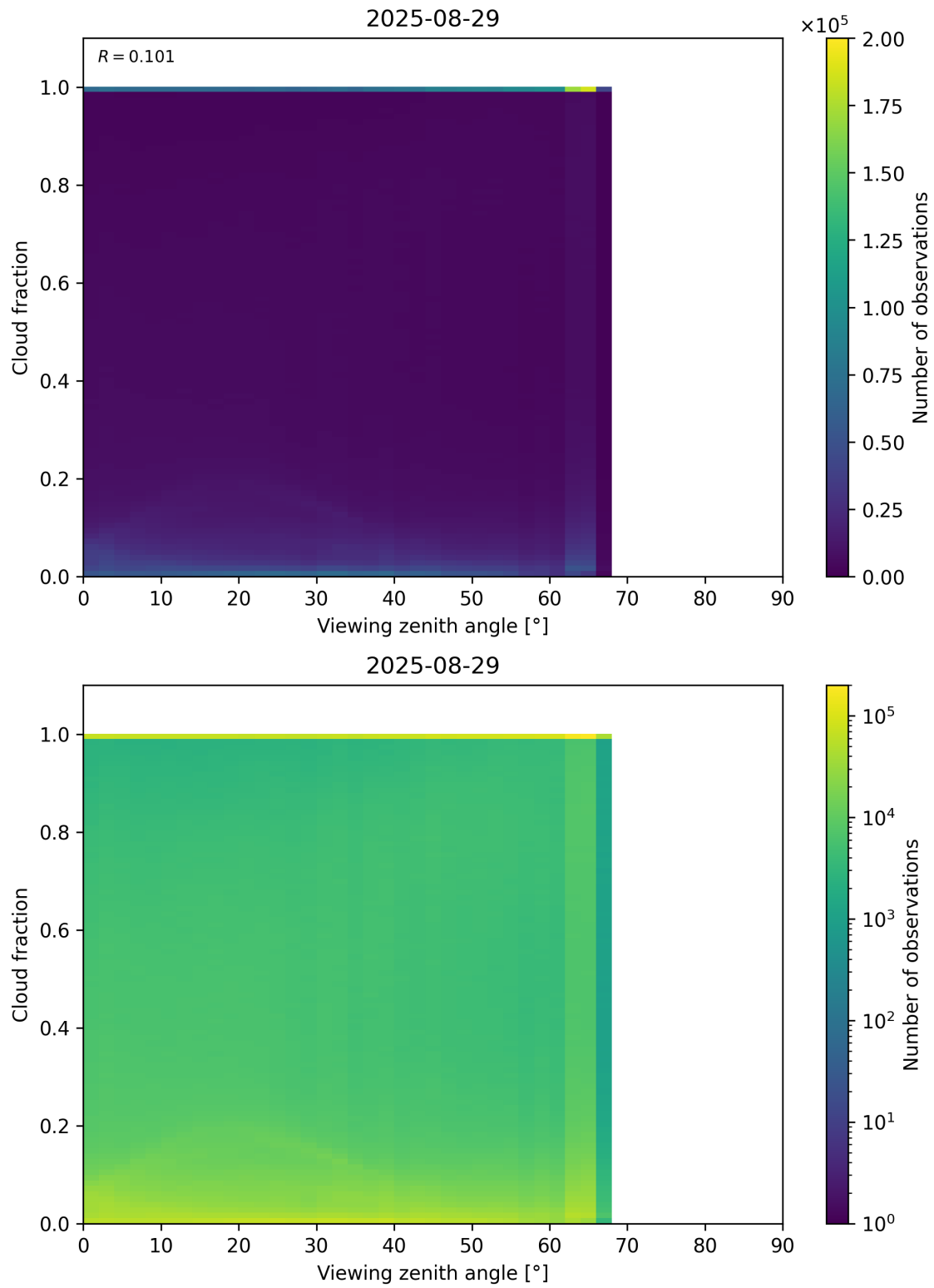
Figure 120: Scatter density plot of “Viewing zenith angle” against “Cloud fraction” for 2025-08-28 to 2025-08-30.
