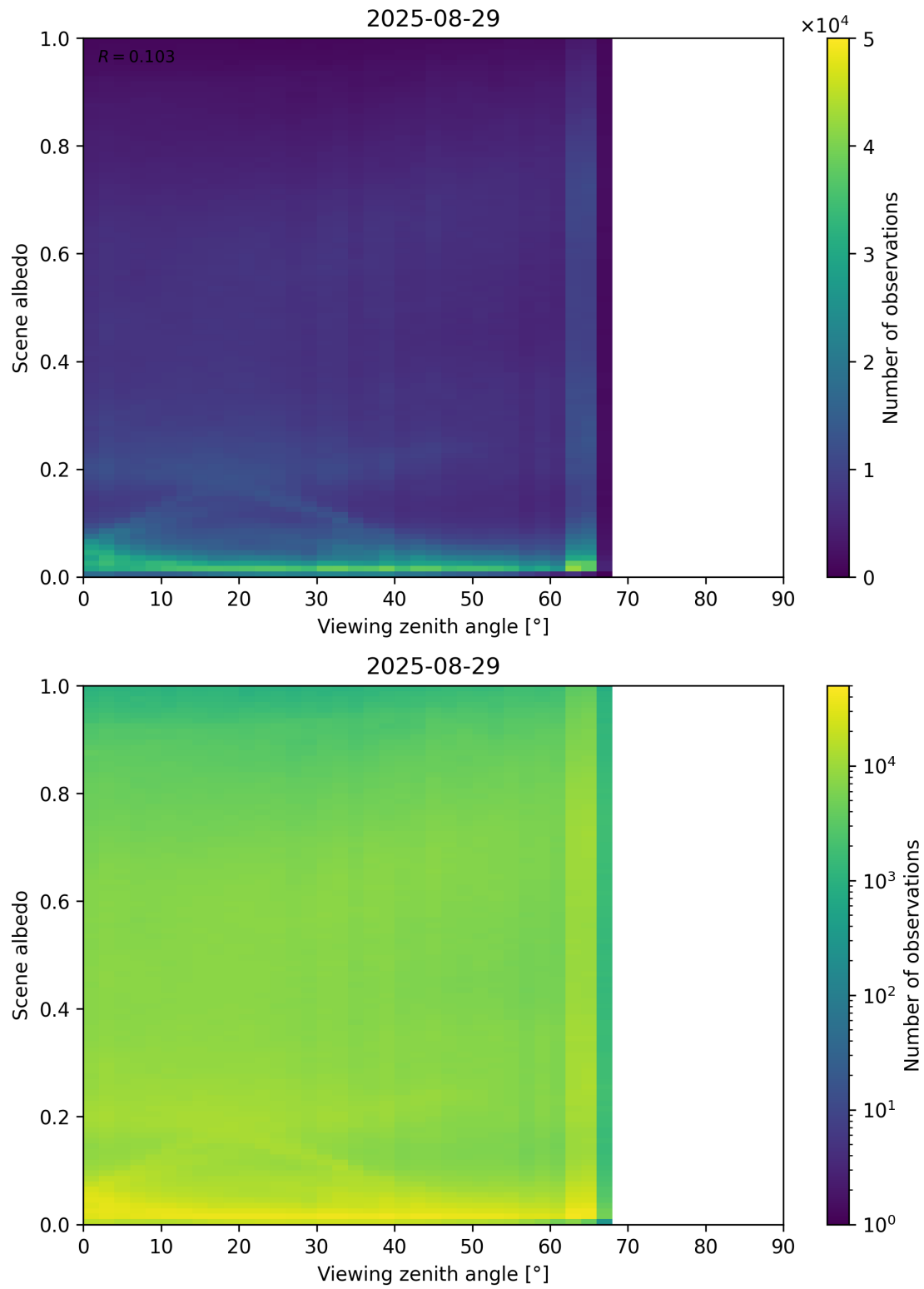
Figure 126: Scatter density plot of “Viewing zenith angle” against “Scene albedo” for 2025-08-28 to 2025-08-30.
