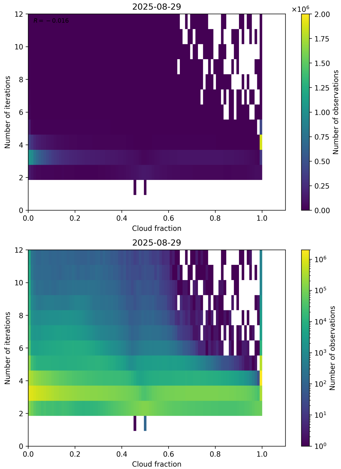
Figure 73: Scatter density plot of “Cloud fraction” against “Number of iterations” for 2025-08-28 to 2025-08-30.
