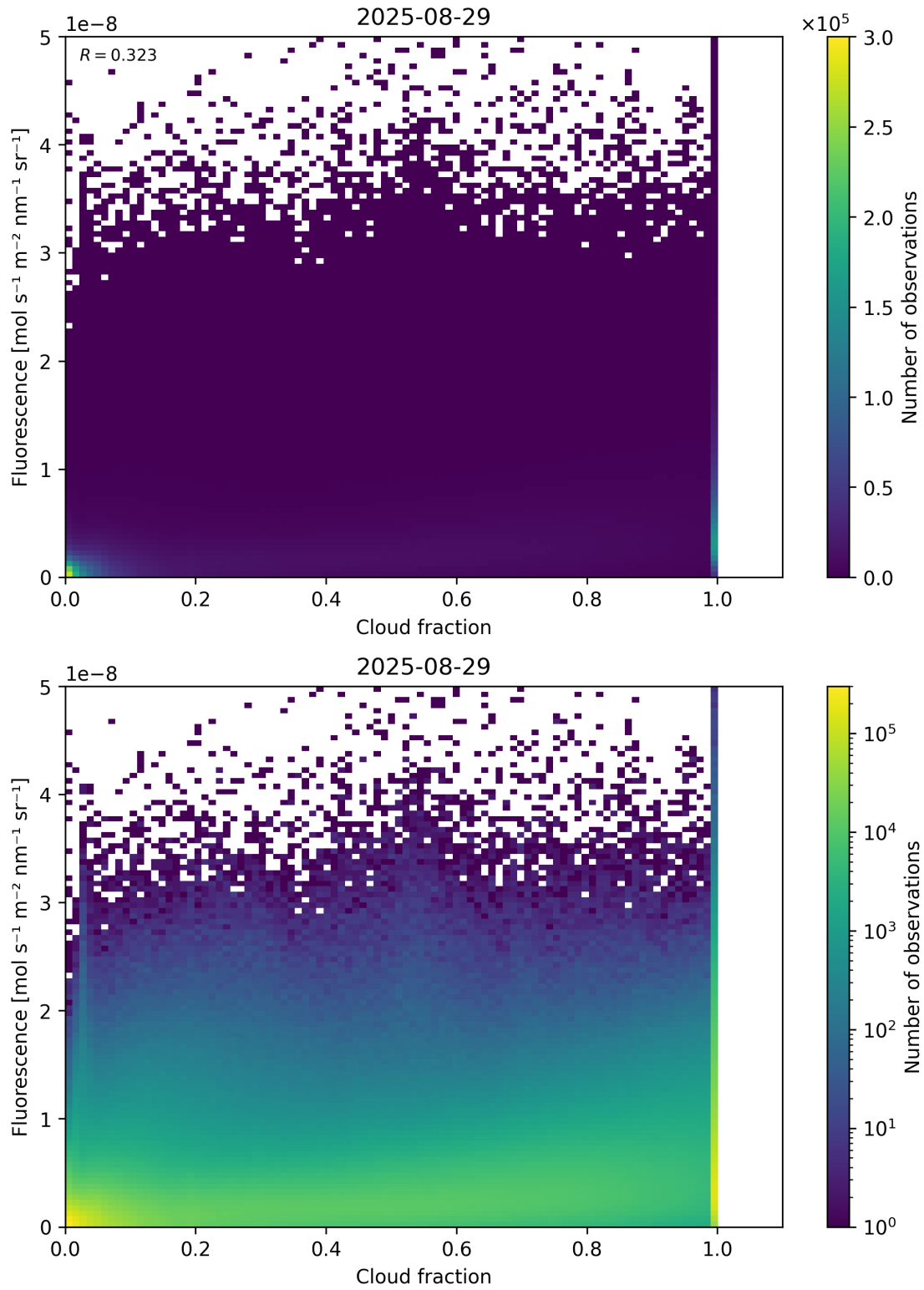
Figure 72: Scatter density plot of “Cloud fraction” against “Fluorescence” for 2025-08-28 to 2025-08-30.
