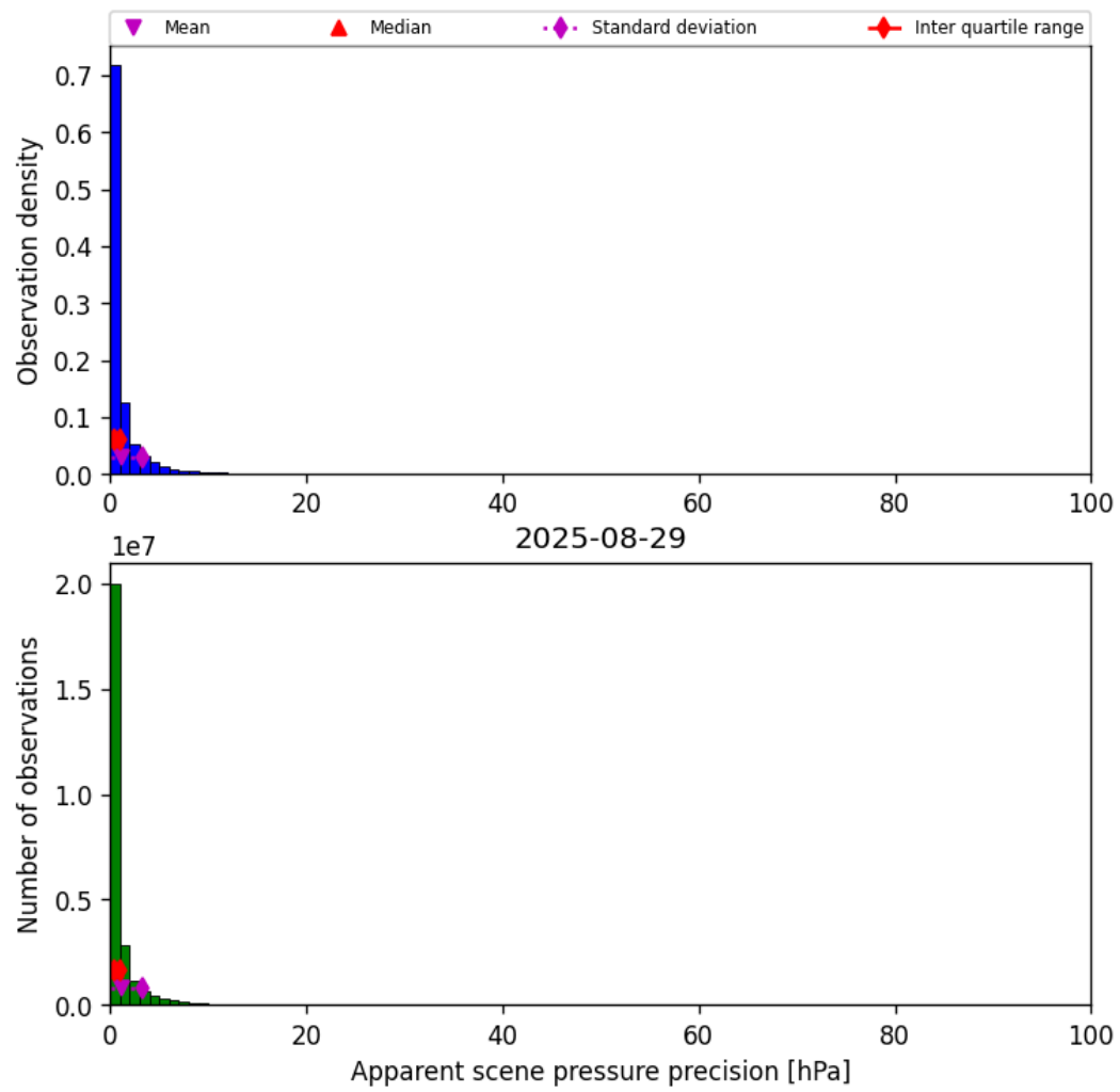
Figure 37: Histogram of “Apparent scene pressure precision” for 2025-08-28 to 2025-08-30
