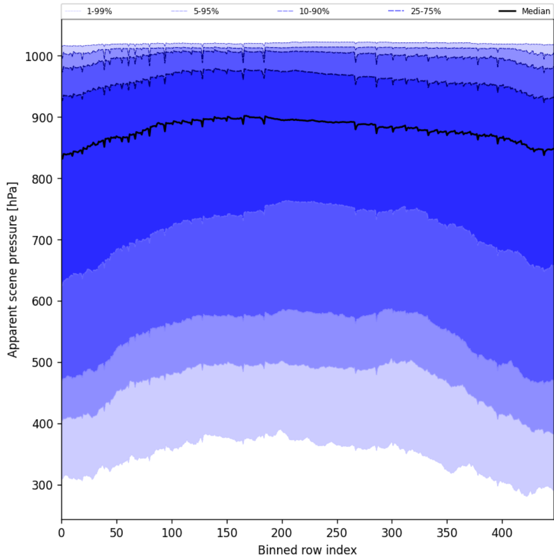
Figure 53: Along track statistics of “Apparent scene pressure” for 2025-08-28 to 2025-08-30
