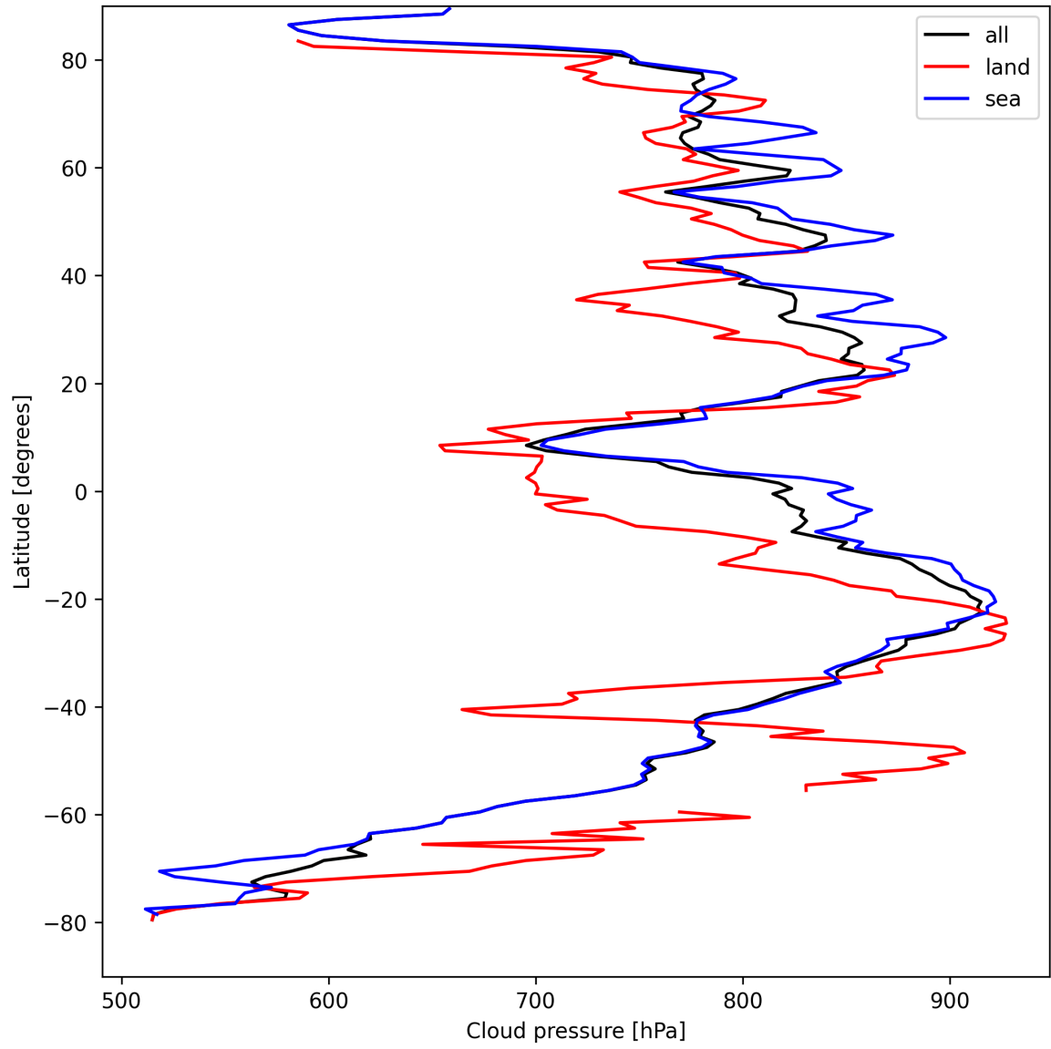
Figure 13: Zonal average of “Cloud pressure” for 2025-08-28 to 2025-08-30.
