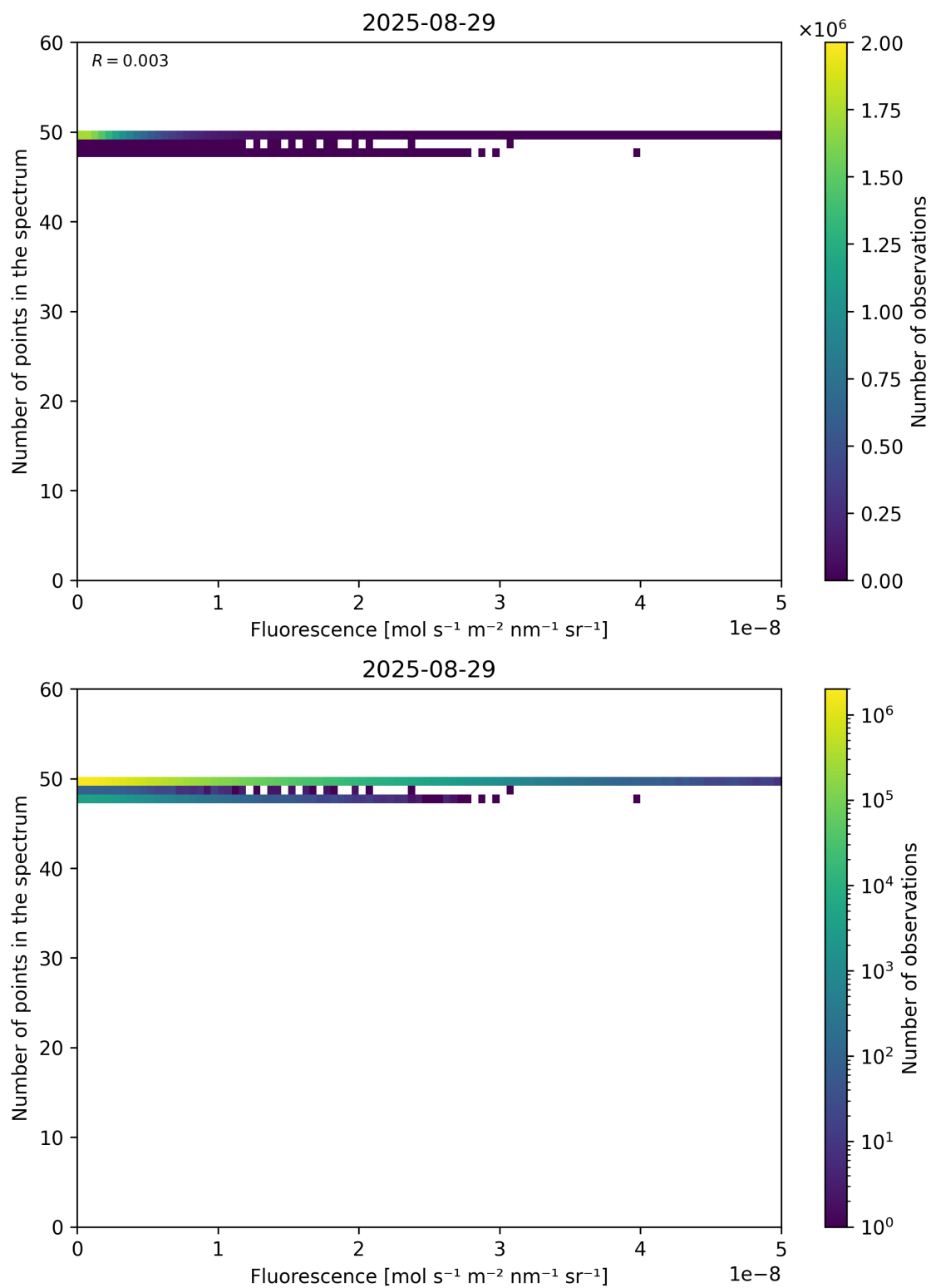
Figure 86: Scatter density plot of “Fluorescence” against “Number of points in the spectrum” for 2025-08-28 to 2025-08-30.
