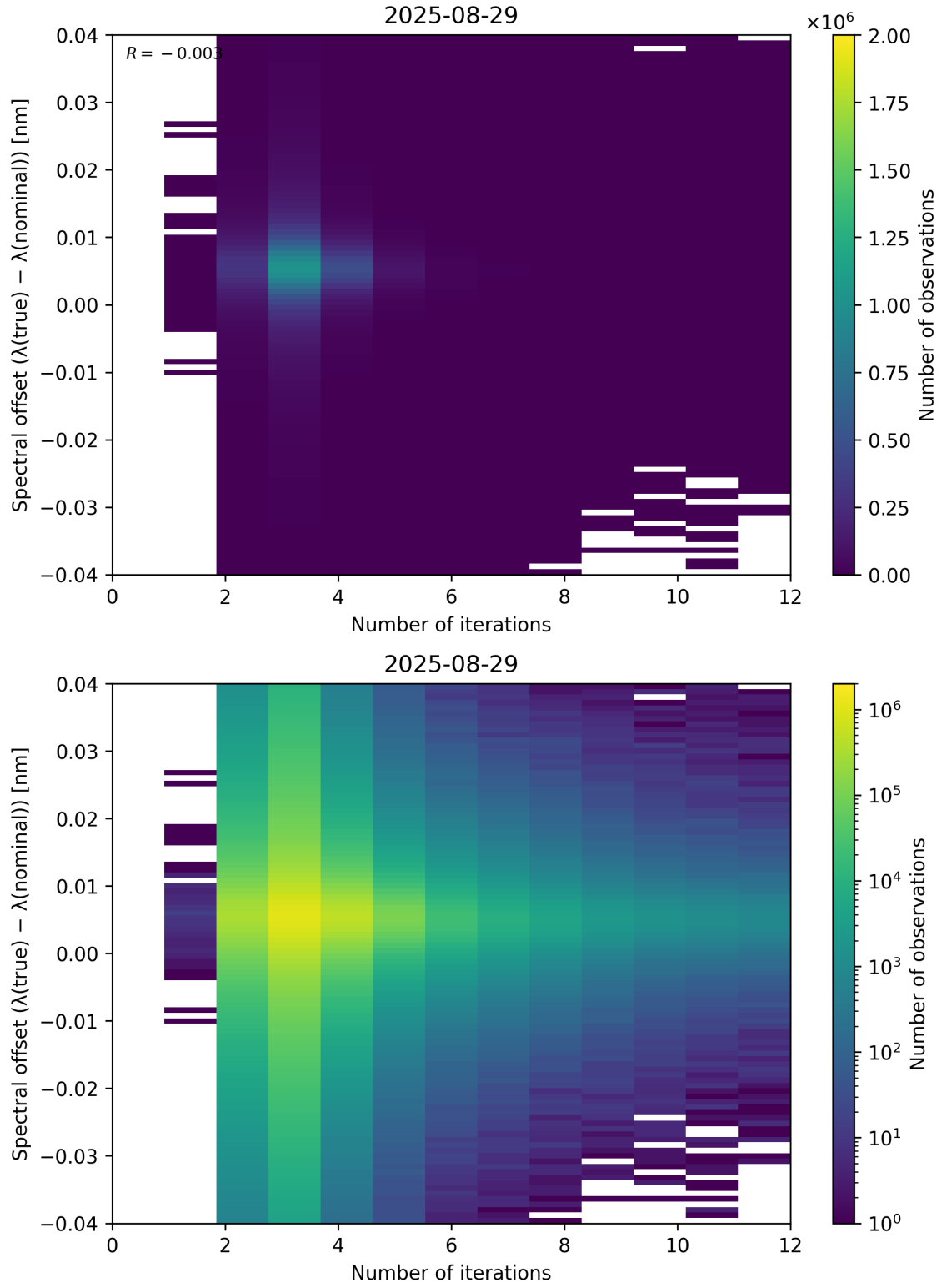
Figure 100: Scatter density plot of “Number of iterations” against “Spectral offset ( \lambda_{\text{true}} - \lambda_{\text{nominal}} )” for 2025-08-28 to 2025-08-30.
