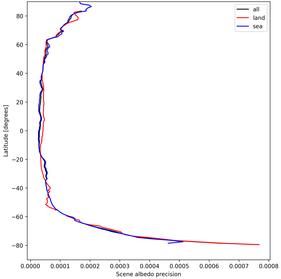
Figure 18: Zonal average of “Scene albedo precision” for 2025-08-28 to 2025-08-30.
