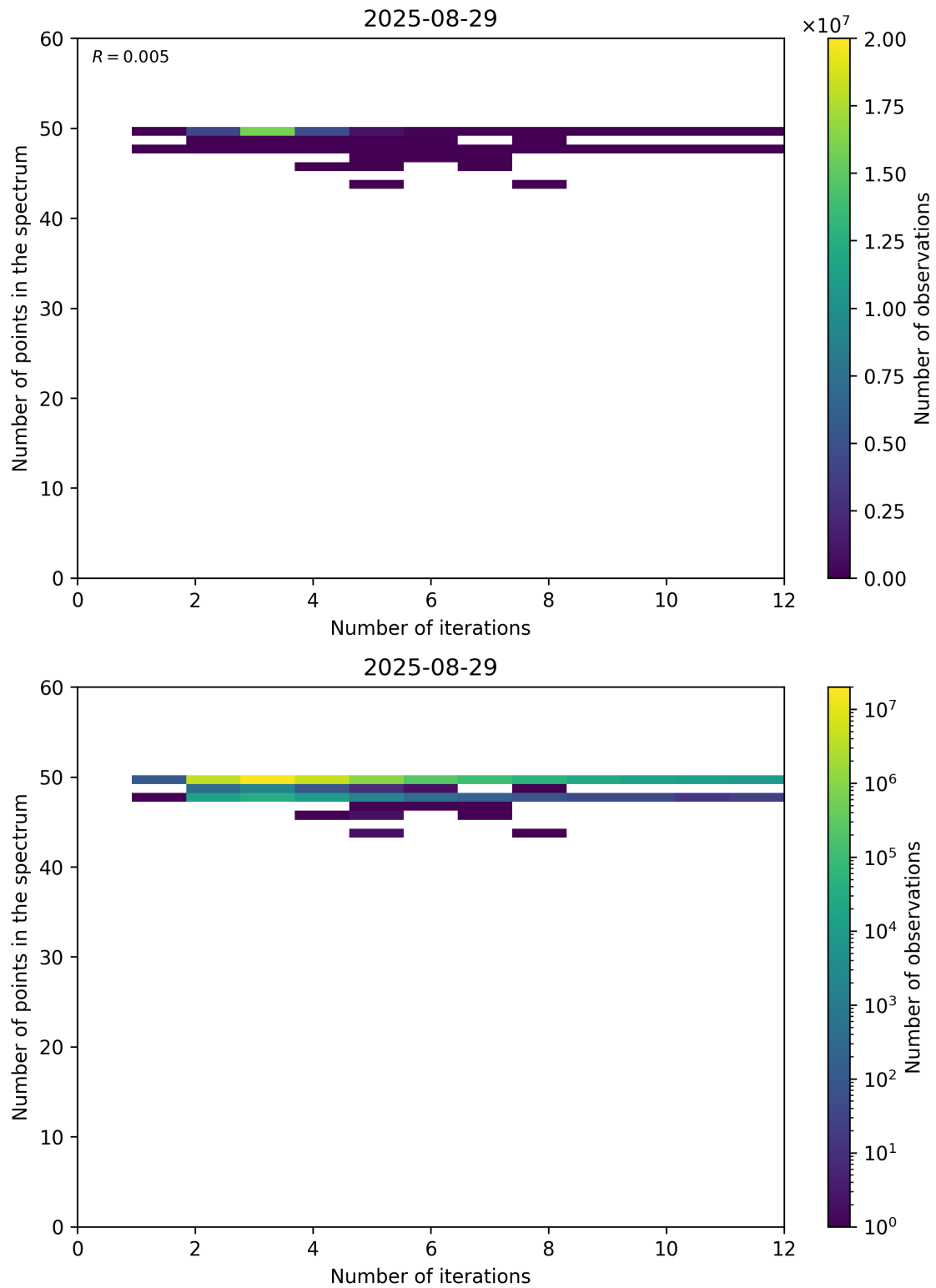
Figure 99: Scatter density plot of “Number of iterations” against “Number of points in the spectrum” for 2025-08-28 to 2025-08-30.
