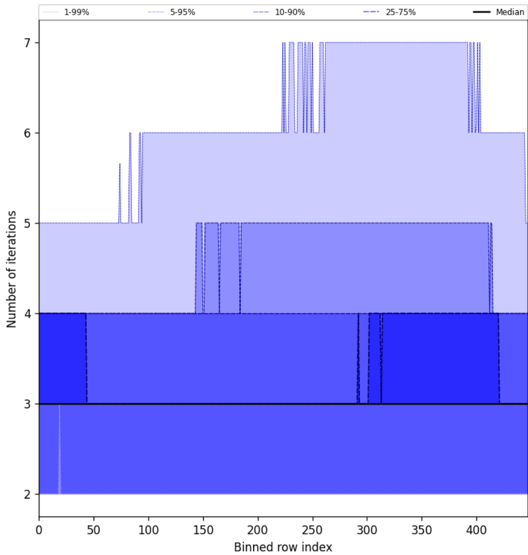
Figure 56: Along track statistics of “Number of iterations” for 2025-08-28 to 2025-08-30
