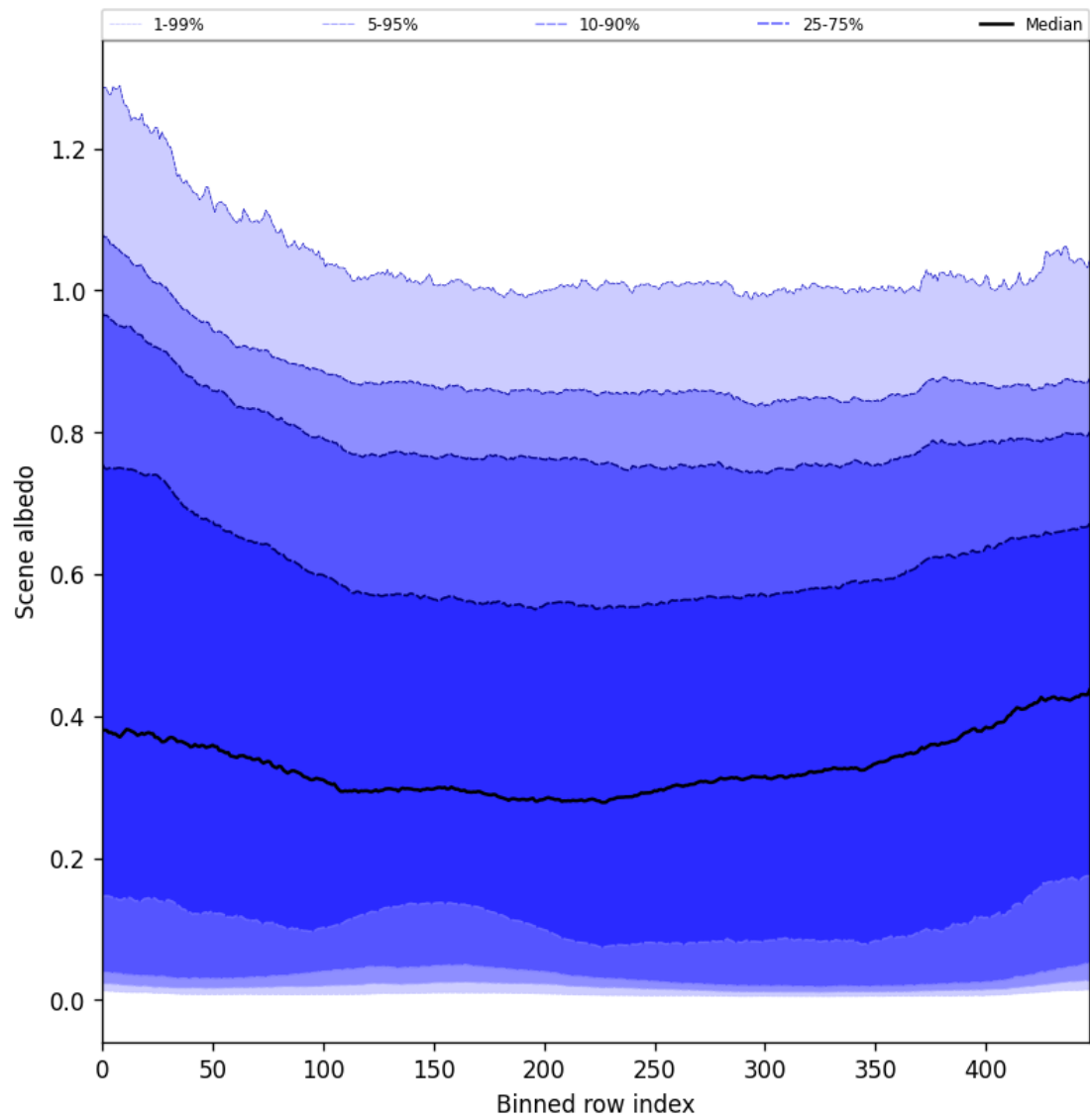
Figure 51: Along track statistics of “Scene albedo” for 2025-08-28 to 2025-08-30
