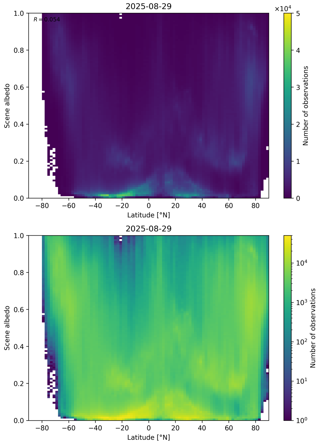
Figure 95: Scatter density plot of “Latitude” against “Scene albedo” for 2025-08-28 to 2025-08-30.
