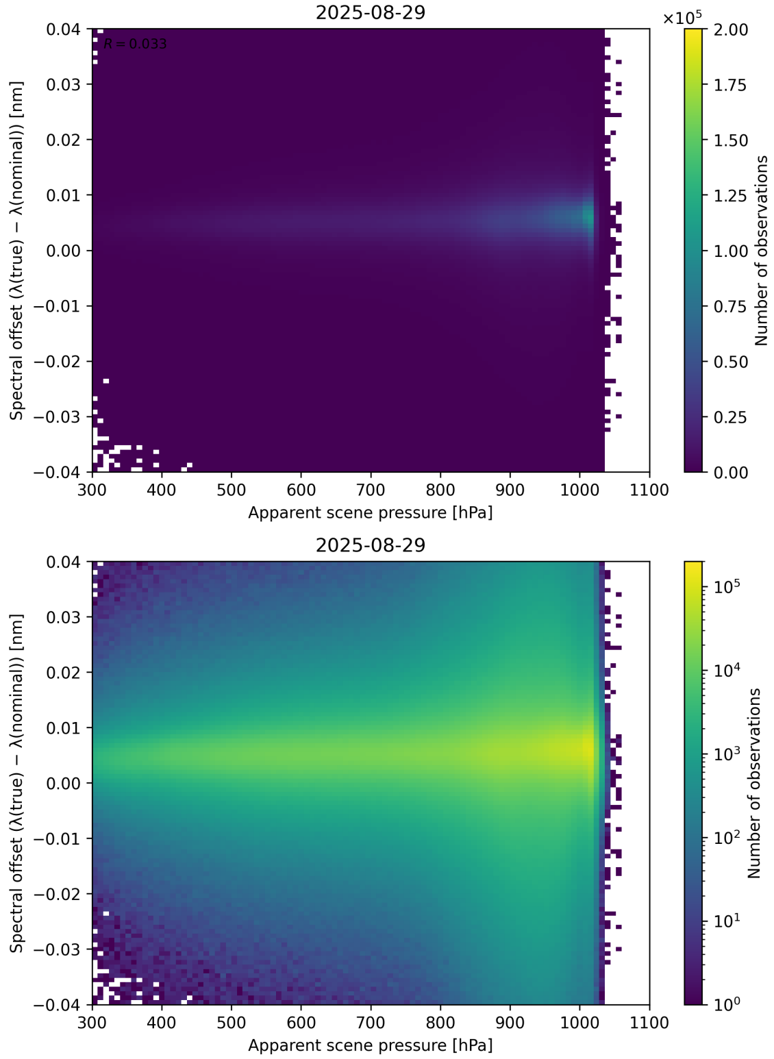
Figure 67: Scatter density plot of “Apparent scene pressure” against “Spectral offset ( \lambda_{\text{true}} - \lambda_{\text{nominal}} )” for 2025-08-28 to 2025-08-30.
