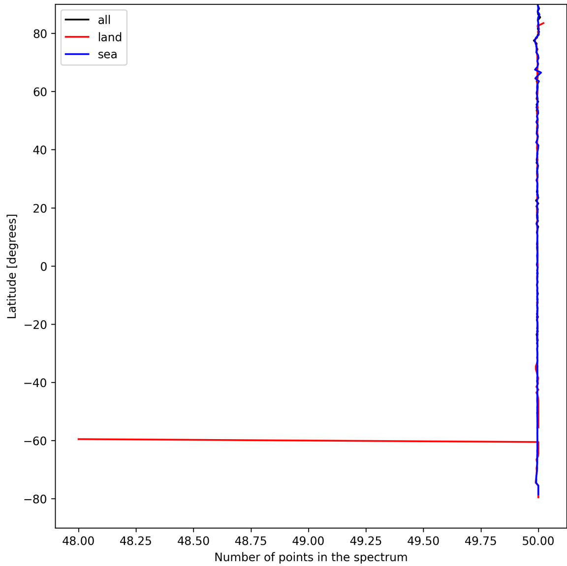
Figure 27: Zonal average of “Number of points in the spectrum” for 2025-08-28 to 2025-08-30.
