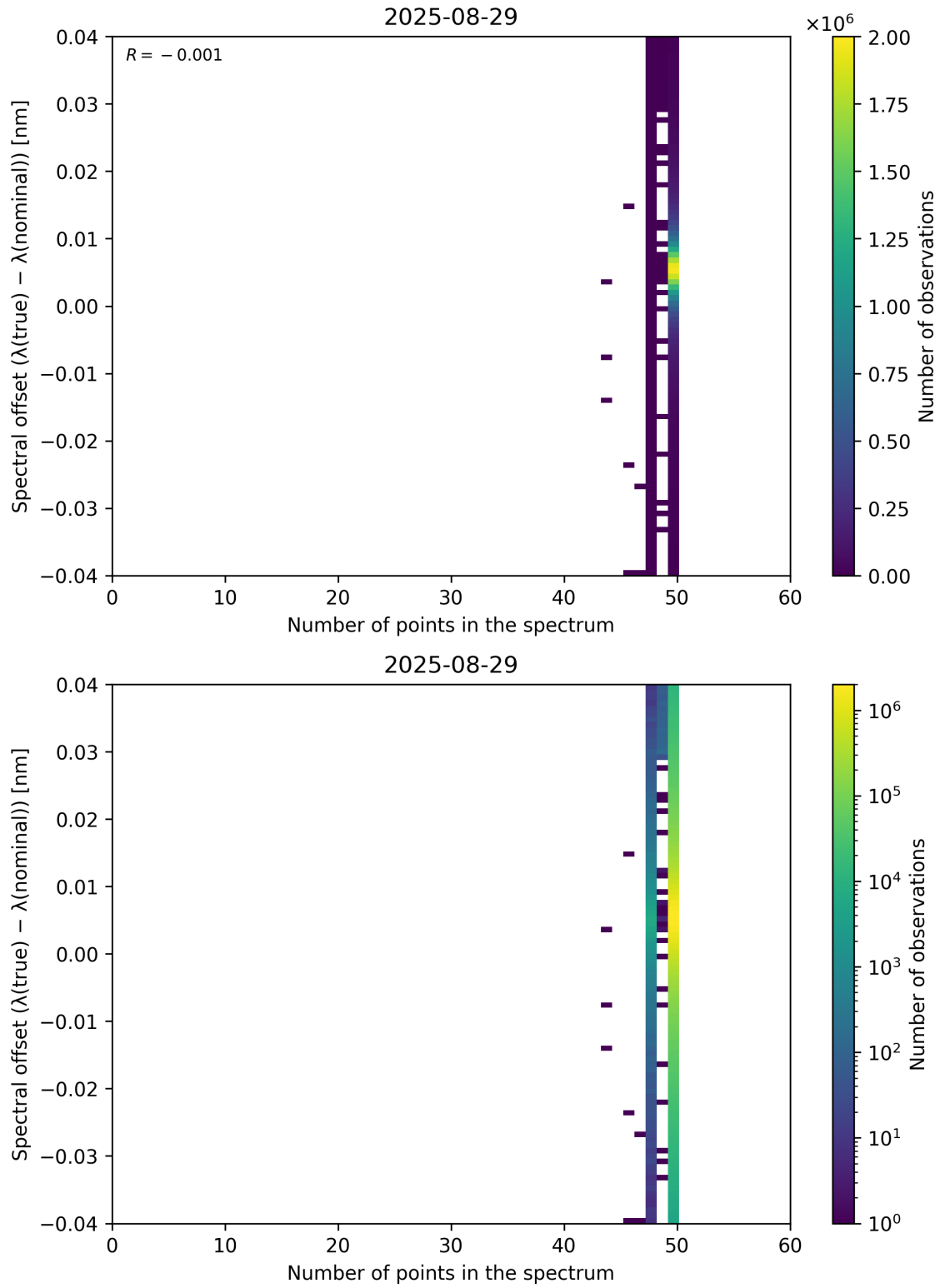
Figure 101: Scatter density plot of “Number of points in the spectrum” against “Spectral offset ( \lambda_{\text{true}} - \lambda_{\text{nominal}} )” for 2025-08-28 to 2025-08-30.
