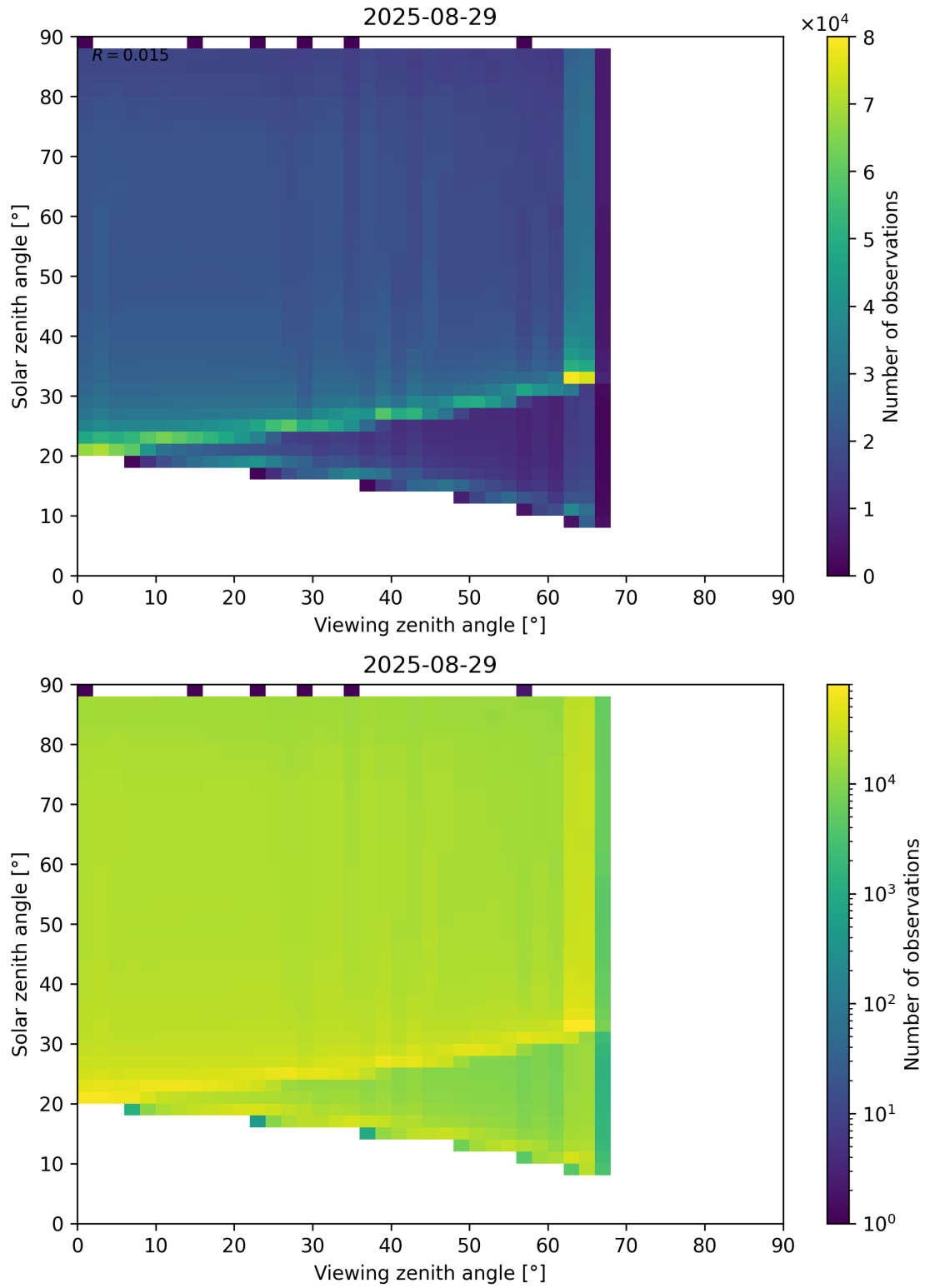
Figure 127: Scatter density plot of “Viewing zenith angle” against “Solar zenith angle” for 2025-08-28 to 2025-08-30.
