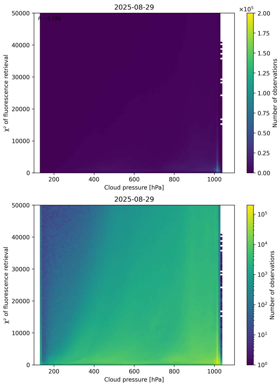
Figure 78: Scatter density plot of “Cloud pressure” against “ \chi^2 of fluorescence retrieval” for 2025-08-28 to 2025-08-30.
