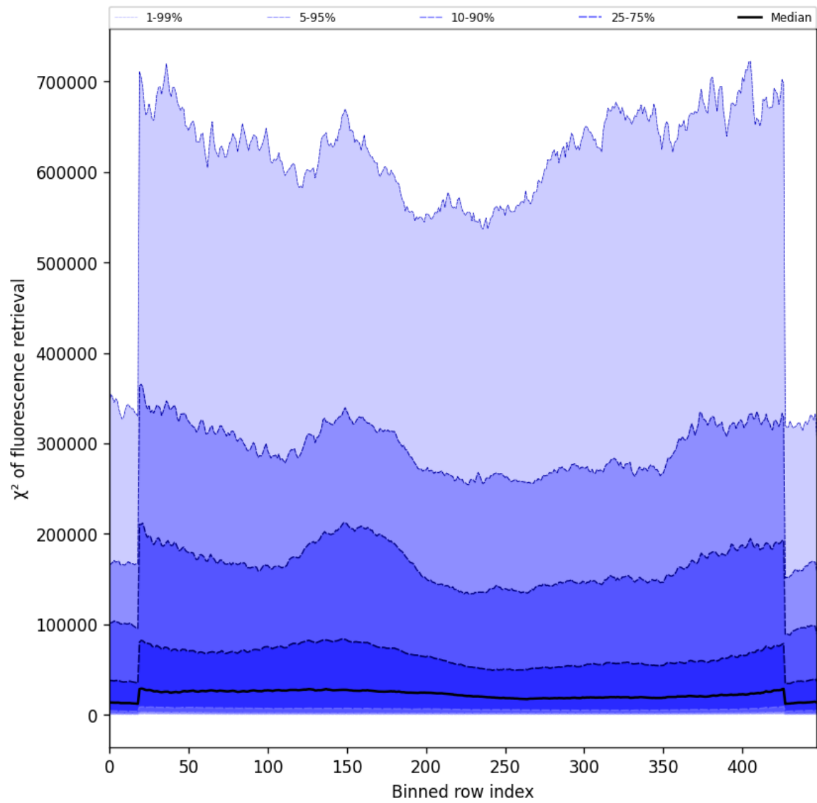
Figure 59: Along track statistics of “ \chi^2 of fluorescence retrieval” for 2025-08-28 to 2025-08-30
