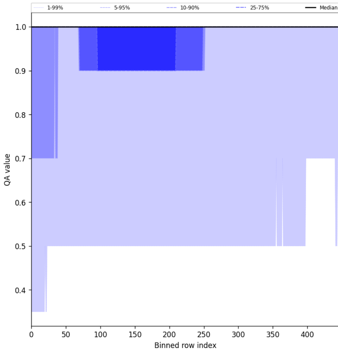
Figure 46: Along track statistics of “QA value” for 2025-08-28 to 2025-08-30
