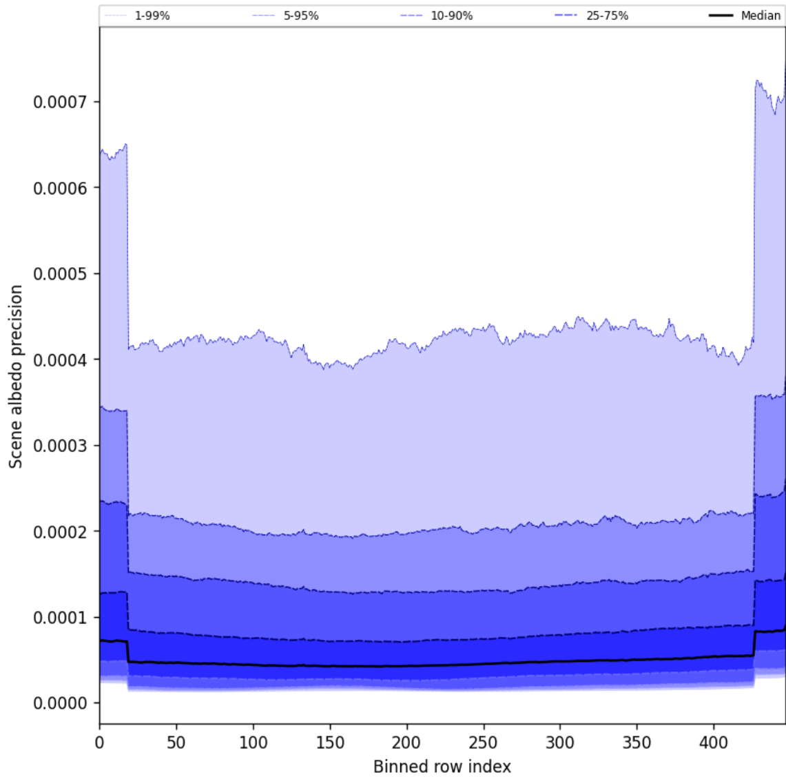
Figure 52: Along track statistics of “Scene albedo precision” for 2025-08-28 to 2025-08-30
