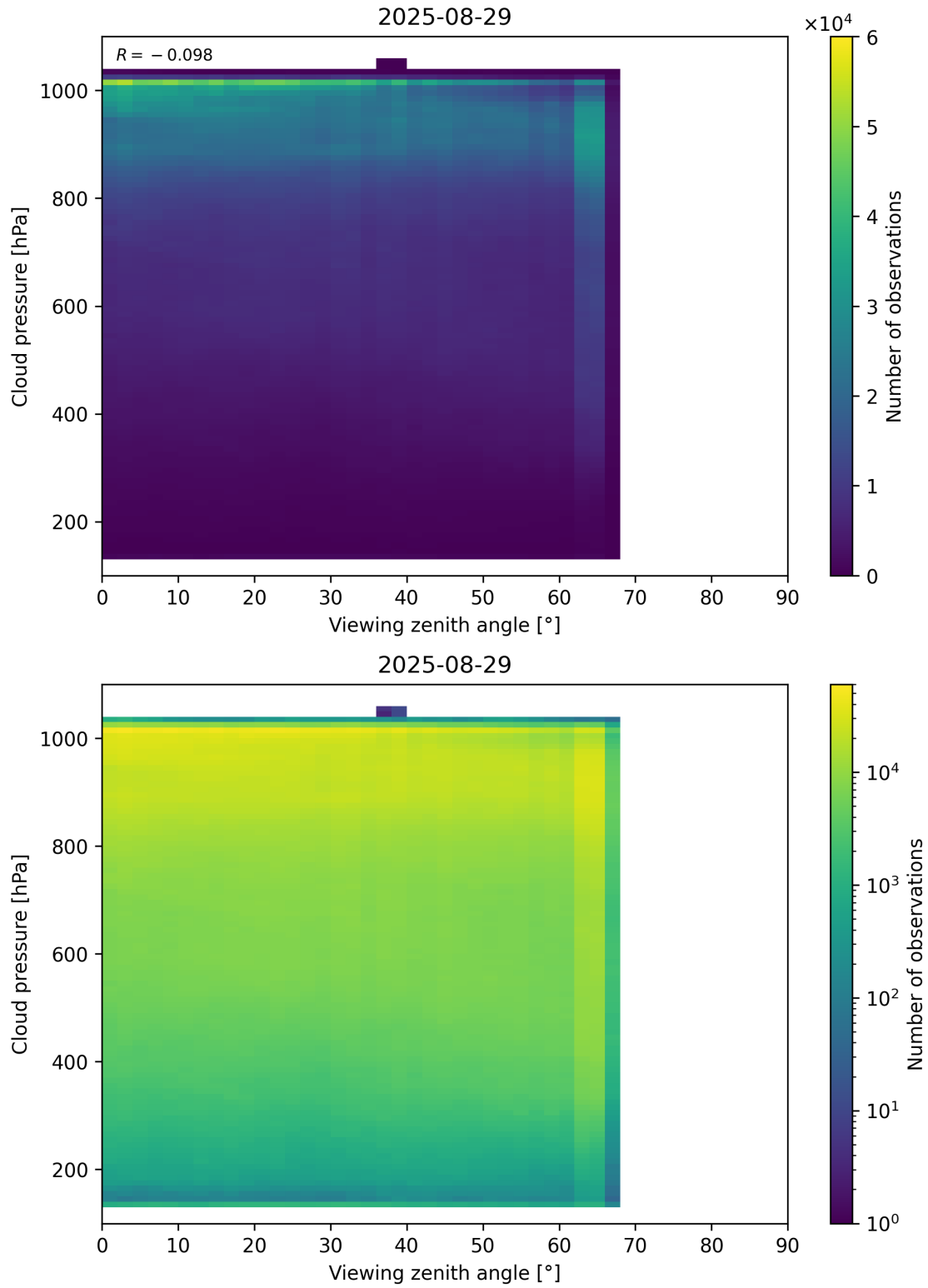
Figure 121: Scatter density plot of “Viewing zenith angle” against “Cloud pressure” for 2025-08-28 to 2025-08-30.
