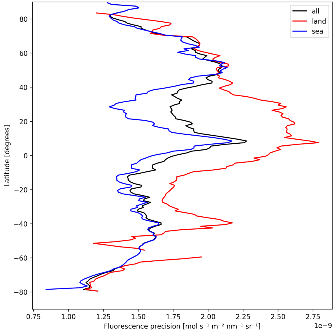
Figure 24: Zonal average of “Fluorescence precision” for 2025-08-28 to 2025-08-30.
