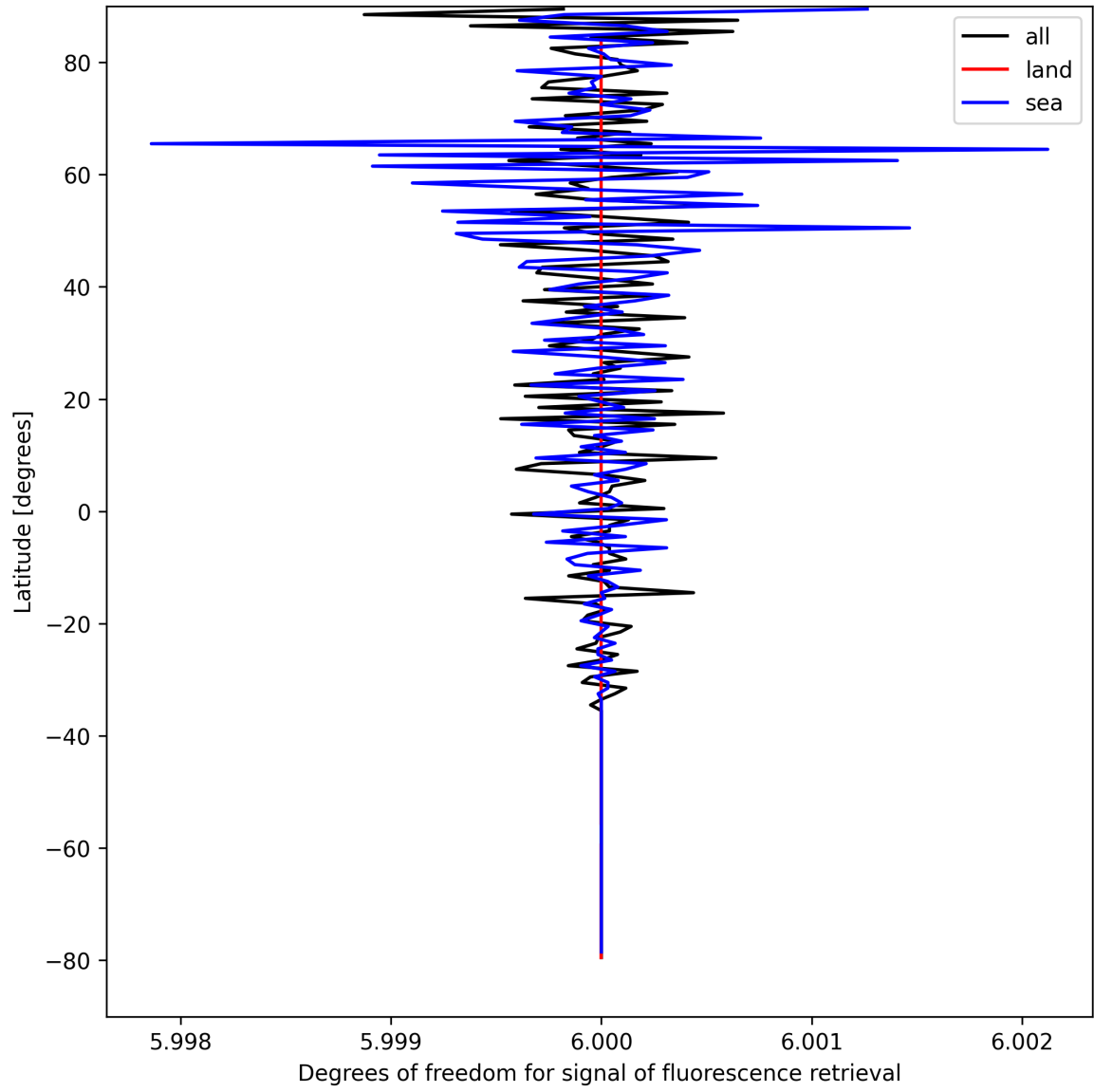
Figure 26: Zonal average of “Degrees of freedom for signal of fluorescence retrieval” for 2025-08-28 to 2025-08-30.
