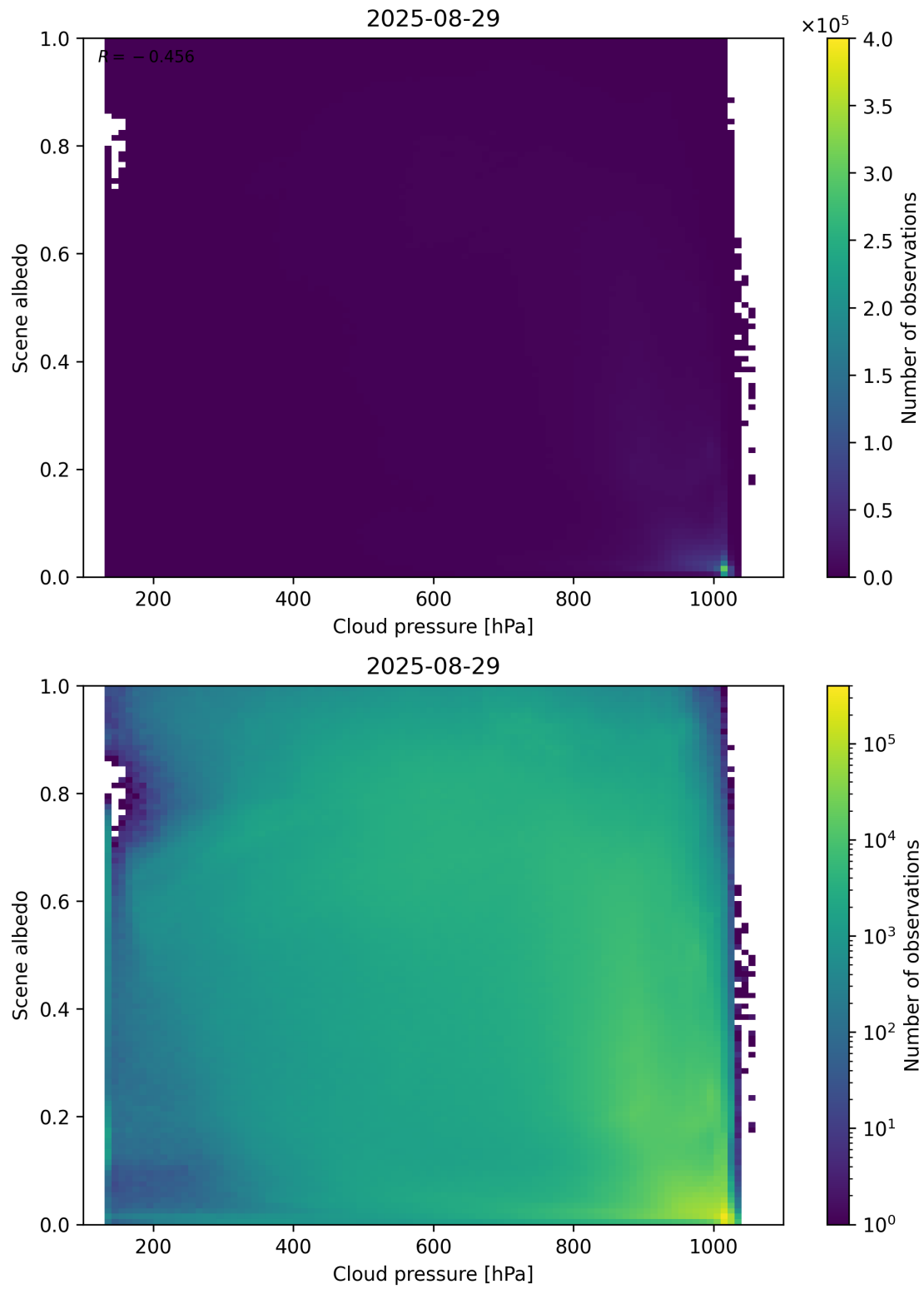
Figure 83: Scatter density plot of “Cloud pressure” against “Scene albedo” for 2025-08-28 to 2025-08-30.
