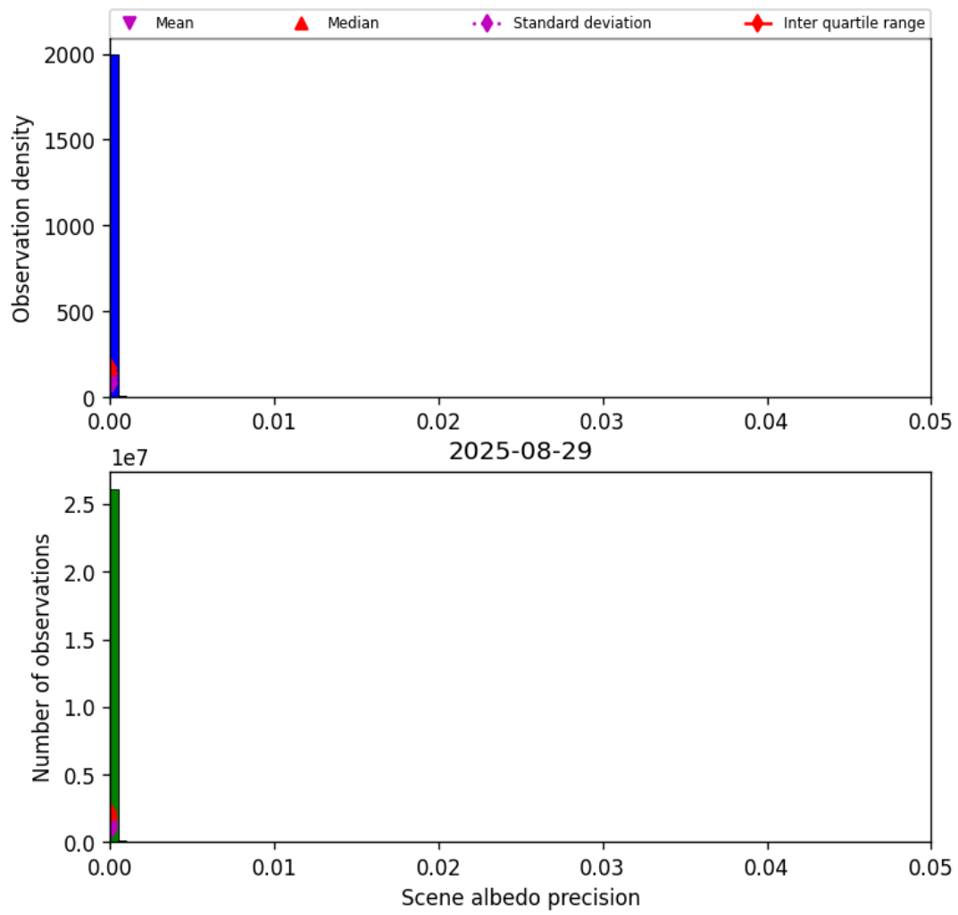
Figure 35: Histogram of “Scene albedo precision” for 2025-08-28 to 2025-08-30
