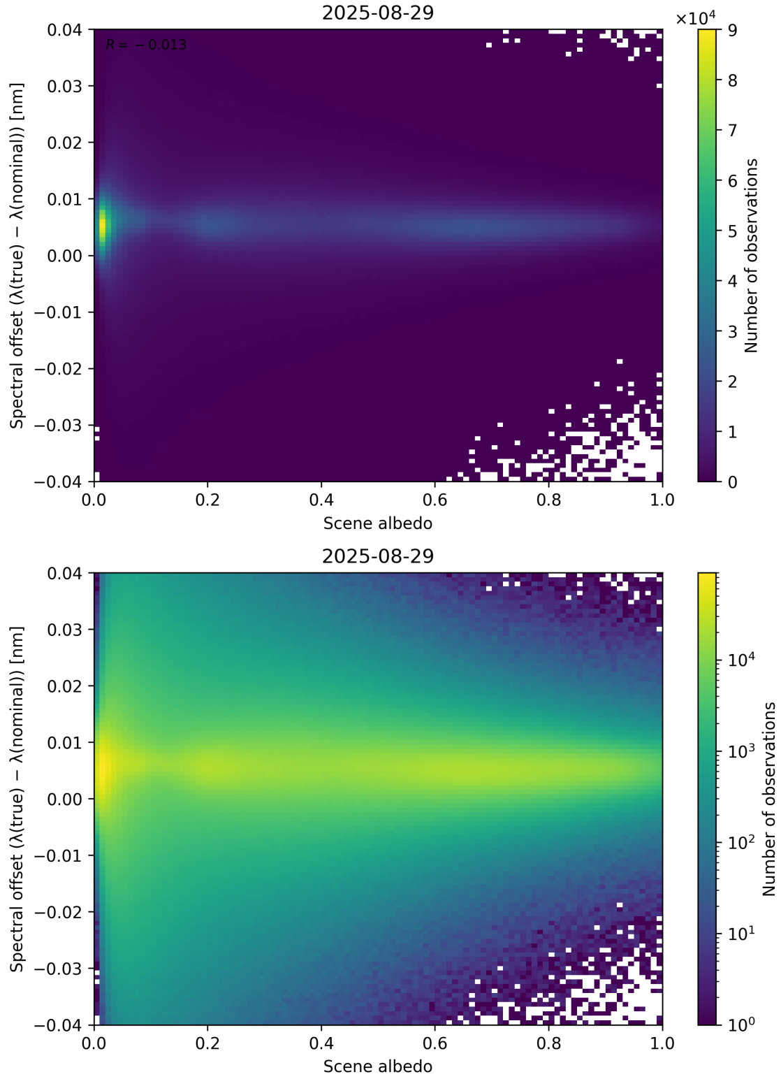
Figure 107: Scatter density plot of “Scene albedo” against “Spectral offset ( \lambda_{\text{true}} - \lambda_{\text{nominal}} )” for 2025-08-28 to 2025-08-30.
