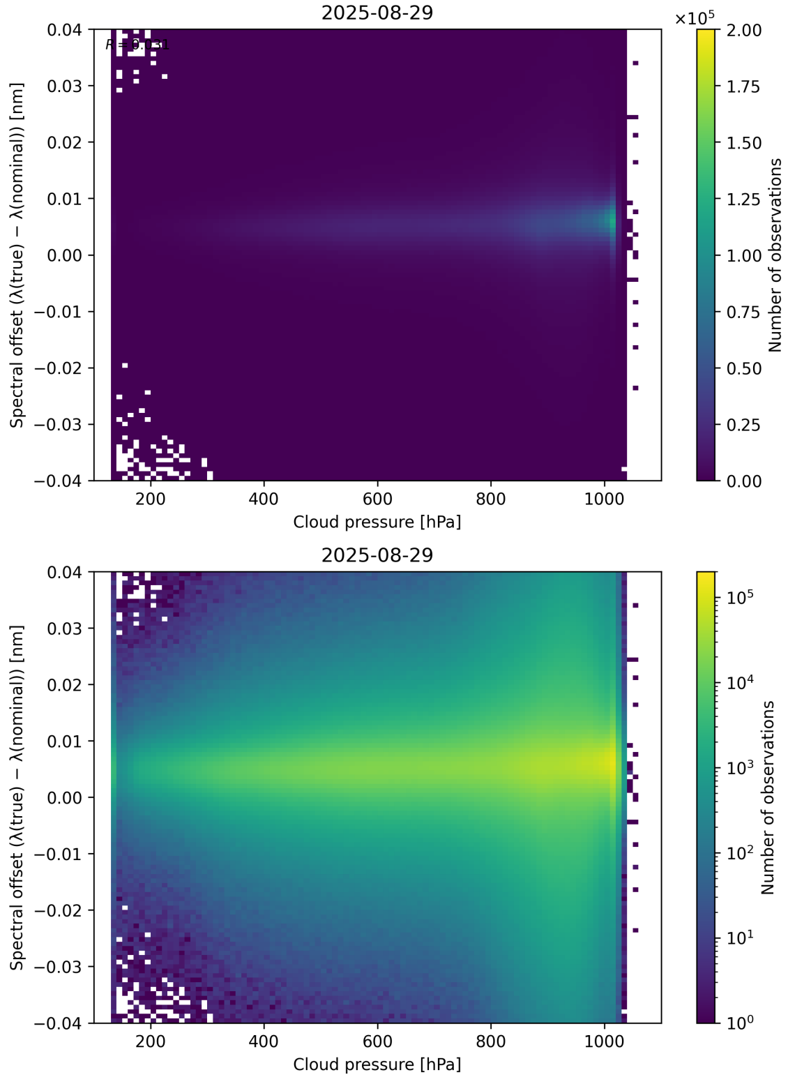
Figure 84: Scatter density plot of “Cloud pressure” against “Spectral offset ( \lambda_{\text{true}} - \lambda_{\text{nominal}} )” for 2025-08-28 to 2025-08-30.
