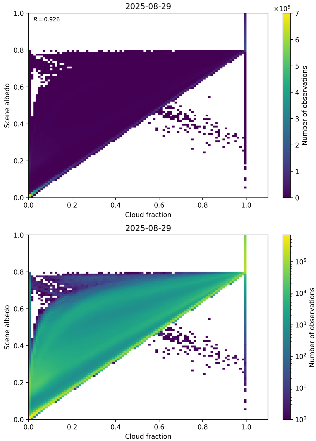
Figure 75: Scatter density plot of “Cloud fraction” against “Scene albedo” for 2025-08-28 to 2025-08-30.
