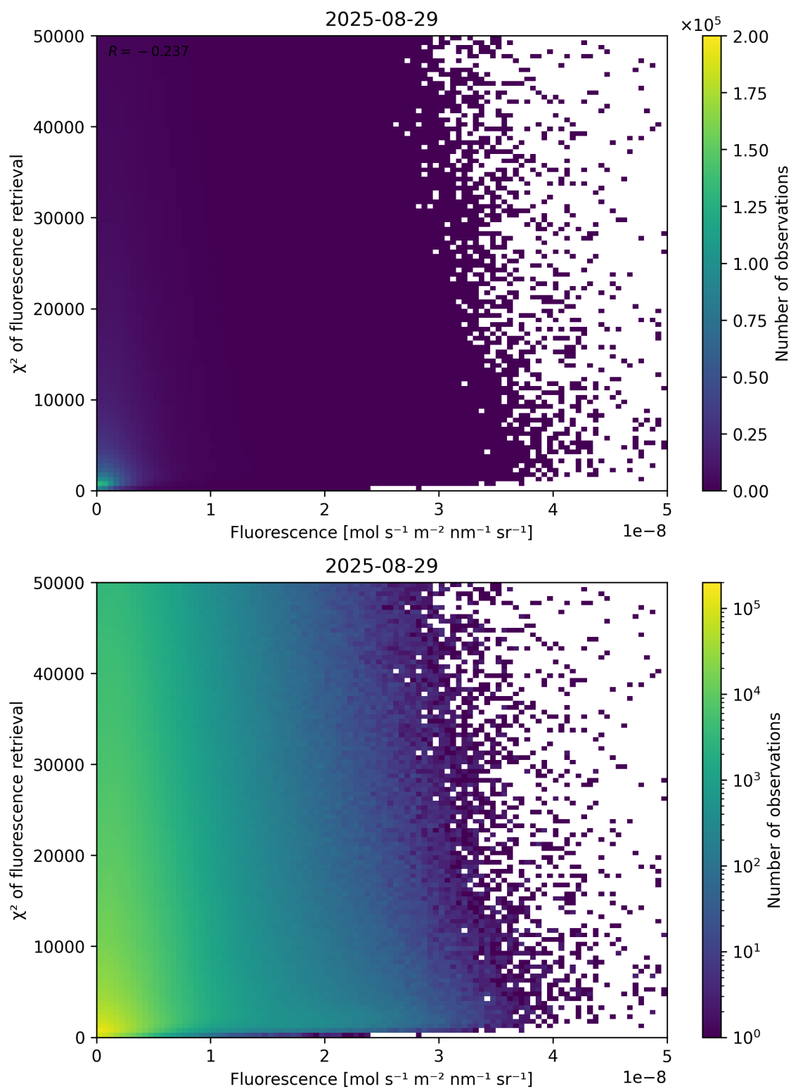
Figure 85: Scatter density plot of “Fluorescence” against “ \chi^2 of fluorescence retrieval” for 2025-08-28 to 2025-08-30.
