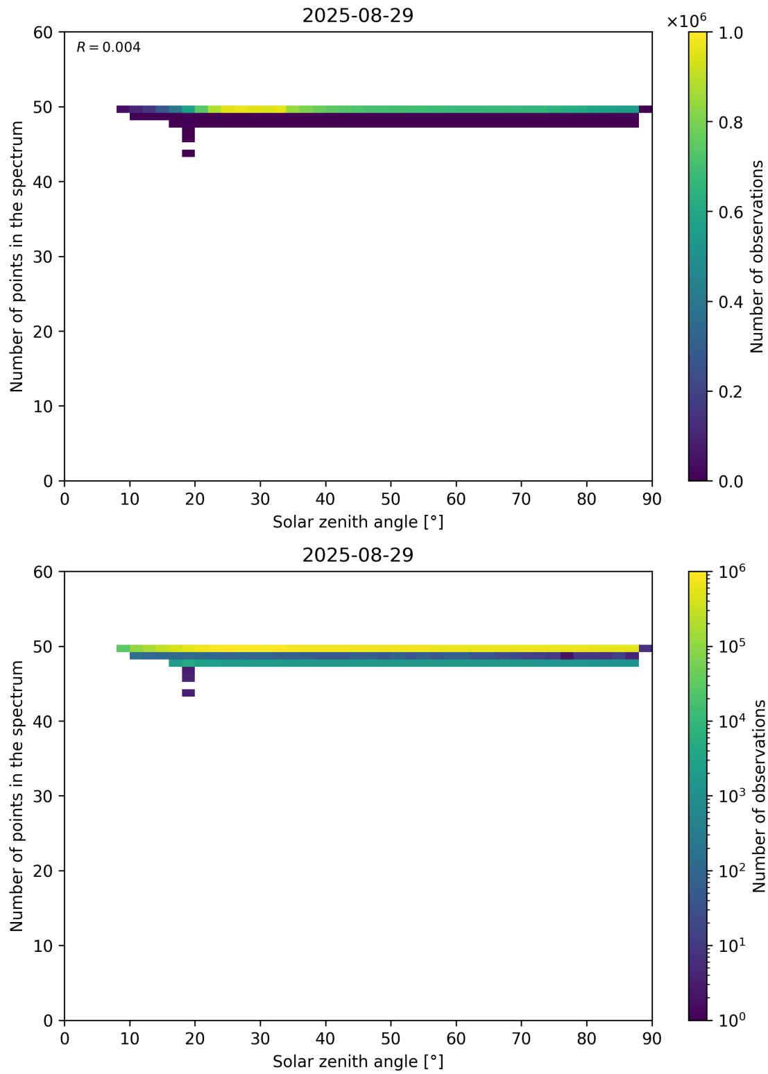
Figure 115: Scatter density plot of “Solar zenith angle” against “Number of points in the spectrum” for 2025-08-28 to 2025-08-30.
