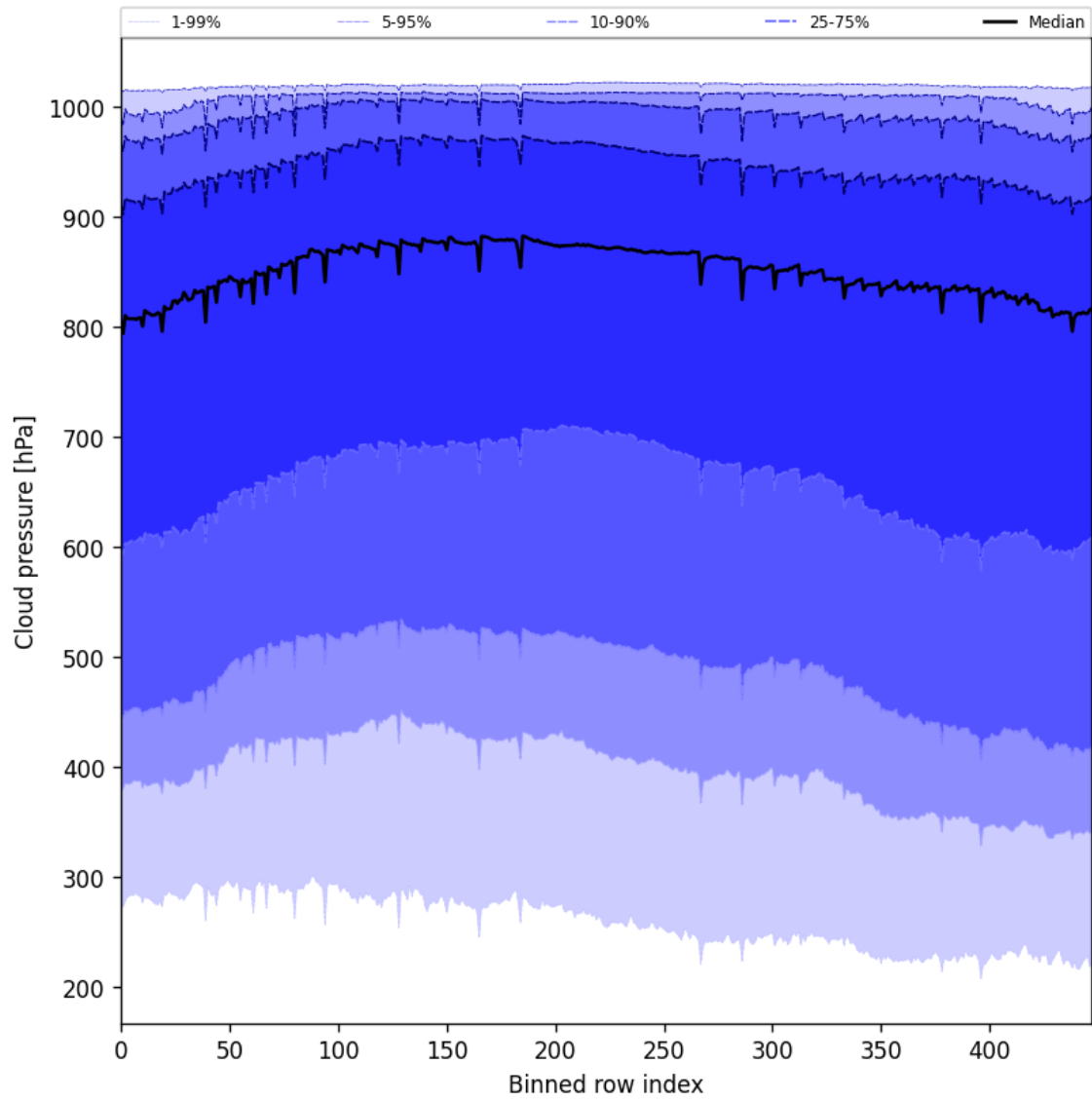
Figure 47: Along track statistics of “Cloud pressure” for 2025-08-28 to 2025-08-30
