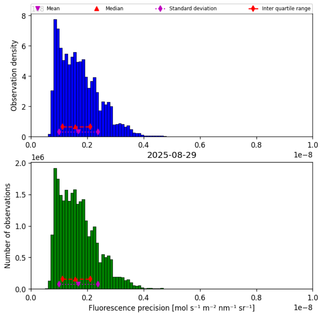
Figure 41: Histogram of “Fluorescence precision” for 2025-08-28 to 2025-08-30
