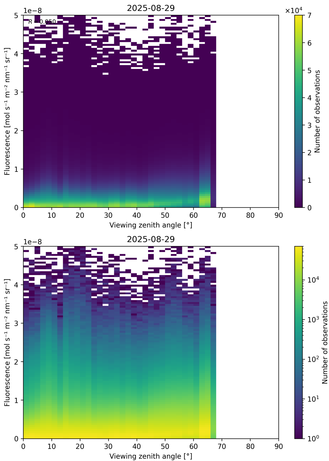
Figure 122: Scatter density plot of “Viewing zenith angle” against “Fluorescence” for 2025-08-28 to 2025-08-30.
