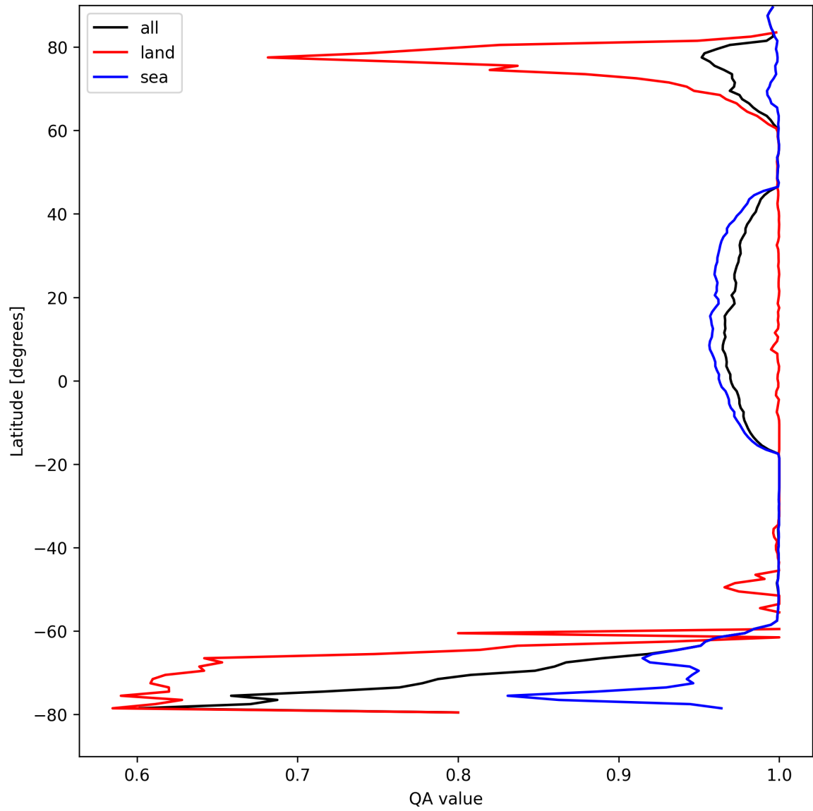
Figure 12: Zonal average of "QA value" for 2025-08-28 to 2025-08-30.
