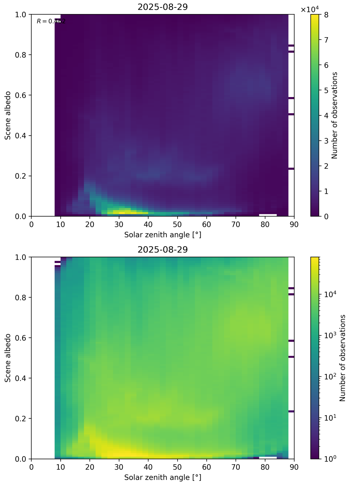
Figure 116: Scatter density plot of “Solar zenith angle” against “Scene albedo” for 2025-08-28 to 2025-08-30.
