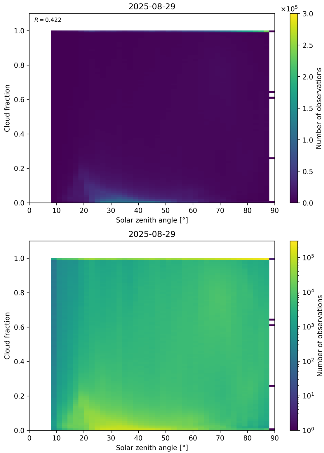
Figure 110: Scatter density plot of “Solar zenith angle” against “Cloud fraction” for 2025-08-28 to 2025-08-30.
