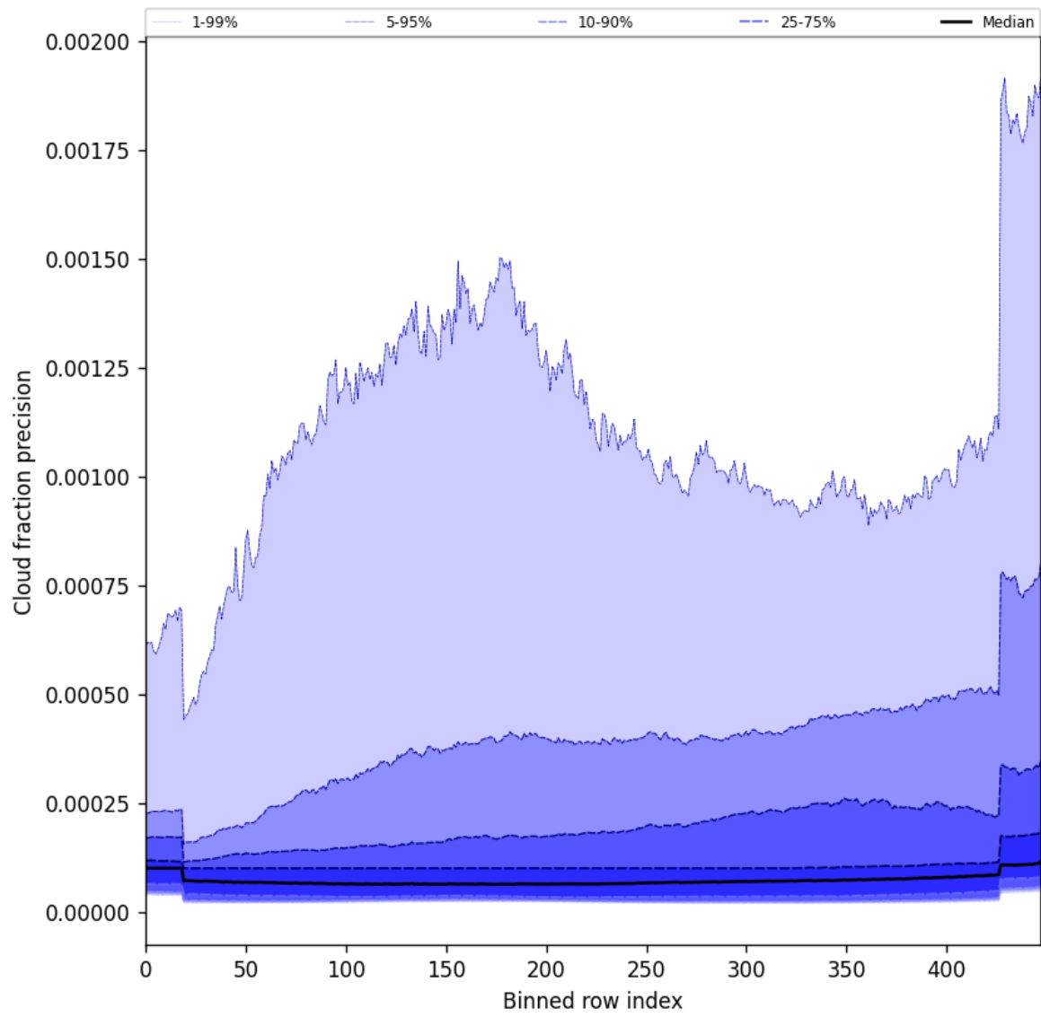
Figure 50: Along track statistics of “Cloud fraction precision” for 2025-08-28 to 2025-08-30
