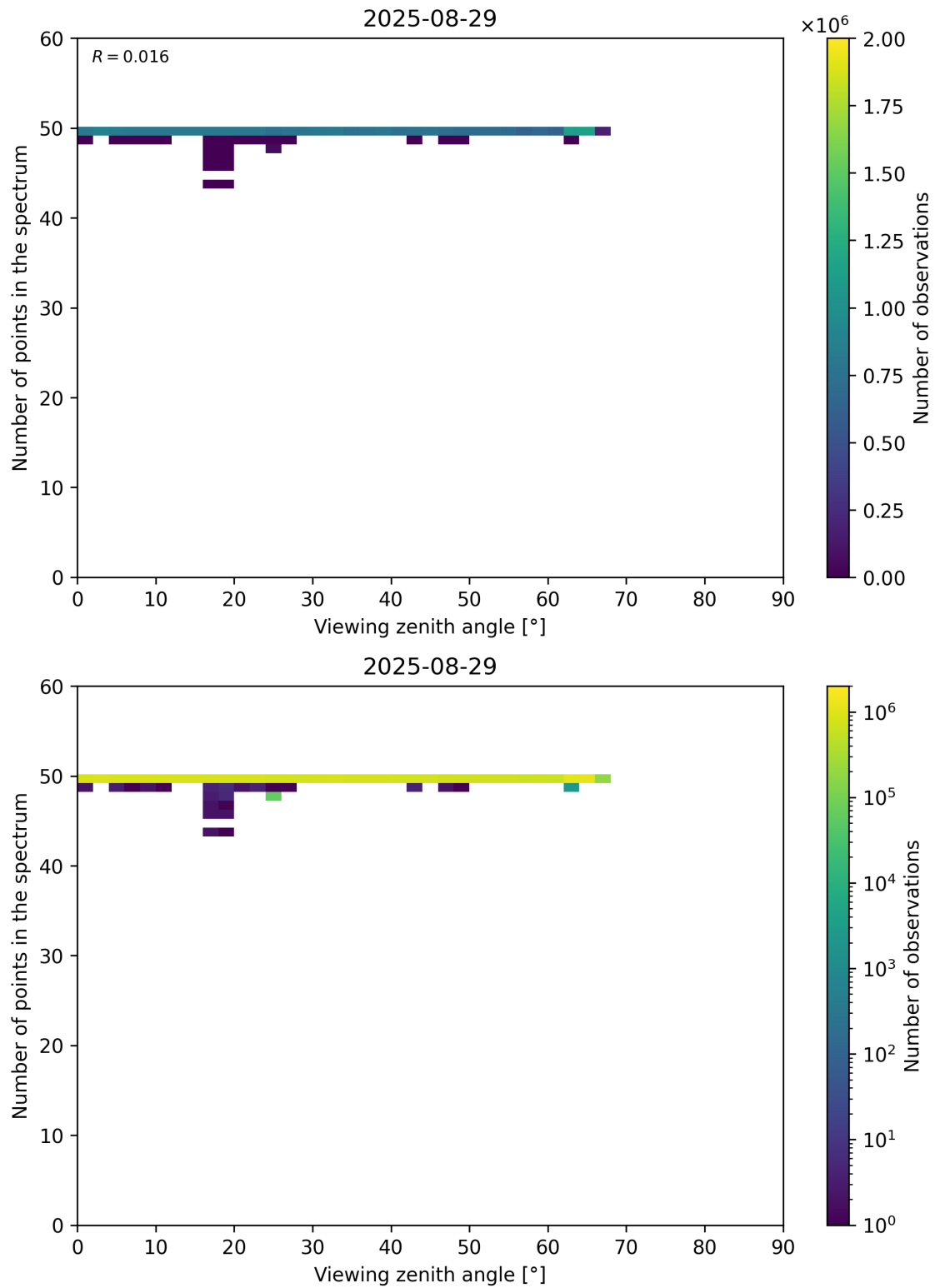
Figure 125: Scatter density plot of “Viewing zenith angle” against “Number of points in the spectrum” for 2025-08-28 to 2025-08-30.
