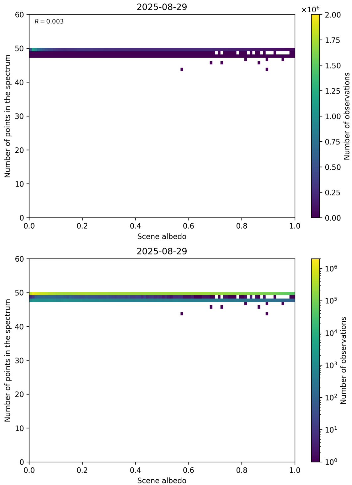
Figure 106: Scatter density plot of “Scene albedo” against “Number of points in the spectrum” for 2025-08-28 to 2025-08-30.
