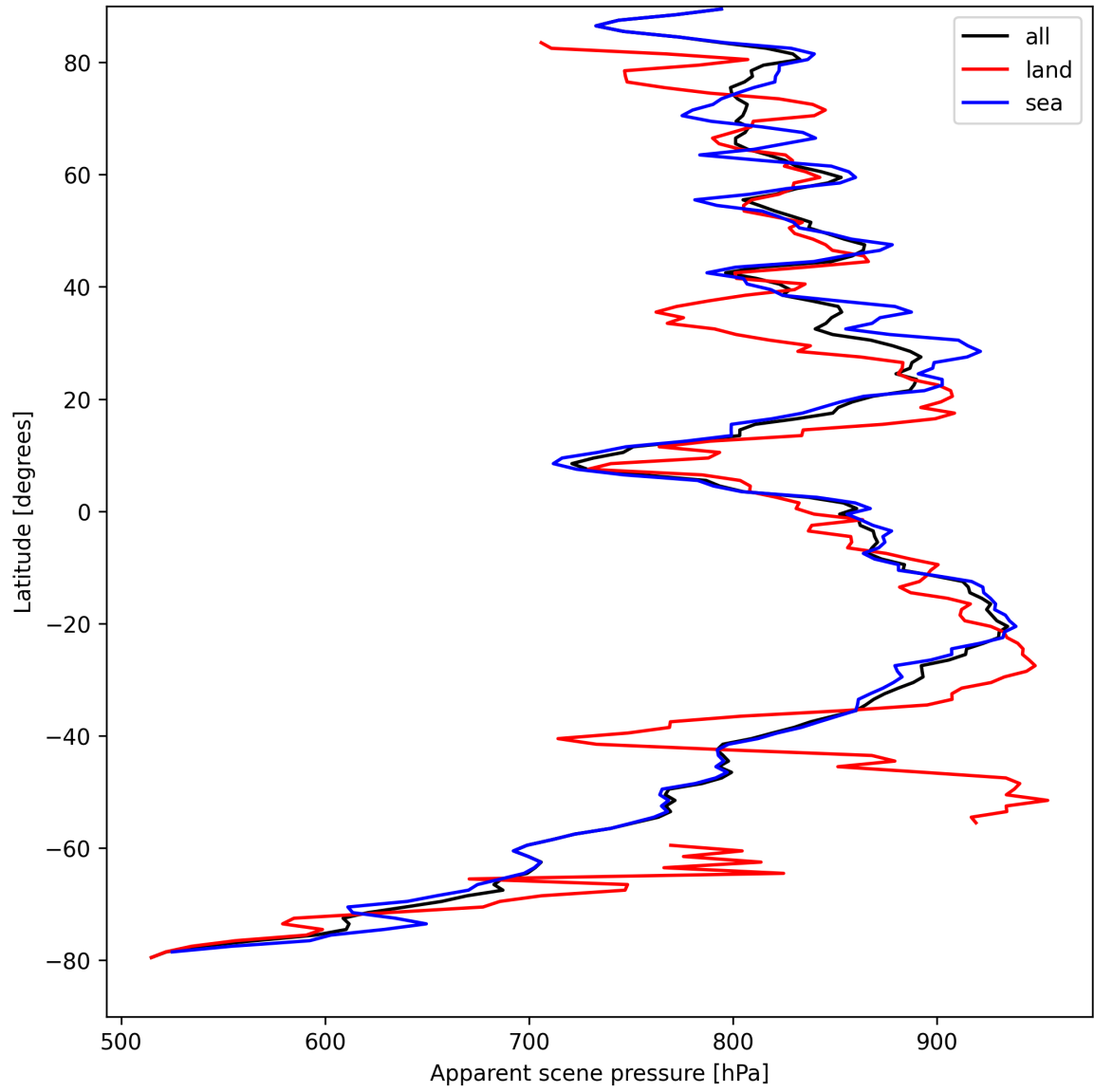
Figure 19: Zonal average of “Apparent scene pressure” for 2025-08-28 to 2025-08-30.
