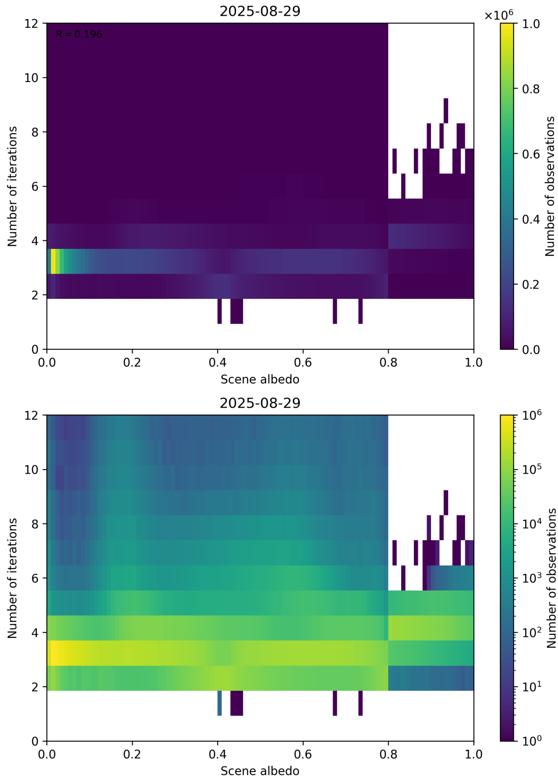
Figure 105: Scatter density plot of “Scene albedo” against “Number of iterations” for 2025-08-28 to 2025-08-30.
