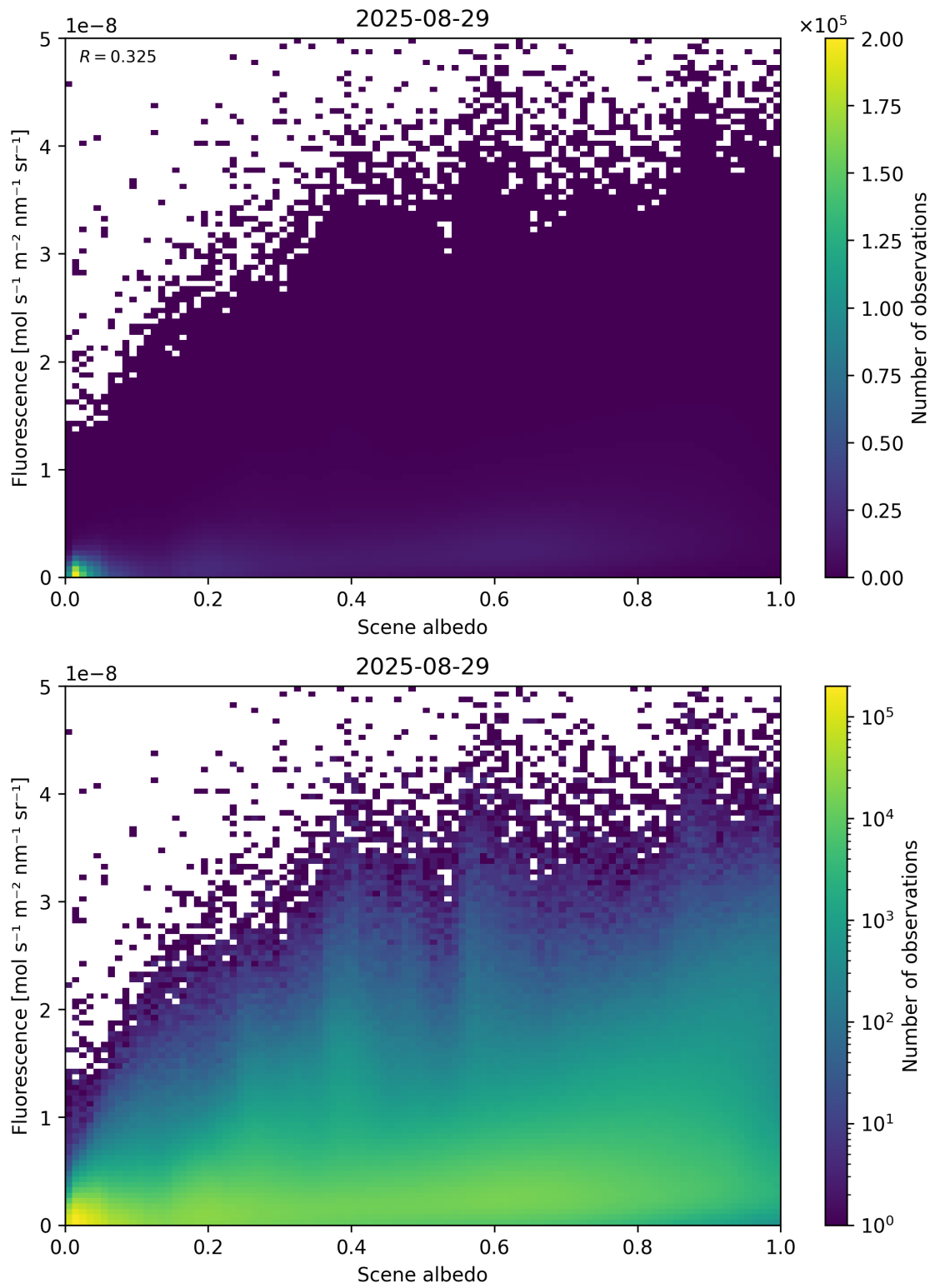
Figure 104: Scatter density plot of “Scene albedo” against “Fluorescence” for 2025-08-28 to 2025-08-30.
