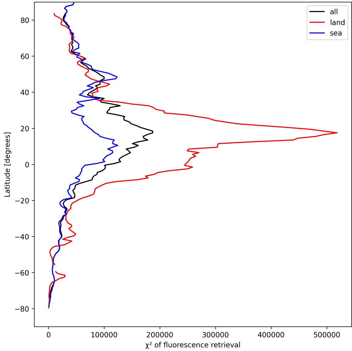
Figure 25: Zonal average of “ \chi^2 of fluorescence retrieval” for 2025-08-28 to 2025-08-30.
