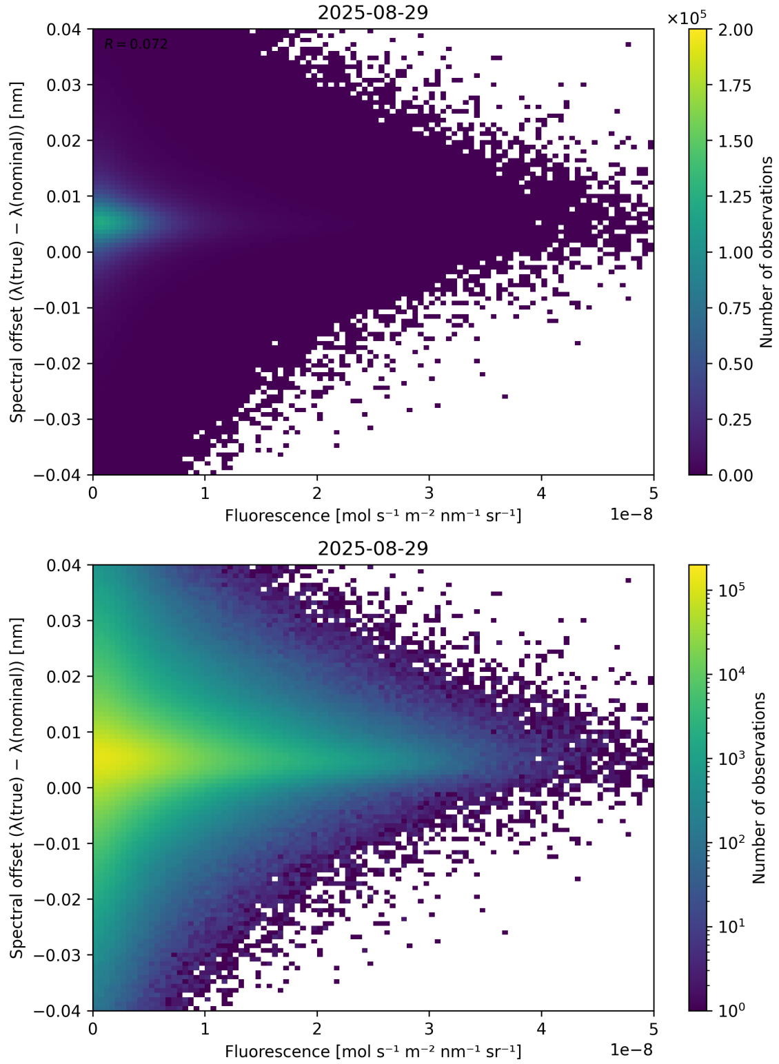
Figure 87: Scatter density plot of “Fluorescence” against “Spectral offset ( \lambda_{\text{true}} - \lambda_{\text{nominal}} )” for 2025-08-28 to 2025-08-30.
