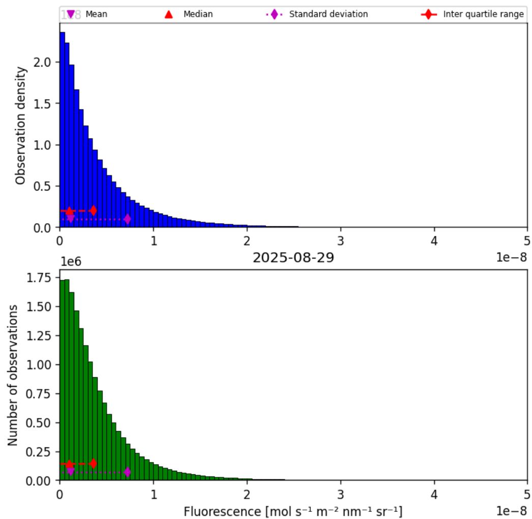
Figure 40: Histogram of “Fluorescence” for 2025-08-28 to 2025-08-30
