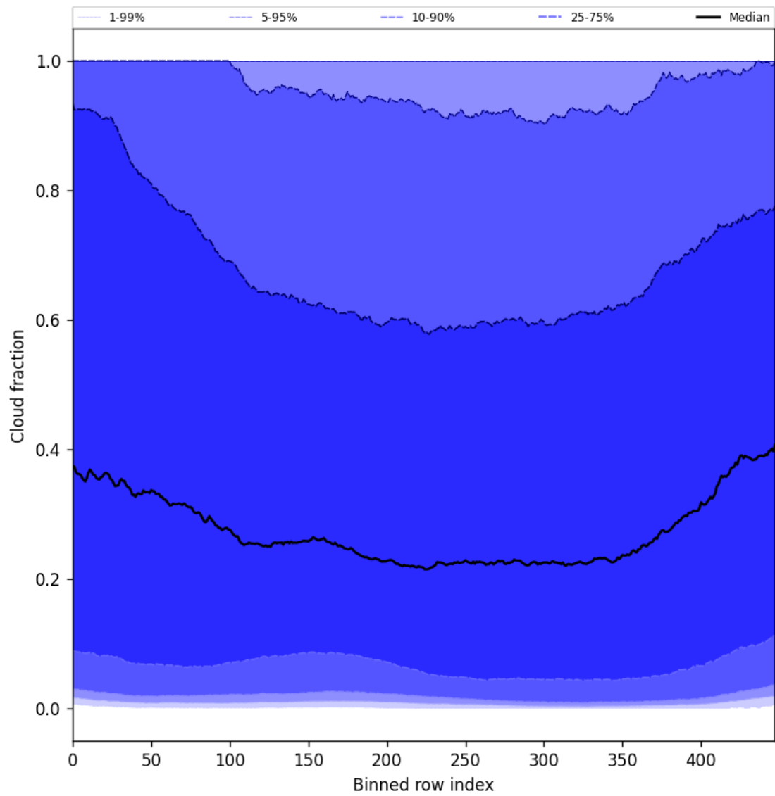
Figure 49: Along track statistics of “Cloud fraction” for 2025-08-28 to 2025-08-30
