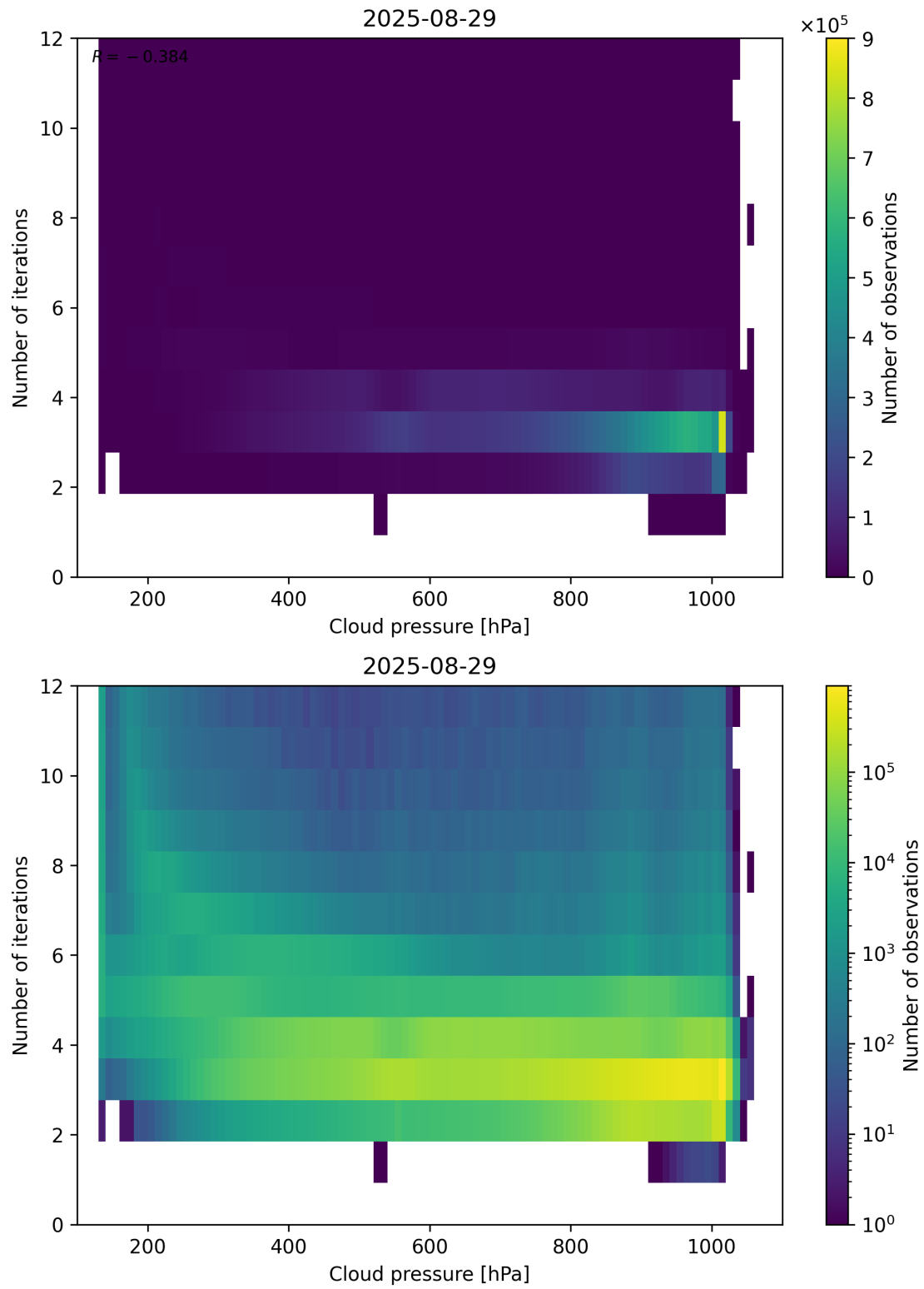
Figure 81: Scatter density plot of “Cloud pressure” against “Number of iterations” for 2025-08-28 to 2025-08-30.
