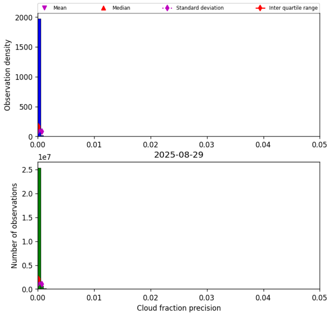
Figure 33: Histogram of “Cloud fraction precision” for 2025-08-28 to 2025-08-30
