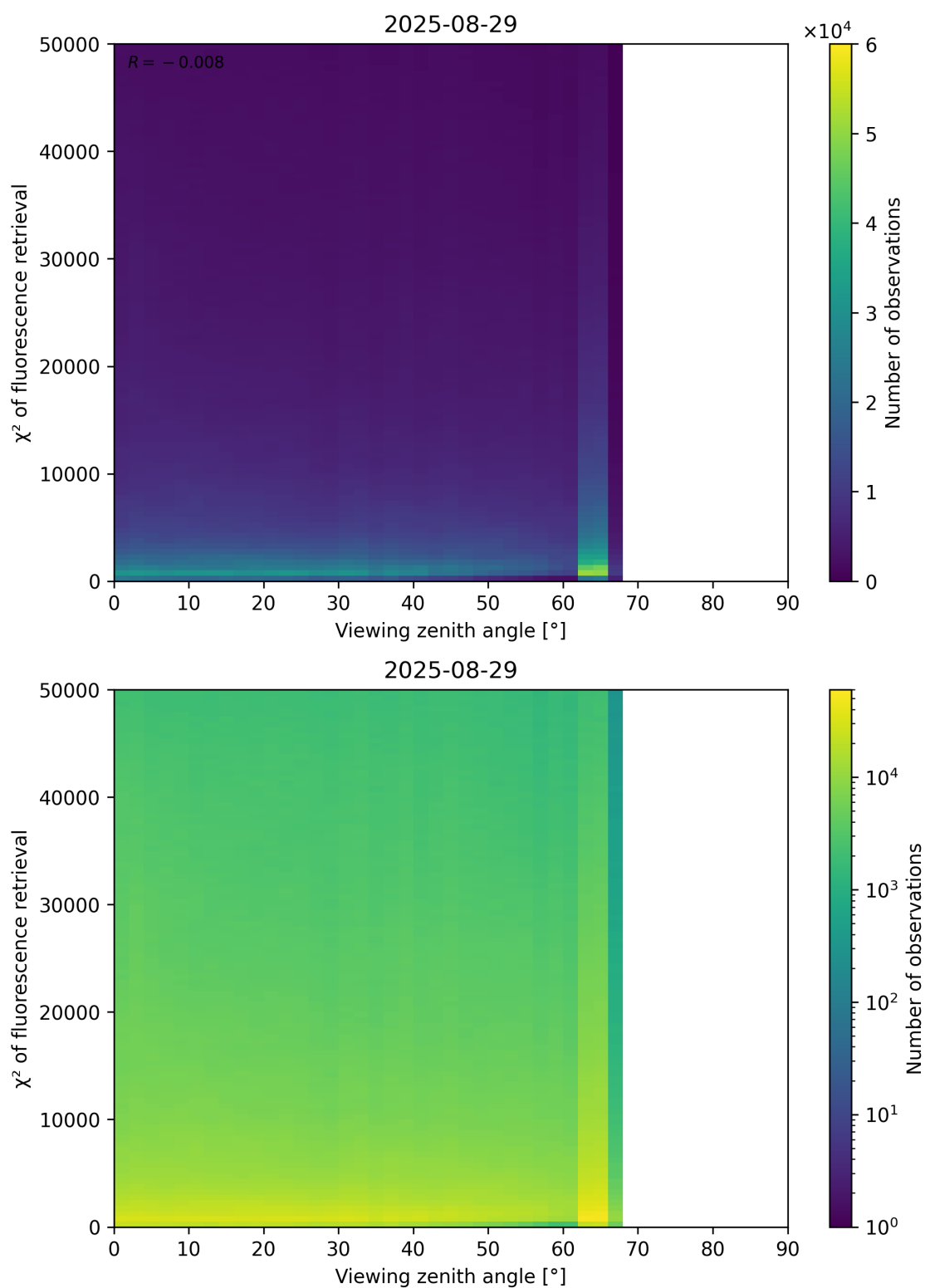
Figure 119: Scatter density plot of “Viewing zenith angle” against “ \chi^2 of fluorescence retrieval” for 2025-08-28 to 2025-08-30.
