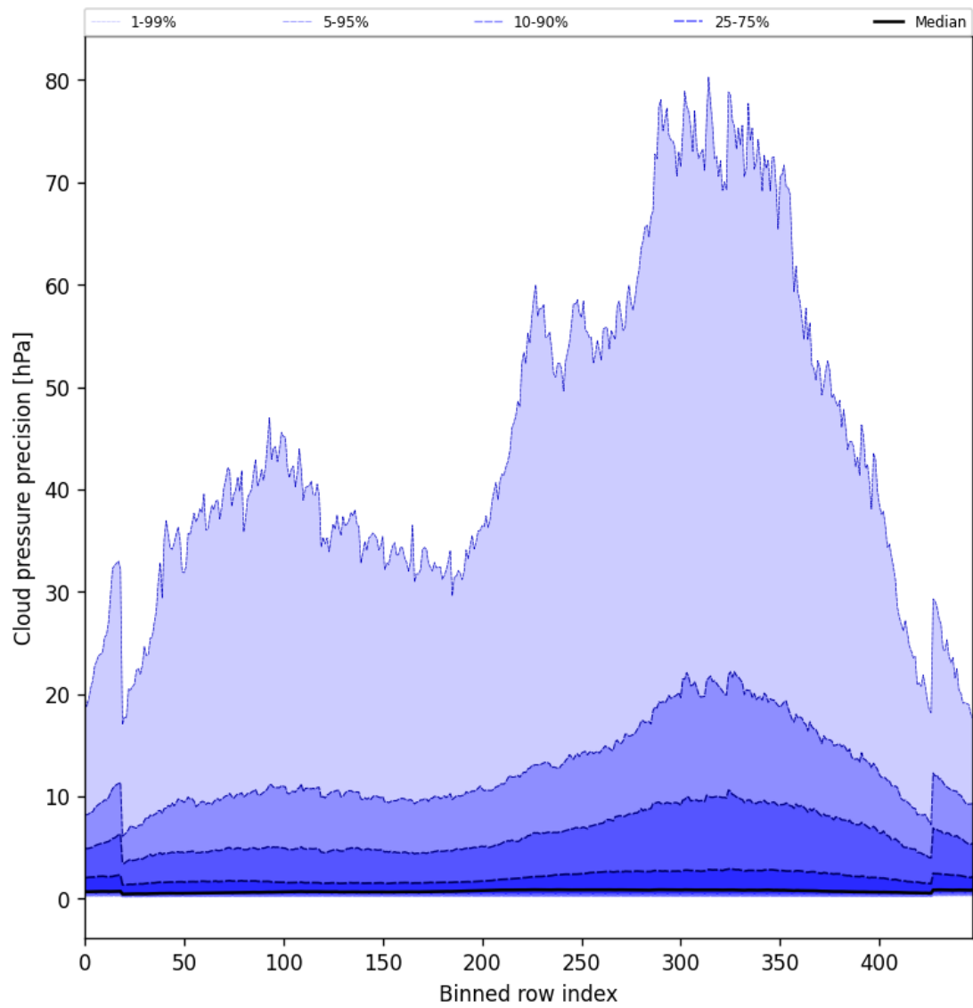
Figure 48: Along track statistics of “Cloud pressure precision” for 2025-08-28 to 2025-08-30
