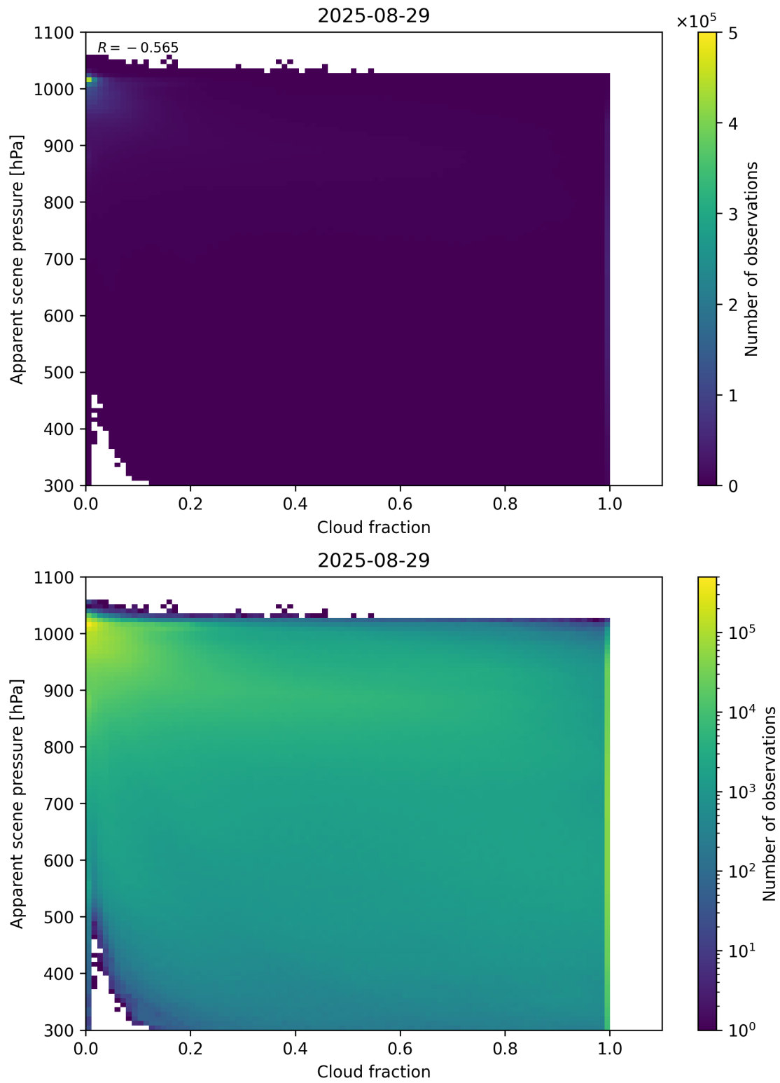
Figure 70: Scatter density plot of “Cloud fraction” against “Apparent scene pressure” for 2025-08-28 to 2025-08-30.
