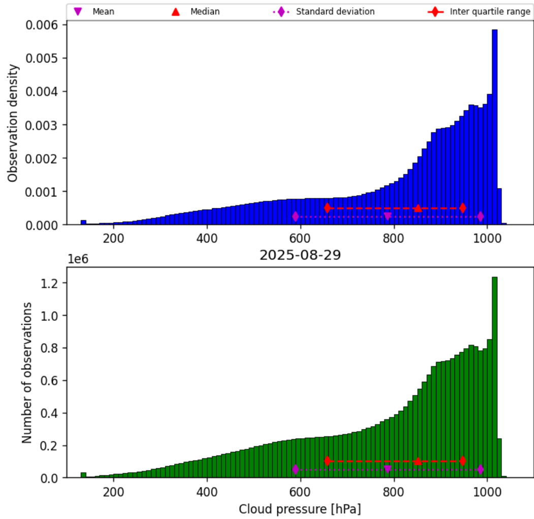
Figure 30: Histogram of “Cloud pressure” for 2025-08-28 to 2025-08-30
