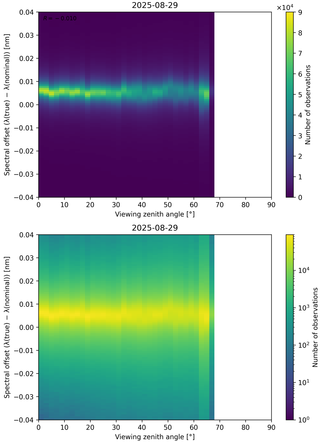
Figure 128: Scatter density plot of “Viewing zenith angle” against “Spectral offset ( \lambda_{\text{true}} - \lambda_{\text{nominal}} )” for 2025-08-28 to 2025-08-30.
