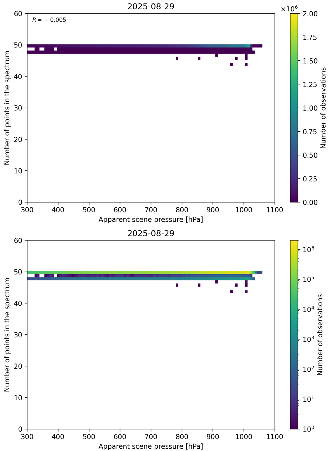
Figure 66: Scatter density plot of “Apparent scene pressure” against “Number of points in the spectrum” for 2025-08-28 to 2025-08-30.
