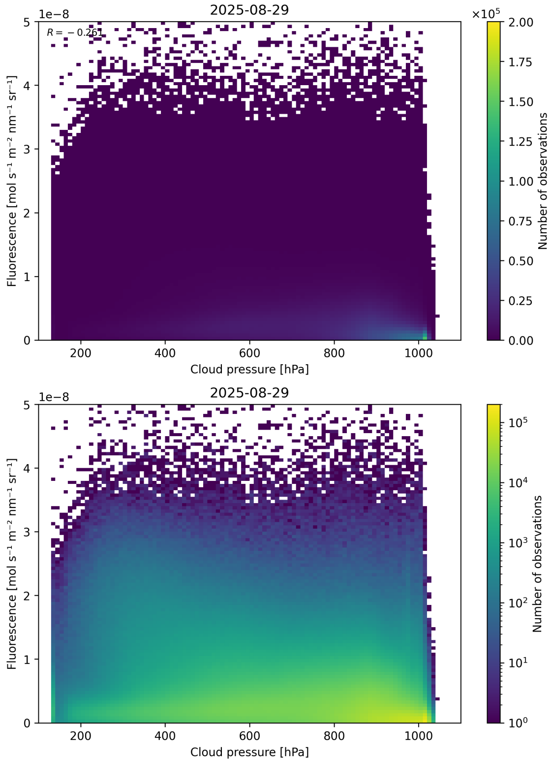
Figure 80: Scatter density plot of “Cloud pressure” against “Fluorescence” for 2025-08-28 to 2025-08-30.
