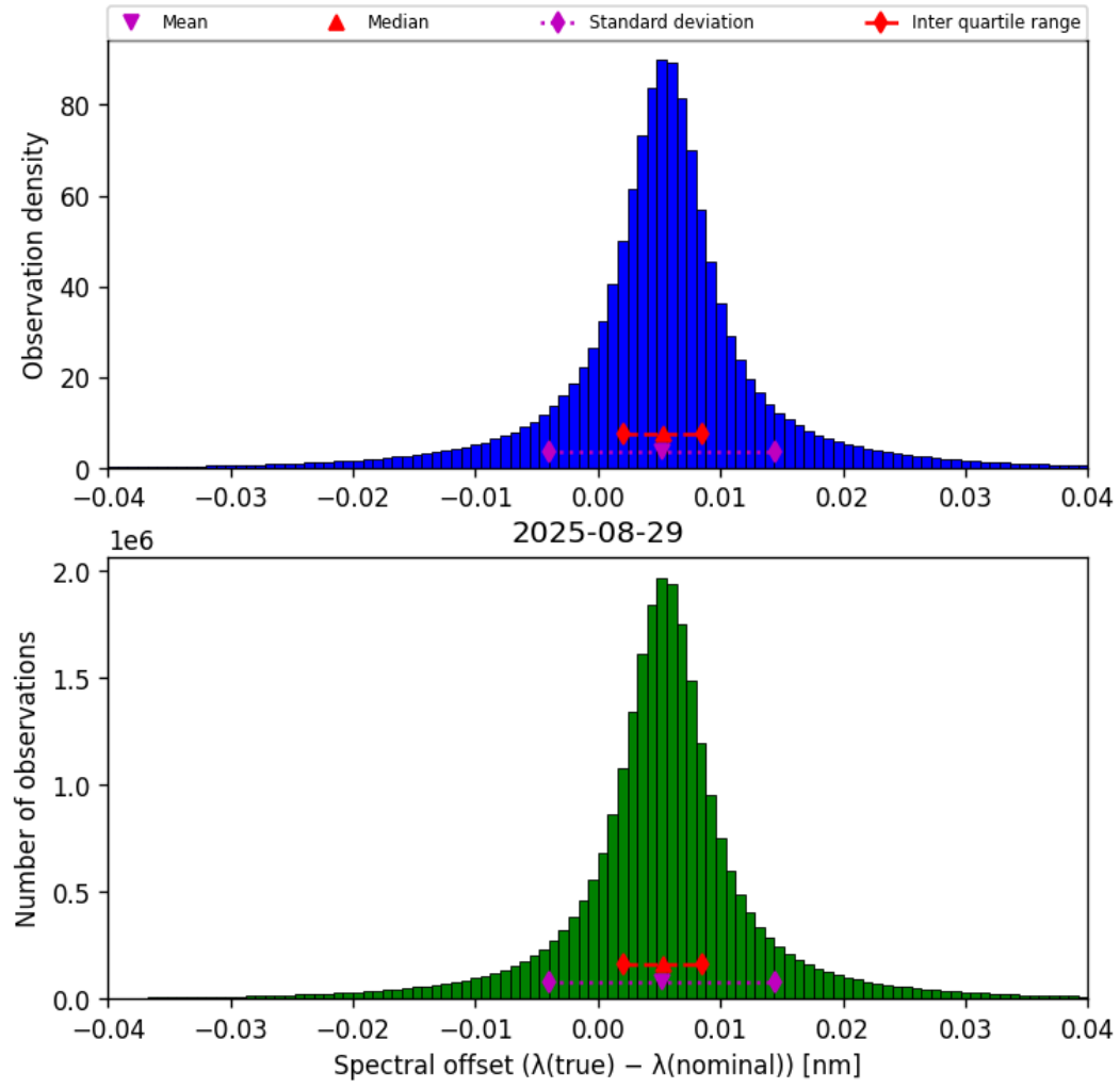
Figure 45: Histogram of “Spectral offset ( \lambda_{\text{true}} - \lambda_{\text{nominal}} )” for 2025-08-28 to 2025-08-30
