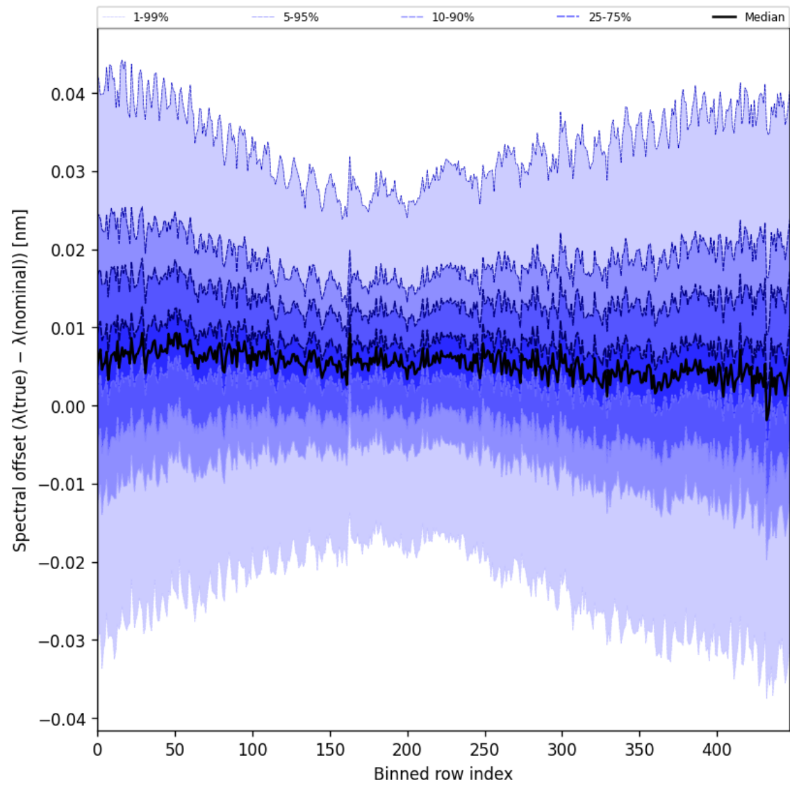
Figure 62: Along track statistics of “Spectral offset ( \lambda_{\text{true}} - \lambda_{\text{nominal}} )” for 2025-08-28 to 2025-08-30
