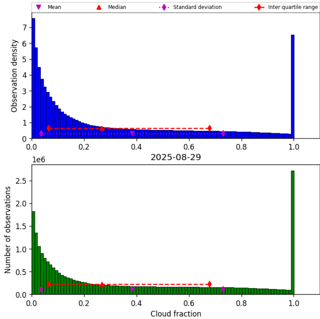
Figure 32: Histogram of “Cloud fraction” for 2025-08-28 to 2025-08-30
