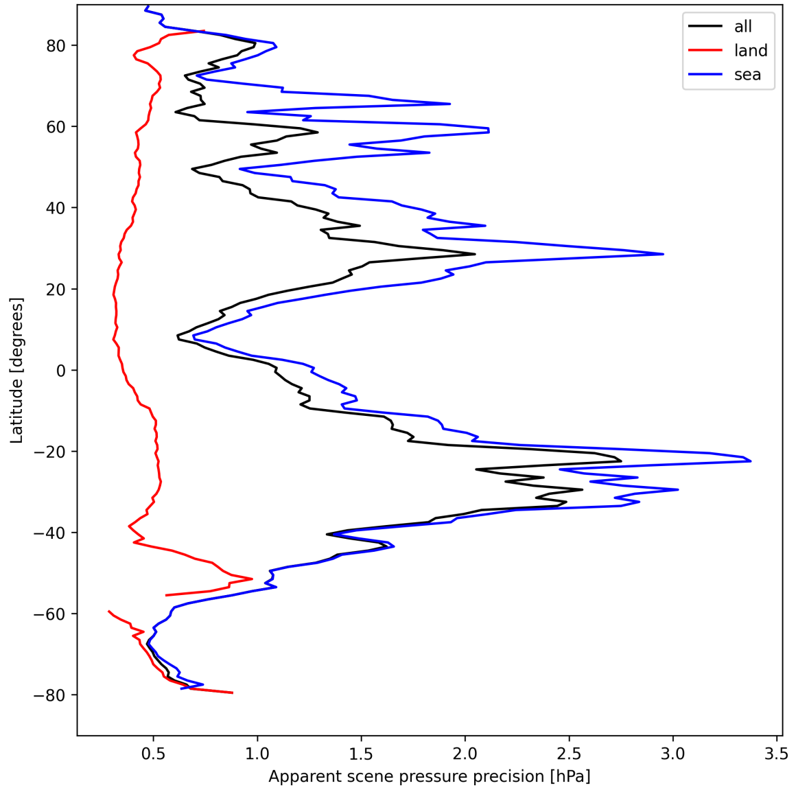
Figure 20: Zonal average of “Apparent scene pressure precision” for 2025-08-28 to 2025-08-30.
