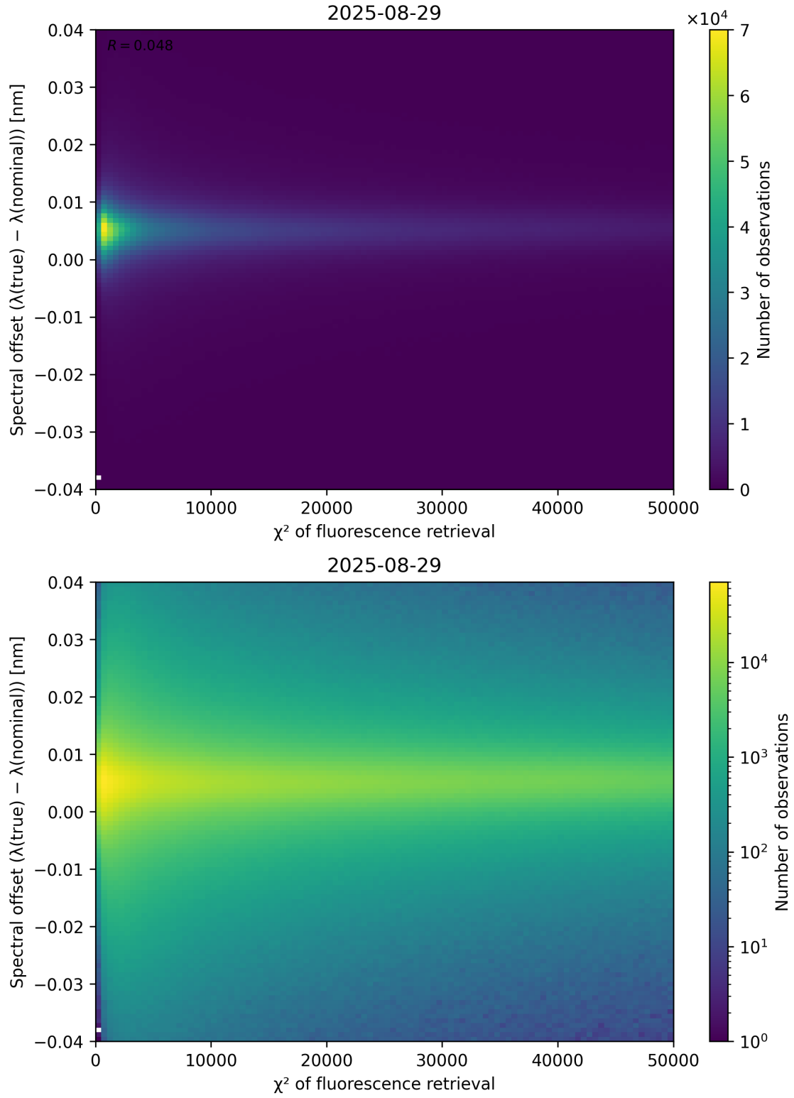
Figure 69: Scatter density plot of “ \chi^2 of fluorescence retrieval” against “Spectral offset ( \lambda_{\text{true}} - \lambda_{\text{nominal}} )” for 2025-08-28 to 2025-08-30.
