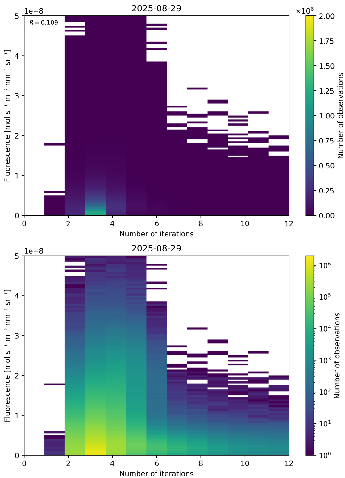
Figure 98: Scatter density plot of “Number of iterations” against “Fluorescence” for 2025-08-28 to 2025-08-30.
