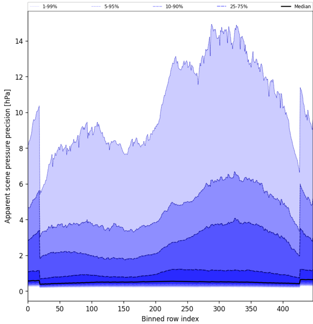
Figure 54: Along track statistics of “Apparent scene pressure precision” for 2025-08-28 to 2025-08-30
