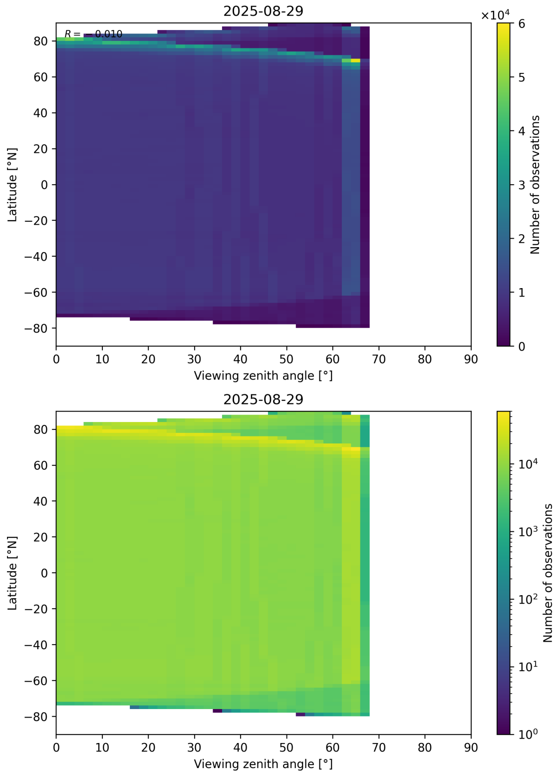
Figure 123: Scatter density plot of “Viewing zenith angle” against “Latitude” for 2025-08-28 to 2025-08-30.
