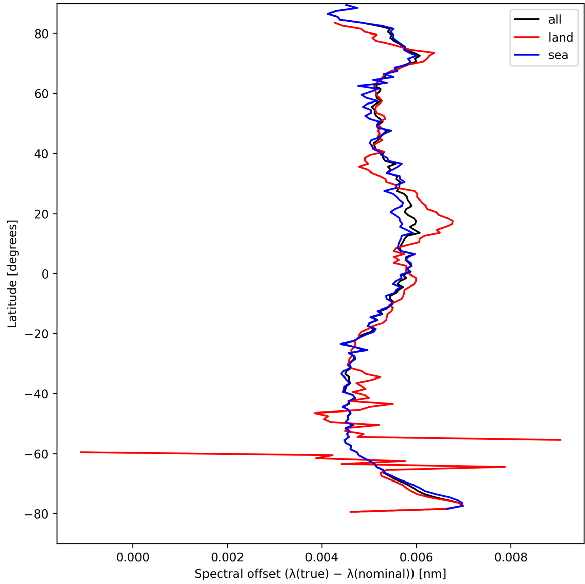
Figure 28: Zonal average of “Spectral offset ( \lambda_{\text{true}} - \lambda_{\text{nominal}} )” for 2025-08-28 to 2025-08-30.
