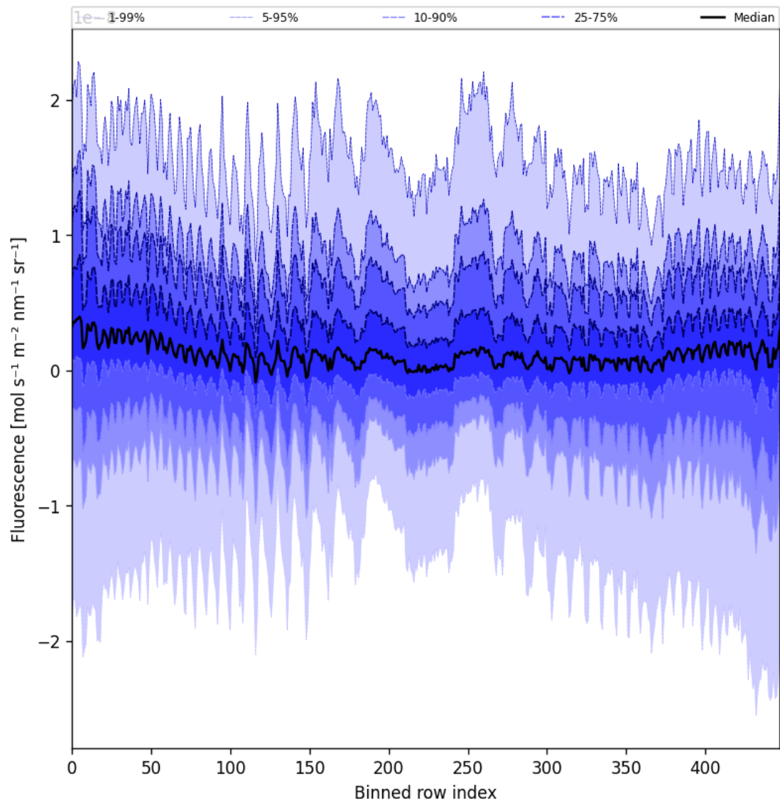
Figure 57: Along track statistics of “Fluorescence” for 2025-08-28 to 2025-08-30
