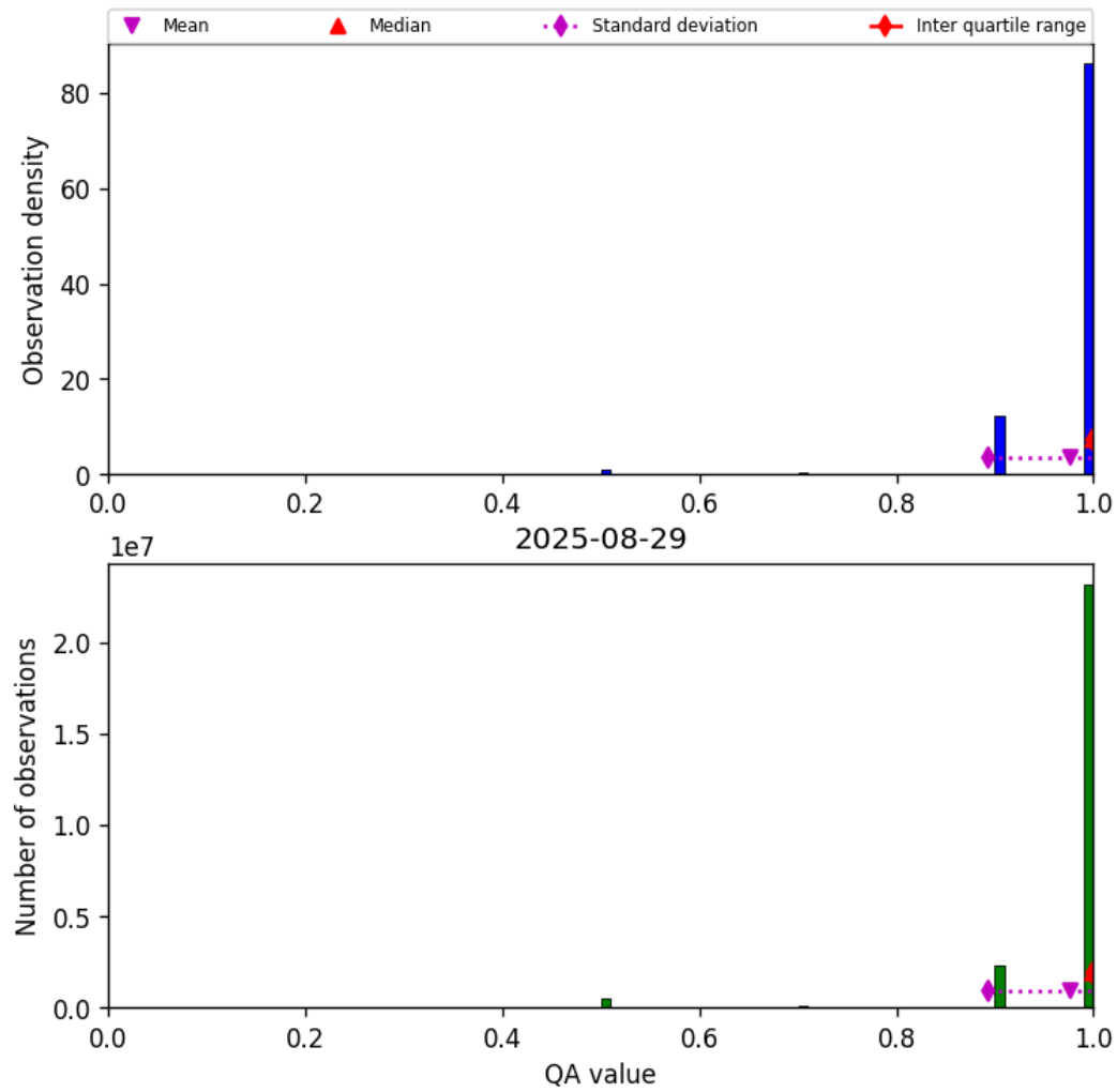
Figure 29: Histogram of “QA value” for 2025-08-28 to 2025-08-30
