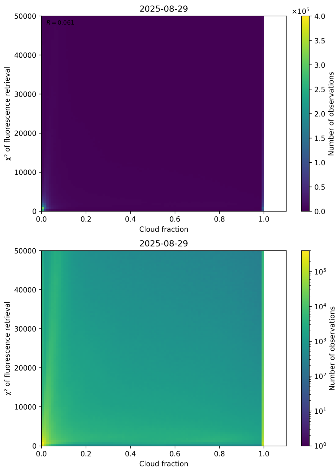
Figure 71: Scatter density plot of “Cloud fraction” against “ \chi^2 of fluorescence retrieval” for 2025-08-28 to 2025-08-30.
