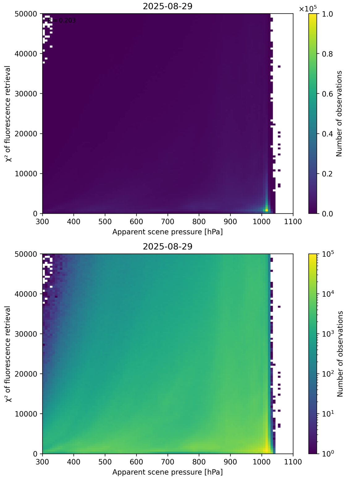
Figure 63: Scatter density plot of “Apparent scene pressure” against “ \chi^2 of fluorescence retrieval” for 2025-08-28 to 2025-08-30.
