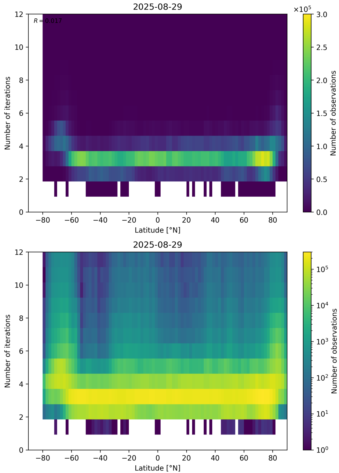
Figure 93: Scatter density plot of “Latitude” against “Number of iterations” for 2025-08-28 to 2025-08-30.
