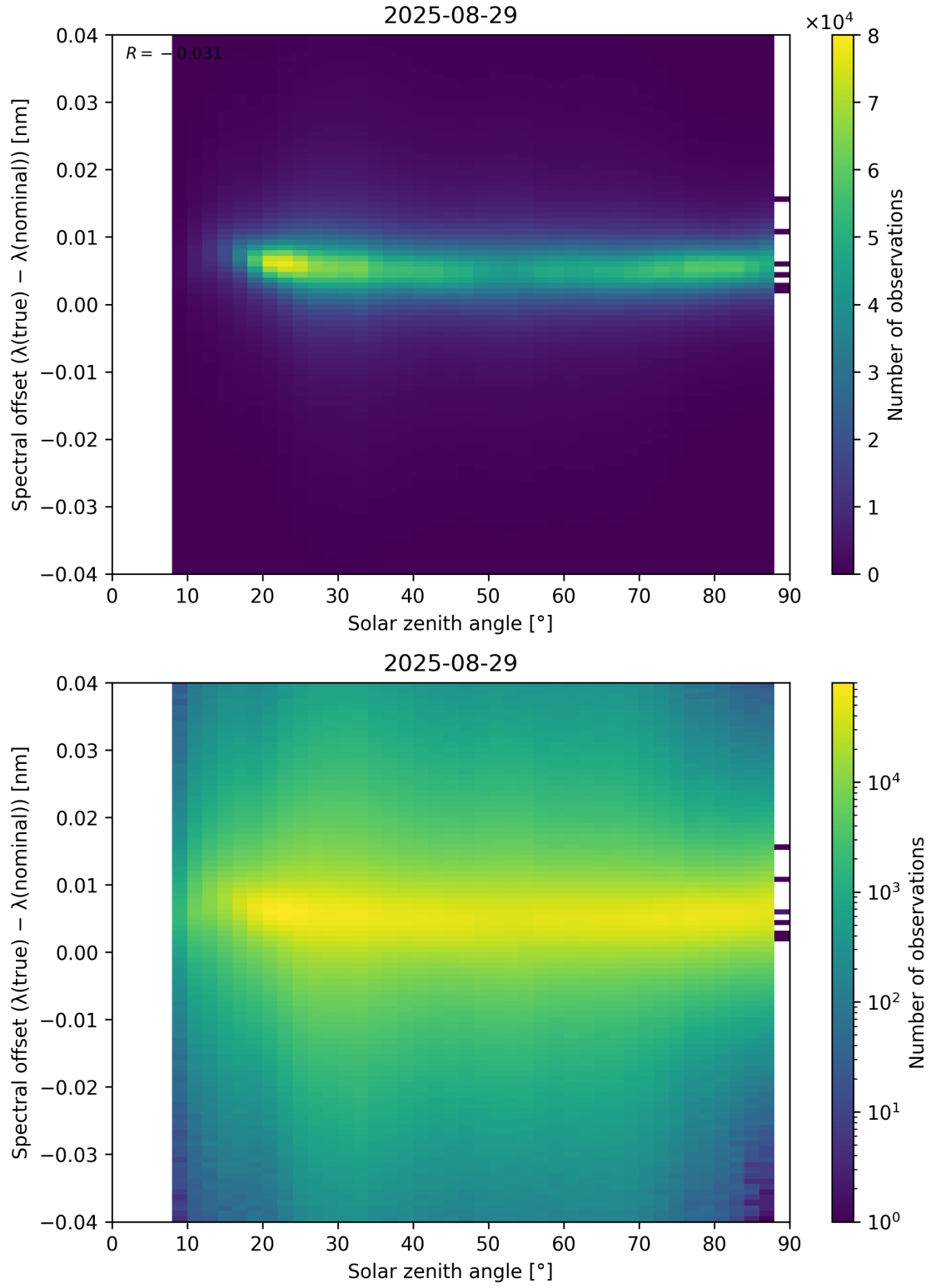
Figure 117: Scatter density plot of “Solar zenith angle” against “Spectral offset ( \lambda_{\text{true}} - \lambda_{\text{nominal}} )” for 2025-08-28 to 2025-08-30.
