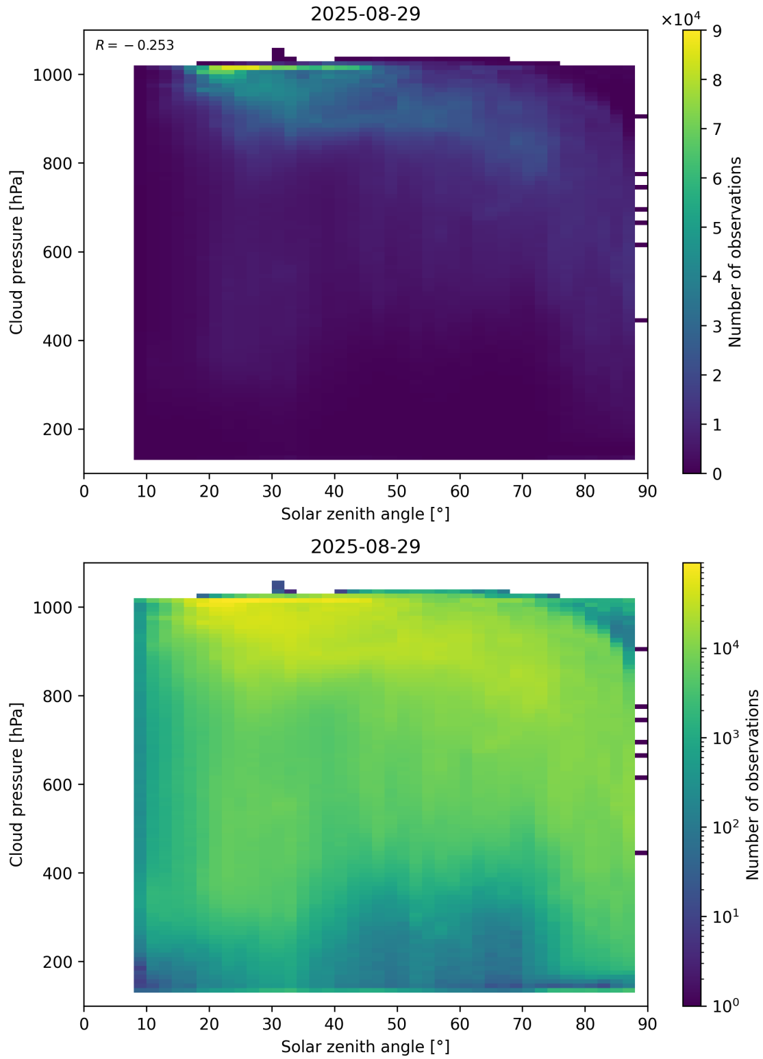
Figure 111: Scatter density plot of “Solar zenith angle” against “Cloud pressure” for 2025-08-28 to 2025-08-30.
