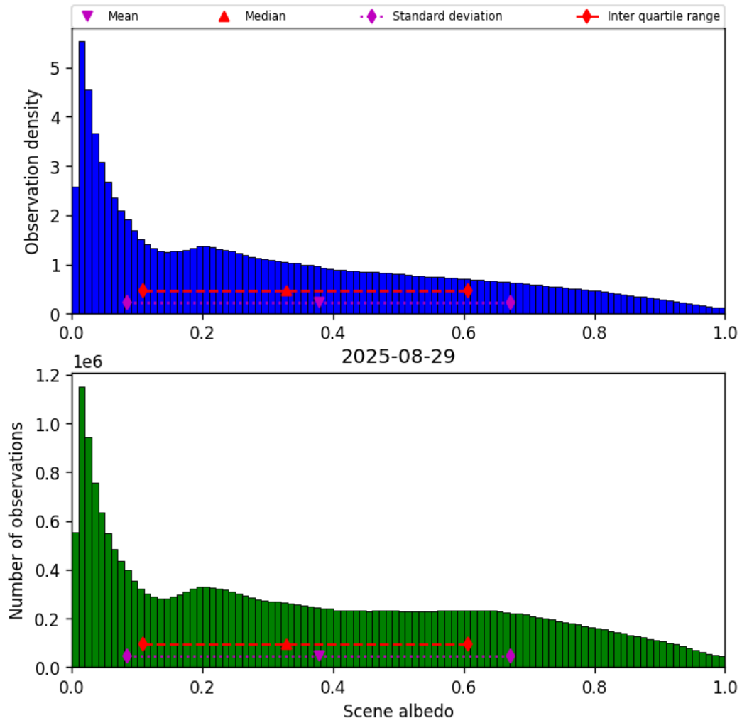
Figure 34: Histogram of “Scene albedo” for 2025-08-28 to 2025-08-30
