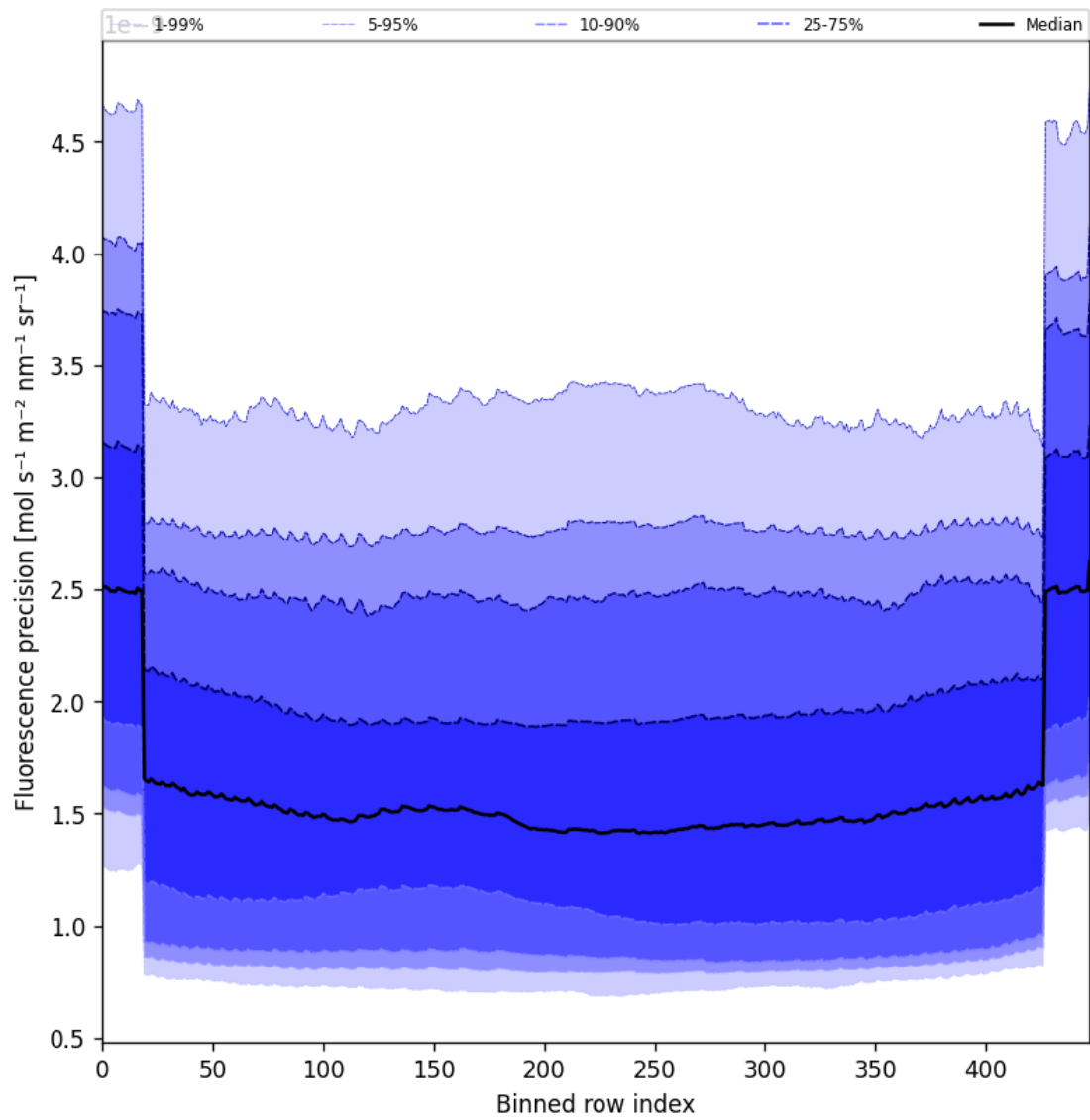
Figure 58: Along track statistics of “Fluorescence precision” for 2025-08-28 to 2025-08-30
