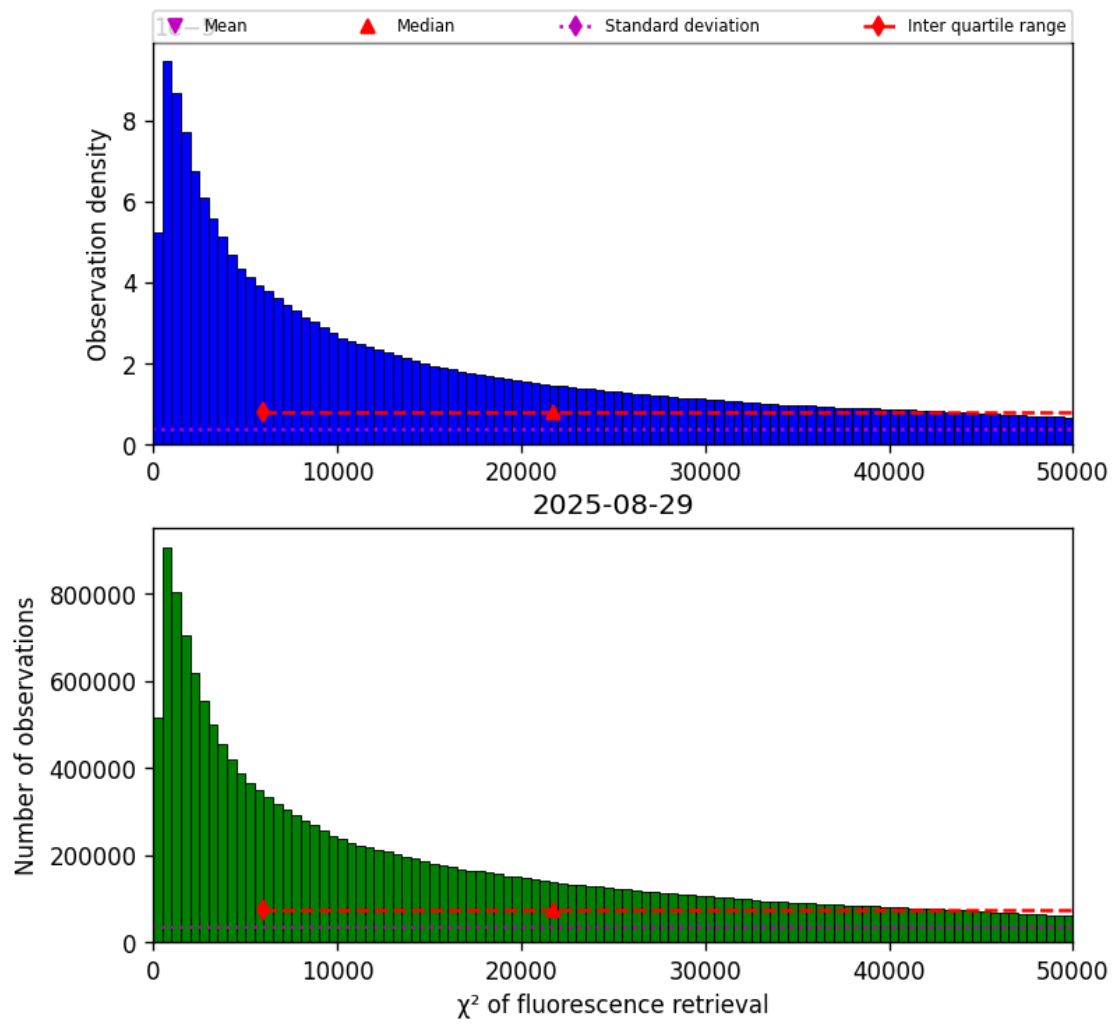
Figure 42: Histogram of “ \chi^2 of fluorescence retrieval” for 2025-08-28 to 2025-08-30
