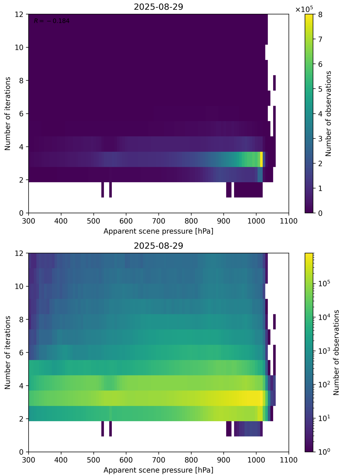
Figure 65: Scatter density plot of “Apparent scene pressure” against “Number of iterations” for 2025-08-28 to 2025-08-30.
