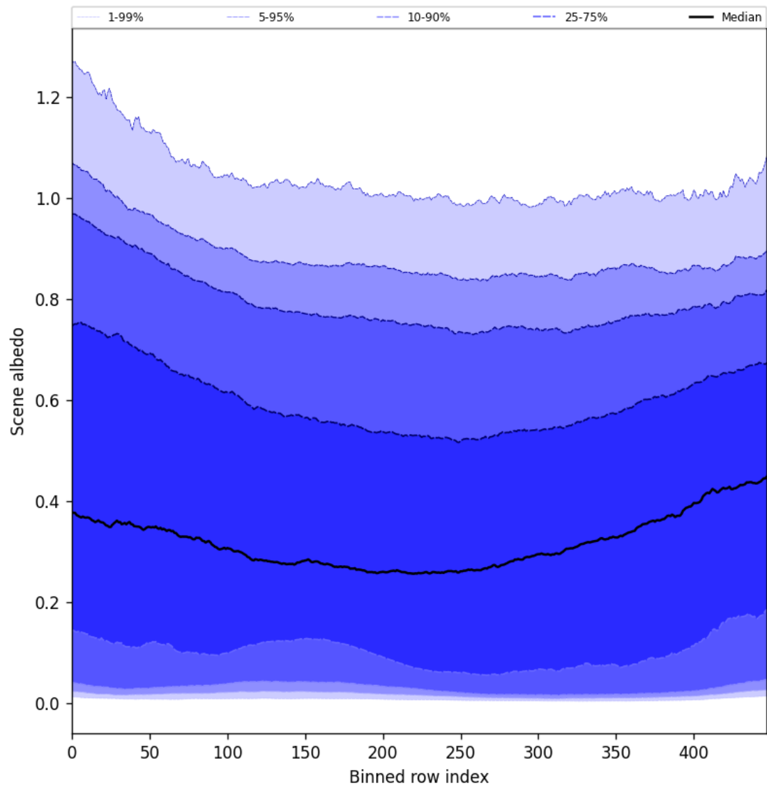
Figure 51: Along track statistics of “Scene albedo” for 2025-08-30 to 2025-08-31
