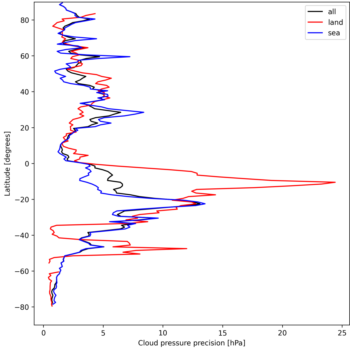
Figure 14: Zonal average of “Cloud pressure precision” for 2025-08-30 to 2025-08-31.
