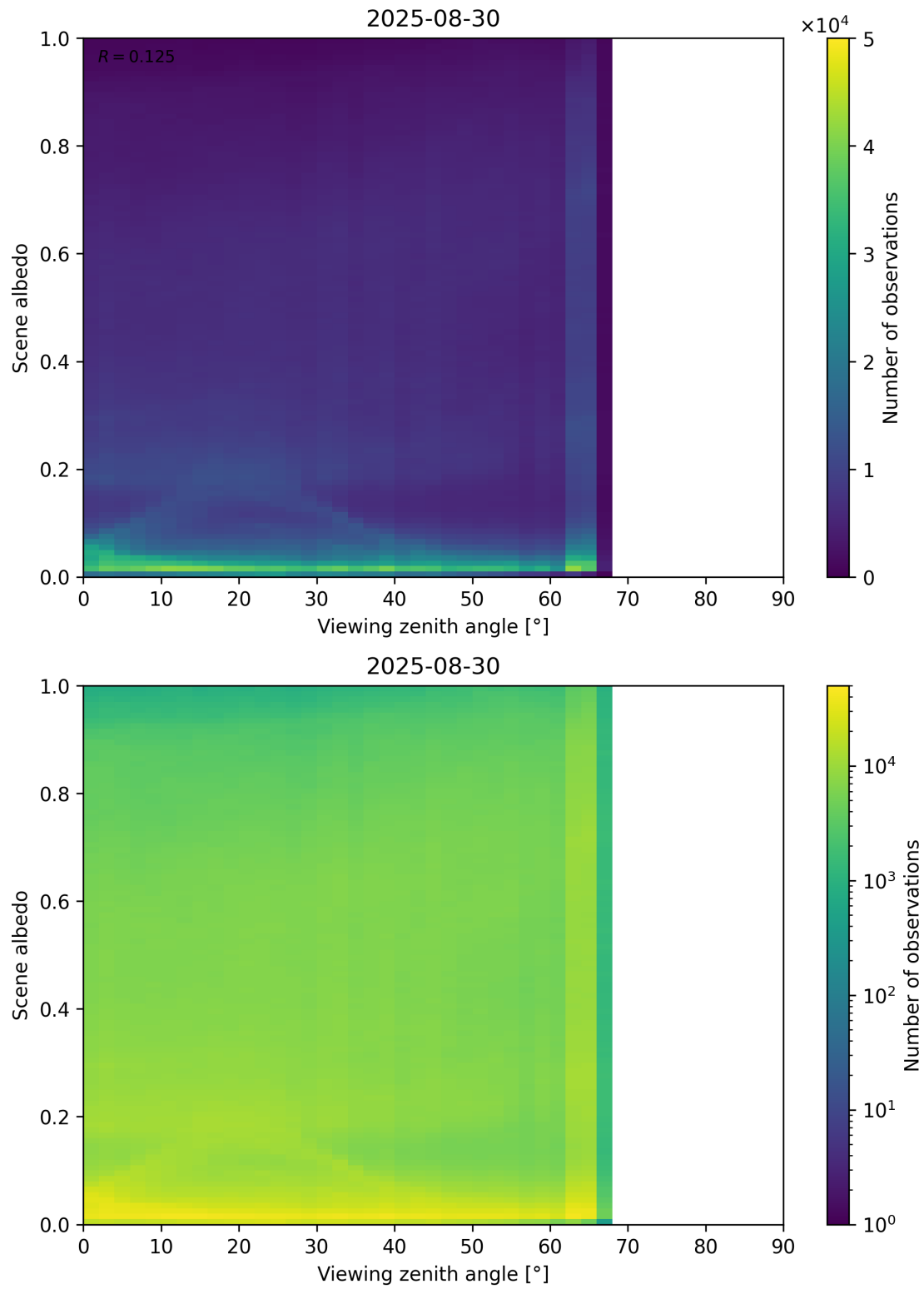
Figure 126: Scatter density plot of “Viewing zenith angle” against “Scene albedo” for 2025-08-30 to 2025-08-31.
