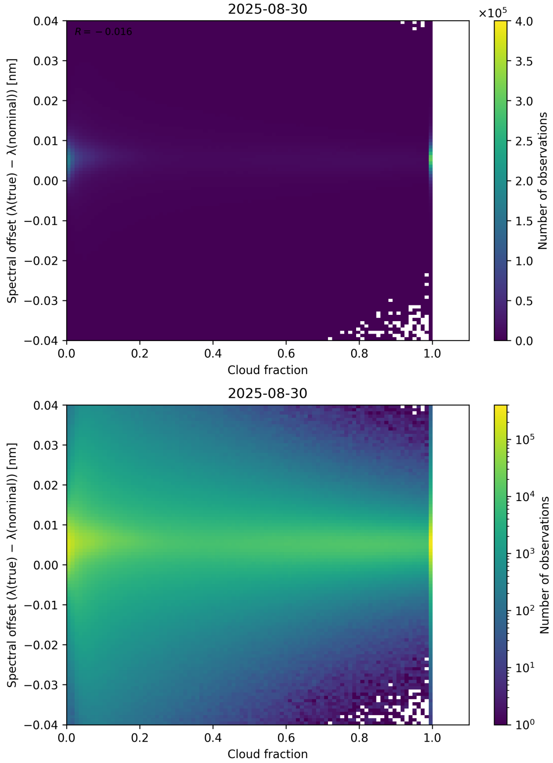
Figure 76: Scatter density plot of “Cloud fraction” against “Spectral offset ( \lambda_{\text{true}} - \lambda_{\text{nominal}} )” for 2025-08-30 to 2025-08-31.
