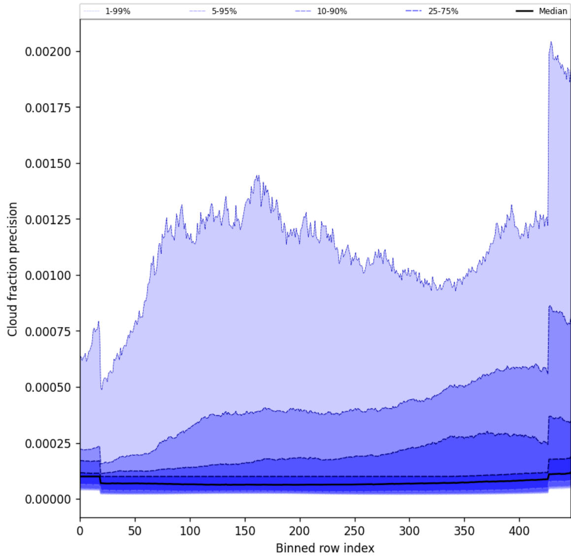
Figure 50: Along track statistics of “Cloud fraction precision” for 2025-08-30 to 2025-08-31
