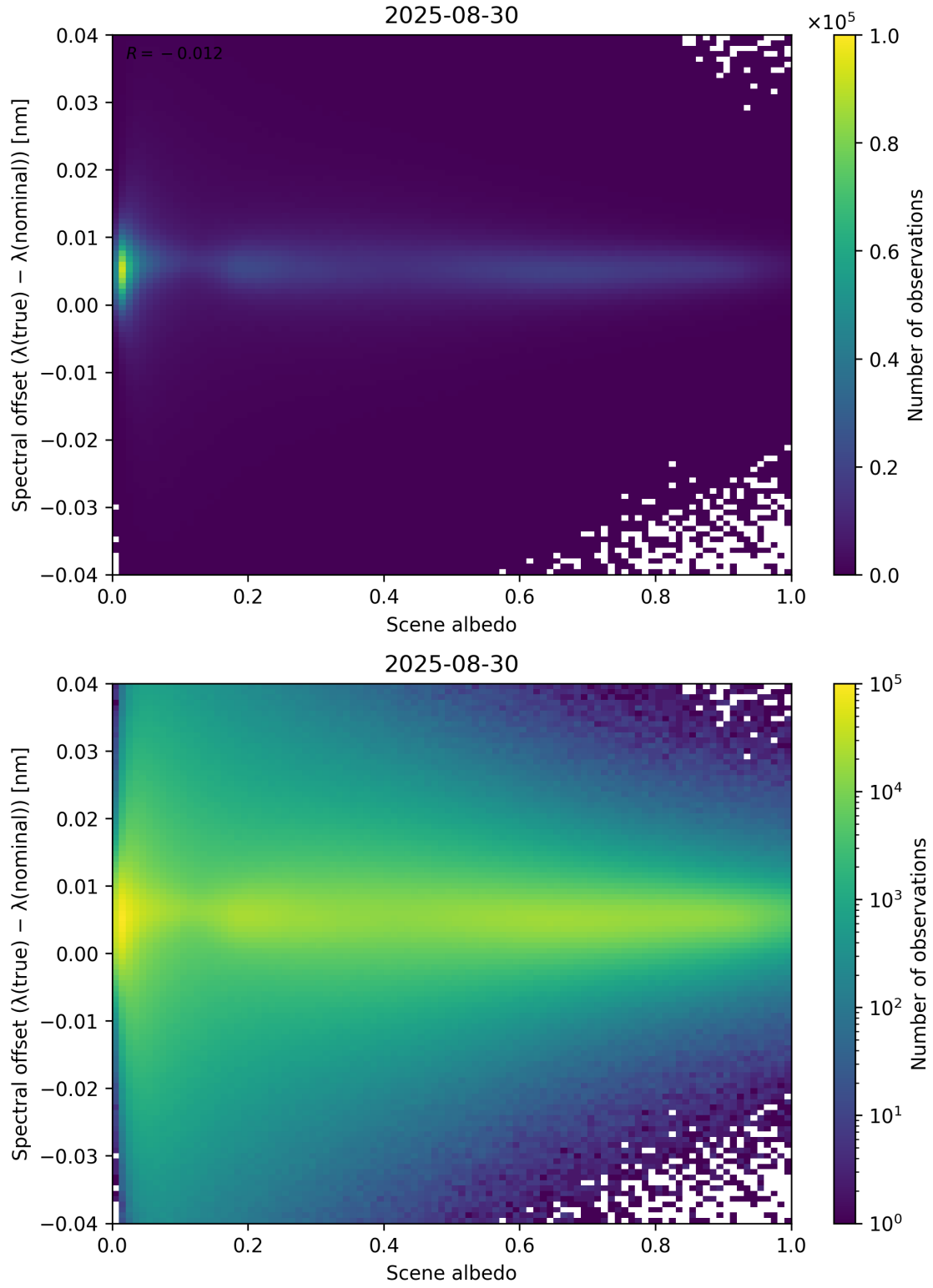
Figure 107: Scatter density plot of “Scene albedo” against “Spectral offset ( \lambda_{\text{true}} - \lambda_{\text{nominal}} )” for 2025-08-30 to 2025-08-31.
