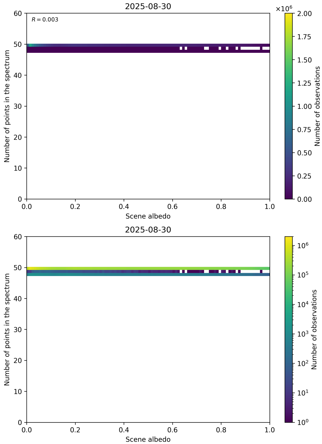
Figure 106: Scatter density plot of “Scene albedo” against “Number of points in the spectrum” for 2025-08-30 to 2025-08-31.
