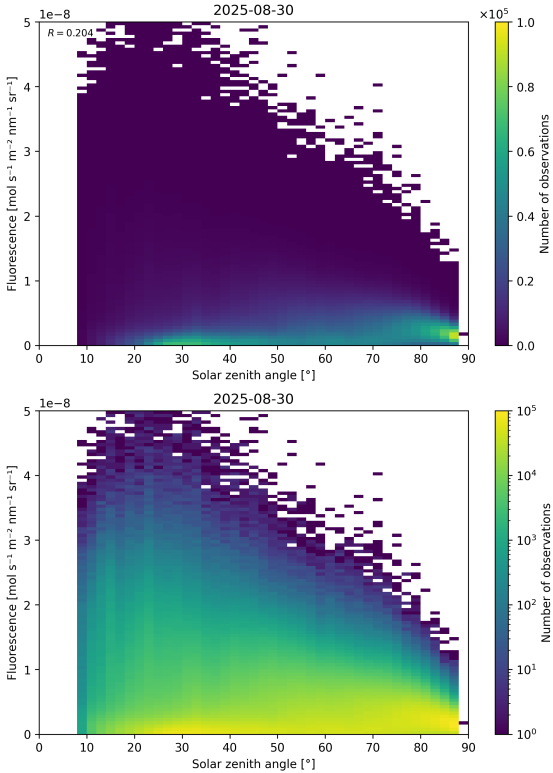
Figure 112: Scatter density plot of “Solar zenith angle” against “Fluorescence” for 2025-08-30 to 2025-08-31.
