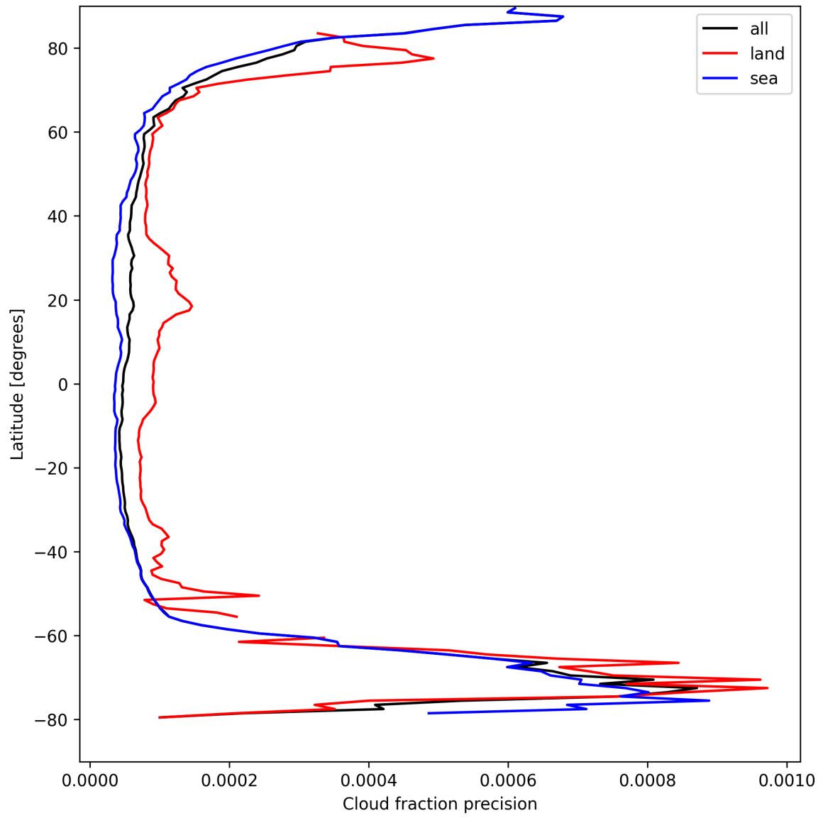
Figure 16: Zonal average of “Cloud fraction precision” for 2025-08-30 to 2025-08-31.
