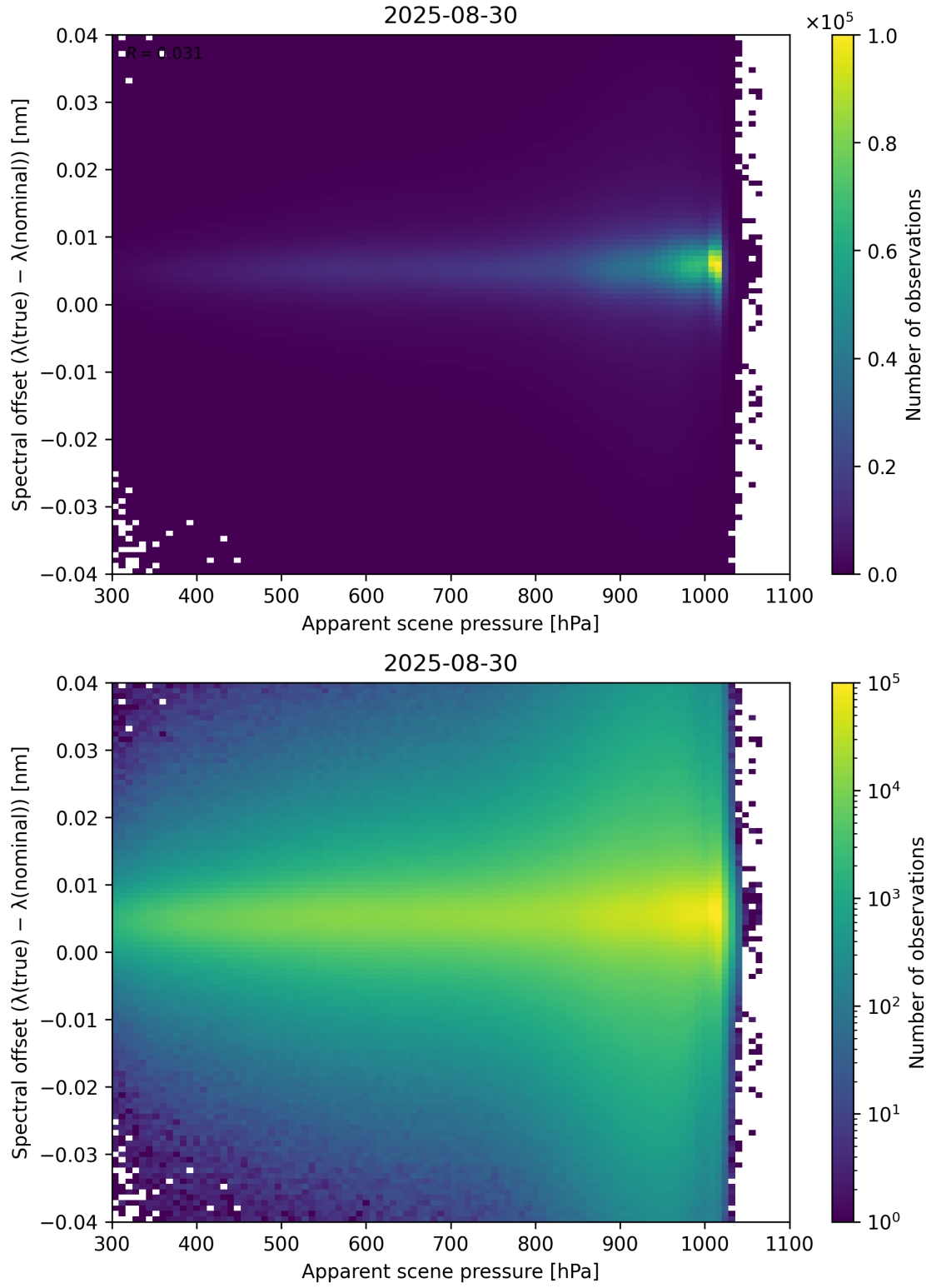
Figure 67: Scatter density plot of “Apparent scene pressure” against “Spectral offset ( \lambda_{\text{true}} - \lambda_{\text{nominal}} )” for 2025-08-30 to 2025-08-31.
