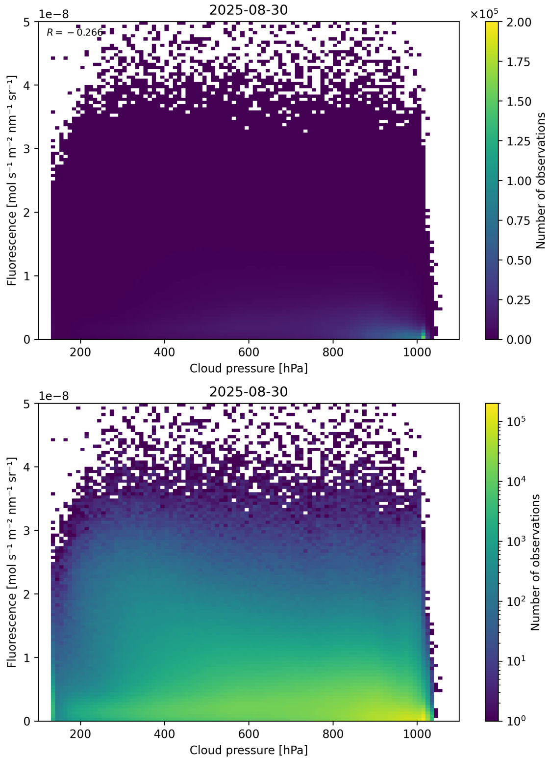
Figure 80: Scatter density plot of “Cloud pressure” against “Fluorescence” for 2025-08-30 to 2025-08-31.
