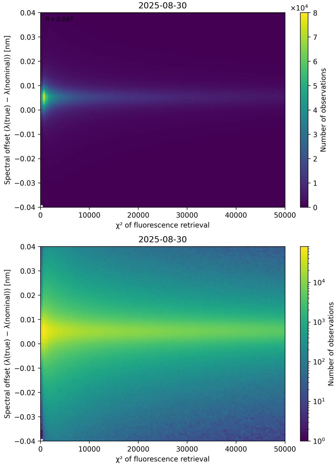
Figure 69: Scatter density plot of “ \chi^2 of fluorescence retrieval” against “Spectral offset ( \lambda_{\text{true}} - \lambda_{\text{nominal}} )” for 2025-08-30 to 2025-08-31.
