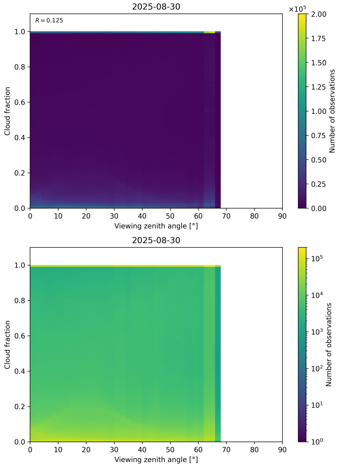
Figure 120: Scatter density plot of “Viewing zenith angle” against “Cloud fraction” for 2025-08-30 to 2025-08-31.
