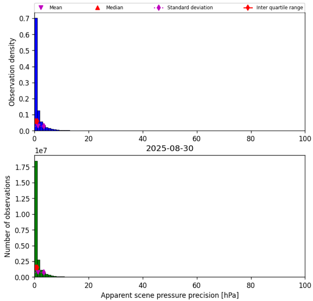
Figure 37: Histogram of “Apparent scene pressure precision” for 2025-08-30 to 2025-08-31
