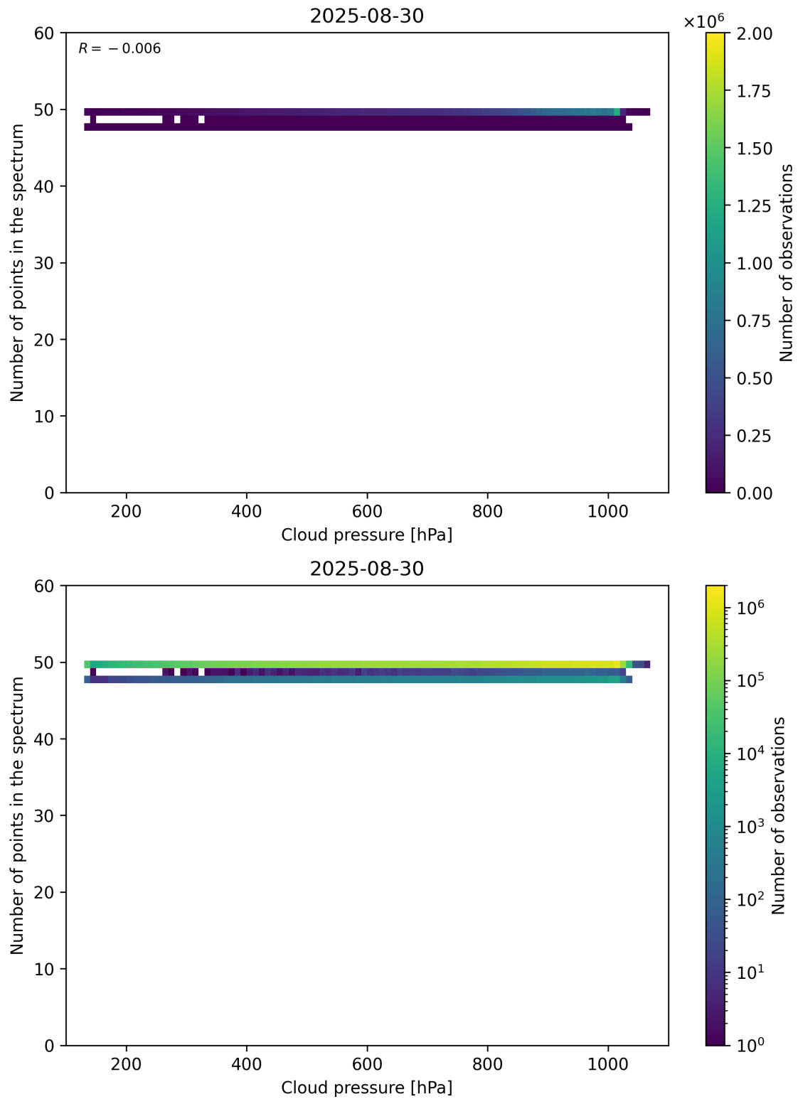
Figure 82: Scatter density plot of “Cloud pressure” against “Number of points in the spectrum” for 2025-08-30 to 2025-08-31.
