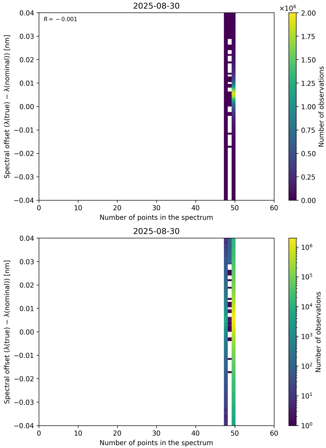
Figure 101: Scatter density plot of “Number of points in the spectrum” against “Spectral offset ( \lambda_{\text{true}} - \lambda_{\text{nominal}} )” for 2025-08-30 to 2025-08-31.
