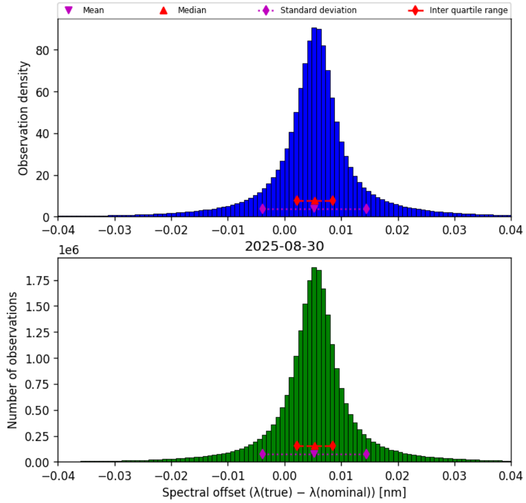
Figure 45: Histogram of “Spectral offset ( \lambda_{\text{true}} - \lambda_{\text{nominal}} )” for 2025-08-30 to 2025-08-31
