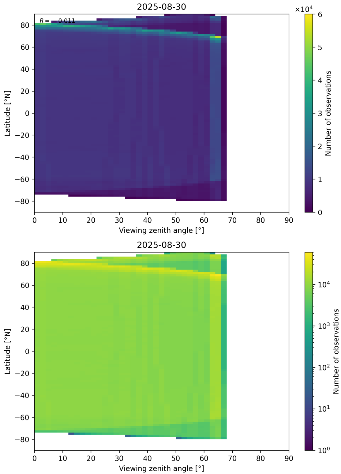
Figure 123: Scatter density plot of “Viewing zenith angle” against “Latitude” for 2025-08-30 to 2025-08-31.
