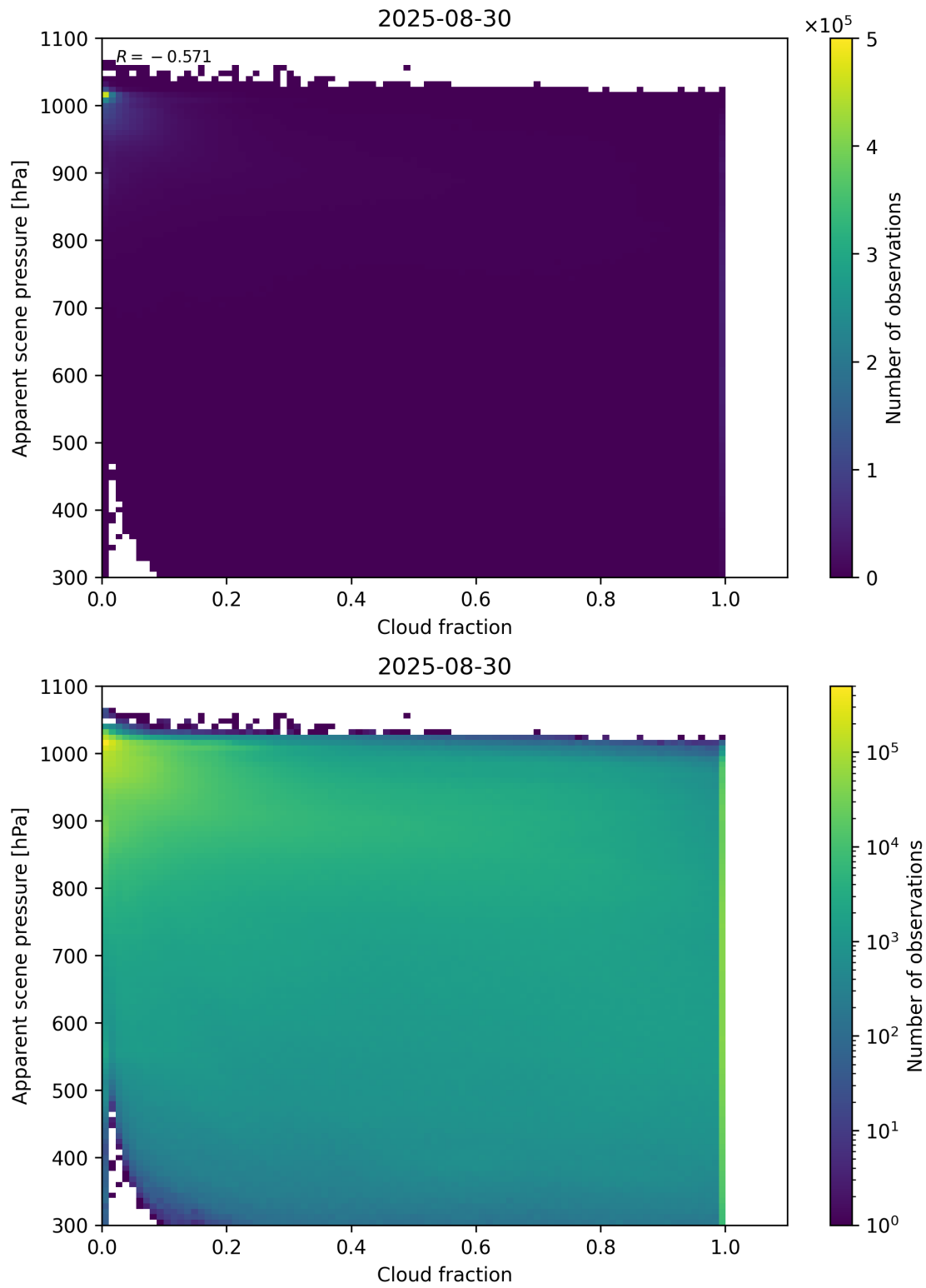
Figure 70: Scatter density plot of “Cloud fraction” against “Apparent scene pressure” for 2025-08-30 to 2025-08-31.
