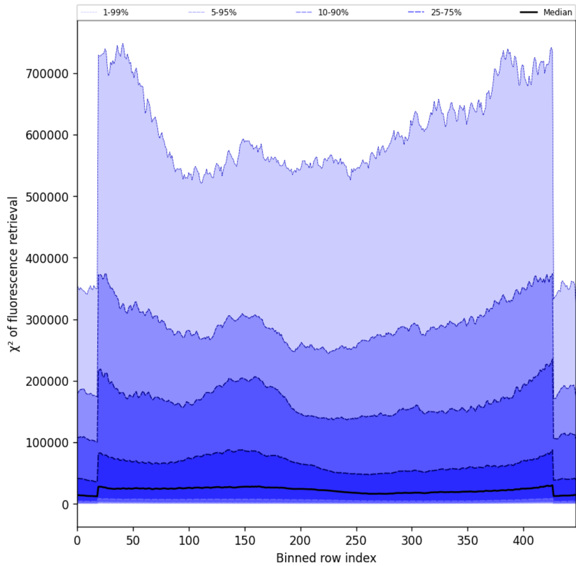
Figure 59: Along track statistics of “ \chi^2 of fluorescence retrieval” for 2025-08-30 to 2025-08-31
