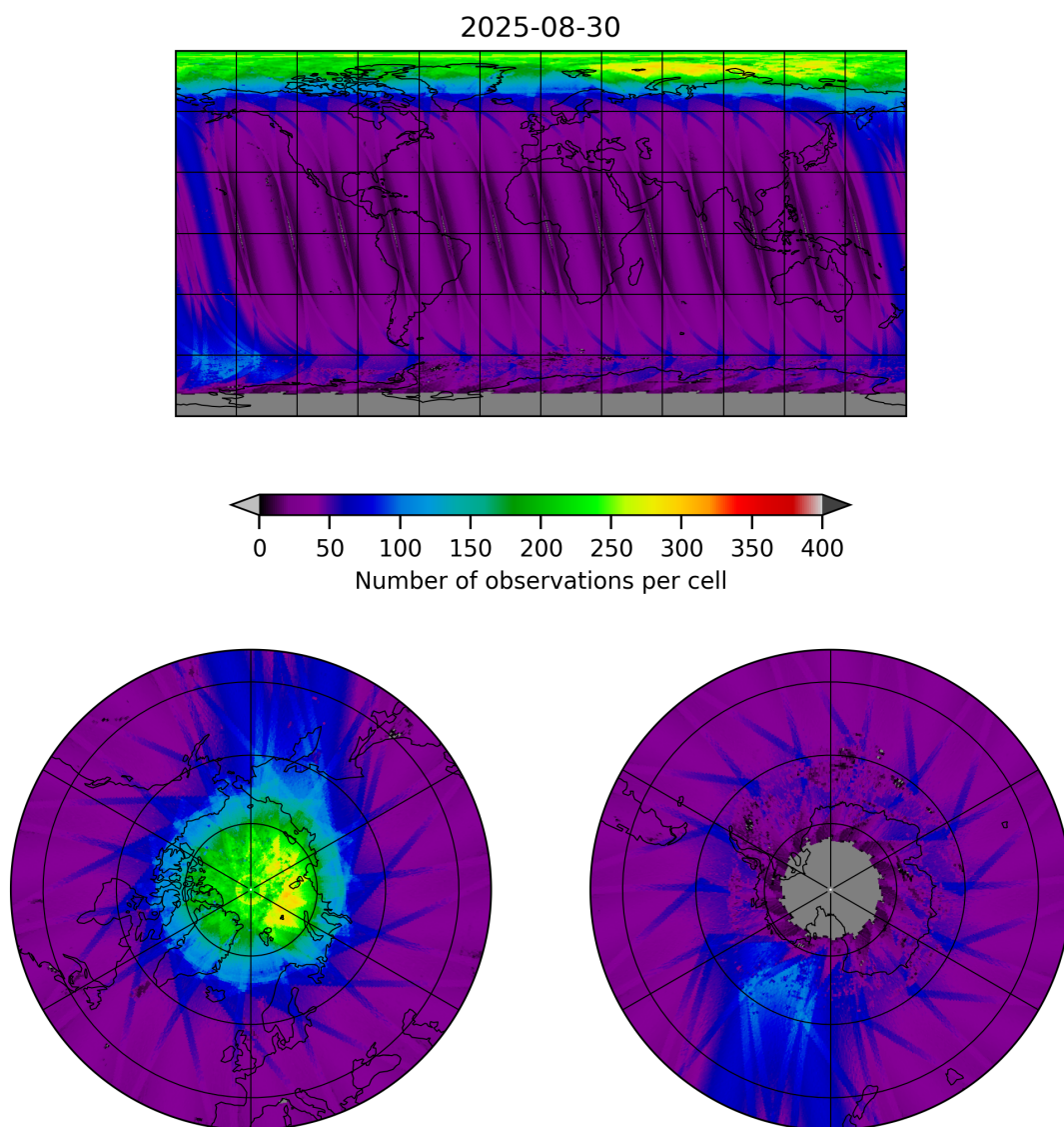
Figure 11: Map of the number of observations for 2025-08-30 to 2025-08-31
