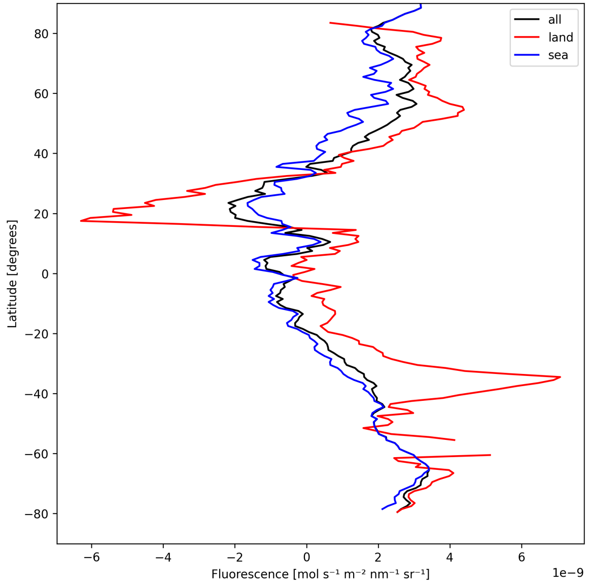
Figure 23: Zonal average of “Fluorescence” for 2025-08-30 to 2025-08-31.
