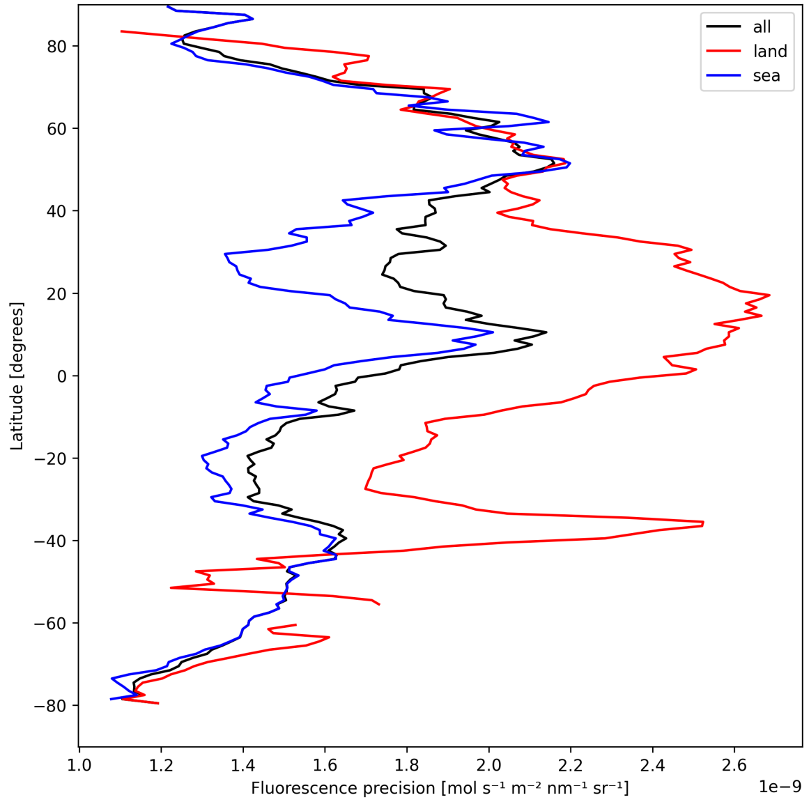
Figure 24: Zonal average of “Fluorescence precision” for 2025-08-30 to 2025-08-31.
