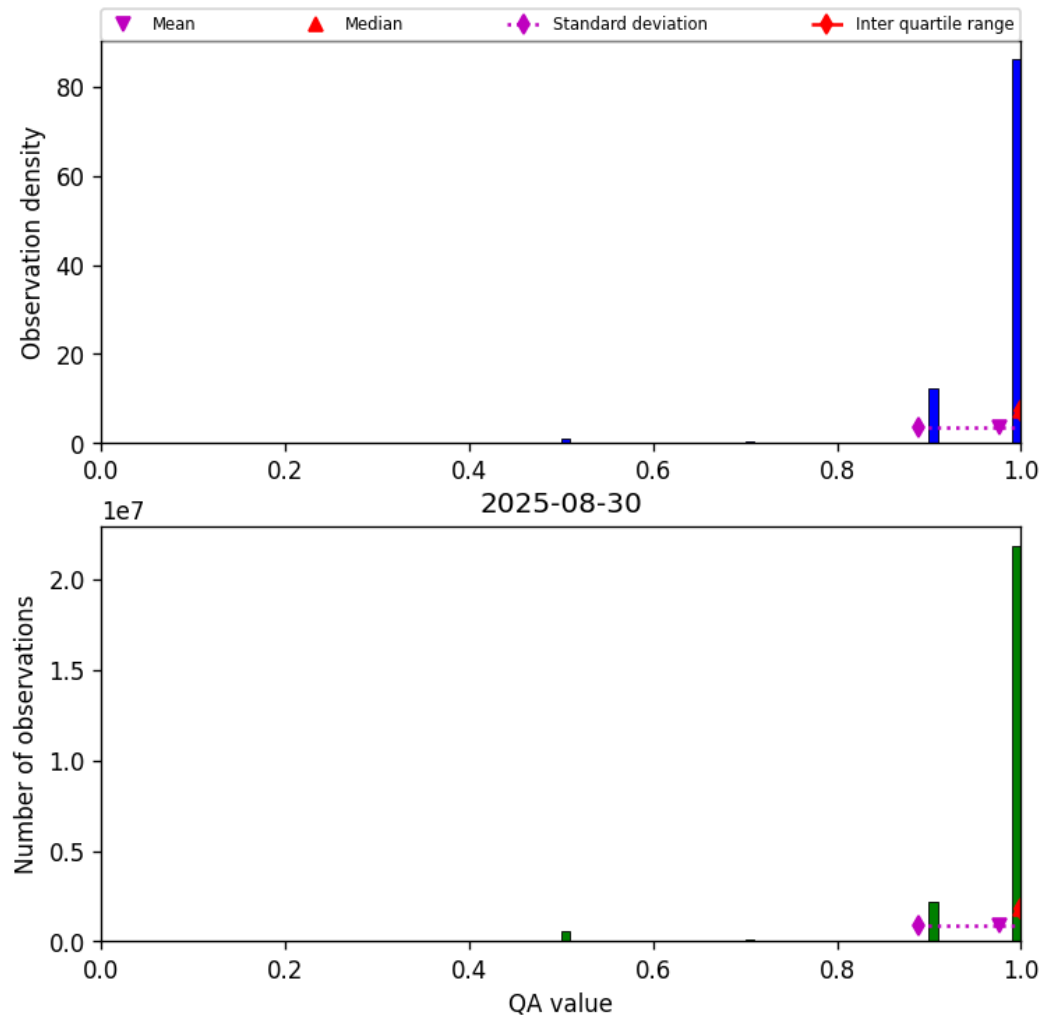
Figure 29: Histogram of “QA value” for 2025-08-30 to 2025-08-31
