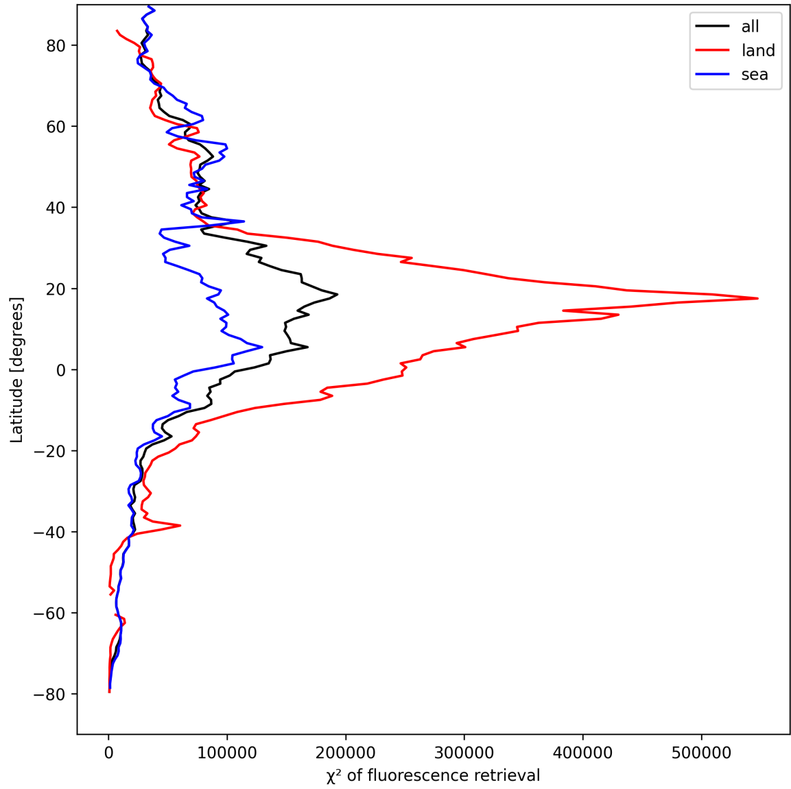
Figure 25: Zonal average of “ \chi^2 of fluorescence retrieval” for 2025-08-30 to 2025-08-31.
