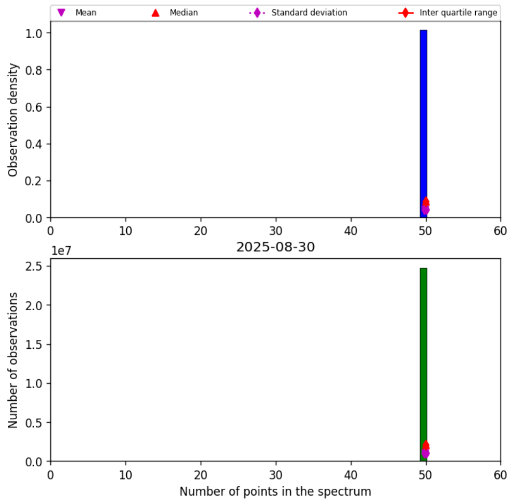
Figure 44: Histogram of “Number of points in the spectrum” for 2025-08-30 to 2025-08-31
