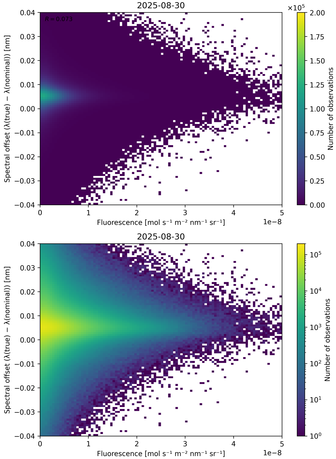
Figure 87: Scatter density plot of “Fluorescence” against “Spectral offset ( \lambda_{\text{true}} - \lambda_{\text{nominal}} )” for 2025-08-30 to 2025-08-31.
