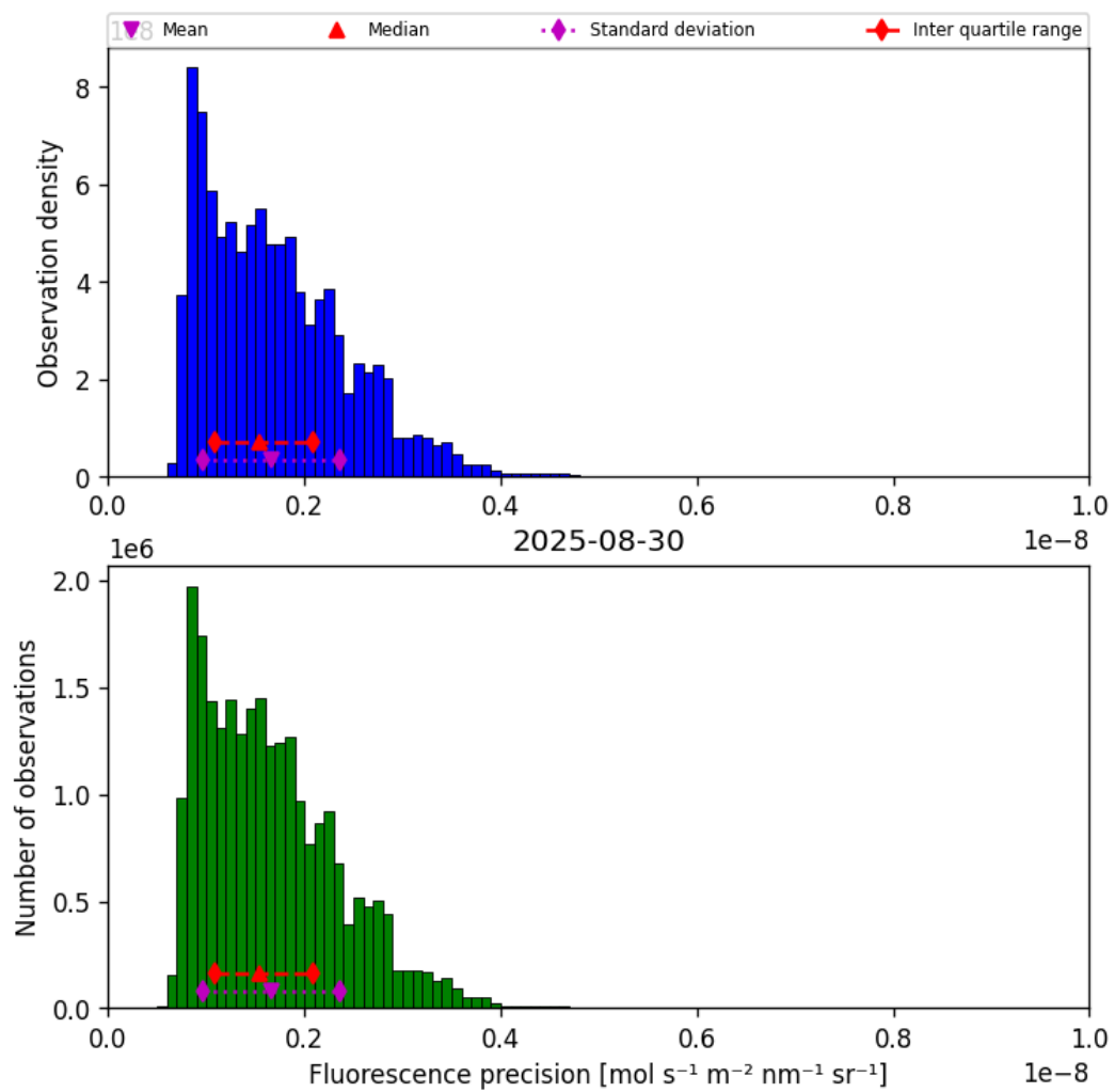
Figure 41: Histogram of “Fluorescence precision” for 2025-08-30 to 2025-08-31
