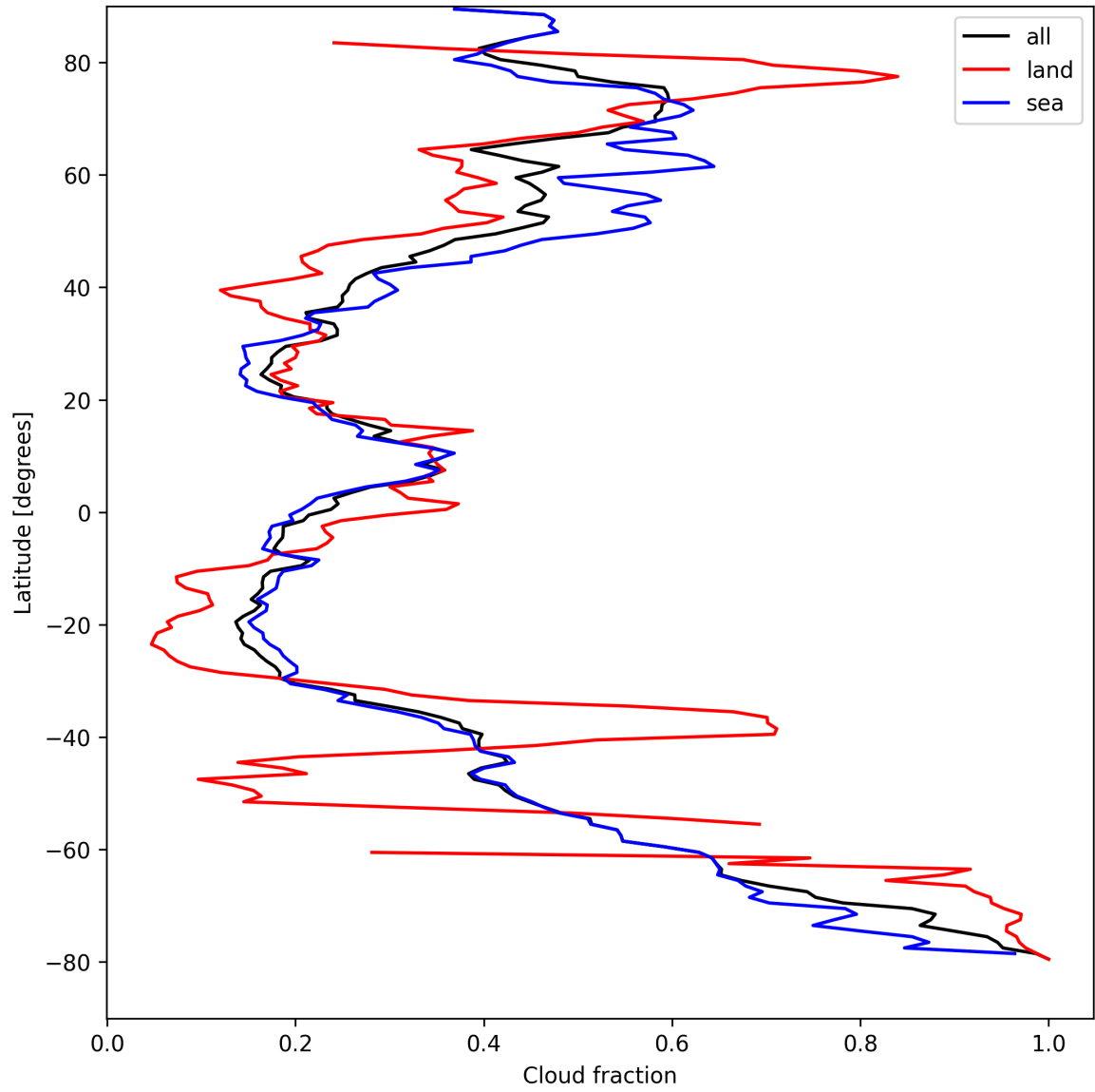
Figure 15: Zonal average of “Cloud fraction” for 2025-08-30 to 2025-08-31.
