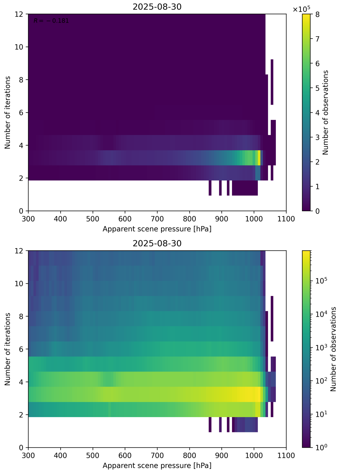
Figure 65: Scatter density plot of “Apparent scene pressure” against “Number of iterations” for 2025-08-30 to 2025-08-31.
