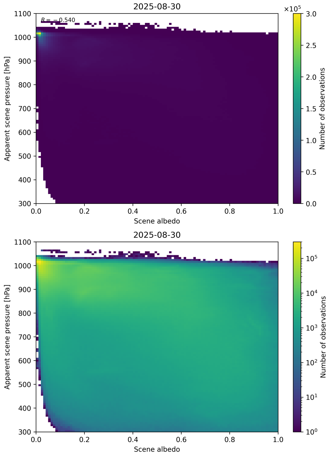
Figure 102: Scatter density plot of “Scene albedo” against “Apparent scene pressure” for 2025-08-30 to 2025-08-31.
