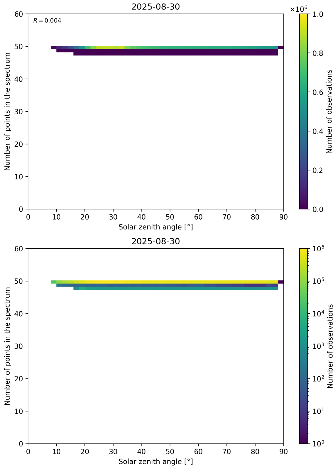
Figure 115: Scatter density plot of “Solar zenith angle” against “Number of points in the spectrum” for 2025-08-30 to 2025-08-31.
