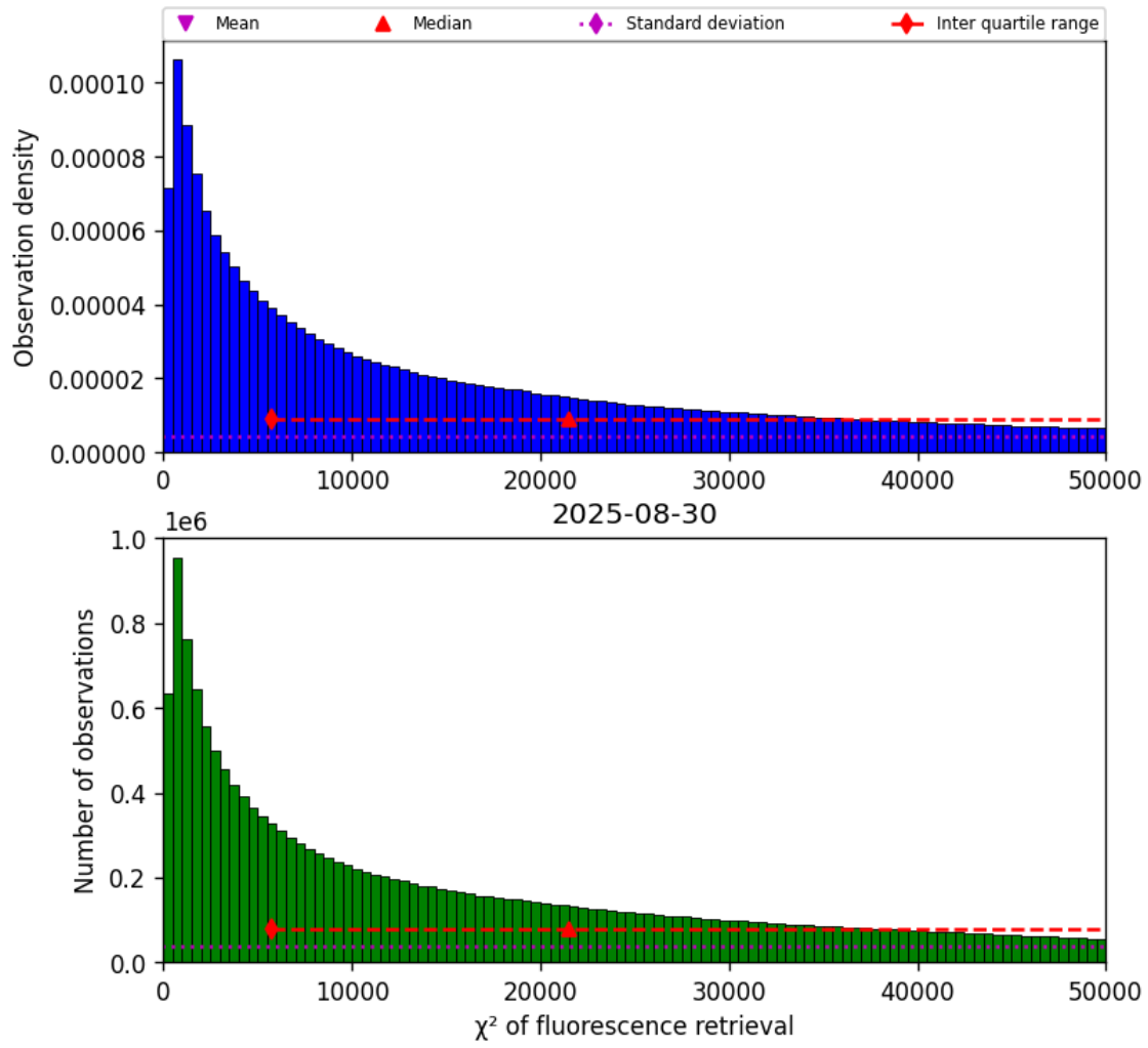
Figure 42: Histogram of “ \chi^2 of fluorescence retrieval” for 2025-08-30 to 2025-08-31
