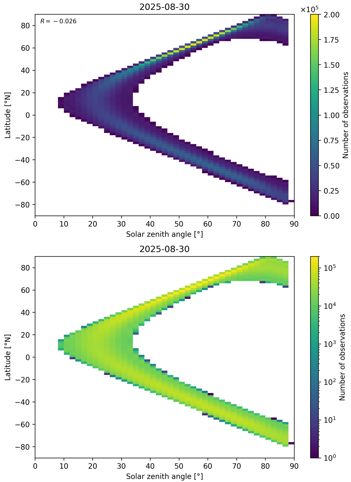
Figure 113: Scatter density plot of “Solar zenith angle” against “Latitude” for 2025-08-30 to 2025-08-31.
