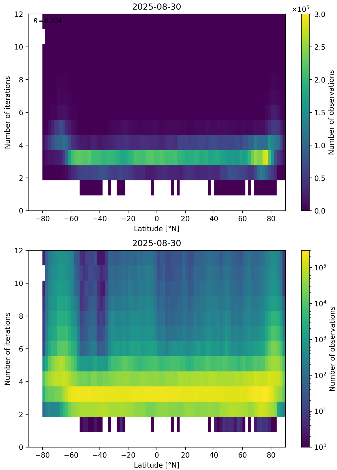
Figure 93: Scatter density plot of “Latitude” against “Number of iterations” for 2025-08-30 to 2025-08-31.
