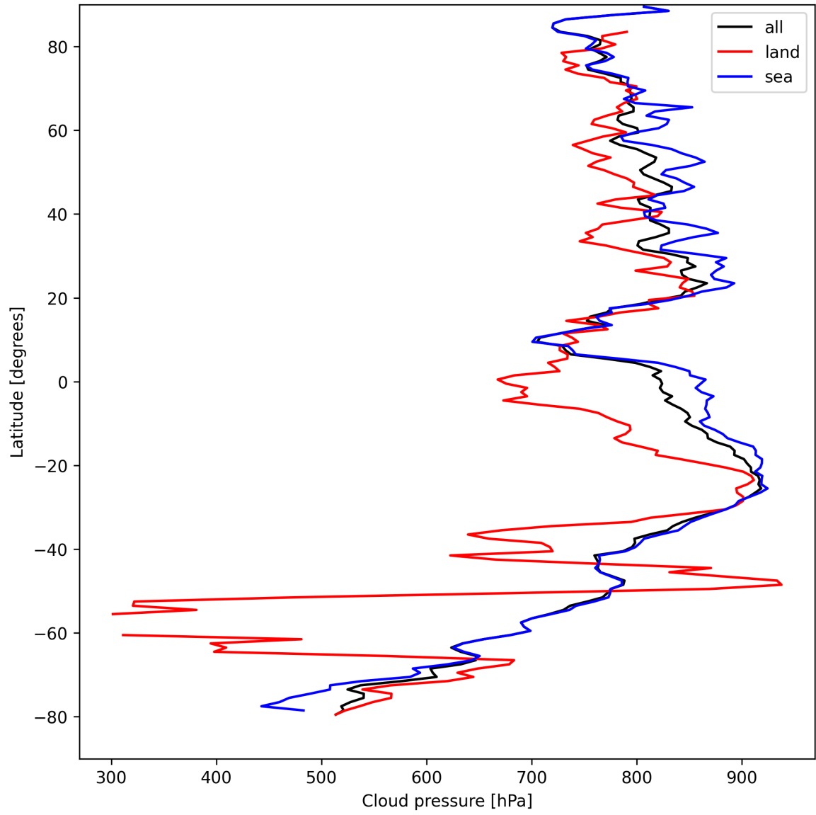
Figure 13: Zonal average of “Cloud pressure” for 2025-08-30 to 2025-08-31.
