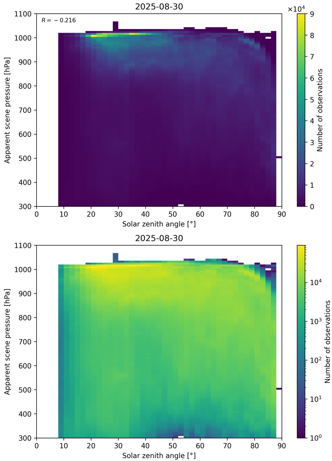
Figure 108: Scatter density plot of “Solar zenith angle” against “Apparent scene pressure” for 2025-08-30 to 2025-08-31.
