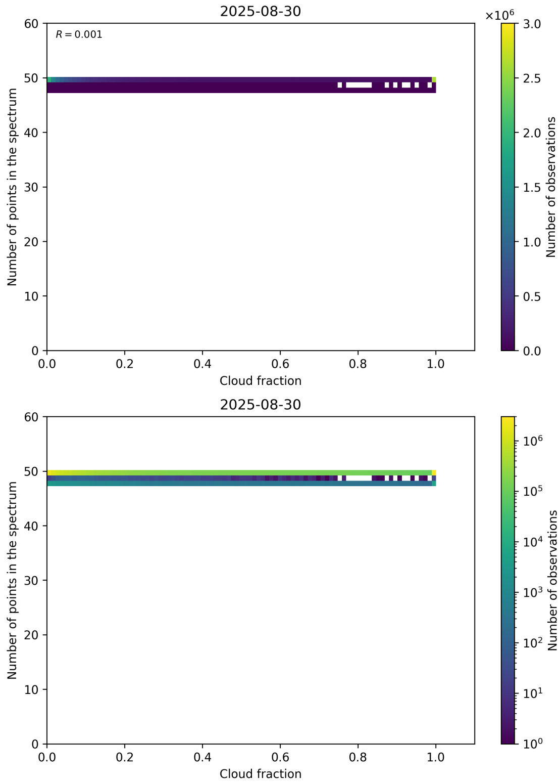
Figure 74: Scatter density plot of “Cloud fraction” against “Number of points in the spectrum” for 2025-08-30 to 2025-08-31.
