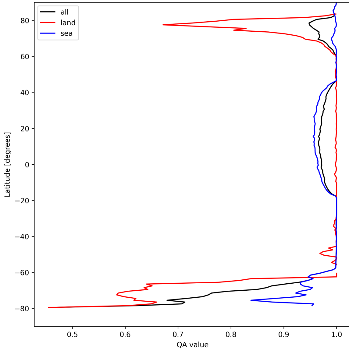
Figure 12: Zonal average of “QA value” for 2025-08-30 to 2025-08-31.
