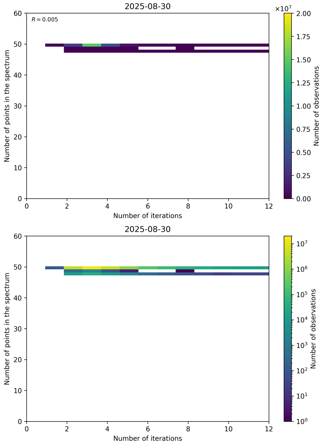
Figure 99: Scatter density plot of “Number of iterations” against “Number of points in the spectrum” for 2025-08-30 to 2025-08-31.
