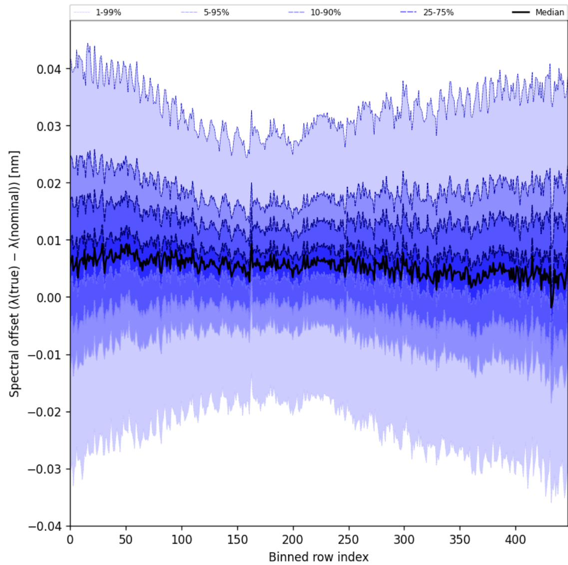
Figure 62: Along track statistics of “Spectral offset ( \lambda_{\text{true}} - \lambda_{\text{nominal}} )” for 2025-08-30 to 2025-08-31
