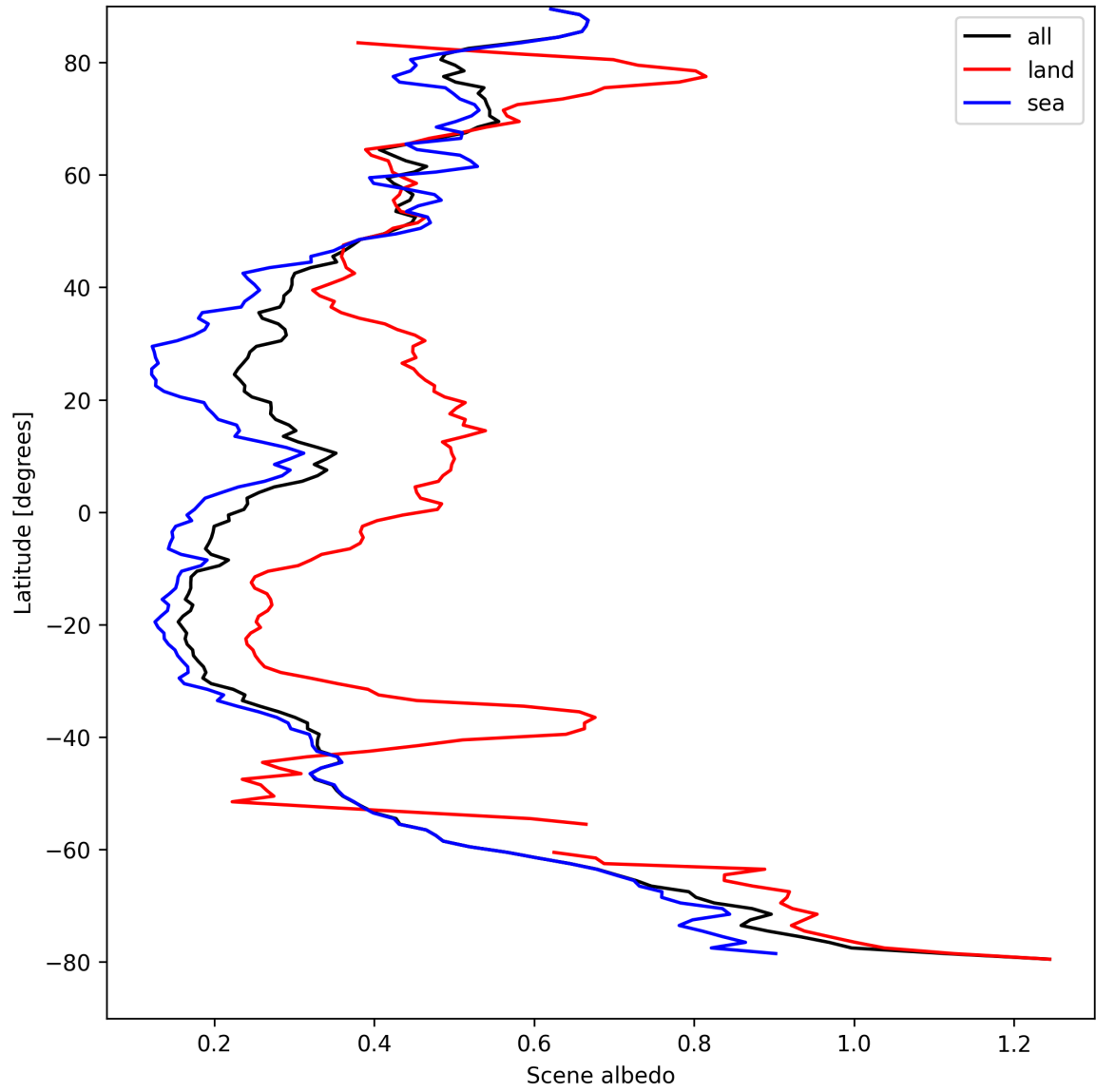
Figure 17: Zonal average of “Scene albedo” for 2025-08-30 to 2025-08-31.
