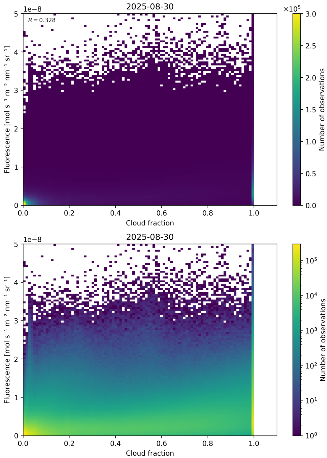
Figure 72: Scatter density plot of “Cloud fraction” against “Fluorescence” for 2025-08-30 to 2025-08-31.
