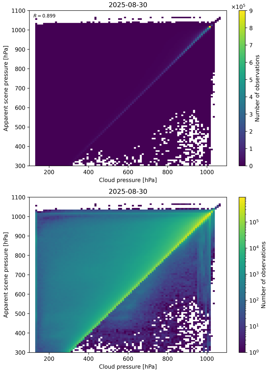
Figure 77: Scatter density plot of “Cloud pressure” against “Apparent scene pressure” for 2025-08-30 to 2025-08-31.
