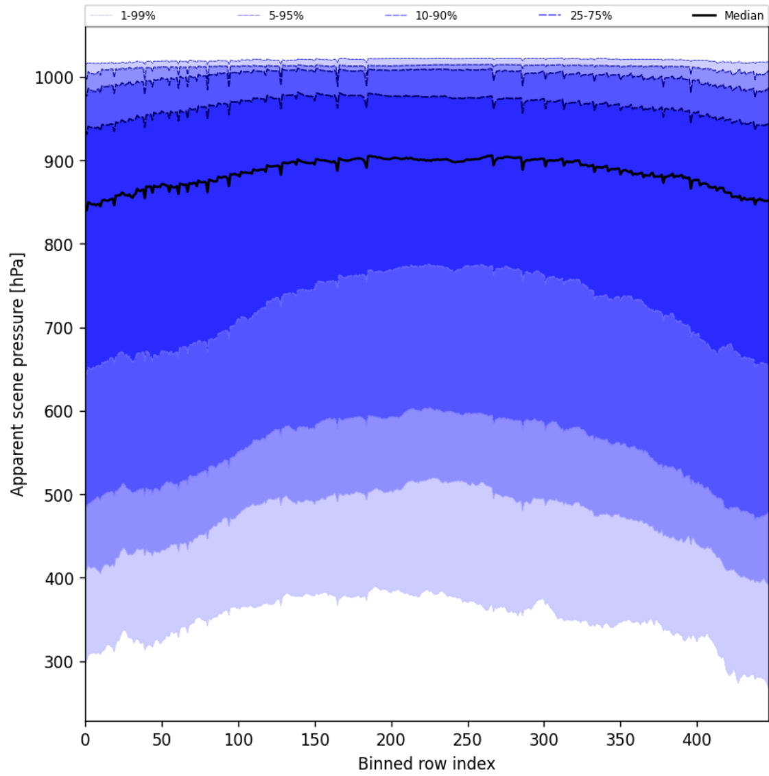
Figure 53: Along track statistics of “Apparent scene pressure” for 2025-08-30 to 2025-08-31
