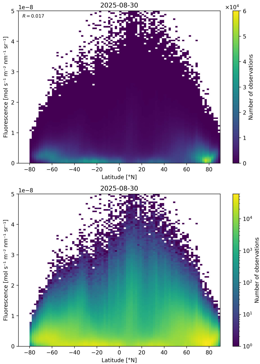
Figure 92: Scatter density plot of “Latitude” against “Fluorescence” for 2025-08-30 to 2025-08-31.
