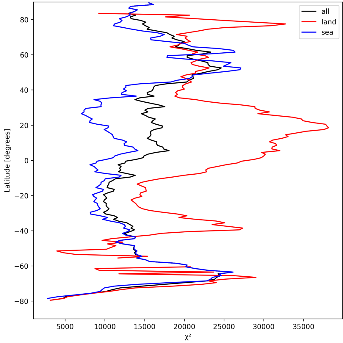
Figure 21: Zonal average of “ \chi^2 ” for 2025-08-30 to 2025-08-31.
