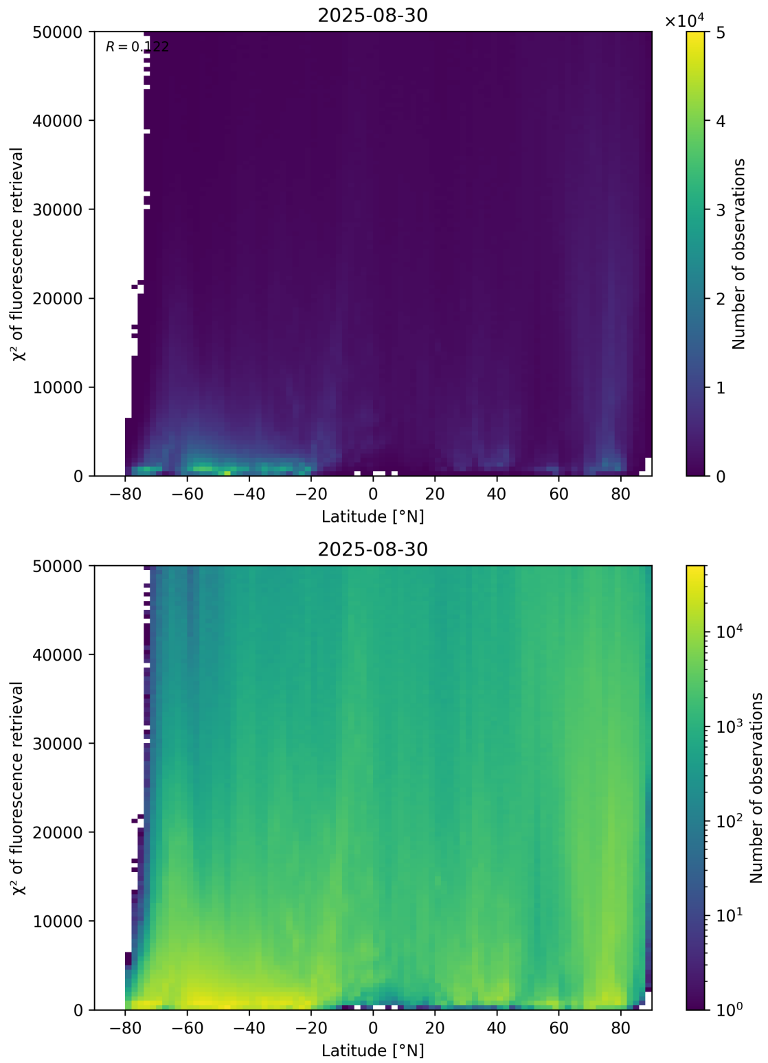
Figure 89: Scatter density plot of “Latitude” against “ \chi^2 of fluorescence retrieval” for 2025-08-30 to 2025-08-31.
