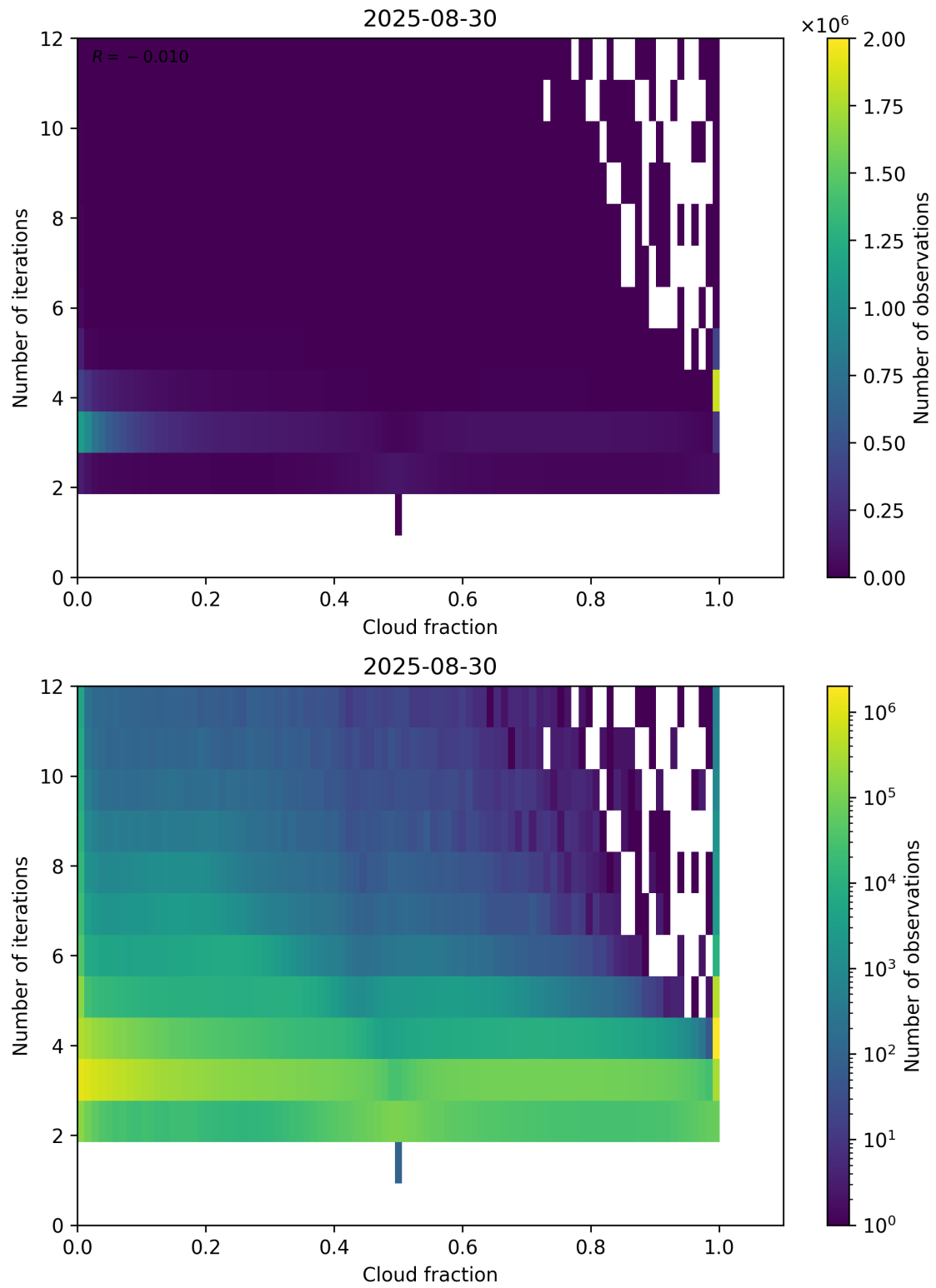
Figure 73: Scatter density plot of “Cloud fraction” against “Number of iterations” for 2025-08-30 to 2025-08-31.
