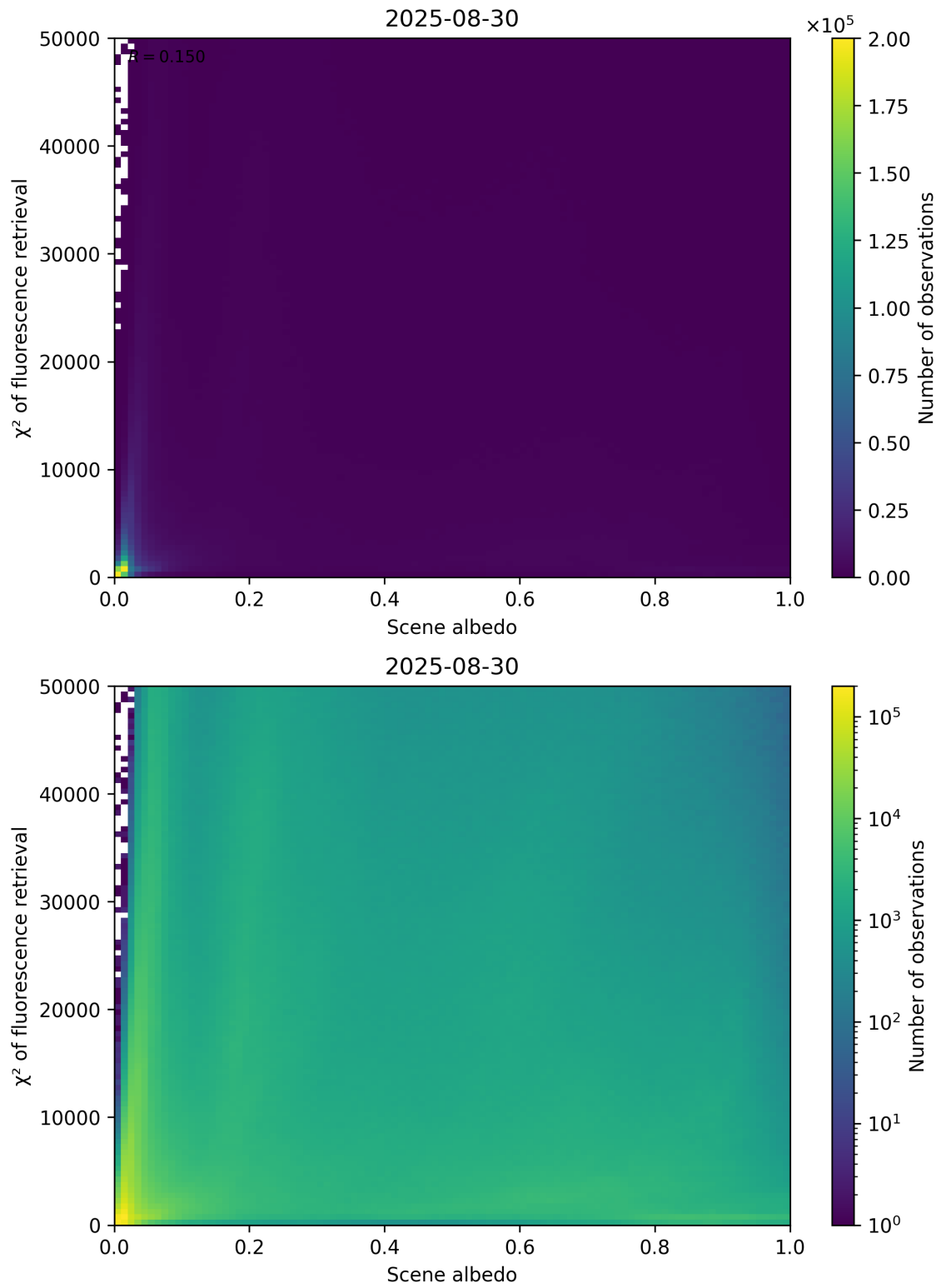
Figure 103: Scatter density plot of “Scene albedo” against “ \chi^2 of fluorescence retrieval” for 2025-08-30 to 2025-08-31.
