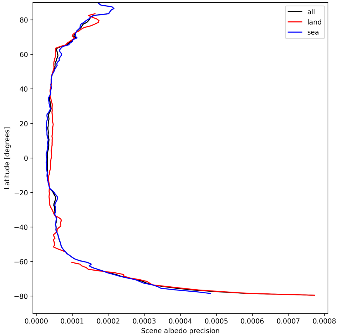
Figure 18: Zonal average of “Scene albedo precision” for 2025-08-30 to 2025-08-31.
