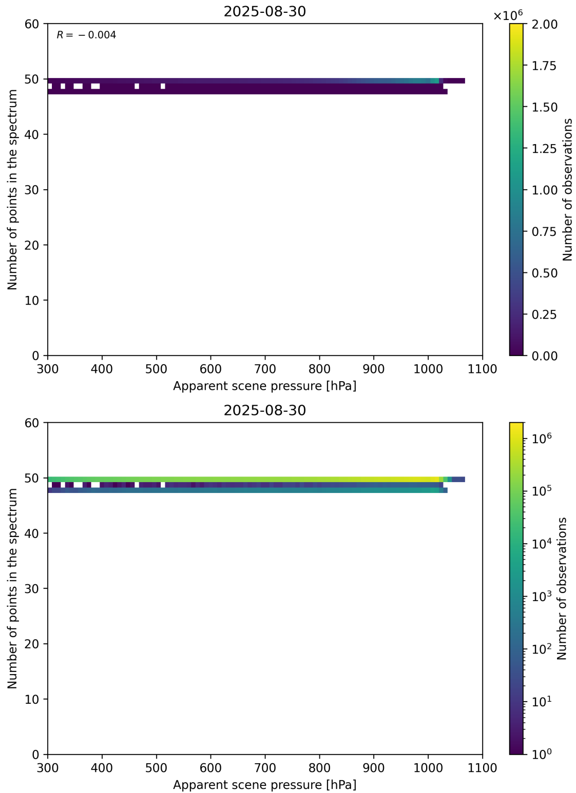
Figure 66: Scatter density plot of “Apparent scene pressure” against “Number of points in the spectrum” for 2025-08-30 to 2025-08-31.
