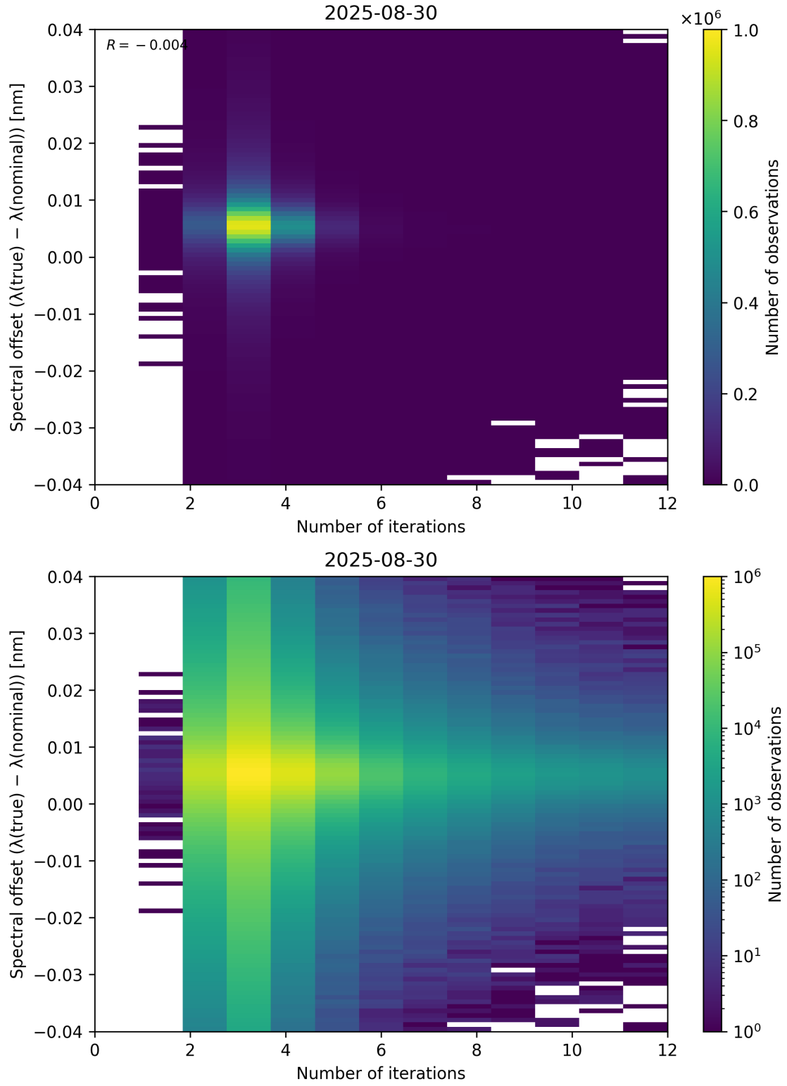
Figure 100: Scatter density plot of “Number of iterations” against “Spectral offset ( \lambda_{\text{true}} - \lambda_{\text{nominal}} )” for 2025-08-30 to 2025-08-31.
