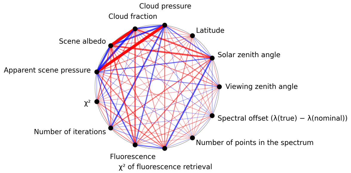
Figure 1: Map of correlation graph for 2025-08-30 to 2025-08-31.
