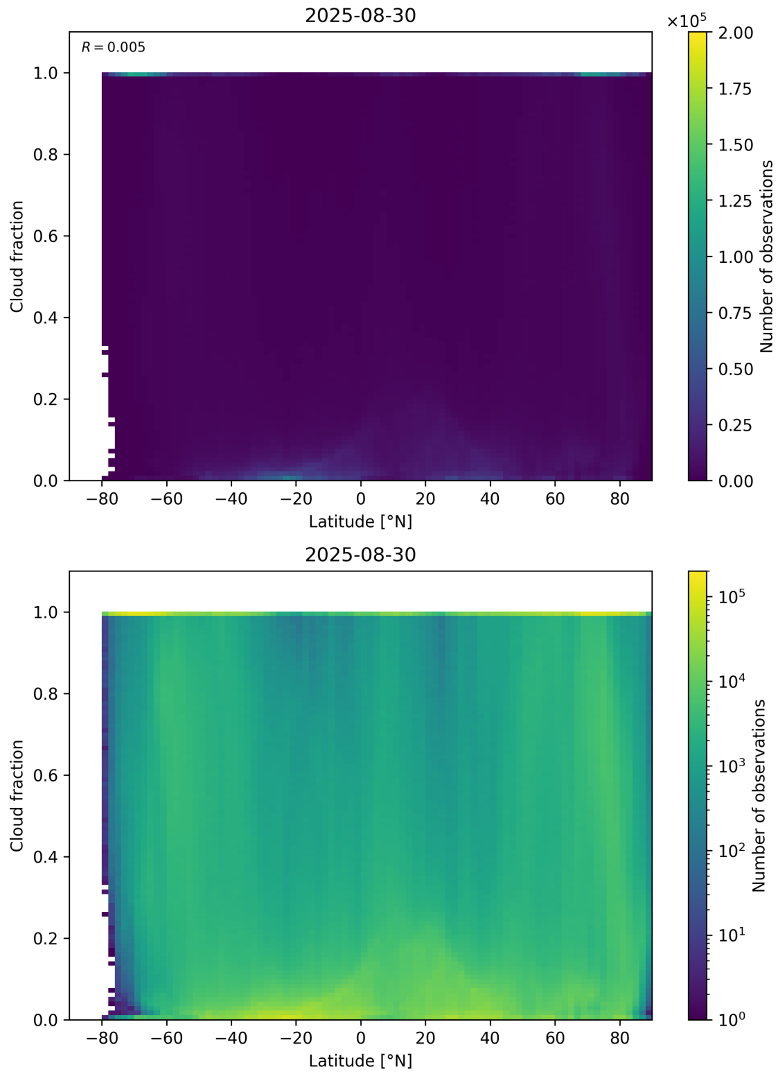
Figure 90: Scatter density plot of “Latitude” against “Cloud fraction” for 2025-08-30 to 2025-08-31.
