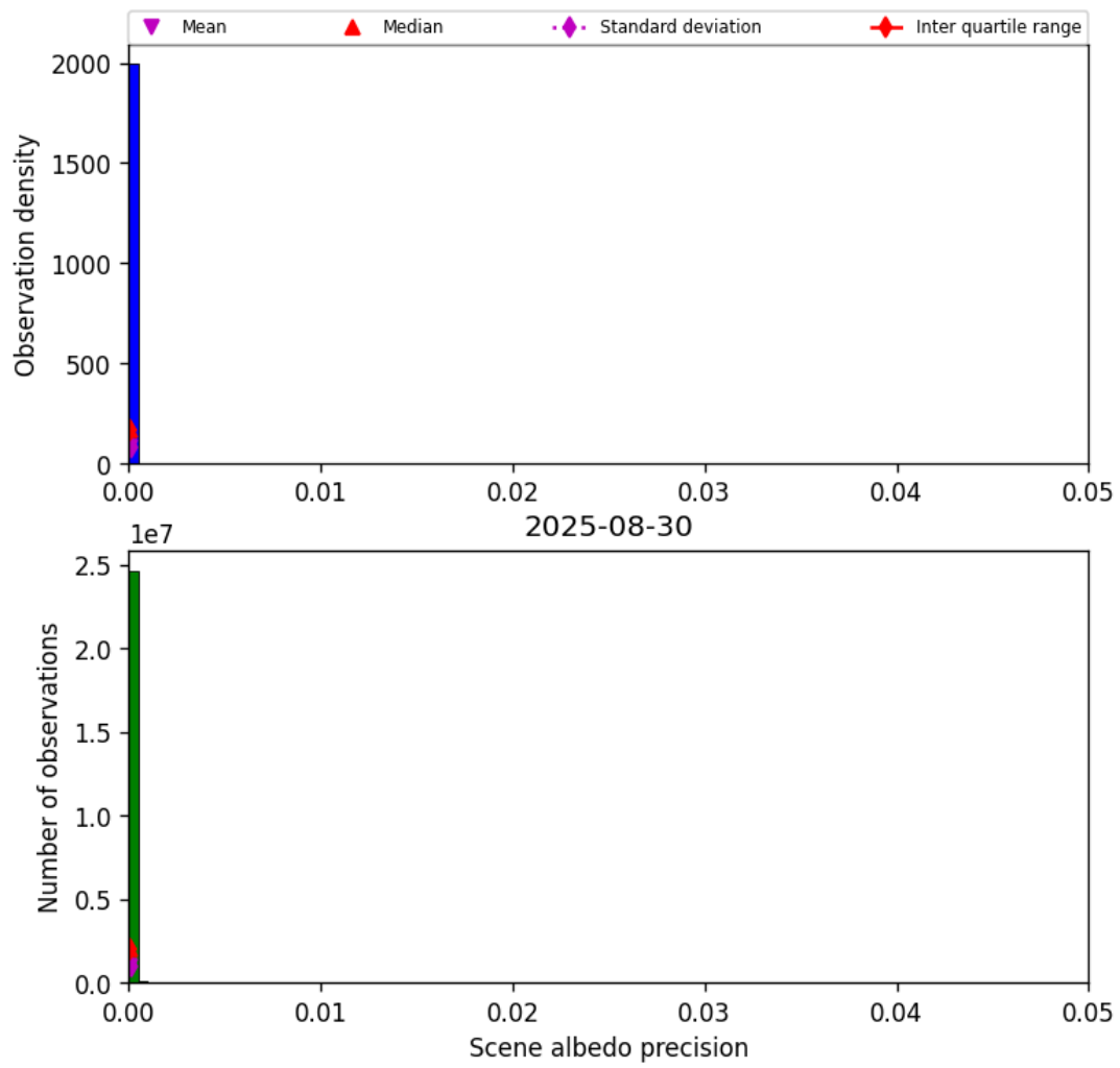
Figure 35: Histogram of “Scene albedo precision” for 2025-08-30 to 2025-08-31
