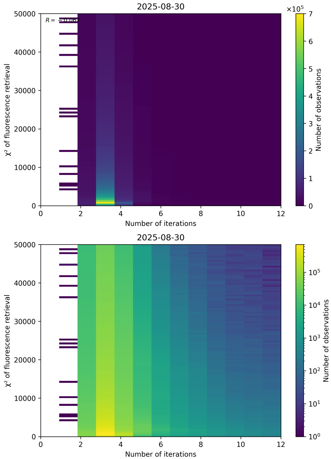
Figure 97: Scatter density plot of “Number of iterations” against “ \chi^2 of fluorescence retrieval” for 2025-08-30 to 2025-08-31.
