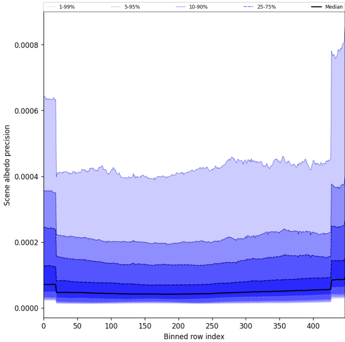
Figure 52: Along track statistics of “Scene albedo precision” for 2025-08-30 to 2025-08-31
