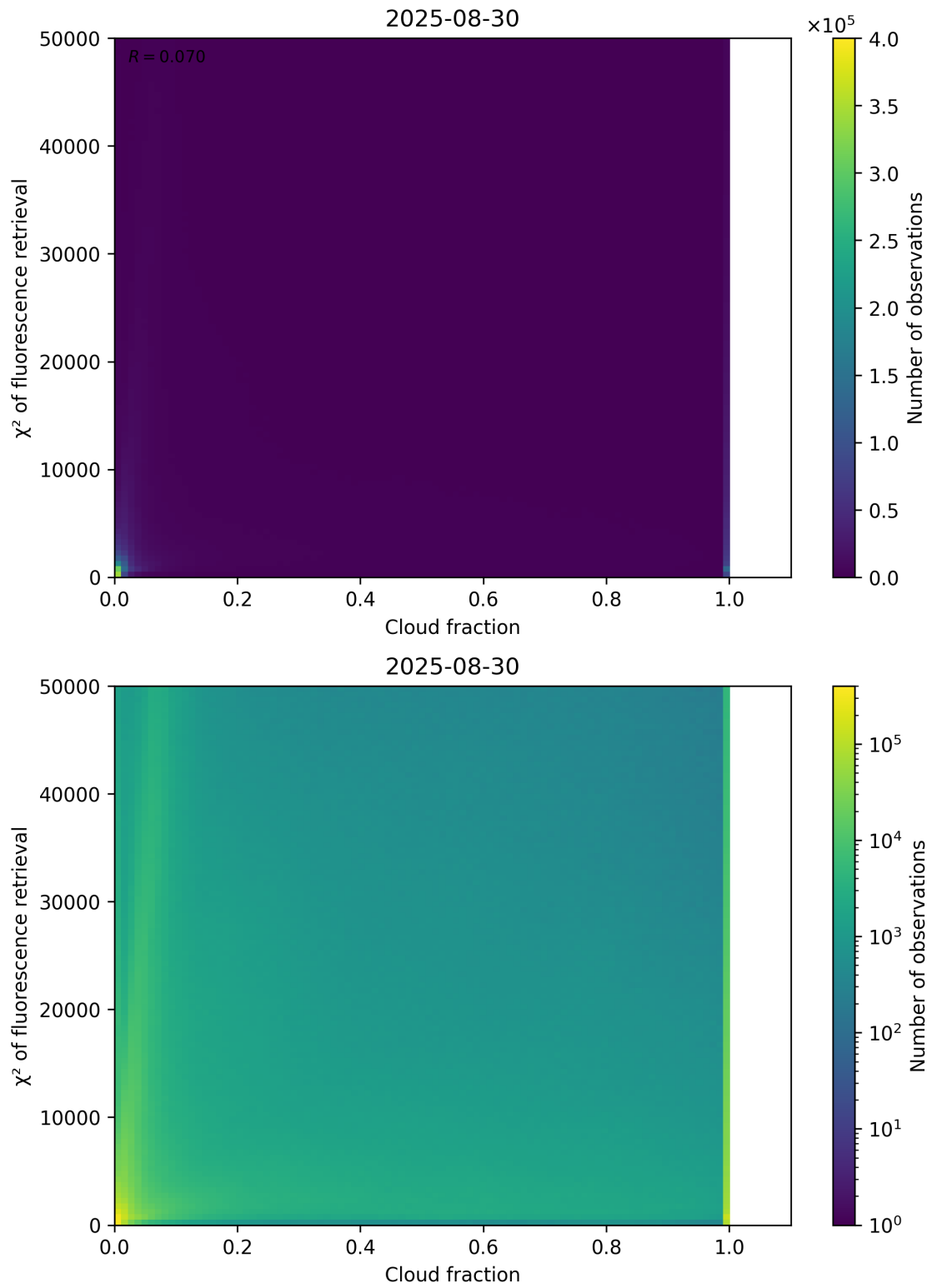
Figure 71: Scatter density plot of “Cloud fraction” against “ \chi^2 of fluorescence retrieval” for 2025-08-30 to 2025-08-31.
