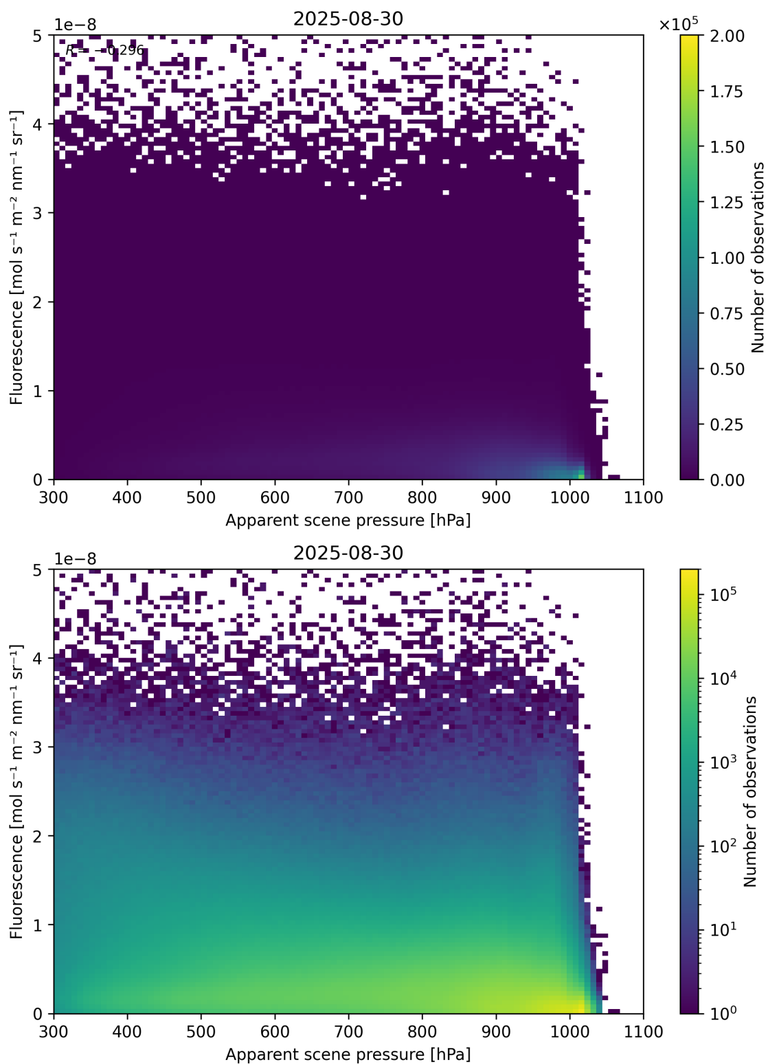
Figure 64: Scatter density plot of “Apparent scene pressure” against “Fluorescence” for 2025-08-30 to 2025-08-31.
