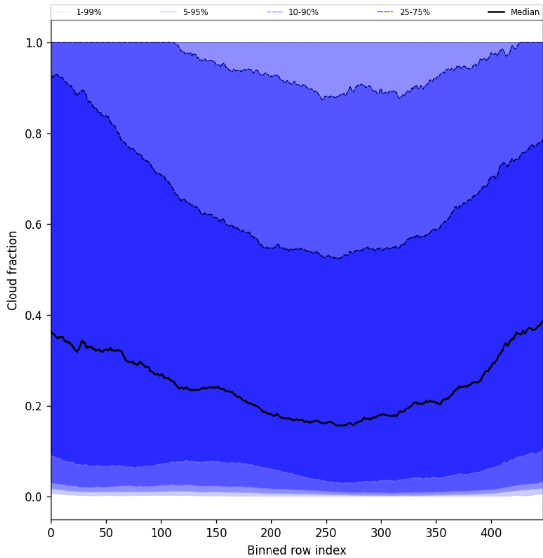
Figure 49: Along track statistics of “Cloud fraction” for 2025-08-30 to 2025-08-31
