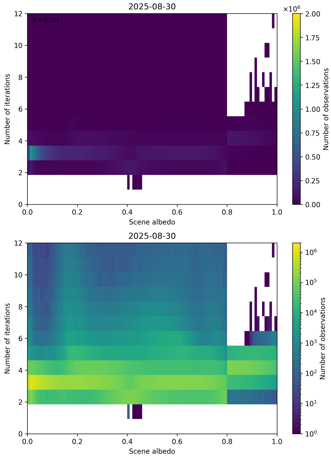
Figure 105: Scatter density plot of “Scene albedo” against “Number of iterations” for 2025-08-30 to 2025-08-31.
