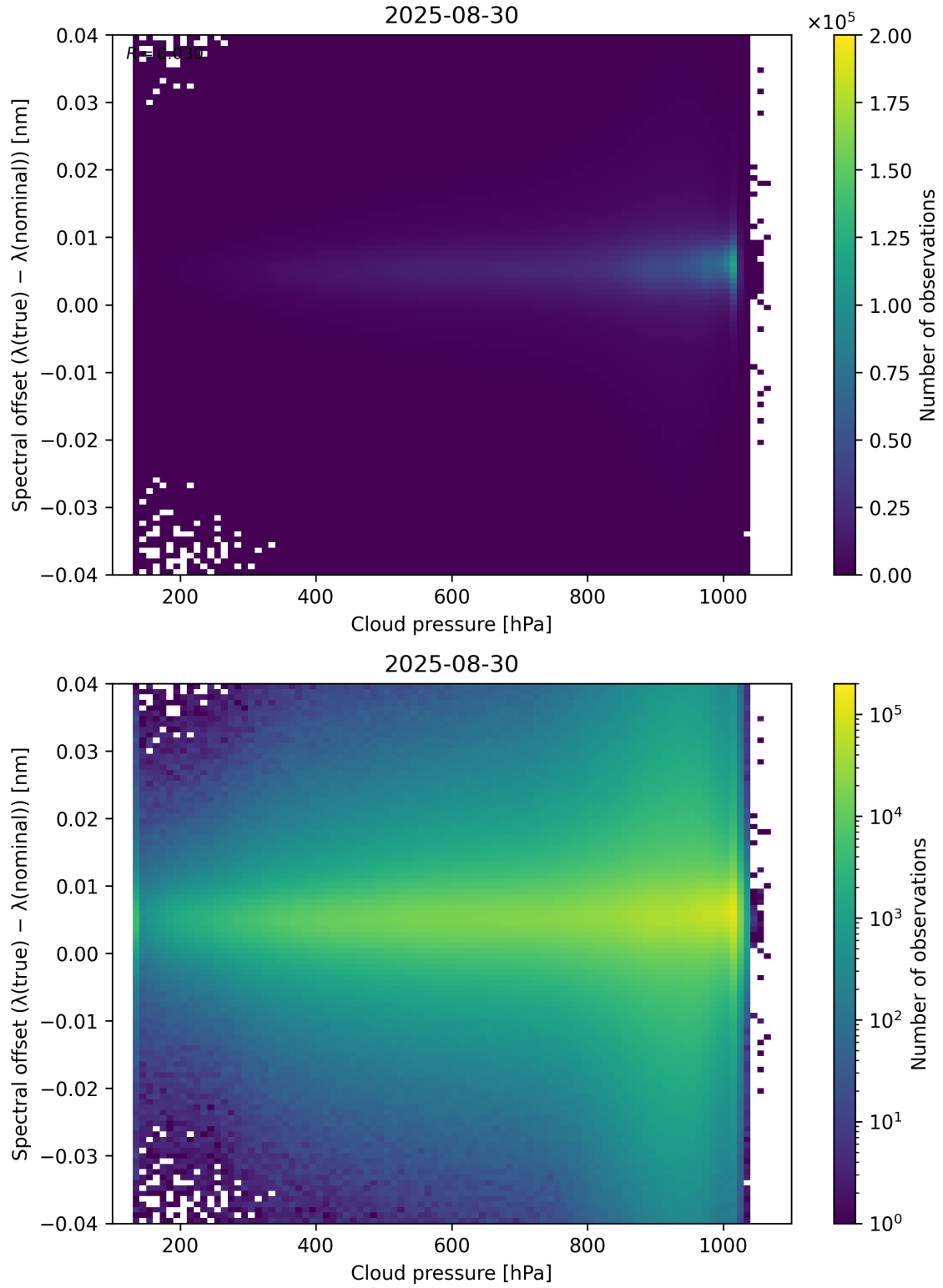
Figure 84: Scatter density plot of “Cloud pressure” against “Spectral offset ( \lambda_{\text{true}} - \lambda_{\text{nominal}} )” for 2025-08-30 to 2025-08-31.
