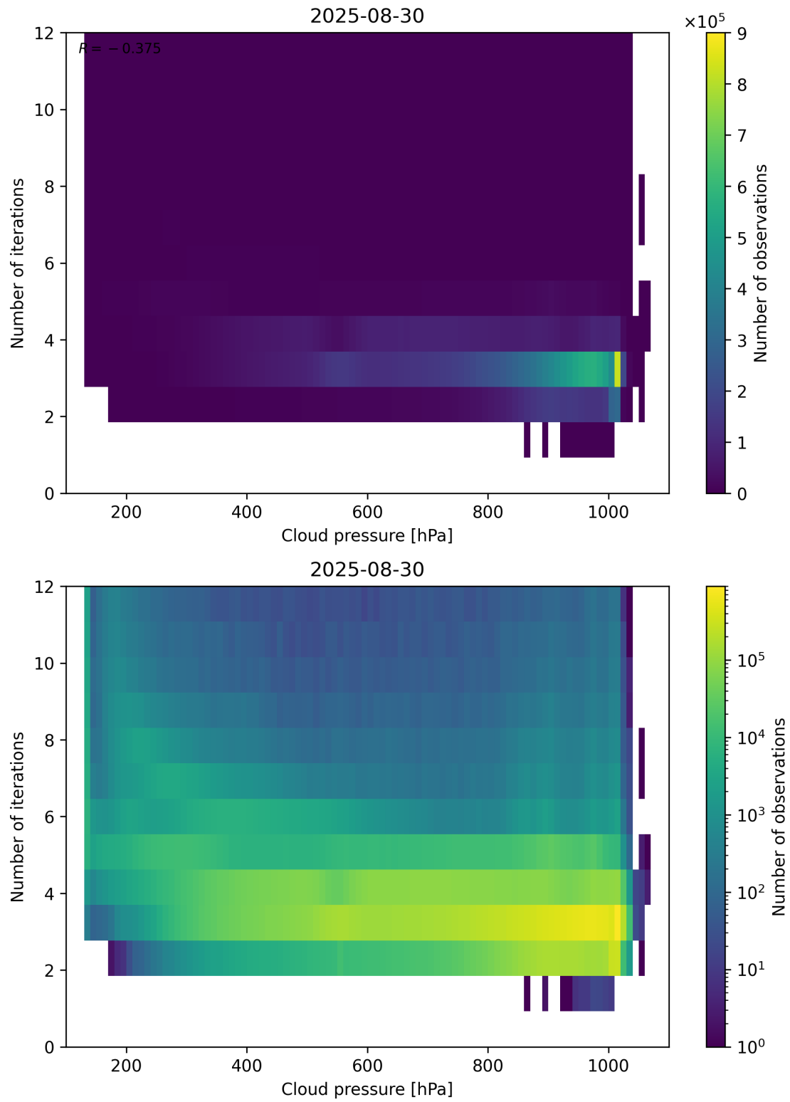
Figure 81: Scatter density plot of “Cloud pressure” against “Number of iterations” for 2025-08-30 to 2025-08-31.
