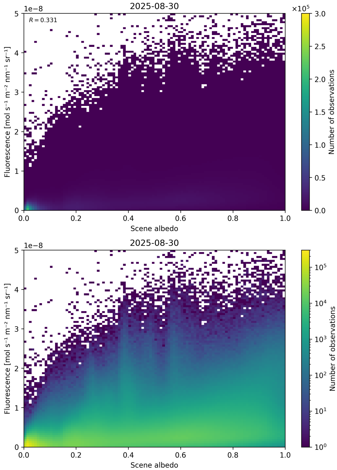
Figure 104: Scatter density plot of “Scene albedo” against “Fluorescence” for 2025-08-30 to 2025-08-31.
