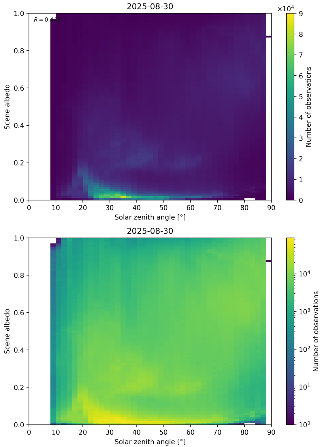
Figure 116: Scatter density plot of “Solar zenith angle” against “Scene albedo” for 2025-08-30 to 2025-08-31.
