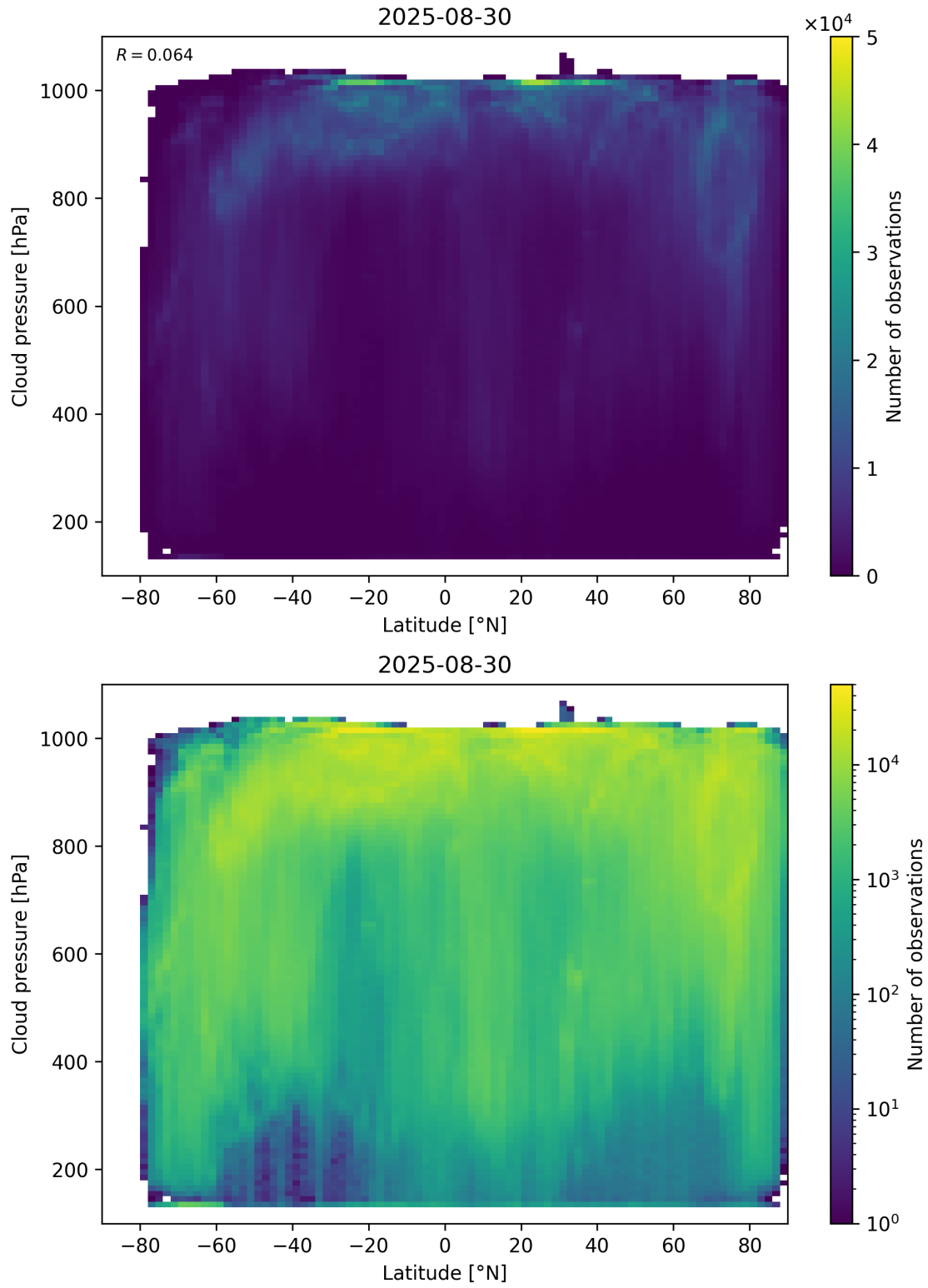
Figure 91: Scatter density plot of “Latitude” against “Cloud pressure” for 2025-08-30 to 2025-08-31.
