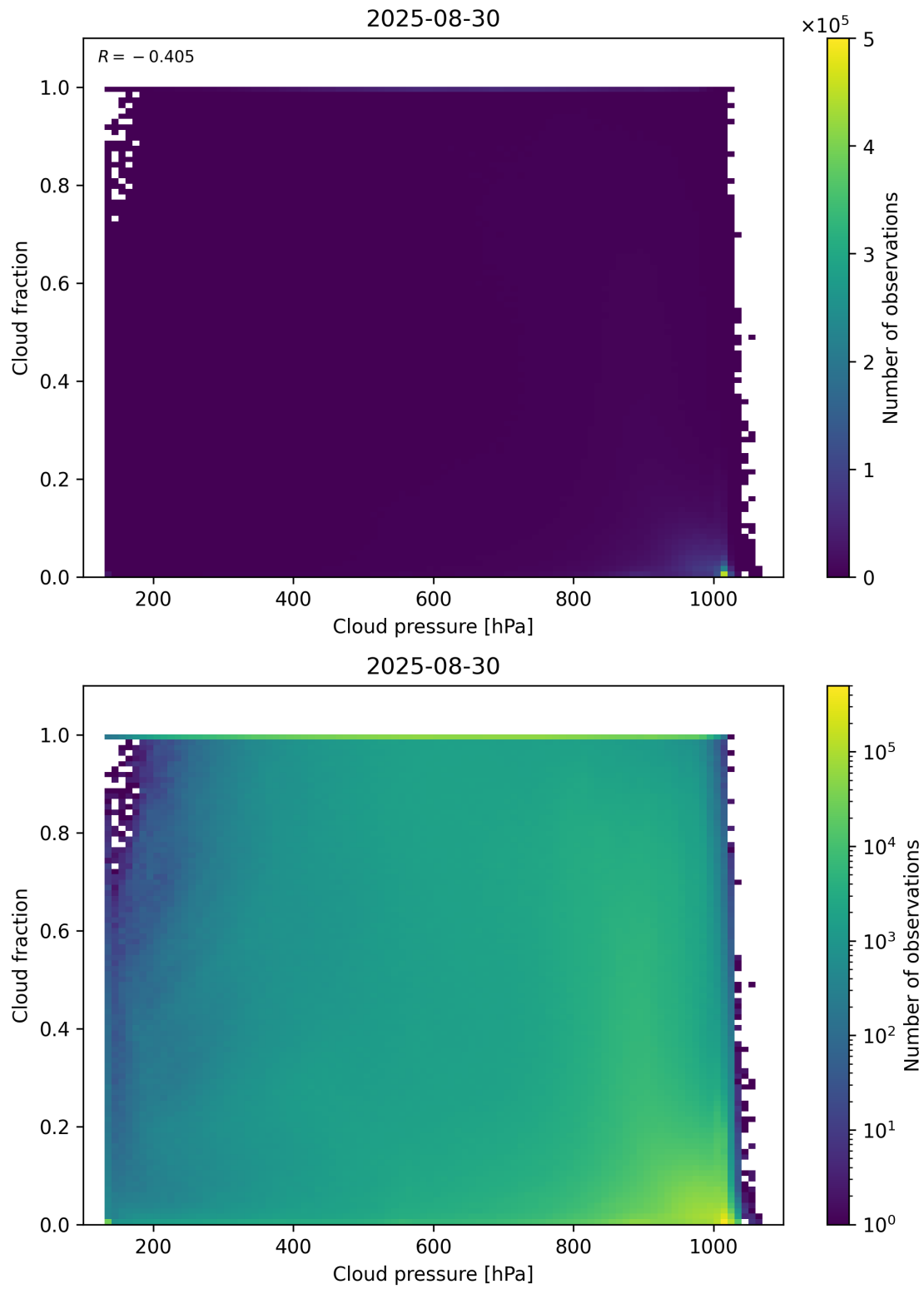
Figure 79: Scatter density plot of “Cloud pressure” against “Cloud fraction” for 2025-08-30 to 2025-08-31.
