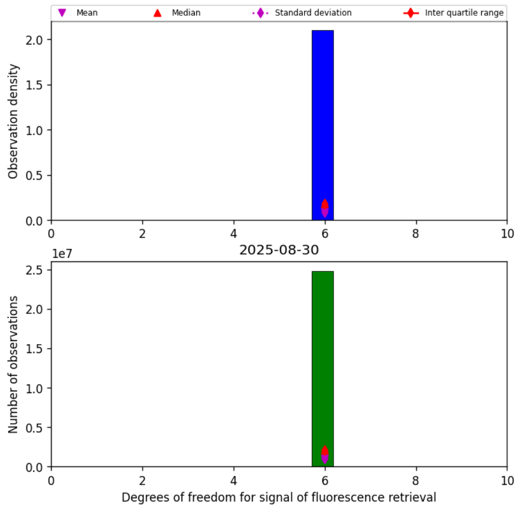
Figure 43: Histogram of “Degrees of freedom for signal of fluorescence retrieval” for 2025-08-30 to 2025-08-31
