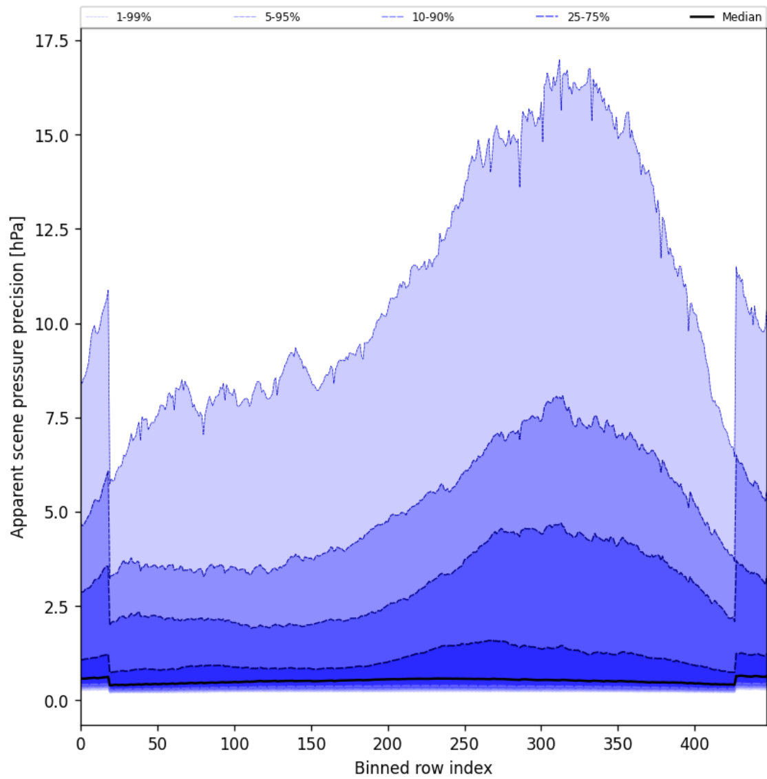
Figure 54: Along track statistics of “Apparent scene pressure precision” for 2025-08-30 to 2025-08-31
