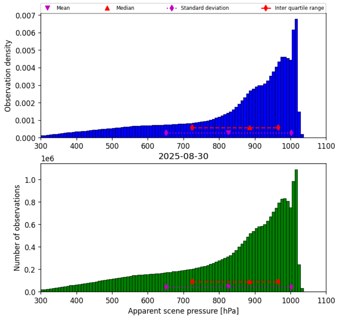
Figure 36: Histogram of “Apparent scene pressure” for 2025-08-30 to 2025-08-31
