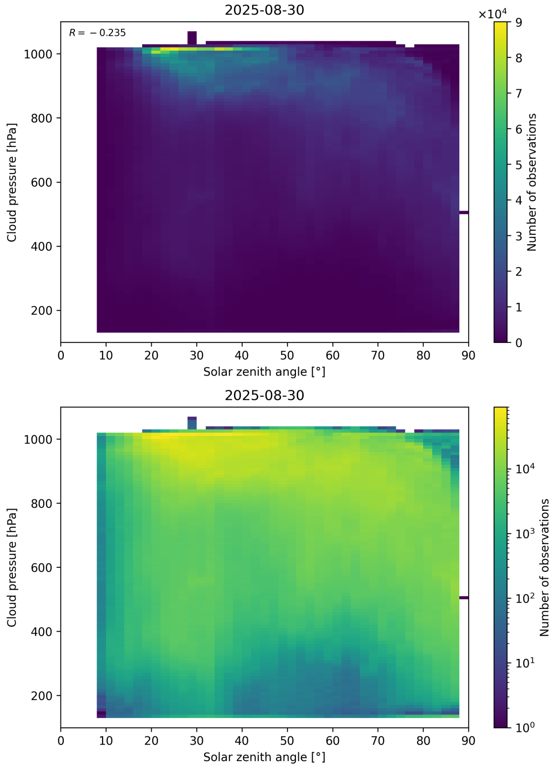
Figure 111: Scatter density plot of “Solar zenith angle” against “Cloud pressure” for 2025-08-30 to 2025-08-31.
