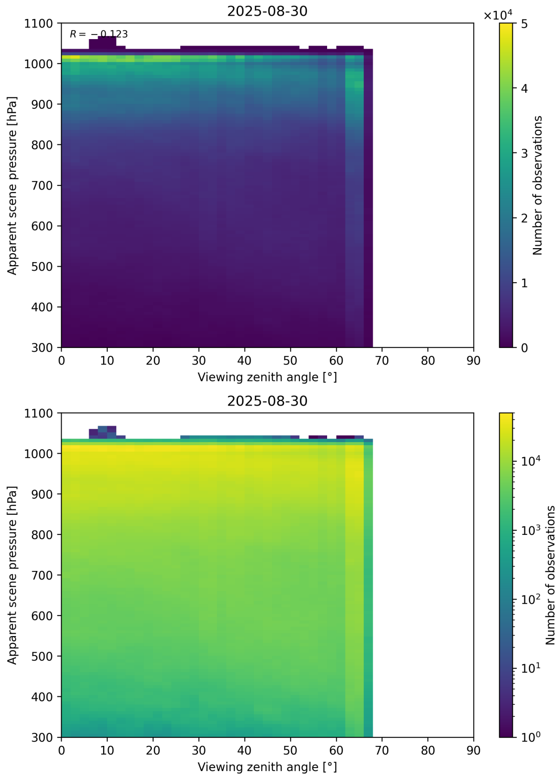
Figure 118: Scatter density plot of “Viewing zenith angle” against “Apparent scene pressure” for 2025-08-30 to 2025-08-31.
