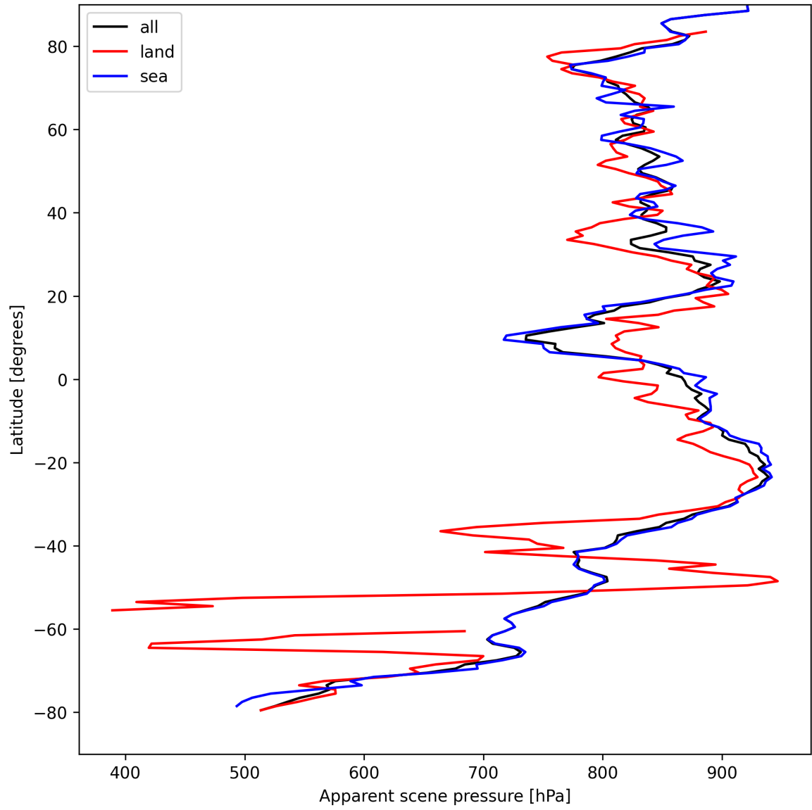
Figure 19: Zonal average of “Apparent scene pressure” for 2025-08-30 to 2025-08-31.
