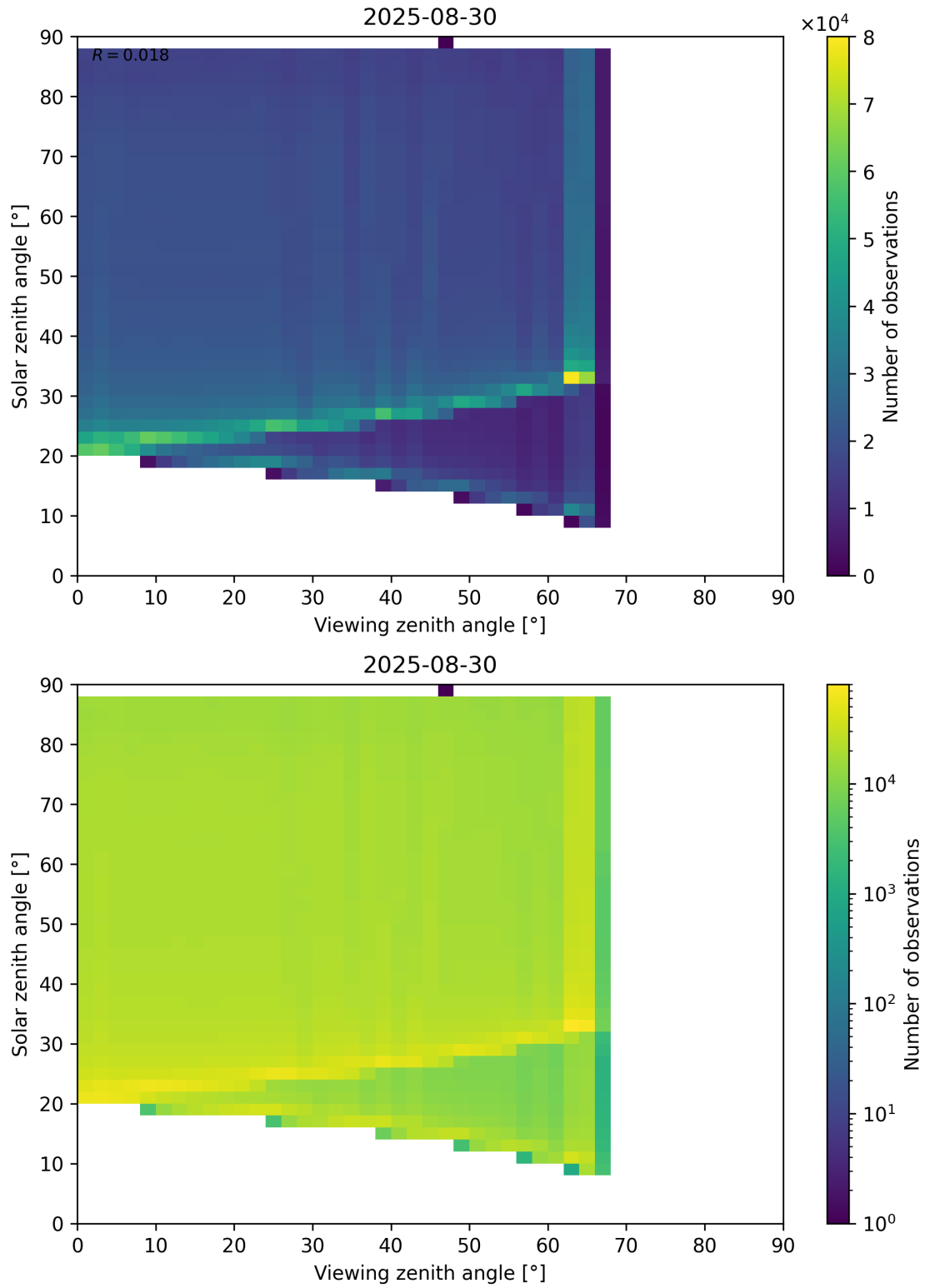
Figure 127: Scatter density plot of “Viewing zenith angle” against “Solar zenith angle” for 2025-08-30 to 2025-08-31.
