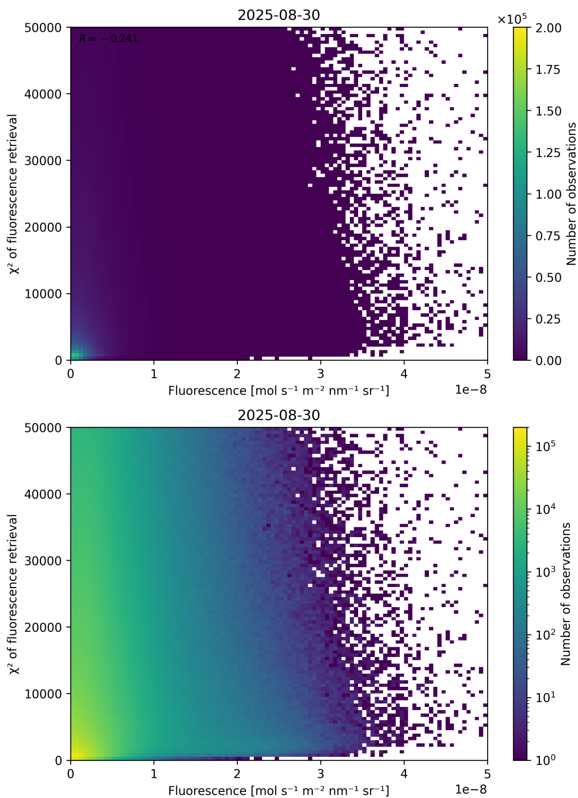
Figure 85: Scatter density plot of “Fluorescence” against “ \chi^2 of fluorescence retrieval” for 2025-08-30 to 2025-08-31.
