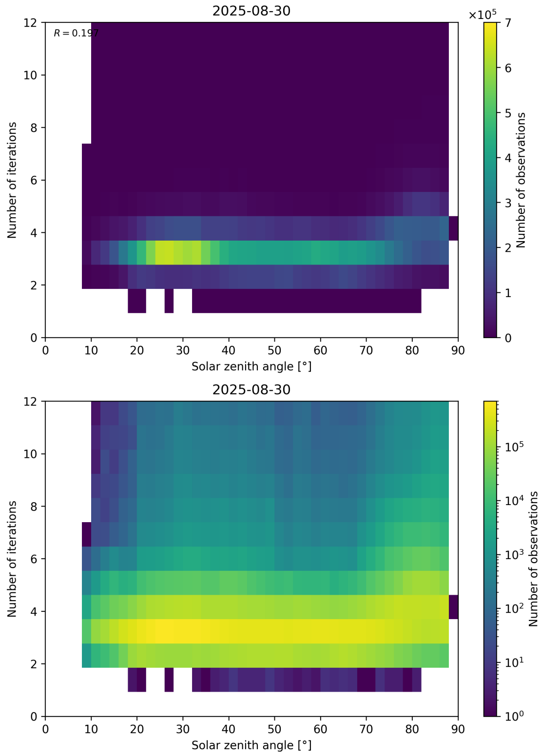
Figure 114: Scatter density plot of “Solar zenith angle” against “Number of iterations” for 2025-08-30 to 2025-08-31.
