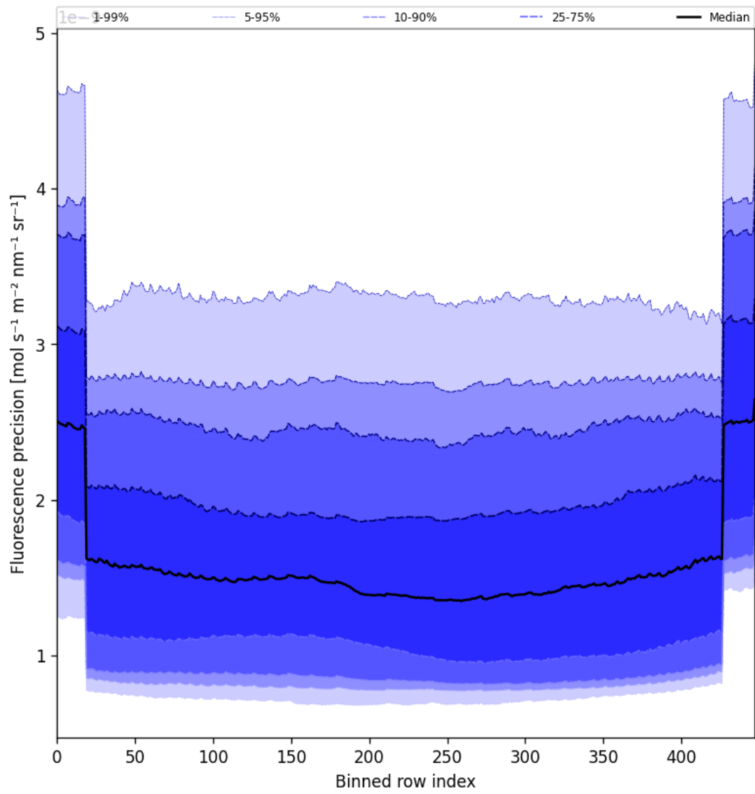
Figure 58: Along track statistics of “Fluorescence precision” for 2025-08-30 to 2025-08-31
