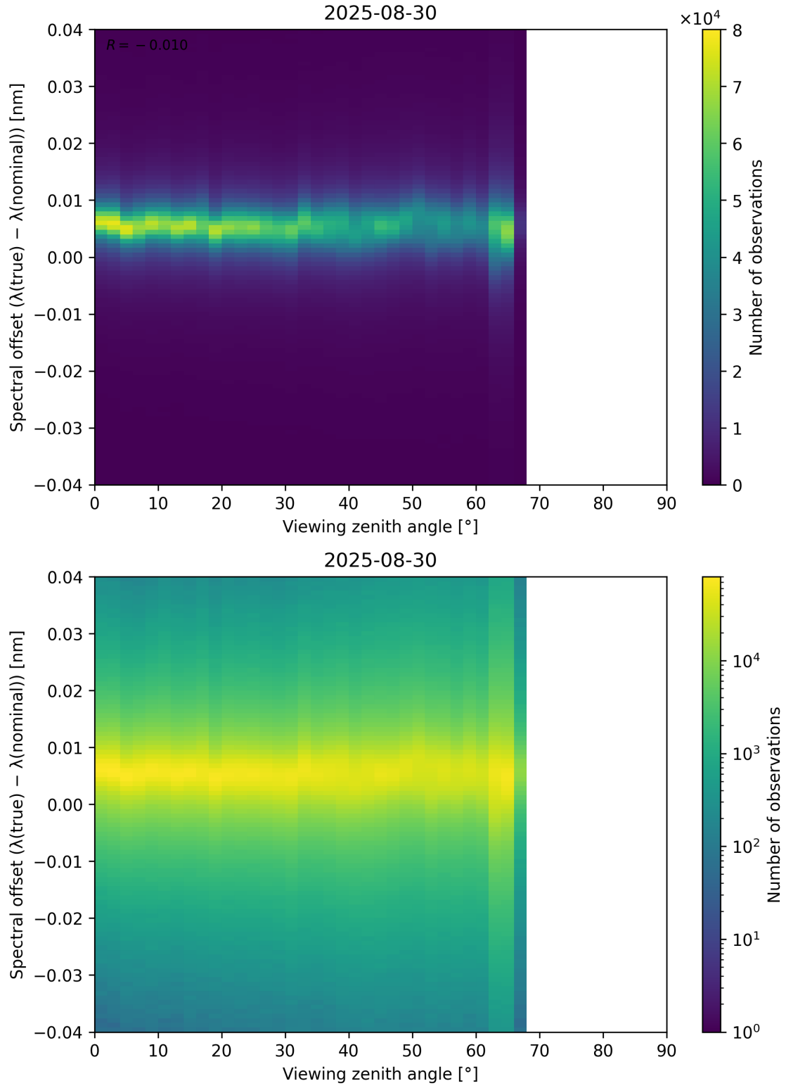
Figure 128: Scatter density plot of “Viewing zenith angle” against “Spectral offset ( \lambda_{\text{true}} - \lambda_{\text{nominal}} )” for 2025-08-30 to 2025-08-31.
