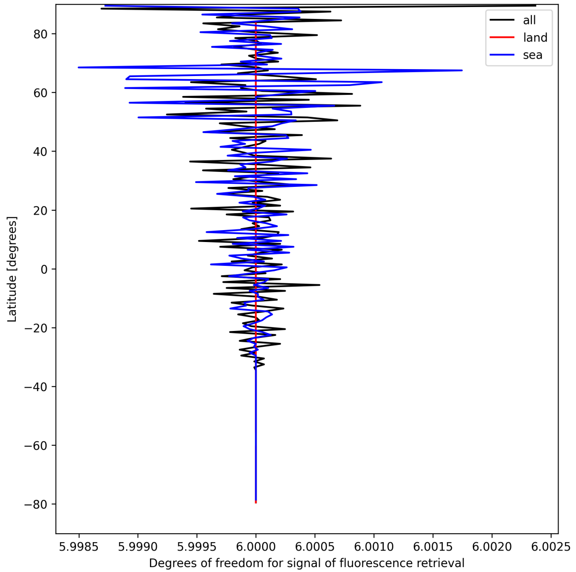
Figure 26: Zonal average of “Degrees of freedom for signal of fluorescence retrieval” for 2025-08-30 to 2025-08-31.
