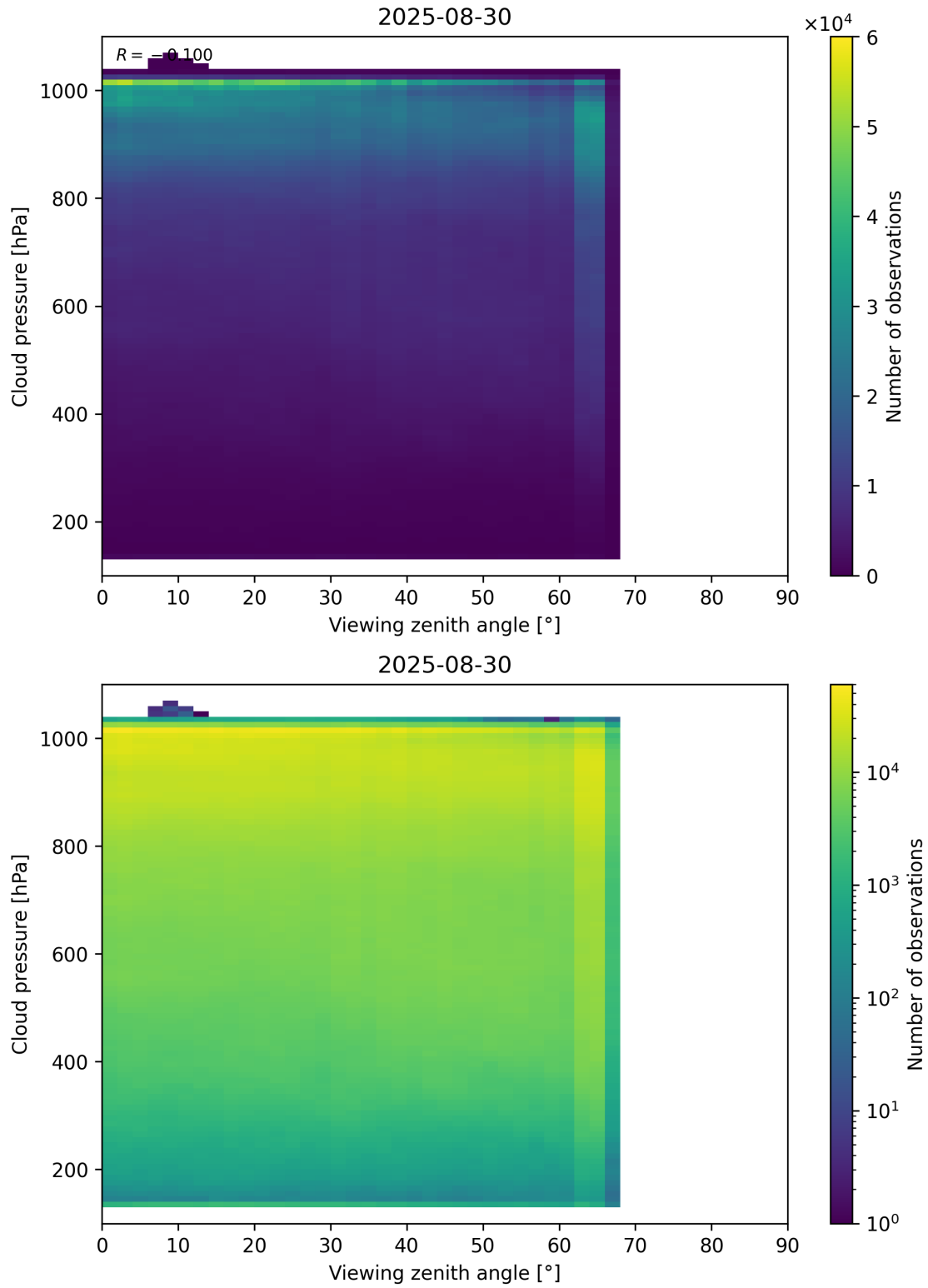
Figure 121: Scatter density plot of “Viewing zenith angle” against “Cloud pressure” for 2025-08-30 to 2025-08-31.
