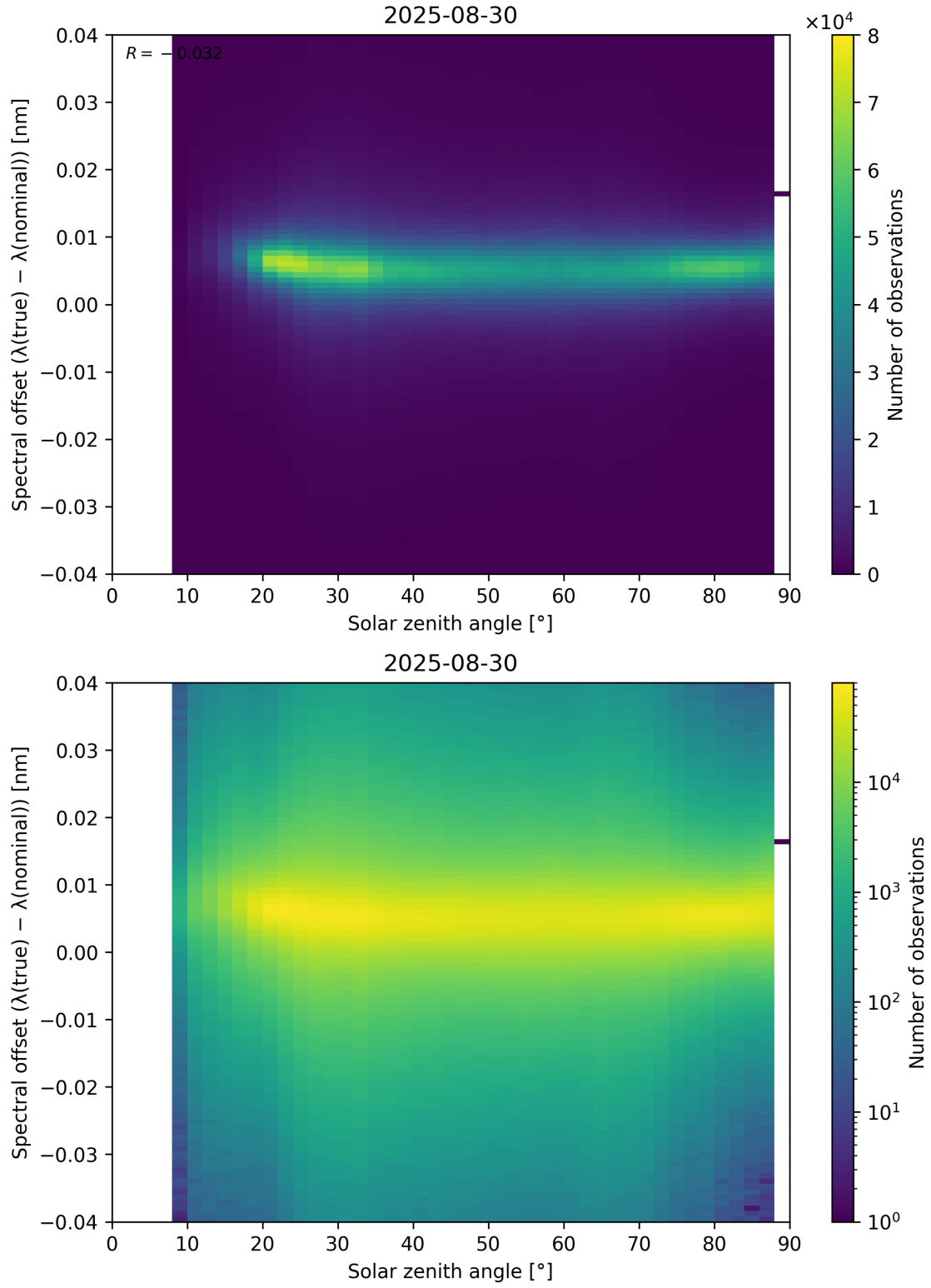
Figure 117: Scatter density plot of “Solar zenith angle” against “Spectral offset ( \lambda_{\text{true}} - \lambda_{\text{nominal}} )” for 2025-08-30 to 2025-08-31.
