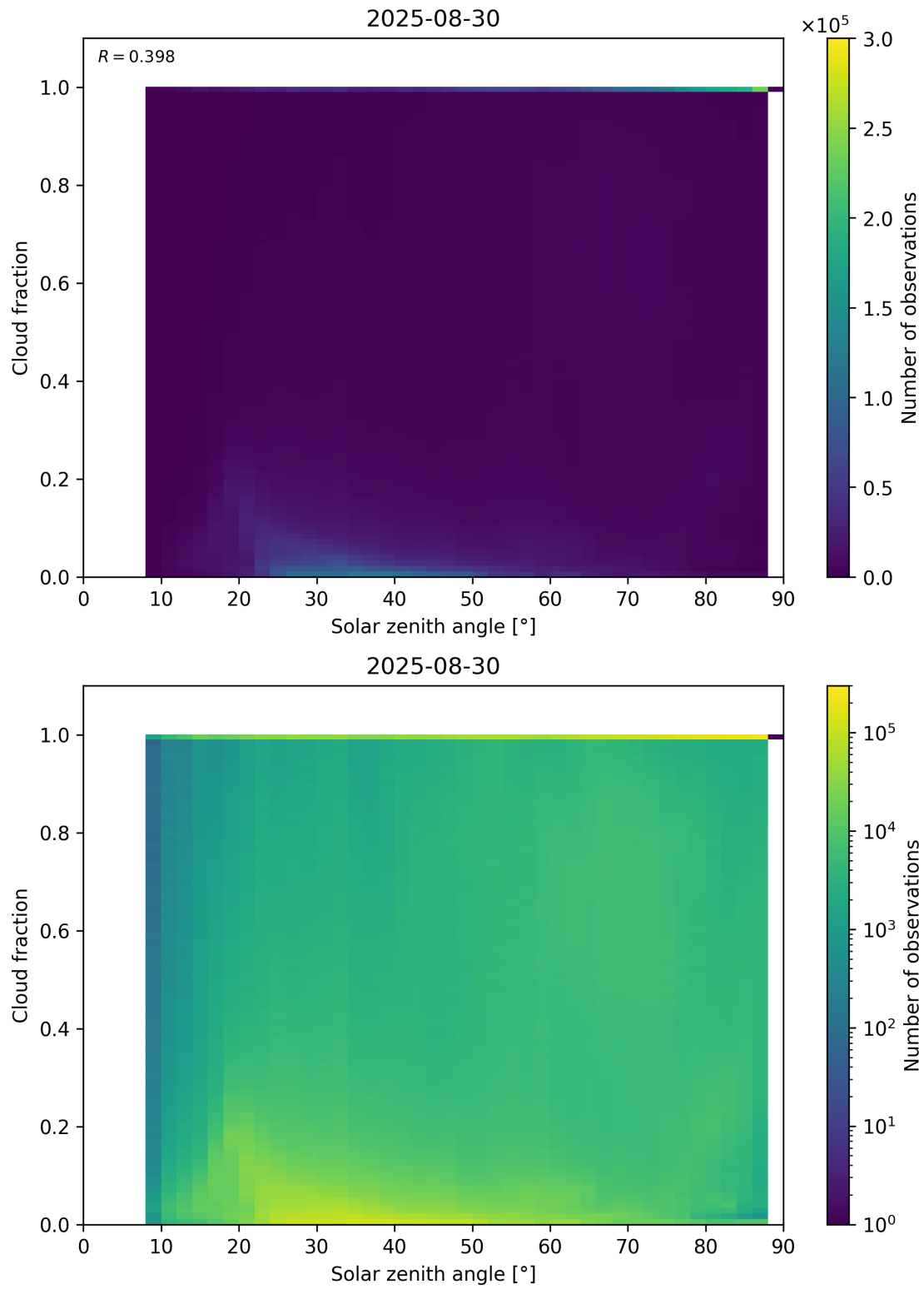
Figure 110: Scatter density plot of “Solar zenith angle” against “Cloud fraction” for 2025-08-30 to 2025-08-31.
