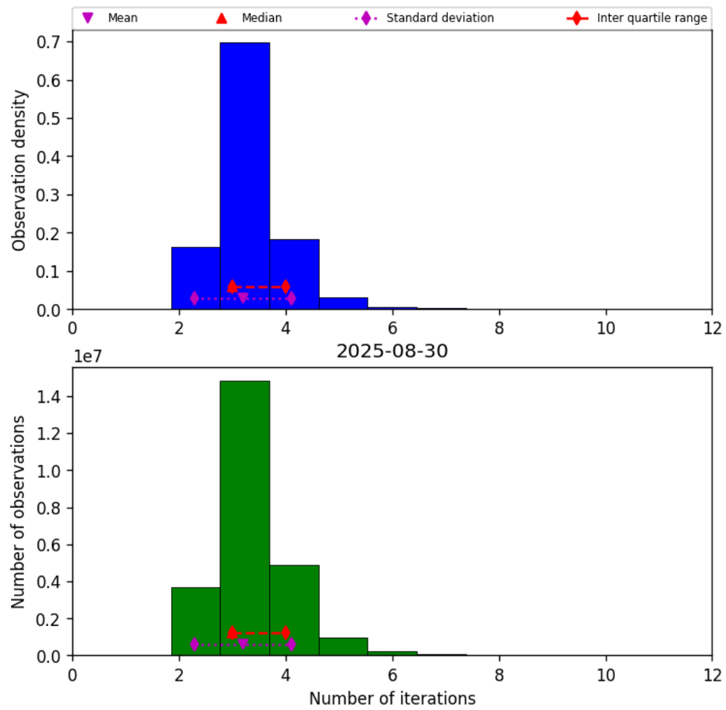
Figure 39: Histogram of “Number of iterations” for 2025-08-30 to 2025-08-31
