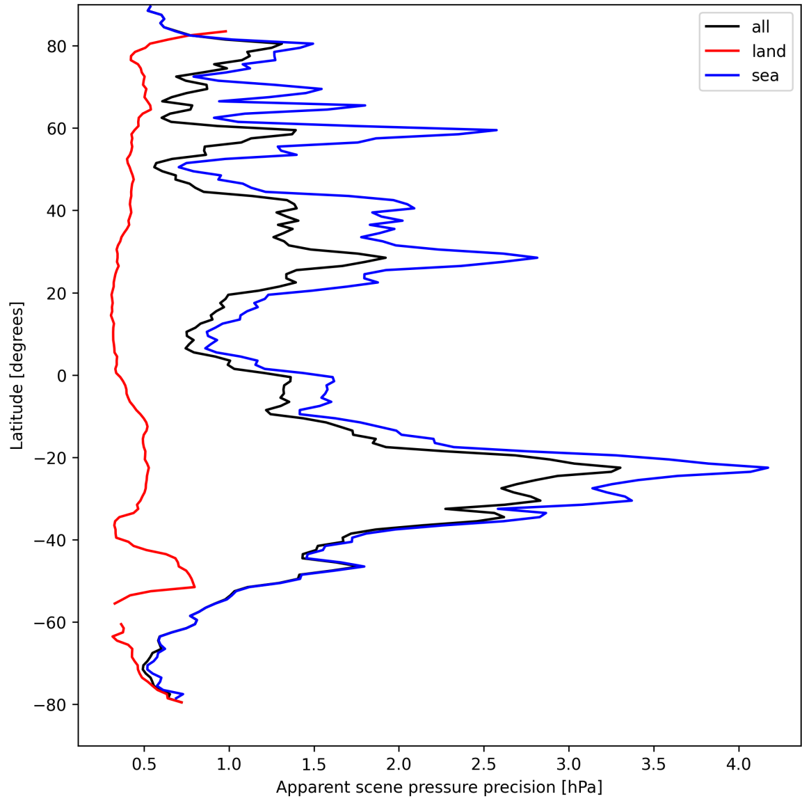
Figure 20: Zonal average of “Apparent scene pressure precision” for 2025-08-30 to 2025-08-31.
