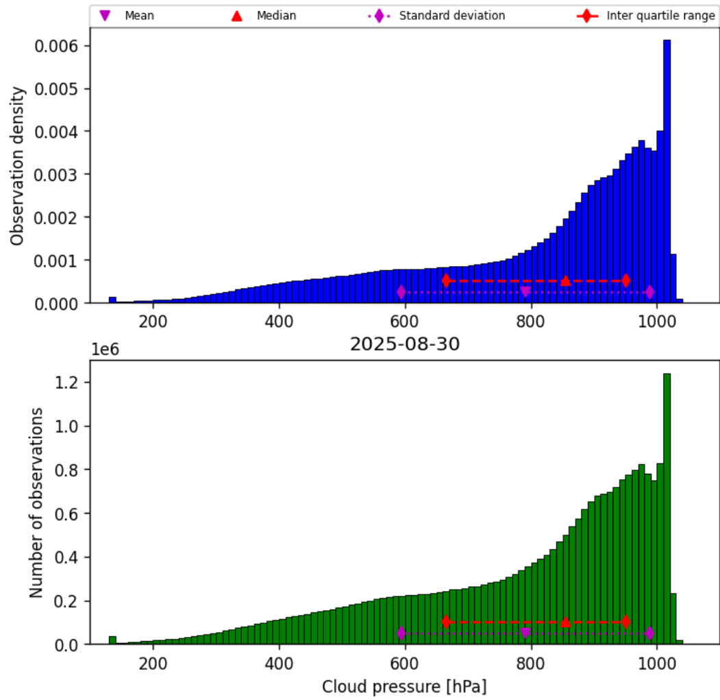
Figure 30: Histogram of “Cloud pressure” for 2025-08-30 to 2025-08-31
