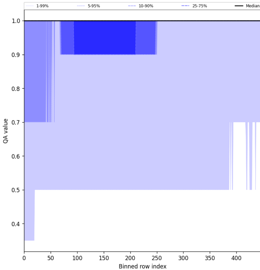
Figure 46: Along track statistics of “QA value” for 2025-08-30 to 2025-08-31
