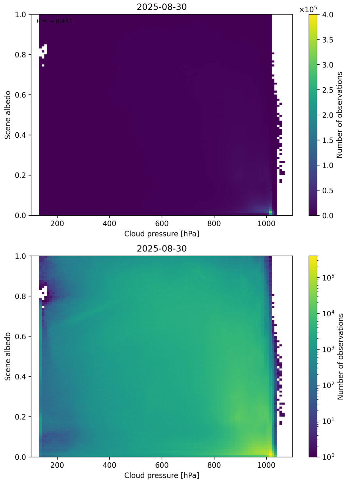
Figure 83: Scatter density plot of “Cloud pressure” against “Scene albedo” for 2025-08-30 to 2025-08-31.
