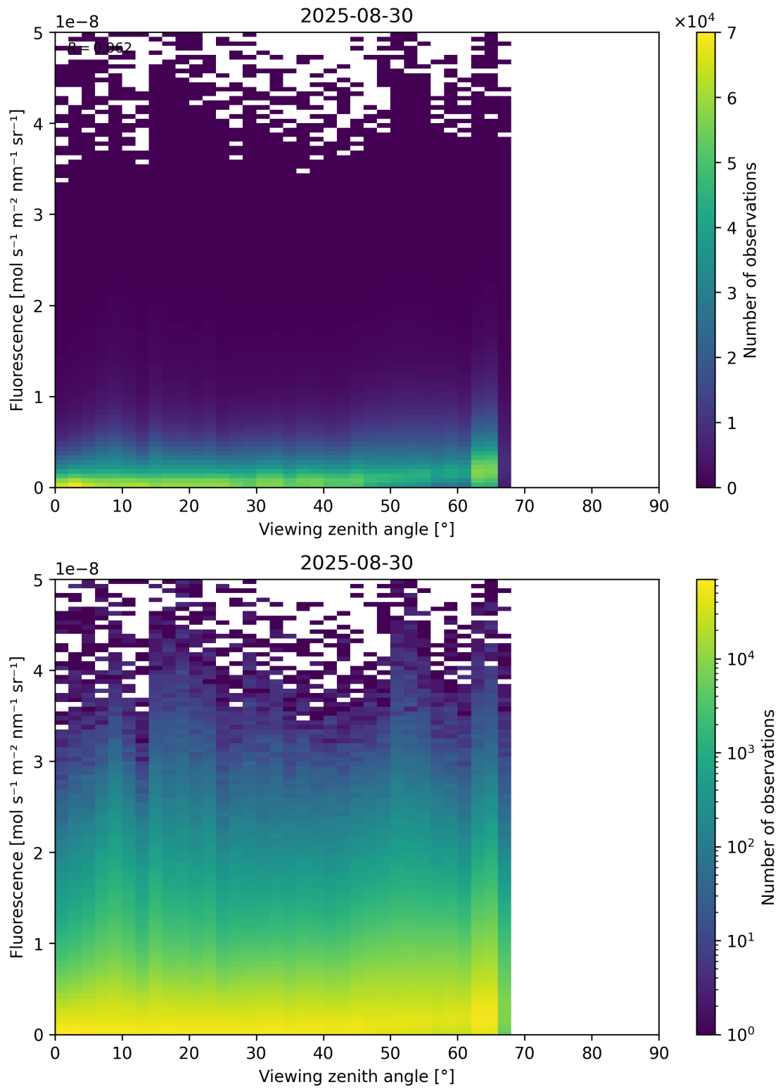
Figure 122: Scatter density plot of “Viewing zenith angle” against “Fluorescence” for 2025-08-30 to 2025-08-31.
