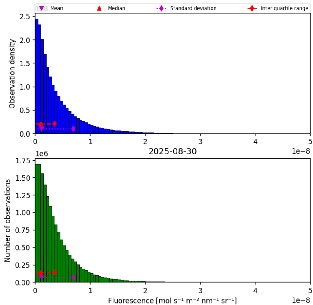
Figure 40: Histogram of “Fluorescence” for 2025-08-30 to 2025-08-31
