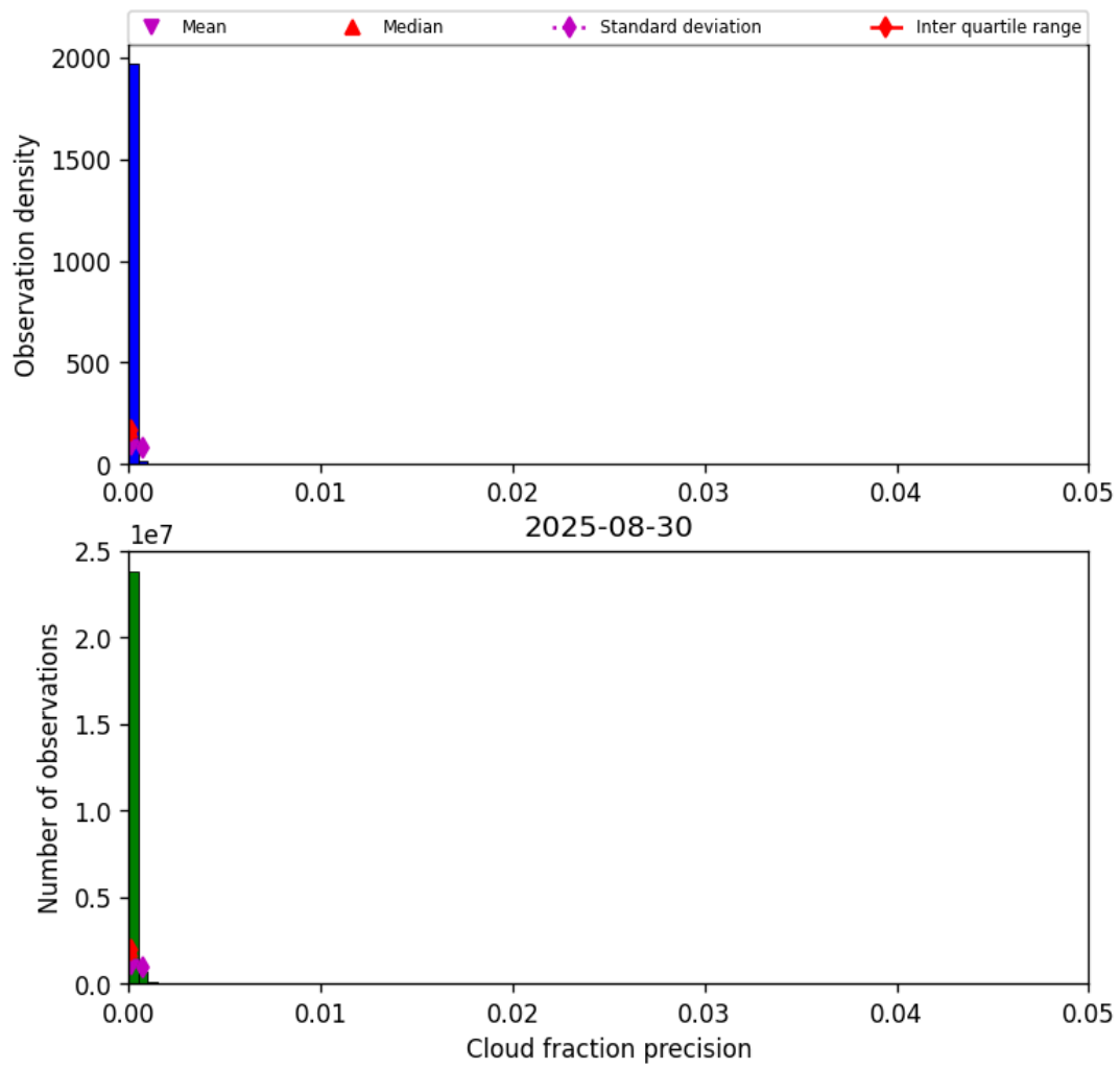
Figure 33: Histogram of “Cloud fraction precision” for 2025-08-30 to 2025-08-31
