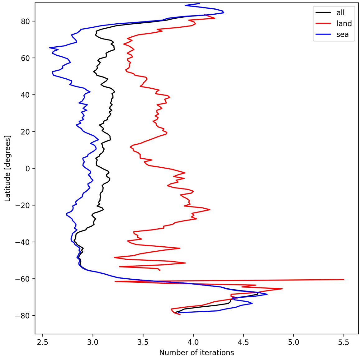
Figure 22: Zonal average of “Number of iterations” for 2025-08-30 to 2025-08-31.
