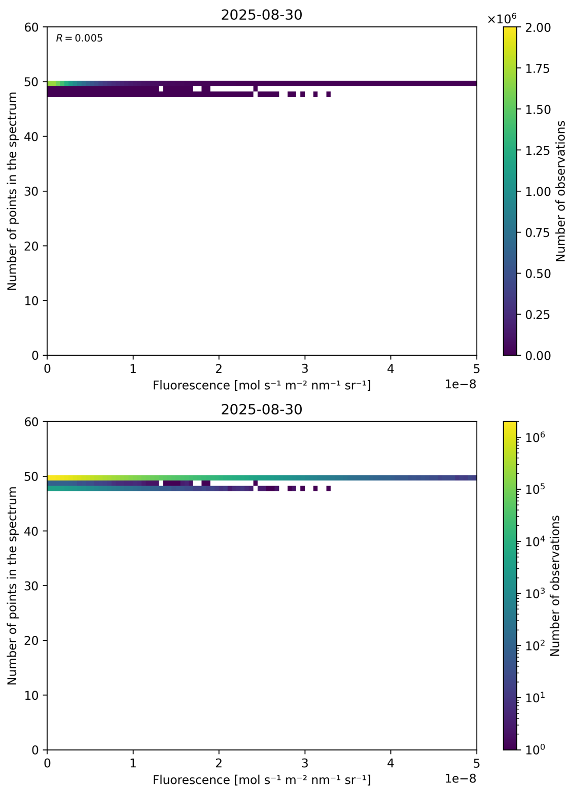
Figure 86: Scatter density plot of “Fluorescence” against “Number of points in the spectrum” for 2025-08-30 to 2025-08-31.
