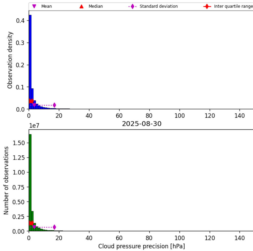
Figure 31: Histogram of “Cloud pressure precision” for 2025-08-30 to 2025-08-31
