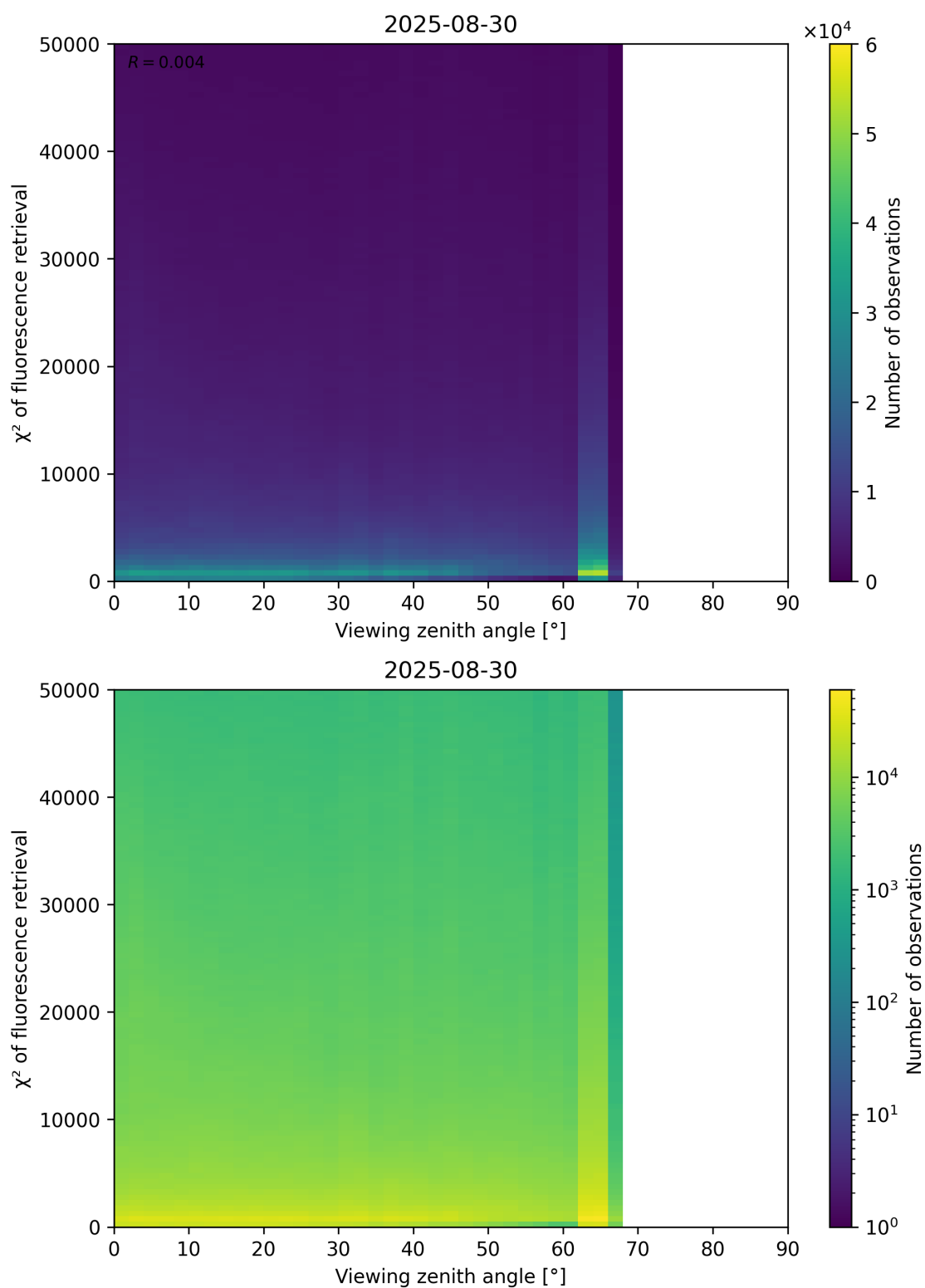
Figure 119: Scatter density plot of “Viewing zenith angle” against “ \chi^2 of fluorescence retrieval” for 2025-08-30 to 2025-08-31.
