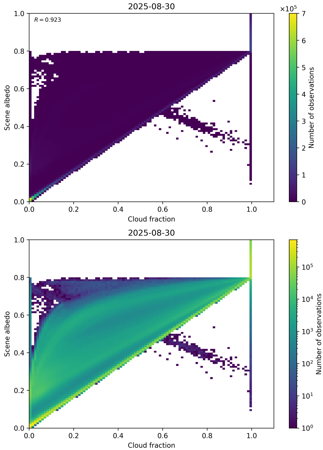
Figure 75: Scatter density plot of “Cloud fraction” against “Scene albedo” for 2025-08-30 to 2025-08-31.
