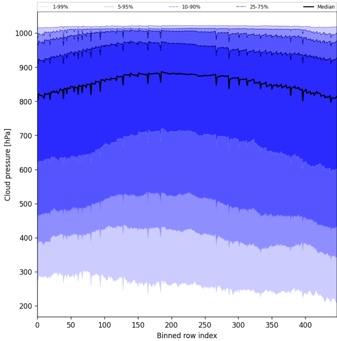
Figure 47: Along track statistics of “Cloud pressure” for 2025-08-30 to 2025-08-31
