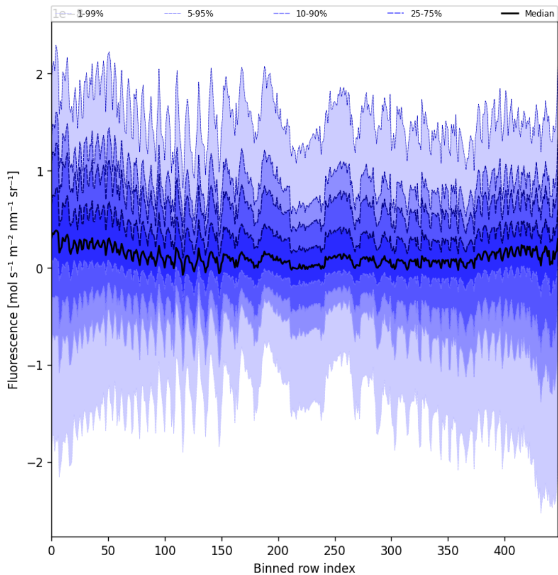
Figure 57: Along track statistics of “Fluorescence” for 2025-08-30 to 2025-08-31
