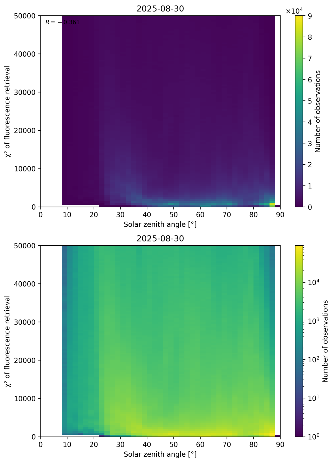
Figure 109: Scatter density plot of “Solar zenith angle” against “ \chi^2 of fluorescence retrieval” for 2025-08-30 to 2025-08-31.
