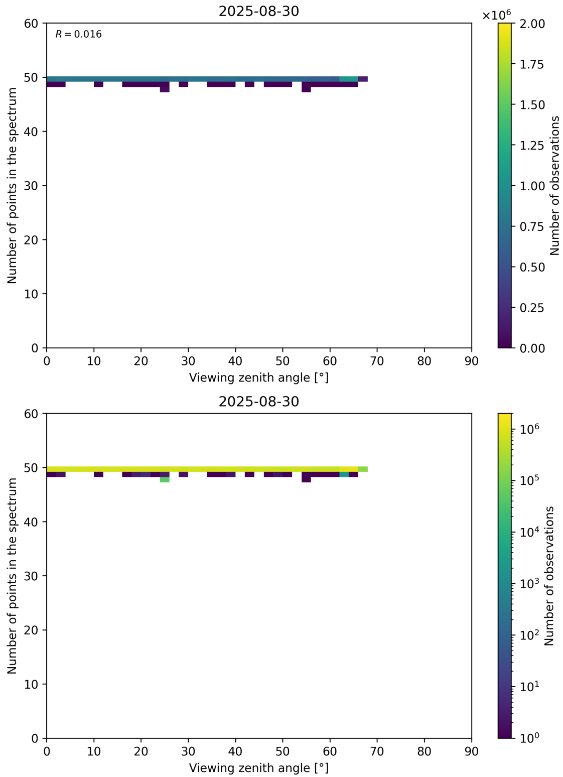
Figure 125: Scatter density plot of “Viewing zenith angle” against “Number of points in the spectrum” for 2025-08-30 to 2025-08-31.
