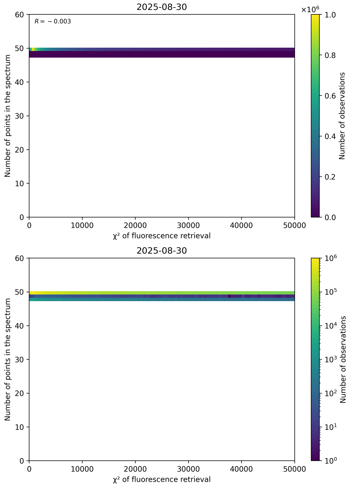
Figure 68: Scatter density plot of “ \chi^2 of fluorescence retrieval” against “Number of points in the spectrum” for 2025-08-30 to 2025-08-31.
