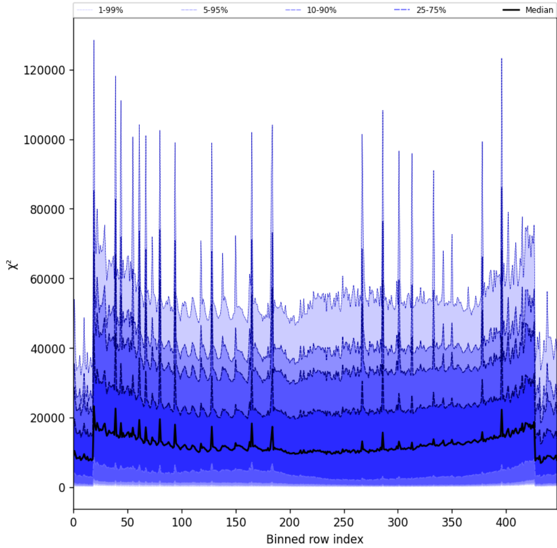
Figure 55: Along track statistics of “ \chi^2 ” for 2025-08-30 to 2025-08-31
