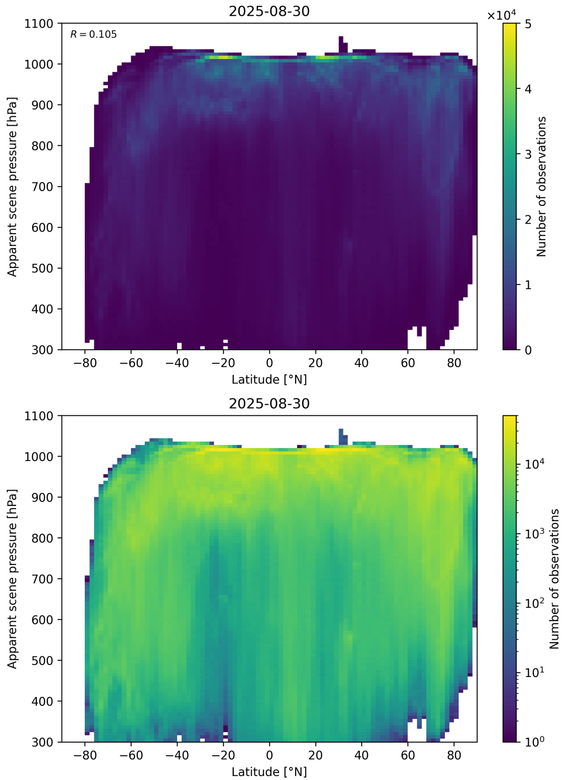
Figure 88: Scatter density plot of “Latitude” against “Apparent scene pressure” for 2025-08-30 to 2025-08-31.
