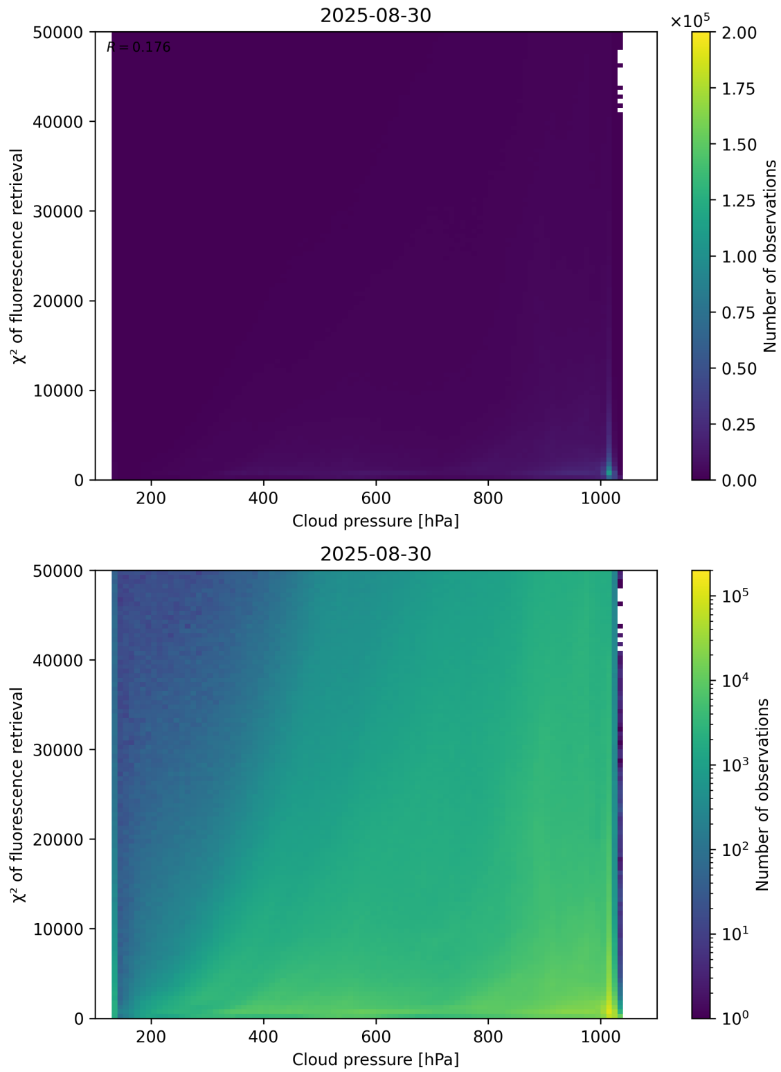
Figure 78: Scatter density plot of “Cloud pressure” against “ \chi^2 of fluorescence retrieval” for 2025-08-30 to 2025-08-31.
