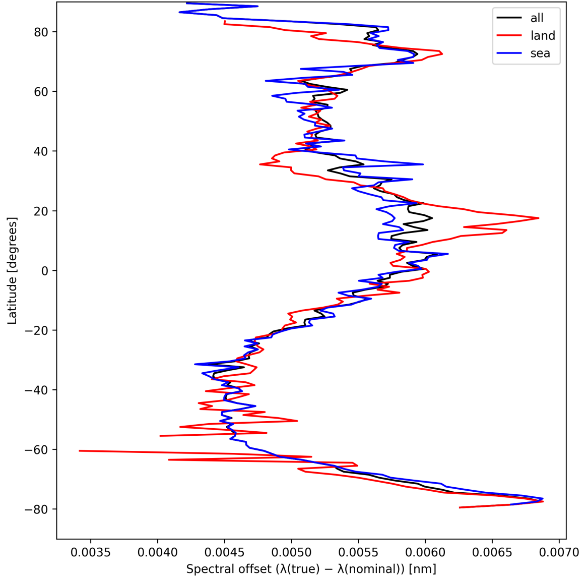
Figure 28: Zonal average of “Spectral offset ( \lambda_{\text{true}} - \lambda_{\text{nominal}} )” for 2025-08-30 to 2025-08-31.
