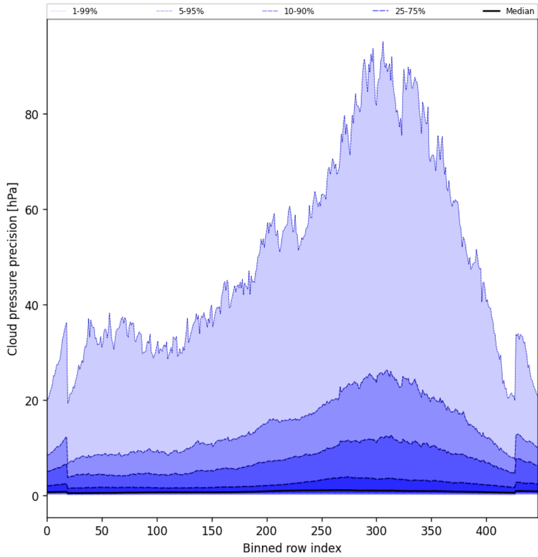
Figure 48: Along track statistics of “Cloud pressure precision” for 2025-08-30 to 2025-08-31
