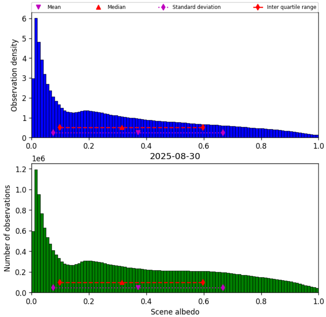
Figure 34: Histogram of “Scene albedo” for 2025-08-30 to 2025-08-31
