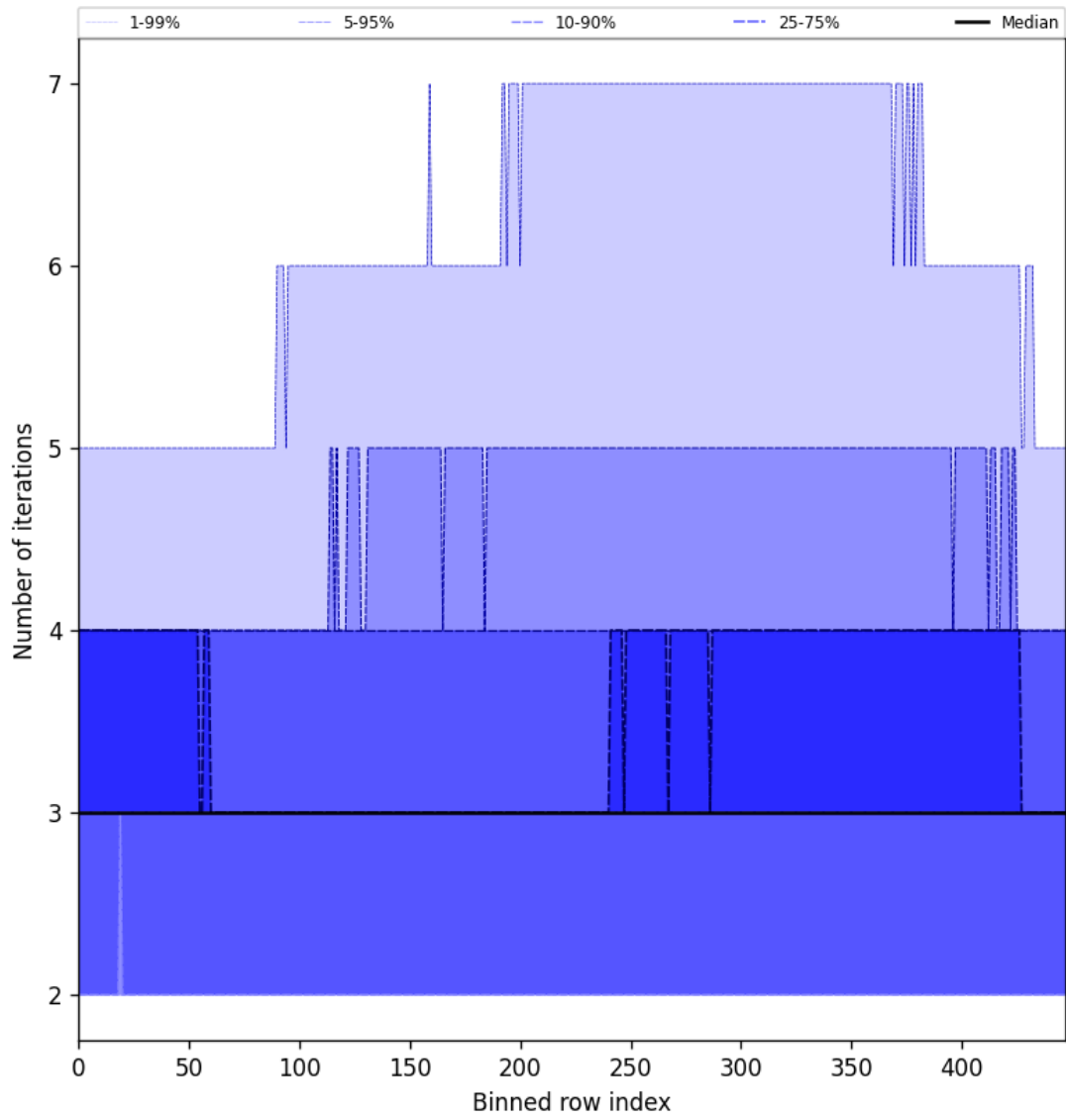
Figure 56: Along track statistics of “Number of iterations” for 2025-08-30 to 2025-08-31
