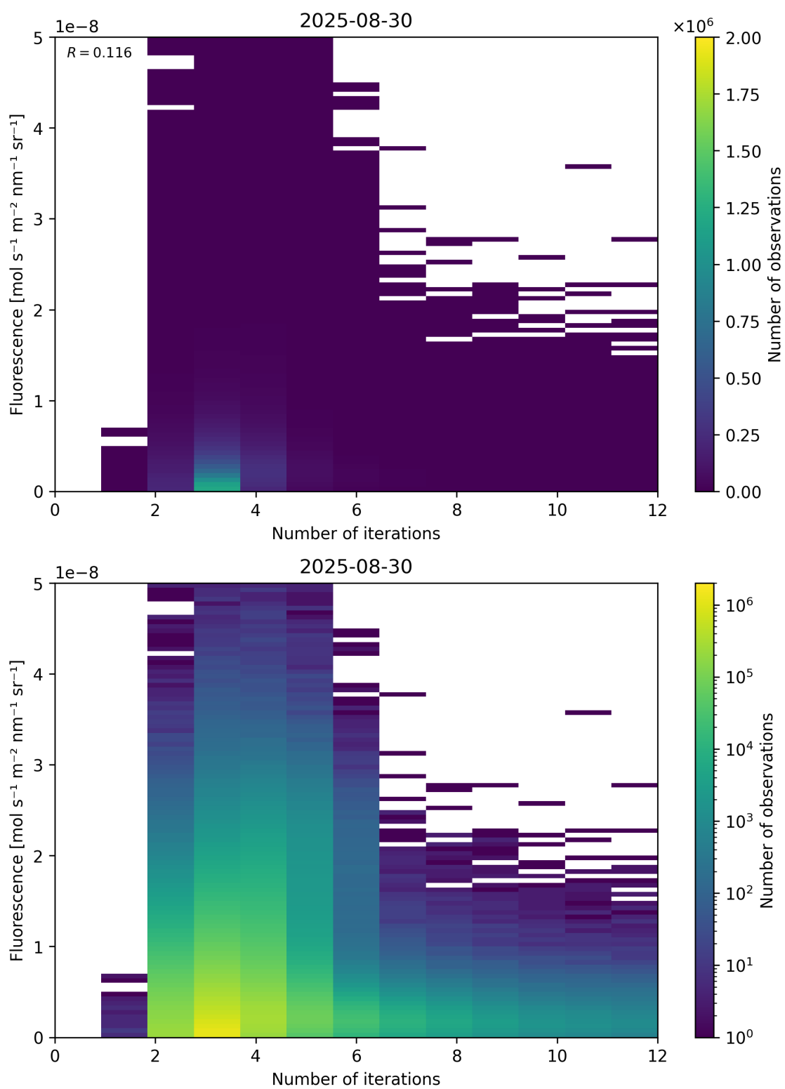
Figure 98: Scatter density plot of "Number of iterations" against "Fluorescence" for 2025-08-30 to 2025-08-31.
