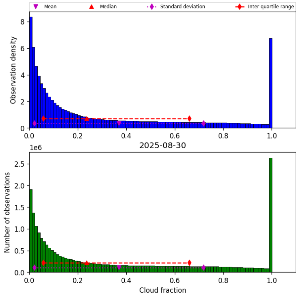
Figure 32: Histogram of “Cloud fraction” for 2025-08-30 to 2025-08-31
