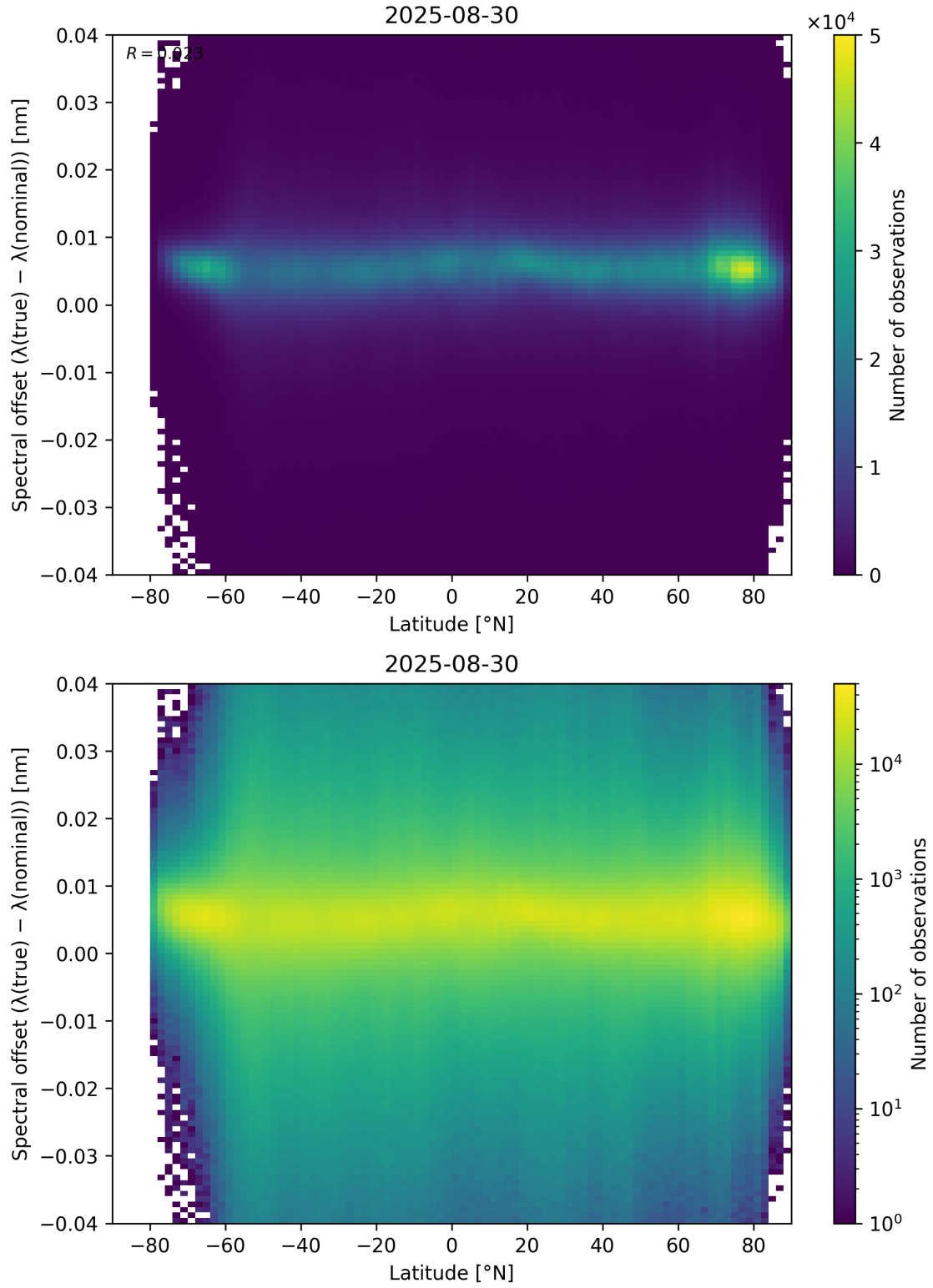
Figure 96: Scatter density plot of “Latitude” against “Spectral offset ( \lambda_{\text{true}} - \lambda_{\text{nominal}} )” for 2025-08-30 to 2025-08-31.
