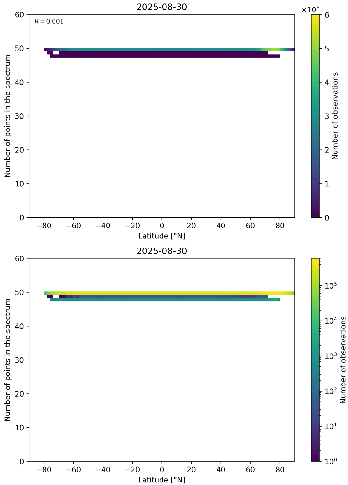
Figure 94: Scatter density plot of “Latitude” against “Number of points in the spectrum” for 2025-08-30 to 2025-08-31.
