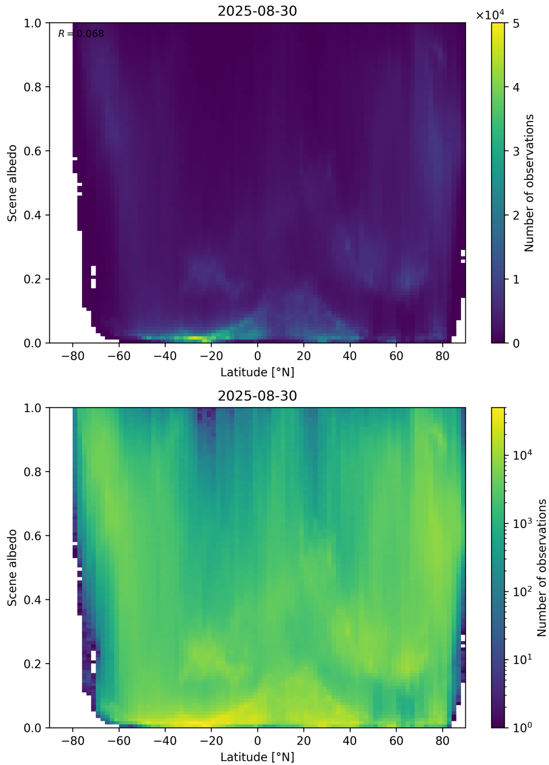
Figure 95: Scatter density plot of “Latitude” against “Scene albedo” for 2025-08-30 to 2025-08-31.
