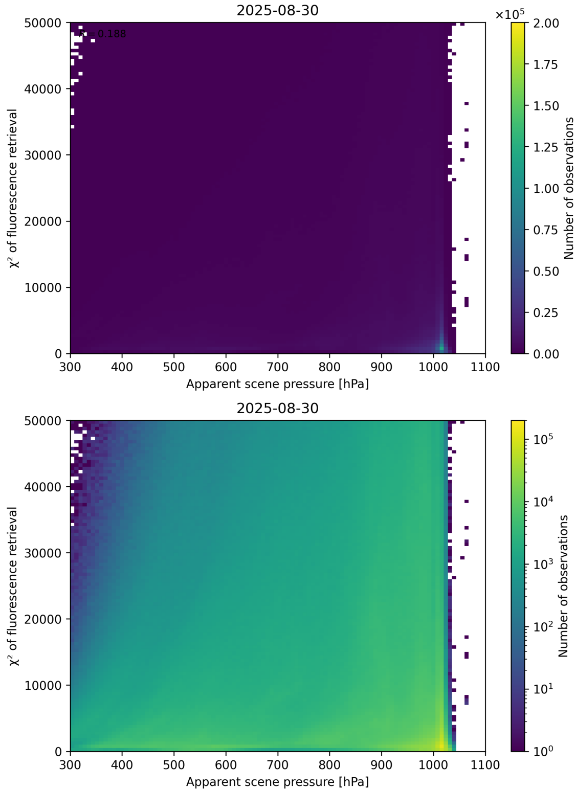
Figure 63: Scatter density plot of “Apparent scene pressure” against “ \chi^2 of fluorescence retrieval” for 2025-08-30 to 2025-08-31.
