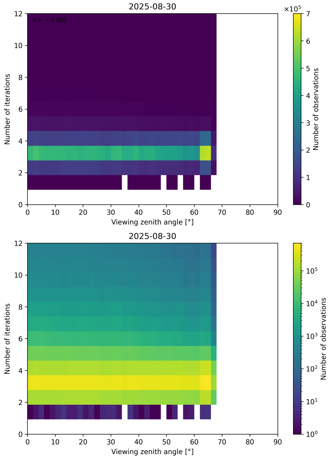
Figure 124: Scatter density plot of “Viewing zenith angle” against “Number of iterations” for 2025-08-30 to 2025-08-31.
