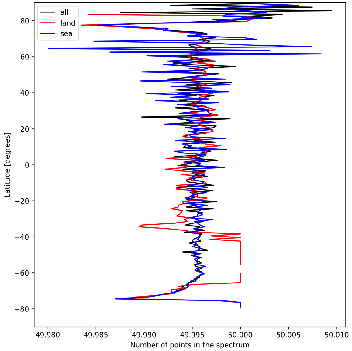
Figure 27: Zonal average of “Number of points in the spectrum” for 2025-08-30 to 2025-08-31.
