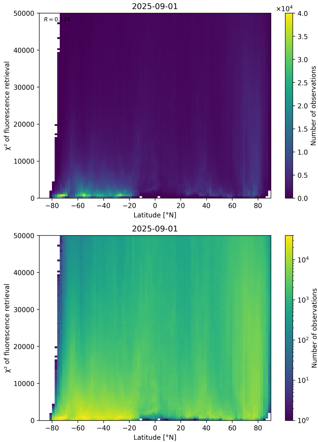
Figure 89: Scatter density plot of “Latitude” against “ \chi^2 of fluorescence retrieval” for 2025-08-31 to 2025-09-02.
