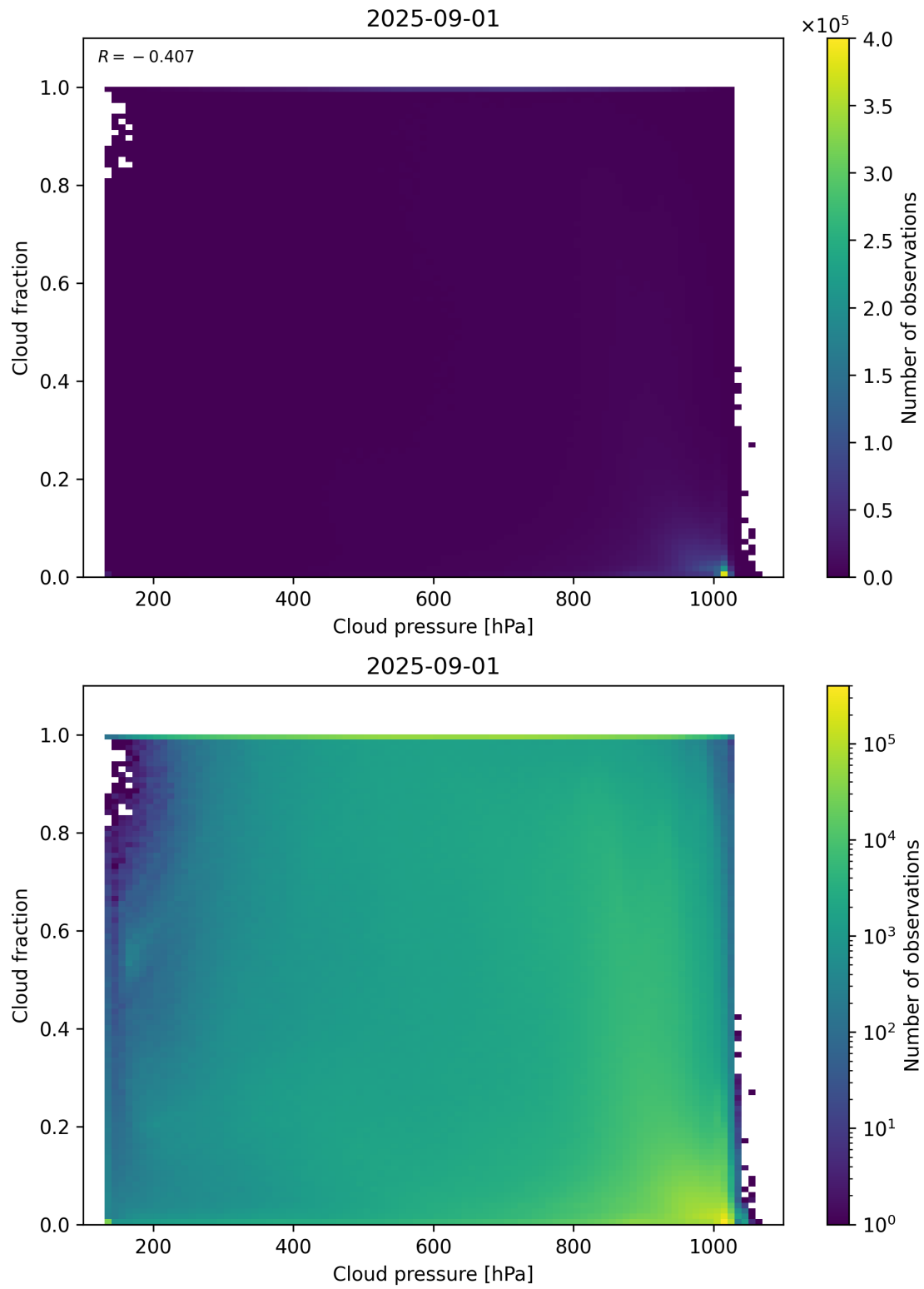
Figure 79: Scatter density plot of “Cloud pressure” against “Cloud fraction” for 2025-08-31 to 2025-09-02.
