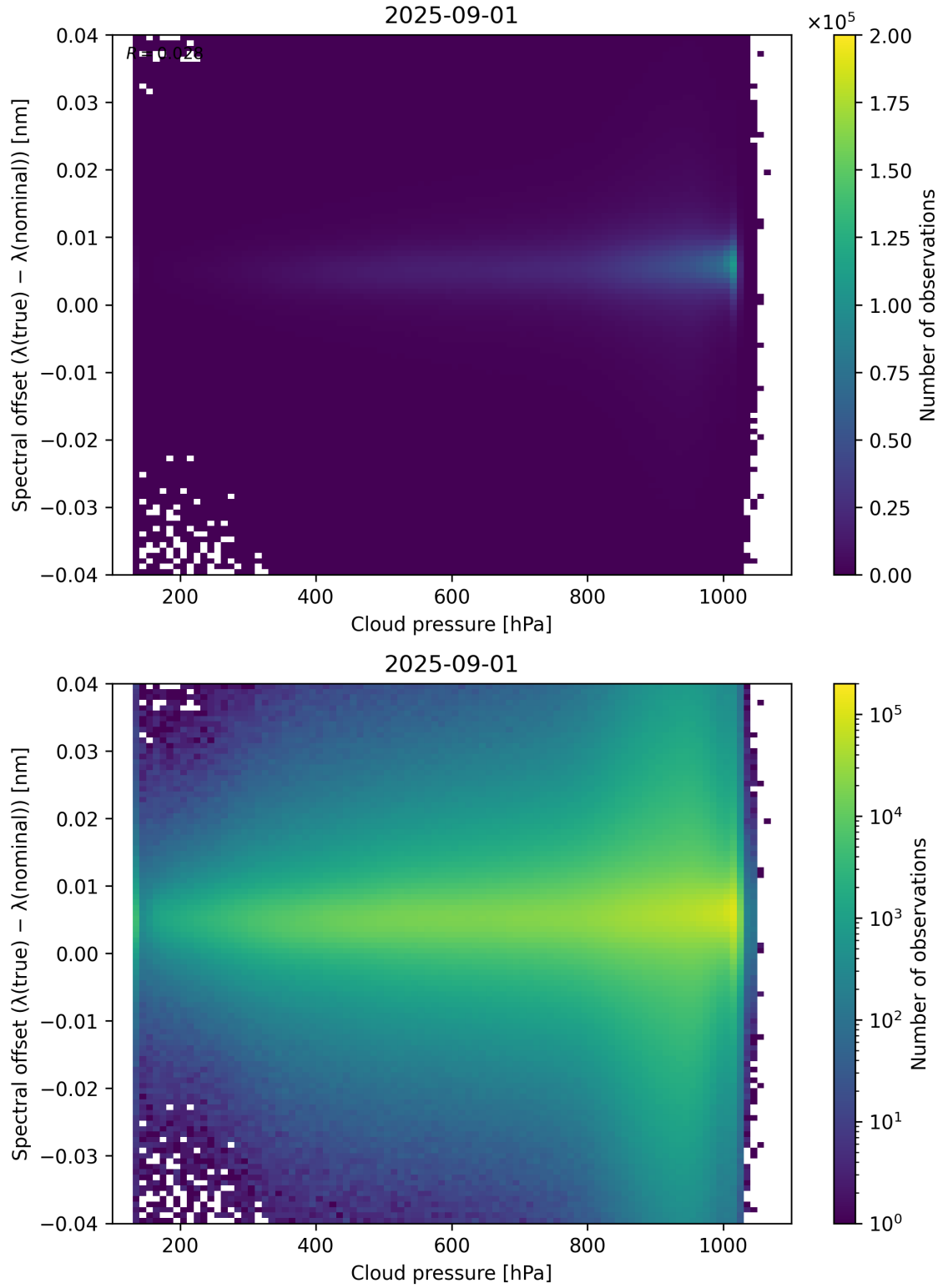
Figure 84: Scatter density plot of “Cloud pressure” against “Spectral offset ( \lambda_{\text{true}} - \lambda_{\text{nominal}} )” for 2025-08-31 to 2025-09-02.
