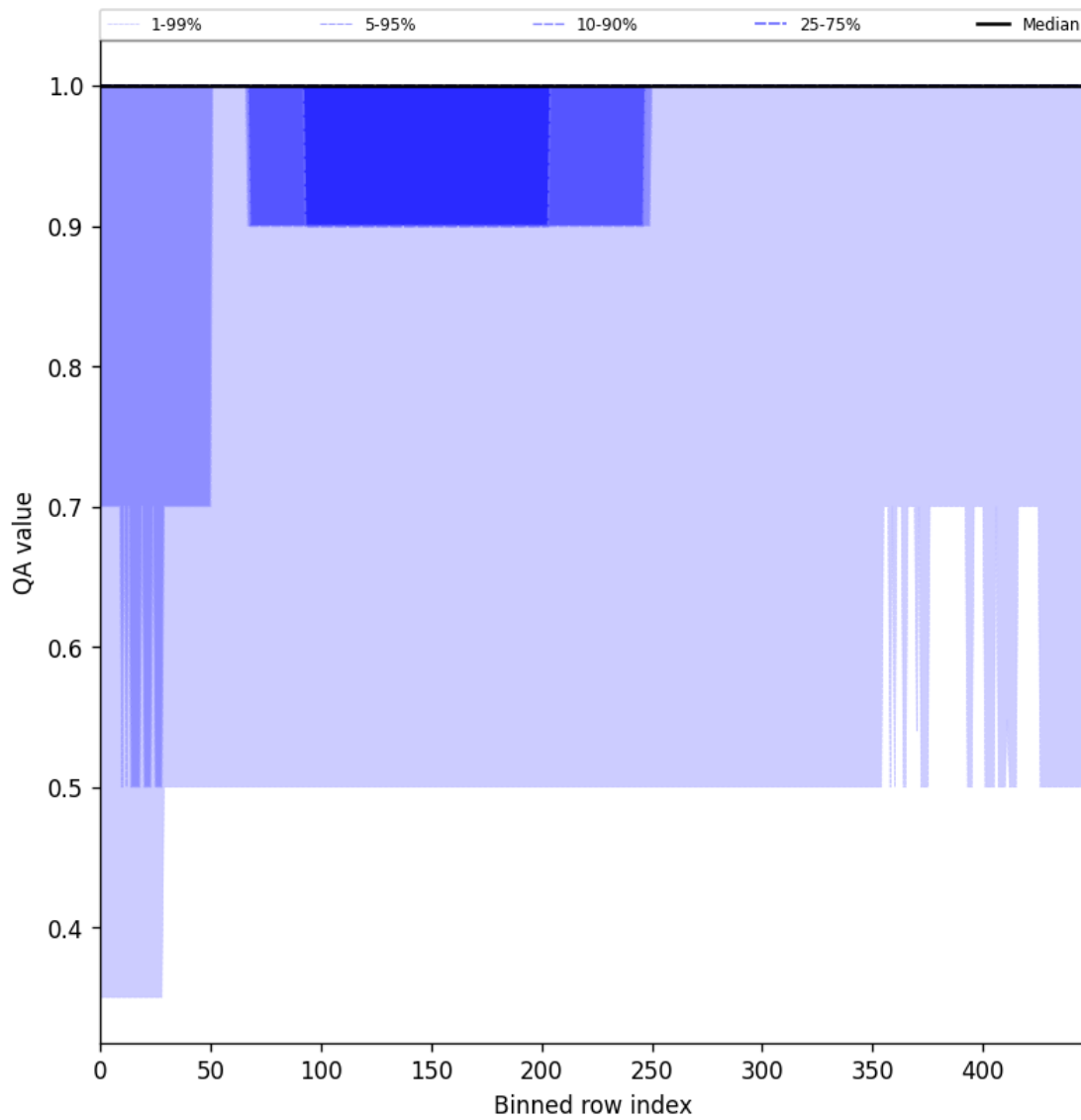
Figure 46: Along track statistics of “QA value” for 2025-08-31 to 2025-09-02
