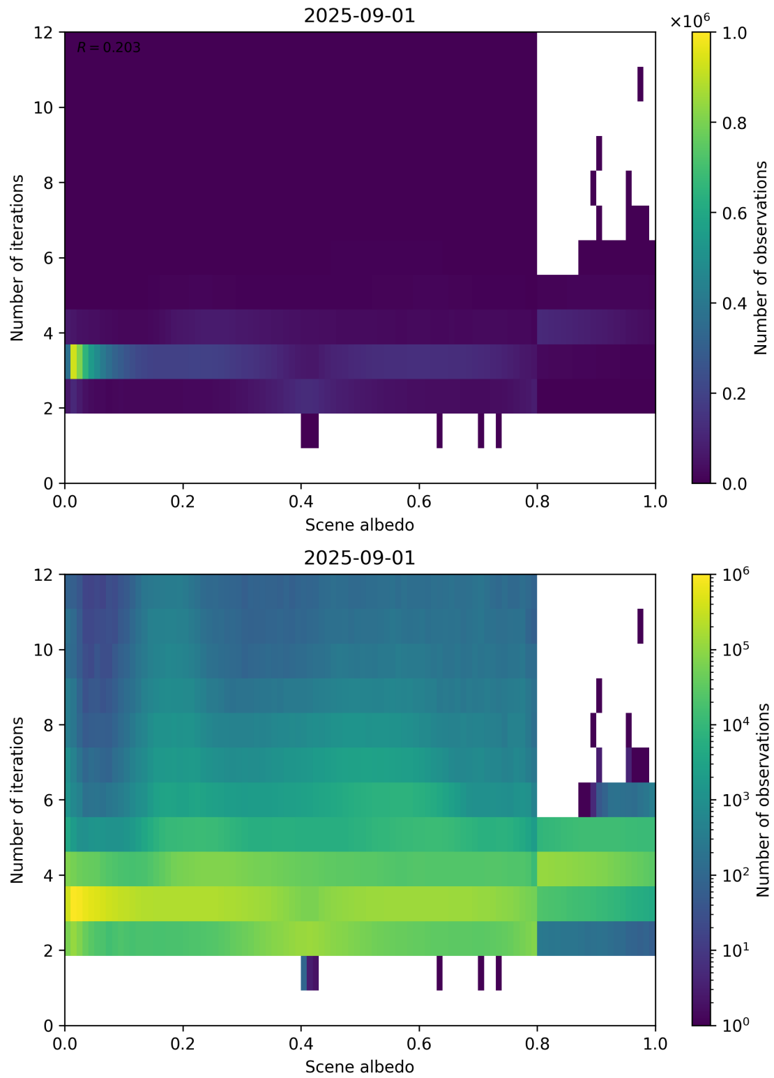
Figure 105: Scatter density plot of “Scene albedo” against “Number of iterations” for 2025-08-31 to 2025-09-02.
