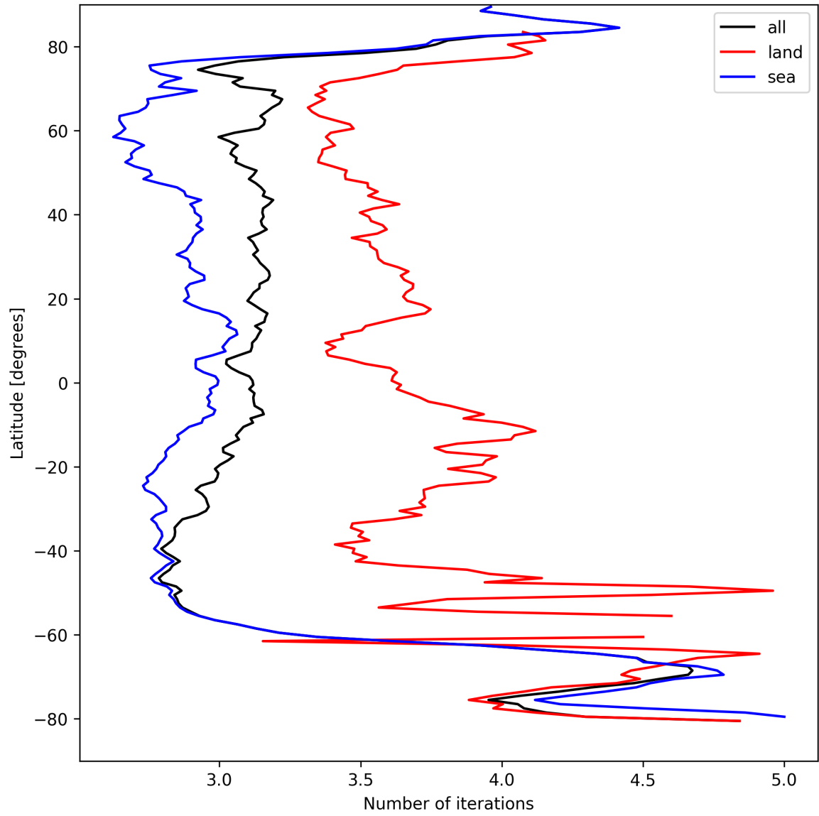
Figure 22: Zonal average of “Number of iterations” for 2025-08-31 to 2025-09-02.
