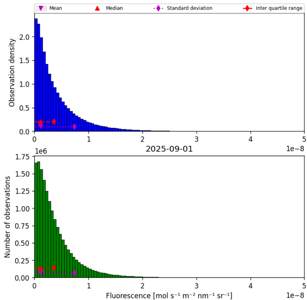
Figure 40: Histogram of “Fluorescence” for 2025-08-31 to 2025-09-02
