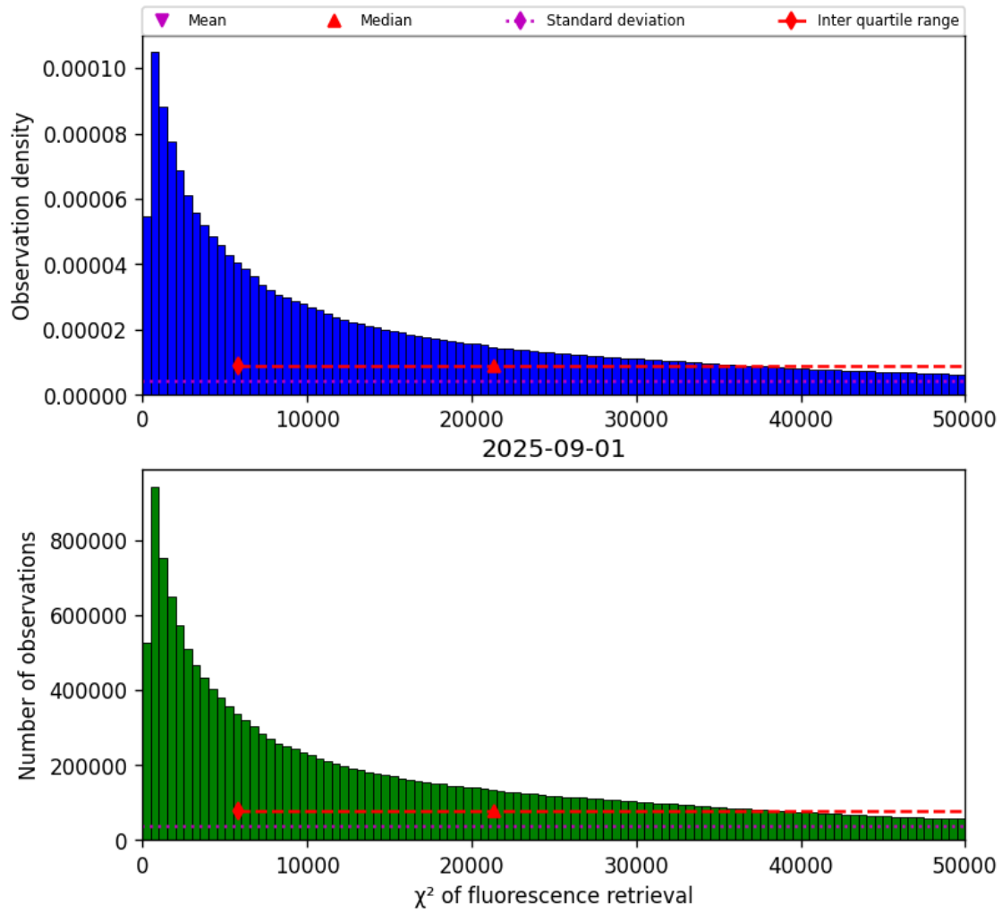
Figure 42: Histogram of “ \chi^2 of fluorescence retrieval” for 2025-08-31 to 2025-09-02
