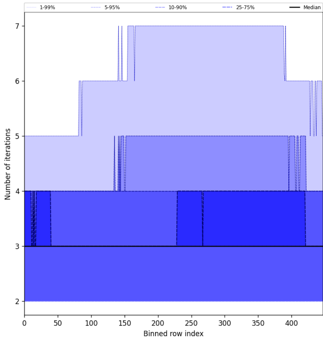
Figure 56: Along track statistics of “Number of iterations” for 2025-08-31 to 2025-09-02
