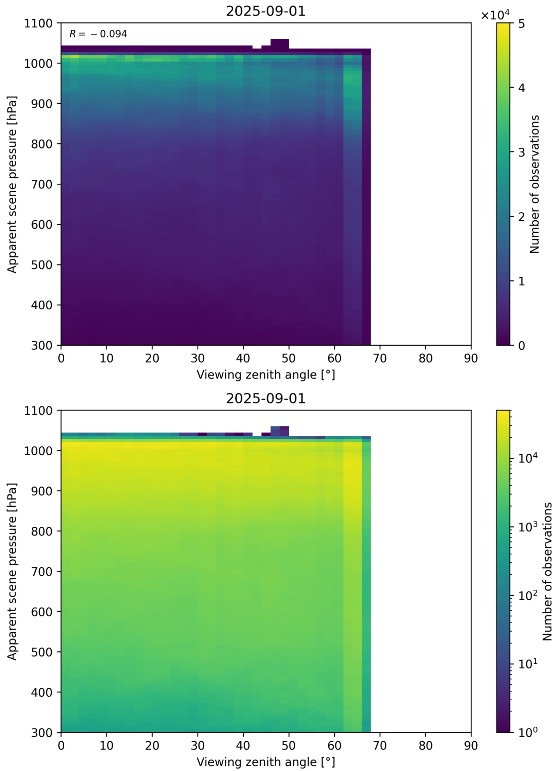
Figure 118: Scatter density plot of “Viewing zenith angle” against “Apparent scene pressure” for 2025-08-31 to 2025-09-02.
