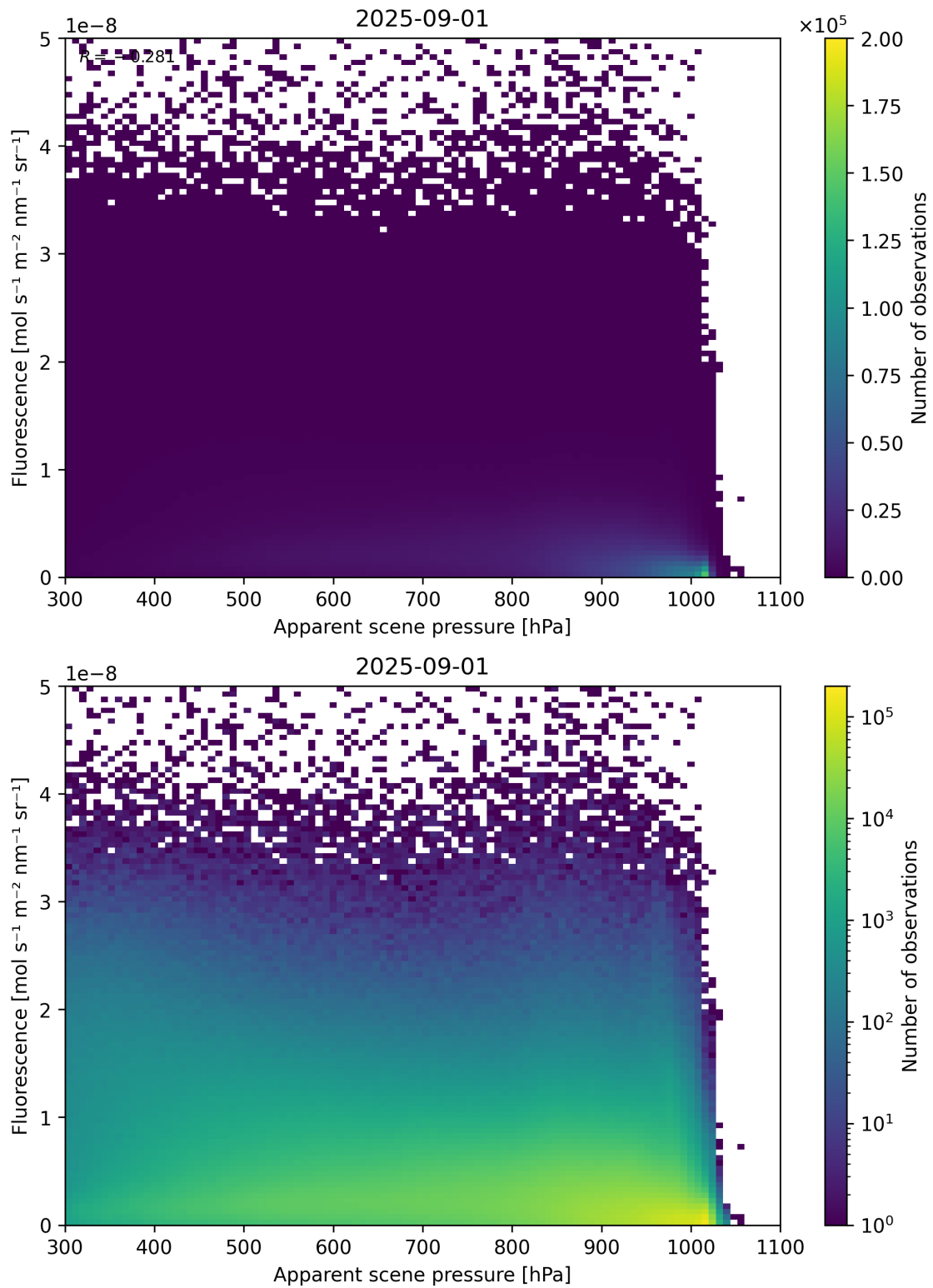
Figure 64: Scatter density plot of “Apparent scene pressure” against “Fluorescence” for 2025-08-31 to 2025-09-02.
