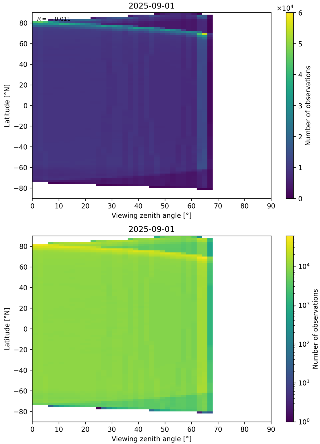
Figure 123: Scatter density plot of “Viewing zenith angle” against “Latitude” for 2025-08-31 to 2025-09-02.
