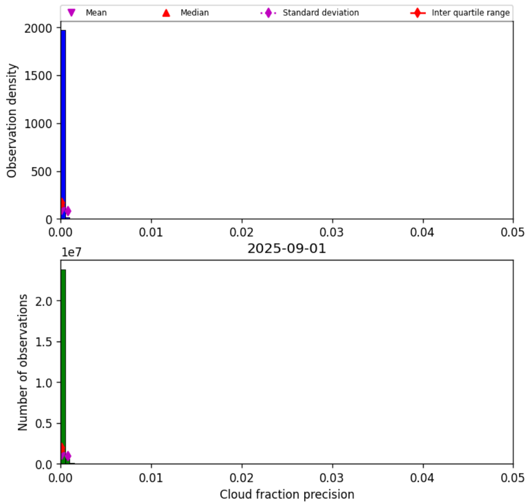
Figure 33: Histogram of “Cloud fraction precision” for 2025-08-31 to 2025-09-02
