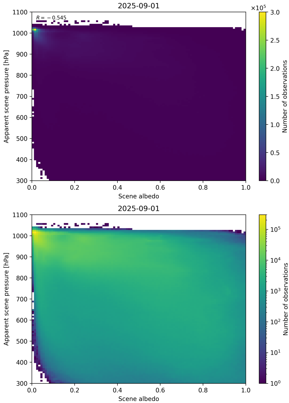
Figure 102: Scatter density plot of “Scene albedo” against “Apparent scene pressure” for 2025-08-31 to 2025-09-02.
