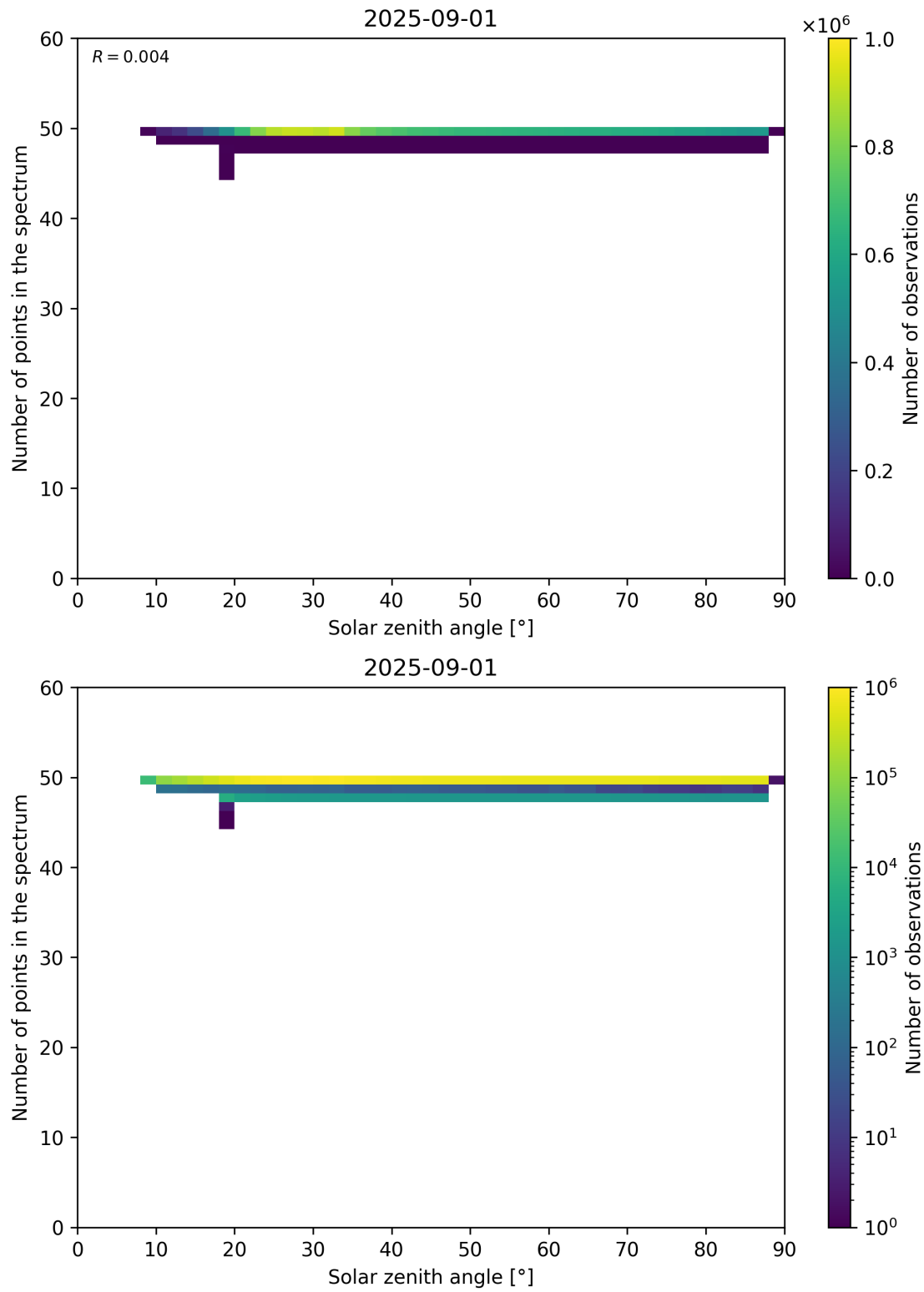
Figure 115: Scatter density plot of “Solar zenith angle” against “Number of points in the spectrum” for 2025-08-31 to 2025-09-02.
