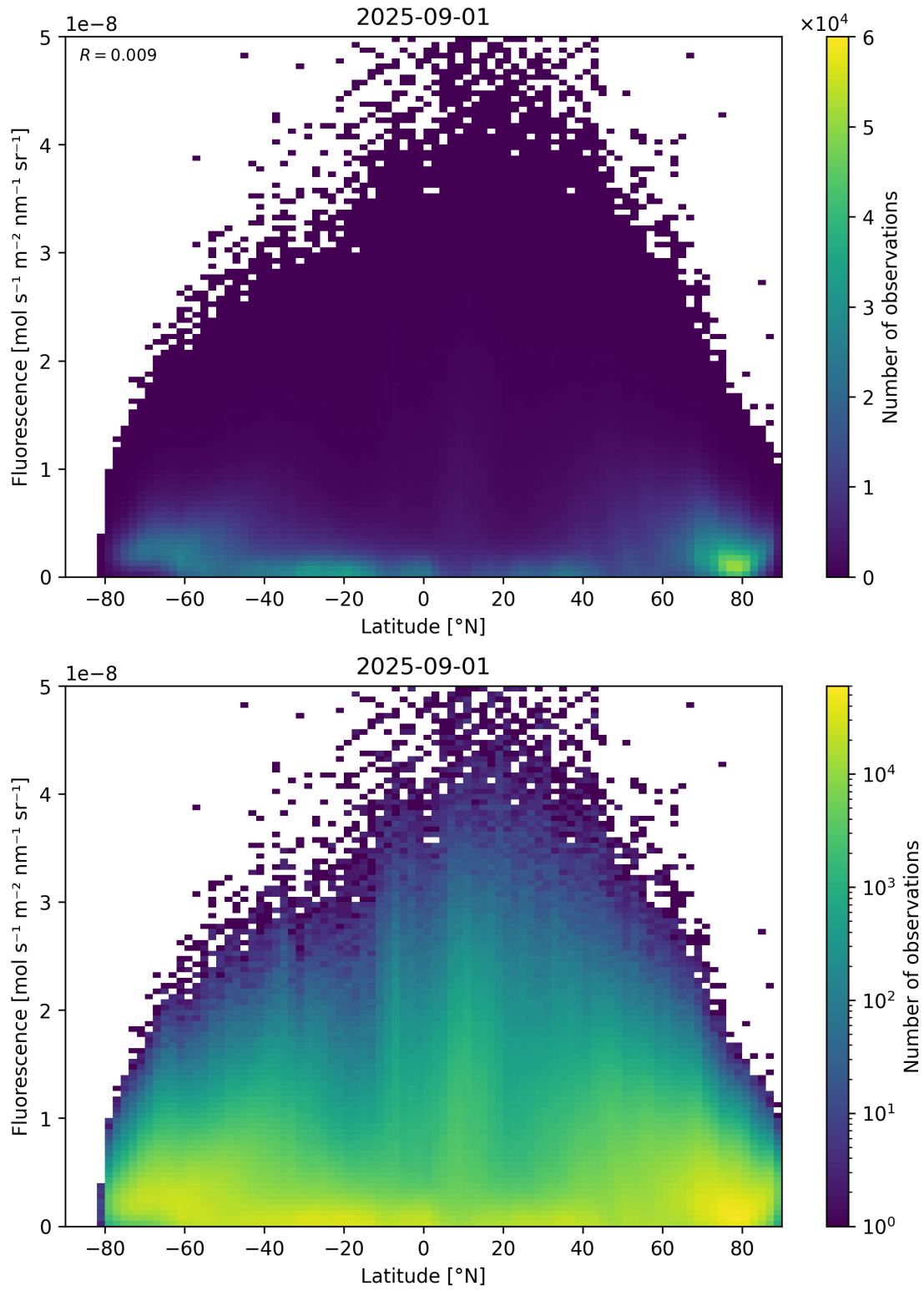
Figure 92: Scatter density plot of “Latitude” against “Fluorescence” for 2025-08-31 to 2025-09-02.
