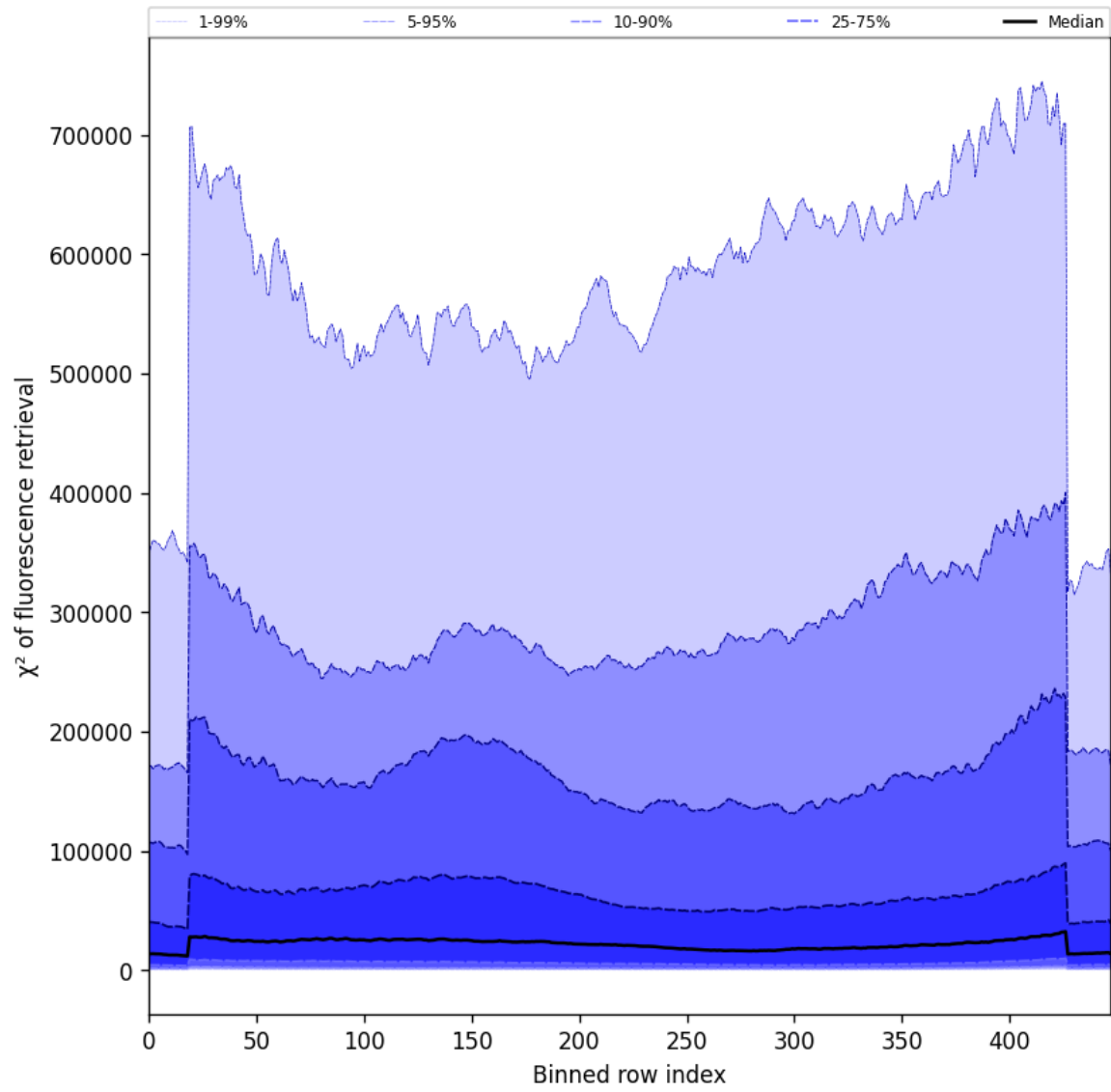
Figure 59: Along track statistics of “ \chi^2 of fluorescence retrieval” for 2025-08-31 to 2025-09-02
