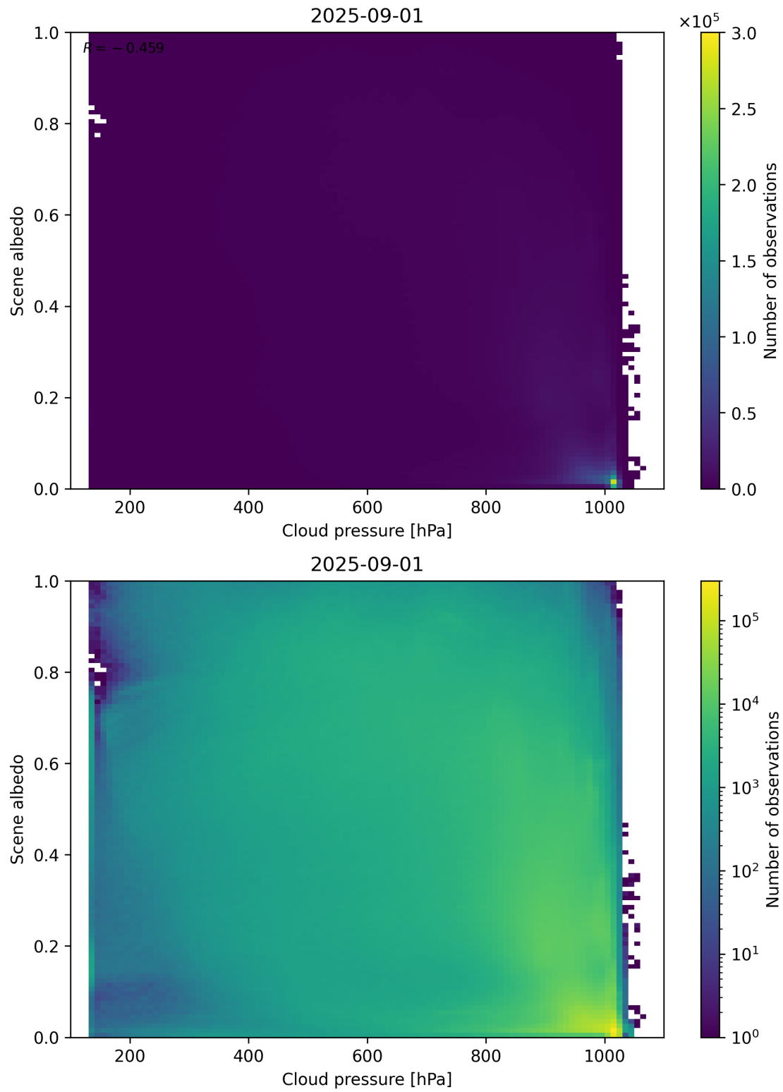
Figure 83: Scatter density plot of “Cloud pressure” against “Scene albedo” for 2025-08-31 to 2025-09-02.
