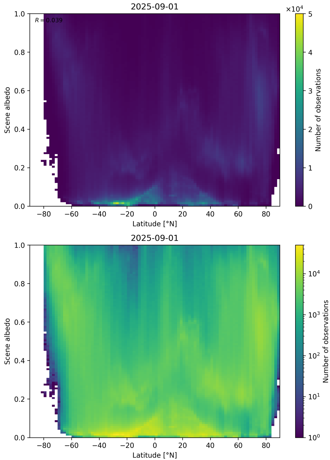
Figure 95: Scatter density plot of “Latitude” against “Scene albedo” for 2025-08-31 to 2025-09-02.
