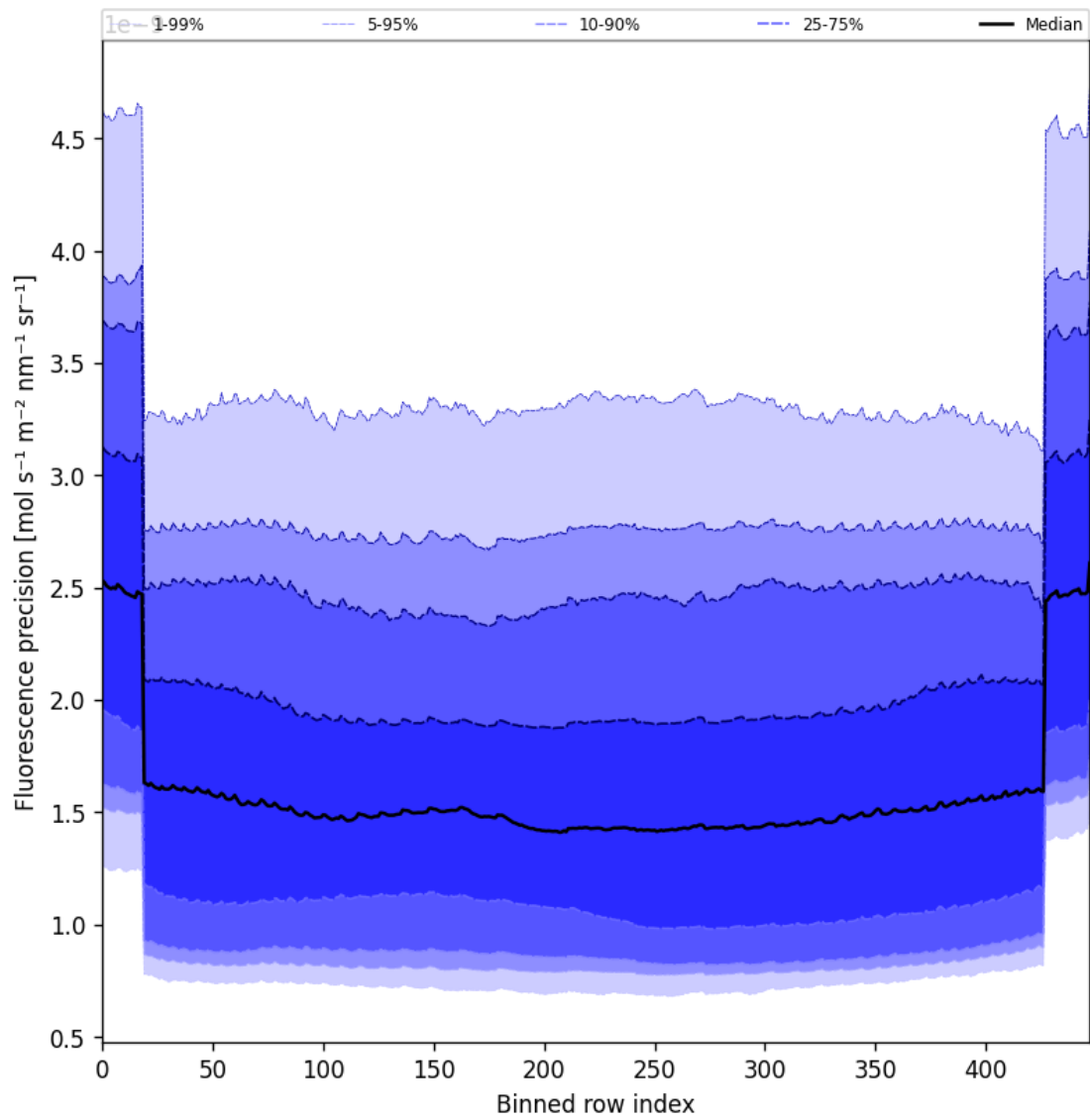
Figure 58: Along track statistics of “Fluorescence precision” for 2025-08-31 to 2025-09-02
