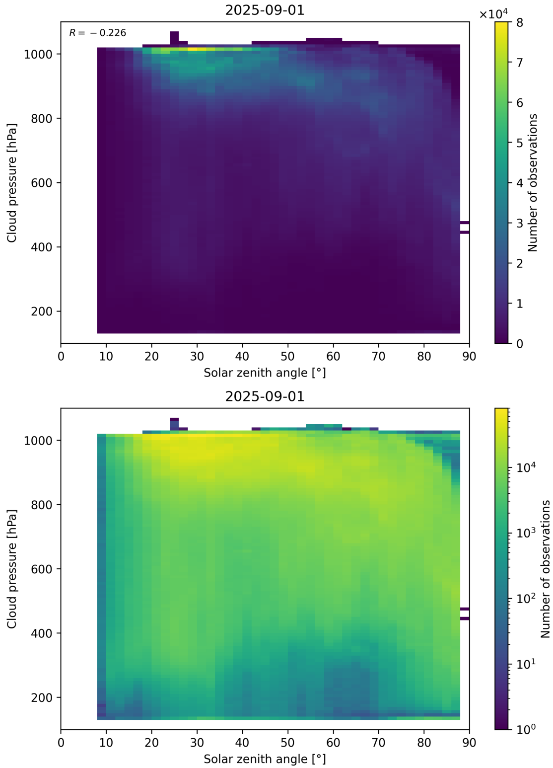
Figure 111: Scatter density plot of “Solar zenith angle” against “Cloud pressure” for 2025-08-31 to 2025-09-02.
