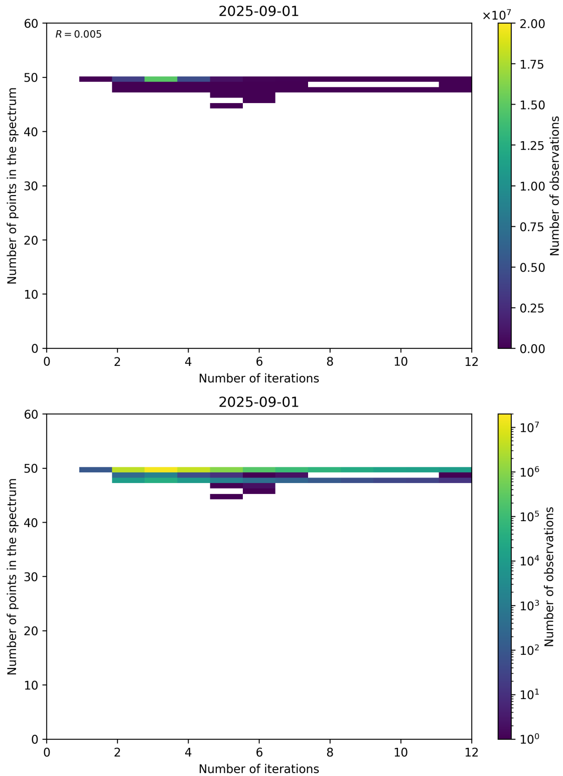
Figure 99: Scatter density plot of “Number of iterations” against “Number of points in the spectrum” for 2025-08-31 to 2025-09-02.
