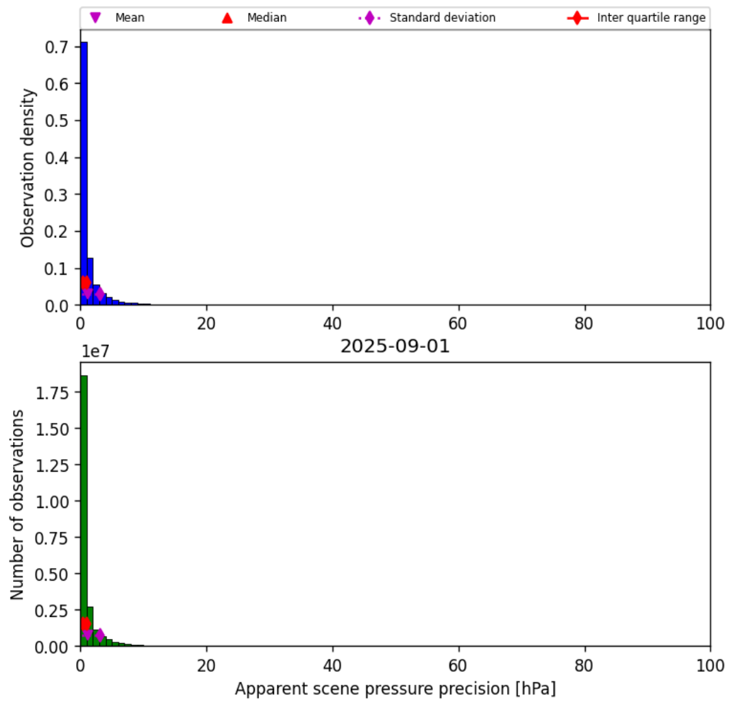
Figure 37: Histogram of “Apparent scene pressure precision” for 2025-08-31 to 2025-09-02
