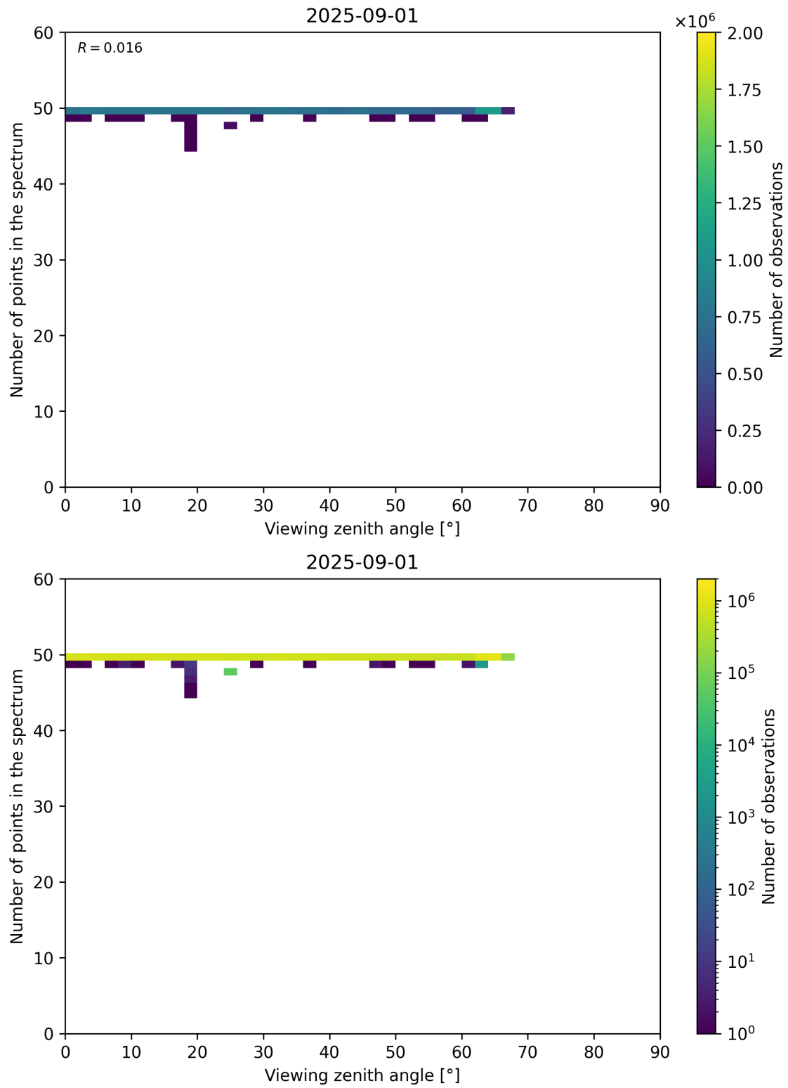
Figure 125: Scatter density plot of “Viewing zenith angle” against “Number of points in the spectrum” for 2025-08-31 to 2025-09-02.
