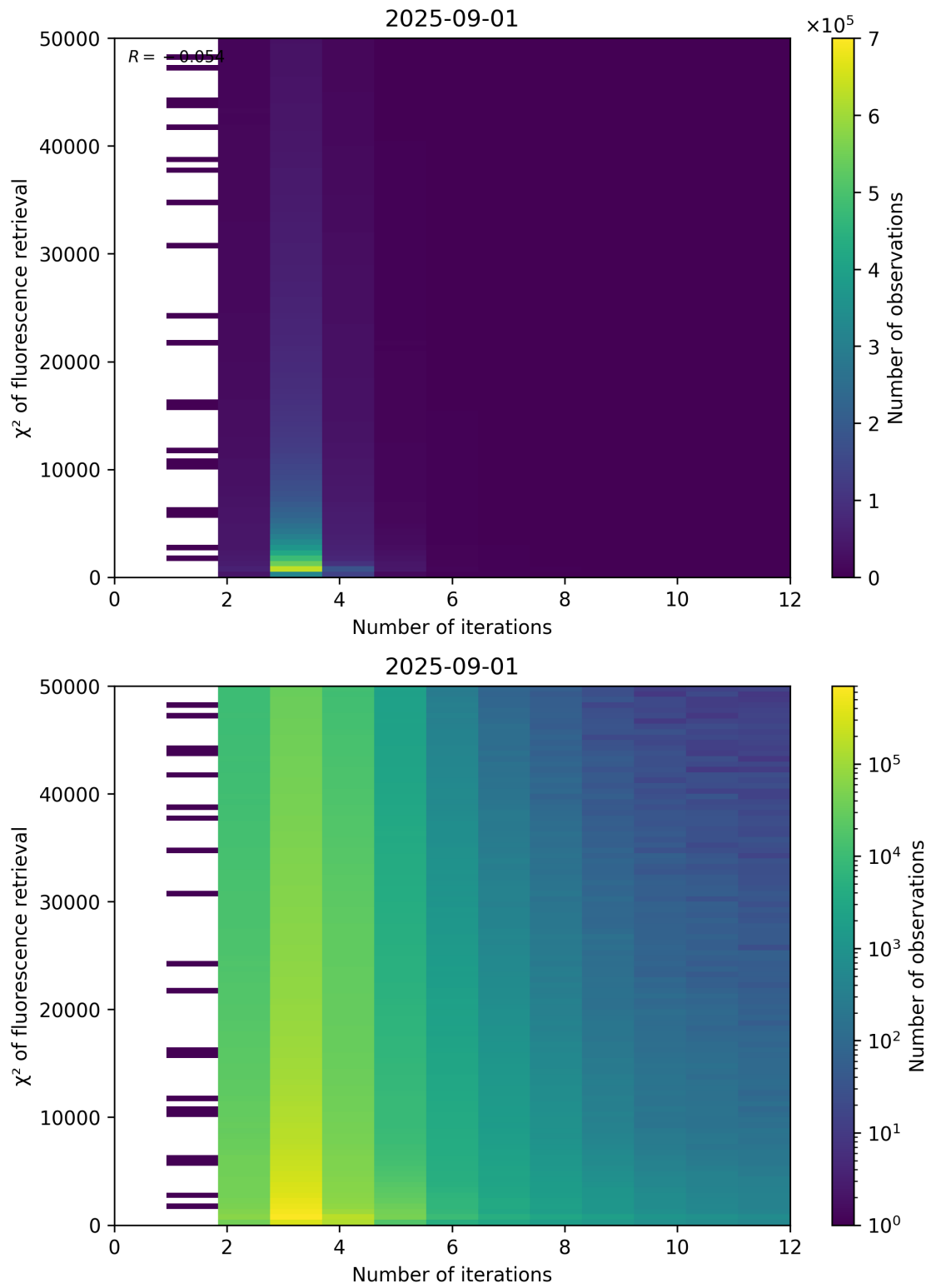
Figure 97: Scatter density plot of “Number of iterations” against “ \chi^2 of fluorescence retrieval” for 2025-08-31 to 2025-09-02.
