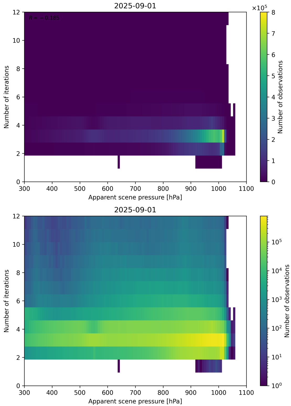
Figure 65: Scatter density plot of “Apparent scene pressure” against “Number of iterations” for 2025-08-31 to 2025-09-02.
