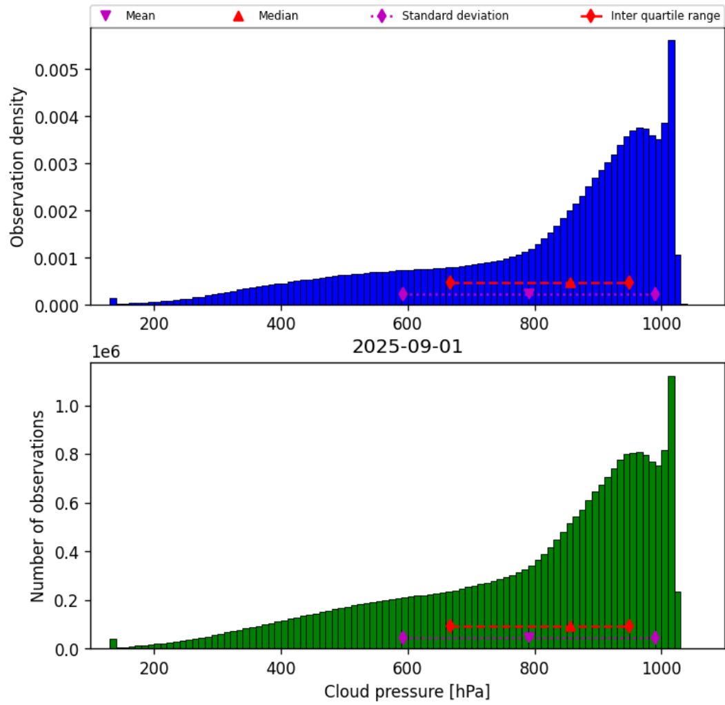
Figure 30: Histogram of “Cloud pressure” for 2025-08-31 to 2025-09-02
