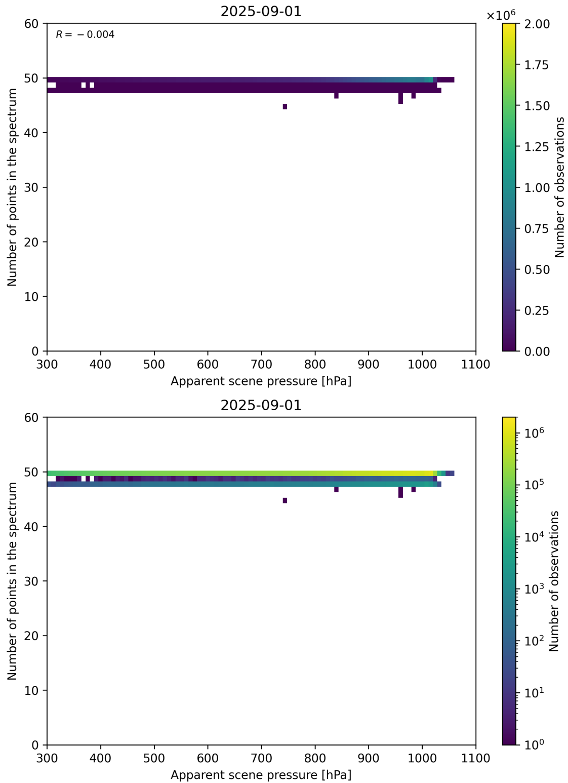
Figure 66: Scatter density plot of “Apparent scene pressure” against “Number of points in the spectrum” for 2025-08-31 to 2025-09-02.
