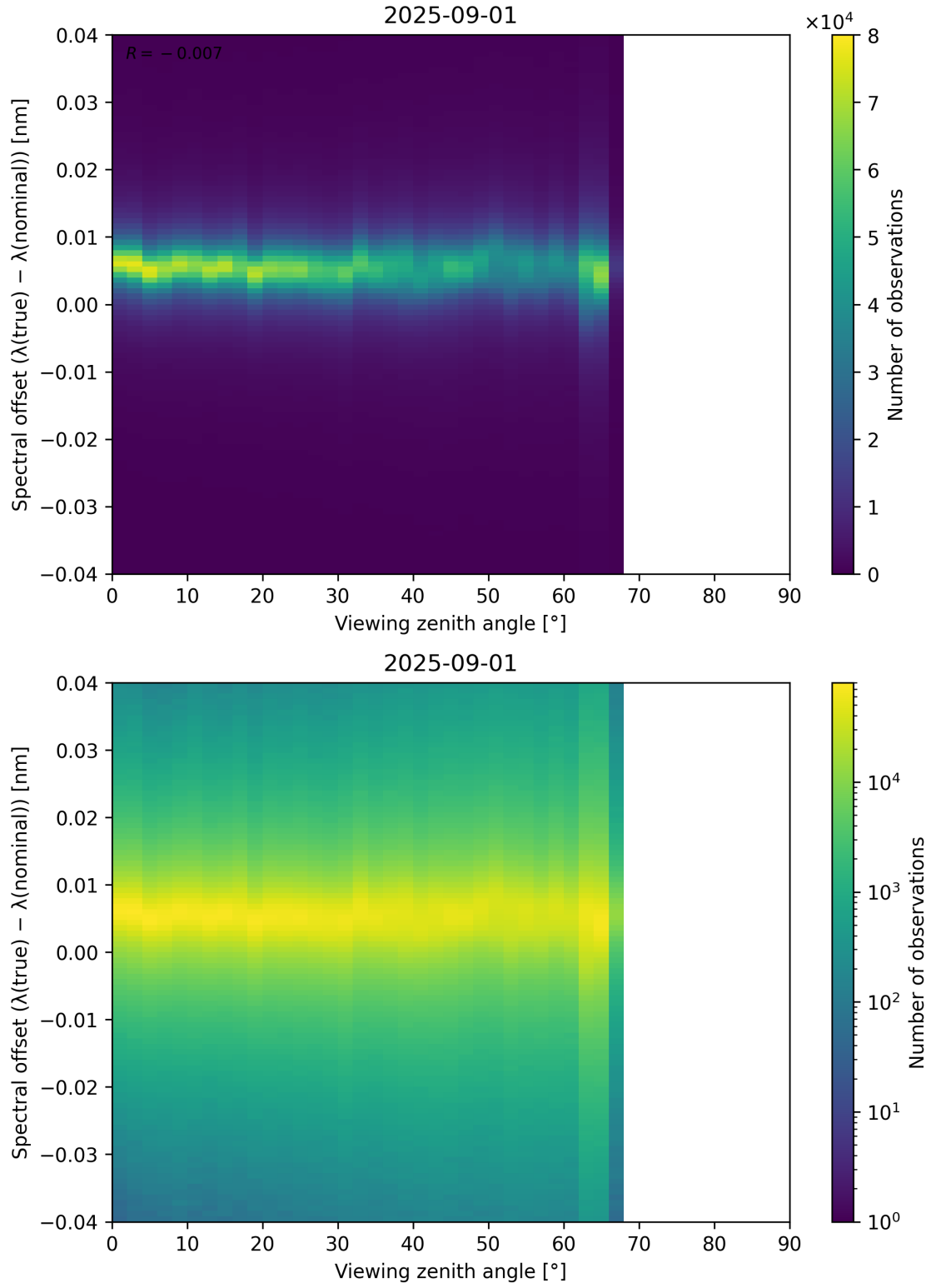
Figure 128: Scatter density plot of “Viewing zenith angle” against “Spectral offset ( \lambda_{\text{true}} - \lambda_{\text{nominal}} )” for 2025-08-31 to 2025-09-02.
