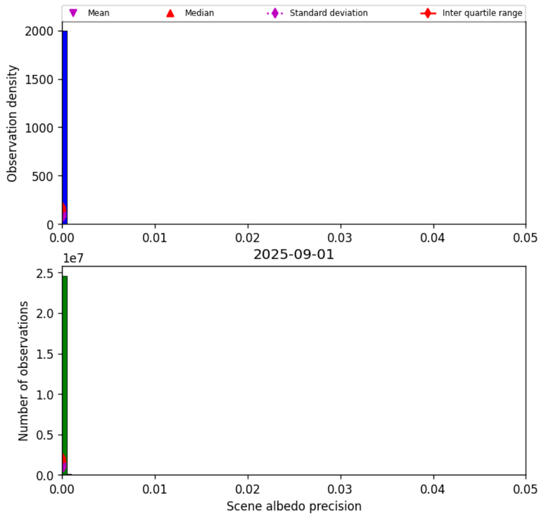
Figure 35: Histogram of “Scene albedo precision” for 2025-08-31 to 2025-09-02
