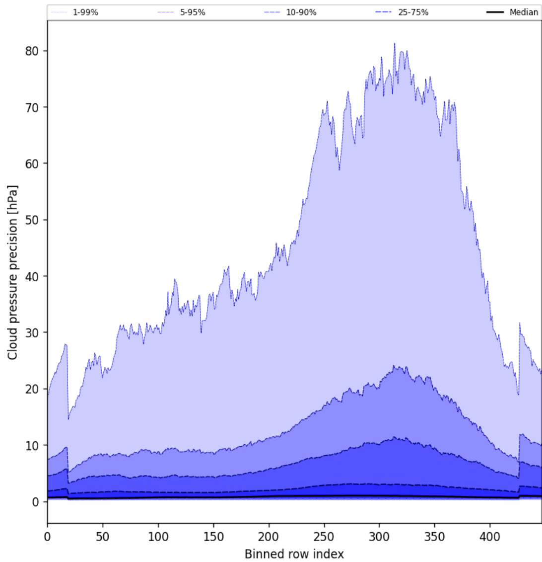
Figure 48: Along track statistics of “Cloud pressure precision” for 2025-08-31 to 2025-09-02
