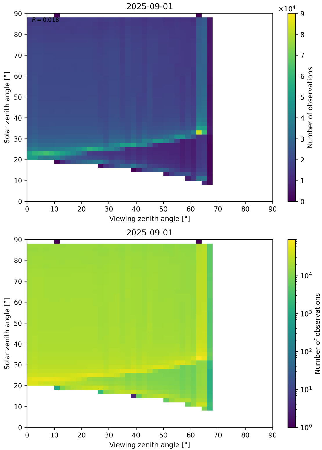
Figure 127: Scatter density plot of “Viewing zenith angle” against “Solar zenith angle” for 2025-08-31 to 2025-09-02.
