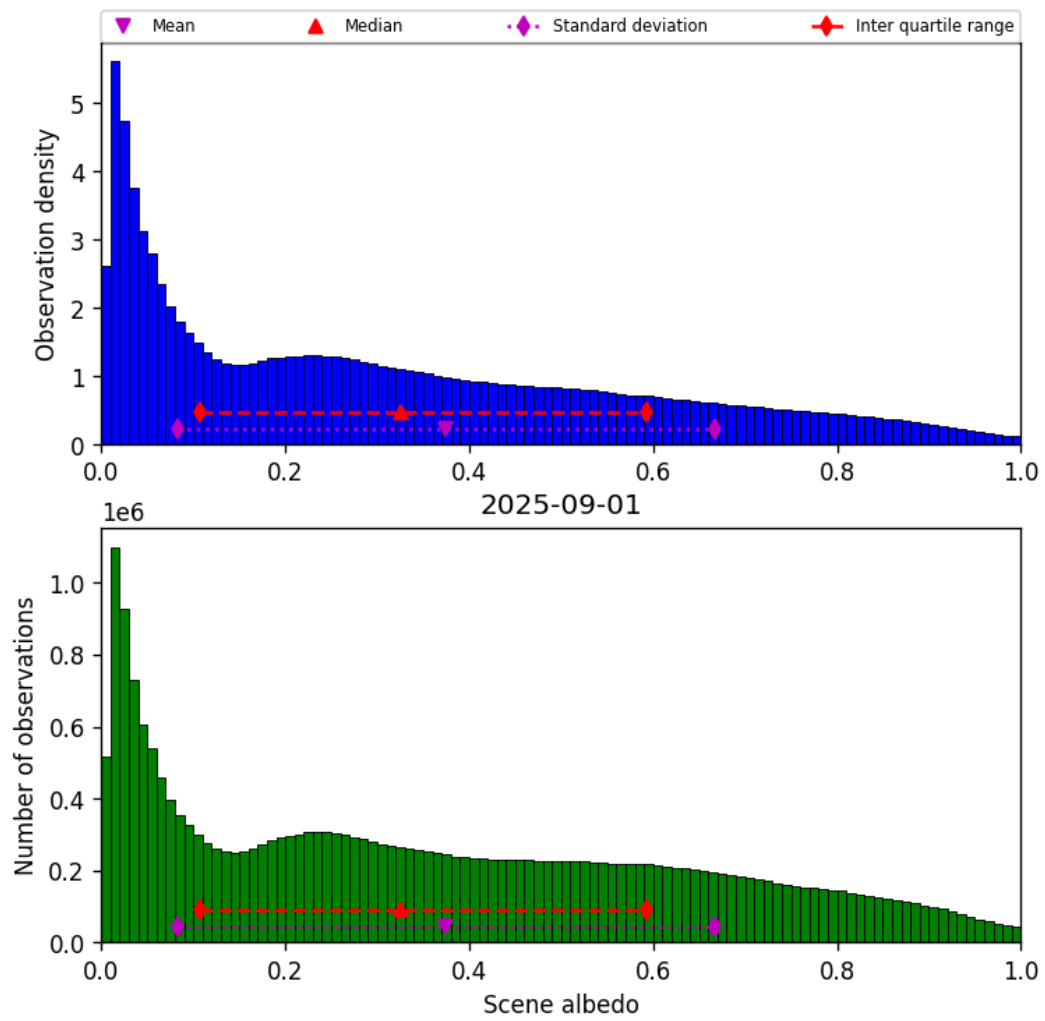
Figure 34: Histogram of “Scene albedo” for 2025-08-31 to 2025-09-02
