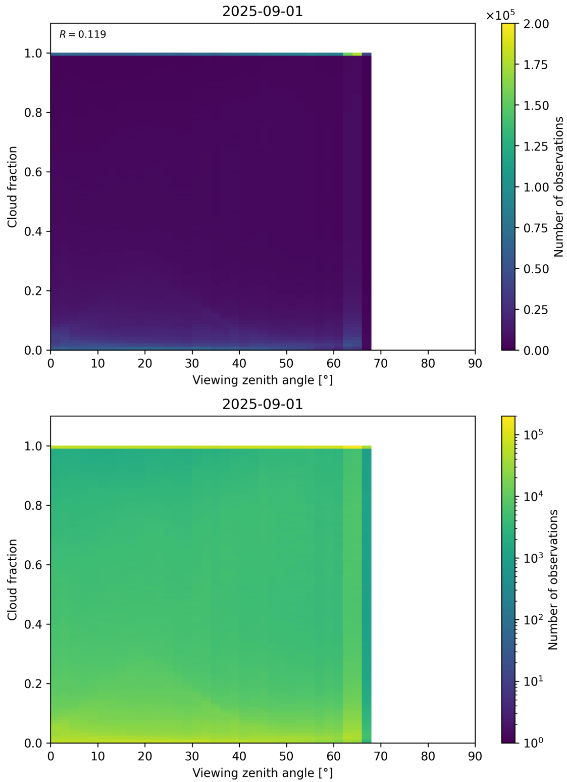
Figure 120: Scatter density plot of “Viewing zenith angle” against “Cloud fraction” for 2025-08-31 to 2025-09-02.
