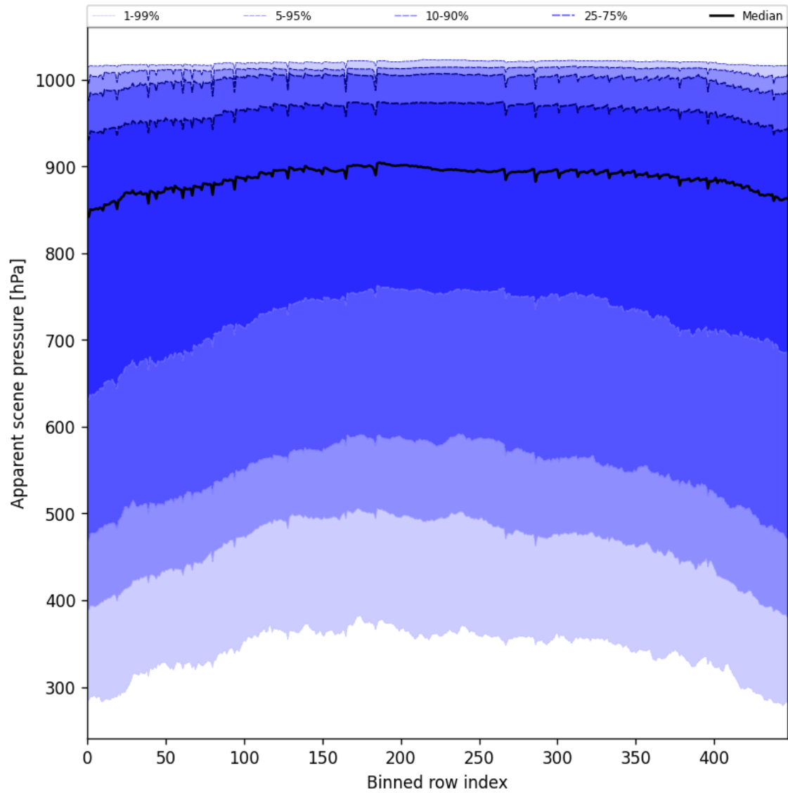
Figure 53: Along track statistics of “Apparent scene pressure” for 2025-08-31 to 2025-09-02
