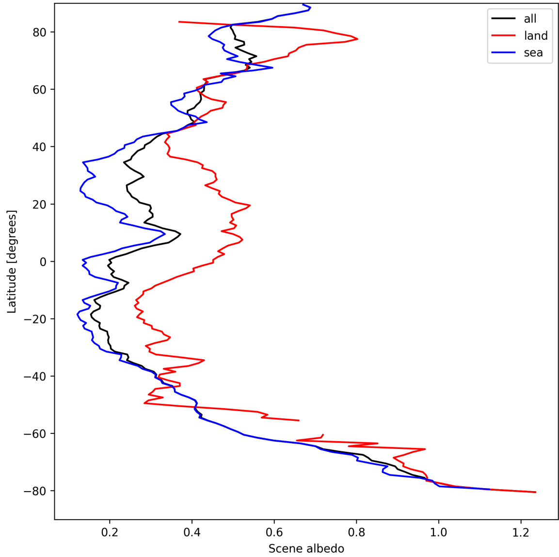
Figure 17: Zonal average of “Scene albedo” for 2025-08-31 to 2025-09-02.
