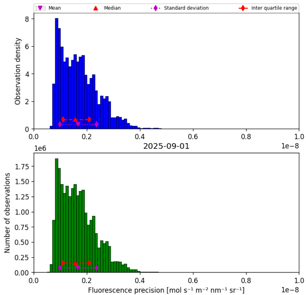
Figure 41: Histogram of “Fluorescence precision” for 2025-08-31 to 2025-09-02
