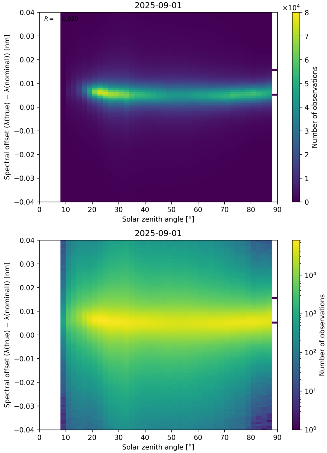
Figure 117: Scatter density plot of “Solar zenith angle” against “Spectral offset ( \lambda_{\text{true}} - \lambda_{\text{nominal}} )” for 2025-08-31 to 2025-09-02.
