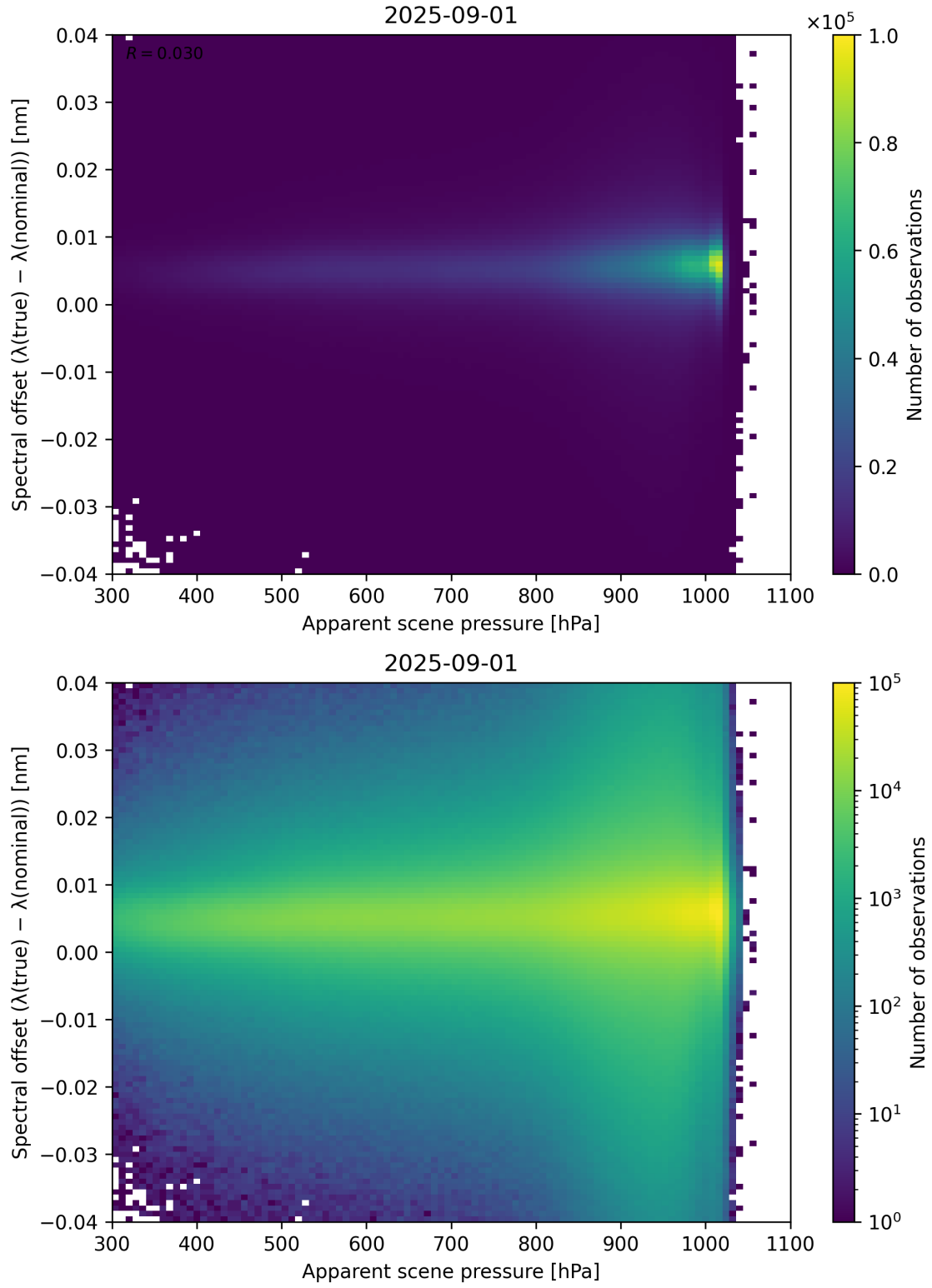
Figure 67: Scatter density plot of “Apparent scene pressure” against “Spectral offset ( \lambda_{\text{true}} - \lambda_{\text{nominal}} )” for 2025-08-31 to 2025-09-02.
