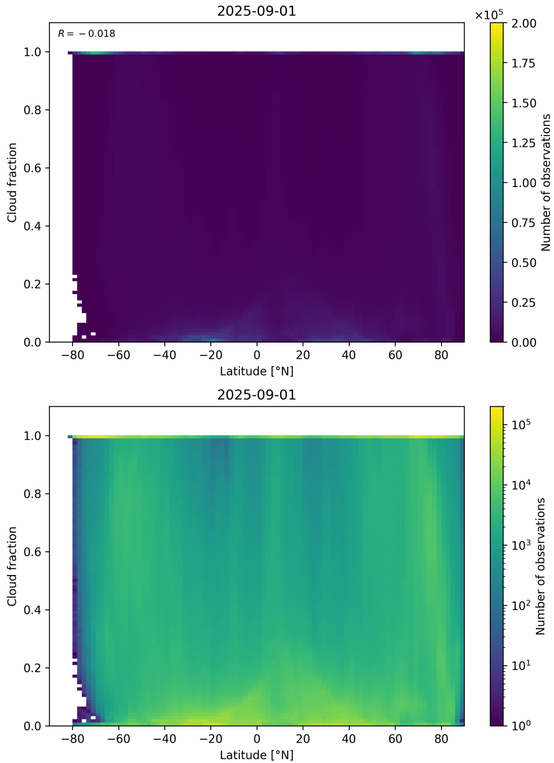
Figure 90: Scatter density plot of “Latitude” against “Cloud fraction” for 2025-08-31 to 2025-09-02.
