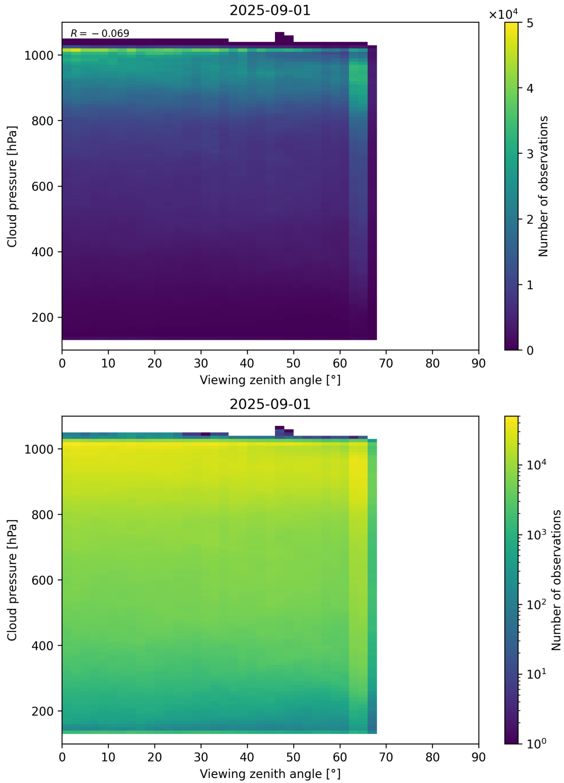
Figure 121: Scatter density plot of “Viewing zenith angle” against “Cloud pressure” for 2025-08-31 to 2025-09-02.
