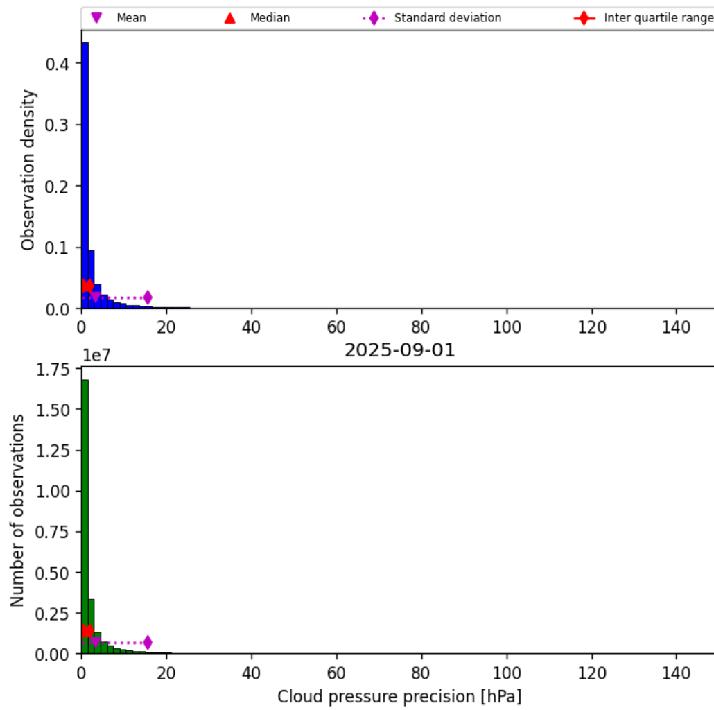
Figure 31: Histogram of “Cloud pressure precision” for 2025-08-31 to 2025-09-02
