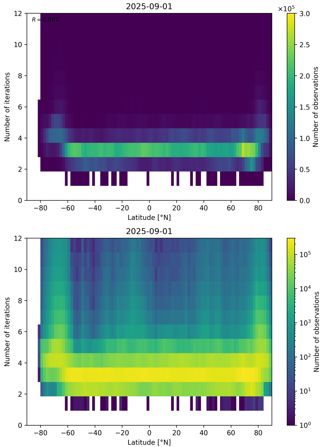
Figure 93: Scatter density plot of “Latitude” against “Number of iterations” for 2025-08-31 to 2025-09-02.
