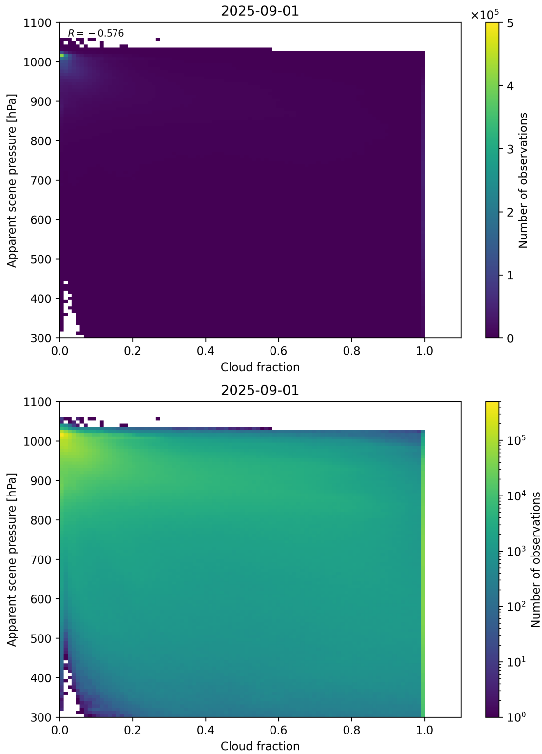
Figure 70: Scatter density plot of “Cloud fraction” against “Apparent scene pressure” for 2025-08-31 to 2025-09-02.
