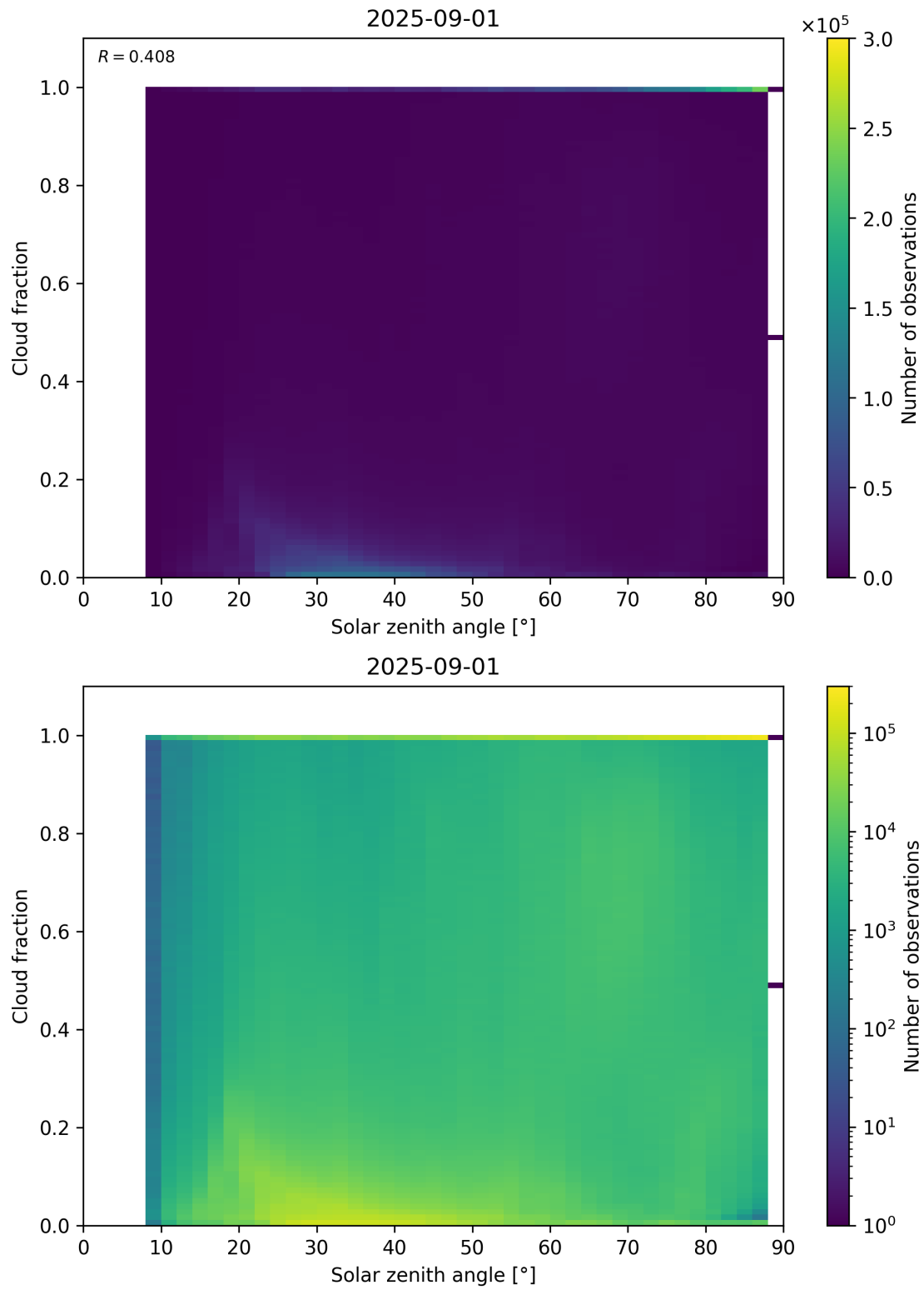
Figure 110: Scatter density plot of “Solar zenith angle” against “Cloud fraction” for 2025-08-31 to 2025-09-02.
