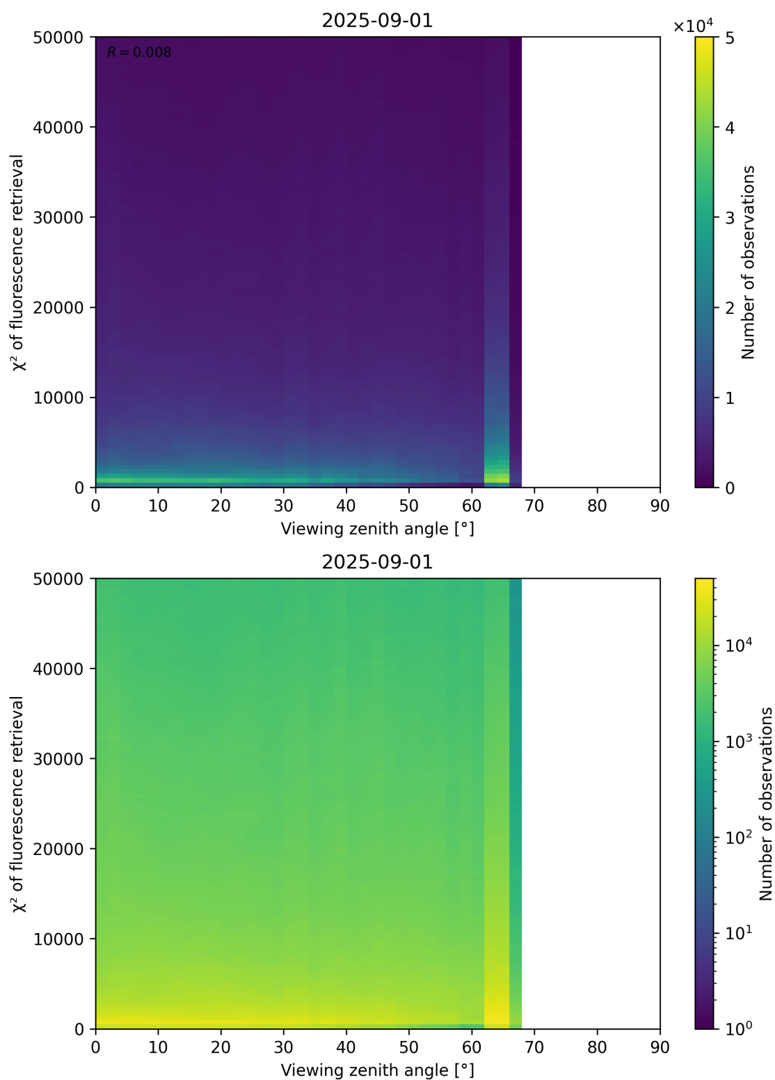
Figure 119: Scatter density plot of “Viewing zenith angle” against “ \chi^2 of fluorescence retrieval” for 2025-08-31 to 2025-09-02.
