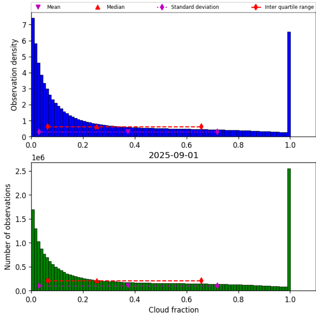
Figure 32: Histogram of “Cloud fraction” for 2025-08-31 to 2025-09-02
