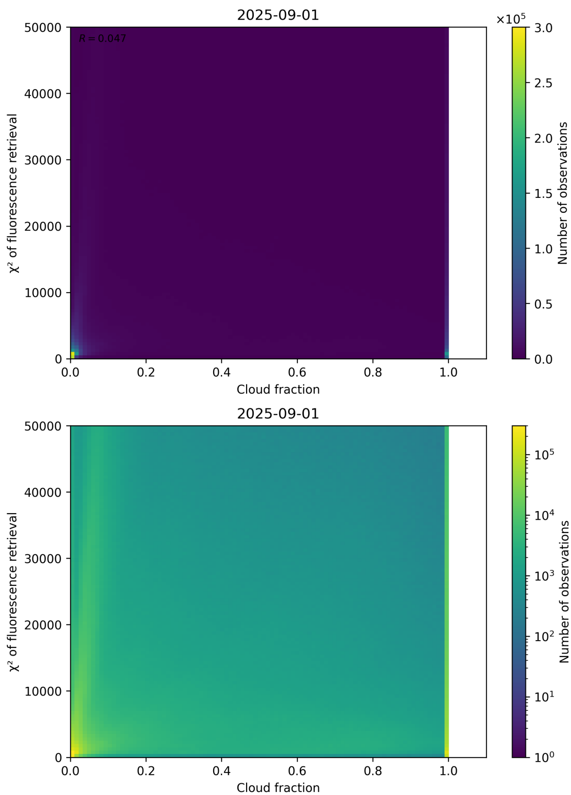
Figure 71: Scatter density plot of “Cloud fraction” against “ \chi^2 of fluorescence retrieval” for 2025-08-31 to 2025-09-02.
