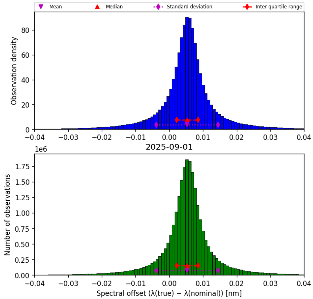
Figure 45: Histogram of “Spectral offset ( \lambda_{\text{true}} - \lambda_{\text{nominal}} )” for 2025-08-31 to 2025-09-02
