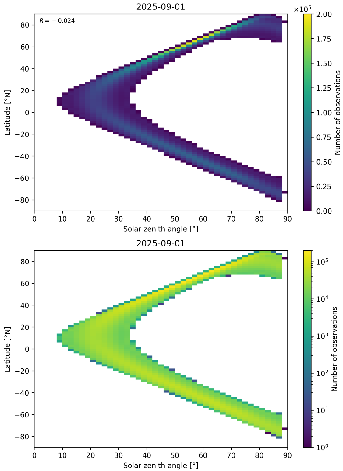
Figure 113: Scatter density plot of “Solar zenith angle” against “Latitude” for 2025-08-31 to 2025-09-02.
