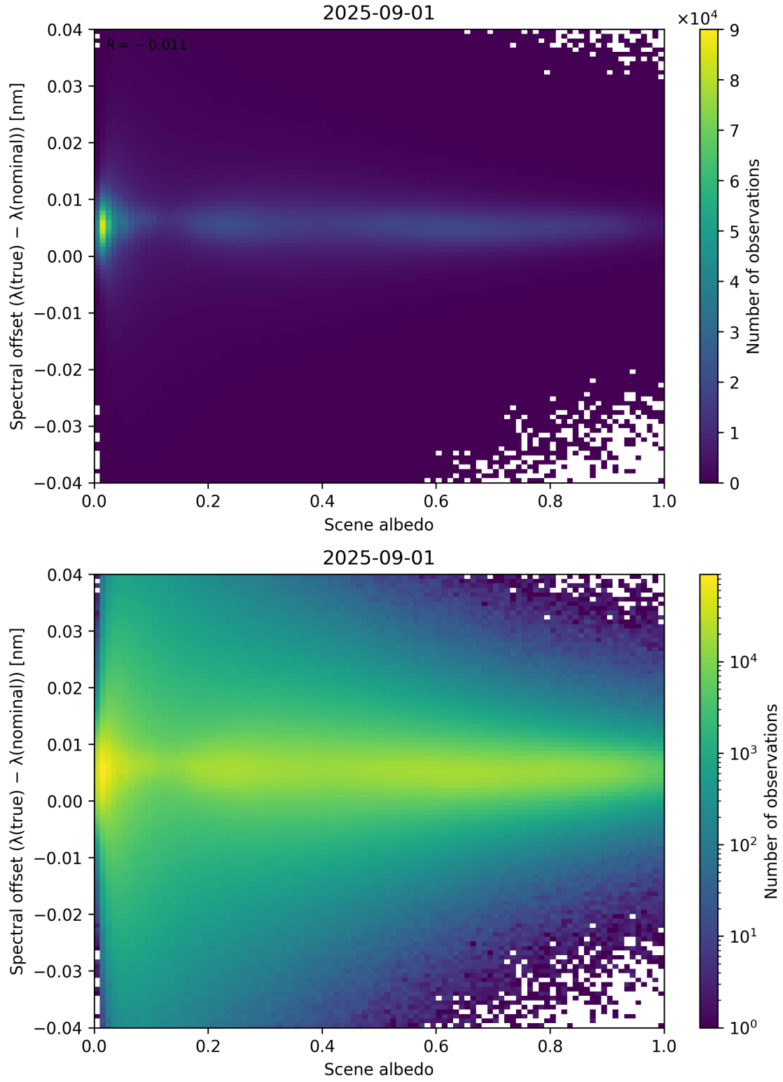
Figure 107: Scatter density plot of “Scene albedo” against “Spectral offset ( \lambda_{\text{true}} - \lambda_{\text{nominal}} )” for 2025-08-31 to 2025-09-02.
