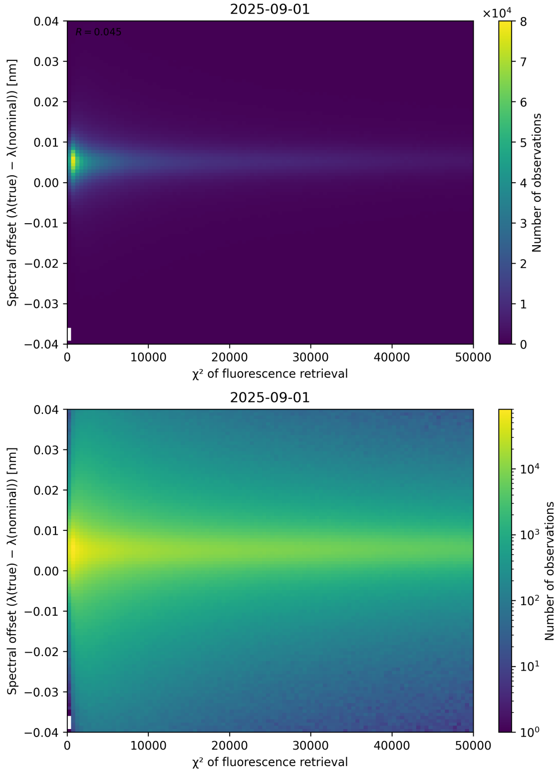
Figure 69: Scatter density plot of “ \chi^2 of fluorescence retrieval” against “Spectral offset ( \lambda_{\text{true}} - \lambda_{\text{nominal}} )” for 2025-08-31 to 2025-09-02.
