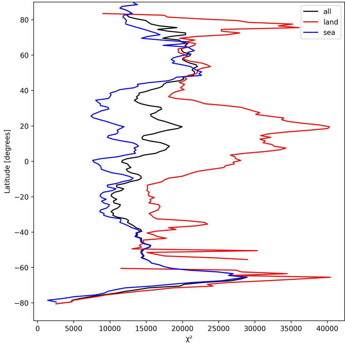
Figure 21: Zonal average of “ \chi^2 ” for 2025-08-31 to 2025-09-02.
