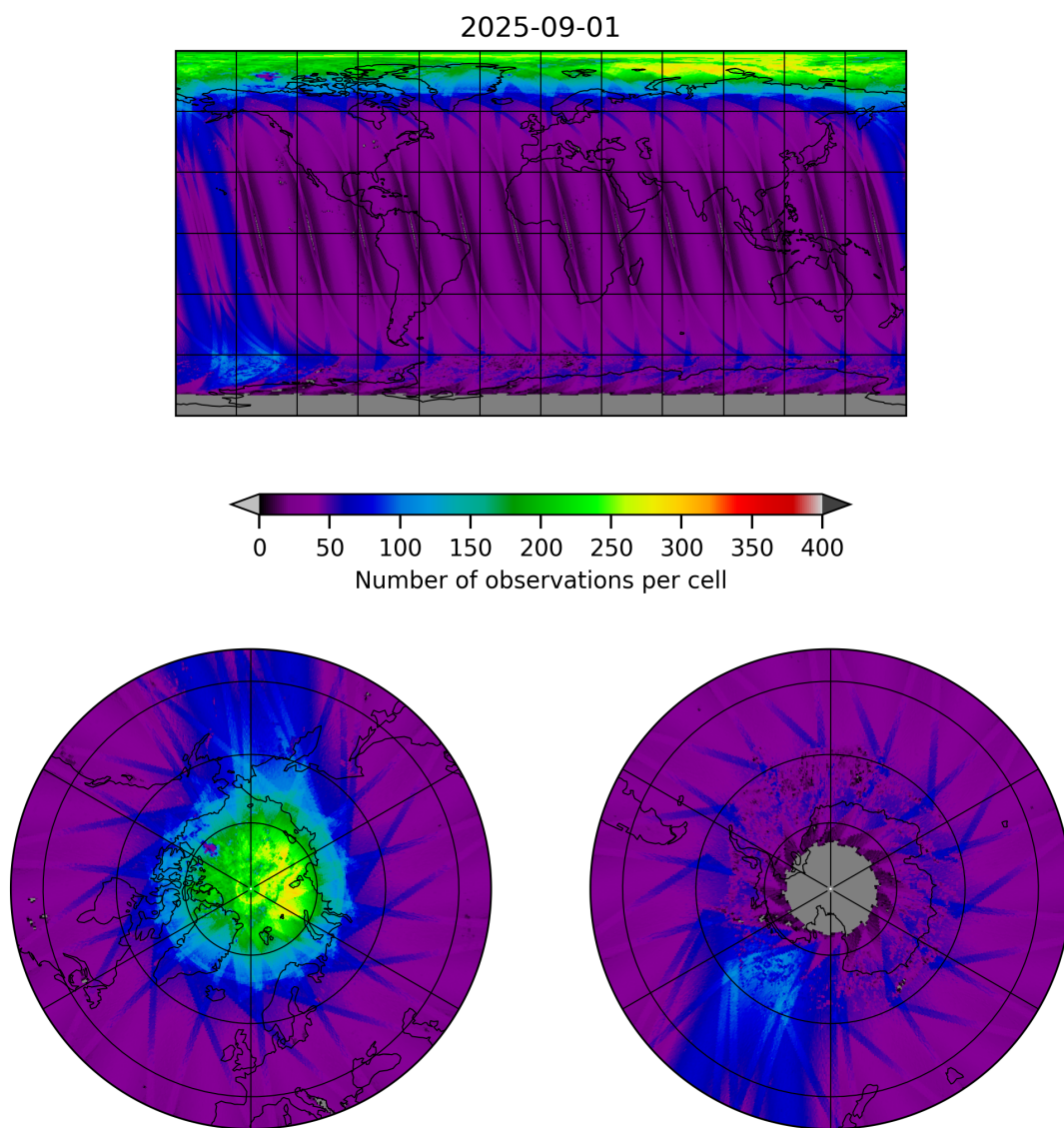
Figure 11: Map of the number of observations for 2025-08-31 to 2025-09-02
