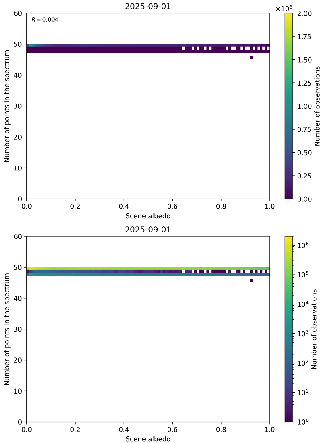
Figure 106: Scatter density plot of “Scene albedo” against “Number of points in the spectrum” for 2025-08-31 to 2025-09-02.
