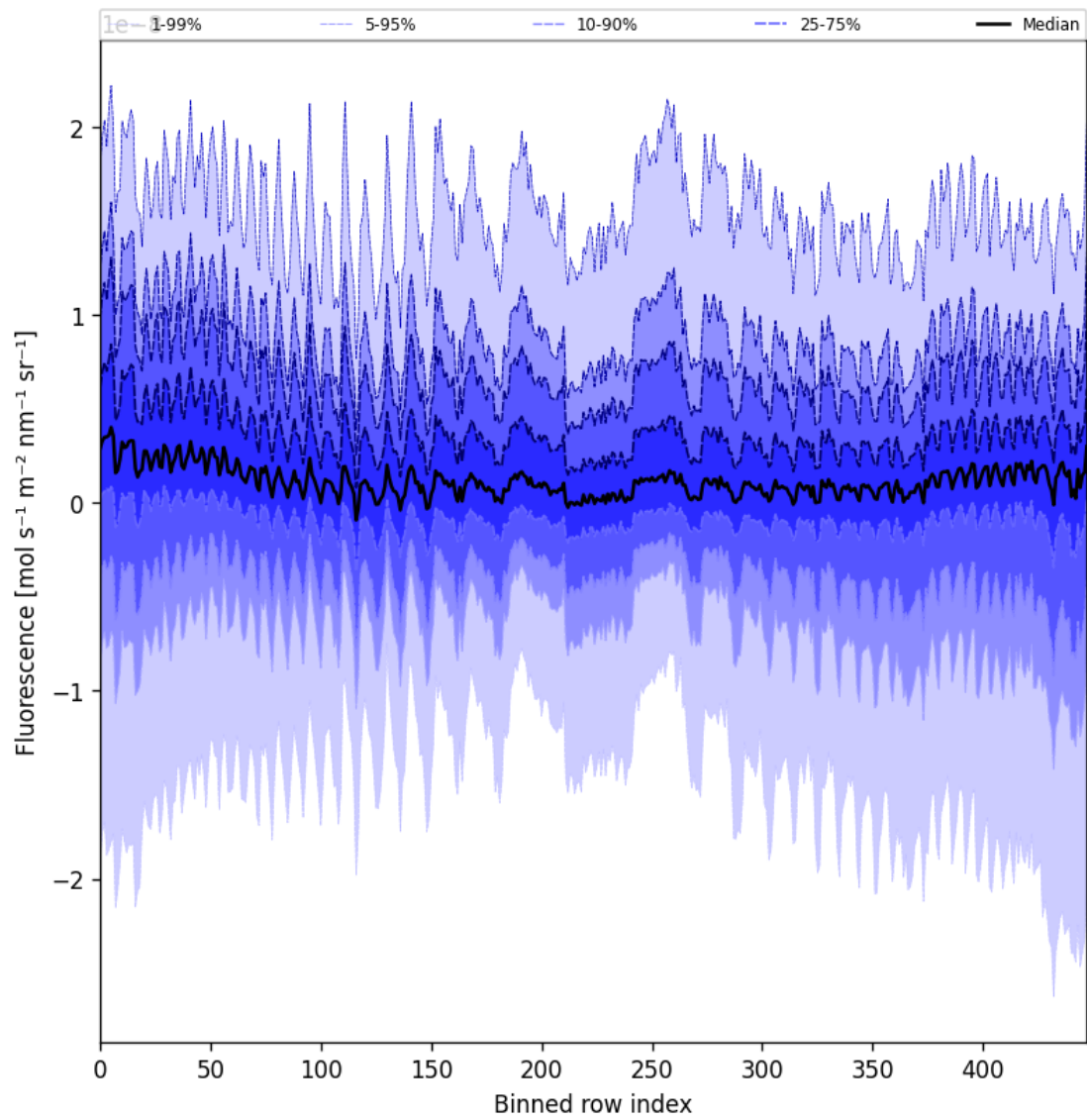
Figure 57: Along track statistics of “Fluorescence” for 2025-08-31 to 2025-09-02
