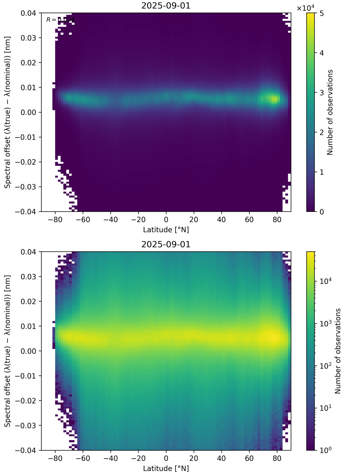
Figure 96: Scatter density plot of “Latitude” against “Spectral offset ( \lambda_{\text{true}} - \lambda_{\text{nominal}} )” for 2025-08-31 to 2025-09-02.
