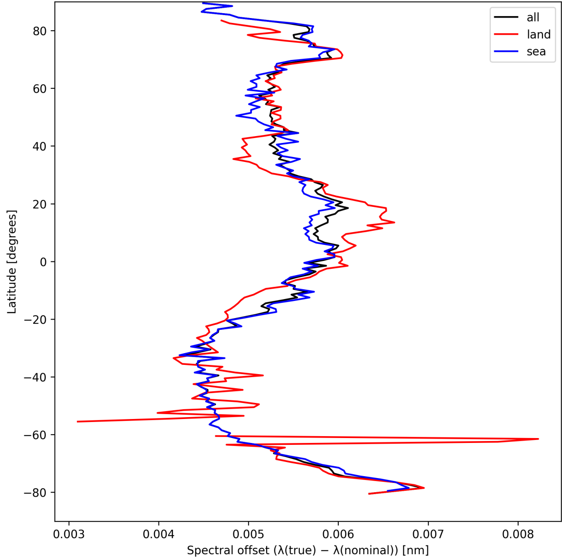
Figure 28: Zonal average of “Spectral offset ( \lambda_{\text{true}} - \lambda_{\text{nominal}} )” for 2025-08-31 to 2025-09-02.
