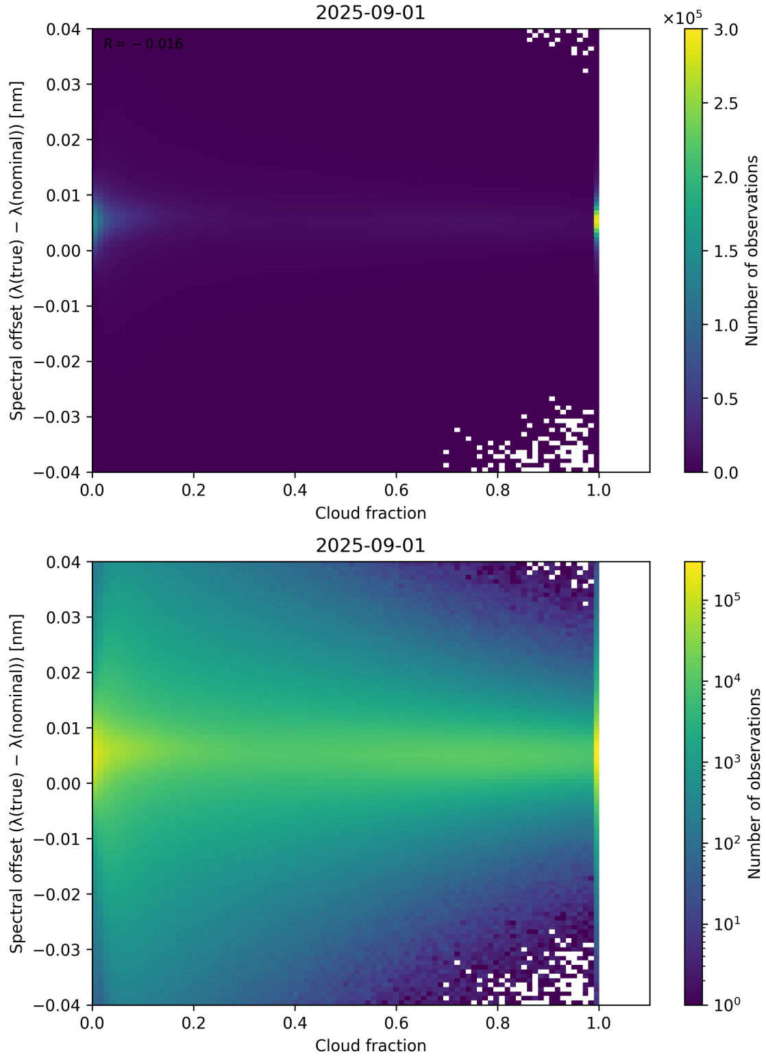
Figure 76: Scatter density plot of “Cloud fraction” against “Spectral offset ( \lambda_{\text{true}} - \lambda_{\text{nominal}} )” for 2025-08-31 to 2025-09-02.
