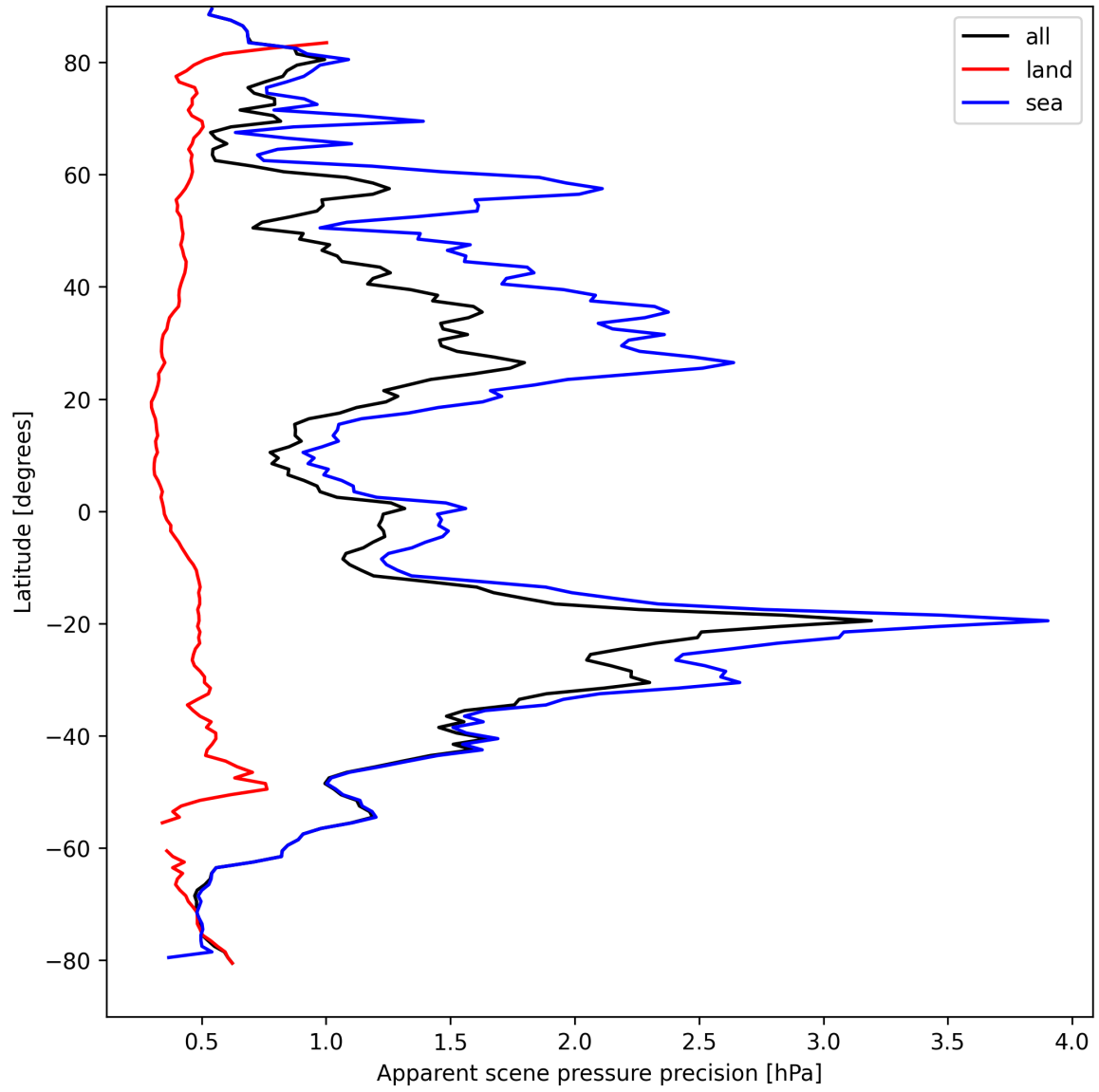
Figure 20: Zonal average of “Apparent scene pressure precision” for 2025-08-31 to 2025-09-02.
