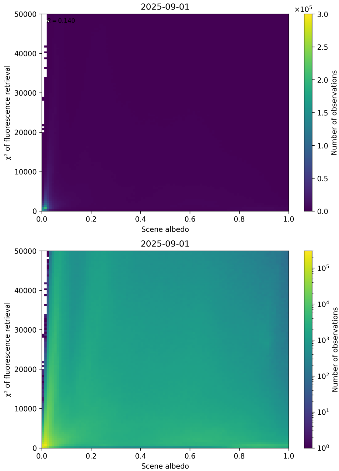
Figure 103: Scatter density plot of “Scene albedo” against “ \chi^2 of fluorescence retrieval” for 2025-08-31 to 2025-09-02.
