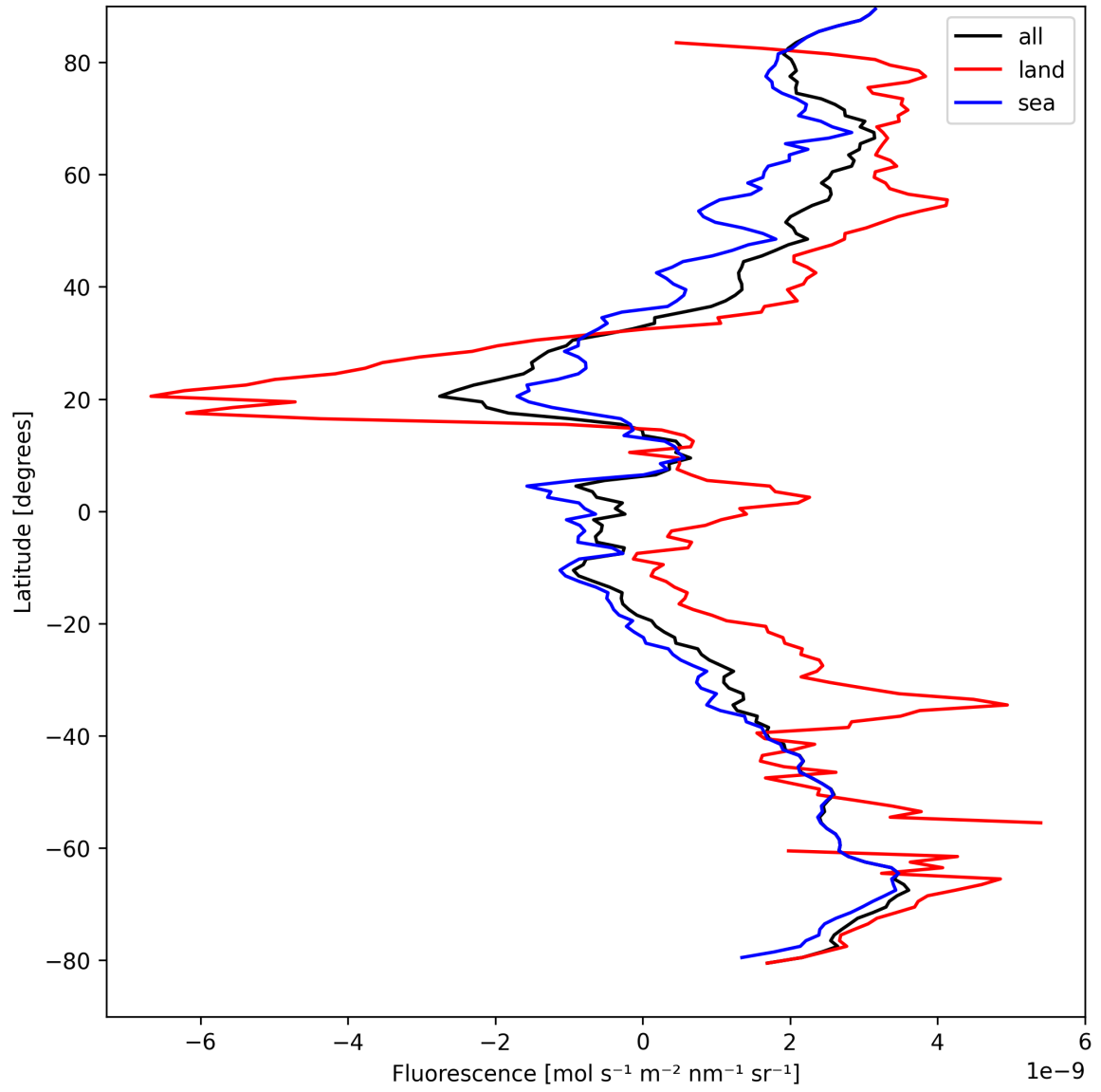
Figure 23: Zonal average of “Fluorescence” for 2025-08-31 to 2025-09-02.
