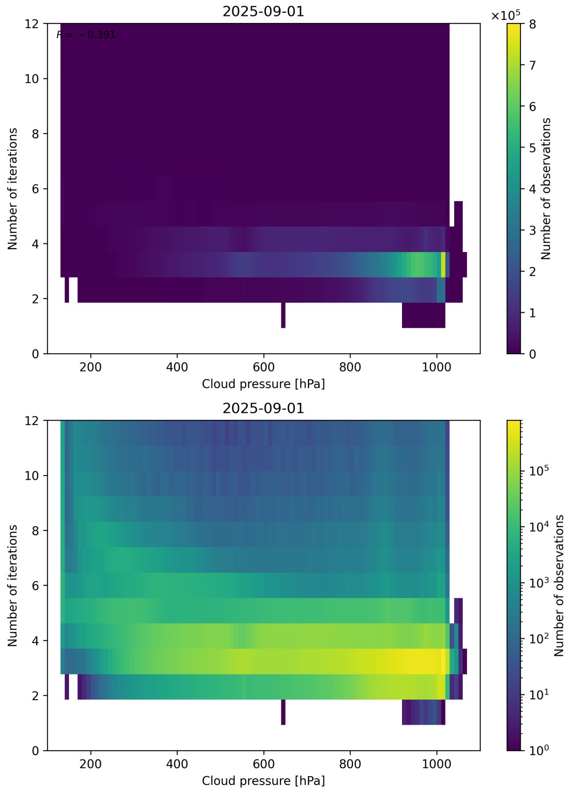
Figure 81: Scatter density plot of “Cloud pressure” against “Number of iterations” for 2025-08-31 to 2025-09-02.
