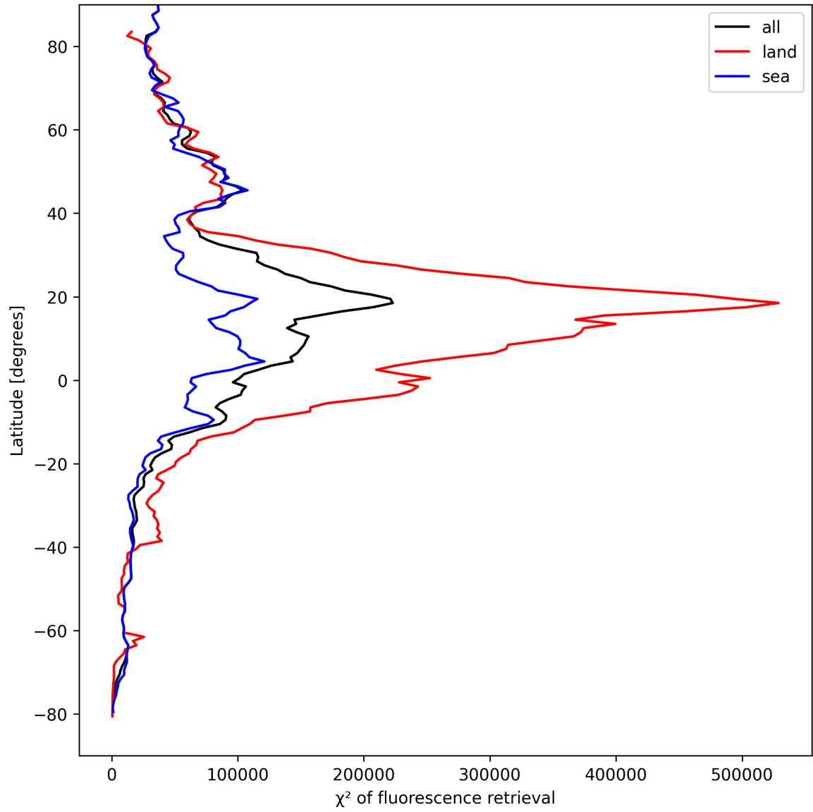
Figure 25: Zonal average of “ \chi^2 of fluorescence retrieval” for 2025-08-31 to 2025-09-02.
