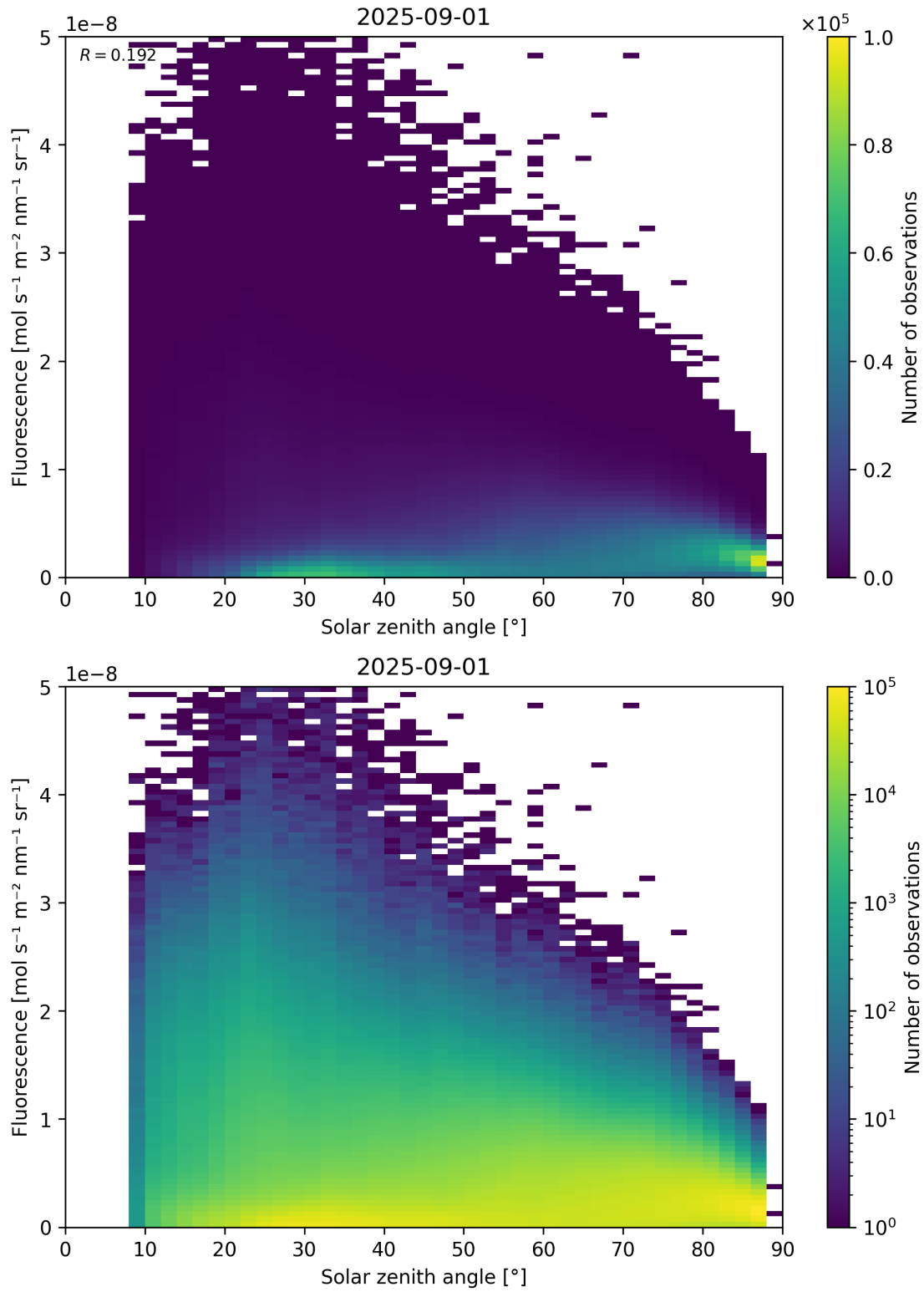
Figure 112: Scatter density plot of “Solar zenith angle” against “Fluorescence” for 2025-08-31 to 2025-09-02.
