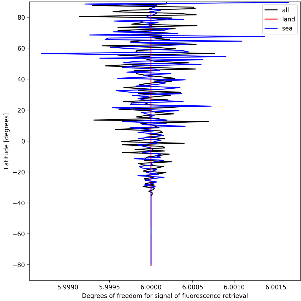
Figure 26: Zonal average of “Degrees of freedom for signal of fluorescence retrieval” for 2025-08-31 to 2025-09-02.
