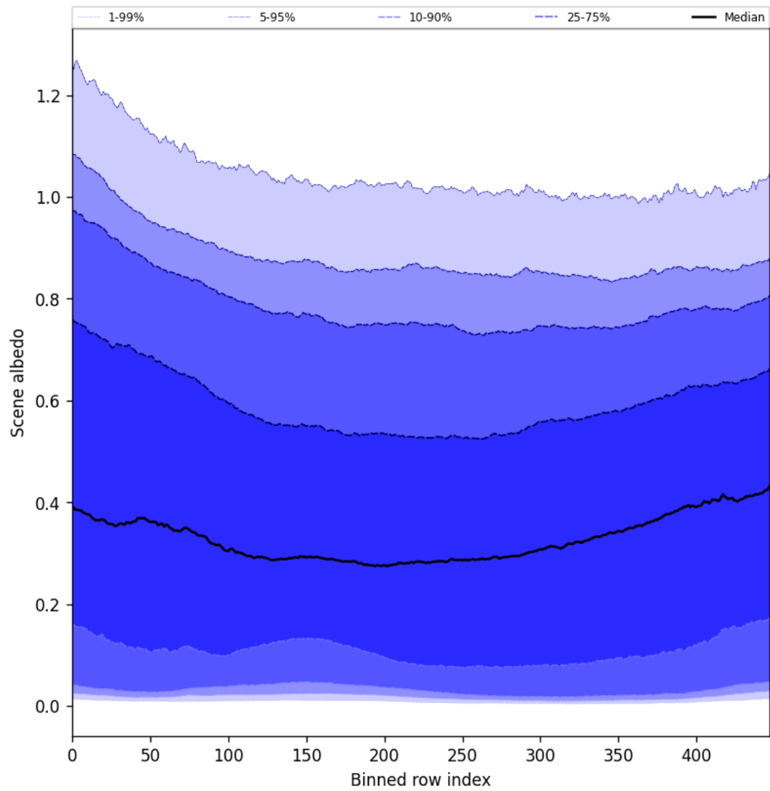
Figure 51: Along track statistics of “Scene albedo” for 2025-08-31 to 2025-09-02
