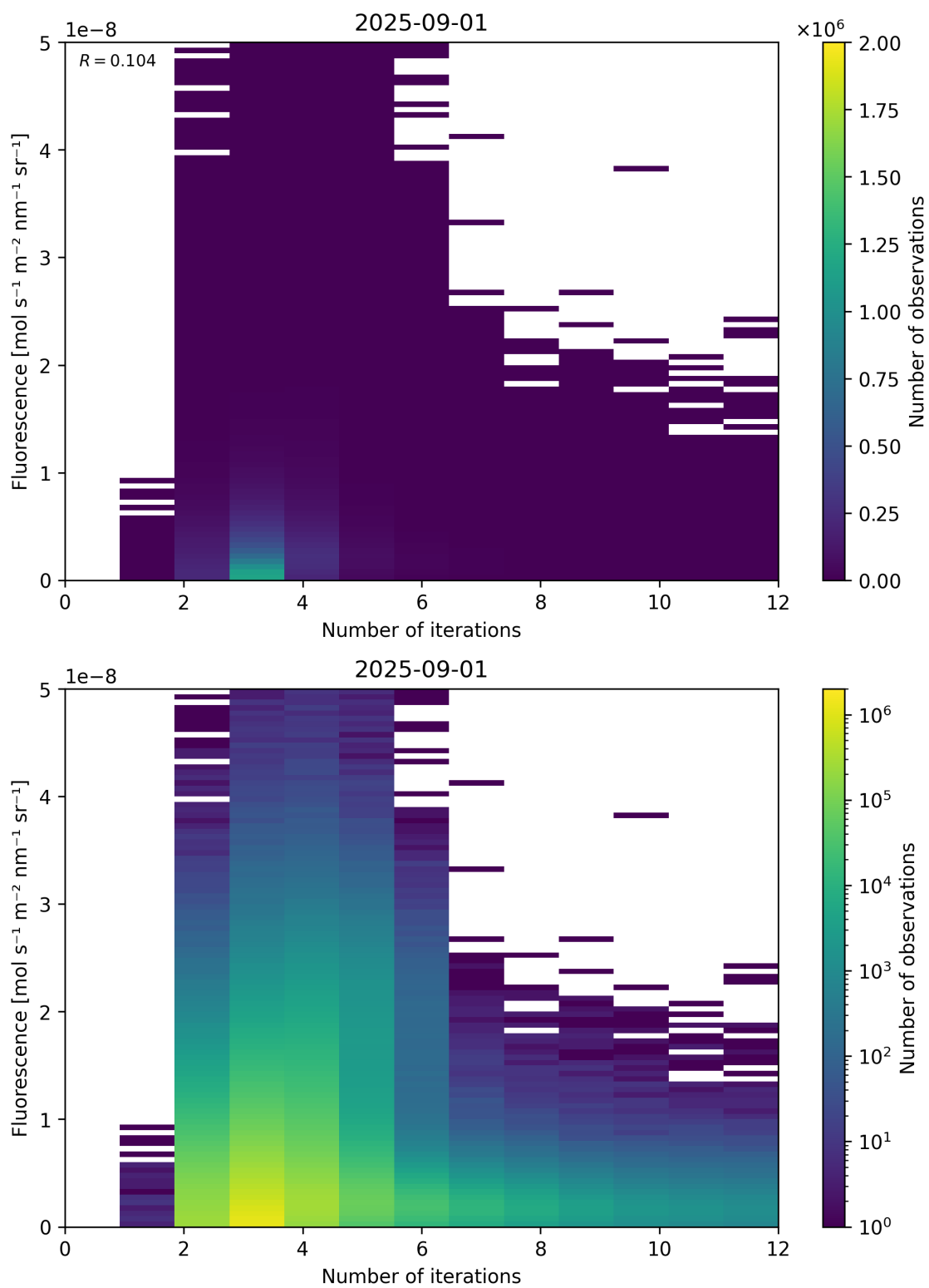
Figure 98: Scatter density plot of “Number of iterations” against “Fluorescence” for 2025-08-31 to 2025-09-02.
