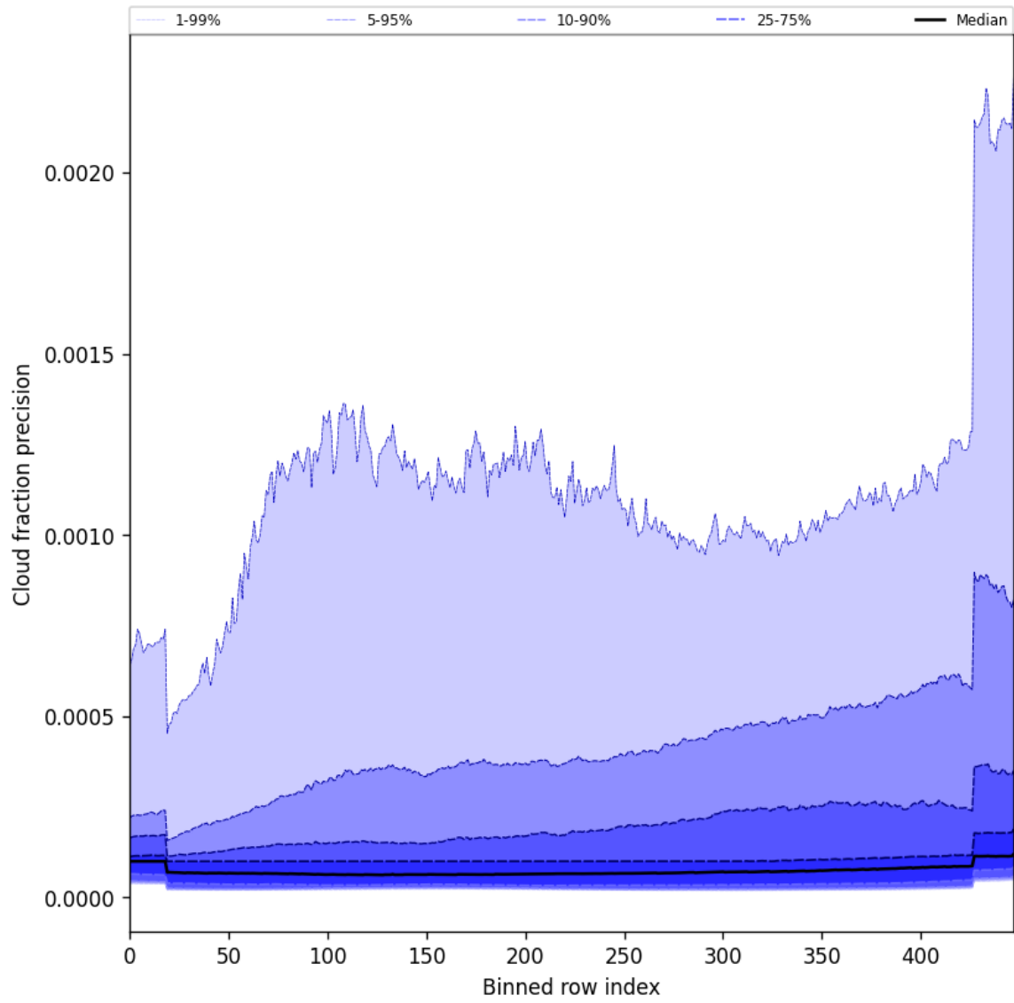
Figure 50: Along track statistics of “Cloud fraction precision” for 2025-08-31 to 2025-09-02
