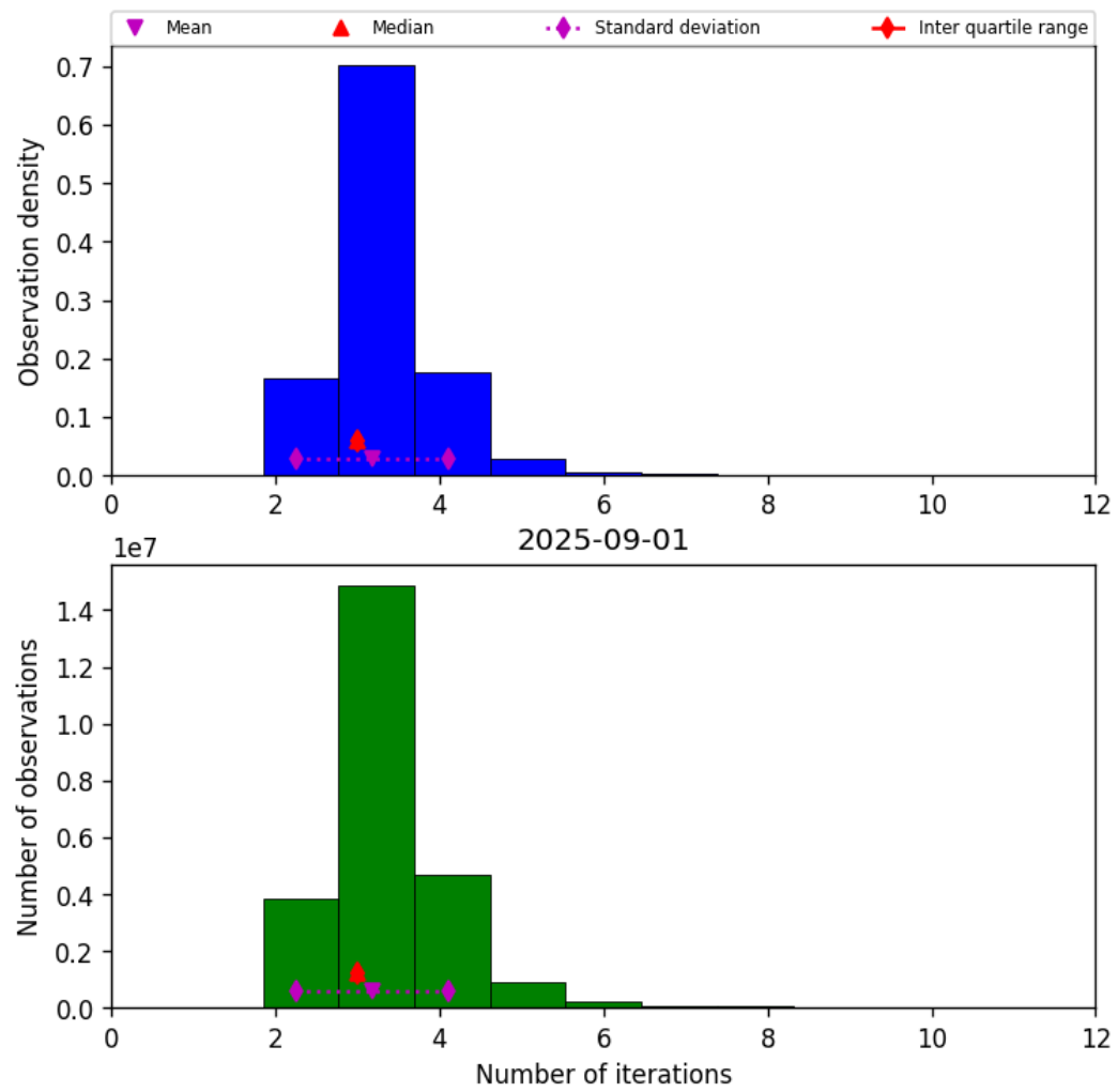
Figure 39: Histogram of “Number of iterations” for 2025-08-31 to 2025-09-02
