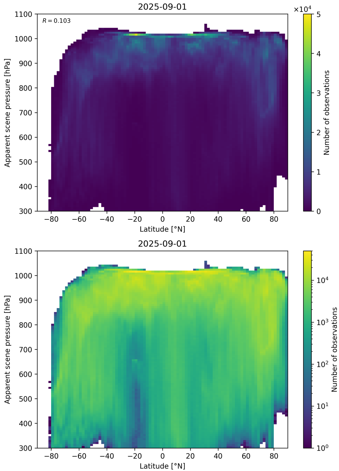
Figure 88: Scatter density plot of “Latitude” against “Apparent scene pressure” for 2025-08-31 to 2025-09-02.
