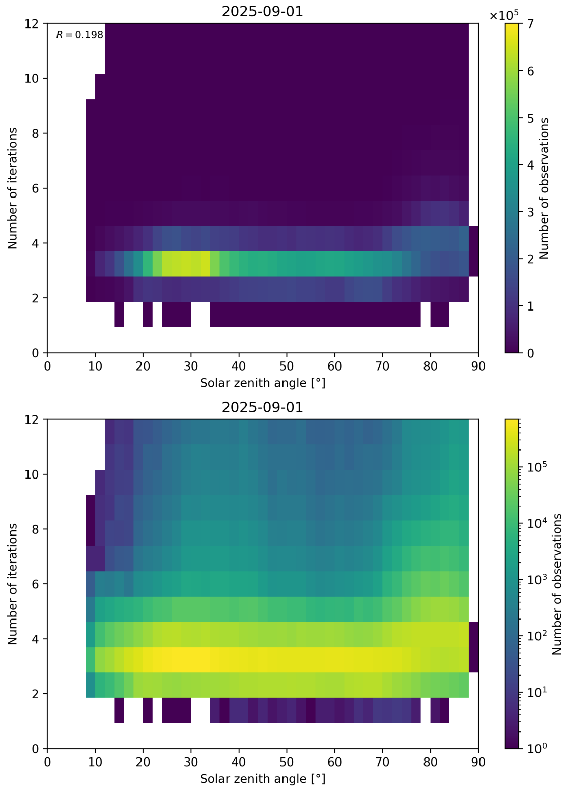
Figure 114: Scatter density plot of “Solar zenith angle” against “Number of iterations” for 2025-08-31 to 2025-09-02.
