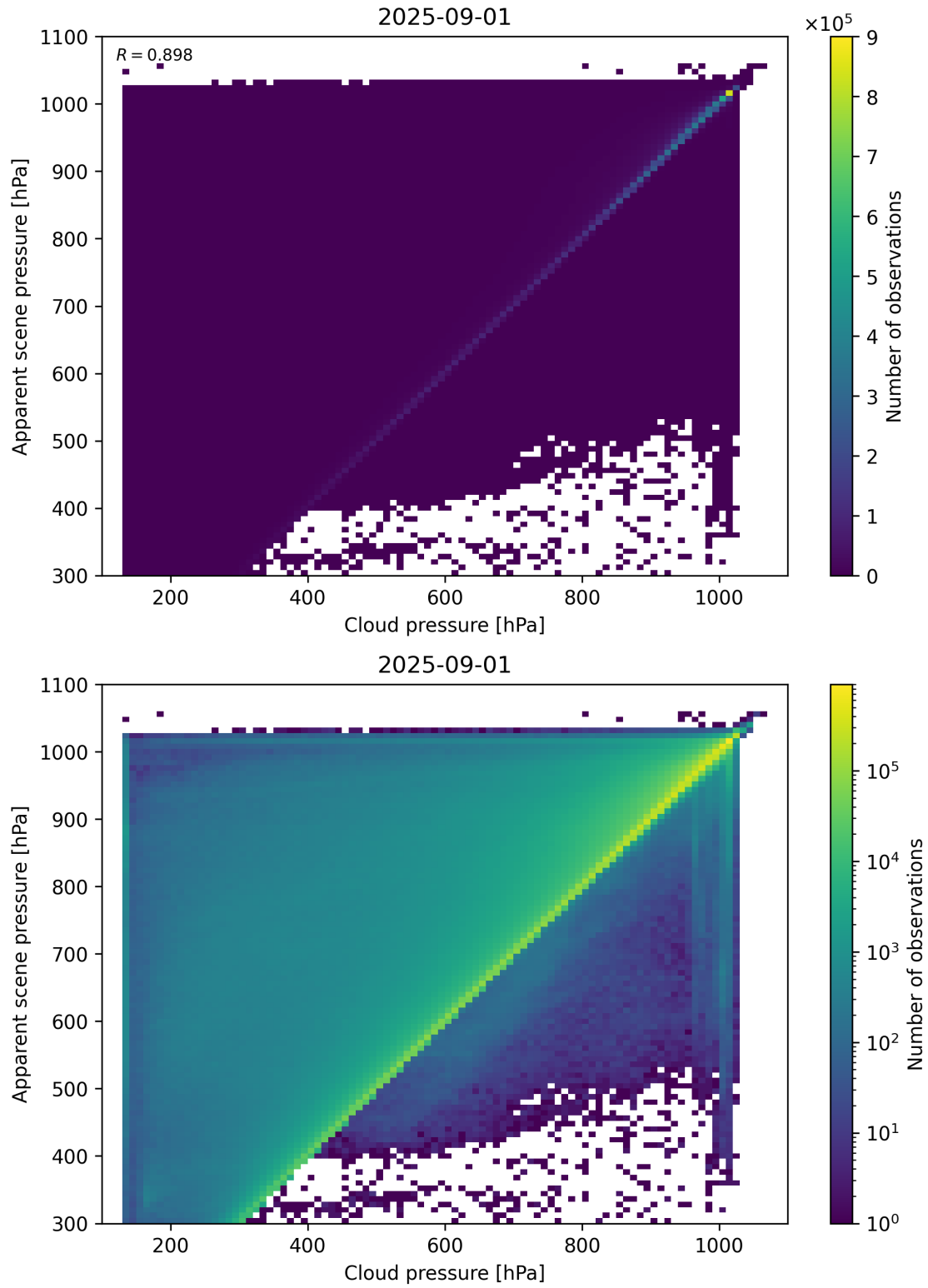
Figure 77: Scatter density plot of “Cloud pressure” against “Apparent scene pressure” for 2025-08-31 to 2025-09-02.
