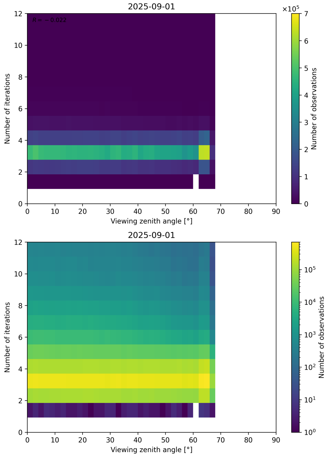
Figure 124: Scatter density plot of “Viewing zenith angle” against “Number of iterations” for 2025-08-31 to 2025-09-02.
