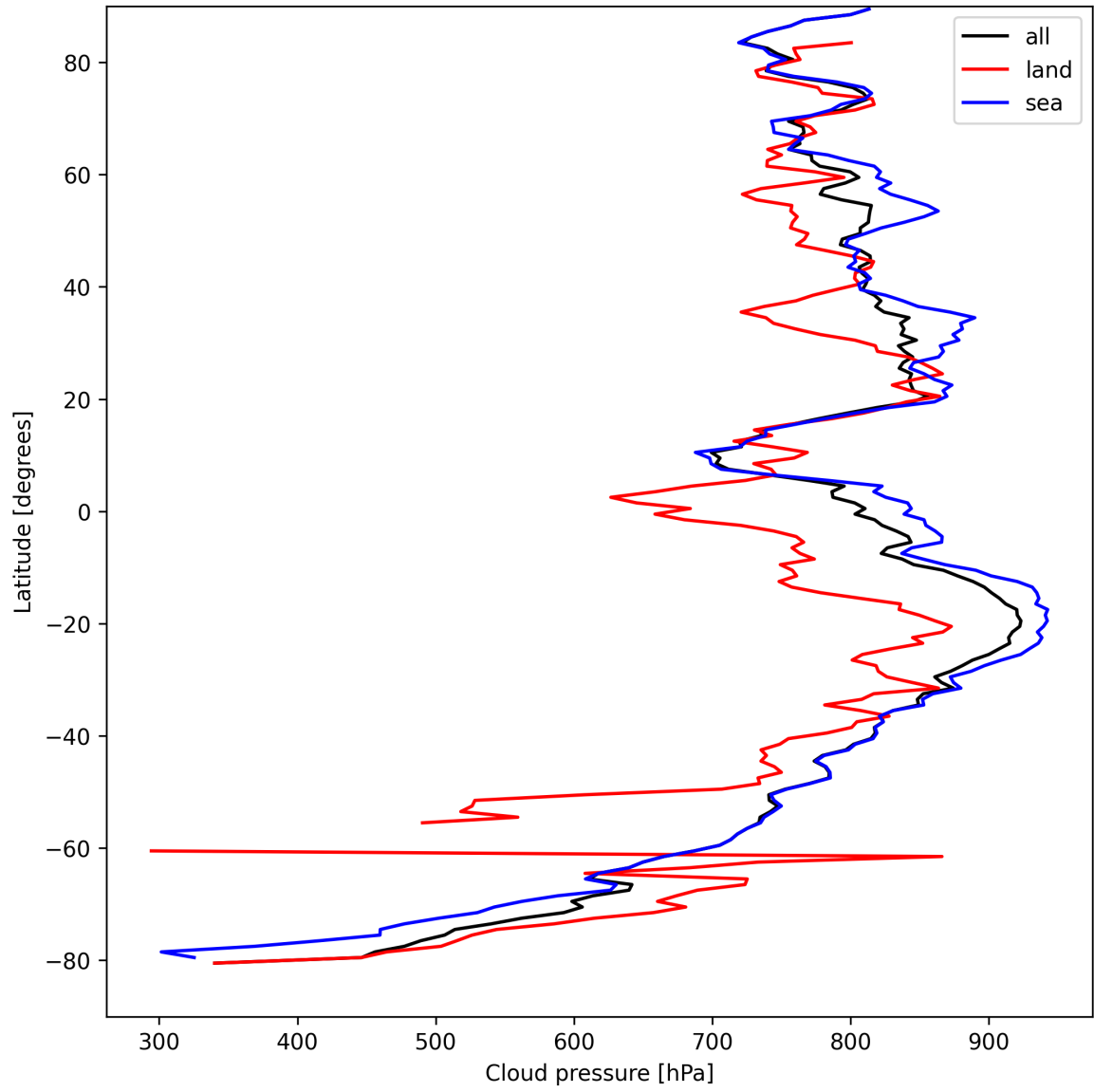
Figure 13: Zonal average of “Cloud pressure” for 2025-08-31 to 2025-09-02.
