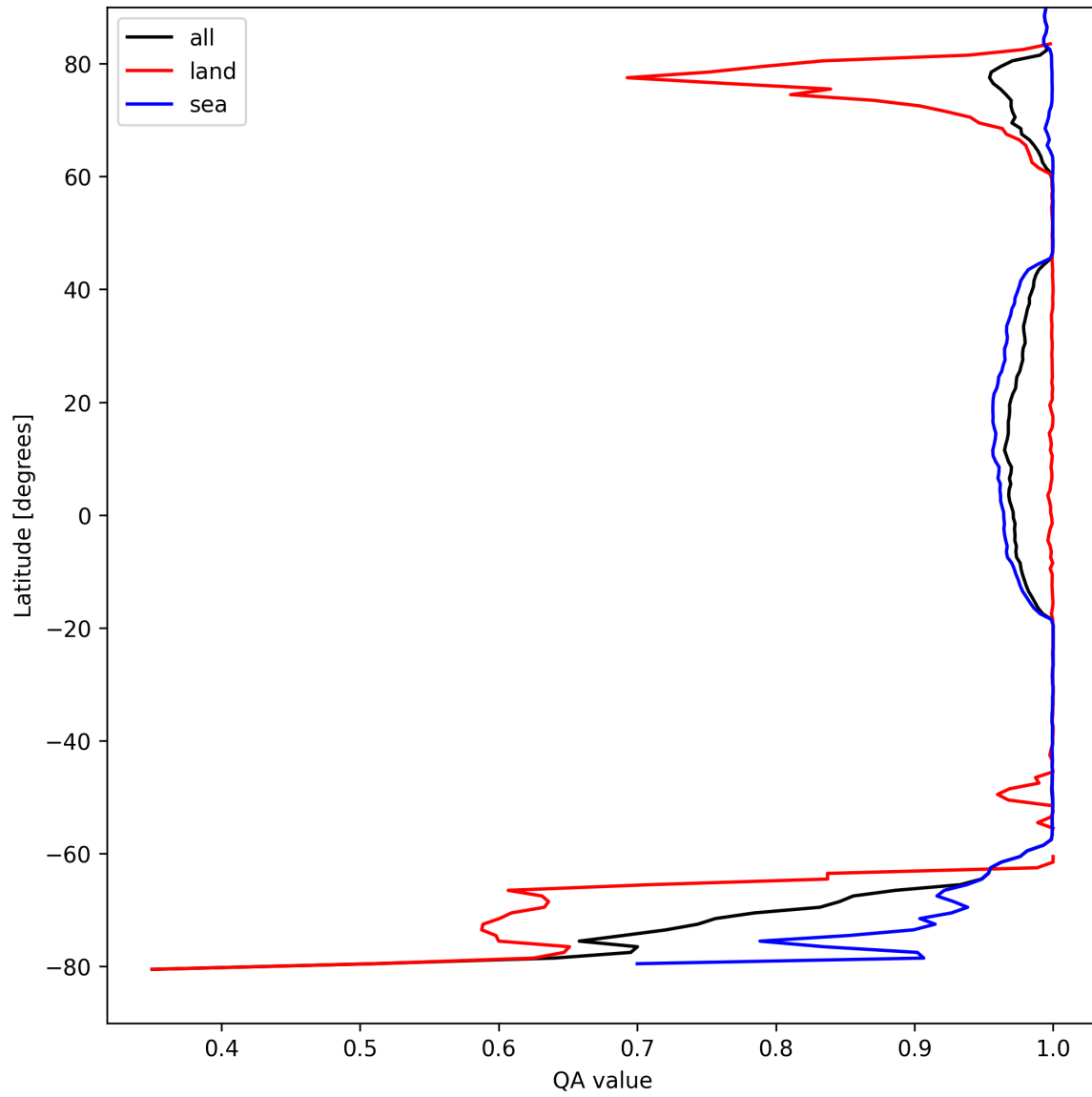
Figure 12: Zonal average of "QA value" for 2025-08-31 to 2025-09-02.
