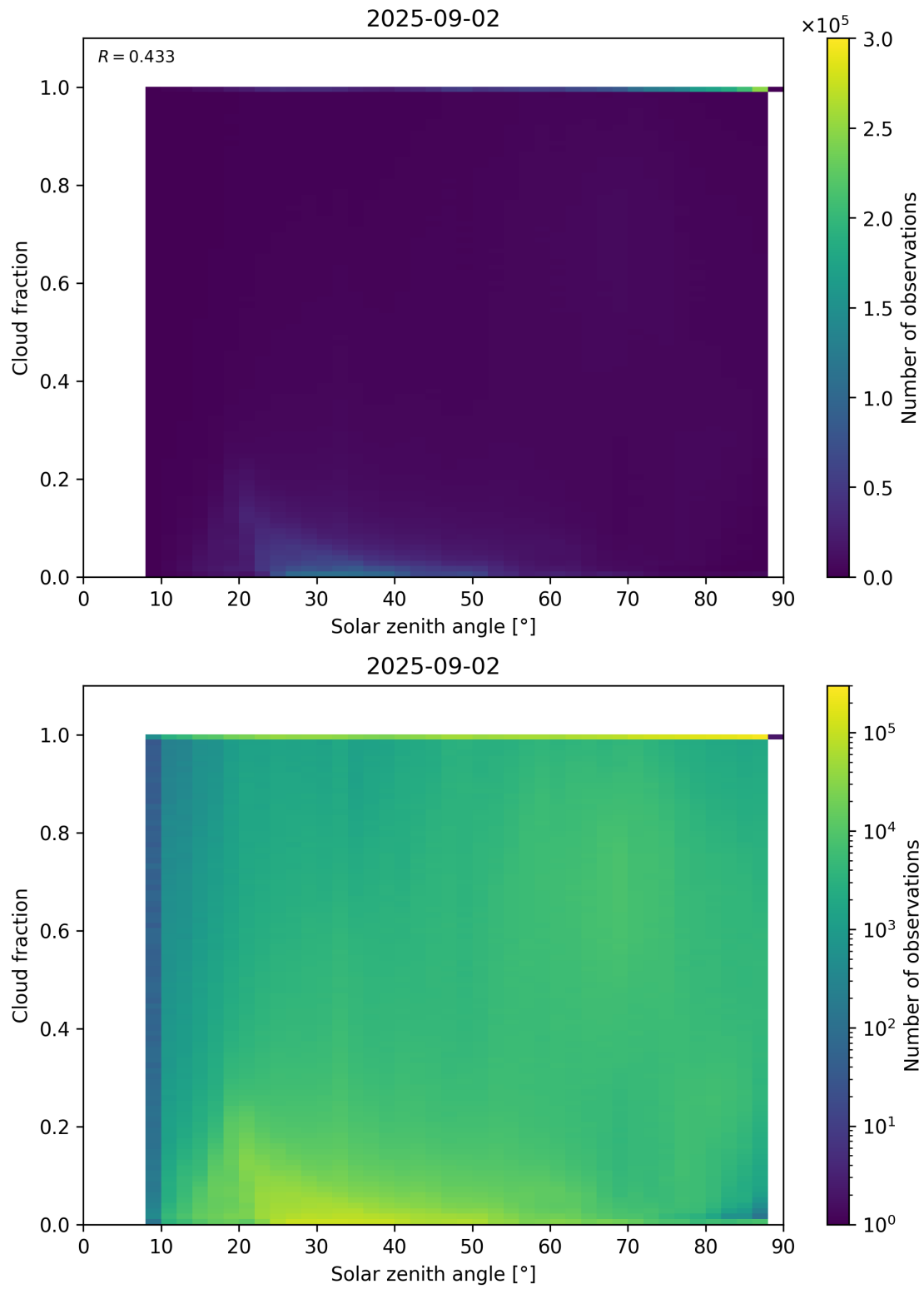
Figure 110: Scatter density plot of “Solar zenith angle” against “Cloud fraction” for 2025-09-01 to 2025-09-03.
