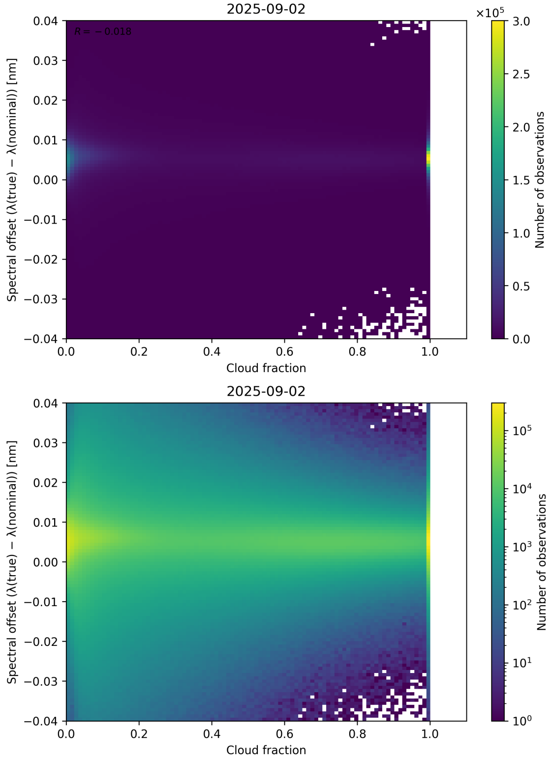
Figure 76: Scatter density plot of “Cloud fraction” against “Spectral offset ( \lambda_{\text{true}} - \lambda_{\text{nominal}} )” for 2025-09-01 to 2025-09-03.
