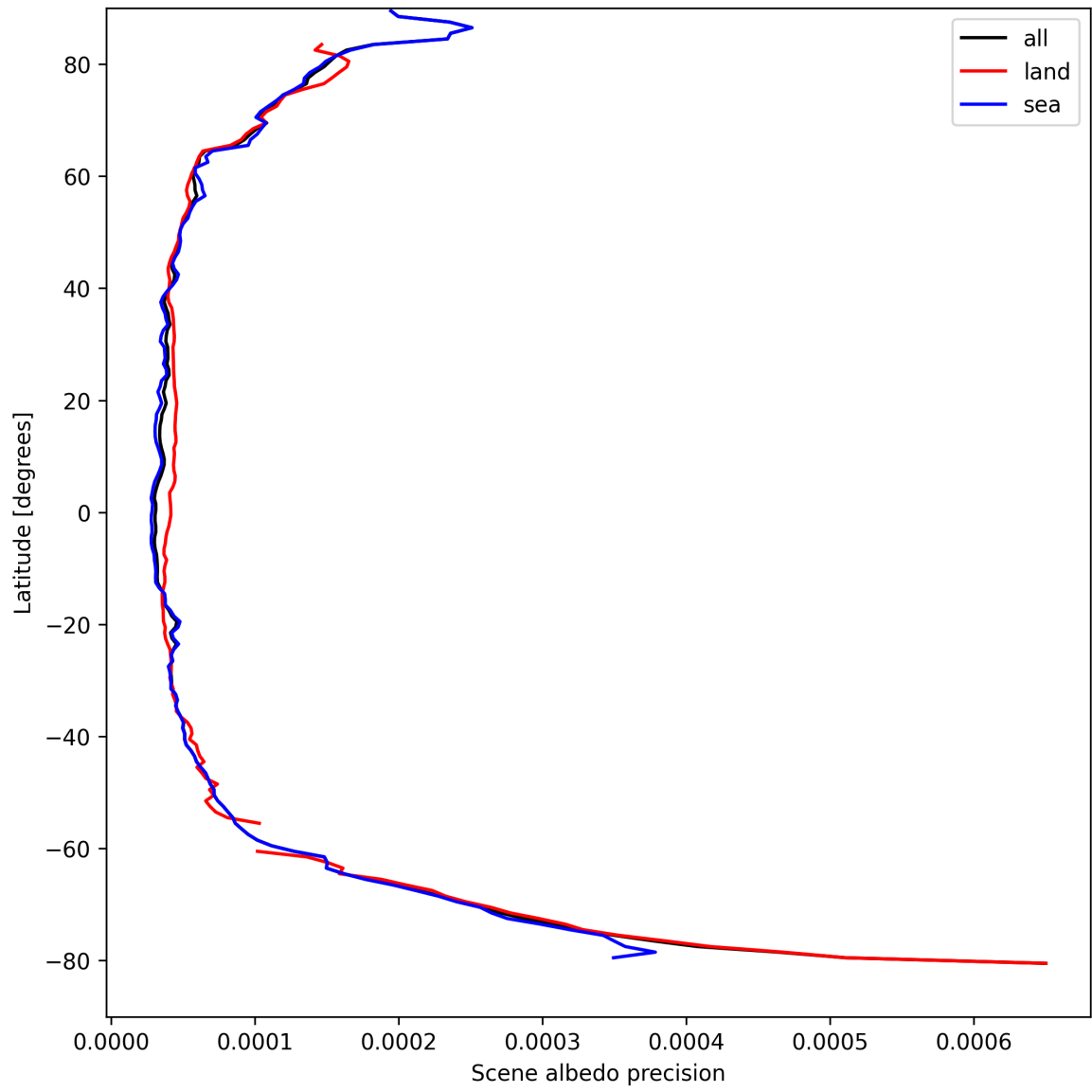
Figure 18: Zonal average of “Scene albedo precision” for 2025-09-01 to 2025-09-03.
