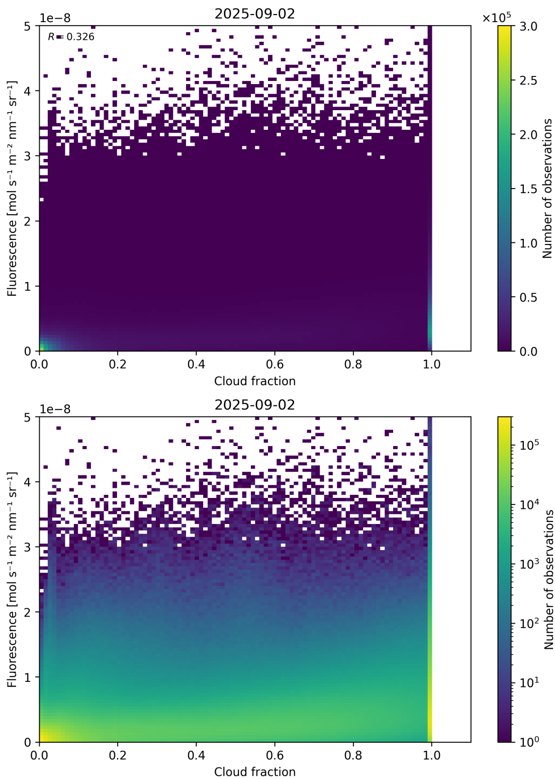
Figure 72: Scatter density plot of “Cloud fraction” against “Fluorescence” for 2025-09-01 to 2025-09-03.
