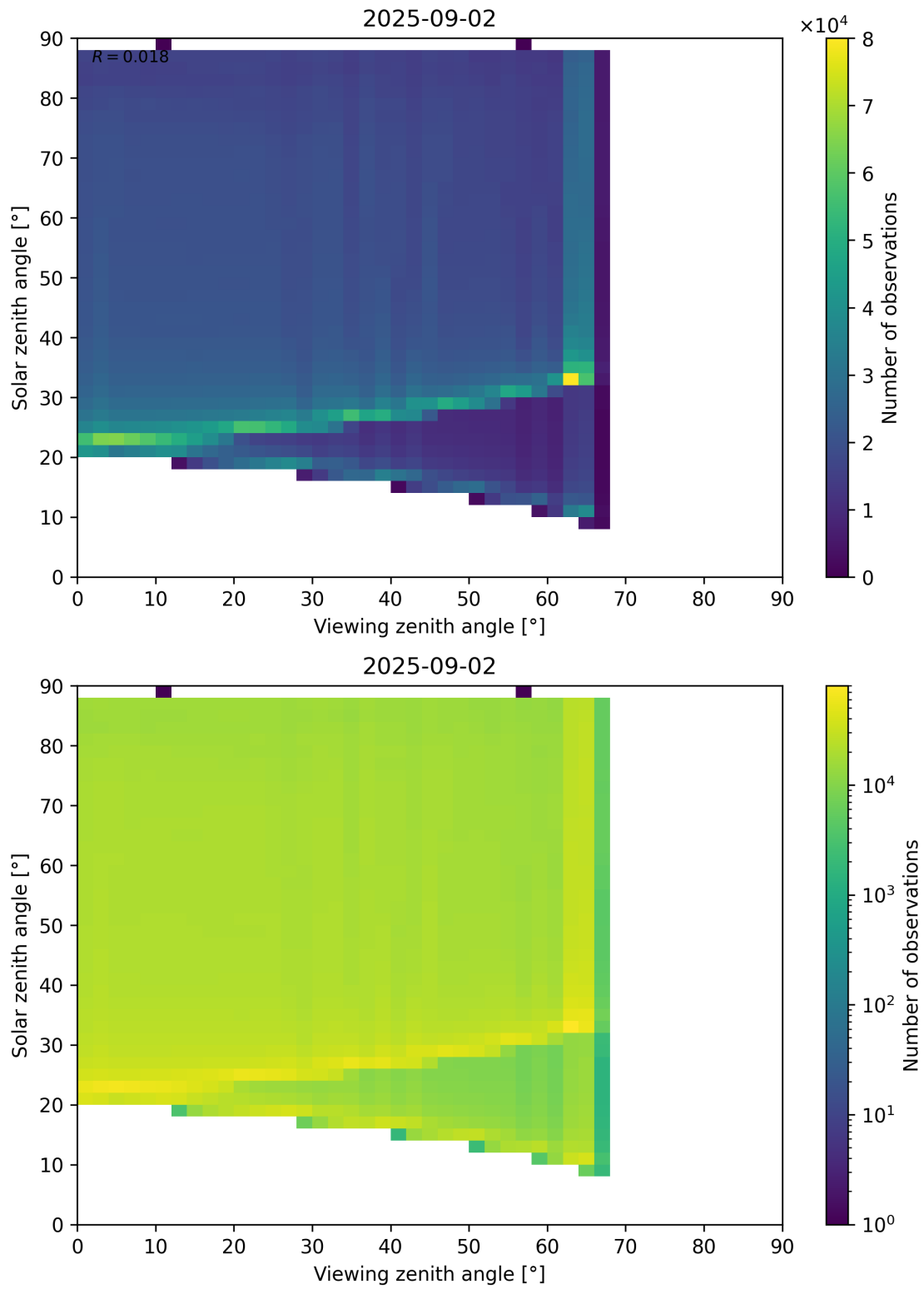
Figure 127: Scatter density plot of “Viewing zenith angle” against “Solar zenith angle” for 2025-09-01 to 2025-09-03.
