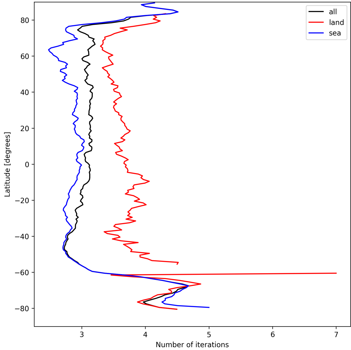
Figure 22: Zonal average of “Number of iterations” for 2025-09-01 to 2025-09-03.
