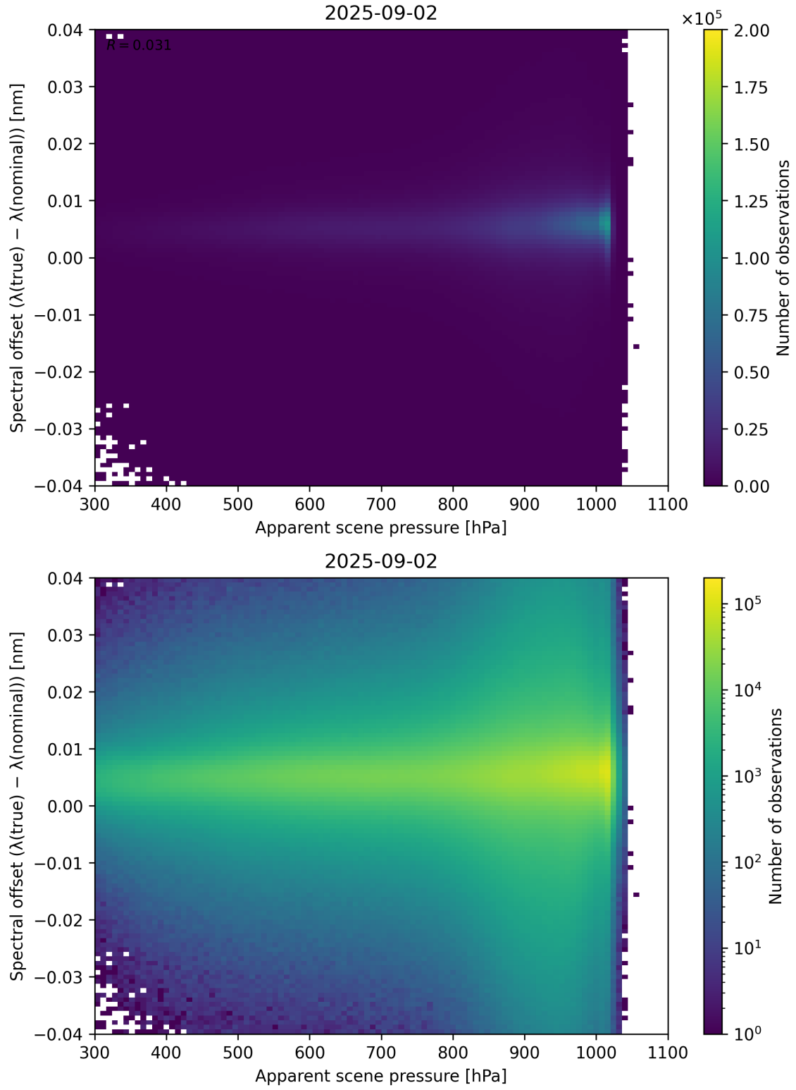
Figure 67: Scatter density plot of “Apparent scene pressure” against “Spectral offset ( \lambda_{\text{true}} - \lambda_{\text{nominal}} )” for 2025-09-01 to 2025-09-03.
