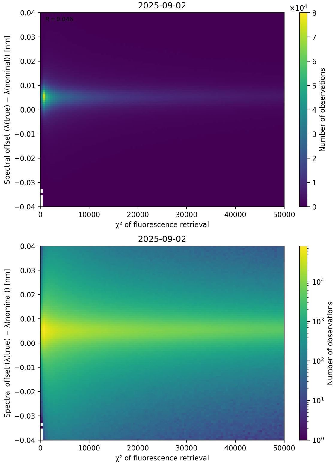
Figure 69: Scatter density plot of “ \chi^2 of fluorescence retrieval” against “Spectral offset ( \lambda_{\text{true}} - \lambda_{\text{nominal}} )” for 2025-09-01 to 2025-09-03.
