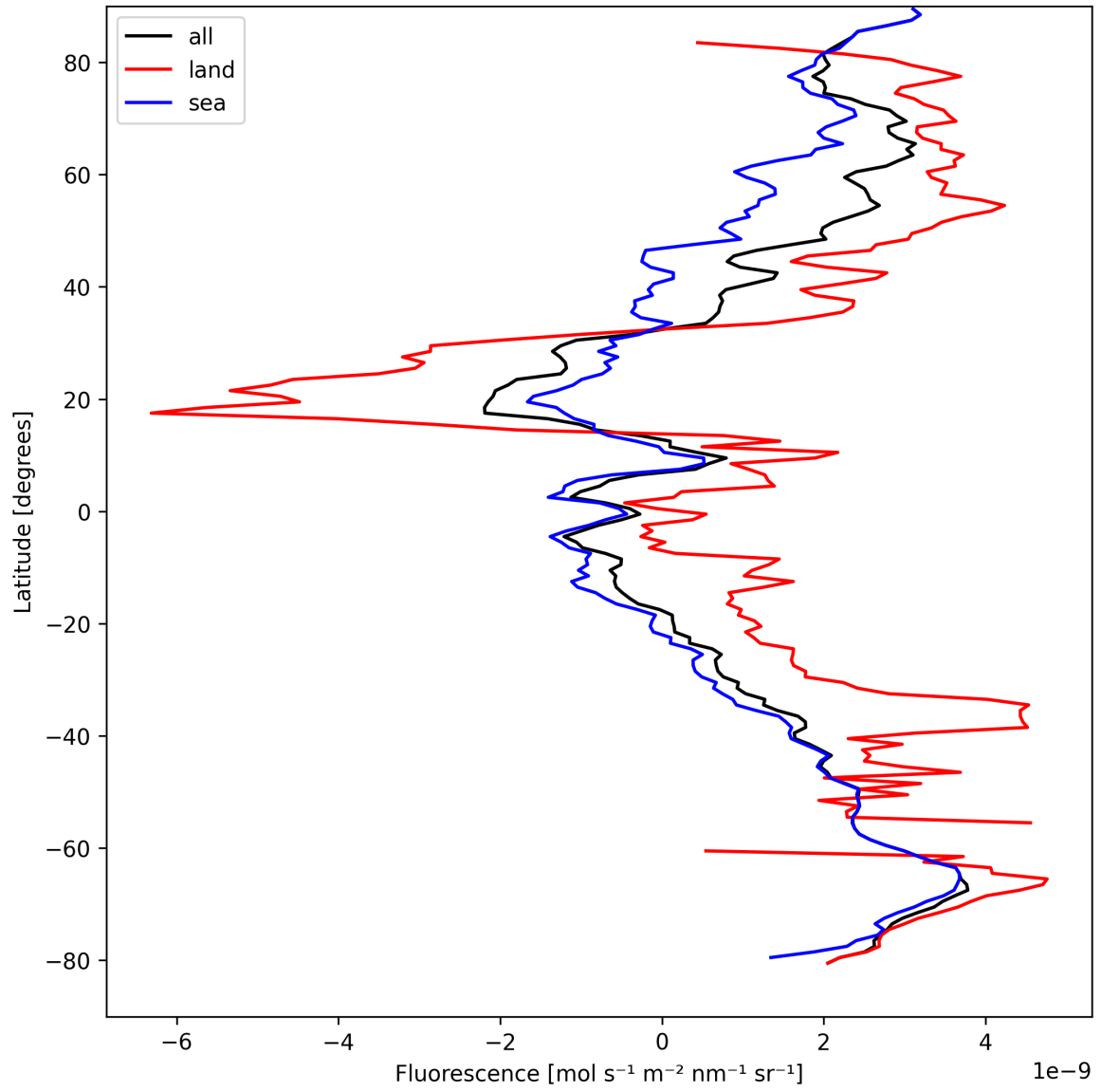
Figure 23: Zonal average of “Fluorescence” for 2025-09-01 to 2025-09-03.
