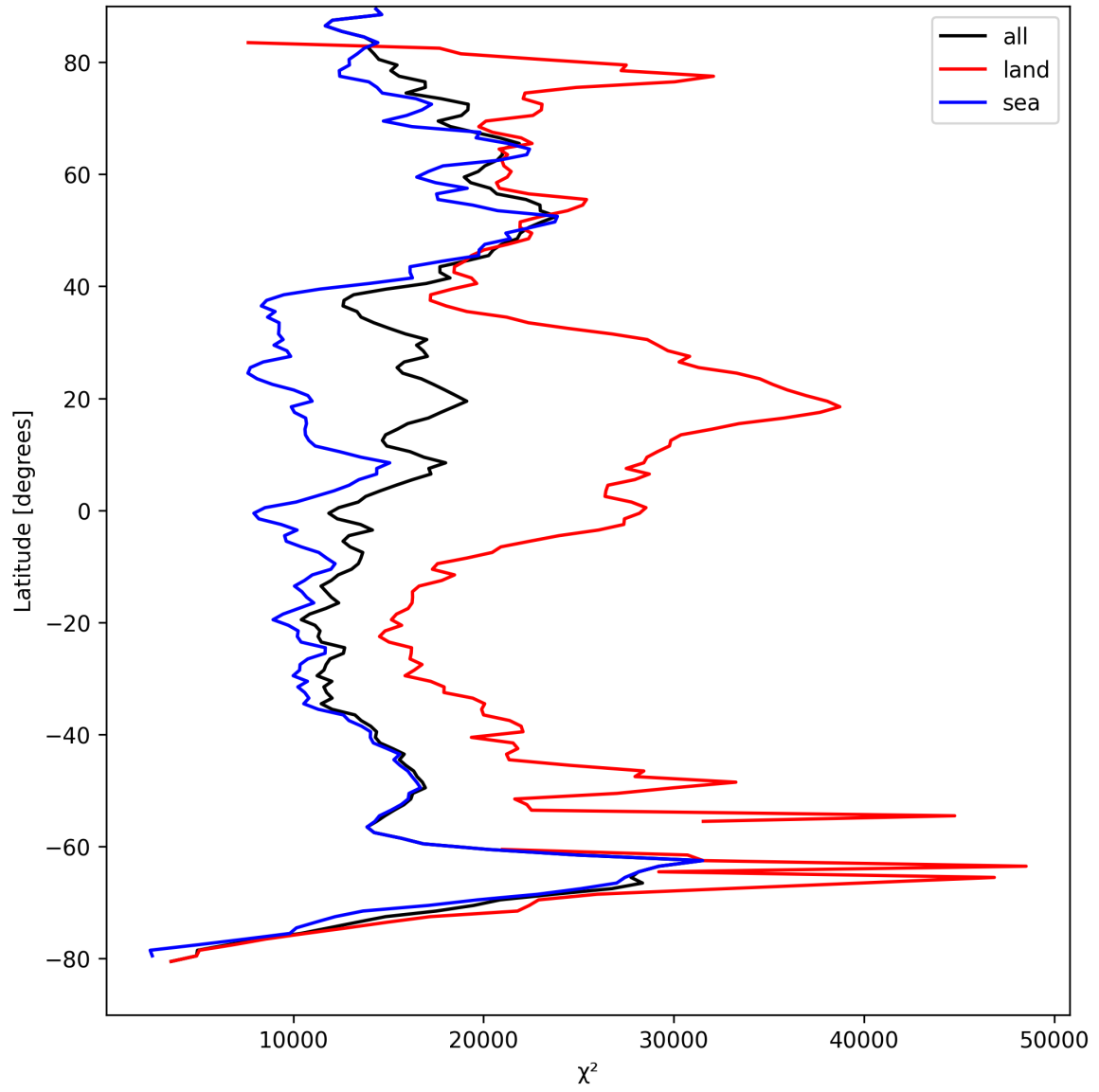
Figure 21: Zonal average of “ \chi^2 ” for 2025-09-01 to 2025-09-03.
