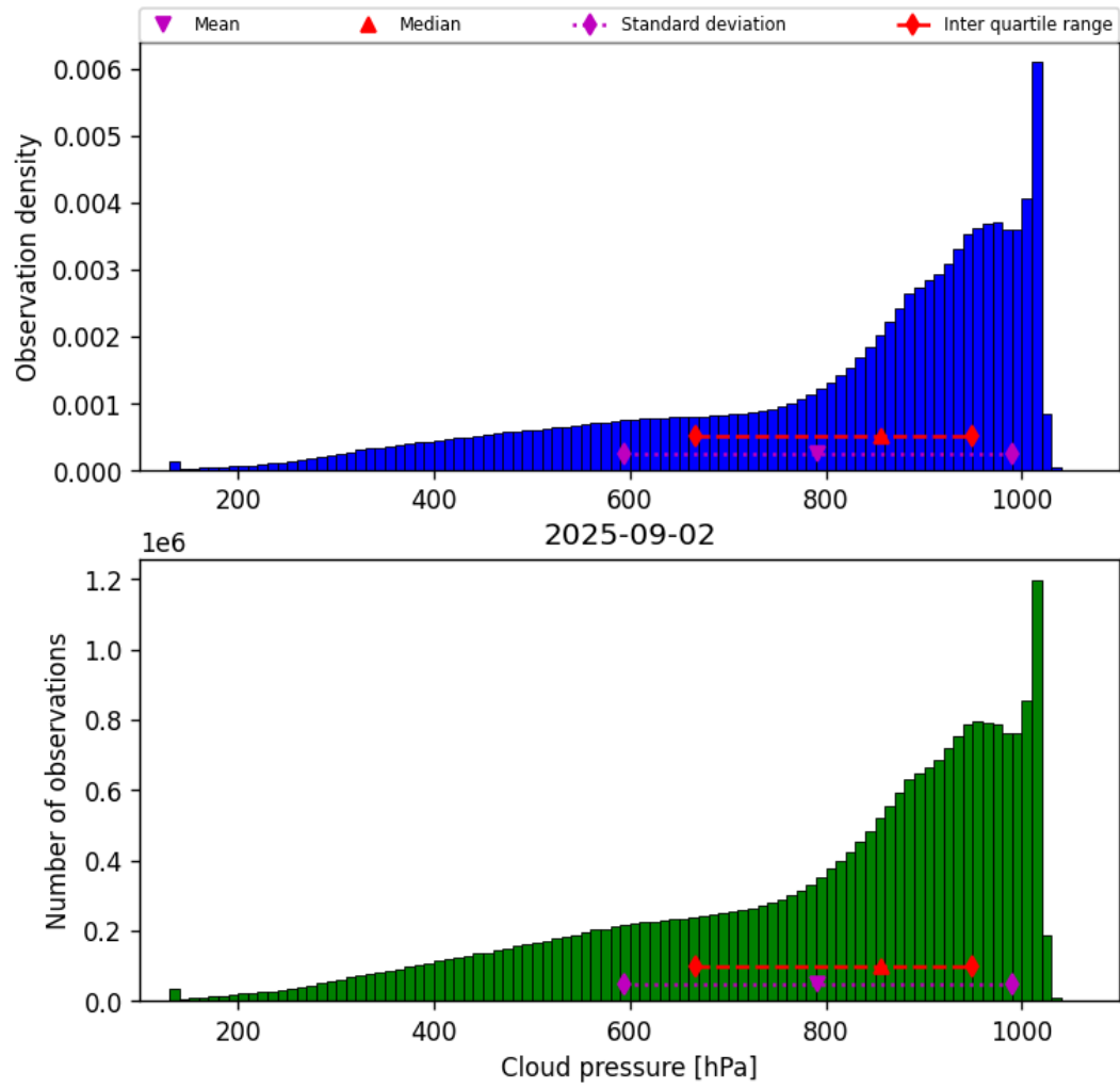
Figure 30: Histogram of “Cloud pressure” for 2025-09-01 to 2025-09-03
