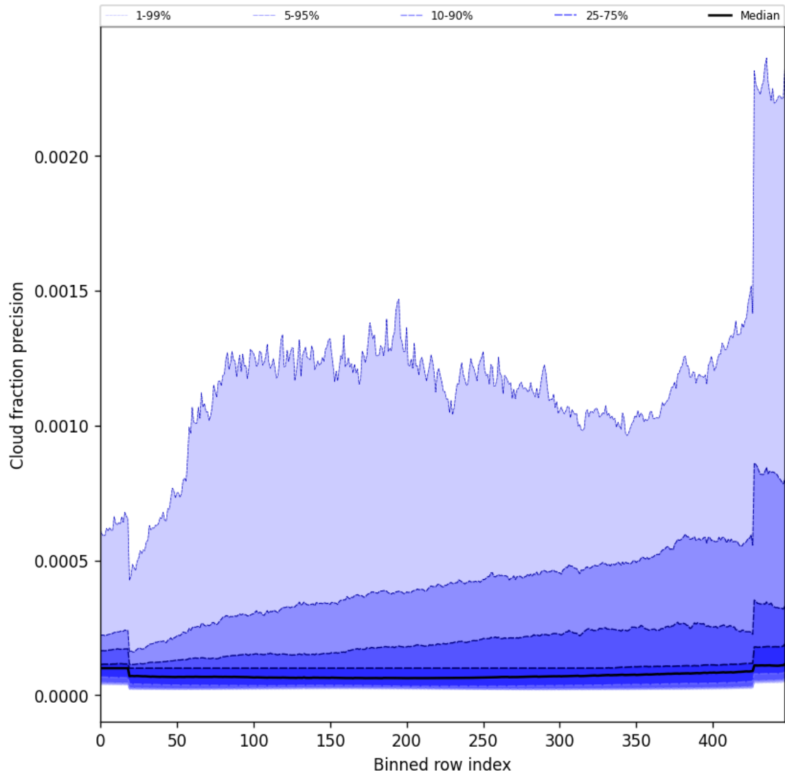
Figure 50: Along track statistics of “Cloud fraction precision” for 2025-09-01 to 2025-09-03
