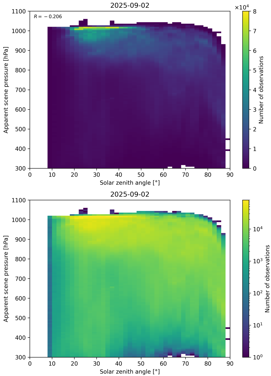
Figure 108: Scatter density plot of “Solar zenith angle” against “Apparent scene pressure” for 2025-09-01 to 2025-09-03.
