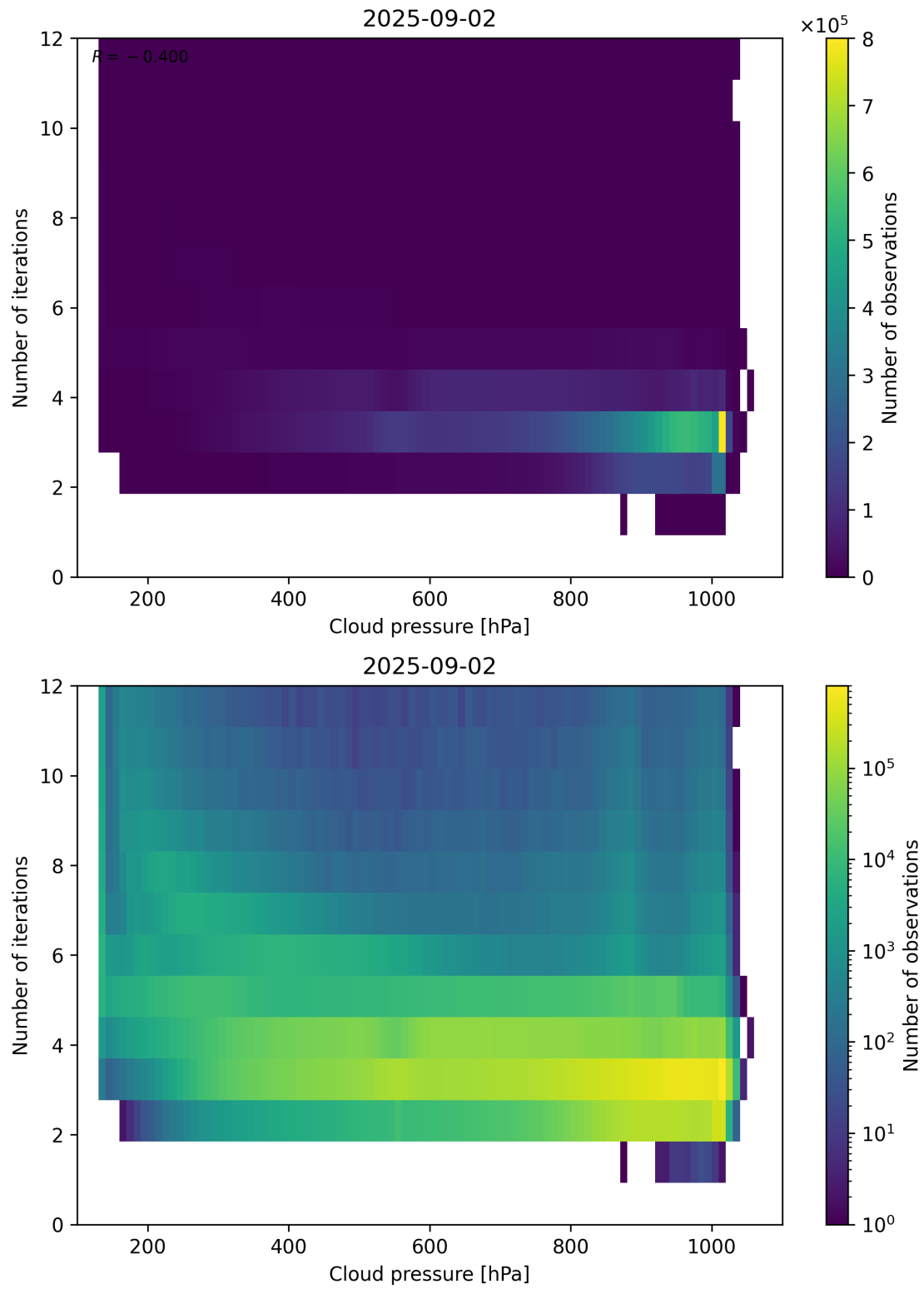
Figure 81: Scatter density plot of “Cloud pressure” against “Number of iterations” for 2025-09-01 to 2025-09-03.
