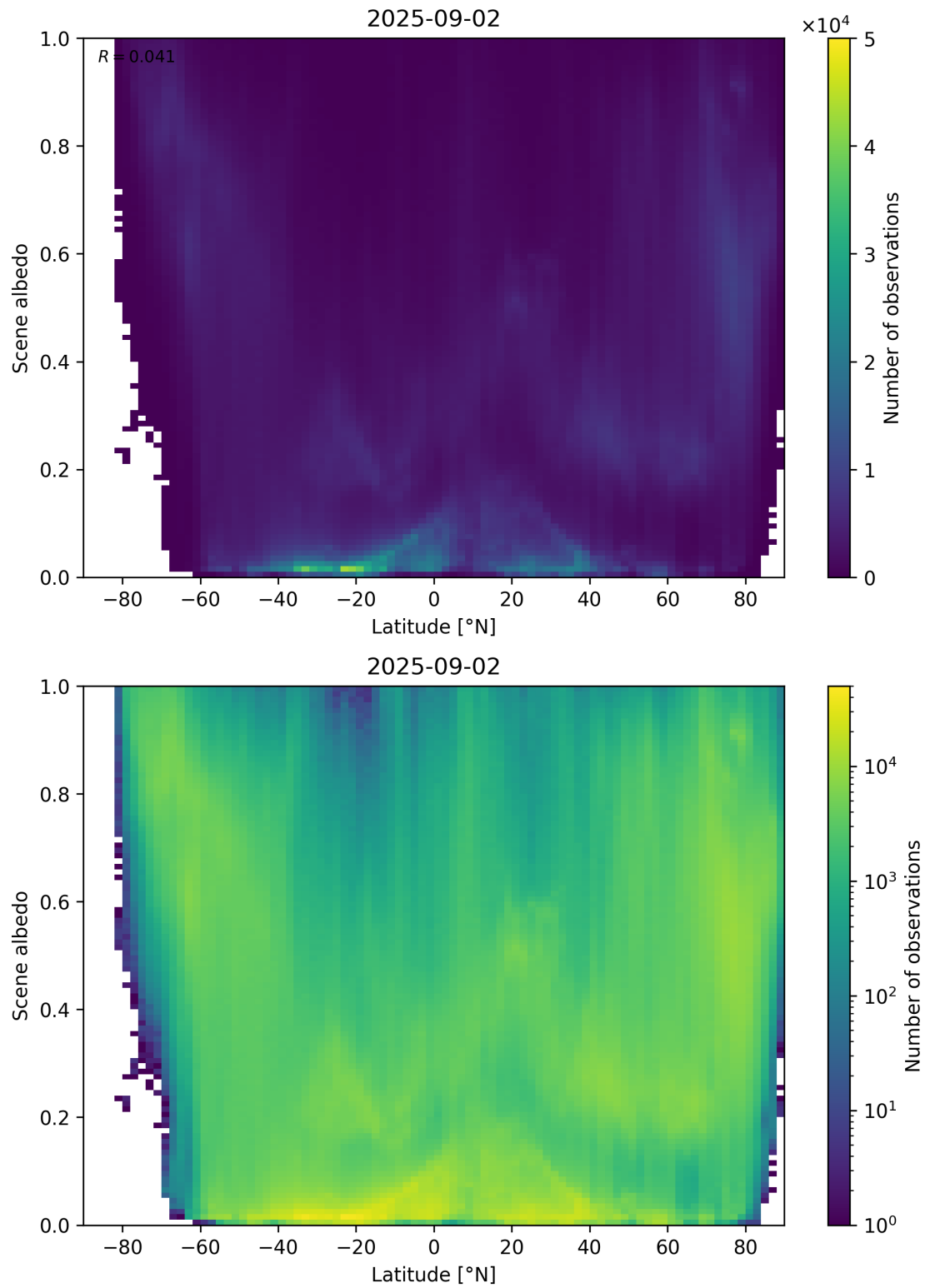
Figure 95: Scatter density plot of “Latitude” against “Scene albedo” for 2025-09-01 to 2025-09-03.
