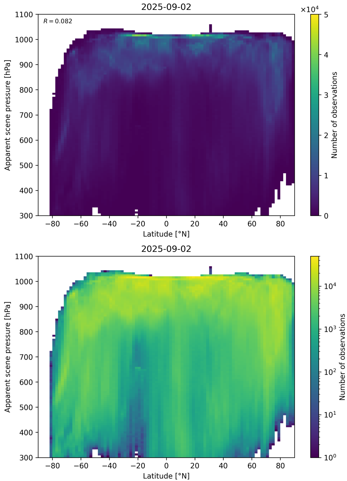
Figure 88: Scatter density plot of “Latitude” against “Apparent scene pressure” for 2025-09-01 to 2025-09-03.
