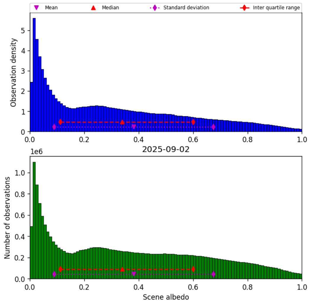
Figure 34: Histogram of “Scene albedo” for 2025-09-01 to 2025-09-03
