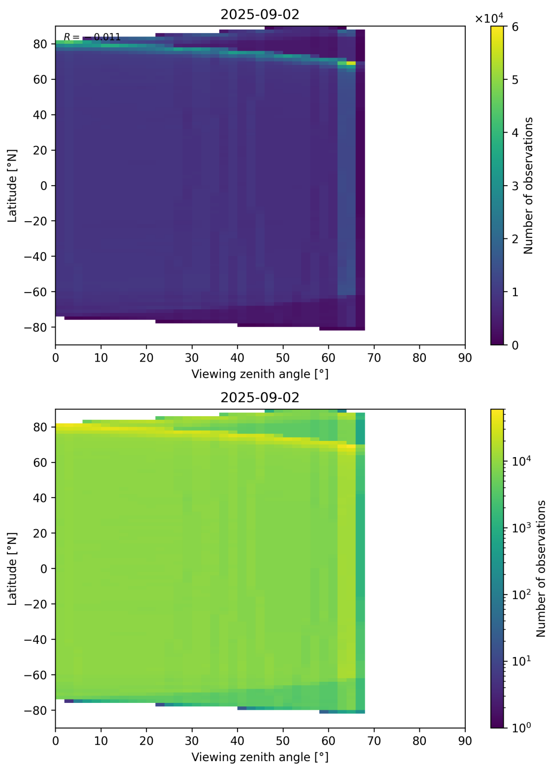
Figure 123: Scatter density plot of “Viewing zenith angle” against “Latitude” for 2025-09-01 to 2025-09-03.
