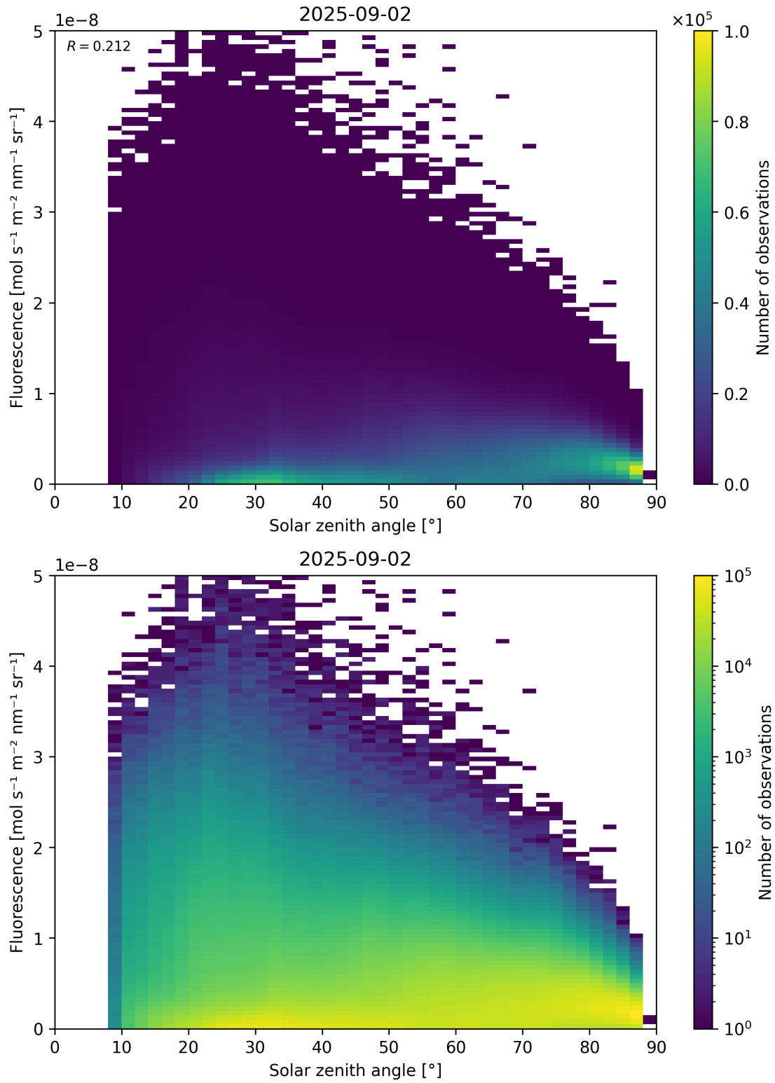
Figure 112: Scatter density plot of “Solar zenith angle” against “Fluorescence” for 2025-09-01 to 2025-09-03.
