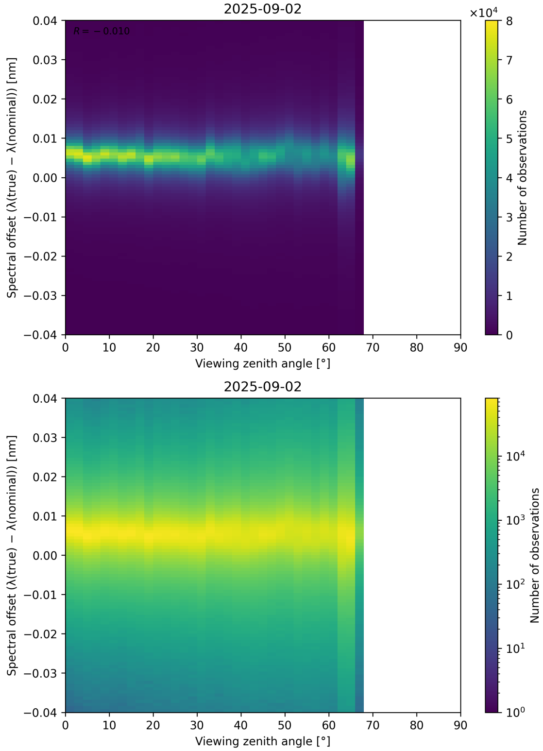
Figure 128: Scatter density plot of “Viewing zenith angle” against “Spectral offset ( \lambda_{\text{true}} - \lambda_{\text{nominal}} )” for 2025-09-01 to 2025-09-03.
