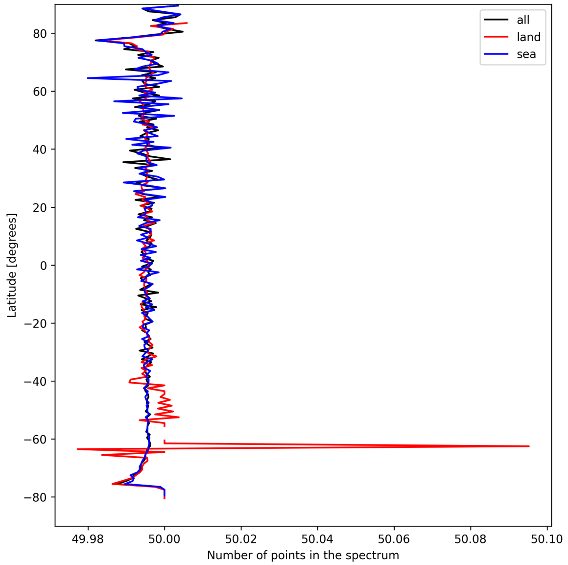
Figure 27: Zonal average of “Number of points in the spectrum” for 2025-09-01 to 2025-09-03.
