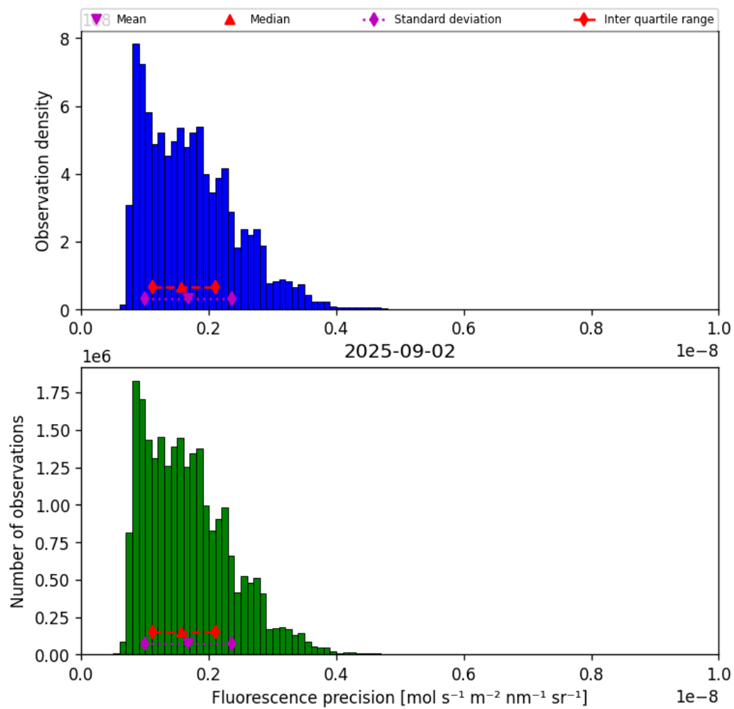
Figure 41: Histogram of “Fluorescence precision” for 2025-09-01 to 2025-09-03
