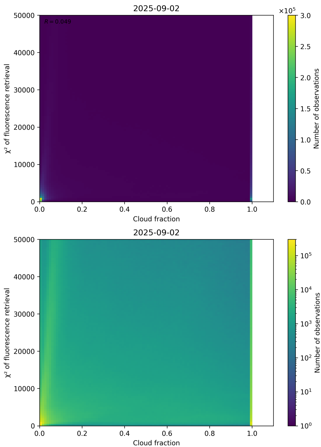
Figure 71: Scatter density plot of “Cloud fraction” against “ \chi^2 of fluorescence retrieval” for 2025-09-01 to 2025-09-03.
