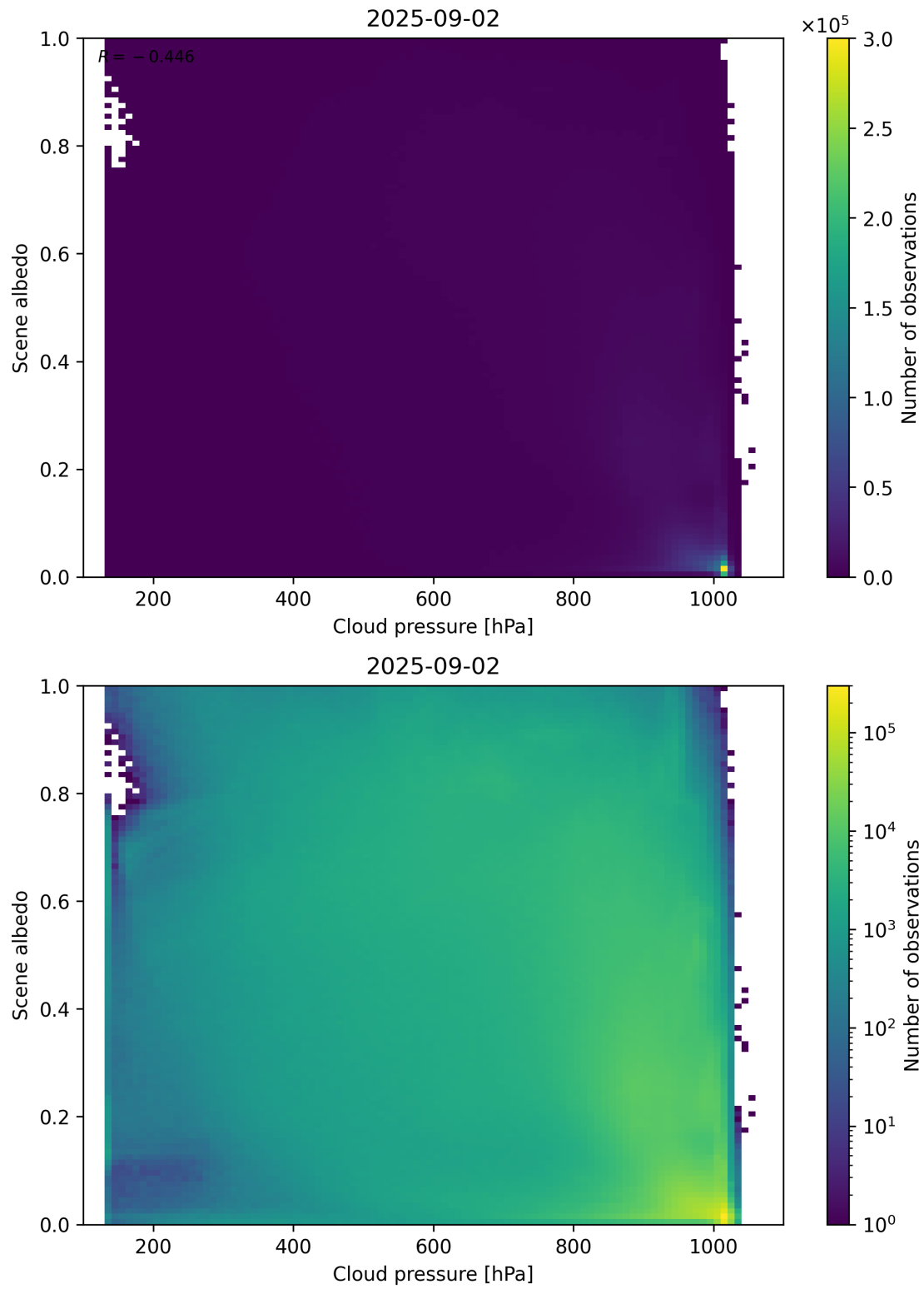
Figure 83: Scatter density plot of “Cloud pressure” against “Scene albedo” for 2025-09-01 to 2025-09-03.
