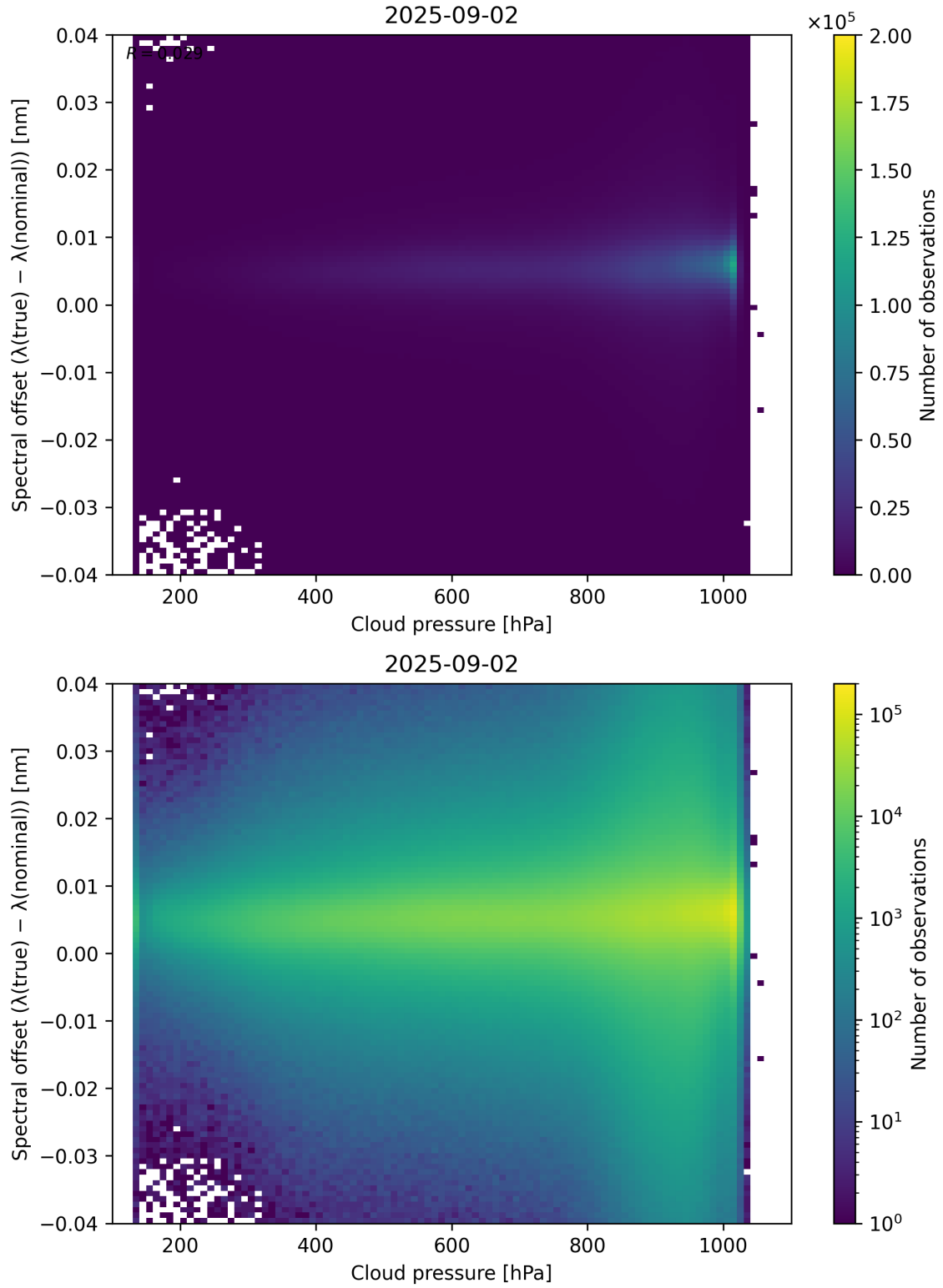
Figure 84: Scatter density plot of “Cloud pressure” against “Spectral offset ( \lambda_{\text{true}} - \lambda_{\text{nominal}} )” for 2025-09-01 to 2025-09-03.
