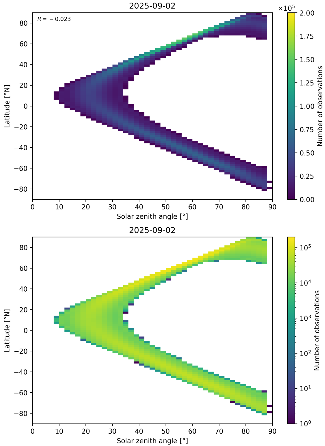
Figure 113: Scatter density plot of “Solar zenith angle” against “Latitude” for 2025-09-01 to 2025-09-03.
