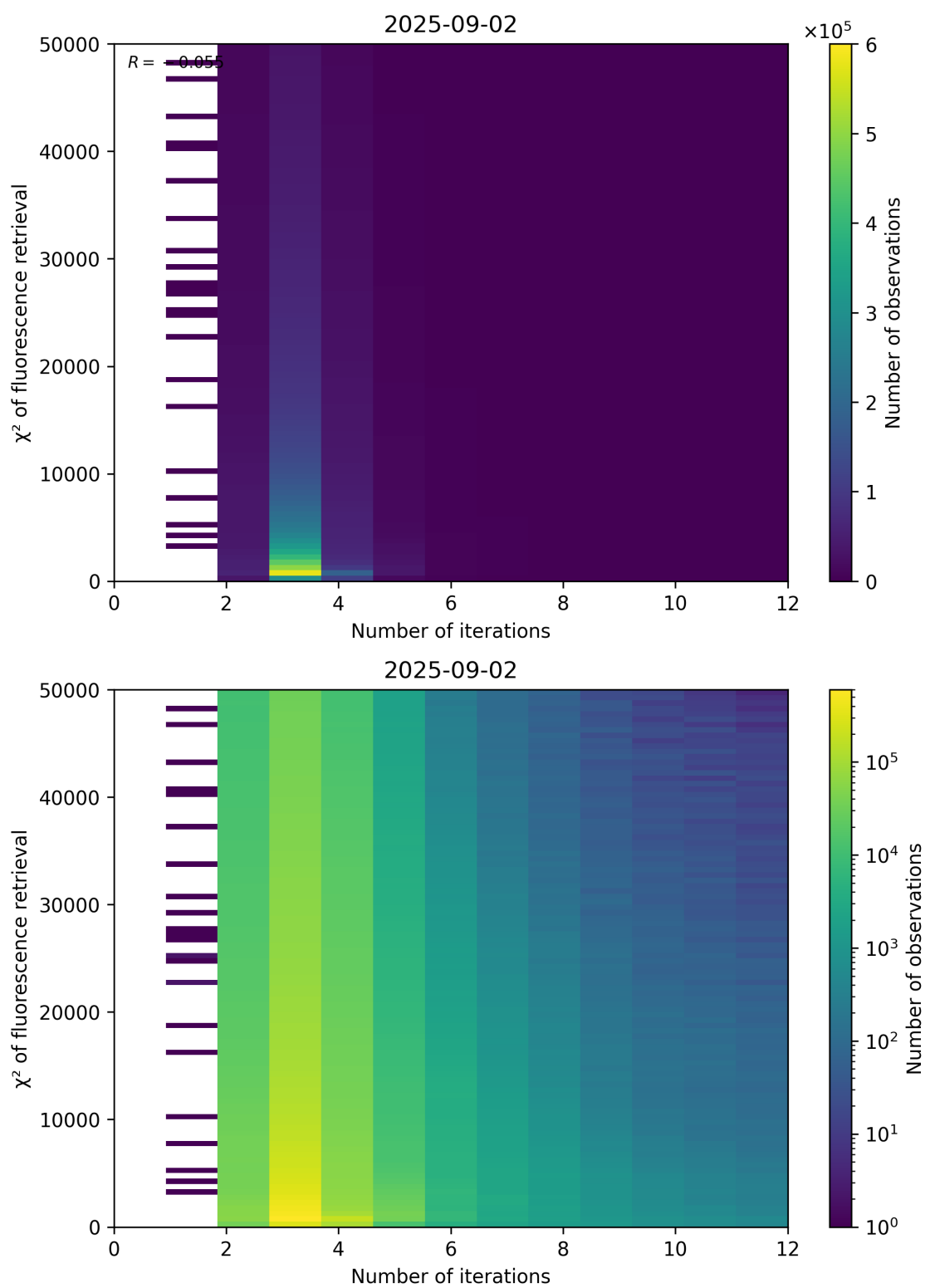
Figure 97: Scatter density plot of “Number of iterations” against “ \chi^2 of fluorescence retrieval” for 2025-09-01 to 2025-09-03.
