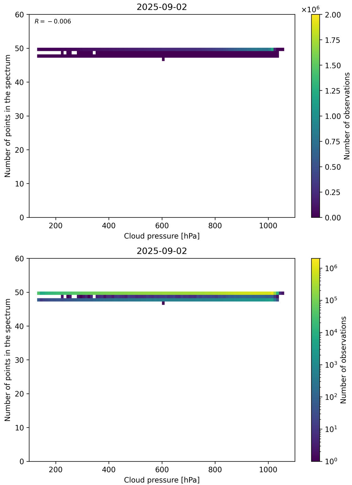
Figure 82: Scatter density plot of “Cloud pressure” against “Number of points in the spectrum” for 2025-09-01 to 2025-09-03.
