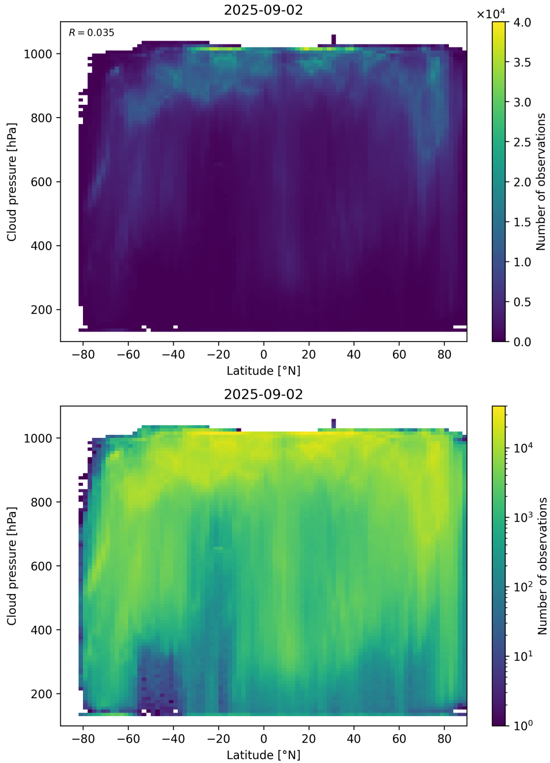
Figure 91: Scatter density plot of “Latitude” against “Cloud pressure” for 2025-09-01 to 2025-09-03.
