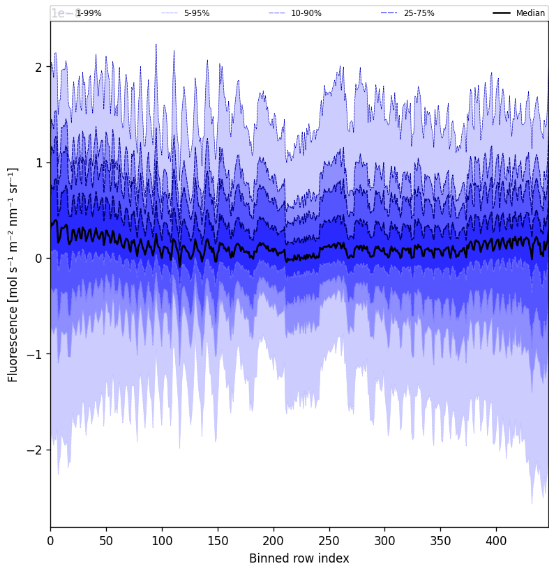
Figure 57: Along track statistics of “Fluorescence” for 2025-09-01 to 2025-09-03
