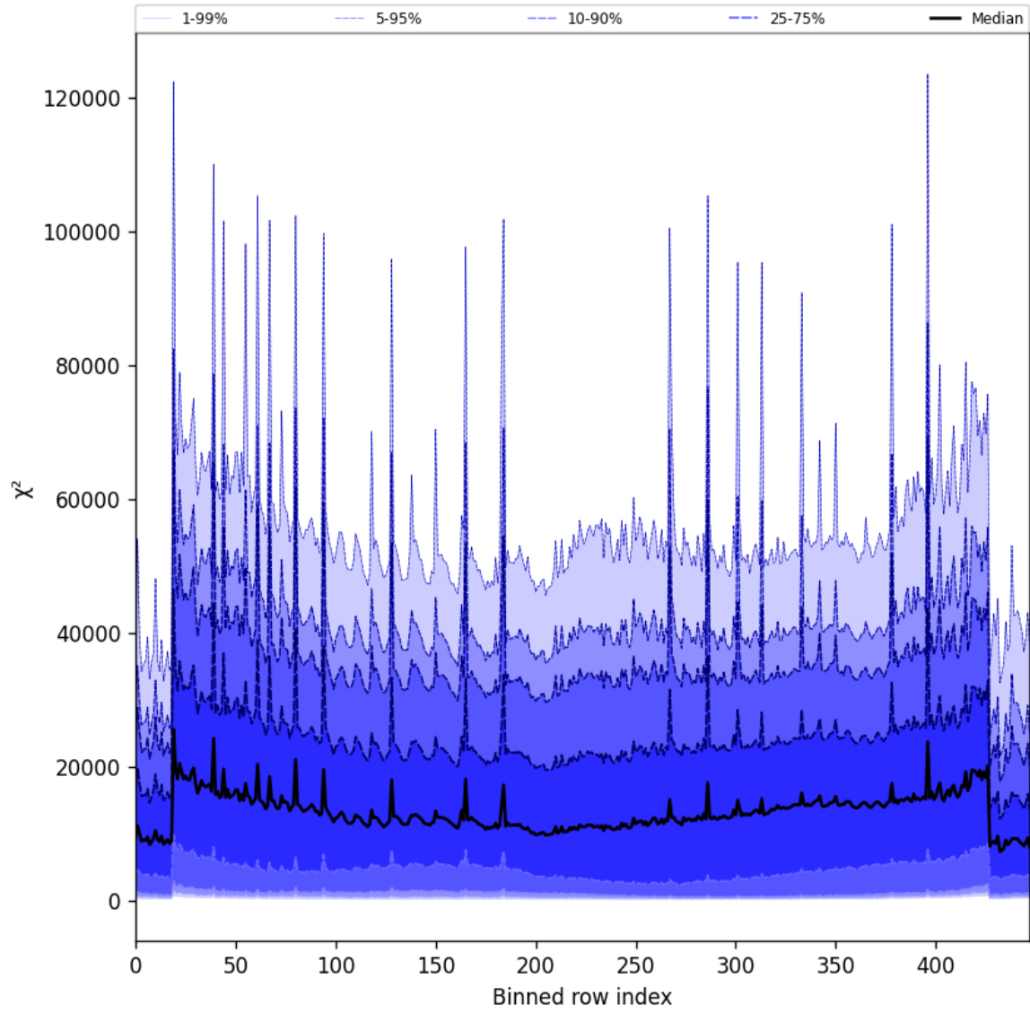
Figure 55: Along track statistics of “ \chi^2 ” for 2025-09-01 to 2025-09-03
