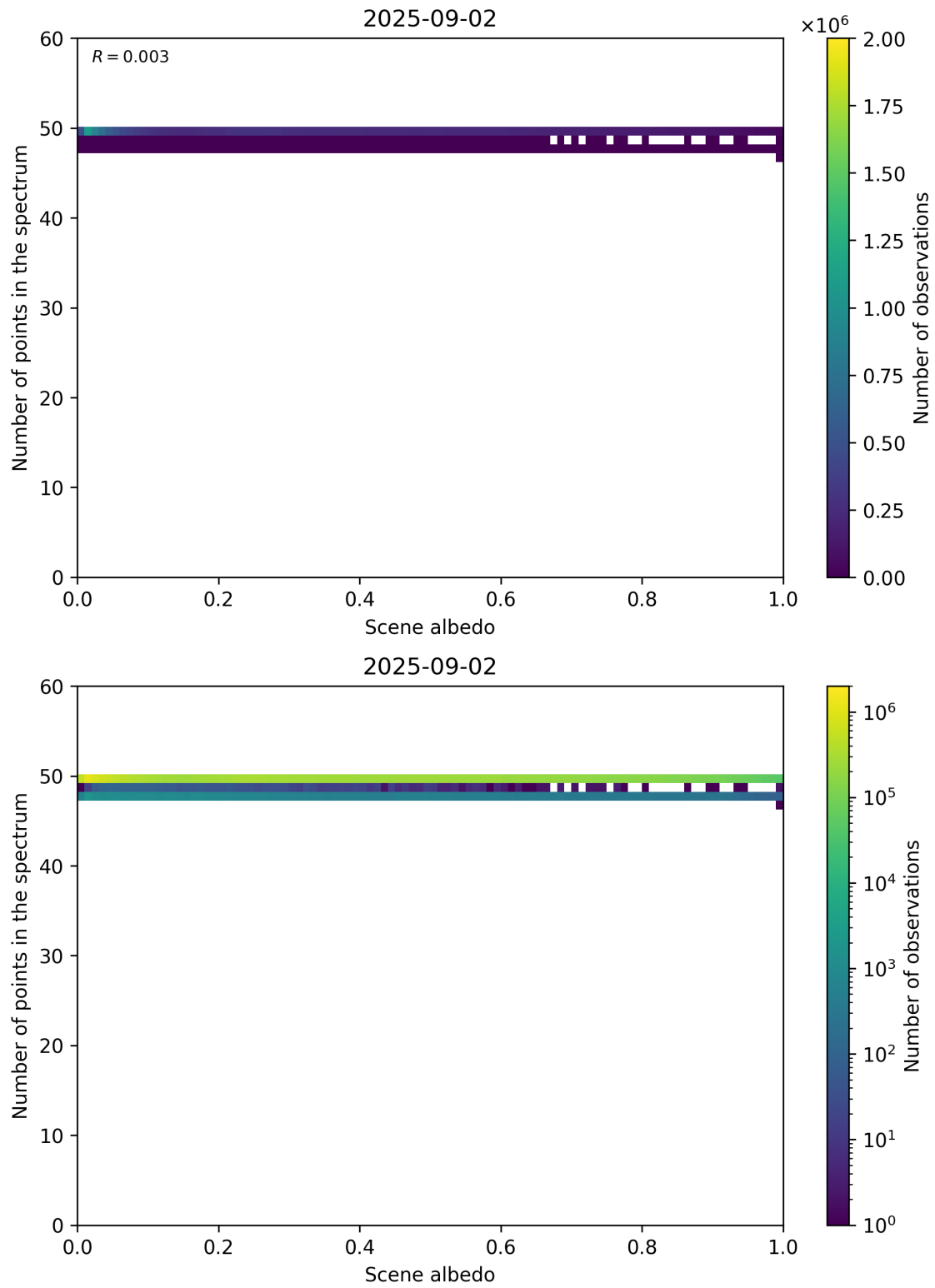
Figure 106: Scatter density plot of “Scene albedo” against “Number of points in the spectrum” for 2025-09-01 to 2025-09-03.
