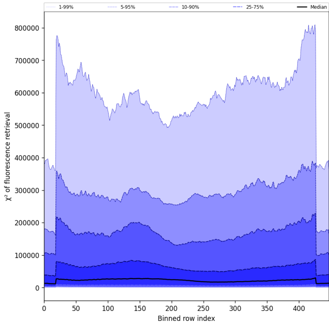
Figure 59: Along track statistics of “ \chi^2 of fluorescence retrieval” for 2025-09-01 to 2025-09-03
