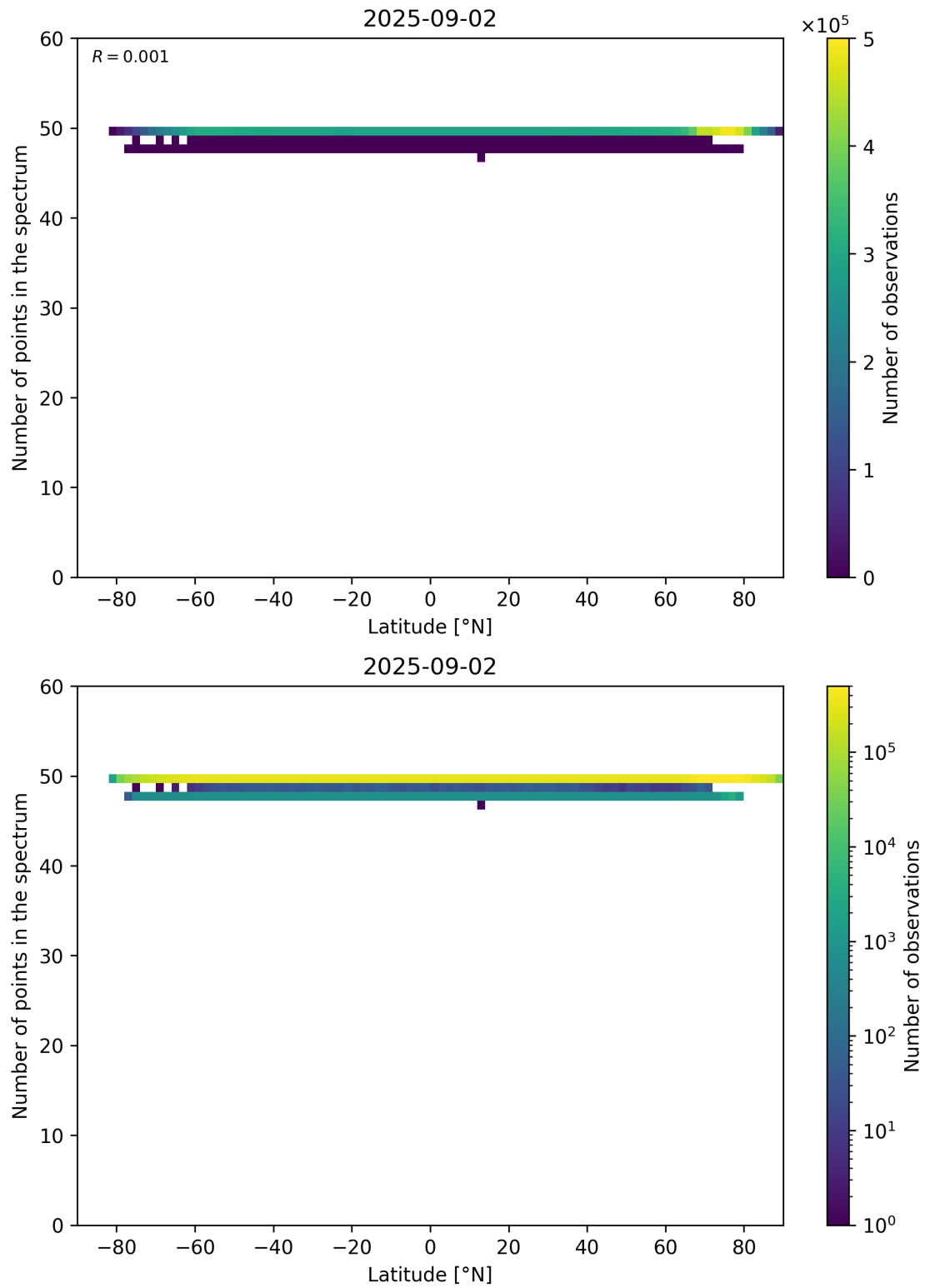
Figure 94: Scatter density plot of “Latitude” against “Number of points in the spectrum” for 2025-09-01 to 2025-09-03.
