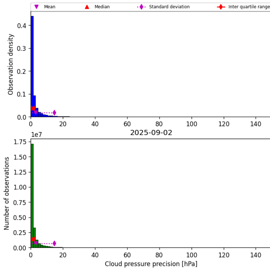
Figure 31: Histogram of “Cloud pressure precision” for 2025-09-01 to 2025-09-03
