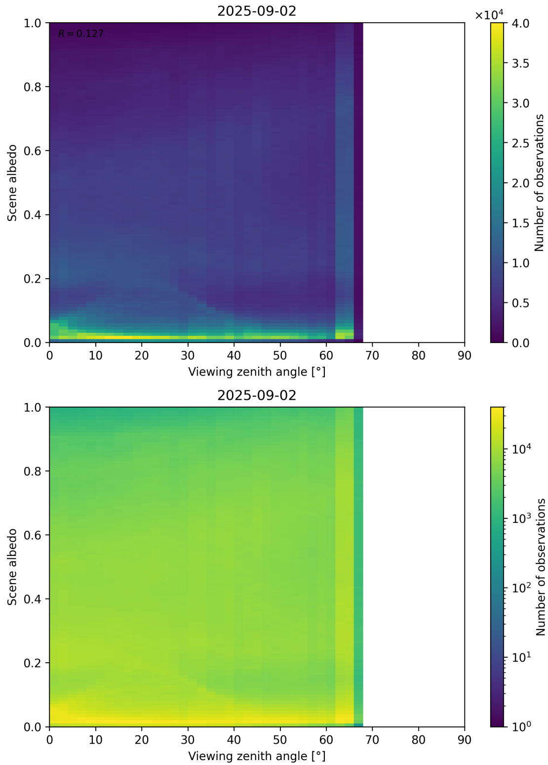
Figure 126: Scatter density plot of “Viewing zenith angle” against “Scene albedo” for 2025-09-01 to 2025-09-03.
