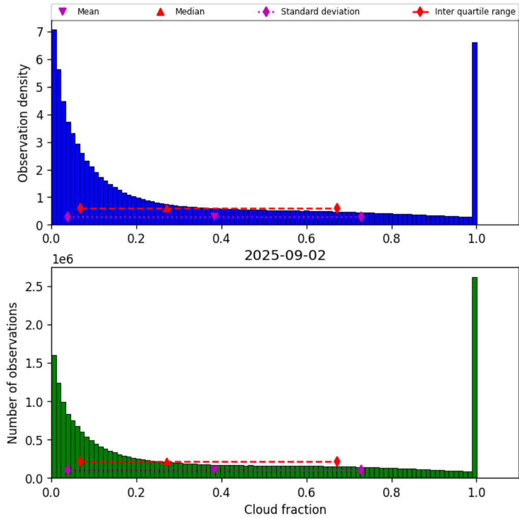
Figure 32: Histogram of “Cloud fraction” for 2025-09-01 to 2025-09-03
