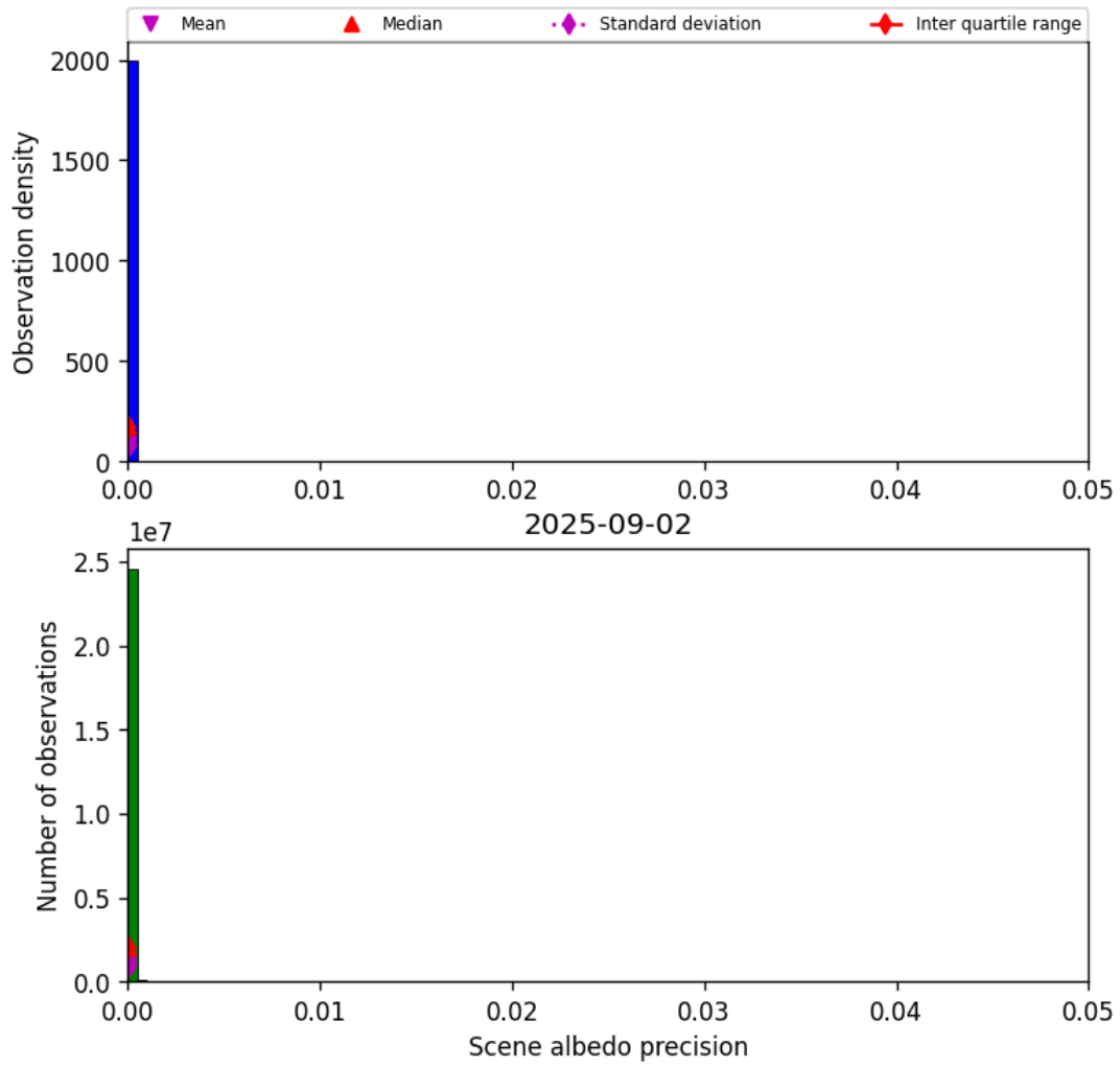
Figure 35: Histogram of “Scene albedo precision” for 2025-09-01 to 2025-09-03
