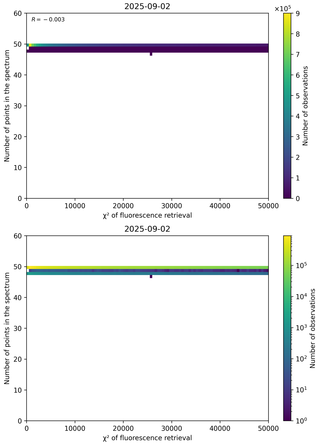
Figure 68: Scatter density plot of “ \chi^2 of fluorescence retrieval” against “Number of points in the spectrum” for 2025-09-01 to 2025-09-03.
