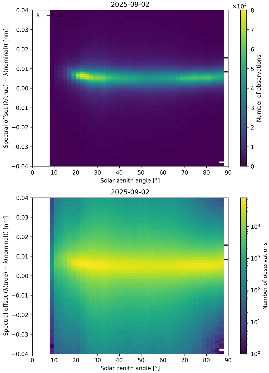
Figure 117: Scatter density plot of “Solar zenith angle” against “Spectral offset ( \lambda_{\text{true}} - \lambda_{\text{nominal}} )” for 2025-09-01 to 2025-09-03.
