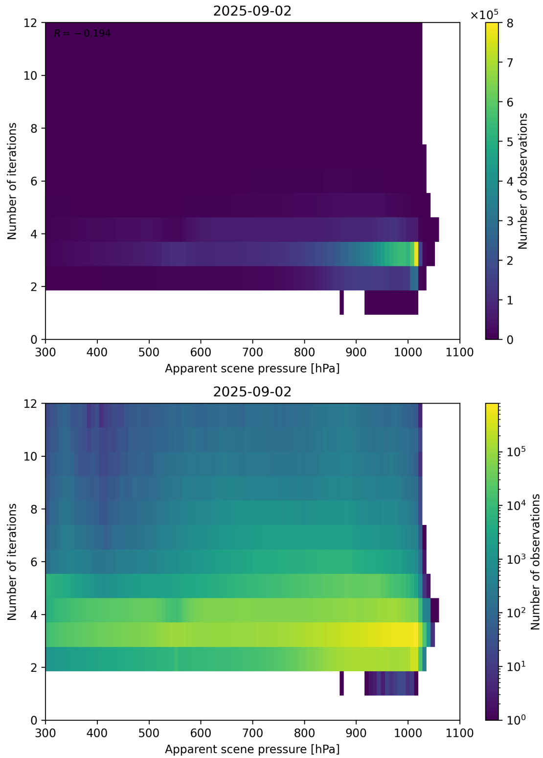
Figure 65: Scatter density plot of “Apparent scene pressure” against “Number of iterations” for 2025-09-01 to 2025-09-03.
