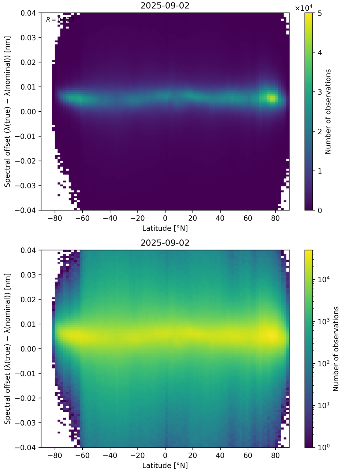
Figure 96: Scatter density plot of “Latitude” against “Spectral offset ( \lambda_{\text{true}} - \lambda_{\text{nominal}} )” for 2025-09-01 to 2025-09-03.
