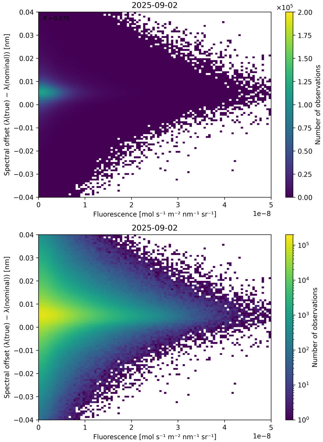
Figure 87: Scatter density plot of “Fluorescence” against “Spectral offset ( \lambda_{\text{true}} - \lambda_{\text{nominal}} )” for 2025-09-01 to 2025-09-03.
