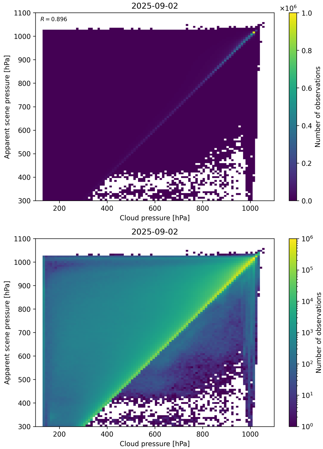
Figure 77: Scatter density plot of “Cloud pressure” against “Apparent scene pressure” for 2025-09-01 to 2025-09-03.
