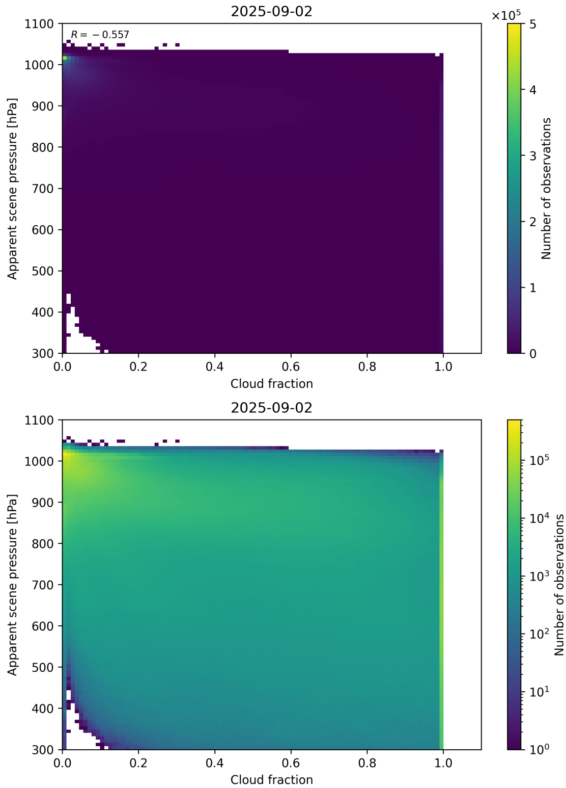
Figure 70: Scatter density plot of “Cloud fraction” against “Apparent scene pressure” for 2025-09-01 to 2025-09-03.
