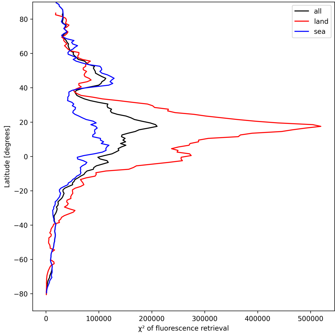
Figure 25: Zonal average of “ \chi^2 of fluorescence retrieval” for 2025-09-01 to 2025-09-03.
