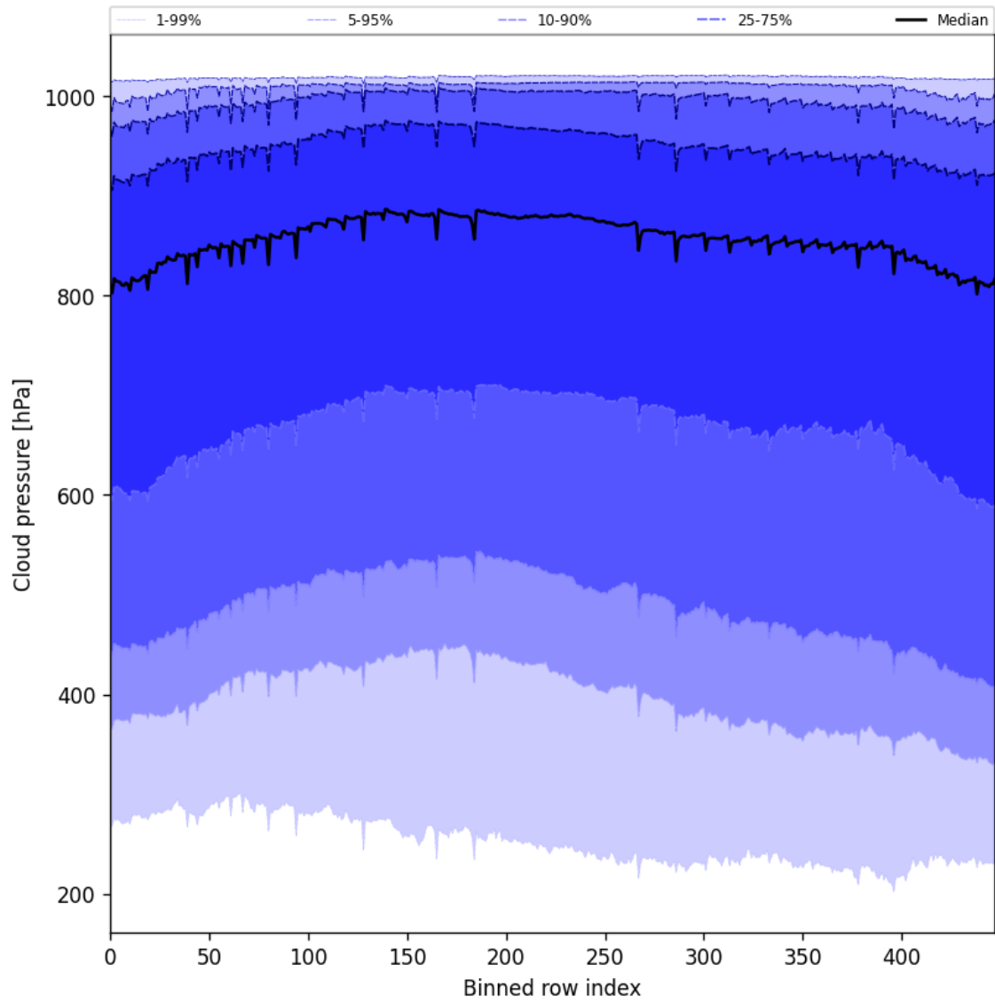
Figure 47: Along track statistics of “Cloud pressure” for 2025-09-01 to 2025-09-03
