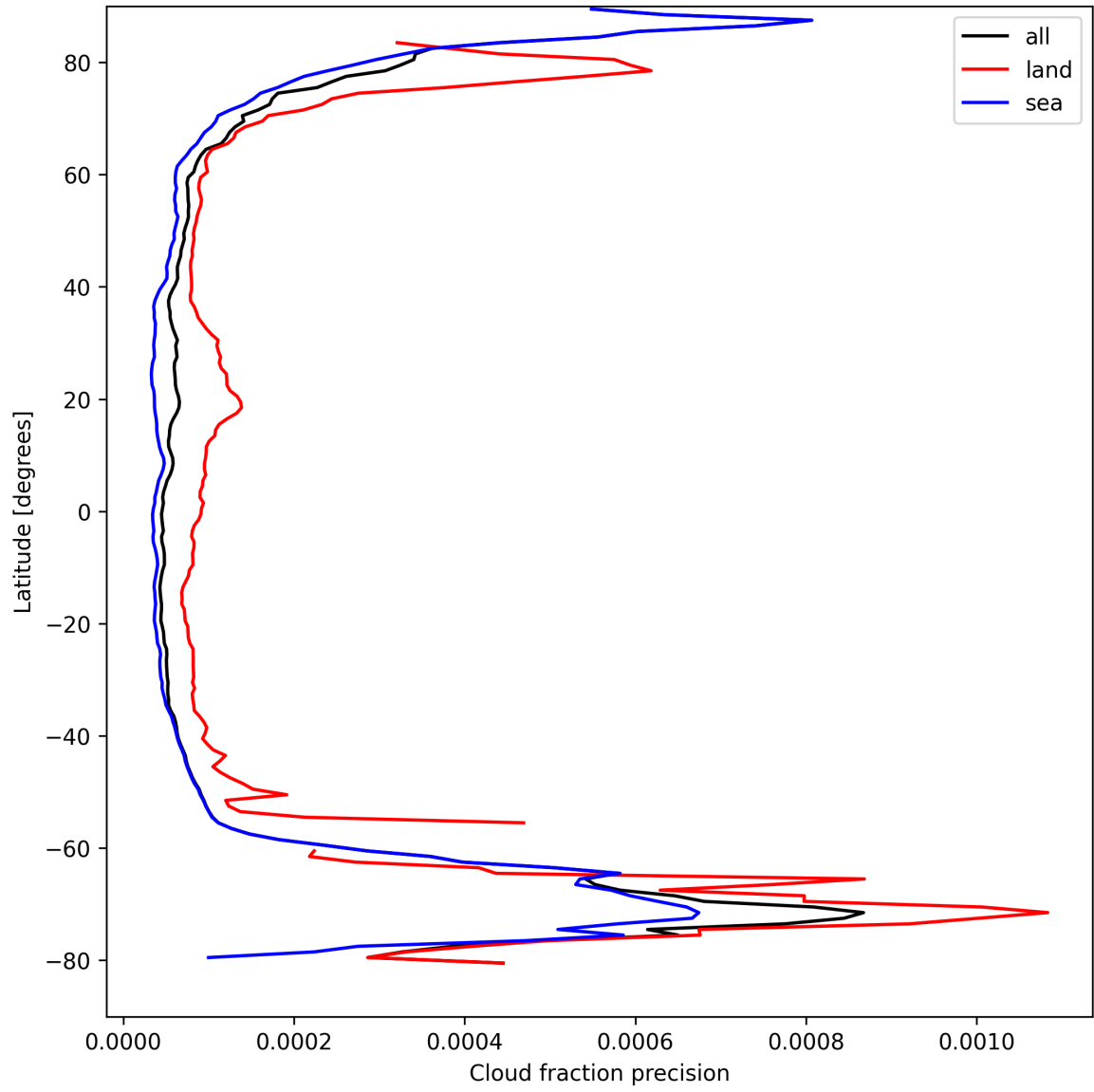
Figure 16: Zonal average of “Cloud fraction precision” for 2025-09-01 to 2025-09-03.
