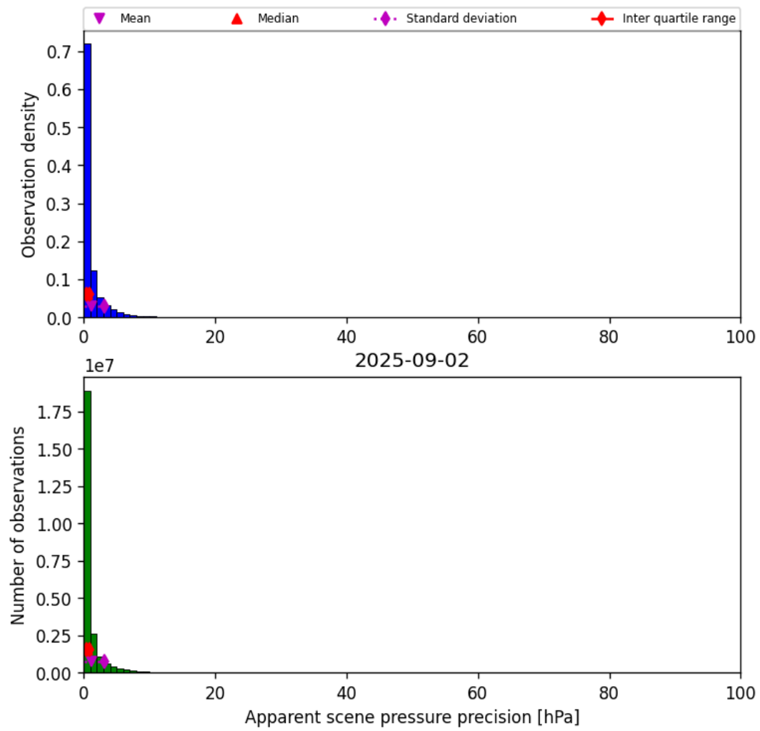
Figure 37: Histogram of “Apparent scene pressure precision” for 2025-09-01 to 2025-09-03
