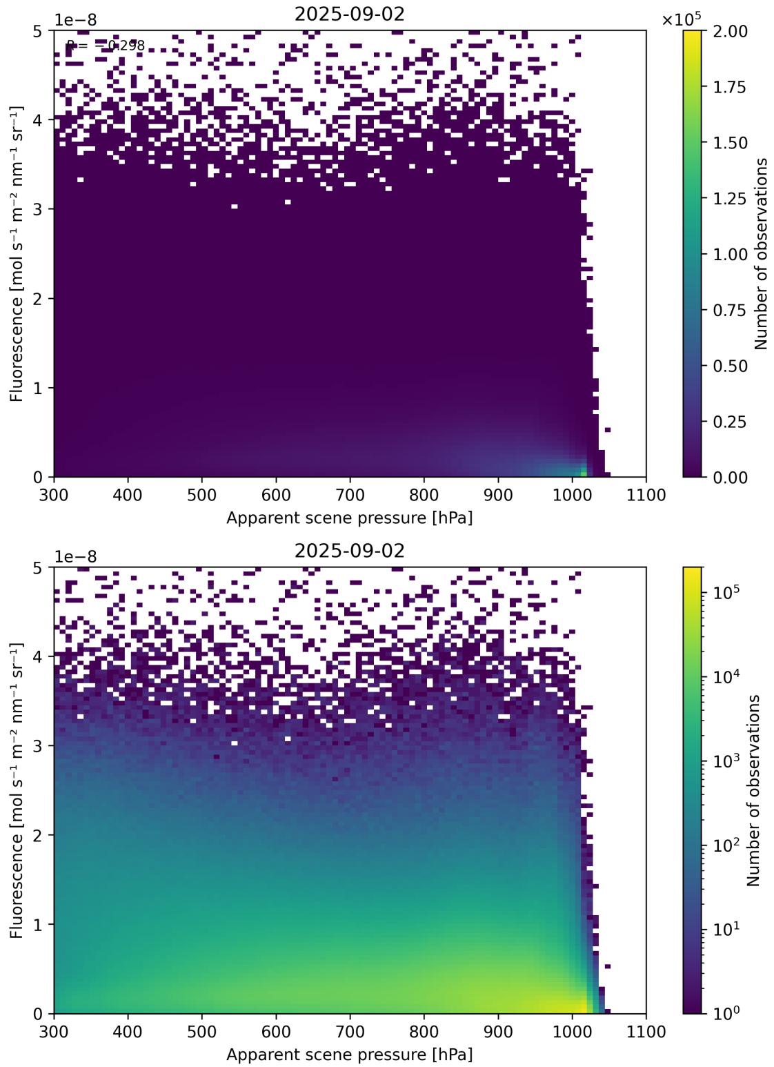
Figure 64: Scatter density plot of “Apparent scene pressure” against “Fluorescence” for 2025-09-01 to 2025-09-03.
