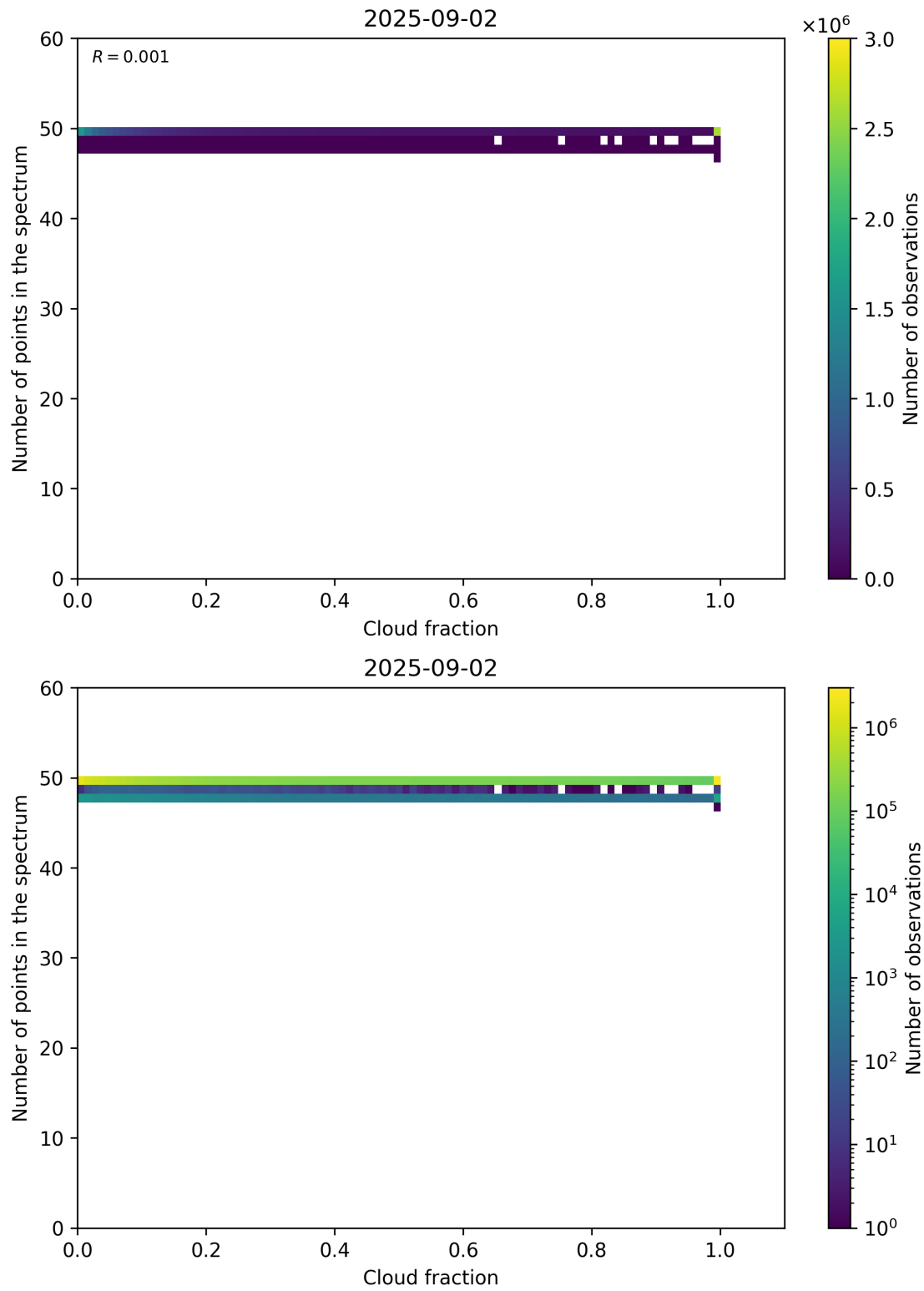
Figure 74: Scatter density plot of “Cloud fraction” against “Number of points in the spectrum” for 2025-09-01 to 2025-09-03.
