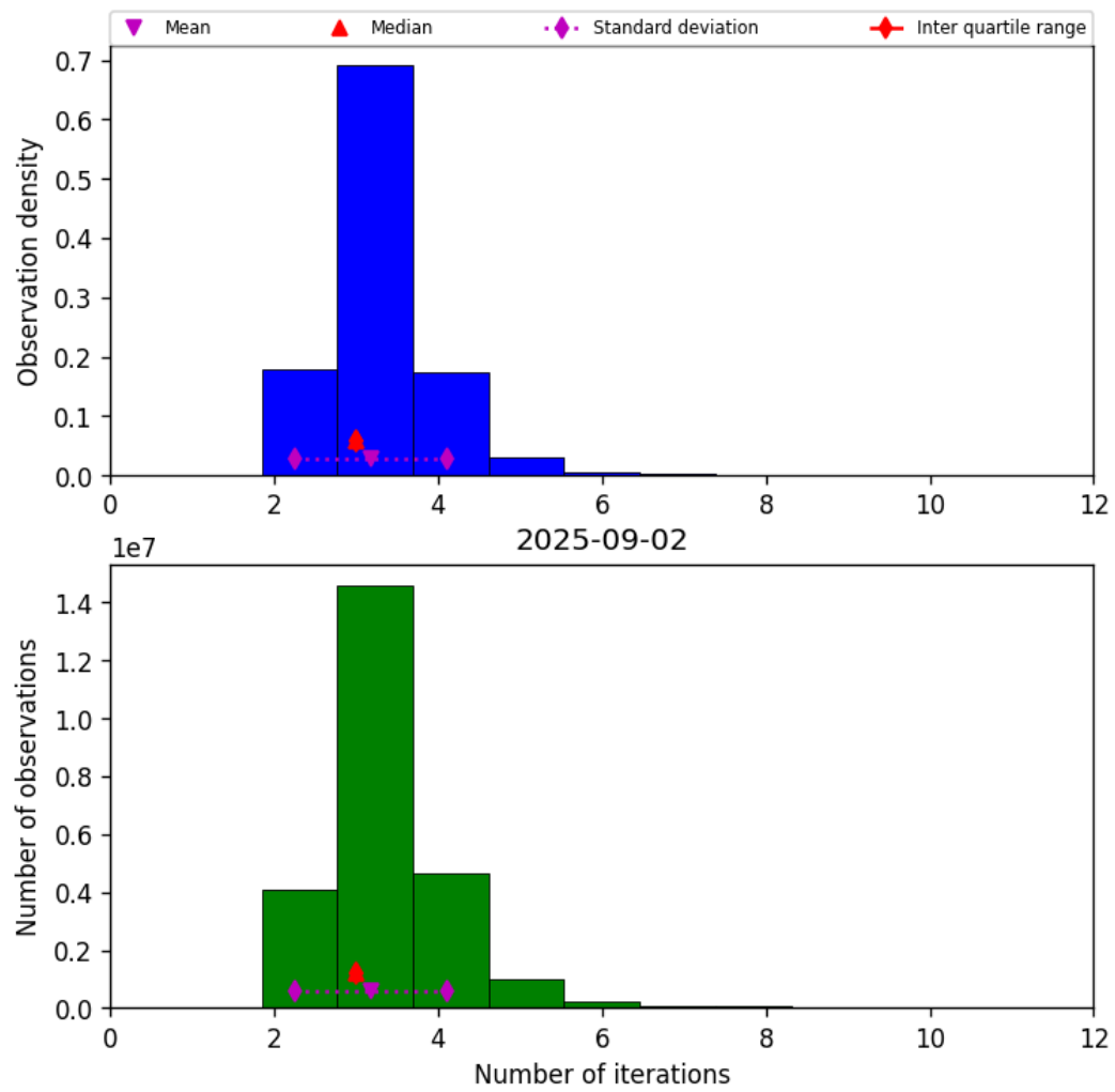
Figure 39: Histogram of “Number of iterations” for 2025-09-01 to 2025-09-03
