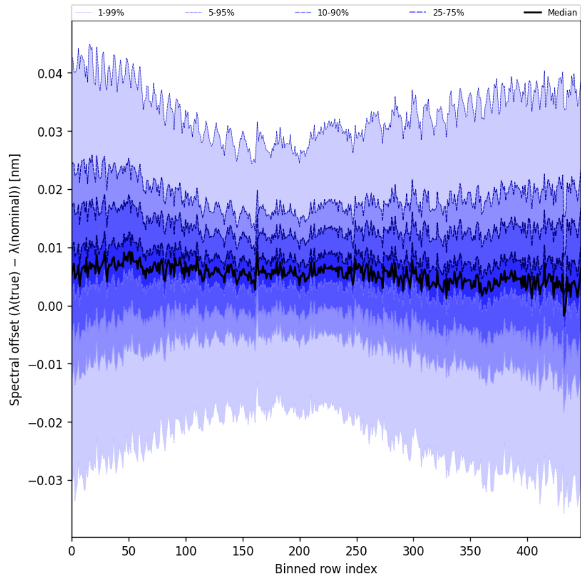
Figure 62: Along track statistics of “Spectral offset ( \lambda_{\text{true}} - \lambda_{\text{nominal}} )” for 2025-09-01 to 2025-09-03
