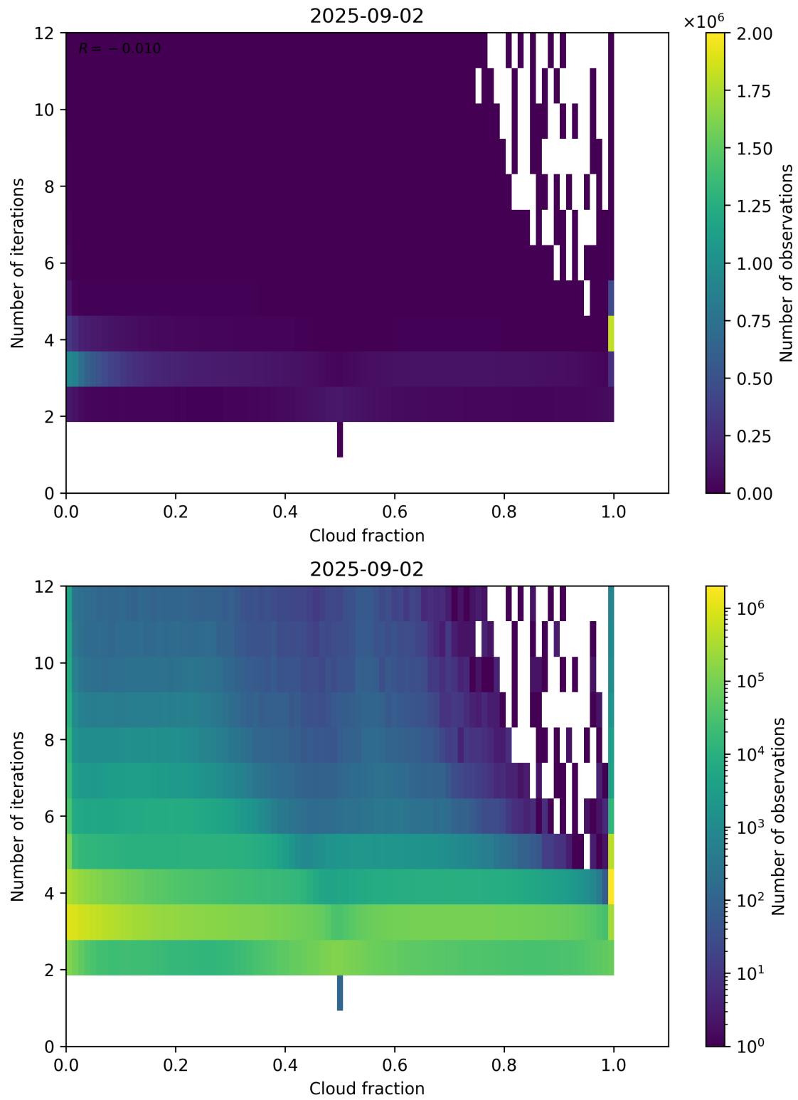
Figure 73: Scatter density plot of “Cloud fraction” against “Number of iterations” for 2025-09-01 to 2025-09-03.
