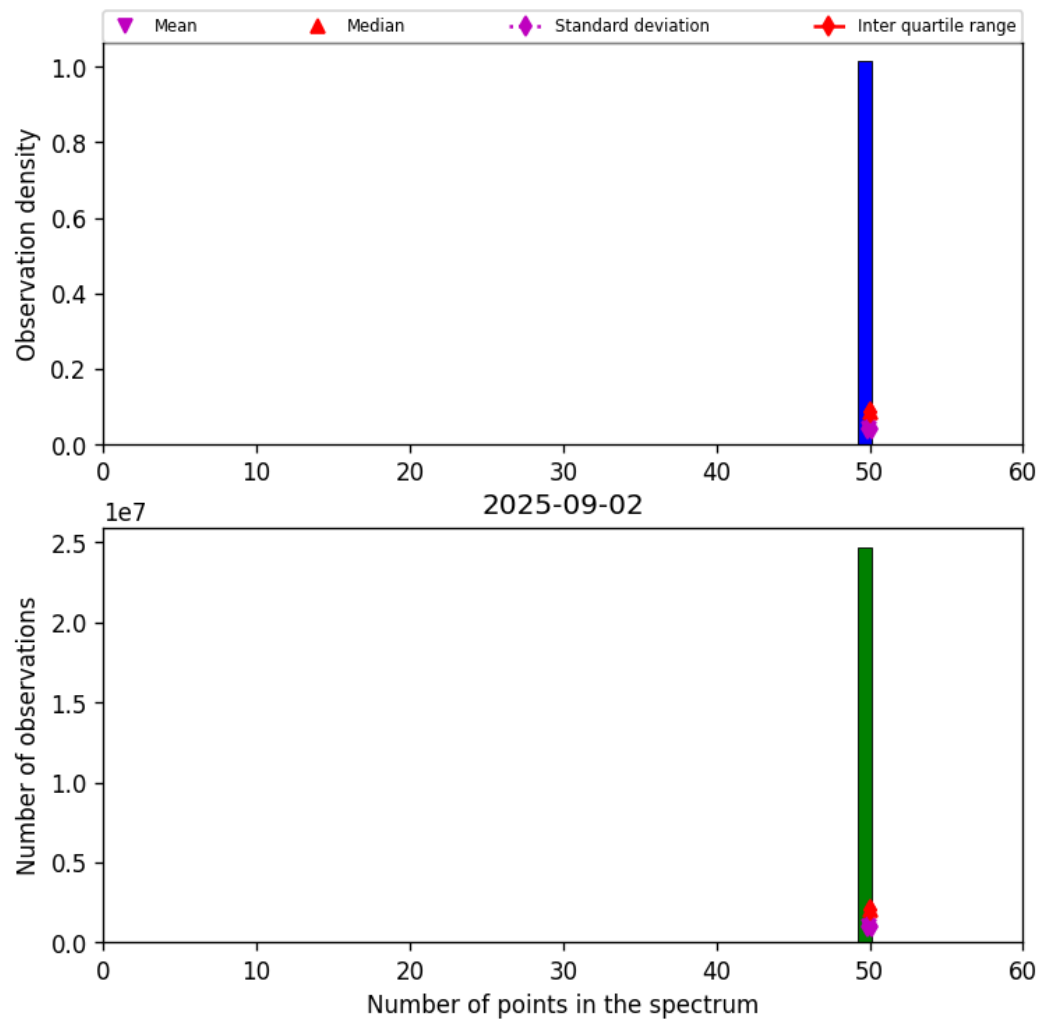
Figure 44: Histogram of "Number of points in the spectrum" for 2025-09-01 to 2025-09-03
