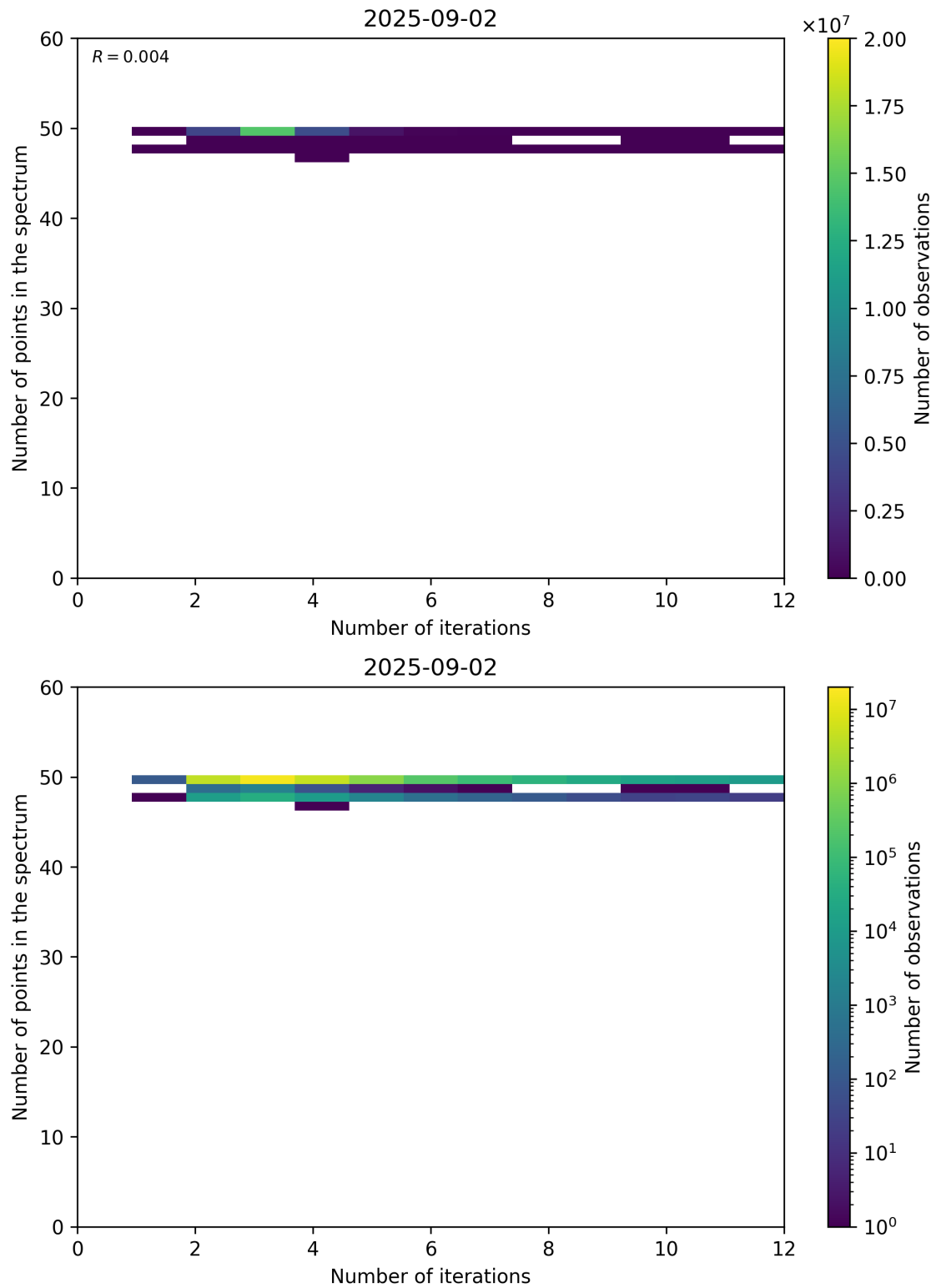
Figure 99: Scatter density plot of “Number of iterations” against “Number of points in the spectrum” for 2025-09-01 to 2025-09-03.
