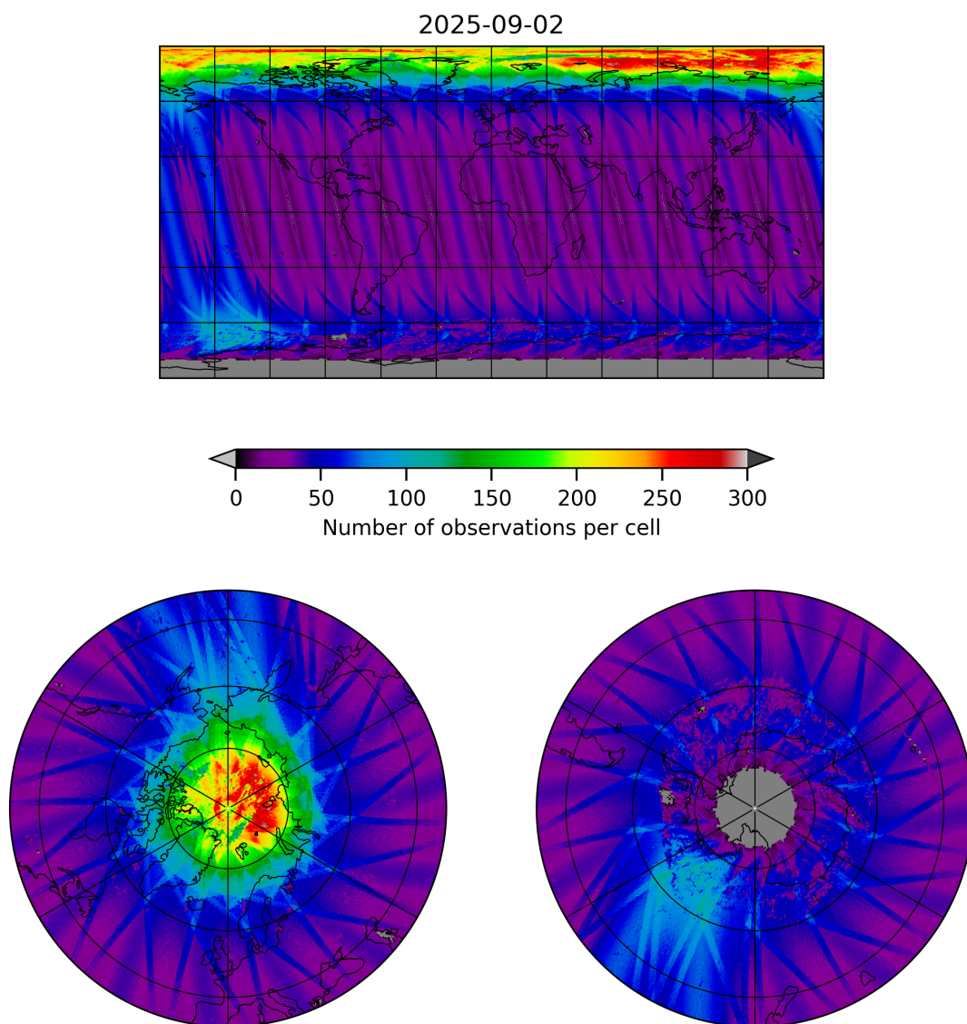
Figure 11: Map of the number of observations for 2025-09-01 to 2025-09-03
