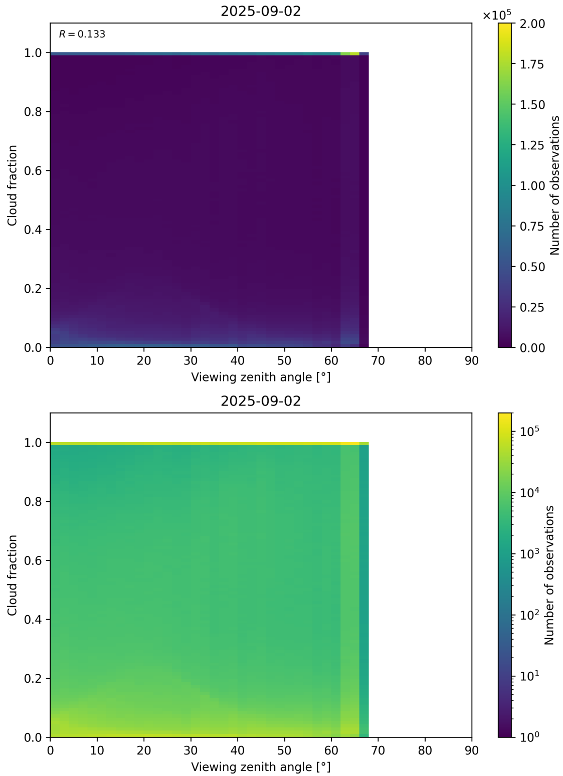
Figure 120: Scatter density plot of “Viewing zenith angle” against “Cloud fraction” for 2025-09-01 to 2025-09-03.
