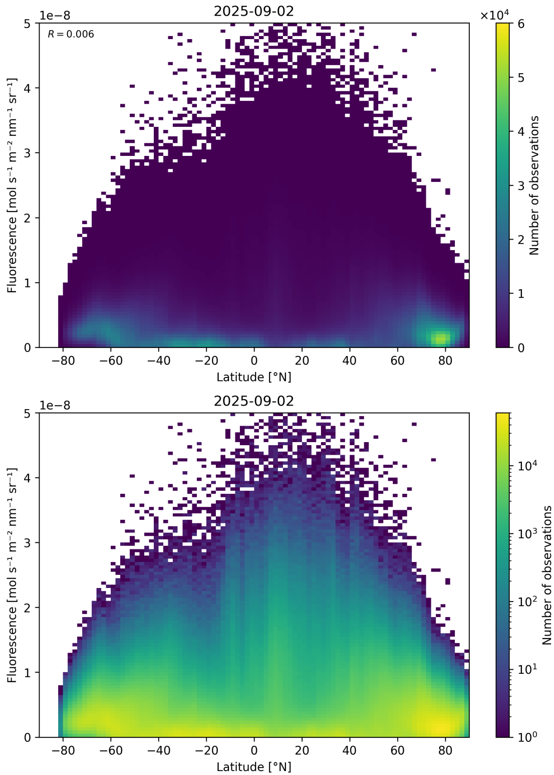
Figure 92: Scatter density plot of “Latitude” against “Fluorescence” for 2025-09-01 to 2025-09-03.
