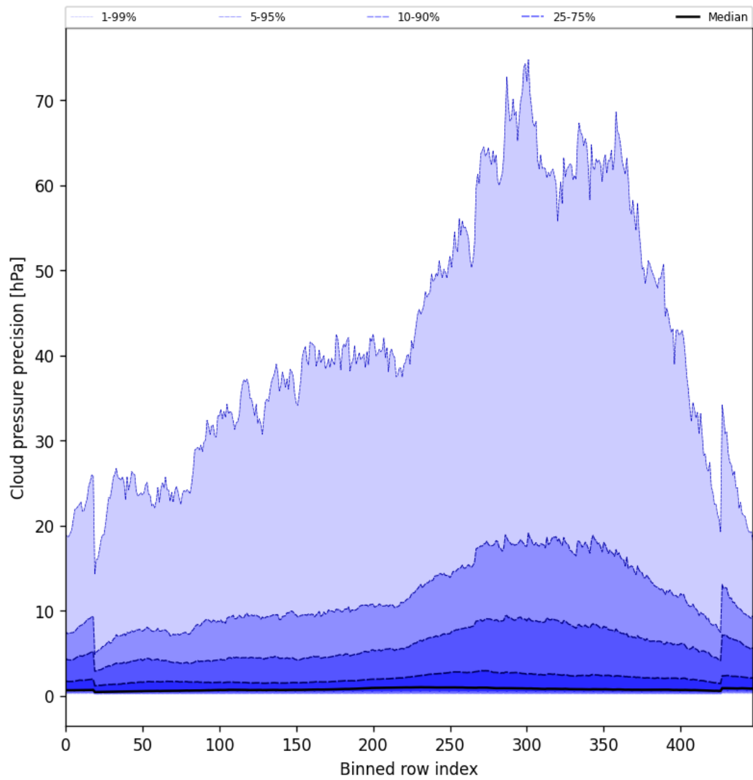
Figure 48: Along track statistics of “Cloud pressure precision” for 2025-09-01 to 2025-09-03
