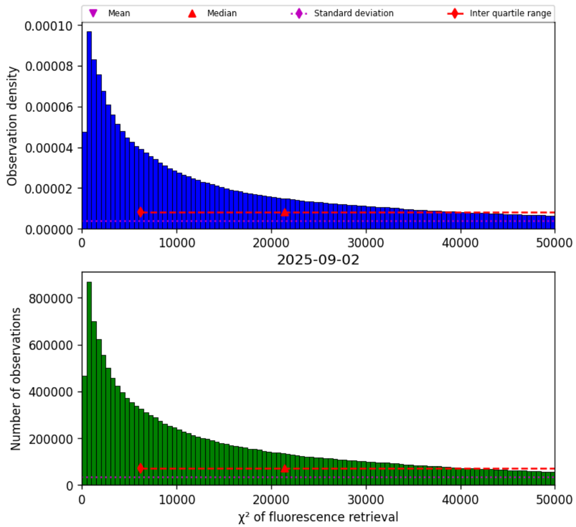
Figure 42: Histogram of “ \chi^2 of fluorescence retrieval” for 2025-09-01 to 2025-09-03
