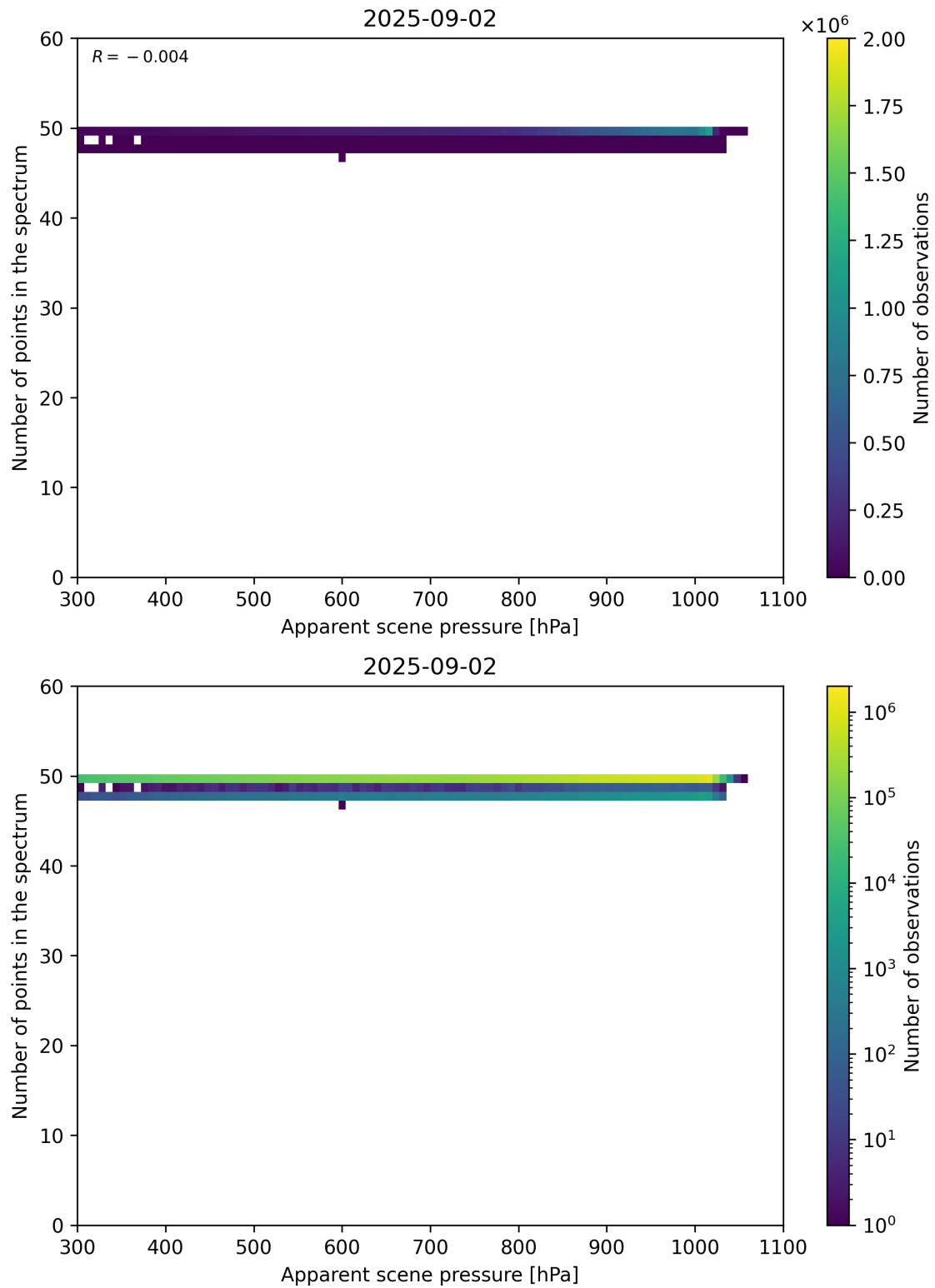
Figure 66: Scatter density plot of “Apparent scene pressure” against “Number of points in the spectrum” for 2025-09-01 to 2025-09-03.
