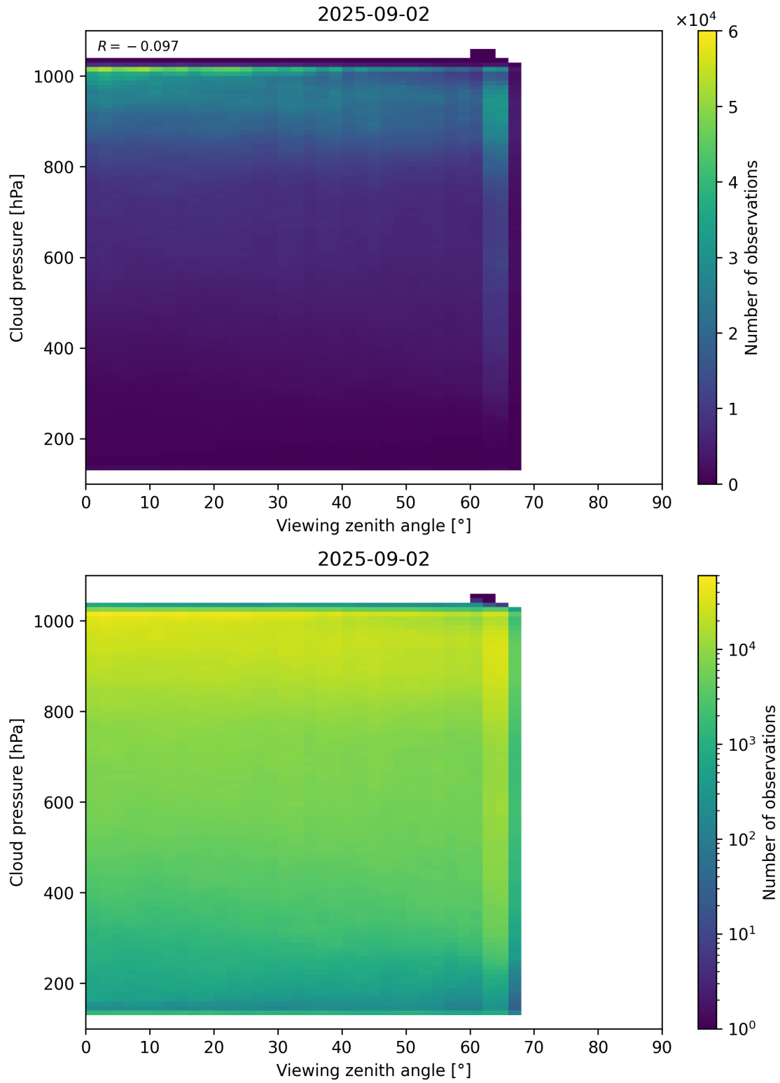
Figure 121: Scatter density plot of “Viewing zenith angle” against “Cloud pressure” for 2025-09-01 to 2025-09-03.
