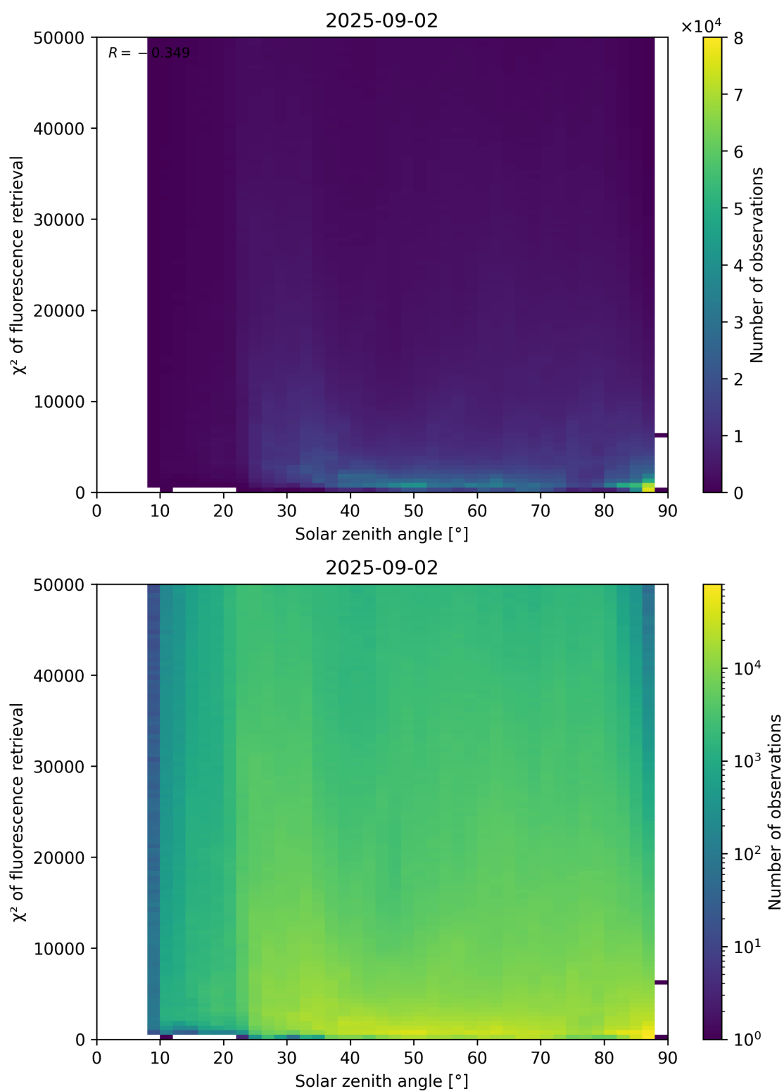
Figure 109: Scatter density plot of “Solar zenith angle” against “ \chi^2 of fluorescence retrieval” for 2025-09-01 to 2025-09-03.
