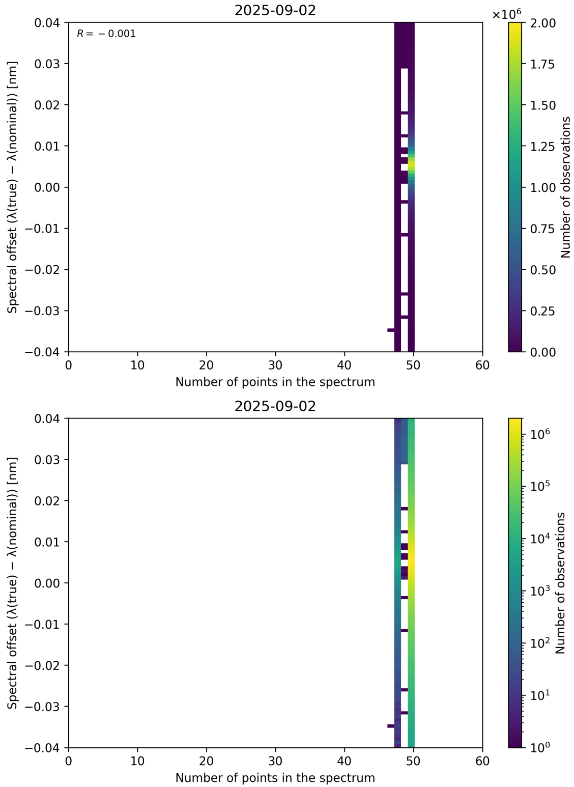
Figure 101: Scatter density plot of “Number of points in the spectrum” against “Spectral offset ( \lambda_{\text{true}} - \lambda_{\text{nominal}} )” for 2025-09-01 to 2025-09-03.
