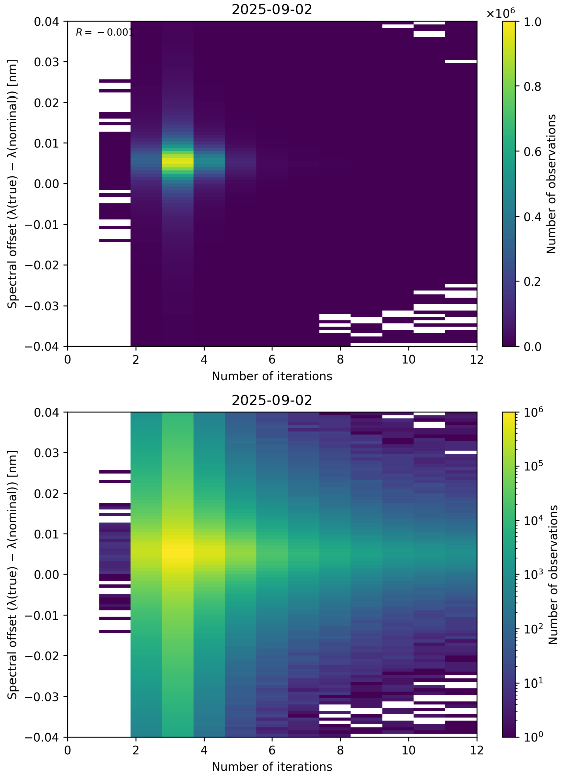
Figure 100: Scatter density plot of “Number of iterations” against “Spectral offset ( \lambda_{\text{true}} - \lambda_{\text{nominal}} )” for 2025-09-01 to 2025-09-03.
