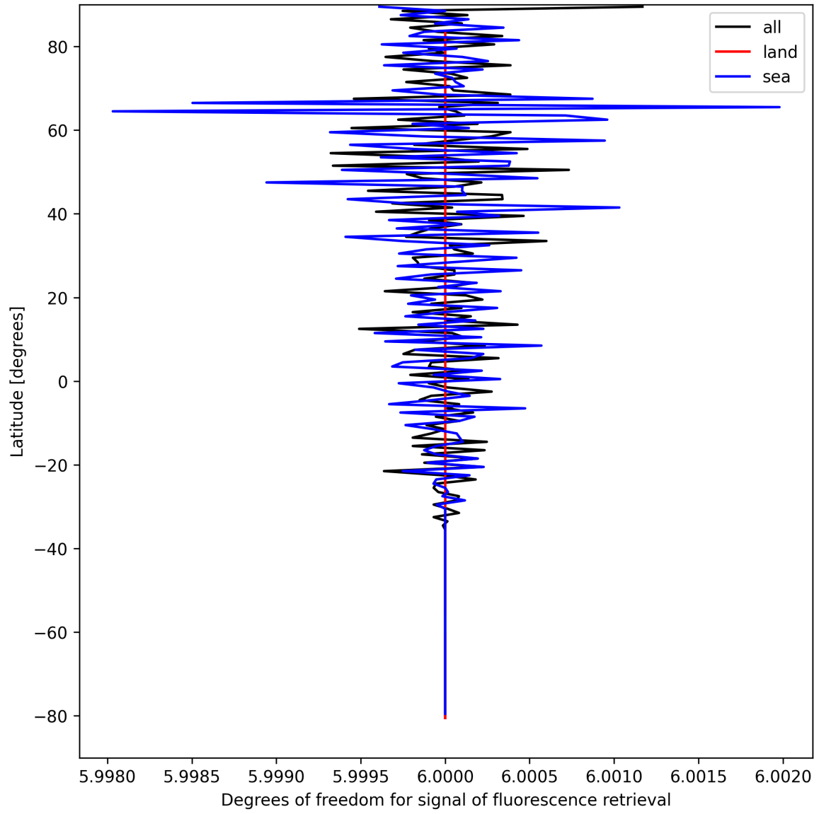
Figure 26: Zonal average of “Degrees of freedom for signal of fluorescence retrieval” for 2025-09-01 to 2025-09-03.
