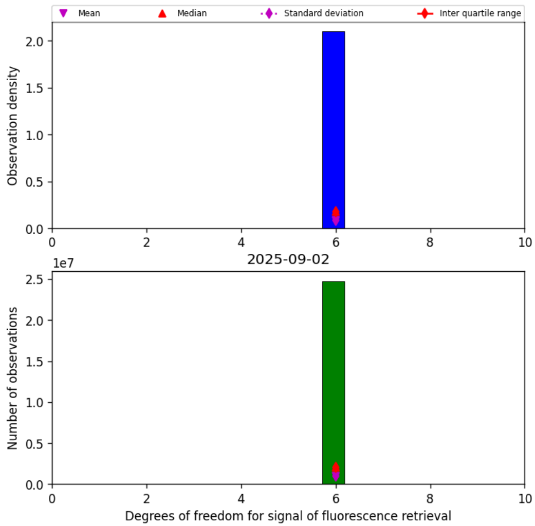
Figure 43: Histogram of "Degrees of freedom for signal of fluorescence retrieval" for 2025-09-01 to 2025-09-03
