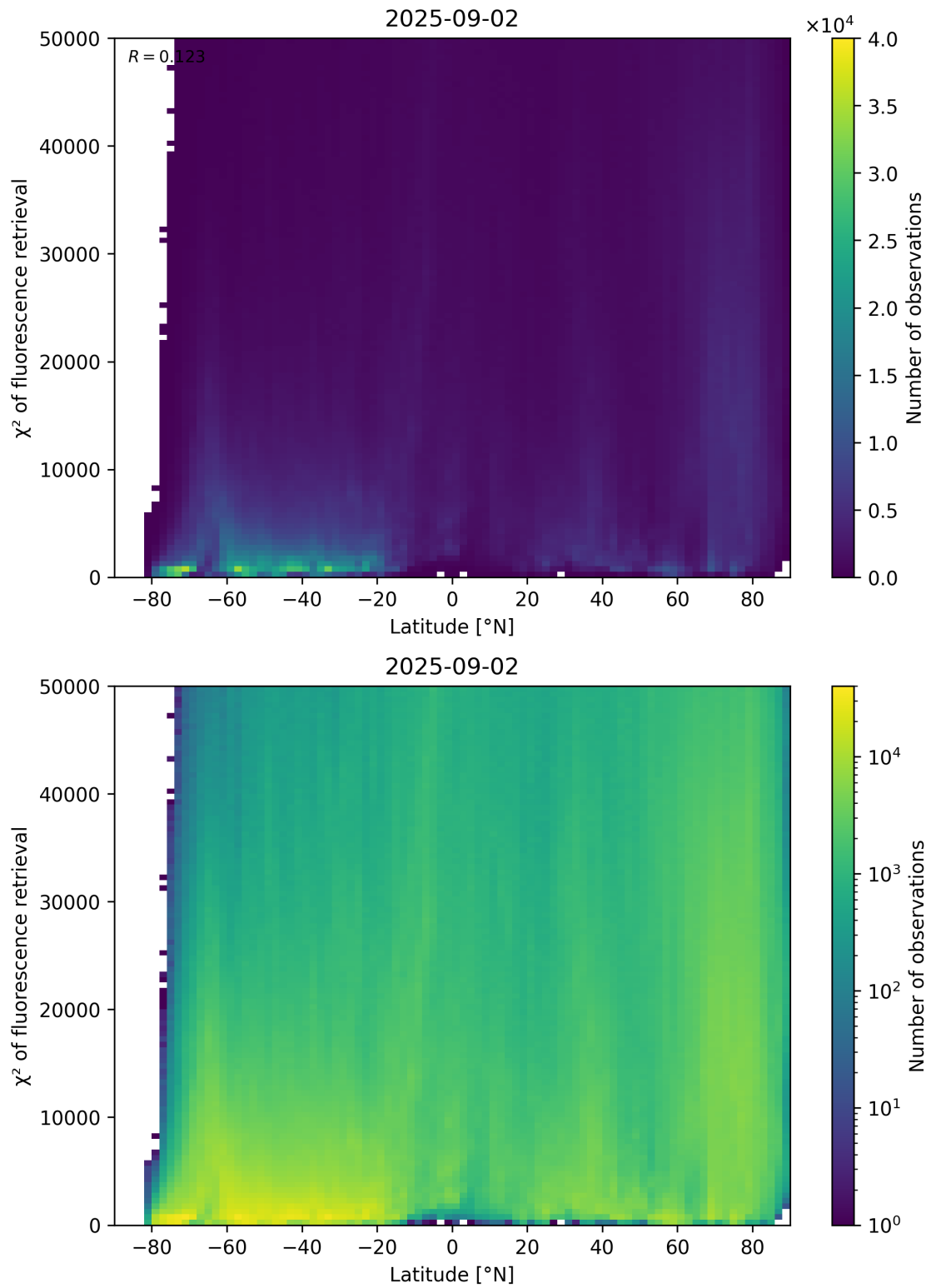
Figure 89: Scatter density plot of “Latitude” against “ \chi^2 of fluorescence retrieval” for 2025-09-01 to 2025-09-03.
