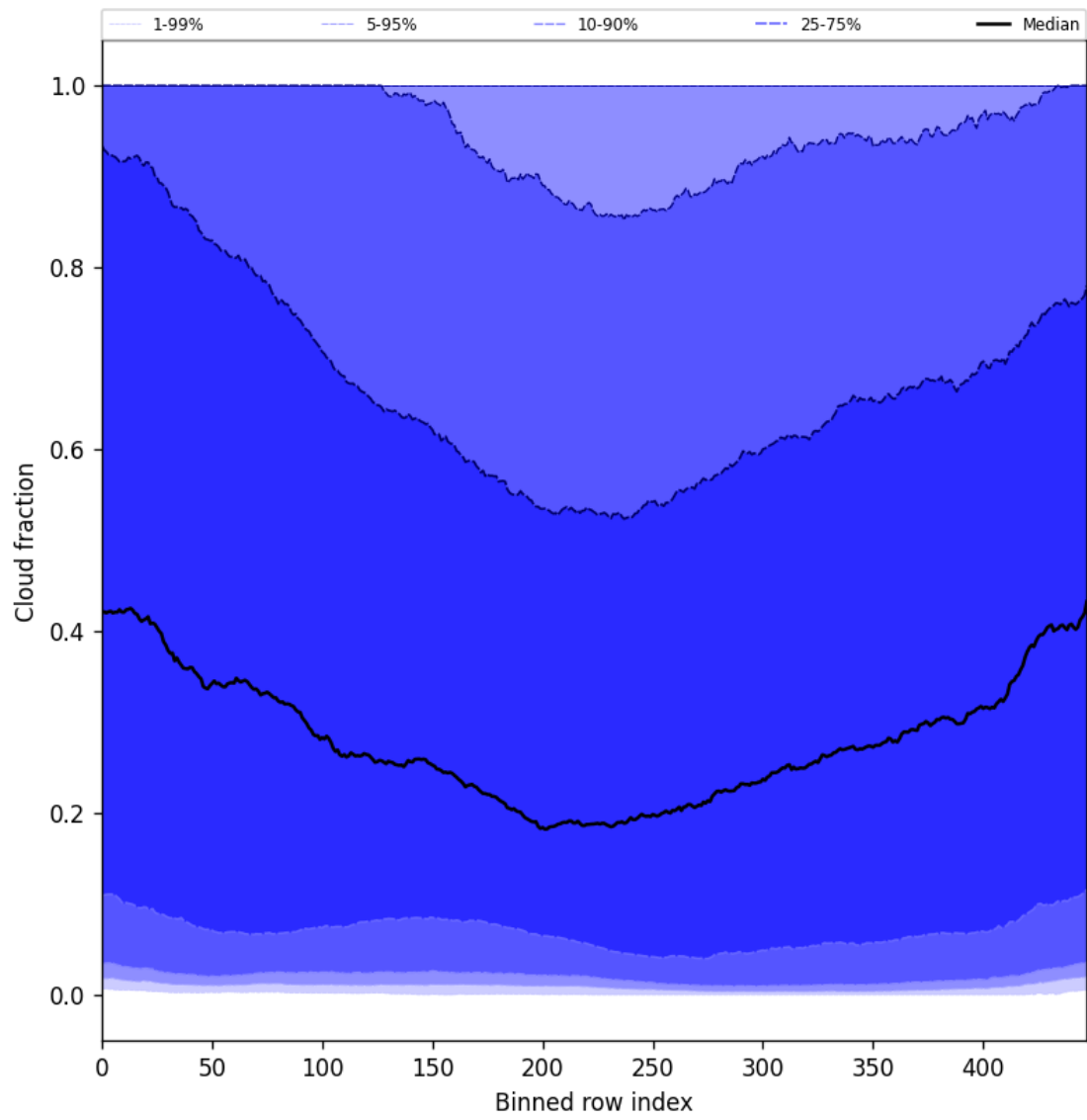
Figure 49: Along track statistics of “Cloud fraction” for 2025-09-01 to 2025-09-03
