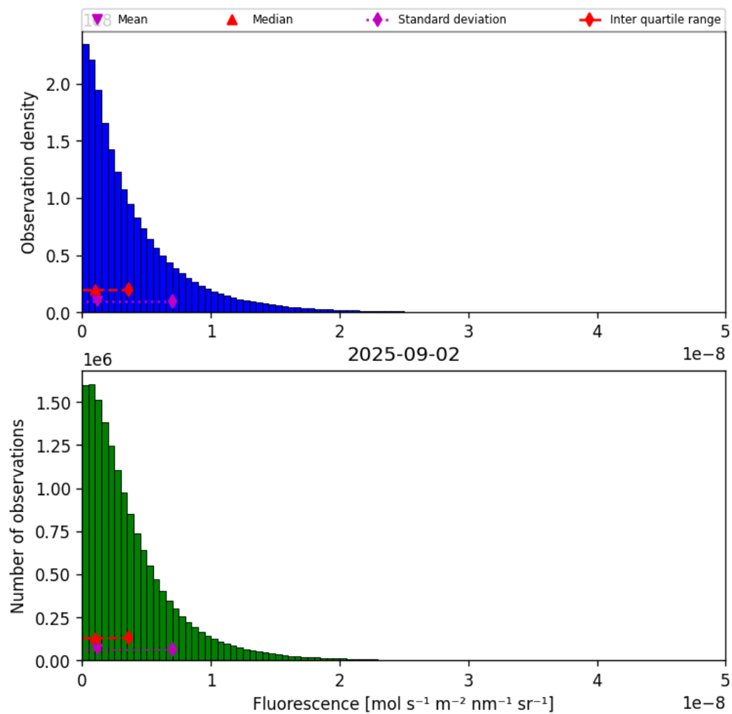
Figure 40: Histogram of “Fluorescence” for 2025-09-01 to 2025-09-03
