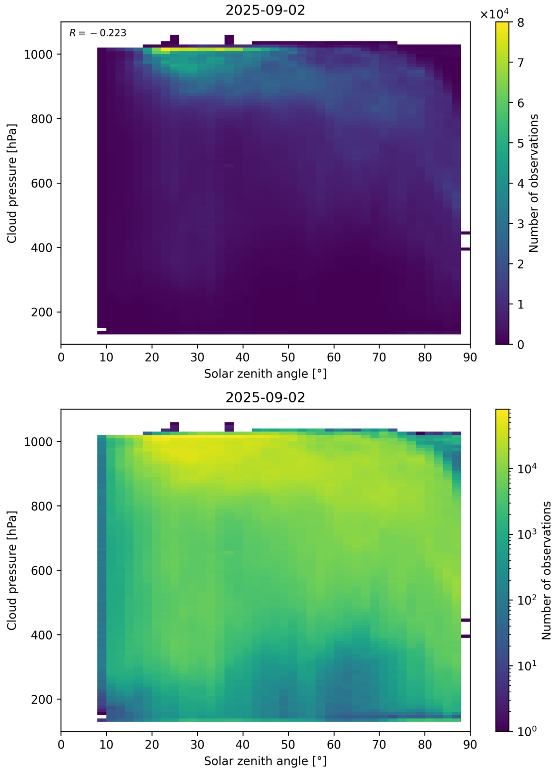
Figure 111: Scatter density plot of “Solar zenith angle” against “Cloud pressure” for 2025-09-01 to 2025-09-03.
