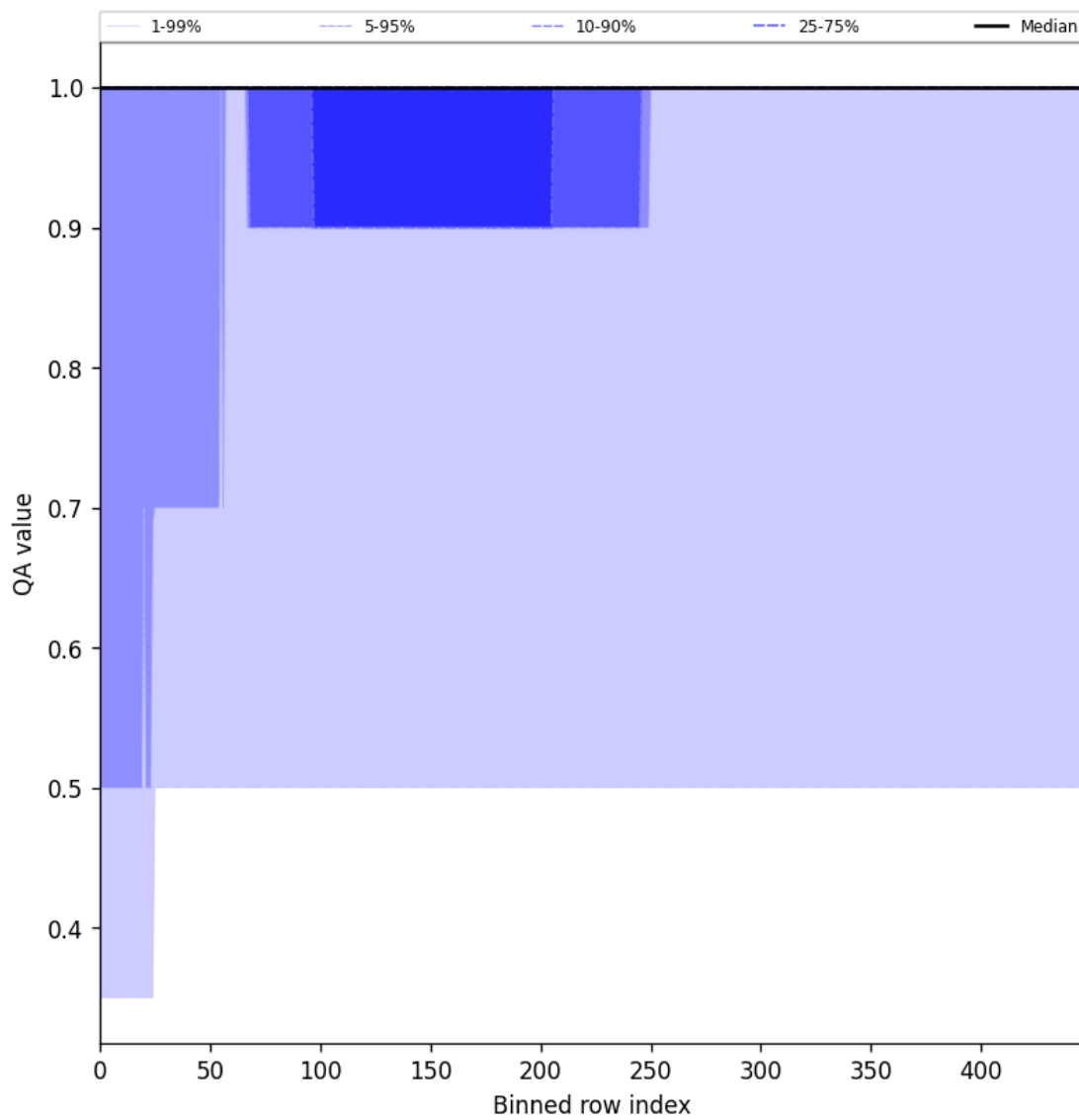
Figure 46: Along track statistics of “QA value” for 2025-09-01 to 2025-09-03
