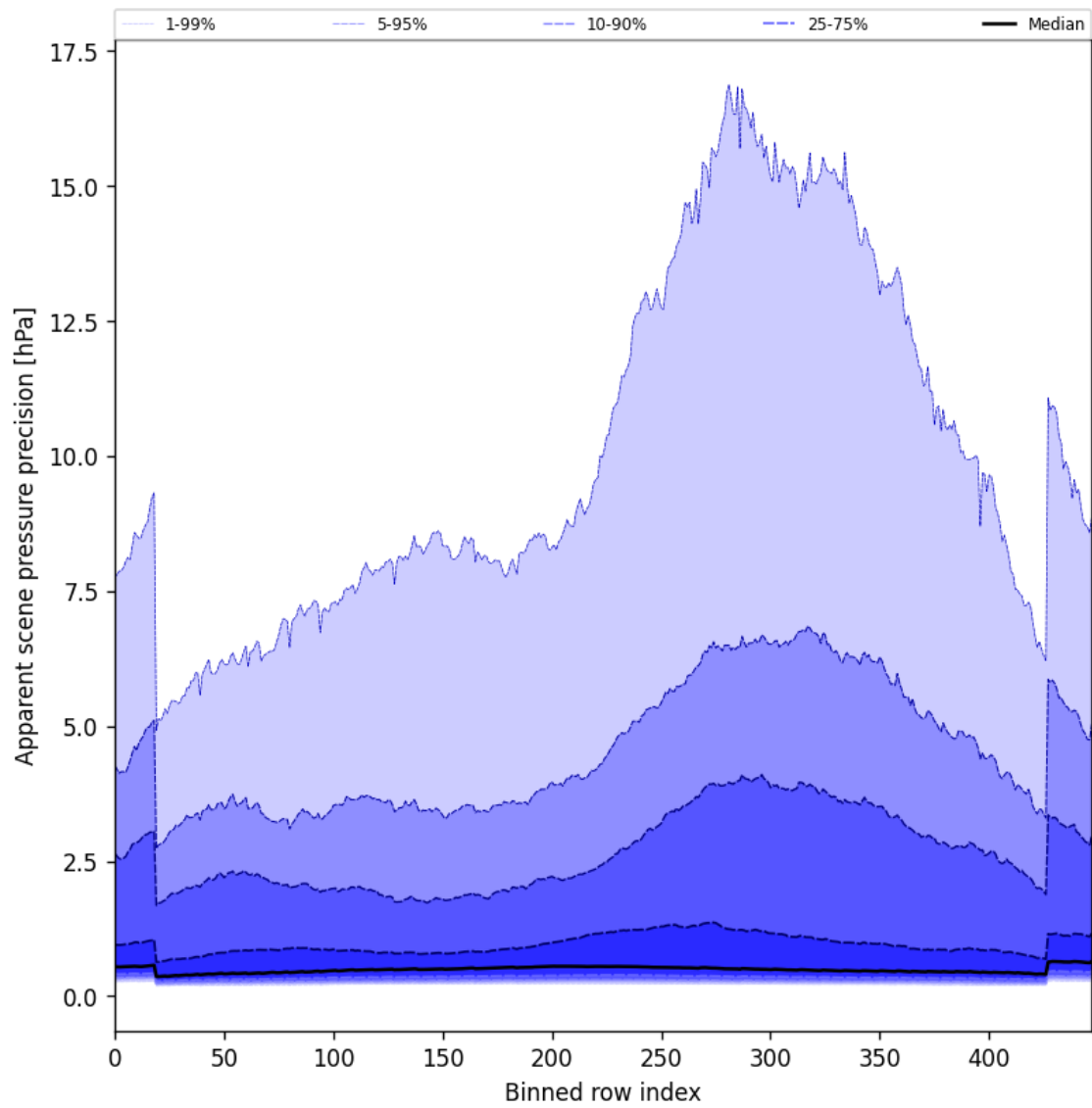
Figure 54: Along track statistics of “Apparent scene pressure precision” for 2025-09-01 to 2025-09-03
