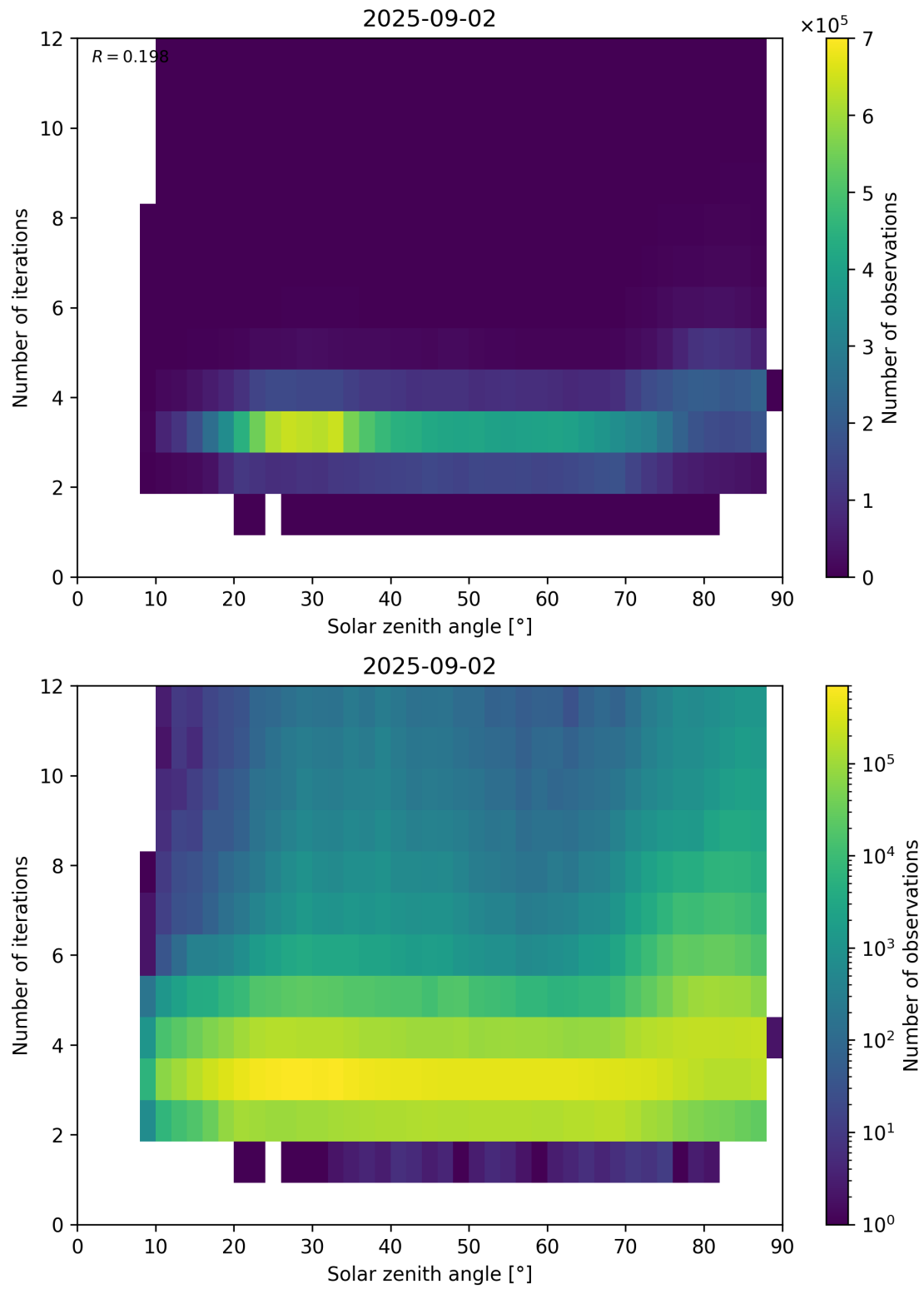
Figure 114: Scatter density plot of “Solar zenith angle” against “Number of iterations” for 2025-09-01 to 2025-09-03.
