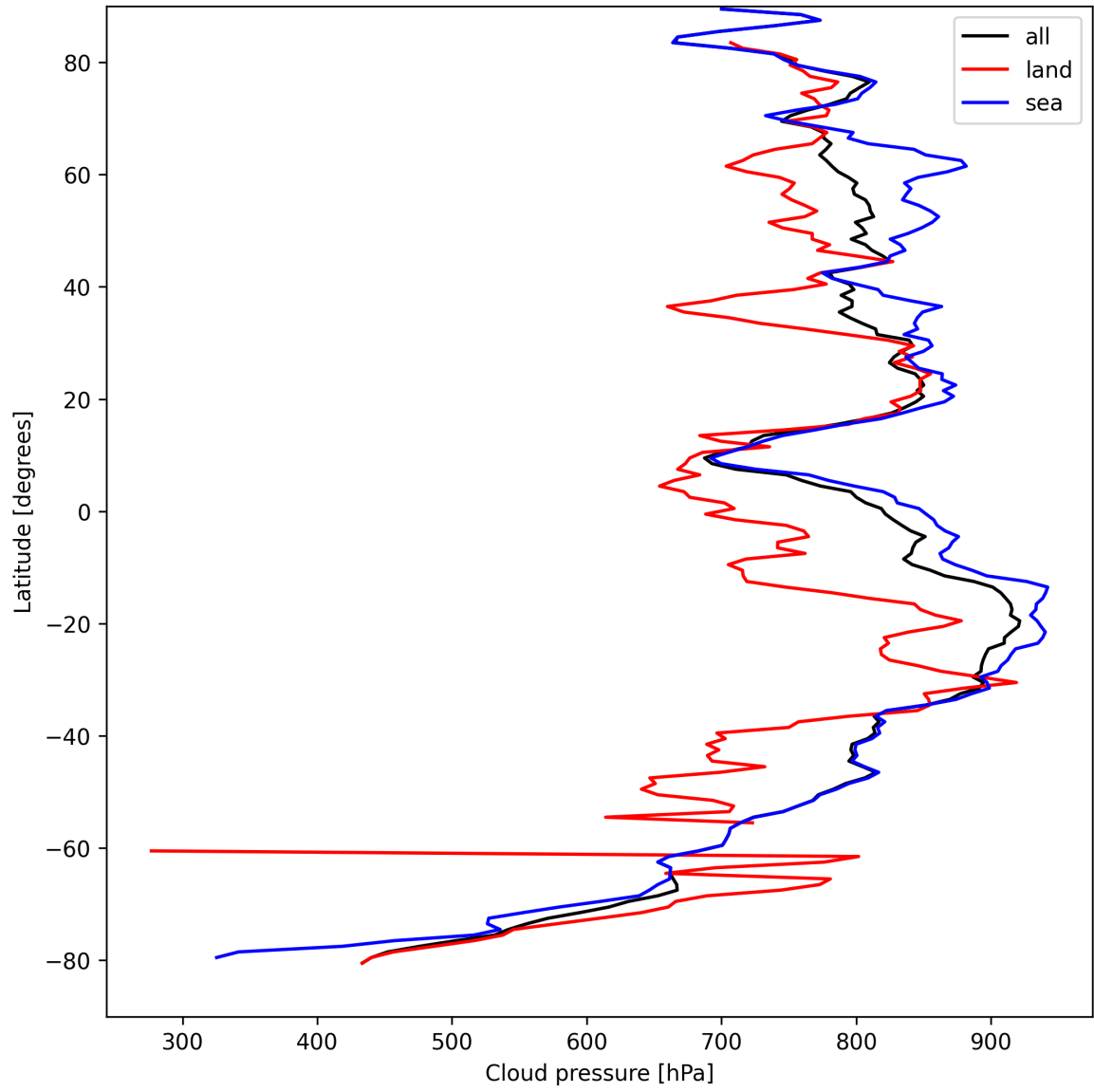
Figure 13: Zonal average of “Cloud pressure” for 2025-09-01 to 2025-09-03.
