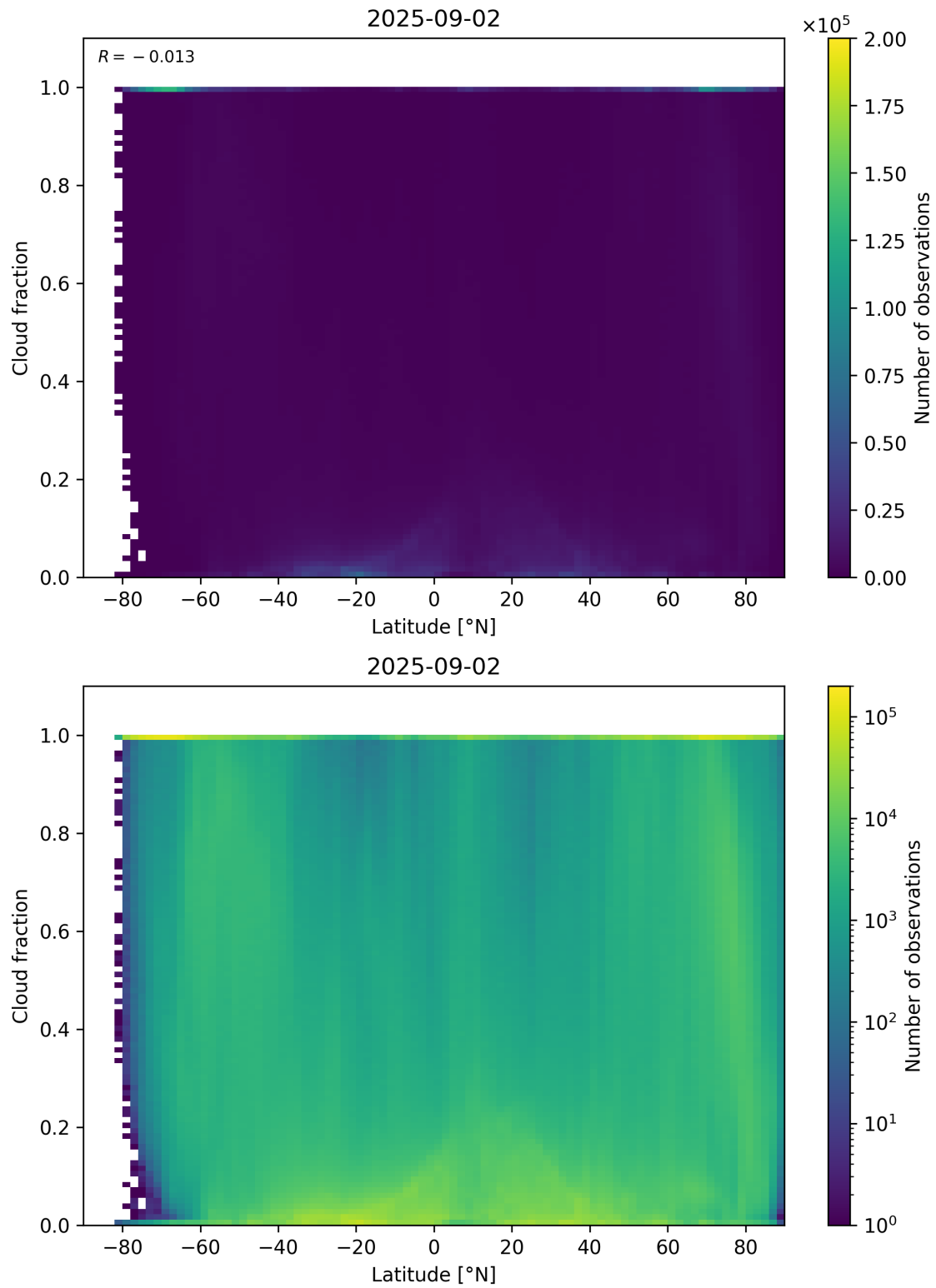
Figure 90: Scatter density plot of “Latitude” against “Cloud fraction” for 2025-09-01 to 2025-09-03.
