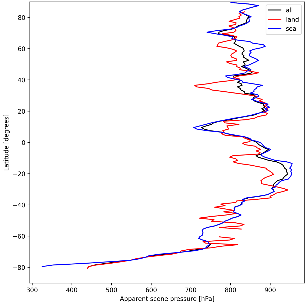
Figure 19: Zonal average of “Apparent scene pressure” for 2025-09-01 to 2025-09-03.
