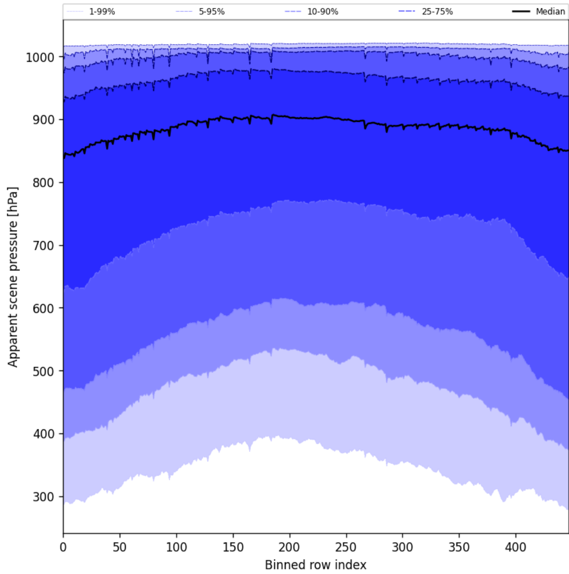
Figure 53: Along track statistics of “Apparent scene pressure” for 2025-09-01 to 2025-09-03
