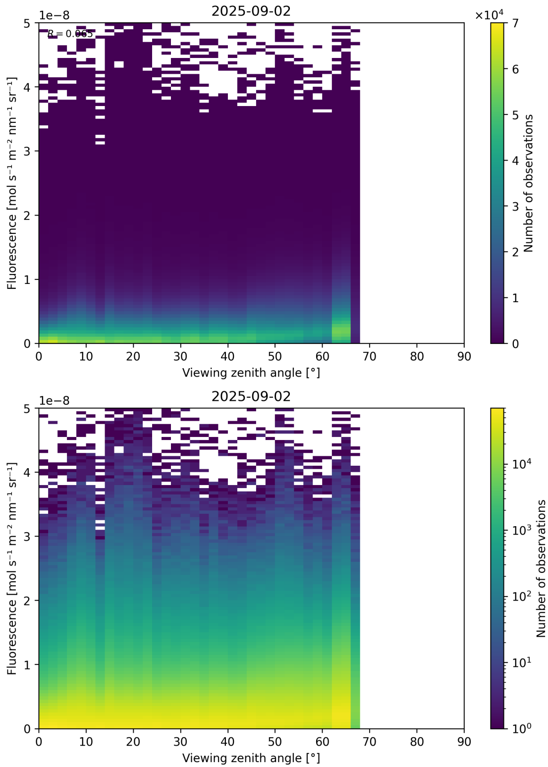
Figure 122: Scatter density plot of “Viewing zenith angle” against “Fluorescence” for 2025-09-01 to 2025-09-03.
