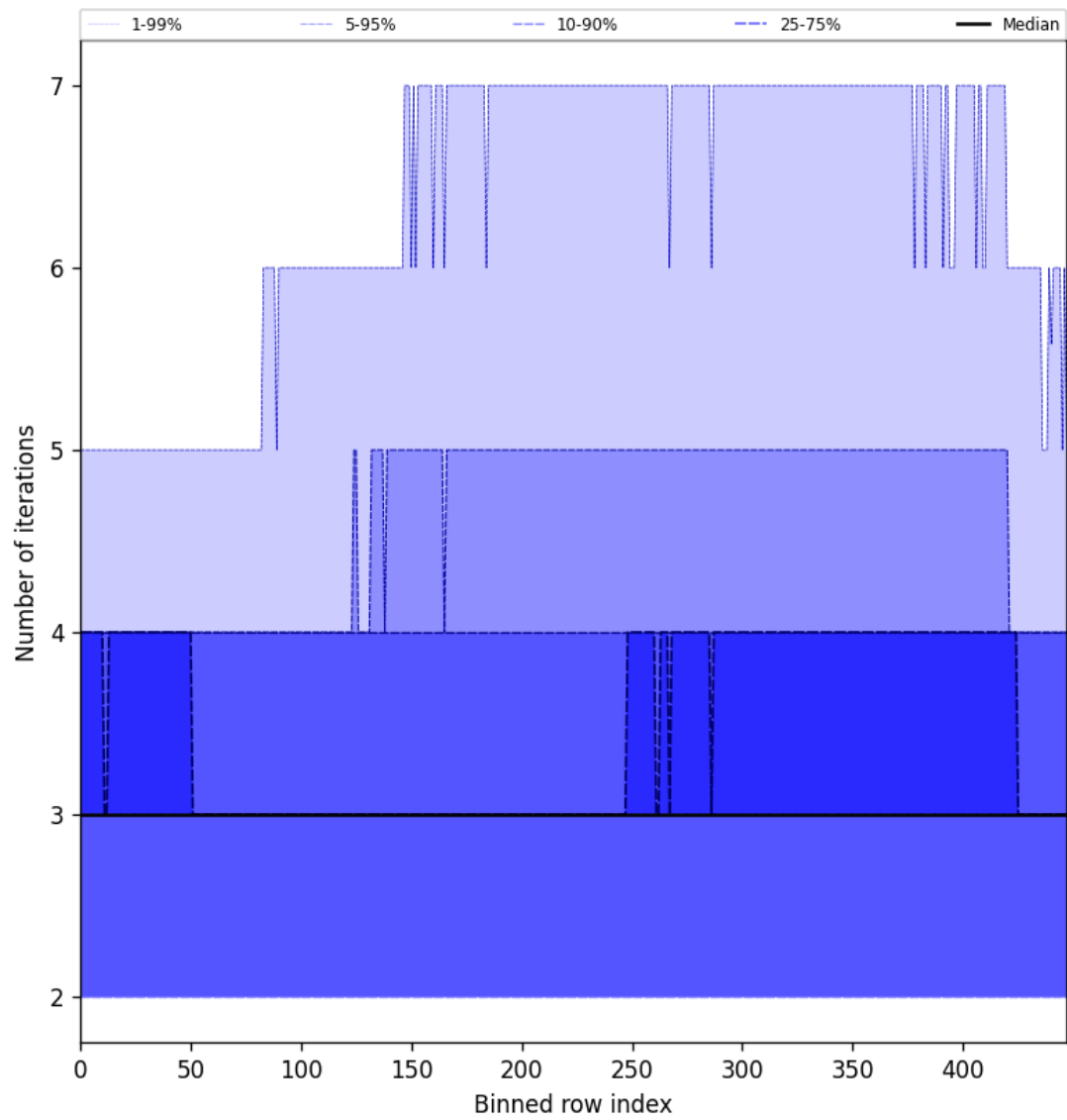
Figure 56: Along track statistics of “Number of iterations” for 2025-09-01 to 2025-09-03
