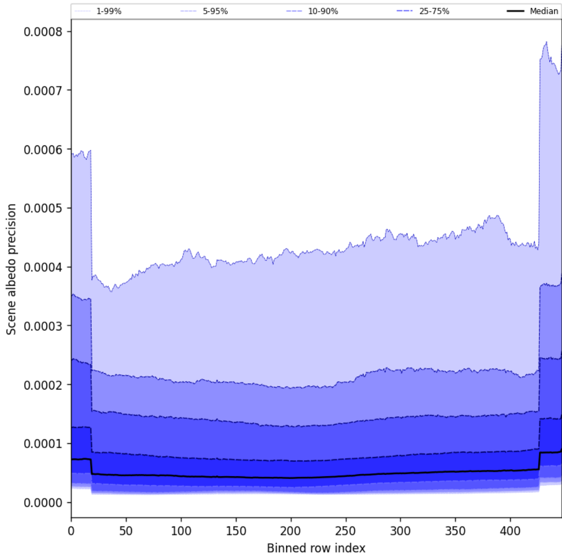
Figure 52: Along track statistics of “Scene albedo precision” for 2025-09-01 to 2025-09-03
