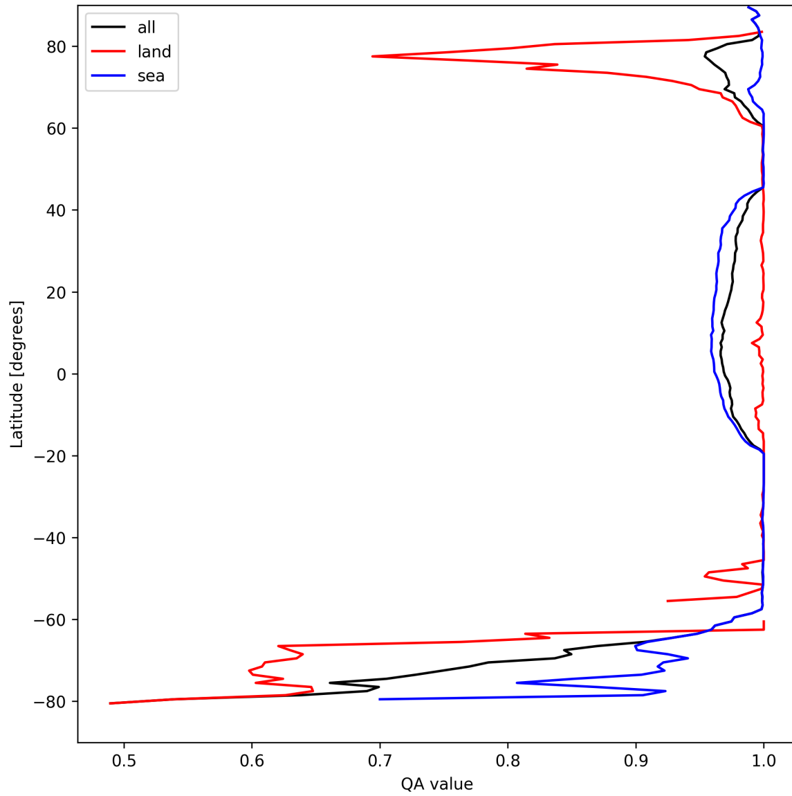
Figure 12: Zonal average of "QA value" for 2025-09-01 to 2025-09-03.
