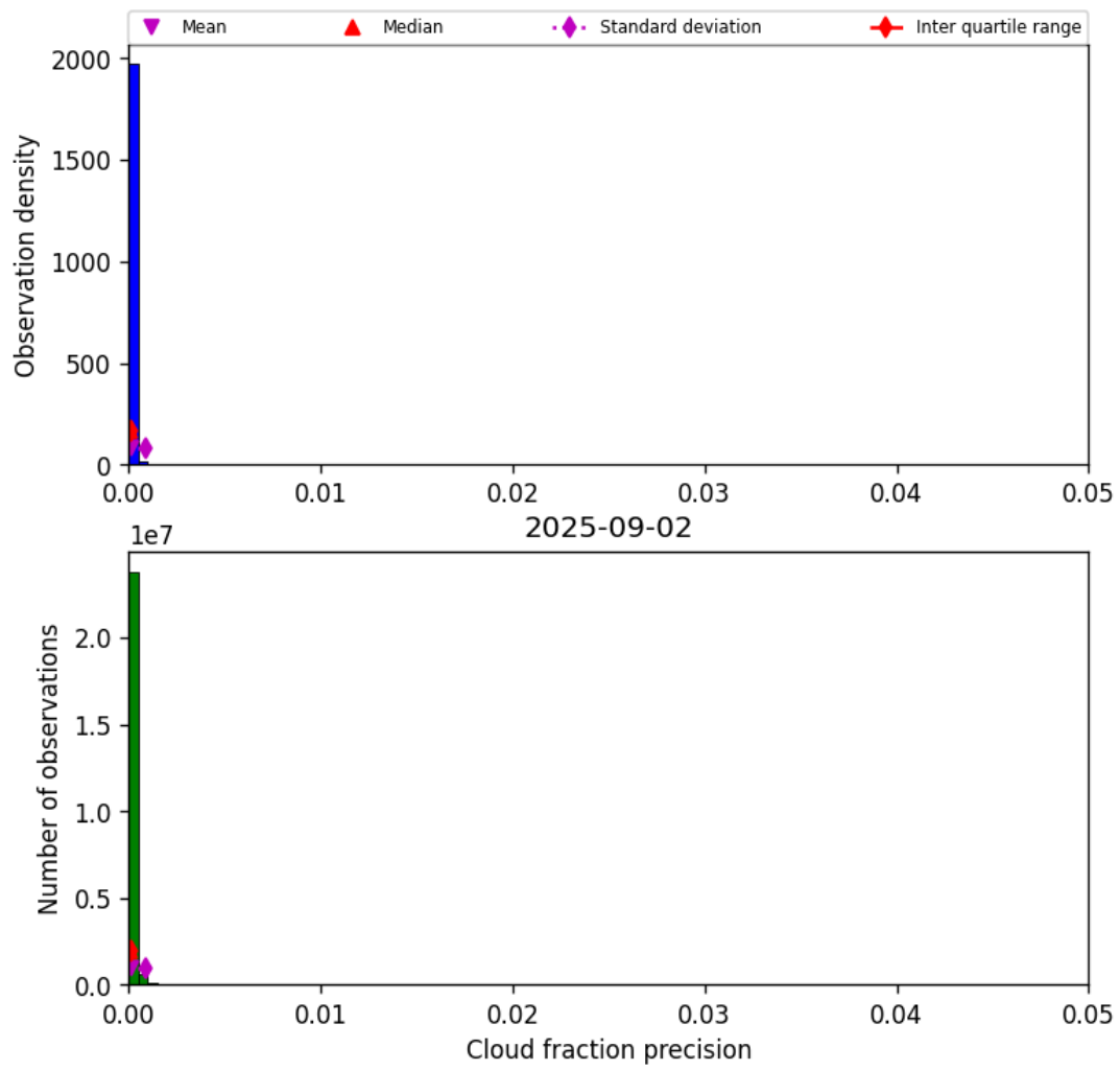
Figure 33: Histogram of “Cloud fraction precision” for 2025-09-01 to 2025-09-03
