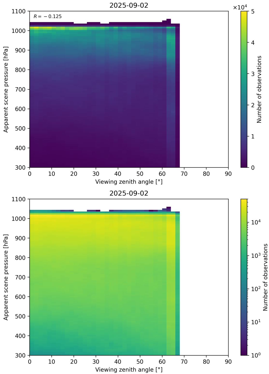
Figure 118: Scatter density plot of “Viewing zenith angle” against “Apparent scene pressure” for 2025-09-01 to 2025-09-03.
