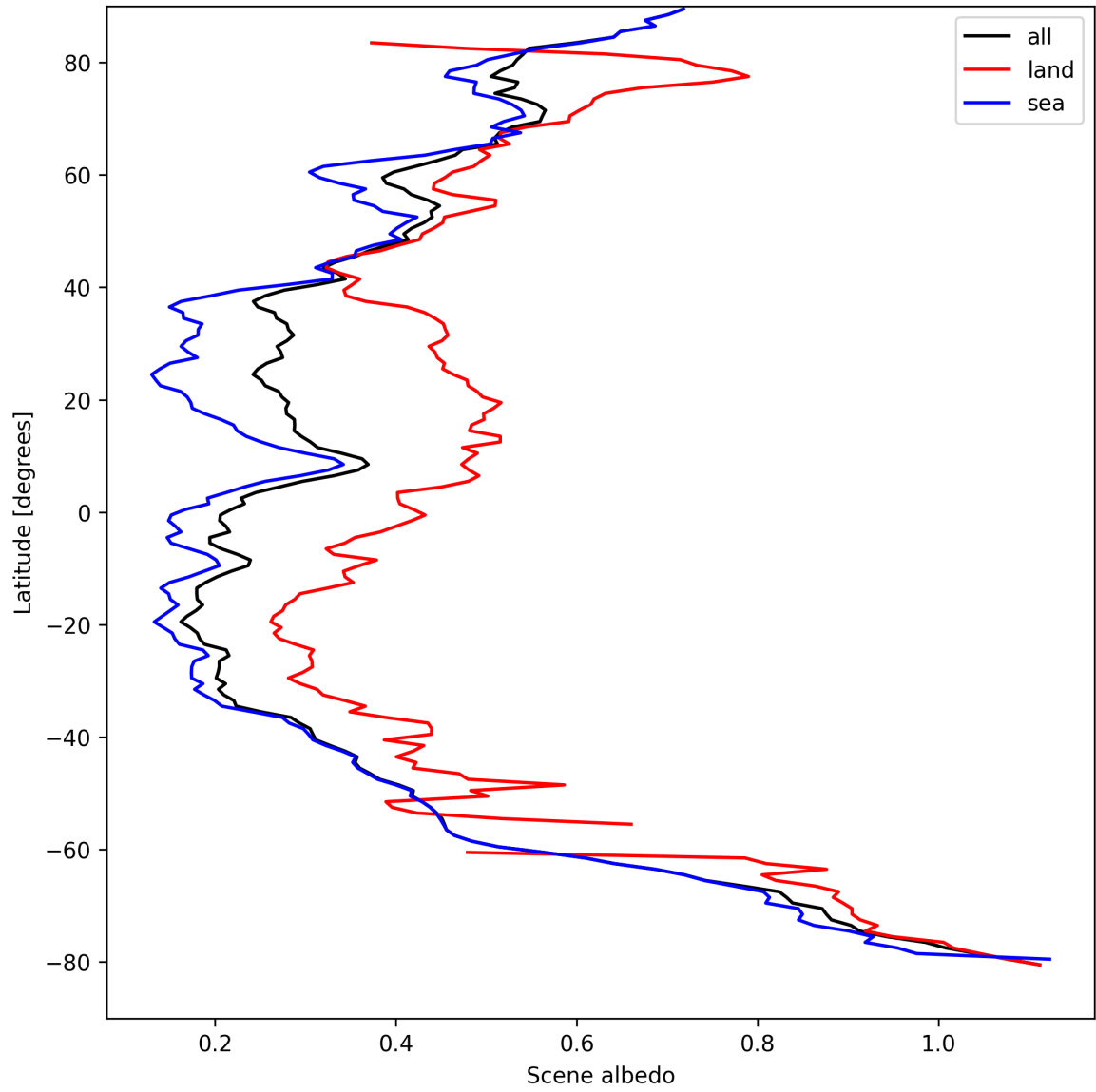
Figure 17: Zonal average of “Scene albedo” for 2025-09-01 to 2025-09-03.
