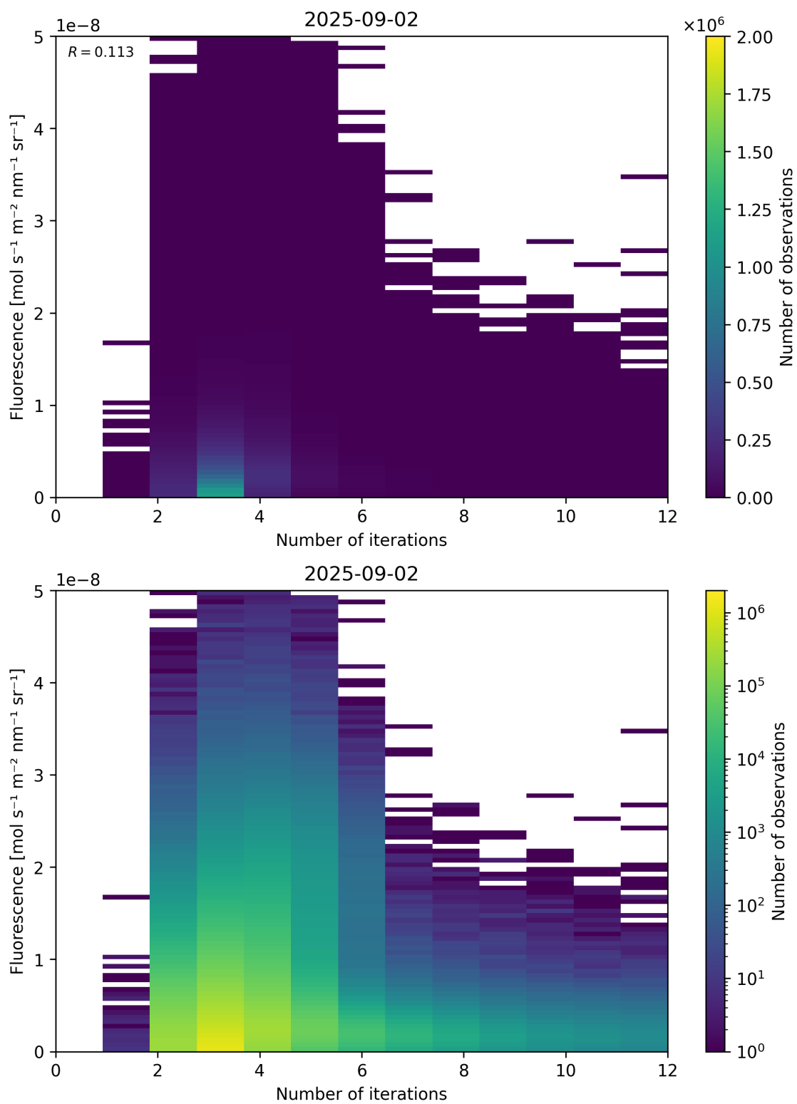
Figure 98: Scatter density plot of “Number of iterations” against “Fluorescence” for 2025-09-01 to 2025-09-03.
