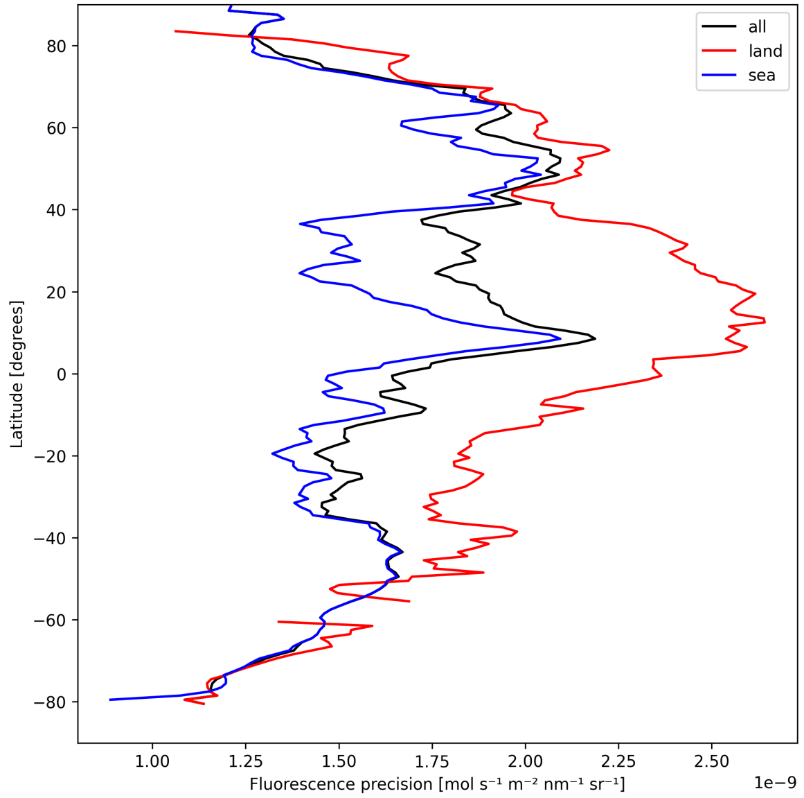
Figure 24: Zonal average of “Fluorescence precision” for 2025-09-01 to 2025-09-03.
