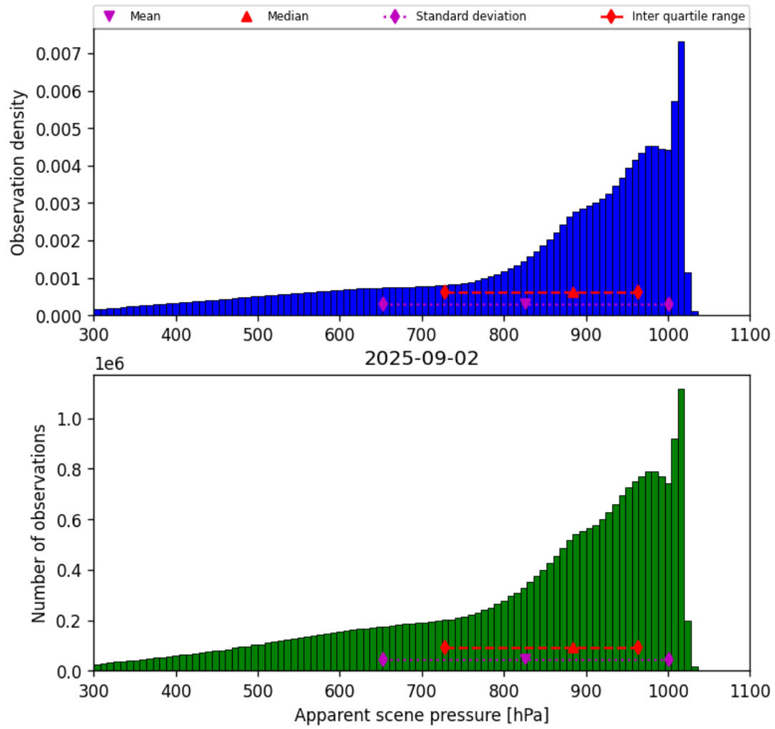
Figure 36: Histogram of “Apparent scene pressure” for 2025-09-01 to 2025-09-03
