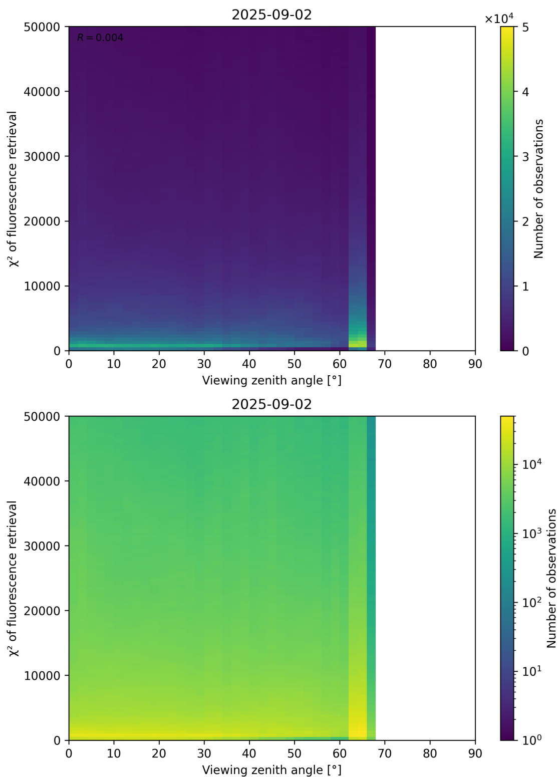
Figure 119: Scatter density plot of “Viewing zenith angle” against “ \chi^2 of fluorescence retrieval” for 2025-09-01 to 2025-09-03.
