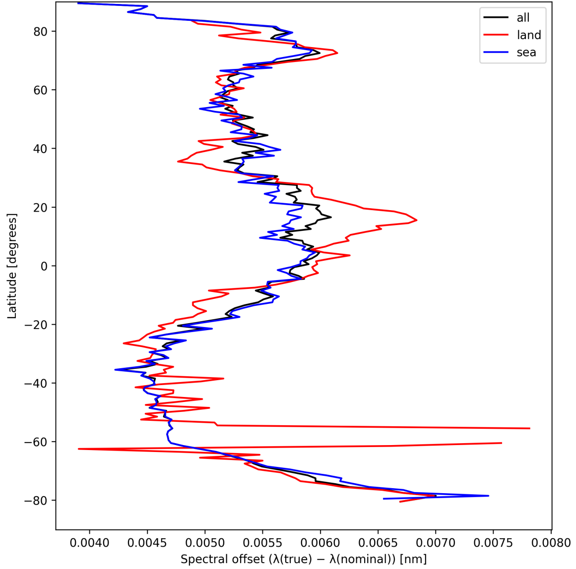
Figure 28: Zonal average of “Spectral offset ( \lambda_{\text{true}} - \lambda_{\text{nominal}} )” for 2025-09-01 to 2025-09-03.
