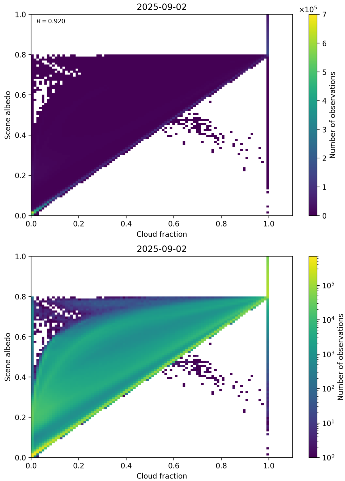
Figure 75: Scatter density plot of “Cloud fraction” against “Scene albedo” for 2025-09-01 to 2025-09-03.
