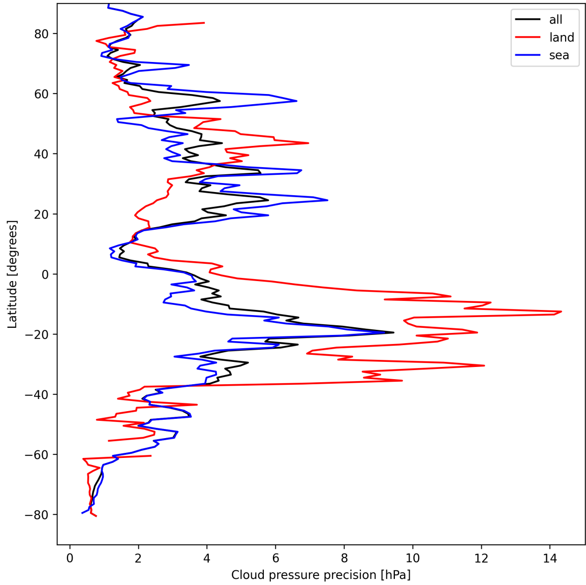
Figure 14: Zonal average of “Cloud pressure precision” for 2025-09-01 to 2025-09-03.
