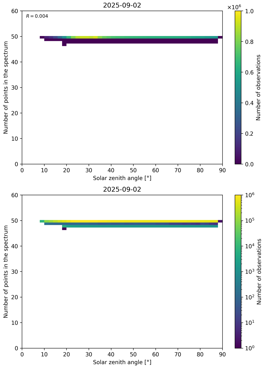
Figure 115: Scatter density plot of “Solar zenith angle” against “Number of points in the spectrum” for 2025-09-01 to 2025-09-03.
