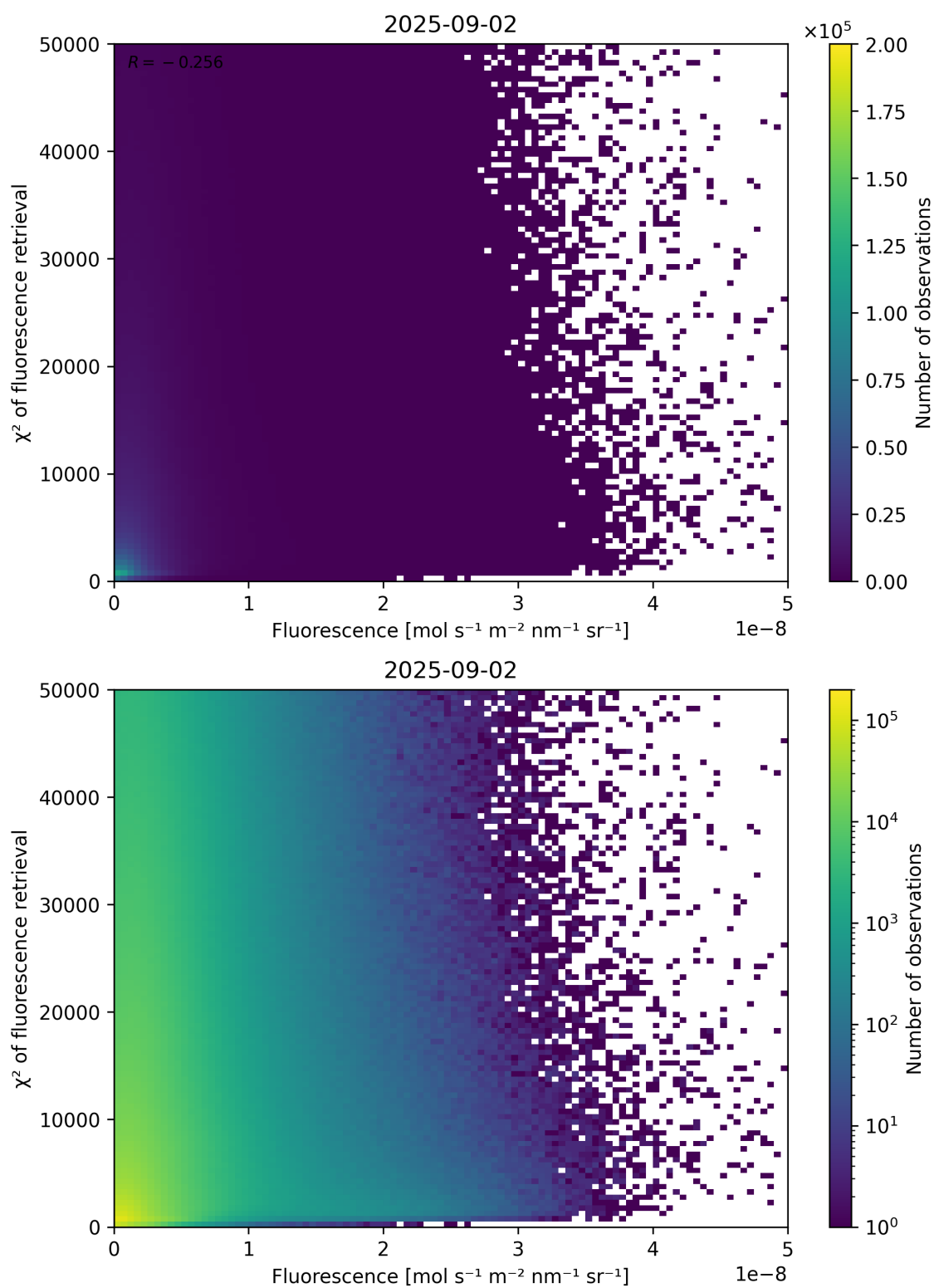
Figure 85: Scatter density plot of “Fluorescence” against “ \chi^2 of fluorescence retrieval” for 2025-09-01 to 2025-09-03.
