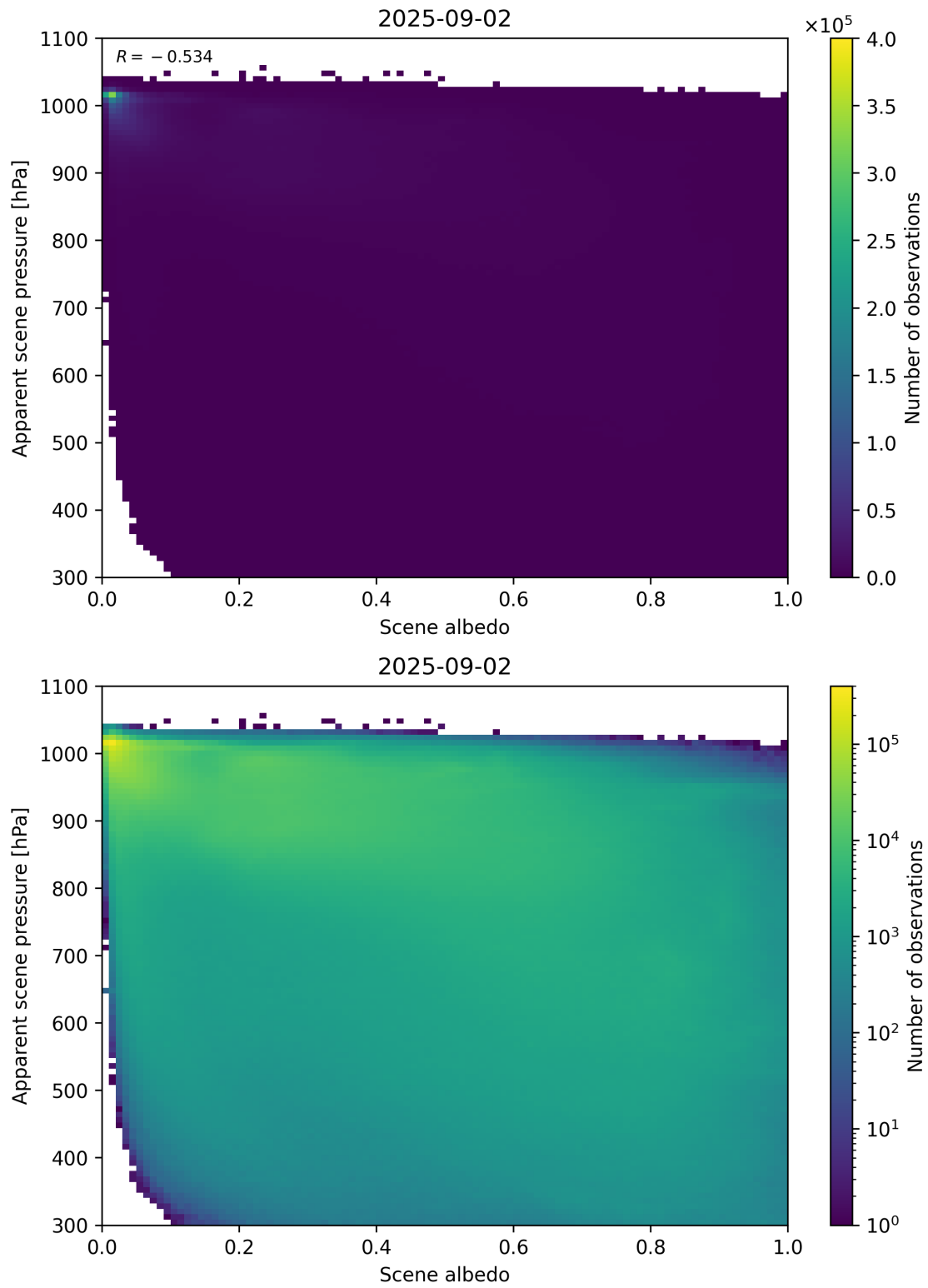
Figure 102: Scatter density plot of “Scene albedo” against “Apparent scene pressure” for 2025-09-01 to 2025-09-03.
