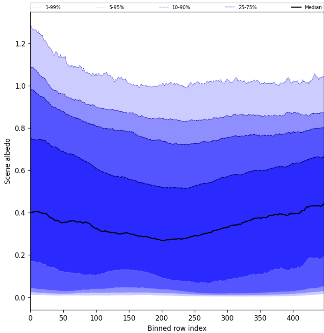
Figure 51: Along track statistics of “Scene albedo” for 2025-09-01 to 2025-09-03
