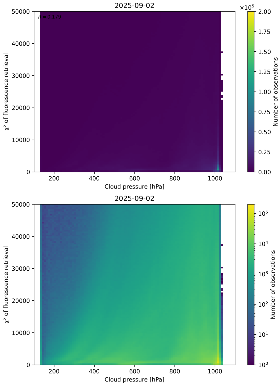
Figure 78: Scatter density plot of “Cloud pressure” against “ \chi^2 of fluorescence retrieval” for 2025-09-01 to 2025-09-03.
