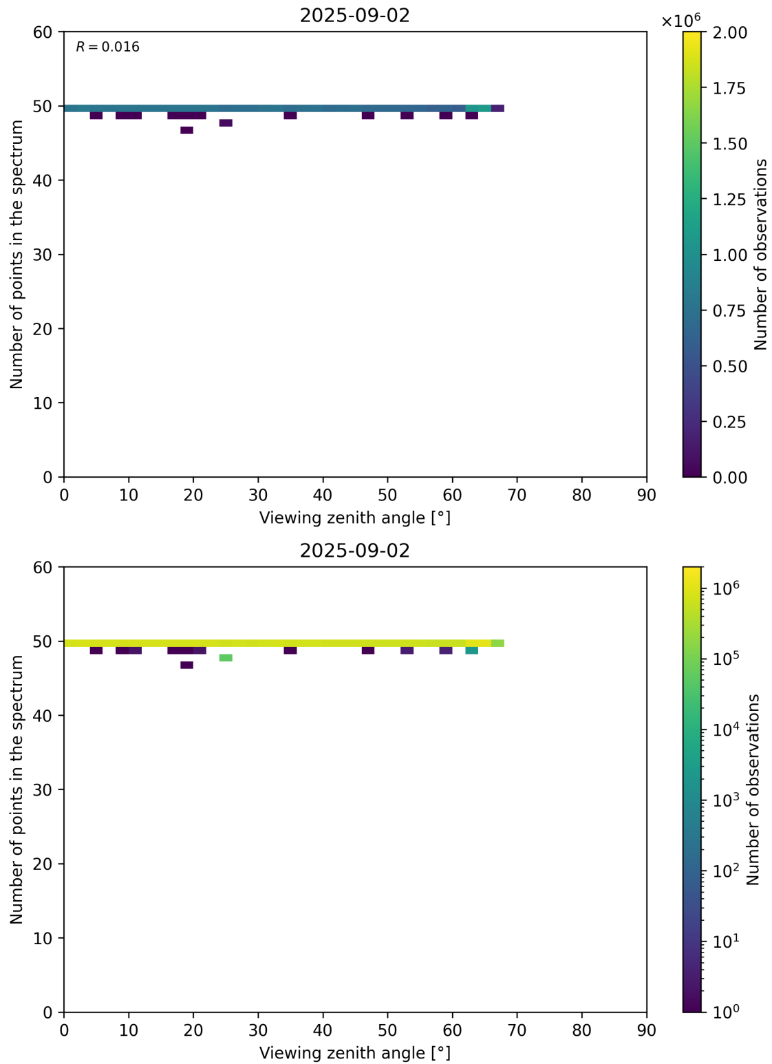
Figure 125: Scatter density plot of “Viewing zenith angle” against “Number of points in the spectrum” for 2025-09-01 to 2025-09-03.
