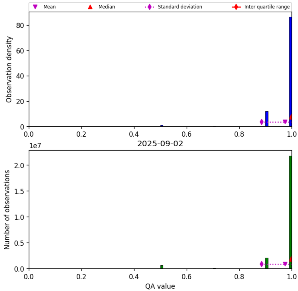
Figure 29: Histogram of “QA value” for 2025-09-01 to 2025-09-03
