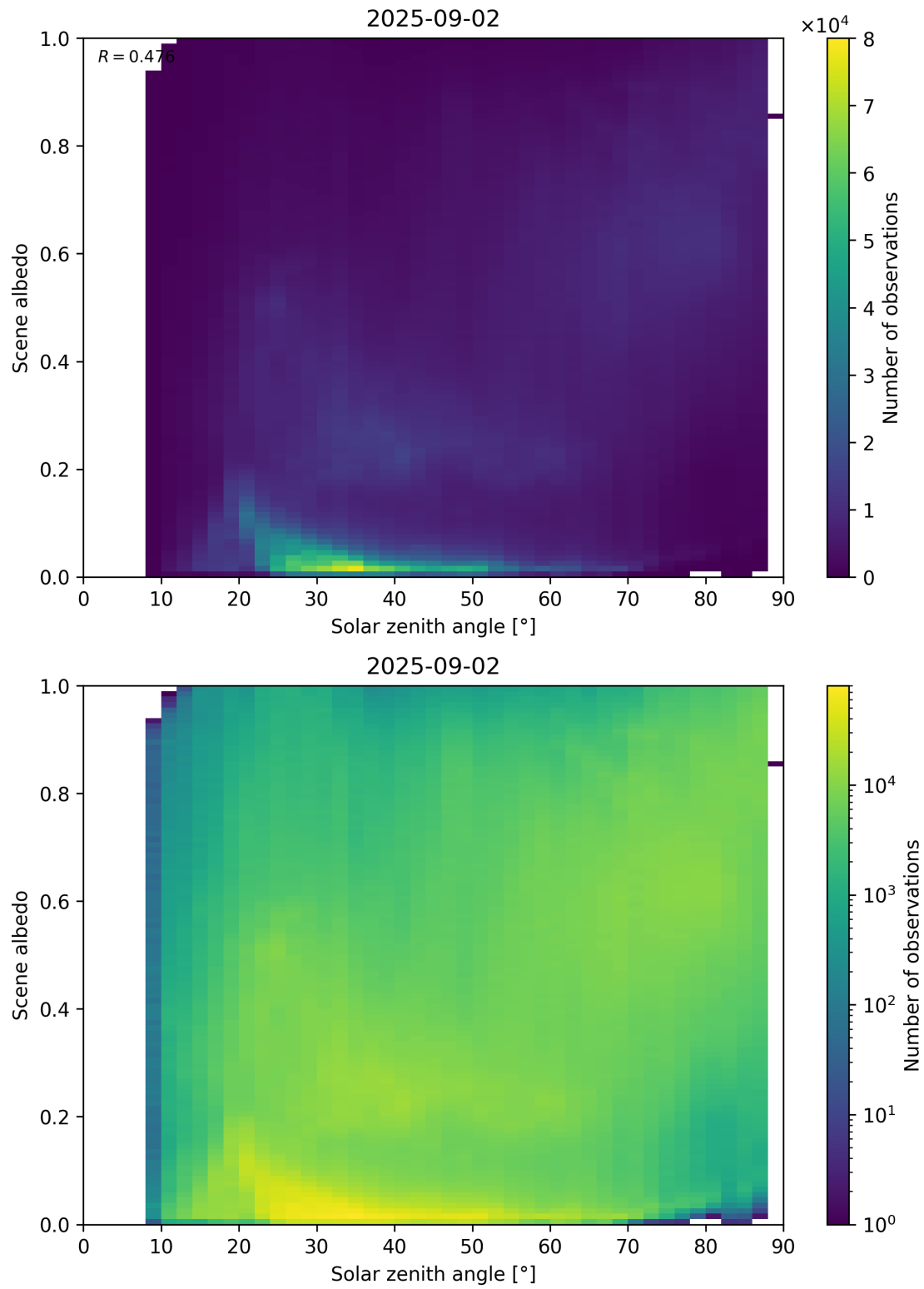
Figure 116: Scatter density plot of “Solar zenith angle” against “Scene albedo” for 2025-09-01 to 2025-09-03.
