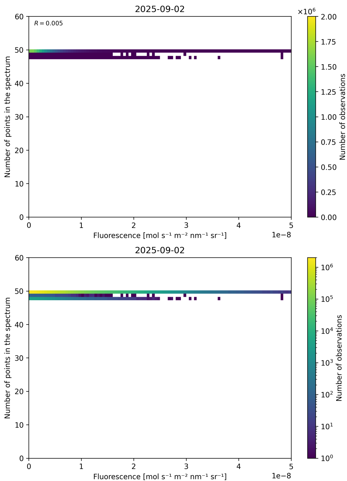
Figure 86: Scatter density plot of “Fluorescence” against “Number of points in the spectrum” for 2025-09-01 to 2025-09-03.
