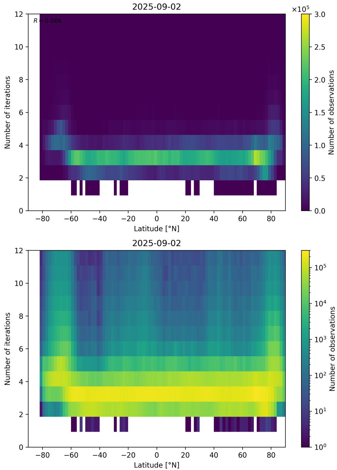
Figure 93: Scatter density plot of “Latitude” against “Number of iterations” for 2025-09-01 to 2025-09-03.
