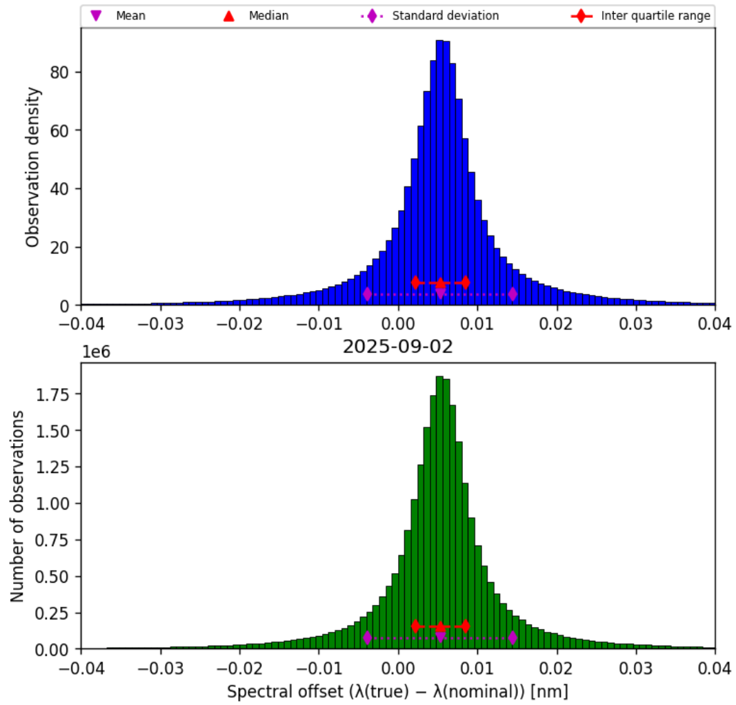
Figure 45: Histogram of “Spectral offset ( \lambda_{\text{true}} - \lambda_{\text{nominal}} )” for 2025-09-01 to 2025-09-03
