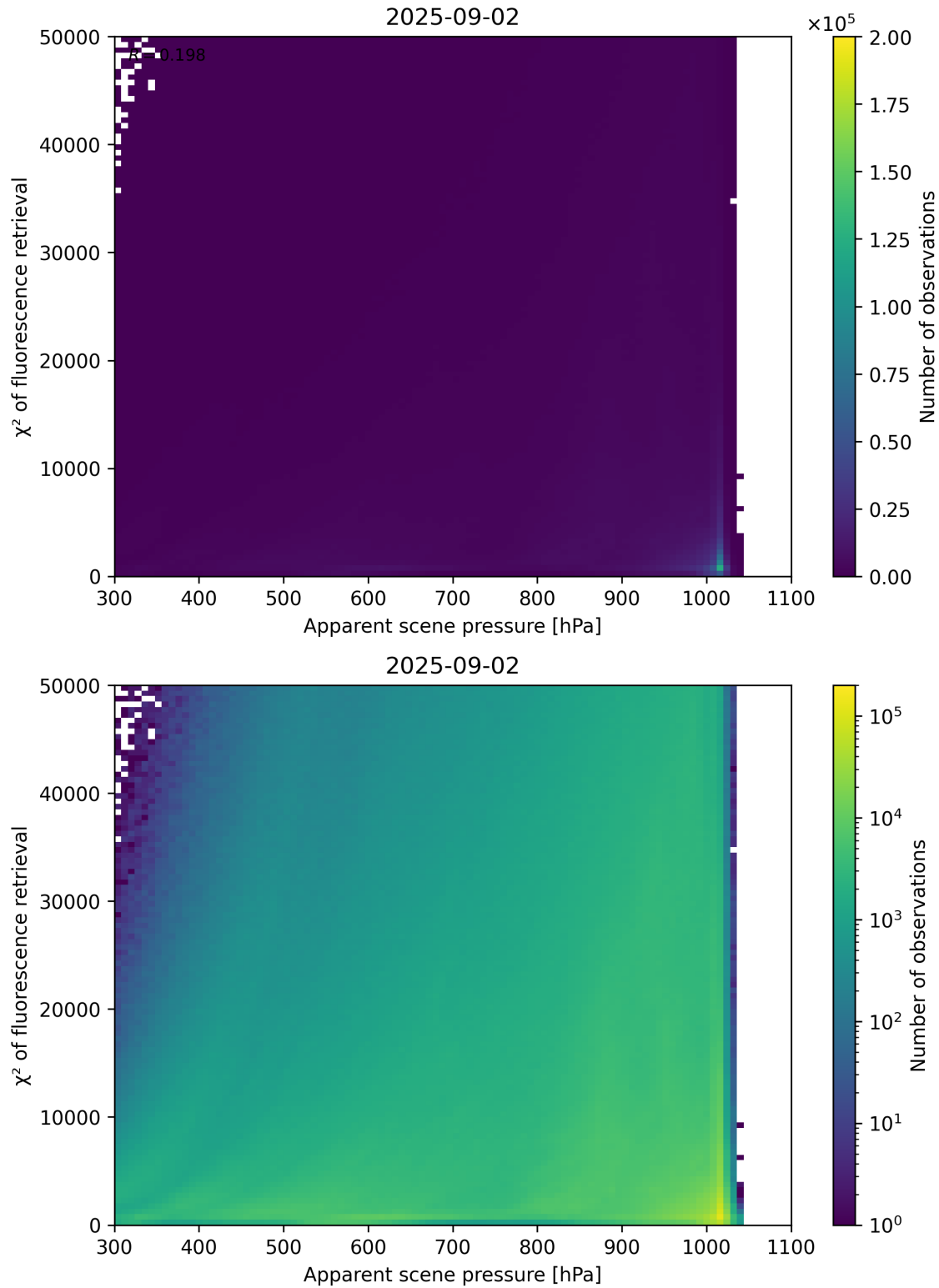
Figure 63: Scatter density plot of “Apparent scene pressure” against “ \chi^2 of fluorescence retrieval” for 2025-09-01 to 2025-09-03.
