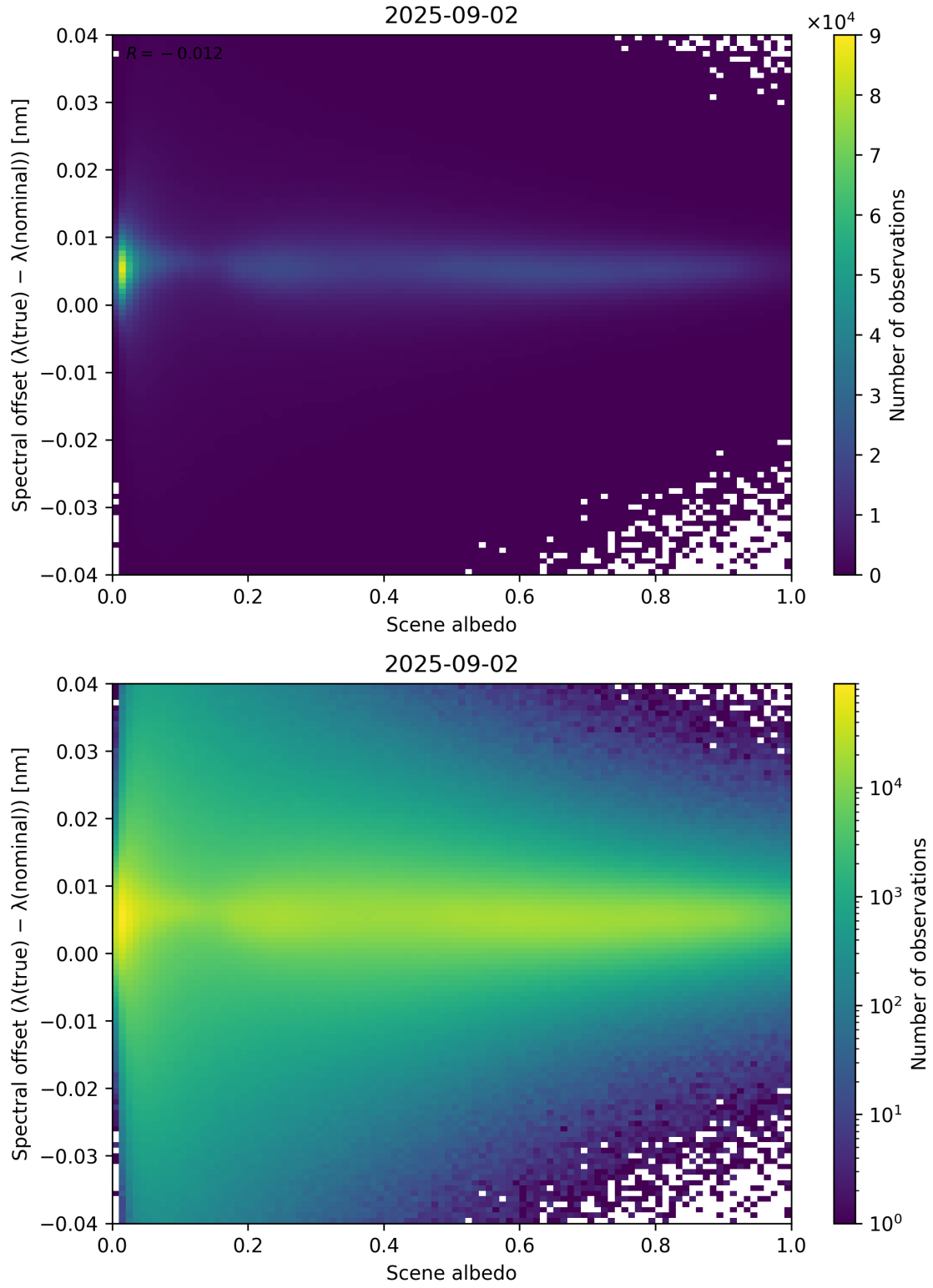
Figure 107: Scatter density plot of “Scene albedo” against “Spectral offset ( \lambda_{\text{true}} - \lambda_{\text{nominal}} )” for 2025-09-01 to 2025-09-03.
