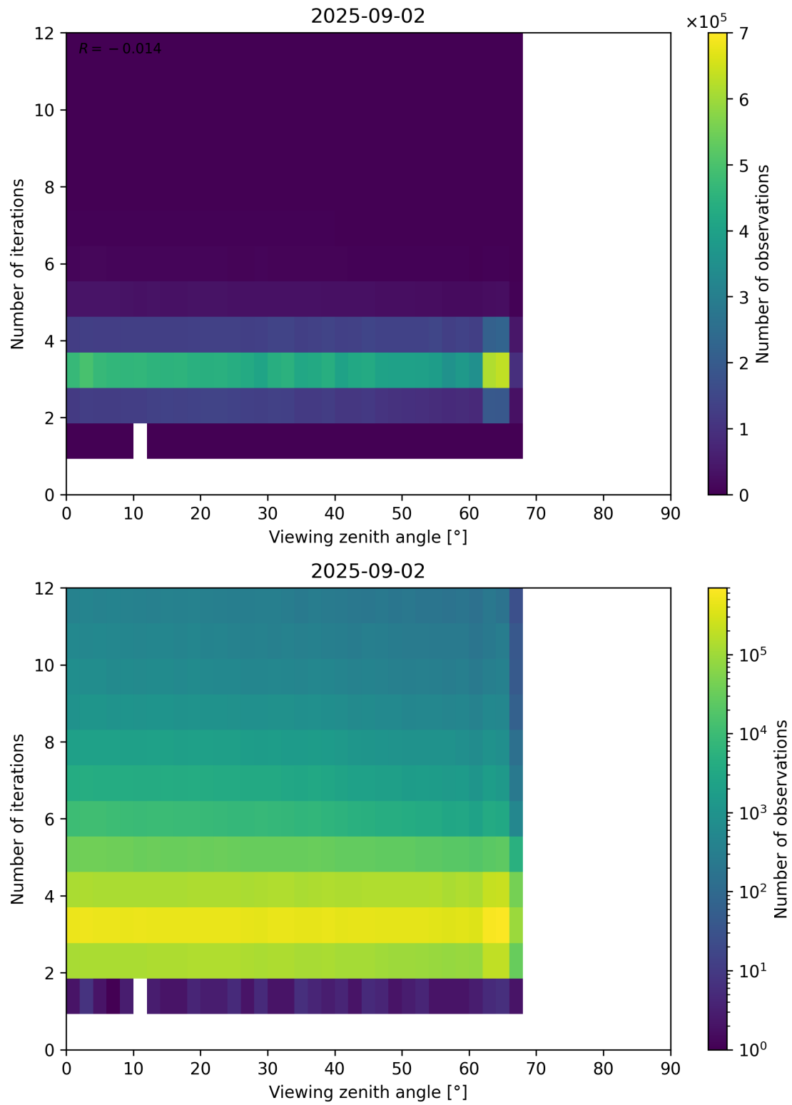
Figure 124: Scatter density plot of “Viewing zenith angle” against “Number of iterations” for 2025-09-01 to 2025-09-03.
