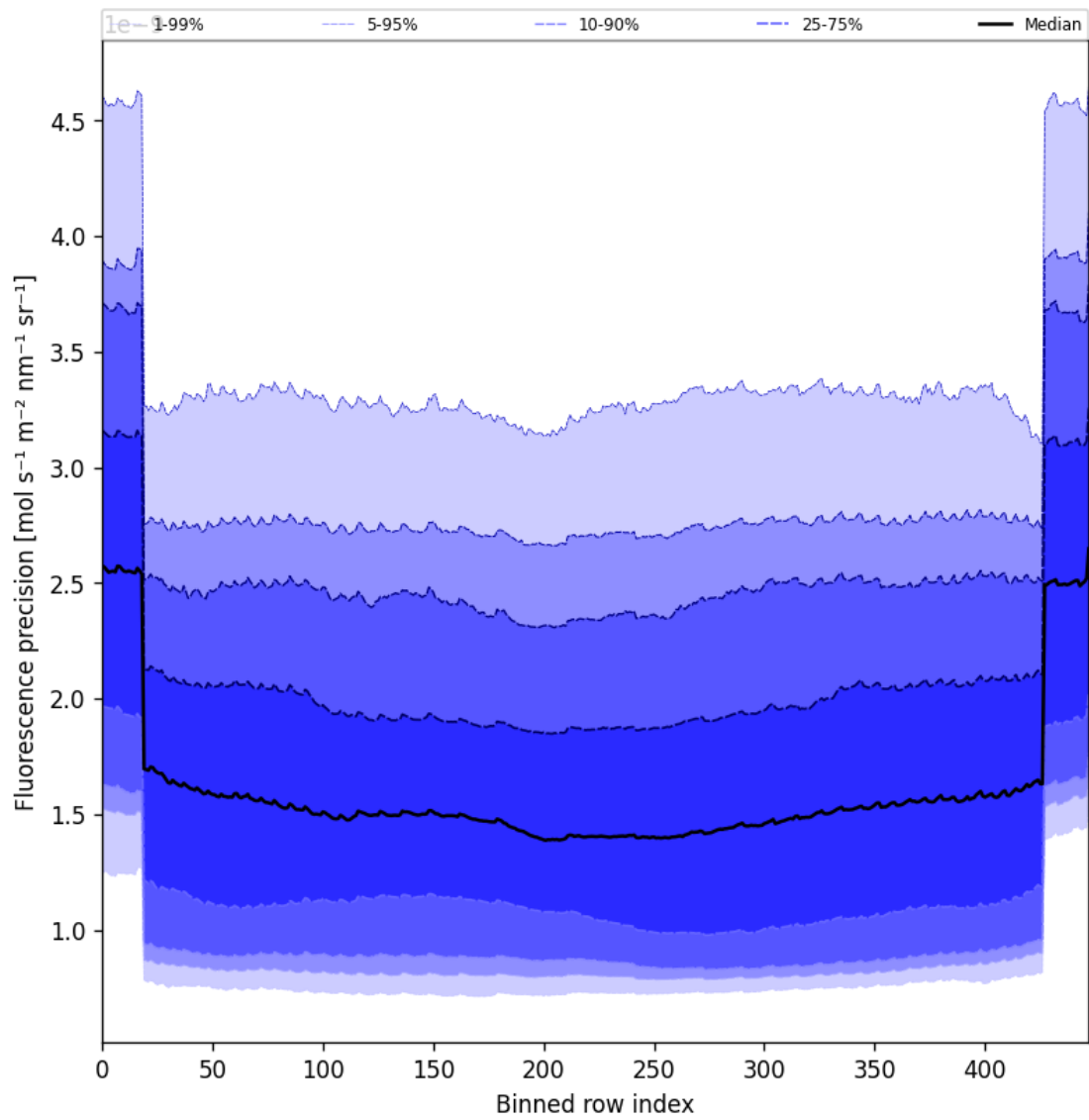
Figure 58: Along track statistics of “Fluorescence precision” for 2025-09-01 to 2025-09-03
