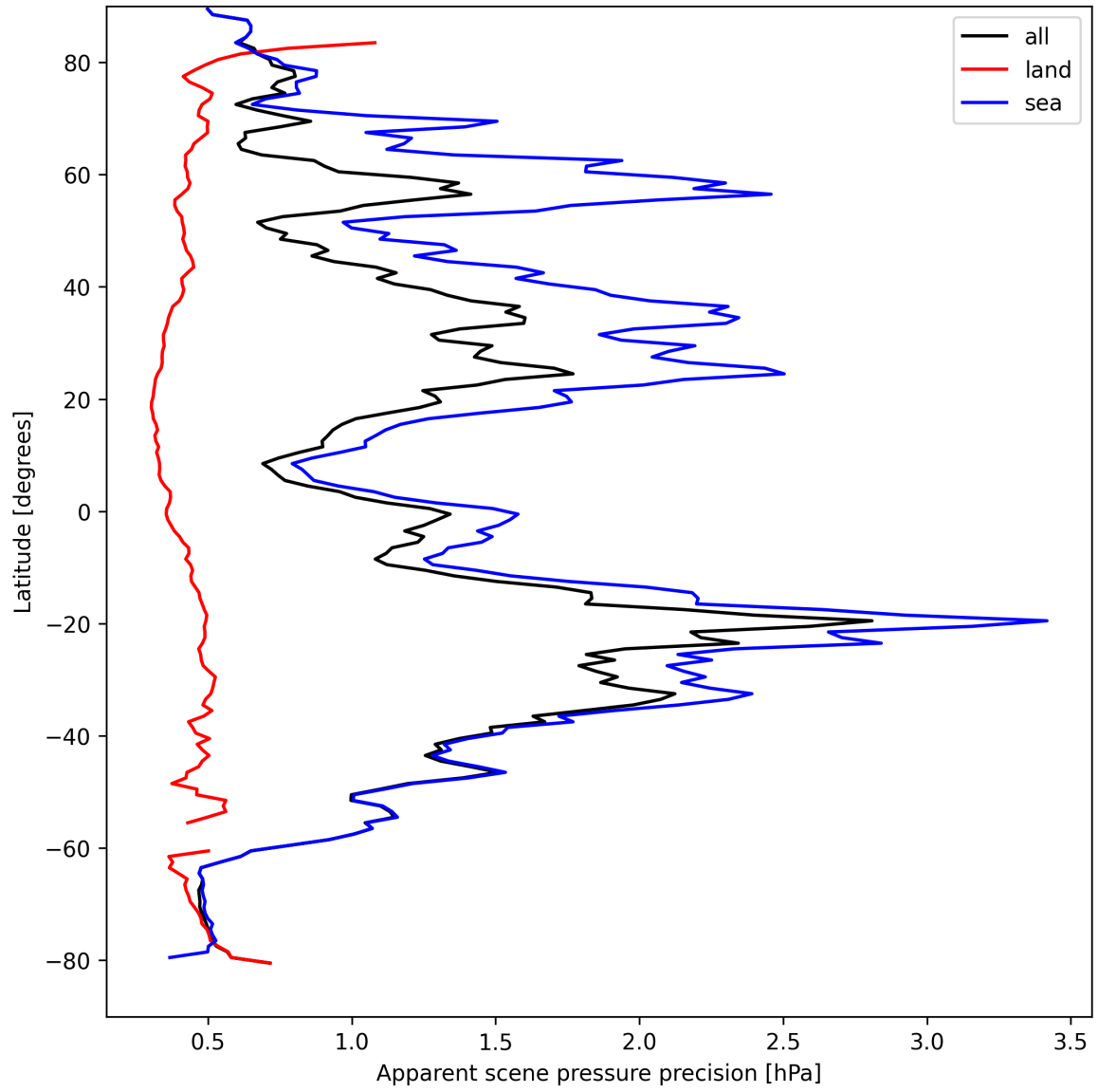
Figure 20: Zonal average of “Apparent scene pressure precision” for 2025-09-01 to 2025-09-03.
