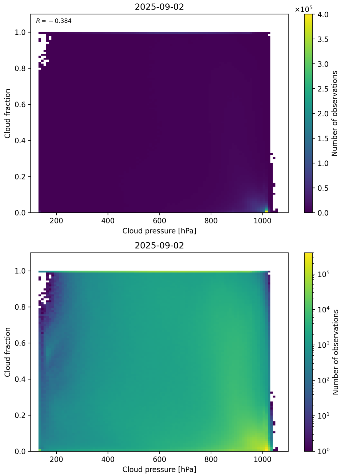
Figure 79: Scatter density plot of “Cloud pressure” against “Cloud fraction” for 2025-09-01 to 2025-09-03.
