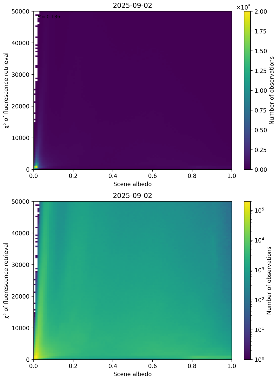
Figure 103: Scatter density plot of “Scene albedo” against “ \chi^2 of fluorescence retrieval” for 2025-09-01 to 2025-09-03.
