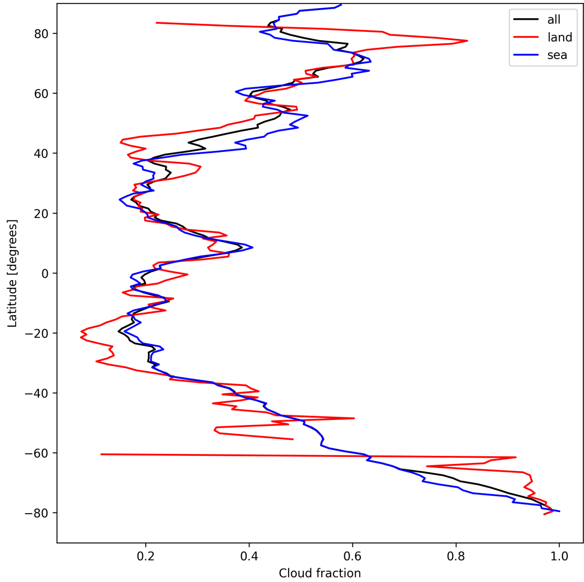
Figure 15: Zonal average of “Cloud fraction” for 2025-09-01 to 2025-09-03.
