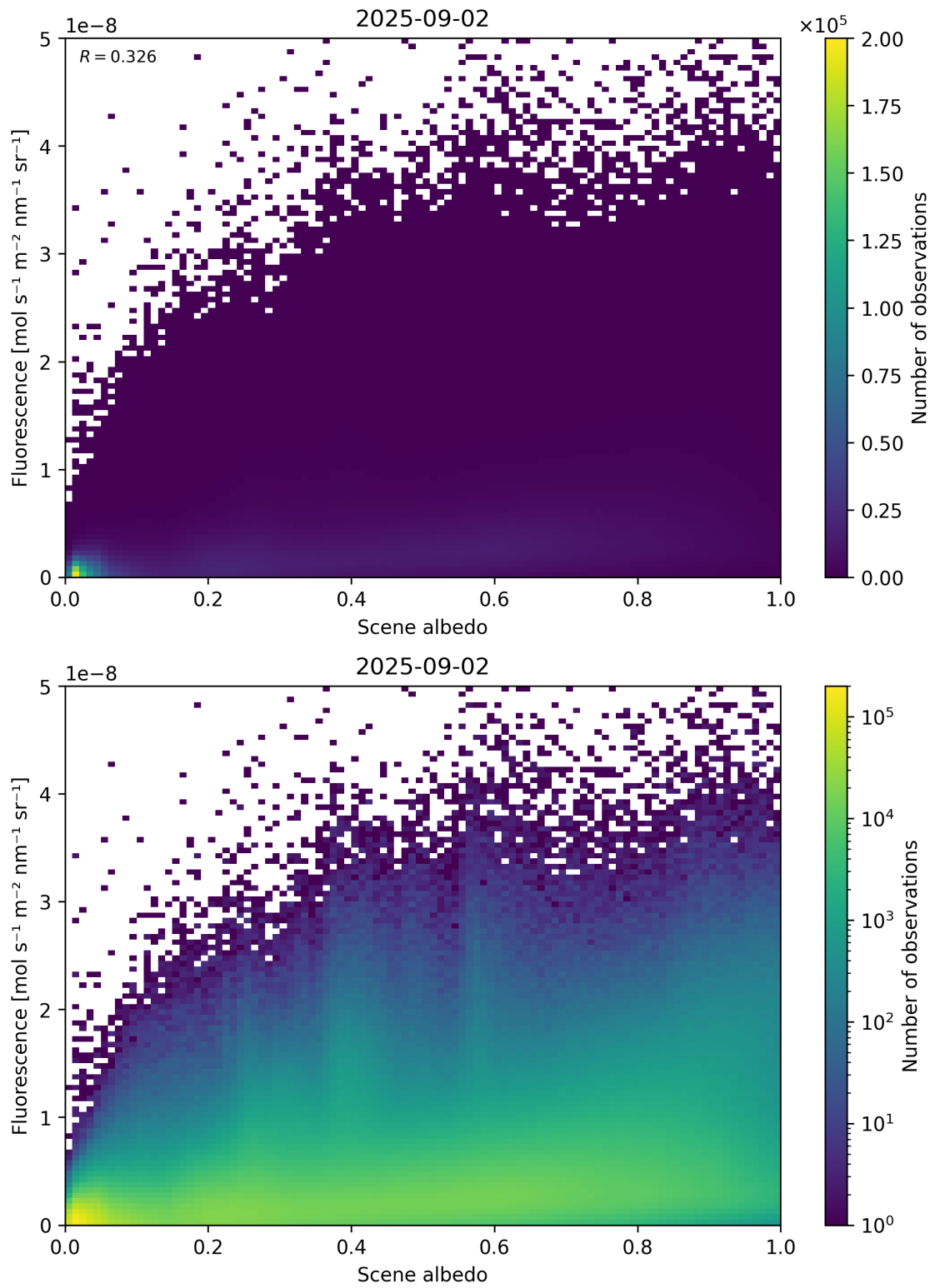
Figure 104: Scatter density plot of “Scene albedo” against “Fluorescence” for 2025-09-01 to 2025-09-03.
