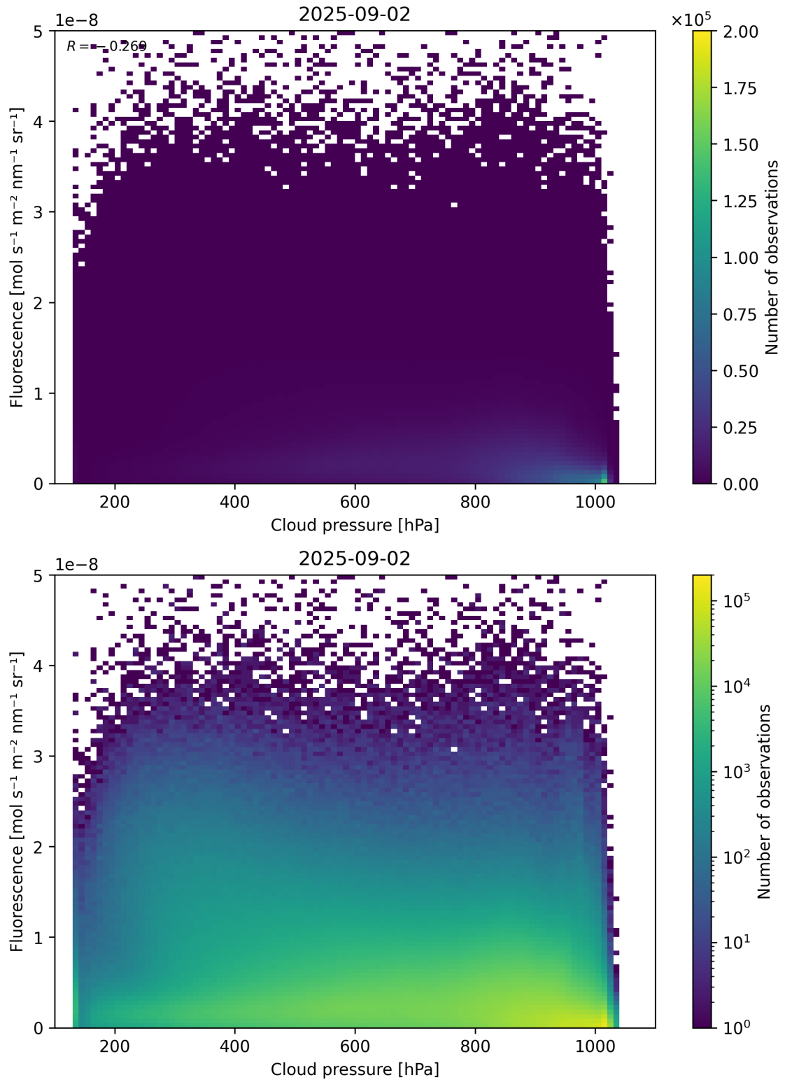
Figure 80: Scatter density plot of “Cloud pressure” against “Fluorescence” for 2025-09-01 to 2025-09-03.
