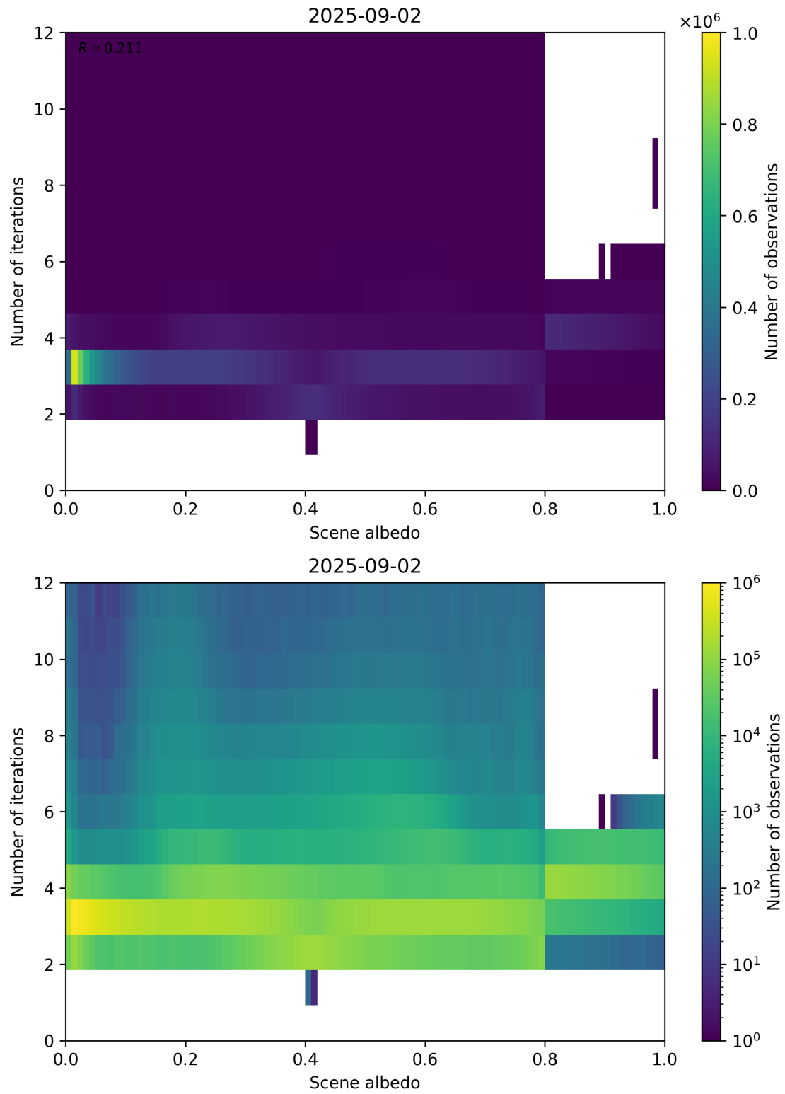
Figure 105: Scatter density plot of “Scene albedo” against “Number of iterations” for 2025-09-01 to 2025-09-03.
