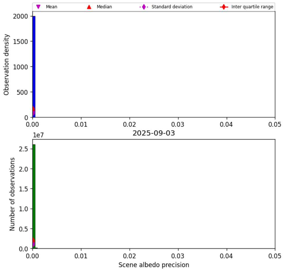
Figure 35: Histogram of “Scene albedo precision” for 2025-09-02 to 2025-09-04
