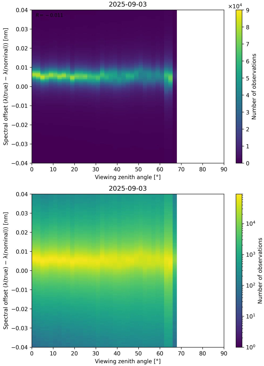
Figure 128: Scatter density plot of “Viewing zenith angle” against “Spectral offset ( \lambda_{\text{true}} - \lambda_{\text{nominal}} )” for 2025-09-02 to 2025-09-04.
