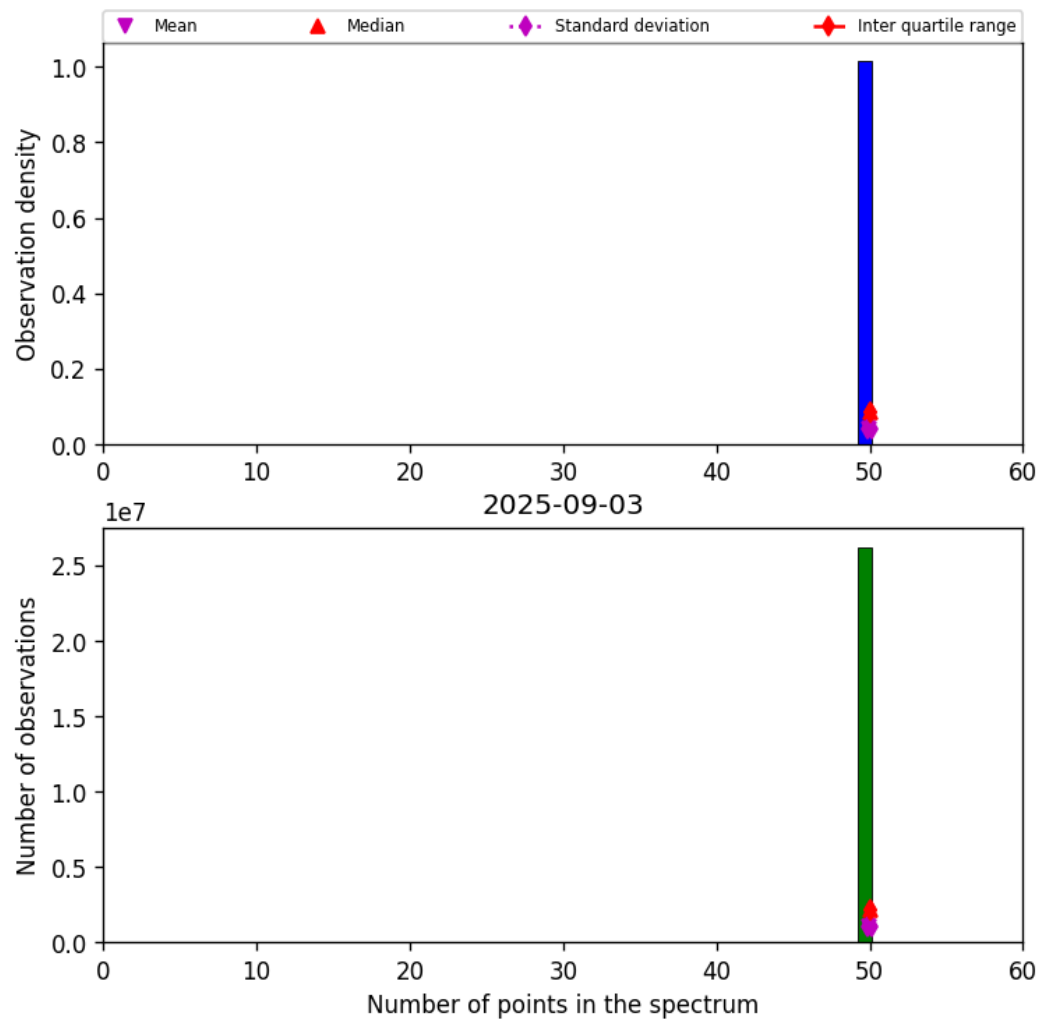
Figure 44: Histogram of “Number of points in the spectrum” for 2025-09-02 to 2025-09-04
