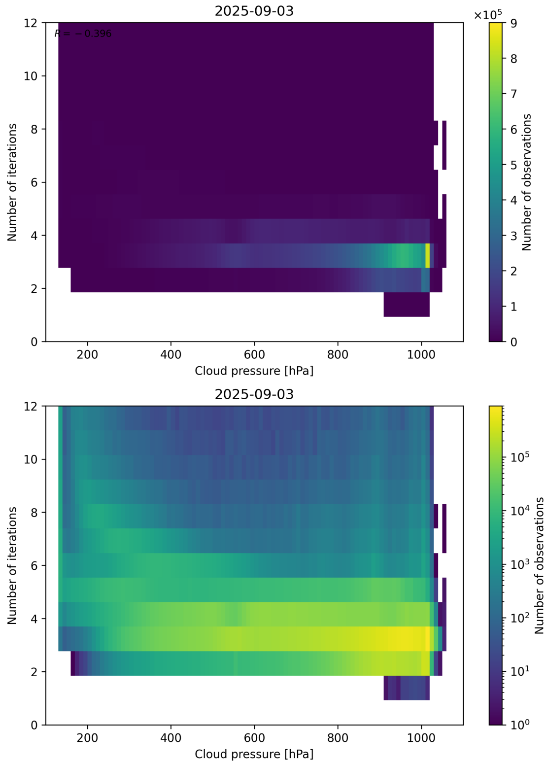
Figure 81: Scatter density plot of “Cloud pressure” against “Number of iterations” for 2025-09-02 to 2025-09-04.
