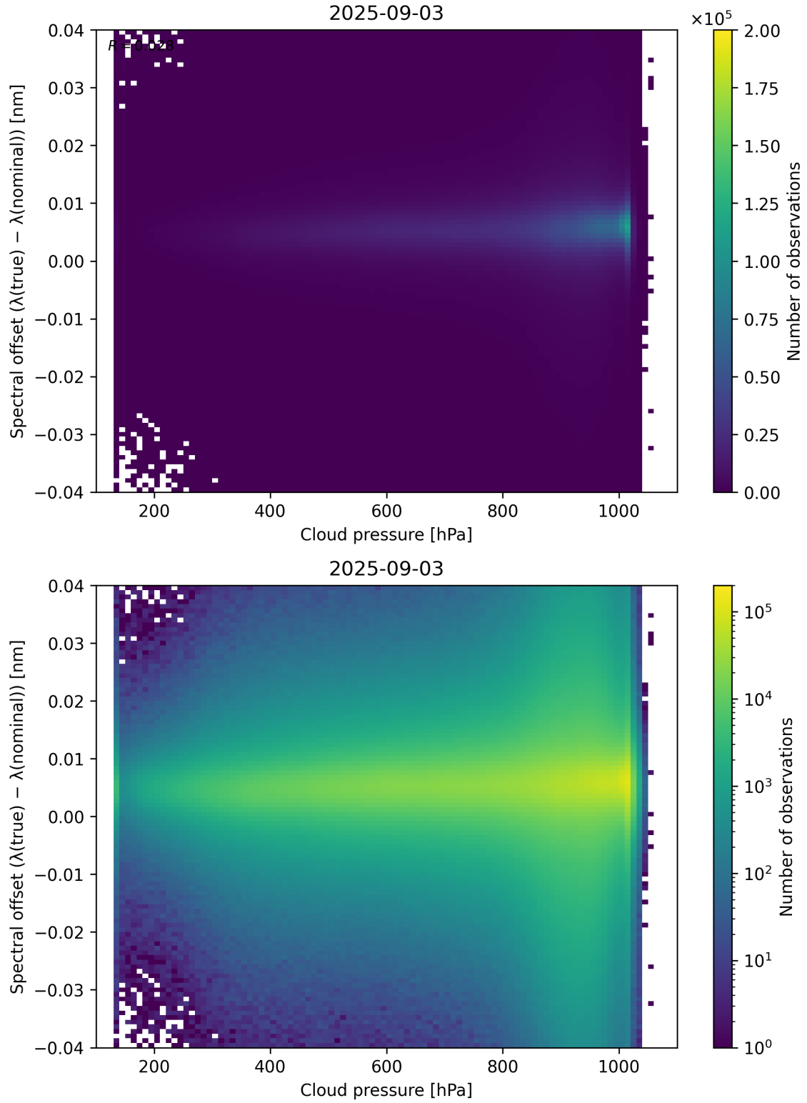
Figure 84: Scatter density plot of “Cloud pressure” against “Spectral offset ( \lambda_{\text{true}} - \lambda_{\text{nominal}} )” for 2025-09-02 to 2025-09-04.
