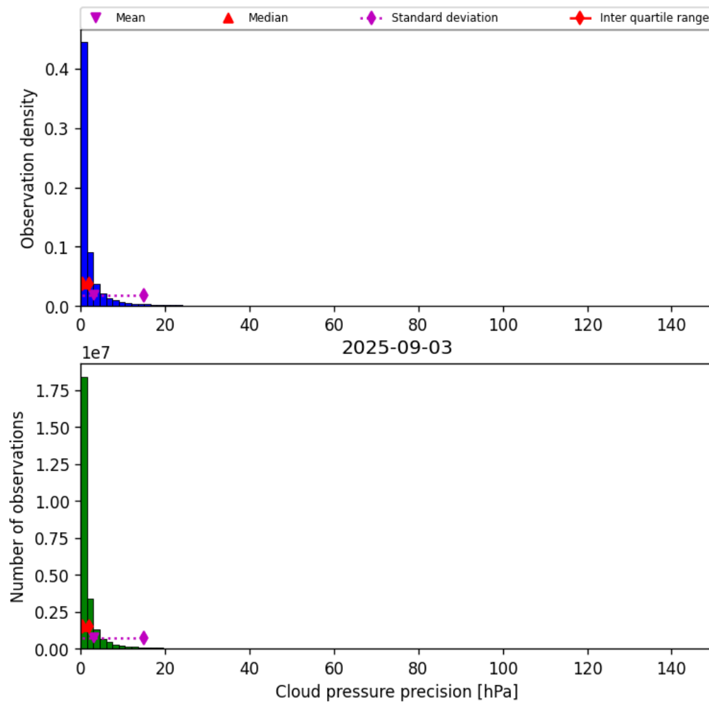
Figure 31: Histogram of “Cloud pressure precision” for 2025-09-02 to 2025-09-04
