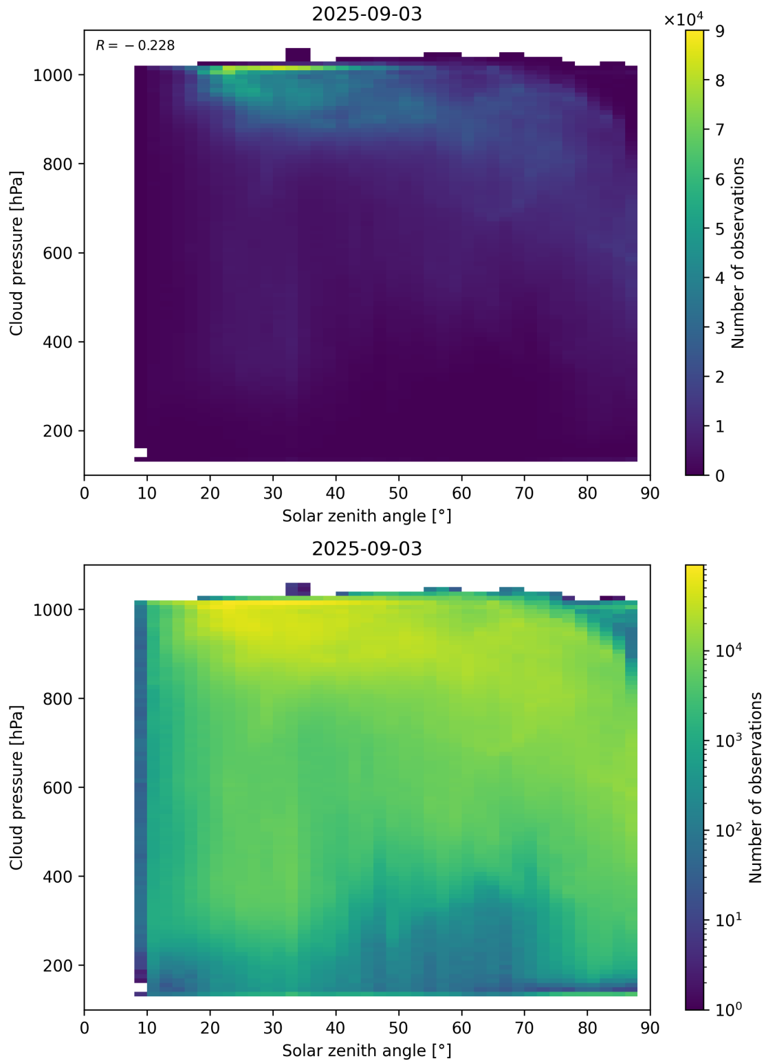
Figure 111: Scatter density plot of “Solar zenith angle” against “Cloud pressure” for 2025-09-02 to 2025-09-04.
