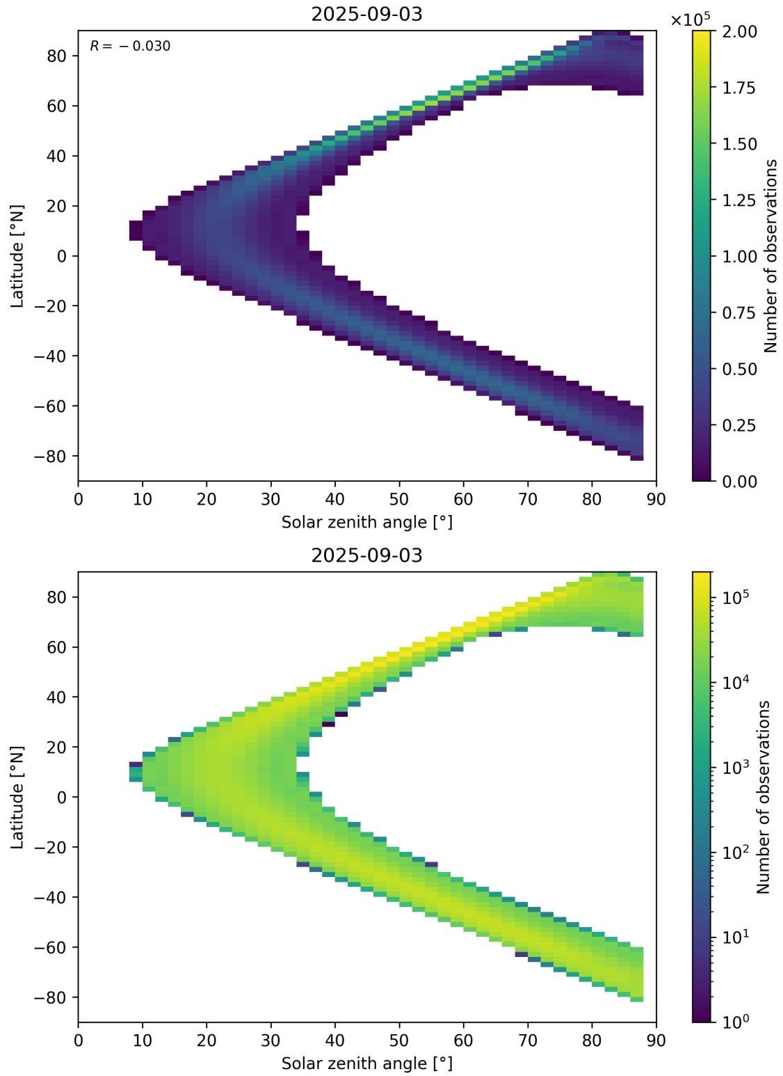
Figure 113: Scatter density plot of “Solar zenith angle” against “Latitude” for 2025-09-02 to 2025-09-04.
