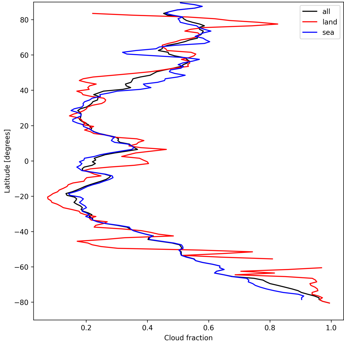
Figure 15: Zonal average of “Cloud fraction” for 2025-09-02 to 2025-09-04.
