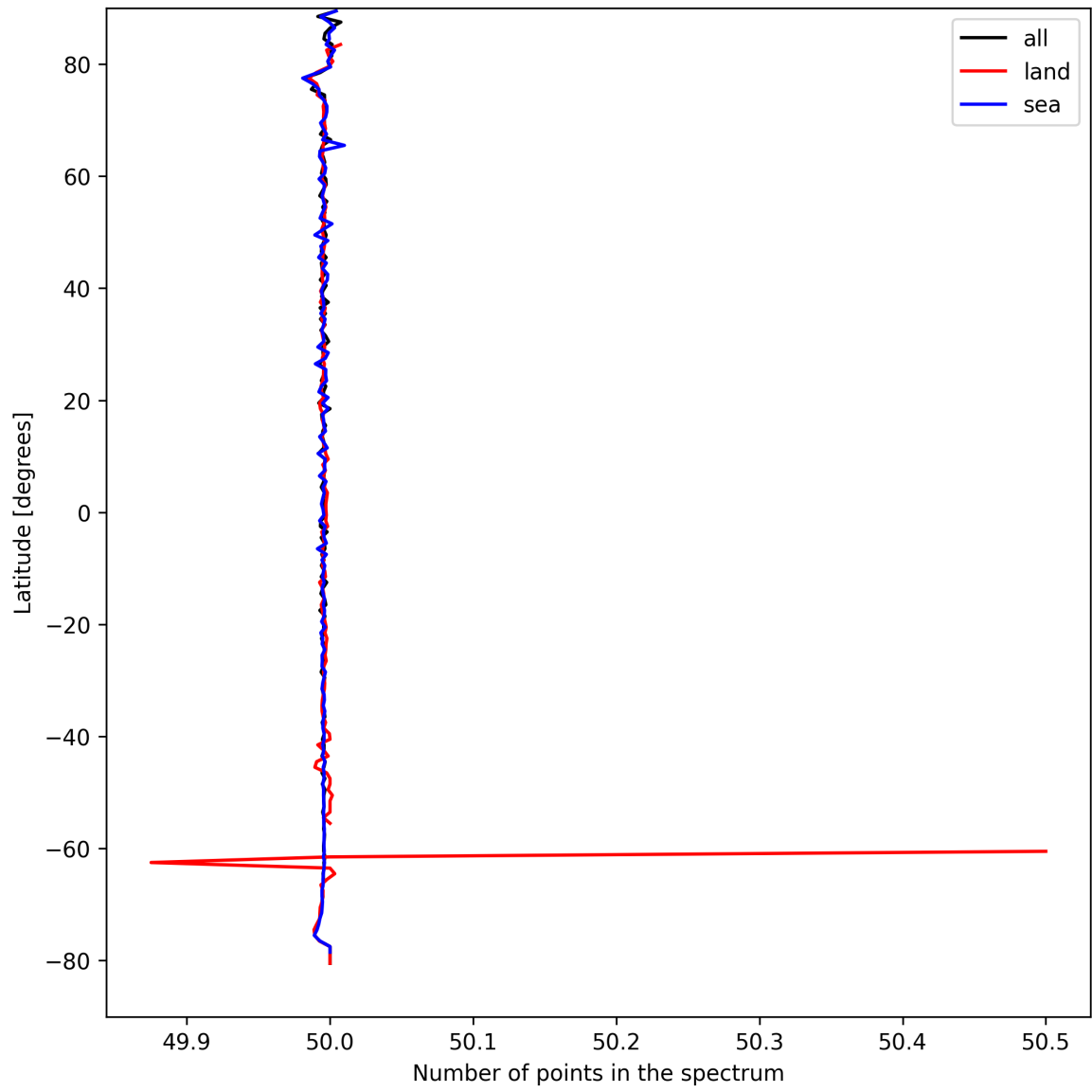
Figure 27: Zonal average of “Number of points in the spectrum” for 2025-09-02 to 2025-09-04.
