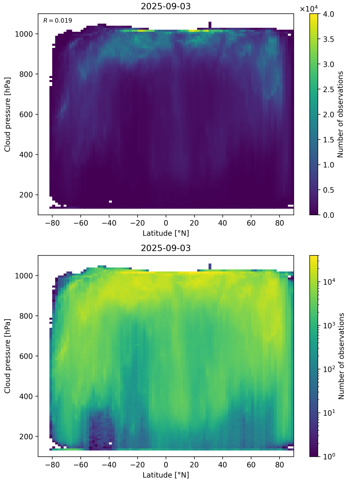
Figure 91: Scatter density plot of “Latitude” against “Cloud pressure” for 2025-09-02 to 2025-09-04.
