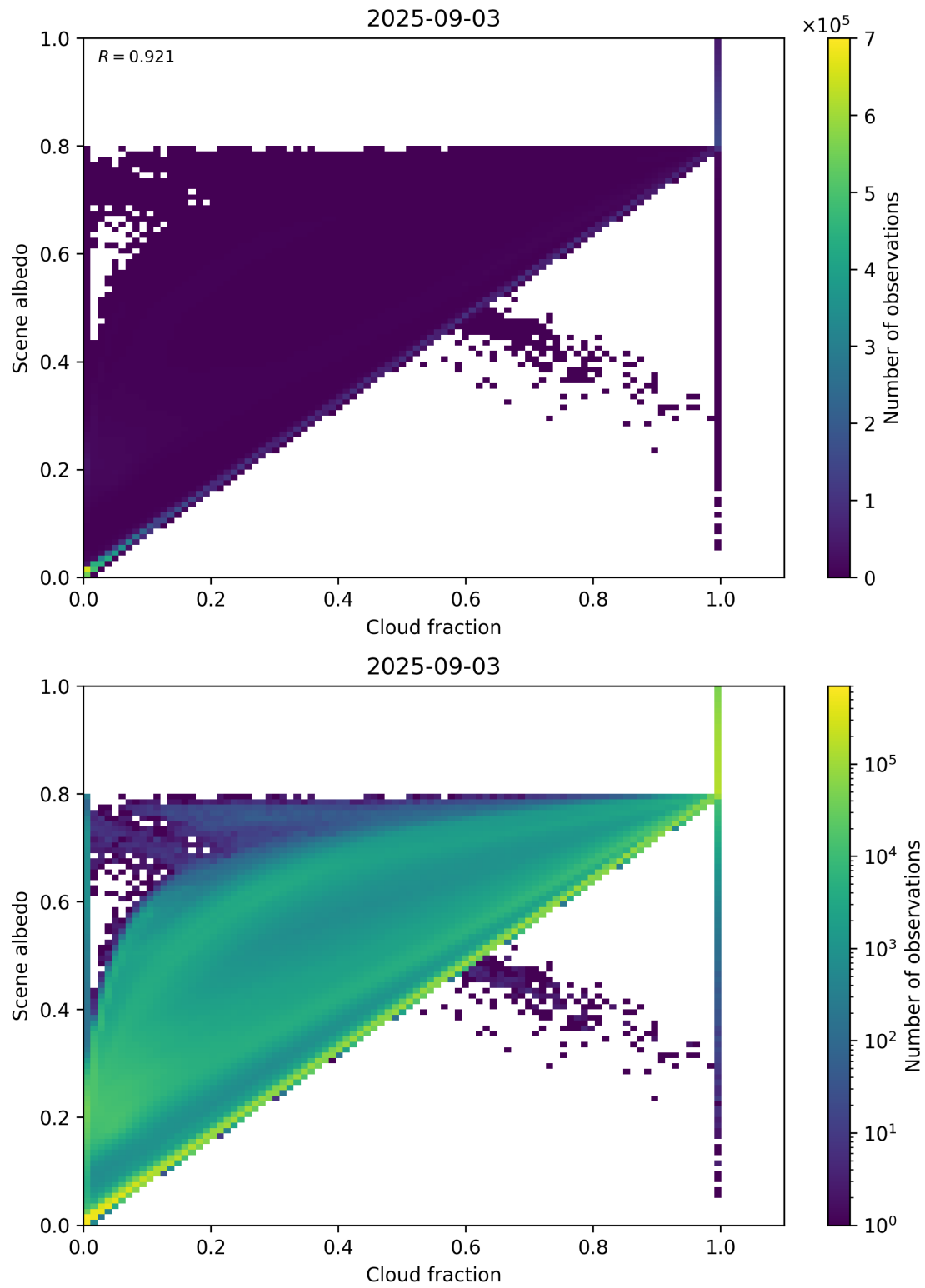
Figure 75: Scatter density plot of “Cloud fraction” against “Scene albedo” for 2025-09-02 to 2025-09-04.
