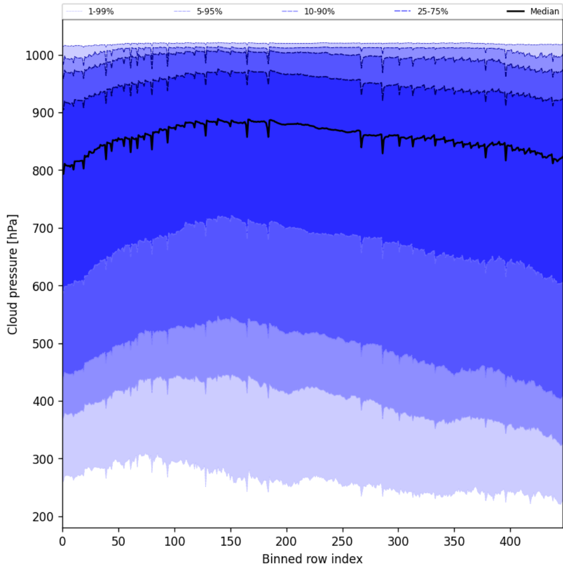
Figure 47: Along track statistics of “Cloud pressure” for 2025-09-02 to 2025-09-04
