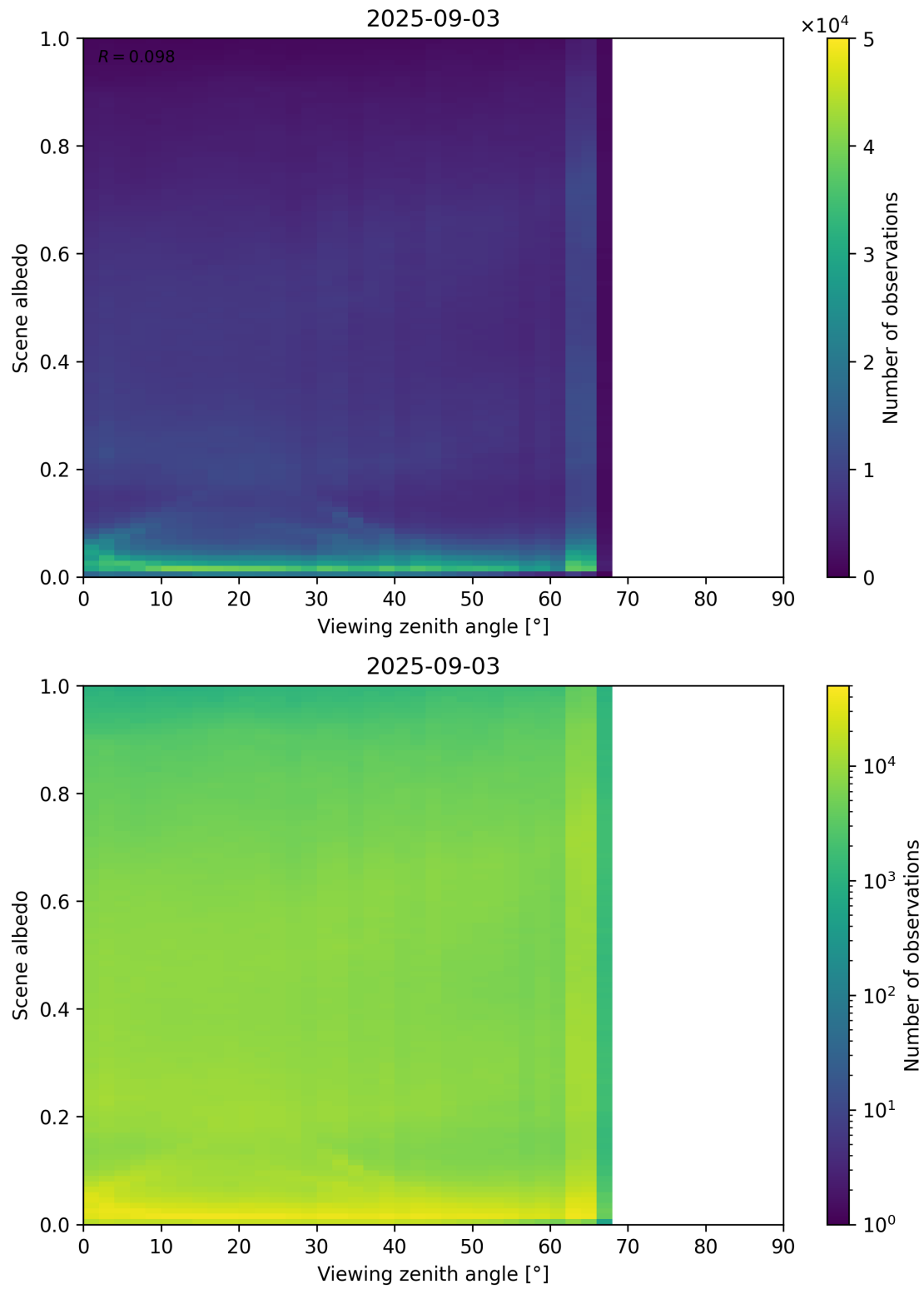
Figure 126: Scatter density plot of “Viewing zenith angle” against “Scene albedo” for 2025-09-02 to 2025-09-04.
