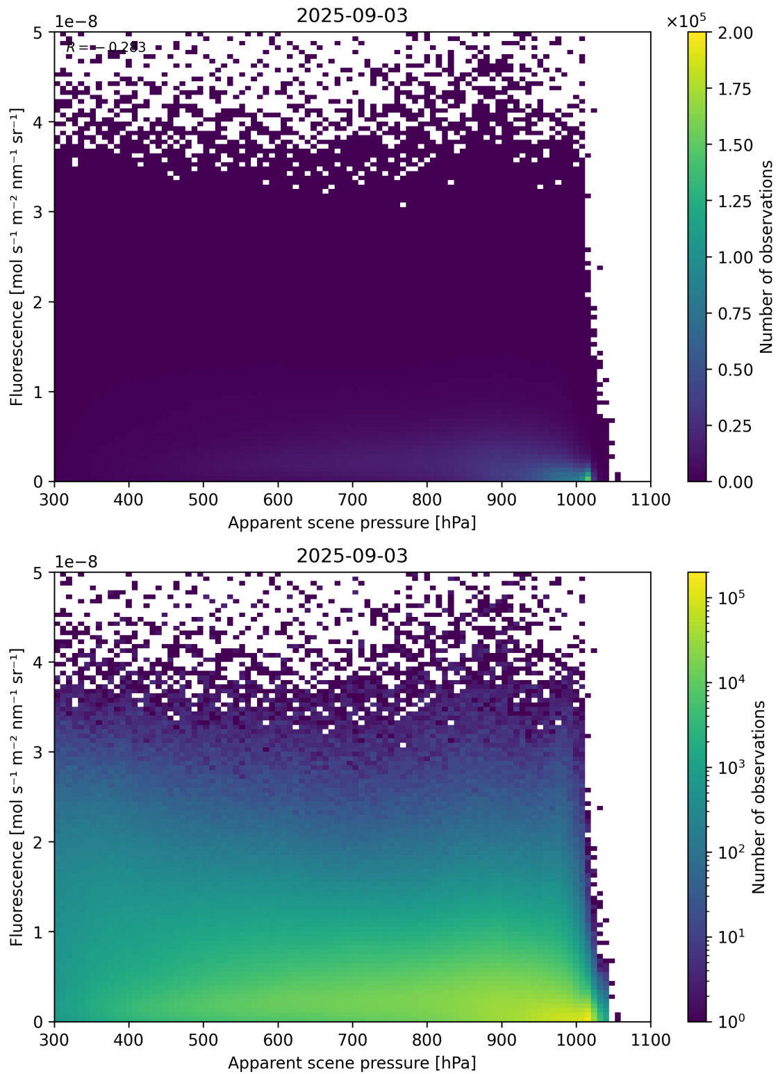
Figure 64: Scatter density plot of “Apparent scene pressure” against “Fluorescence” for 2025-09-02 to 2025-09-04.
