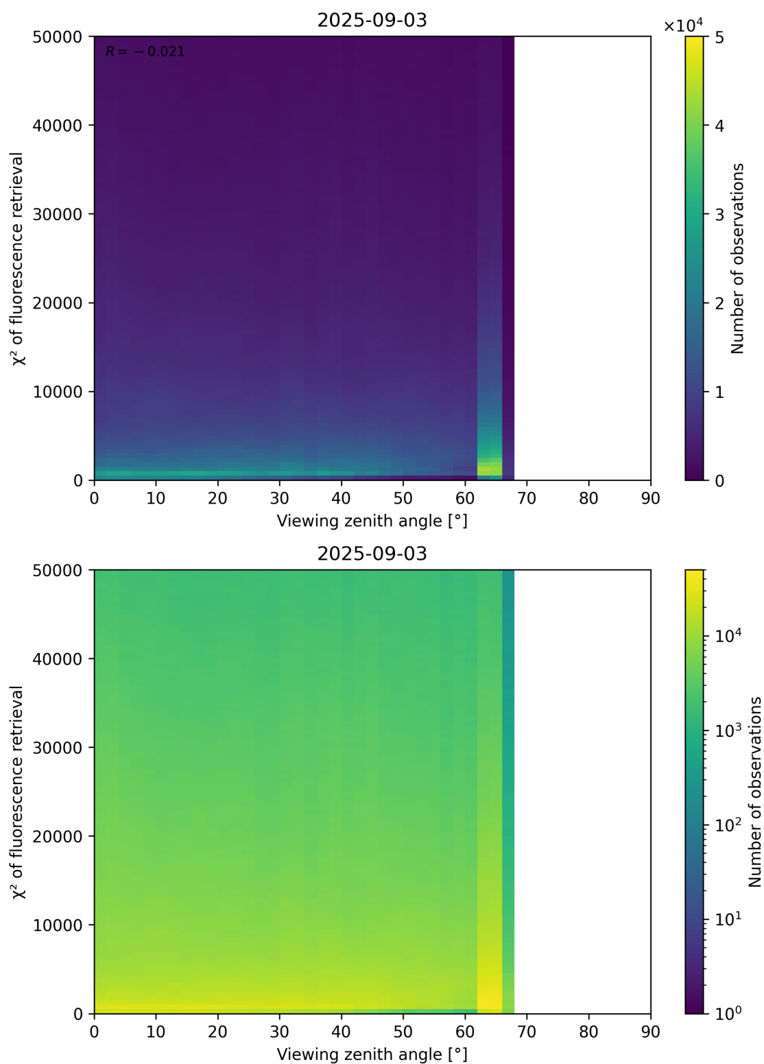
Figure 119: Scatter density plot of “Viewing zenith angle” against “ \chi^2 of fluorescence retrieval” for 2025-09-02 to 2025-09-04.
