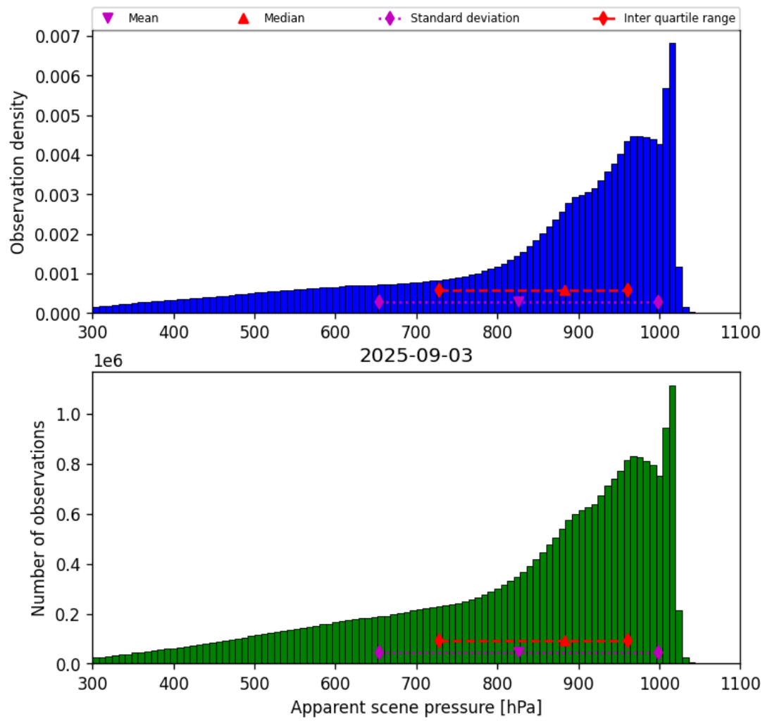
Figure 36: Histogram of “Apparent scene pressure” for 2025-09-02 to 2025-09-04
