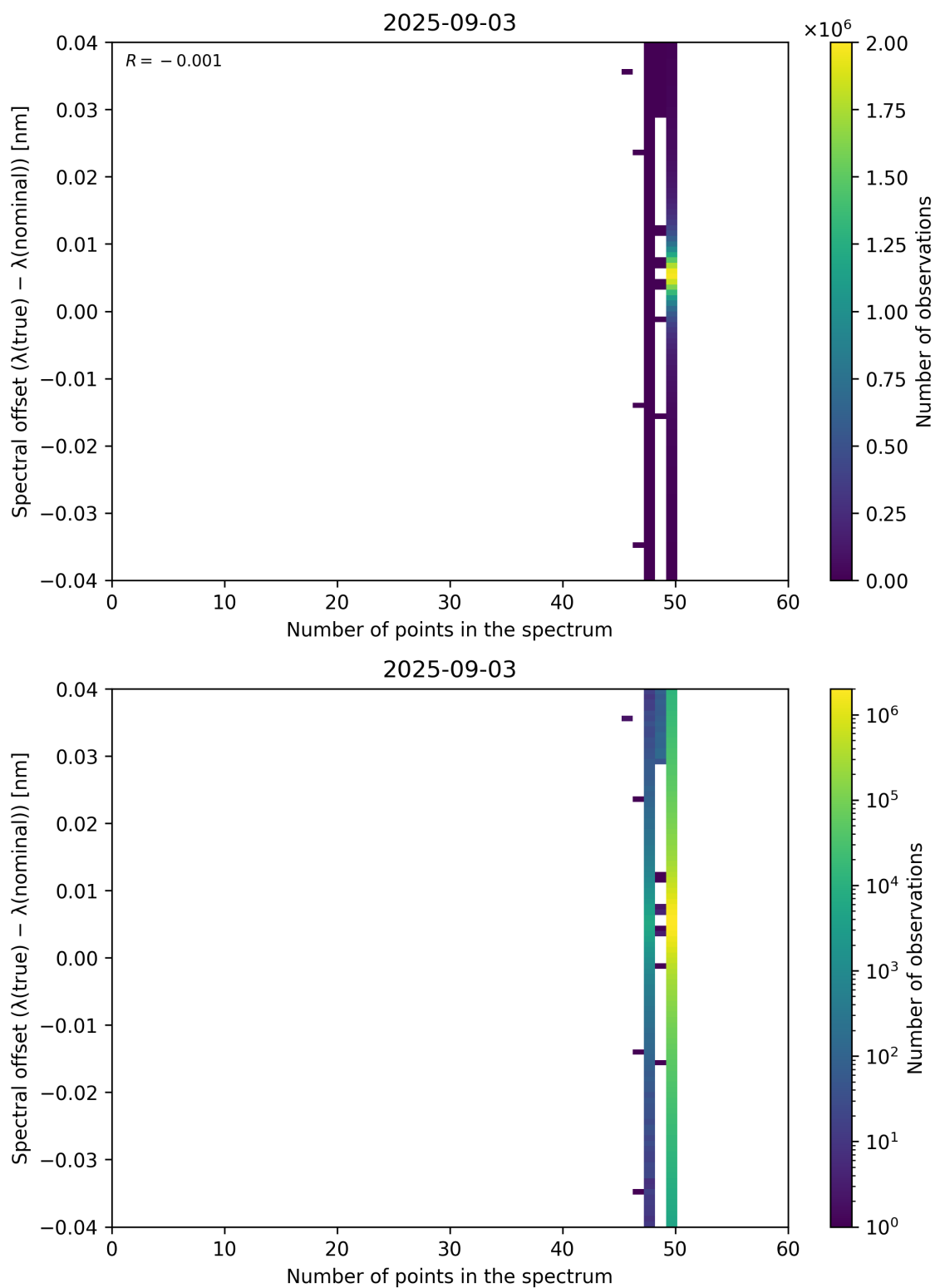
Figure 101: Scatter density plot of “Number of points in the spectrum” against “Spectral offset ( \lambda_{\text{true}} - \lambda_{\text{nominal}} )” for 2025-09-02 to 2025-09-04.
