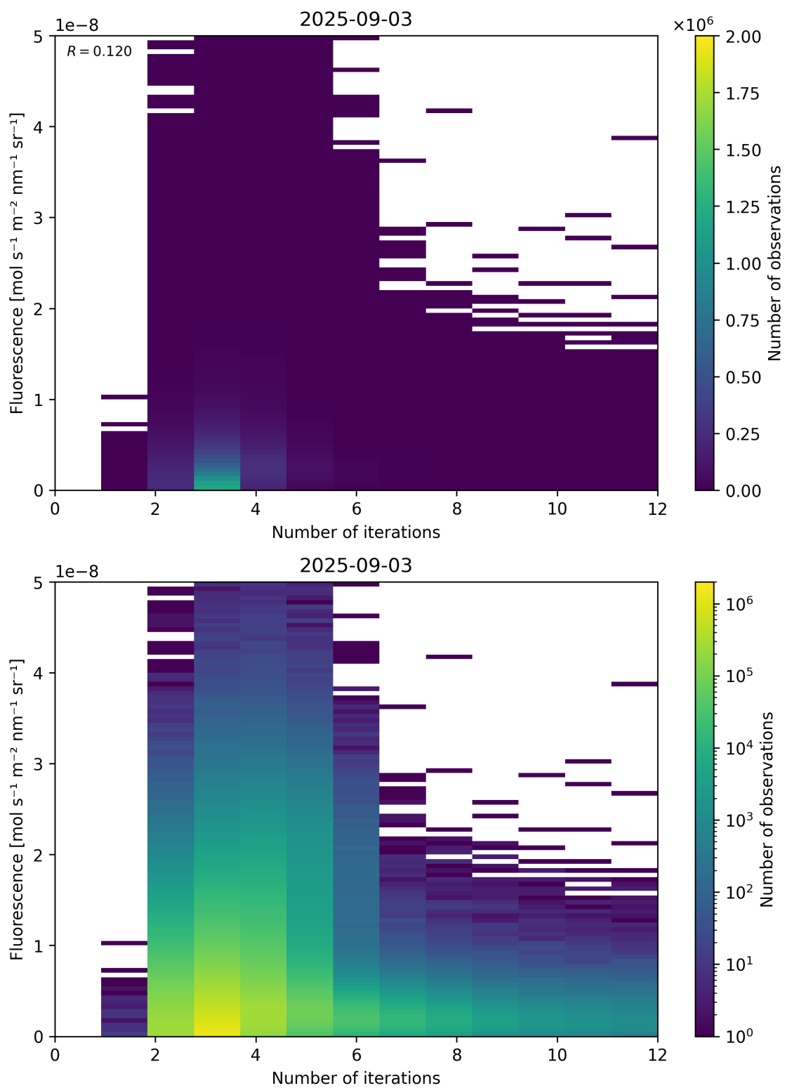
Figure 98: Scatter density plot of “Number of iterations” against “Fluorescence” for 2025-09-02 to 2025-09-04.
