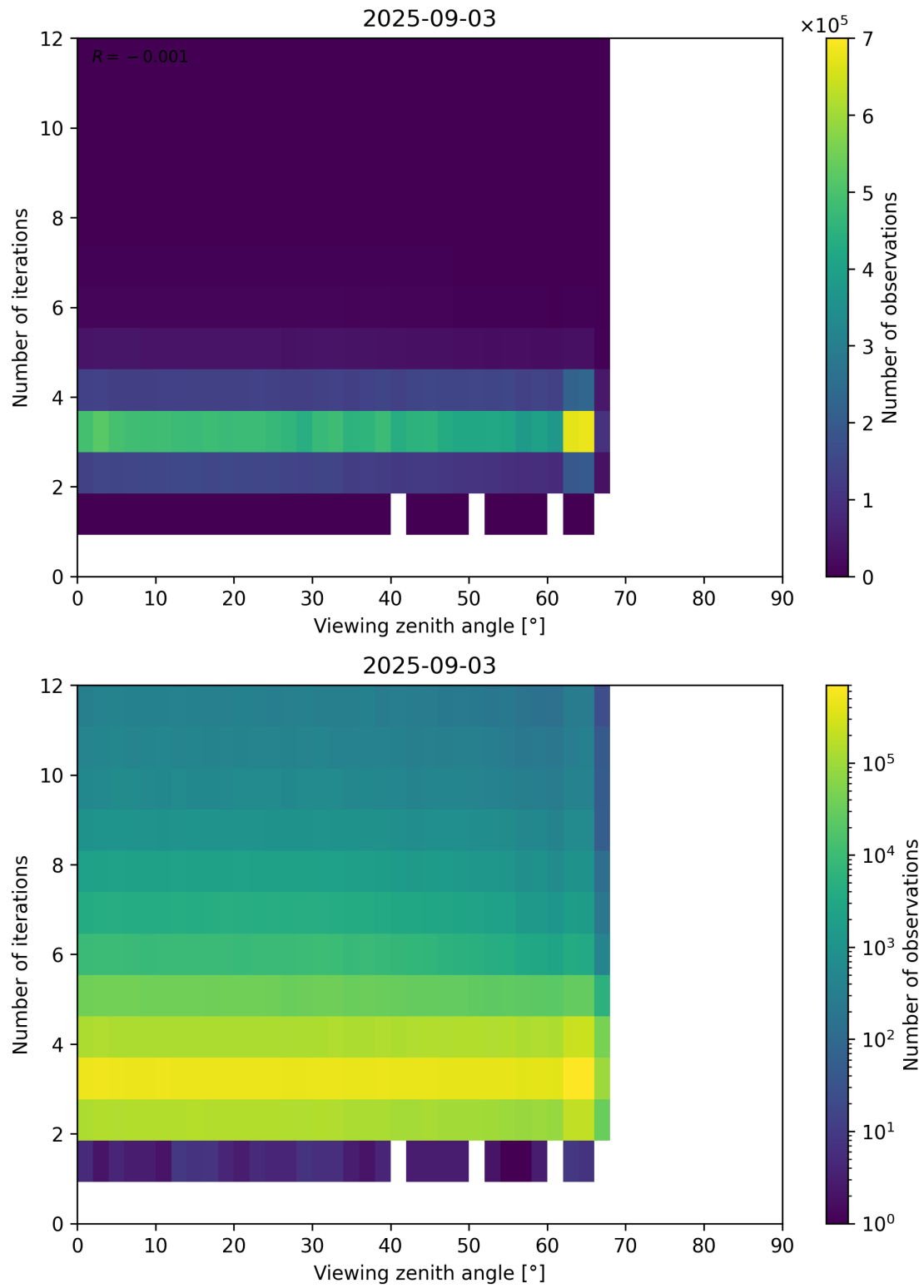
Figure 124: Scatter density plot of “Viewing zenith angle” against “Number of iterations” for 2025-09-02 to 2025-09-04.
