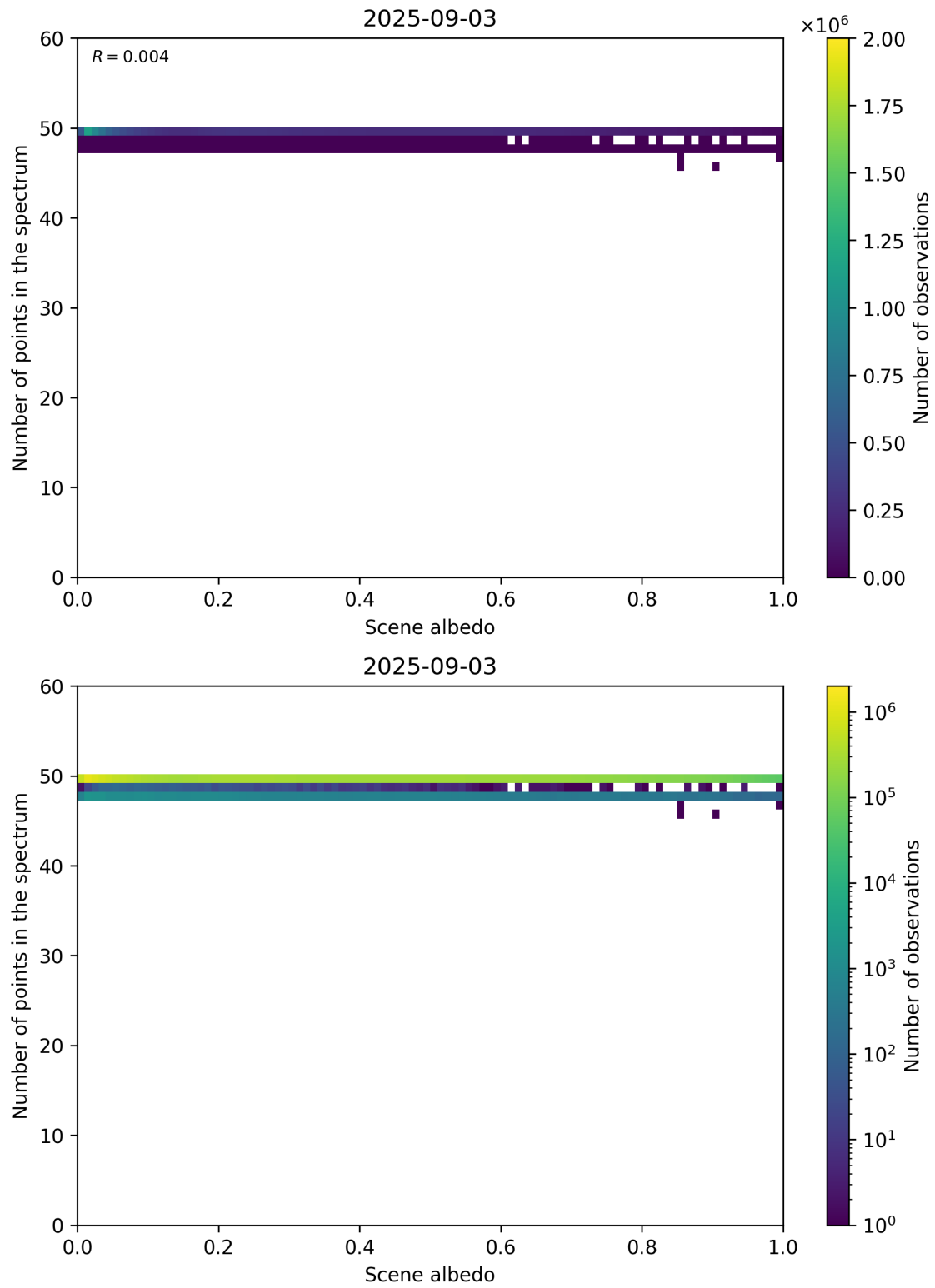
Figure 106: Scatter density plot of “Scene albedo” against “Number of points in the spectrum” for 2025-09-02 to 2025-09-04.
