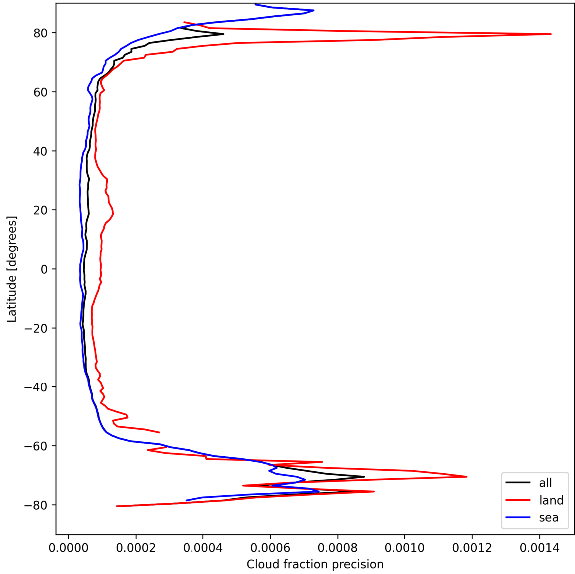
Figure 16: Zonal average of “Cloud fraction precision” for 2025-09-02 to 2025-09-04.
