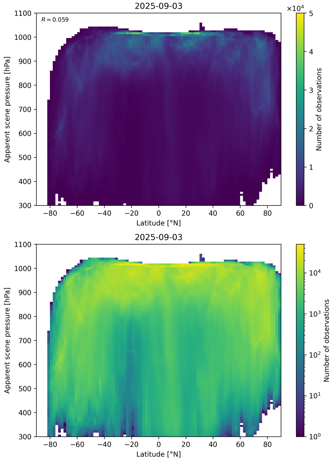
Figure 88: Scatter density plot of “Latitude” against “Apparent scene pressure” for 2025-09-02 to 2025-09-04.
