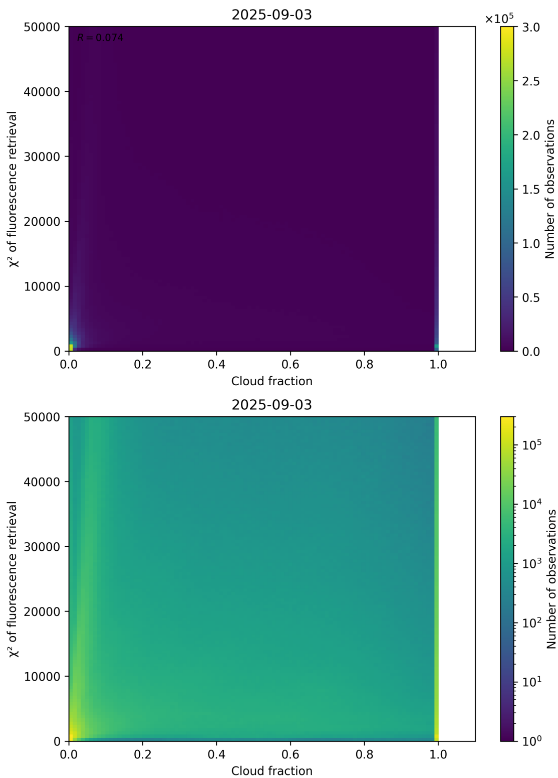
Figure 71: Scatter density plot of “Cloud fraction” against “ \chi^2 of fluorescence retrieval” for 2025-09-02 to 2025-09-04.
