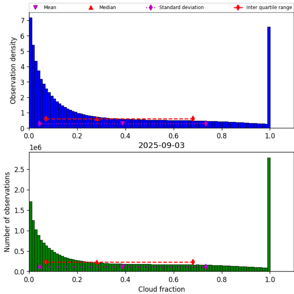
Figure 32: Histogram of “Cloud fraction” for 2025-09-02 to 2025-09-04
