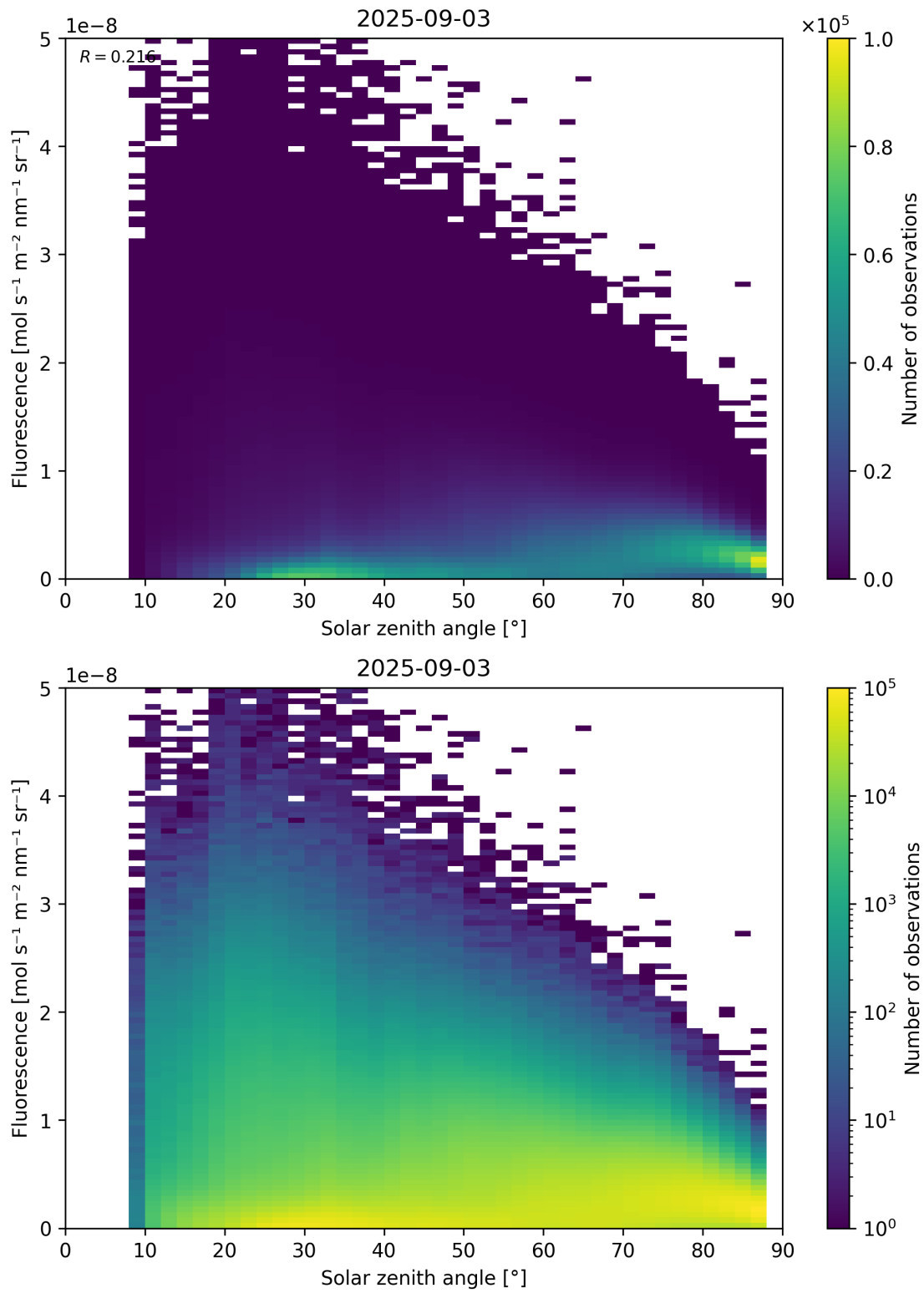
Figure 112: Scatter density plot of “Solar zenith angle” against “Fluorescence” for 2025-09-02 to 2025-09-04.
