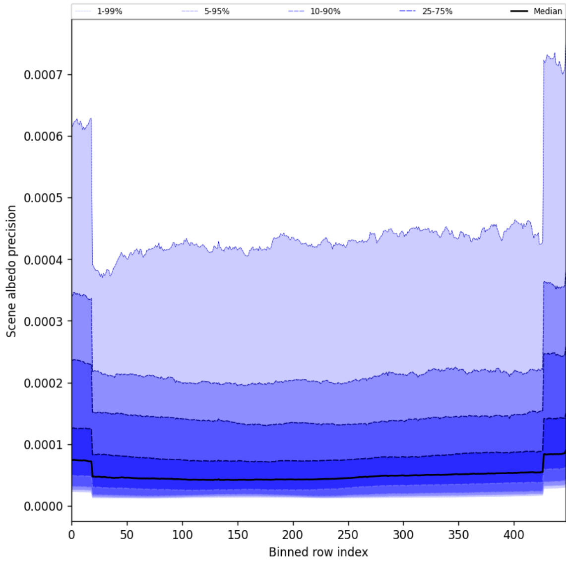
Figure 52: Along track statistics of “Scene albedo precision” for 2025-09-02 to 2025-09-04
