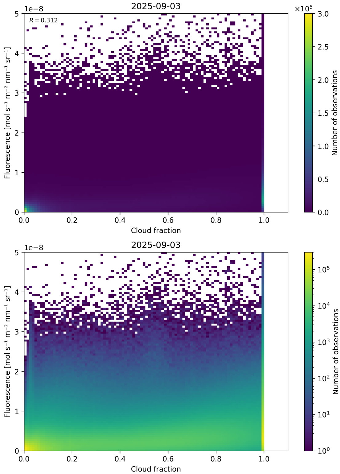
Figure 72: Scatter density plot of “Cloud fraction” against “Fluorescence” for 2025-09-02 to 2025-09-04.
