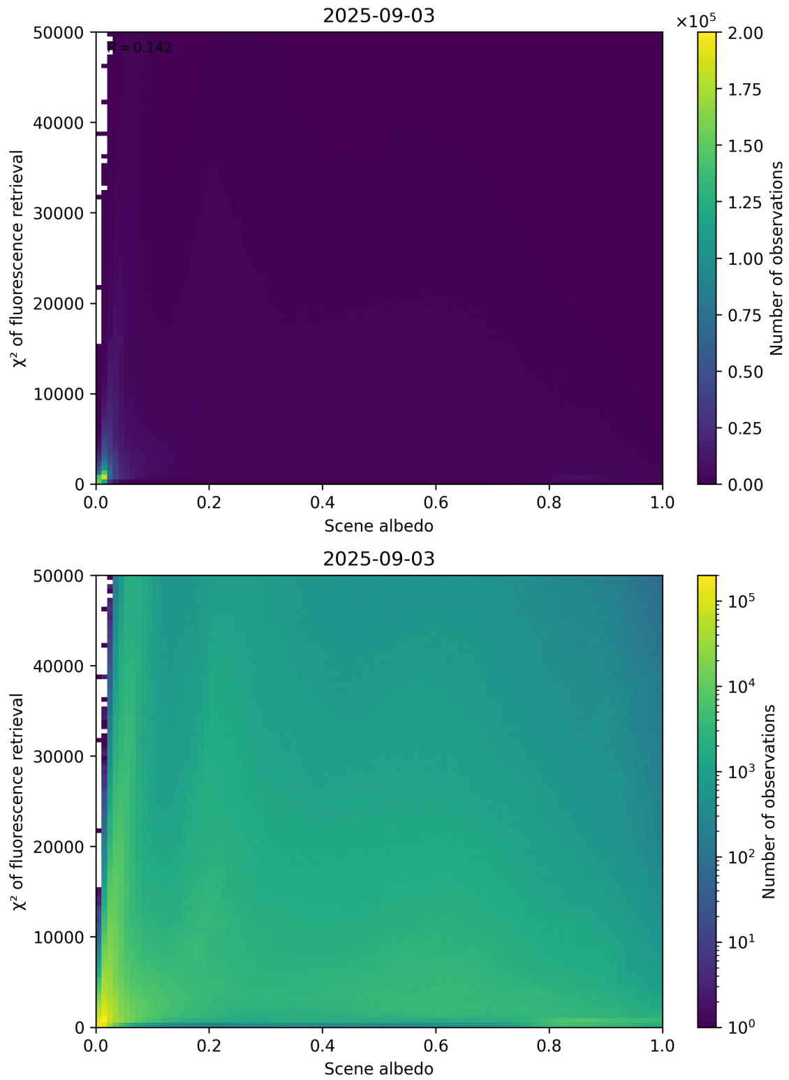
Figure 103: Scatter density plot of “Scene albedo” against “ \chi^2 of fluorescence retrieval” for 2025-09-02 to 2025-09-04.
