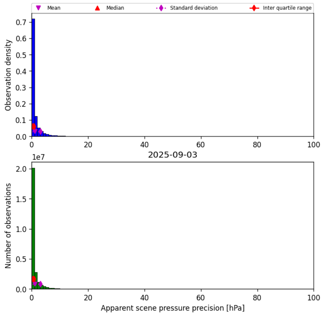
Figure 37: Histogram of “Apparent scene pressure precision” for 2025-09-02 to 2025-09-04
