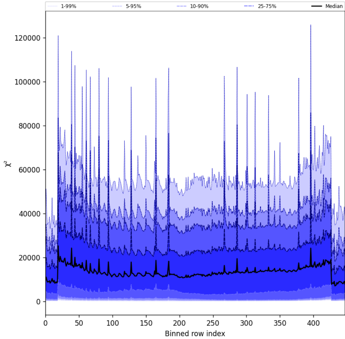
Figure 55: Along track statistics of " \chi^2 " for 2025-09-02 to 2025-09-04
