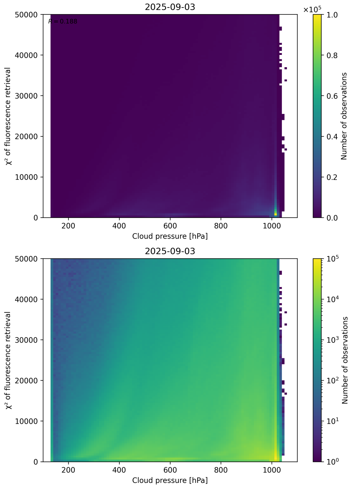
Figure 78: Scatter density plot of “Cloud pressure” against “ \chi^2 of fluorescence retrieval” for 2025-09-02 to 2025-09-04.
