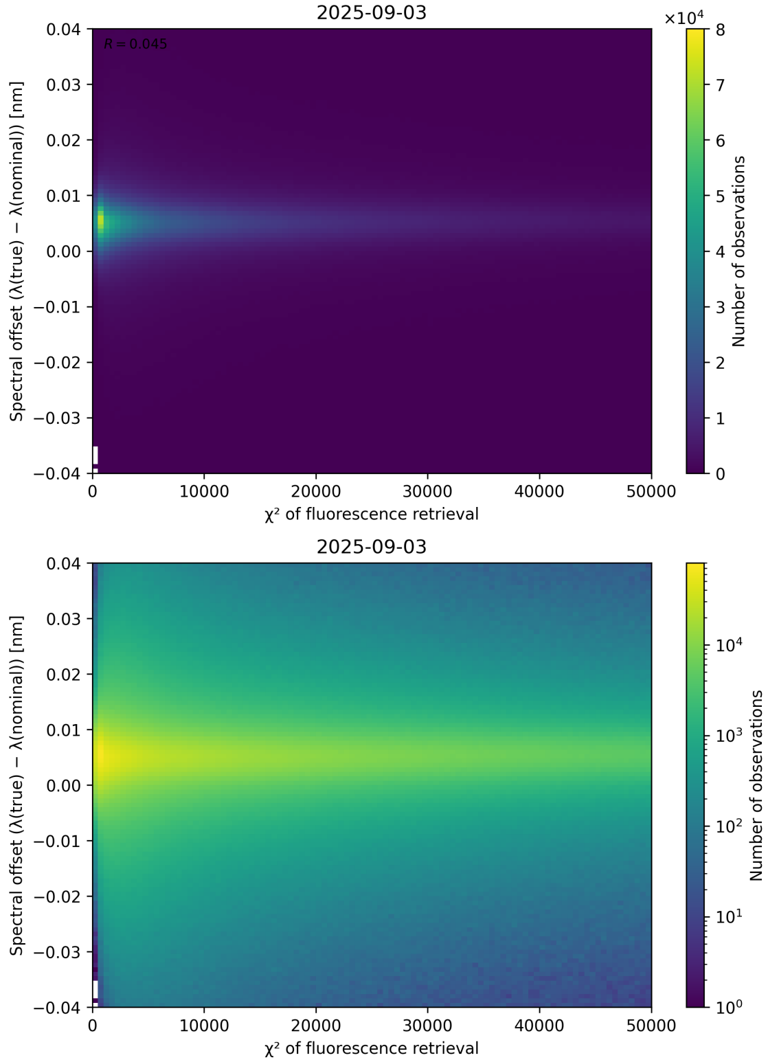
Figure 69: Scatter density plot of “ \chi^2 of fluorescence retrieval” against “Spectral offset ( \lambda_{\text{true}} - \lambda_{\text{nominal}} )” for 2025-09-02 to 2025-09-04.
