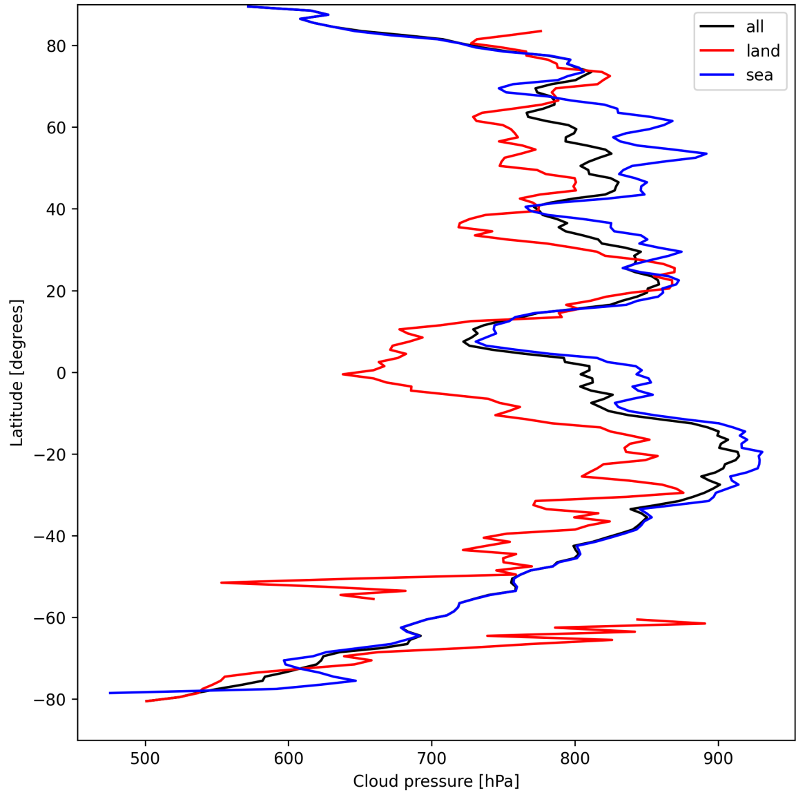
Figure 13: Zonal average of “Cloud pressure” for 2025-09-02 to 2025-09-04.
