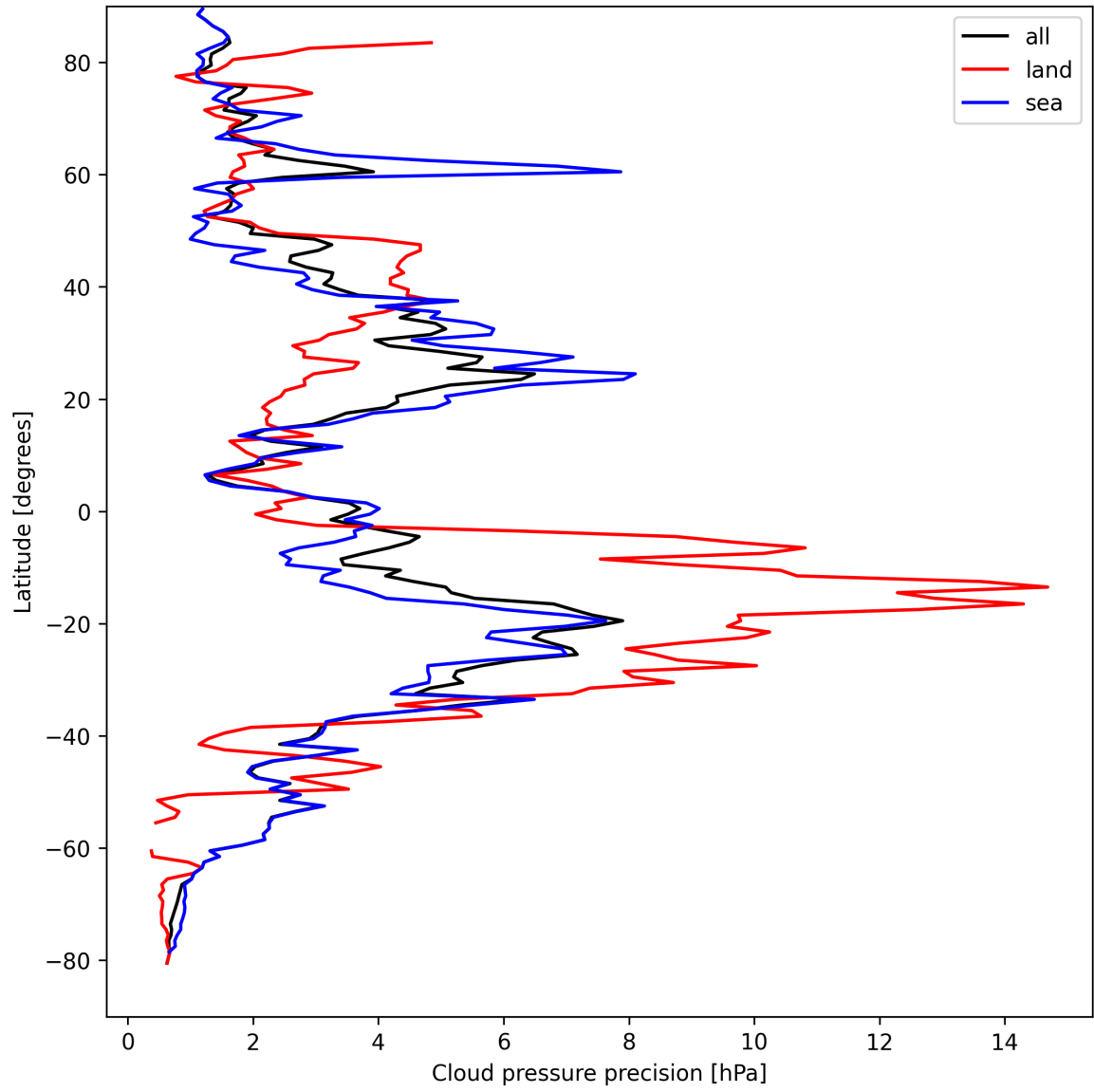
Figure 14: Zonal average of “Cloud pressure precision” for 2025-09-02 to 2025-09-04.
