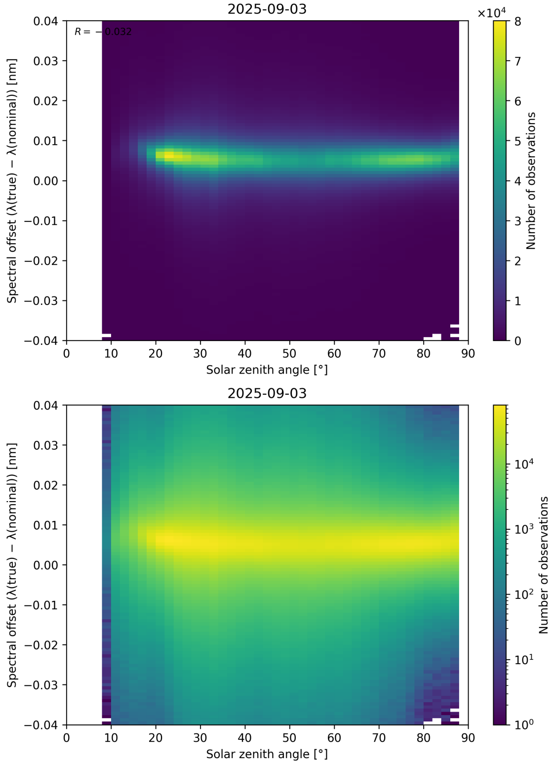
Figure 117: Scatter density plot of “Solar zenith angle” against “Spectral offset ( \lambda_{\text{true}} - \lambda_{\text{nominal}} )” for 2025-09-02 to 2025-09-04.
