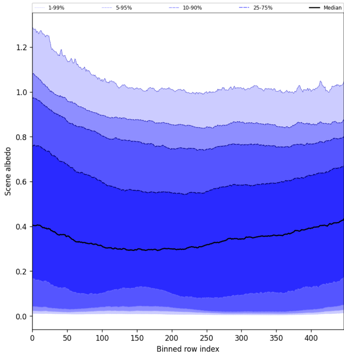
Figure 51: Along track statistics of “Scene albedo” for 2025-09-02 to 2025-09-04
