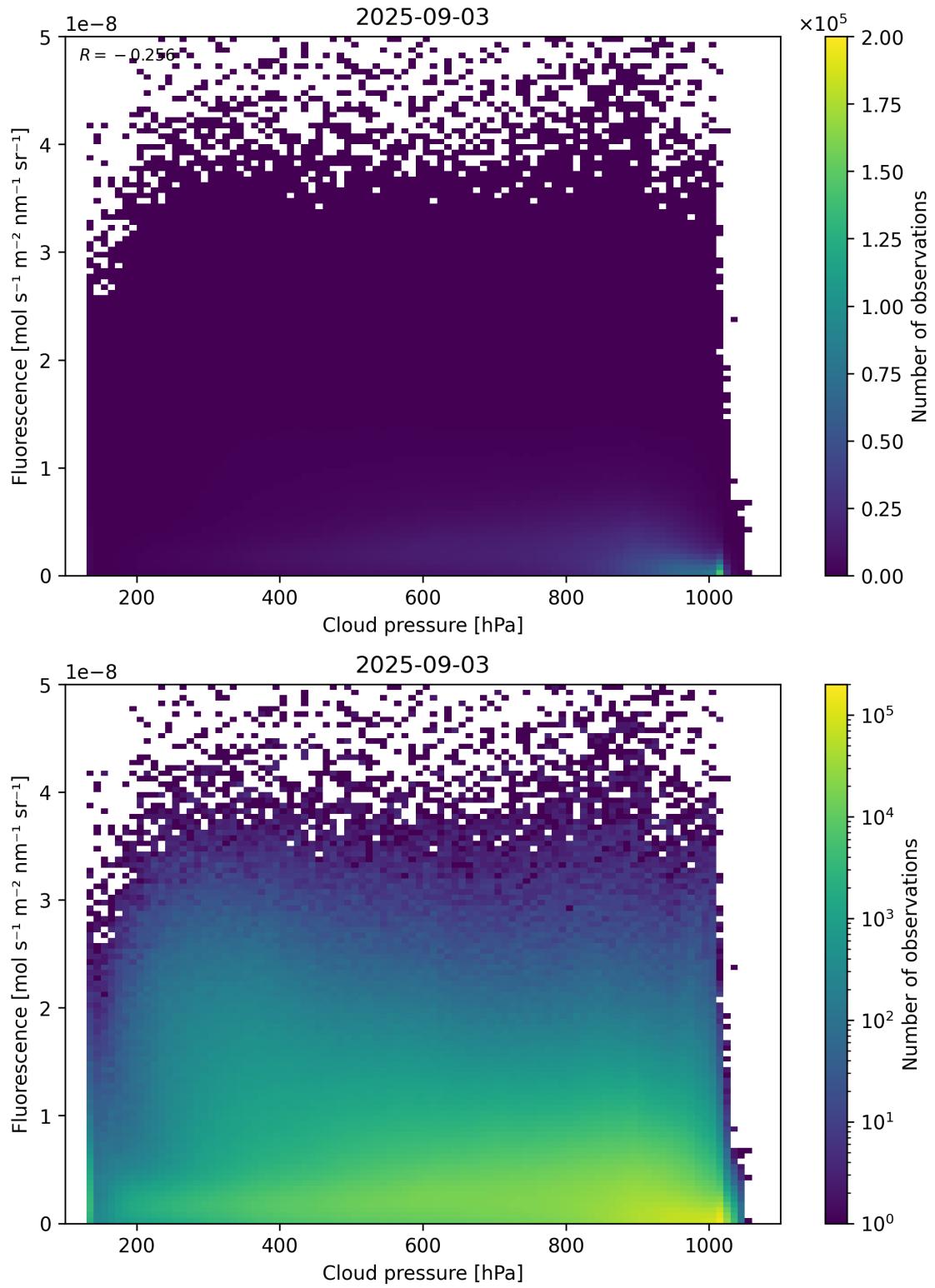
Figure 80: Scatter density plot of “Cloud pressure” against “Fluorescence” for 2025-09-02 to 2025-09-04.
