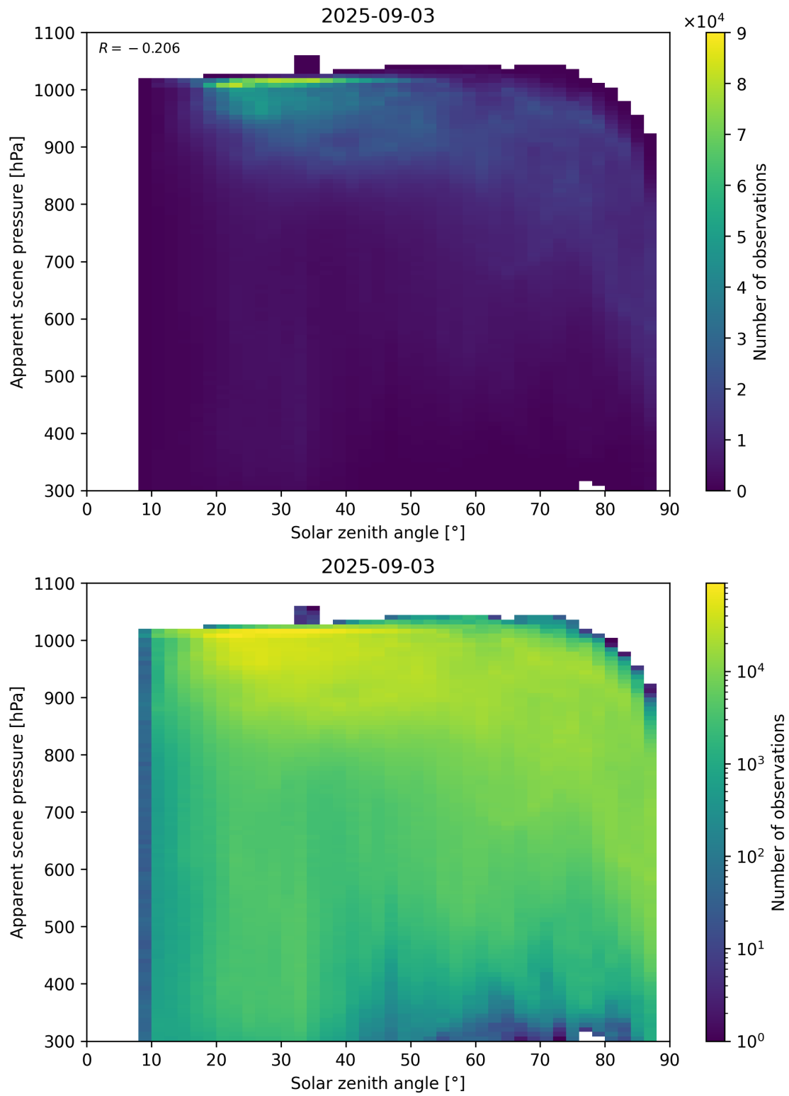
Figure 108: Scatter density plot of “Solar zenith angle” against “Apparent scene pressure” for 2025-09-02 to 2025-09-04.
