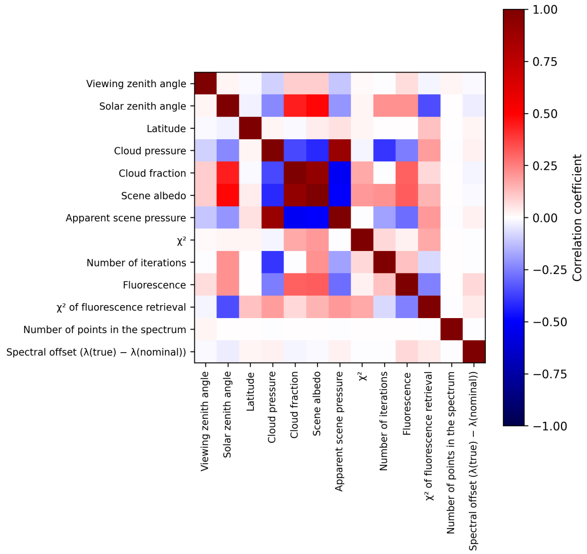
Figure 2: Map of correlation matrix for 2025-09-02 to 2025-09-04.
