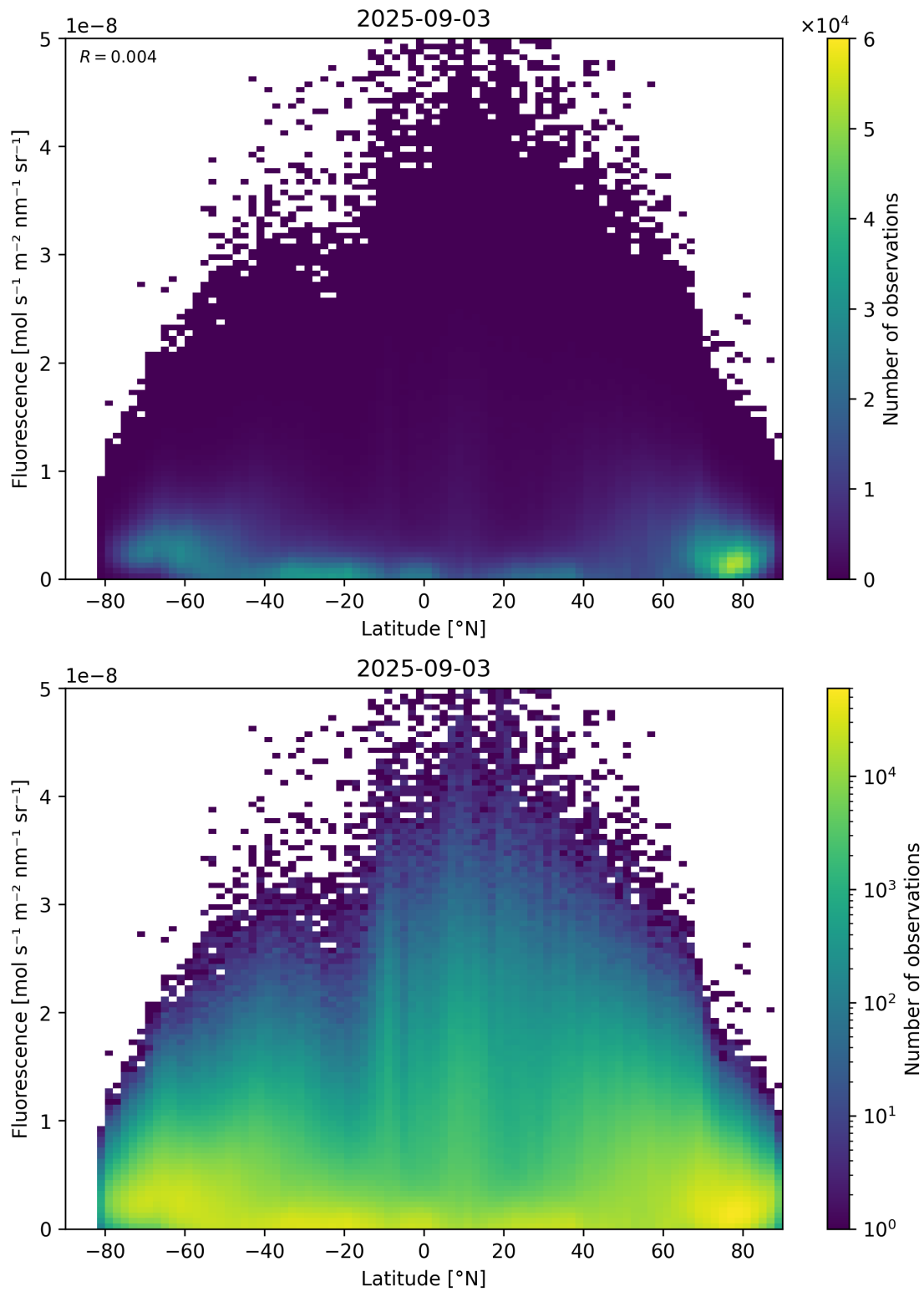
Figure 92: Scatter density plot of “Latitude” against “Fluorescence” for 2025-09-02 to 2025-09-04.
