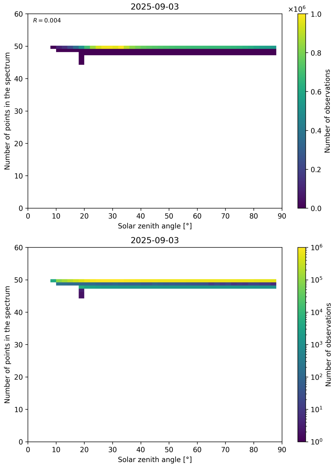
Figure 115: Scatter density plot of “Solar zenith angle” against “Number of points in the spectrum” for 2025-09-02 to 2025-09-04.
