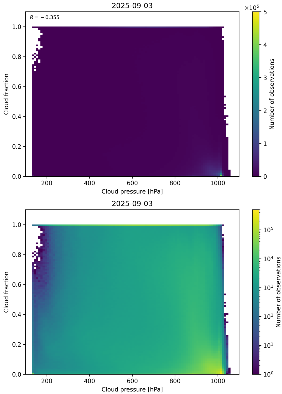
Figure 79: Scatter density plot of “Cloud pressure” against “Cloud fraction” for 2025-09-02 to 2025-09-04.
