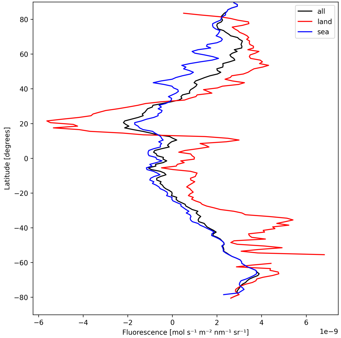
Figure 23: Zonal average of “Fluorescence” for 2025-09-02 to 2025-09-04.
