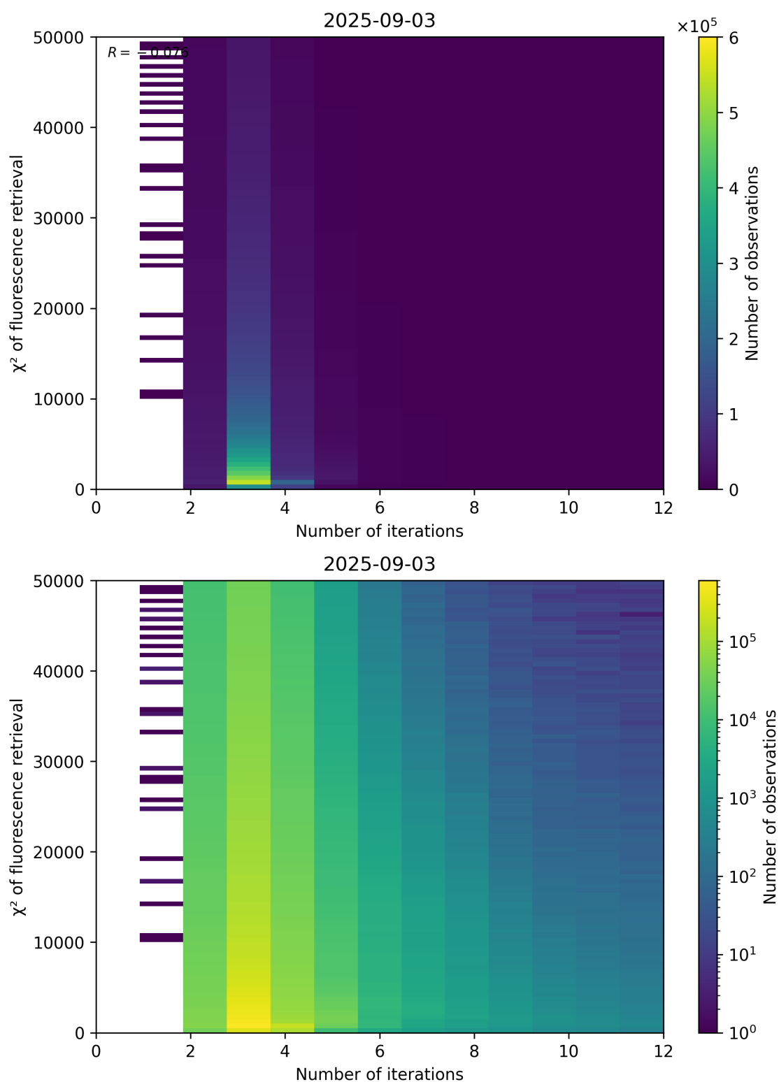
Figure 97: Scatter density plot of “Number of iterations” against “ \chi^2 of fluorescence retrieval” for 2025-09-02 to 2025-09-04.
