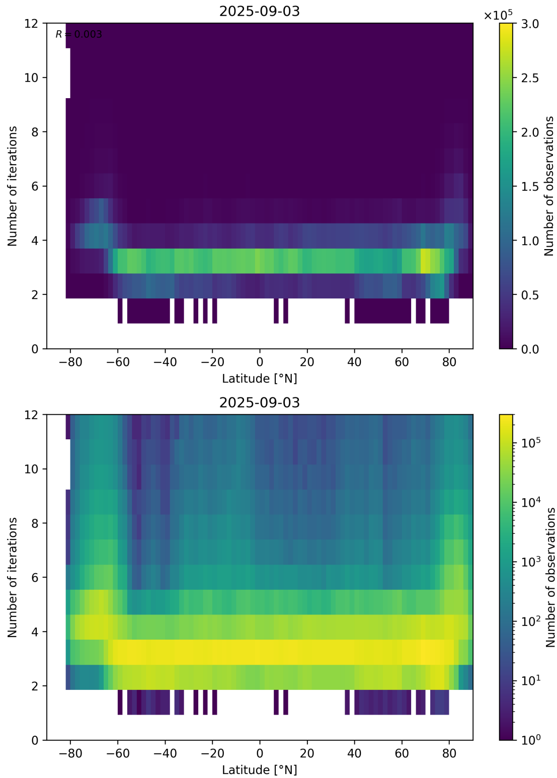
Figure 93: Scatter density plot of “Latitude” against “Number of iterations” for 2025-09-02 to 2025-09-04.
