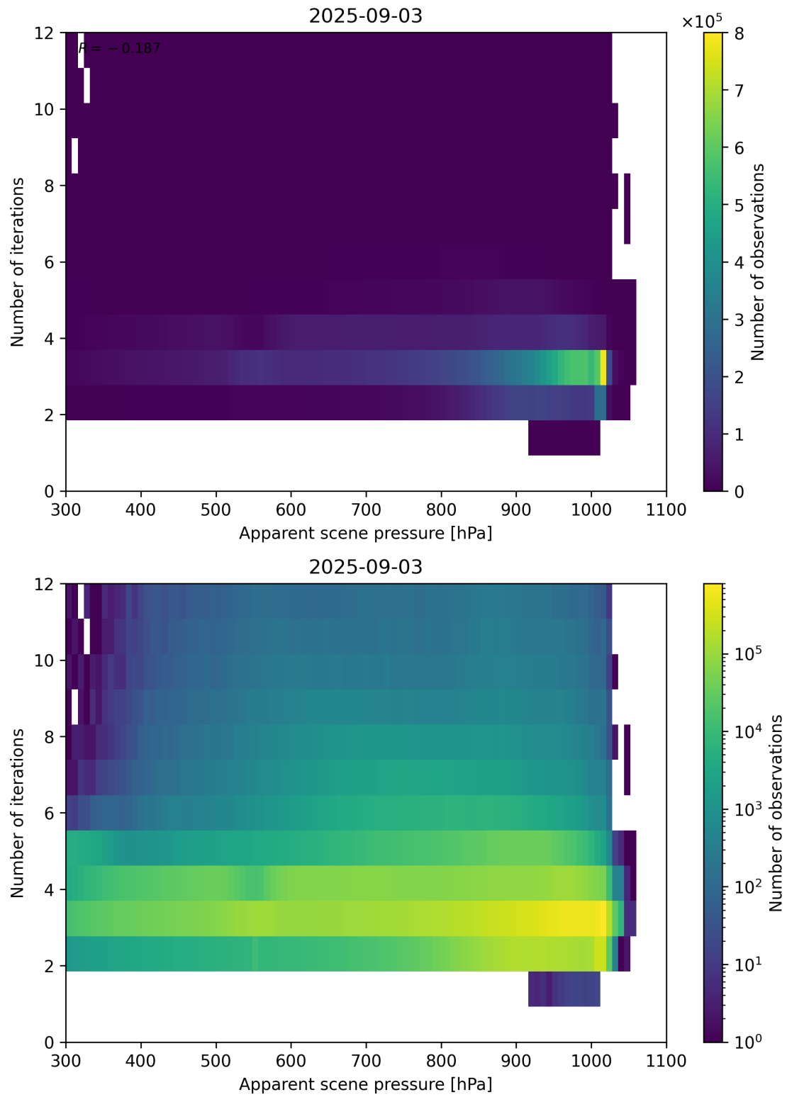
Figure 65: Scatter density plot of “Apparent scene pressure” against “Number of iterations” for 2025-09-02 to 2025-09-04.
