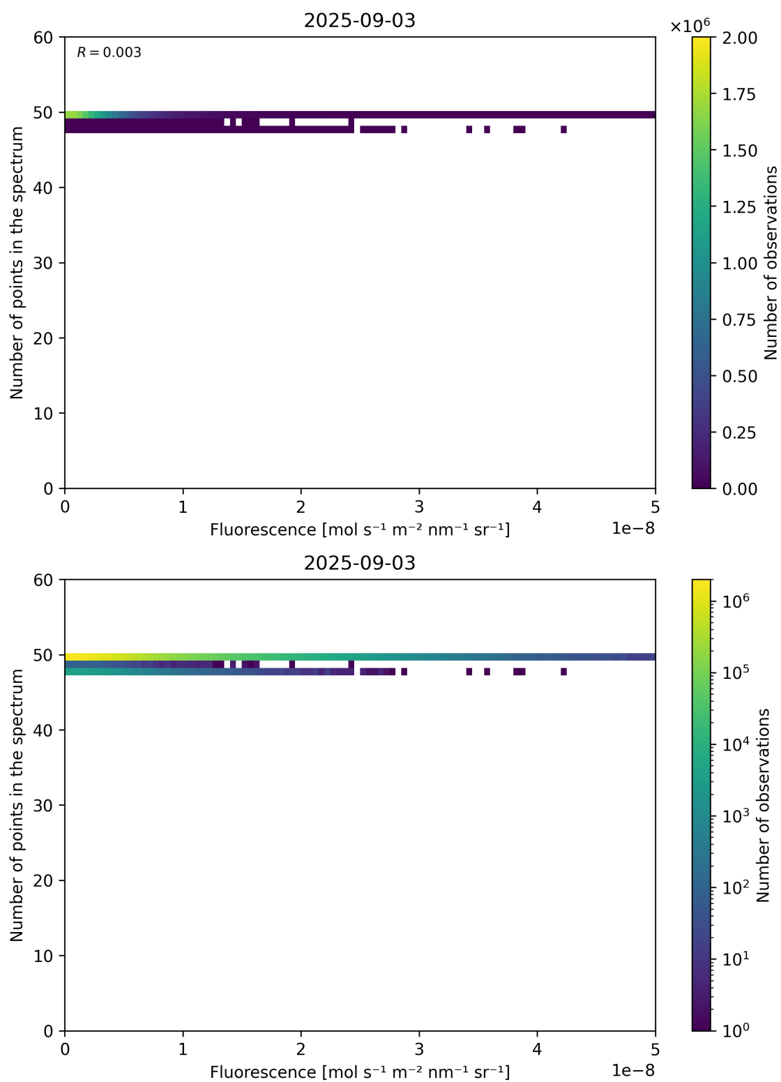
Figure 86: Scatter density plot of “Fluorescence” against “Number of points in the spectrum” for 2025-09-02 to 2025-09-04.
