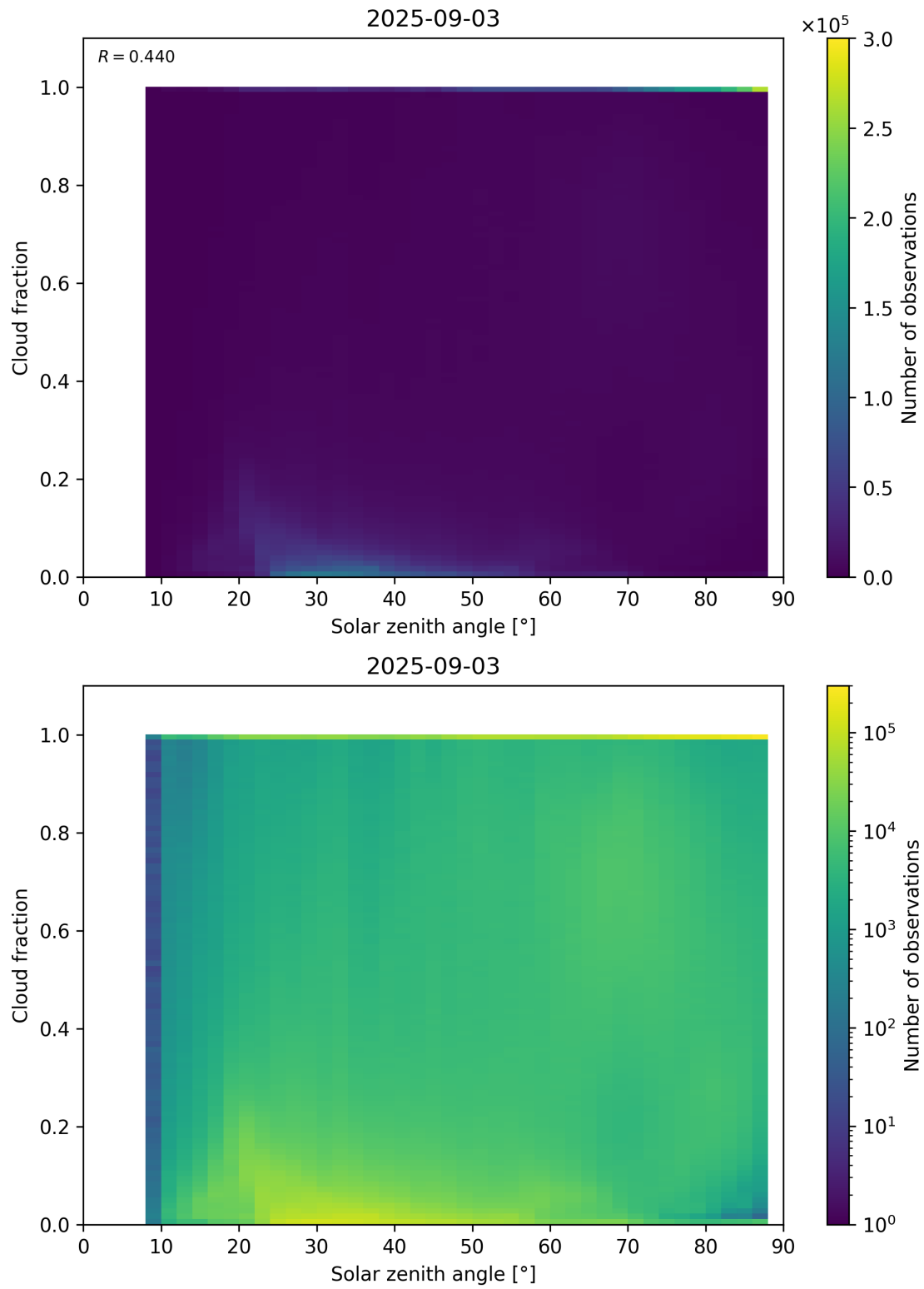
Figure 110: Scatter density plot of “Solar zenith angle” against “Cloud fraction” for 2025-09-02 to 2025-09-04.
