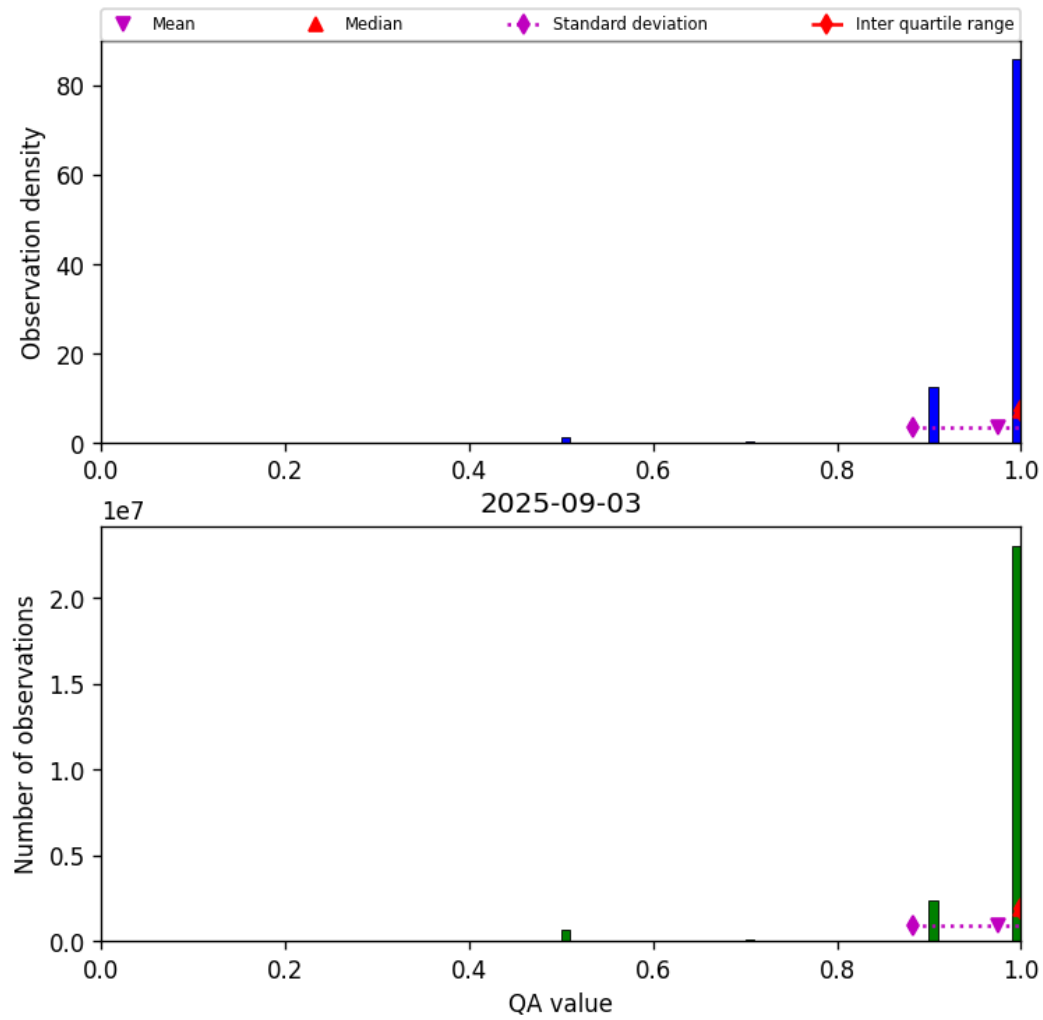
Figure 29: Histogram of “QA value” for 2025-09-02 to 2025-09-04
