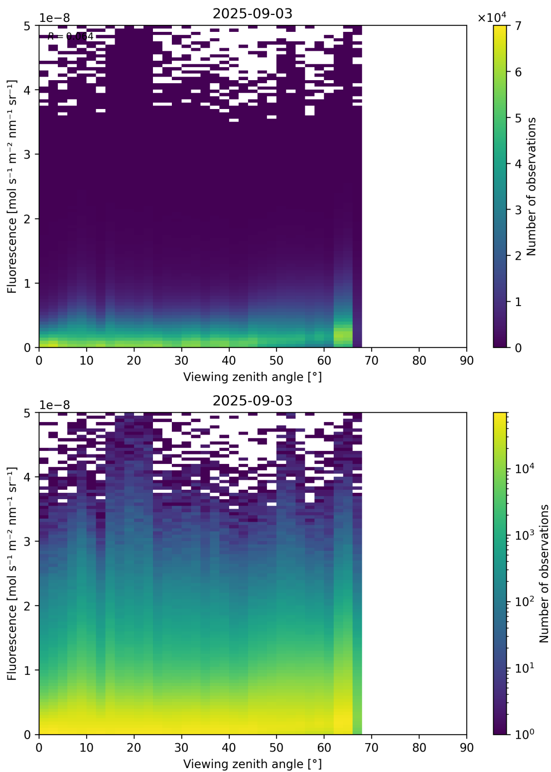
Figure 122: Scatter density plot of “Viewing zenith angle” against “Fluorescence” for 2025-09-02 to 2025-09-04.
