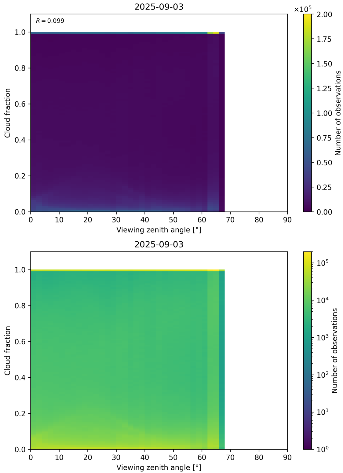
Figure 120: Scatter density plot of “Viewing zenith angle” against “Cloud fraction” for 2025-09-02 to 2025-09-04.
