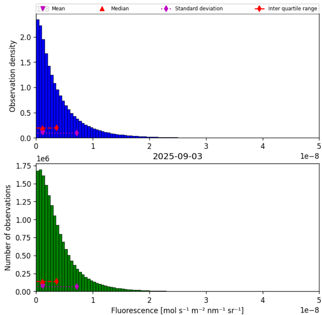
Figure 40: Histogram of “Fluorescence” for 2025-09-02 to 2025-09-04
