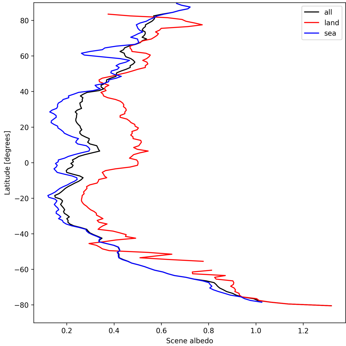
Figure 17: Zonal average of “Scene albedo” for 2025-09-02 to 2025-09-04.
