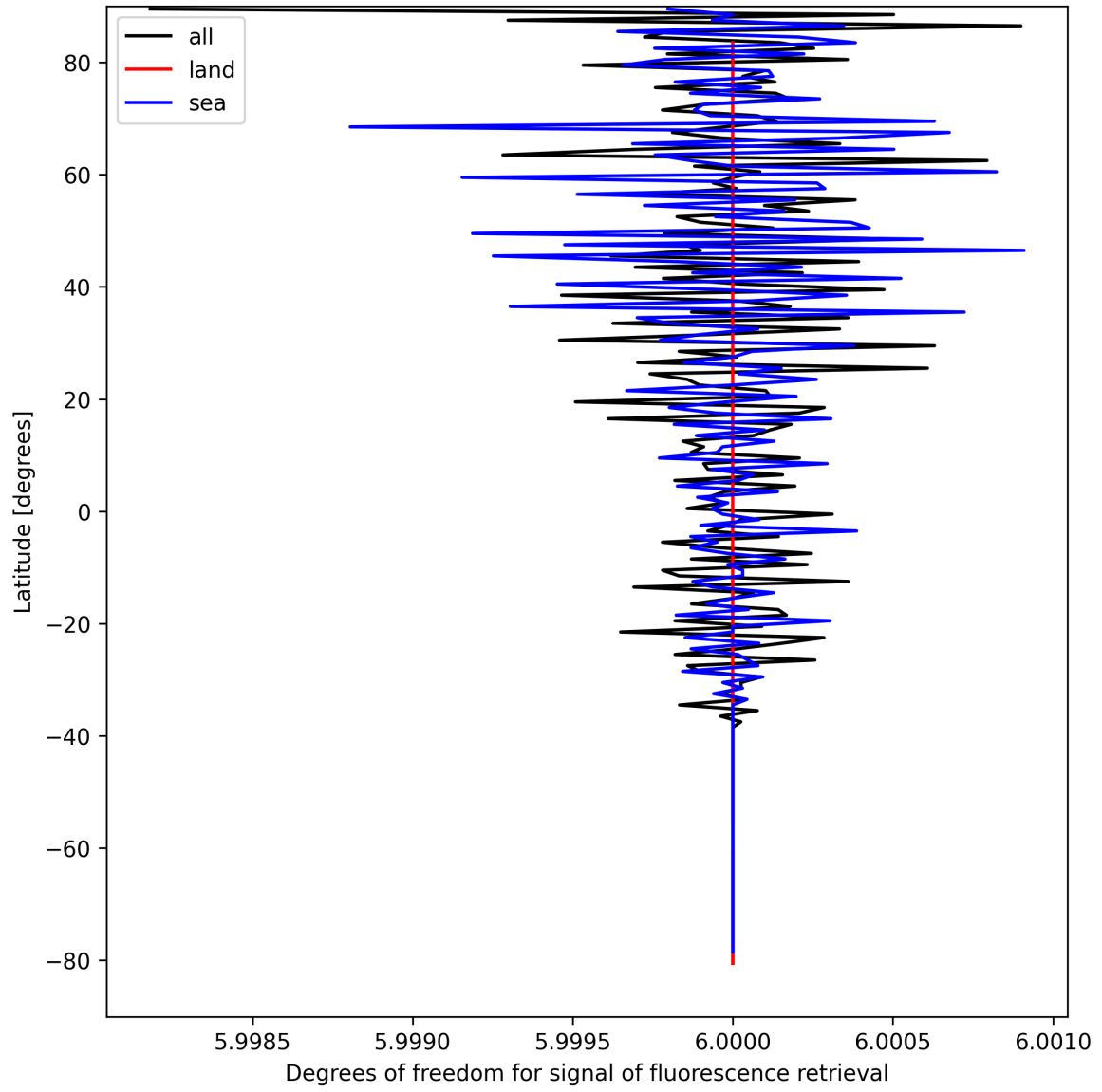
Figure 26: Zonal average of “Degrees of freedom for signal of fluorescence retrieval” for 2025-09-02 to 2025-09-04.
