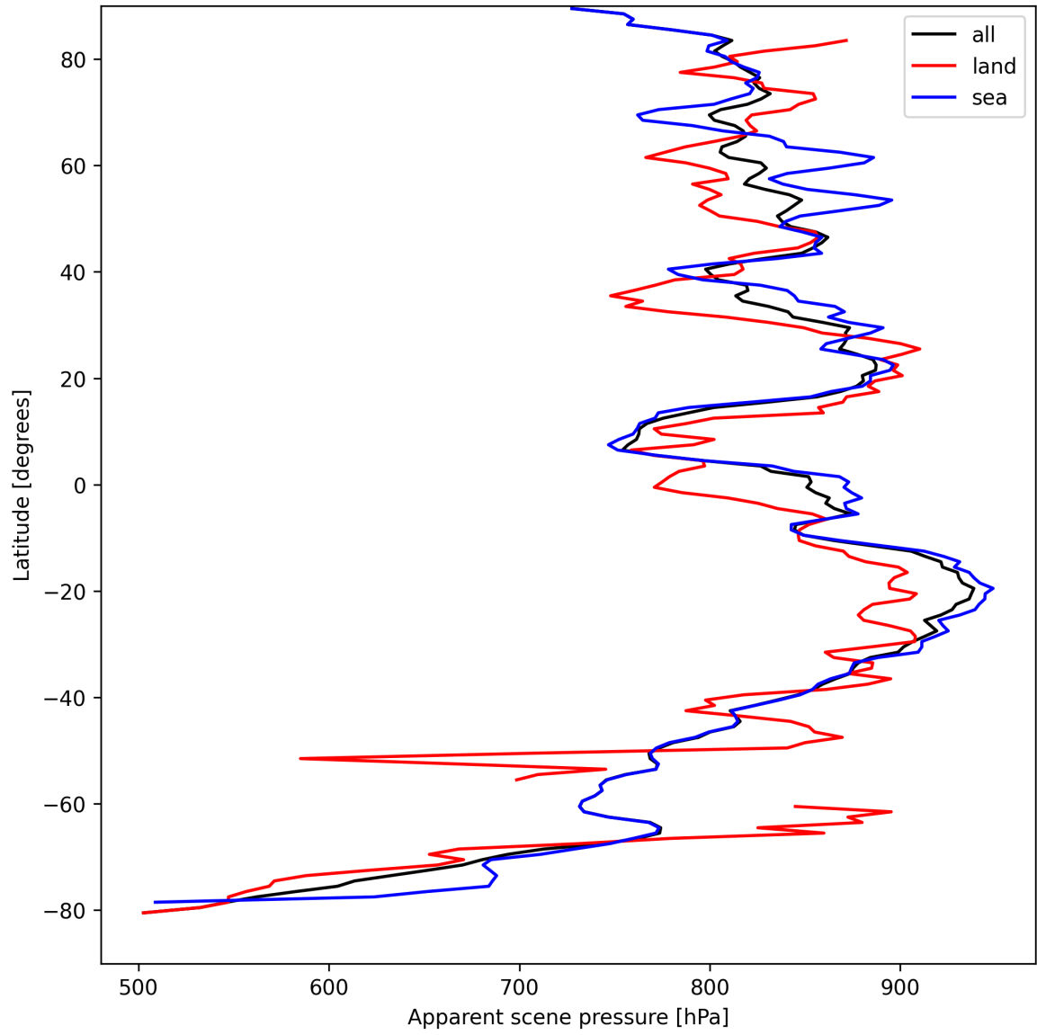
Figure 19: Zonal average of “Apparent scene pressure” for 2025-09-02 to 2025-09-04.
