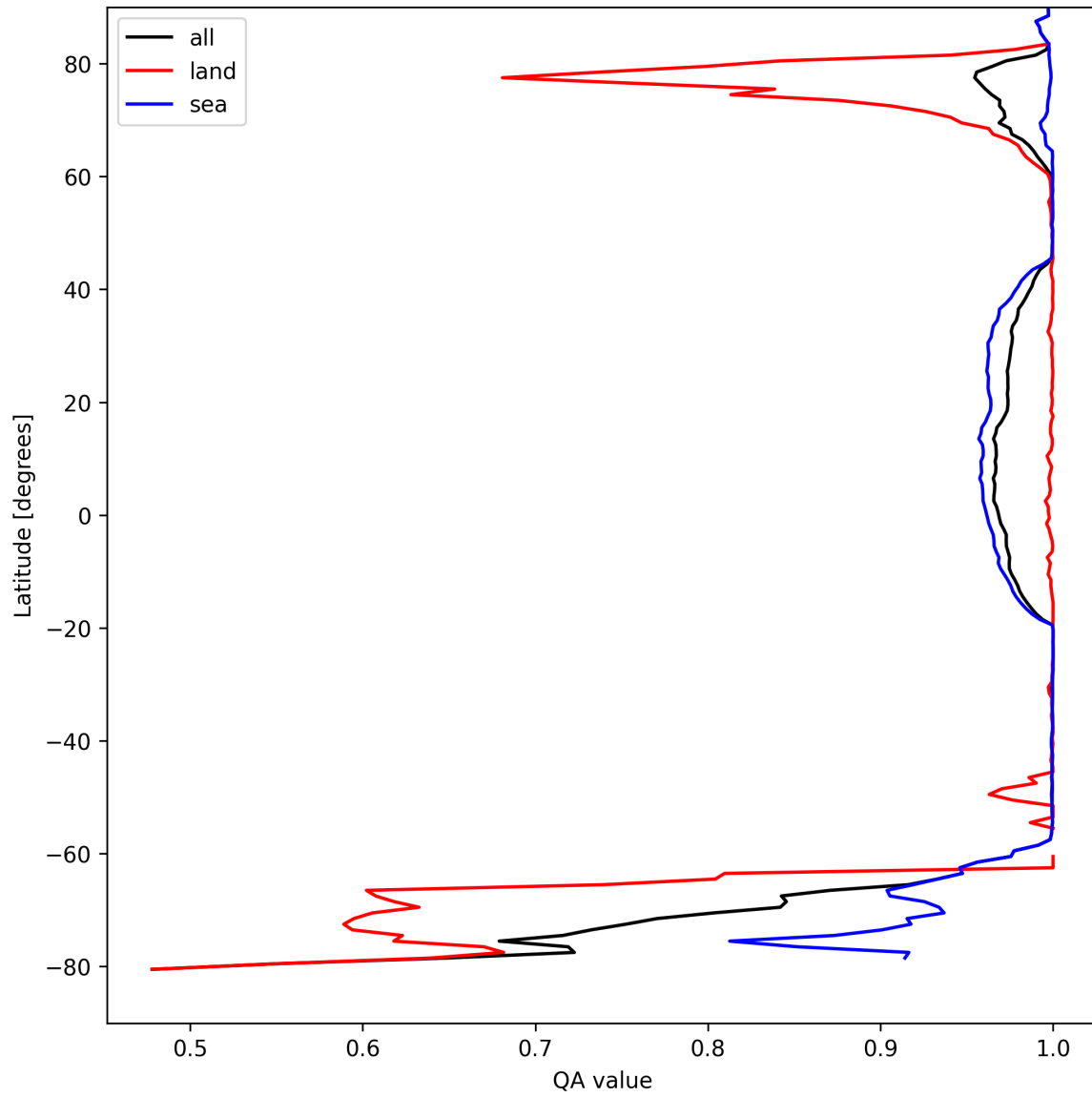
Figure 12: Zonal average of “QA value” for 2025-09-02 to 2025-09-04.
