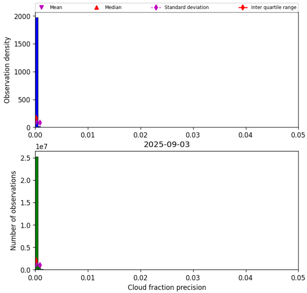
Figure 33: Histogram of “Cloud fraction precision” for 2025-09-02 to 2025-09-04
