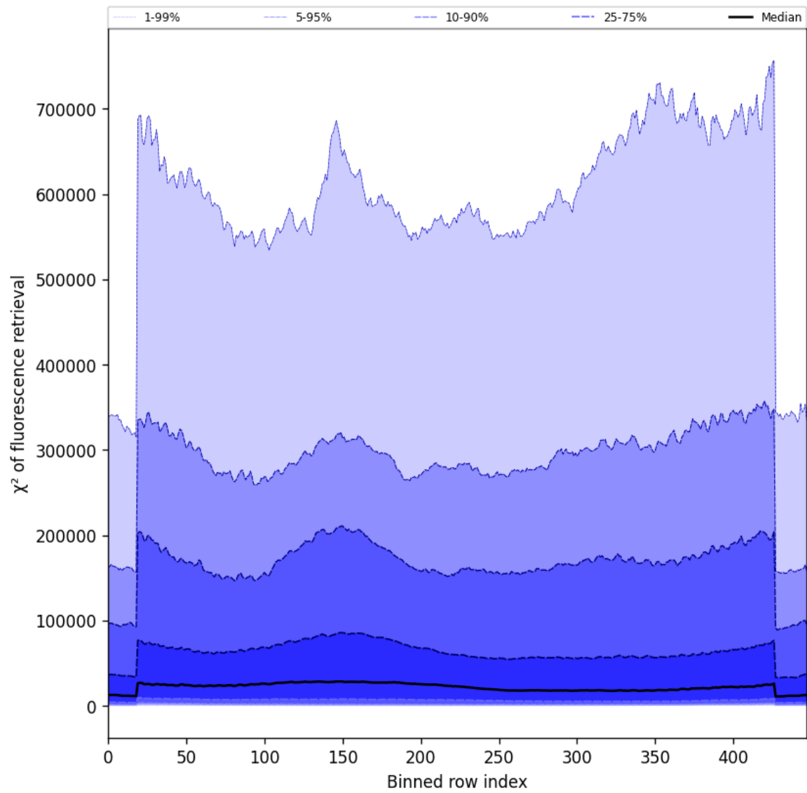
Figure 59: Along track statistics of “ \chi^2 of fluorescence retrieval” for 2025-09-02 to 2025-09-04
