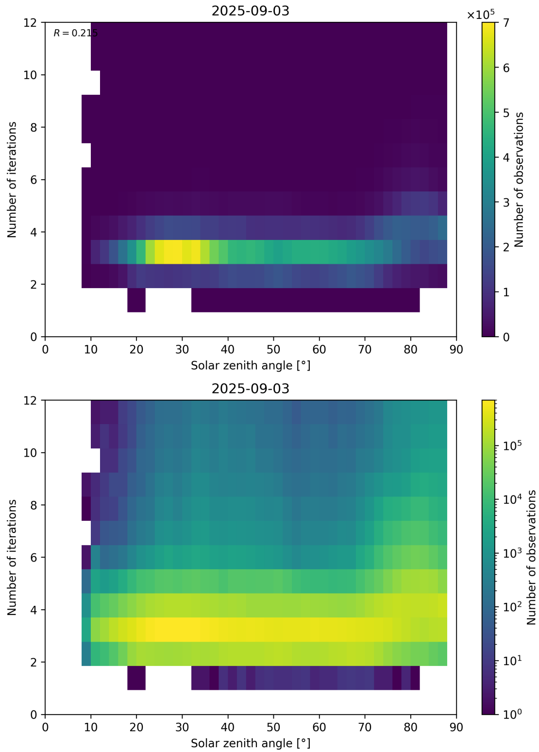
Figure 114: Scatter density plot of “Solar zenith angle” against “Number of iterations” for 2025-09-02 to 2025-09-04.
