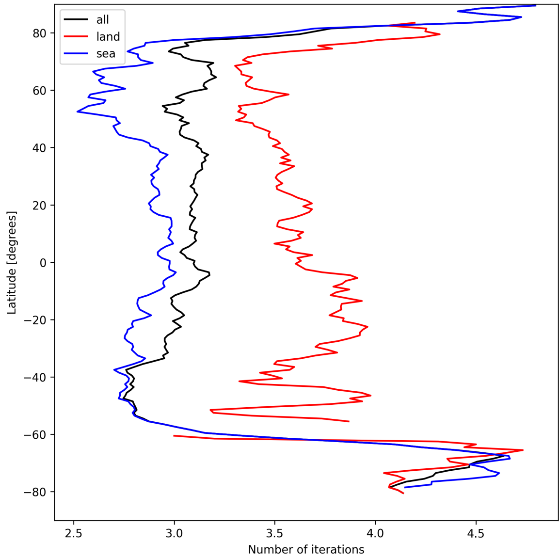
Figure 22: Zonal average of “Number of iterations” for 2025-09-02 to 2025-09-04.
