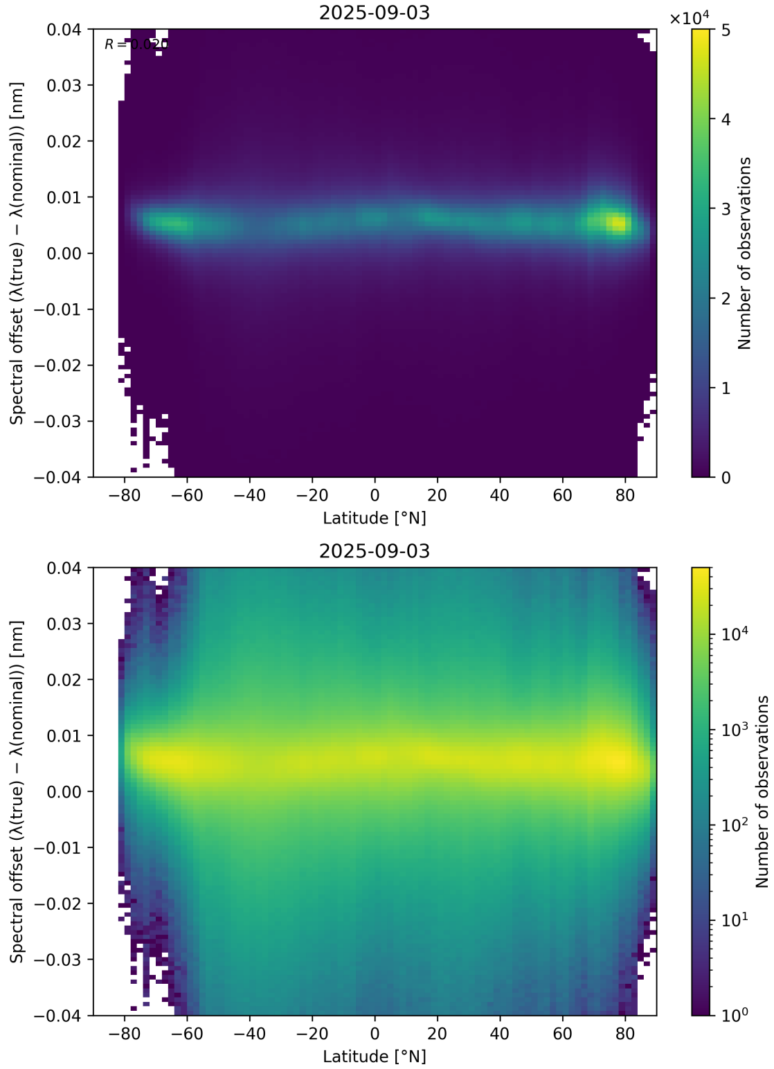
Figure 96: Scatter density plot of “Latitude” against “Spectral offset ( \lambda_{\text{true}} - \lambda_{\text{nominal}} )” for 2025-09-02 to 2025-09-04.
