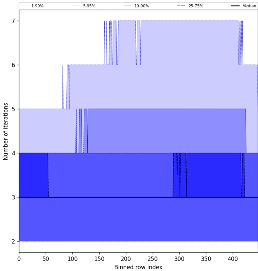
Figure 56: Along track statistics of “Number of iterations” for 2025-09-02 to 2025-09-04
