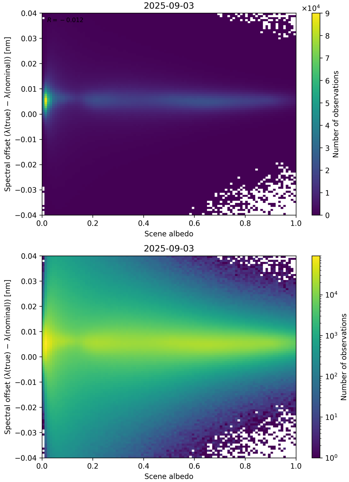
Figure 107: Scatter density plot of “Scene albedo” against “Spectral offset ( \lambda_{\text{true}} - \lambda_{\text{nominal}} )” for 2025-09-02 to 2025-09-04.
