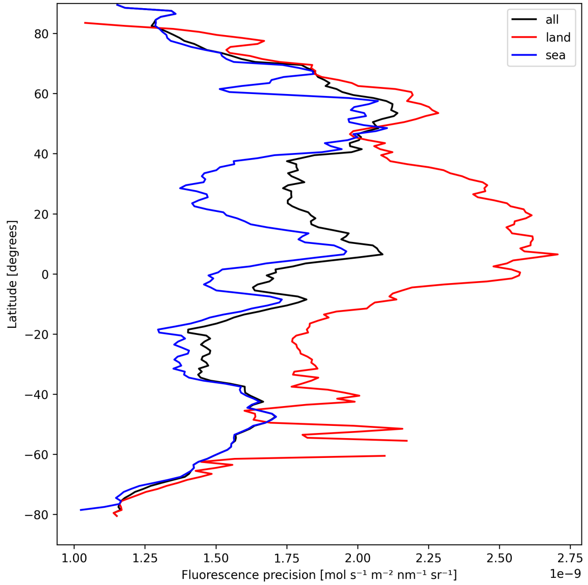
Figure 24: Zonal average of “Fluorescence precision” for 2025-09-02 to 2025-09-04.
