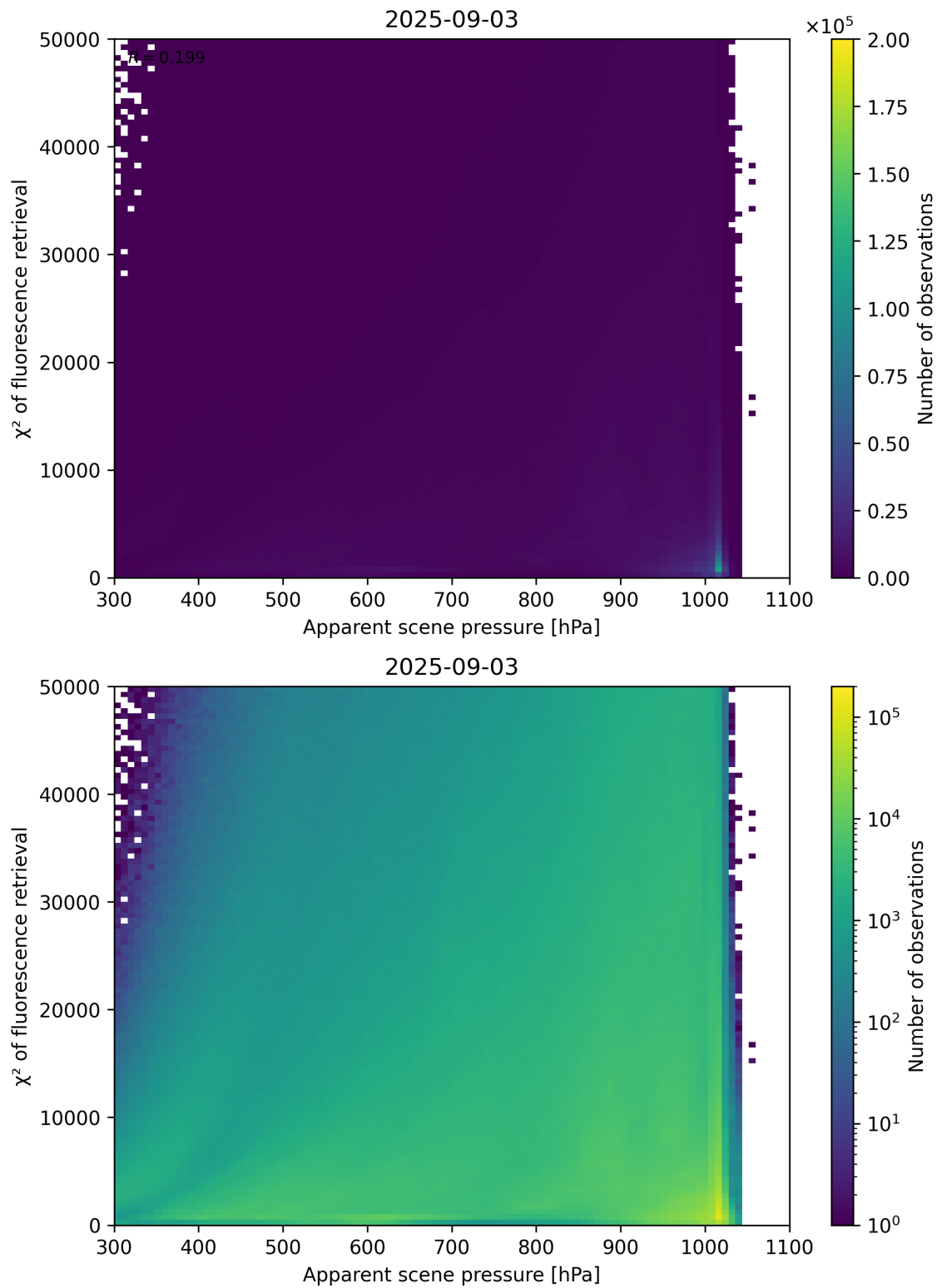
Figure 63: Scatter density plot of “Apparent scene pressure” against “ \chi^2 of fluorescence retrieval” for 2025-09-02 to 2025-09-04.
