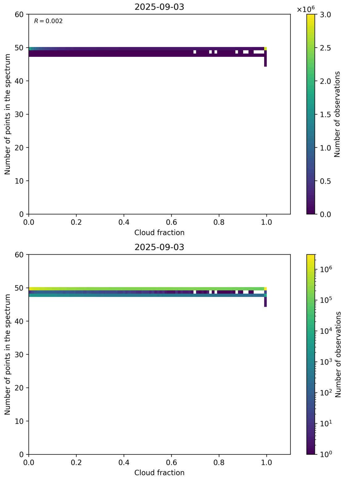
Figure 74: Scatter density plot of “Cloud fraction” against “Number of points in the spectrum” for 2025-09-02 to 2025-09-04.
