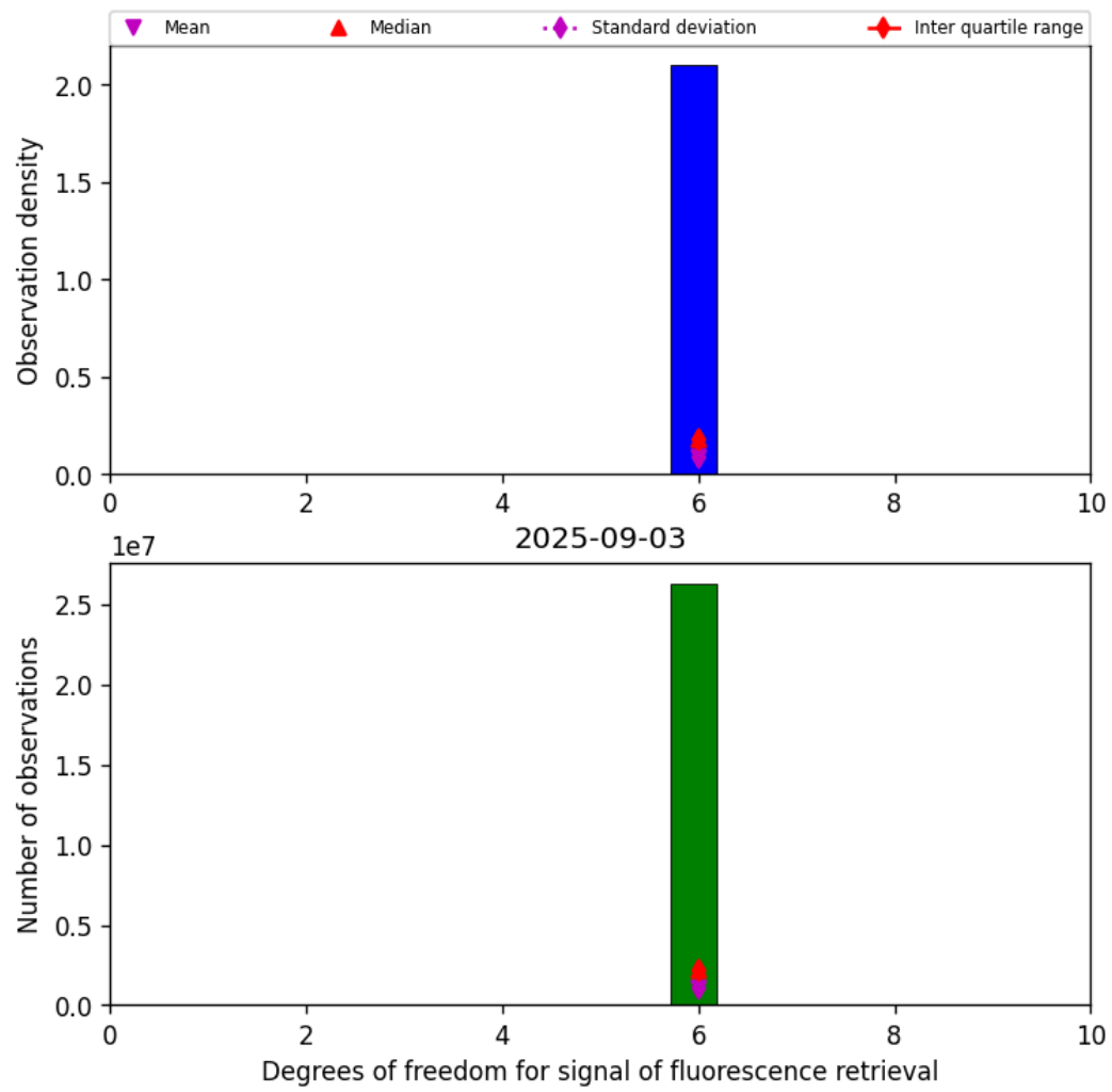
Figure 43: Histogram of "Degrees of freedom for signal of fluorescence retrieval" for 2025-09-02 to 2025-09-04
