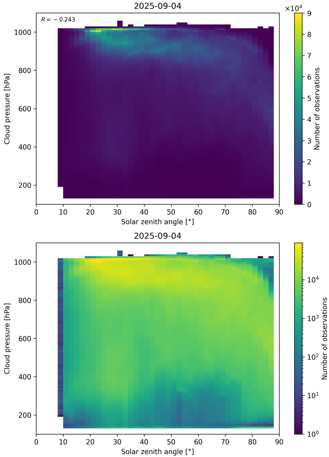
Figure 111: Scatter density plot of “Solar zenith angle” against “Cloud pressure” for 2025-09-04 to 2025-09-05.
