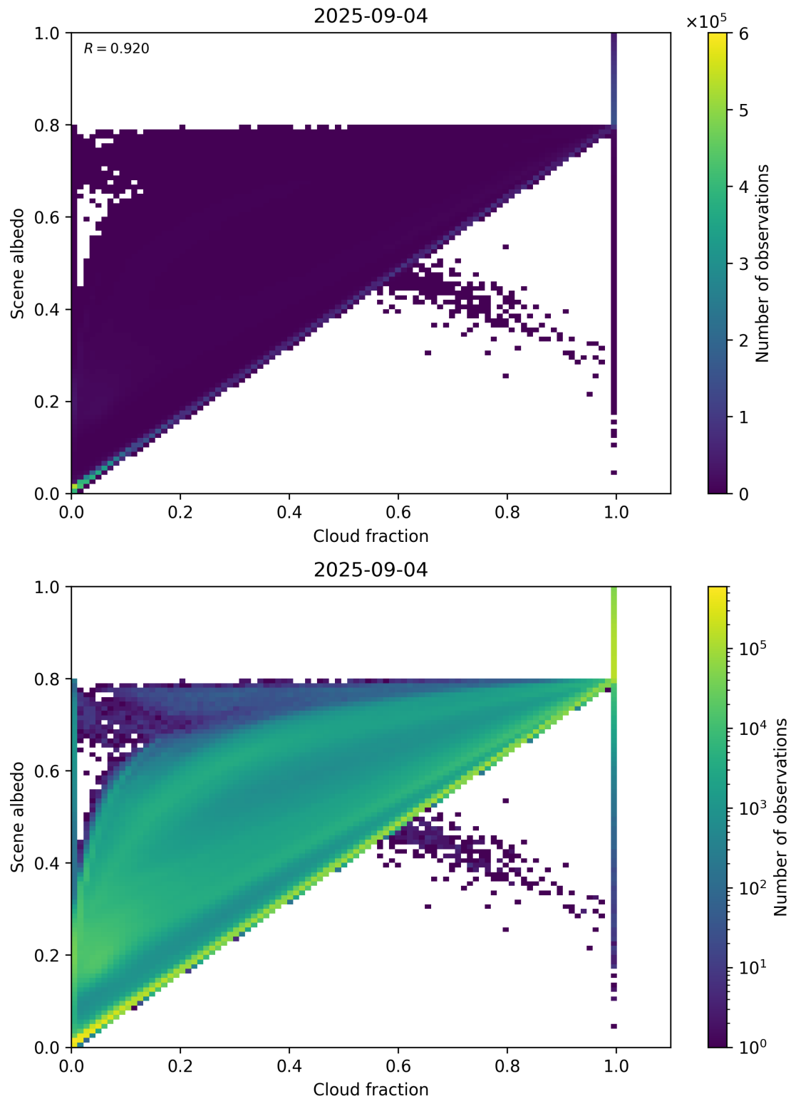
Figure 75: Scatter density plot of “Cloud fraction” against “Scene albedo” for 2025-09-04 to 2025-09-05.
