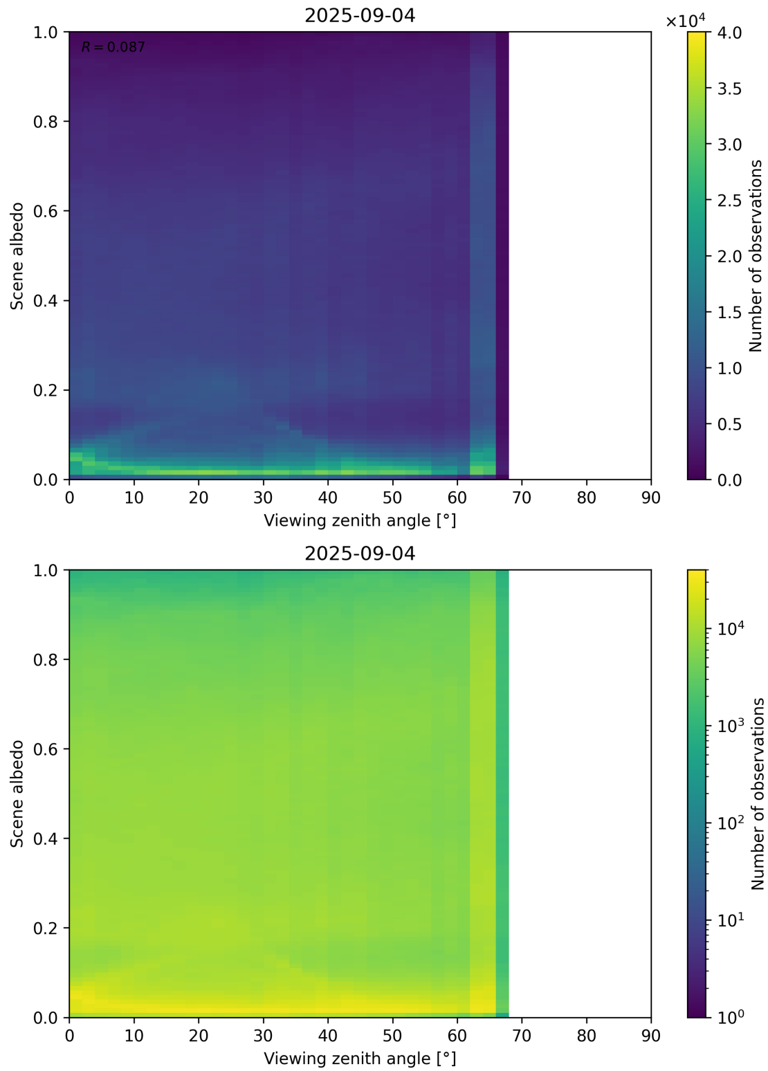
Figure 126: Scatter density plot of “Viewing zenith angle” against “Scene albedo” for 2025-09-04 to 2025-09-05.
