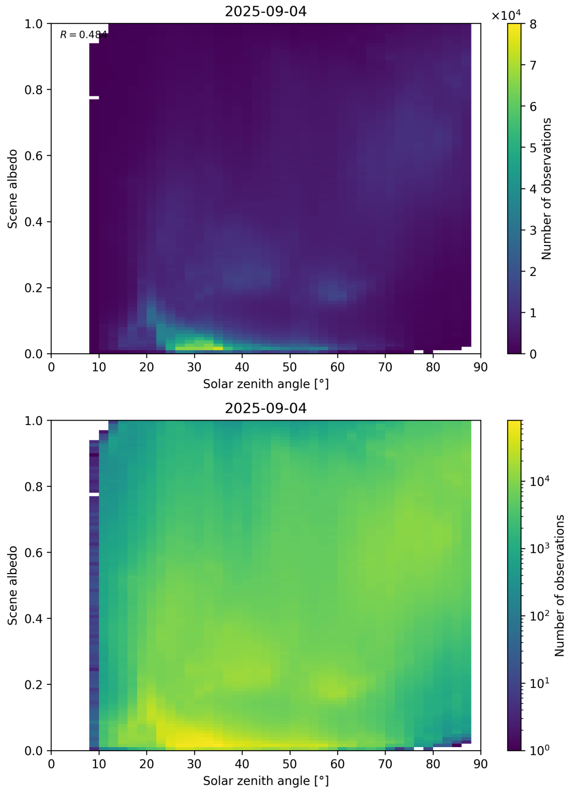
Figure 116: Scatter density plot of “Solar zenith angle” against “Scene albedo” for 2025-09-04 to 2025-09-05.
