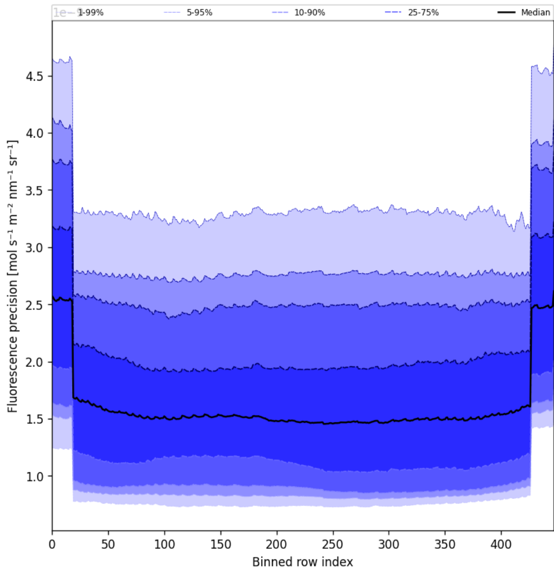
Figure 58: Along track statistics of “Fluorescence precision” for 2025-09-04 to 2025-09-05
