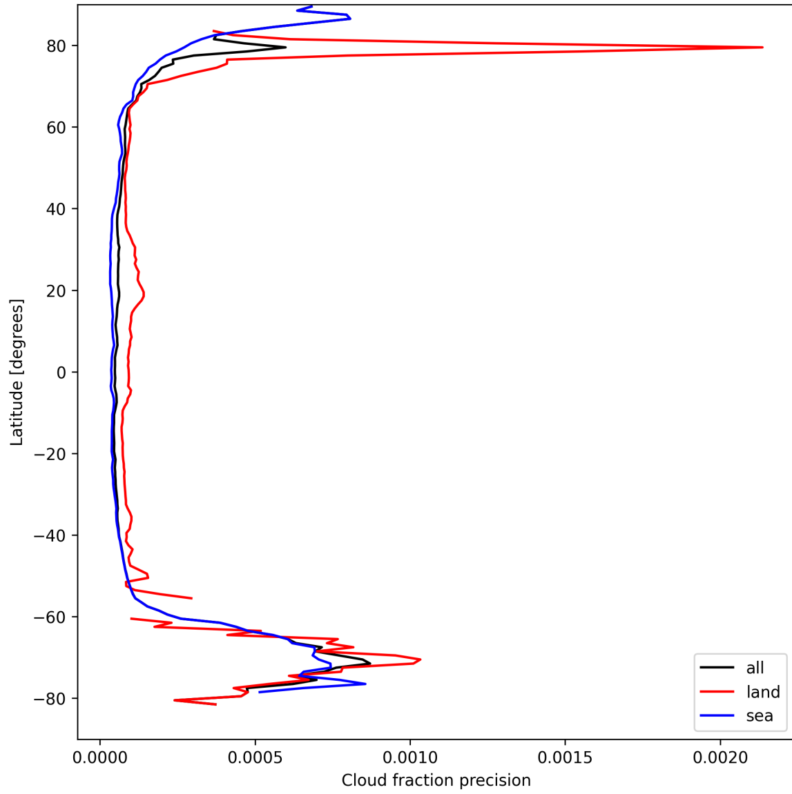
Figure 16: Zonal average of “Cloud fraction precision” for 2025-09-04 to 2025-09-05.
