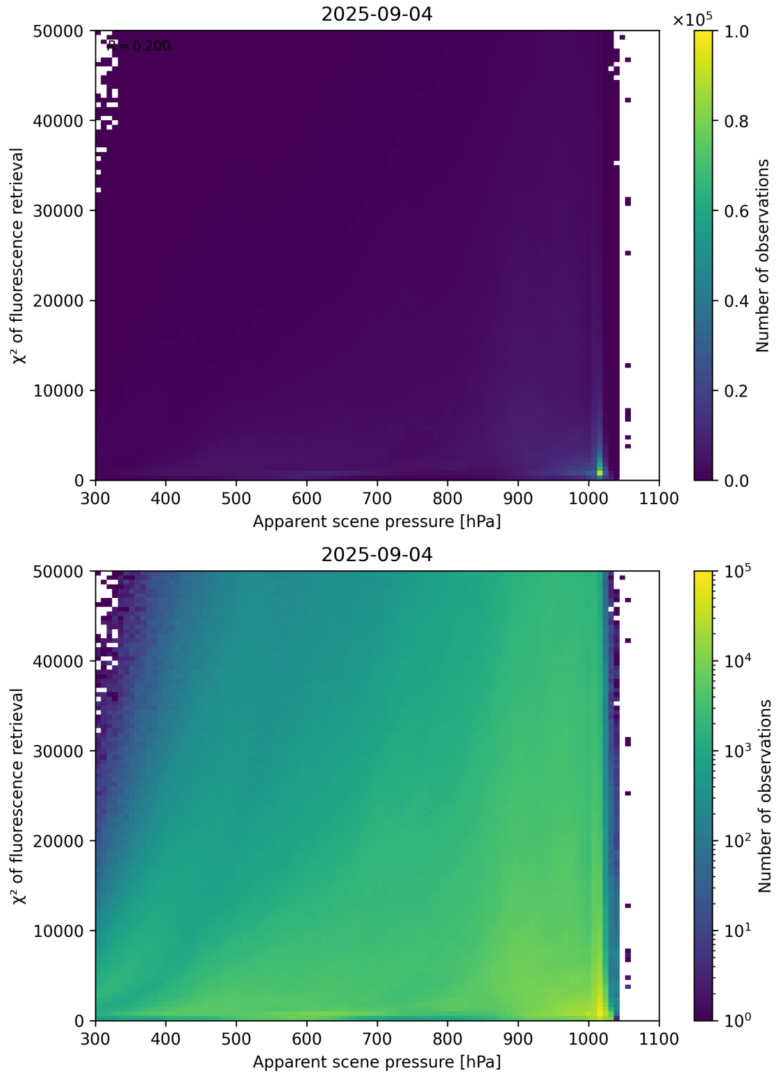
Figure 63: Scatter density plot of “Apparent scene pressure” against “ \chi^2 of fluorescence retrieval” for 2025-09-04 to 2025-09-05.
