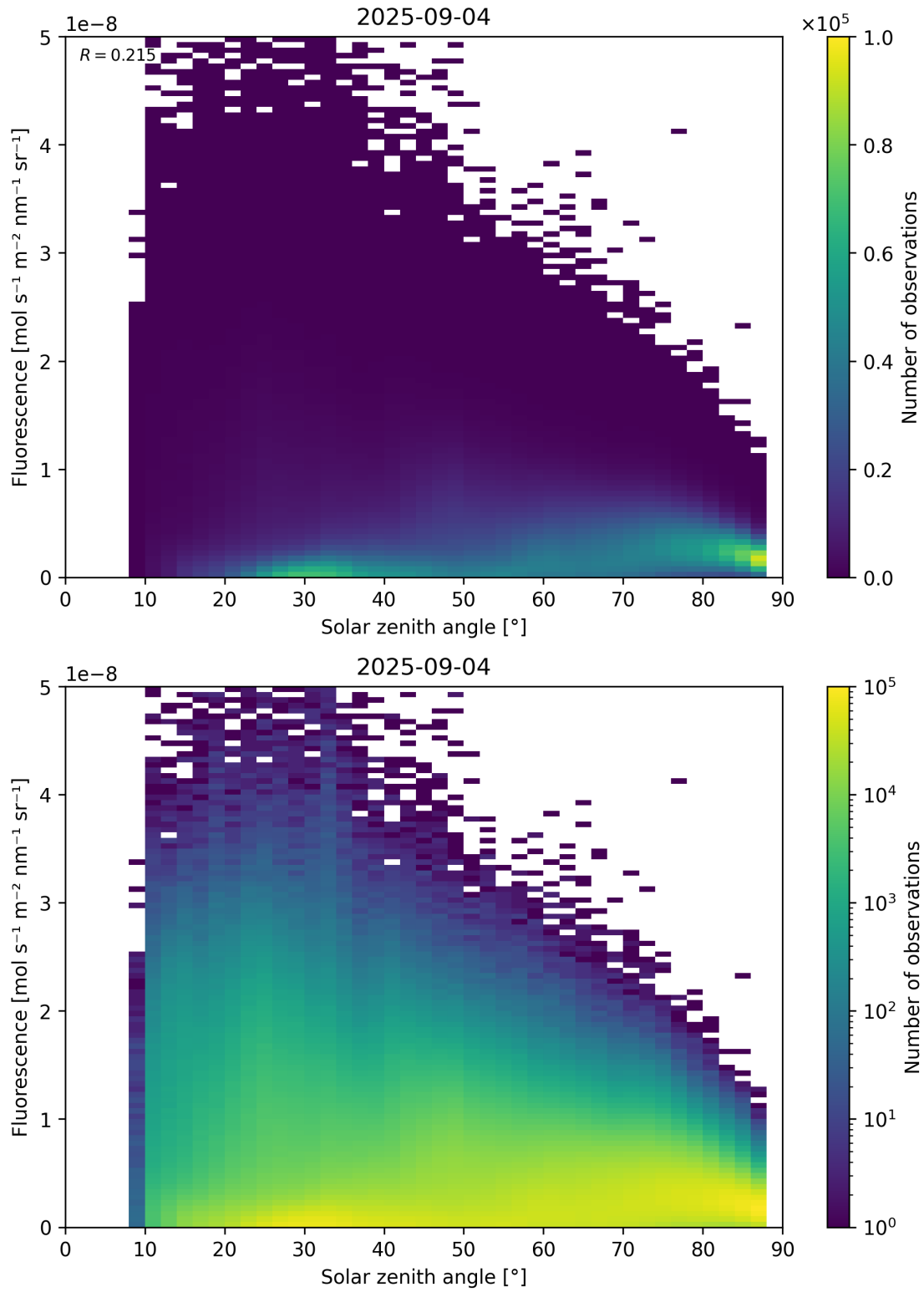
Figure 112: Scatter density plot of “Solar zenith angle” against “Fluorescence” for 2025-09-04 to 2025-09-05.
