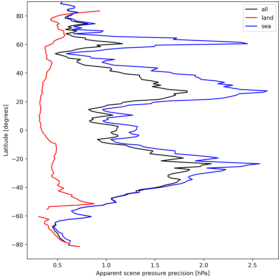
Figure 20: Zonal average of “Apparent scene pressure precision” for 2025-09-04 to 2025-09-05.
