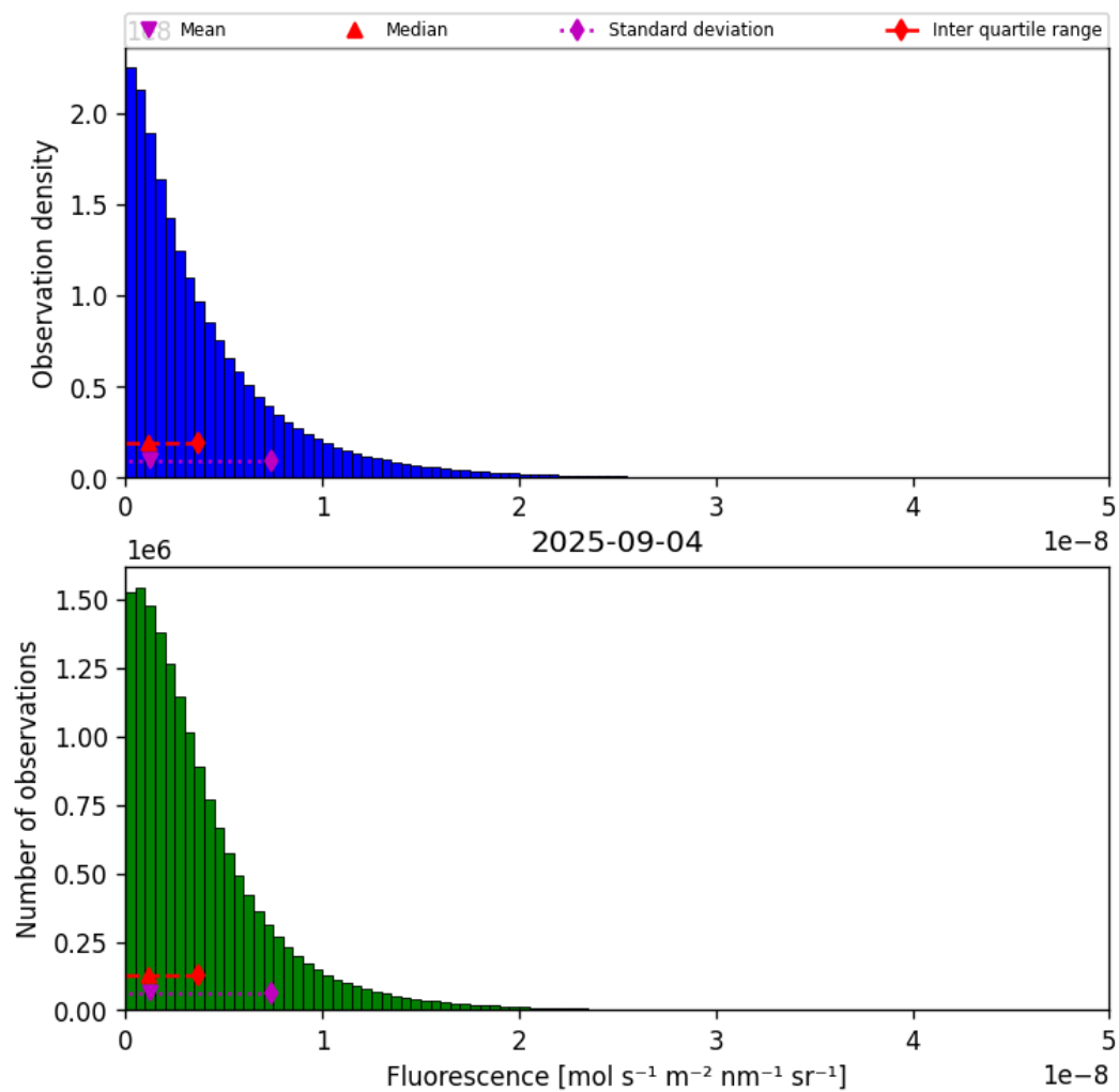
Figure 40: Histogram of “Fluorescence” for 2025-09-04 to 2025-09-05
