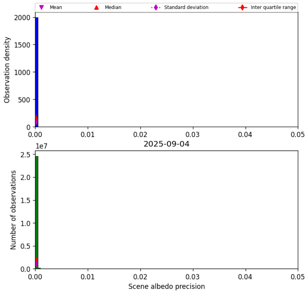
Figure 35: Histogram of “Scene albedo precision” for 2025-09-04 to 2025-09-05
