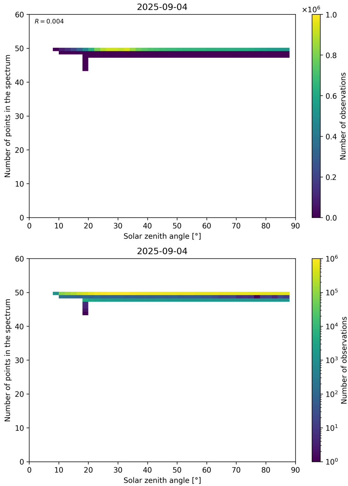
Figure 115: Scatter density plot of “Solar zenith angle” against “Number of points in the spectrum” for 2025-09-04 to 2025-09-05.
