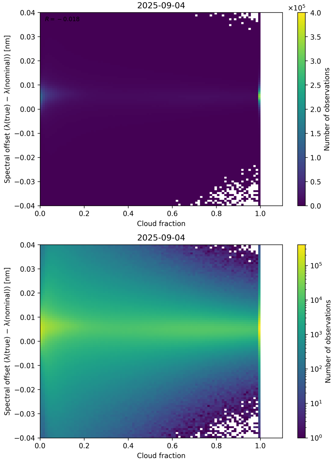
Figure 76: Scatter density plot of “Cloud fraction” against “Spectral offset ( \lambda_{\text{true}} - \lambda_{\text{nominal}} )” for 2025-09-04 to 2025-09-05.
