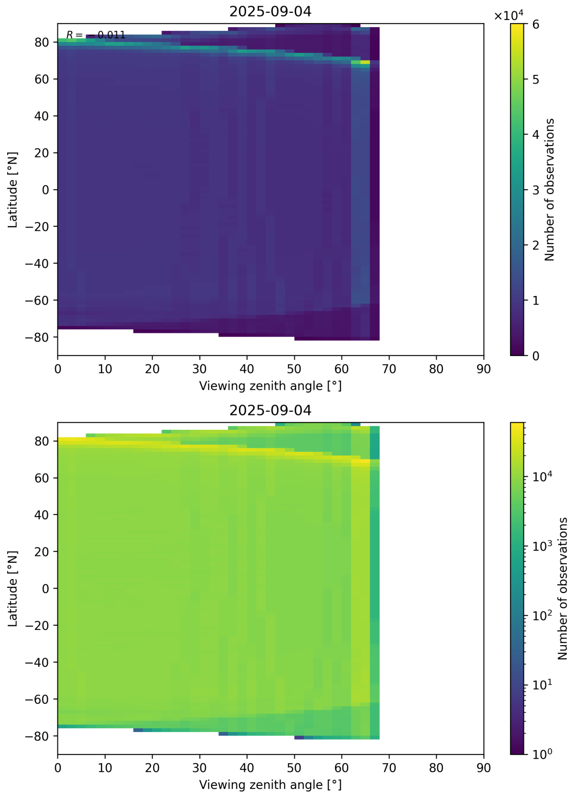
Figure 123: Scatter density plot of “Viewing zenith angle” against “Latitude” for 2025-09-04 to 2025-09-05.
