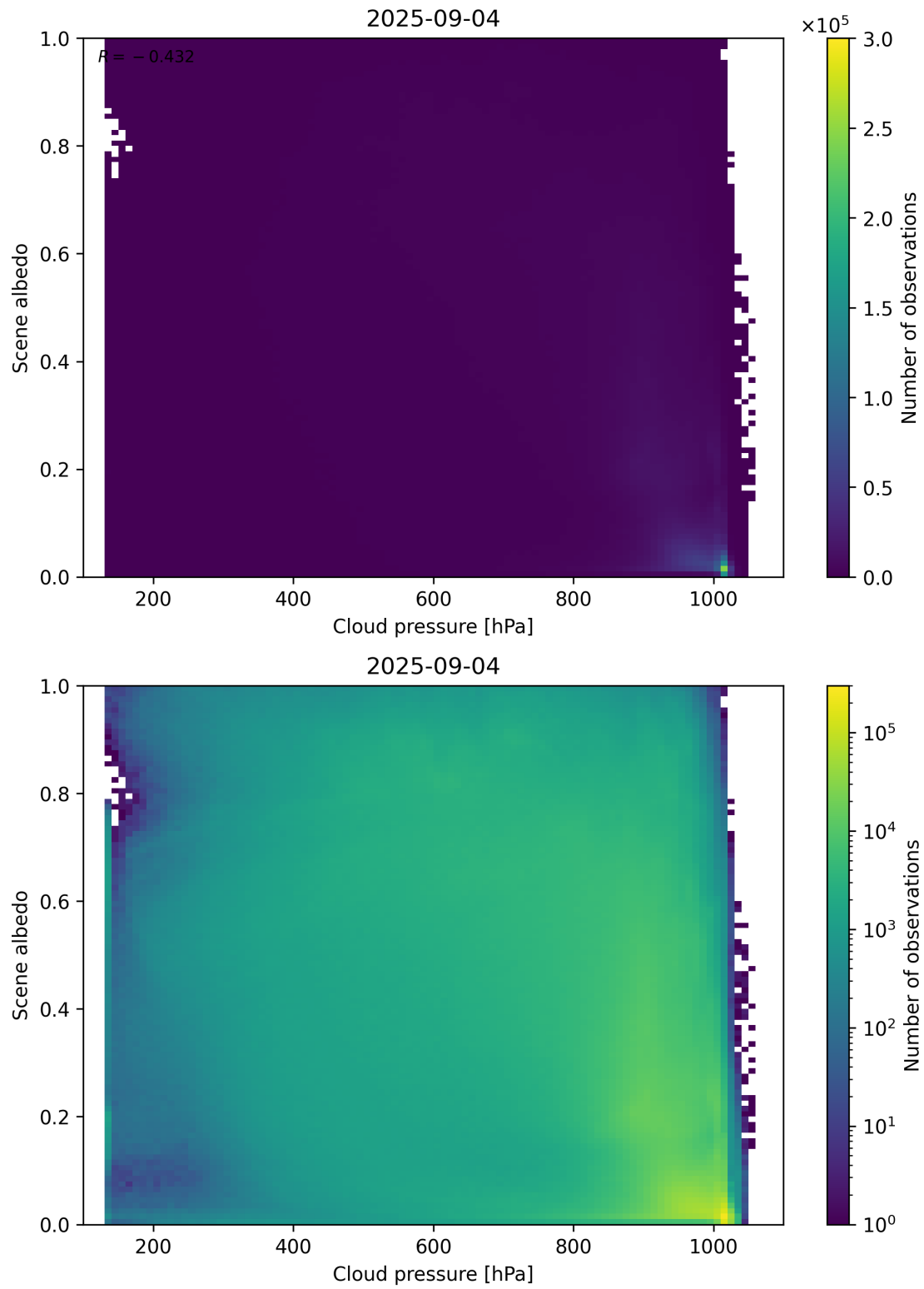
Figure 83: Scatter density plot of “Cloud pressure” against “Scene albedo” for 2025-09-04 to 2025-09-05.
