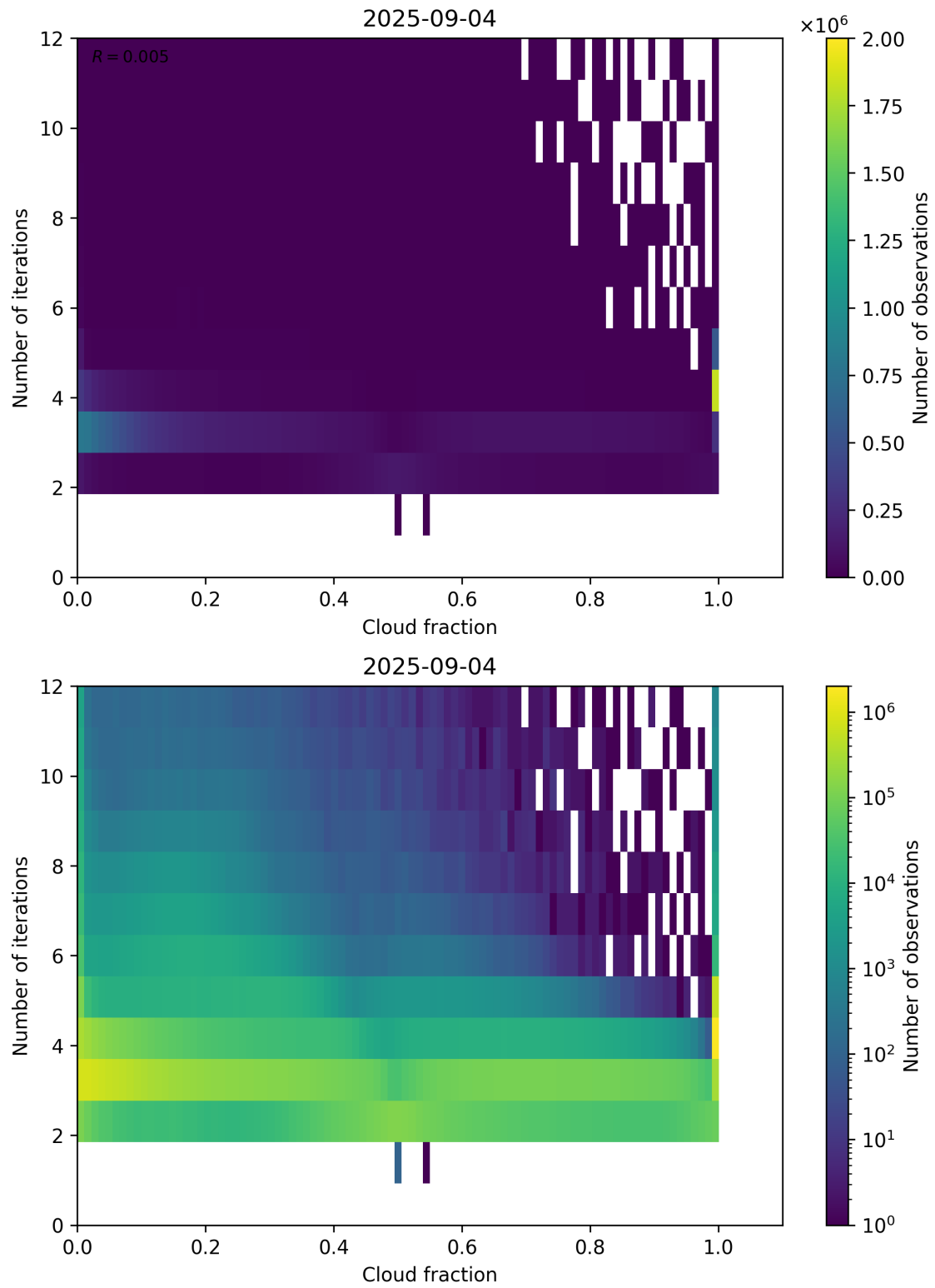
Figure 73: Scatter density plot of “Cloud fraction” against “Number of iterations” for 2025-09-04 to 2025-09-05.
