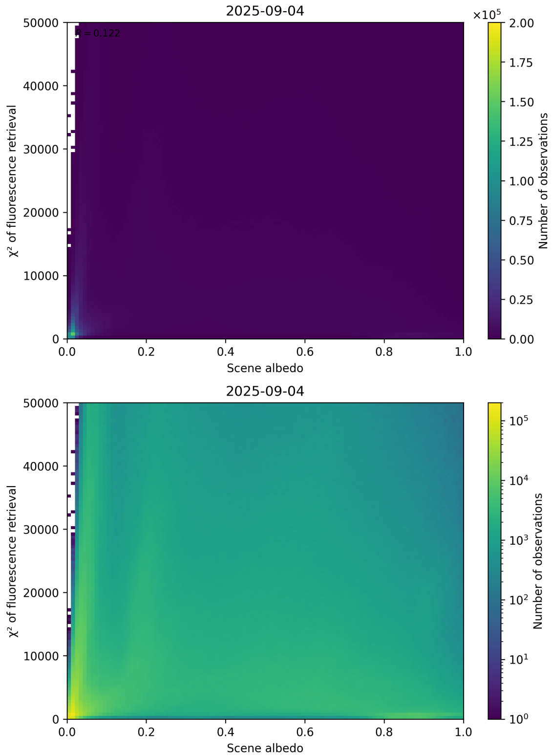
Figure 103: Scatter density plot of “Scene albedo” against “ \chi^2 of fluorescence retrieval” for 2025-09-04 to 2025-09-05.
