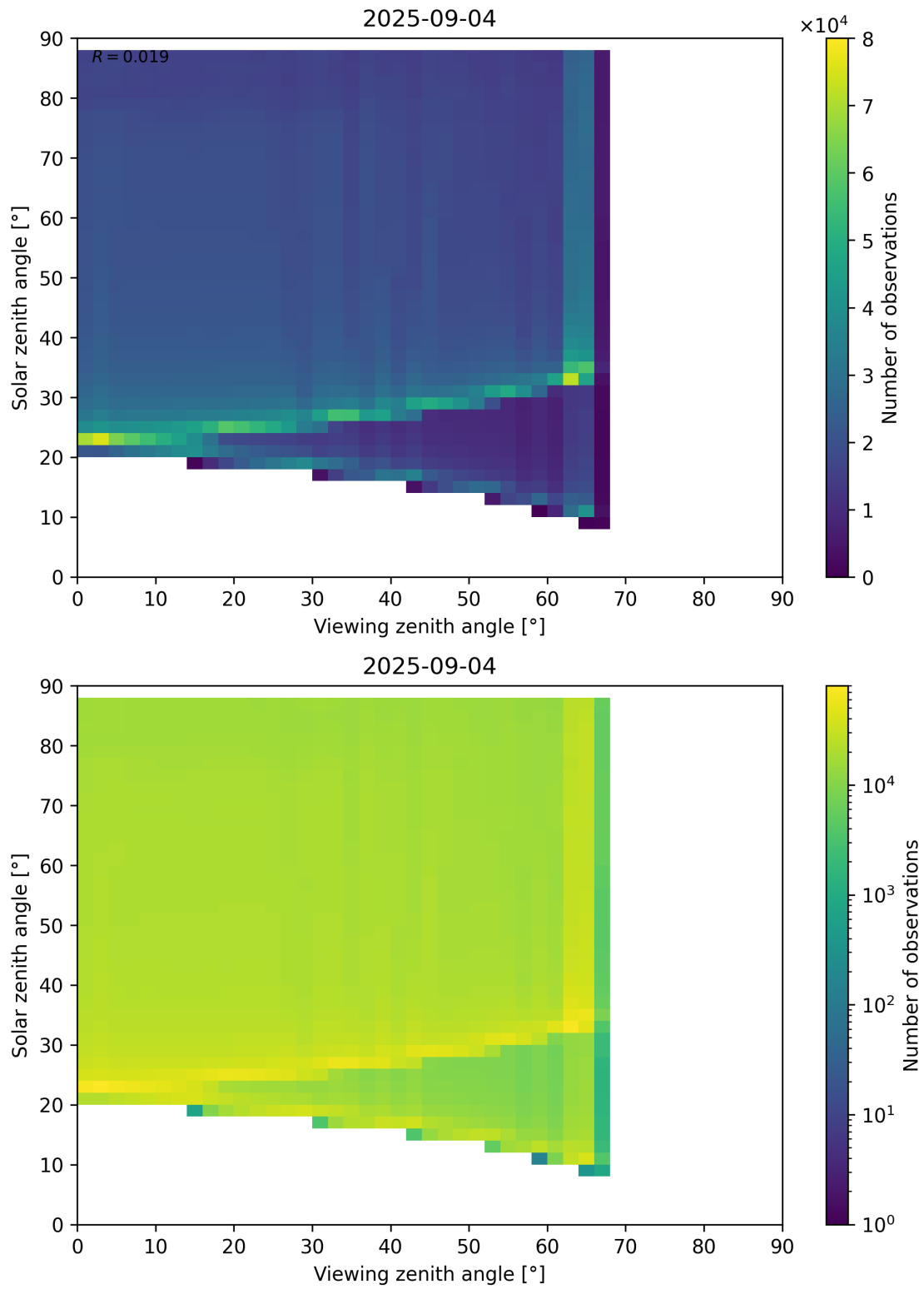
Figure 127: Scatter density plot of “Viewing zenith angle” against “Solar zenith angle” for 2025-09-04 to 2025-09-05.
