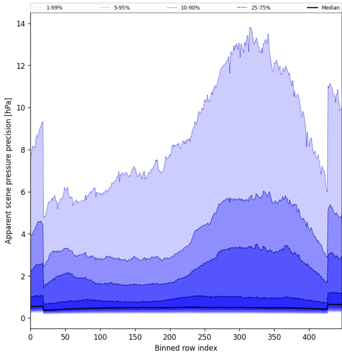
Figure 54: Along track statistics of “Apparent scene pressure precision” for 2025-09-04 to 2025-09-05
