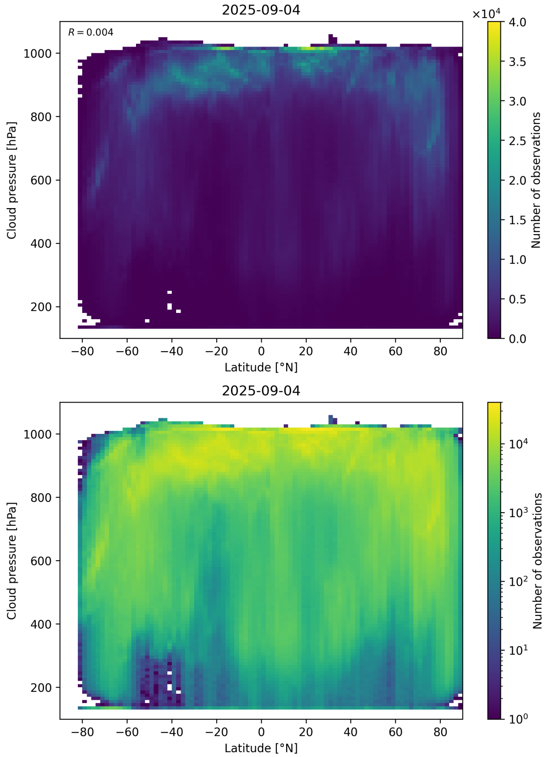
Figure 91: Scatter density plot of “Latitude” against “Cloud pressure” for 2025-09-04 to 2025-09-05.
