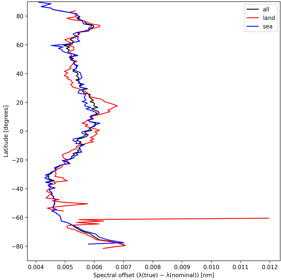
Figure 28: Zonal average of “Spectral offset ( \lambda_{\text{true}} - \lambda_{\text{nominal}} )” for 2025-09-04 to 2025-09-05.
