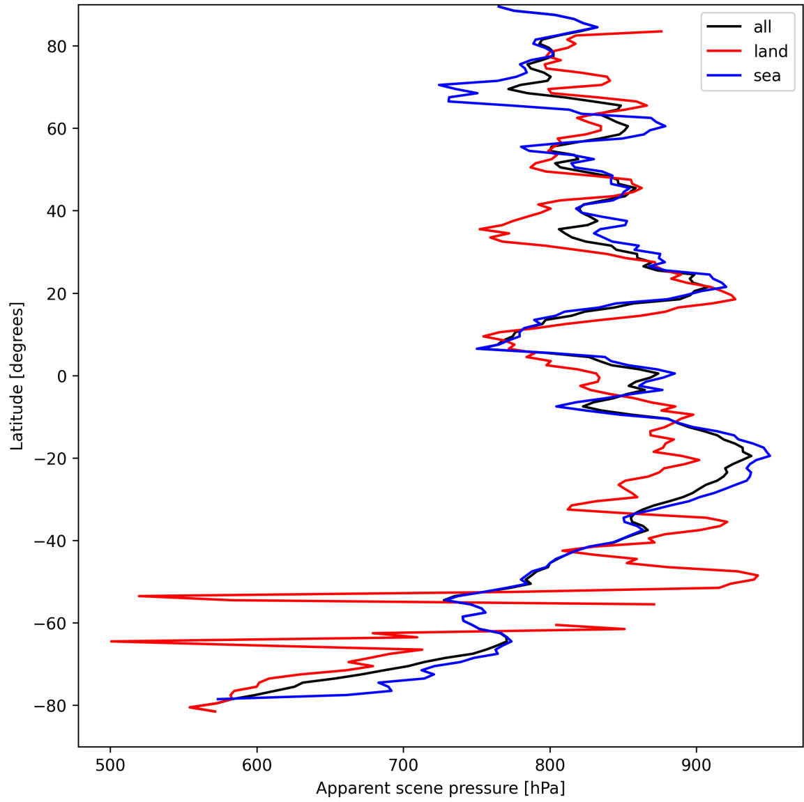
Figure 19: Zonal average of “Apparent scene pressure” for 2025-09-04 to 2025-09-05.
