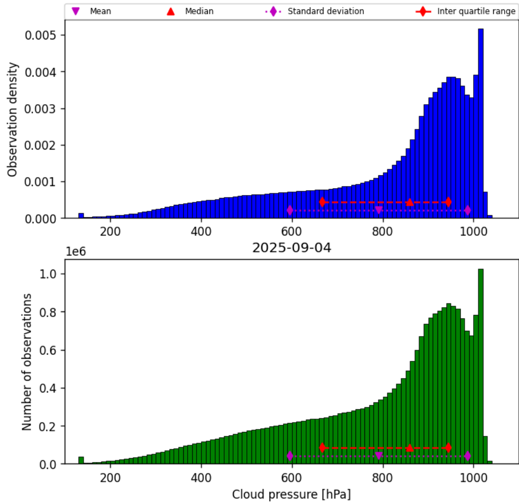
Figure 30: Histogram of “Cloud pressure” for 2025-09-04 to 2025-09-05
