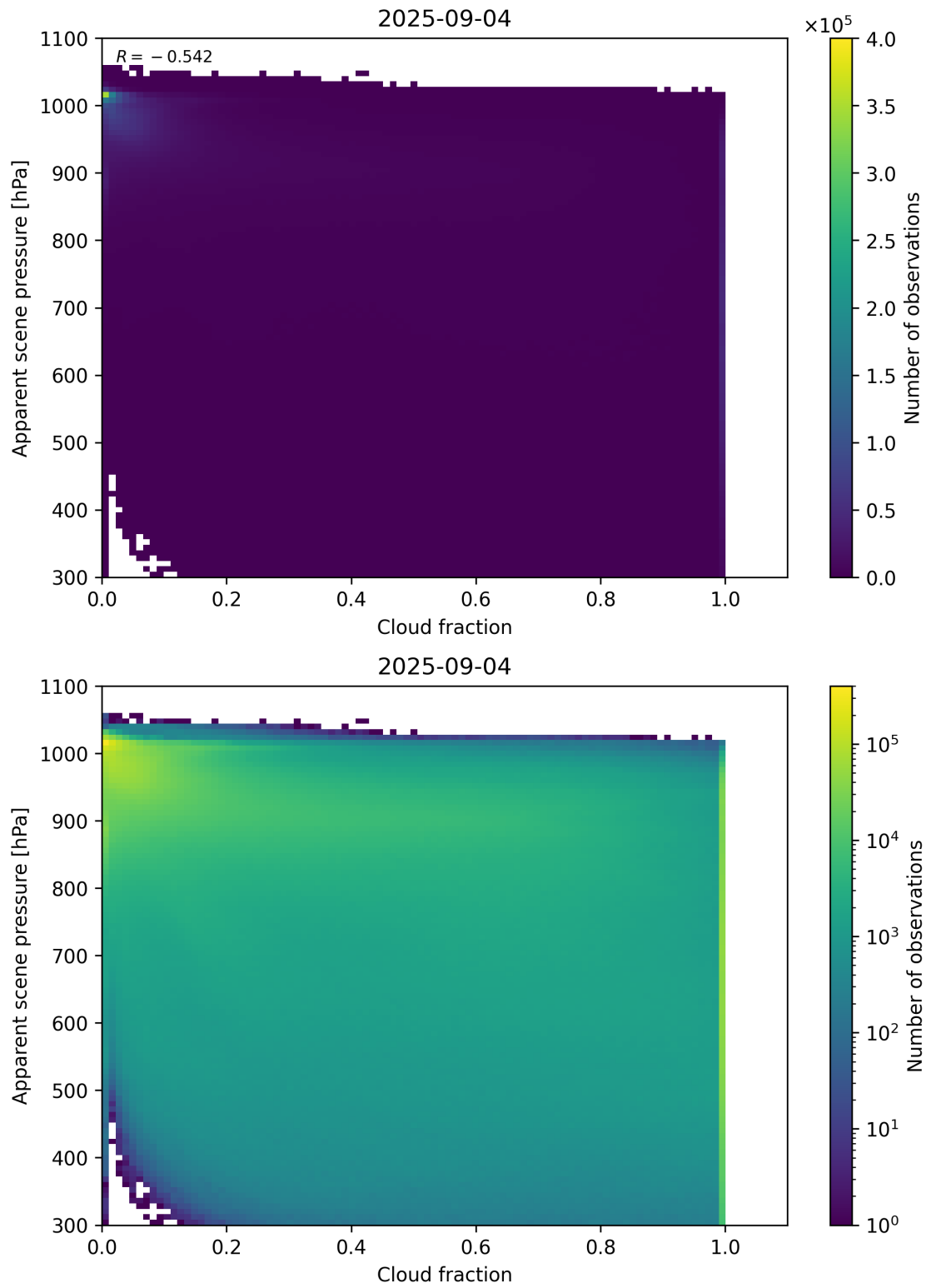
Figure 70: Scatter density plot of “Cloud fraction” against “Apparent scene pressure” for 2025-09-04 to 2025-09-05.
