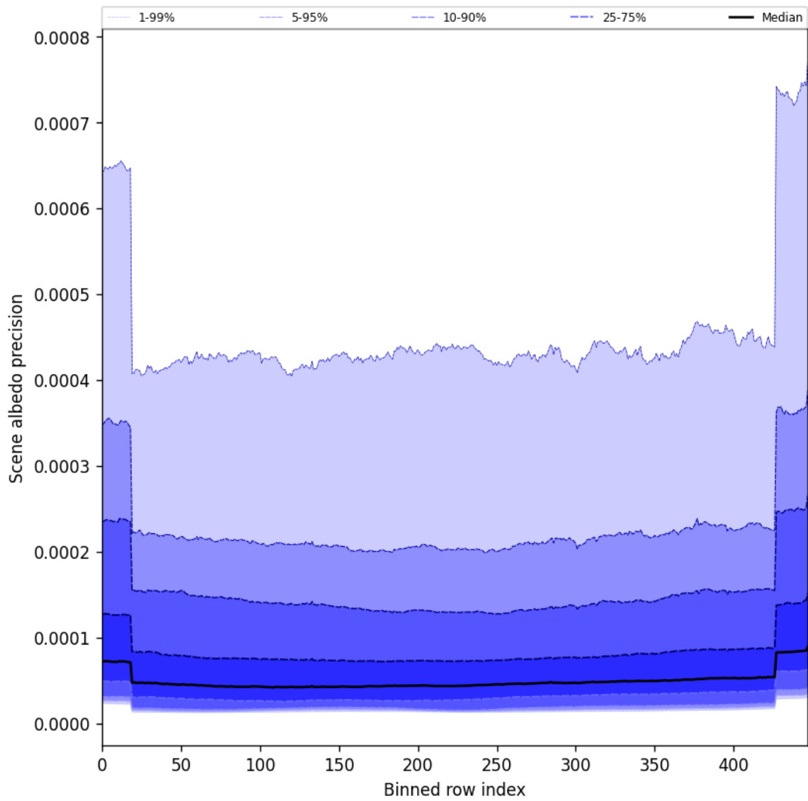
Figure 52: Along track statistics of “Scene albedo precision” for 2025-09-04 to 2025-09-05
