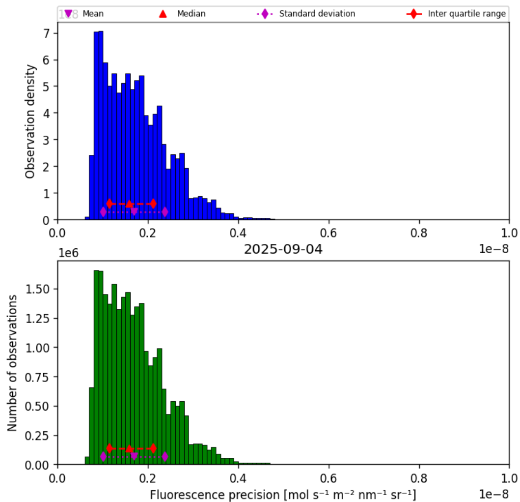
Figure 41: Histogram of “Fluorescence precision” for 2025-09-04 to 2025-09-05
