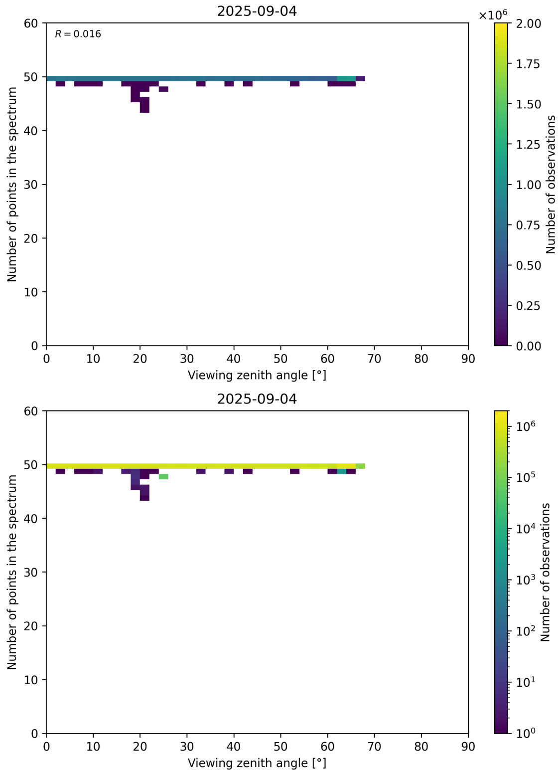
Figure 125: Scatter density plot of “Viewing zenith angle” against “Number of points in the spectrum” for 2025-09-04 to 2025-09-05.
