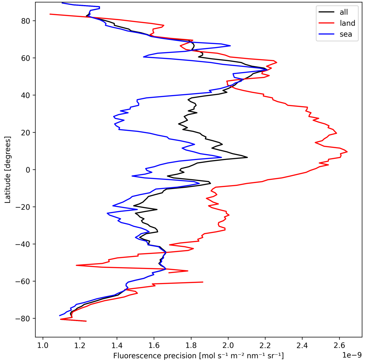
Figure 24: Zonal average of “Fluorescence precision” for 2025-09-04 to 2025-09-05.
