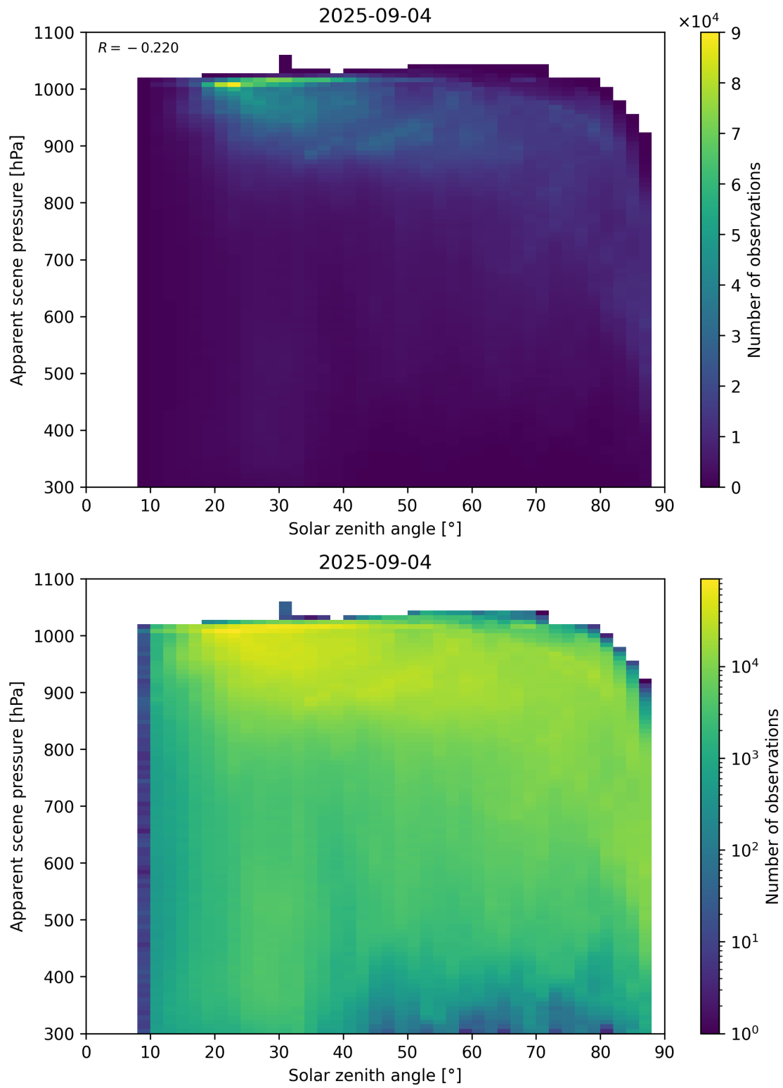
Figure 108: Scatter density plot of “Solar zenith angle” against “Apparent scene pressure” for 2025-09-04 to 2025-09-05.
