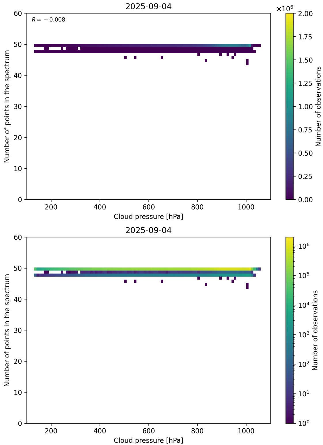
Figure 82: Scatter density plot of “Cloud pressure” against “Number of points in the spectrum” for 2025-09-04 to 2025-09-05.
