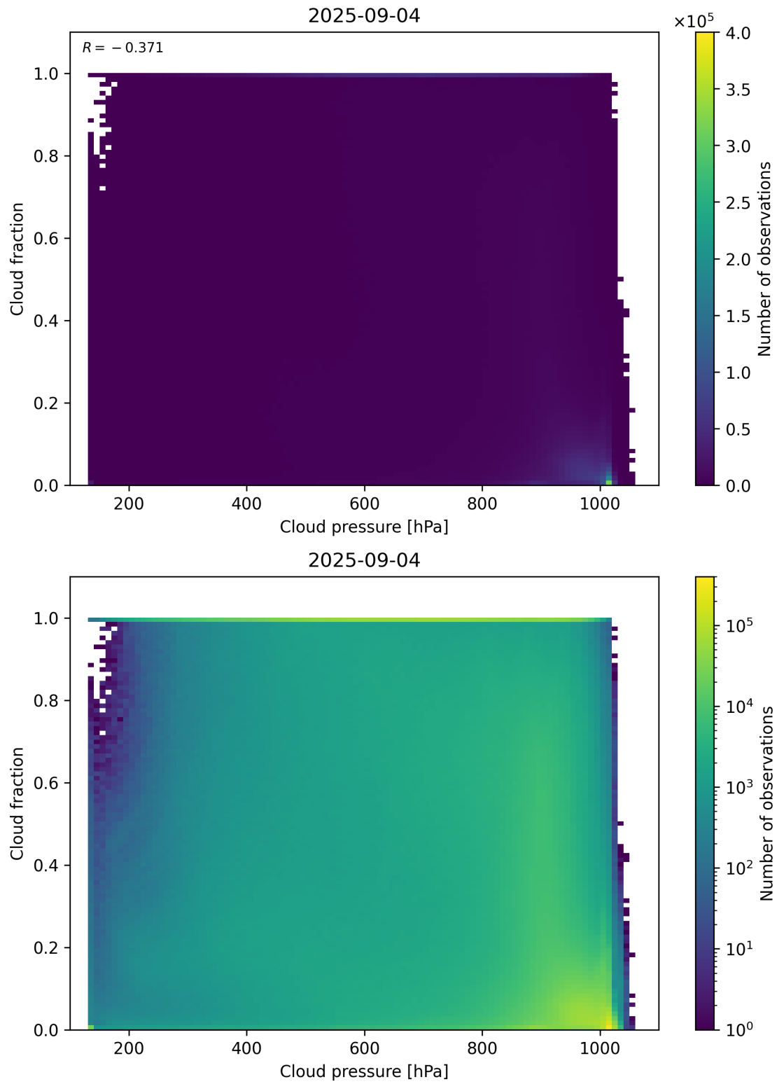
Figure 79: Scatter density plot of “Cloud pressure” against “Cloud fraction” for 2025-09-04 to 2025-09-05.
