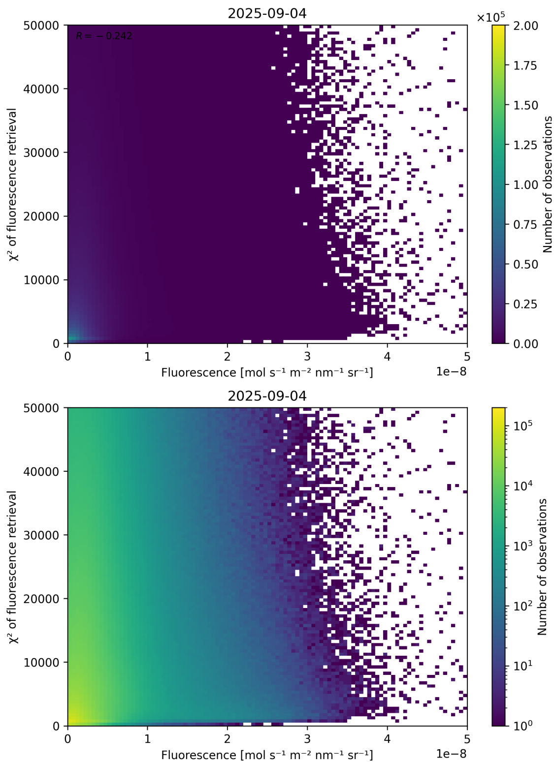
Figure 85: Scatter density plot of “Fluorescence” against “ \chi^2 of fluorescence retrieval” for 2025-09-04 to 2025-09-05.
