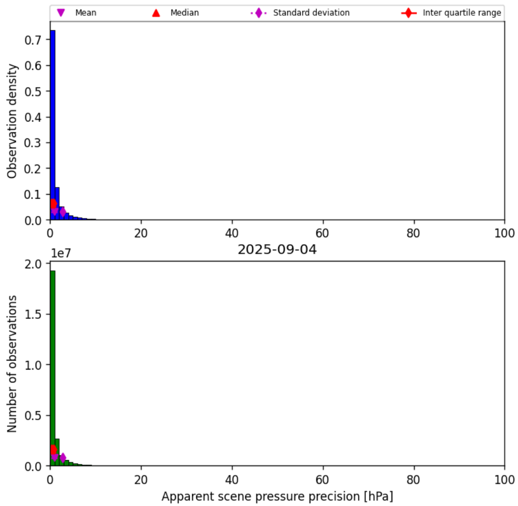
Figure 37: Histogram of “Apparent scene pressure precision” for 2025-09-04 to 2025-09-05
