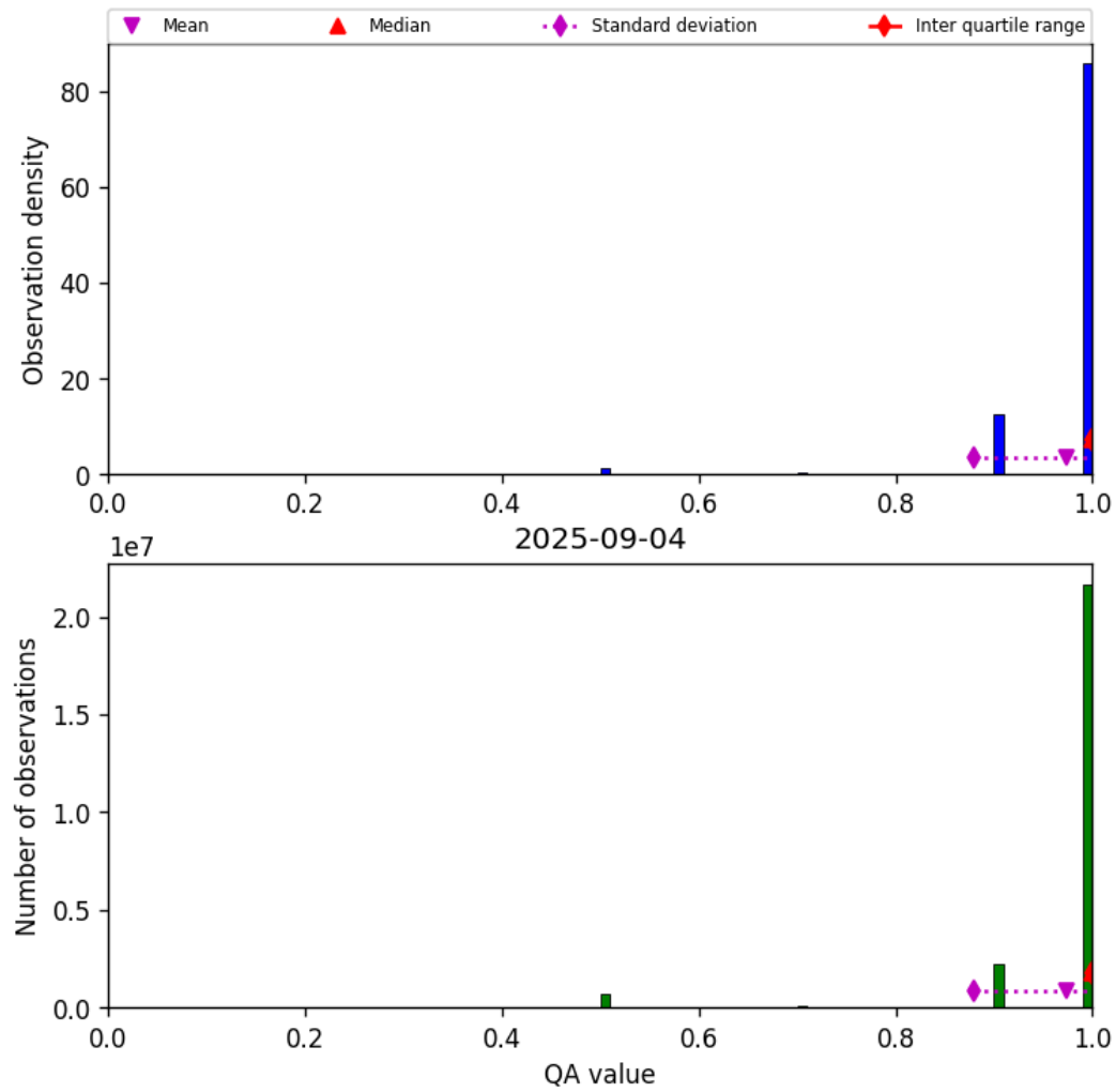
Figure 29: Histogram of “QA value” for 2025-09-04 to 2025-09-05
