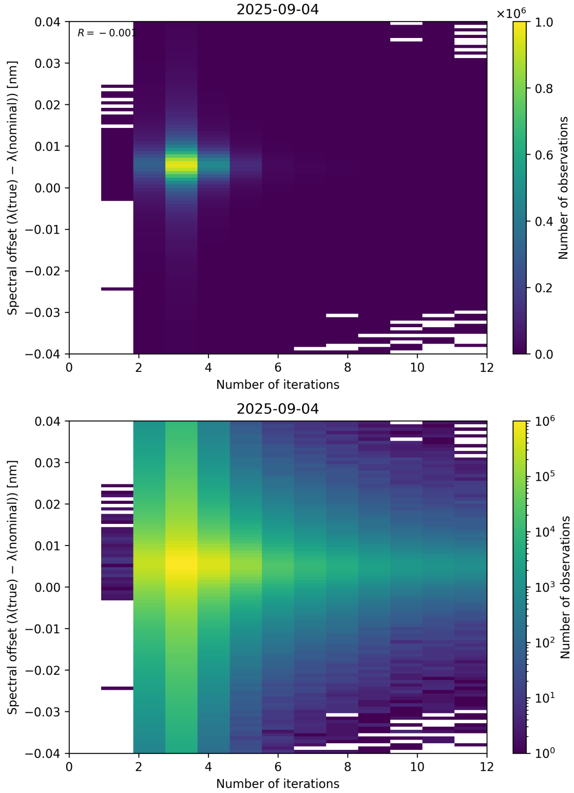
Figure 100: Scatter density plot of “Number of iterations” against “Spectral offset ( \lambda_{\text{true}} - \lambda_{\text{nominal}} )” for 2025-09-04 to 2025-09-05.
