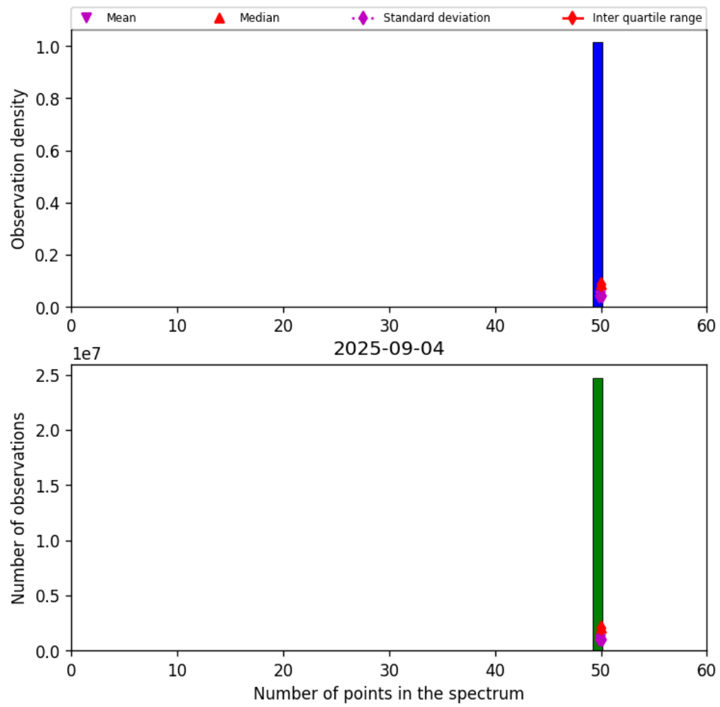
Figure 44: Histogram of “Number of points in the spectrum” for 2025-09-04 to 2025-09-05
