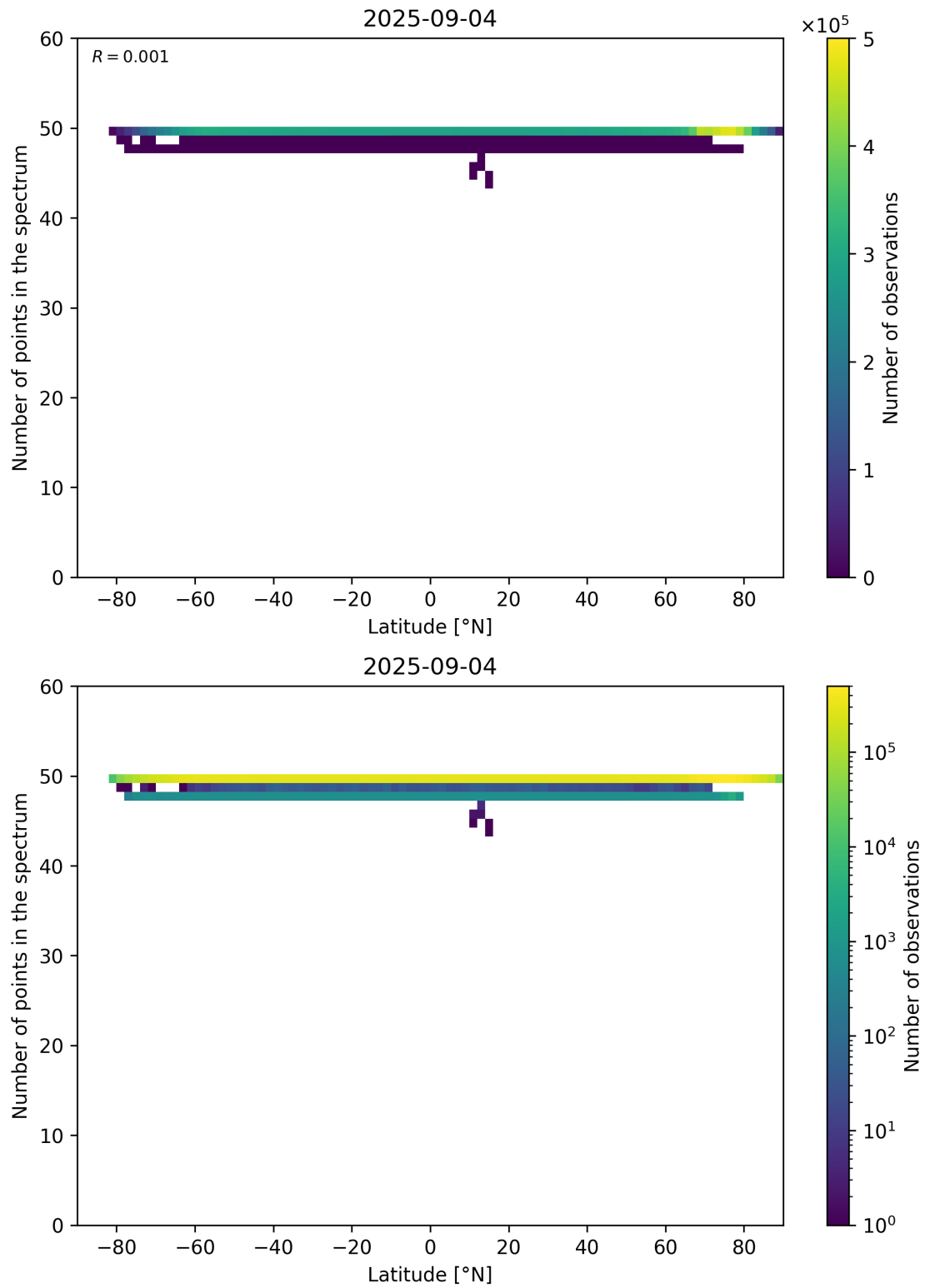
Figure 94: Scatter density plot of “Latitude” against “Number of points in the spectrum” for 2025-09-04 to 2025-09-05.
