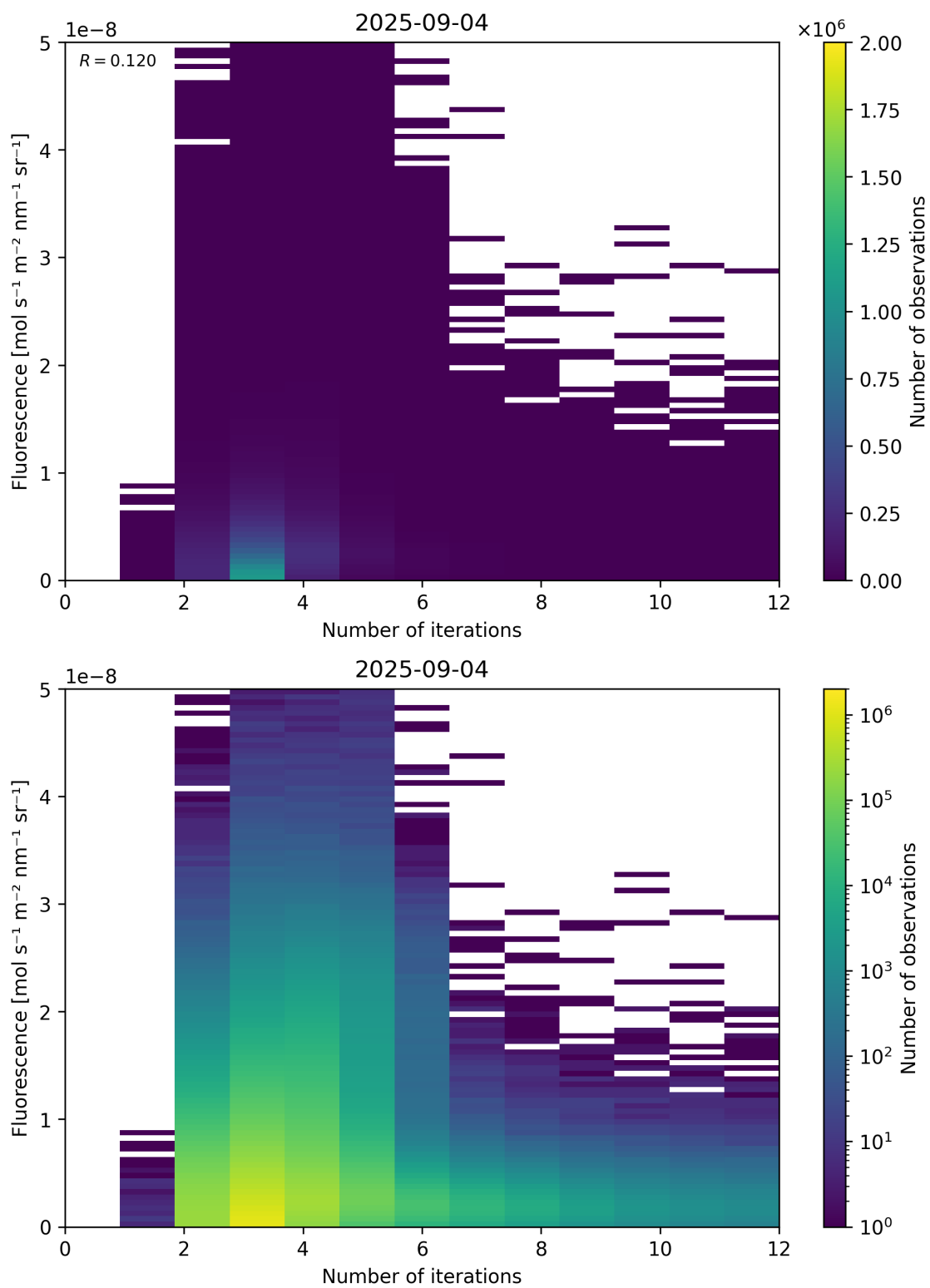
Figure 98: Scatter density plot of “Number of iterations” against “Fluorescence” for 2025-09-04 to 2025-09-05.
