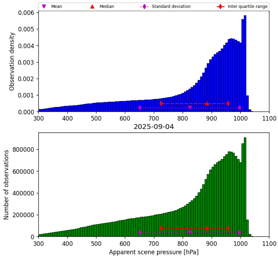
Figure 36: Histogram of “Apparent scene pressure” for 2025-09-04 to 2025-09-05
