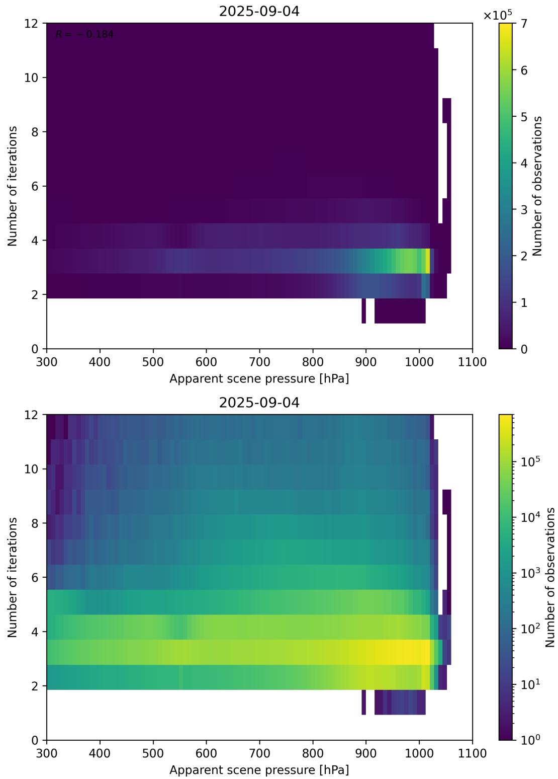
Figure 65: Scatter density plot of “Apparent scene pressure” against “Number of iterations” for 2025-09-04 to 2025-09-05.
