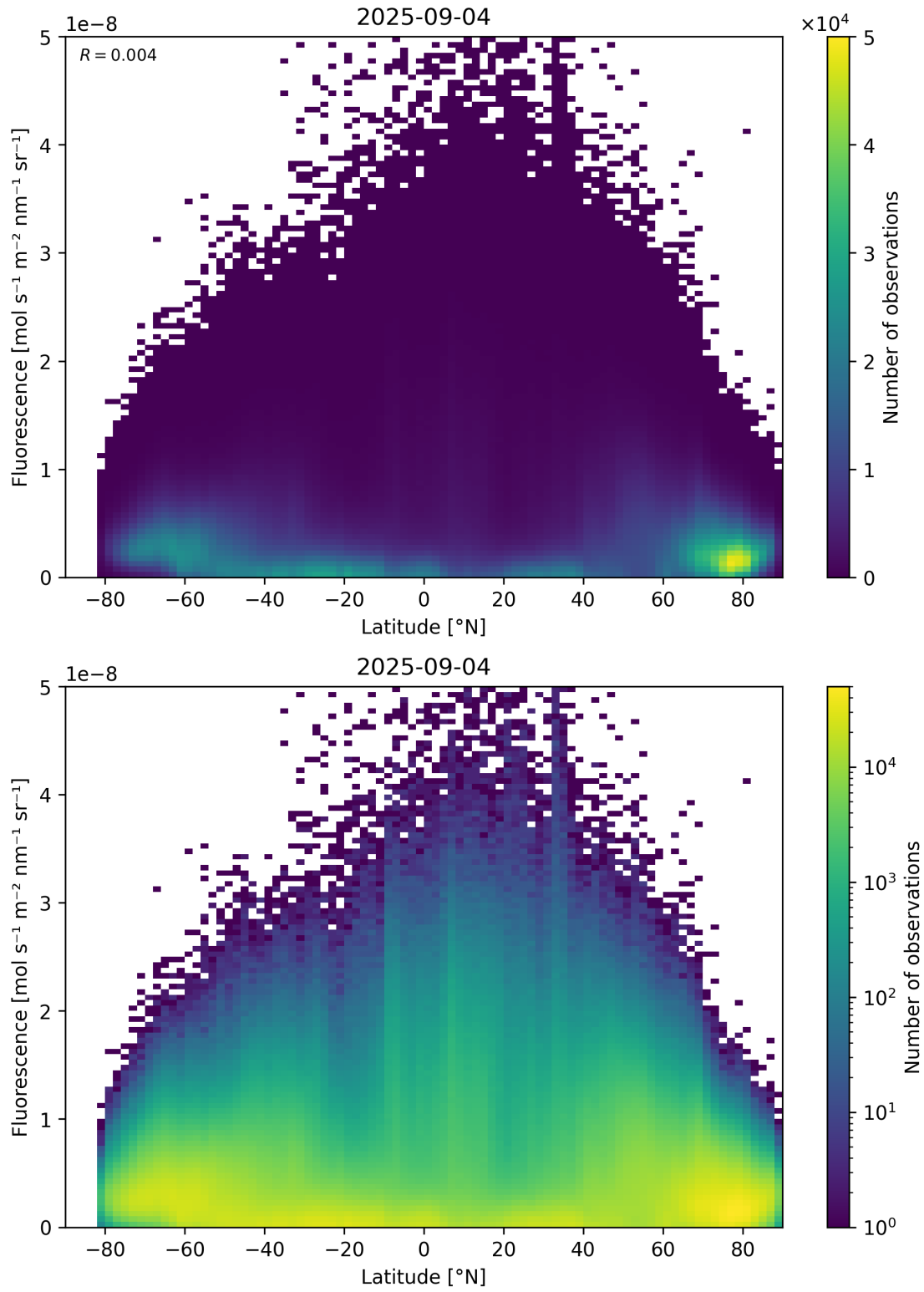
Figure 92: Scatter density plot of “Latitude” against “Fluorescence” for 2025-09-04 to 2025-09-05.
