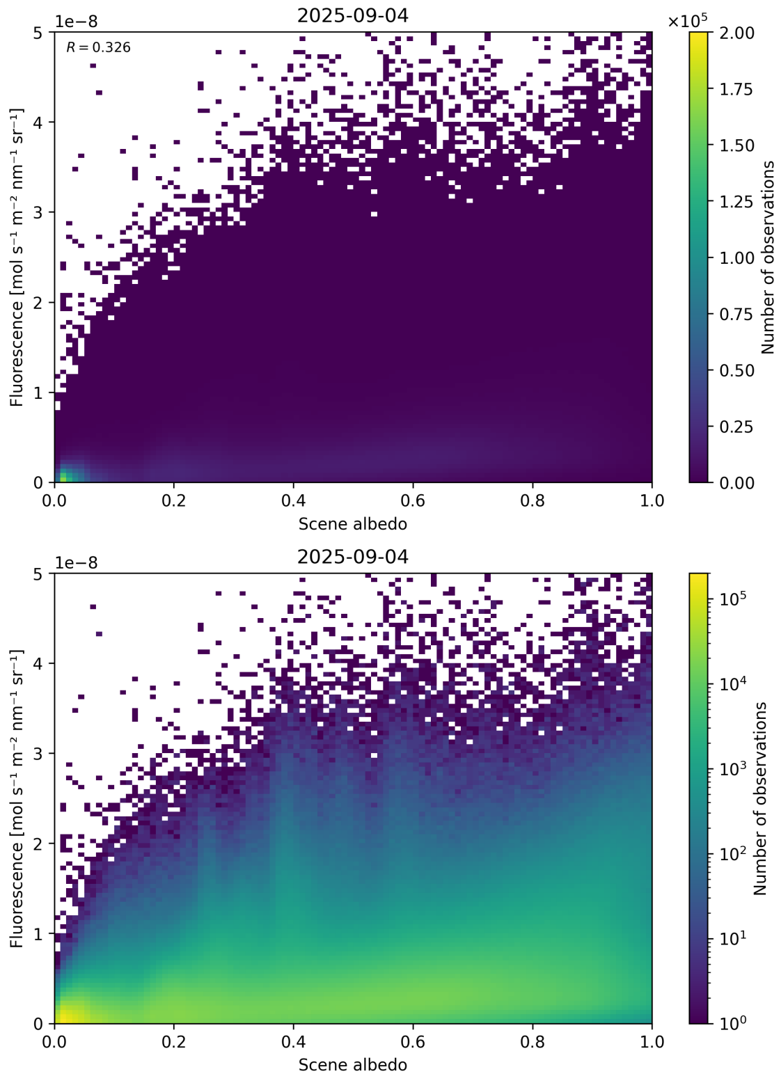
Figure 104: Scatter density plot of “Scene albedo” against “Fluorescence” for 2025-09-04 to 2025-09-05.
