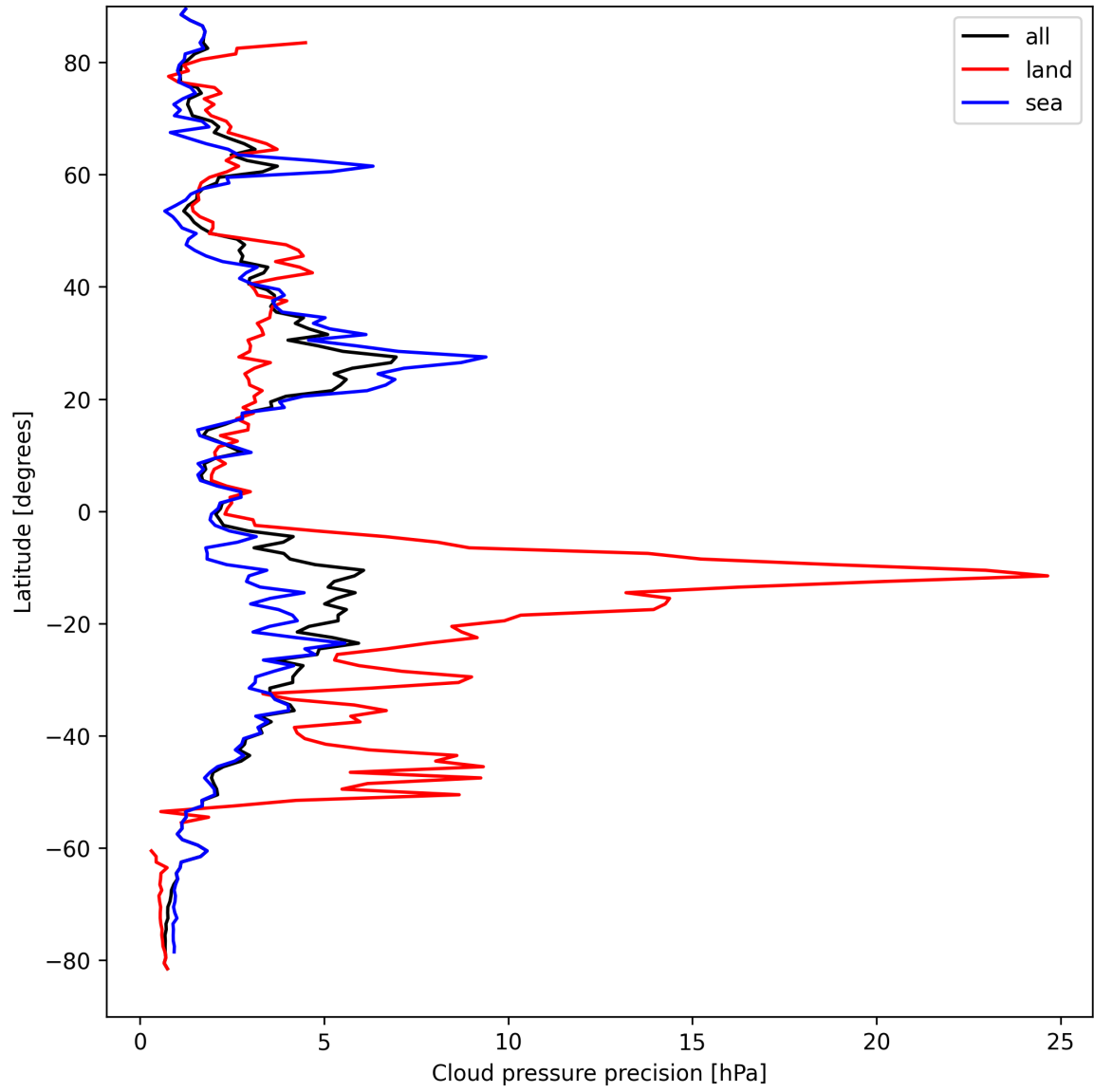
Figure 14: Zonal average of “Cloud pressure precision” for 2025-09-04 to 2025-09-05.
