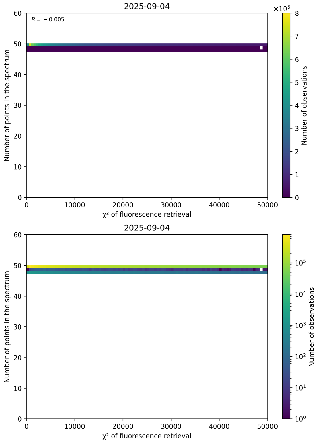
Figure 68: Scatter density plot of “ \chi^2 of fluorescence retrieval” against “Number of points in the spectrum” for 2025-09-04 to 2025-09-05.
