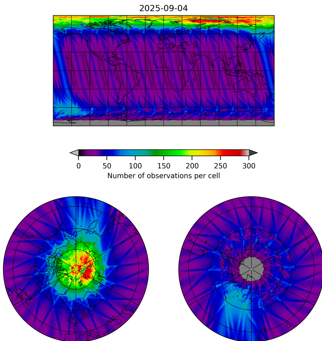
Figure 11: Map of the number of observations for 2025-09-04 to 2025-09-05
