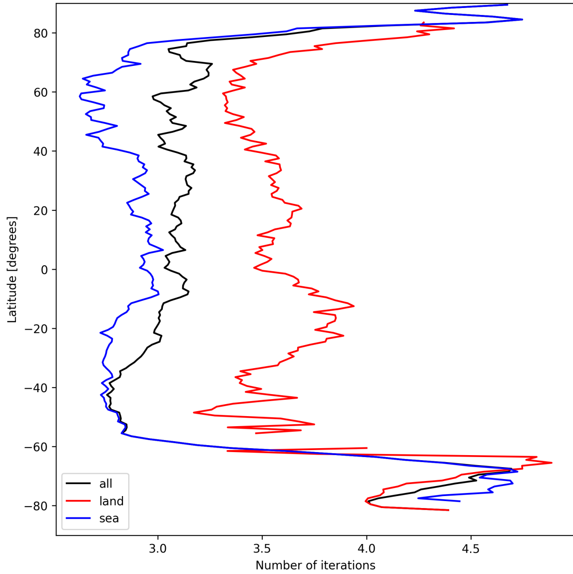
Figure 22: Zonal average of “Number of iterations” for 2025-09-04 to 2025-09-05.
