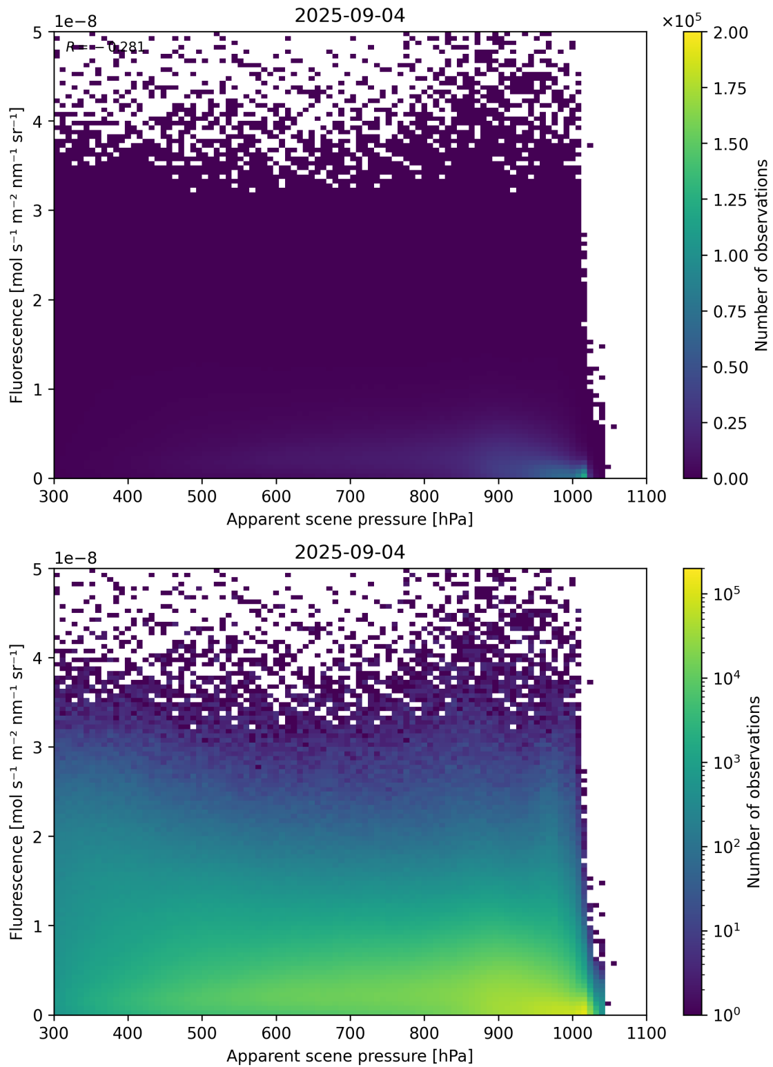
Figure 64: Scatter density plot of “Apparent scene pressure” against “Fluorescence” for 2025-09-04 to 2025-09-05.
