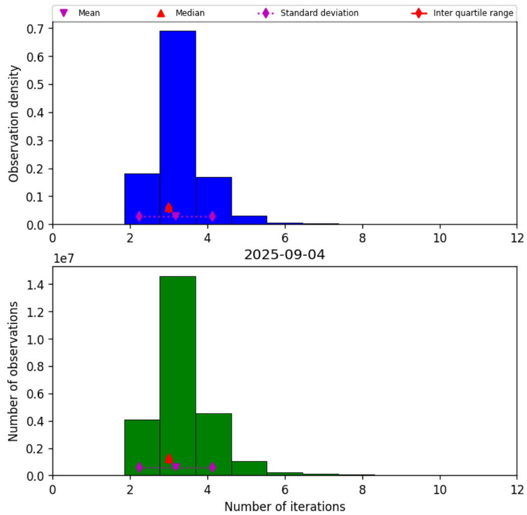
Figure 39: Histogram of “Number of iterations” for 2025-09-04 to 2025-09-05
