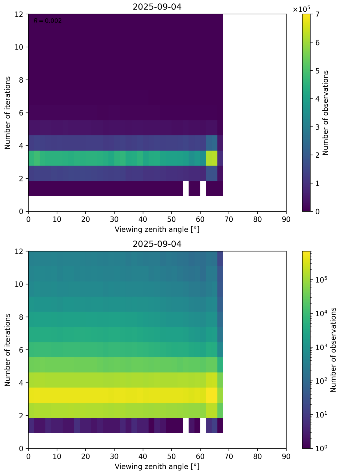
Figure 124: Scatter density plot of “Viewing zenith angle” against “Number of iterations” for 2025-09-04 to 2025-09-05.
