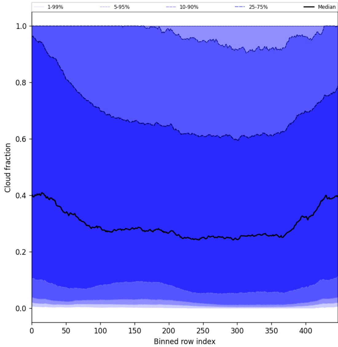
Figure 49: Along track statistics of “Cloud fraction” for 2025-09-04 to 2025-09-05
