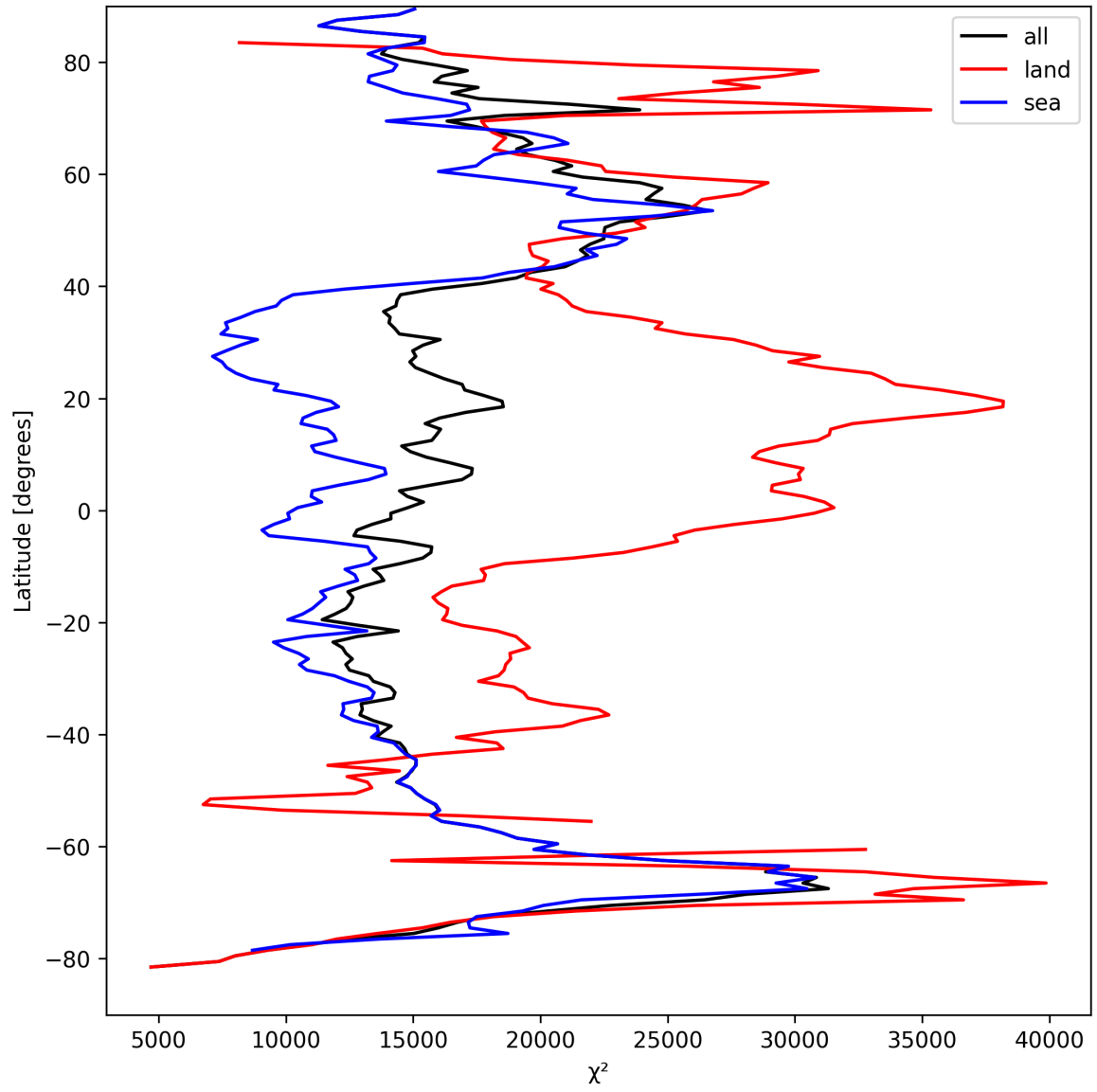
Figure 21: Zonal average of “ \chi^2 ” for 2025-09-04 to 2025-09-05.
