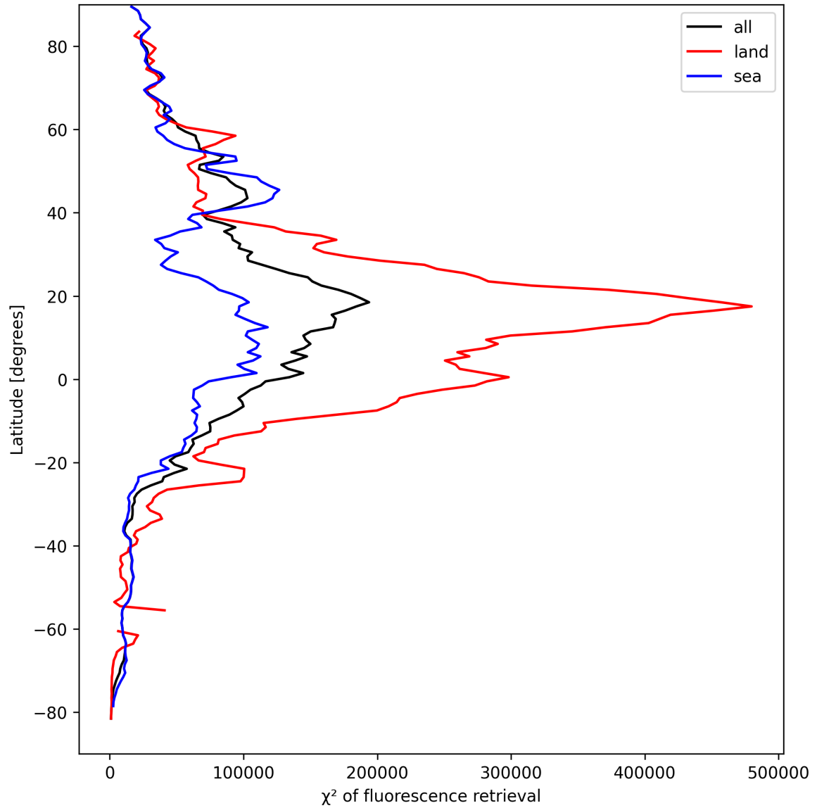
Figure 25: Zonal average of “ \chi^2 of fluorescence retrieval” for 2025-09-04 to 2025-09-05.
