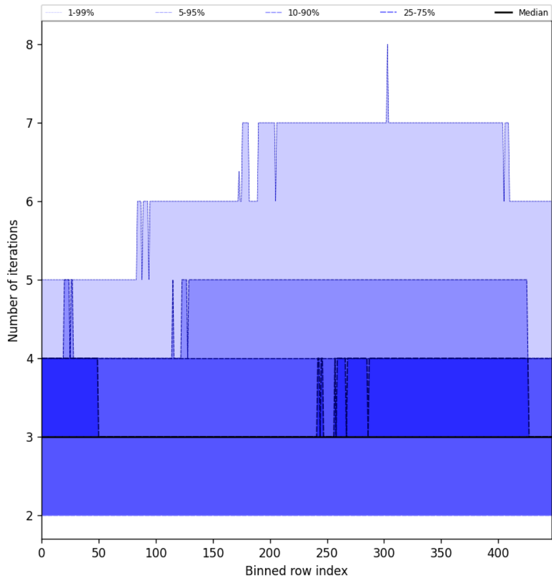
Figure 56: Along track statistics of “Number of iterations” for 2025-09-04 to 2025-09-05
