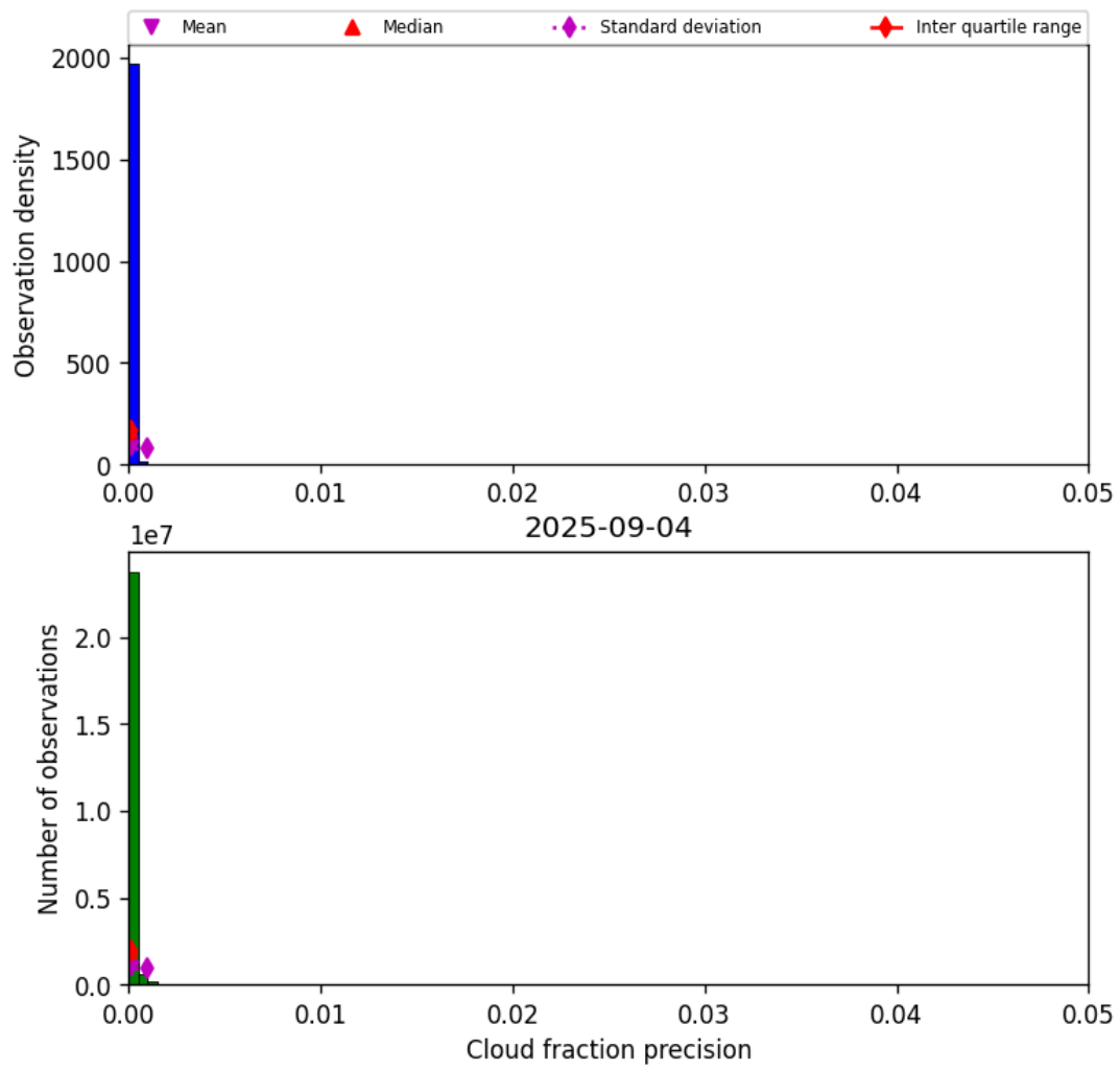
Figure 33: Histogram of “Cloud fraction precision” for 2025-09-04 to 2025-09-05
