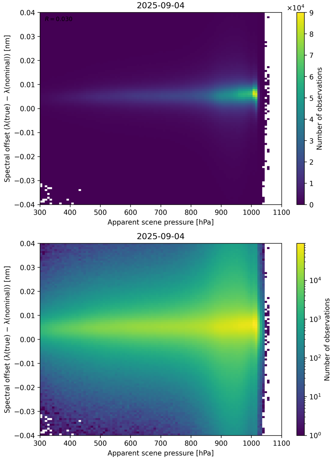
Figure 67: Scatter density plot of “Apparent scene pressure” against “Spectral offset ( \lambda_{\text{true}} - \lambda_{\text{nominal}} )” for 2025-09-04 to 2025-09-05.
