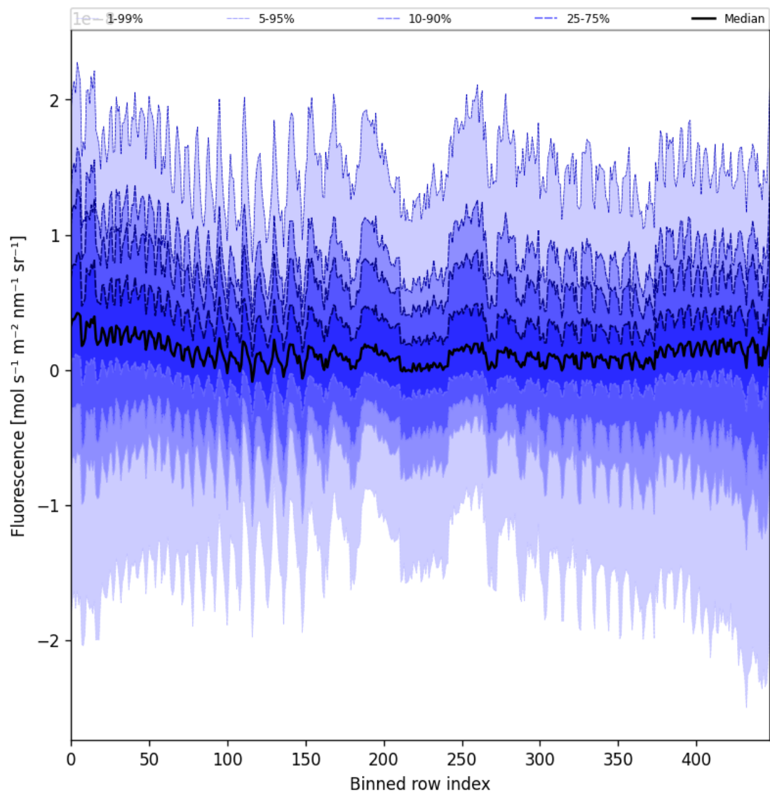
Figure 57: Along track statistics of “Fluorescence” for 2025-09-04 to 2025-09-05
