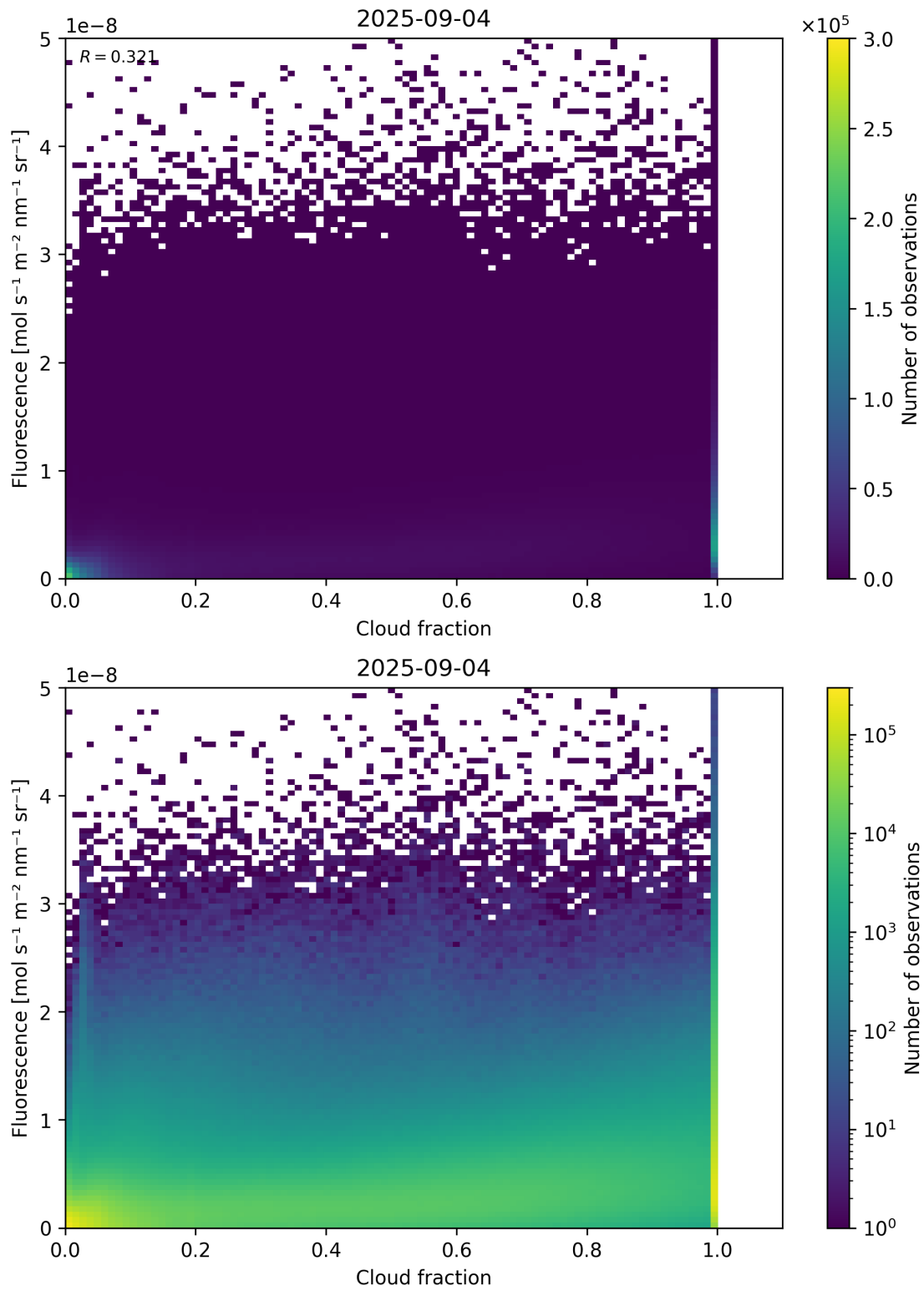
Figure 72: Scatter density plot of “Cloud fraction” against “Fluorescence” for 2025-09-04 to 2025-09-05.
