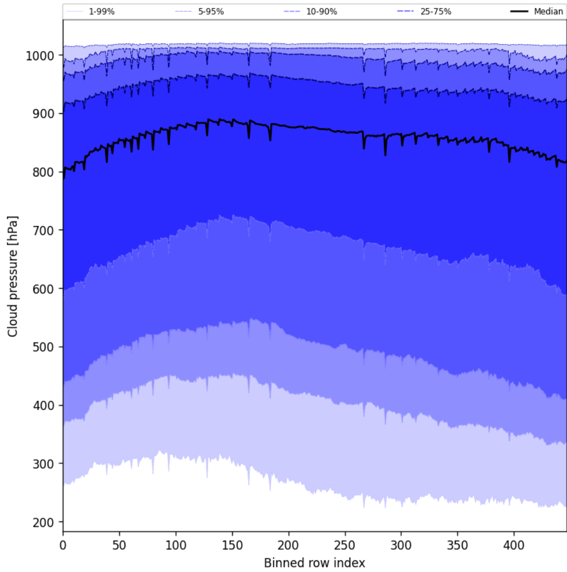
Figure 47: Along track statistics of “Cloud pressure” for 2025-09-04 to 2025-09-05
