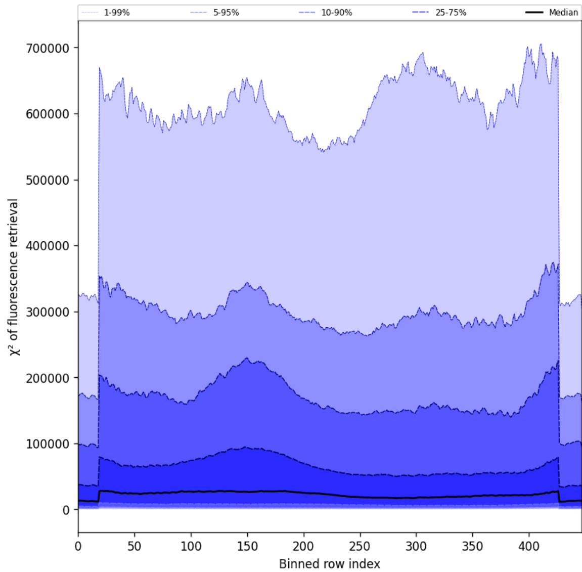
Figure 59: Along track statistics of “ \chi^2 of fluorescence retrieval” for 2025-09-04 to 2025-09-05
