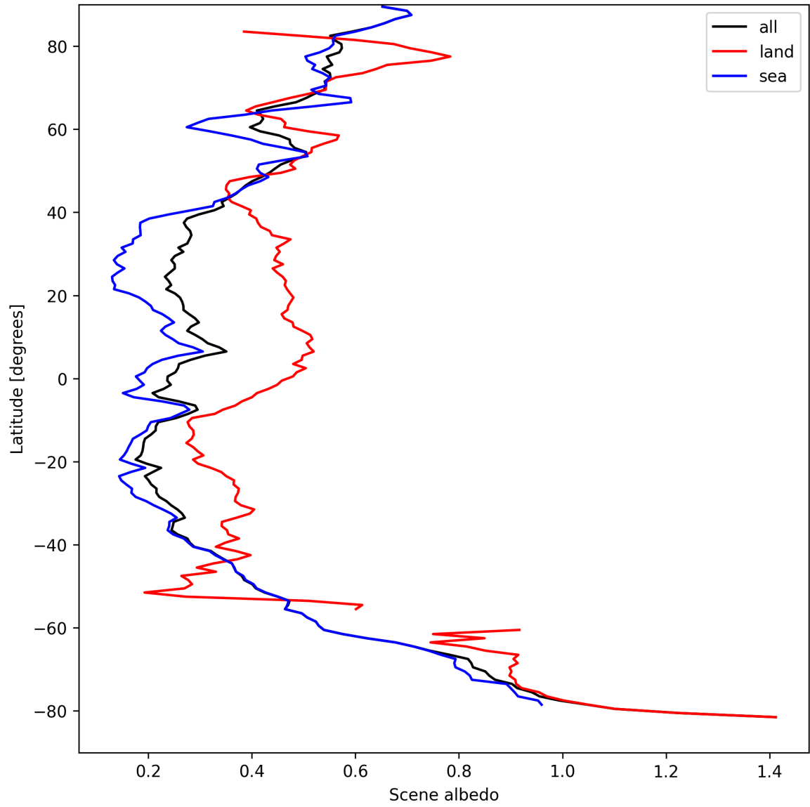
Figure 17: Zonal average of “Scene albedo” for 2025-09-04 to 2025-09-05.
