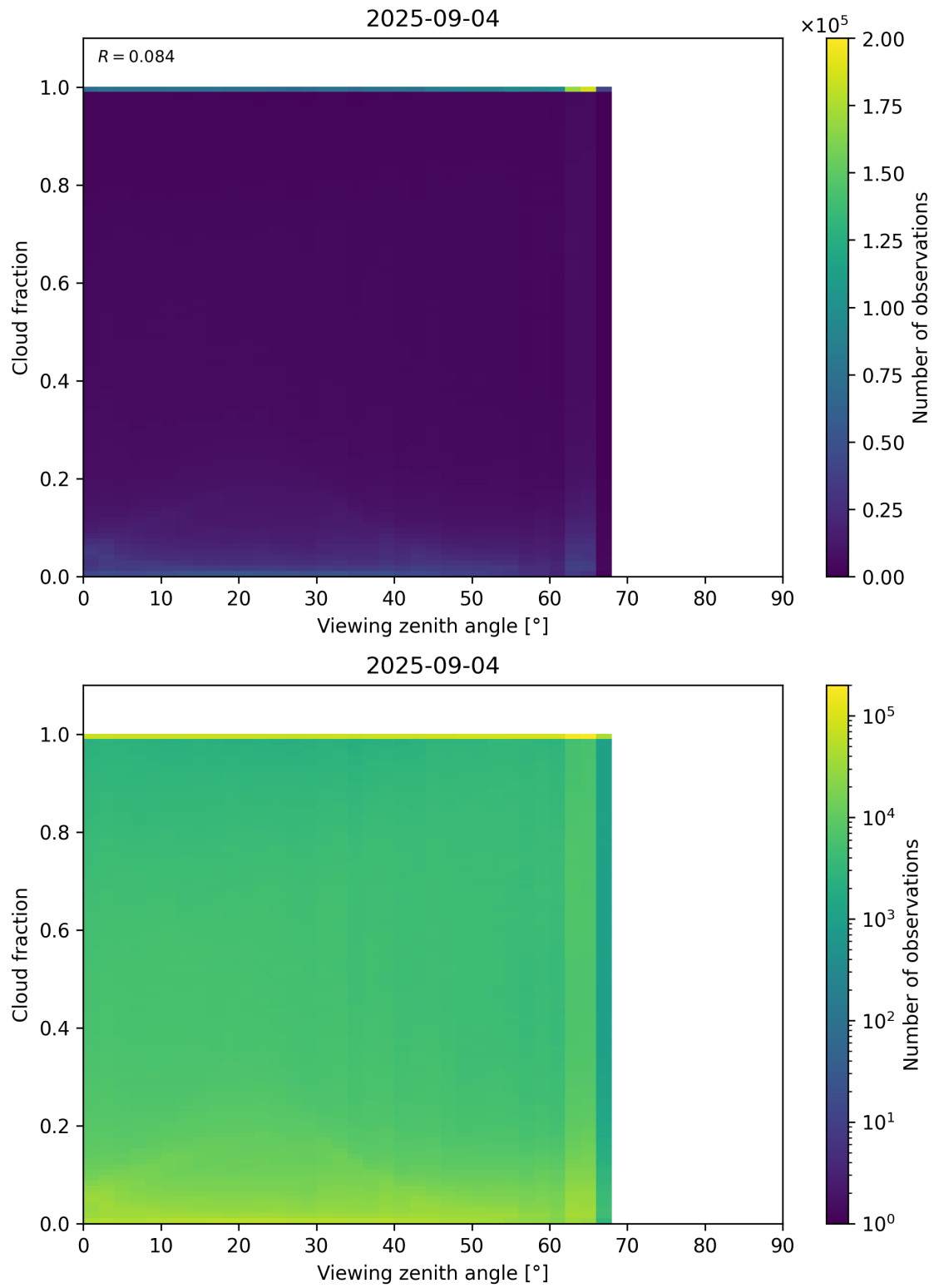
Figure 120: Scatter density plot of “Viewing zenith angle” against “Cloud fraction” for 2025-09-04 to 2025-09-05.
