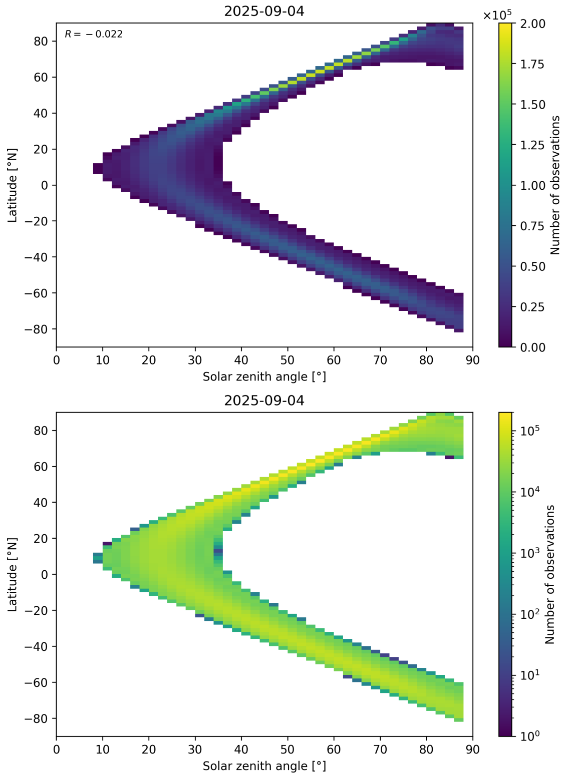
Figure 113: Scatter density plot of “Solar zenith angle” against “Latitude” for 2025-09-04 to 2025-09-05.
