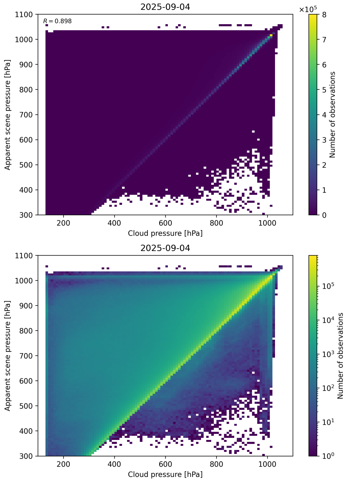
Figure 77: Scatter density plot of “Cloud pressure” against “Apparent scene pressure” for 2025-09-04 to 2025-09-05.
