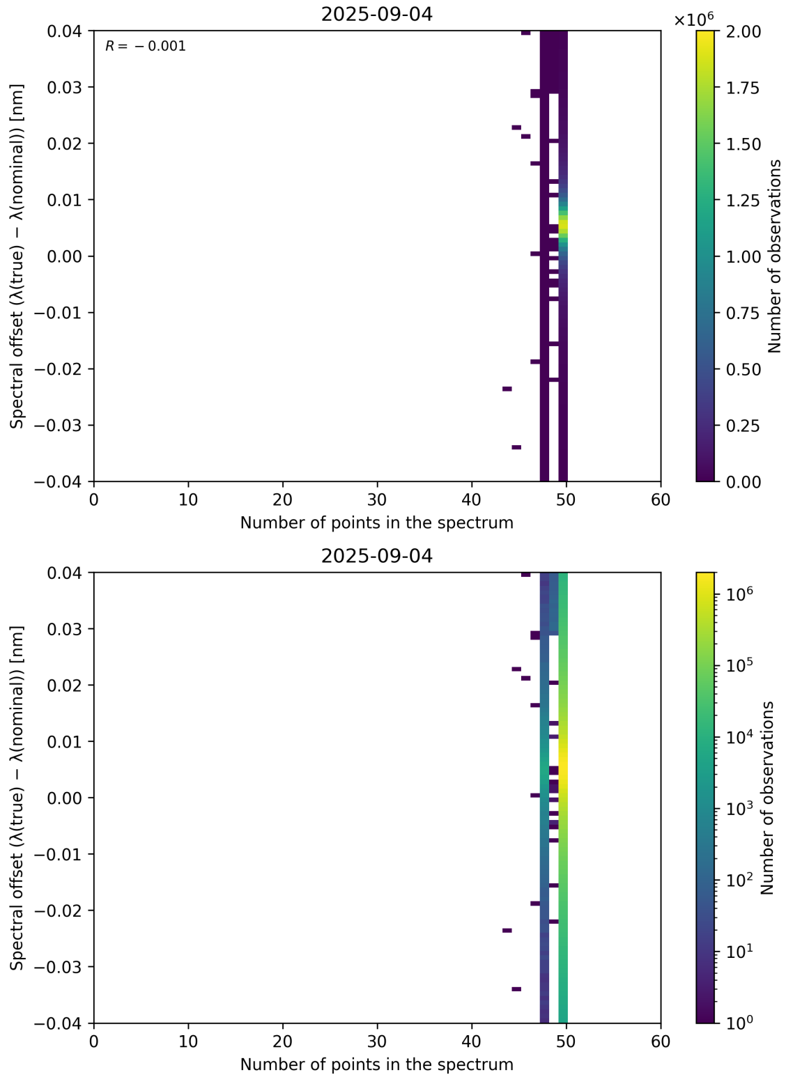
Figure 101: Scatter density plot of “Number of points in the spectrum” against “Spectral offset ( \lambda_{\text{true}} - \lambda_{\text{nominal}} )” for 2025-09-04 to 2025-09-05.
