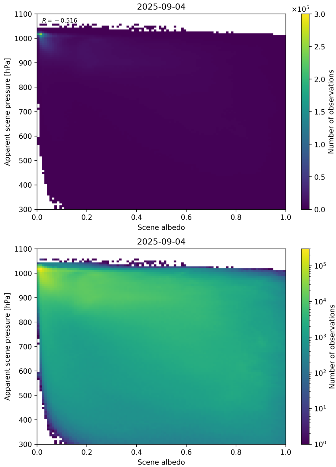
Figure 102: Scatter density plot of “Scene albedo” against “Apparent scene pressure” for 2025-09-04 to 2025-09-05.
