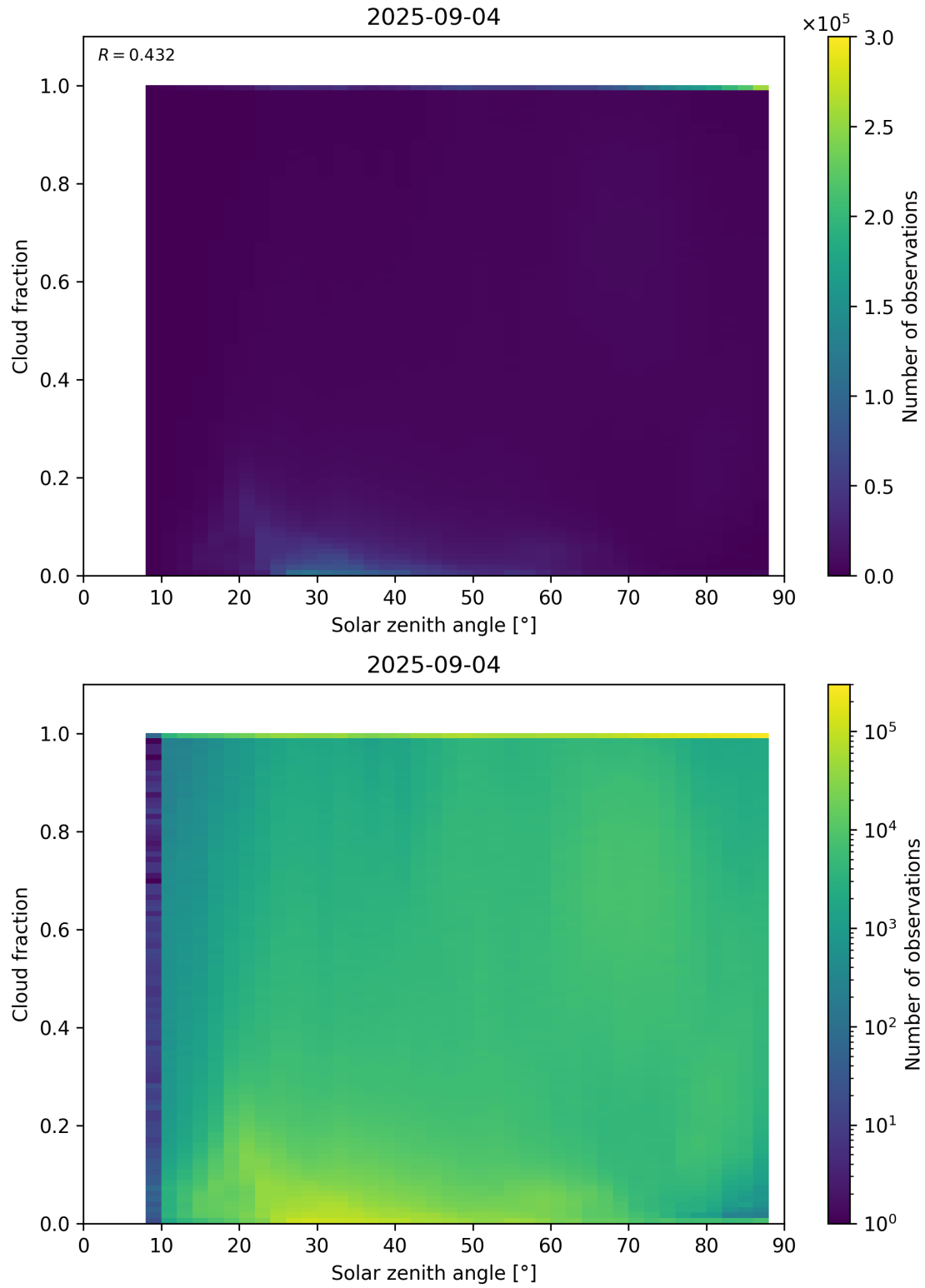
Figure 110: Scatter density plot of “Solar zenith angle” against “Cloud fraction” for 2025-09-04 to 2025-09-05.
