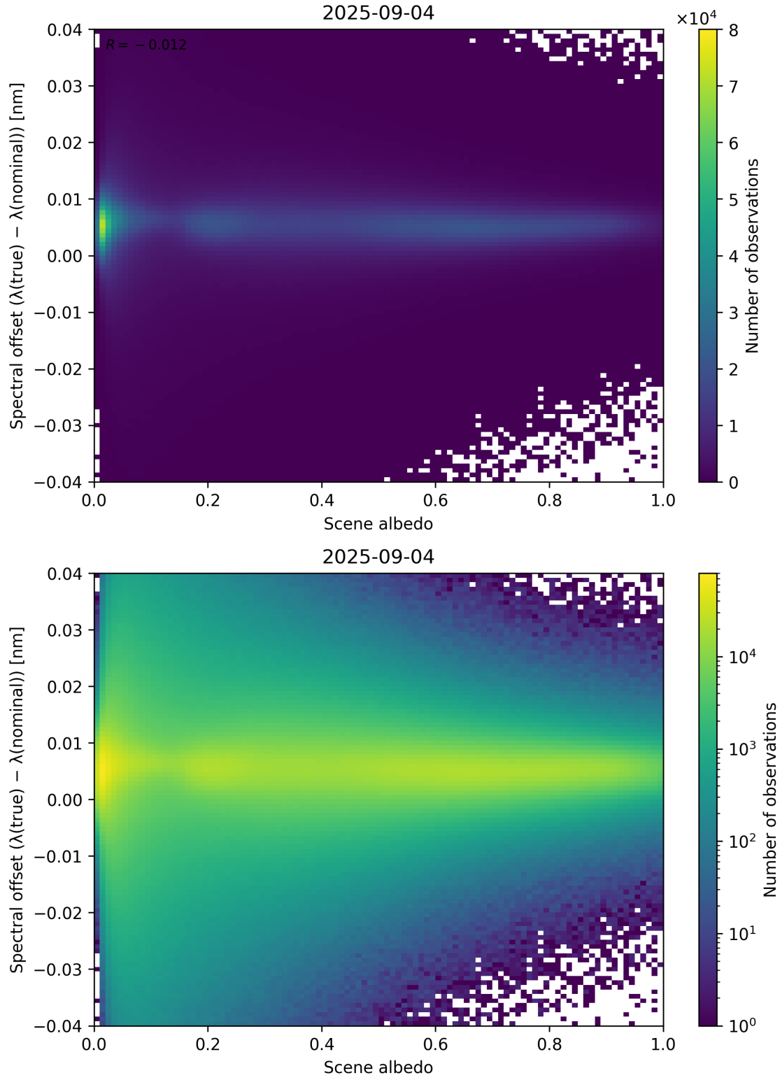
Figure 107: Scatter density plot of “Scene albedo” against “Spectral offset ( \lambda_{\text{true}} - \lambda_{\text{nominal}} )” for 2025-09-04 to 2025-09-05.
