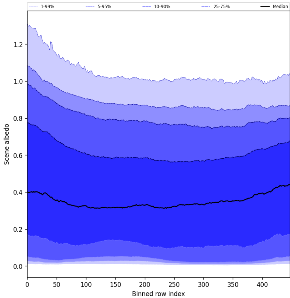
Figure 51: Along track statistics of “Scene albedo” for 2025-09-04 to 2025-09-05
