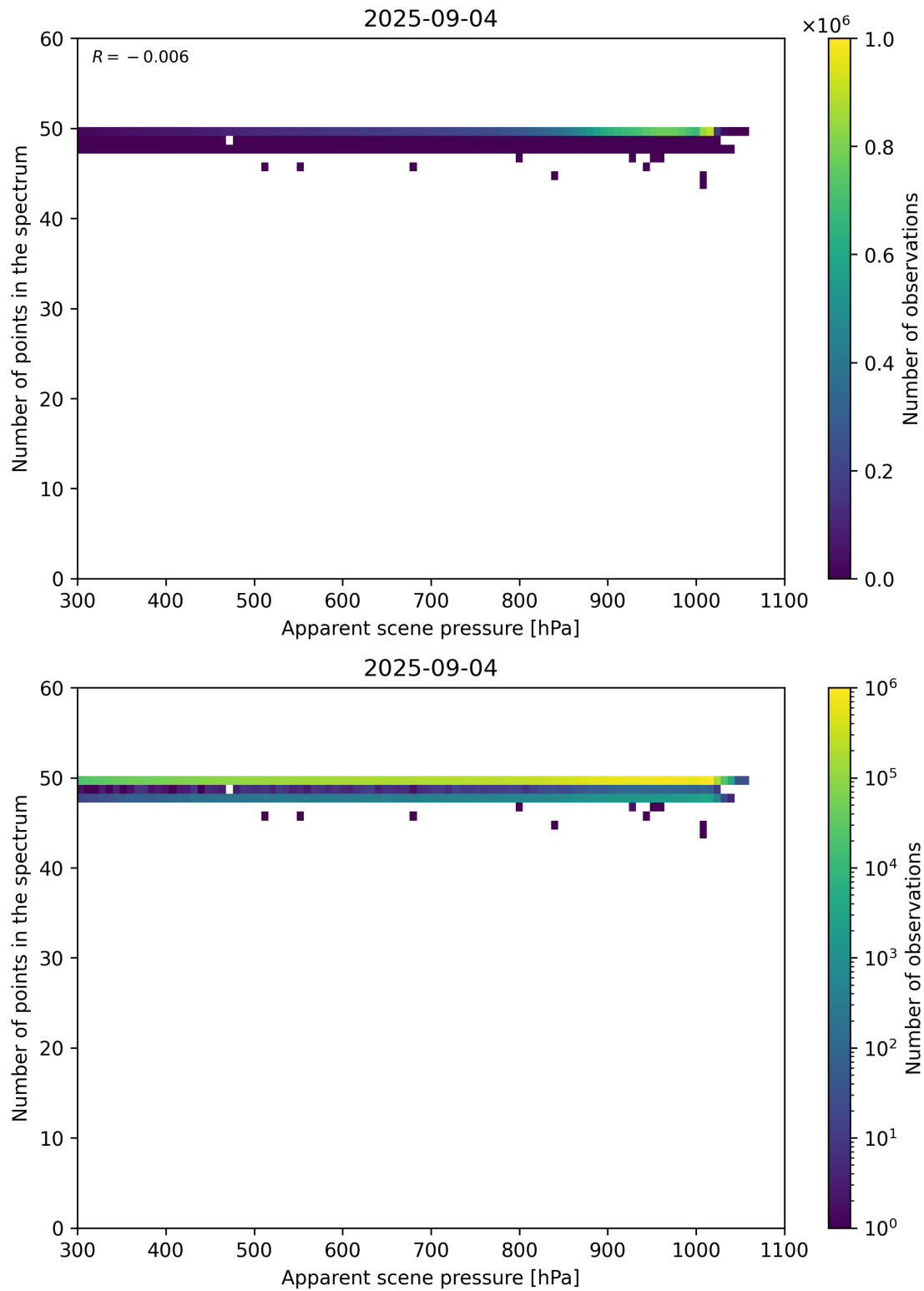
Figure 66: Scatter density plot of “Apparent scene pressure” against “Number of points in the spectrum” for 2025-09-04 to 2025-09-05.
