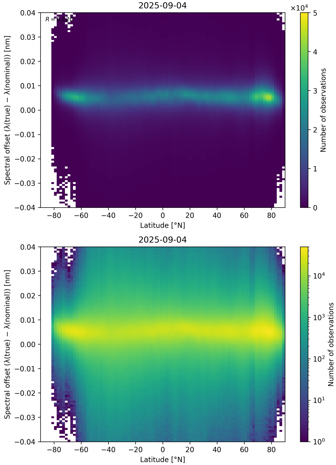
Figure 96: Scatter density plot of “Latitude” against “Spectral offset ( \lambda_{\text{true}} - \lambda_{\text{nominal}} )” for 2025-09-04 to 2025-09-05.
