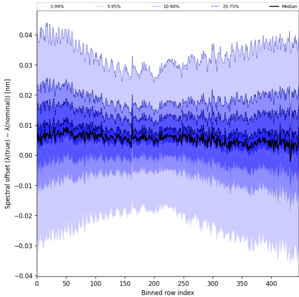
Figure 62: Along track statistics of “Spectral offset ( \lambda_{\text{true}} - \lambda_{\text{nominal}} )” for 2025-09-04 to 2025-09-05
