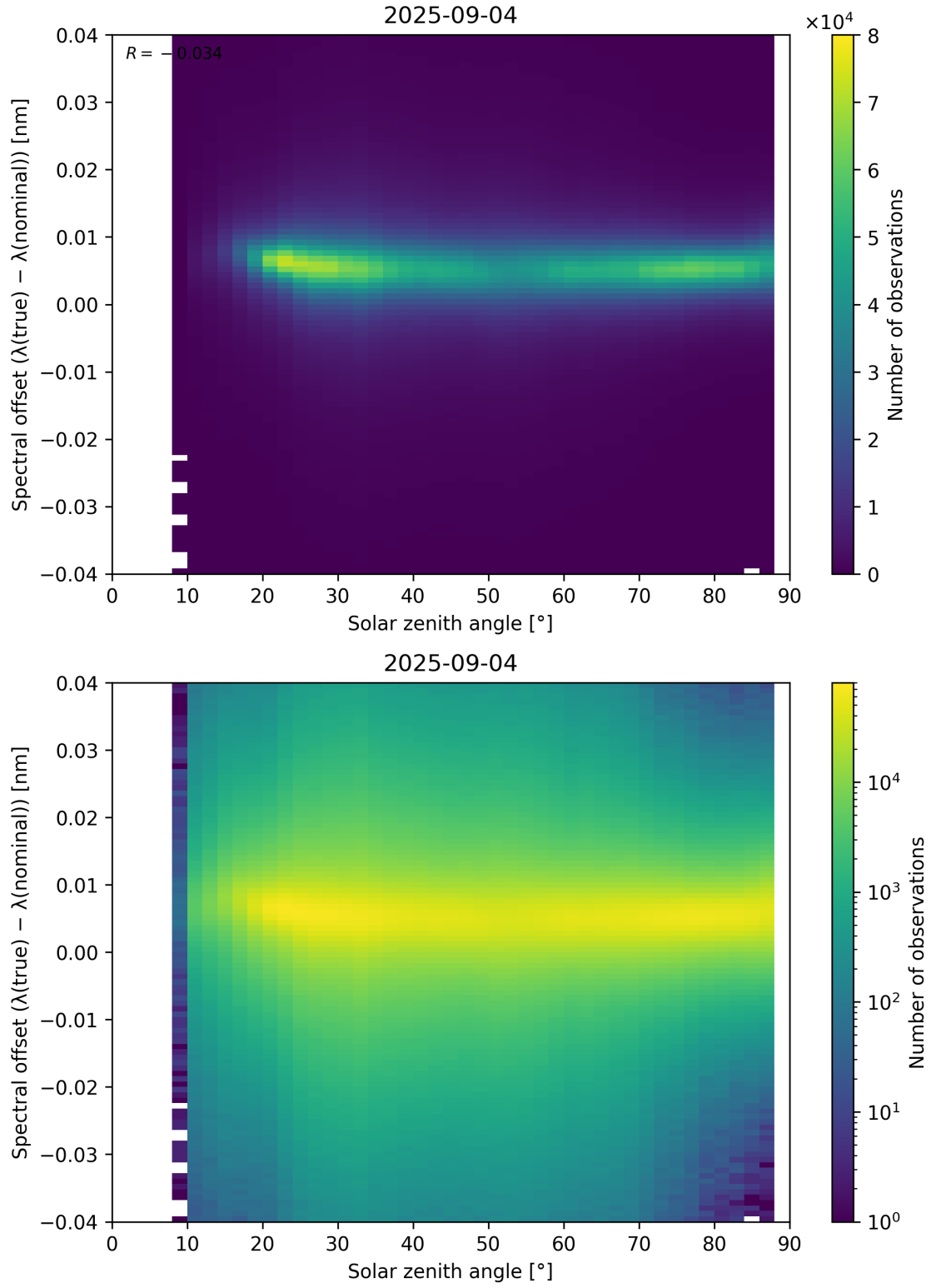
Figure 117: Scatter density plot of “Solar zenith angle” against “Spectral offset ( \lambda_{\text{true}} - \lambda_{\text{nominal}} )” for 2025-09-04 to 2025-09-05.
