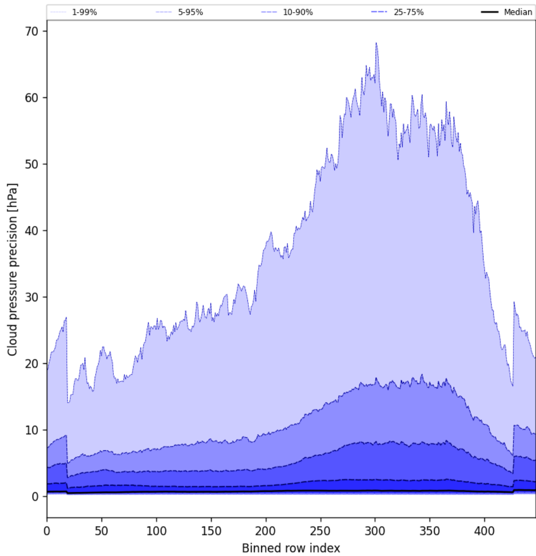
Figure 48: Along track statistics of “Cloud pressure precision” for 2025-09-04 to 2025-09-05
