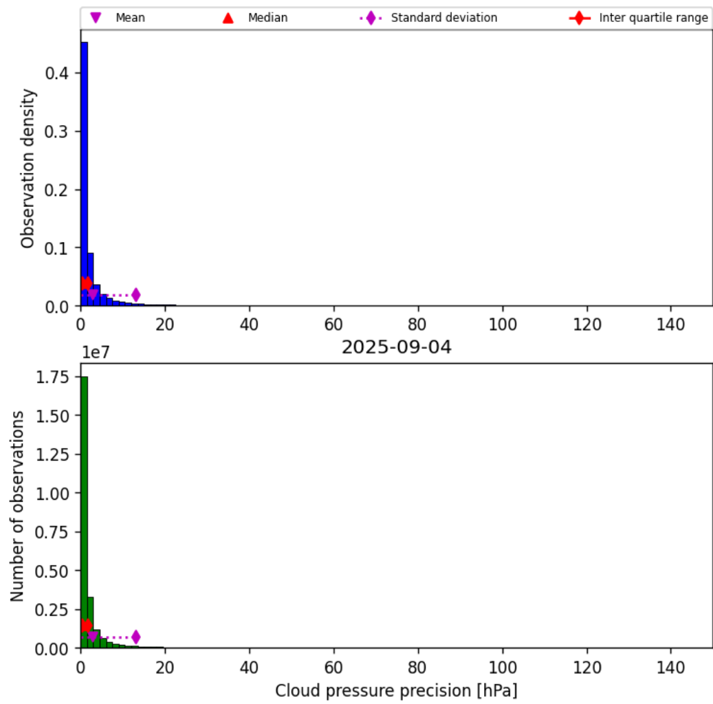
Figure 31: Histogram of “Cloud pressure precision” for 2025-09-04 to 2025-09-05
