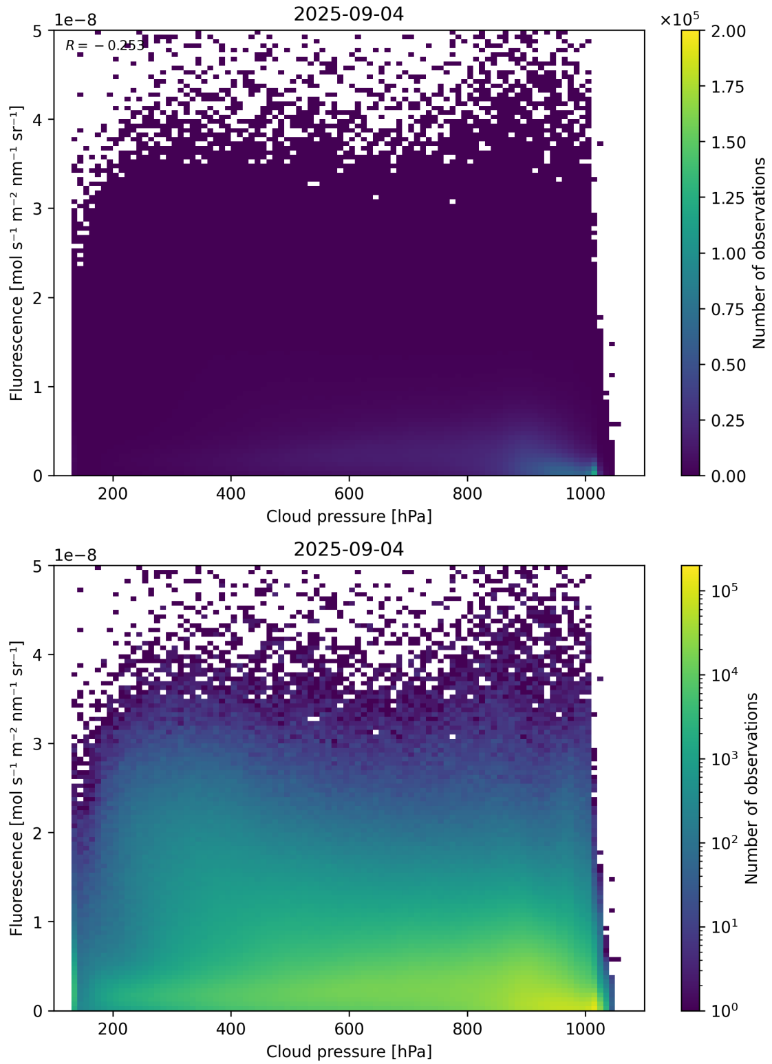
Figure 80: Scatter density plot of “Cloud pressure” against “Fluorescence” for 2025-09-04 to 2025-09-05.
