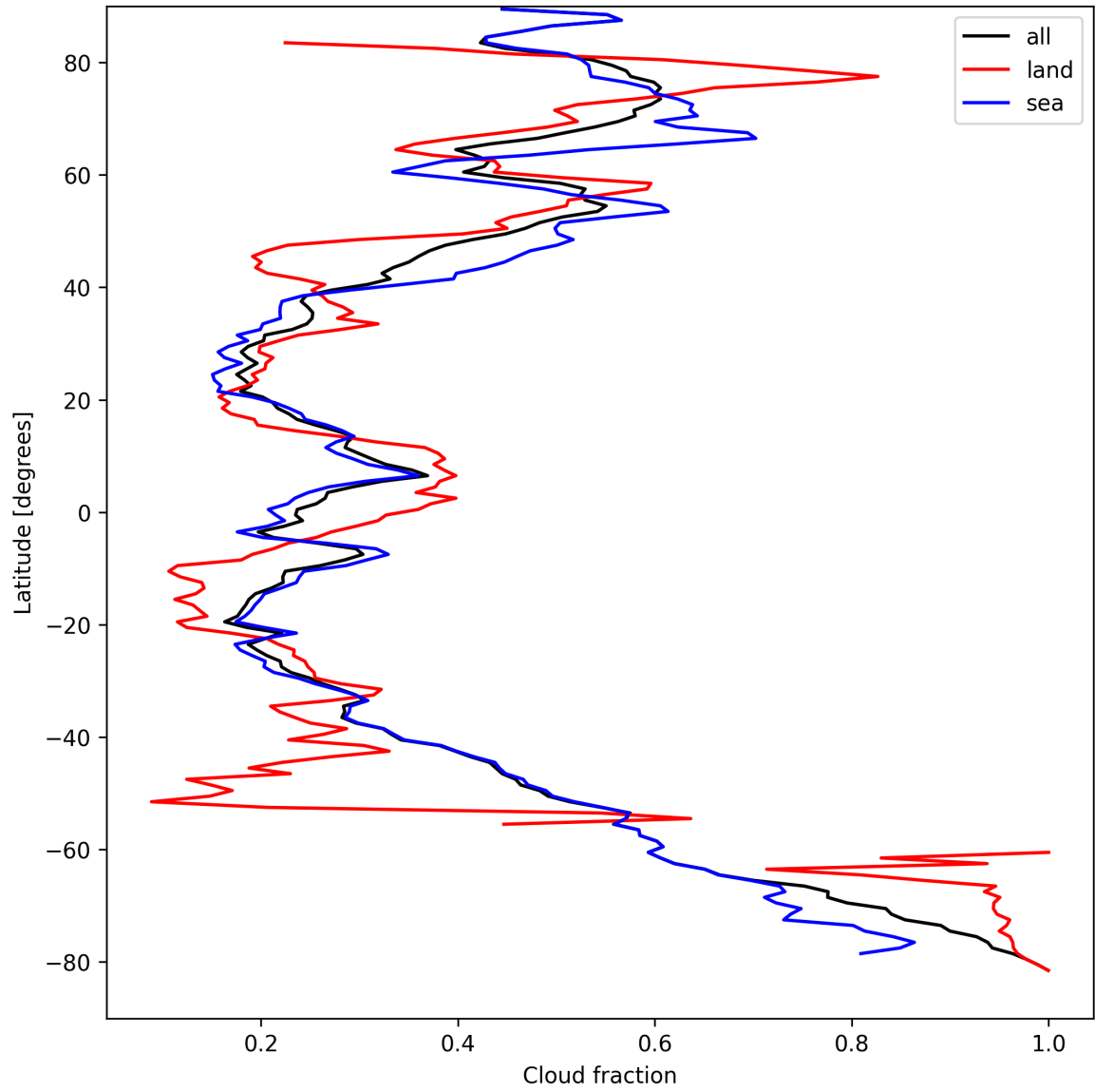
Figure 15: Zonal average of “Cloud fraction” for 2025-09-04 to 2025-09-05.
