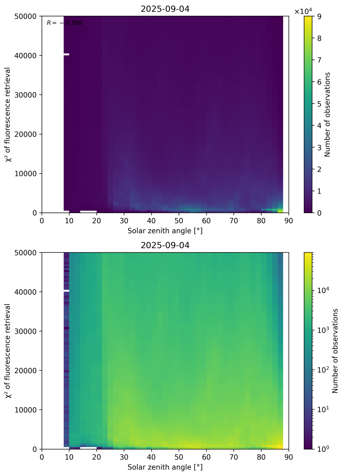
Figure 109: Scatter density plot of “Solar zenith angle” against “ \chi^2 of fluorescence retrieval” for 2025-09-04 to 2025-09-05.
