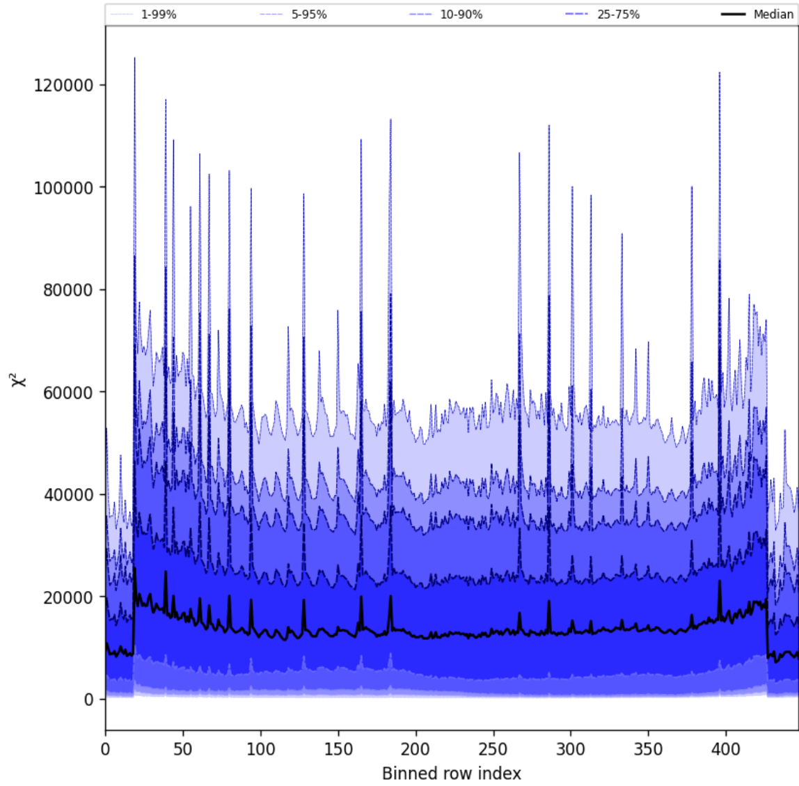
Figure 55: Along track statistics of “ \chi^2 ” for 2025-09-04 to 2025-09-05
