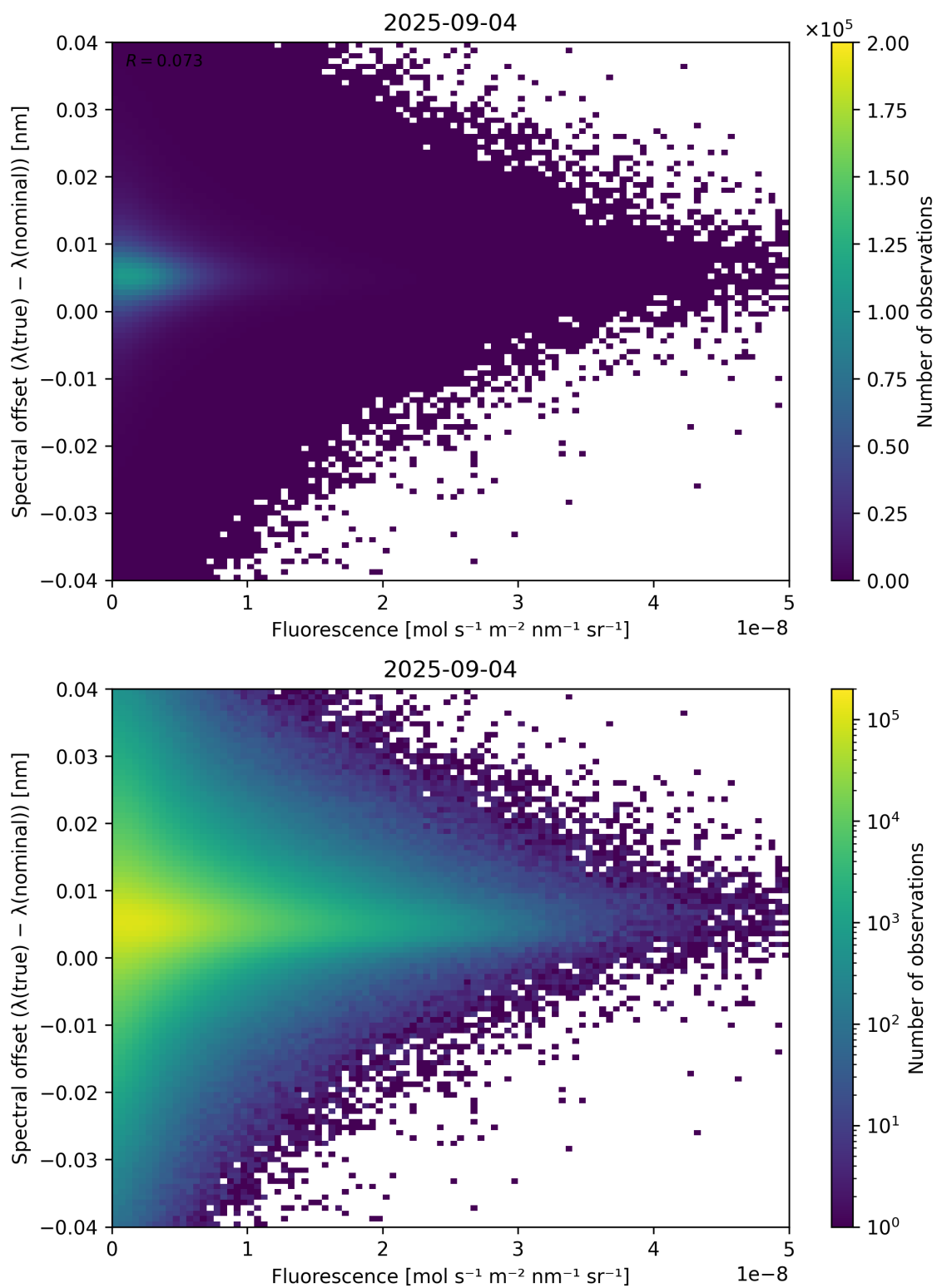
Figure 87: Scatter density plot of “Fluorescence” against “Spectral offset ( \lambda_{\text{true}} - \lambda_{\text{nominal}} )” for 2025-09-04 to 2025-09-05.
