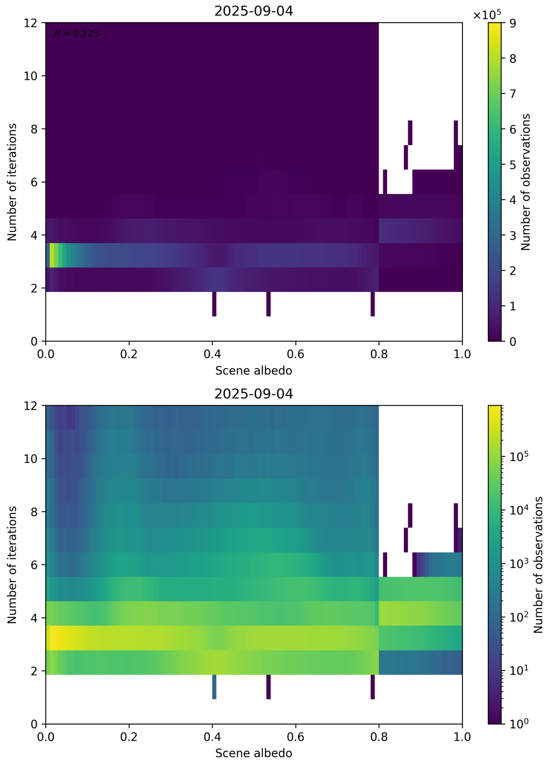
Figure 105: Scatter density plot of “Scene albedo” against “Number of iterations” for 2025-09-04 to 2025-09-05.
