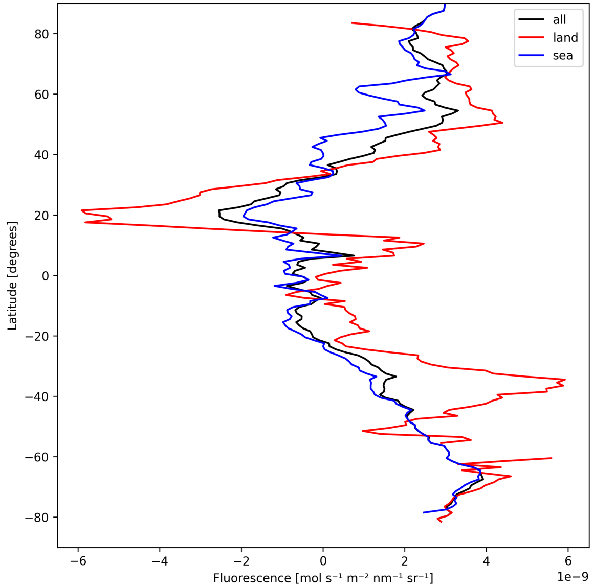
Figure 23: Zonal average of “Fluorescence” for 2025-09-04 to 2025-09-05.
