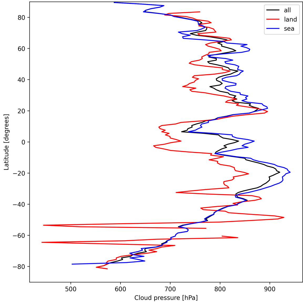
Figure 13: Zonal average of “Cloud pressure” for 2025-09-04 to 2025-09-05.
