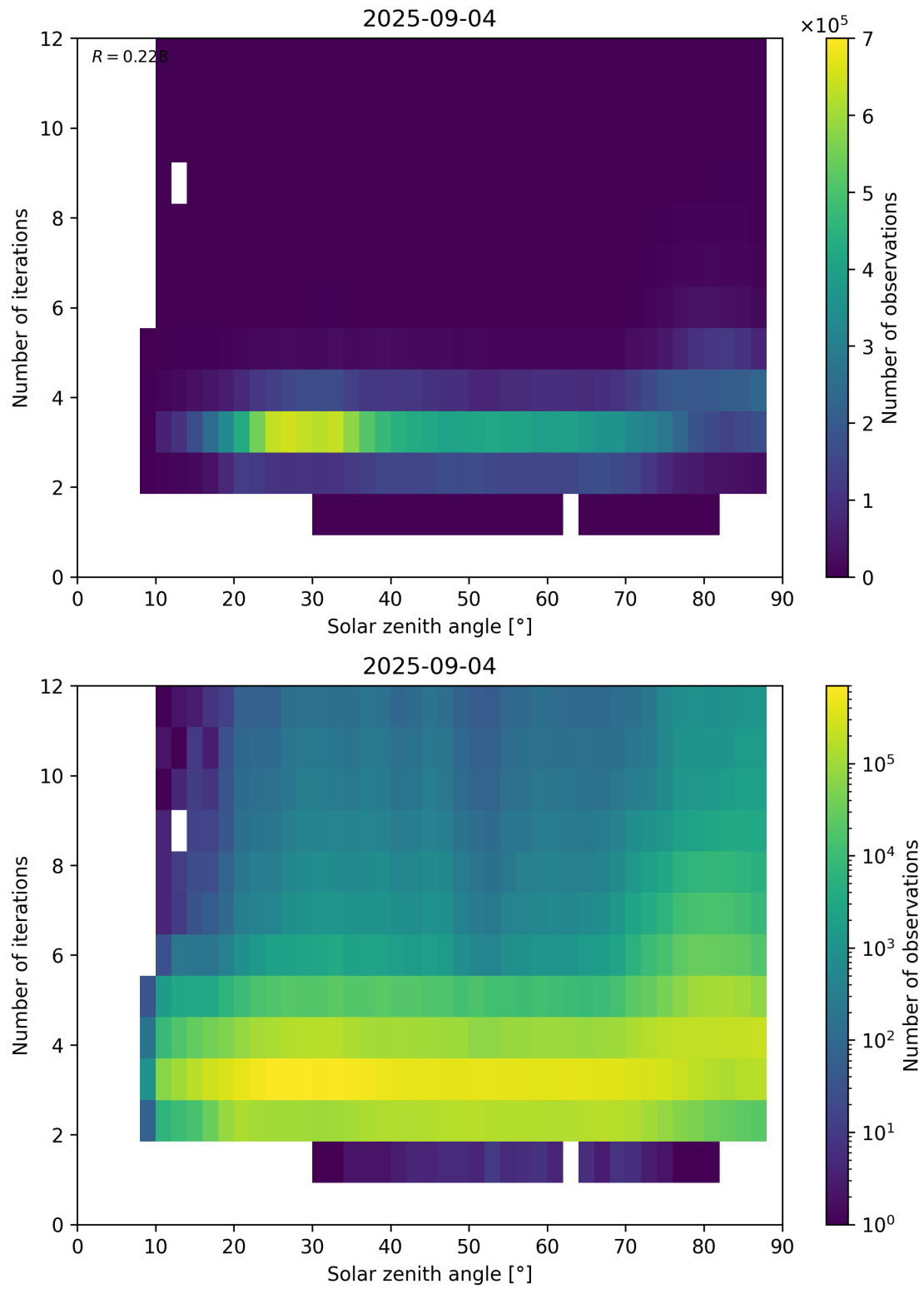
Figure 114: Scatter density plot of “Solar zenith angle” against “Number of iterations” for 2025-09-04 to 2025-09-05.
