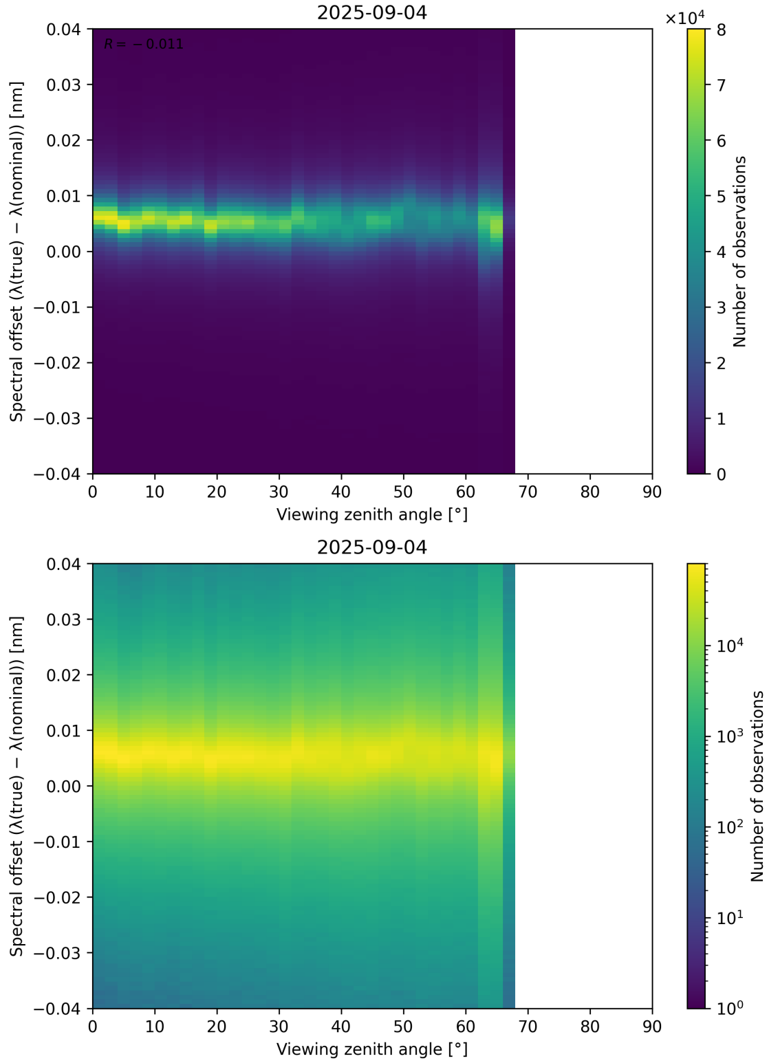
Figure 128: Scatter density plot of “Viewing zenith angle” against “Spectral offset ( \lambda_{\text{true}} - \lambda_{\text{nominal}} )” for 2025-09-04 to 2025-09-05.
