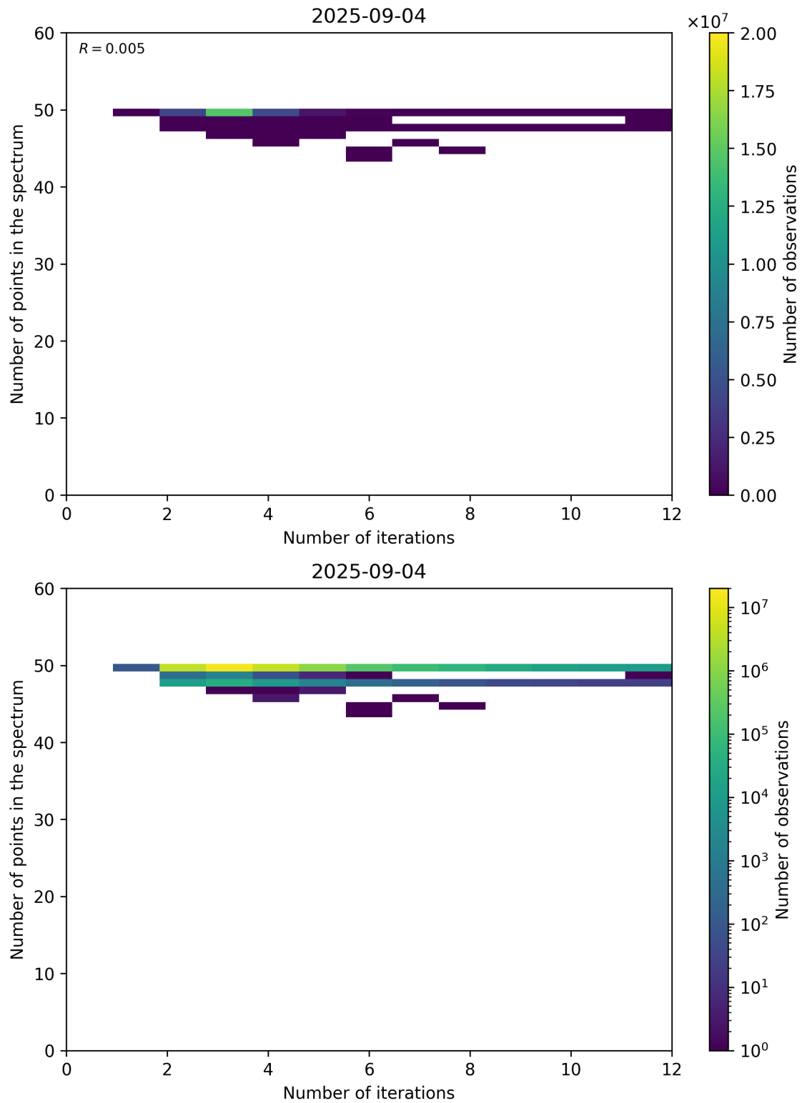
Figure 99: Scatter density plot of “Number of iterations” against “Number of points in the spectrum” for 2025-09-04 to 2025-09-05.
