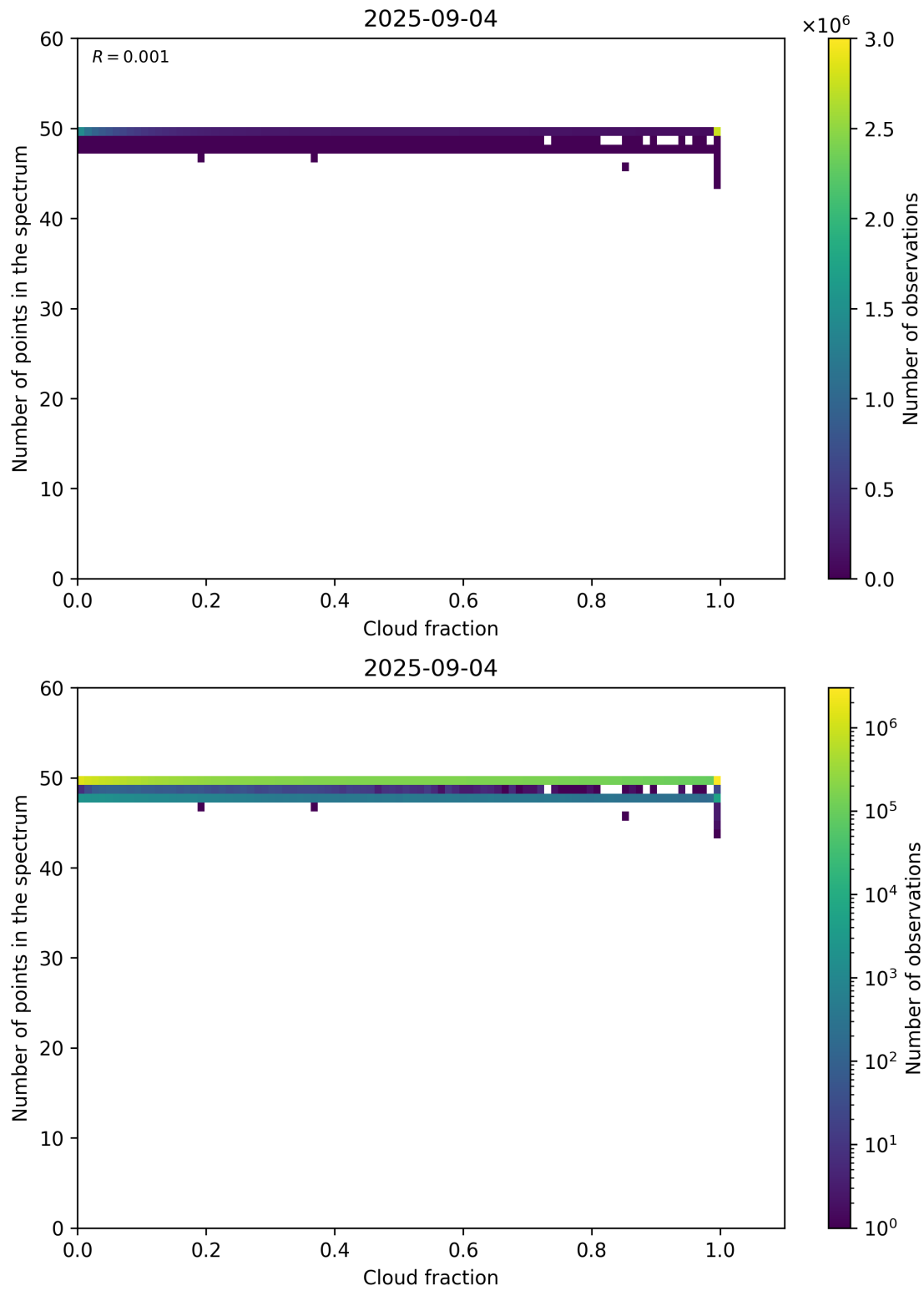
Figure 74: Scatter density plot of “Cloud fraction” against “Number of points in the spectrum” for 2025-09-04 to 2025-09-05.
