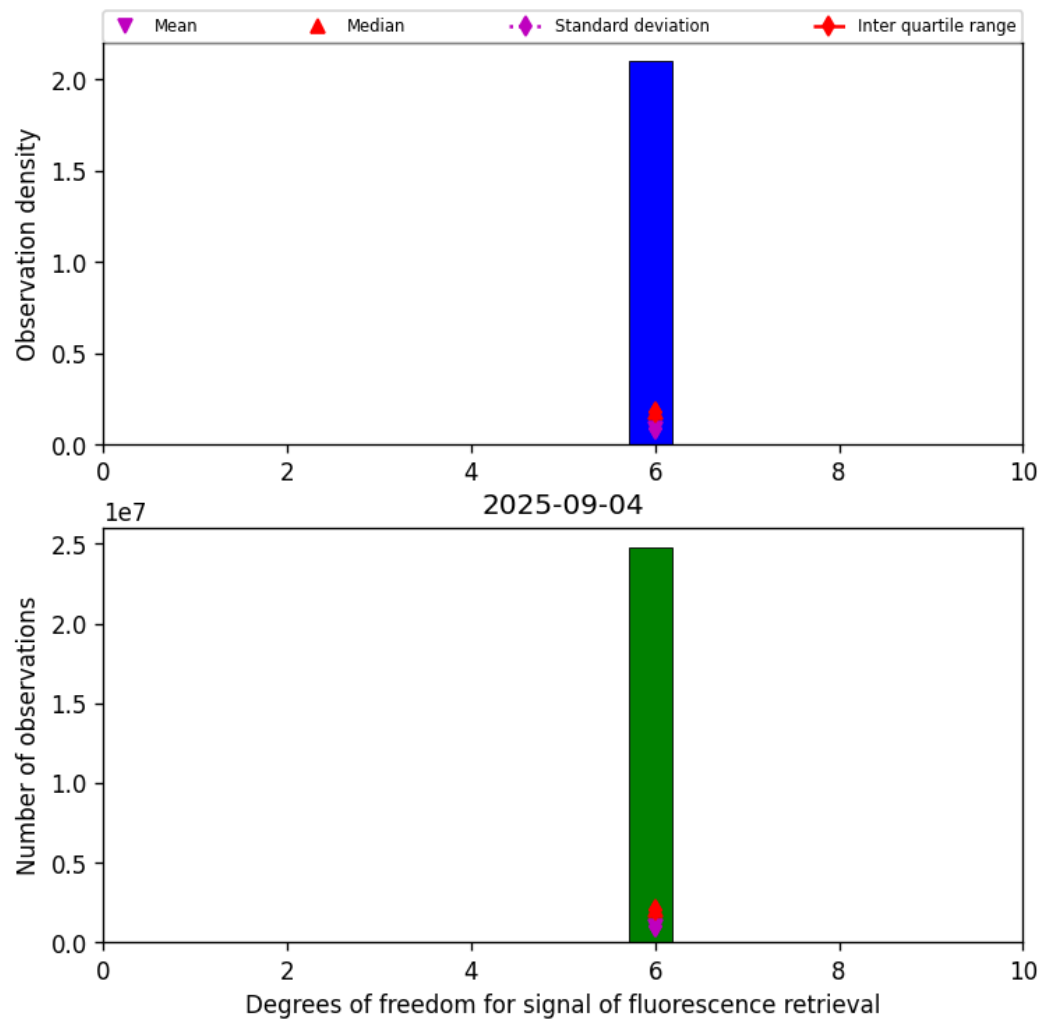
Figure 43: Histogram of “Degrees of freedom for signal of fluorescence retrieval” for 2025-09-04 to 2025-09-05
