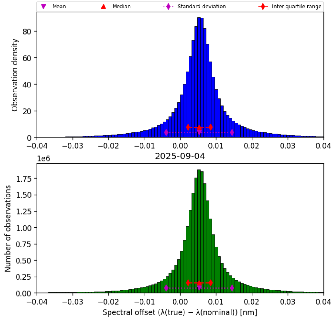
Figure 45: Histogram of “Spectral offset ( \lambda_{\text{true}} - \lambda_{\text{nominal}} )” for 2025-09-04 to 2025-09-05
