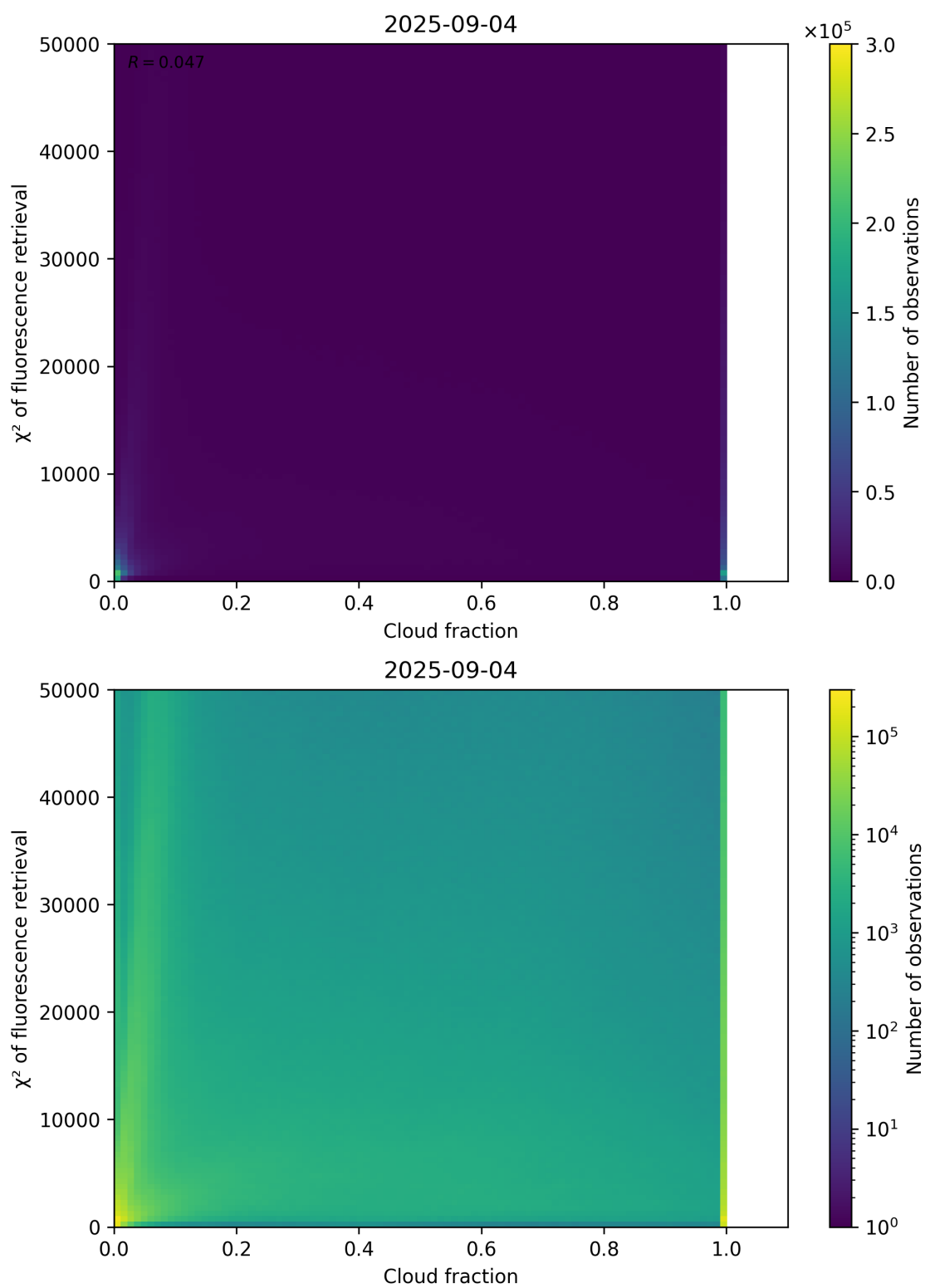
Figure 71: Scatter density plot of “Cloud fraction” against “ \chi^2 of fluorescence retrieval” for 2025-09-04 to 2025-09-05.
