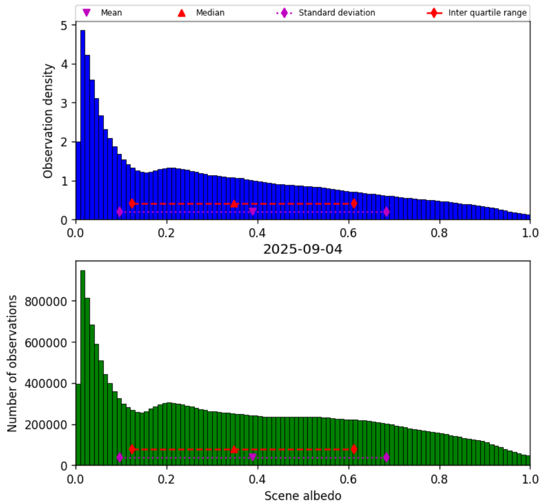
Figure 34: Histogram of “Scene albedo” for 2025-09-04 to 2025-09-05
