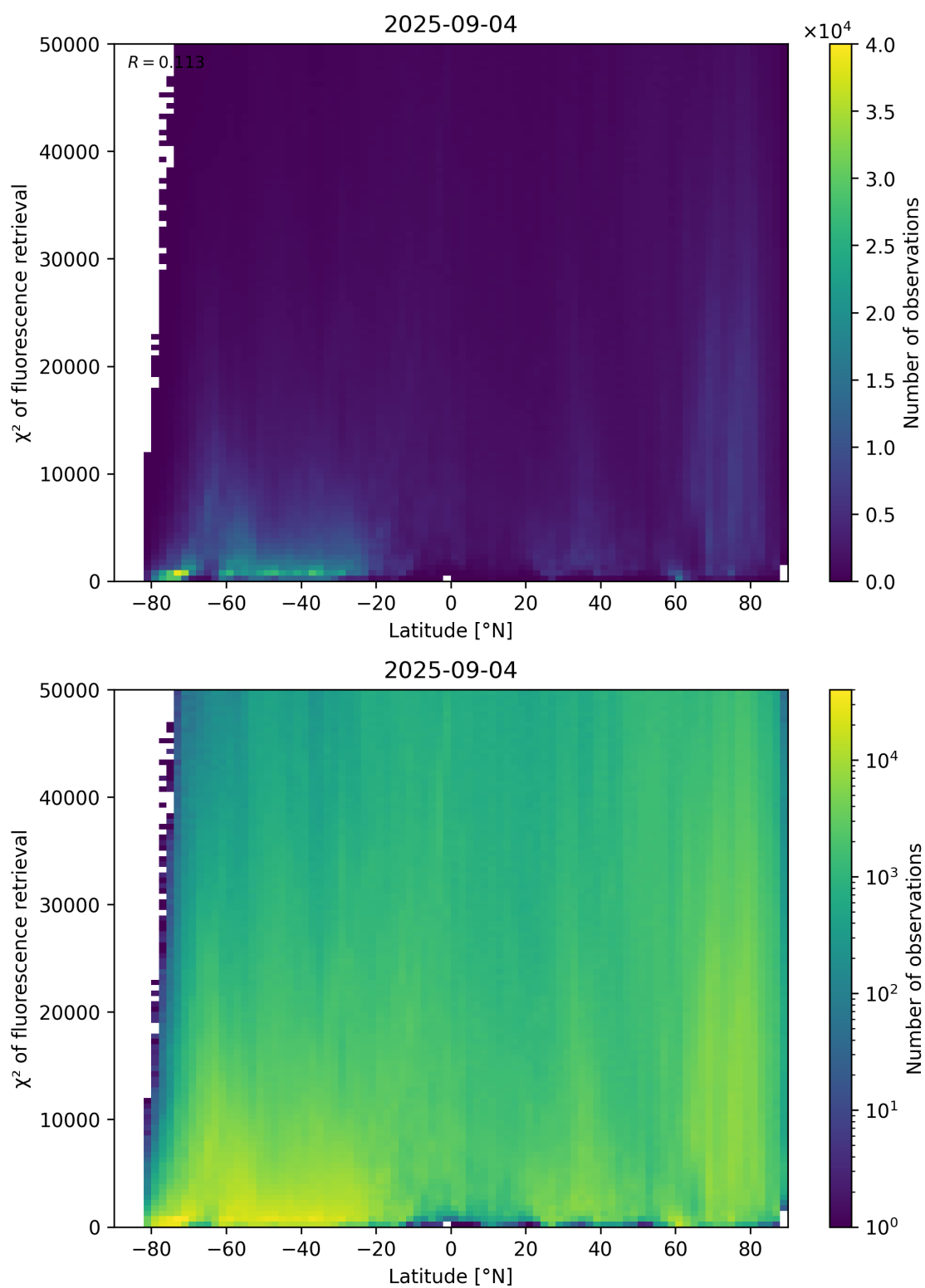
Figure 89: Scatter density plot of “Latitude” against “ \chi^2 of fluorescence retrieval” for 2025-09-04 to 2025-09-05.
