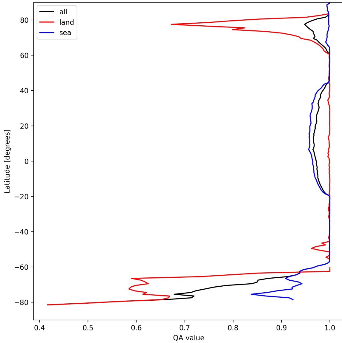
Figure 12: Zonal average of "QA value" for 2025-09-04 to 2025-09-05.
