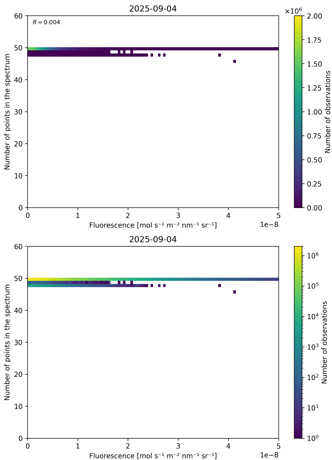
Figure 86: Scatter density plot of “Fluorescence” against “Number of points in the spectrum” for 2025-09-04 to 2025-09-05.
