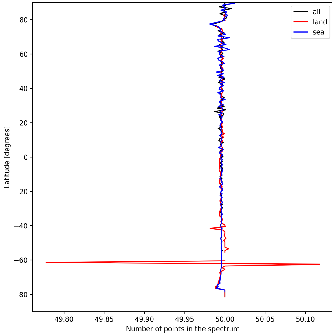
Figure 27: Zonal average of “Number of points in the spectrum” for 2025-09-04 to 2025-09-05.
