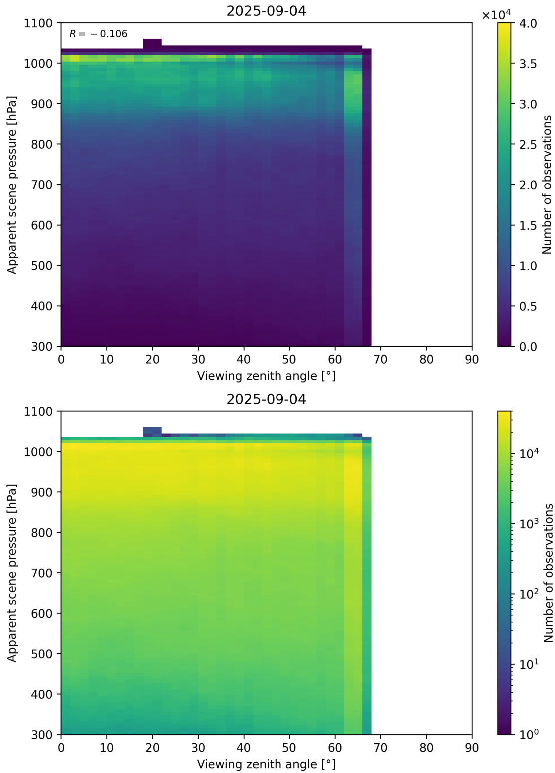
Figure 118: Scatter density plot of “Viewing zenith angle” against “Apparent scene pressure” for 2025-09-04 to 2025-09-05.
