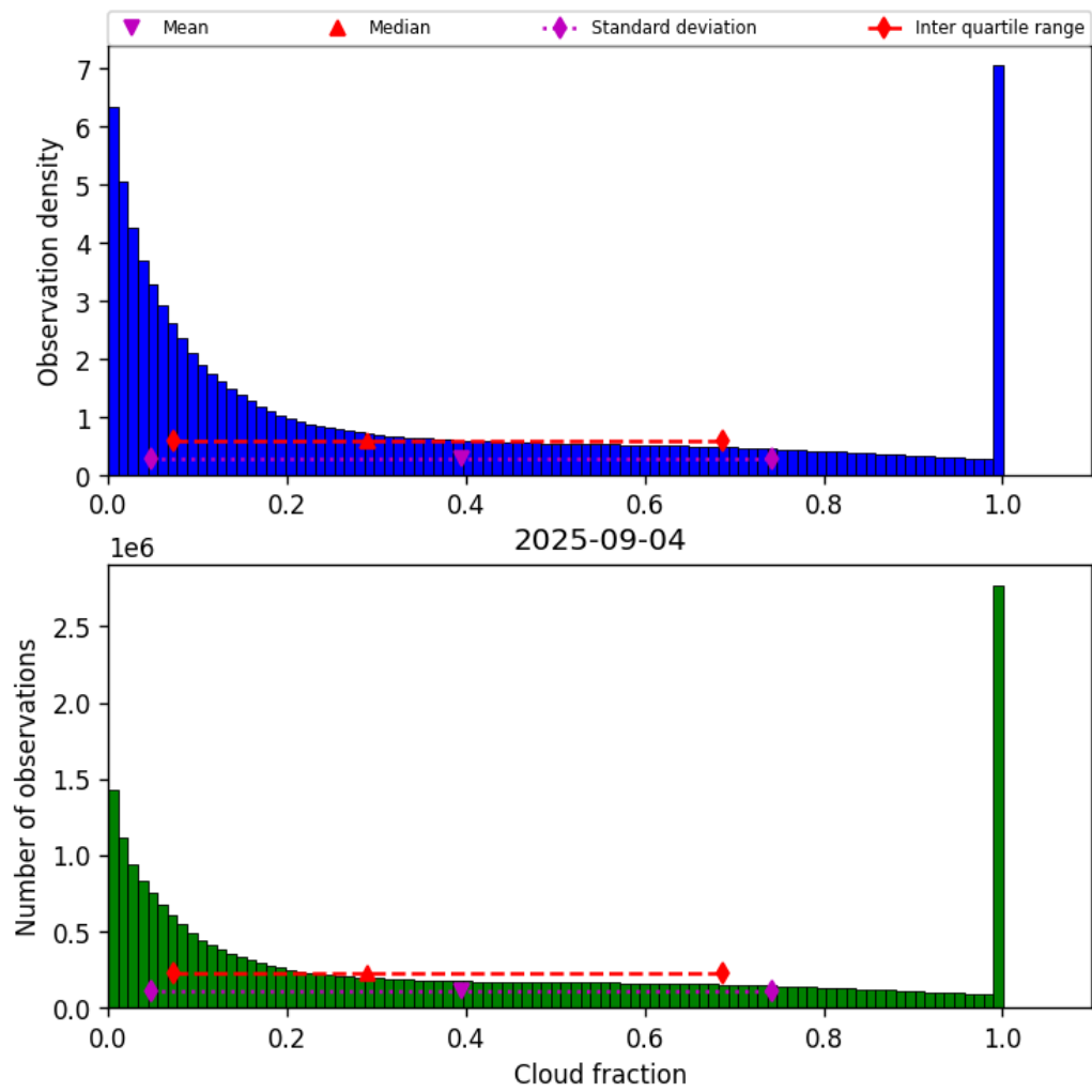
Figure 32: Histogram of “Cloud fraction” for 2025-09-04 to 2025-09-05
