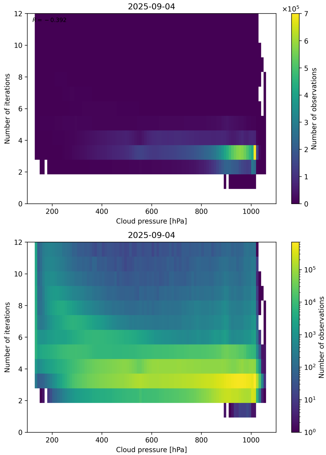
Figure 81: Scatter density plot of “Cloud pressure” against “Number of iterations” for 2025-09-04 to 2025-09-05.
