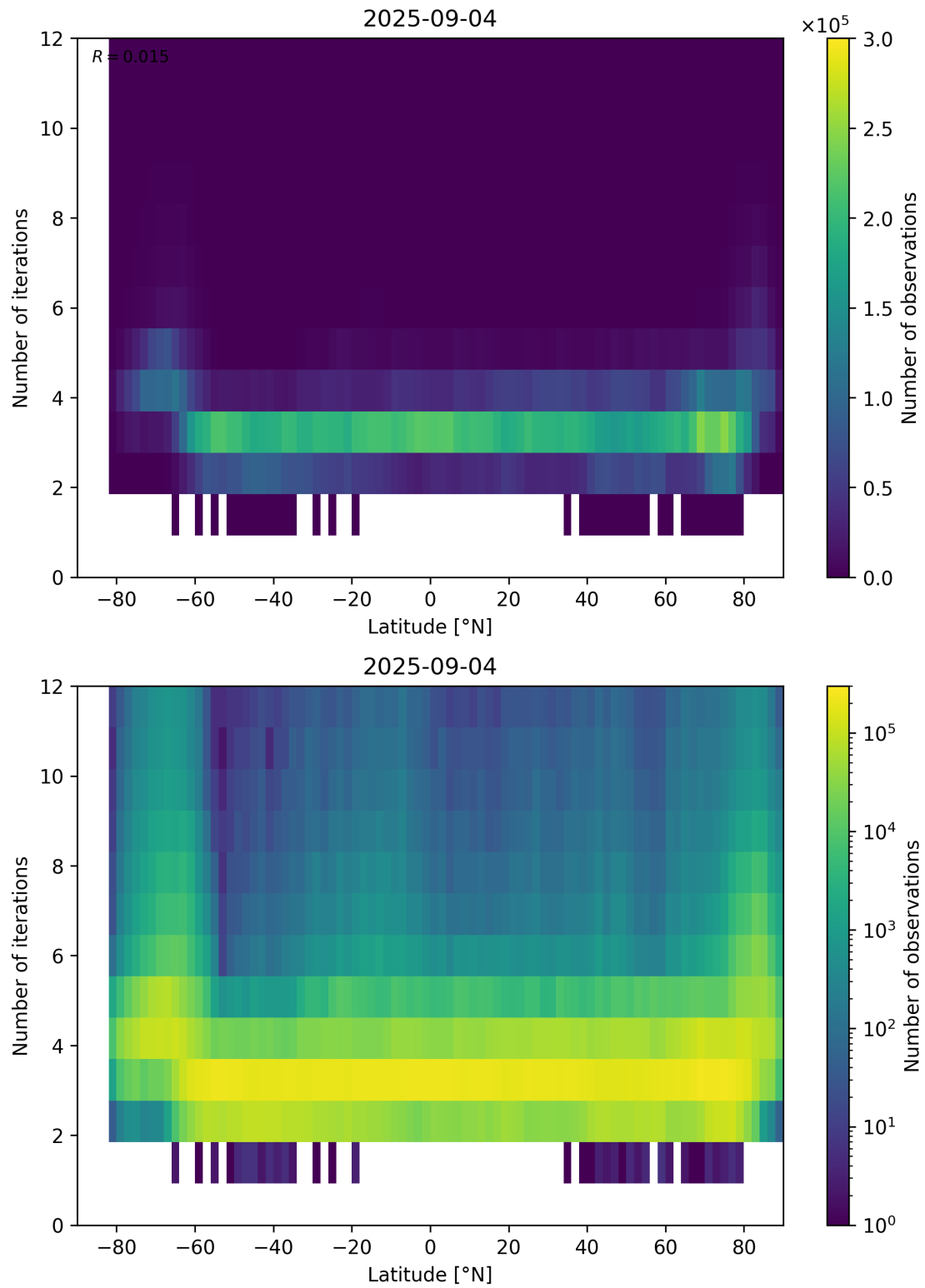
Figure 93: Scatter density plot of “Latitude” against “Number of iterations” for 2025-09-04 to 2025-09-05.
