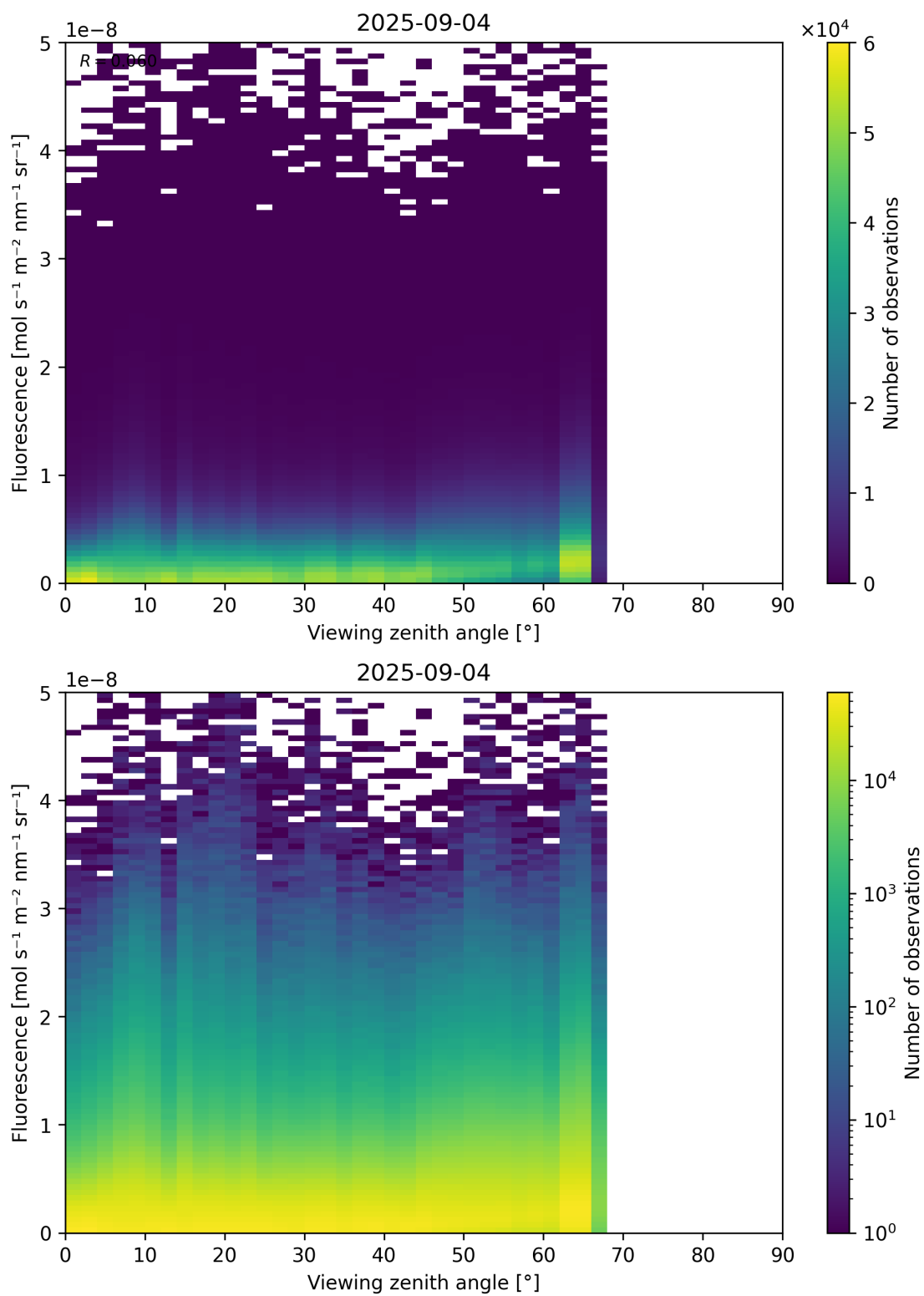
Figure 122: Scatter density plot of “Viewing zenith angle” against “Fluorescence” for 2025-09-04 to 2025-09-05.
