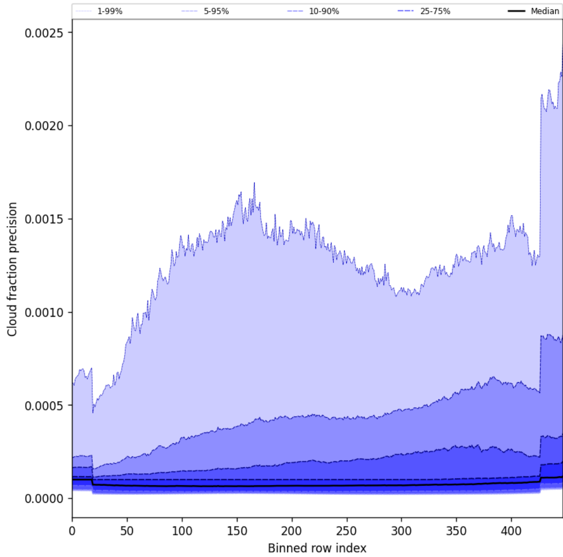
Figure 50: Along track statistics of “Cloud fraction precision” for 2025-09-04 to 2025-09-05
