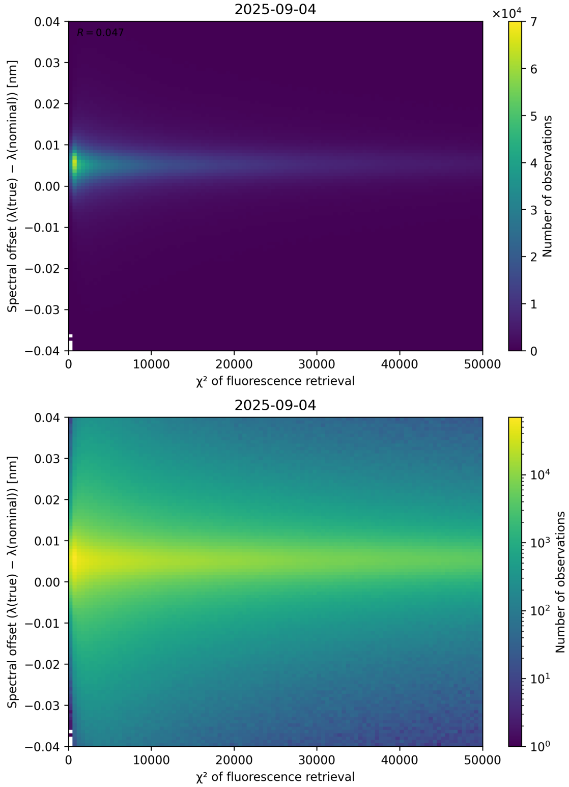
Figure 69: Scatter density plot of “ \chi^2 of fluorescence retrieval” against “Spectral offset ( \lambda_{\text{true}} - \lambda_{\text{nominal}} )” for 2025-09-04 to 2025-09-05.
