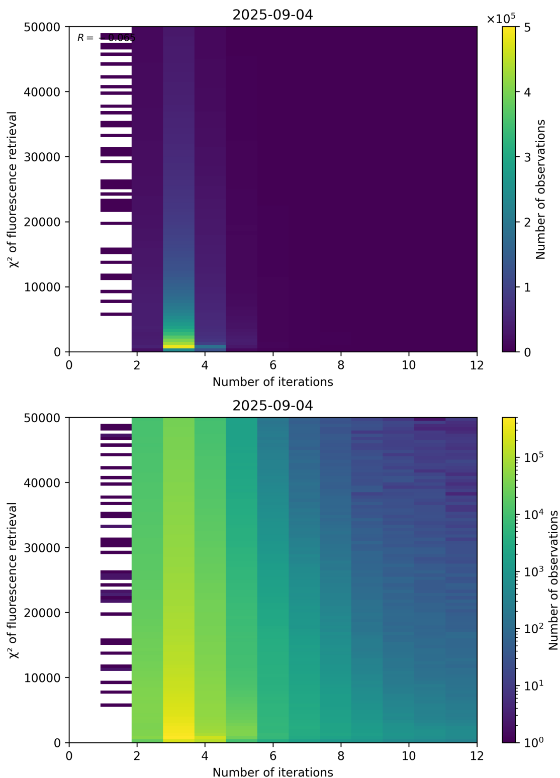
Figure 97: Scatter density plot of “Number of iterations” against “ \chi^2 of fluorescence retrieval” for 2025-09-04 to 2025-09-05.
