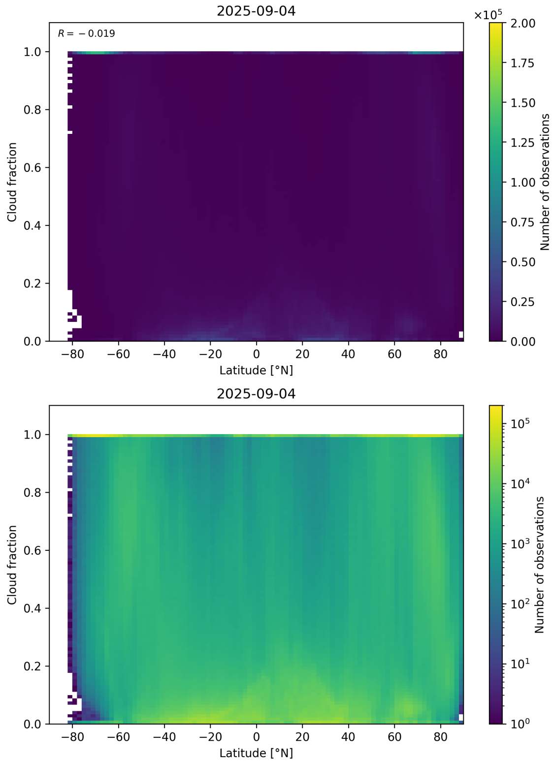
Figure 90: Scatter density plot of “Latitude” against “Cloud fraction” for 2025-09-04 to 2025-09-05.
