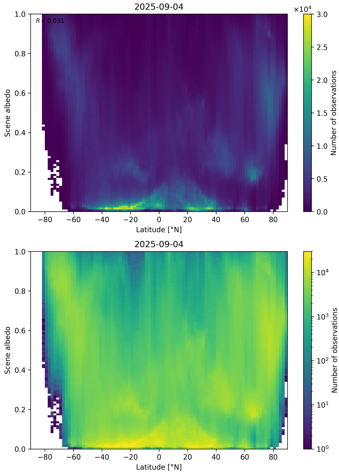
Figure 95: Scatter density plot of “Latitude” against “Scene albedo” for 2025-09-04 to 2025-09-05.
