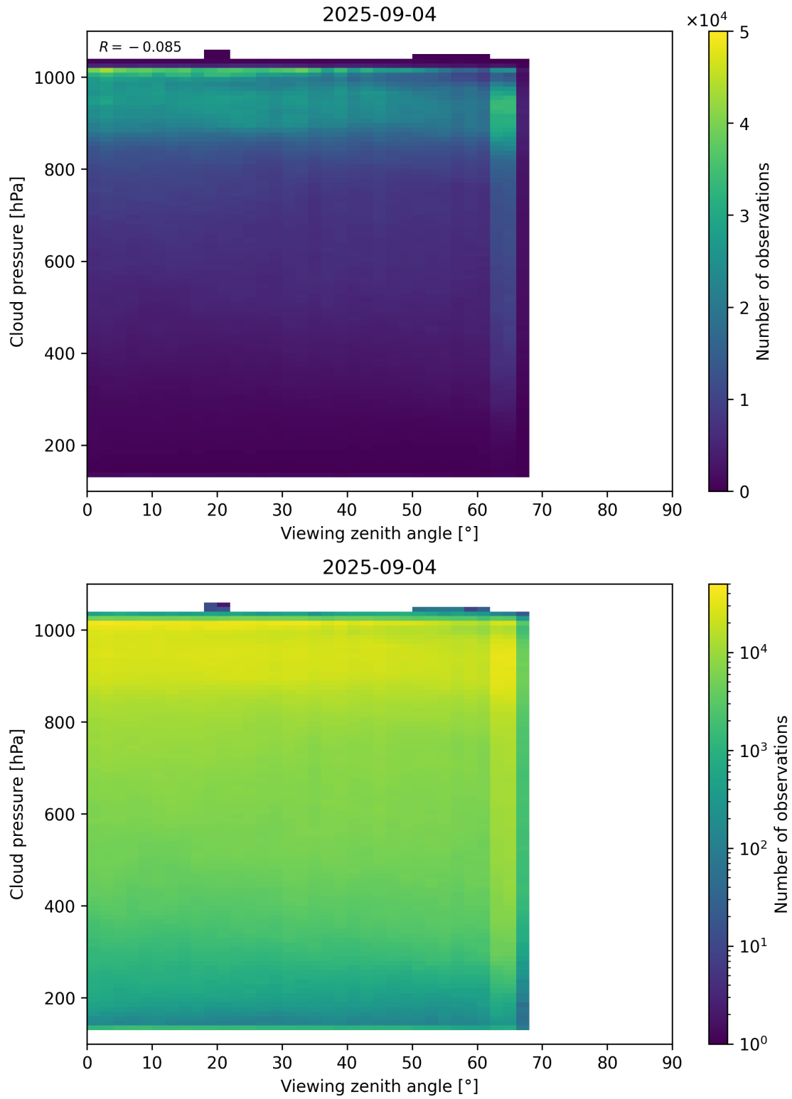
Figure 121: Scatter density plot of “Viewing zenith angle” against “Cloud pressure” for 2025-09-04 to 2025-09-05.
