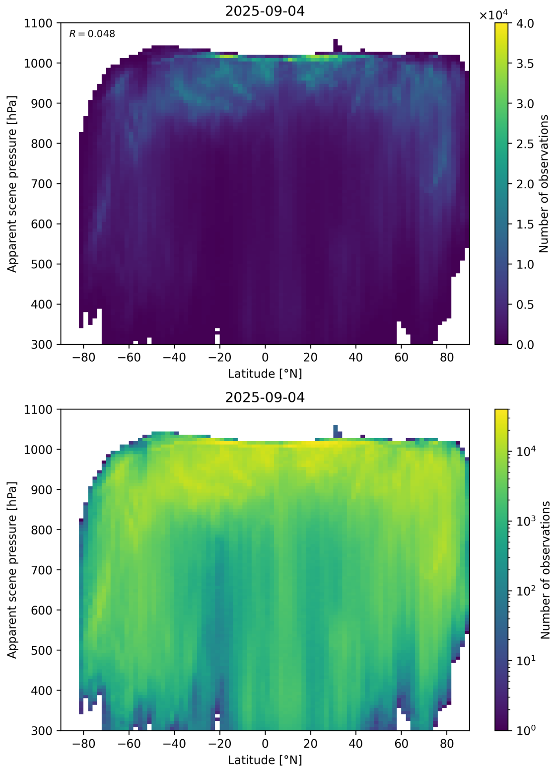
Figure 88: Scatter density plot of “Latitude” against “Apparent scene pressure” for 2025-09-04 to 2025-09-05.
