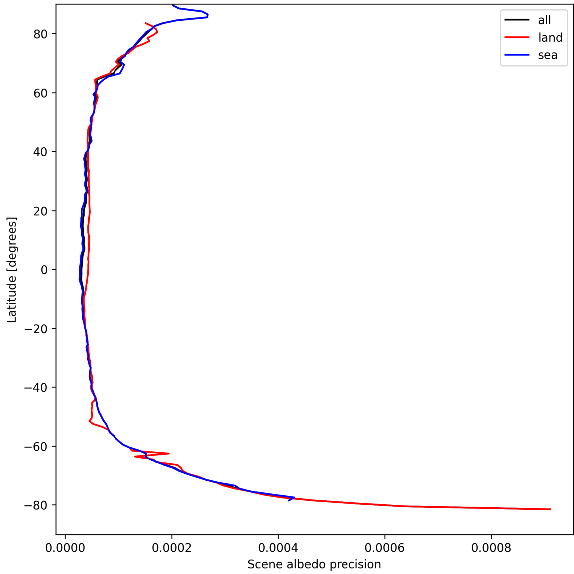
Figure 18: Zonal average of "Scene albedo precision" for 2025-09-04 to 2025-09-05.
