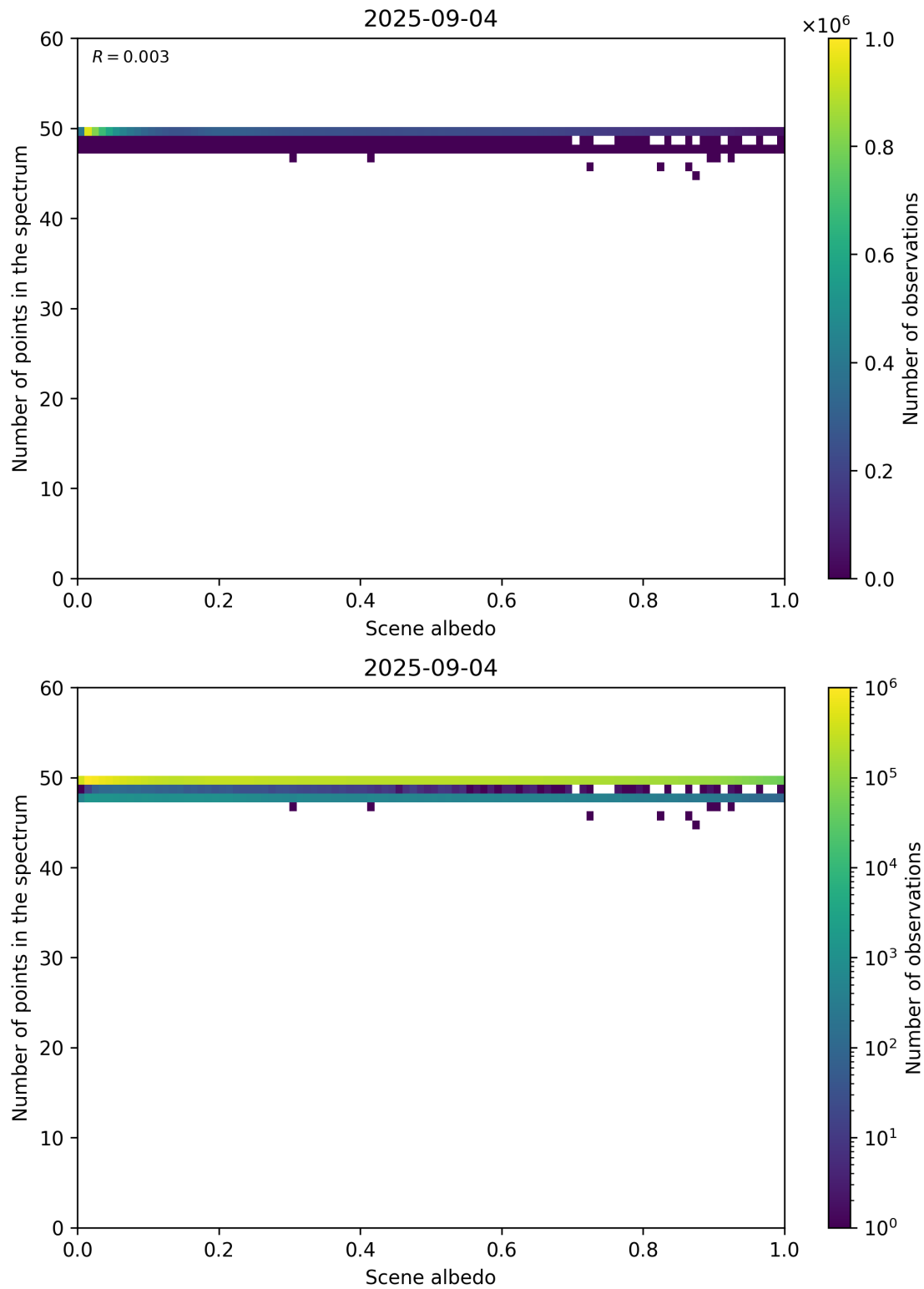
Figure 106: Scatter density plot of “Scene albedo” against “Number of points in the spectrum” for 2025-09-04 to 2025-09-05.
