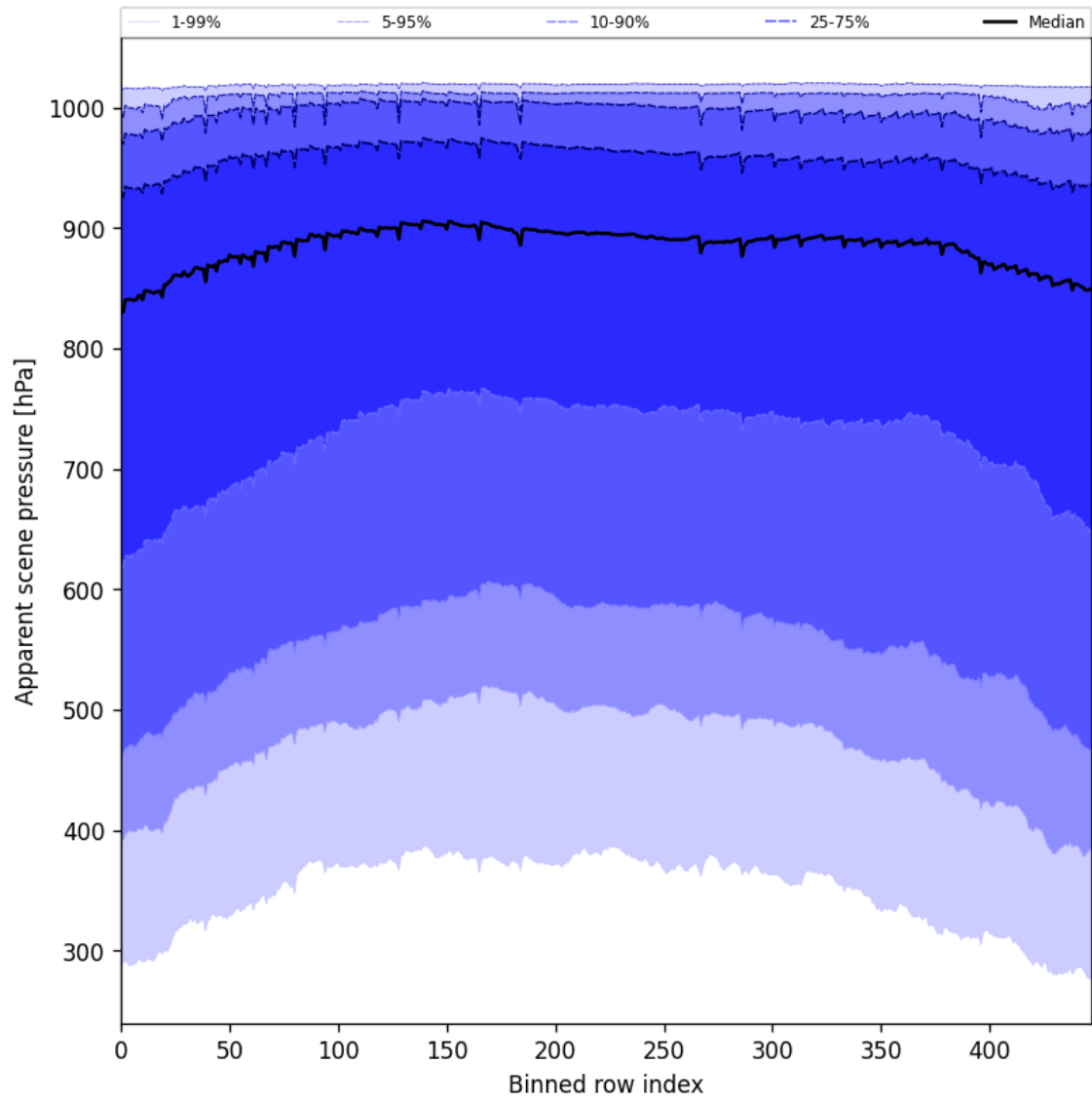
Figure 53: Along track statistics of “Apparent scene pressure” for 2025-09-04 to 2025-09-05
