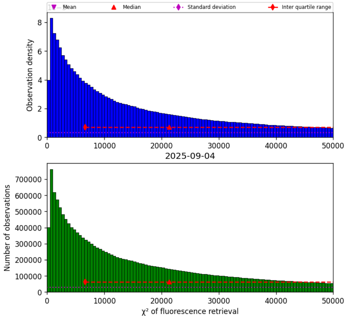
Figure 42: Histogram of “ \chi^2 of fluorescence retrieval” for 2025-09-04 to 2025-09-05
