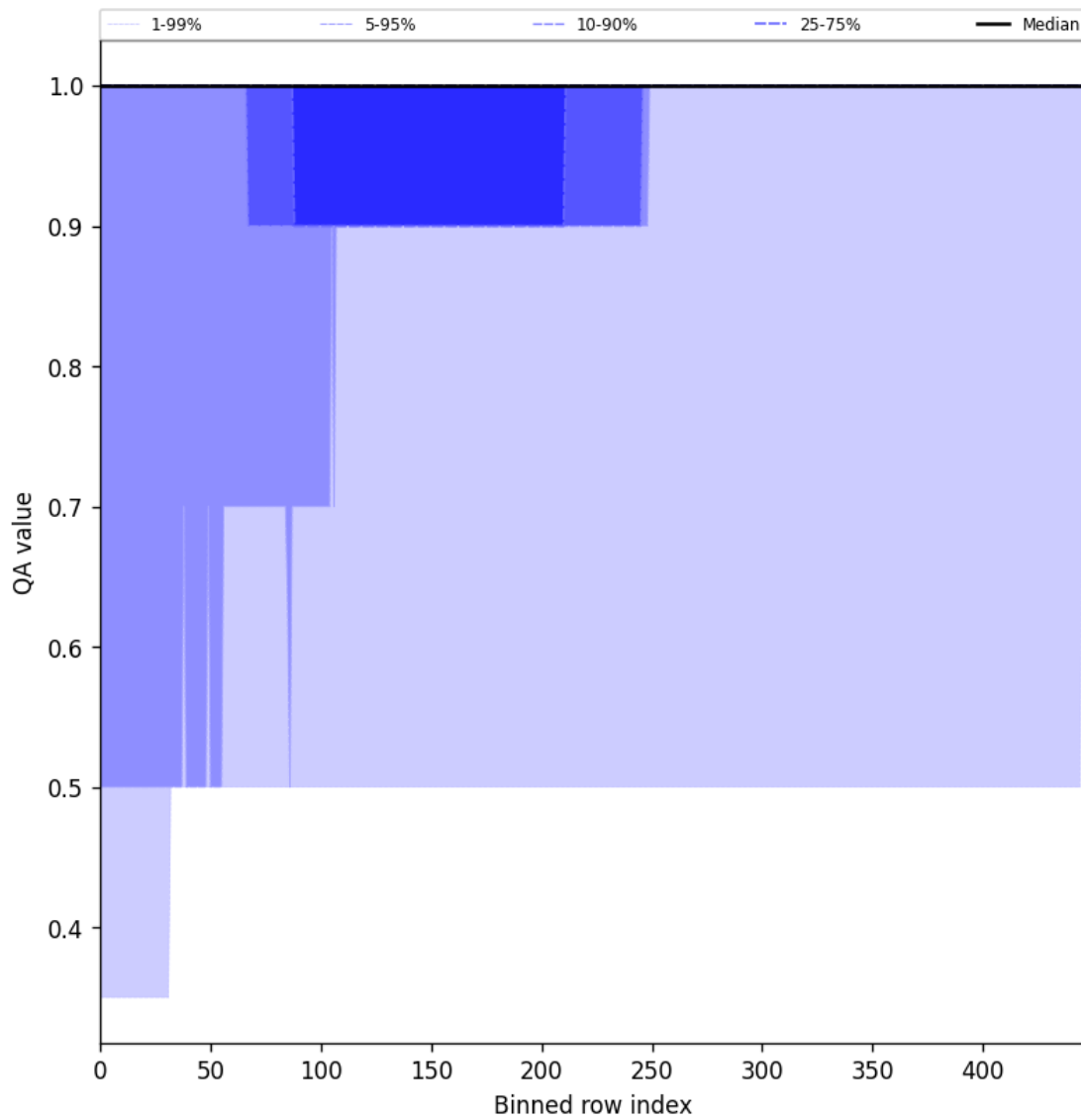
Figure 46: Along track statistics of “QA value” for 2025-09-04 to 2025-09-05
