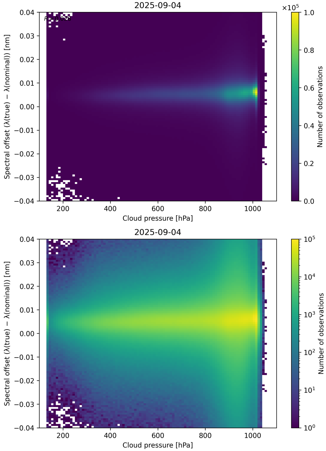
Figure 84: Scatter density plot of “Cloud pressure” against “Spectral offset ( \lambda_{\text{true}} - \lambda_{\text{nominal}} )” for 2025-09-04 to 2025-09-05.
