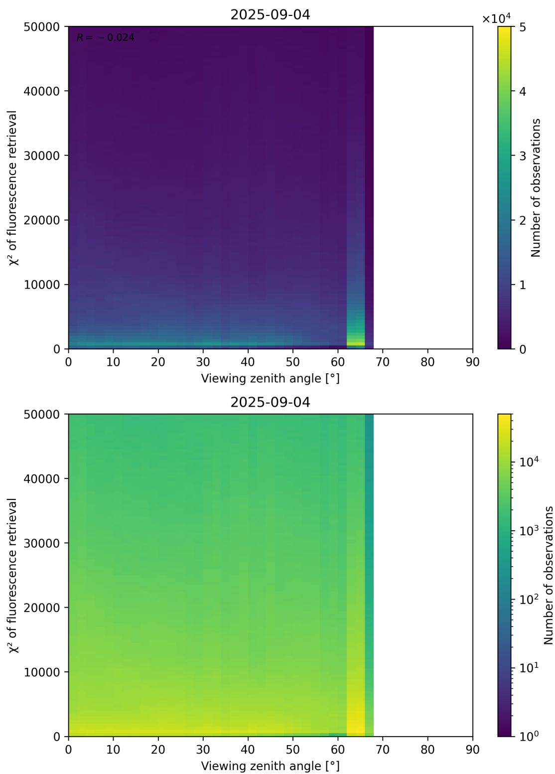
Figure 119: Scatter density plot of “Viewing zenith angle” against “ \chi^2 of fluorescence retrieval” for 2025-09-04 to 2025-09-05.
