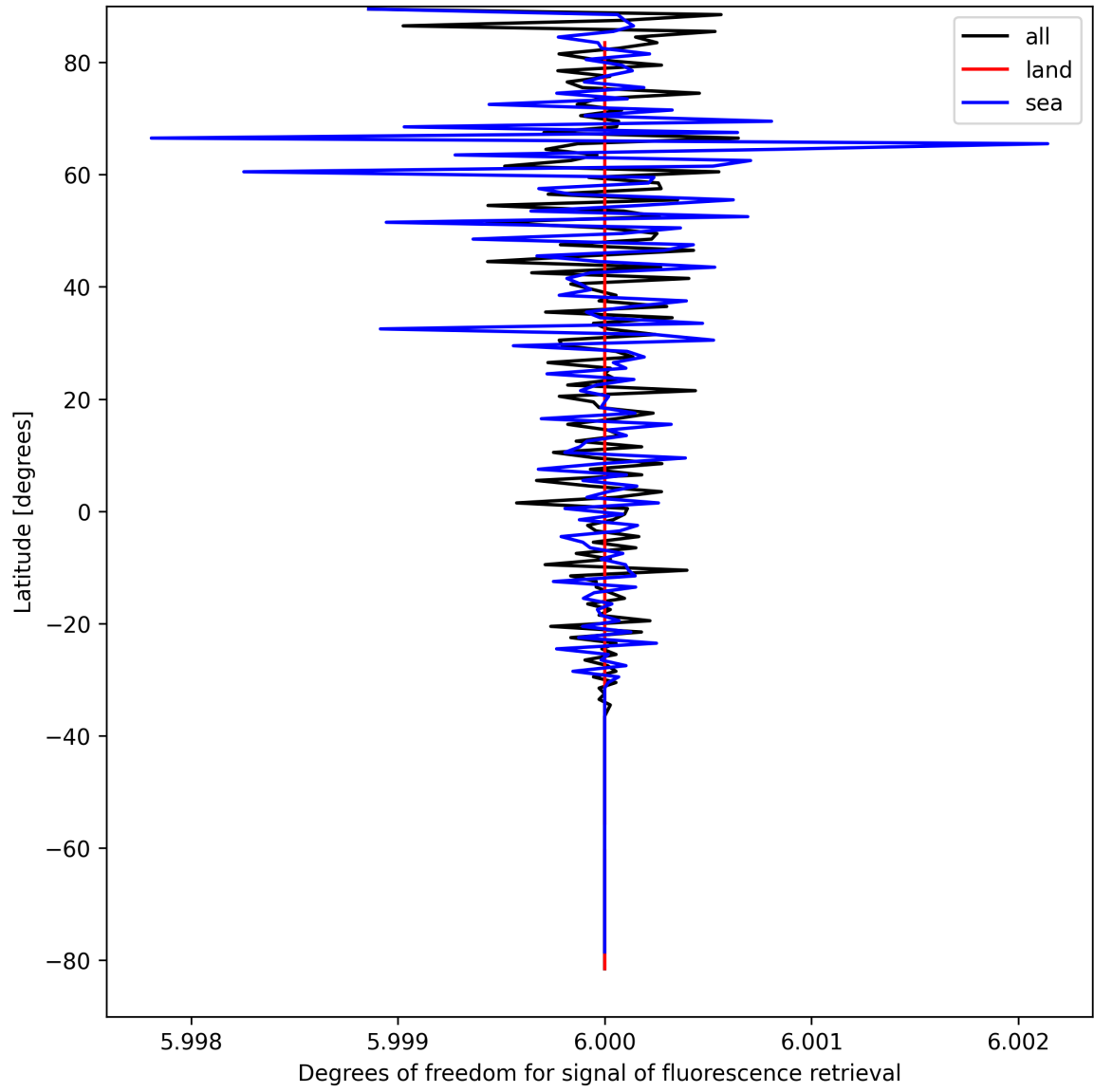
Figure 26: Zonal average of “Degrees of freedom for signal of fluorescence retrieval” for 2025-09-04 to 2025-09-05.
