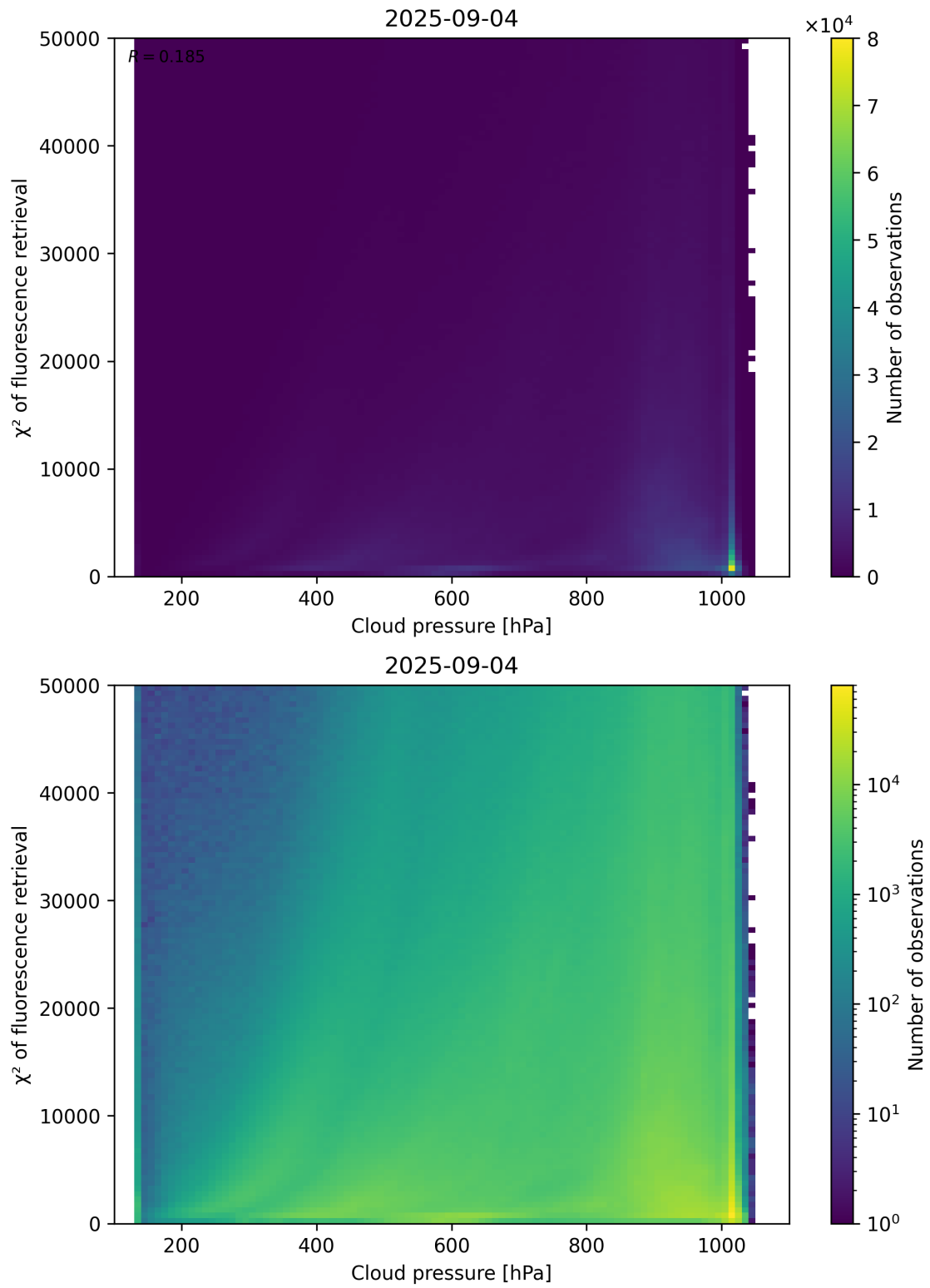
Figure 78: Scatter density plot of “Cloud pressure” against “ \chi^2 of fluorescence retrieval” for 2025-09-04 to 2025-09-05.
