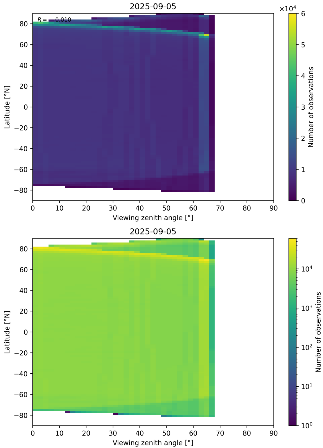
Figure 123: Scatter density plot of “Viewing zenith angle” against “Latitude” for 2025-09-04 to 2025-09-06.
