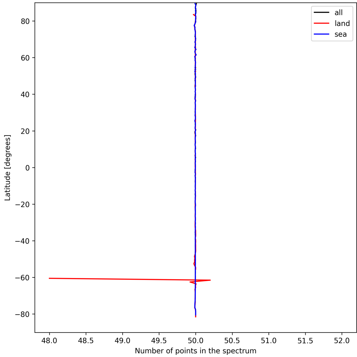
Figure 27: Zonal average of “Number of points in the spectrum” for 2025-09-04 to 2025-09-06.
