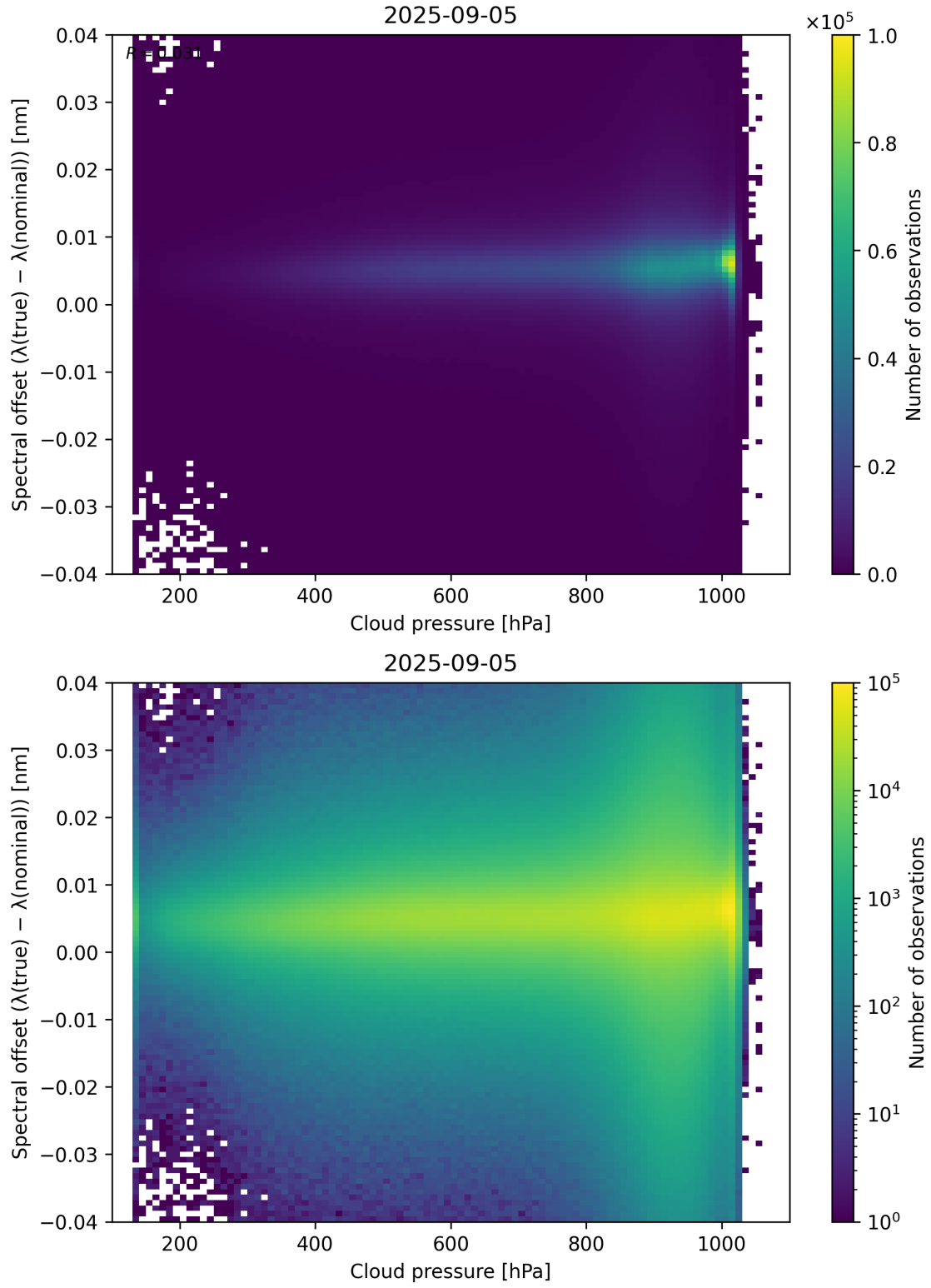
Figure 84: Scatter density plot of “Cloud pressure” against “Spectral offset ( \lambda_{\text{true}} - \lambda_{\text{nominal}} )” for 2025-09-04 to 2025-09-06.
