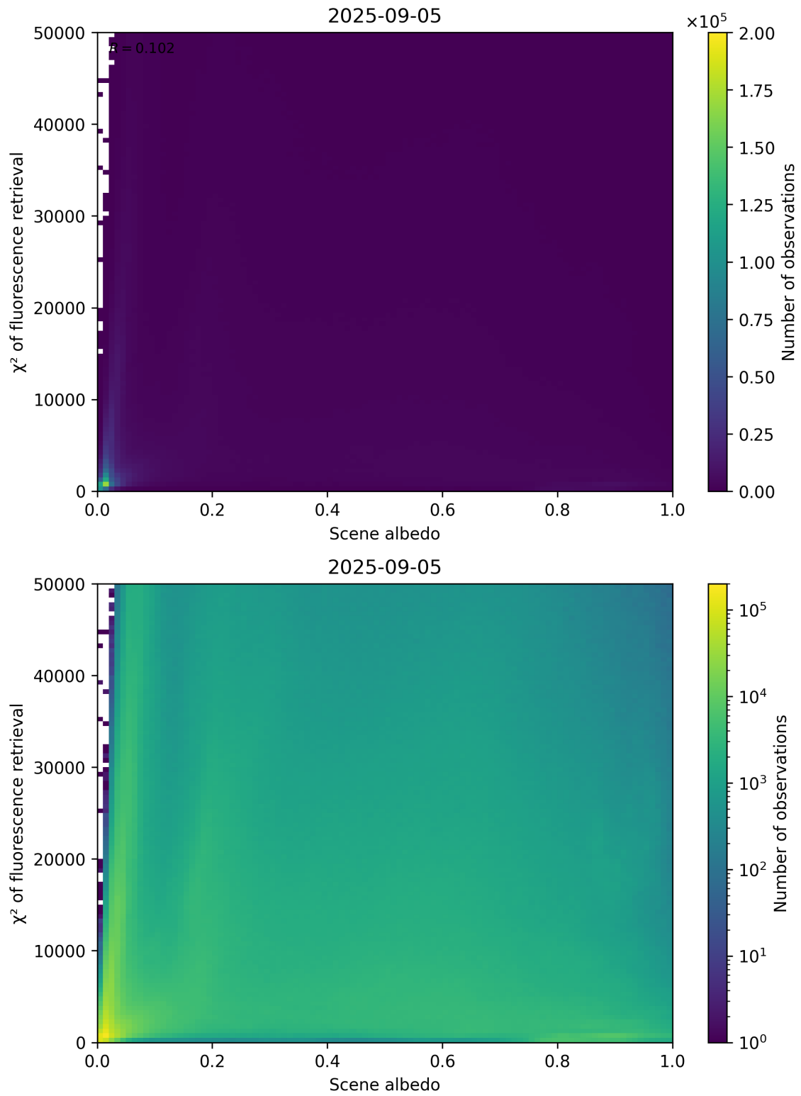
Figure 103: Scatter density plot of “Scene albedo” against “ \chi^2 of fluorescence retrieval” for 2025-09-04 to 2025-09-06.
