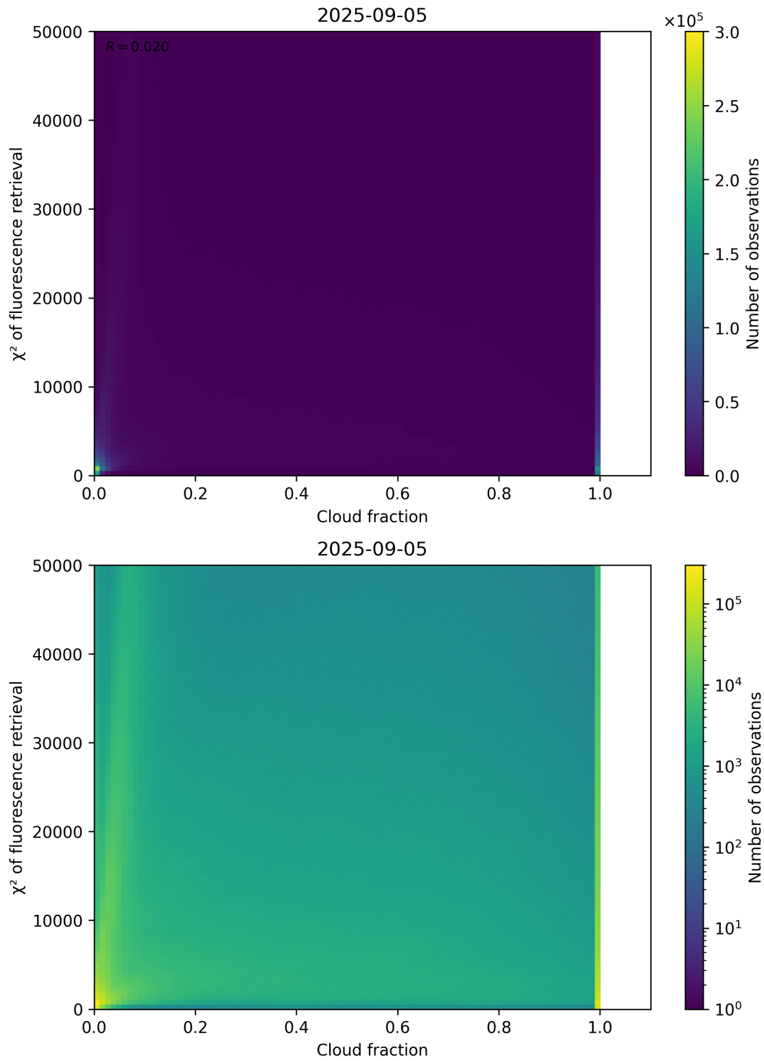
Figure 71: Scatter density plot of “Cloud fraction” against “ \chi^2 of fluorescence retrieval” for 2025-09-04 to 2025-09-06.
