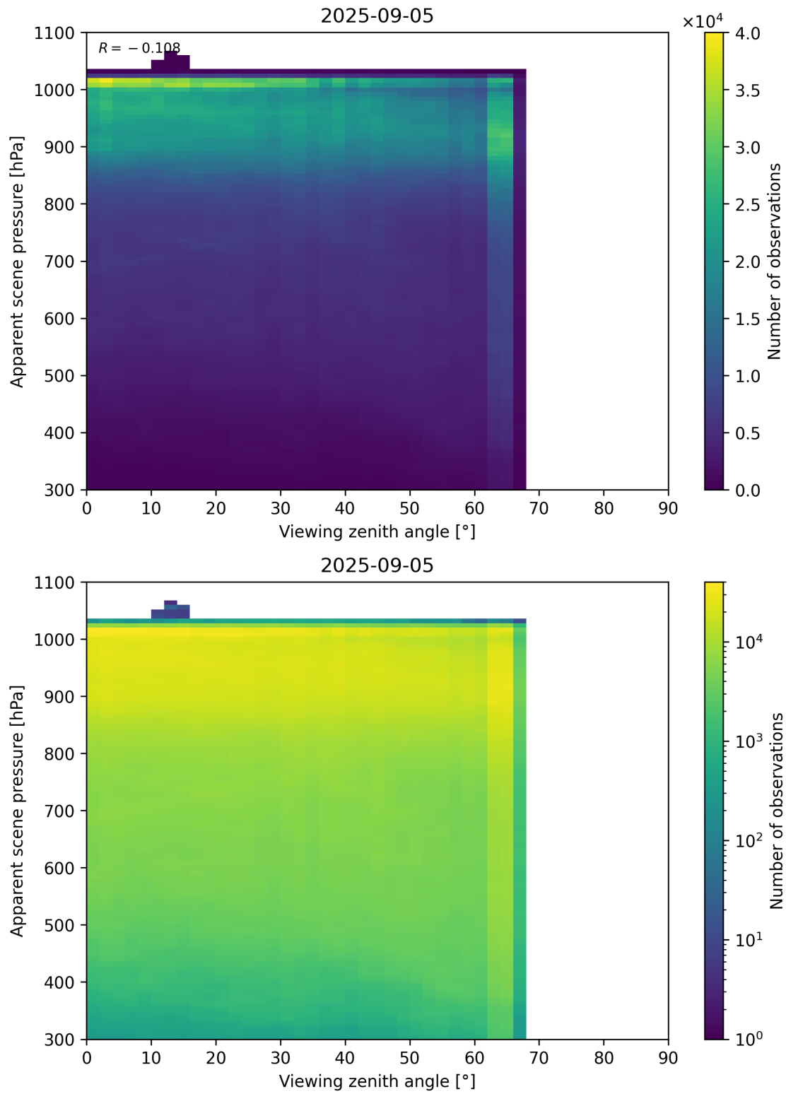
Figure 118: Scatter density plot of “Viewing zenith angle” against “Apparent scene pressure” for 2025-09-04 to 2025-09-06.
