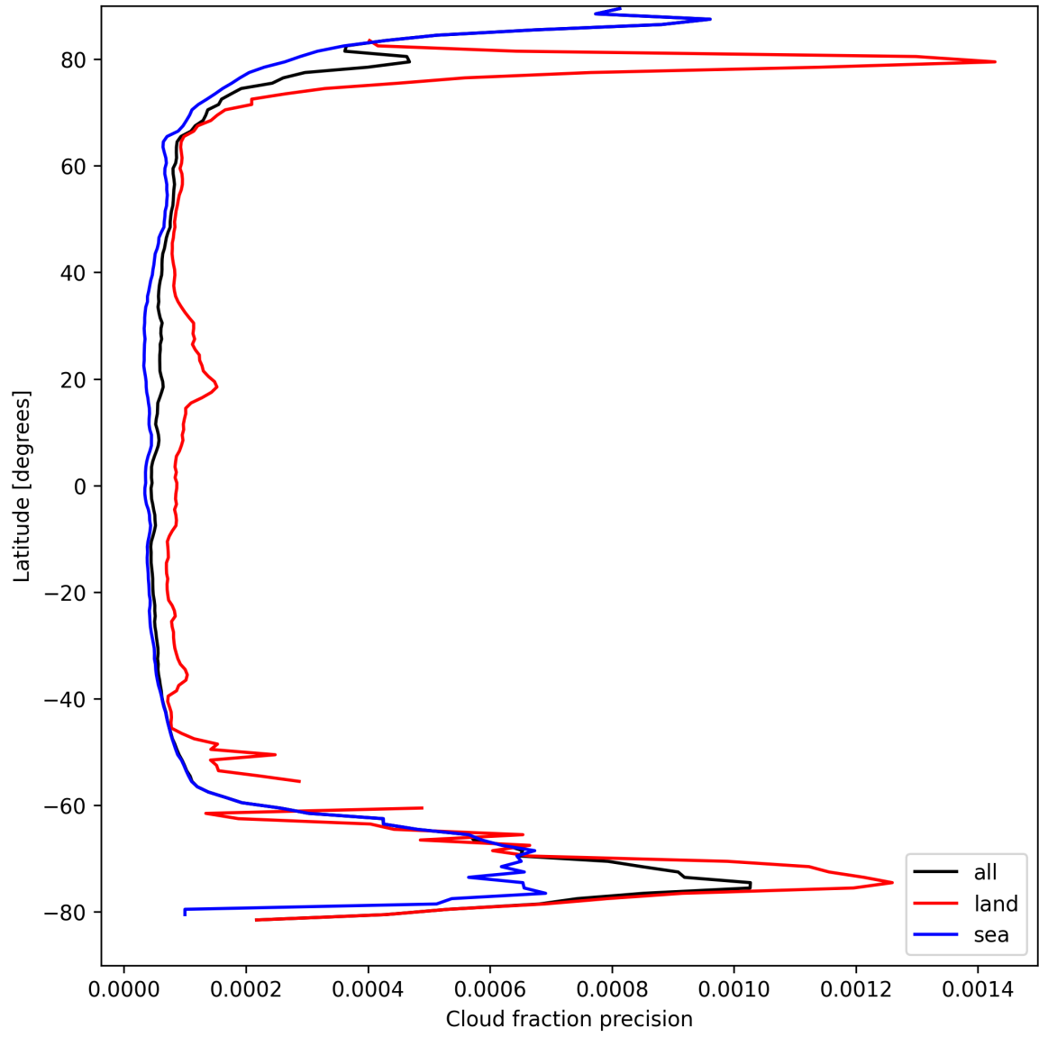
Figure 16: Zonal average of “Cloud fraction precision” for 2025-09-04 to 2025-09-06.
