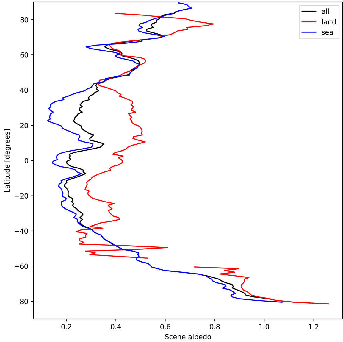
Figure 17: Zonal average of “Scene albedo” for 2025-09-04 to 2025-09-06.
