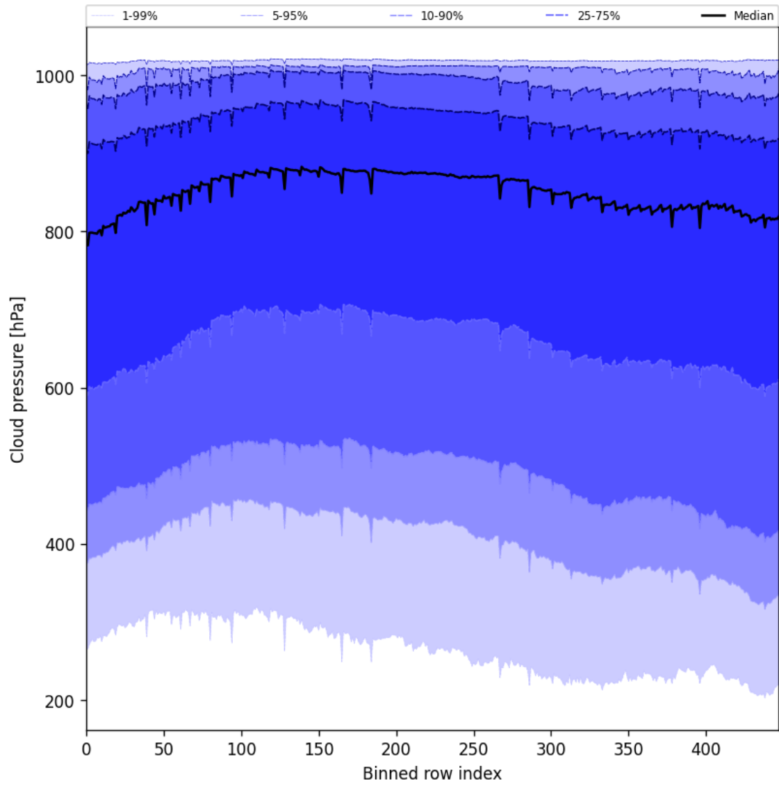
Figure 47: Along track statistics of “Cloud pressure” for 2025-09-04 to 2025-09-06
