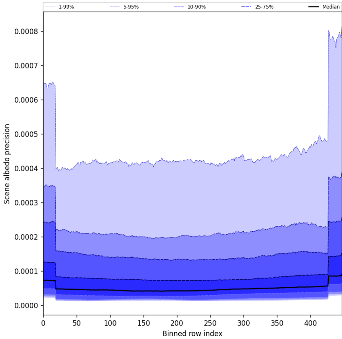
Figure 52: Along track statistics of “Scene albedo precision” for 2025-09-04 to 2025-09-06
