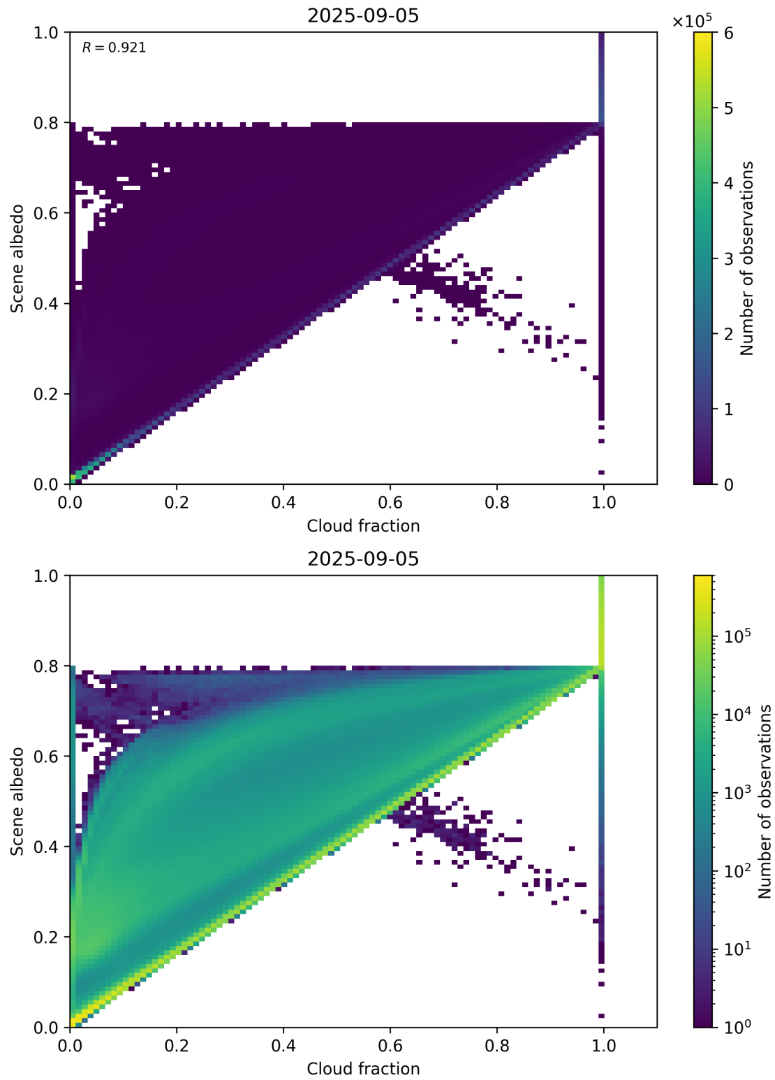
Figure 75: Scatter density plot of “Cloud fraction” against “Scene albedo” for 2025-09-04 to 2025-09-06.
