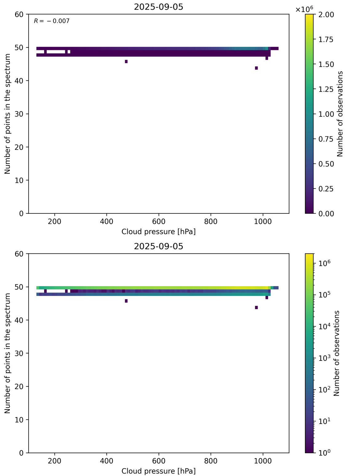
Figure 82: Scatter density plot of “Cloud pressure” against “Number of points in the spectrum” for 2025-09-04 to 2025-09-06.
