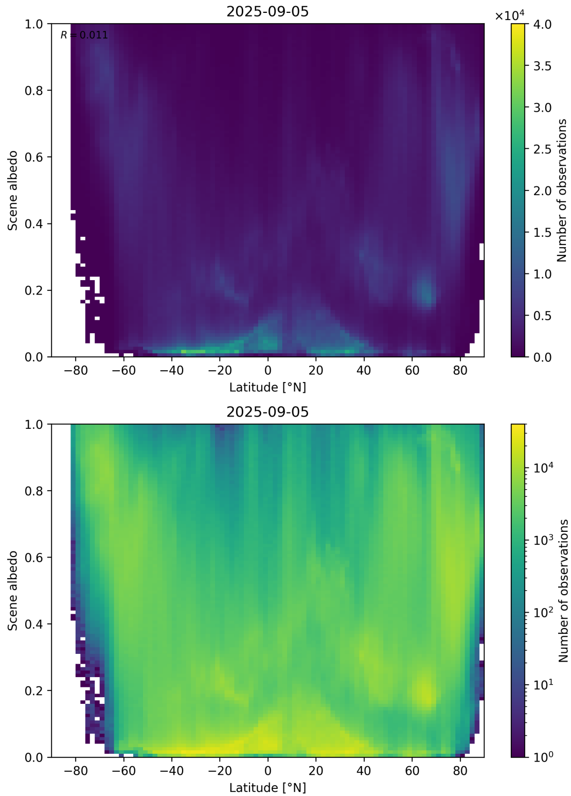
Figure 95: Scatter density plot of “Latitude” against “Scene albedo” for 2025-09-04 to 2025-09-06.
