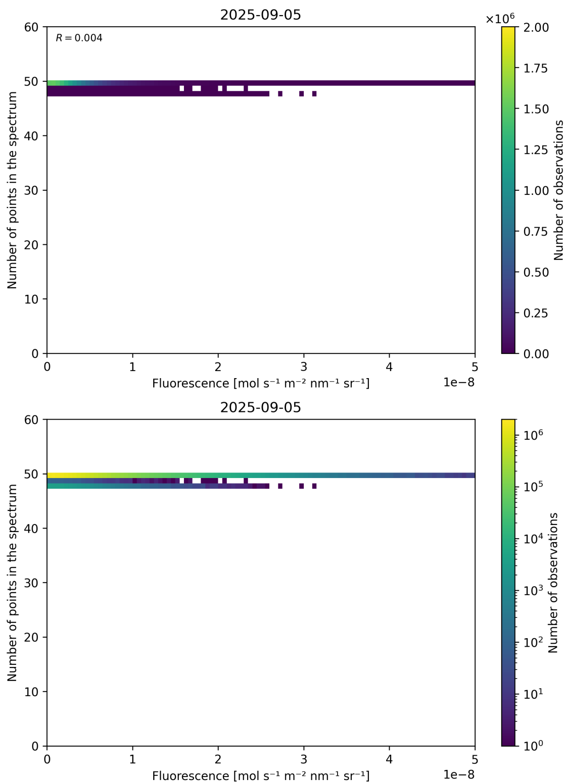
Figure 86: Scatter density plot of “Fluorescence” against “Number of points in the spectrum” for 2025-09-04 to 2025-09-06.
