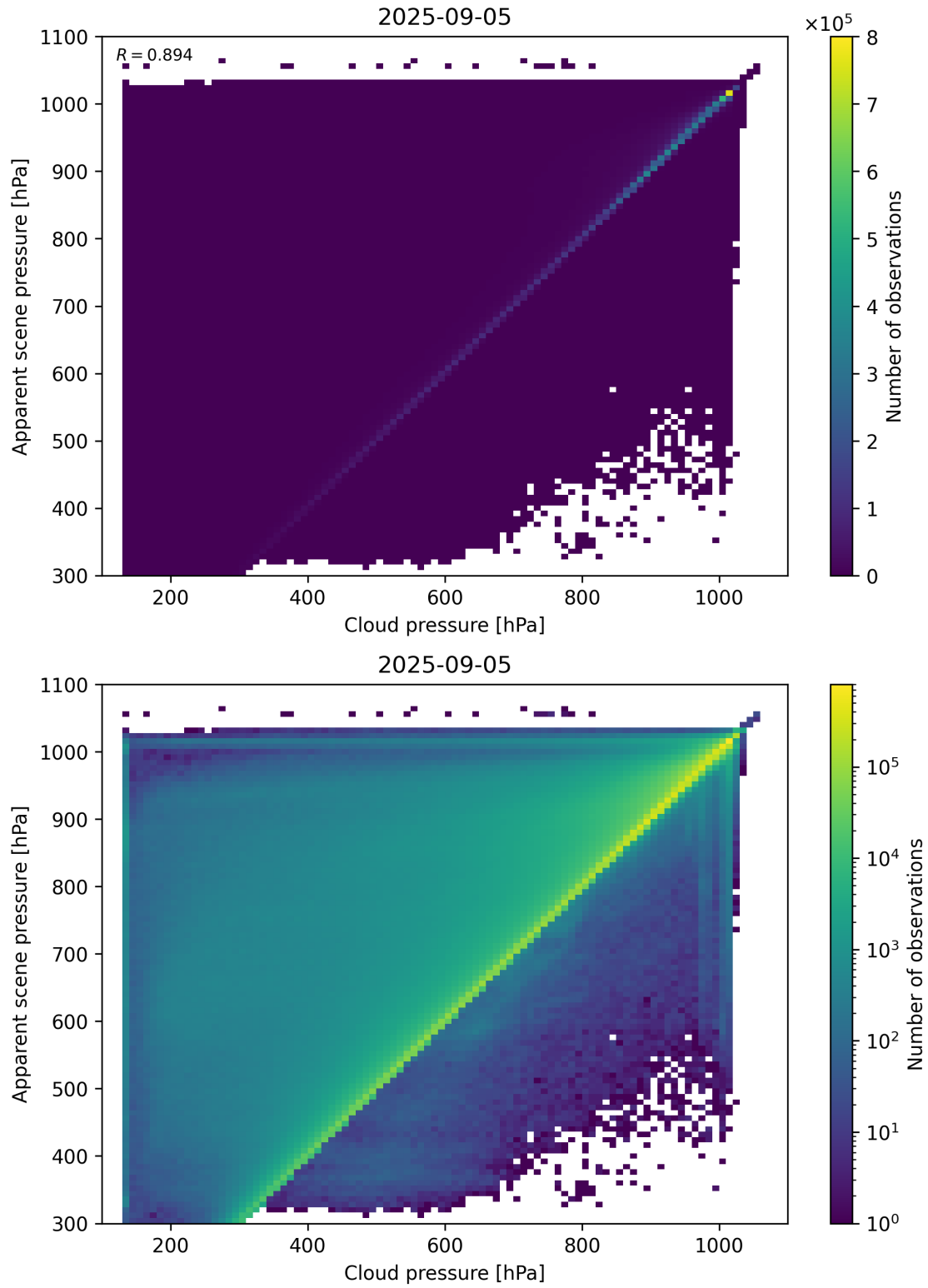
Figure 77: Scatter density plot of “Cloud pressure” against “Apparent scene pressure” for 2025-09-04 to 2025-09-06.
