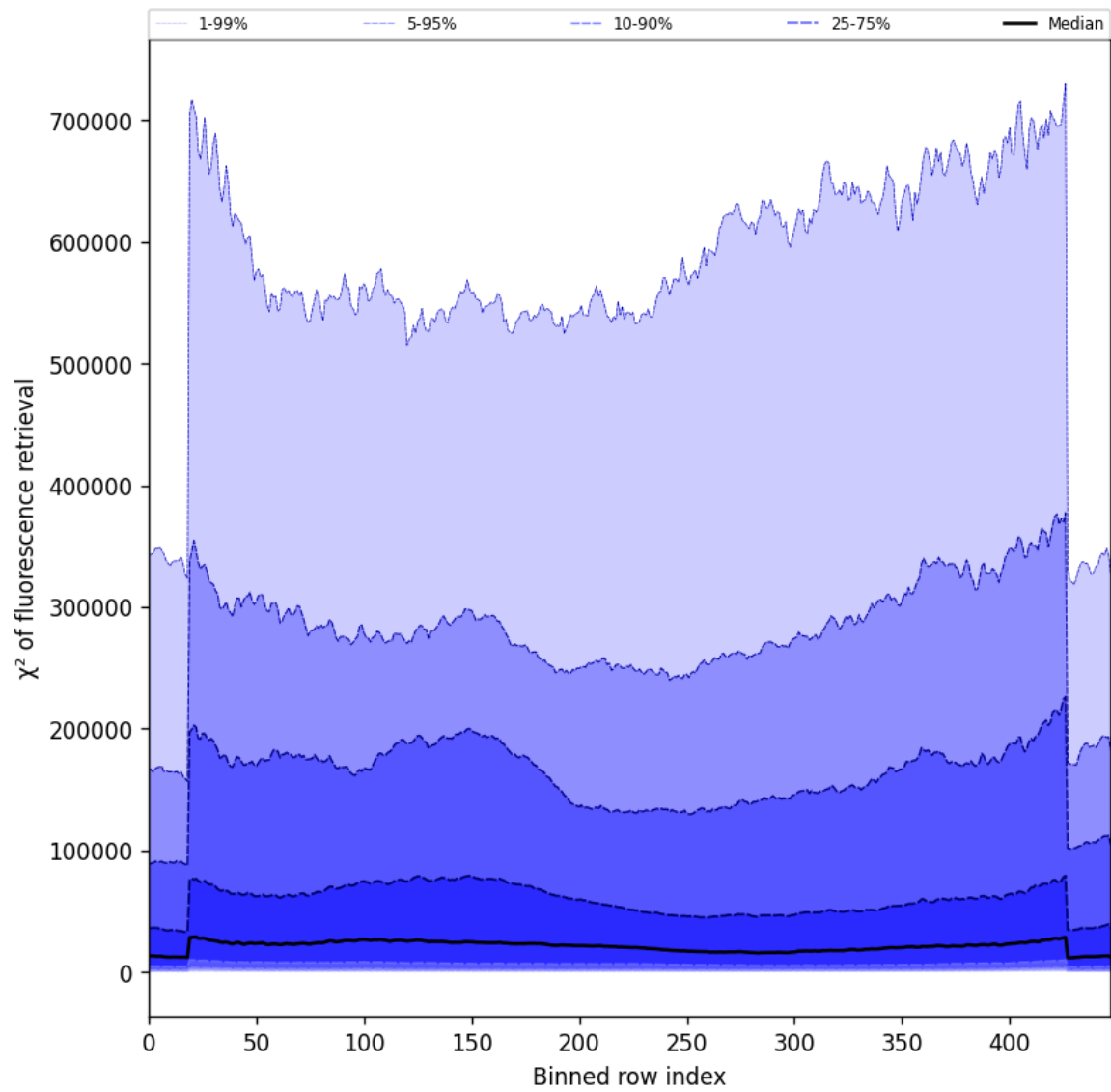
Figure 59: Along track statistics of “ \chi^2 of fluorescence retrieval” for 2025-09-04 to 2025-09-06
