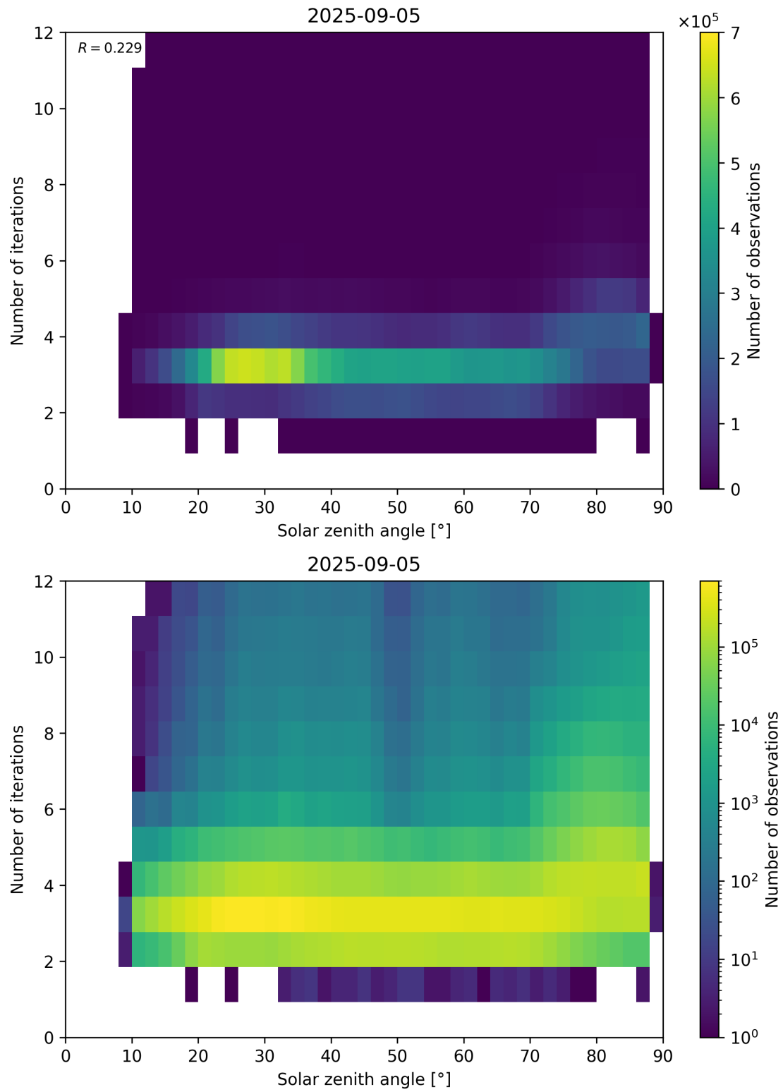
Figure 114: Scatter density plot of “Solar zenith angle” against “Number of iterations” for 2025-09-04 to 2025-09-06.
