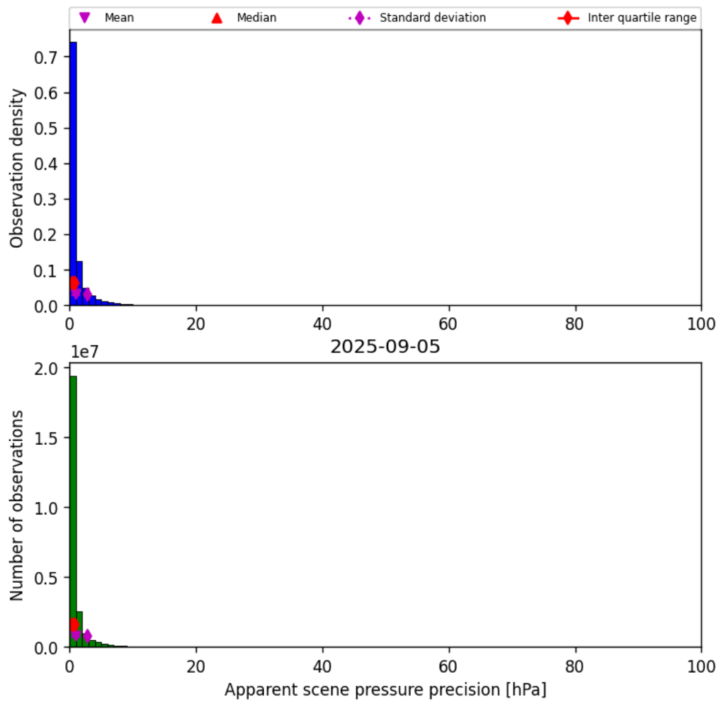
Figure 37: Histogram of “Apparent scene pressure precision” for 2025-09-04 to 2025-09-06
