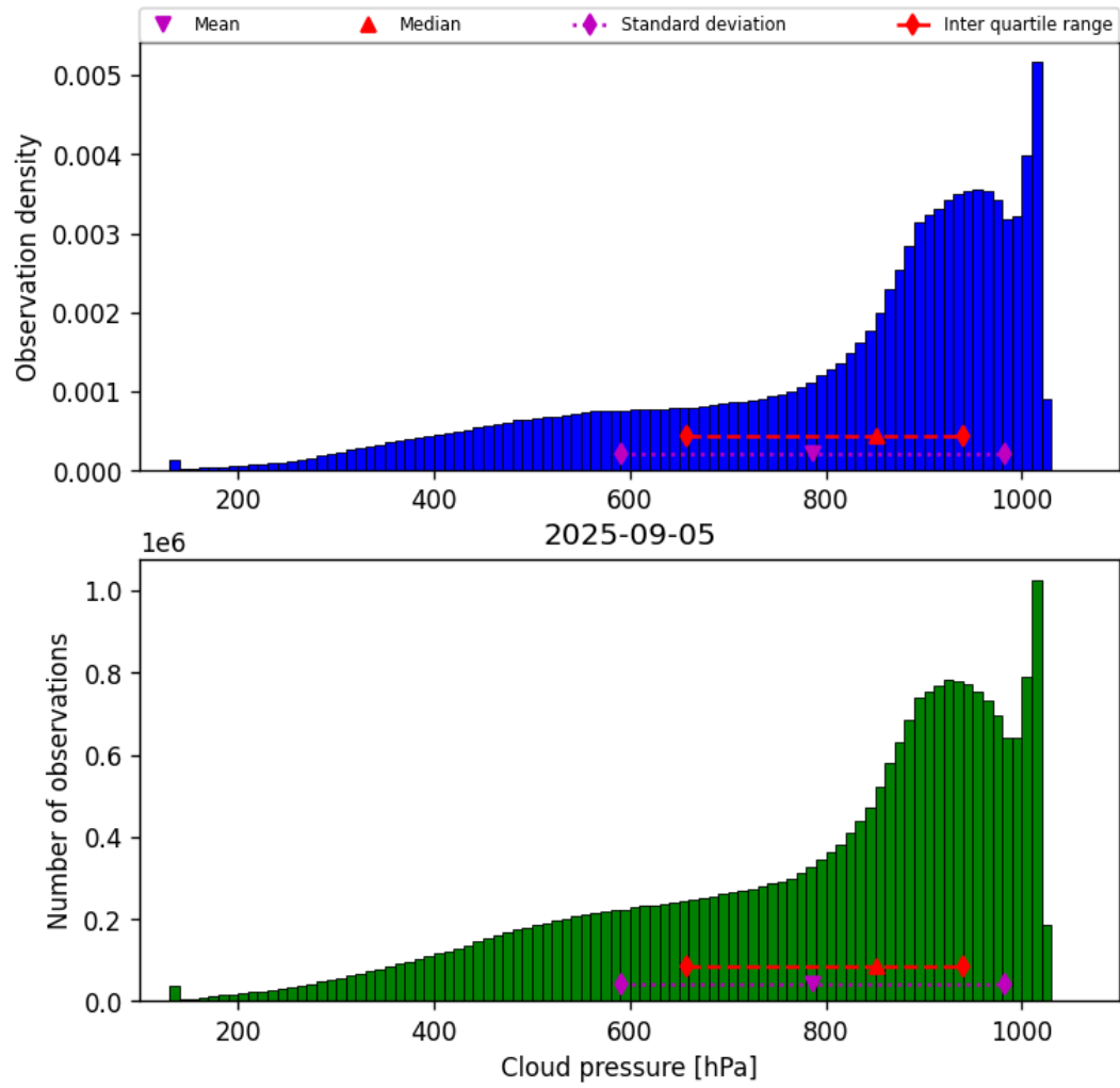
Figure 30: Histogram of “Cloud pressure” for 2025-09-04 to 2025-09-06
