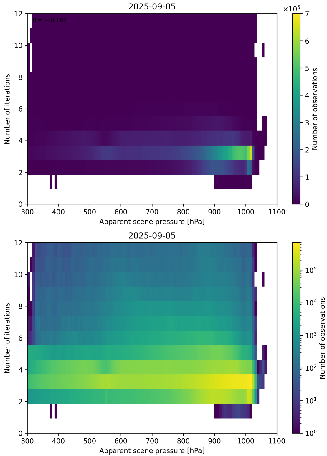
Figure 65: Scatter density plot of “Apparent scene pressure” against “Number of iterations” for 2025-09-04 to 2025-09-06.
