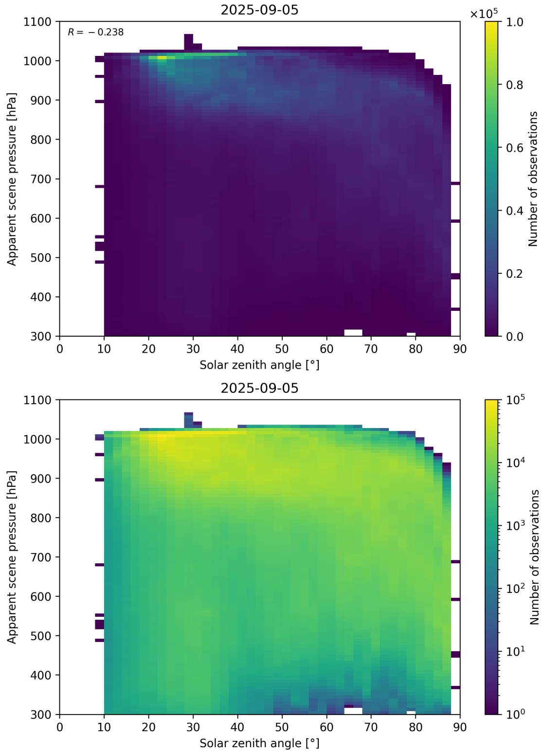
Figure 108: Scatter density plot of “Solar zenith angle” against “Apparent scene pressure” for 2025-09-04 to 2025-09-06.
