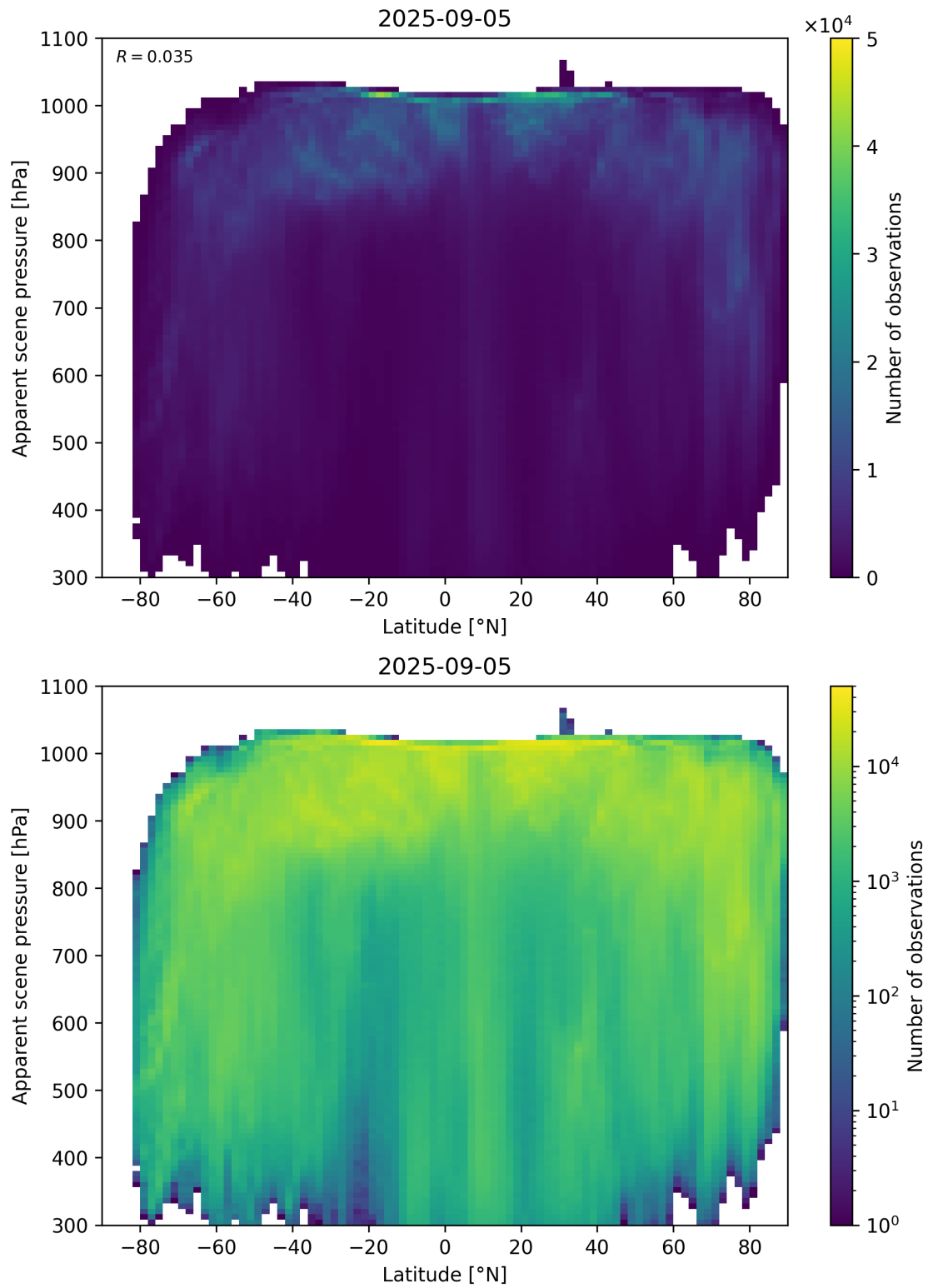
Figure 88: Scatter density plot of “Latitude” against “Apparent scene pressure” for 2025-09-04 to 2025-09-06.
