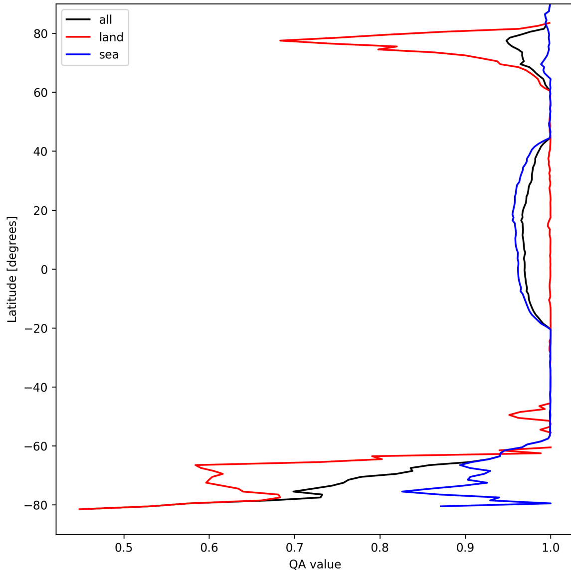
Figure 12: Zonal average of "QA value" for 2025-09-04 to 2025-09-06.
