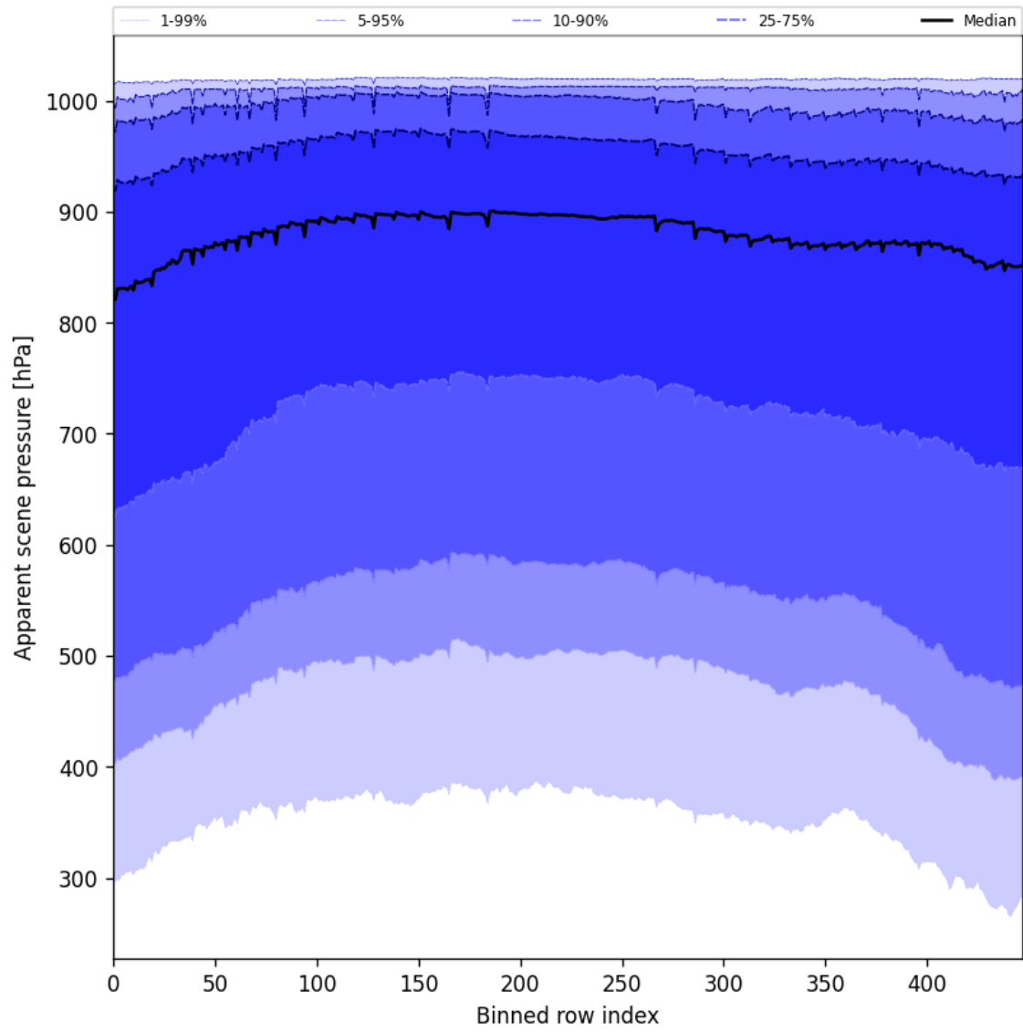
Figure 53: Along track statistics of “Apparent scene pressure” for 2025-09-04 to 2025-09-06
