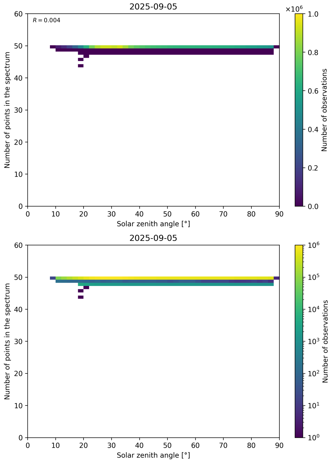
Figure 115: Scatter density plot of “Solar zenith angle” against “Number of points in the spectrum” for 2025-09-04 to 2025-09-06.
