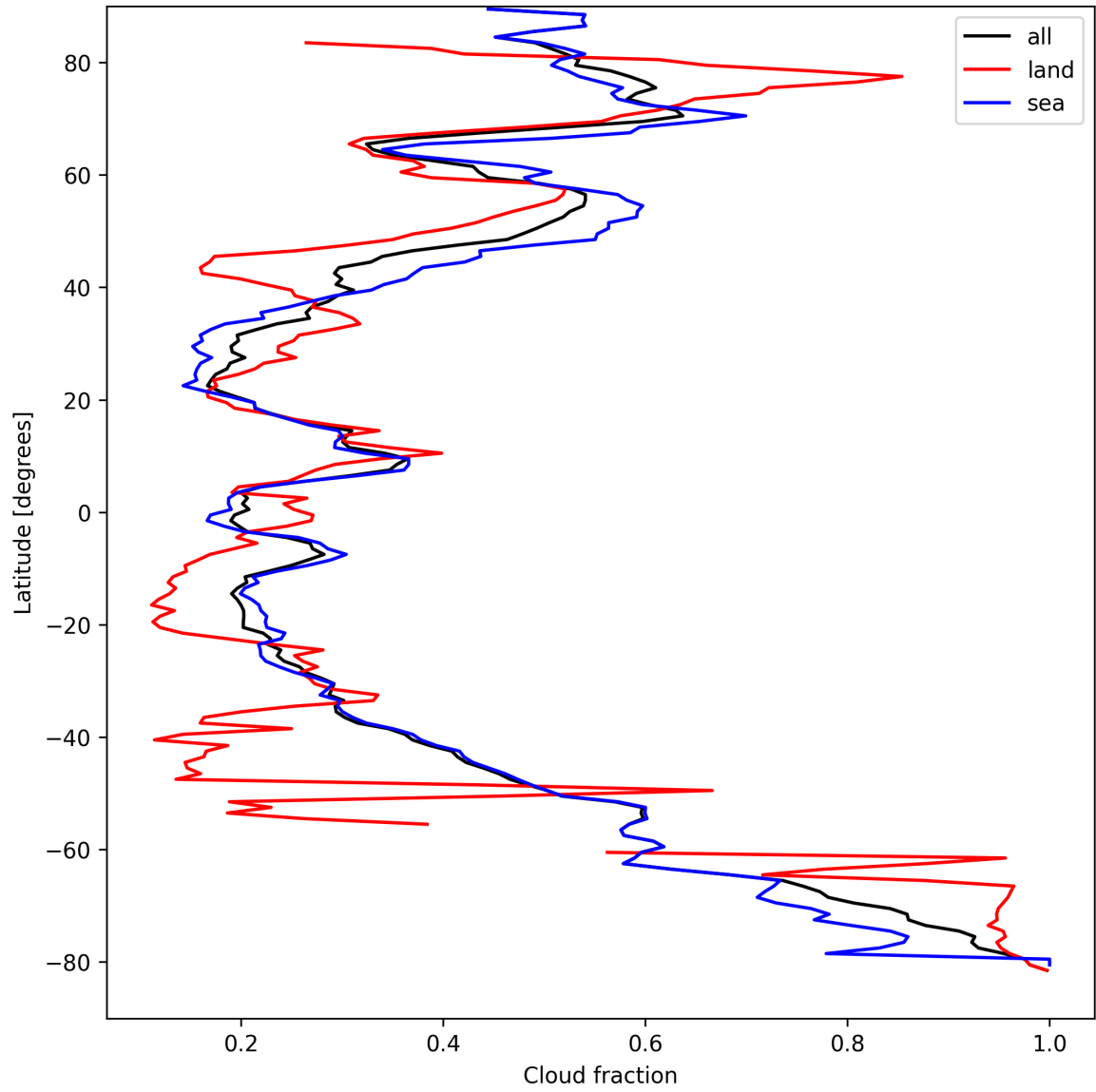
Figure 15: Zonal average of “Cloud fraction” for 2025-09-04 to 2025-09-06.
