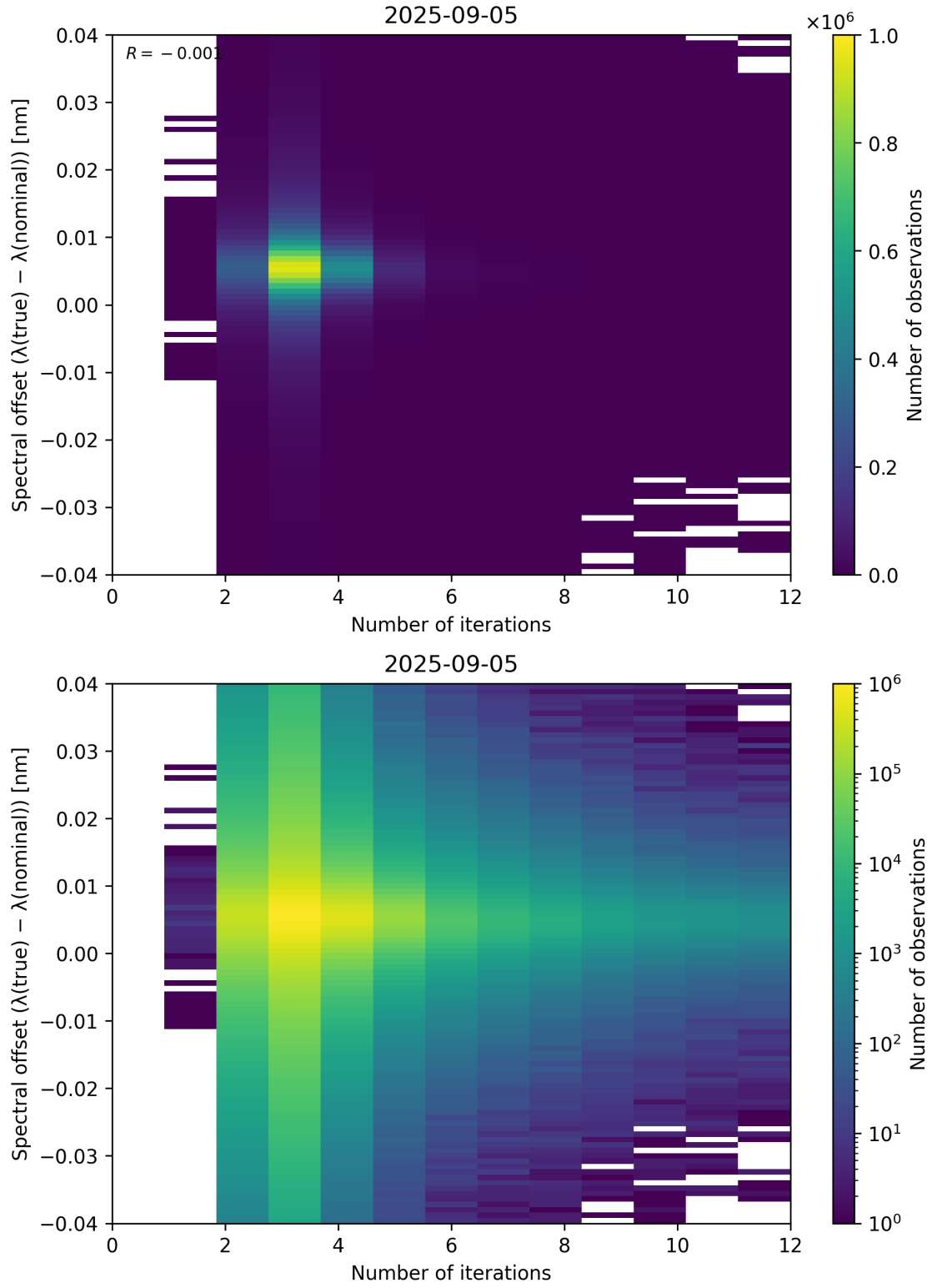
Figure 100: Scatter density plot of “Number of iterations” against “Spectral offset ( \lambda_{\text{true}} - \lambda_{\text{nominal}} )” for 2025-09-04 to 2025-09-06.
