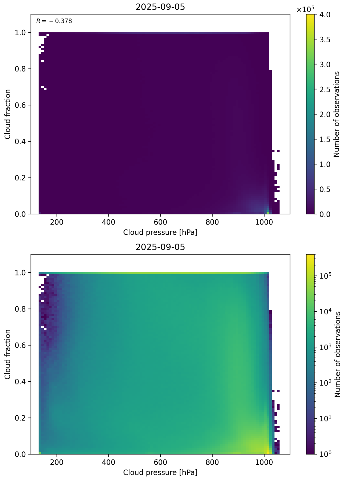
Figure 79: Scatter density plot of “Cloud pressure” against “Cloud fraction” for 2025-09-04 to 2025-09-06.
