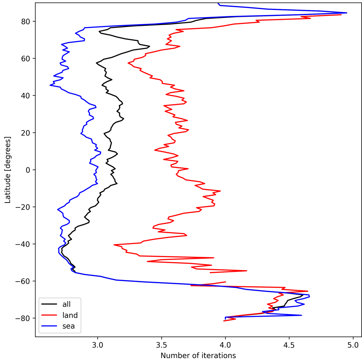
Figure 22: Zonal average of “Number of iterations” for 2025-09-04 to 2025-09-06.
