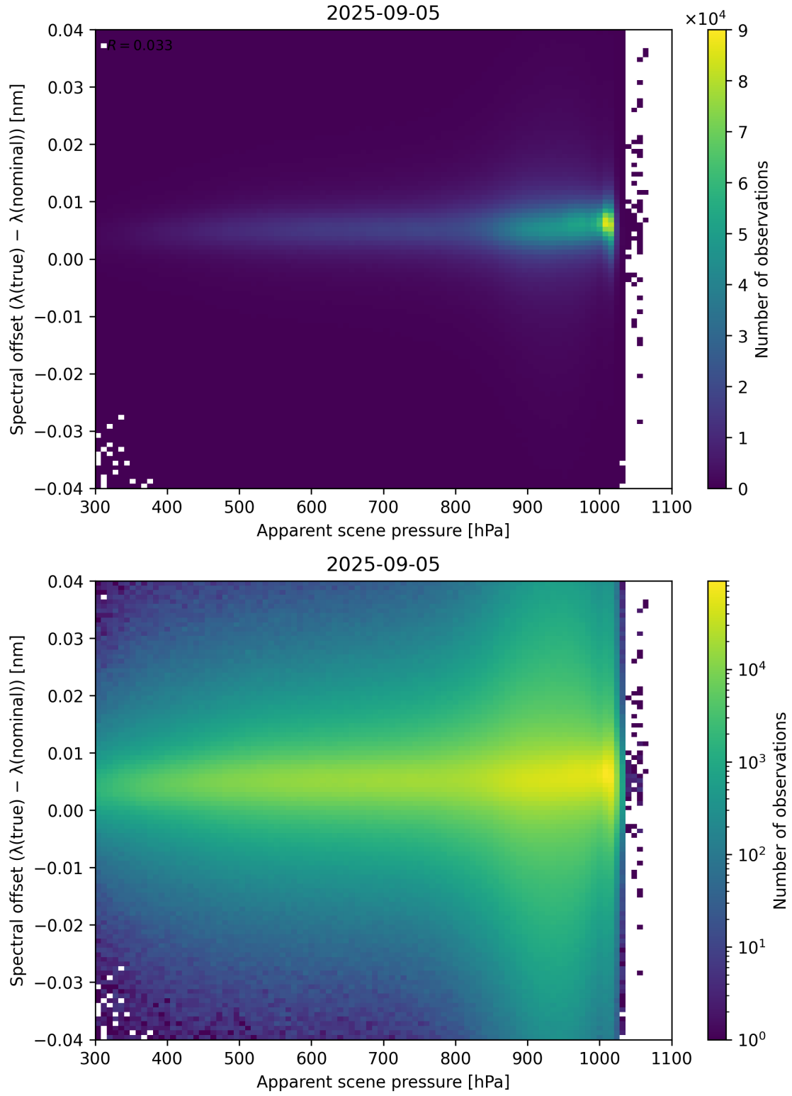
Figure 67: Scatter density plot of “Apparent scene pressure” against “Spectral offset ( \lambda_{\text{true}} - \lambda_{\text{nominal}} )” for 2025-09-04 to 2025-09-06.
