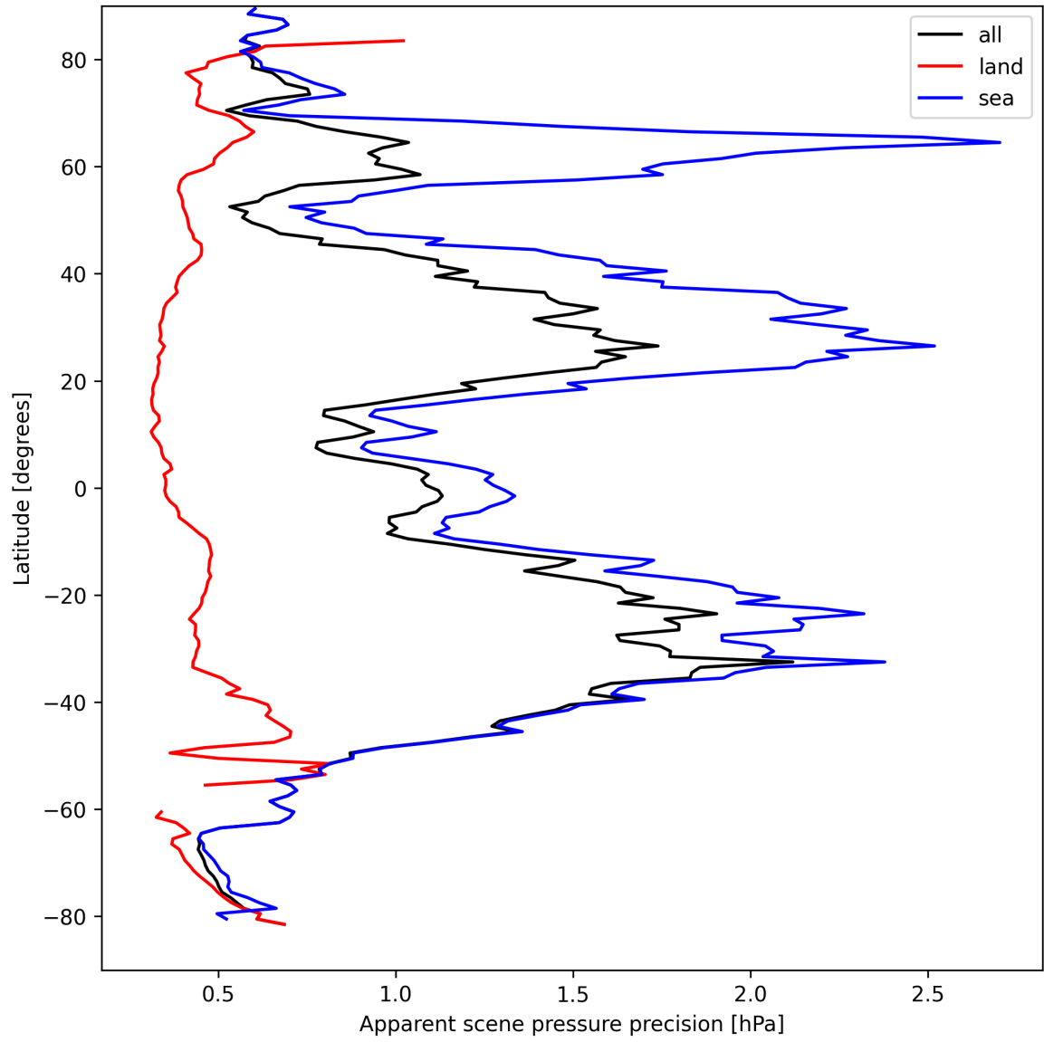
Figure 20: Zonal average of “Apparent scene pressure precision” for 2025-09-04 to 2025-09-06.
