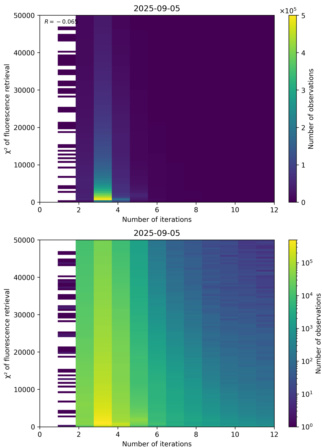
Figure 97: Scatter density plot of “Number of iterations” against “ \chi^2 of fluorescence retrieval” for 2025-09-04 to 2025-09-06.
