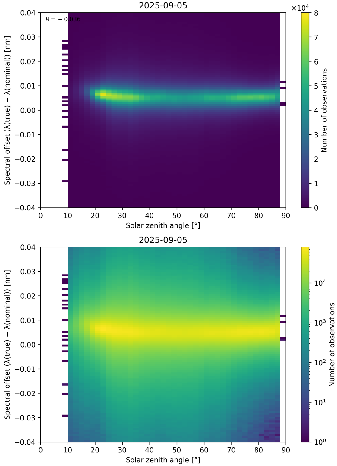
Figure 117: Scatter density plot of “Solar zenith angle” against “Spectral offset ( \lambda_{\text{true}} - \lambda_{\text{nominal}} )” for 2025-09-04 to 2025-09-06.
