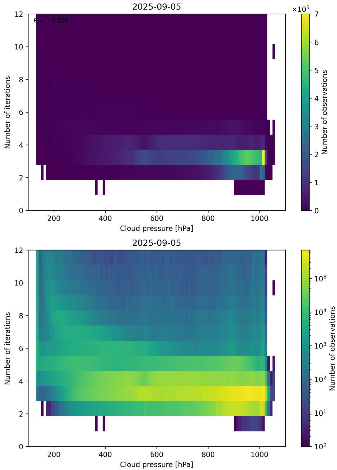
Figure 81: Scatter density plot of “Cloud pressure” against “Number of iterations” for 2025-09-04 to 2025-09-06.
