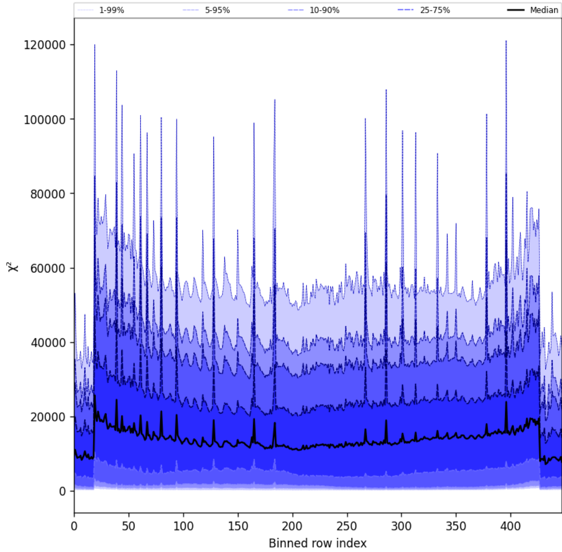
Figure 55: Along track statistics of “ \chi^2 ” for 2025-09-04 to 2025-09-06
