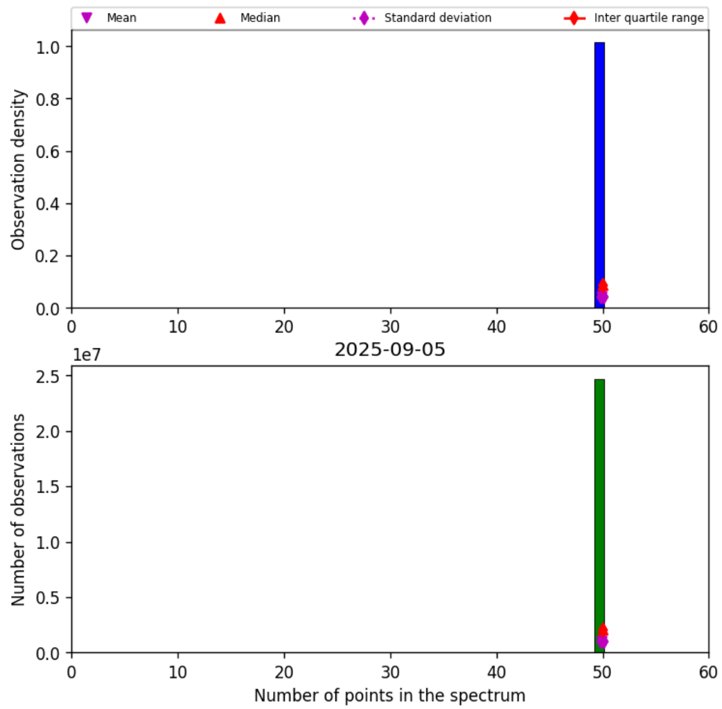
Figure 44: Histogram of “Number of points in the spectrum” for 2025-09-04 to 2025-09-06
