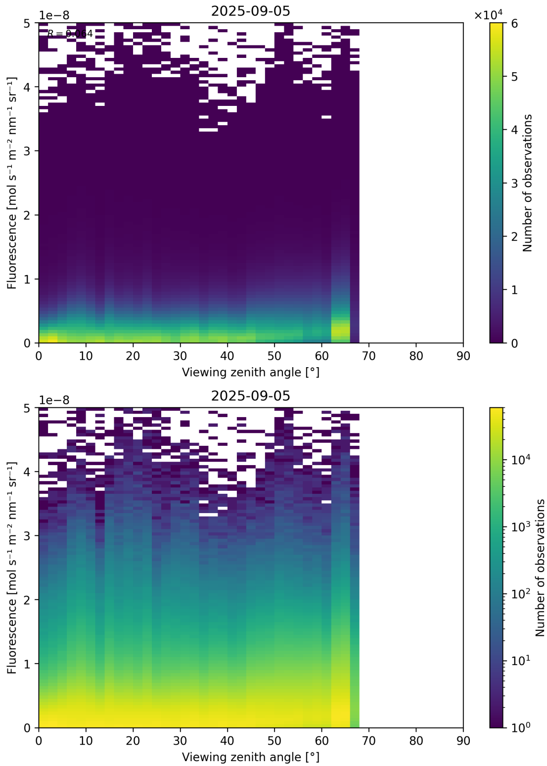
Figure 122: Scatter density plot of “Viewing zenith angle” against “Fluorescence” for 2025-09-04 to 2025-09-06.
