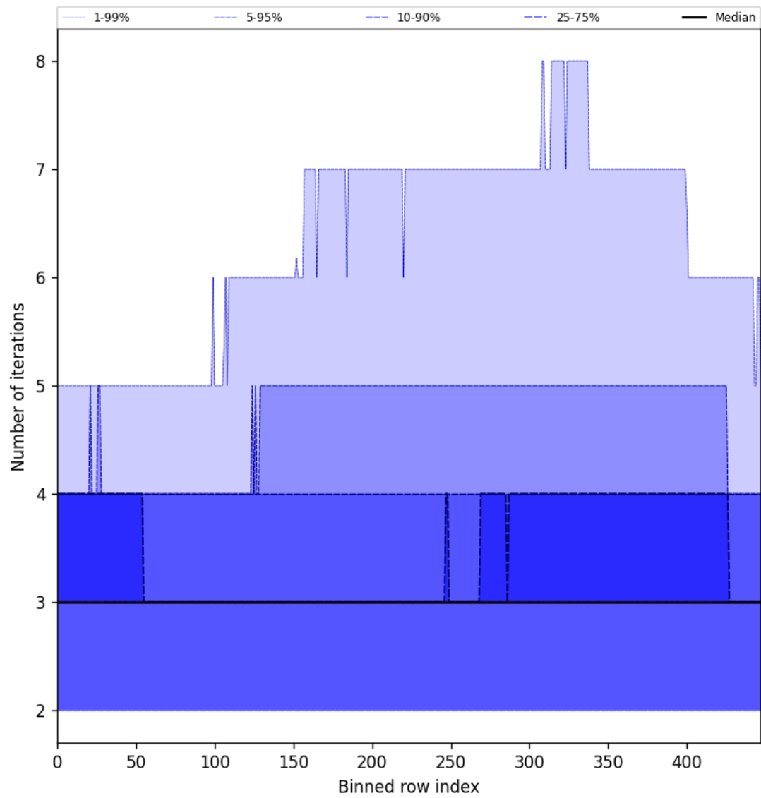
Figure 56: Along track statistics of “Number of iterations” for 2025-09-04 to 2025-09-06
