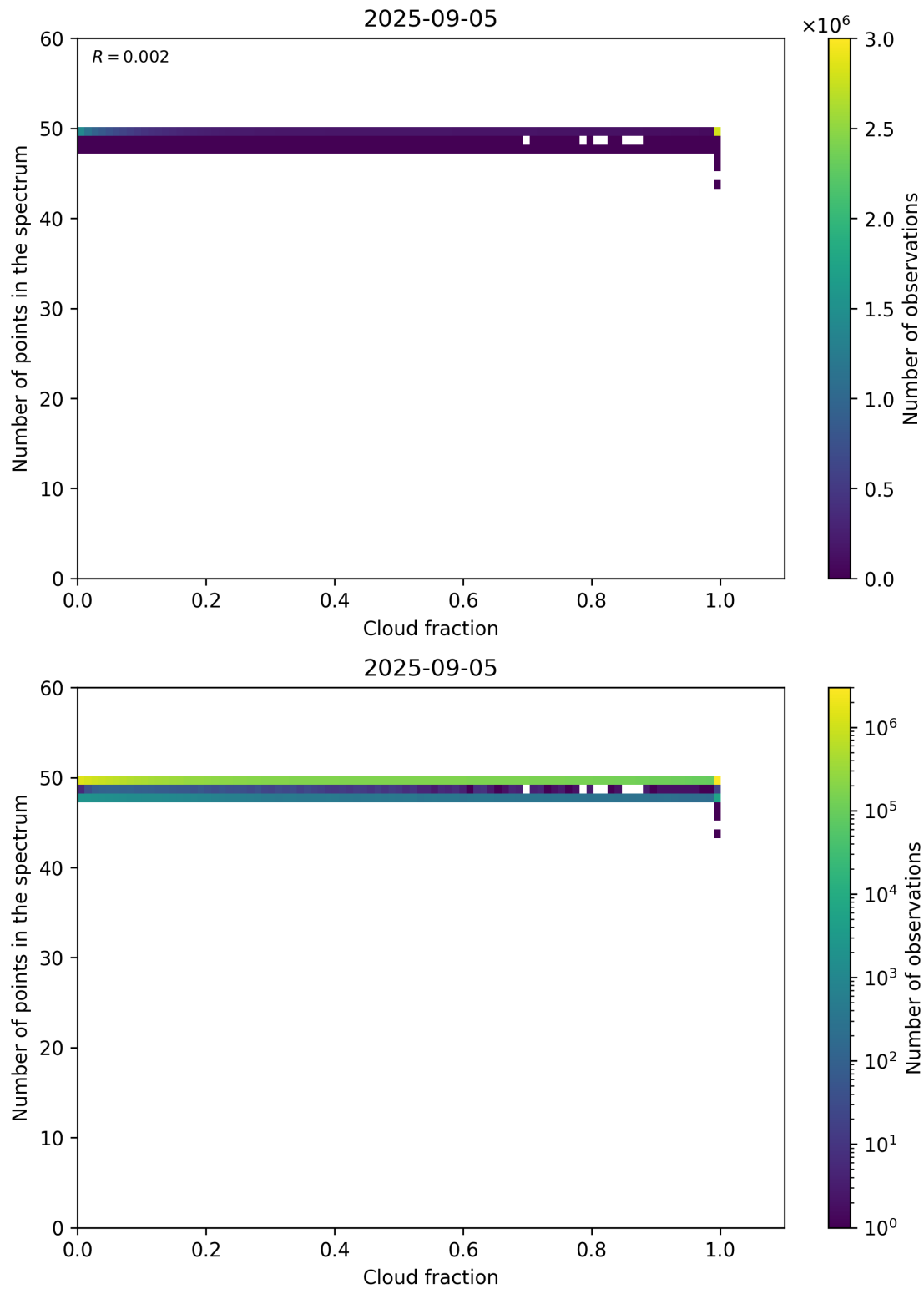
Figure 74: Scatter density plot of “Cloud fraction” against “Number of points in the spectrum” for 2025-09-04 to 2025-09-06.
