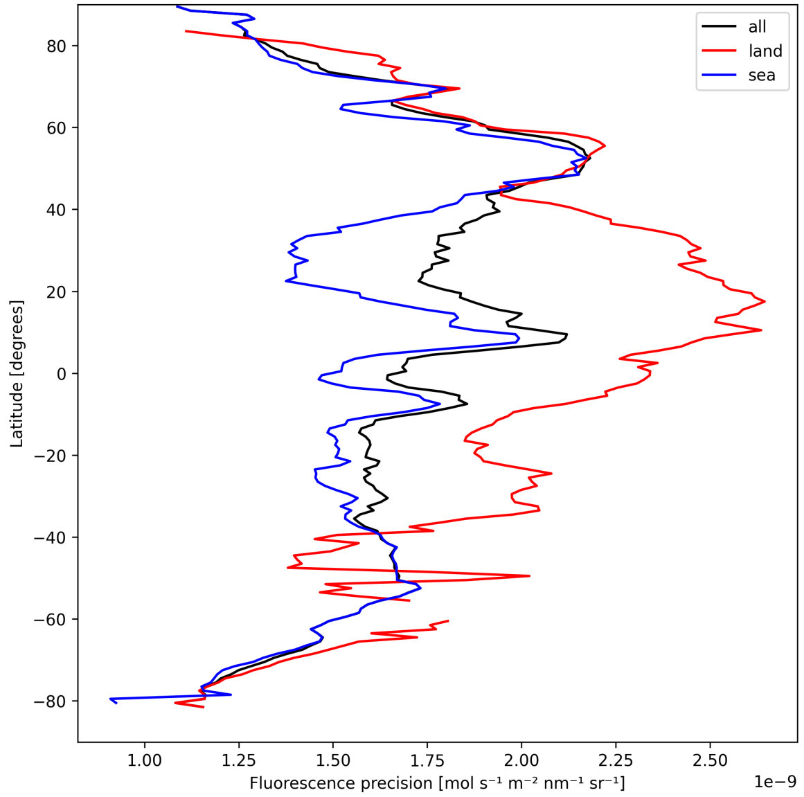
Figure 24: Zonal average of “Fluorescence precision” for 2025-09-04 to 2025-09-06.
