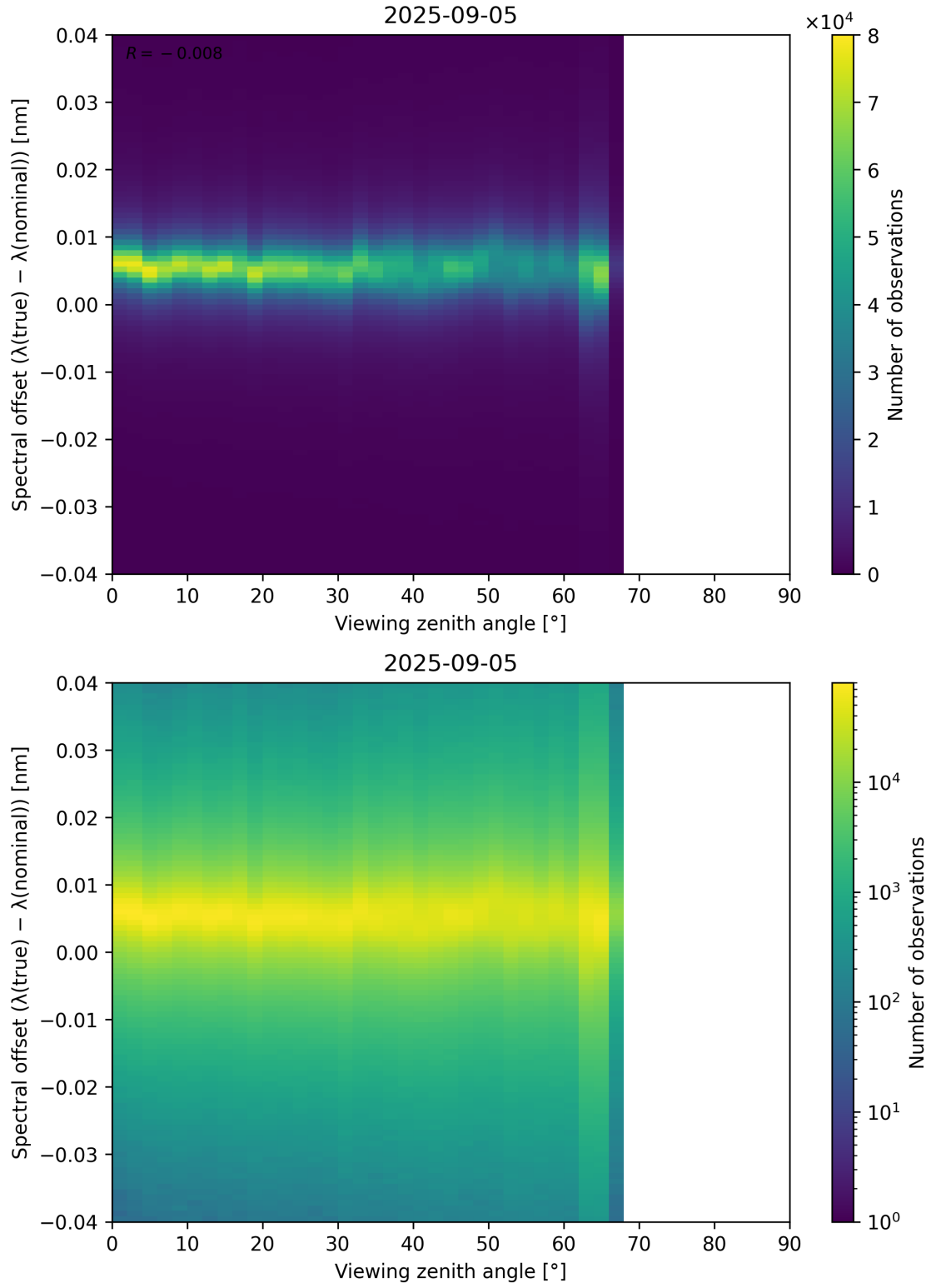
Figure 128: Scatter density plot of “Viewing zenith angle” against “Spectral offset ( \lambda_{\text{true}} - \lambda_{\text{nominal}} )” for 2025-09-04 to 2025-09-06.
