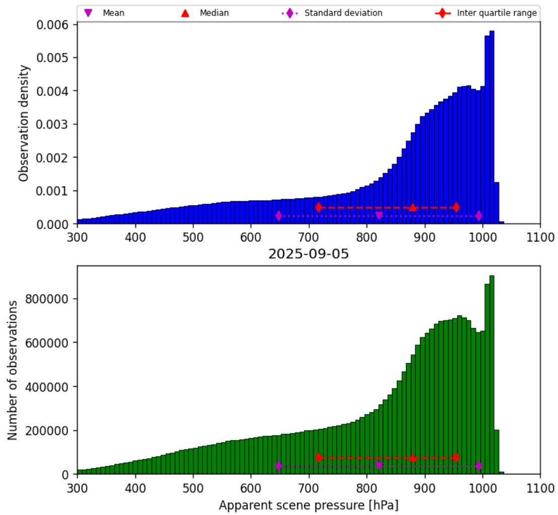
Figure 36: Histogram of “Apparent scene pressure” for 2025-09-04 to 2025-09-06
