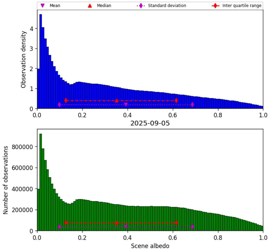
Figure 34: Histogram of “Scene albedo” for 2025-09-04 to 2025-09-06
