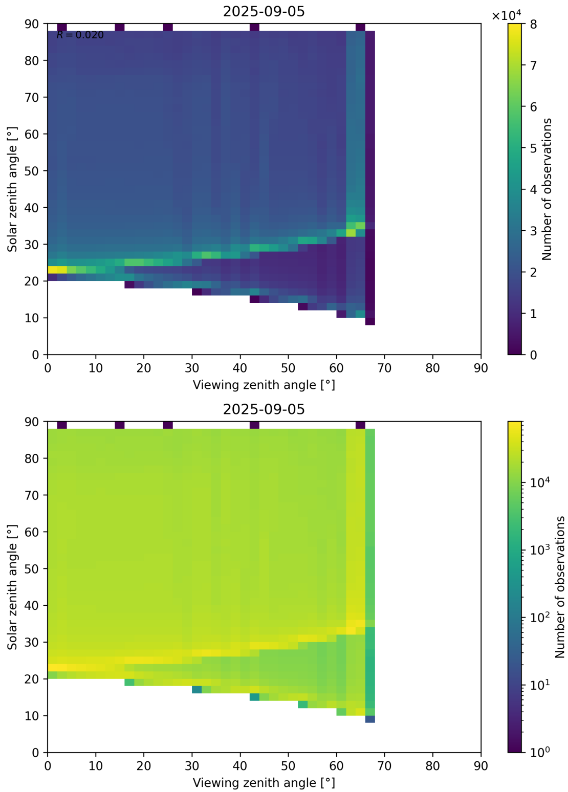
Figure 127: Scatter density plot of “Viewing zenith angle” against “Solar zenith angle” for 2025-09-04 to 2025-09-06.
