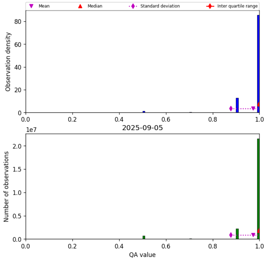
Figure 29: Histogram of “QA value” for 2025-09-04 to 2025-09-06
