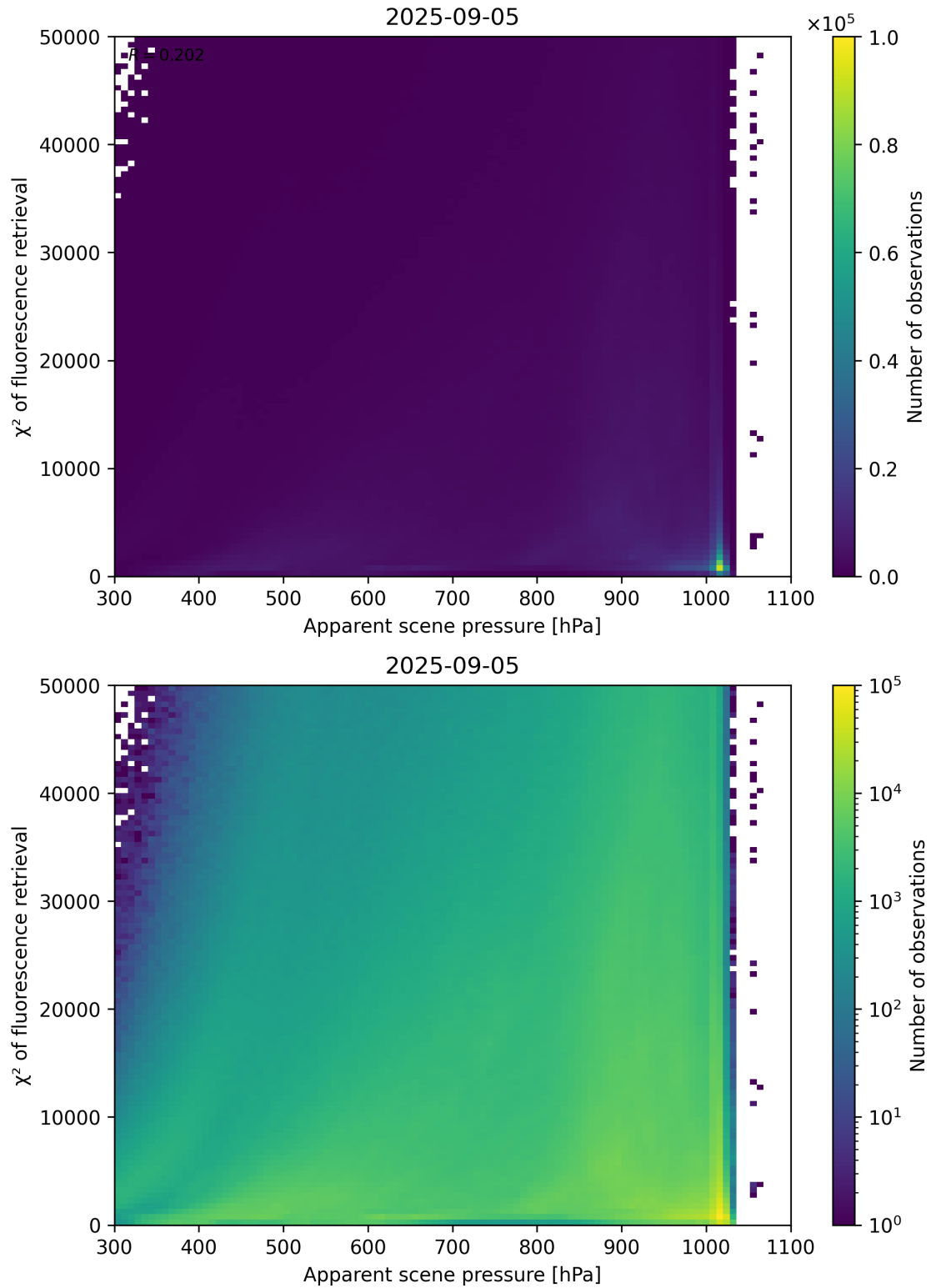
Figure 63: Scatter density plot of “Apparent scene pressure” against “ \chi^2 of fluorescence retrieval” for 2025-09-04 to 2025-09-06.
