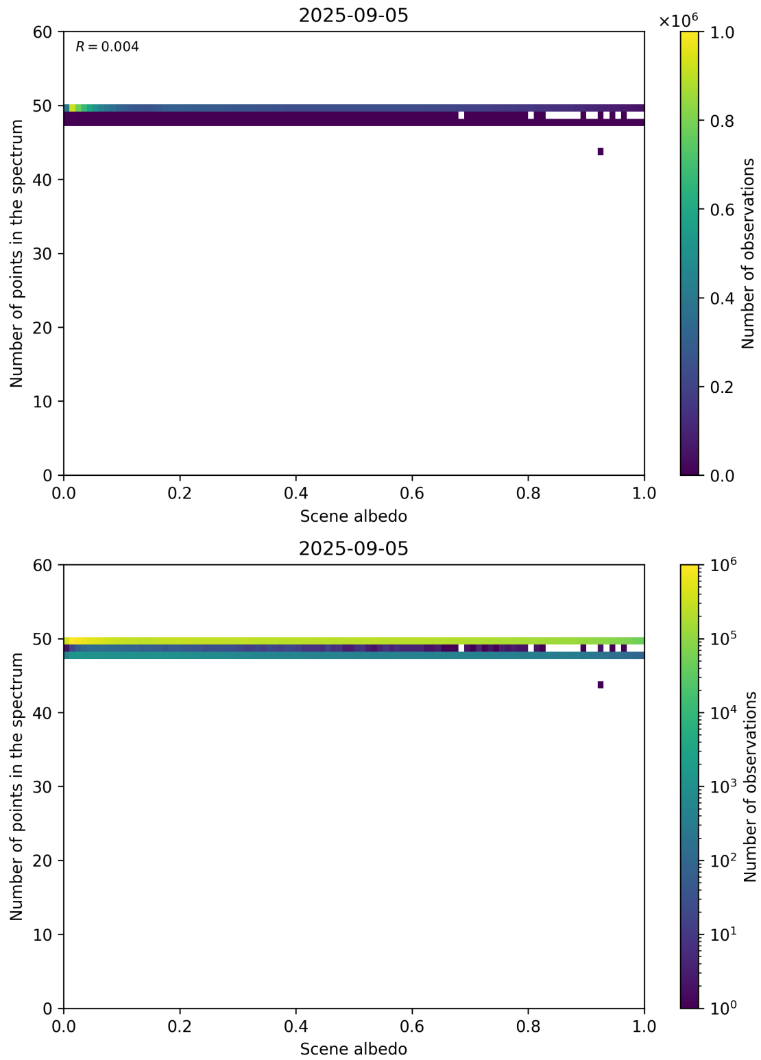
Figure 106: Scatter density plot of “Scene albedo” against “Number of points in the spectrum” for 2025-09-04 to 2025-09-06.
