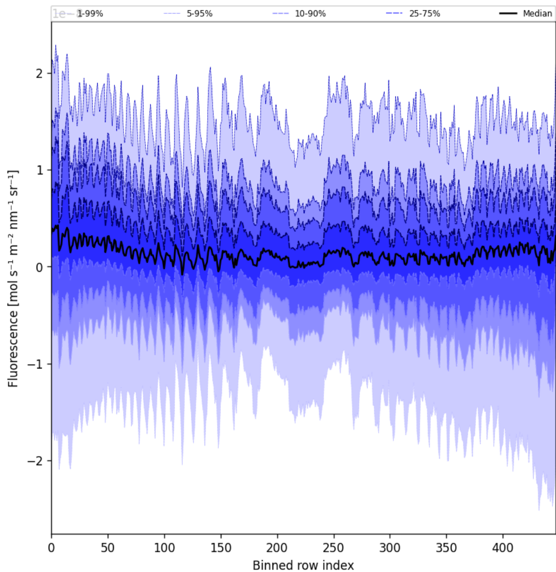
Figure 57: Along track statistics of “Fluorescence” for 2025-09-04 to 2025-09-06
