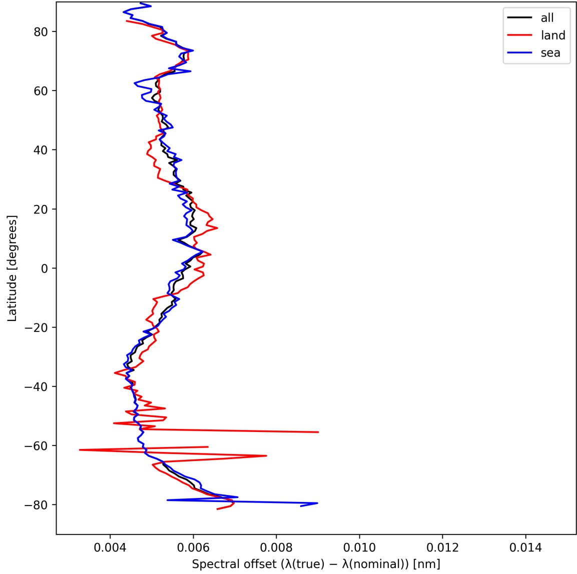
Figure 28: Zonal average of “Spectral offset ( \lambda_{\text{true}} - \lambda_{\text{nominal}} )” for 2025-09-04 to 2025-09-06.
