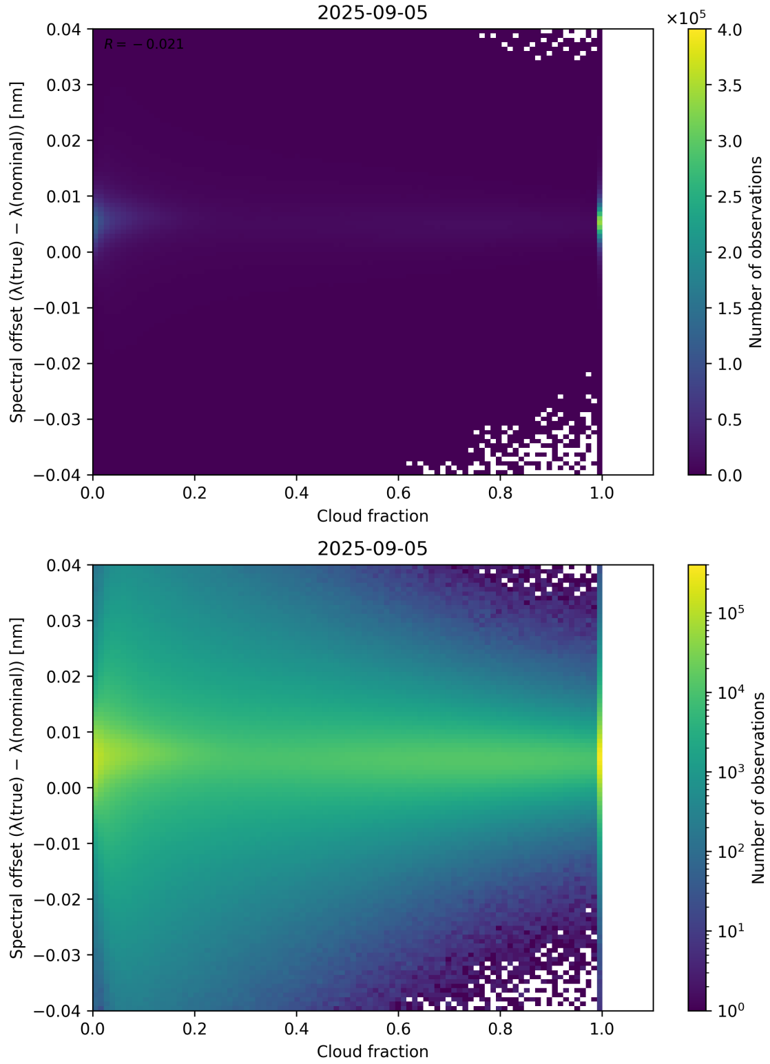
Figure 76: Scatter density plot of “Cloud fraction” against “Spectral offset ( \lambda_{\text{true}} - \lambda_{\text{nominal}} )” for 2025-09-04 to 2025-09-06.
