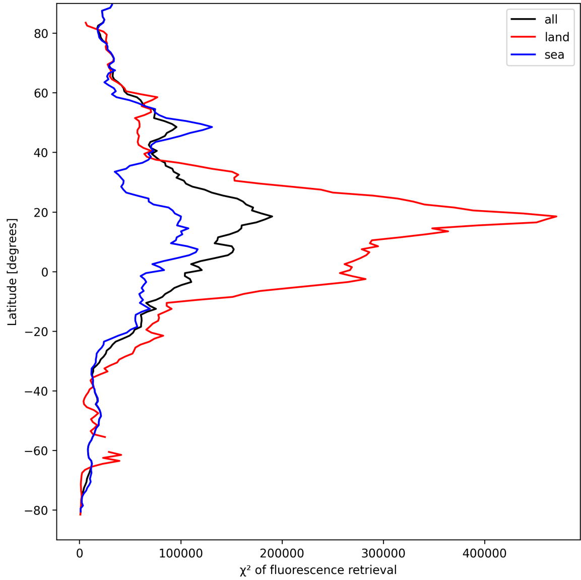
Figure 25: Zonal average of “ \chi^2 of fluorescence retrieval” for 2025-09-04 to 2025-09-06.
