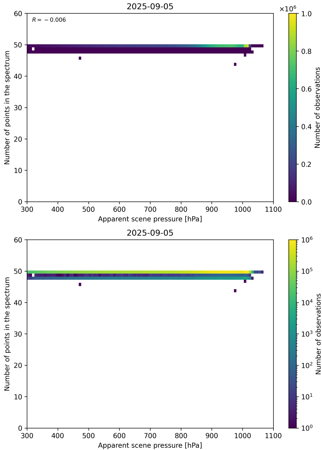
Figure 66: Scatter density plot of “Apparent scene pressure” against “Number of points in the spectrum” for 2025-09-04 to 2025-09-06.
