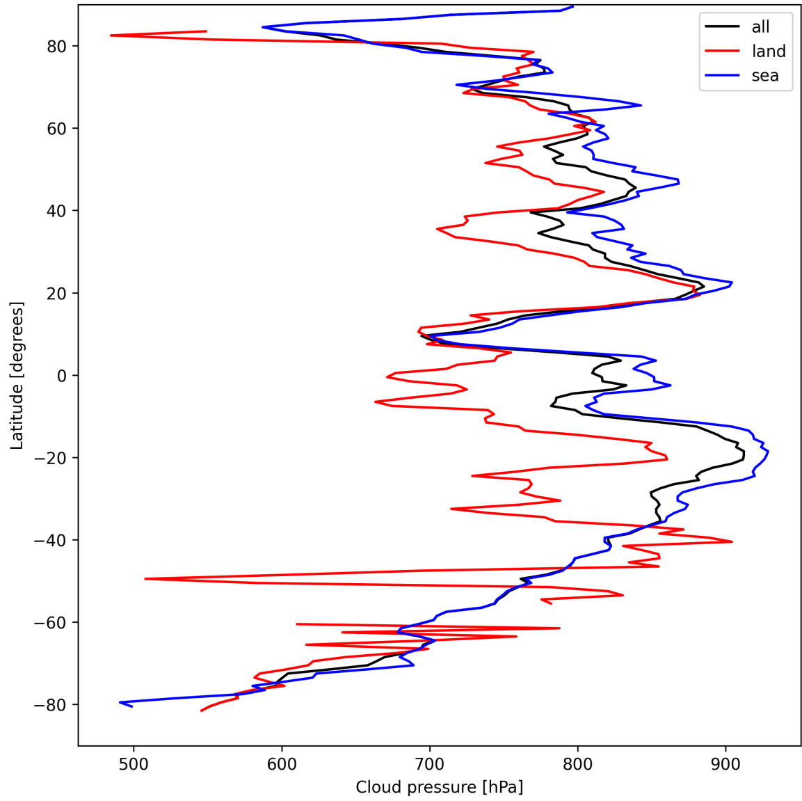
Figure 13: Zonal average of “Cloud pressure” for 2025-09-04 to 2025-09-06.
