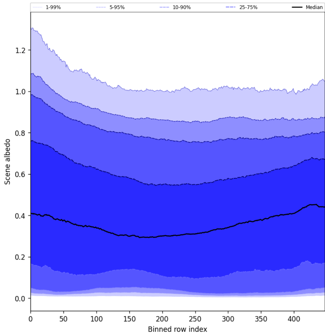
Figure 51: Along track statistics of “Scene albedo” for 2025-09-04 to 2025-09-06
