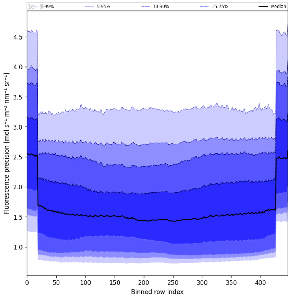
Figure 58: Along track statistics of “Fluorescence precision” for 2025-09-04 to 2025-09-06
