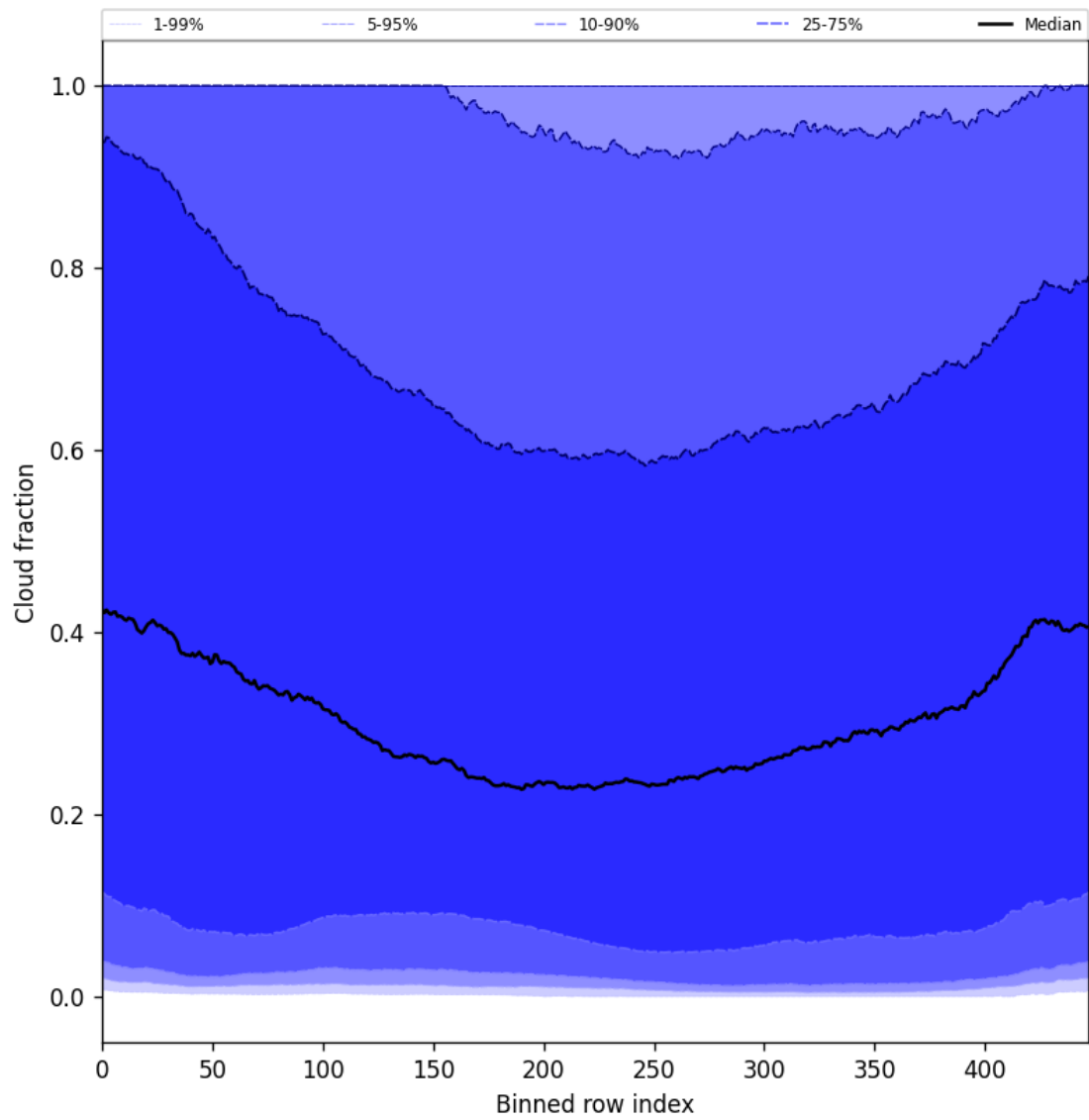
Figure 49: Along track statistics of “Cloud fraction” for 2025-09-04 to 2025-09-06
