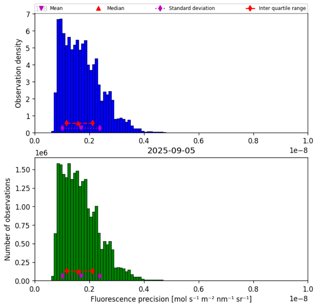
Figure 41: Histogram of “Fluorescence precision” for 2025-09-04 to 2025-09-06
