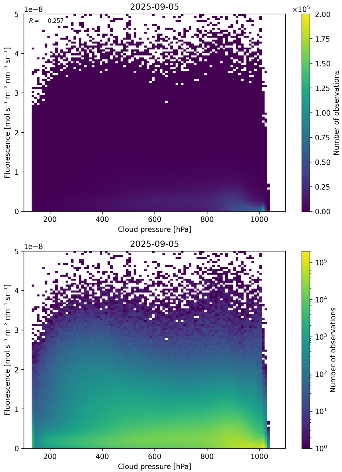
Figure 80: Scatter density plot of “Cloud pressure” against “Fluorescence” for 2025-09-04 to 2025-09-06.
