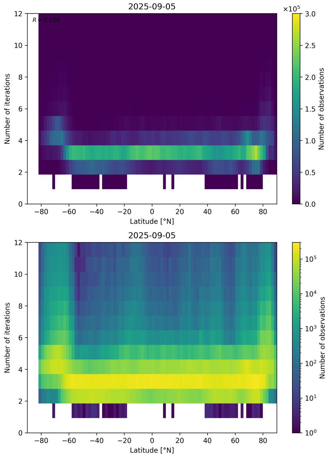
Figure 93: Scatter density plot of “Latitude” against “Number of iterations” for 2025-09-04 to 2025-09-06.
