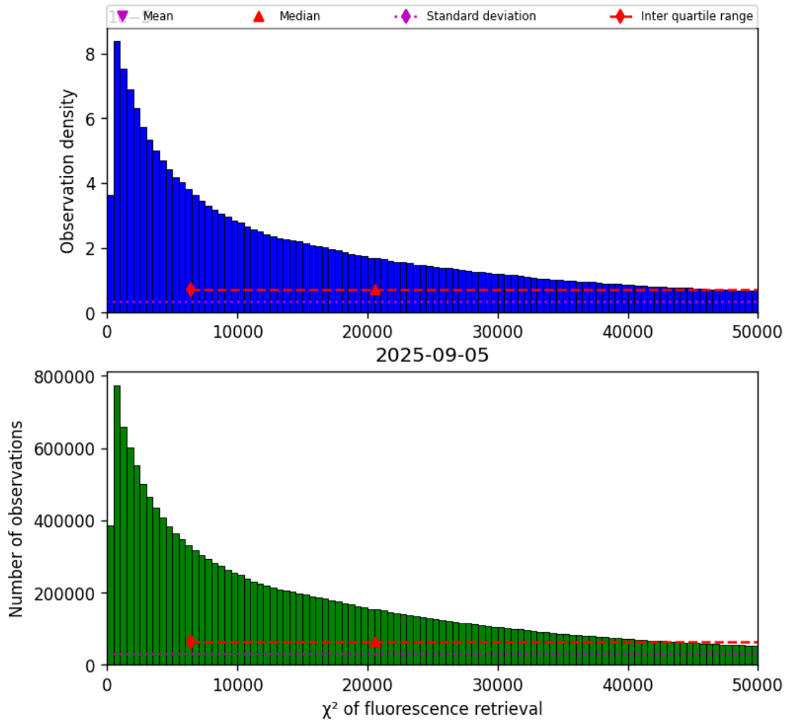
Figure 42: Histogram of “ \chi^2 of fluorescence retrieval” for 2025-09-04 to 2025-09-06
