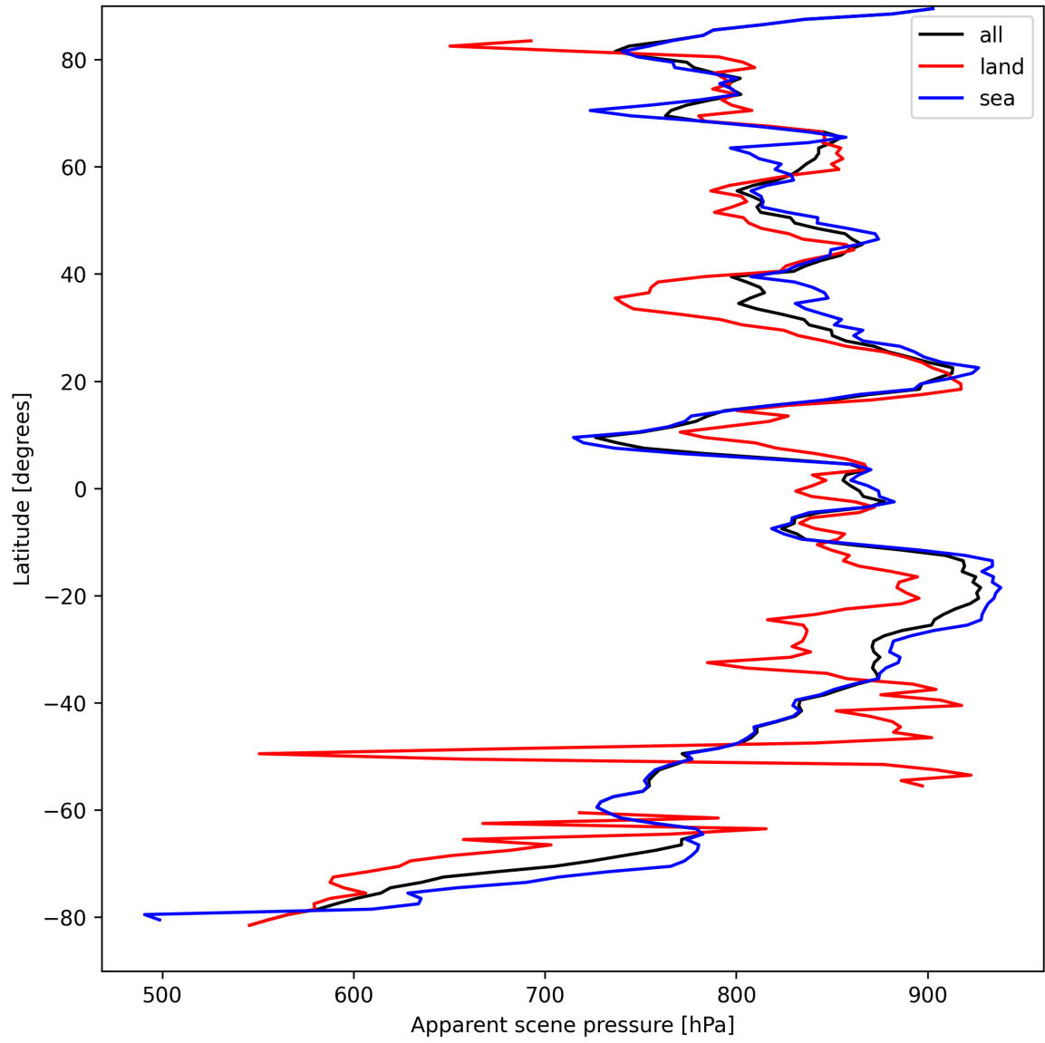
Figure 19: Zonal average of “Apparent scene pressure” for 2025-09-04 to 2025-09-06.
