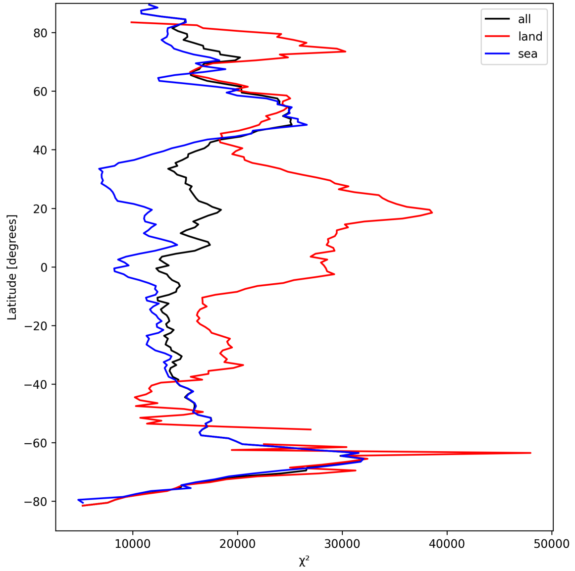
Figure 21: Zonal average of “ \chi^2 ” for 2025-09-04 to 2025-09-06.
