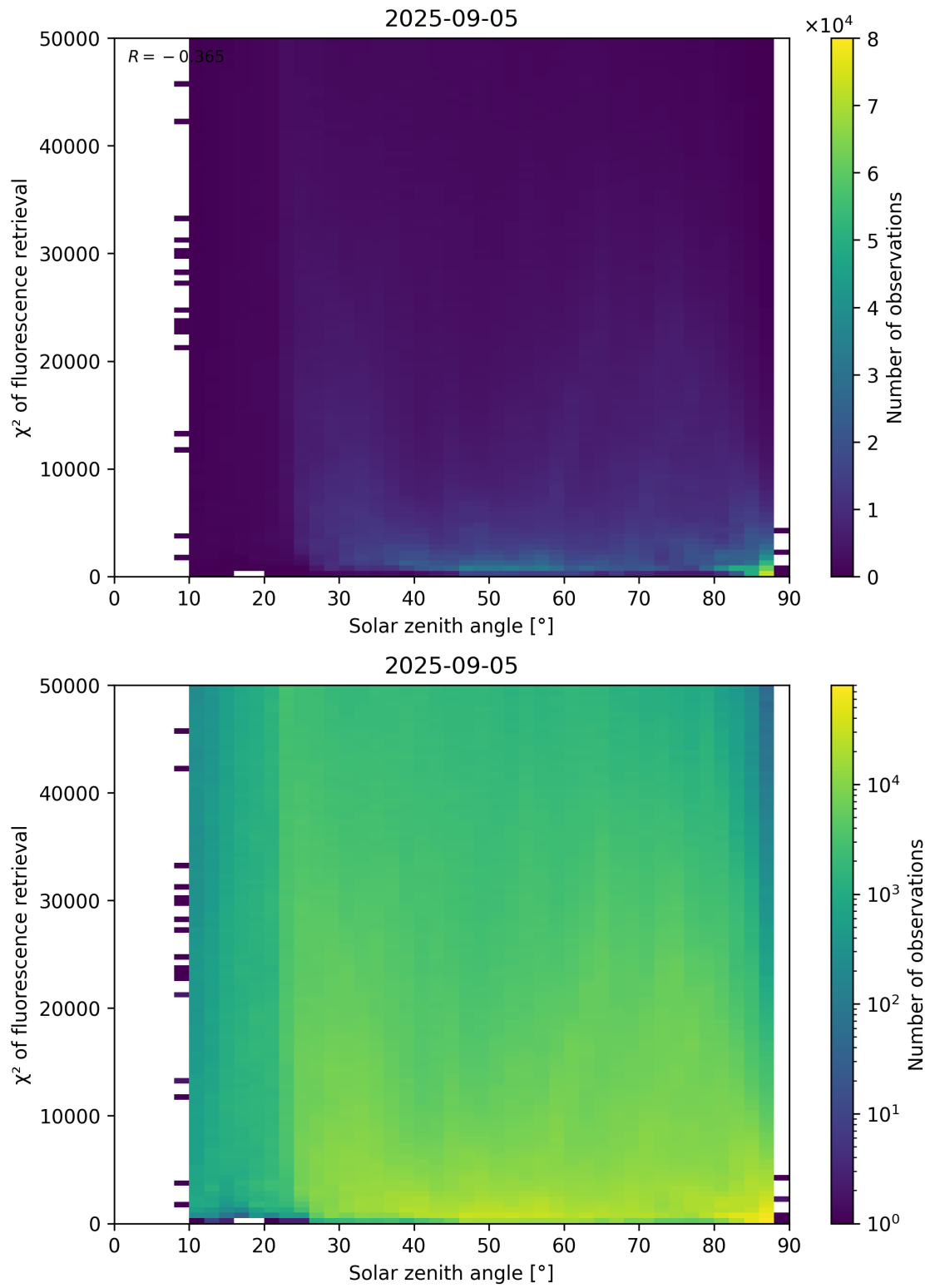
Figure 109: Scatter density plot of “Solar zenith angle” against “ \chi^2 of fluorescence retrieval” for 2025-09-04 to 2025-09-06.
