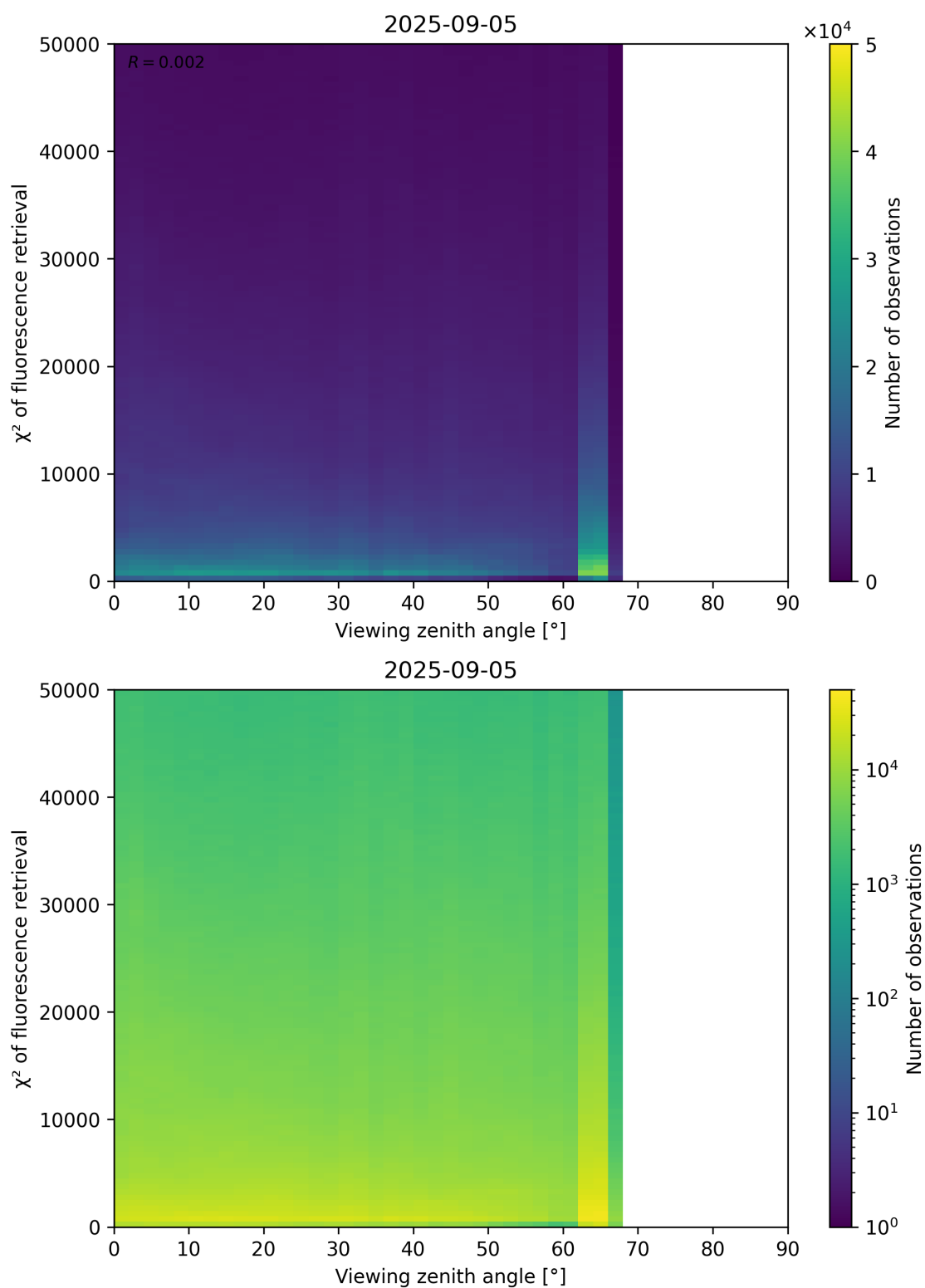
Figure 119: Scatter density plot of “Viewing zenith angle” against “ \chi^2 of fluorescence retrieval” for 2025-09-04 to 2025-09-06.
