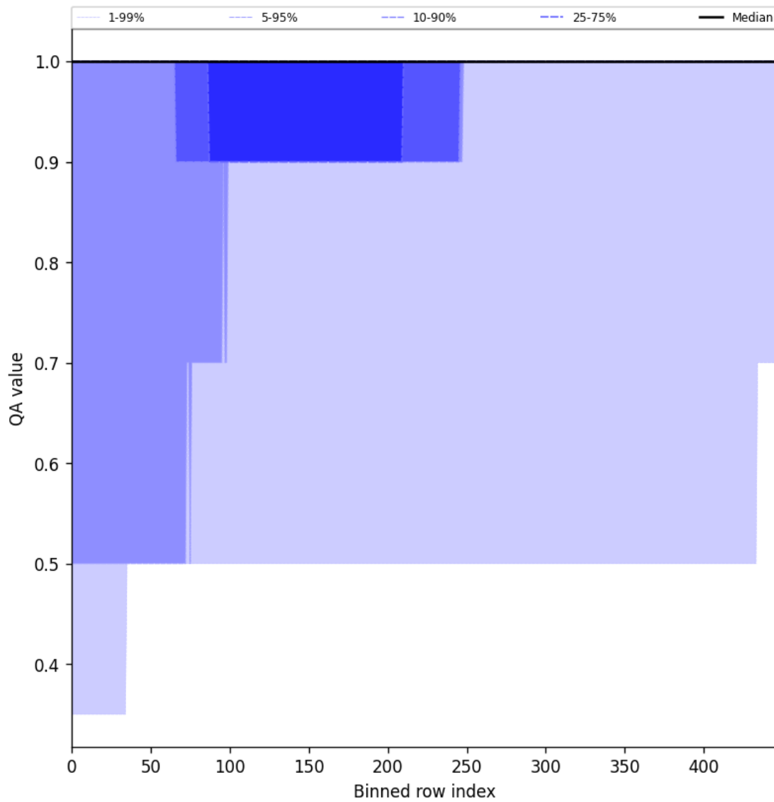
Figure 46: Along track statistics of “QA value” for 2025-09-04 to 2025-09-06
