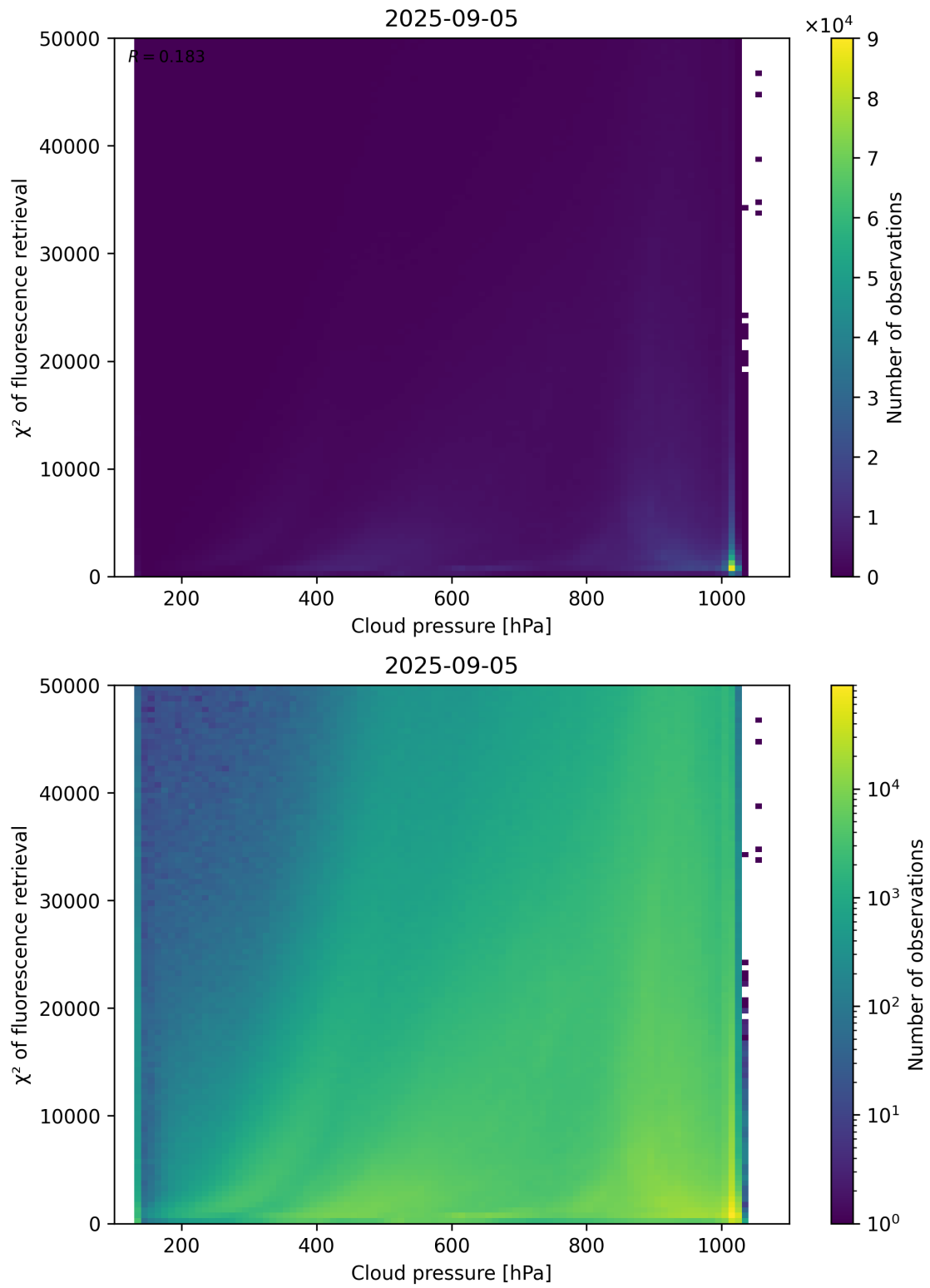
Figure 78: Scatter density plot of “Cloud pressure” against “ \chi^2 of fluorescence retrieval” for 2025-09-04 to 2025-09-06.
