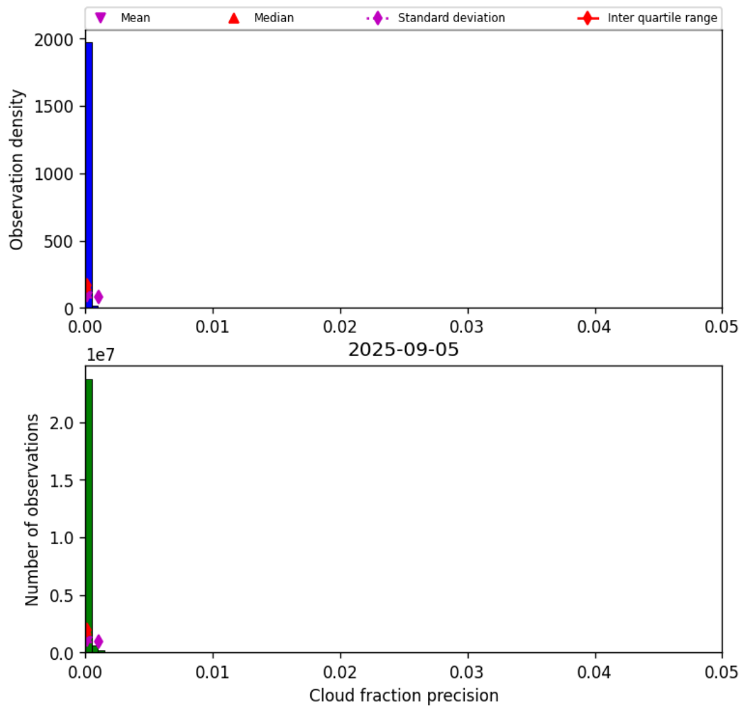
Figure 33: Histogram of “Cloud fraction precision” for 2025-09-04 to 2025-09-06
