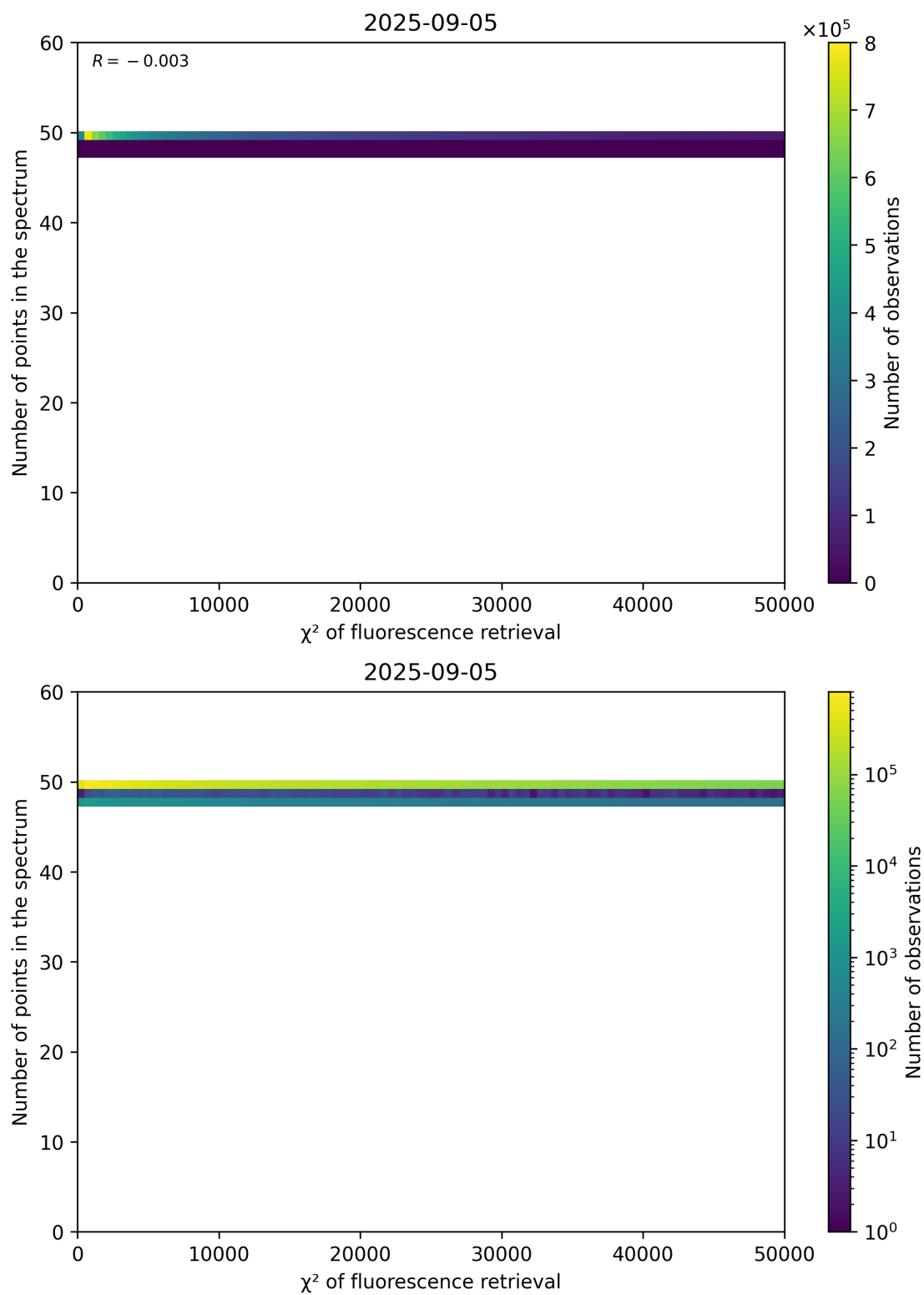
Figure 68: Scatter density plot of " \chi^2 of fluorescence retrieval" against "Number of points in the spectrum" for 2025-09-04 to 2025-09-06.
