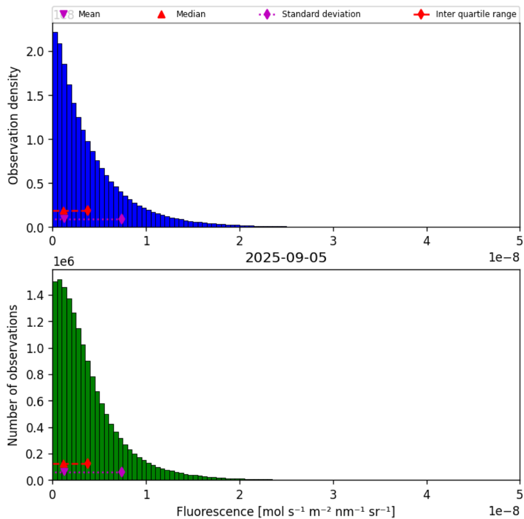
Figure 40: Histogram of “Fluorescence” for 2025-09-04 to 2025-09-06
