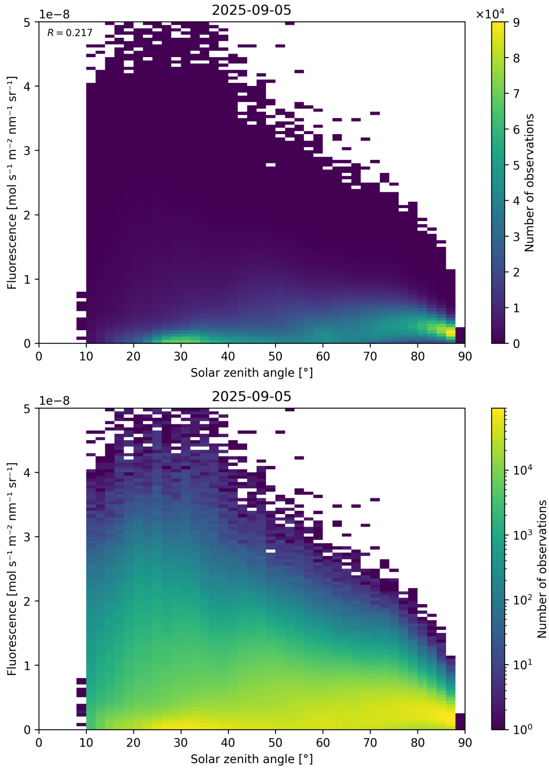
Figure 112: Scatter density plot of “Solar zenith angle” against “Fluorescence” for 2025-09-04 to 2025-09-06.
