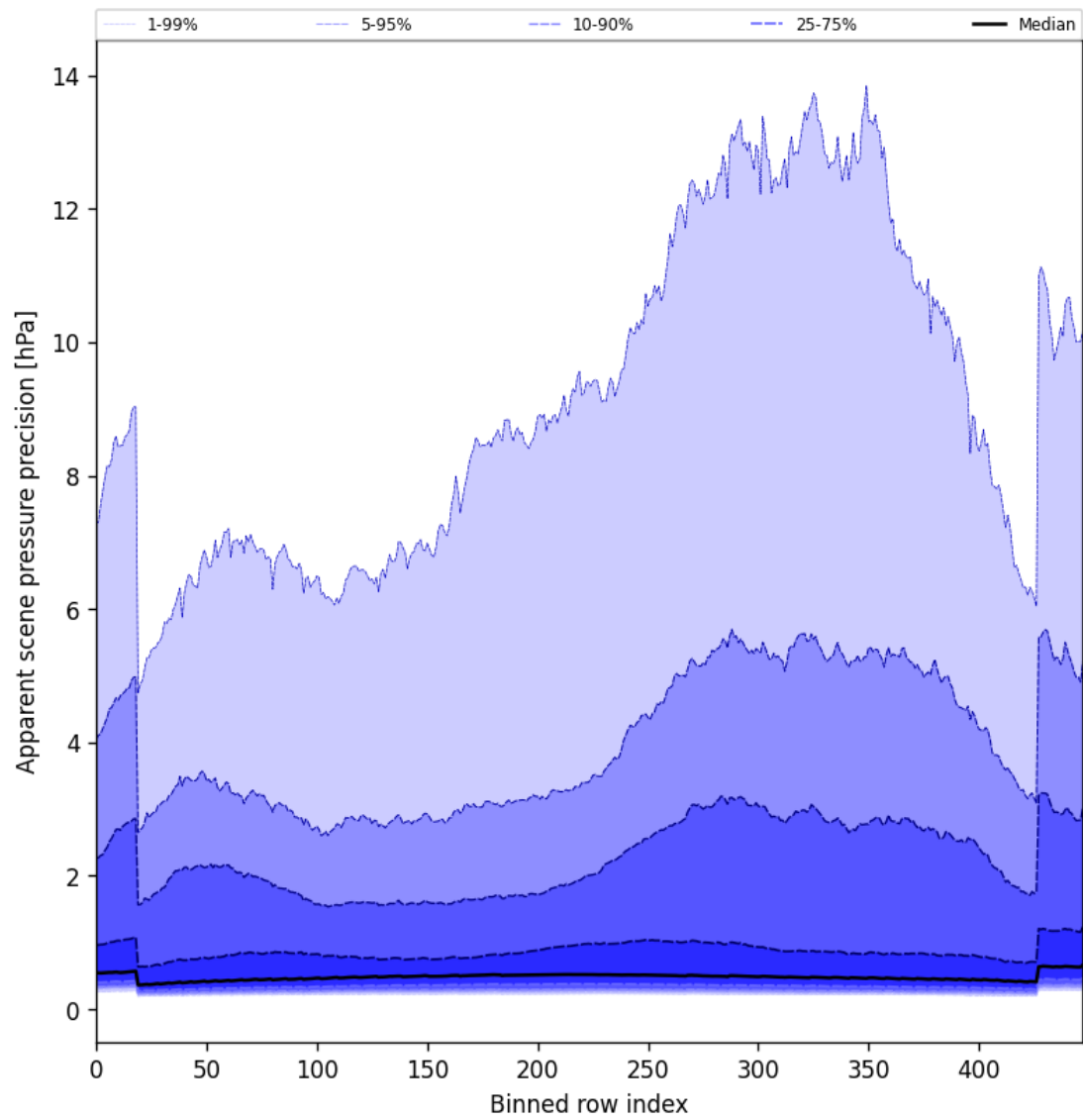
Figure 54: Along track statistics of “Apparent scene pressure precision” for 2025-09-04 to 2025-09-06
