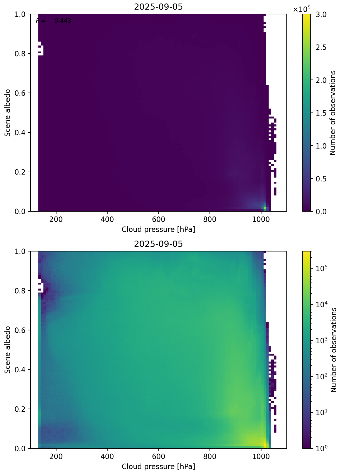
Figure 83: Scatter density plot of “Cloud pressure” against “Scene albedo” for 2025-09-04 to 2025-09-06.
