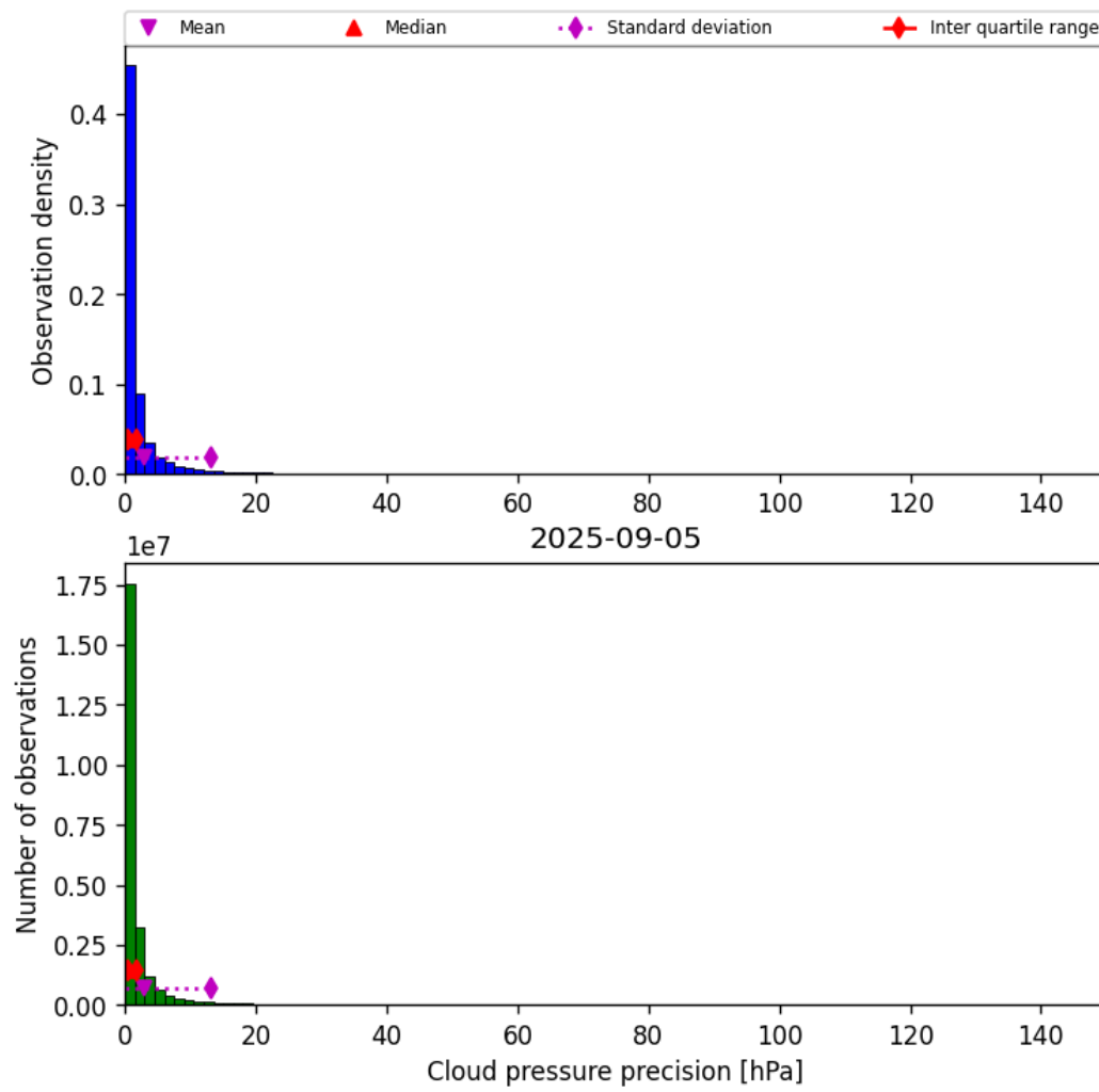
Figure 31: Histogram of “Cloud pressure precision” for 2025-09-04 to 2025-09-06
