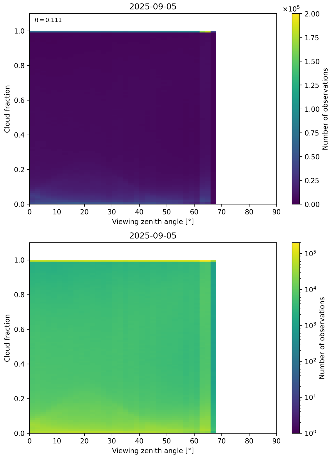
Figure 120: Scatter density plot of “Viewing zenith angle” against “Cloud fraction” for 2025-09-04 to 2025-09-06.
