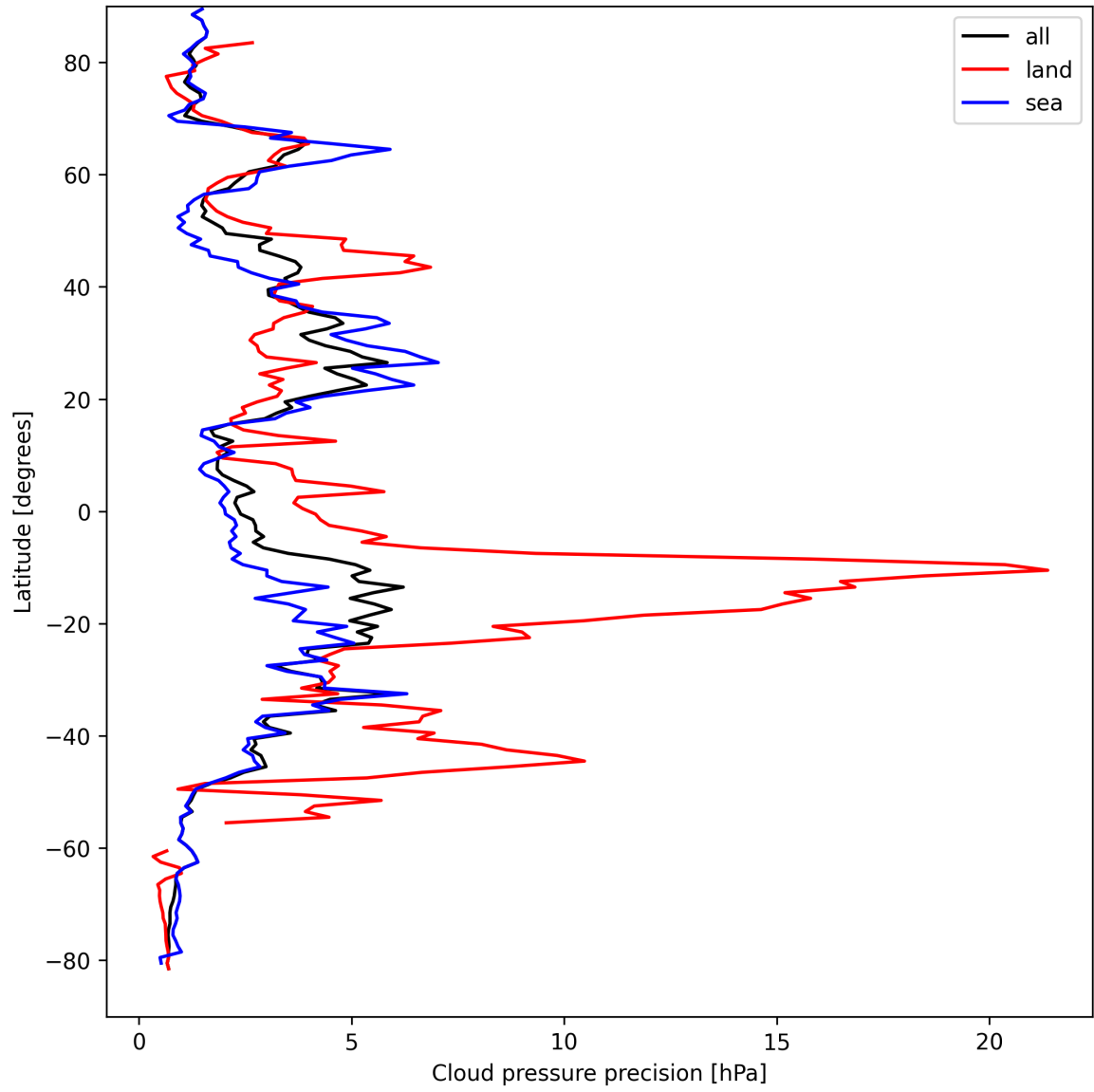
Figure 14: Zonal average of “Cloud pressure precision” for 2025-09-04 to 2025-09-06.
