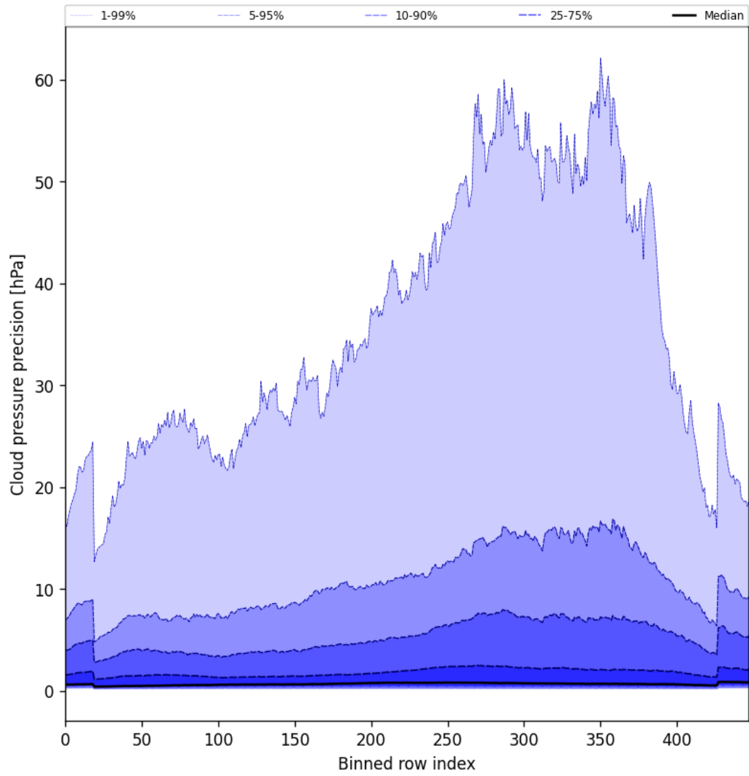
Figure 48: Along track statistics of “Cloud pressure precision” for 2025-09-04 to 2025-09-06
