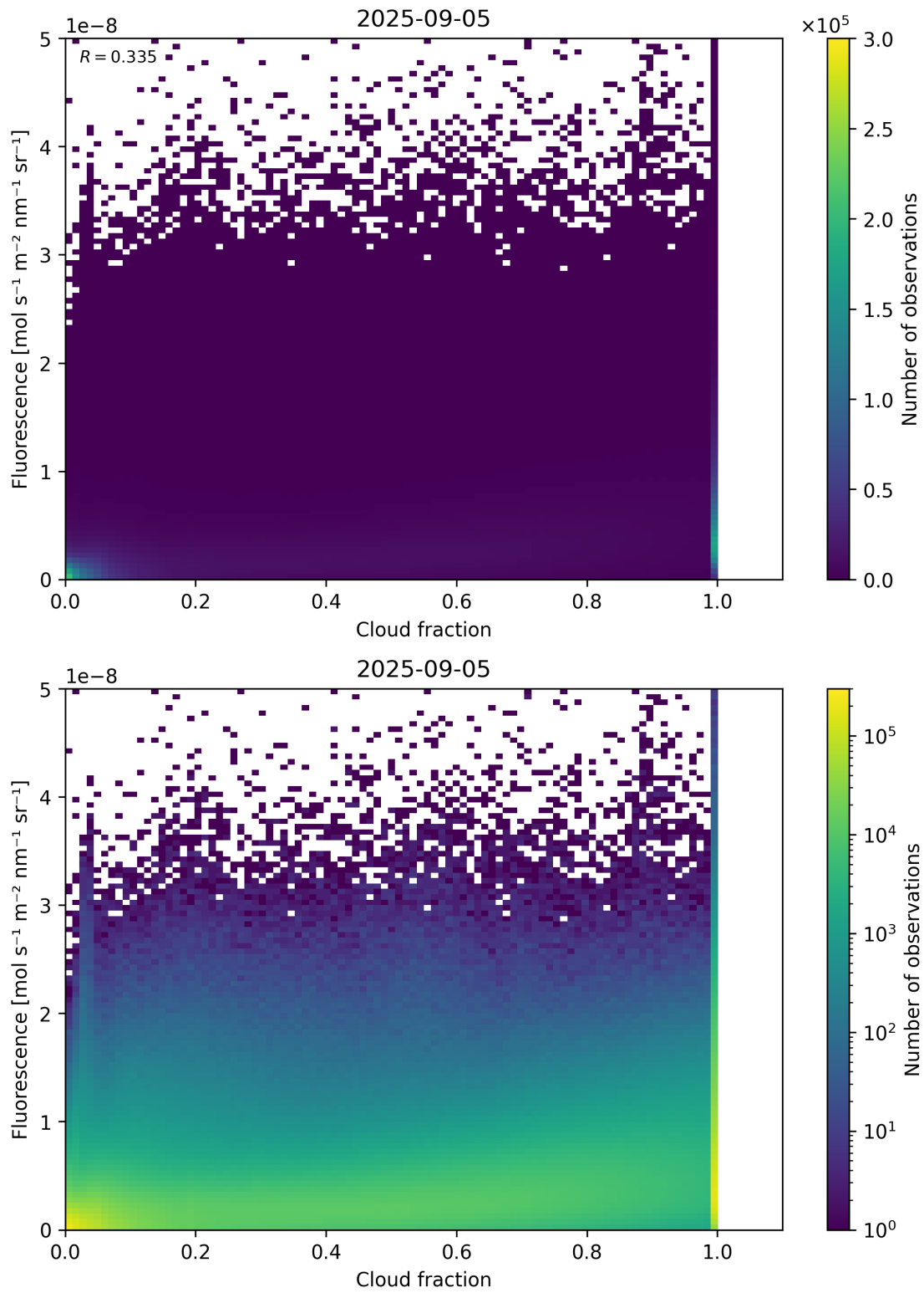
Figure 72: Scatter density plot of “Cloud fraction” against “Fluorescence” for 2025-09-04 to 2025-09-06.
