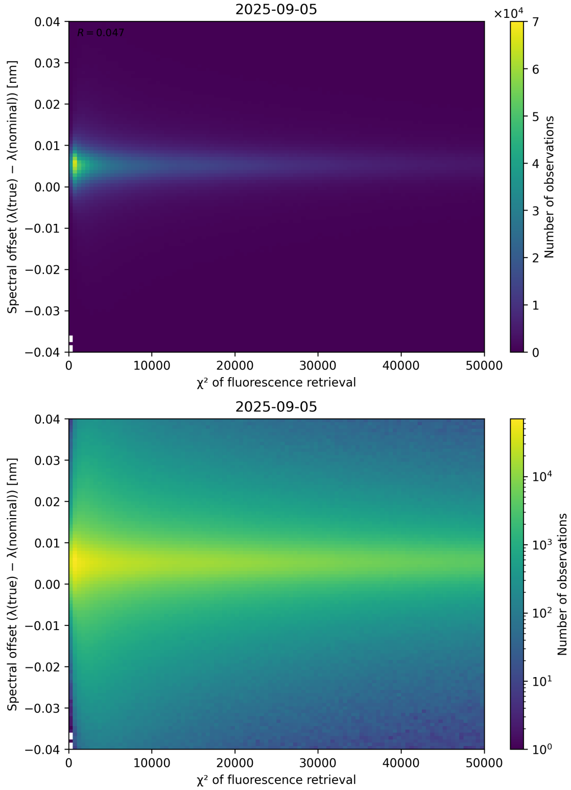
Figure 69: Scatter density plot of “ \chi^2 of fluorescence retrieval” against “Spectral offset ( \lambda_{\text{true}} - \lambda_{\text{nominal}} )” for 2025-09-04 to 2025-09-06.
