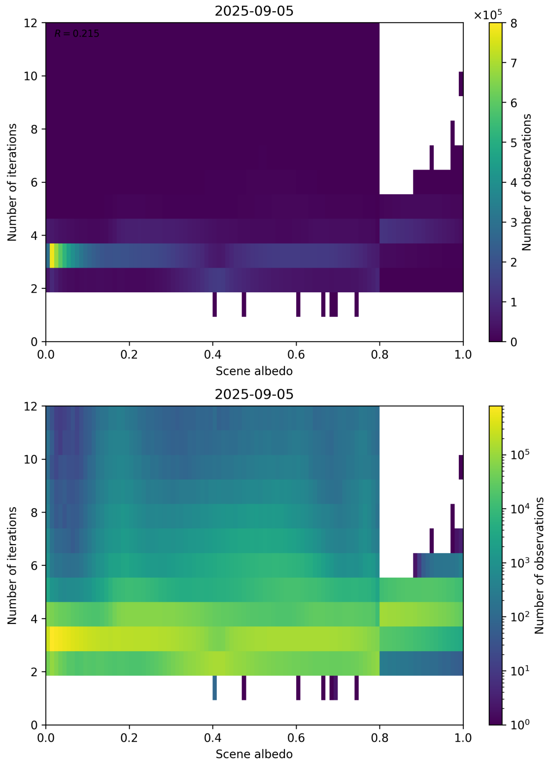
Figure 105: Scatter density plot of “Scene albedo” against “Number of iterations” for 2025-09-04 to 2025-09-06.
