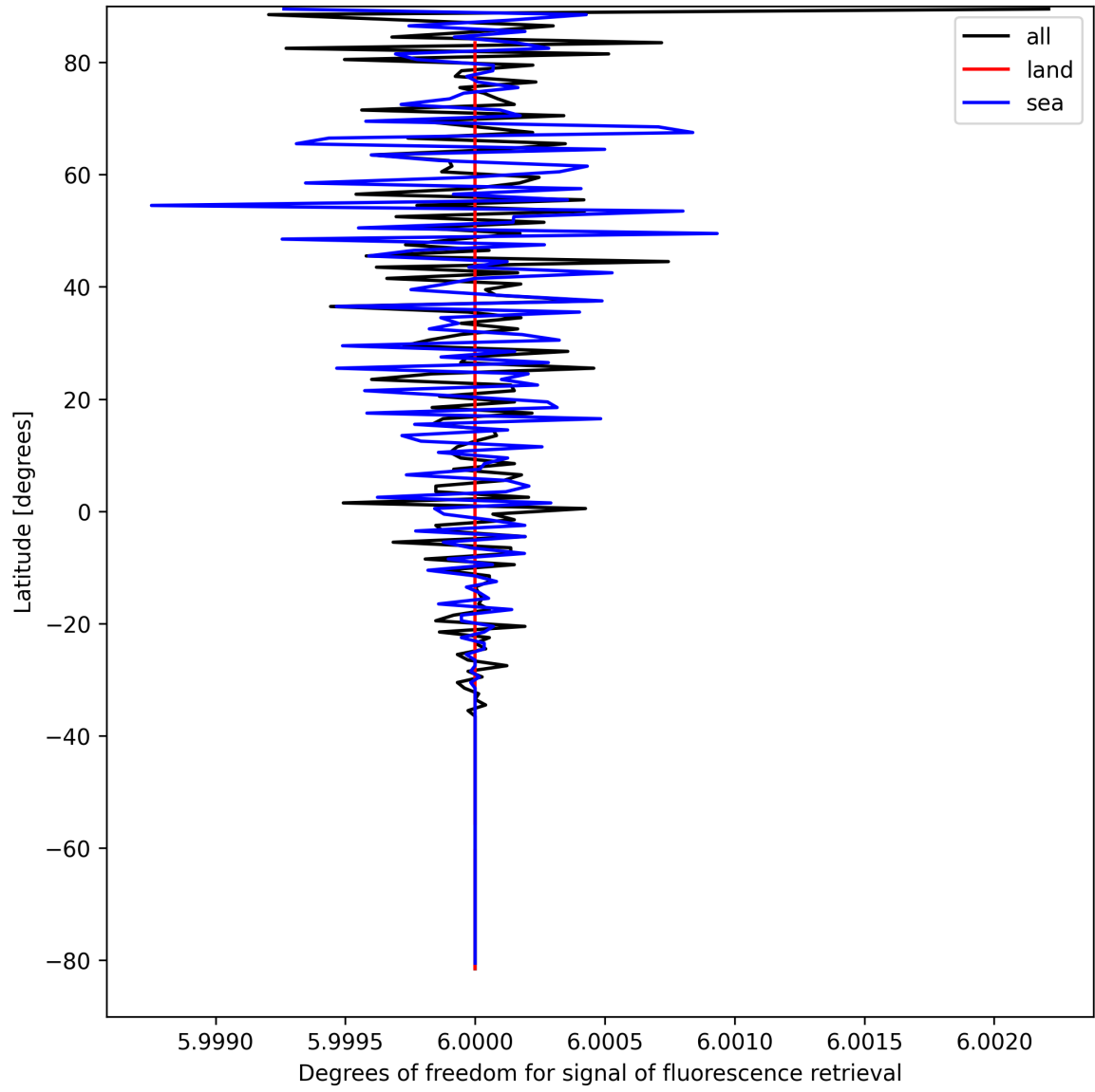
Figure 26: Zonal average of “Degrees of freedom for signal of fluorescence retrieval” for 2025-09-04 to 2025-09-06.
