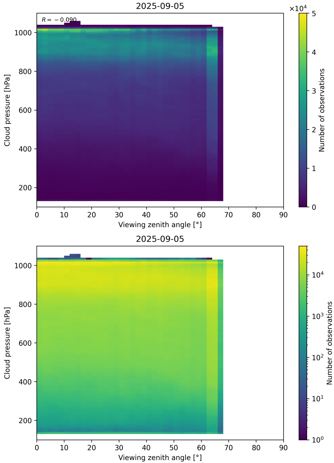
Figure 121: Scatter density plot of “Viewing zenith angle” against “Cloud pressure” for 2025-09-04 to 2025-09-06.
