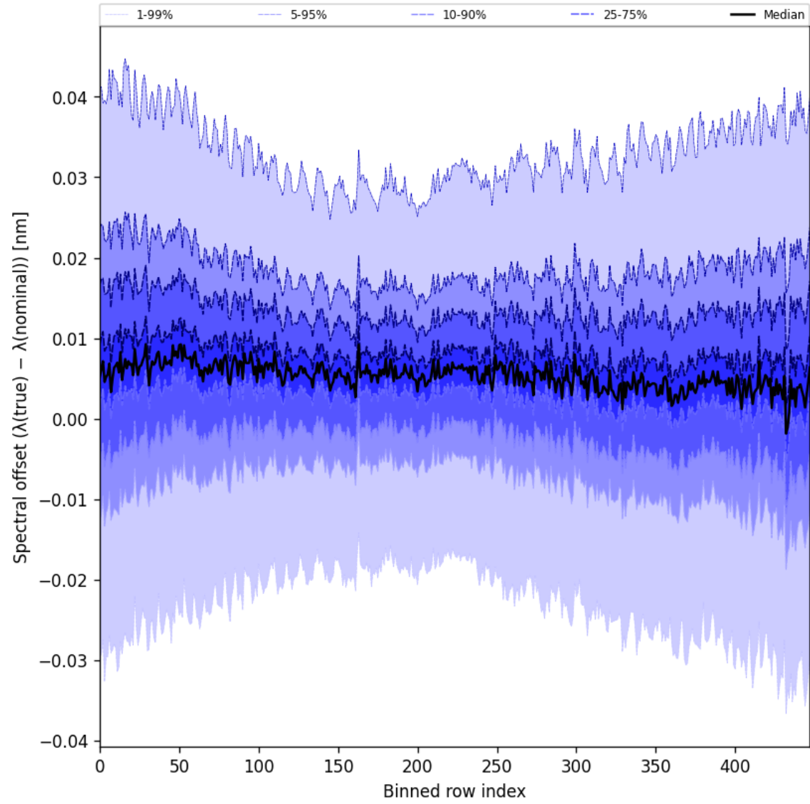
Figure 62: Along track statistics of “Spectral offset ( \lambda_{\text{true}} - \lambda_{\text{nominal}} )” for 2025-09-04 to 2025-09-06
