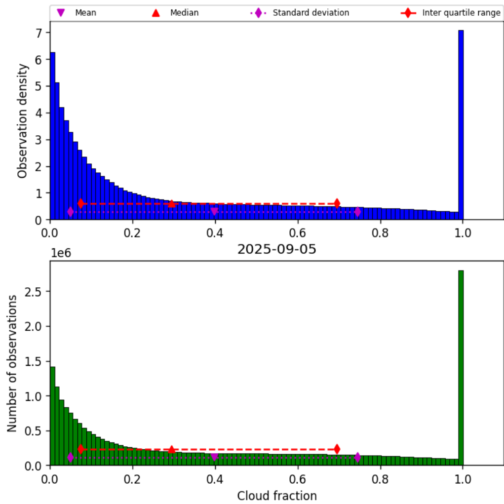
Figure 32: Histogram of “Cloud fraction” for 2025-09-04 to 2025-09-06
