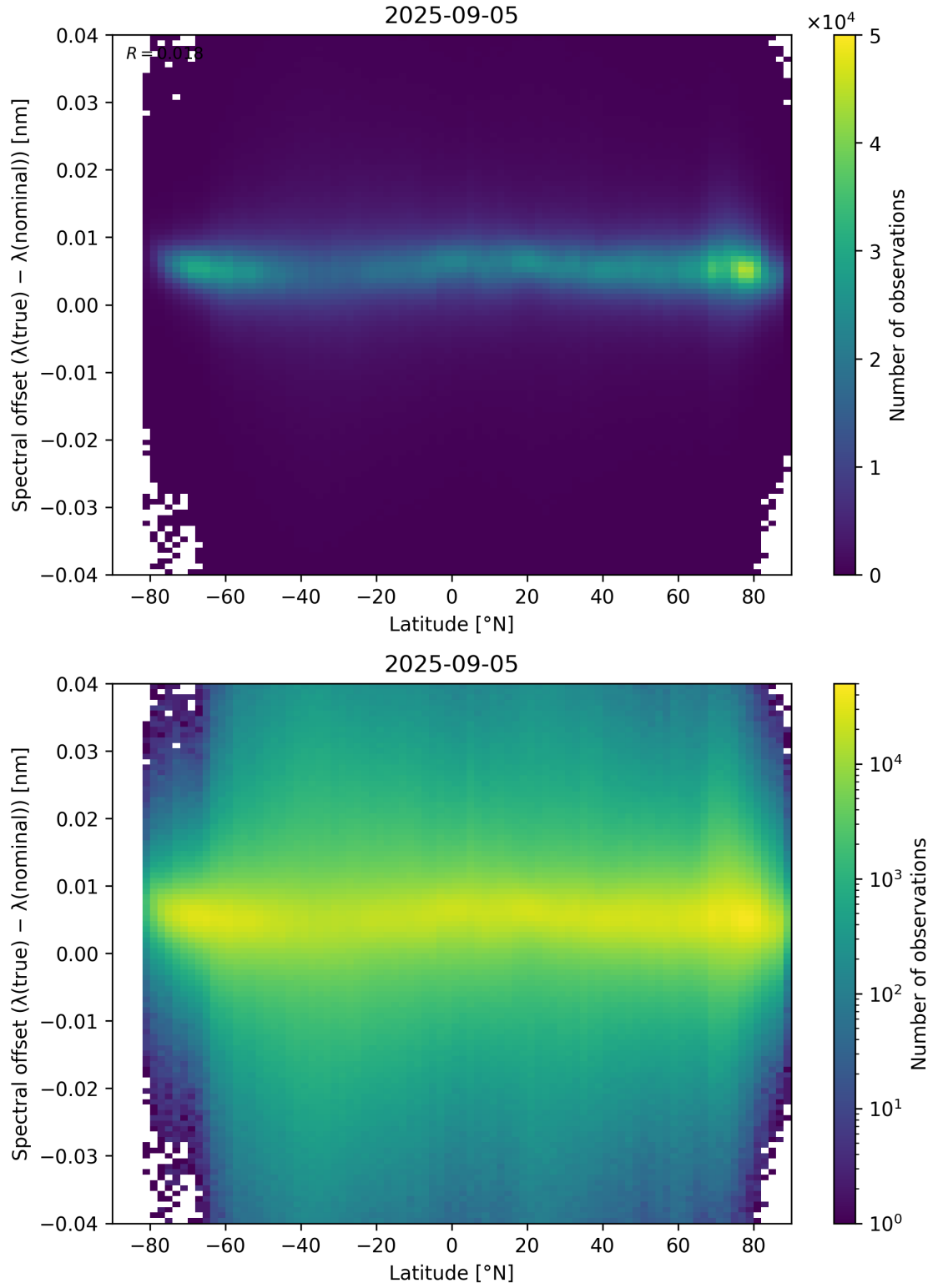
Figure 96: Scatter density plot of “Latitude” against “Spectral offset ( \lambda_{\text{true}} - \lambda_{\text{nominal}} )” for 2025-09-04 to 2025-09-06.
