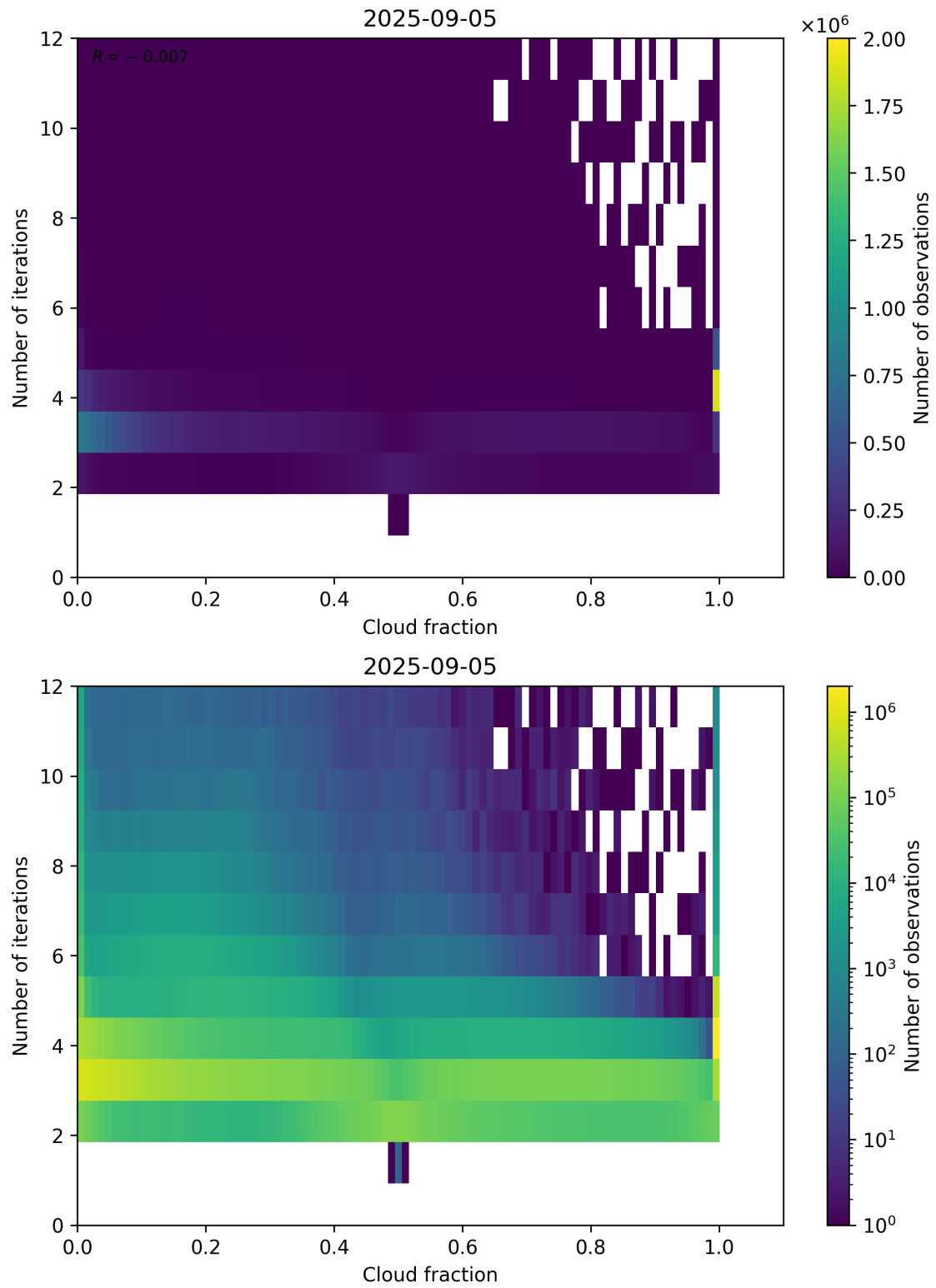
Figure 73: Scatter density plot of “Cloud fraction” against “Number of iterations” for 2025-09-04 to 2025-09-06.
