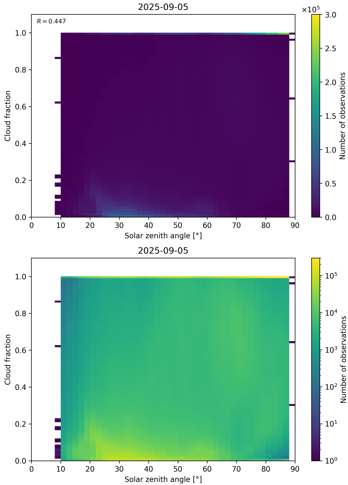
Figure 110: Scatter density plot of “Solar zenith angle” against “Cloud fraction” for 2025-09-04 to 2025-09-06.
