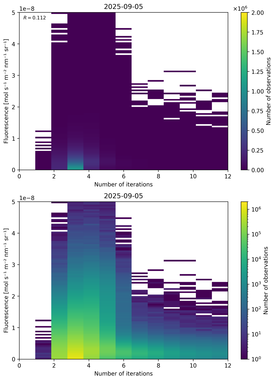
Figure 98: Scatter density plot of “Number of iterations” against “Fluorescence” for 2025-09-04 to 2025-09-06.
