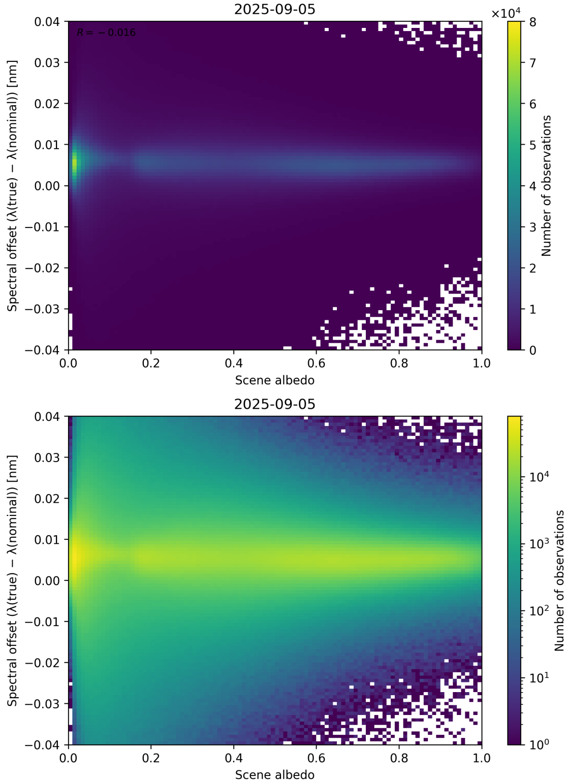
Figure 107: Scatter density plot of “Scene albedo” against “Spectral offset ( \lambda_{\text{true}} - \lambda_{\text{nominal}} )” for 2025-09-04 to 2025-09-06.
