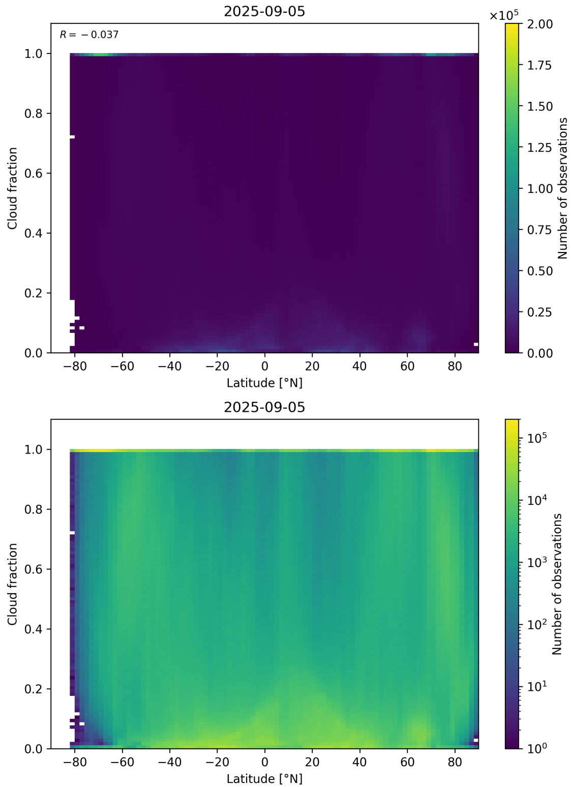
Figure 90: Scatter density plot of “Latitude” against “Cloud fraction” for 2025-09-04 to 2025-09-06.
