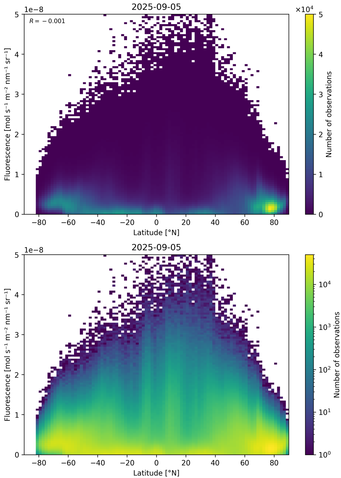
Figure 92: Scatter density plot of “Latitude” against “Fluorescence” for 2025-09-04 to 2025-09-06.
