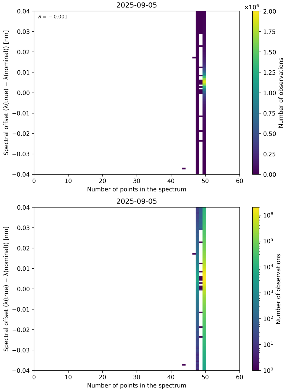
Figure 101: Scatter density plot of “Number of points in the spectrum” against “Spectral offset ( \lambda_{\text{true}} - \lambda_{\text{nominal}} )” for 2025-09-04 to 2025-09-06.
