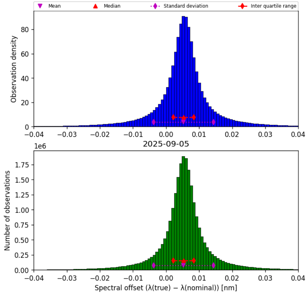
Figure 45: Histogram of “Spectral offset ( \lambda_{\text{true}} - \lambda_{\text{nominal}} )” for 2025-09-04 to 2025-09-06
