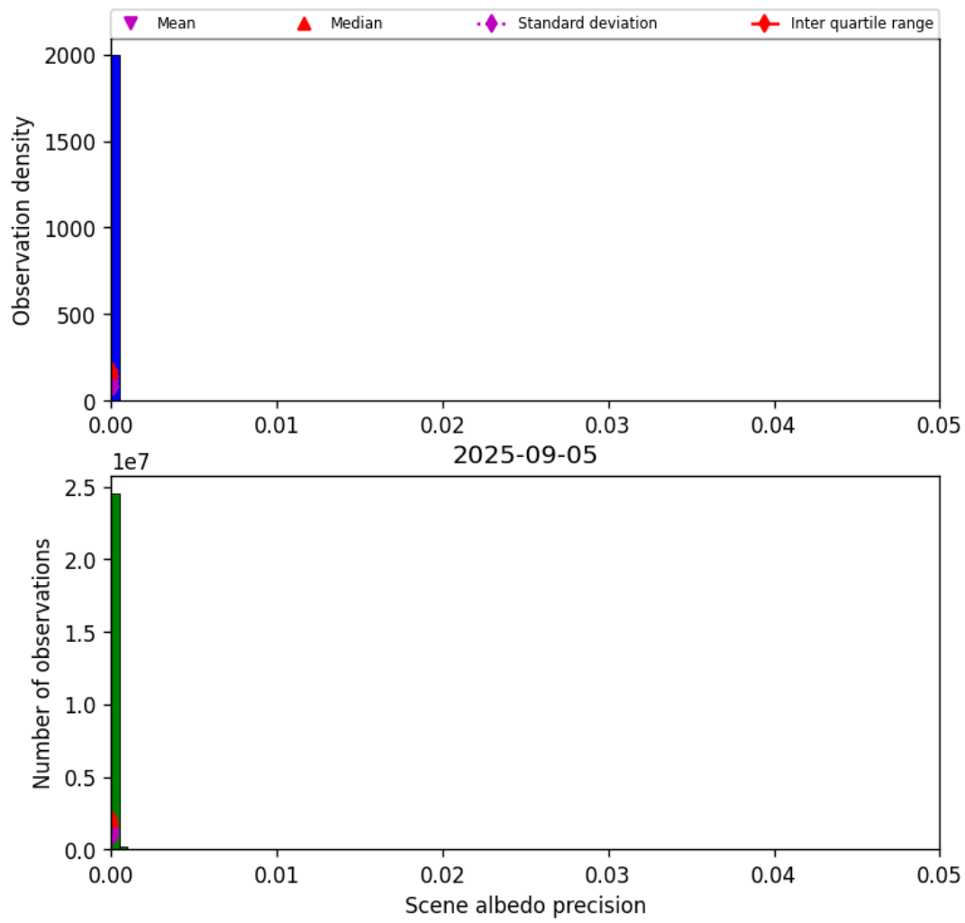
Figure 35: Histogram of “Scene albedo precision” for 2025-09-04 to 2025-09-06
