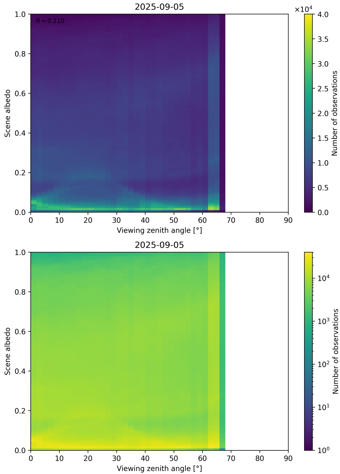
Figure 126: Scatter density plot of “Viewing zenith angle” against “Scene albedo” for 2025-09-04 to 2025-09-06.
