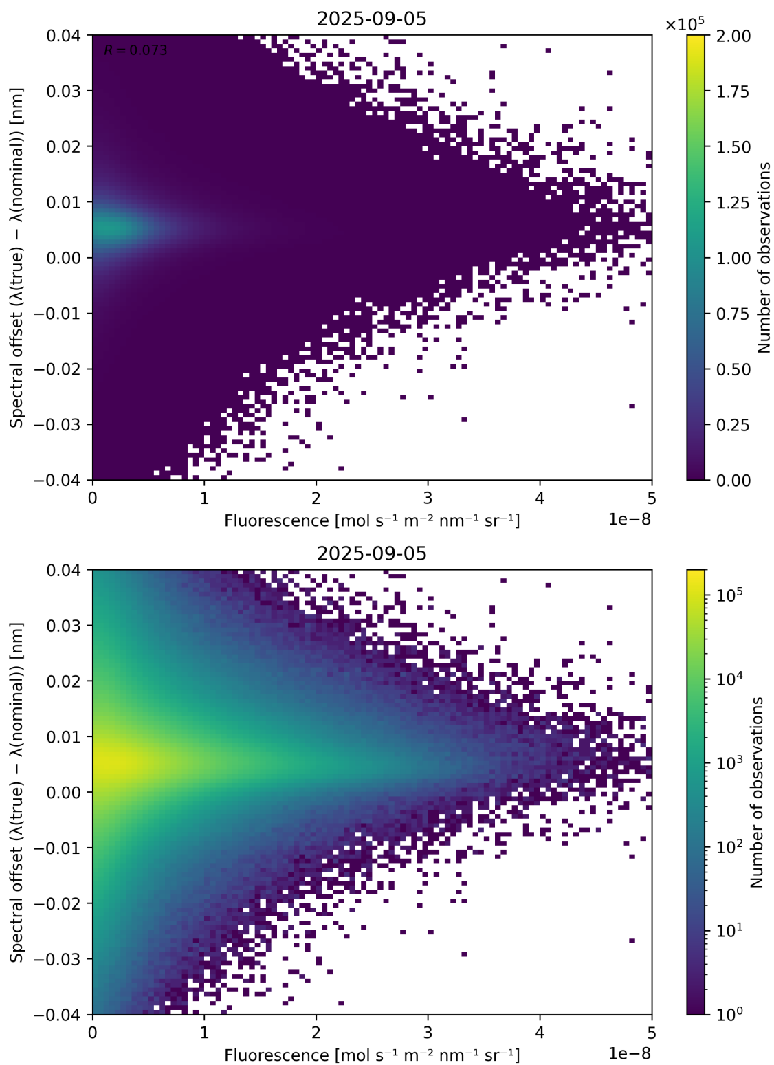
Figure 87: Scatter density plot of “Fluorescence” against “Spectral offset ( \lambda_{\text{true}} - \lambda_{\text{nominal}} )” for 2025-09-04 to 2025-09-06.
