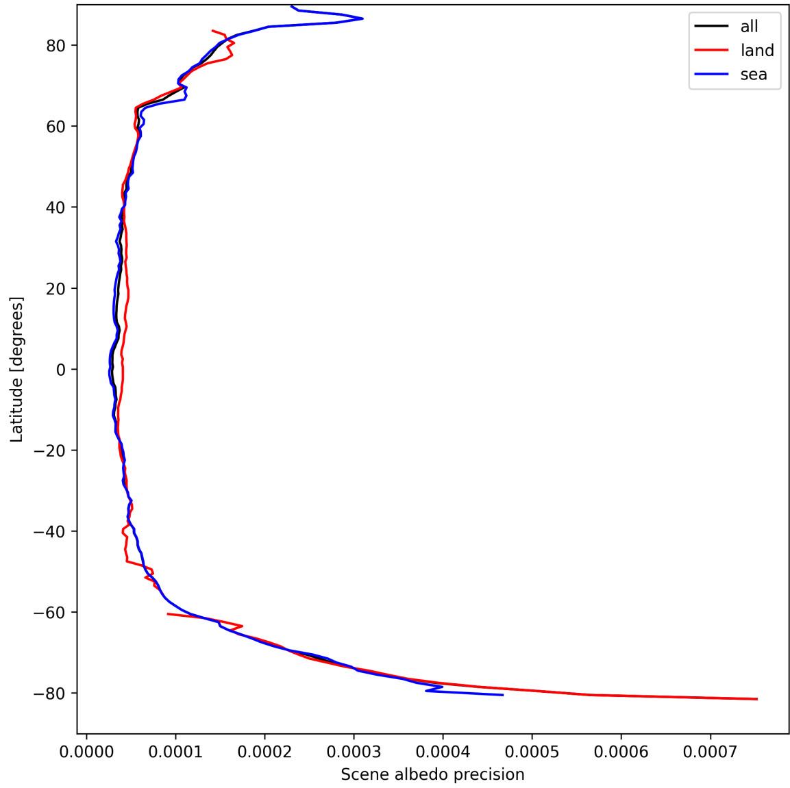
Figure 18: Zonal average of “Scene albedo precision” for 2025-09-04 to 2025-09-06.
