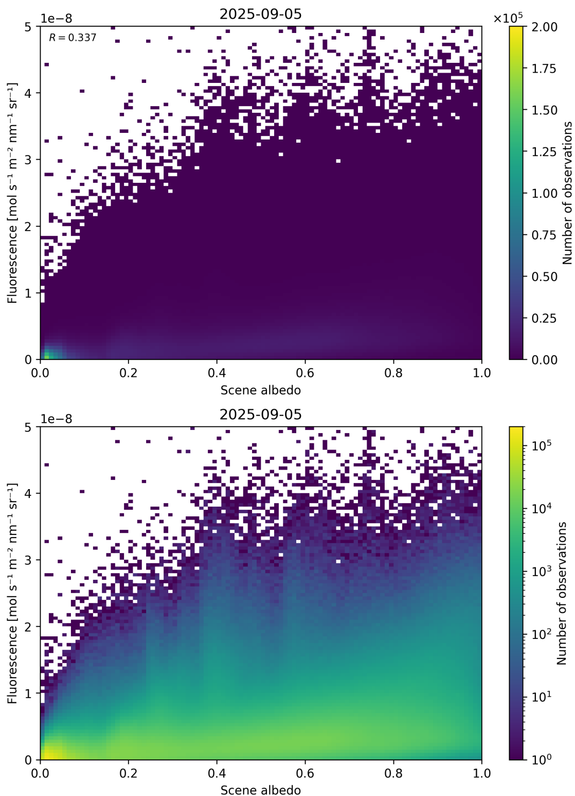
Figure 104: Scatter density plot of “Scene albedo” against “Fluorescence” for 2025-09-04 to 2025-09-06.
