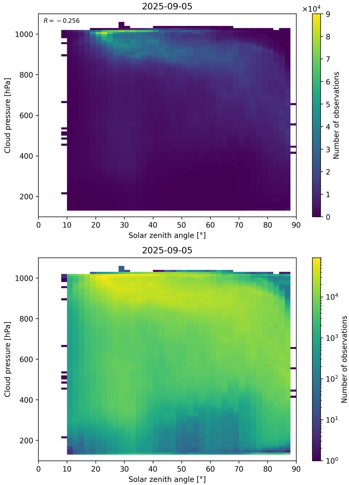
Figure 111: Scatter density plot of “Solar zenith angle” against “Cloud pressure” for 2025-09-04 to 2025-09-06.
