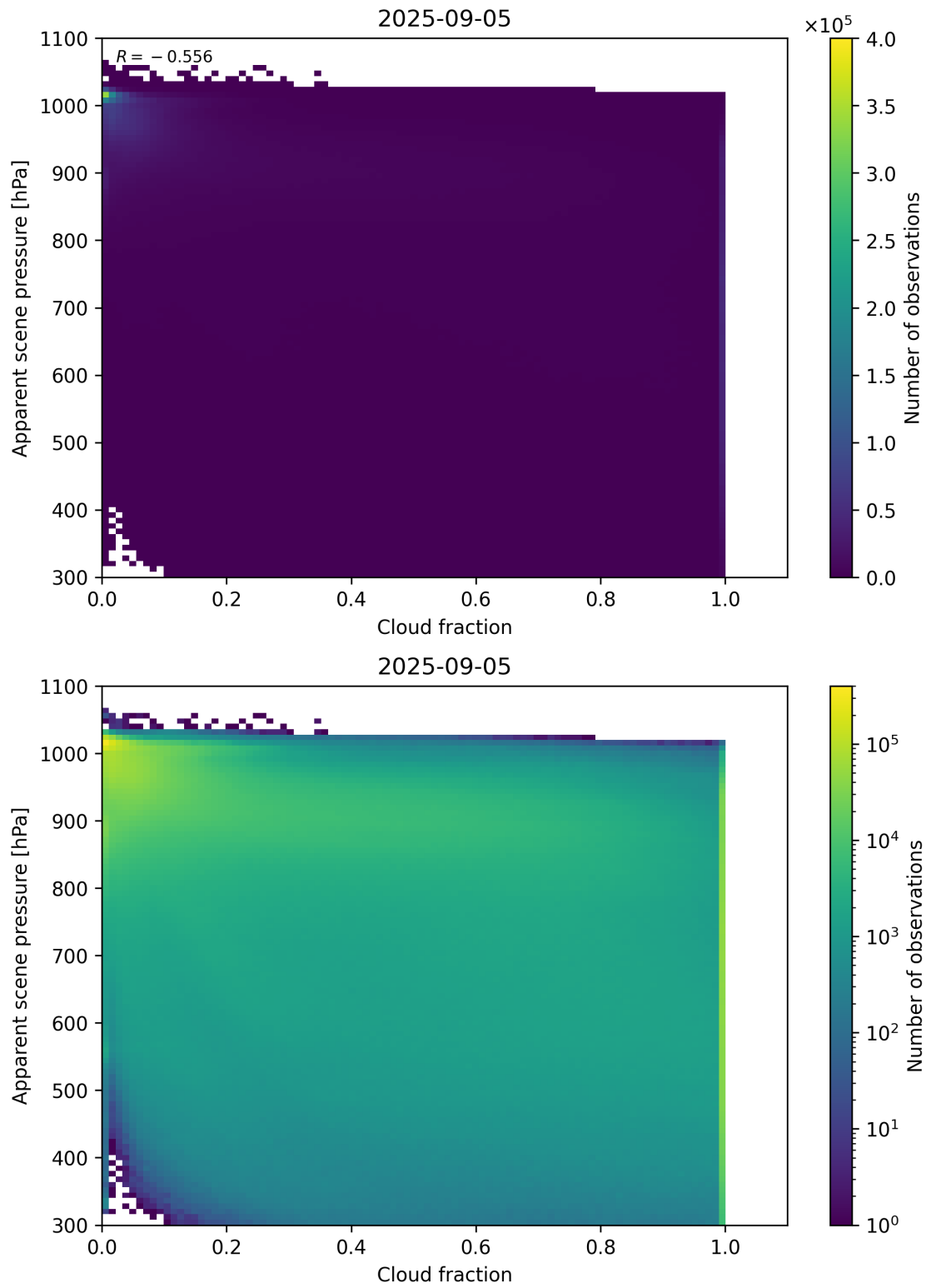
Figure 70: Scatter density plot of “Cloud fraction” against “Apparent scene pressure” for 2025-09-04 to 2025-09-06.
