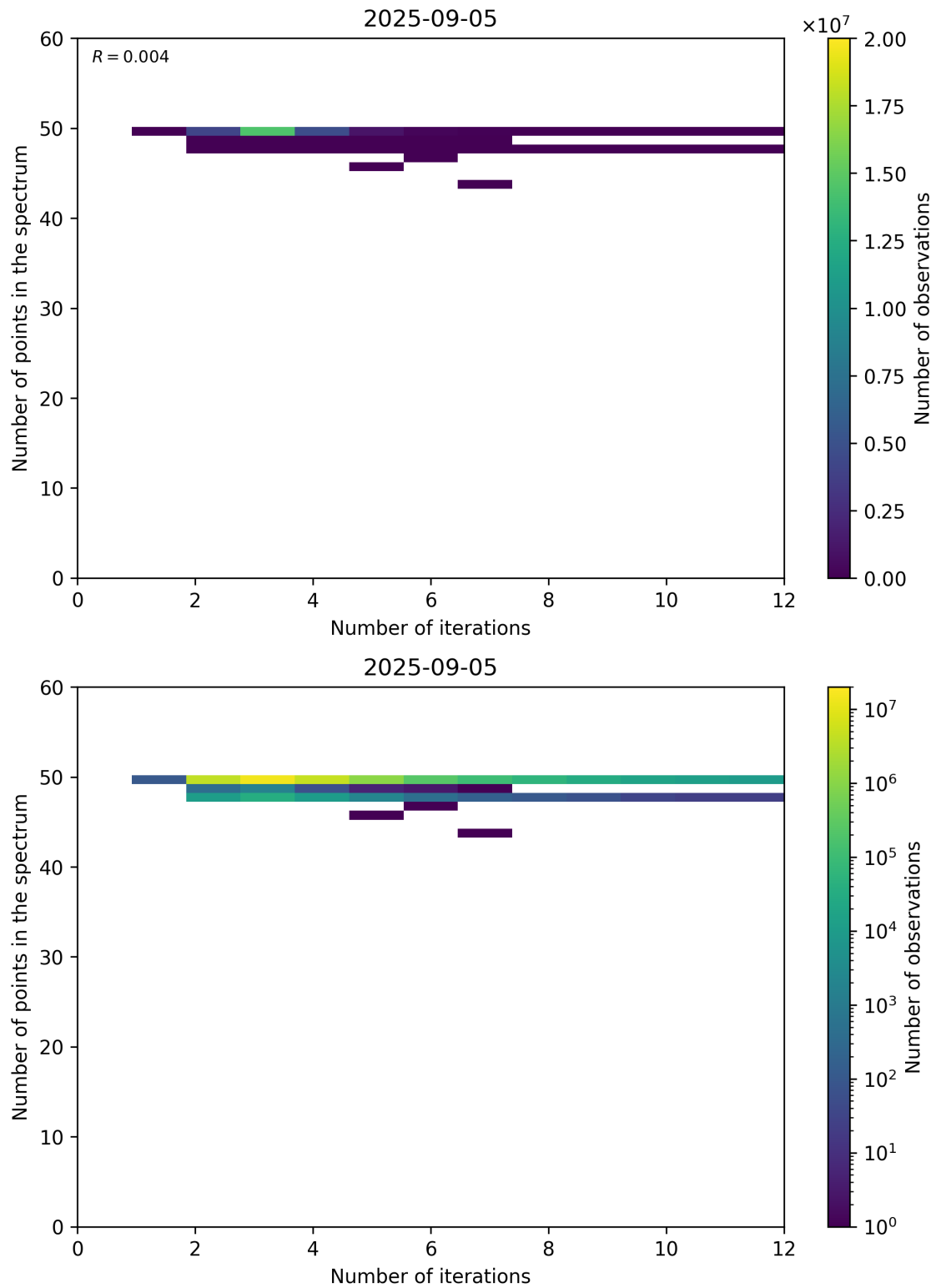
Figure 99: Scatter density plot of “Number of iterations” against “Number of points in the spectrum” for 2025-09-04 to 2025-09-06.
