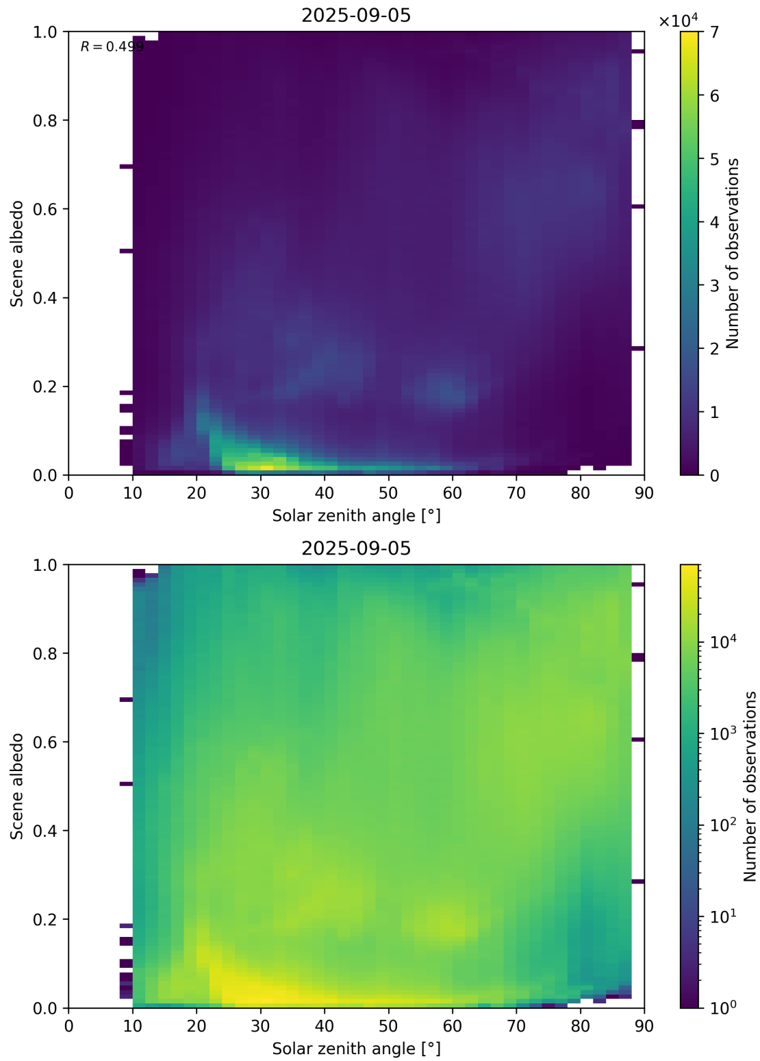
Figure 116: Scatter density plot of “Solar zenith angle” against “Scene albedo” for 2025-09-04 to 2025-09-06.
