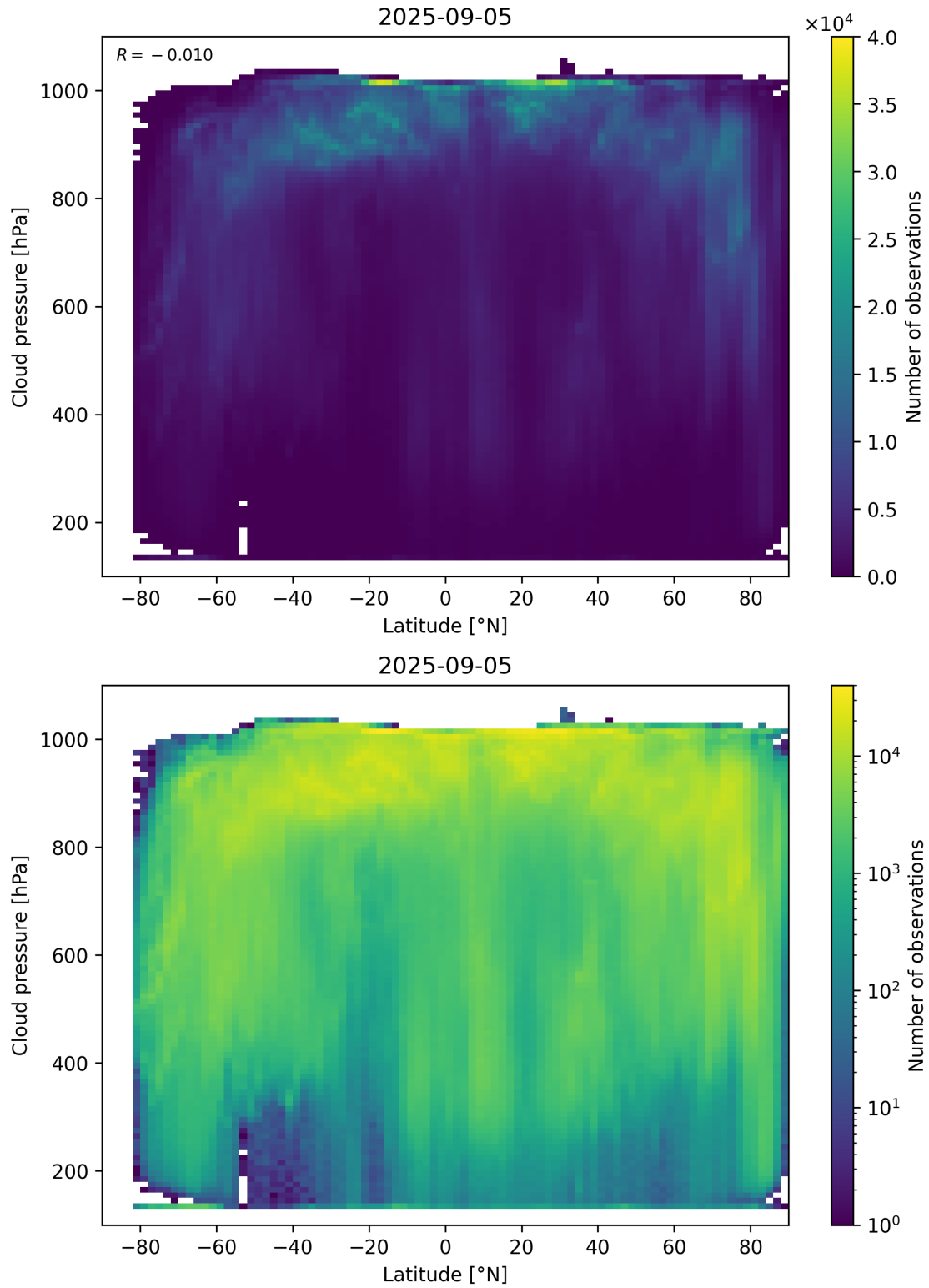
Figure 91: Scatter density plot of “Latitude” against “Cloud pressure” for 2025-09-04 to 2025-09-06.
