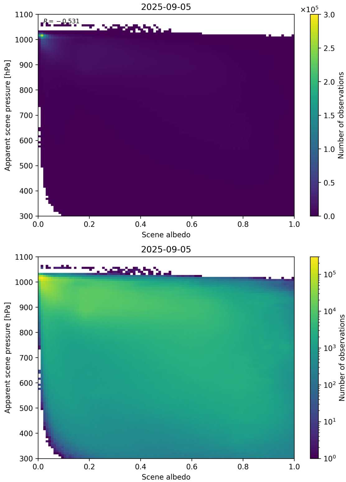
Figure 102: Scatter density plot of “Scene albedo” against “Apparent scene pressure” for 2025-09-04 to 2025-09-06.
