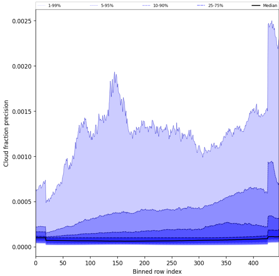
Figure 50: Along track statistics of “Cloud fraction precision” for 2025-09-04 to 2025-09-06
