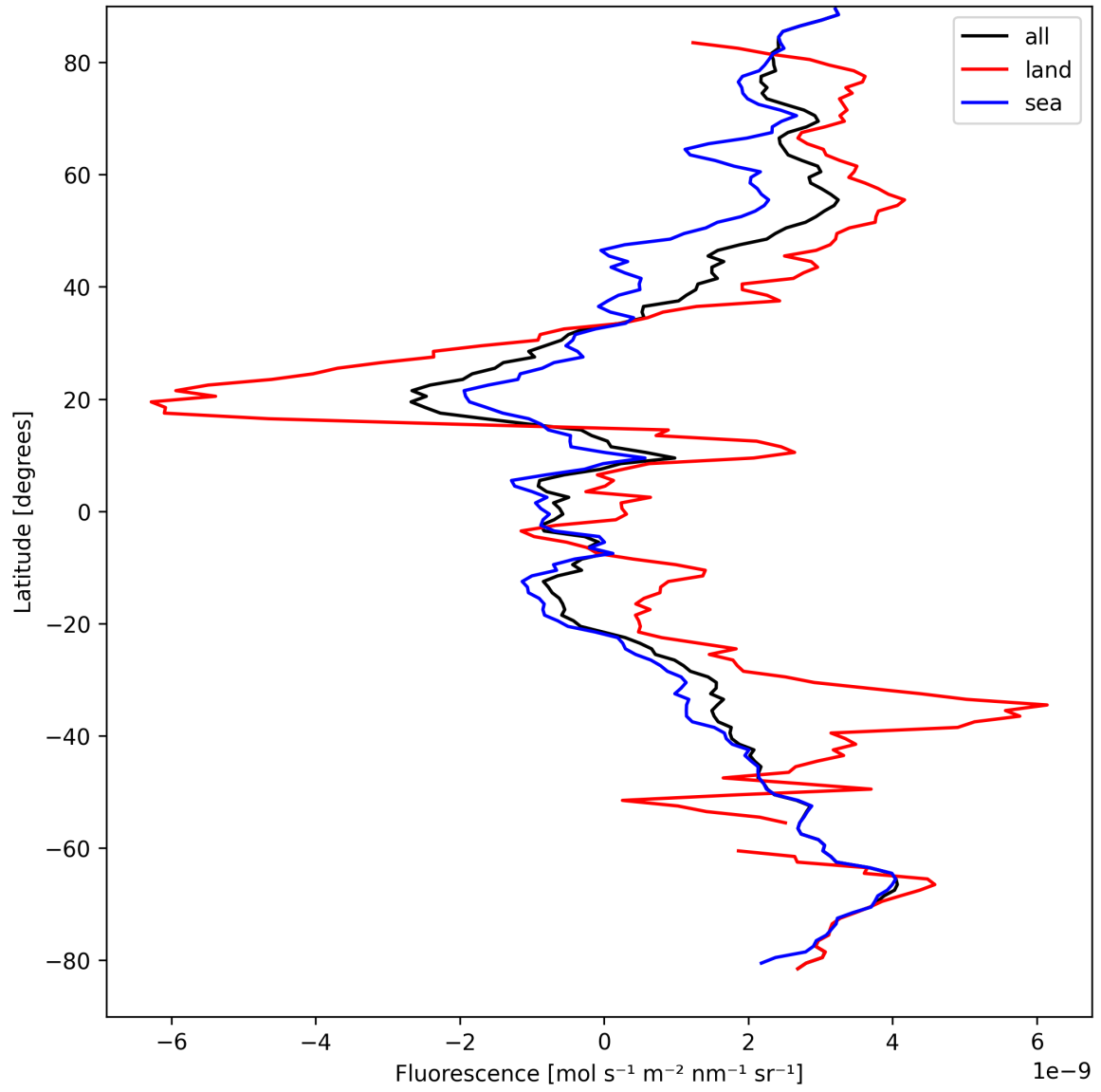
Figure 23: Zonal average of “Fluorescence” for 2025-09-04 to 2025-09-06.
