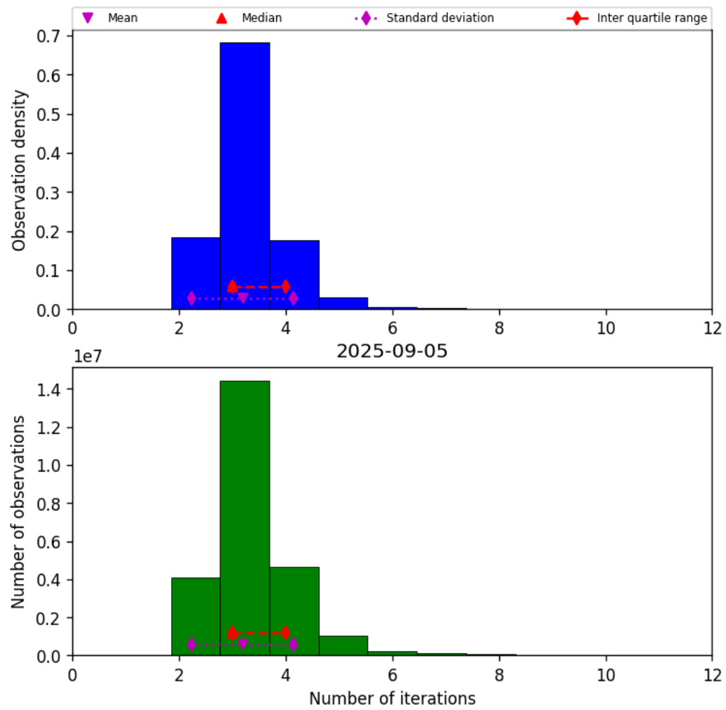
Figure 39: Histogram of “Number of iterations” for 2025-09-04 to 2025-09-06
