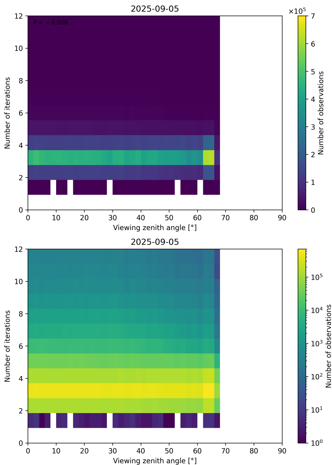
Figure 124: Scatter density plot of “Viewing zenith angle” against “Number of iterations” for 2025-09-04 to 2025-09-06.
