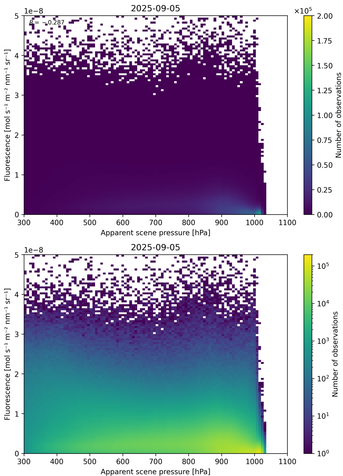
Figure 64: Scatter density plot of “Apparent scene pressure” against “Fluorescence” for 2025-09-04 to 2025-09-06.
