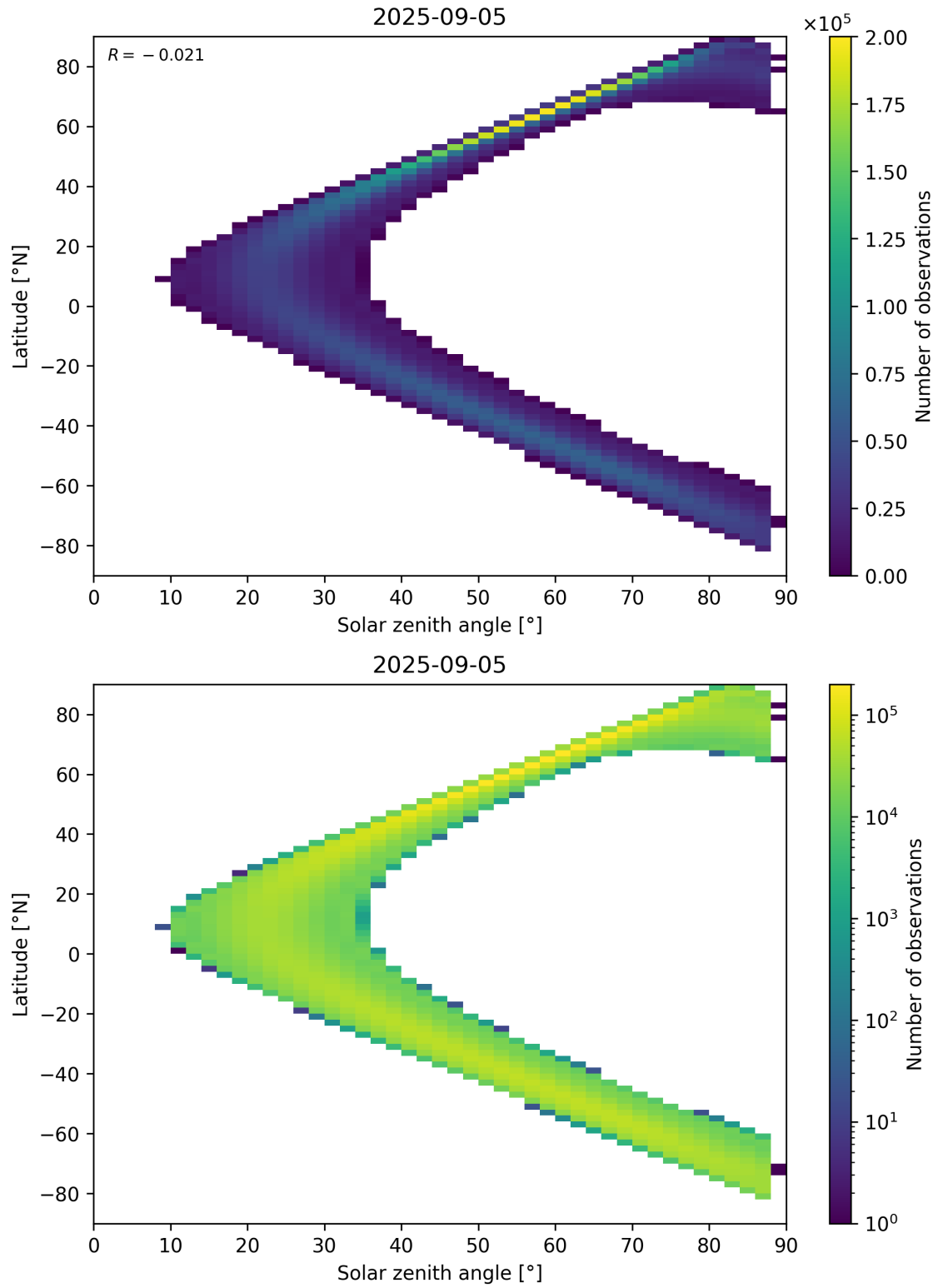
Figure 113: Scatter density plot of “Solar zenith angle” against “Latitude” for 2025-09-04 to 2025-09-06.
