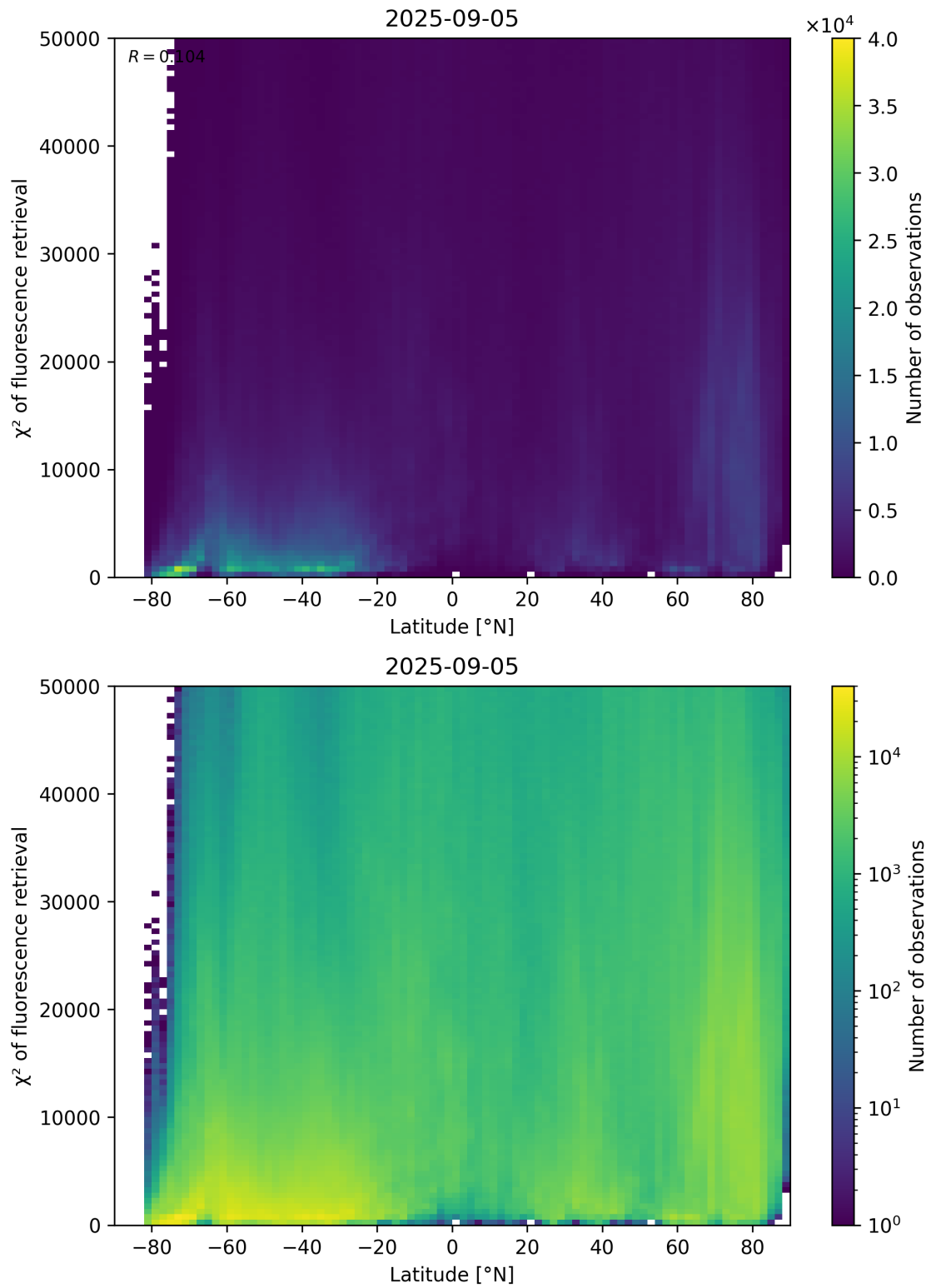
Figure 89: Scatter density plot of “Latitude” against “ \chi^2 of fluorescence retrieval” for 2025-09-04 to 2025-09-06.
