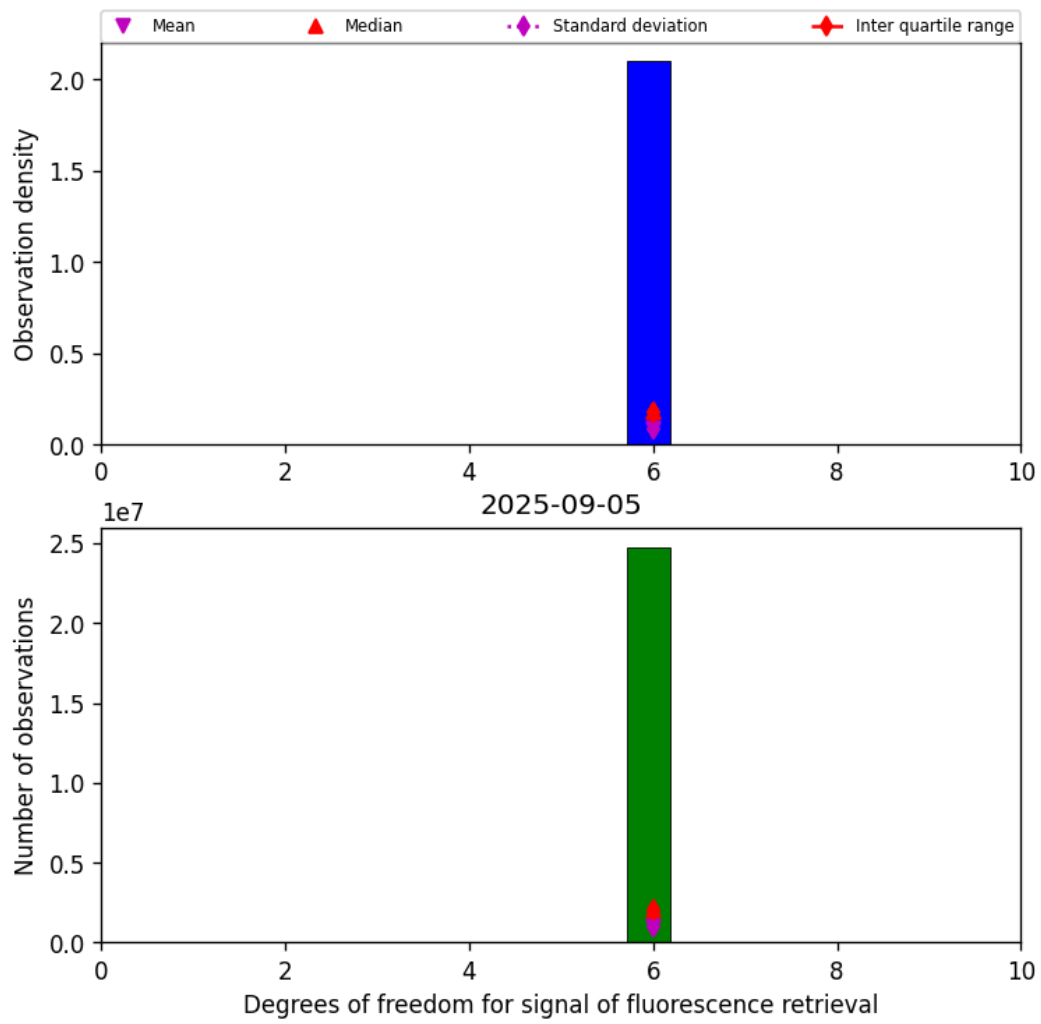
Figure 43: Histogram of “Degrees of freedom for signal of fluorescence retrieval” for 2025-09-04 to 2025-09-06
