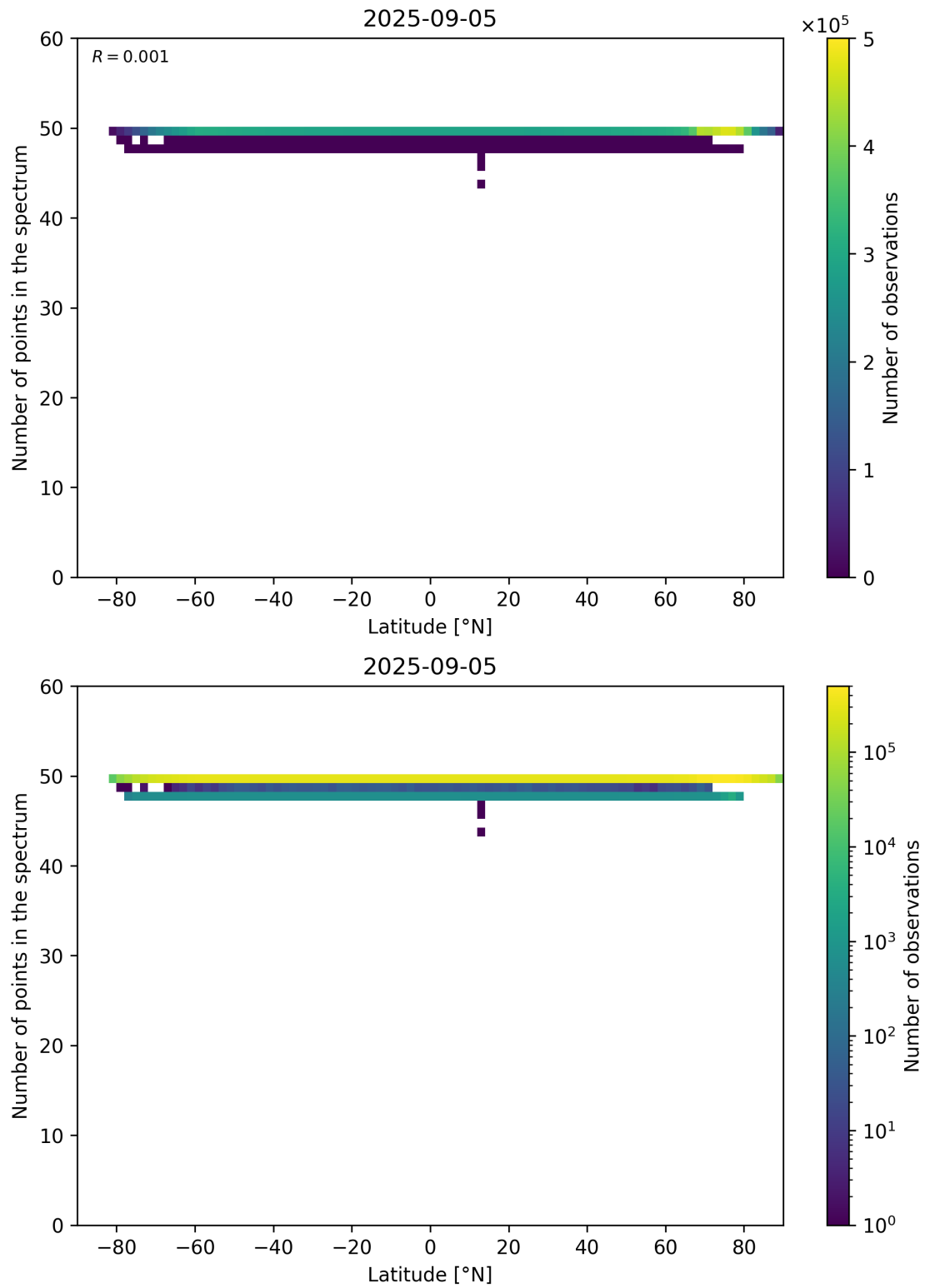
Figure 94: Scatter density plot of “Latitude” against “Number of points in the spectrum” for 2025-09-04 to 2025-09-06.
