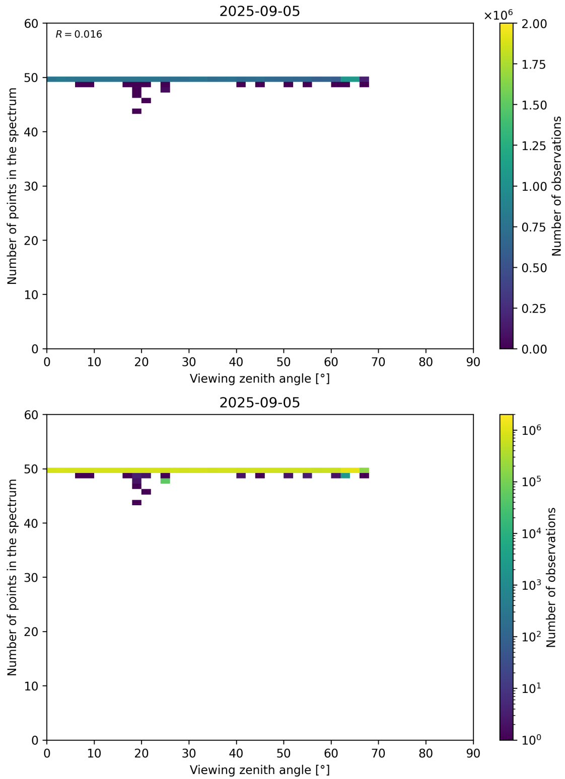
Figure 125: Scatter density plot of “Viewing zenith angle” against “Number of points in the spectrum” for 2025-09-04 to 2025-09-06.
