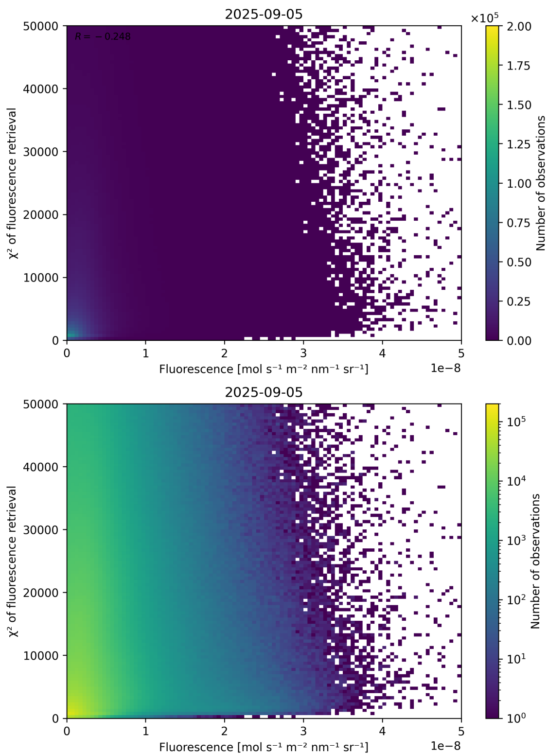
Figure 85: Scatter density plot of “Fluorescence” against “ \chi^2 of fluorescence retrieval” for 2025-09-04 to 2025-09-06.
