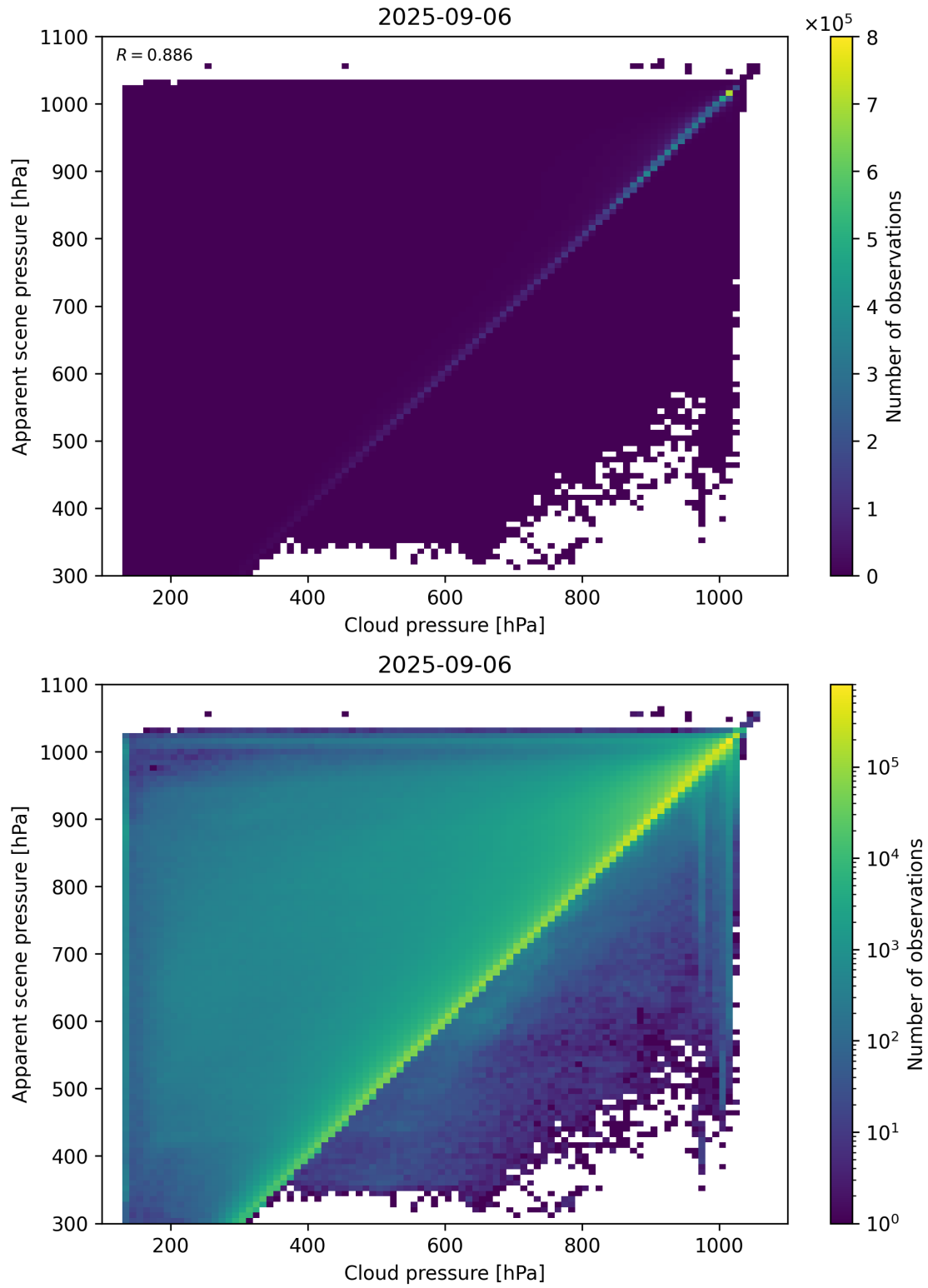
Figure 77: Scatter density plot of “Cloud pressure” against “Apparent scene pressure” for 2025-09-05 to 2025-09-07.
