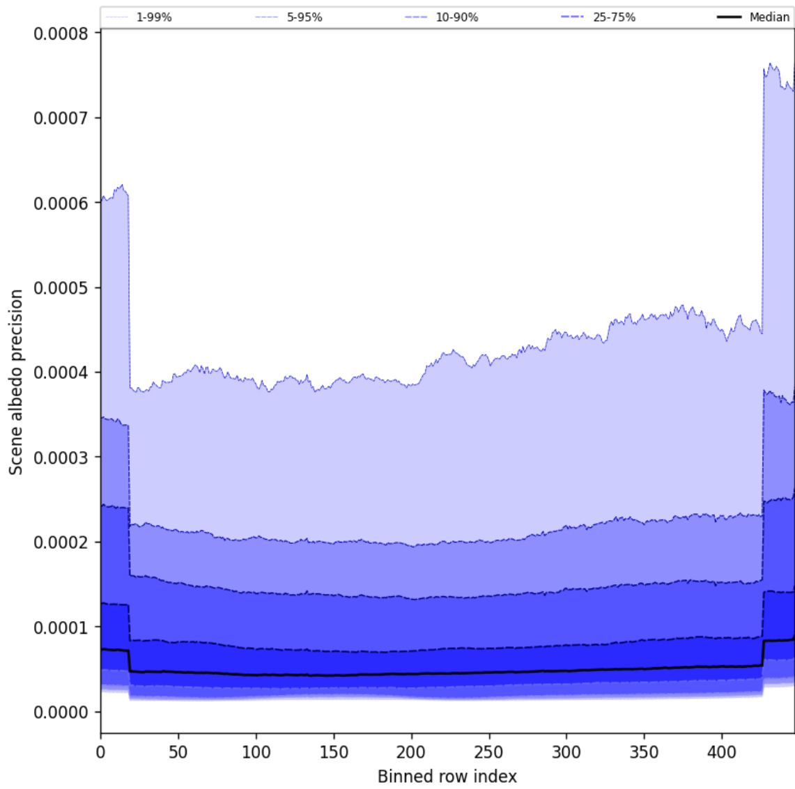
Figure 52: Along track statistics of “Scene albedo precision” for 2025-09-05 to 2025-09-07
