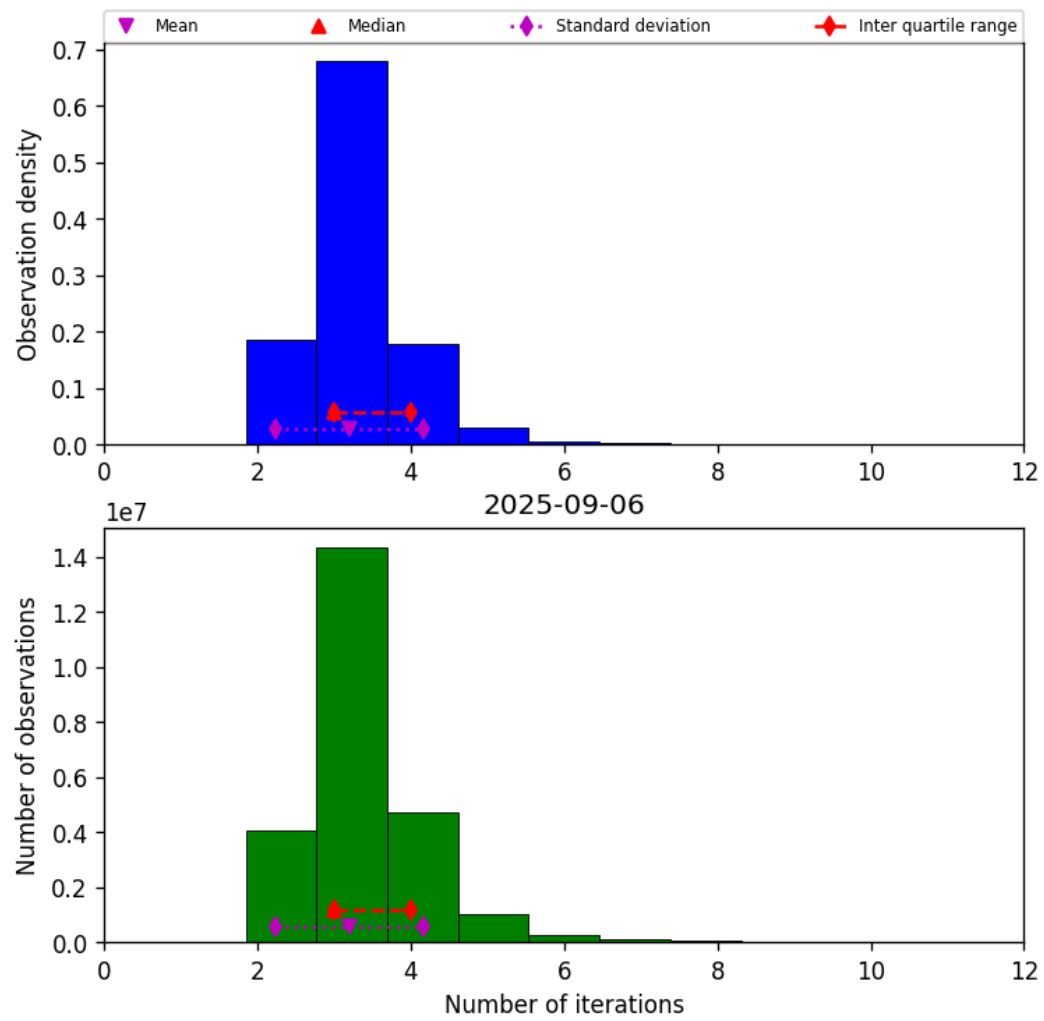
Figure 39: Histogram of “Number of iterations” for 2025-09-05 to 2025-09-07
