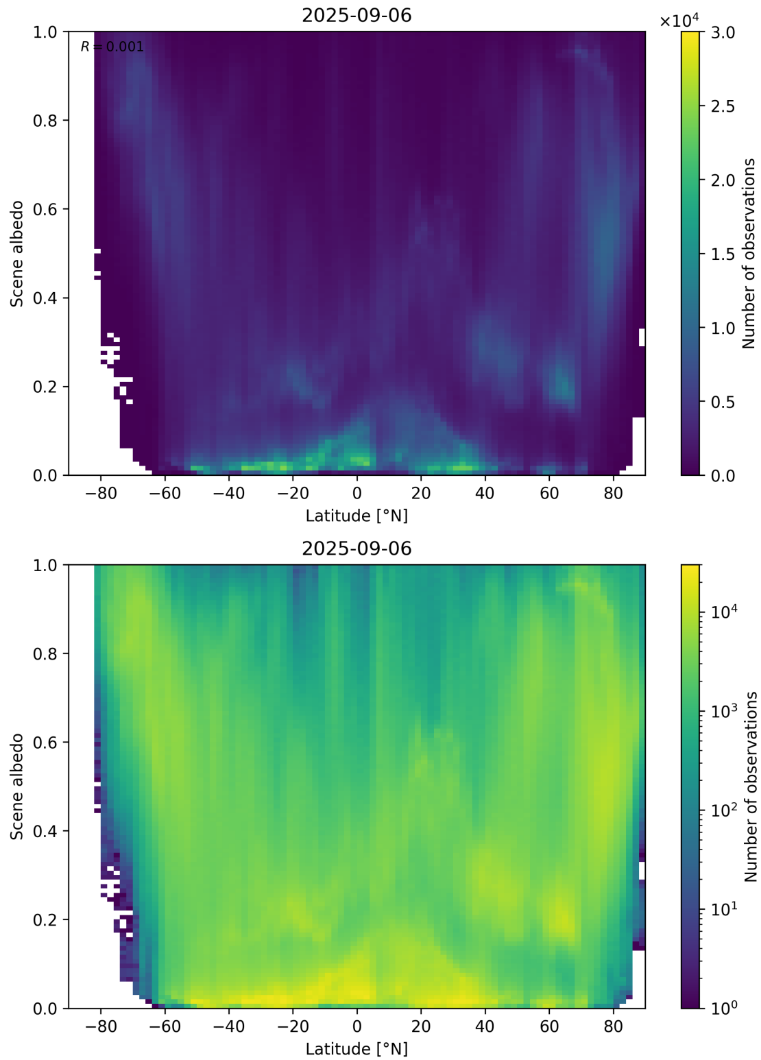
Figure 95: Scatter density plot of “Latitude” against “Scene albedo” for 2025-09-05 to 2025-09-07.
