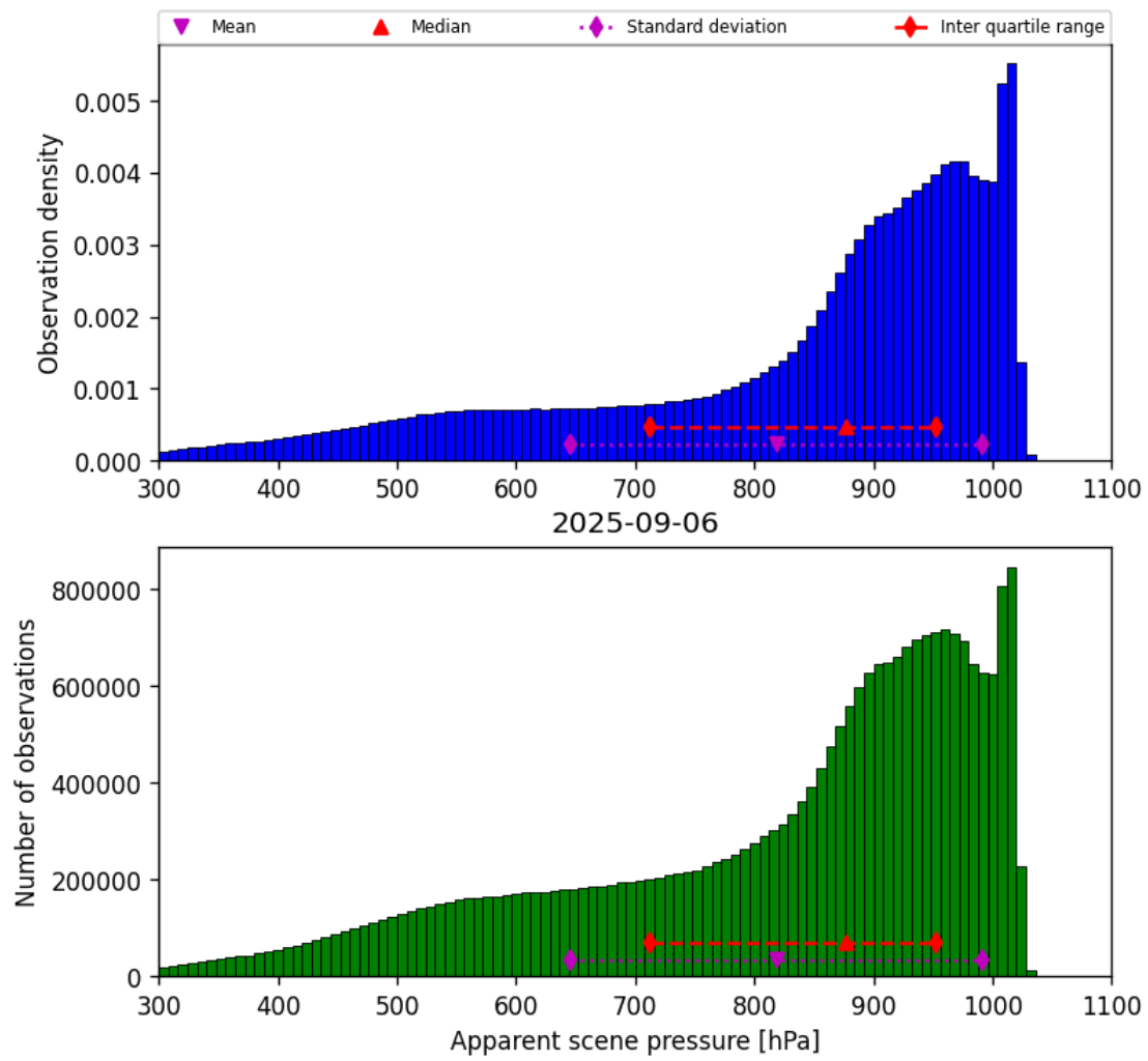
Figure 36: Histogram of “Apparent scene pressure” for 2025-09-05 to 2025-09-07
