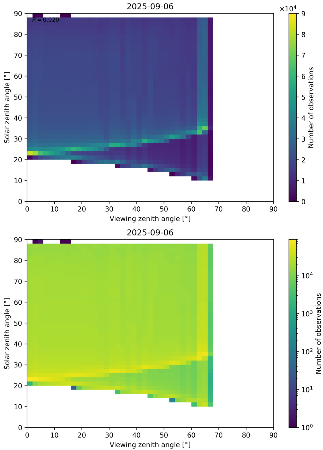
Figure 127: Scatter density plot of “Viewing zenith angle” against “Solar zenith angle” for 2025-09-05 to 2025-09-07.
