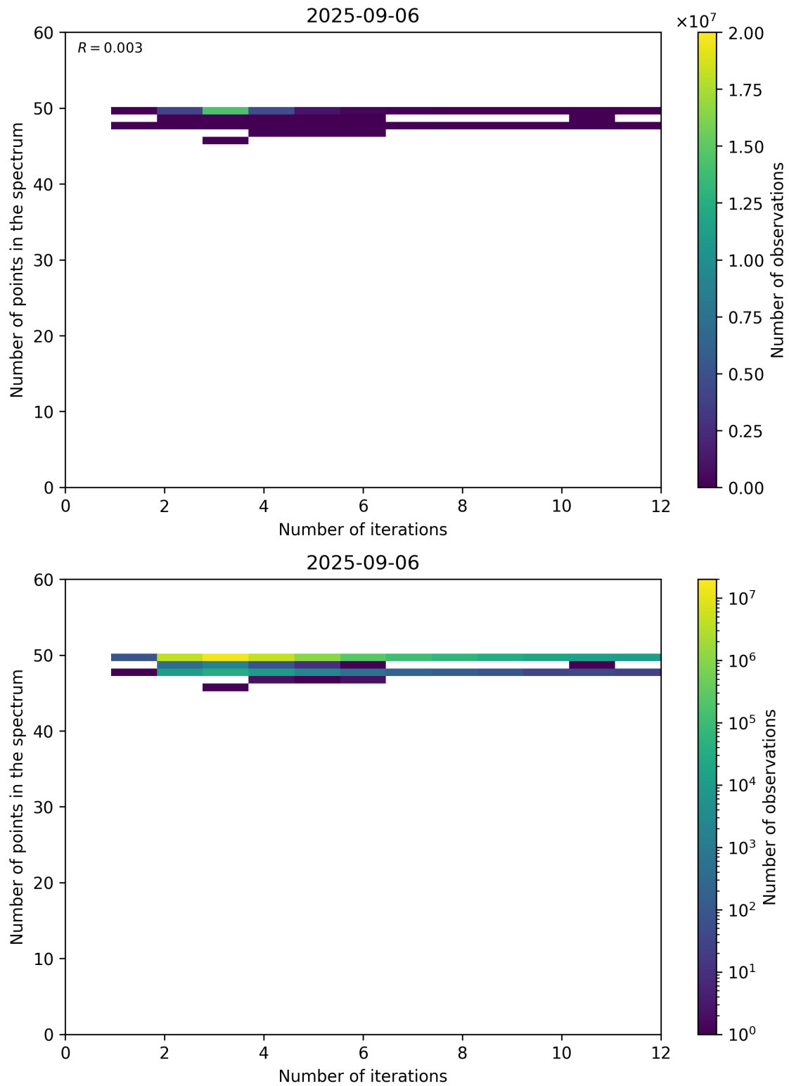
Figure 99: Scatter density plot of “Number of iterations” against “Number of points in the spectrum” for 2025-09-05 to 2025-09-07.
