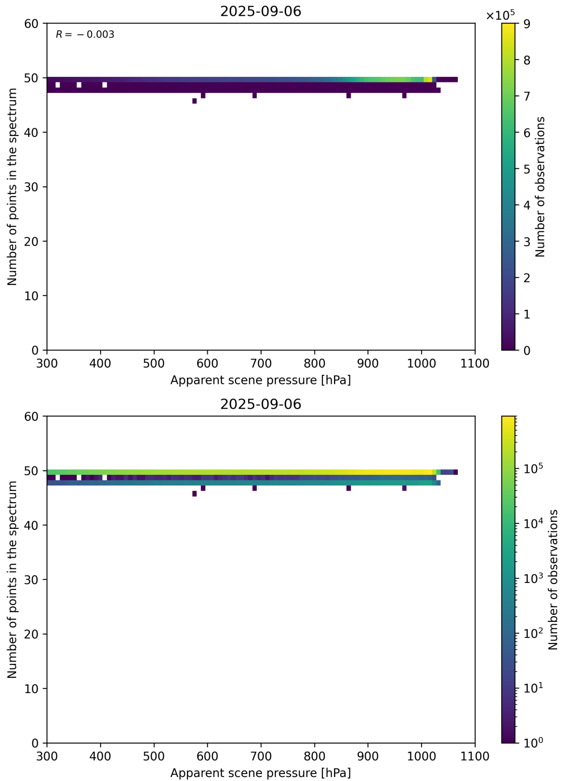
Figure 66: Scatter density plot of “Apparent scene pressure” against “Number of points in the spectrum” for 2025-09-05 to 2025-09-07.
