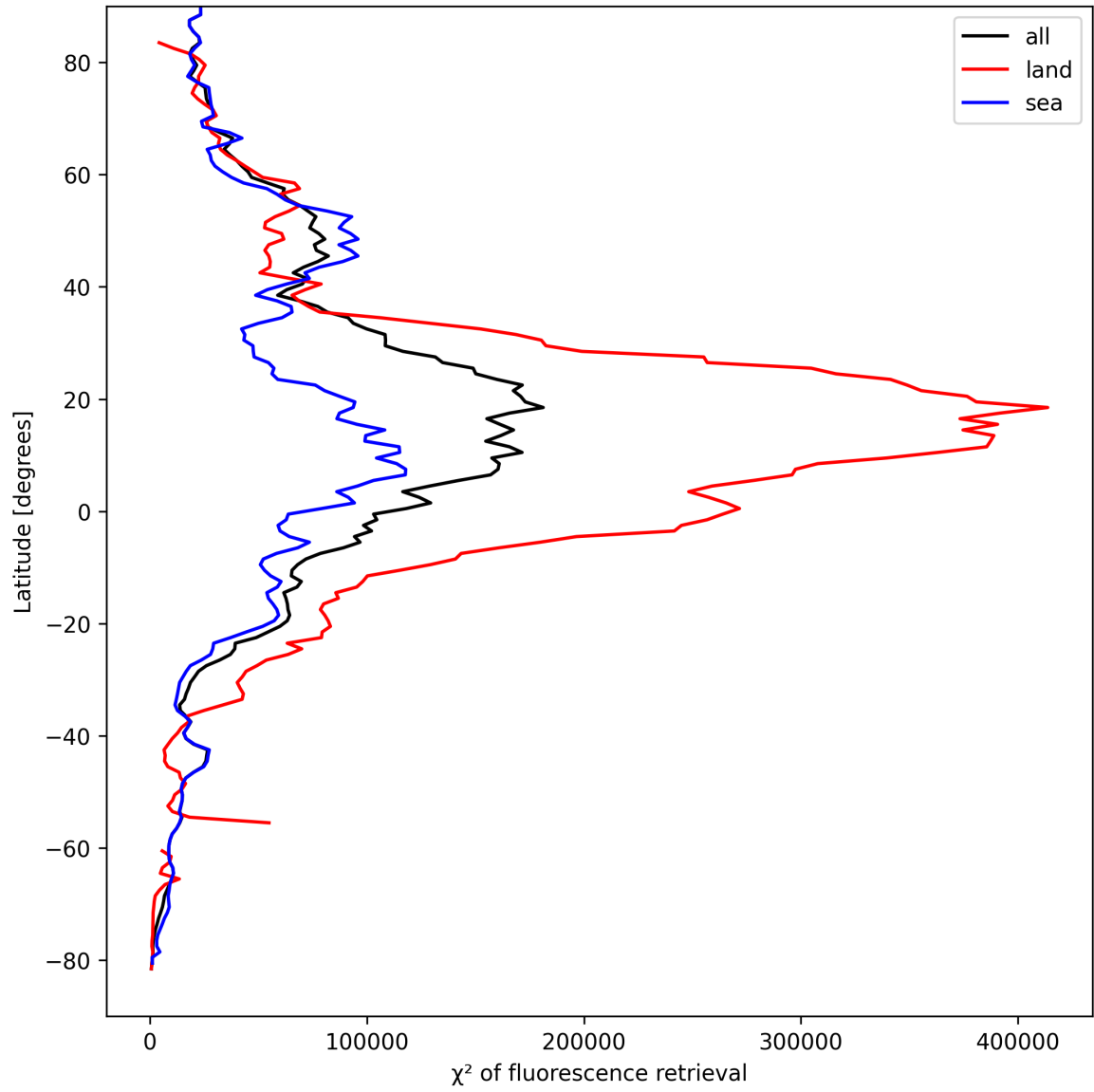
Figure 25: Zonal average of “ \chi^2 of fluorescence retrieval” for 2025-09-05 to 2025-09-07.
