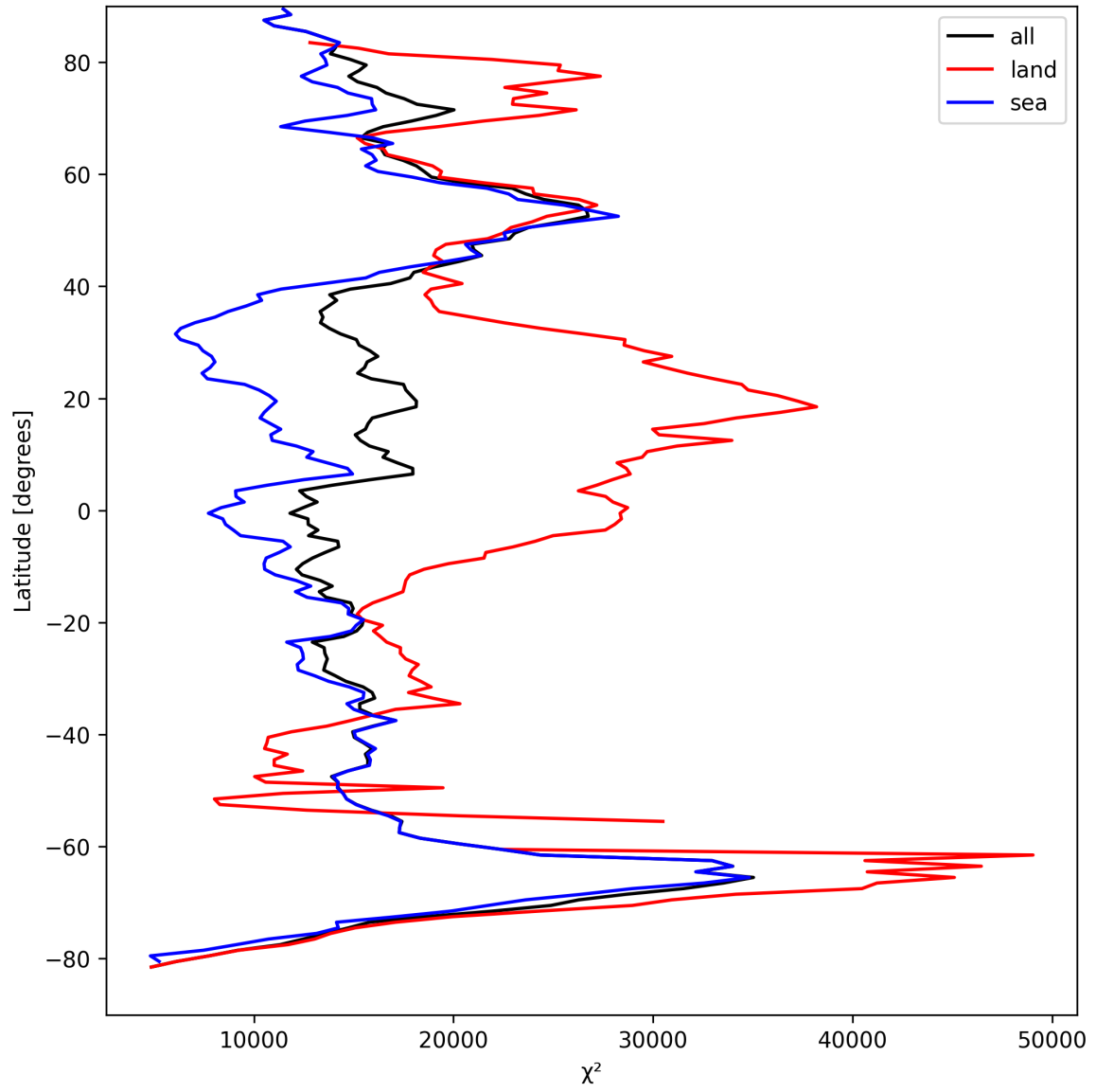
Figure 21: Zonal average of “ \chi^2 ” for 2025-09-05 to 2025-09-07.
