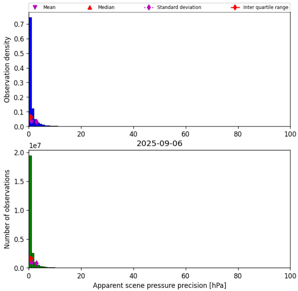
Figure 37: Histogram of “Apparent scene pressure precision” for 2025-09-05 to 2025-09-07
