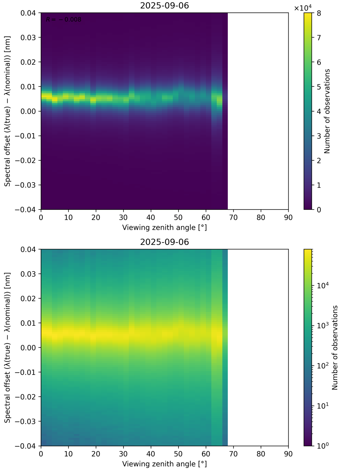
Figure 128: Scatter density plot of “Viewing zenith angle” against “Spectral offset ( \lambda_{\text{true}} - \lambda_{\text{nominal}} )” for 2025-09-05 to 2025-09-07.
