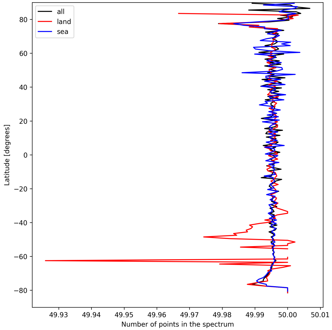
Figure 27: Zonal average of “Number of points in the spectrum” for 2025-09-05 to 2025-09-07.
