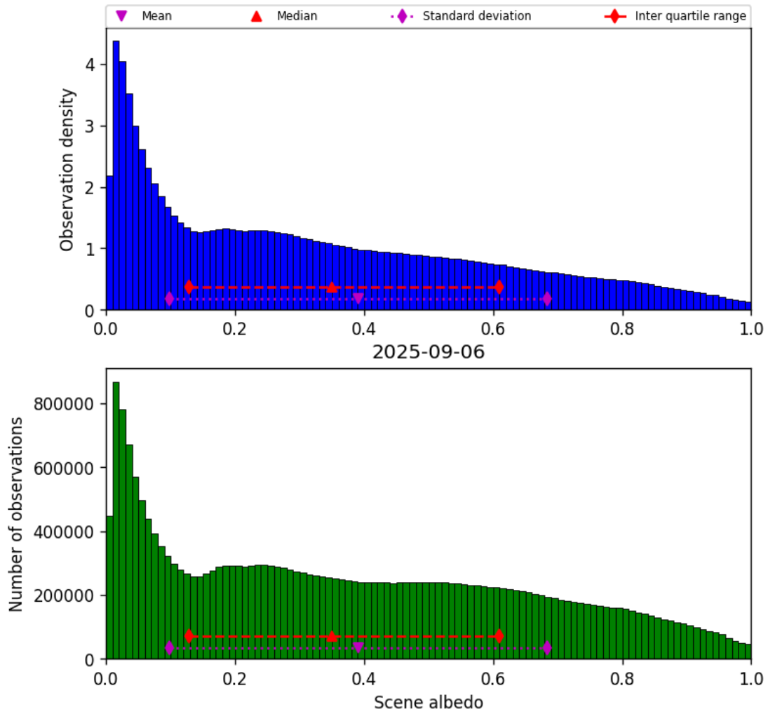
Figure 34: Histogram of “Scene albedo” for 2025-09-05 to 2025-09-07
