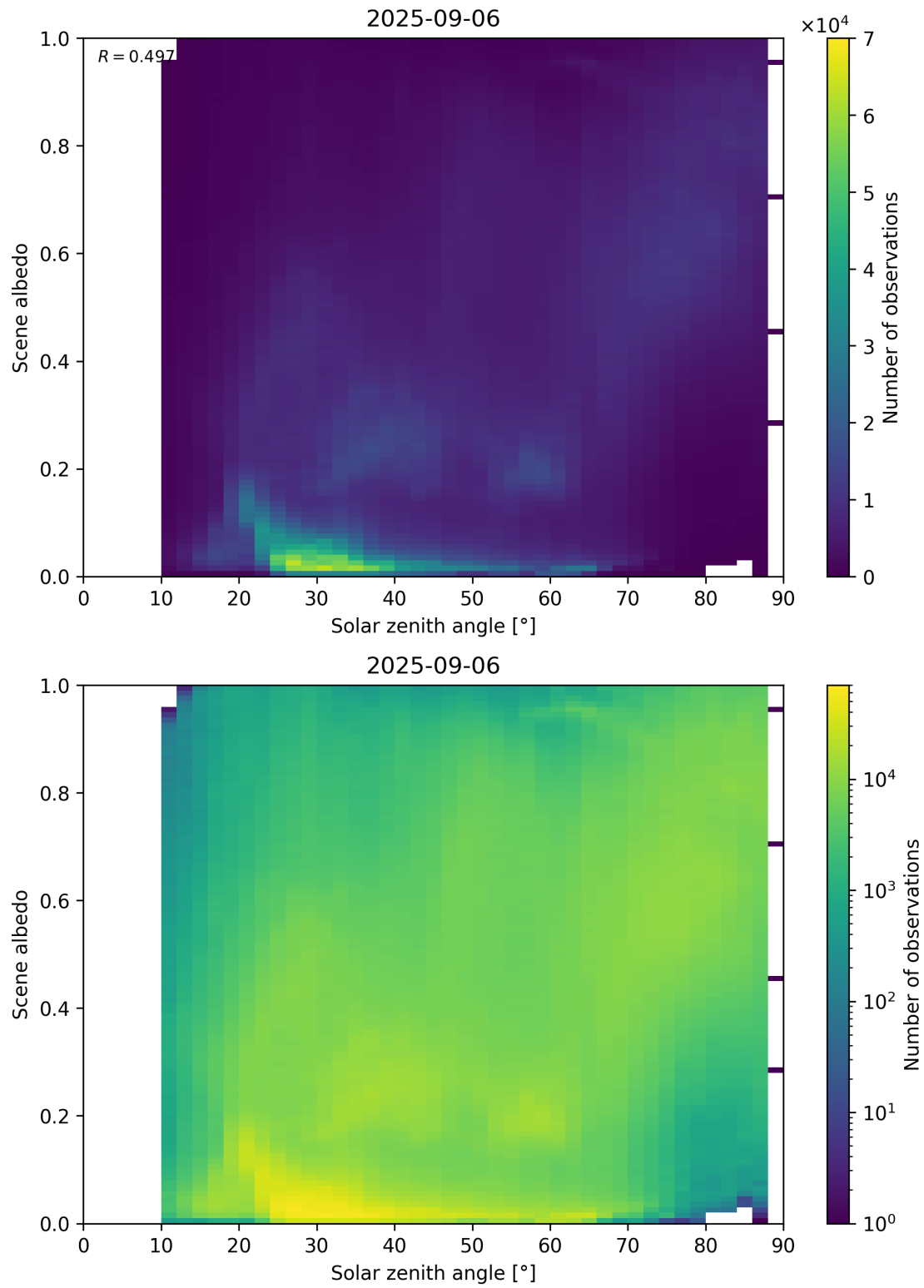
Figure 116: Scatter density plot of “Solar zenith angle” against “Scene albedo” for 2025-09-05 to 2025-09-07.
