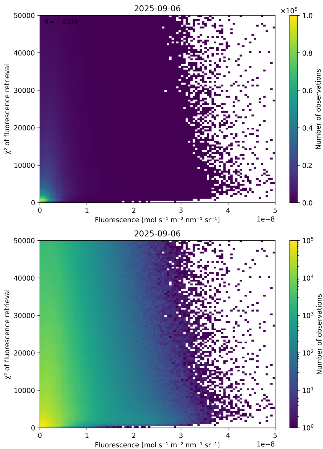
Figure 85: Scatter density plot of “Fluorescence” against “ \chi^2 of fluorescence retrieval” for 2025-09-05 to 2025-09-07.
