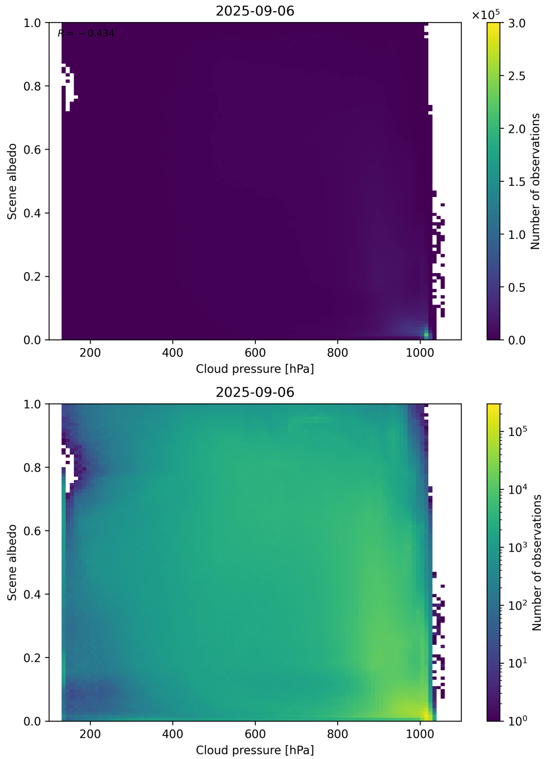
Figure 83: Scatter density plot of “Cloud pressure” against “Scene albedo” for 2025-09-05 to 2025-09-07.
