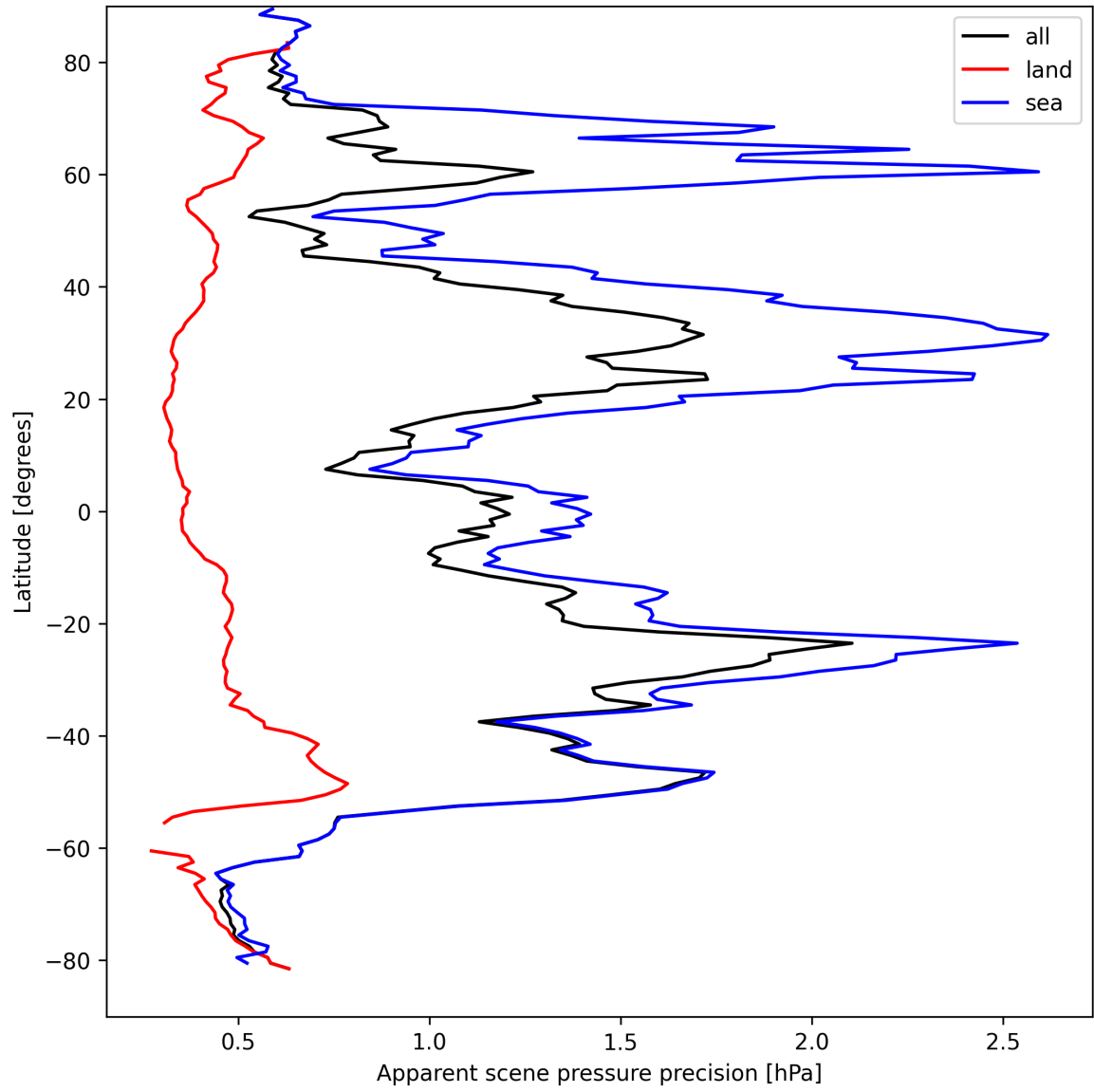
Figure 20: Zonal average of “Apparent scene pressure precision” for 2025-09-05 to 2025-09-07.
