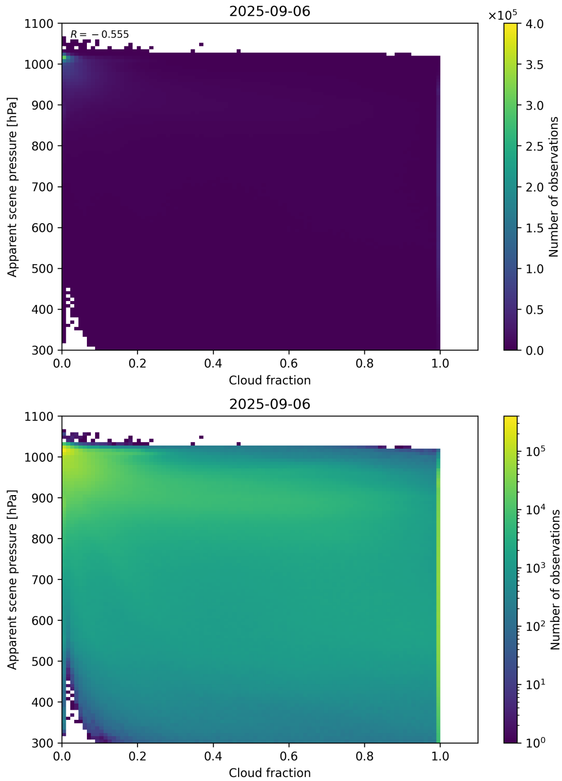
Figure 70: Scatter density plot of “Cloud fraction” against “Apparent scene pressure” for 2025-09-05 to 2025-09-07.
