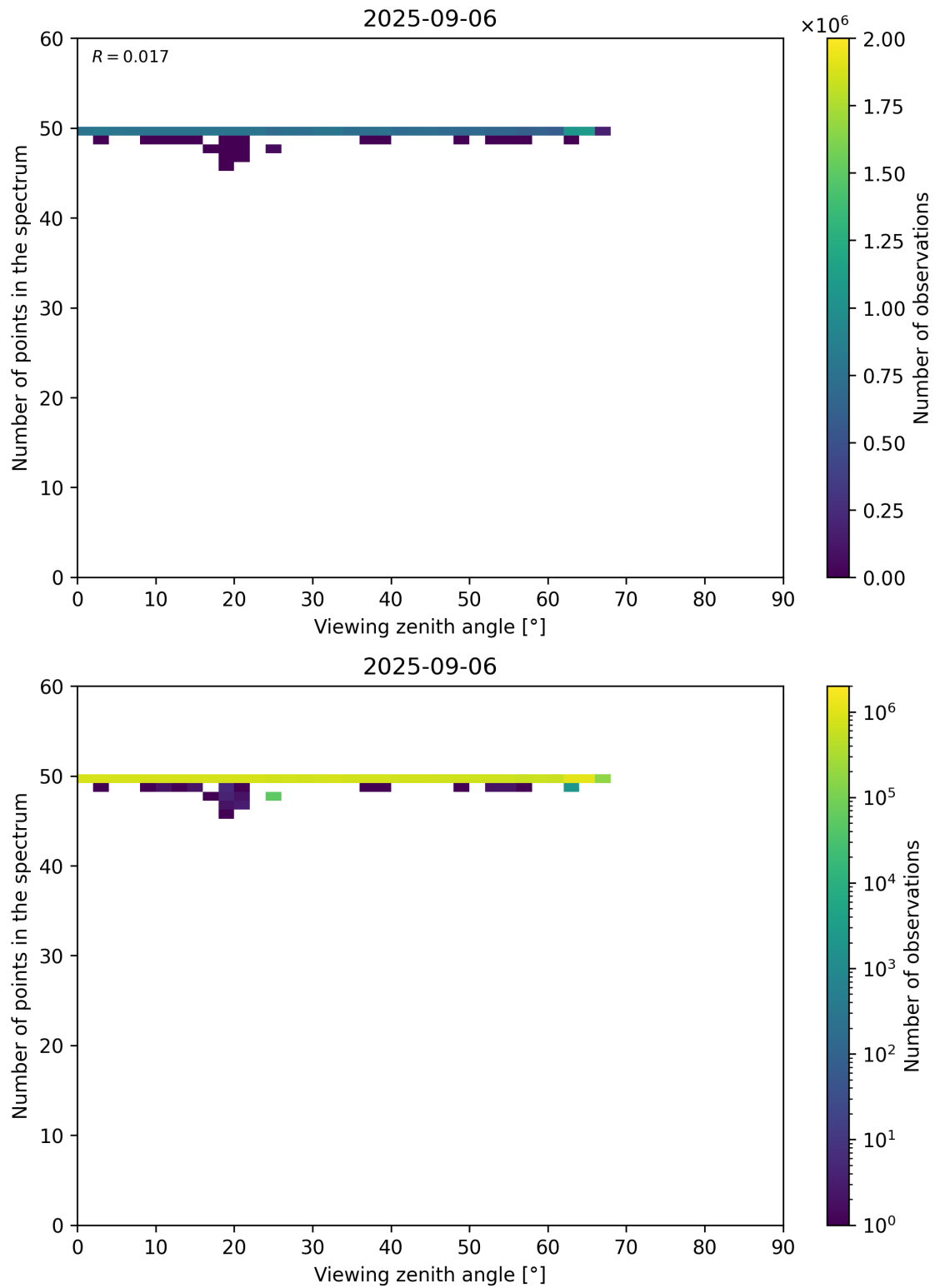
Figure 125: Scatter density plot of “Viewing zenith angle” against “Number of points in the spectrum” for 2025-09-05 to 2025-09-07.
