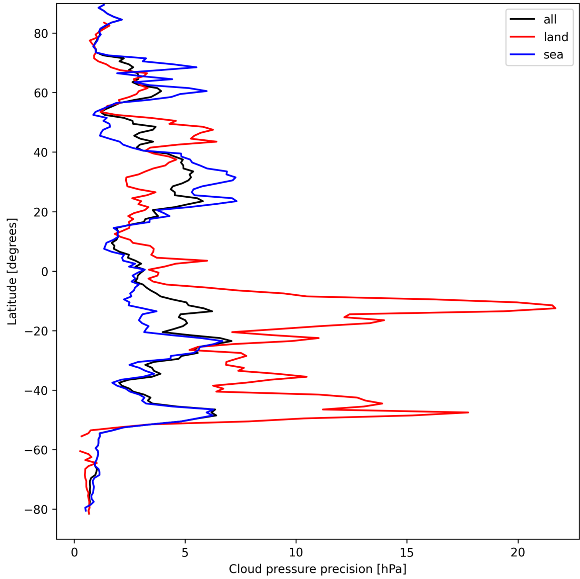
Figure 14: Zonal average of “Cloud pressure precision” for 2025-09-05 to 2025-09-07.
