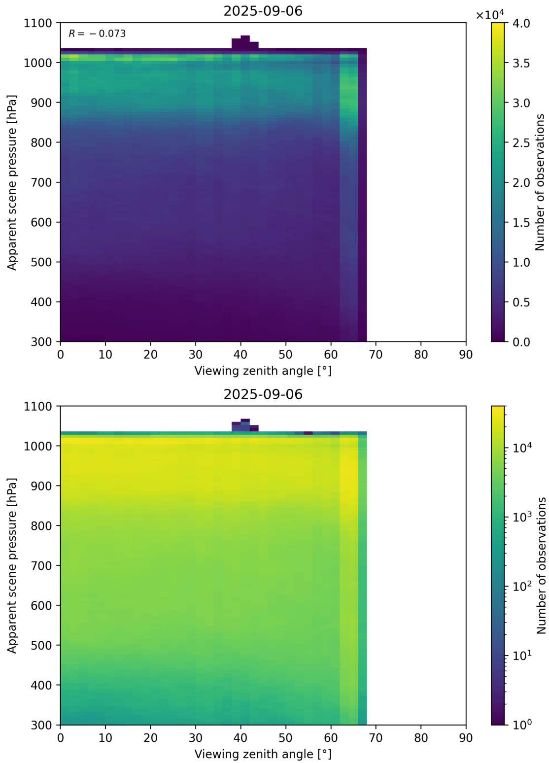
Figure 118: Scatter density plot of “Viewing zenith angle” against “Apparent scene pressure” for 2025-09-05 to 2025-09-07.
