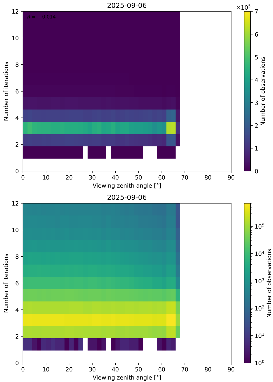
Figure 124: Scatter density plot of “Viewing zenith angle” against “Number of iterations” for 2025-09-05 to 2025-09-07.
