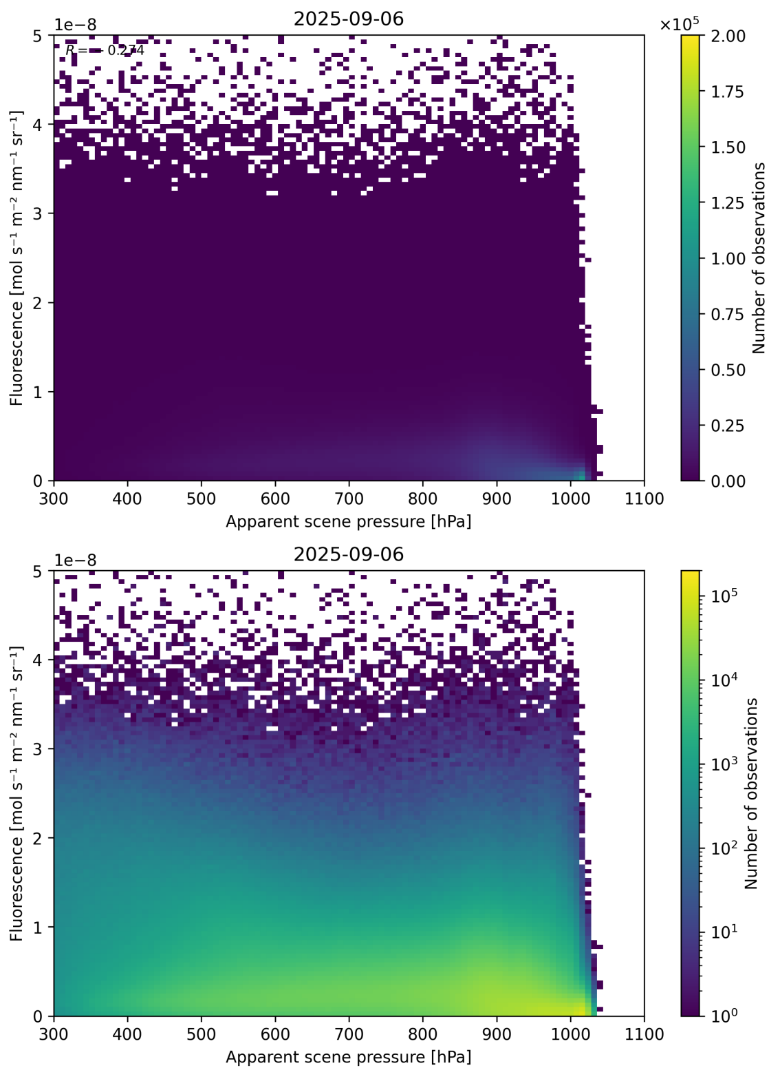
Figure 64: Scatter density plot of “Apparent scene pressure” against “Fluorescence” for 2025-09-05 to 2025-09-07.
