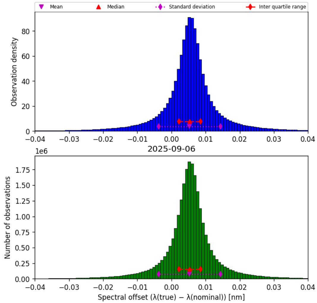
Figure 45: Histogram of “Spectral offset ( \lambda_{\text{true}} - \lambda_{\text{nominal}} )” for 2025-09-05 to 2025-09-07
