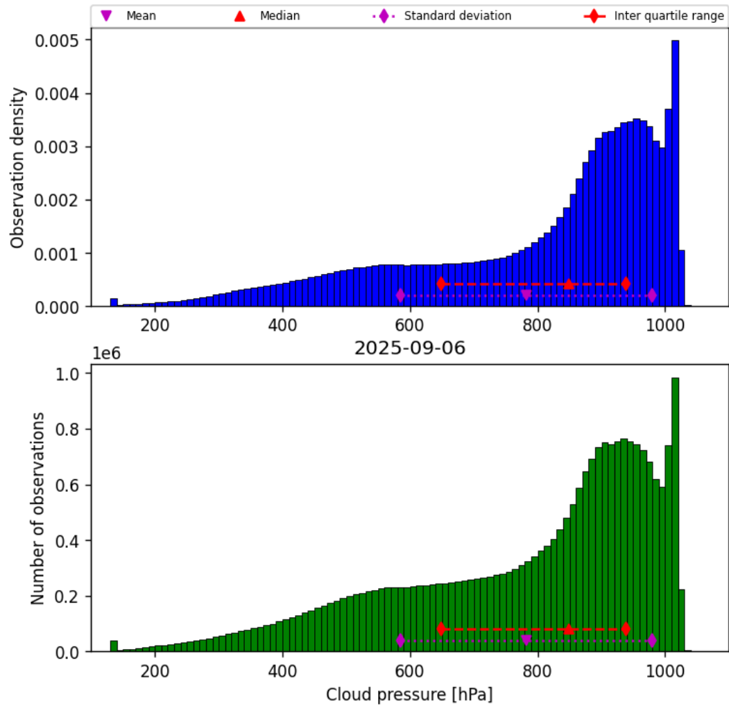
Figure 30: Histogram of “Cloud pressure” for 2025-09-05 to 2025-09-07
