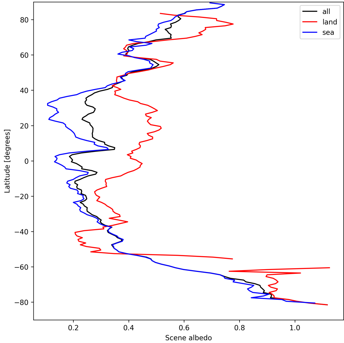
Figure 17: Zonal average of “Scene albedo” for 2025-09-05 to 2025-09-07.
