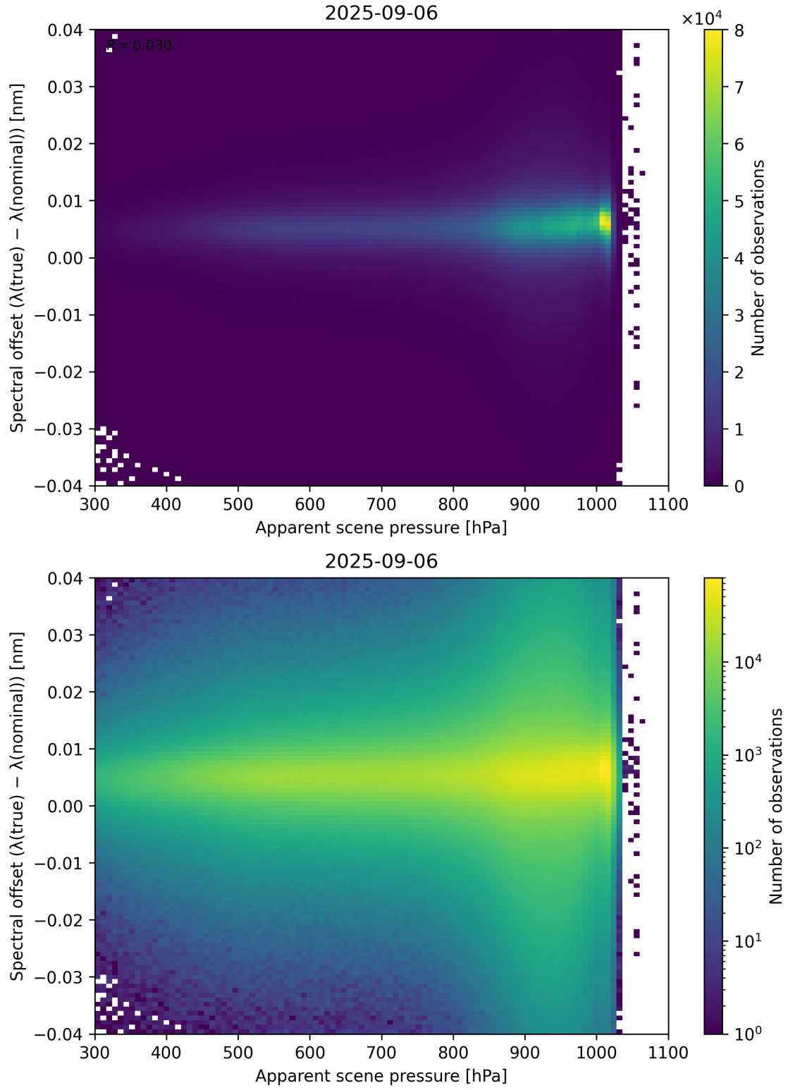
Figure 67: Scatter density plot of “Apparent scene pressure” against “Spectral offset ( \lambda_{\text{true}} - \lambda_{\text{nominal}} )” for 2025-09-05 to 2025-09-07.
