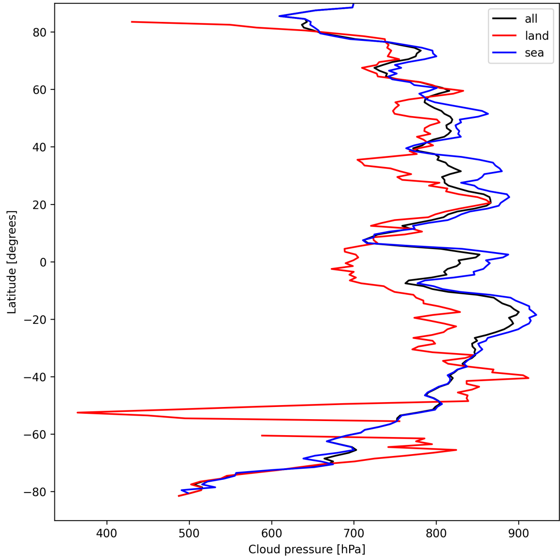
Figure 13: Zonal average of “Cloud pressure” for 2025-09-05 to 2025-09-07.
