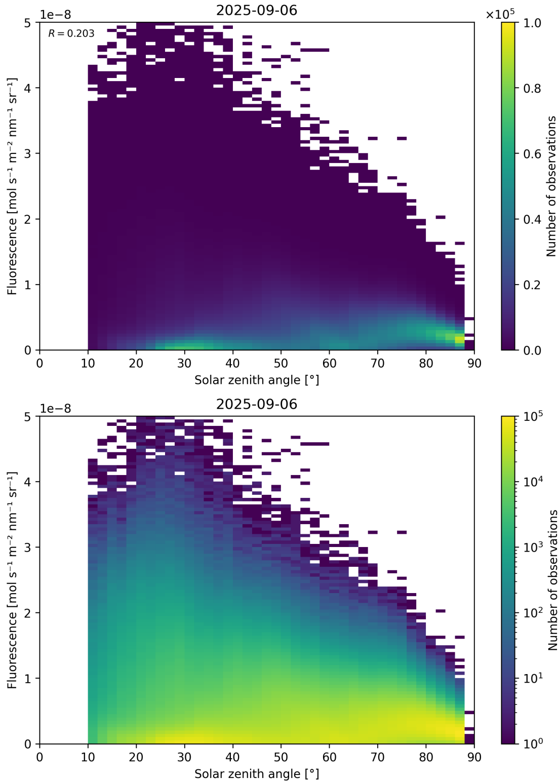
Figure 112: Scatter density plot of “Solar zenith angle” against “Fluorescence” for 2025-09-05 to 2025-09-07.
