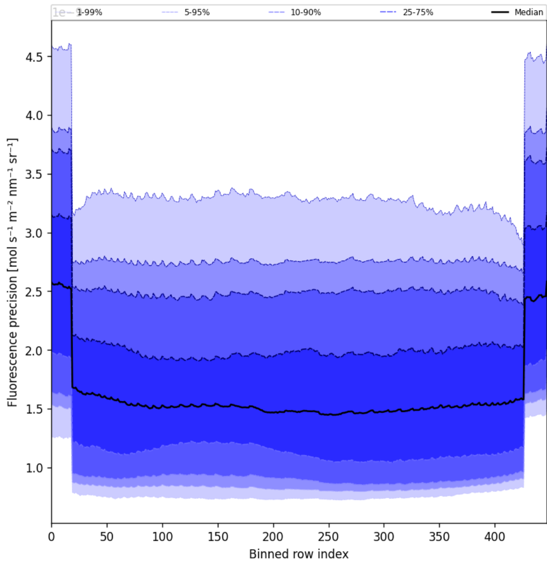
Figure 58: Along track statistics of “Fluorescence precision” for 2025-09-05 to 2025-09-07
