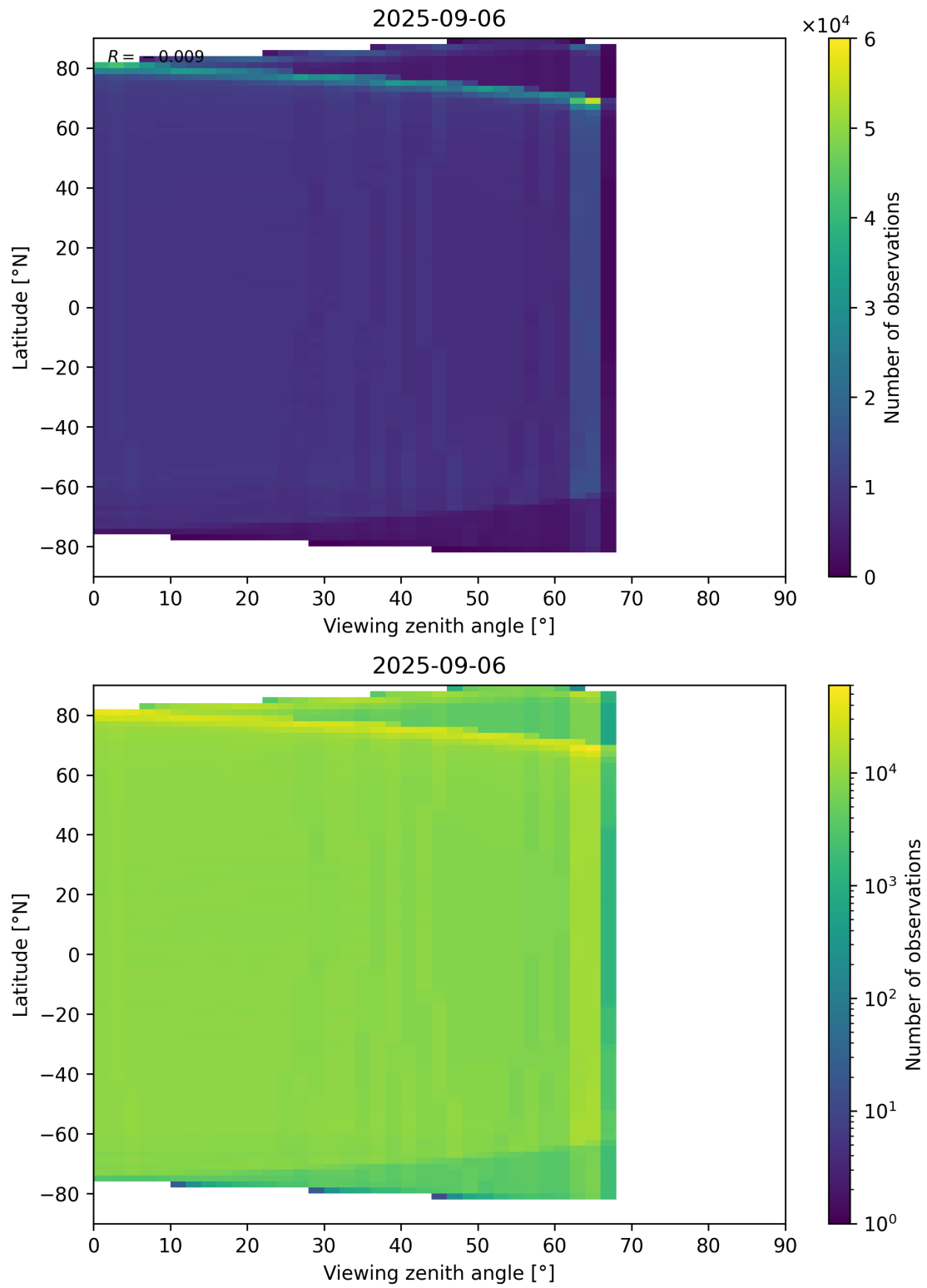
Figure 123: Scatter density plot of “Viewing zenith angle” against “Latitude” for 2025-09-05 to 2025-09-07.
