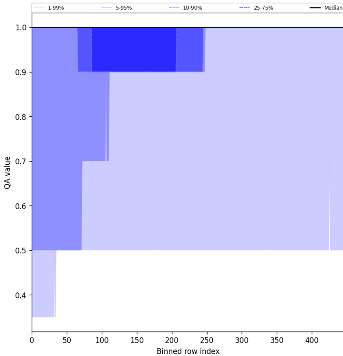
Figure 46: Along track statistics of “QA value” for 2025-09-05 to 2025-09-07
