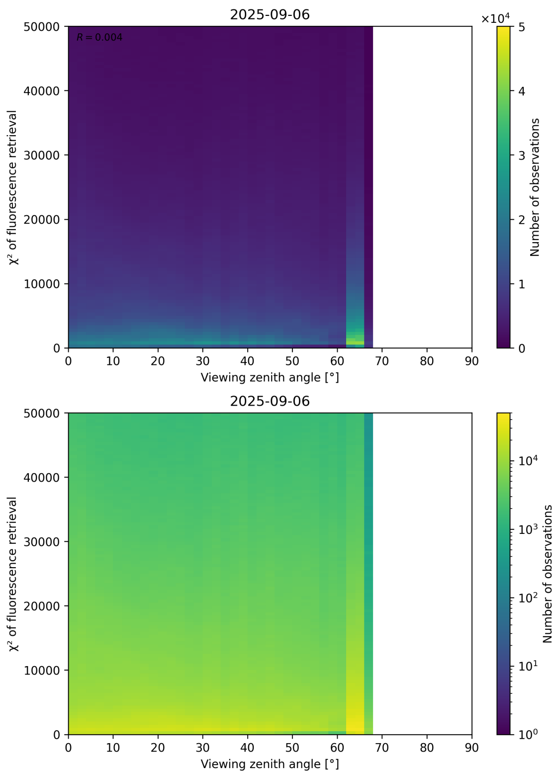
Figure 119: Scatter density plot of “Viewing zenith angle” against “ \chi^2 of fluorescence retrieval” for 2025-09-05 to 2025-09-07.
