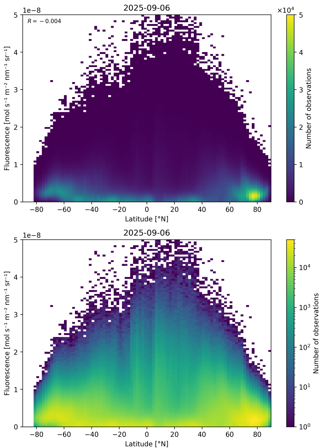
Figure 92: Scatter density plot of “Latitude” against “Fluorescence” for 2025-09-05 to 2025-09-07.
