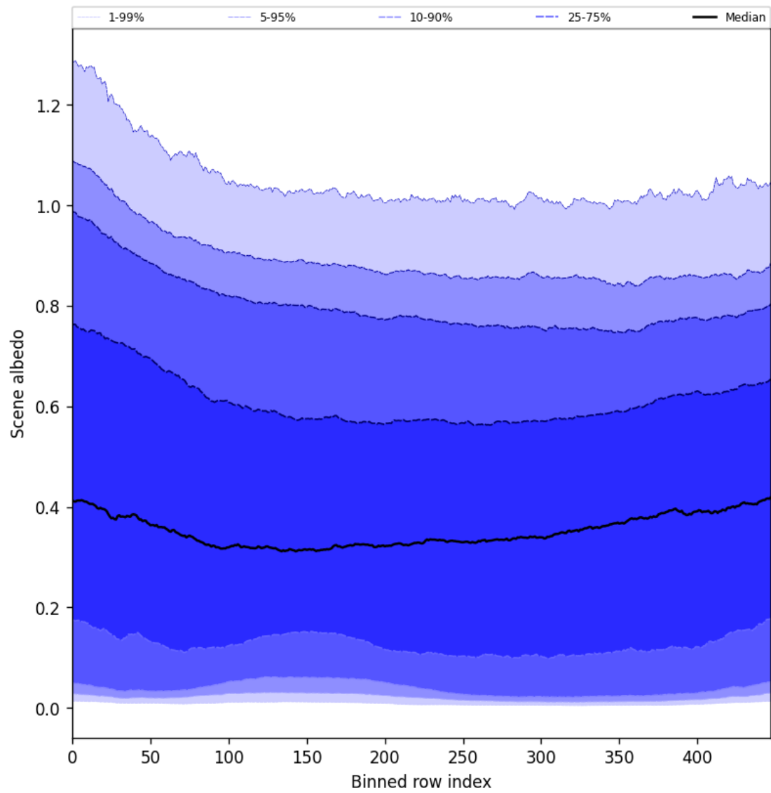
Figure 51: Along track statistics of “Scene albedo” for 2025-09-05 to 2025-09-07
