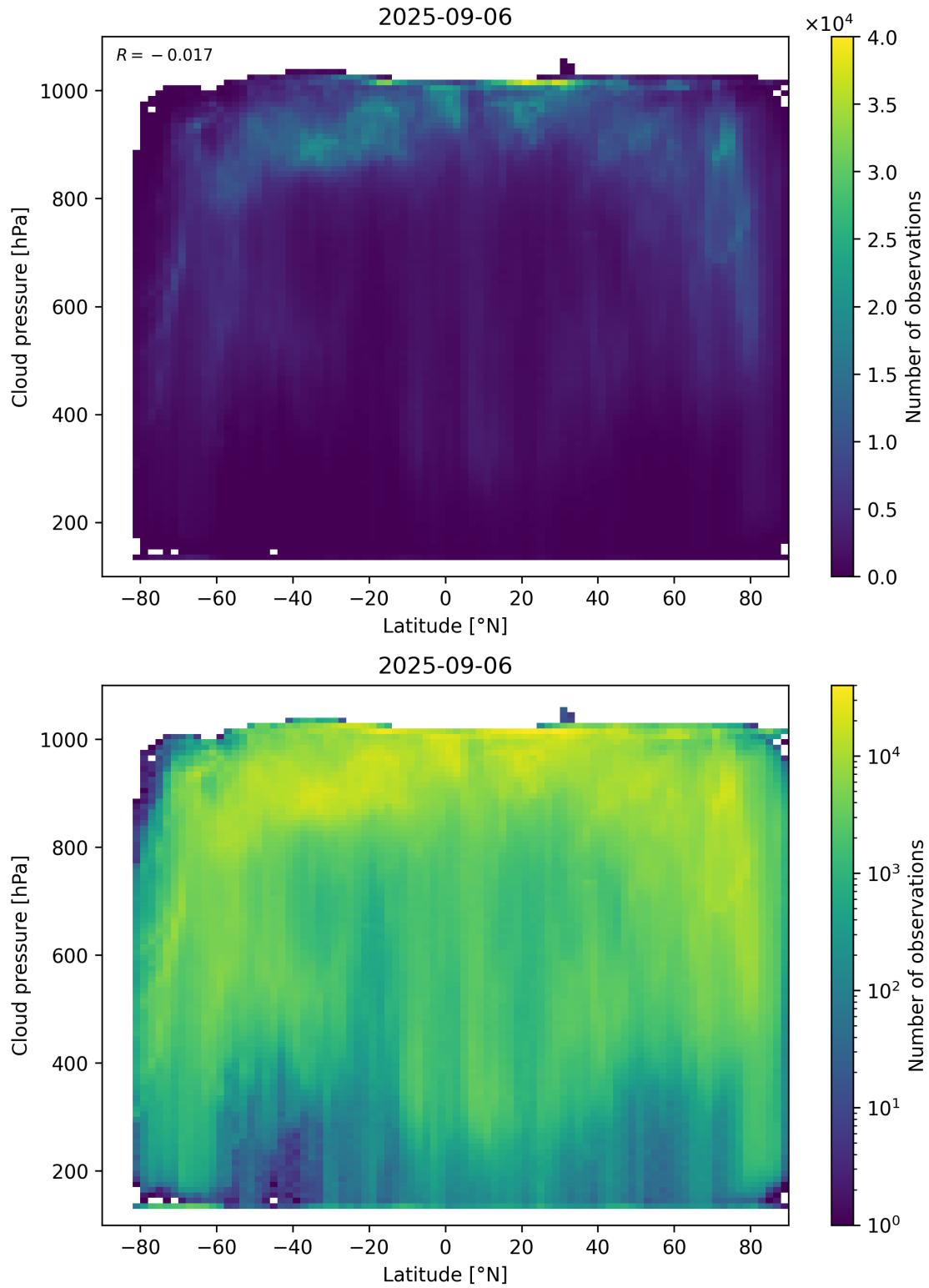
Figure 91: Scatter density plot of “Latitude” against “Cloud pressure” for 2025-09-05 to 2025-09-07.
