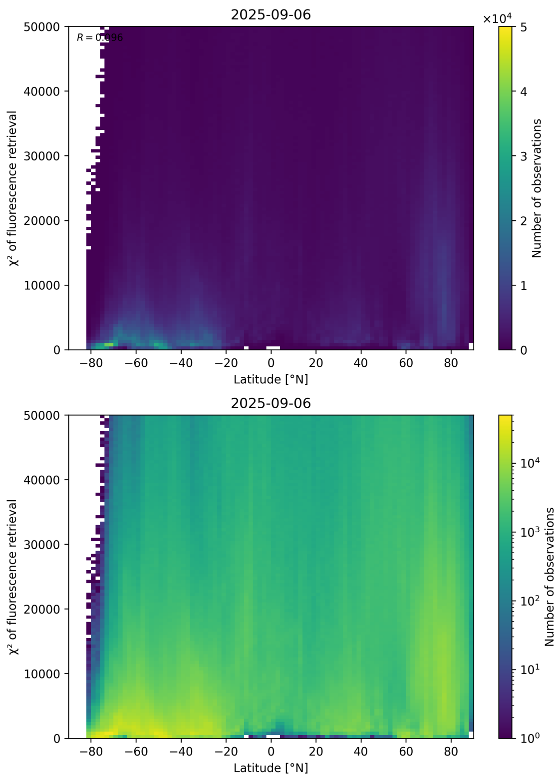
Figure 89: Scatter density plot of “Latitude” against “ \chi^2 of fluorescence retrieval” for 2025-09-05 to 2025-09-07.
