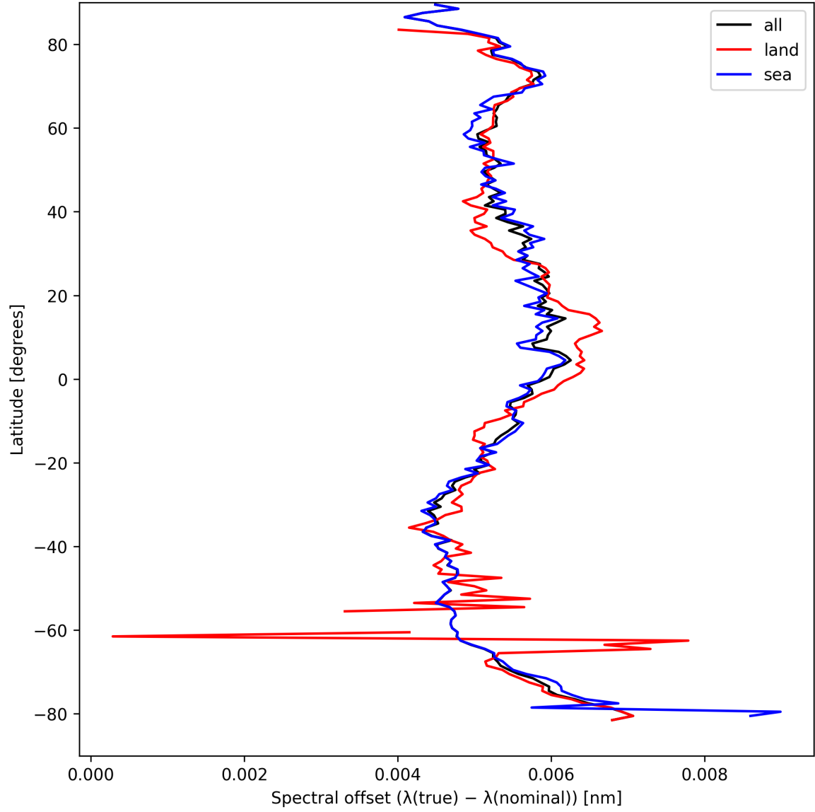
Figure 28: Zonal average of “Spectral offset ( \lambda_{\text{true}} - \lambda_{\text{nominal}} )” for 2025-09-05 to 2025-09-07.
