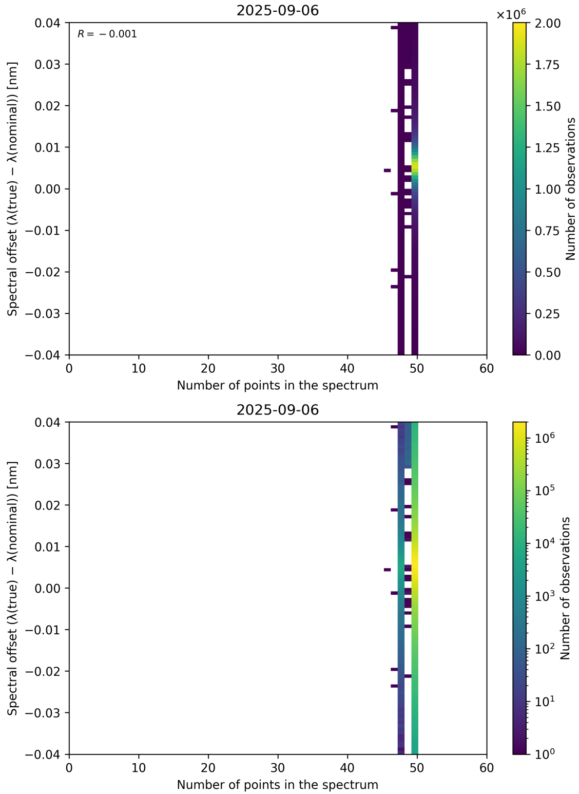
Figure 101: Scatter density plot of “Number of points in the spectrum” against “Spectral offset ( \lambda_{\text{true}} - \lambda_{\text{nominal}} )” for 2025-09-05 to 2025-09-07.
