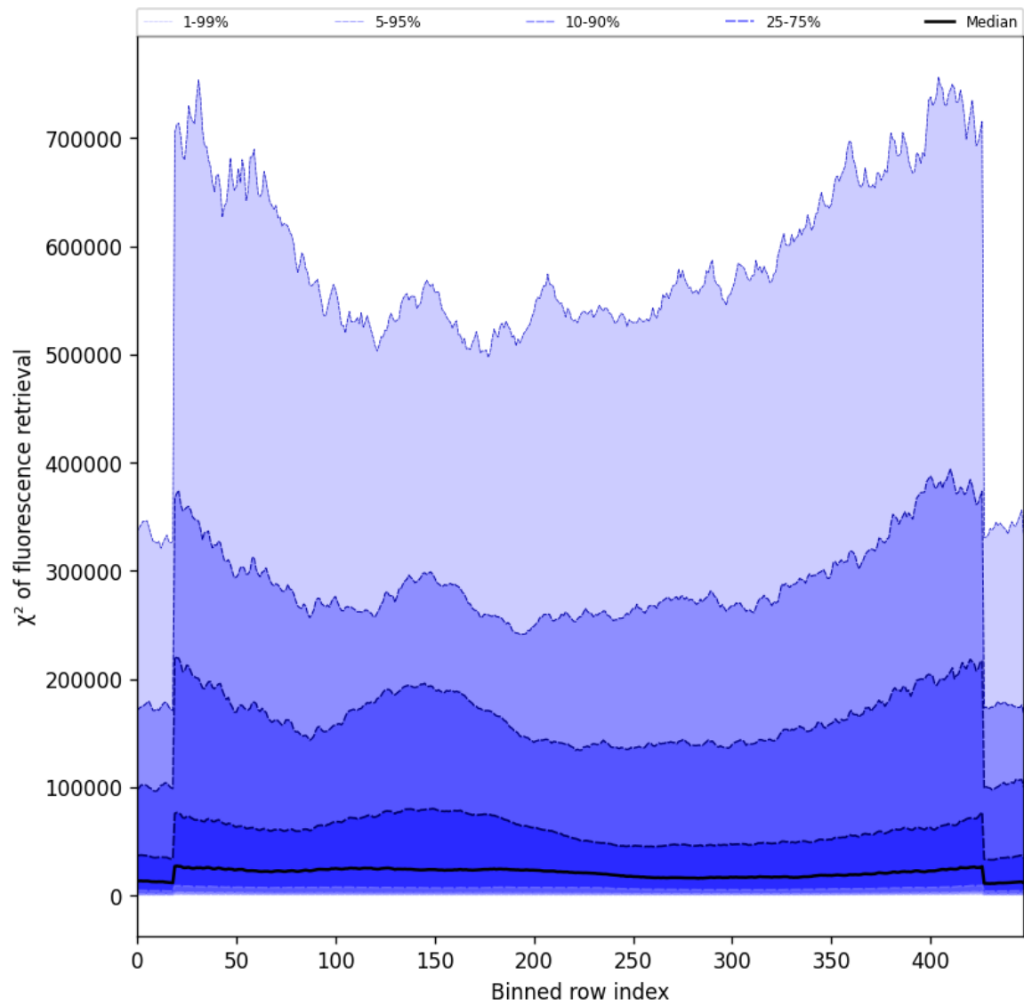
Figure 59: Along track statistics of “ \chi^2 of fluorescence retrieval” for 2025-09-05 to 2025-09-07
