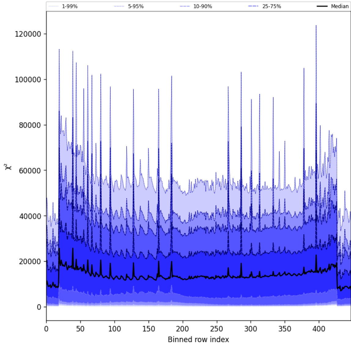
Figure 55: Along track statistics of “ \chi^2 ” for 2025-09-05 to 2025-09-07
