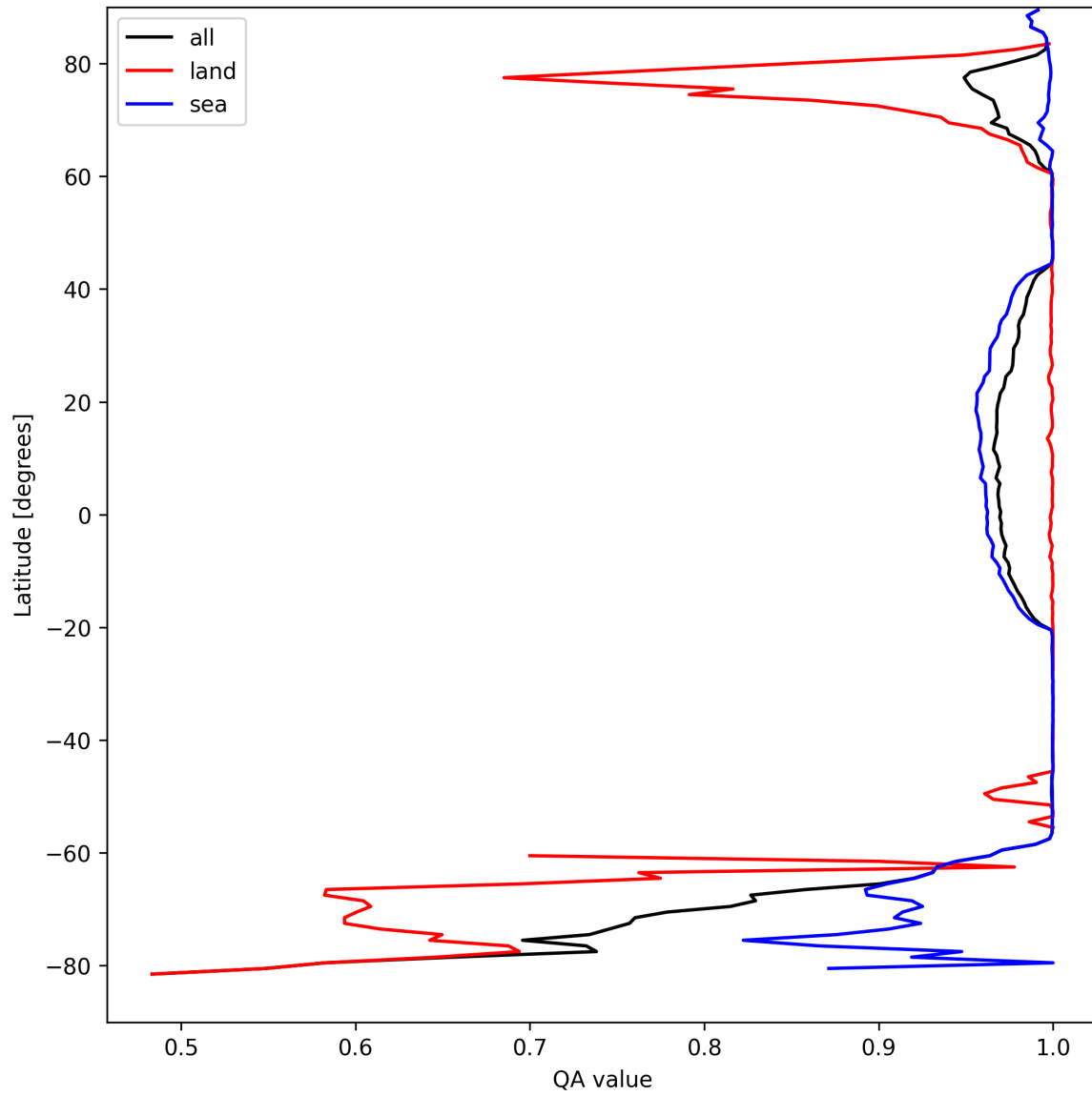
Figure 12: Zonal average of “QA value” for 2025-09-05 to 2025-09-07.
