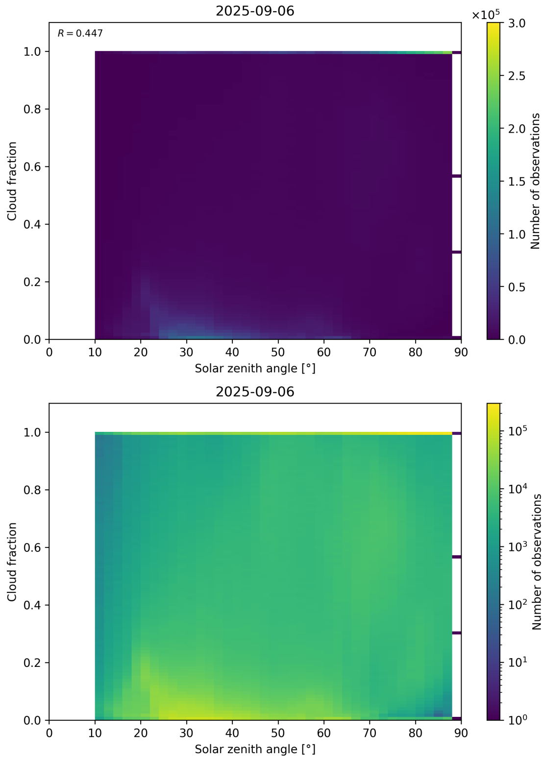
Figure 110: Scatter density plot of “Solar zenith angle” against “Cloud fraction” for 2025-09-05 to 2025-09-07.
