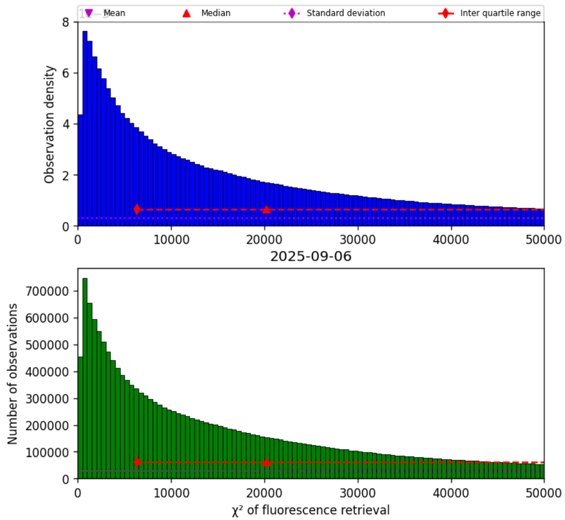
Figure 42: Histogram of “ \chi^2 of fluorescence retrieval” for 2025-09-05 to 2025-09-07
