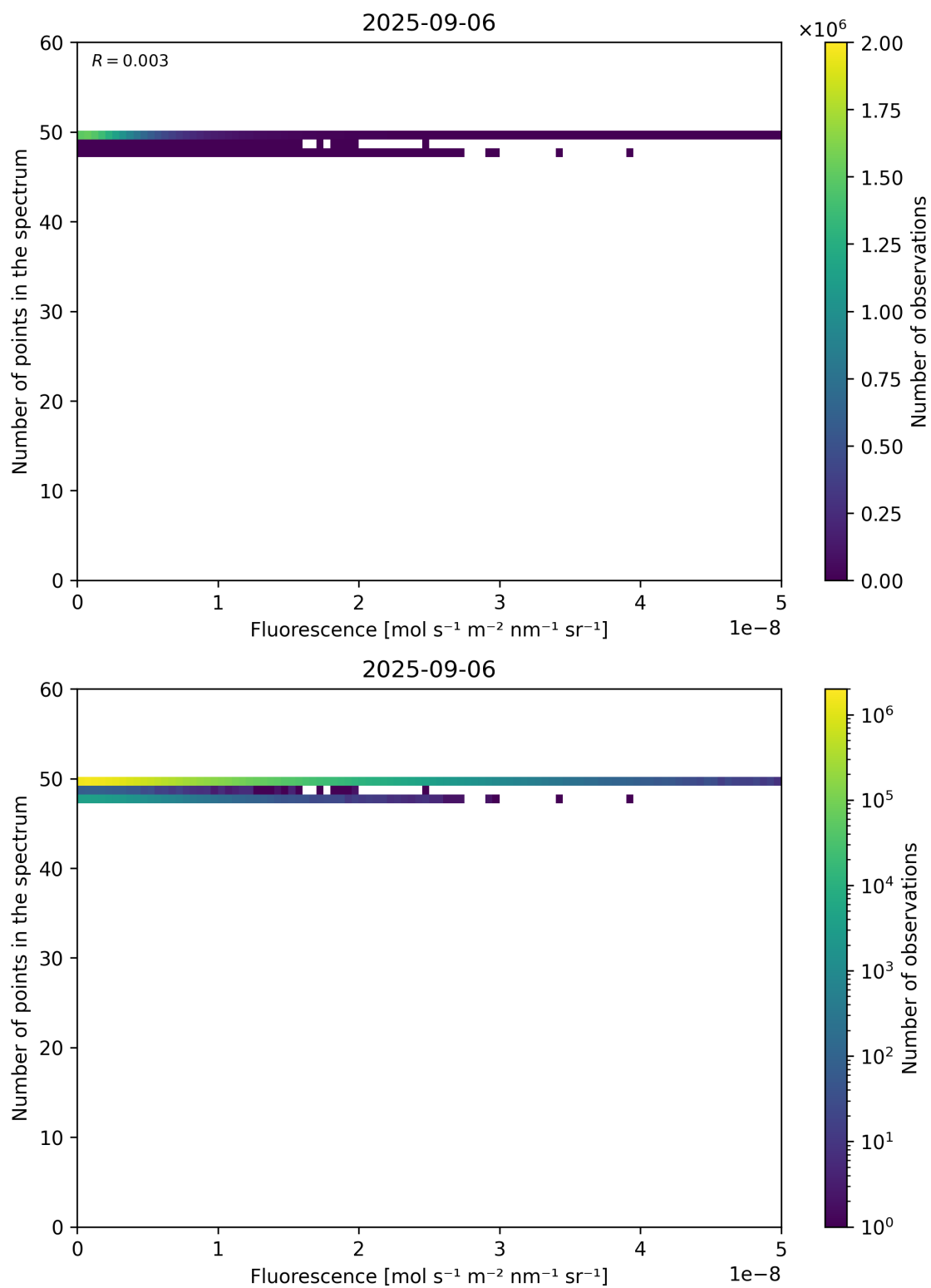
Figure 86: Scatter density plot of “Fluorescence” against “Number of points in the spectrum” for 2025-09-05 to 2025-09-07.
