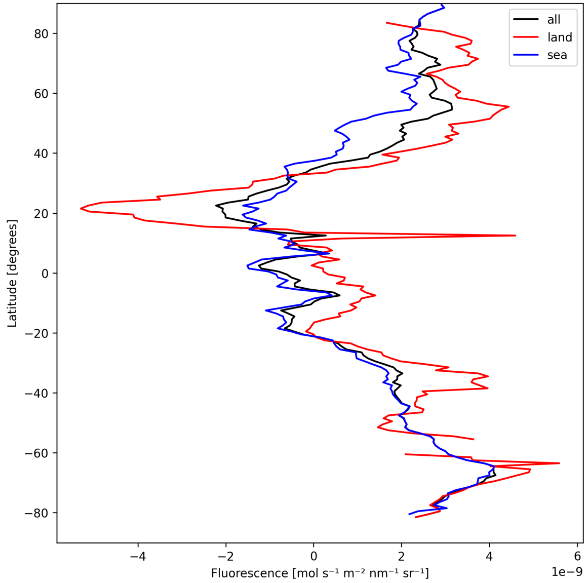
Figure 23: Zonal average of “Fluorescence” for 2025-09-05 to 2025-09-07.
