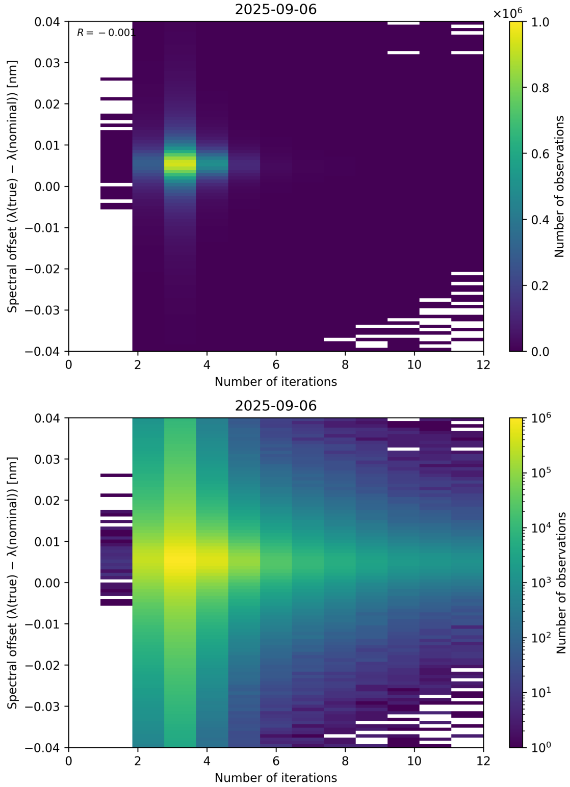
Figure 100: Scatter density plot of “Number of iterations” against “Spectral offset ( \lambda_{\text{true}} - \lambda_{\text{nominal}} )” for 2025-09-05 to 2025-09-07.
