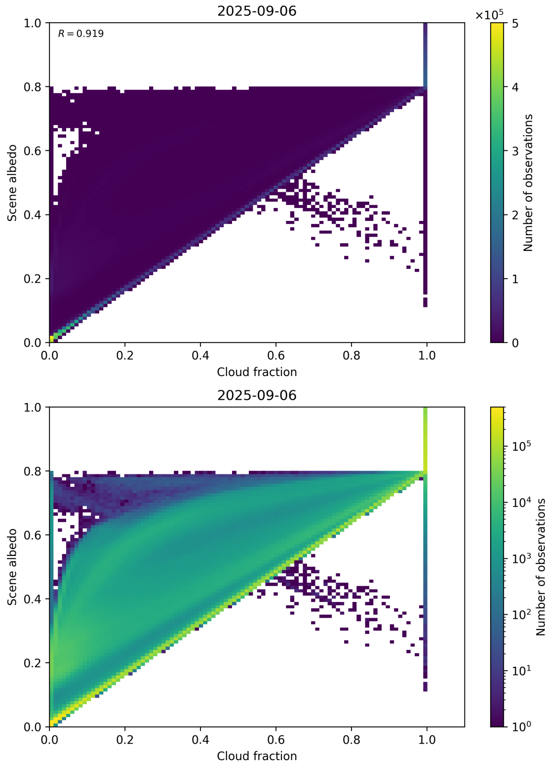
Figure 75: Scatter density plot of “Cloud fraction” against “Scene albedo” for 2025-09-05 to 2025-09-07.
