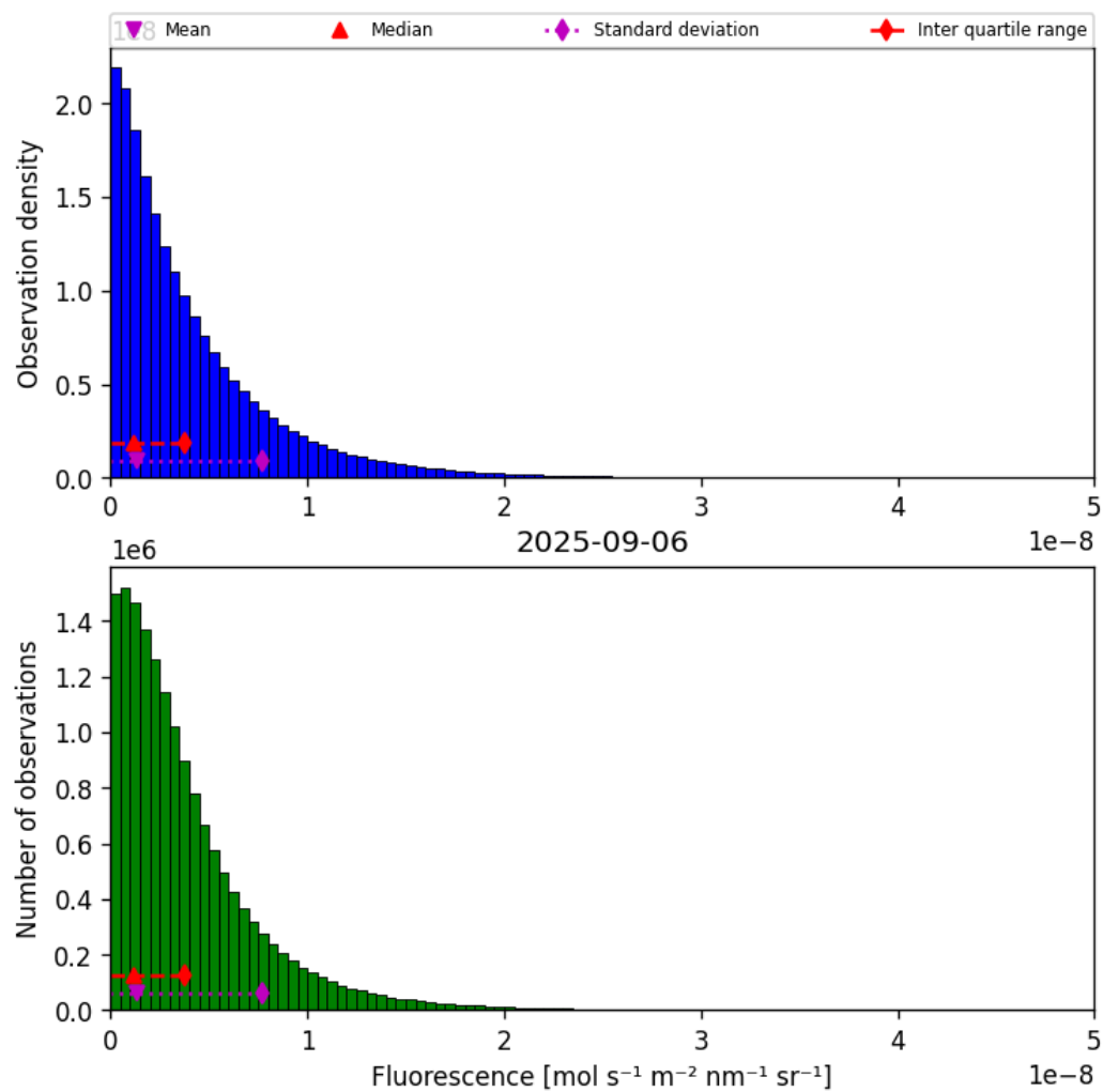
Figure 40: Histogram of “Fluorescence” for 2025-09-05 to 2025-09-07
