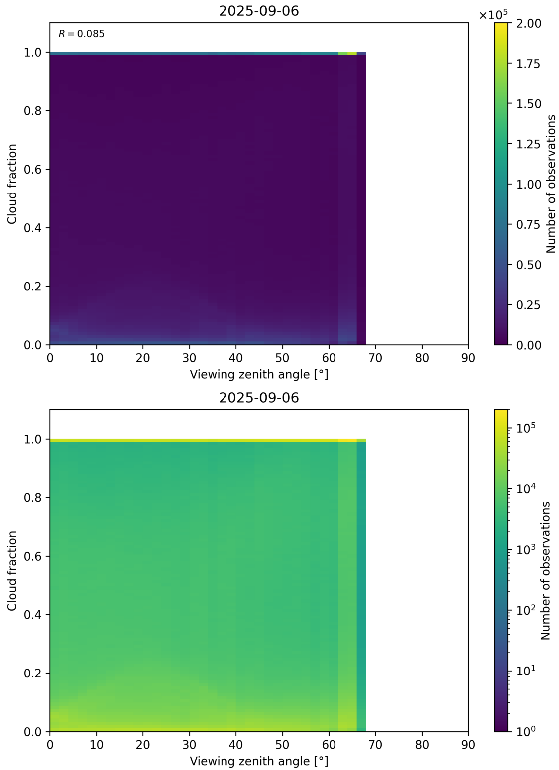
Figure 120: Scatter density plot of “Viewing zenith angle” against “Cloud fraction” for 2025-09-05 to 2025-09-07.
