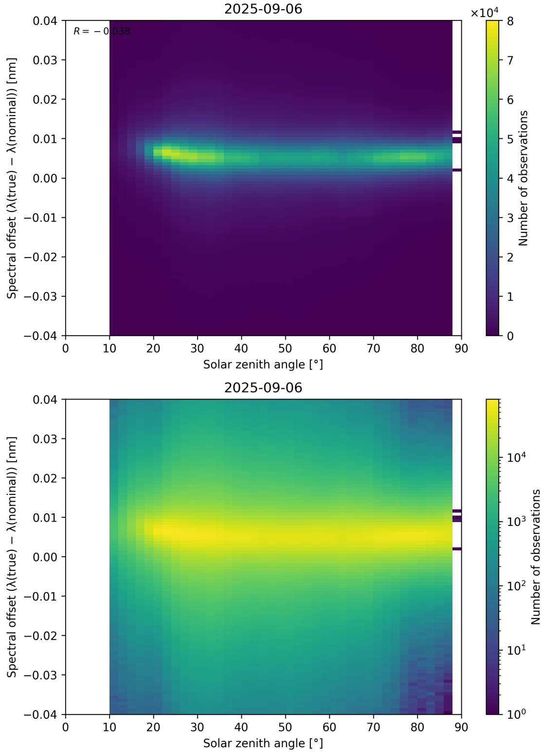
Figure 117: Scatter density plot of “Solar zenith angle” against “Spectral offset ( \lambda_{\text{true}} - \lambda_{\text{nominal}} )” for 2025-09-05 to 2025-09-07.
