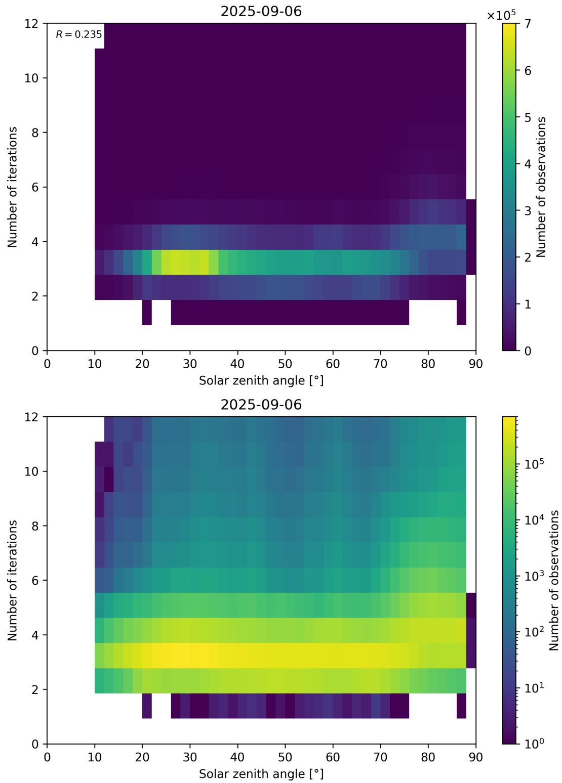
Figure 114: Scatter density plot of “Solar zenith angle” against “Number of iterations” for 2025-09-05 to 2025-09-07.
