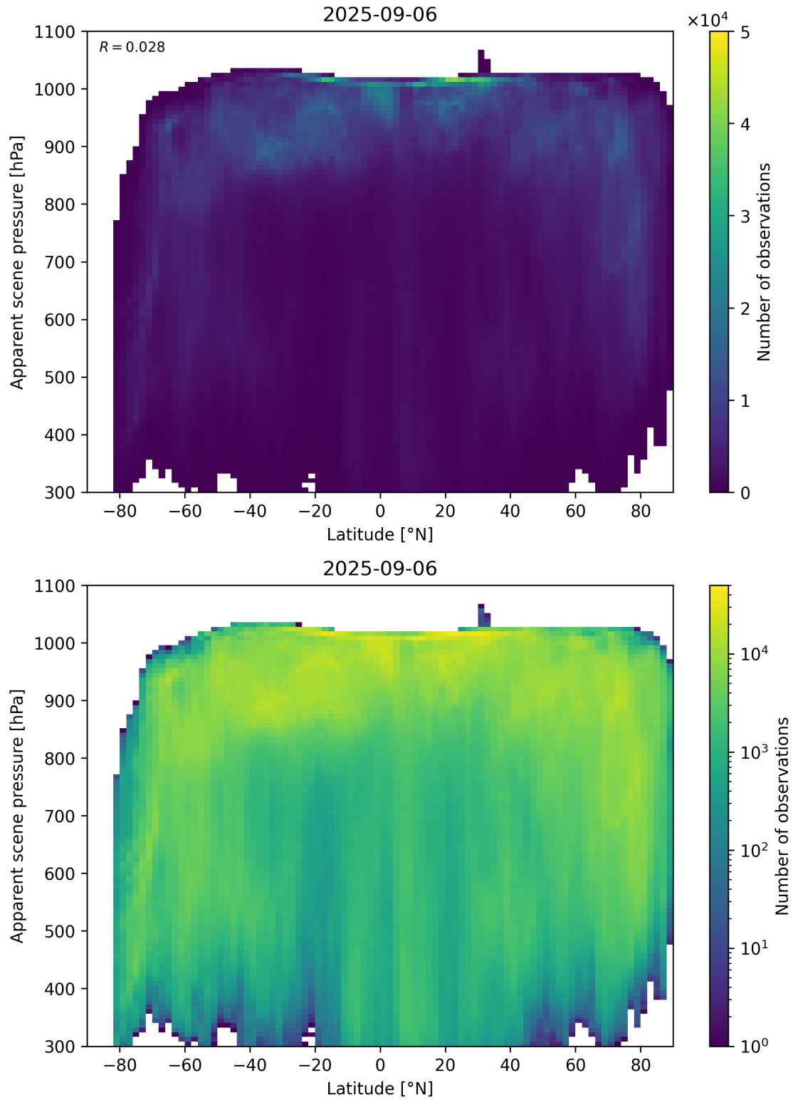
Figure 88: Scatter density plot of “Latitude” against “Apparent scene pressure” for 2025-09-05 to 2025-09-07.
