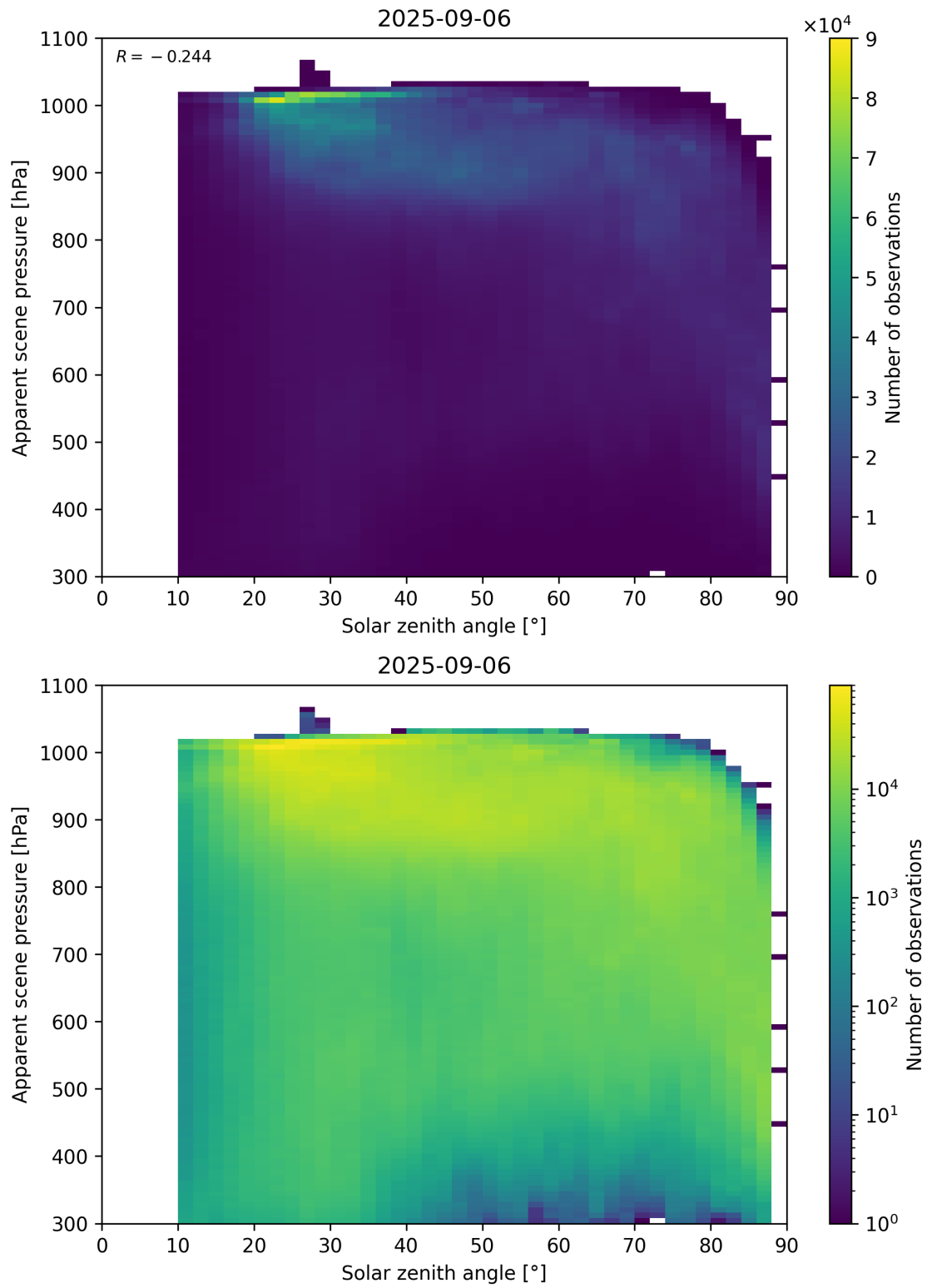
Figure 108: Scatter density plot of “Solar zenith angle” against “Apparent scene pressure” for 2025-09-05 to 2025-09-07.
