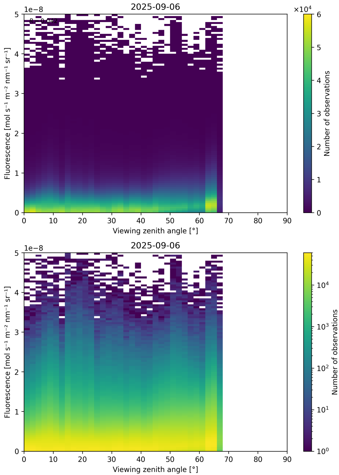
Figure 122: Scatter density plot of “Viewing zenith angle” against “Fluorescence” for 2025-09-05 to 2025-09-07.
