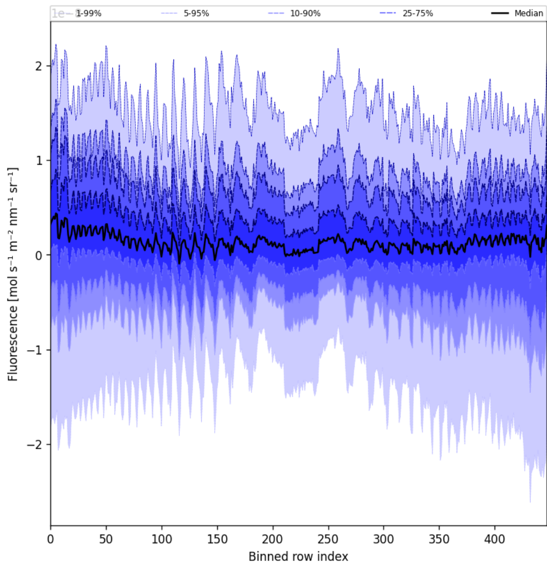
Figure 57: Along track statistics of “Fluorescence” for 2025-09-05 to 2025-09-07
