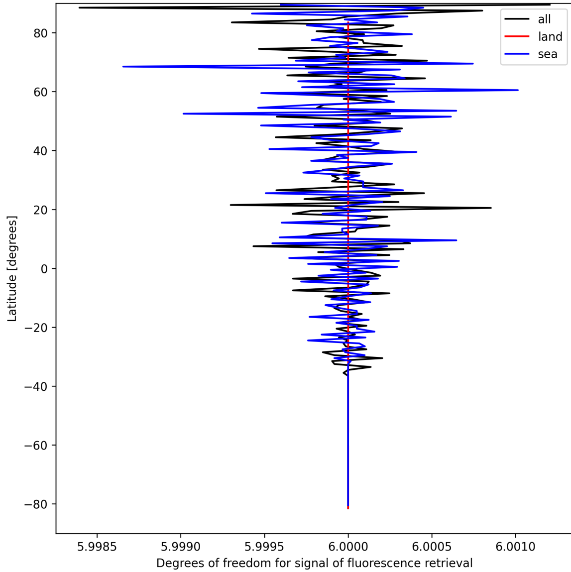
Figure 26: Zonal average of “Degrees of freedom for signal of fluorescence retrieval” for 2025-09-05 to 2025-09-07.
