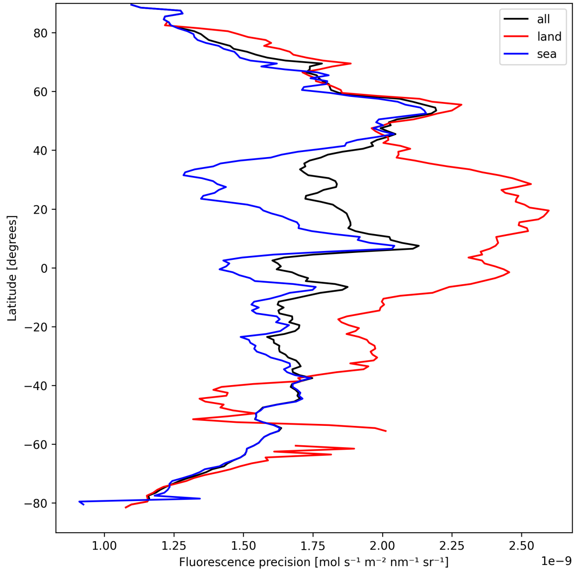
Figure 24: Zonal average of “Fluorescence precision” for 2025-09-05 to 2025-09-07.
