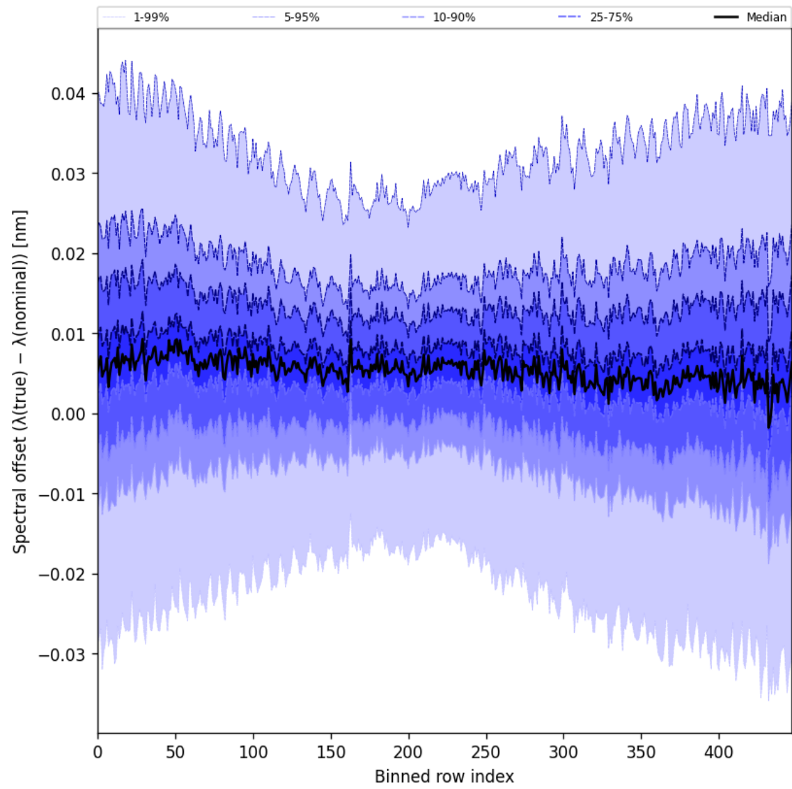
Figure 62: Along track statistics of “Spectral offset ( \lambda_{\text{true}} - \lambda_{\text{nominal}} )” for 2025-09-05 to 2025-09-07
