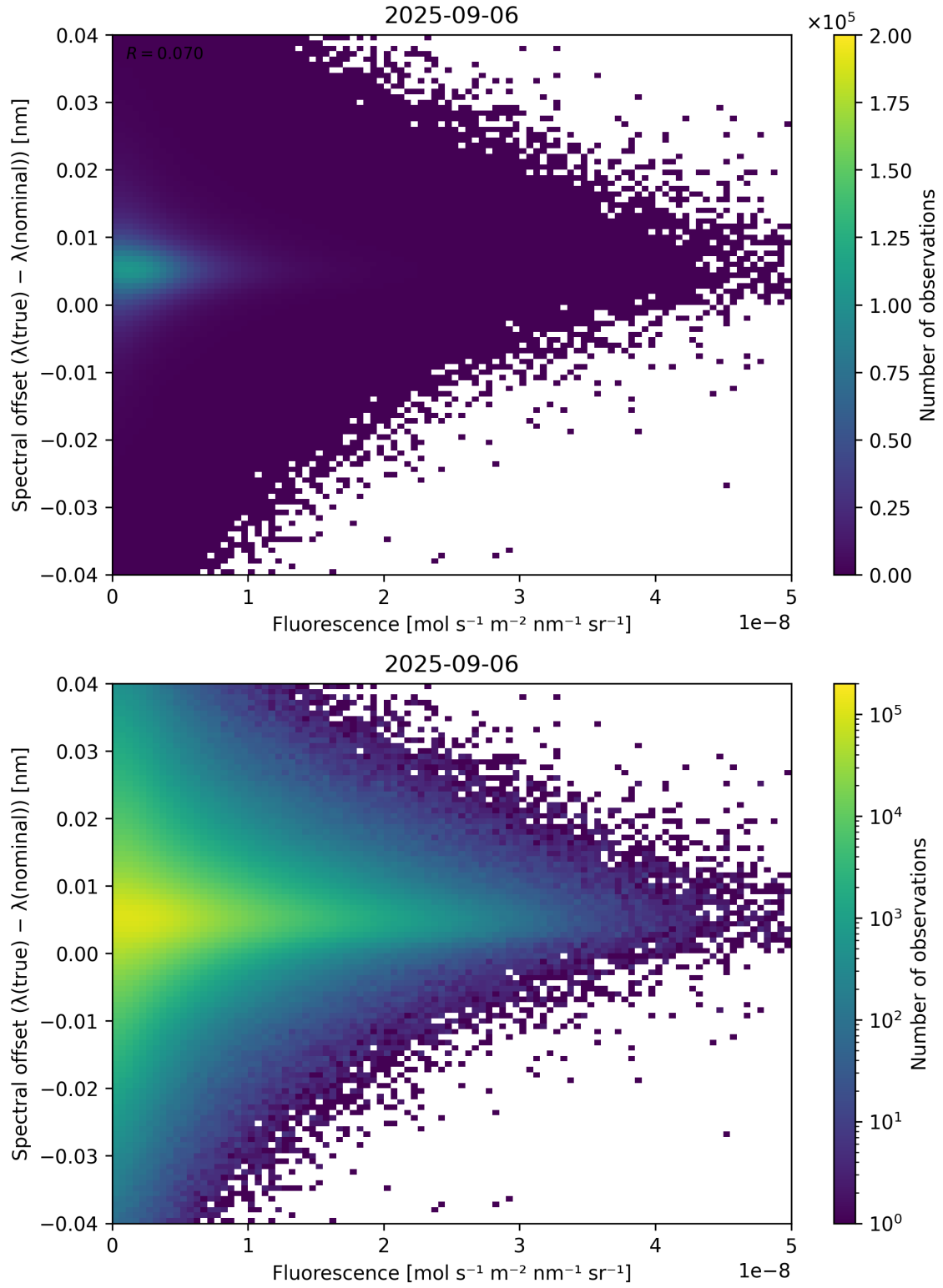
Figure 87: Scatter density plot of “Fluorescence” against “Spectral offset ( \lambda_{\text{true}} - \lambda_{\text{nominal}} )” for 2025-09-05 to 2025-09-07.
