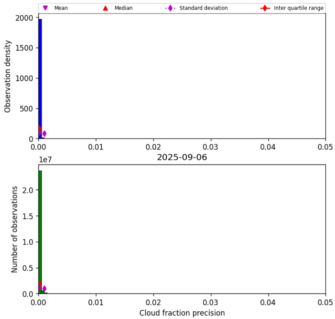
Figure 33: Histogram of “Cloud fraction precision” for 2025-09-05 to 2025-09-07
