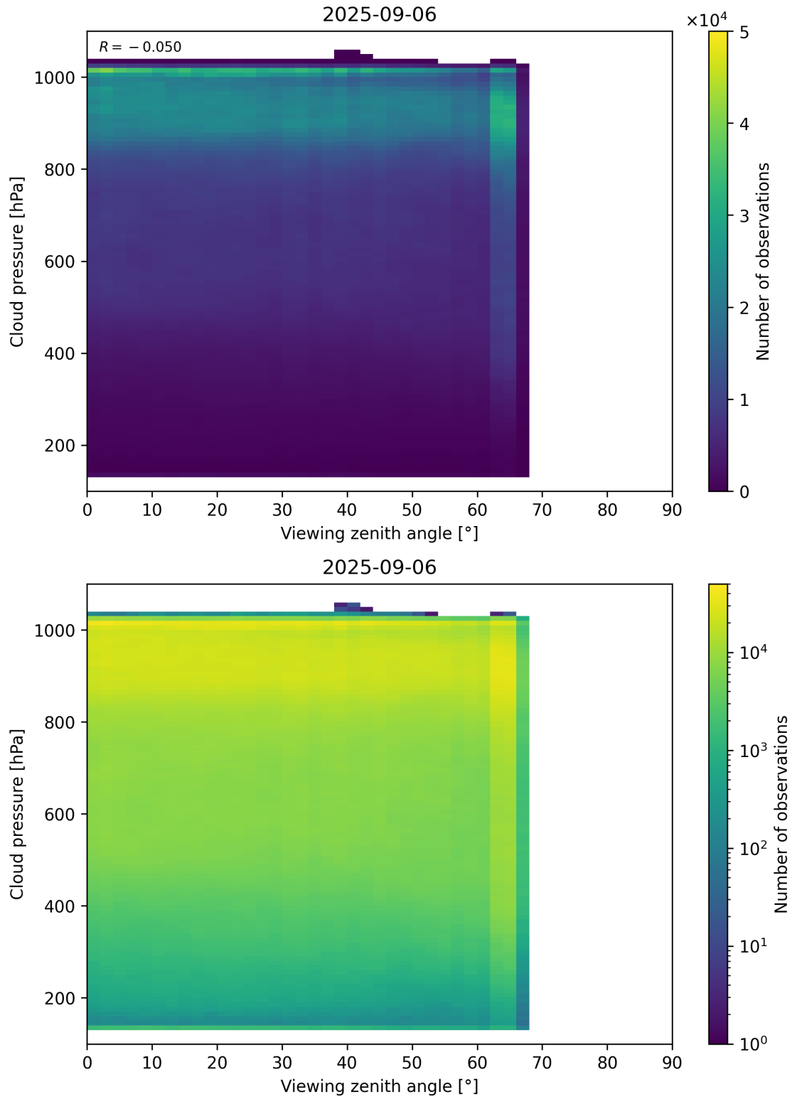
Figure 121: Scatter density plot of “Viewing zenith angle” against “Cloud pressure” for 2025-09-05 to 2025-09-07.
