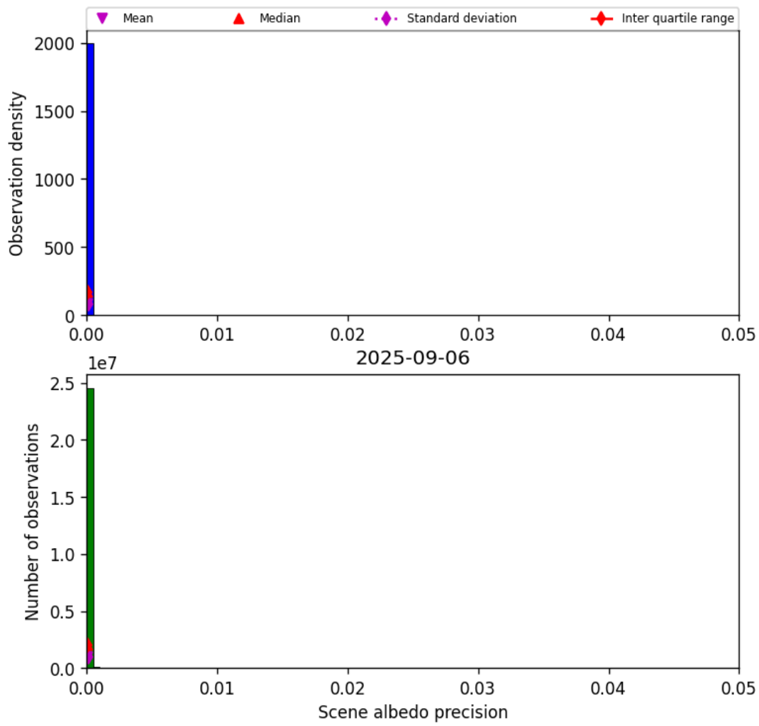
Figure 35: Histogram of “Scene albedo precision” for 2025-09-05 to 2025-09-07
