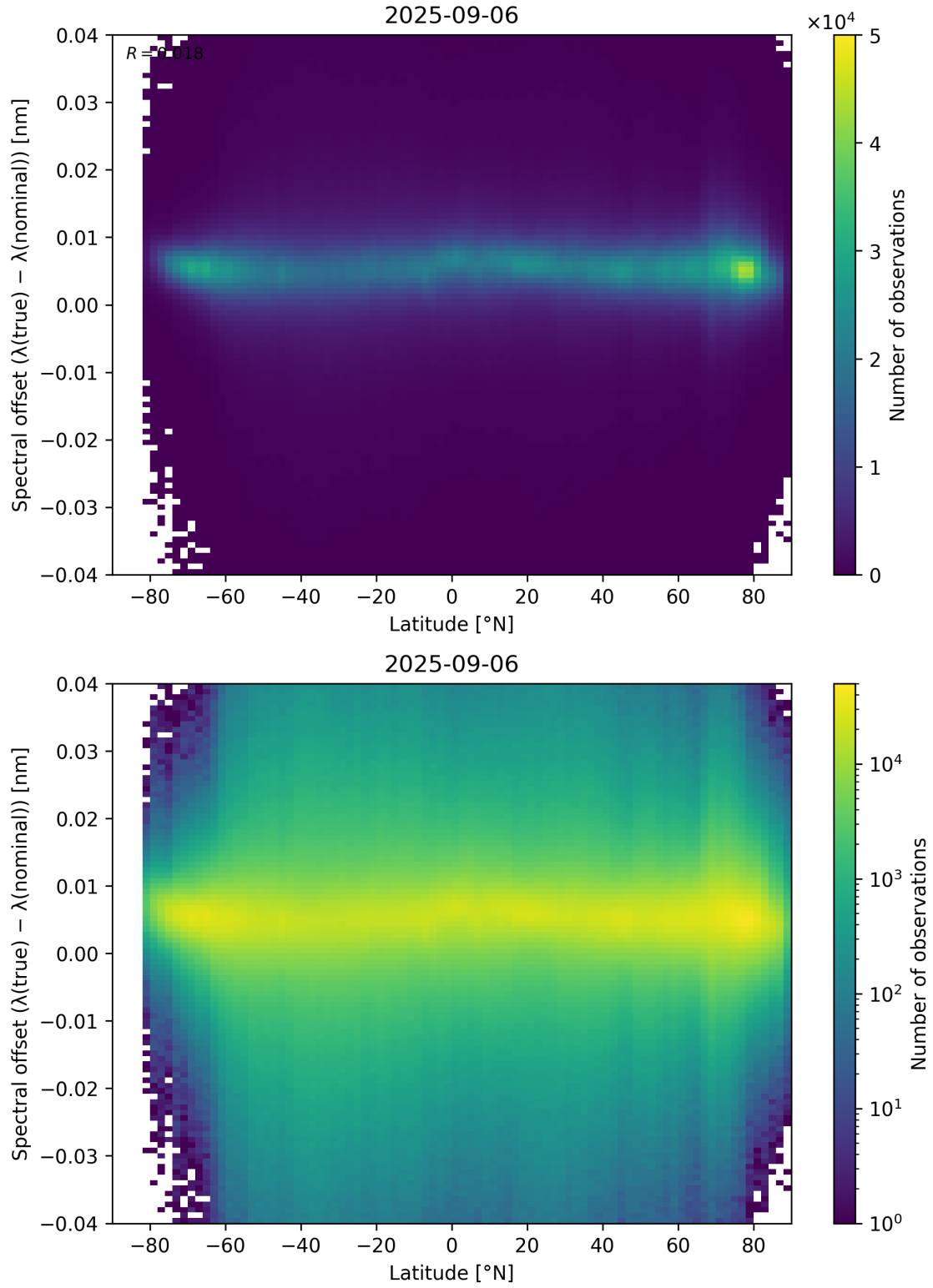
Figure 96: Scatter density plot of “Latitude” against “Spectral offset ( \lambda_{\text{true}} - \lambda_{\text{nominal}} )” for 2025-09-05 to 2025-09-07.
