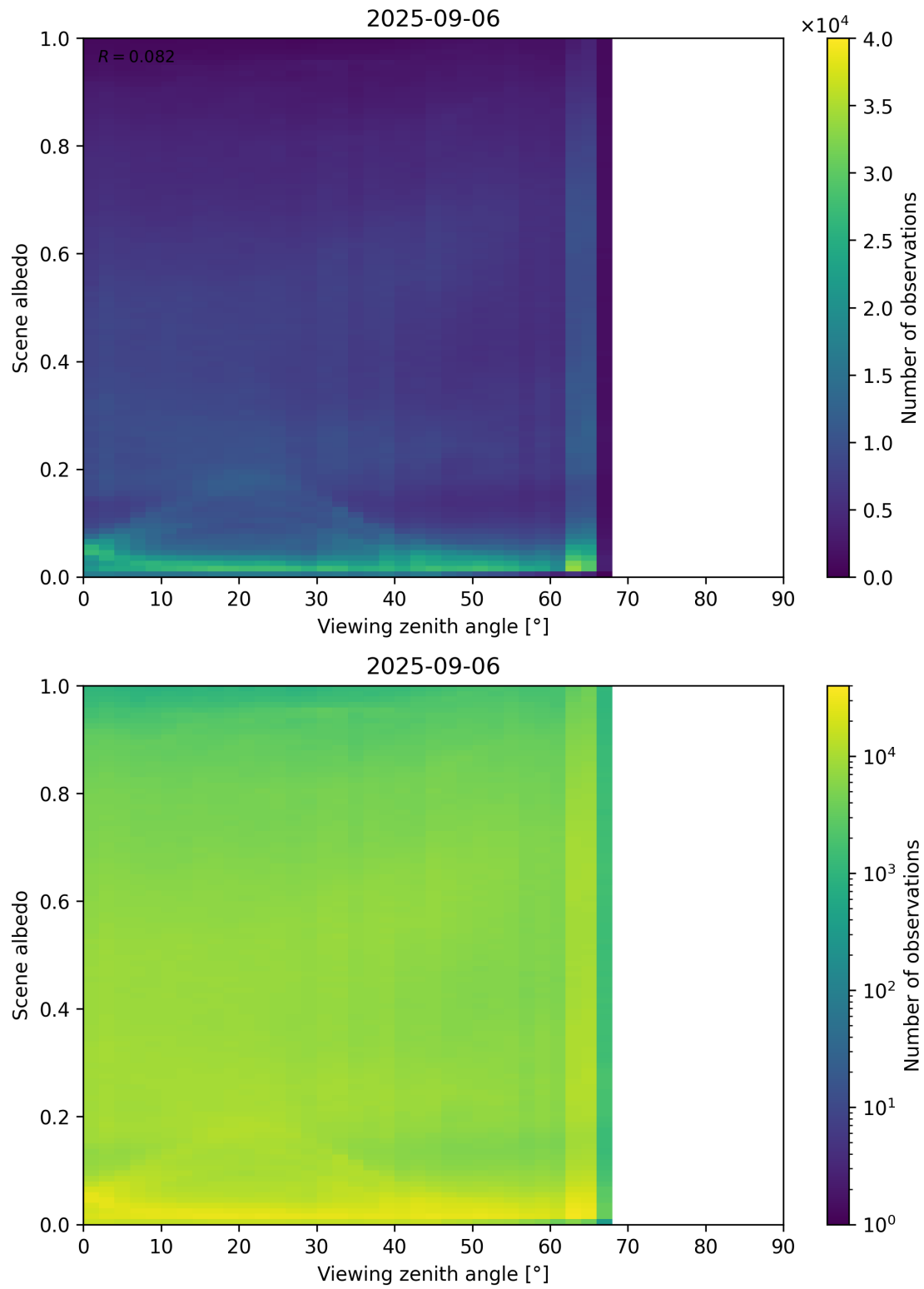
Figure 126: Scatter density plot of “Viewing zenith angle” against “Scene albedo” for 2025-09-05 to 2025-09-07.
