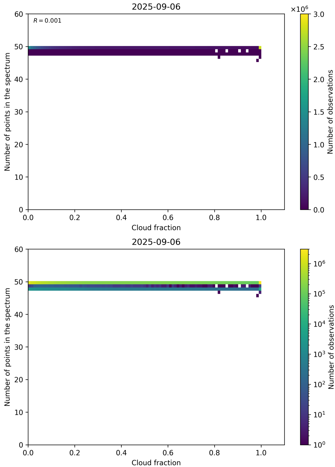
Figure 74: Scatter density plot of “Cloud fraction” against “Number of points in the spectrum” for 2025-09-05 to 2025-09-07.
