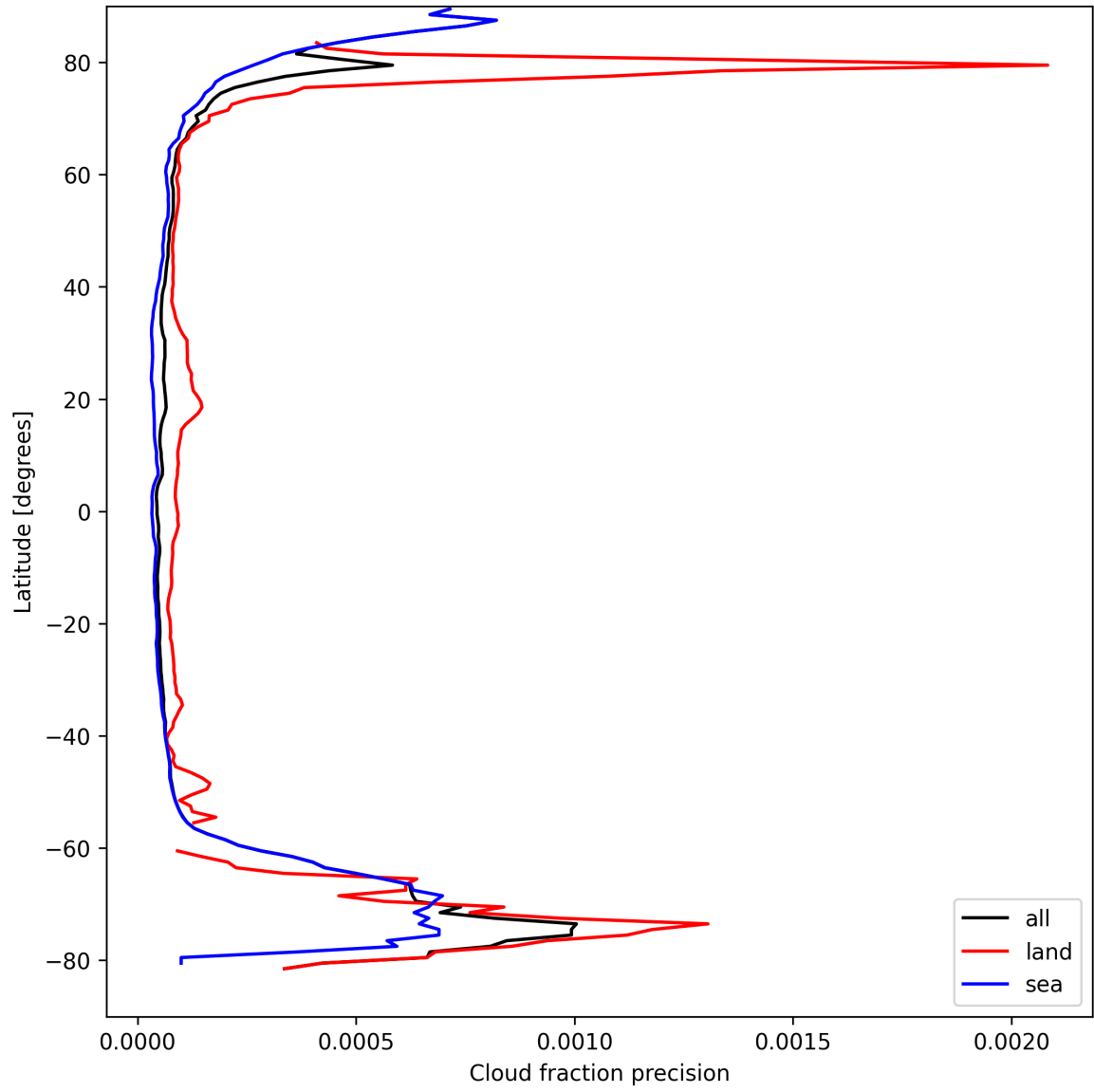
Figure 16: Zonal average of “Cloud fraction precision” for 2025-09-05 to 2025-09-07.
