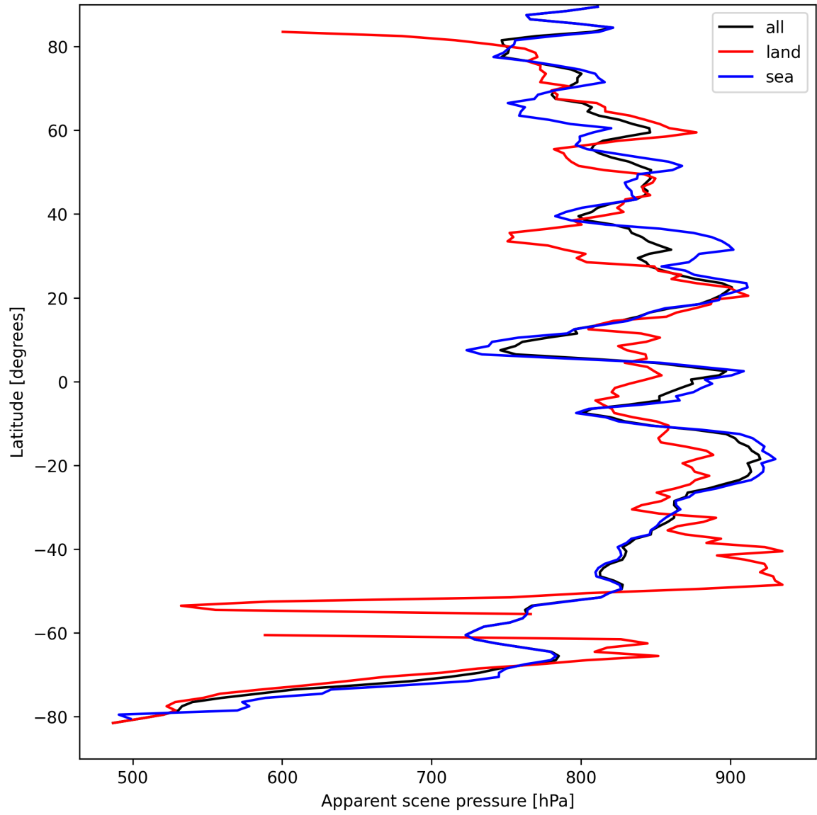
Figure 19: Zonal average of “Apparent scene pressure” for 2025-09-05 to 2025-09-07.
