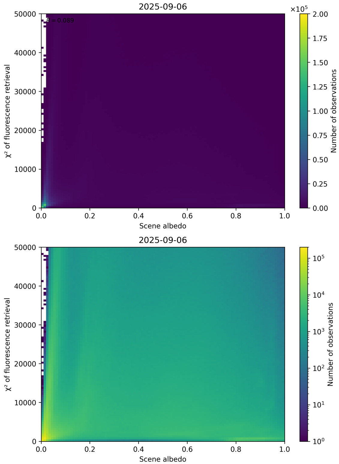
Figure 103: Scatter density plot of “Scene albedo” against “ \chi^2 of fluorescence retrieval” for 2025-09-05 to 2025-09-07.
