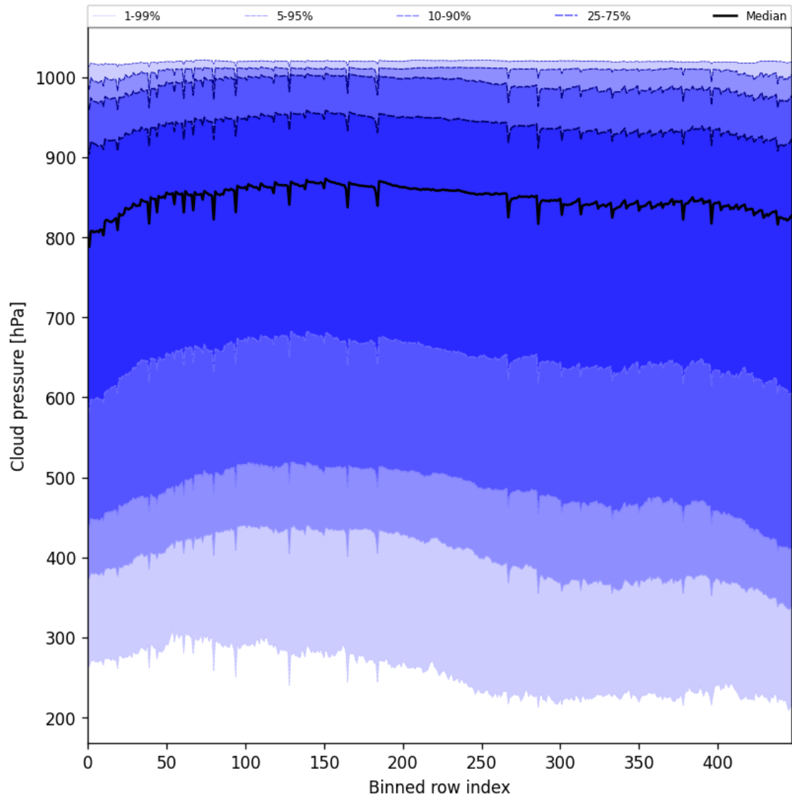
Figure 47: Along track statistics of “Cloud pressure” for 2025-09-05 to 2025-09-07
