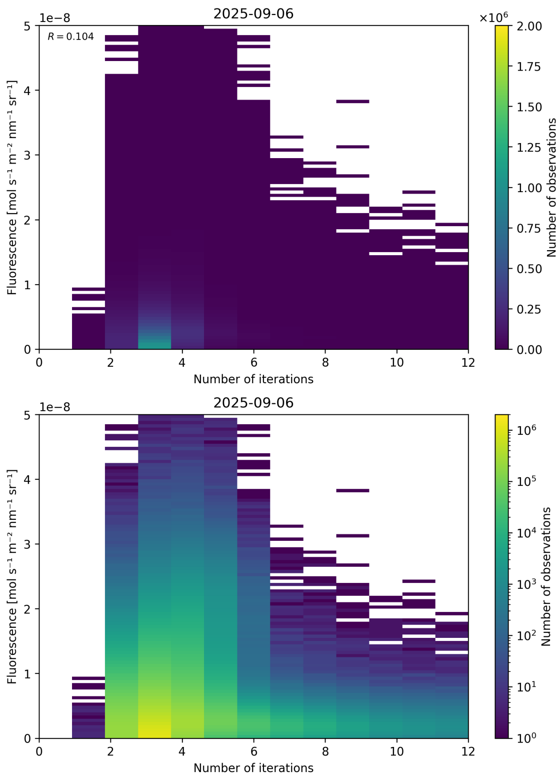
Figure 98: Scatter density plot of “Number of iterations” against “Fluorescence” for 2025-09-05 to 2025-09-07.
