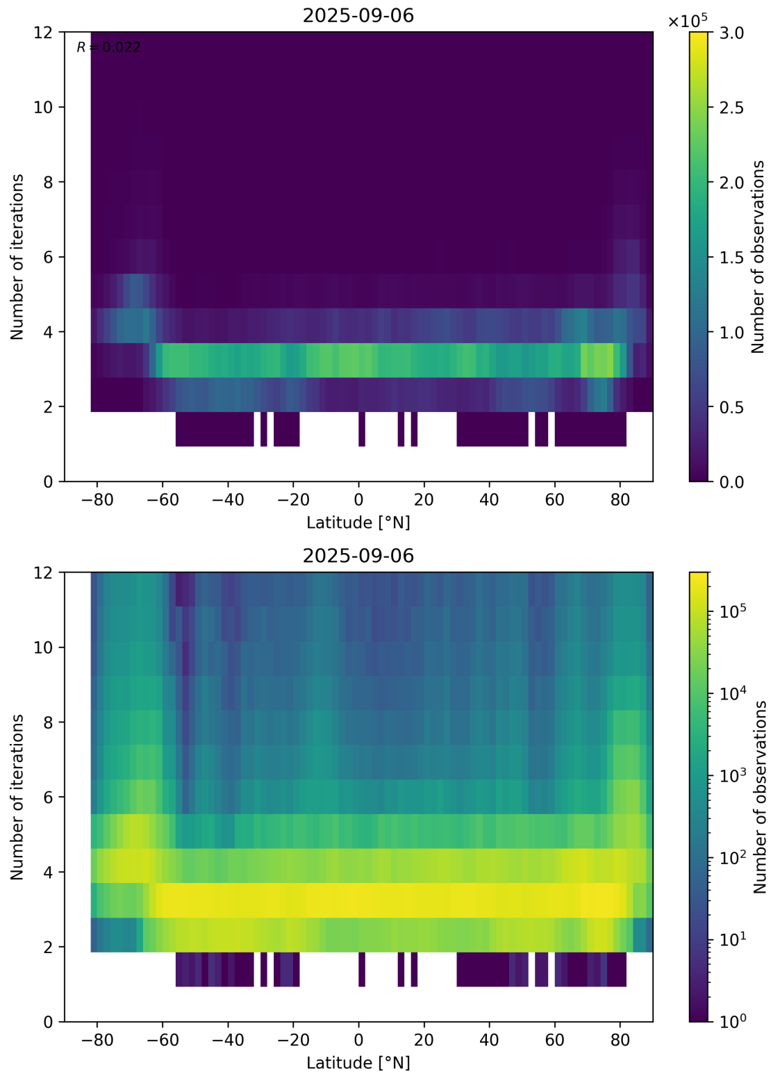
Figure 93: Scatter density plot of “Latitude” against “Number of iterations” for 2025-09-05 to 2025-09-07.
