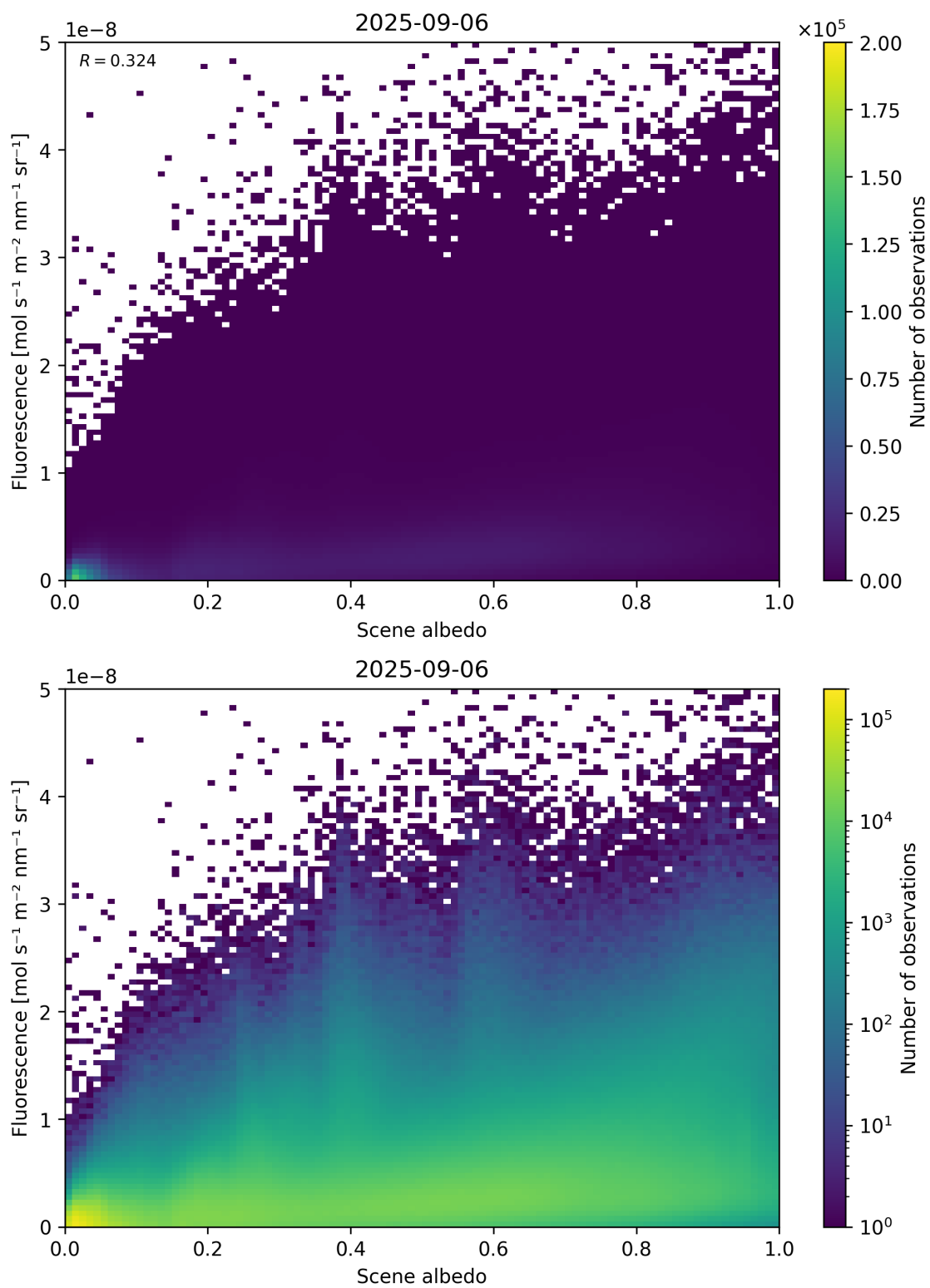
Figure 104: Scatter density plot of “Scene albedo” against “Fluorescence” for 2025-09-05 to 2025-09-07.
