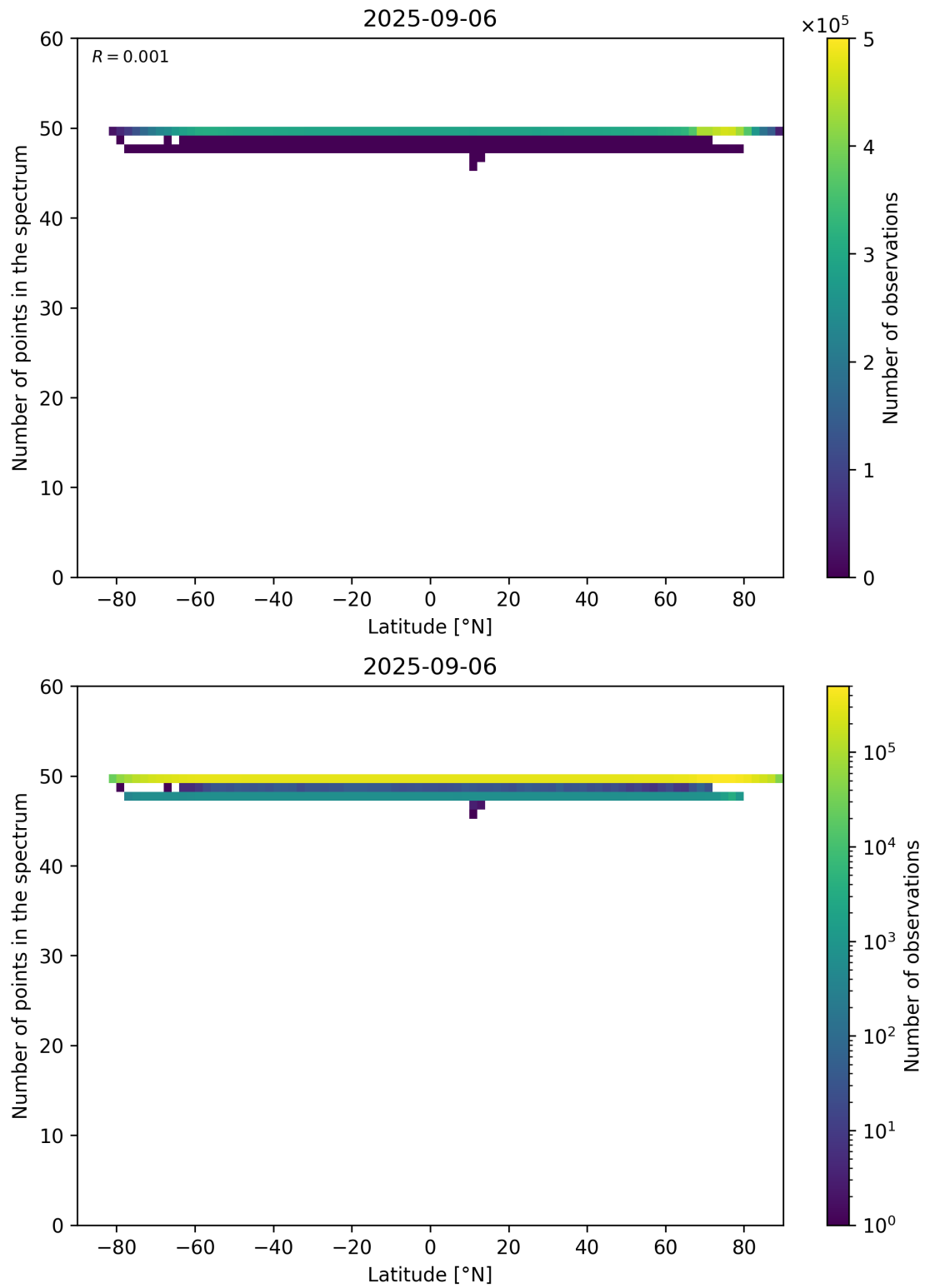
Figure 94: Scatter density plot of “Latitude” against “Number of points in the spectrum” for 2025-09-05 to 2025-09-07.
