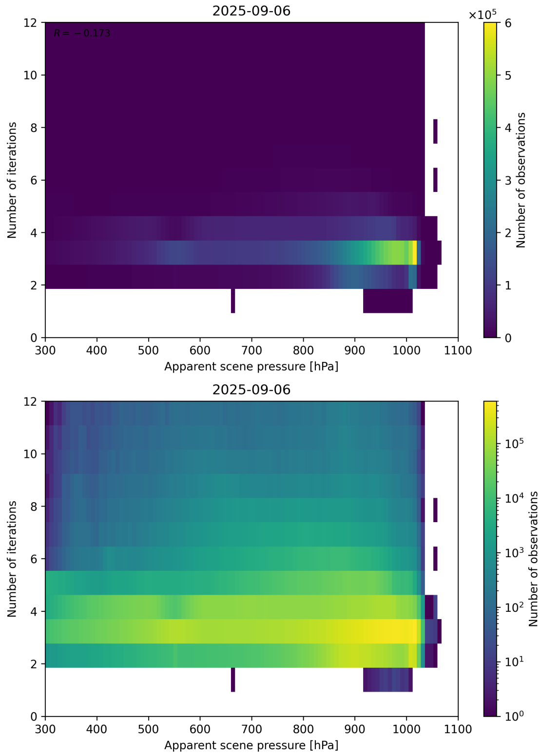
Figure 65: Scatter density plot of “Apparent scene pressure” against “Number of iterations” for 2025-09-05 to 2025-09-07.
