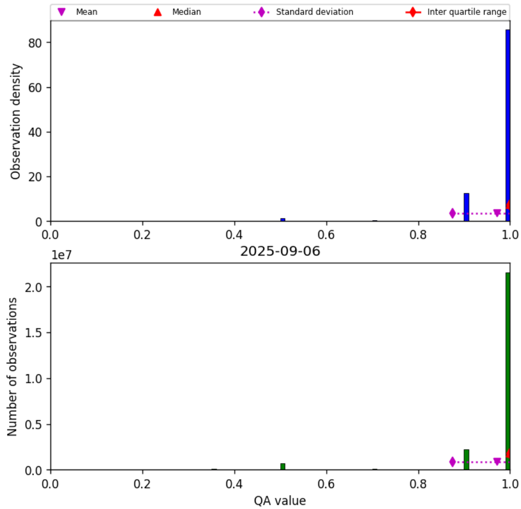
Figure 29: Histogram of “QA value” for 2025-09-05 to 2025-09-07
