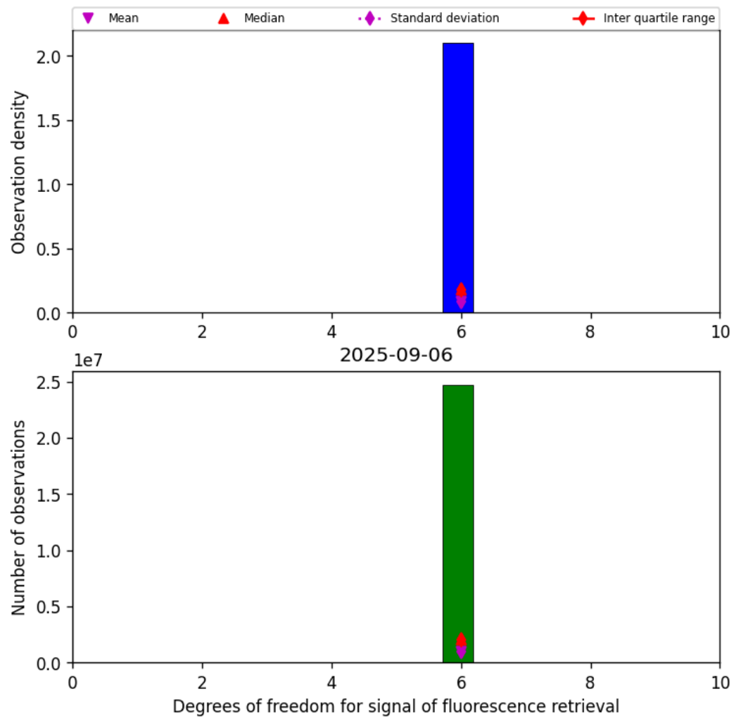
Figure 43: Histogram of “Degrees of freedom for signal of fluorescence retrieval” for 2025-09-05 to 2025-09-07
