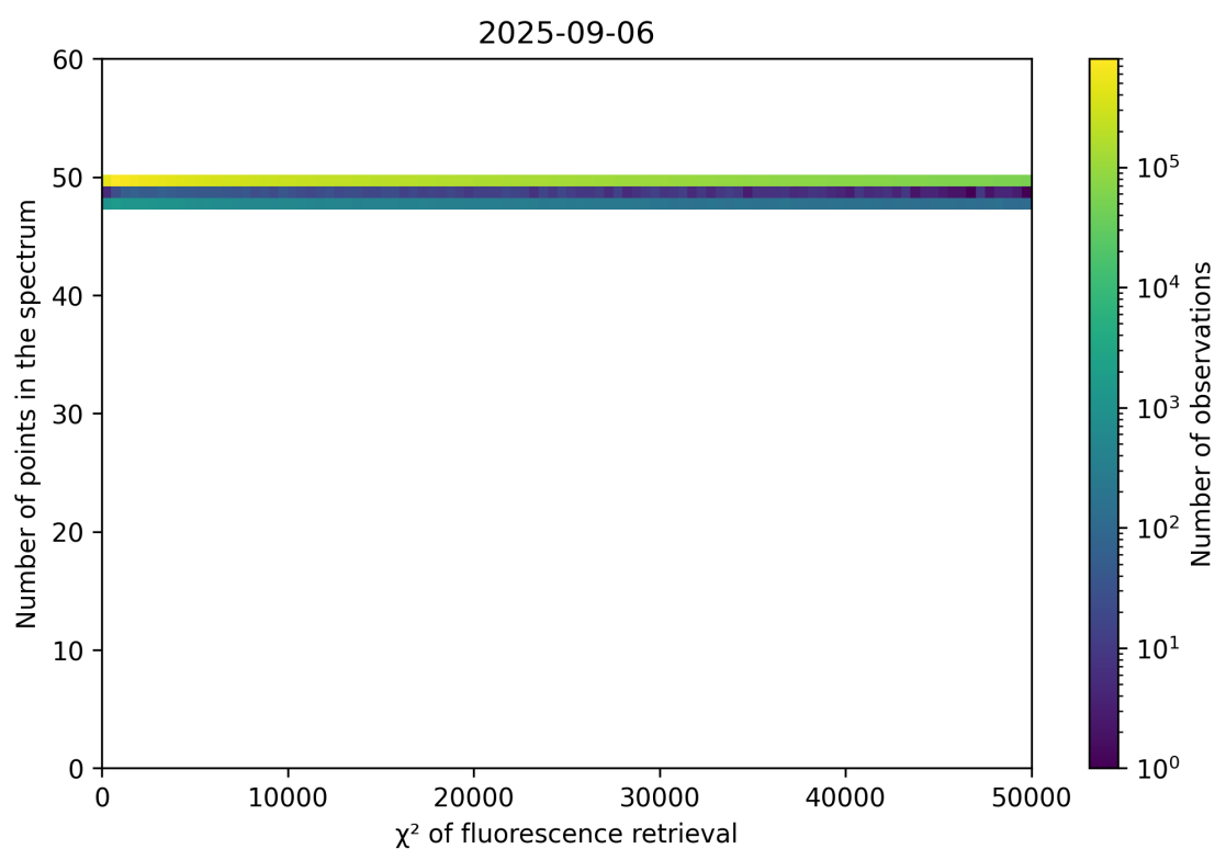
Figure 68: Scatter density plot of “ \chi^2 of fluorescence retrieval” against “Number of points in the spectrum” for 2025-09-05 to 2025-09-07.
