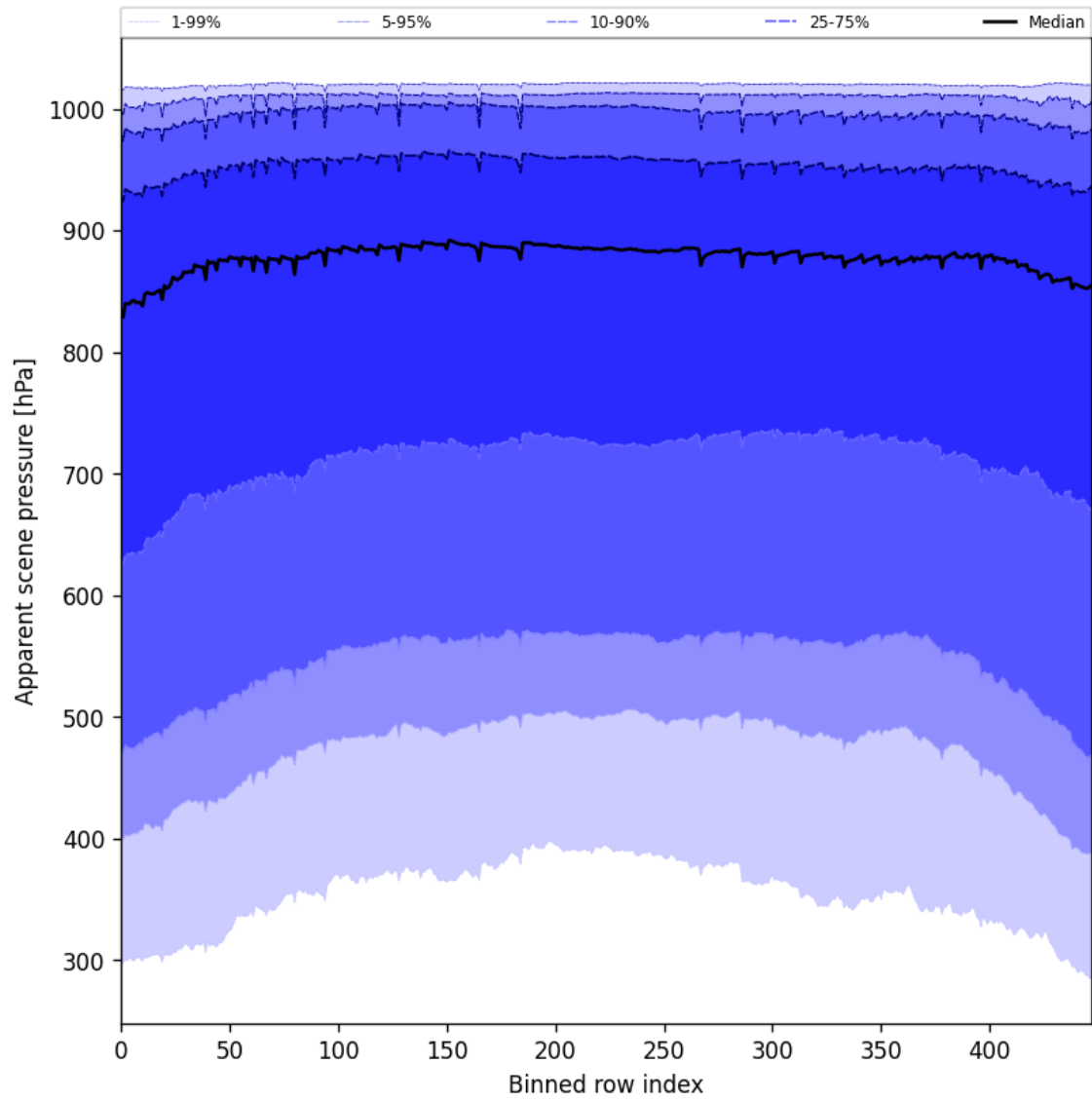
Figure 53: Along track statistics of “Apparent scene pressure” for 2025-09-05 to 2025-09-07
