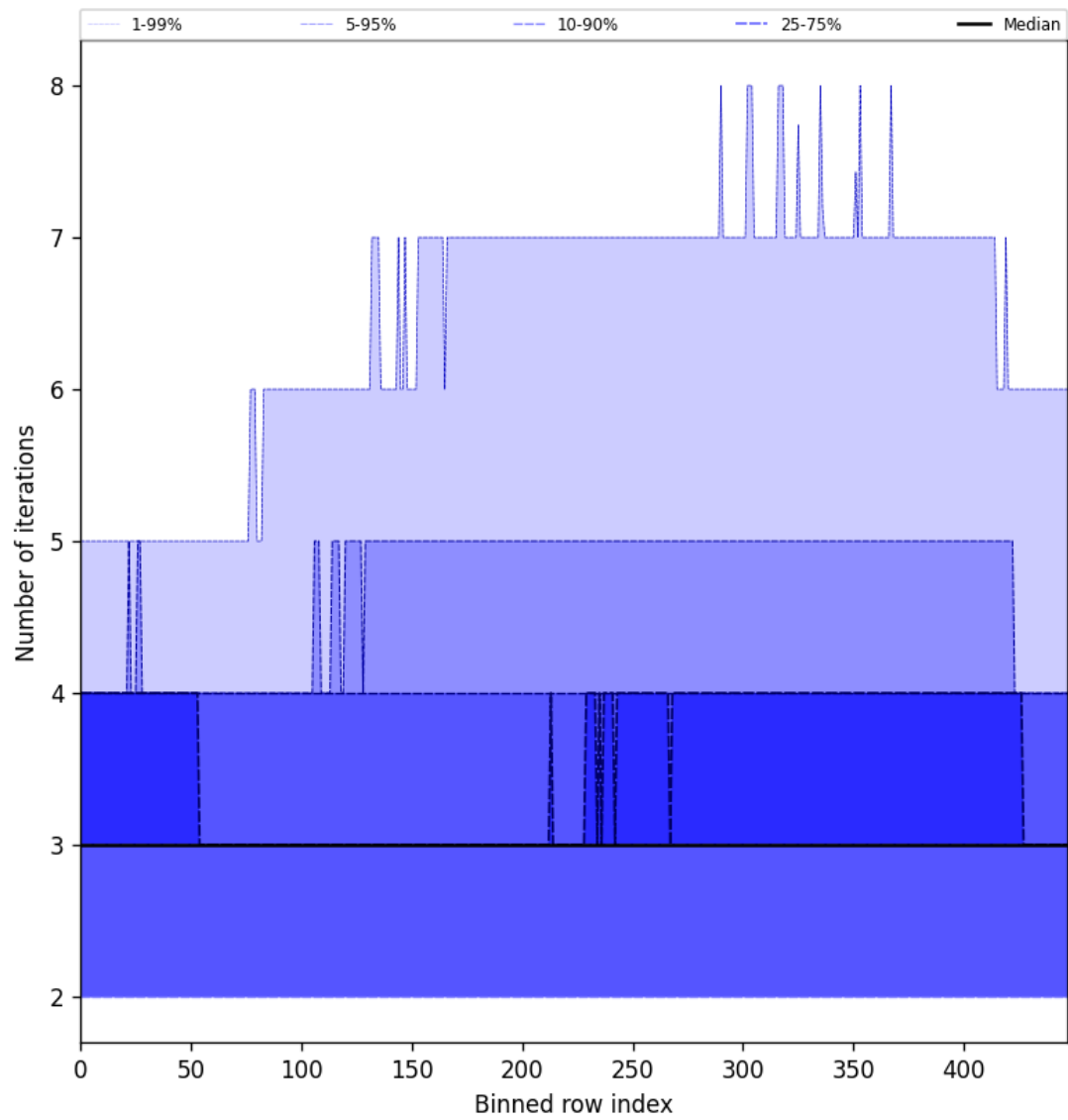
Figure 56: Along track statistics of “Number of iterations” for 2025-09-05 to 2025-09-07
