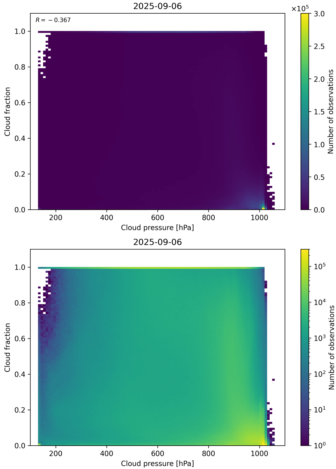
Figure 79: Scatter density plot of “Cloud pressure” against “Cloud fraction” for 2025-09-05 to 2025-09-07.
