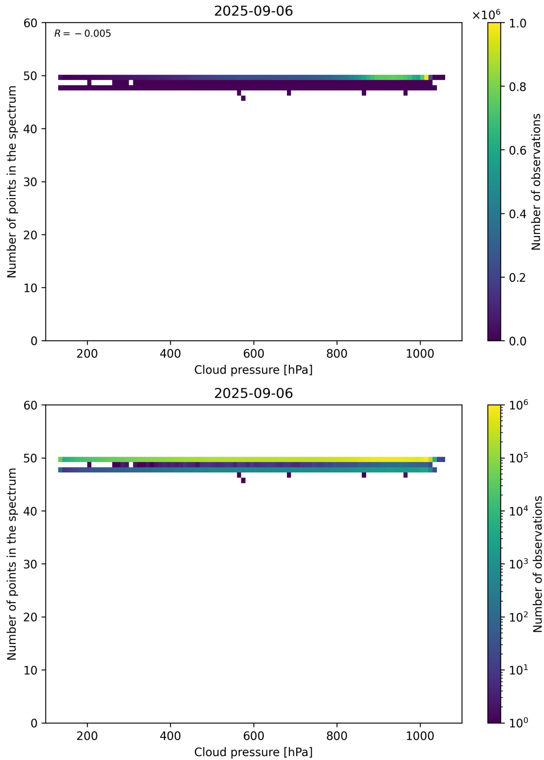
Figure 82: Scatter density plot of “Cloud pressure” against “Number of points in the spectrum” for 2025-09-05 to 2025-09-07.
