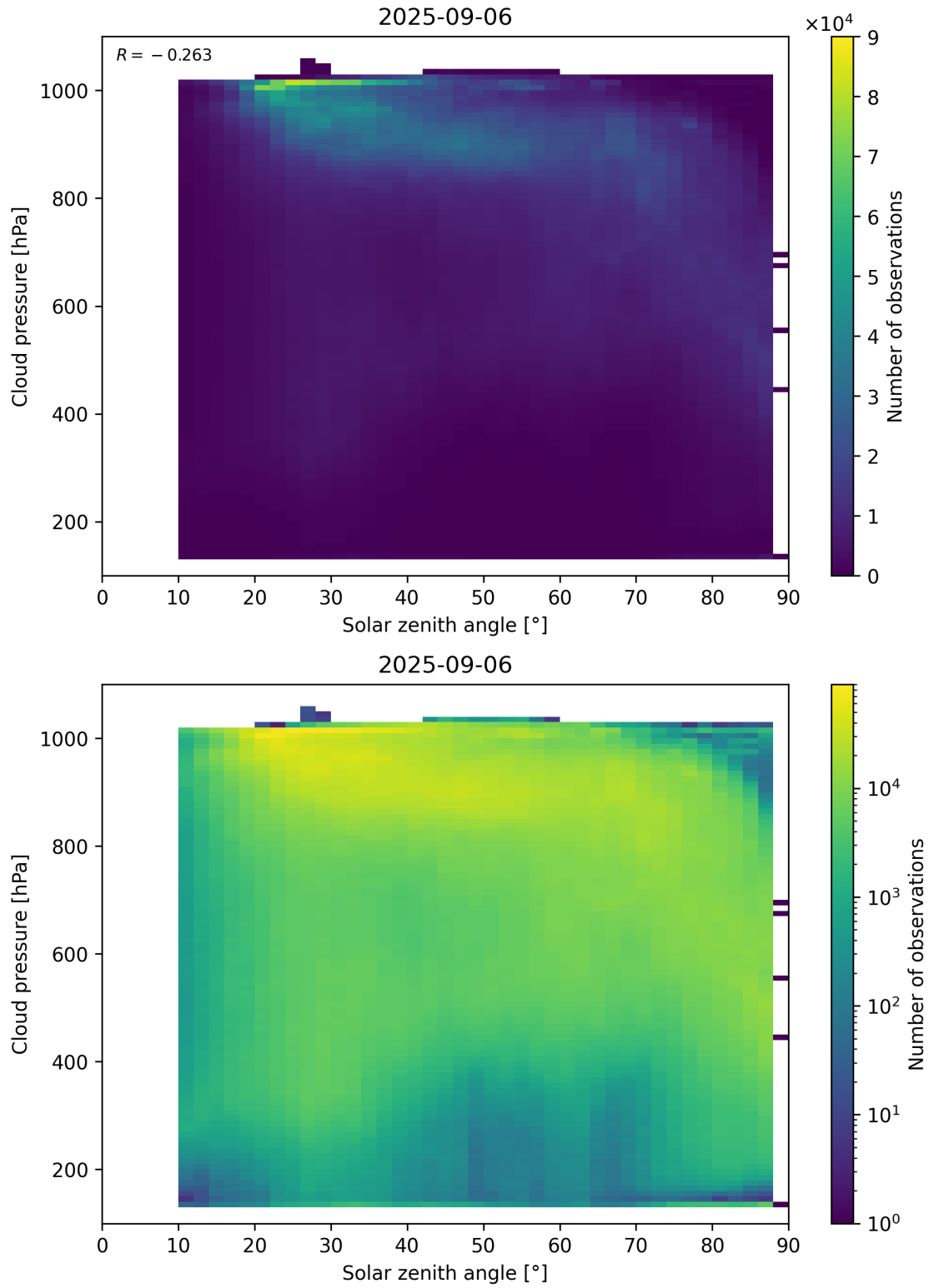
Figure 111: Scatter density plot of “Solar zenith angle” against “Cloud pressure” for 2025-09-05 to 2025-09-07.
