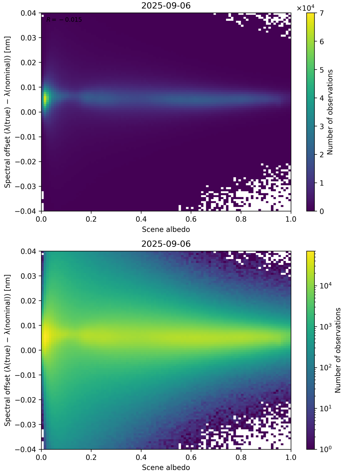
Figure 107: Scatter density plot of “Scene albedo” against “Spectral offset ( \lambda_{\text{true}} - \lambda_{\text{nominal}} )” for 2025-09-05 to 2025-09-07.
