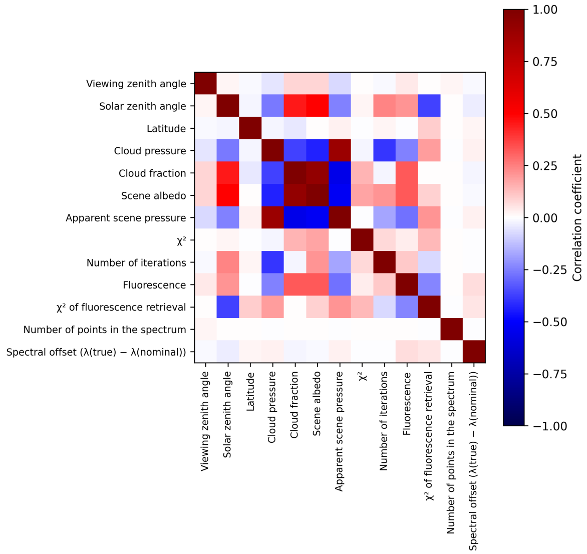
Figure 2: Map of correlation matrix for 2025-09-05 to 2025-09-07.
