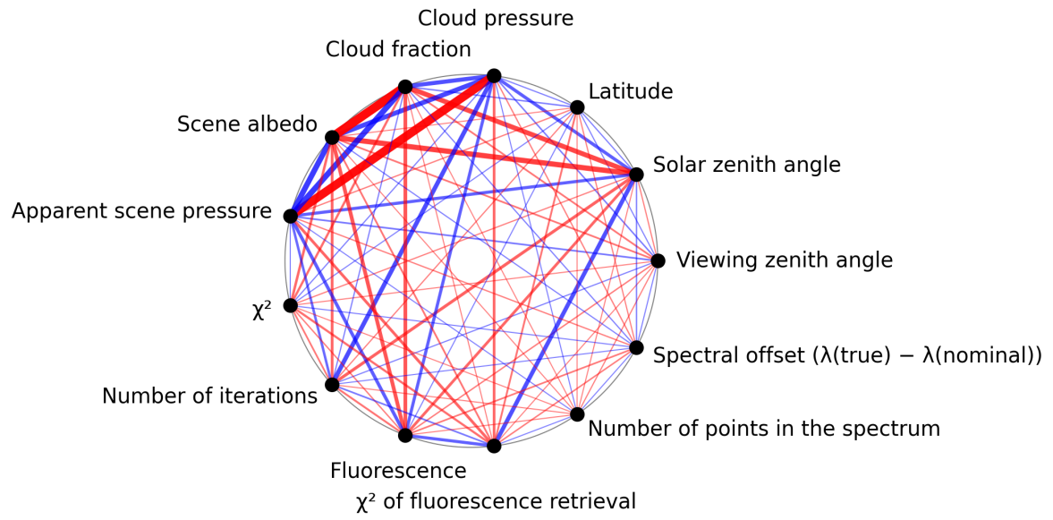
Figure 1: Map of correlation graph for 2025-09-05 to 2025-09-07.
