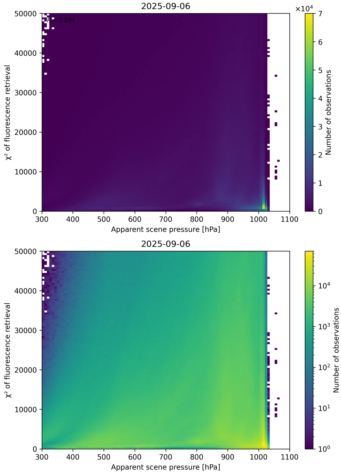
Figure 63: Scatter density plot of “Apparent scene pressure” against “ \chi^2 of fluorescence retrieval” for 2025-09-05 to 2025-09-07.
