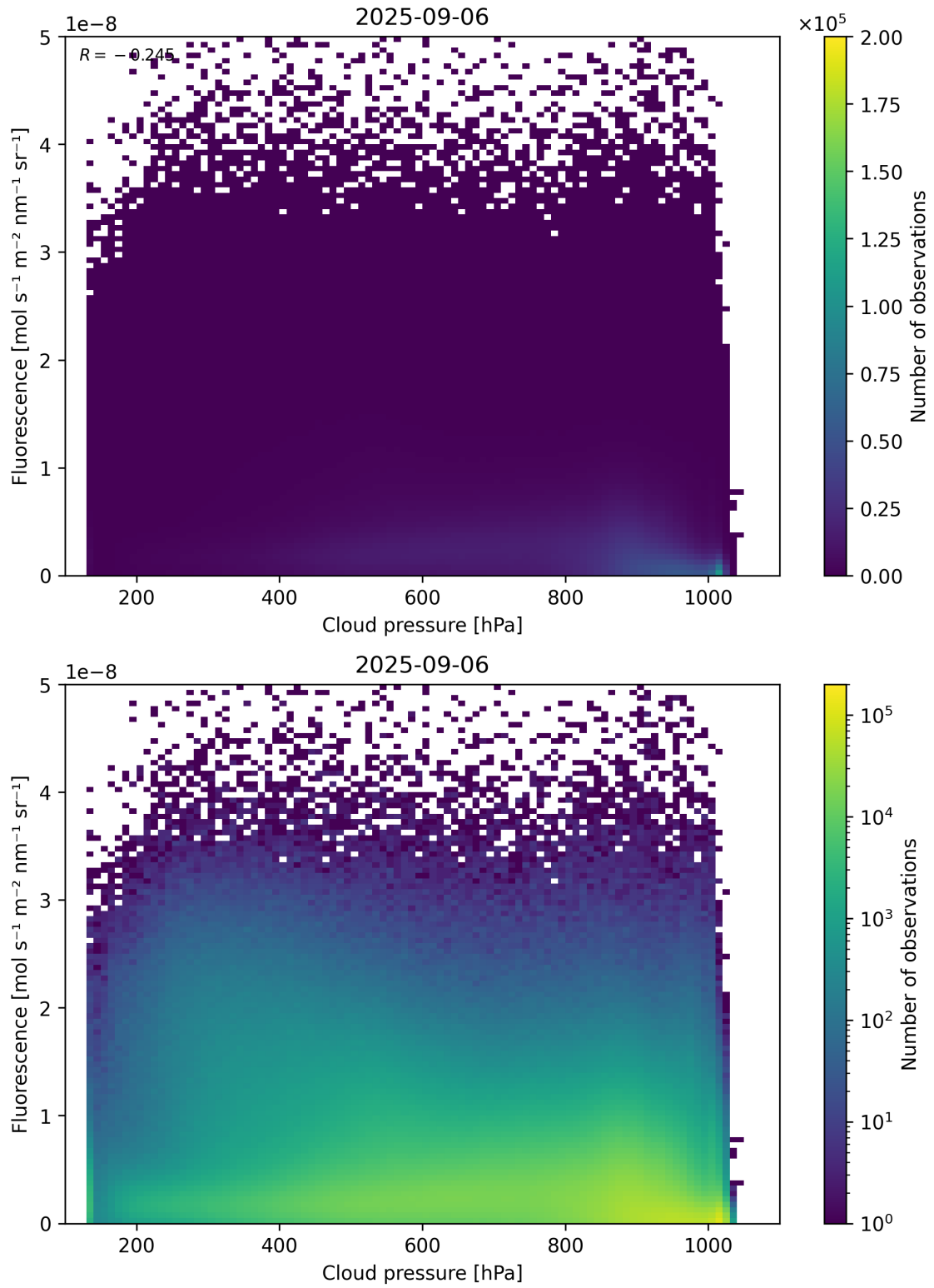
Figure 80: Scatter density plot of “Cloud pressure” against “Fluorescence” for 2025-09-05 to 2025-09-07.
