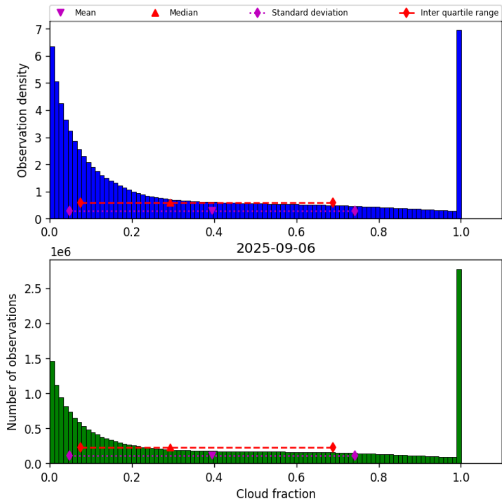
Figure 32: Histogram of “Cloud fraction” for 2025-09-05 to 2025-09-07
