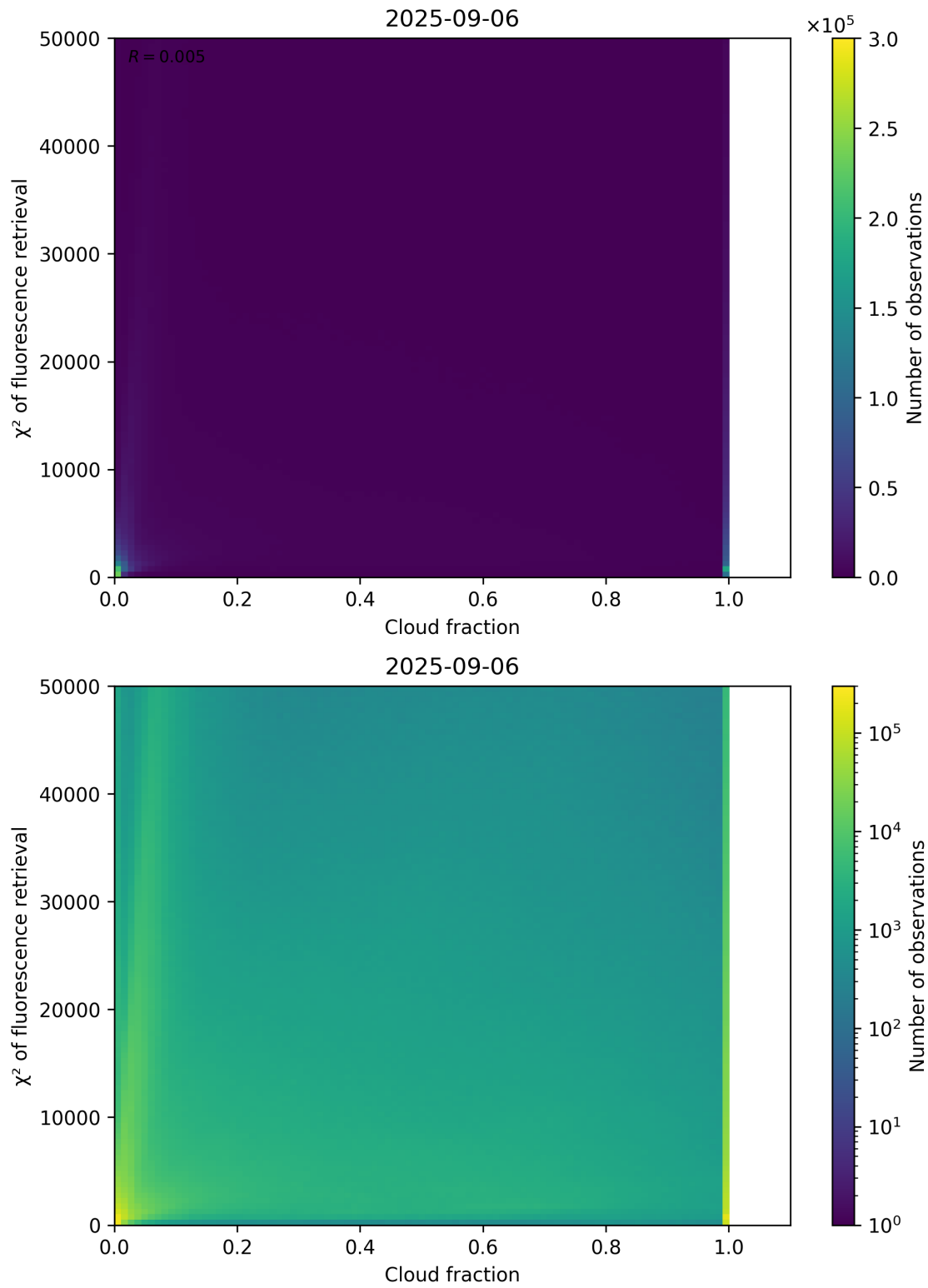
Figure 71: Scatter density plot of “Cloud fraction” against “ \chi^2 of fluorescence retrieval” for 2025-09-05 to 2025-09-07.
