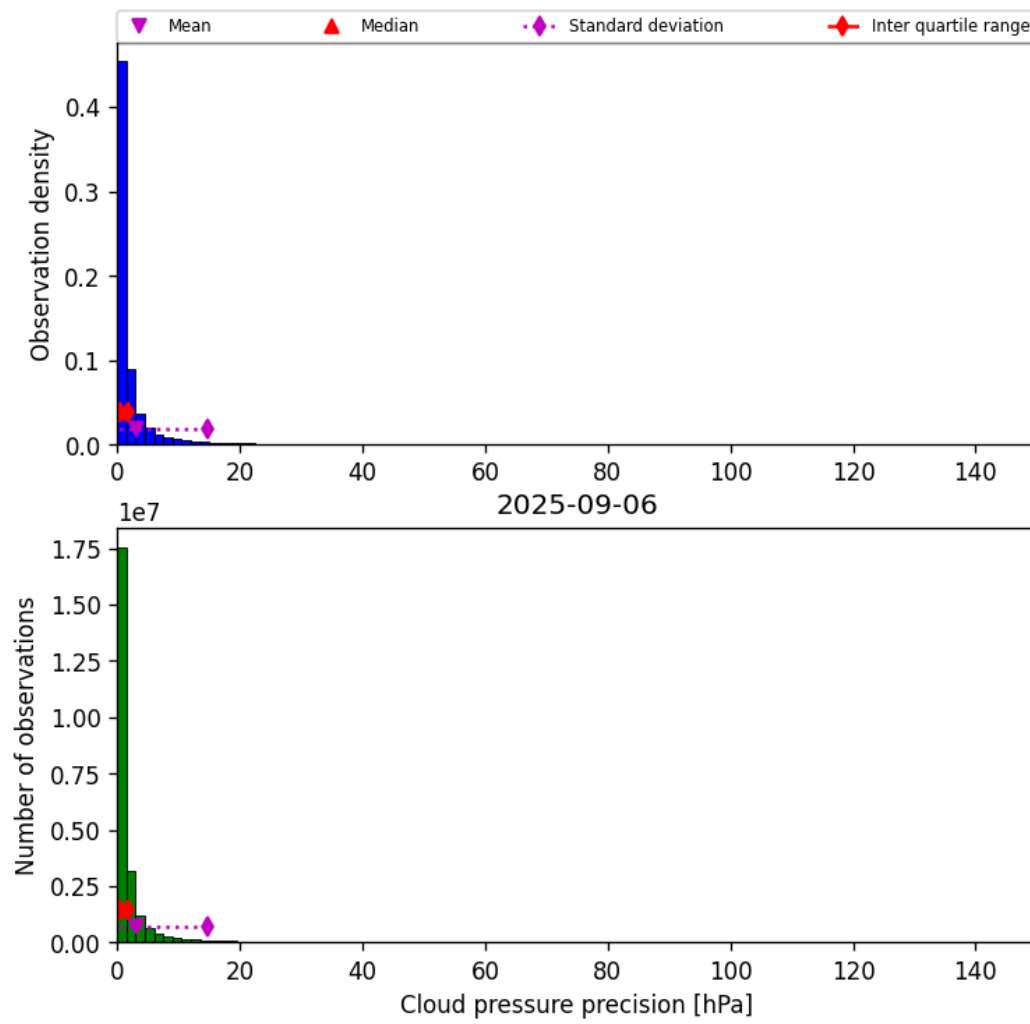
Figure 31: Histogram of “Cloud pressure precision” for 2025-09-05 to 2025-09-07
