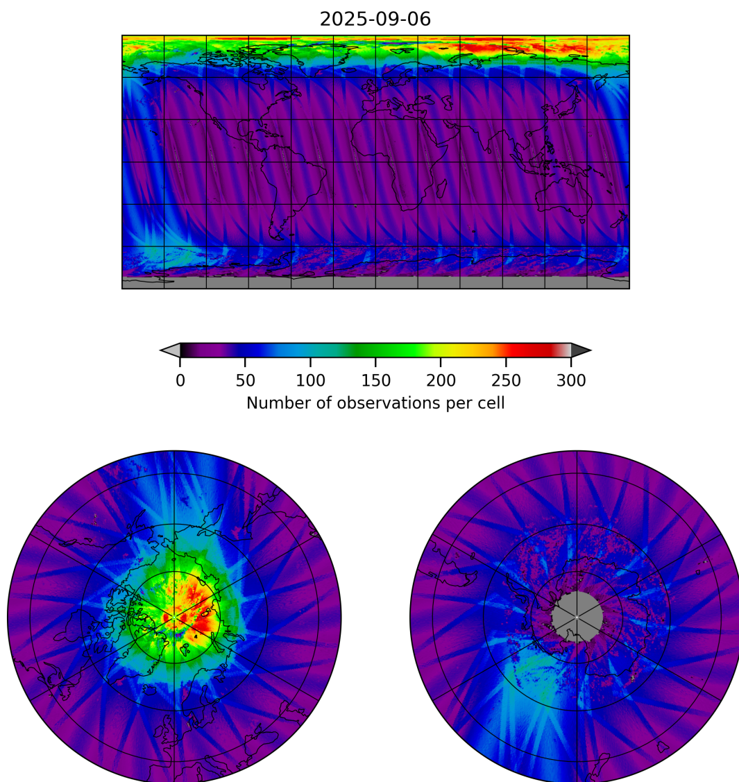
Figure 11: Map of the number of observations for 2025-09-05 to 2025-09-07
