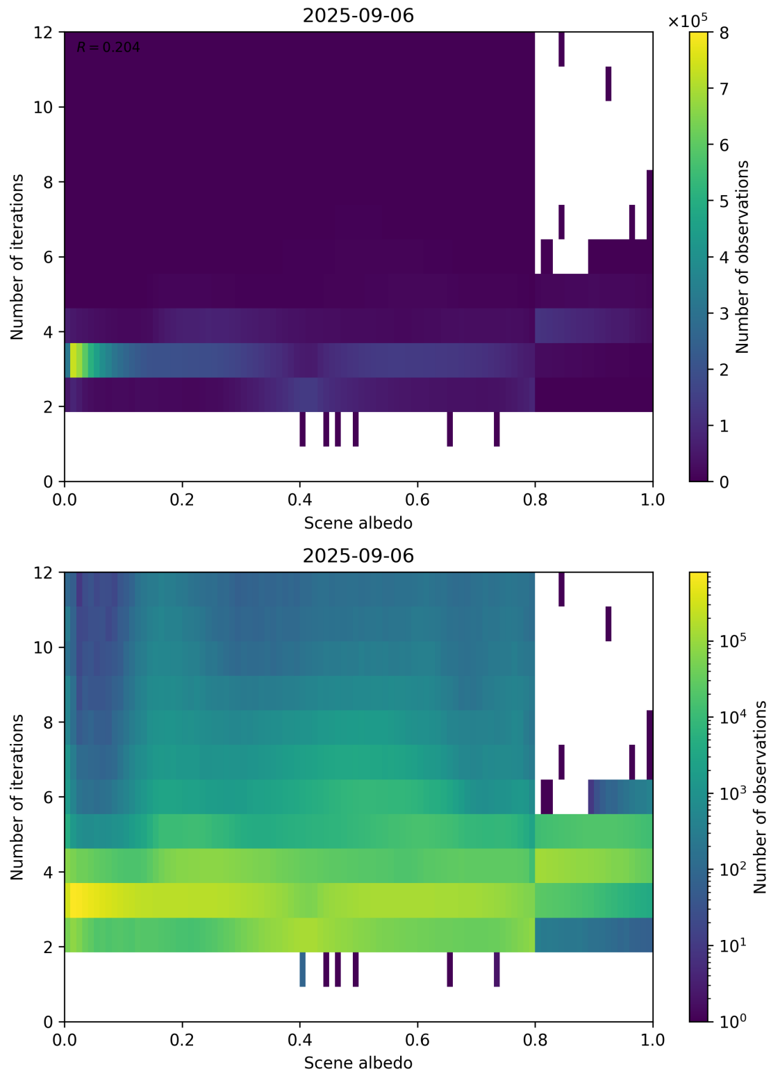
Figure 105: Scatter density plot of “Scene albedo” against “Number of iterations” for 2025-09-05 to 2025-09-07.
