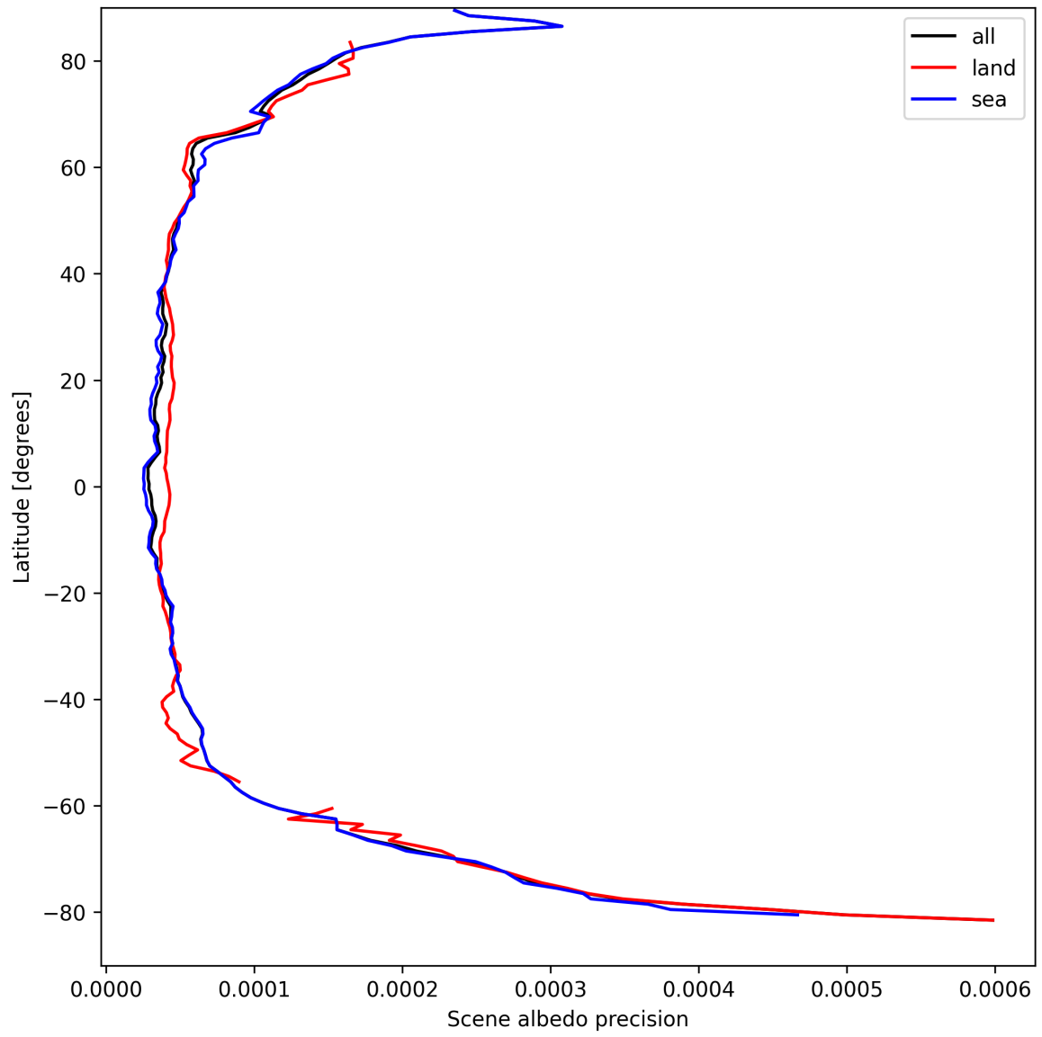
Figure 18: Zonal average of “Scene albedo precision” for 2025-09-05 to 2025-09-07.
