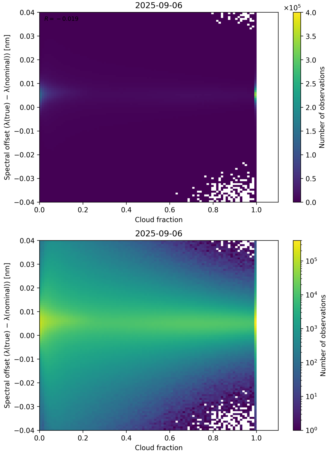
Figure 76: Scatter density plot of “Cloud fraction” against “Spectral offset ( \lambda_{\text{true}} - \lambda_{\text{nominal}} )” for 2025-09-05 to 2025-09-07.
