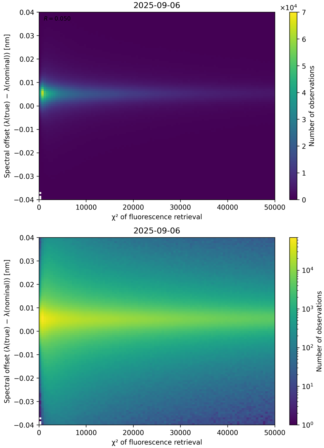
Figure 69: Scatter density plot of “ \chi^2 of fluorescence retrieval” against “Spectral offset ( \lambda_{\text{true}} - \lambda_{\text{nominal}} )” for 2025-09-05 to 2025-09-07.
