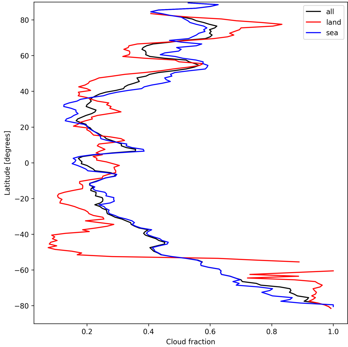
Figure 15: Zonal average of “Cloud fraction” for 2025-09-05 to 2025-09-07.
