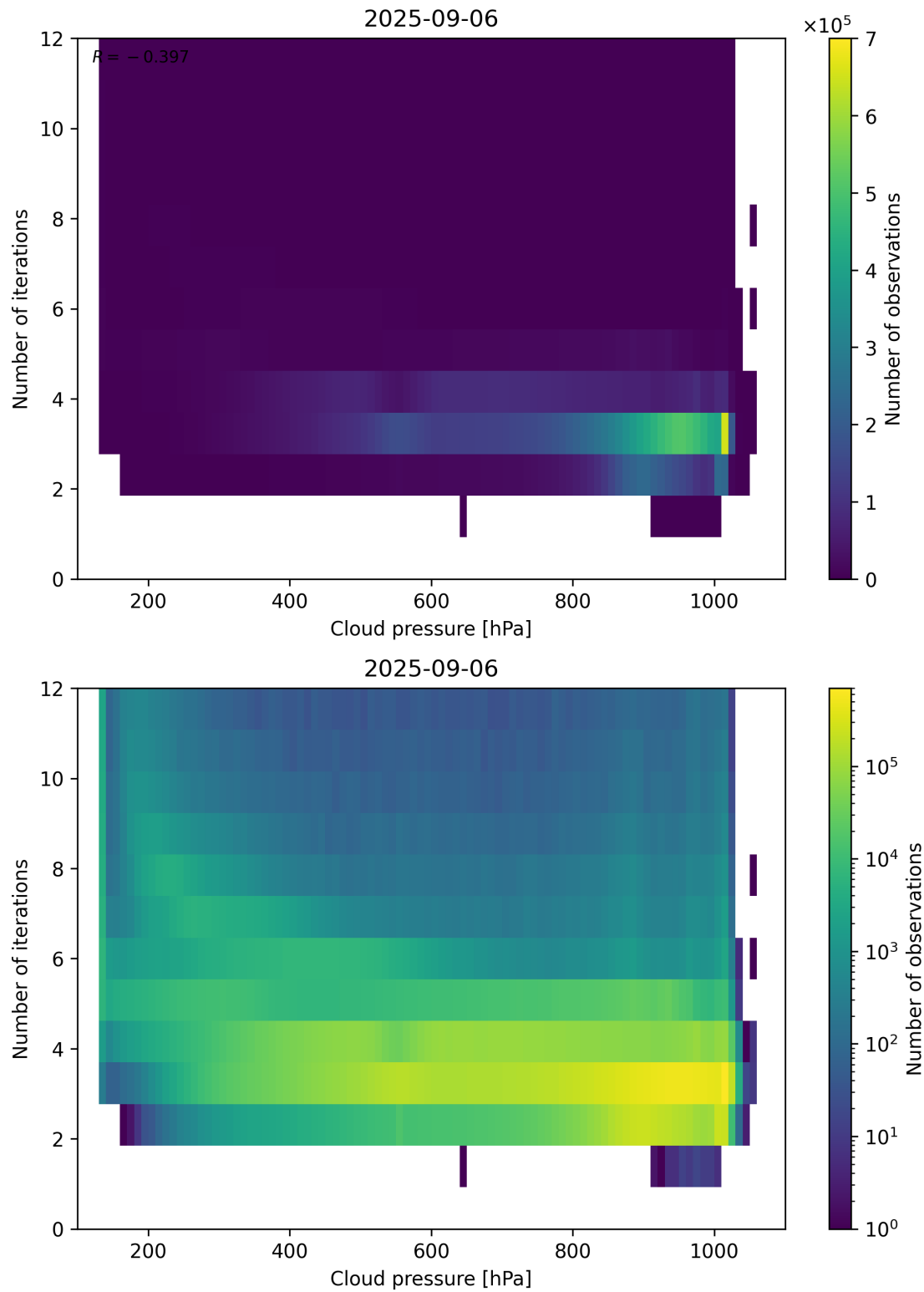
Figure 81: Scatter density plot of “Cloud pressure” against “Number of iterations” for 2025-09-05 to 2025-09-07.
