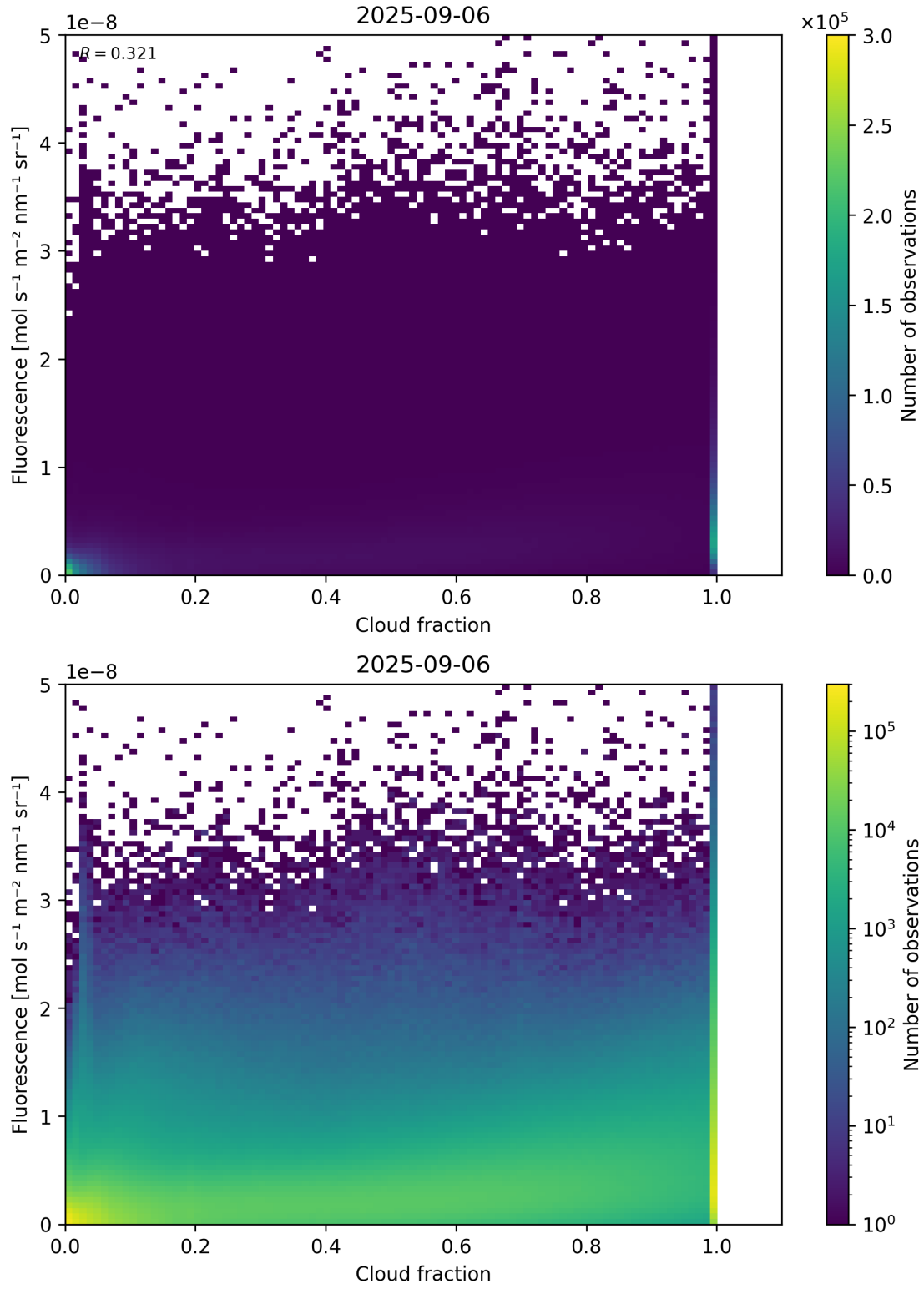
Figure 72: Scatter density plot of “Cloud fraction” against “Fluorescence” for 2025-09-05 to 2025-09-07.
