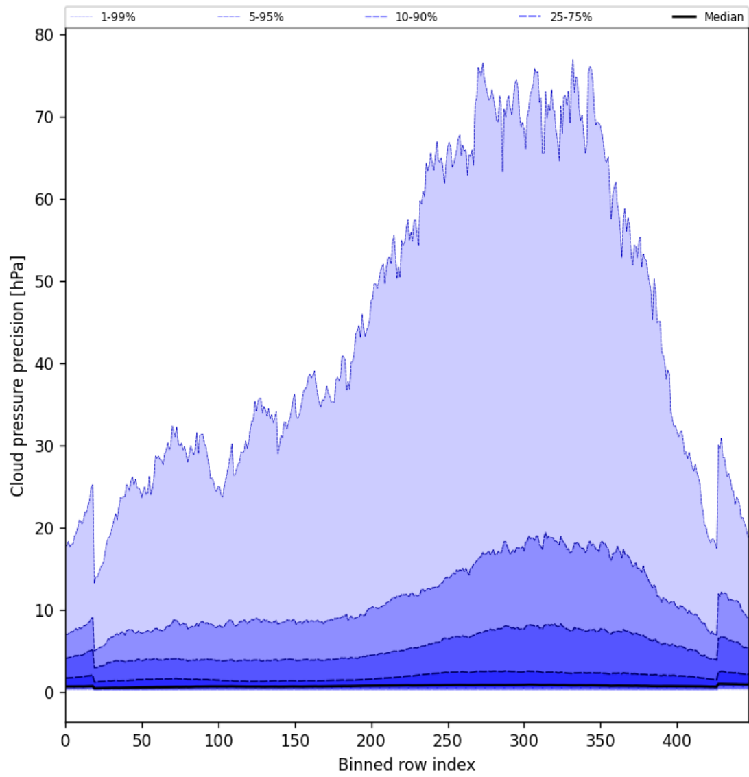
Figure 48: Along track statistics of “Cloud pressure precision” for 2025-09-05 to 2025-09-07
