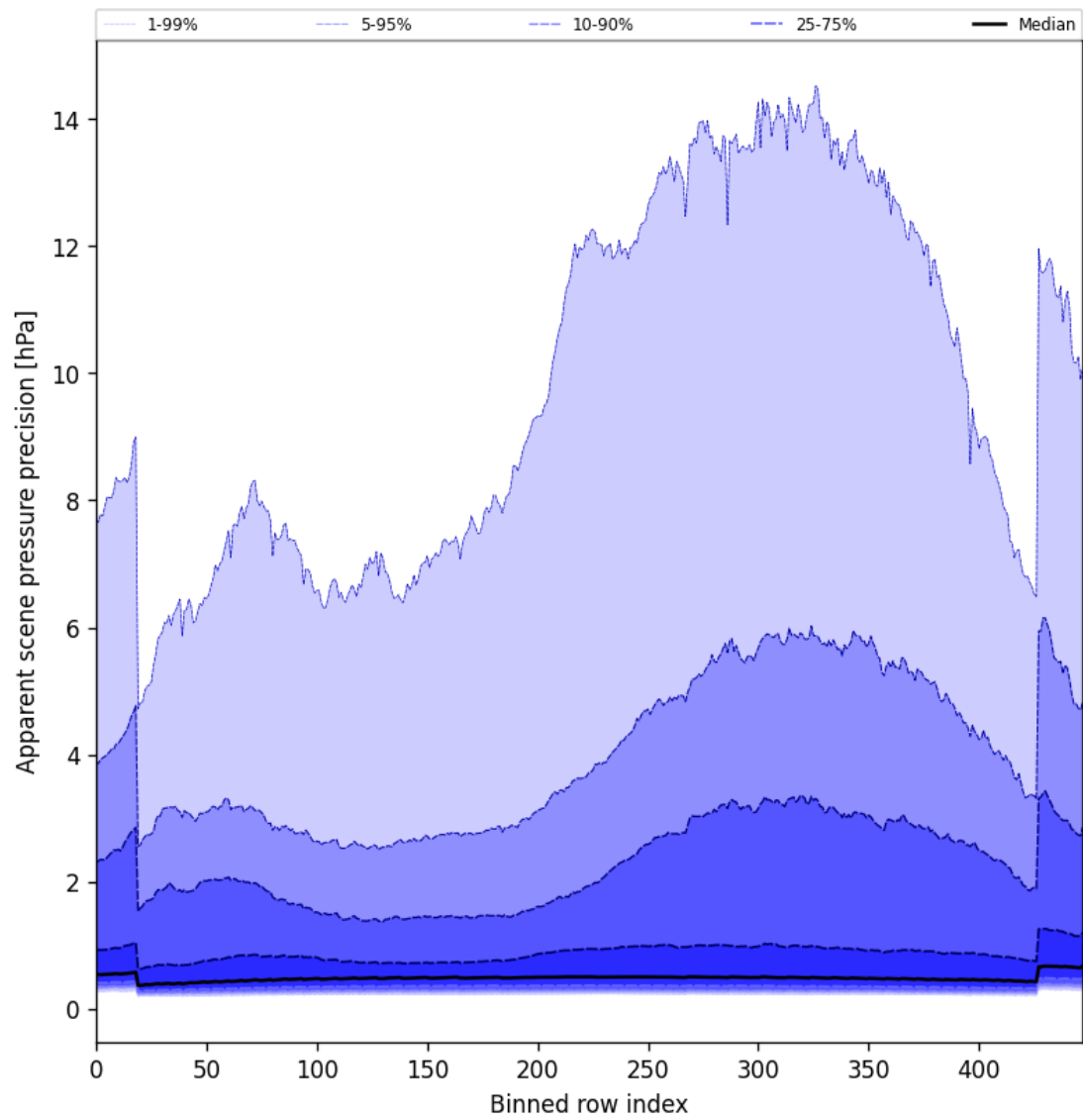
Figure 54: Along track statistics of “Apparent scene pressure precision” for 2025-09-05 to 2025-09-07
