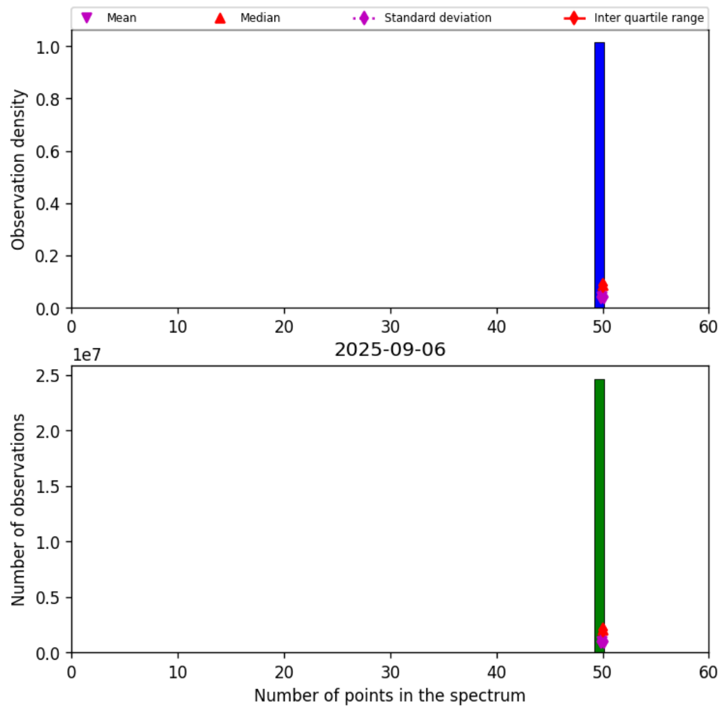
Figure 44: Histogram of “Number of points in the spectrum” for 2025-09-05 to 2025-09-07
