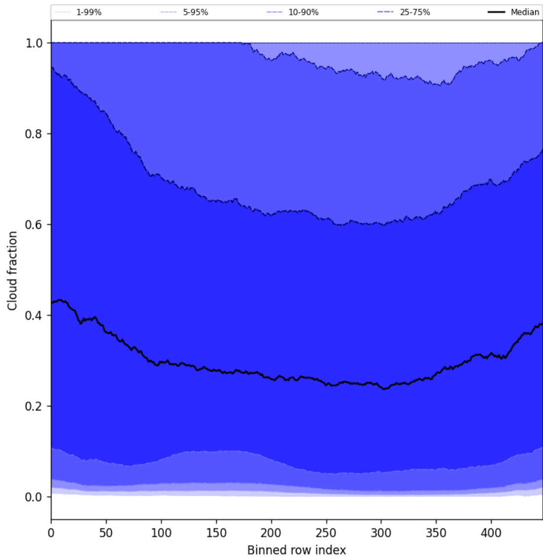
Figure 49: Along track statistics of “Cloud fraction” for 2025-09-05 to 2025-09-07
