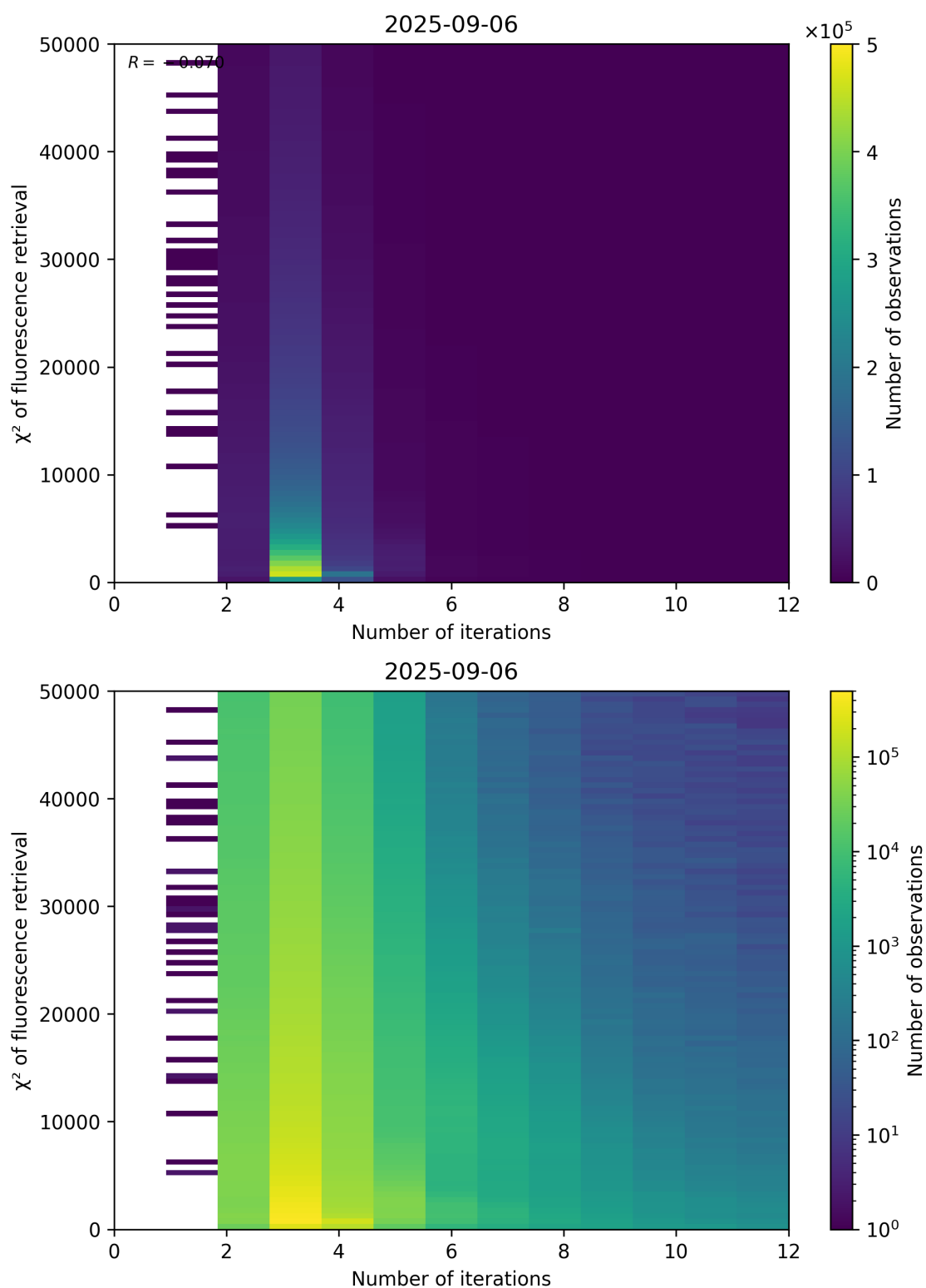
Figure 97: Scatter density plot of “Number of iterations” against “ \chi^2 of fluorescence retrieval” for 2025-09-05 to 2025-09-07.
