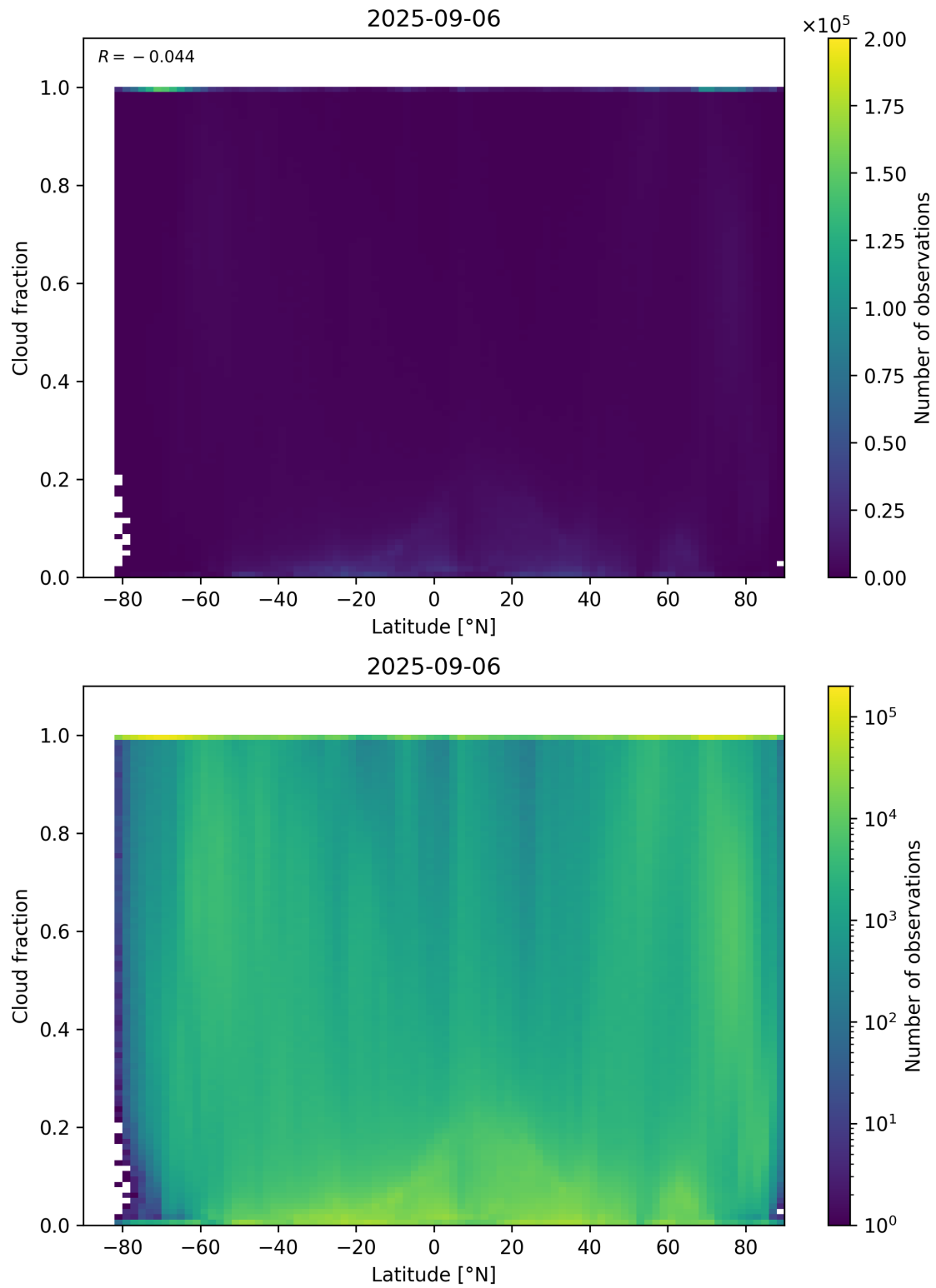
Figure 90: Scatter density plot of “Latitude” against “Cloud fraction” for 2025-09-05 to 2025-09-07.
