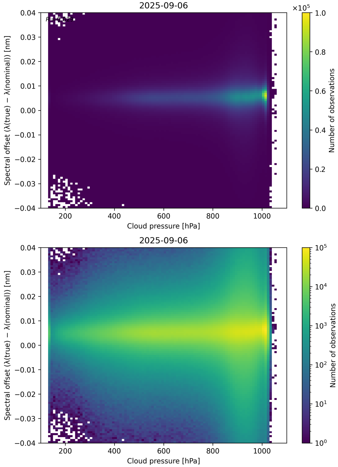
Figure 84: Scatter density plot of “Cloud pressure” against “Spectral offset ( \lambda_{\text{true}} - \lambda_{\text{nominal}} )” for 2025-09-05 to 2025-09-07.
