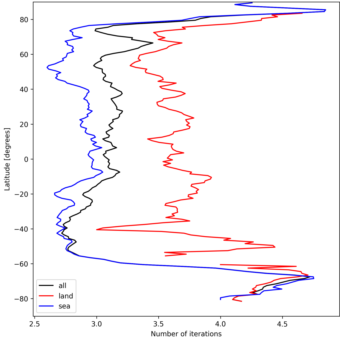
Figure 22: Zonal average of “Number of iterations” for 2025-09-05 to 2025-09-07.
