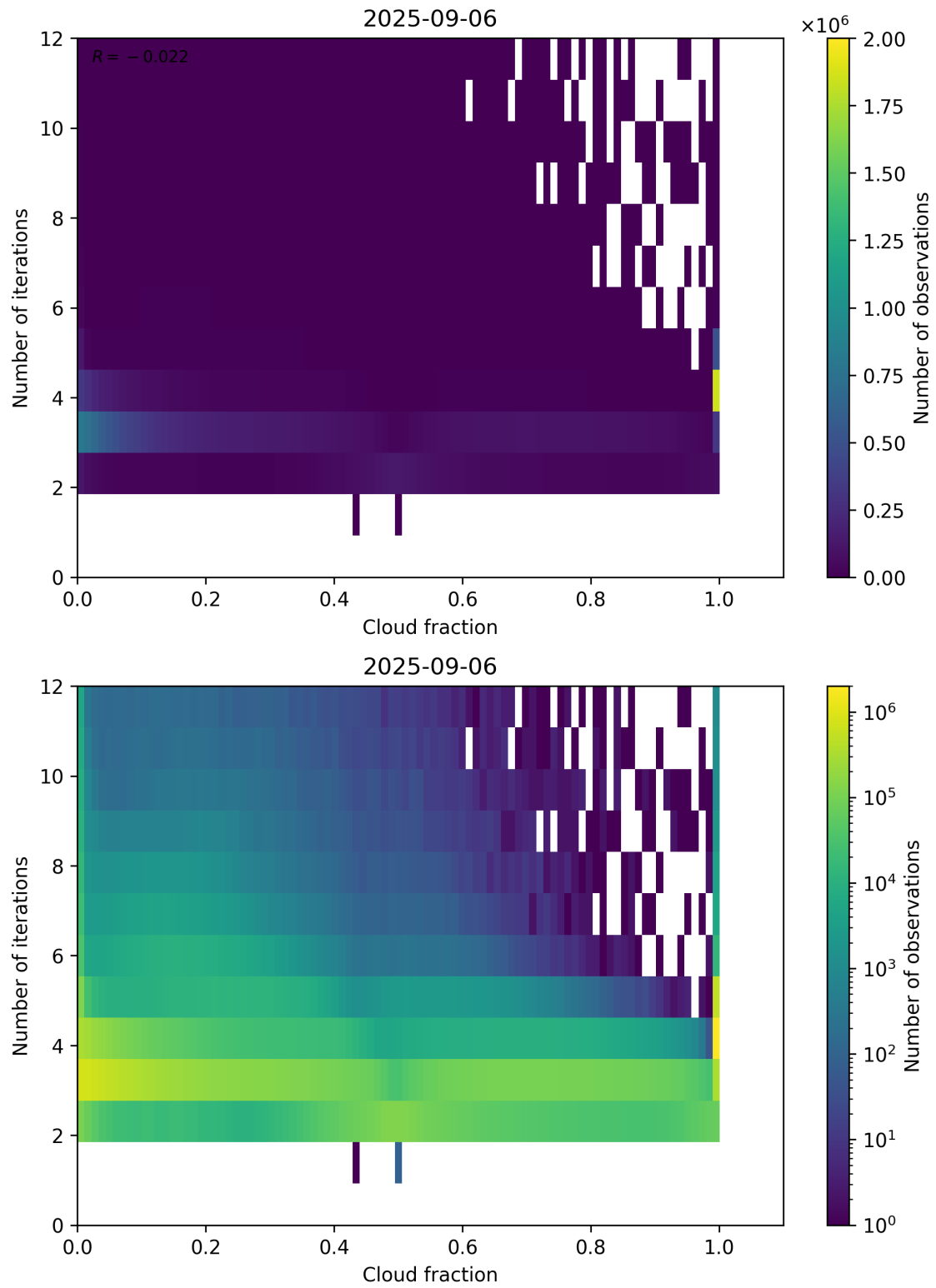
Figure 73: Scatter density plot of “Cloud fraction” against “Number of iterations” for 2025-09-05 to 2025-09-07.
