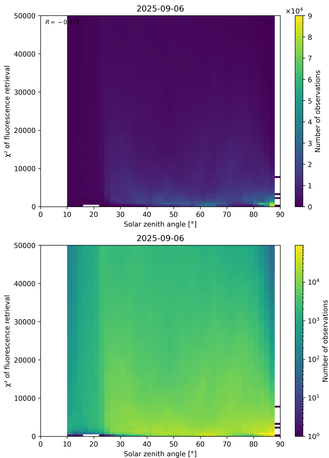
Figure 109: Scatter density plot of “Solar zenith angle” against “ \chi^2 of fluorescence retrieval” for 2025-09-05 to 2025-09-07.
