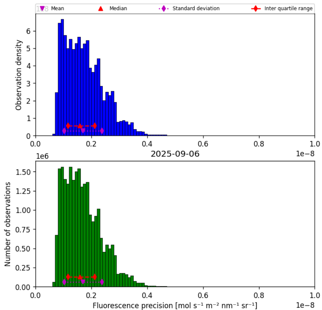
Figure 41: Histogram of “Fluorescence precision” for 2025-09-05 to 2025-09-07
