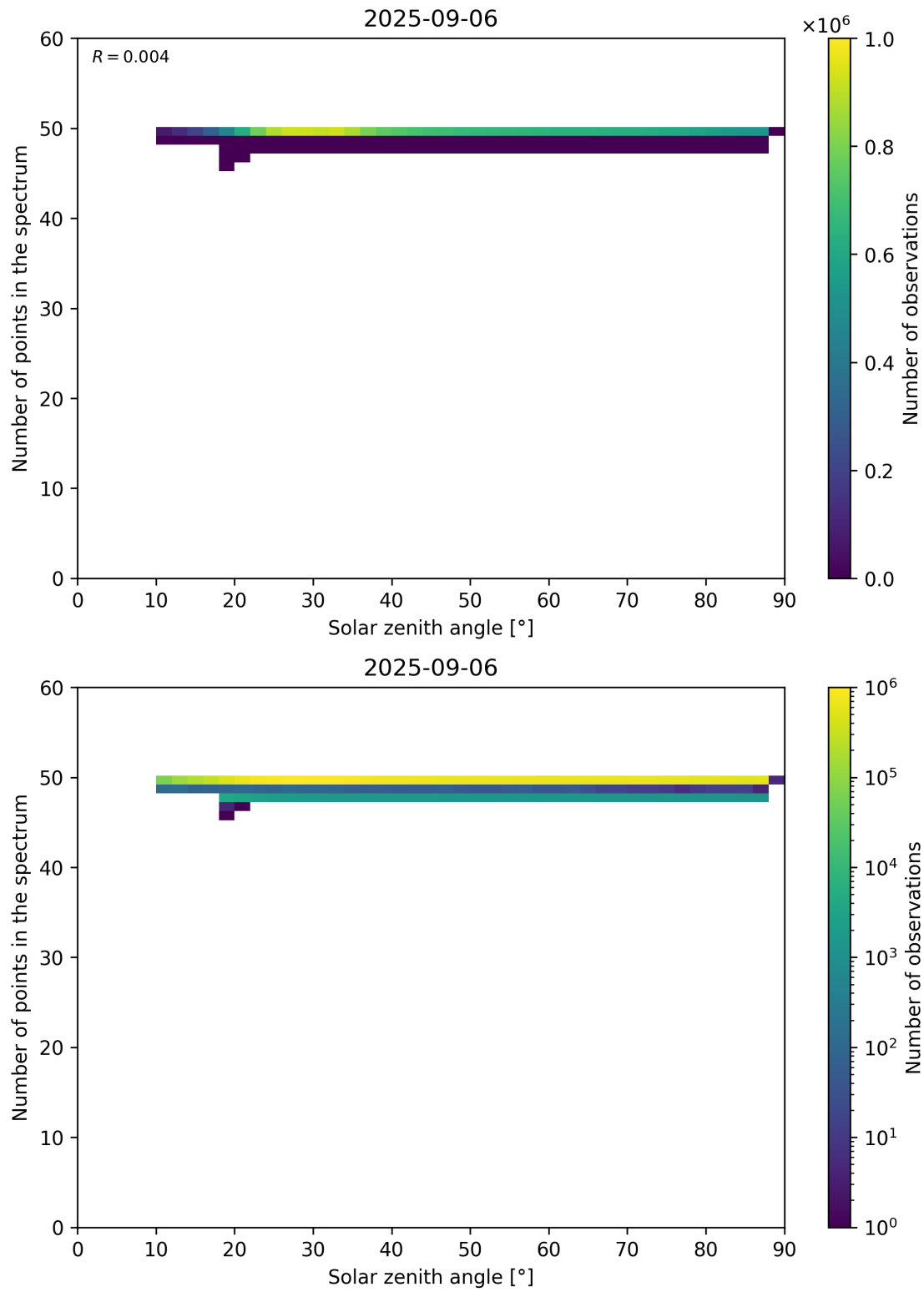
Figure 115: Scatter density plot of “Solar zenith angle” against “Number of points in the spectrum” for 2025-09-05 to 2025-09-07.
