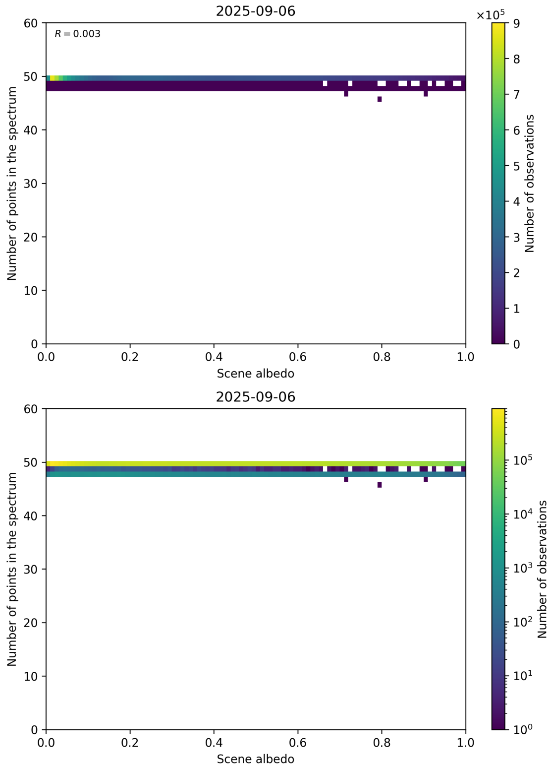
Figure 106: Scatter density plot of “Scene albedo” against “Number of points in the spectrum” for 2025-09-05 to 2025-09-07.
