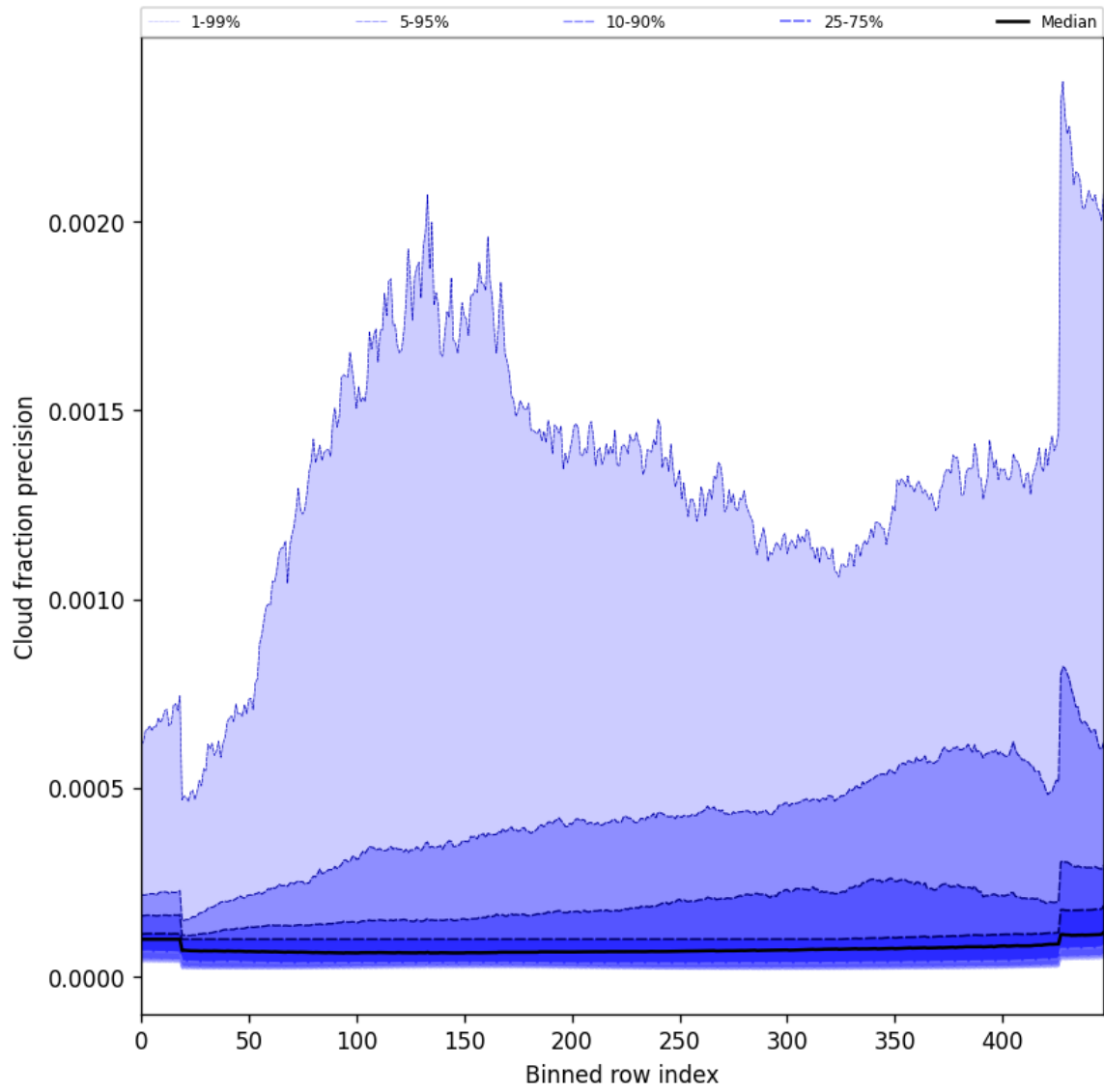
Figure 50: Along track statistics of “Cloud fraction precision” for 2025-09-05 to 2025-09-07
