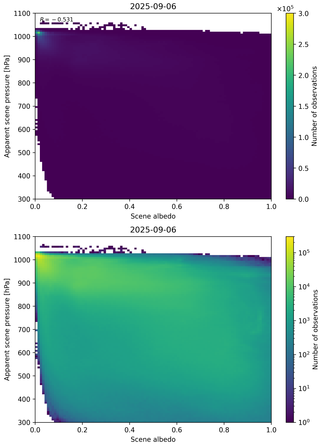
Figure 102: Scatter density plot of “Scene albedo” against “Apparent scene pressure” for 2025-09-05 to 2025-09-07.
