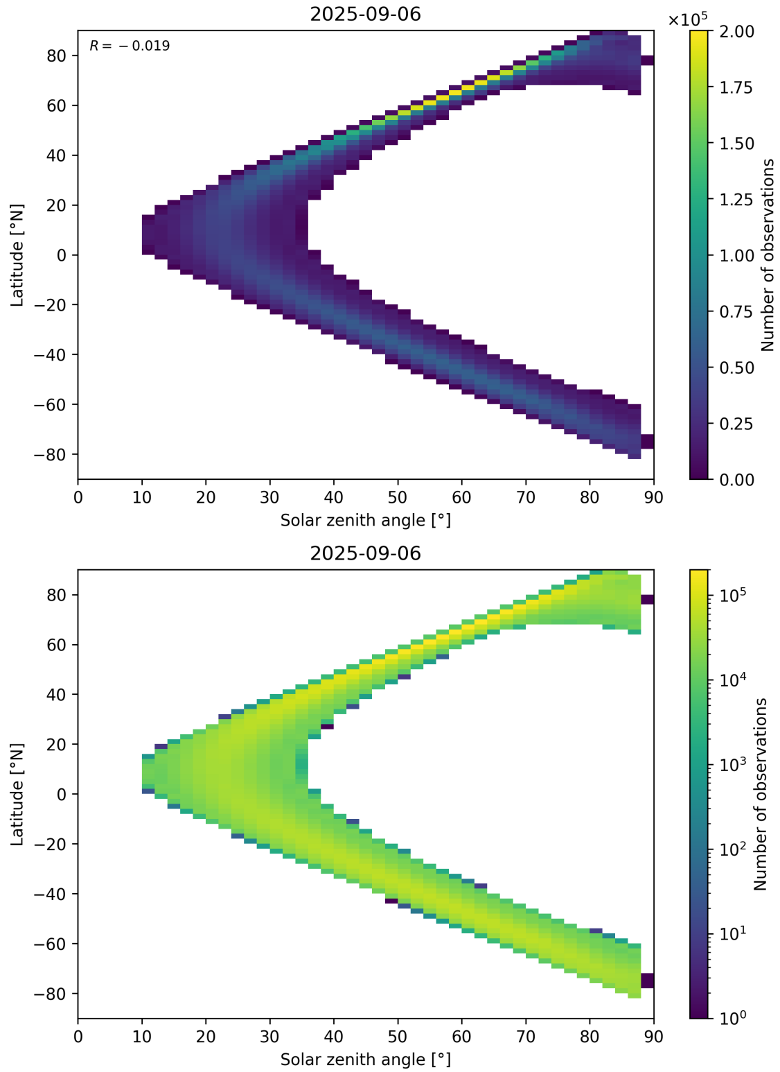
Figure 113: Scatter density plot of “Solar zenith angle” against “Latitude” for 2025-09-05 to 2025-09-07.
