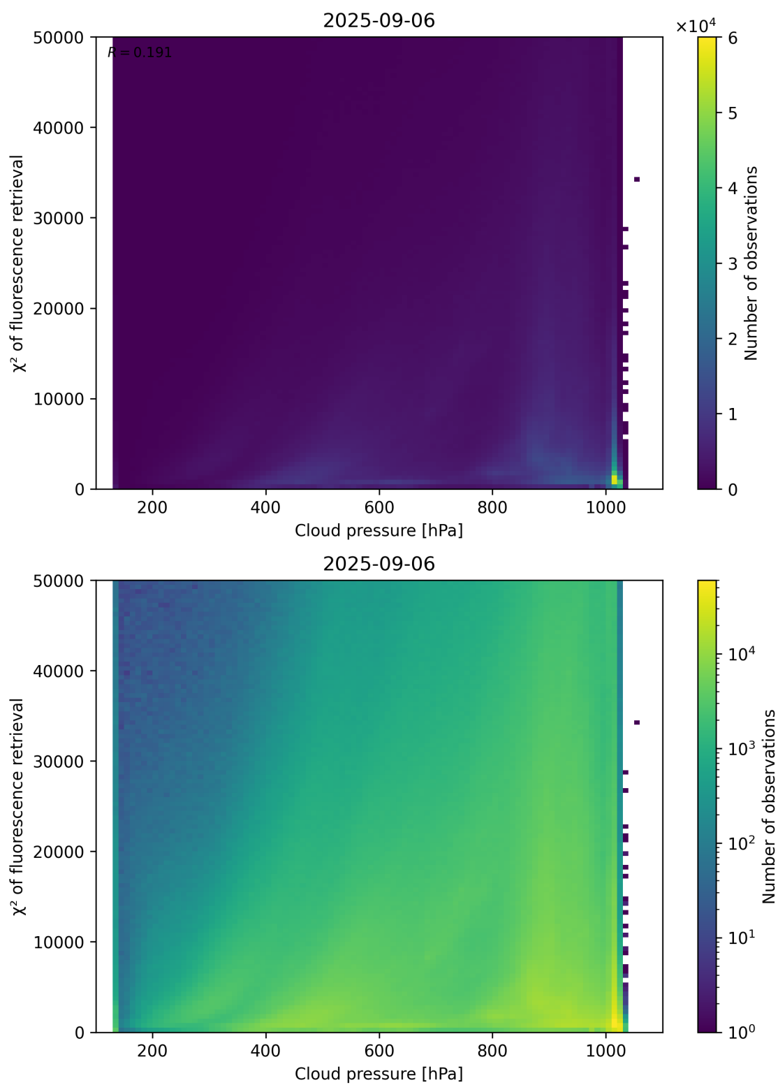
Figure 78: Scatter density plot of “Cloud pressure” against “ \chi^2 of fluorescence retrieval” for 2025-09-05 to 2025-09-07.
