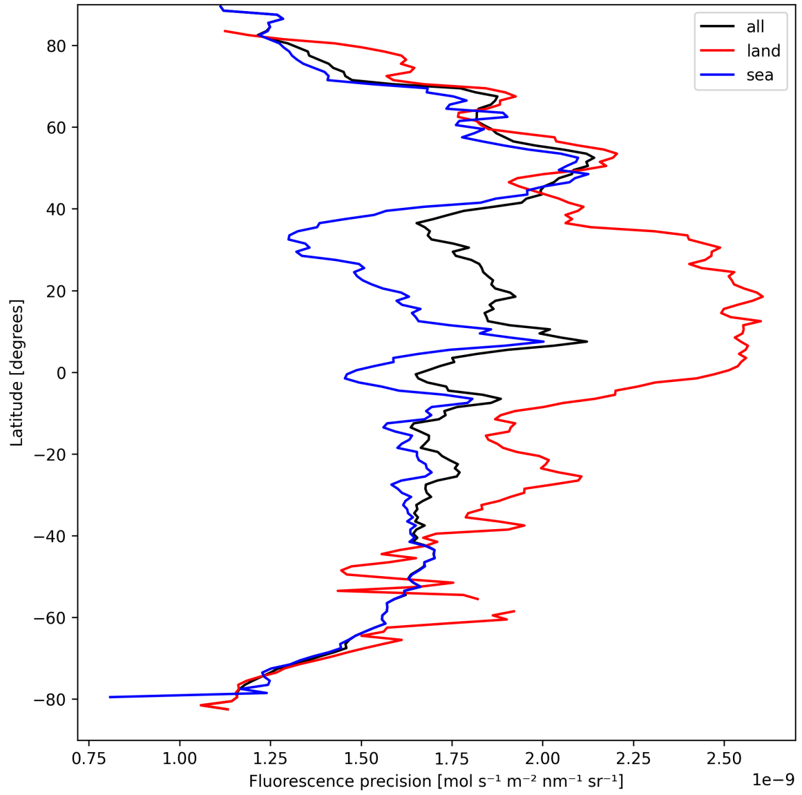
Figure 24: Zonal average of “Fluorescence precision” for 2025-09-06 to 2025-09-08.
