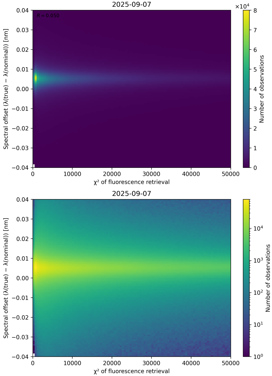
Figure 69: Scatter density plot of “ \chi^2 of fluorescence retrieval” against “Spectral offset ( \lambda_{\text{true}} - \lambda_{\text{nominal}} )” for 2025-09-06 to 2025-09-08.
