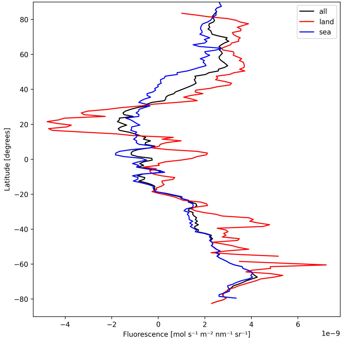
Figure 23: Zonal average of “Fluorescence” for 2025-09-06 to 2025-09-08.
