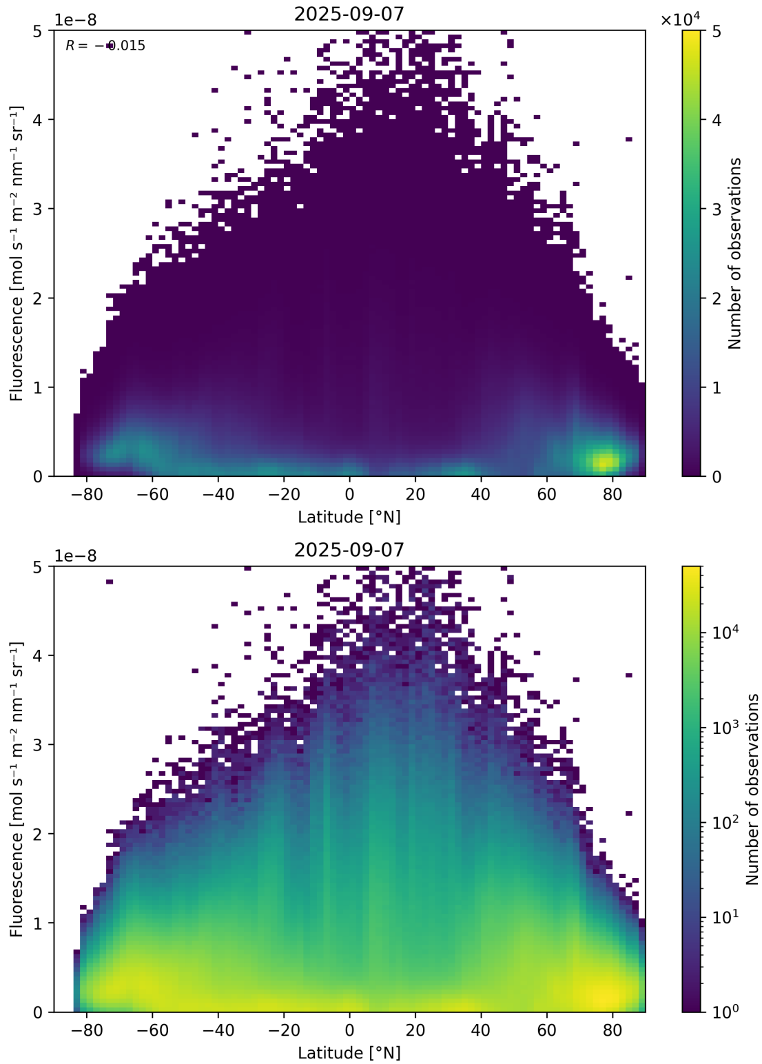
Figure 92: Scatter density plot of “Latitude” against “Fluorescence” for 2025-09-06 to 2025-09-08.
