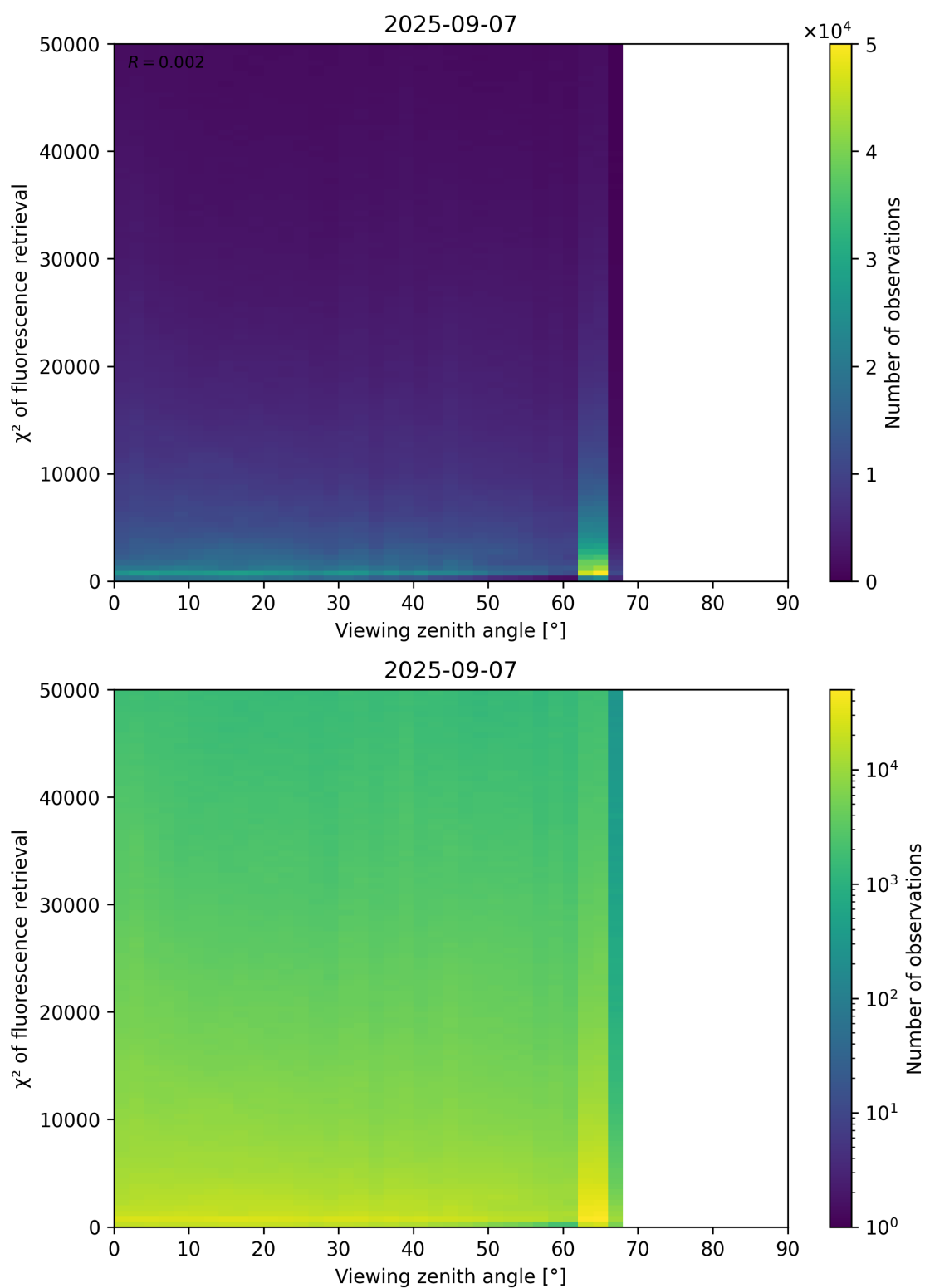
Figure 119: Scatter density plot of “Viewing zenith angle” against “ \chi^2 of fluorescence retrieval” for 2025-09-06 to 2025-09-08.
