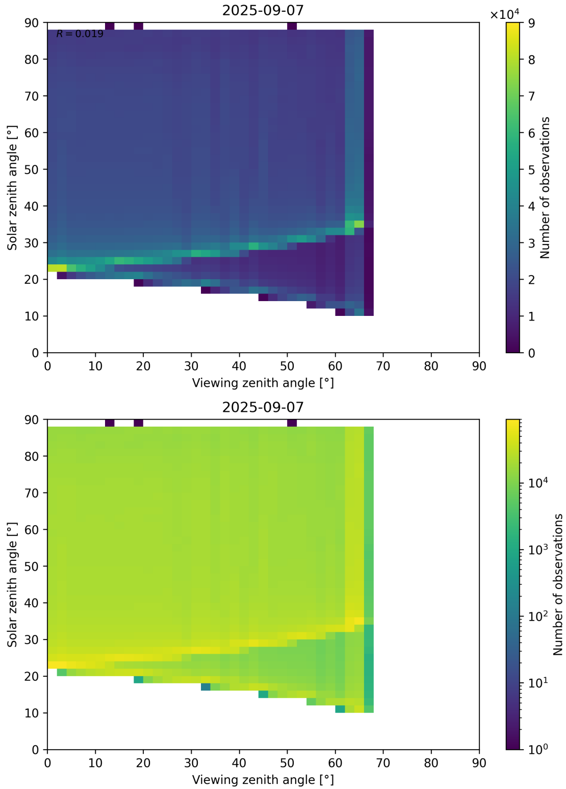
Figure 127: Scatter density plot of “Viewing zenith angle” against “Solar zenith angle” for 2025-09-06 to 2025-09-08.
