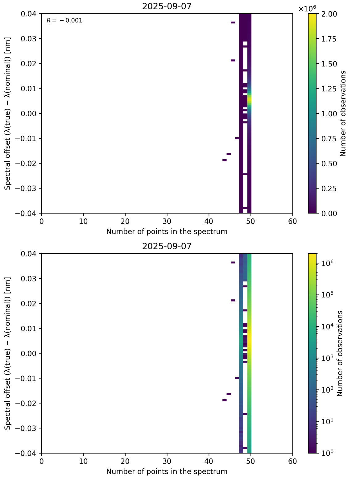
Figure 101: Scatter density plot of “Number of points in the spectrum” against “Spectral offset ( \lambda_{\text{true}} - \lambda_{\text{nominal}} )” for 2025-09-06 to 2025-09-08.
