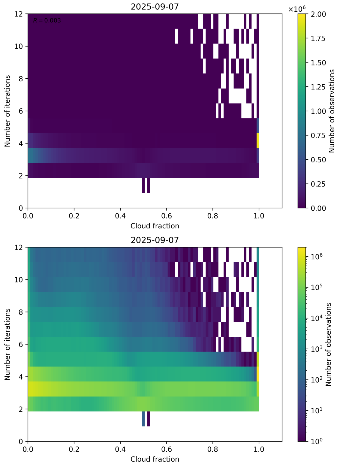
Figure 73: Scatter density plot of “Cloud fraction” against “Number of iterations” for 2025-09-06 to 2025-09-08.
