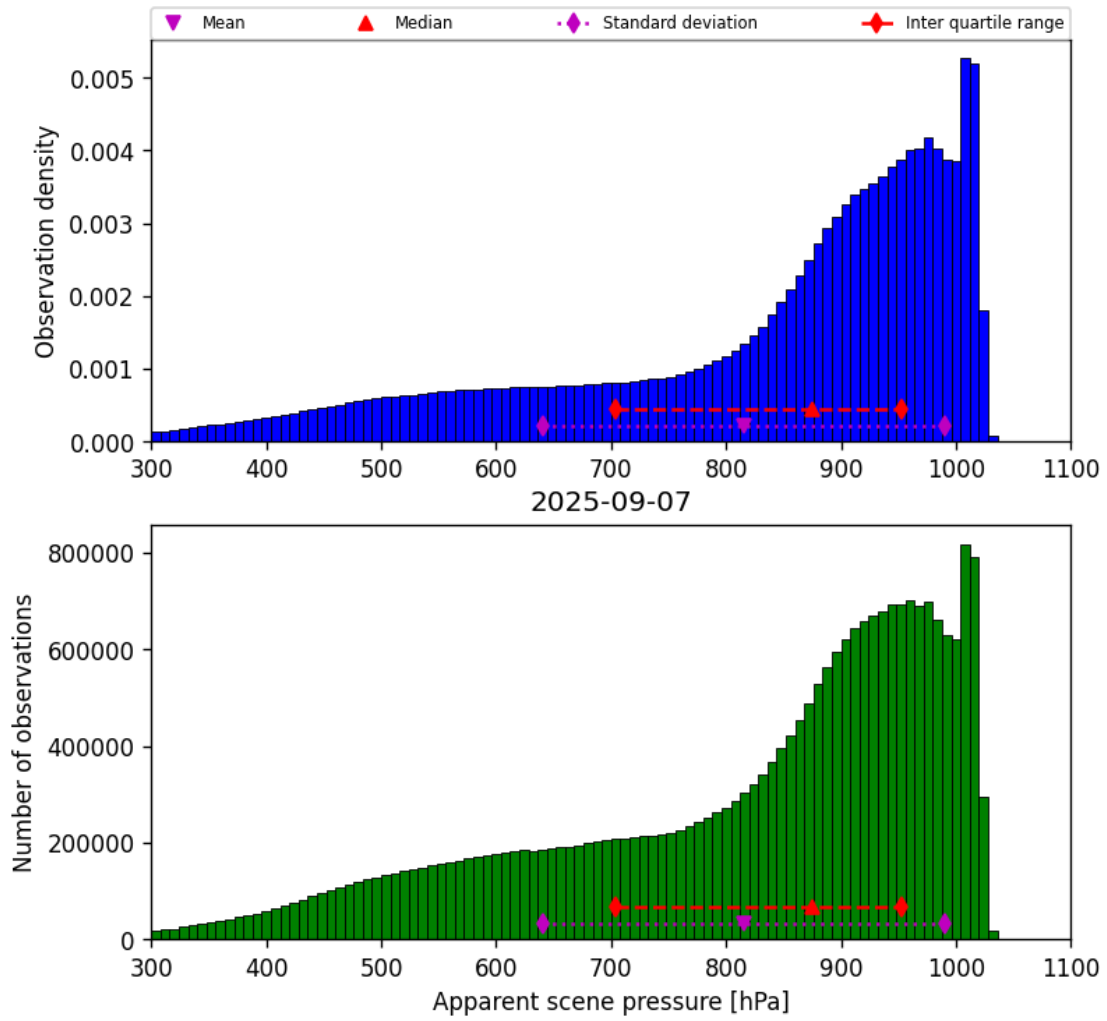
Figure 36: Histogram of “Apparent scene pressure” for 2025-09-06 to 2025-09-08
