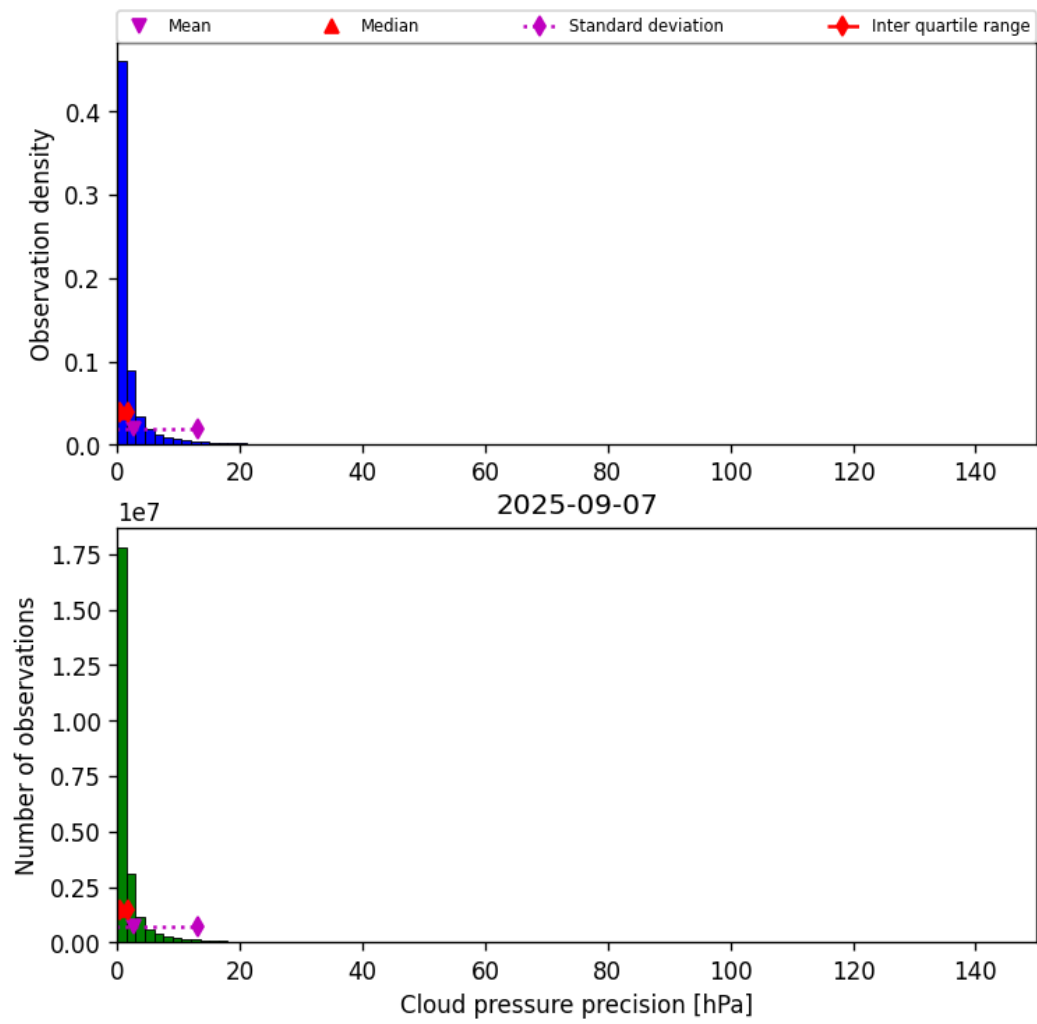
Figure 31: Histogram of “Cloud pressure precision” for 2025-09-06 to 2025-09-08
