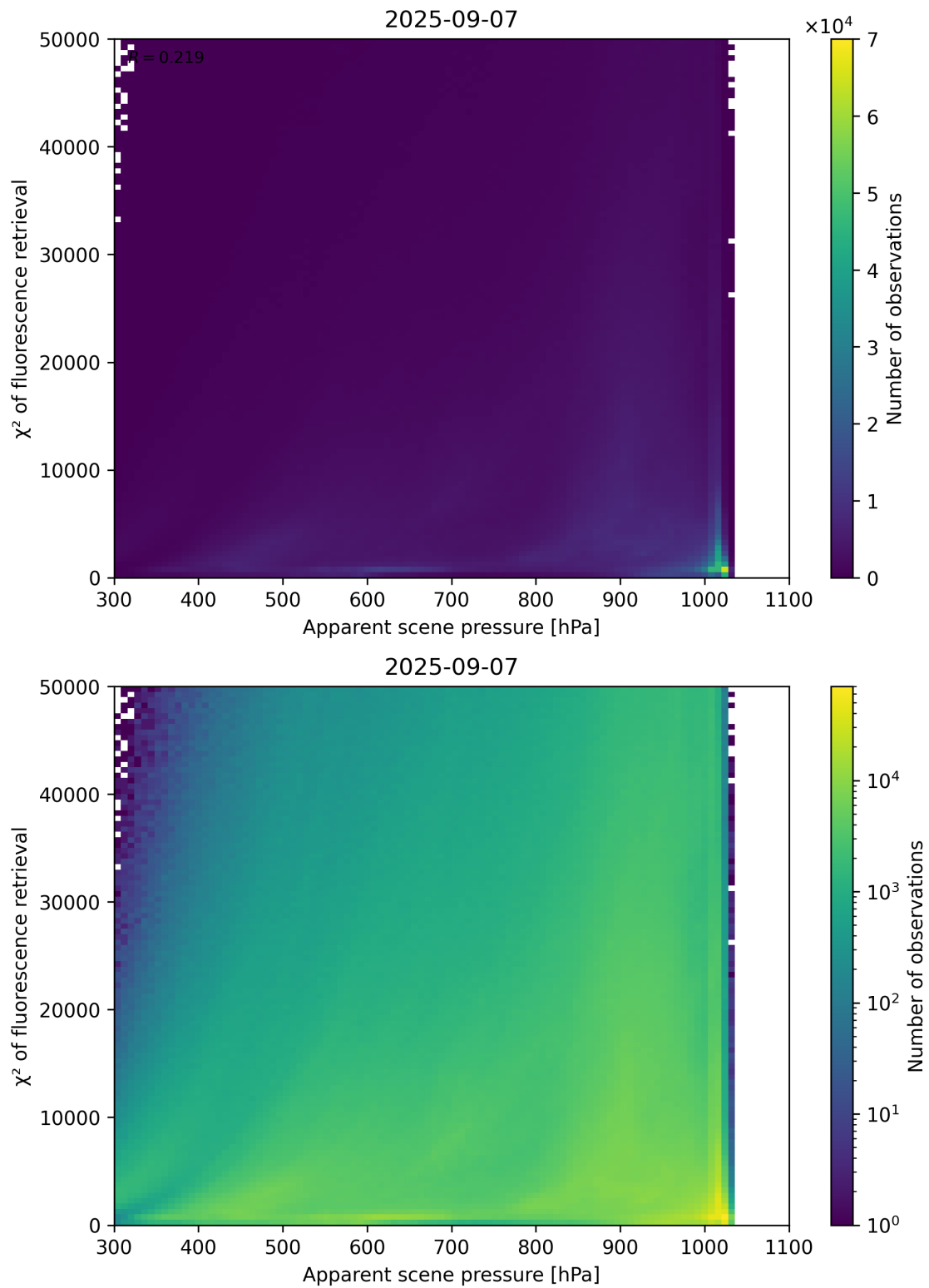
Figure 63: Scatter density plot of “Apparent scene pressure” against “ \chi^2 of fluorescence retrieval” for 2025-09-06 to 2025-09-08.
