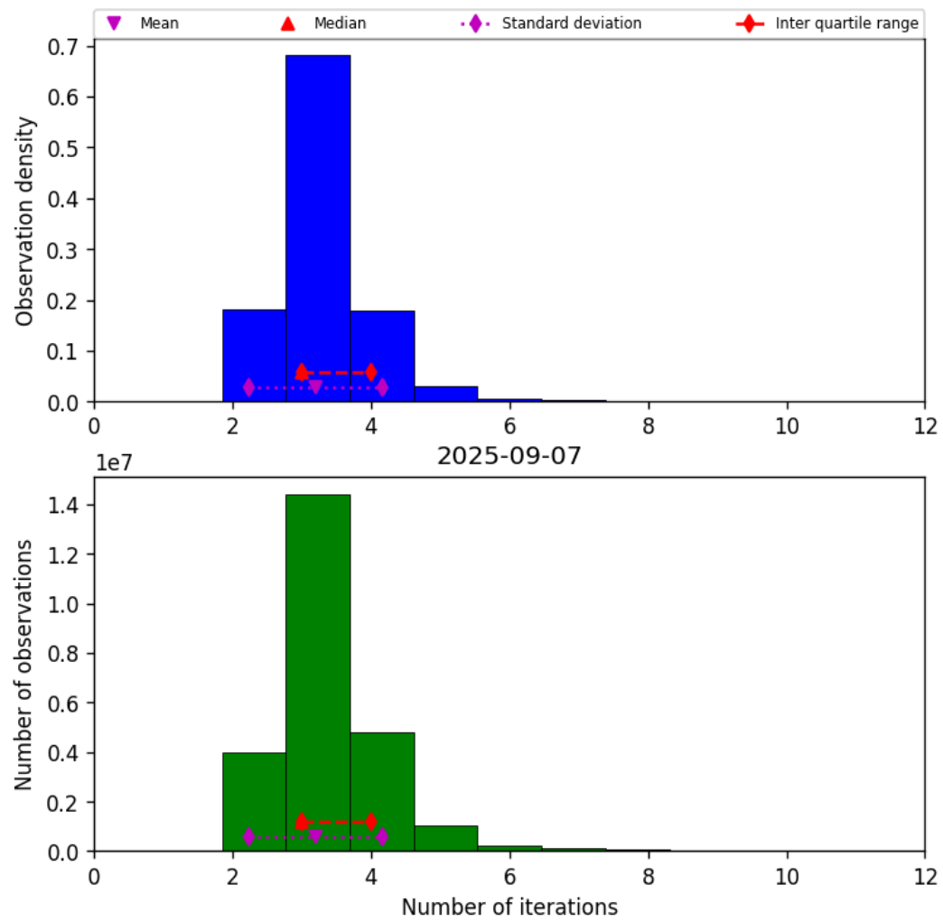
Figure 39: Histogram of “Number of iterations” for 2025-09-06 to 2025-09-08
