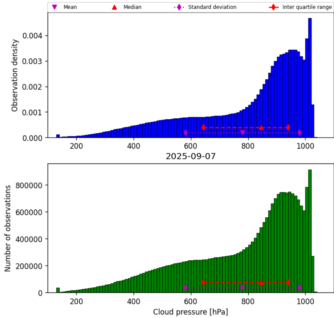
Figure 30: Histogram of “Cloud pressure” for 2025-09-06 to 2025-09-08
