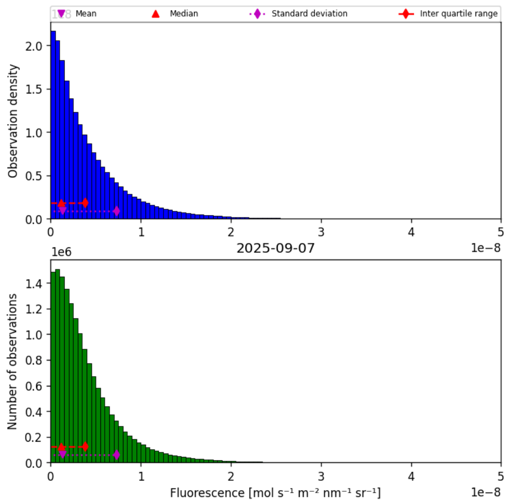
Figure 40: Histogram of “Fluorescence” for 2025-09-06 to 2025-09-08
