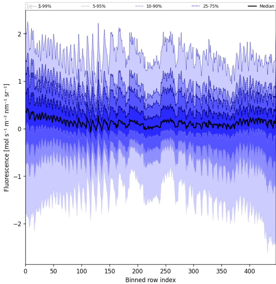
Figure 57: Along track statistics of “Fluorescence” for 2025-09-06 to 2025-09-08
