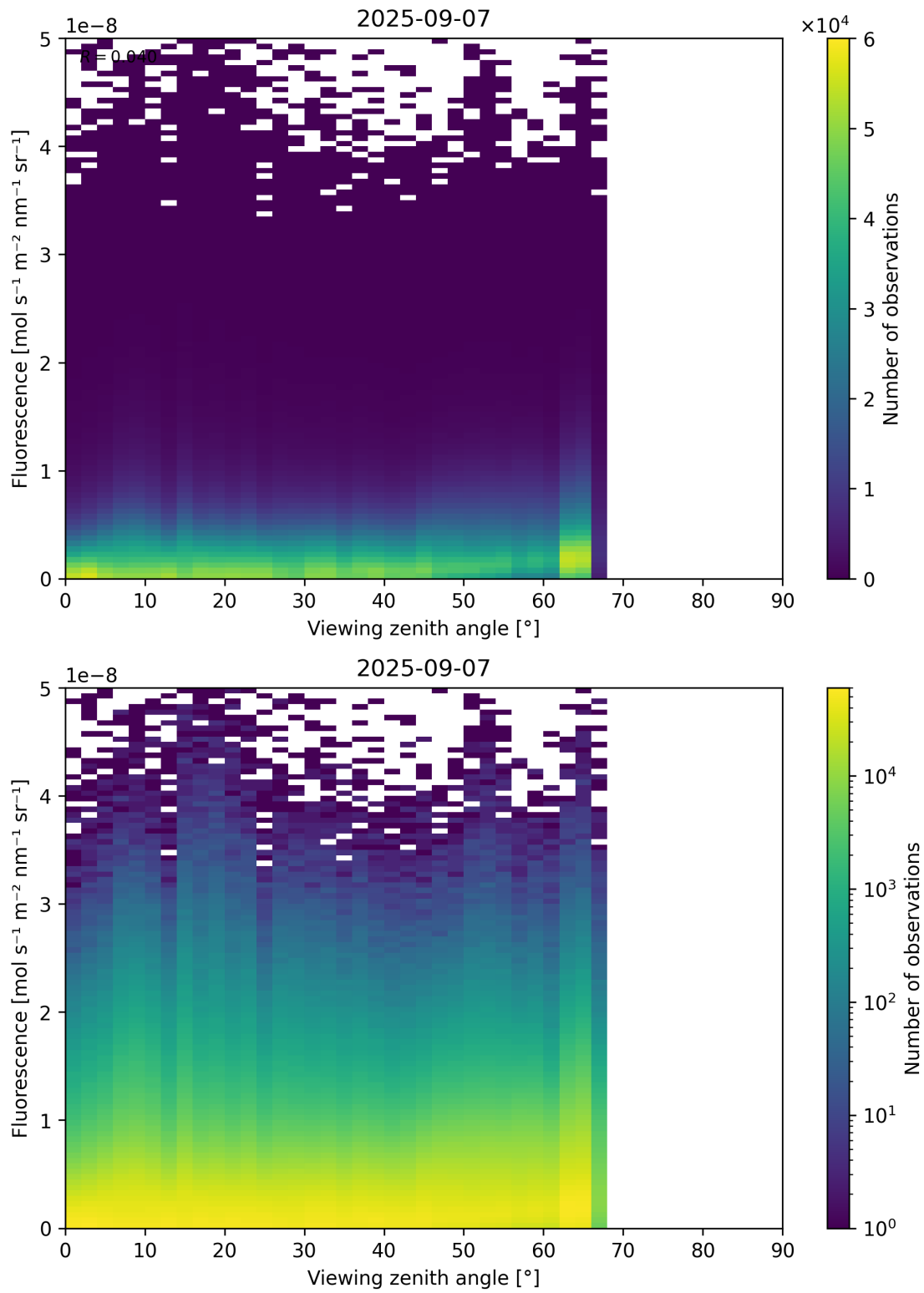
Figure 122: Scatter density plot of “Viewing zenith angle” against “Fluorescence” for 2025-09-06 to 2025-09-08.
