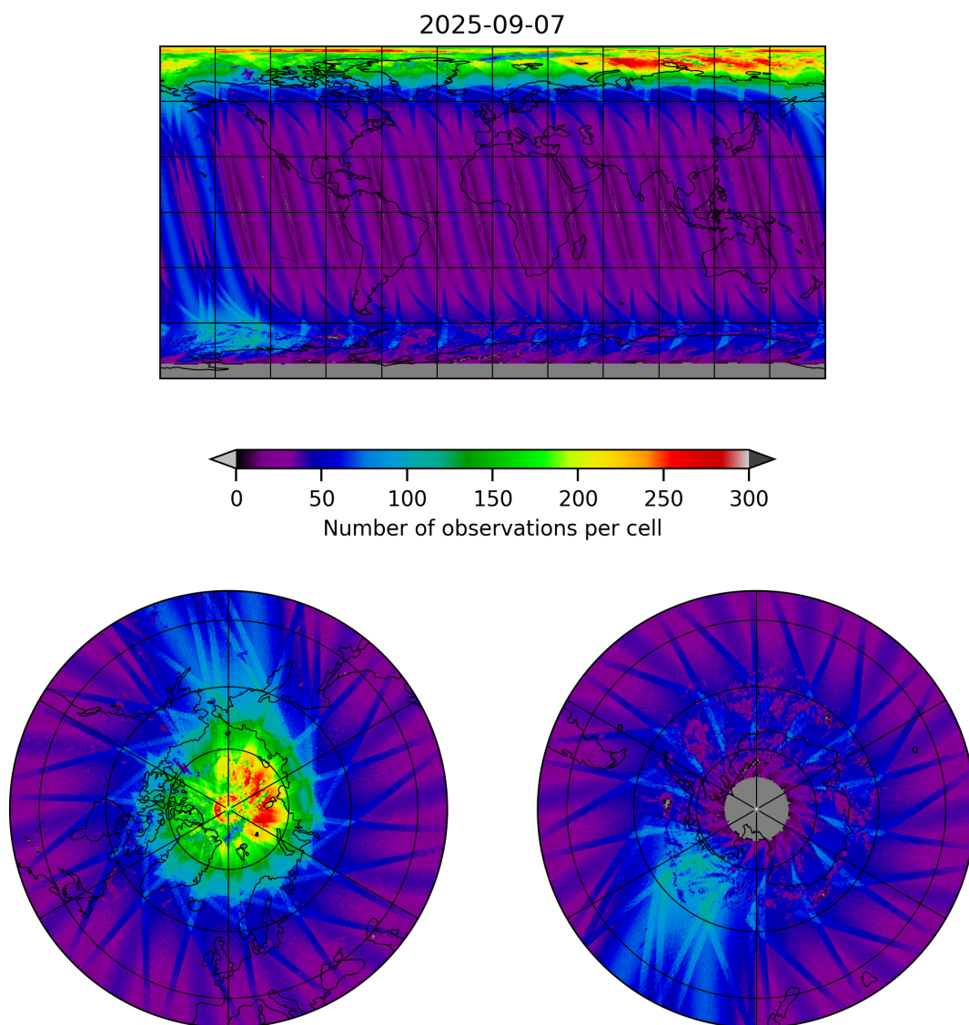
Figure 11: Map of the number of observations for 2025-09-06 to 2025-09-08
