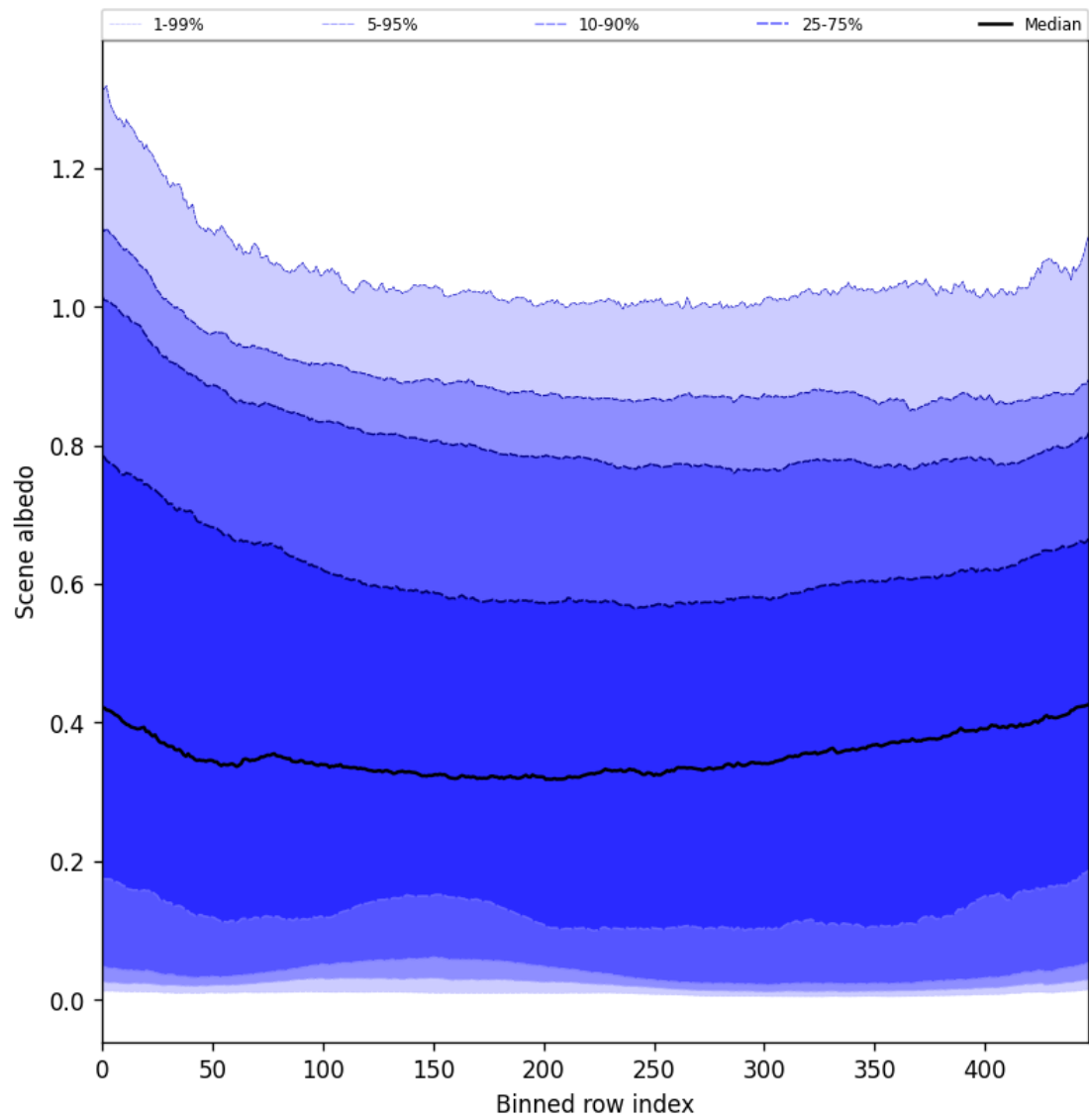
Figure 51: Along track statistics of “Scene albedo” for 2025-09-06 to 2025-09-08
