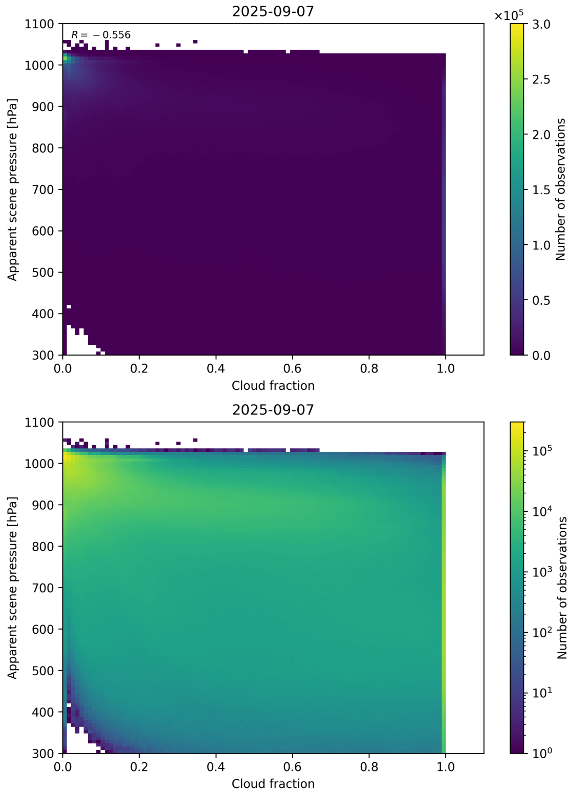
Figure 70: Scatter density plot of “Cloud fraction” against “Apparent scene pressure” for 2025-09-06 to 2025-09-08.
