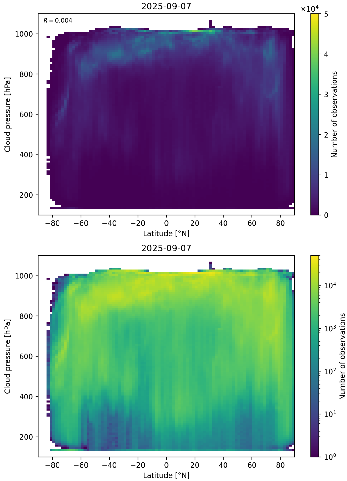
Figure 91: Scatter density plot of “Latitude” against “Cloud pressure” for 2025-09-06 to 2025-09-08.
