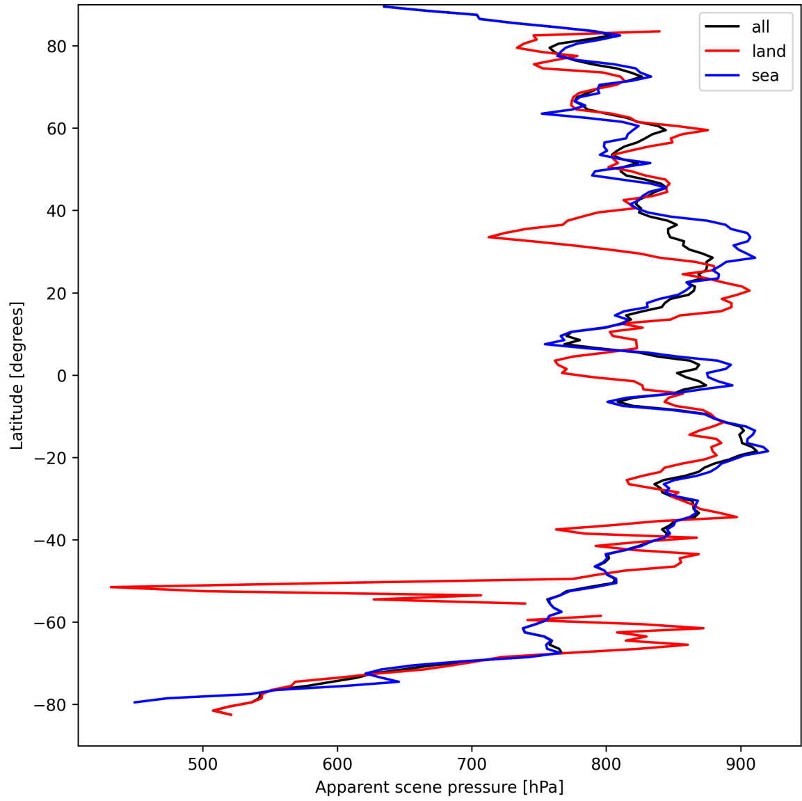
Figure 19: Zonal average of “Apparent scene pressure” for 2025-09-06 to 2025-09-08.
