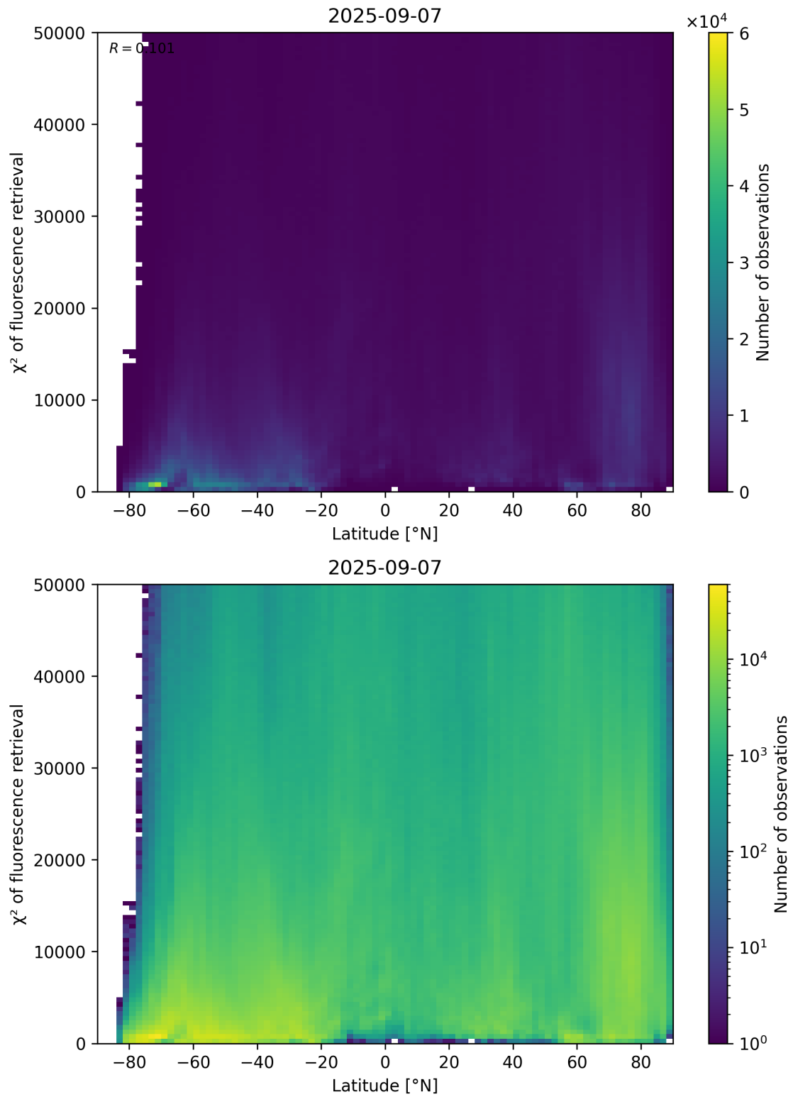
Figure 89: Scatter density plot of “Latitude” against “ \chi^2 of fluorescence retrieval” for 2025-09-06 to 2025-09-08.
