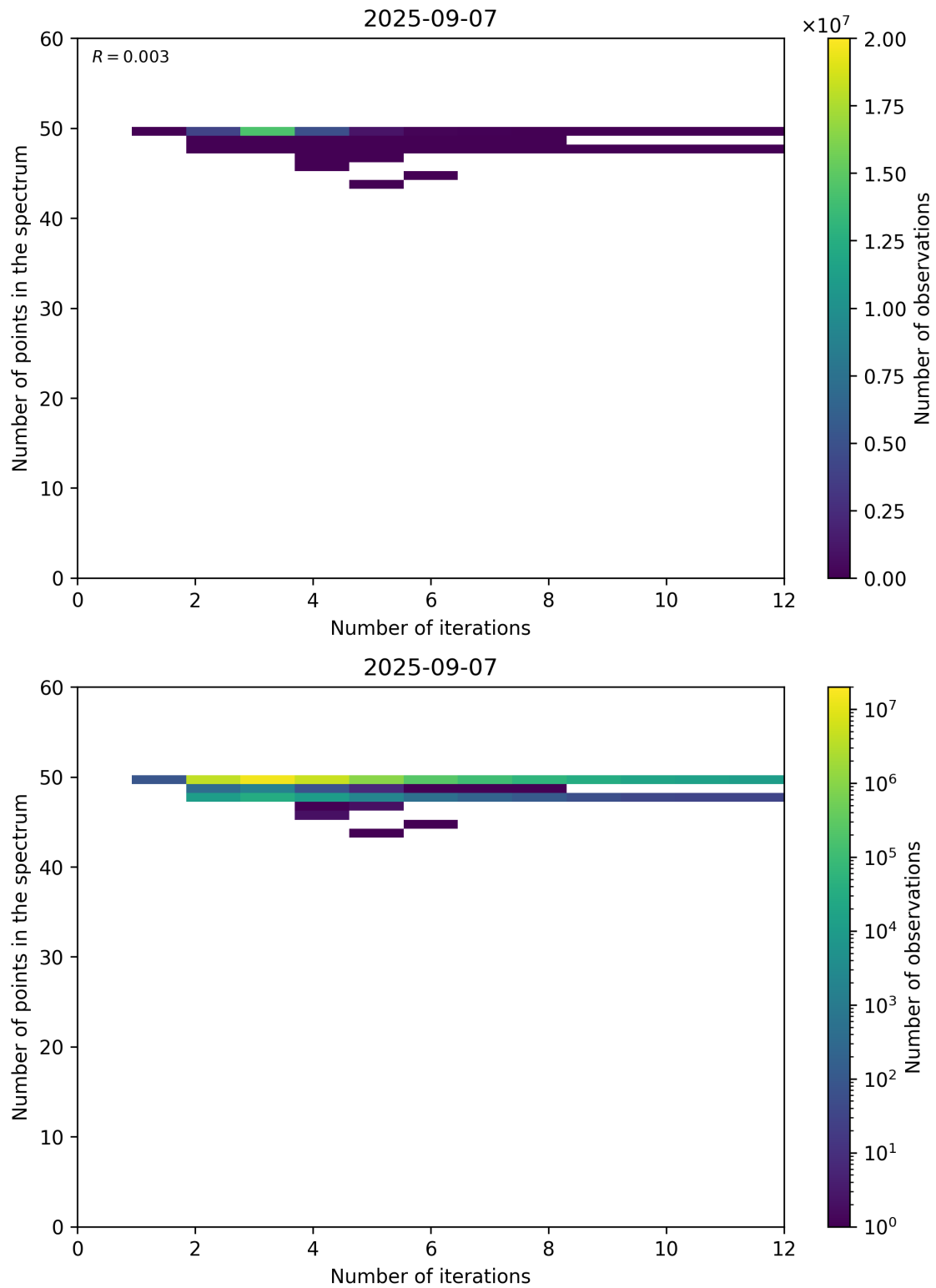
Figure 99: Scatter density plot of “Number of iterations” against “Number of points in the spectrum” for 2025-09-06 to 2025-09-08.
