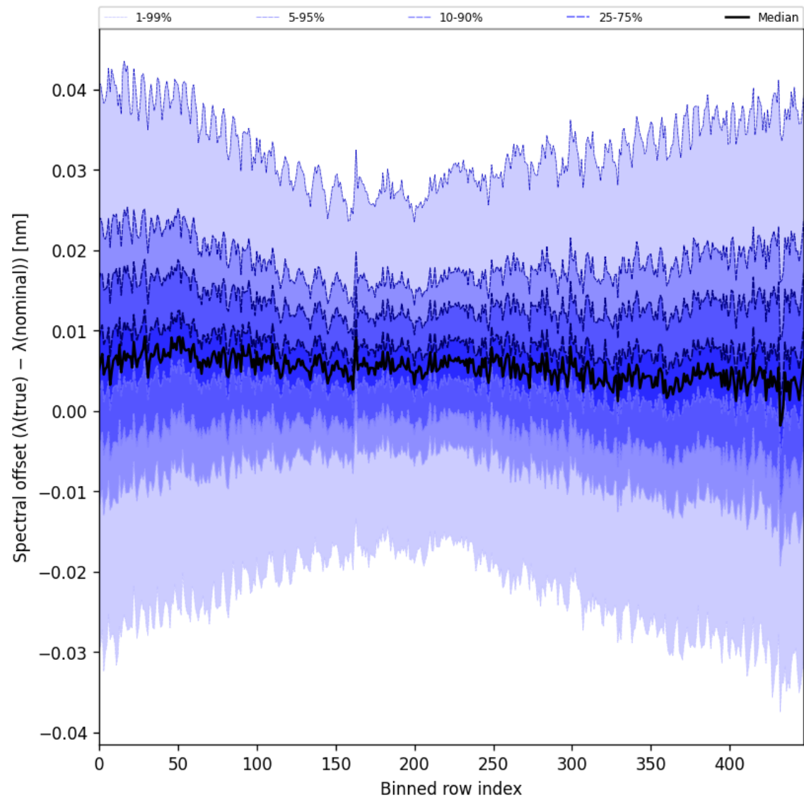
Figure 62: Along track statistics of “Spectral offset ( \lambda_{\text{true}} - \lambda_{\text{nominal}} )” for 2025-09-06 to 2025-09-08
