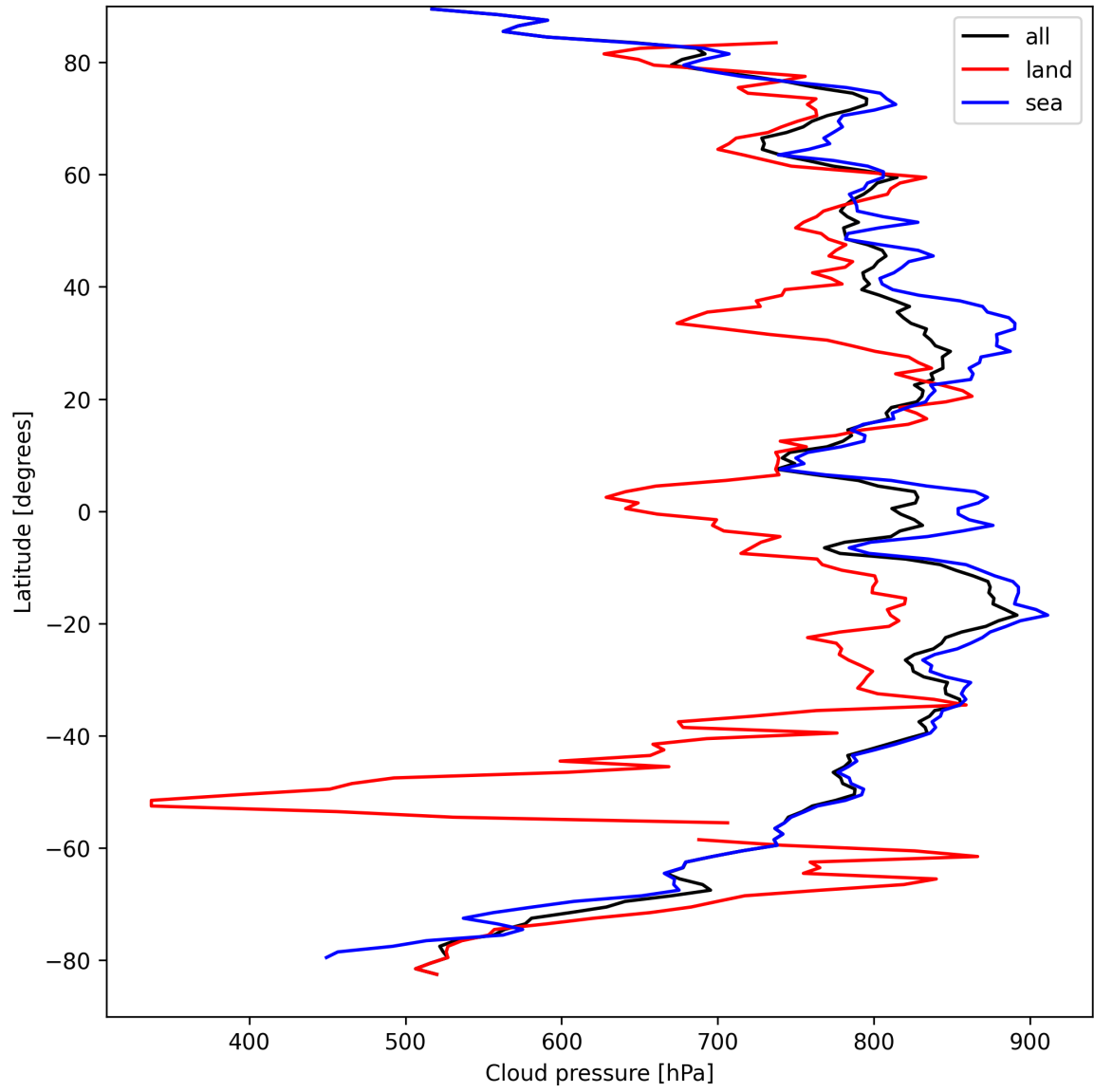
Figure 13: Zonal average of “Cloud pressure” for 2025-09-06 to 2025-09-08.
