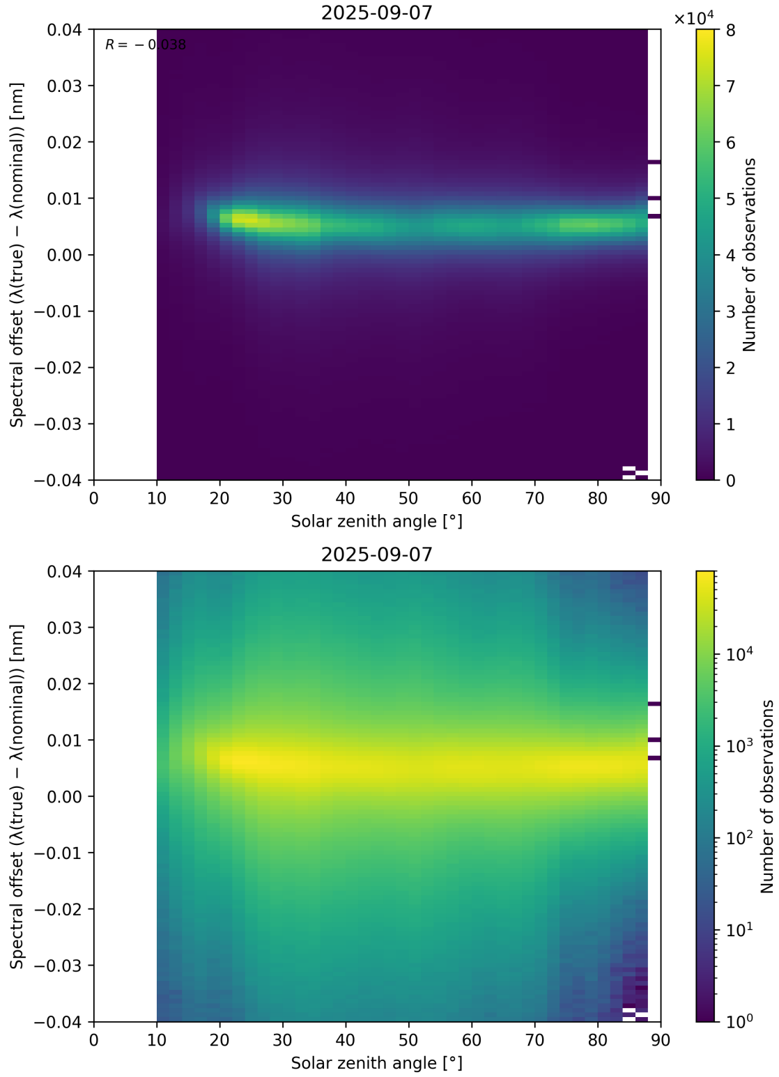
Figure 117: Scatter density plot of “Solar zenith angle” against “Spectral offset ( \lambda_{\text{true}} - \lambda_{\text{nominal}} )” for 2025-09-06 to 2025-09-08.
