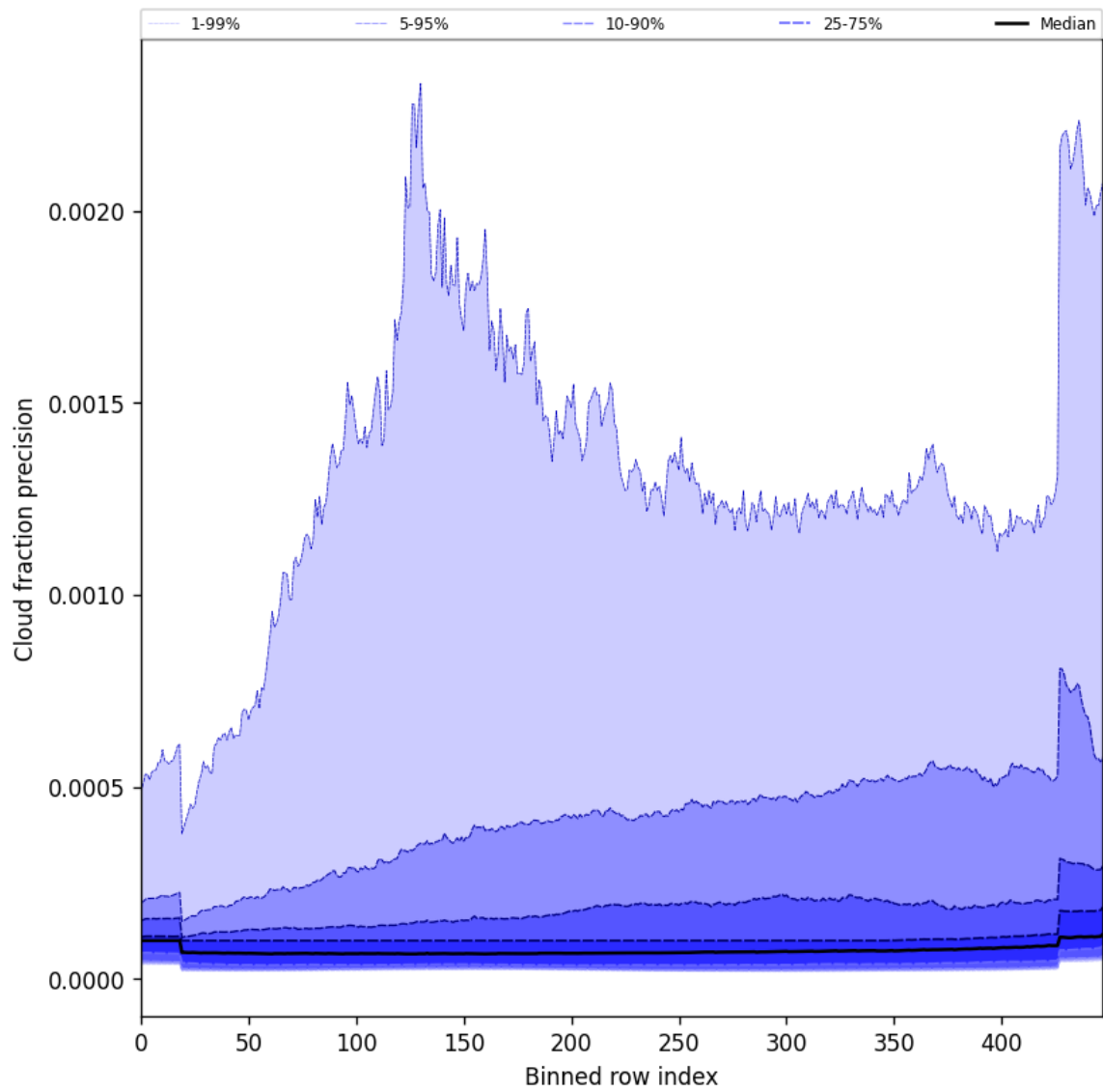
Figure 50: Along track statistics of “Cloud fraction precision” for 2025-09-06 to 2025-09-08
