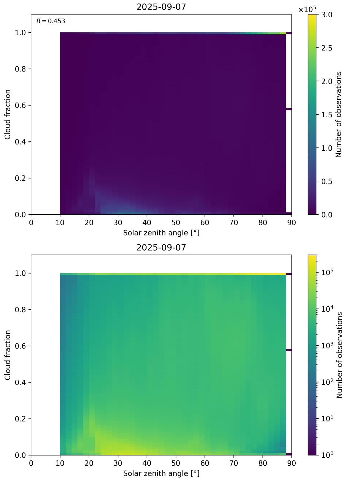
Figure 110: Scatter density plot of “Solar zenith angle” against “Cloud fraction” for 2025-09-06 to 2025-09-08.
