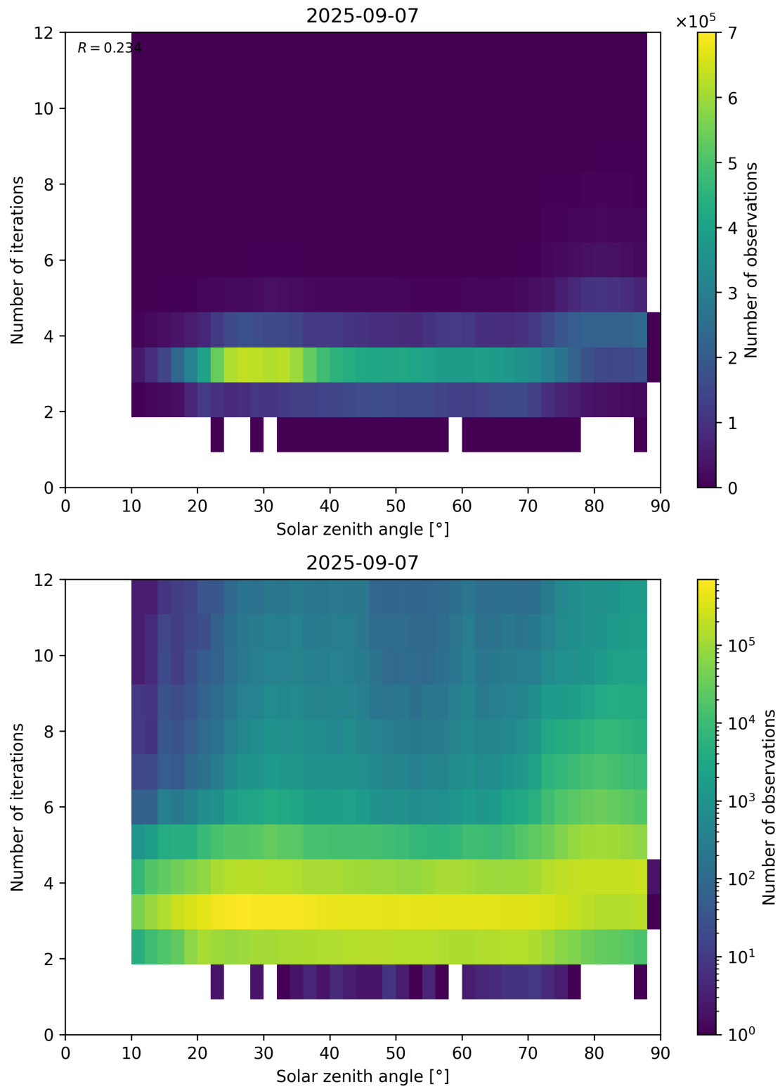
Figure 114: Scatter density plot of “Solar zenith angle” against “Number of iterations” for 2025-09-06 to 2025-09-08.
