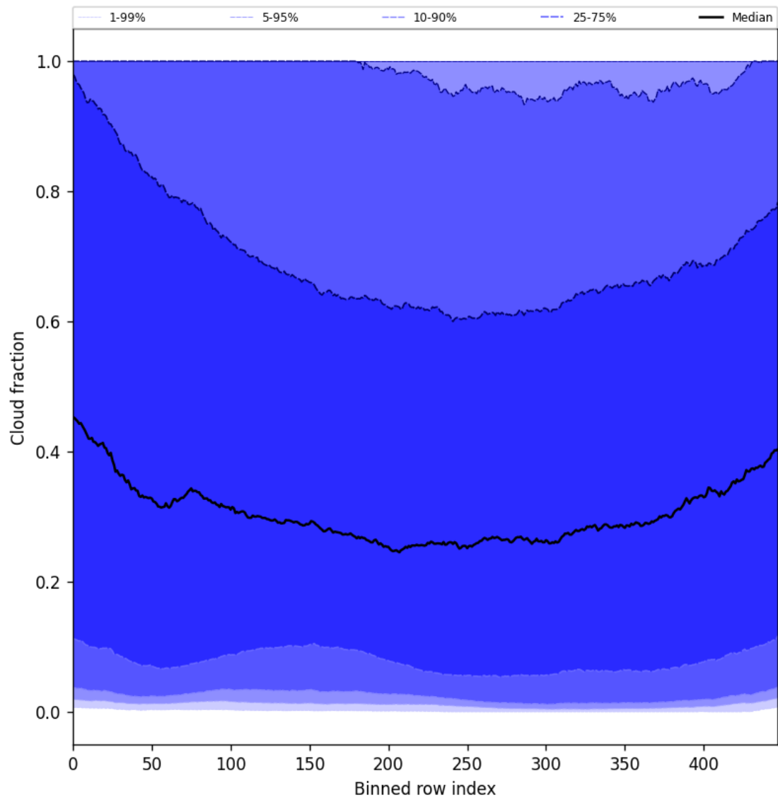
Figure 49: Along track statistics of “Cloud fraction” for 2025-09-06 to 2025-09-08
