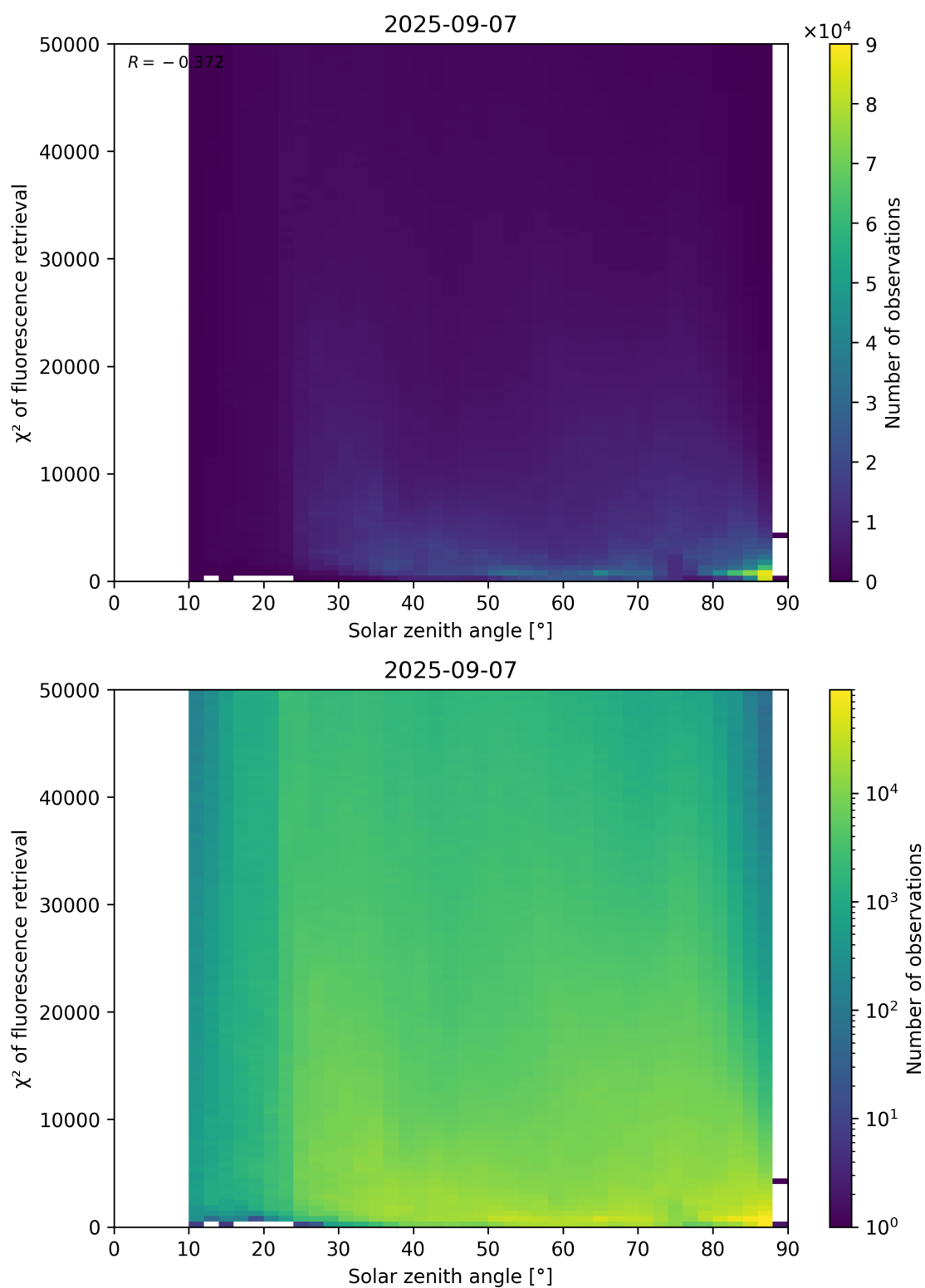
Figure 109: Scatter density plot of “Solar zenith angle” against “ \chi^2 of fluorescence retrieval” for 2025-09-06 to 2025-09-08.
