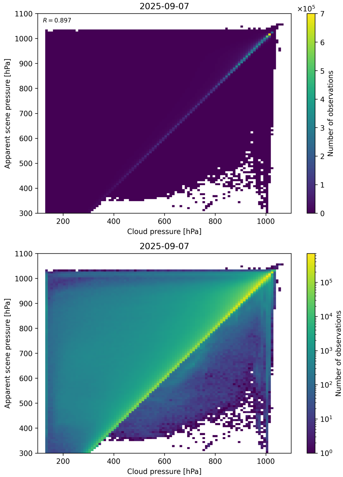
Figure 77: Scatter density plot of “Cloud pressure” against “Apparent scene pressure” for 2025-09-06 to 2025-09-08.
