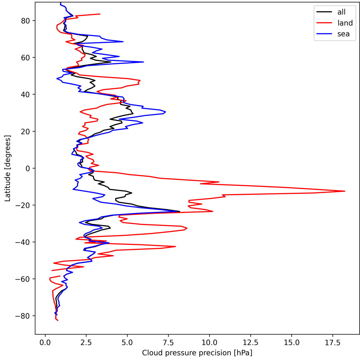
Figure 14: Zonal average of “Cloud pressure precision” for 2025-09-06 to 2025-09-08.
