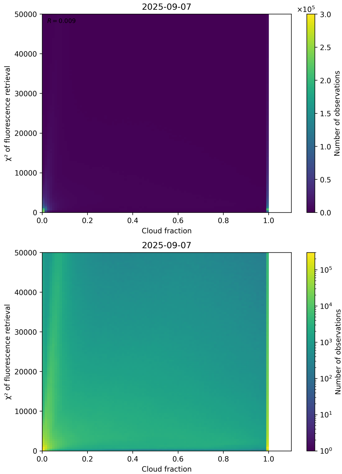
Figure 71: Scatter density plot of “Cloud fraction” against “ \chi^2 of fluorescence retrieval” for 2025-09-06 to 2025-09-08.
