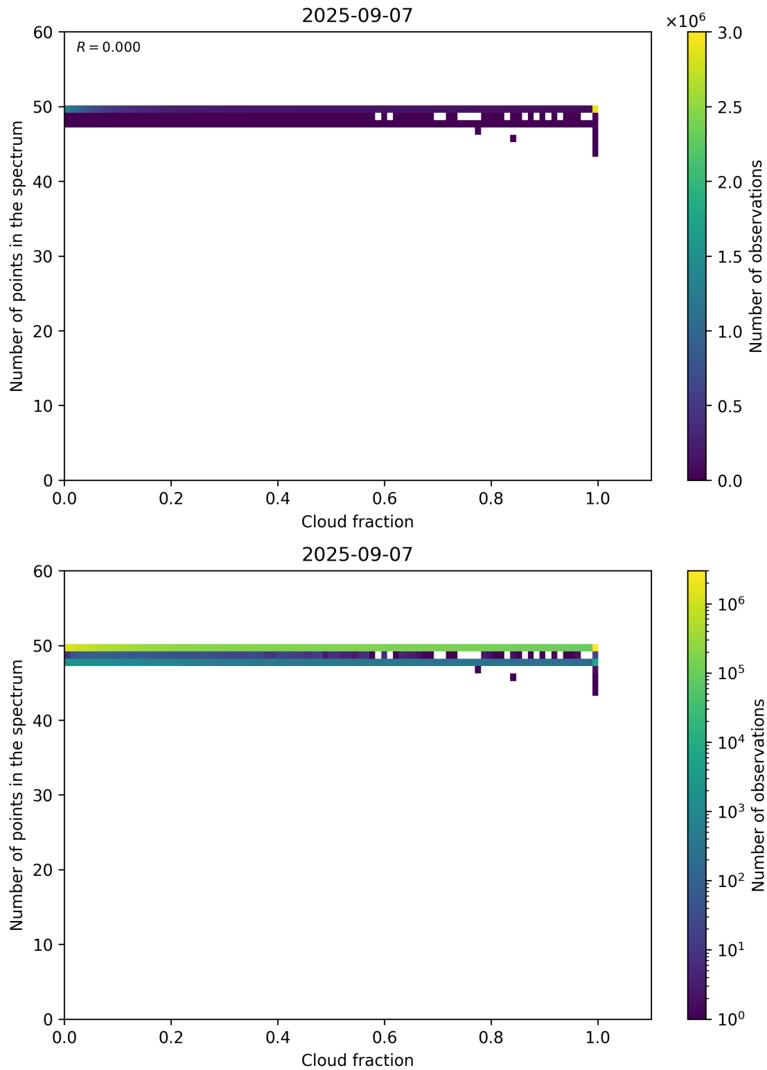
Figure 74: Scatter density plot of “Cloud fraction” against “Number of points in the spectrum” for 2025-09-06 to 2025-09-08.
