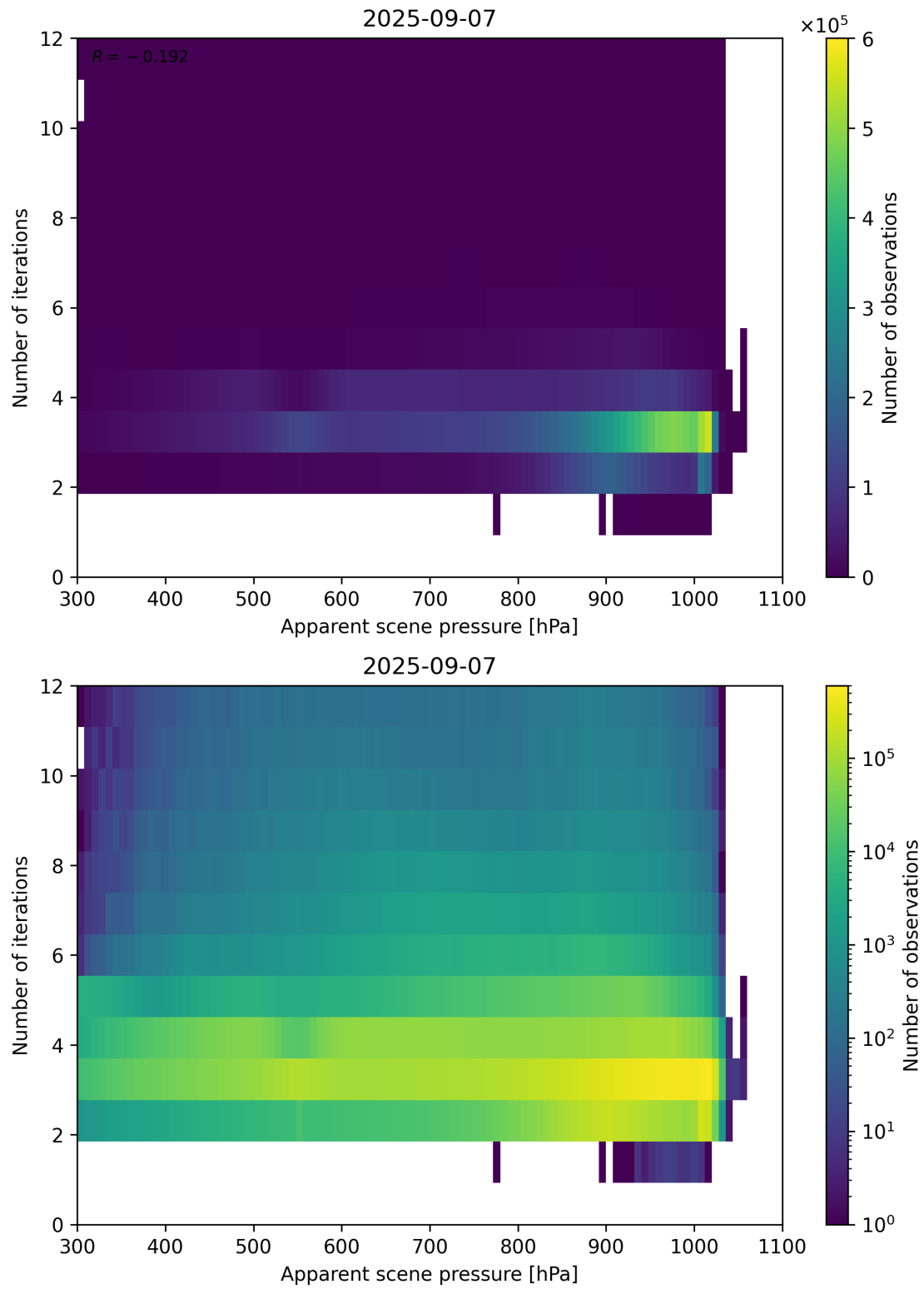
Figure 65: Scatter density plot of “Apparent scene pressure” against “Number of iterations” for 2025-09-06 to 2025-09-08.
