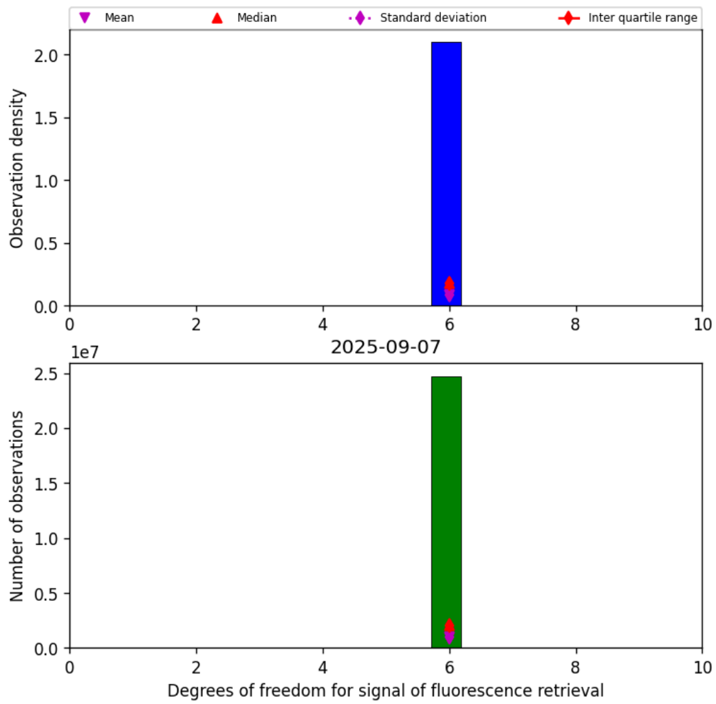
Figure 43: Histogram of “Degrees of freedom for signal of fluorescence retrieval” for 2025-09-06 to 2025-09-08
