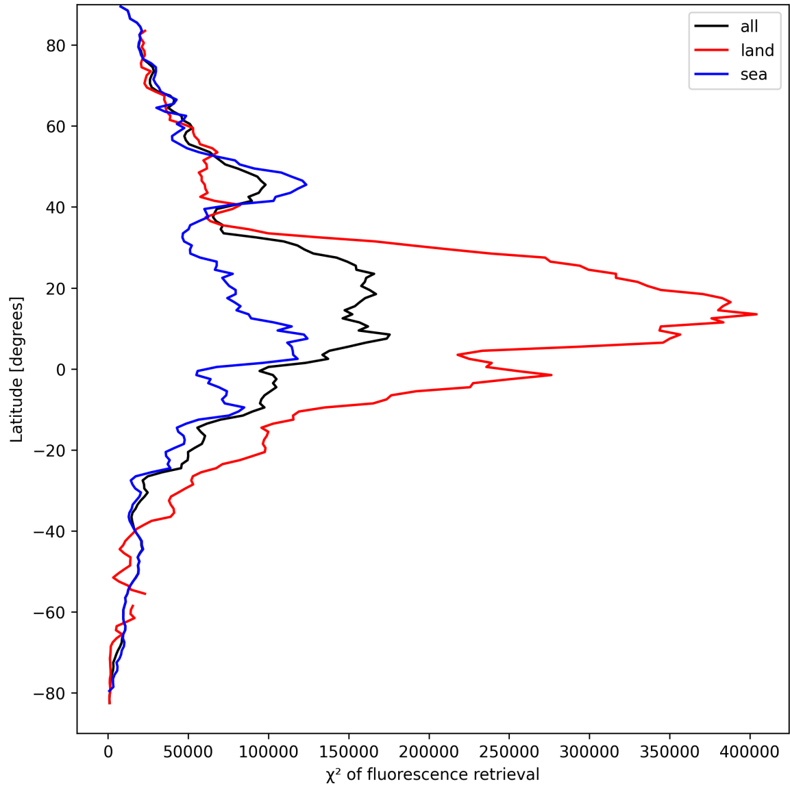
Figure 25: Zonal average of “ \chi^2 of fluorescence retrieval” for 2025-09-06 to 2025-09-08.
