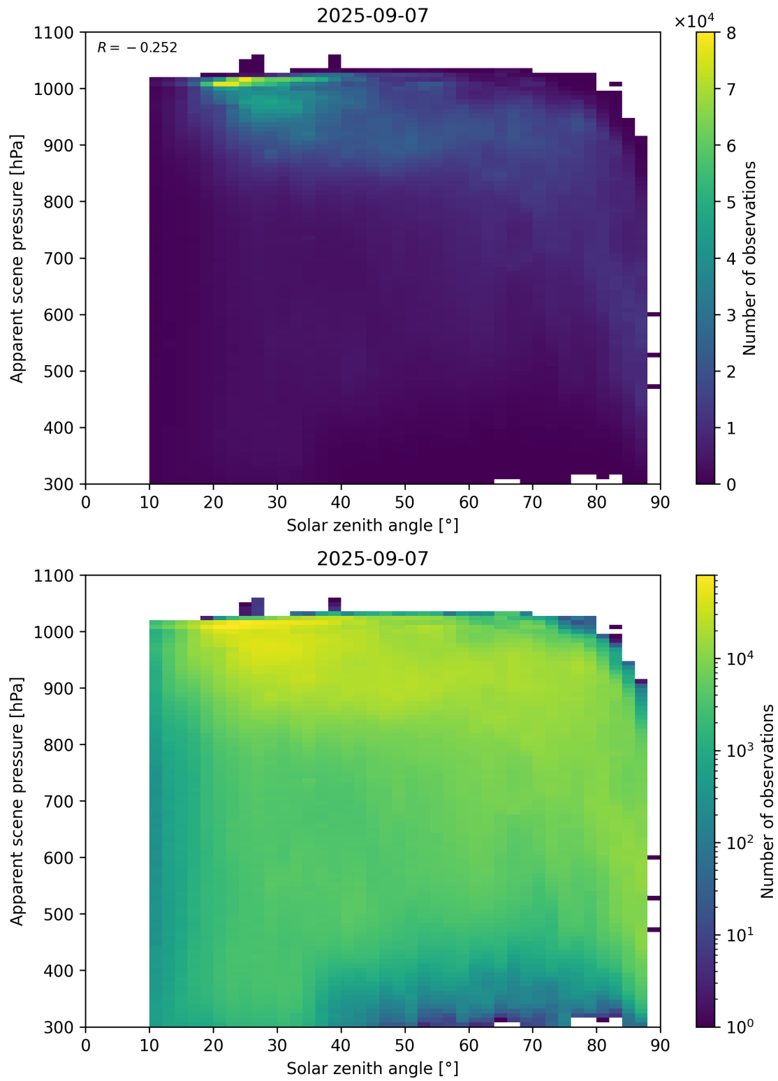
Figure 108: Scatter density plot of “Solar zenith angle” against “Apparent scene pressure” for 2025-09-06 to 2025-09-08.
