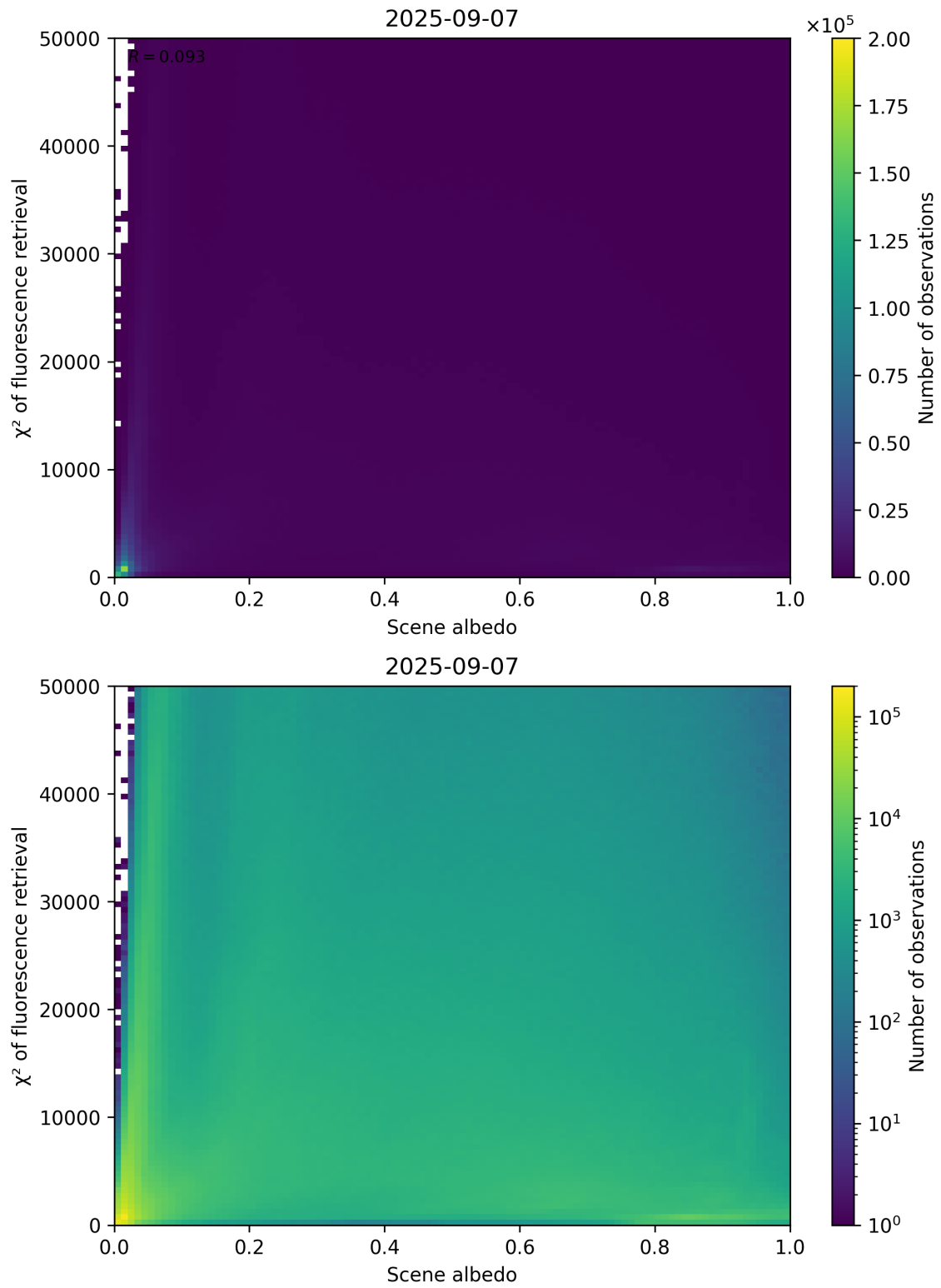
Figure 103: Scatter density plot of “Scene albedo” against “ \chi^2 of fluorescence retrieval” for 2025-09-06 to 2025-09-08.
