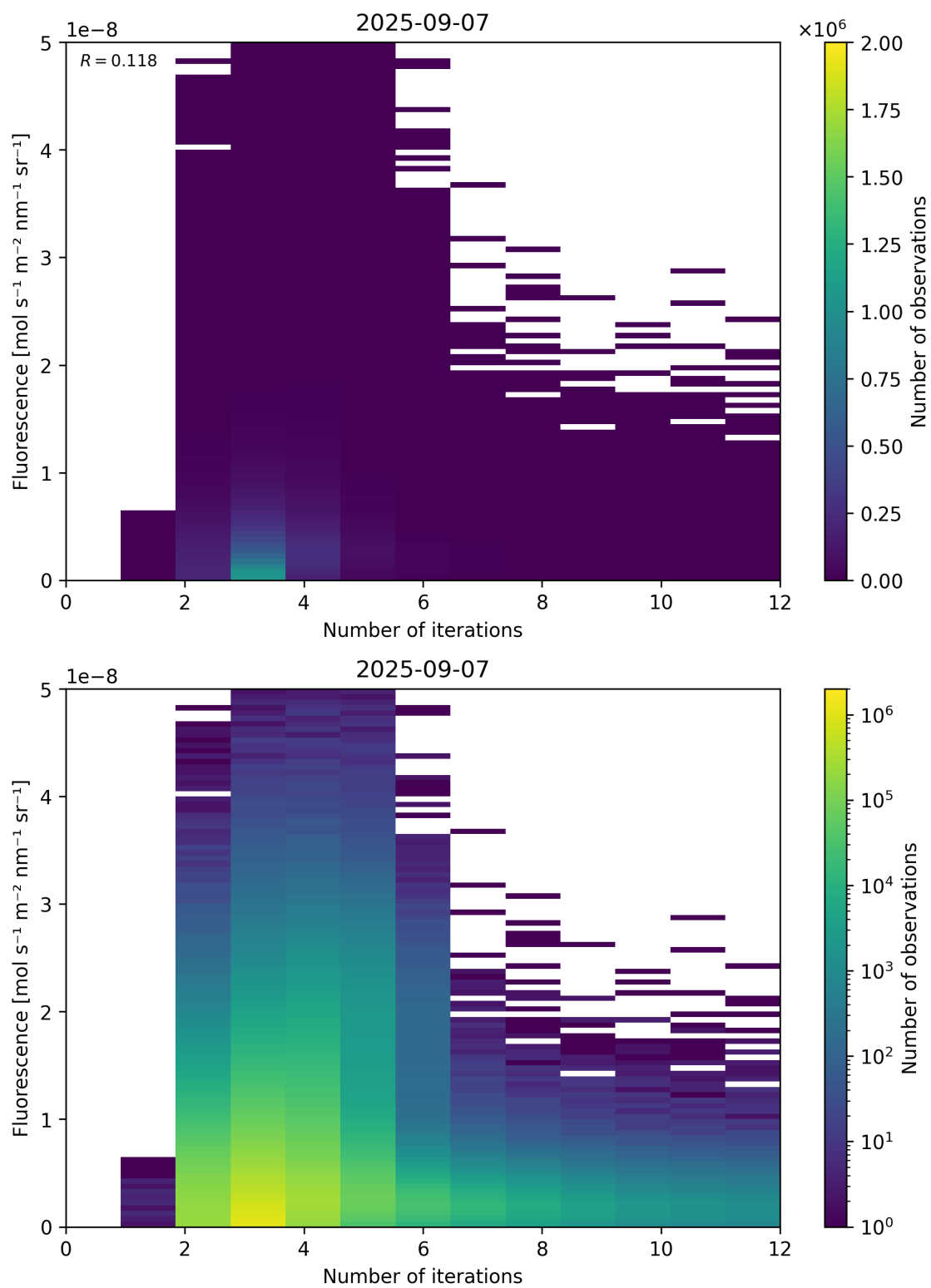
Figure 98: Scatter density plot of “Number of iterations” against “Fluorescence” for 2025-09-06 to 2025-09-08.
