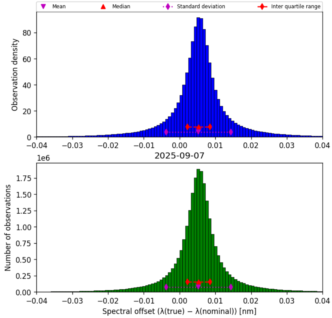
Figure 45: Histogram of “Spectral offset ( \lambda_{\text{true}} - \lambda_{\text{nominal}} )” for 2025-09-06 to 2025-09-08
