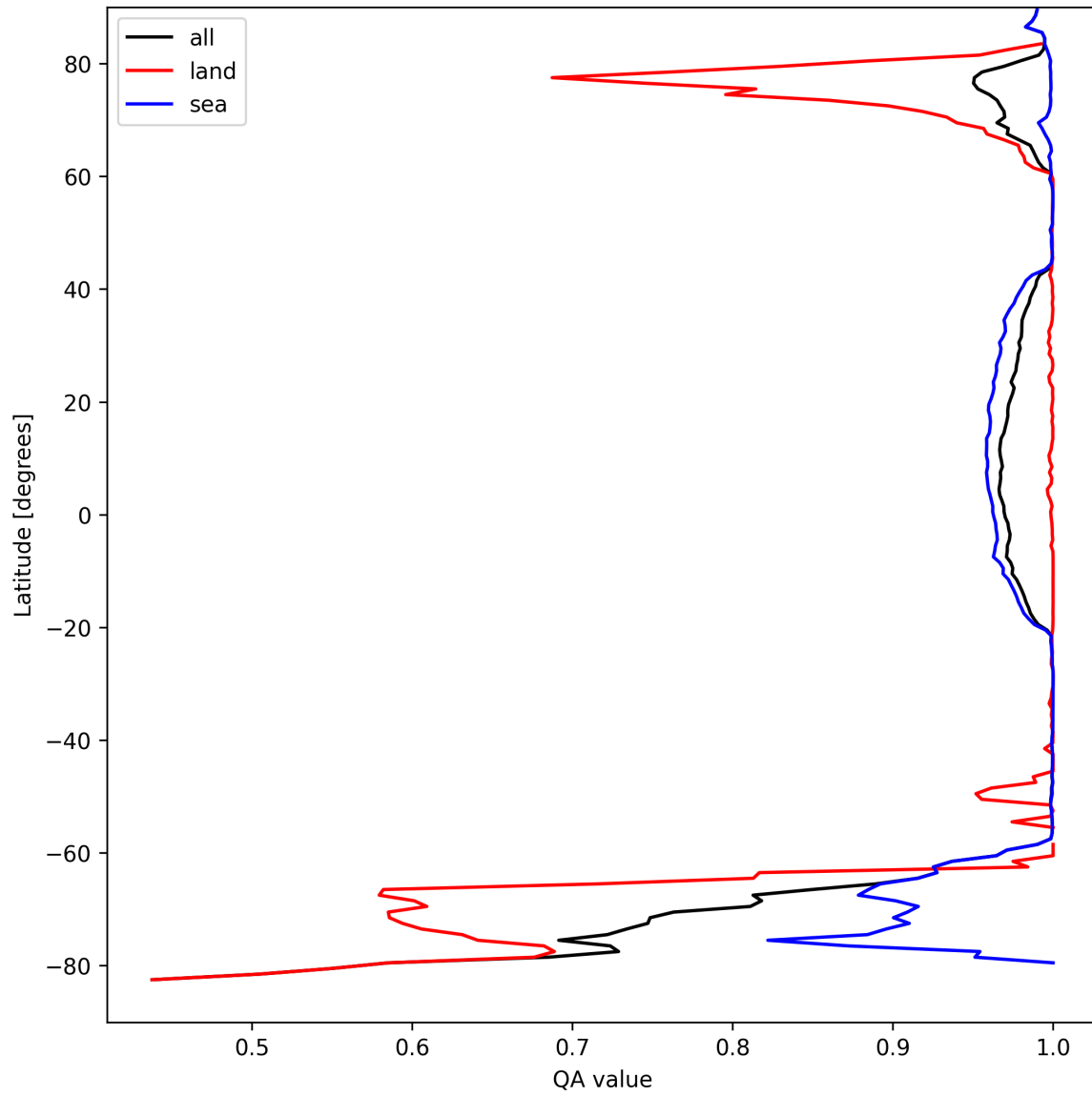
Figure 12: Zonal average of “QA value” for 2025-09-06 to 2025-09-08.
