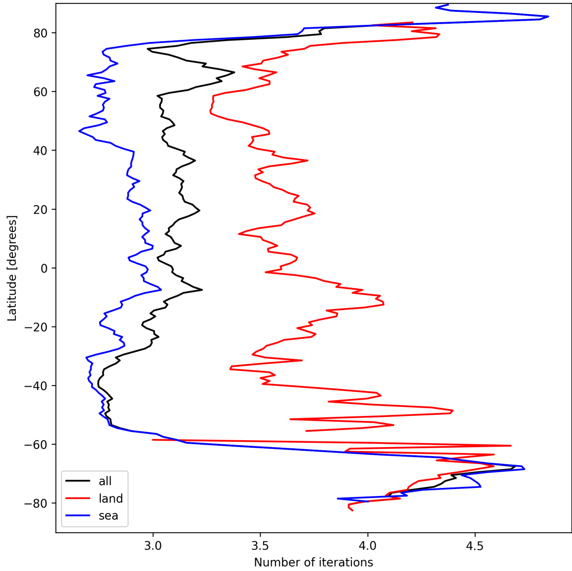
Figure 22: Zonal average of “Number of iterations” for 2025-09-06 to 2025-09-08.
