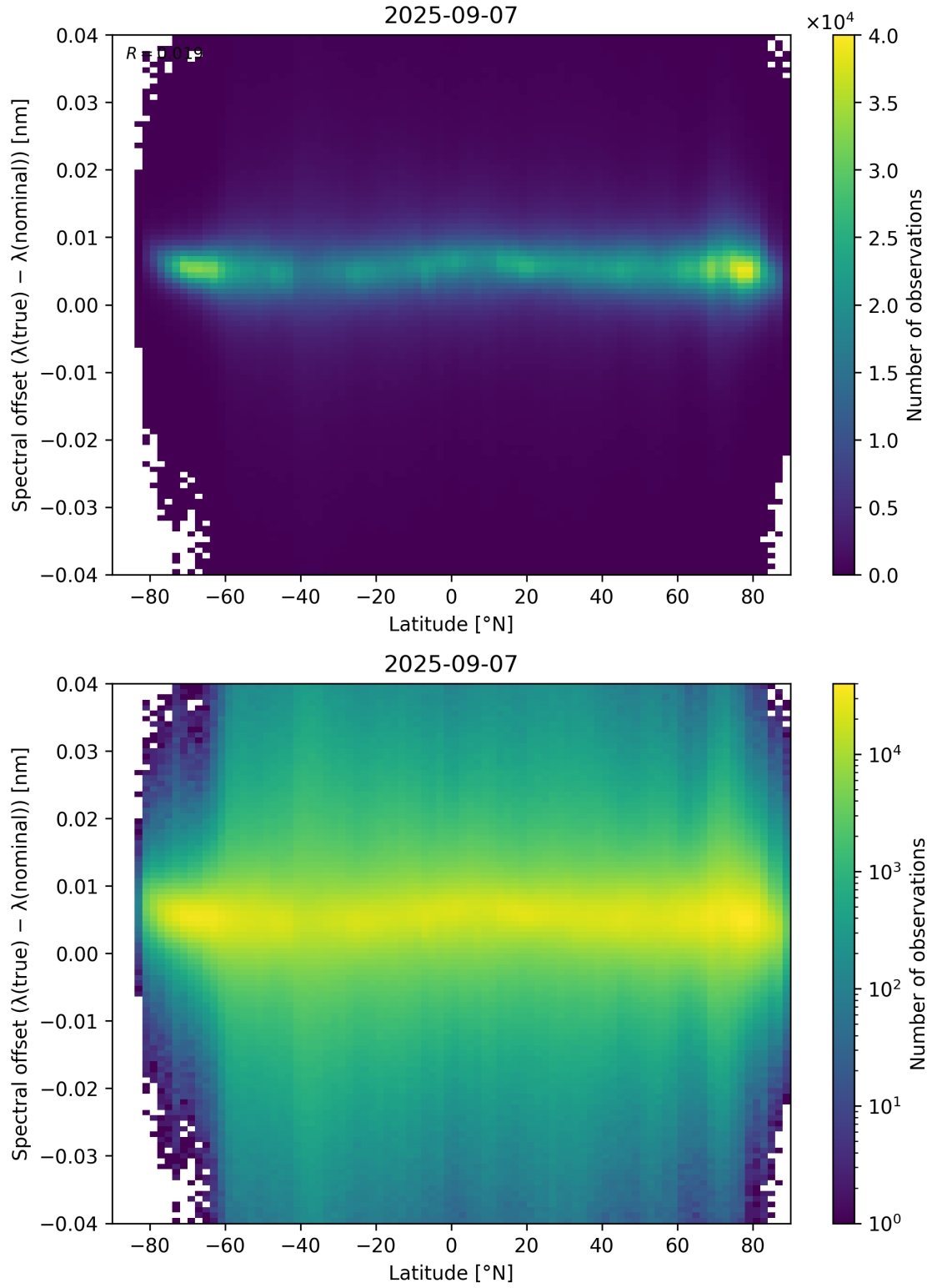
Figure 96: Scatter density plot of “Latitude” against “Spectral offset ( \lambda_{\text{true}} - \lambda_{\text{nominal}} )” for 2025-09-06 to 2025-09-08.
