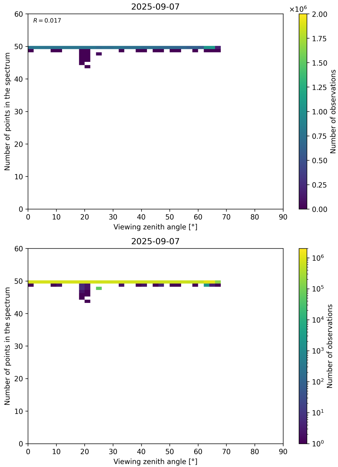
Figure 125: Scatter density plot of “Viewing zenith angle” against “Number of points in the spectrum” for 2025-09-06 to 2025-09-08.
