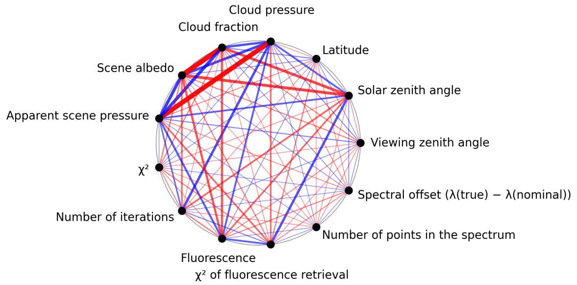
Figure 1: Map of correlation graph for 2025-09-06 to 2025-09-08.
