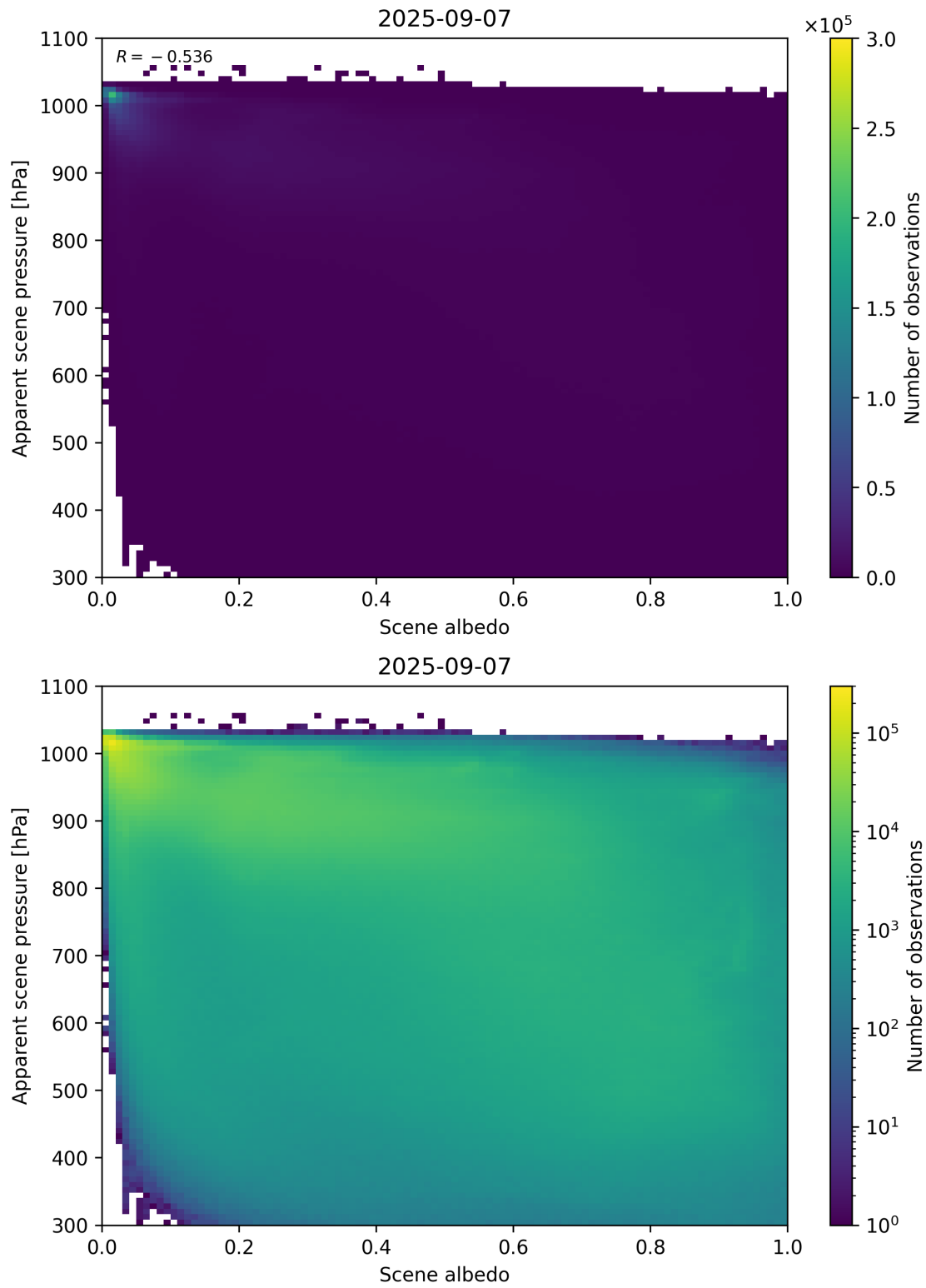
Figure 102: Scatter density plot of “Scene albedo” against “Apparent scene pressure” for 2025-09-06 to 2025-09-08.
