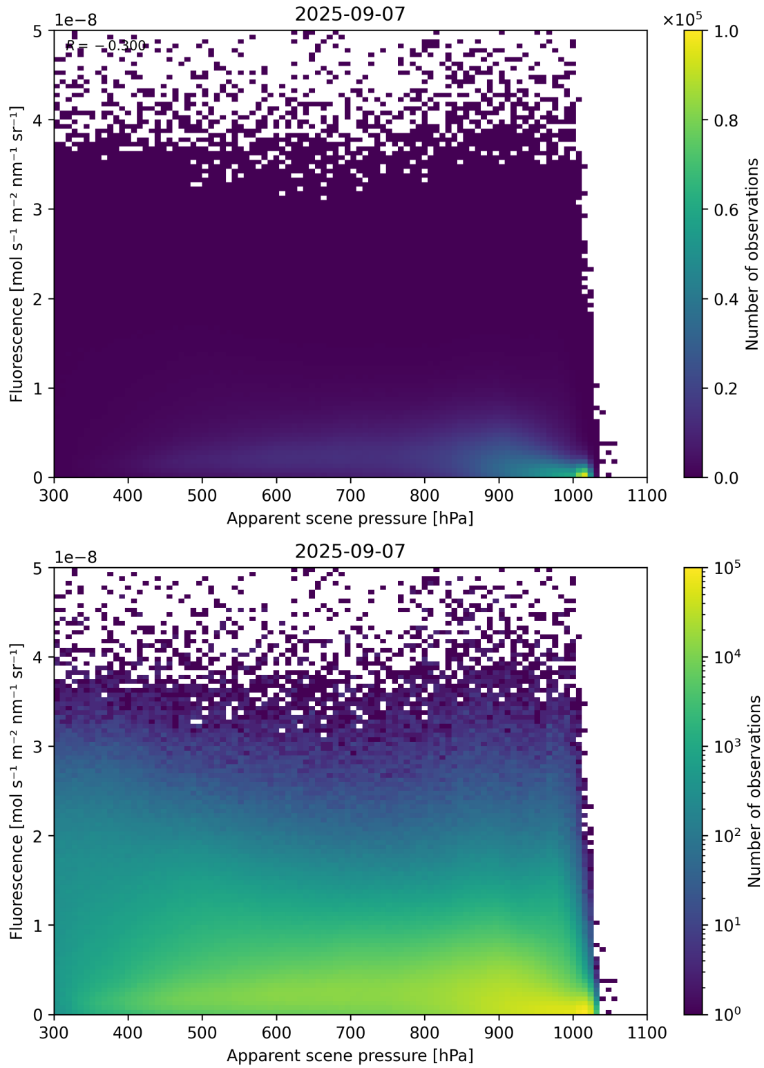
Figure 64: Scatter density plot of “Apparent scene pressure” against “Fluorescence” for 2025-09-06 to 2025-09-08.
