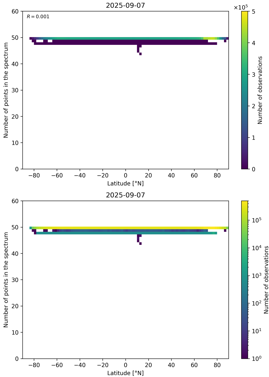
Figure 94: Scatter density plot of “Latitude” against “Number of points in the spectrum” for 2025-09-06 to 2025-09-08.
