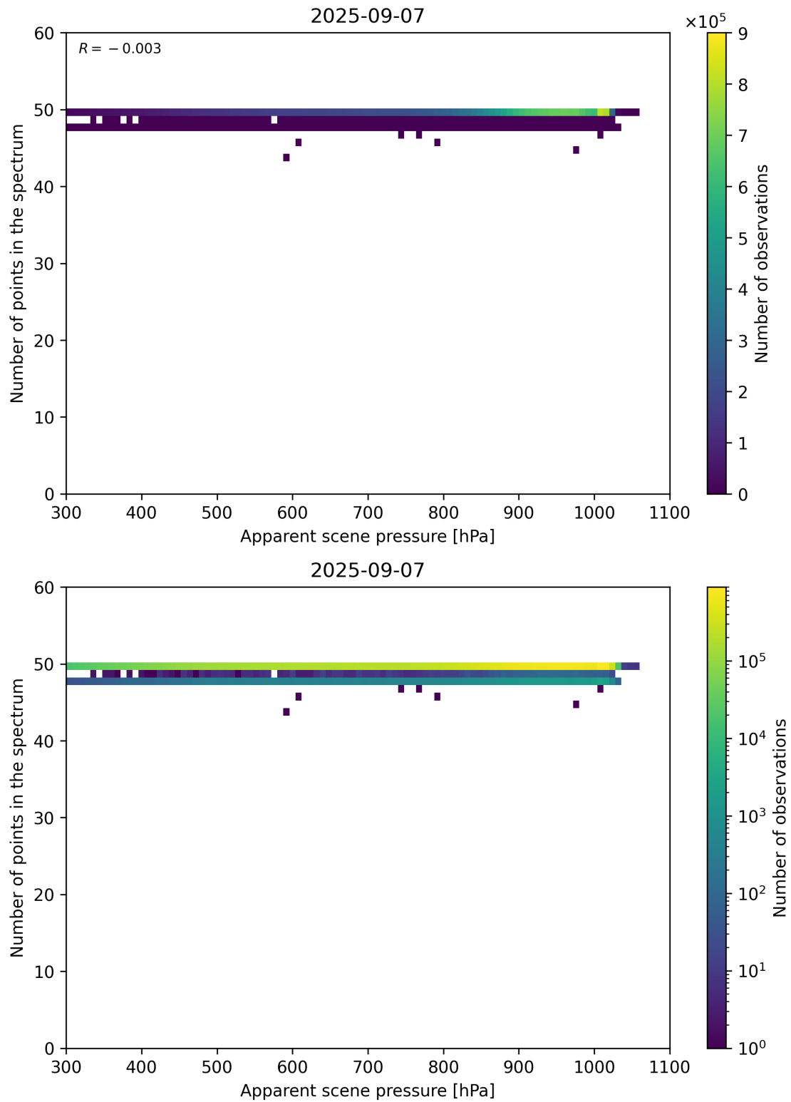
Figure 66: Scatter density plot of “Apparent scene pressure” against “Number of points in the spectrum” for 2025-09-06 to 2025-09-08.
