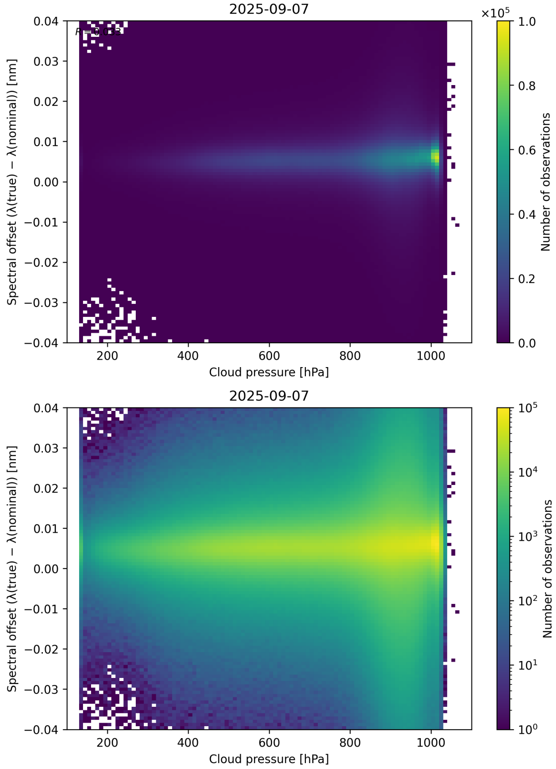
Figure 84: Scatter density plot of “Cloud pressure” against “Spectral offset ( \lambda_{\text{true}} - \lambda_{\text{nominal}} )” for 2025-09-06 to 2025-09-08.
