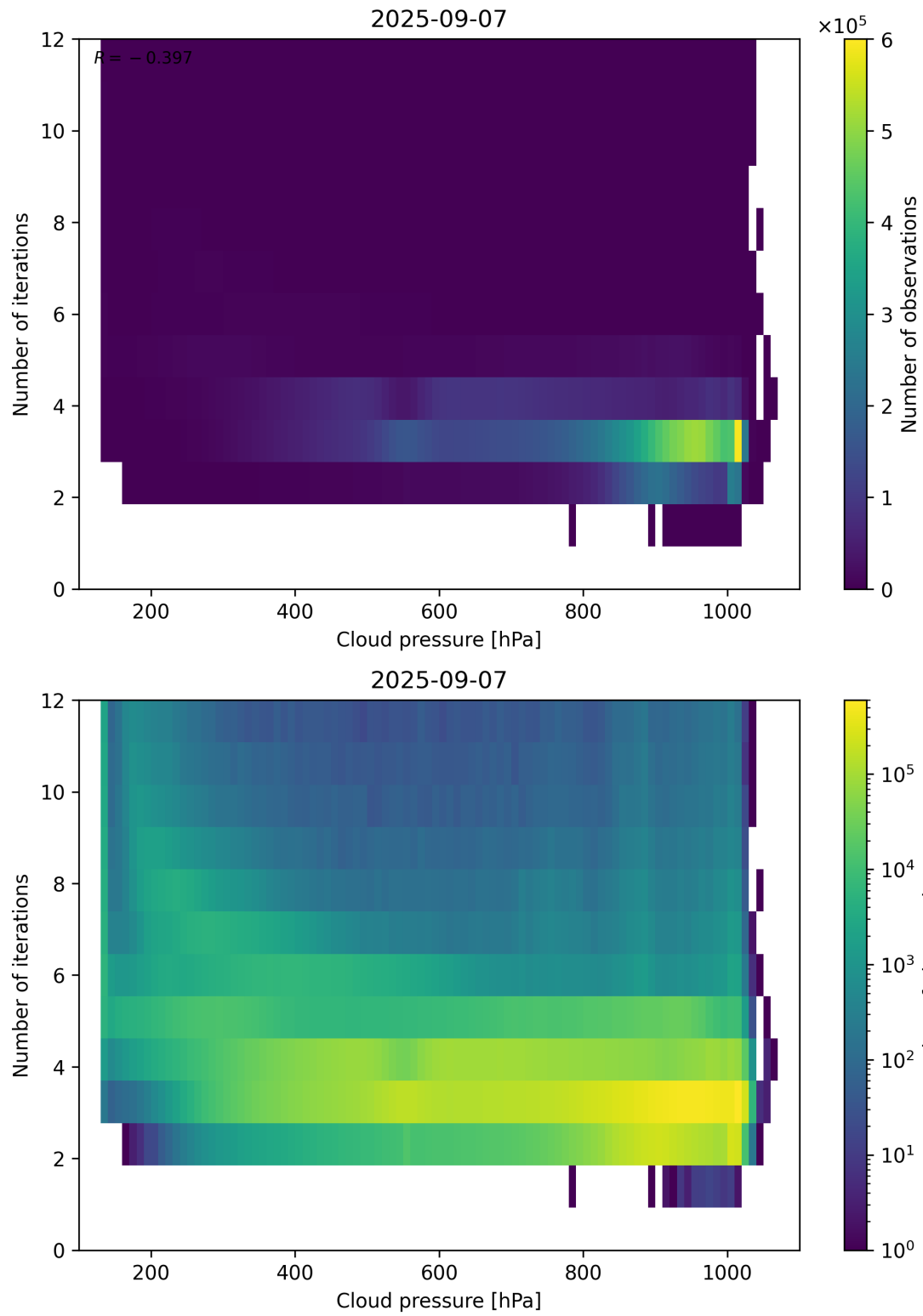
Figure 81: Scatter density plot of “Cloud pressure” against “Number of iterations” for 2025-09-06 to 2025-09-08.
