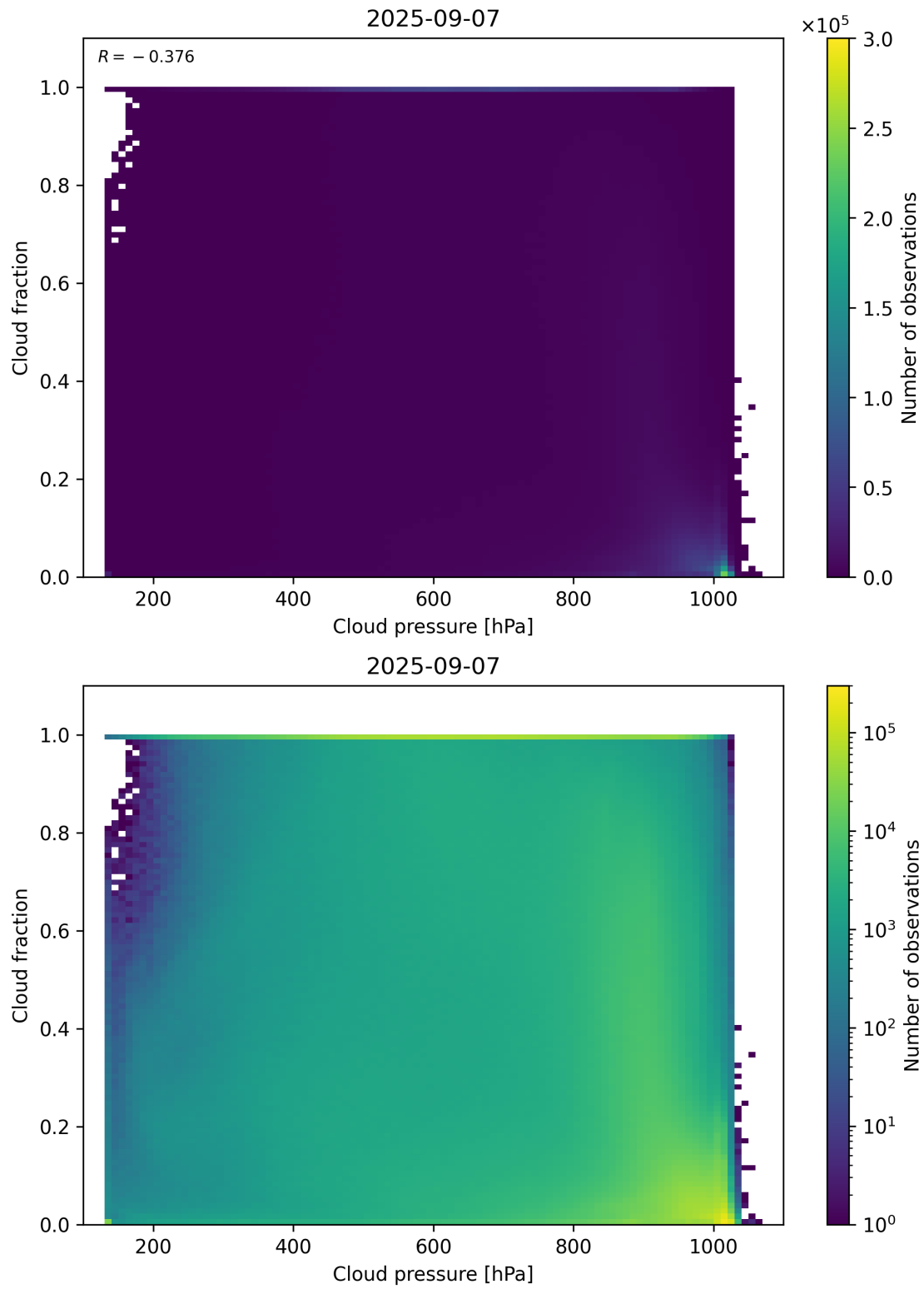
Figure 79: Scatter density plot of “Cloud pressure” against “Cloud fraction” for 2025-09-06 to 2025-09-08.
