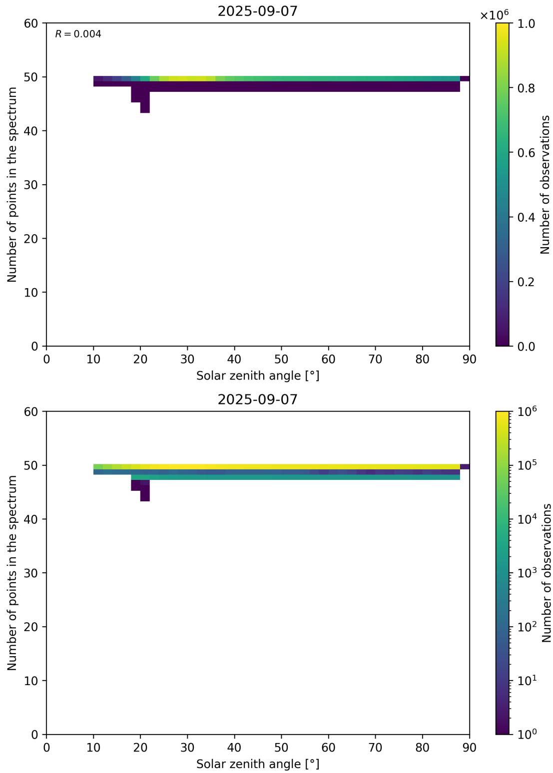
Figure 115: Scatter density plot of “Solar zenith angle” against “Number of points in the spectrum” for 2025-09-06 to 2025-09-08.
