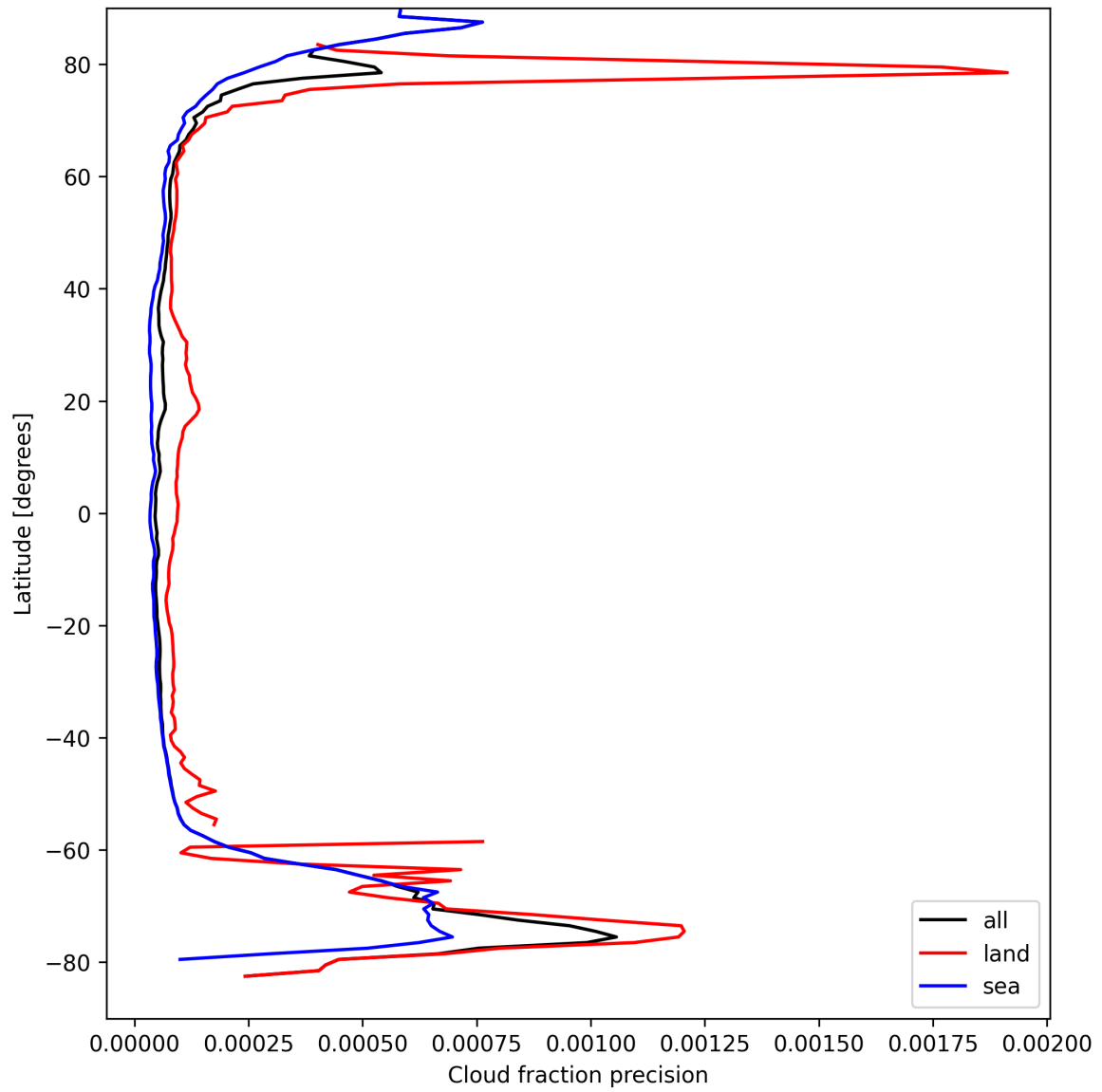
Figure 16: Zonal average of “Cloud fraction precision” for 2025-09-06 to 2025-09-08.
