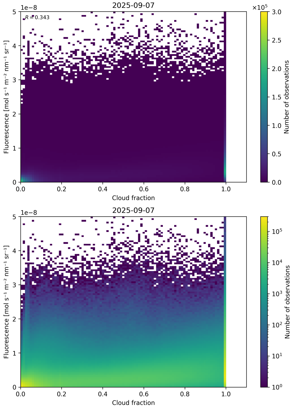
Figure 72: Scatter density plot of “Cloud fraction” against “Fluorescence” for 2025-09-06 to 2025-09-08.
