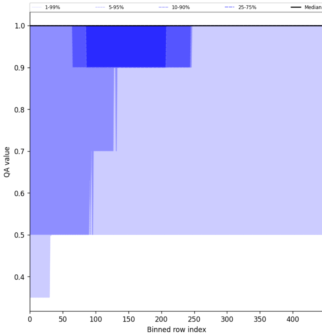
Figure 46: Along track statistics of “QA value” for 2025-09-06 to 2025-09-08
