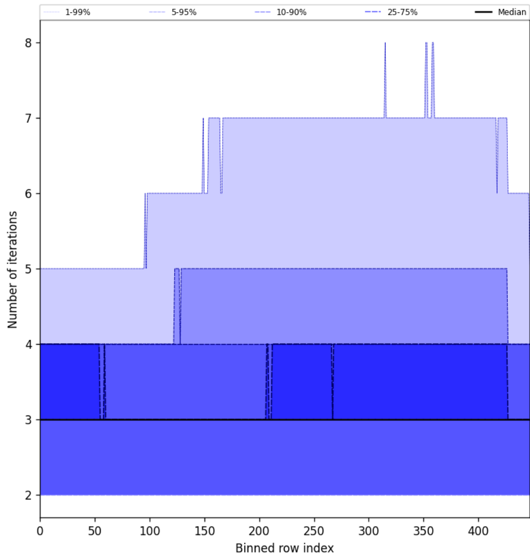
Figure 56: Along track statistics of “Number of iterations” for 2025-09-06 to 2025-09-08
