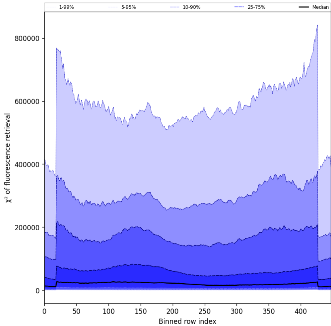
Figure 59: Along track statistics of “ \chi^2 of fluorescence retrieval” for 2025-09-06 to 2025-09-08
