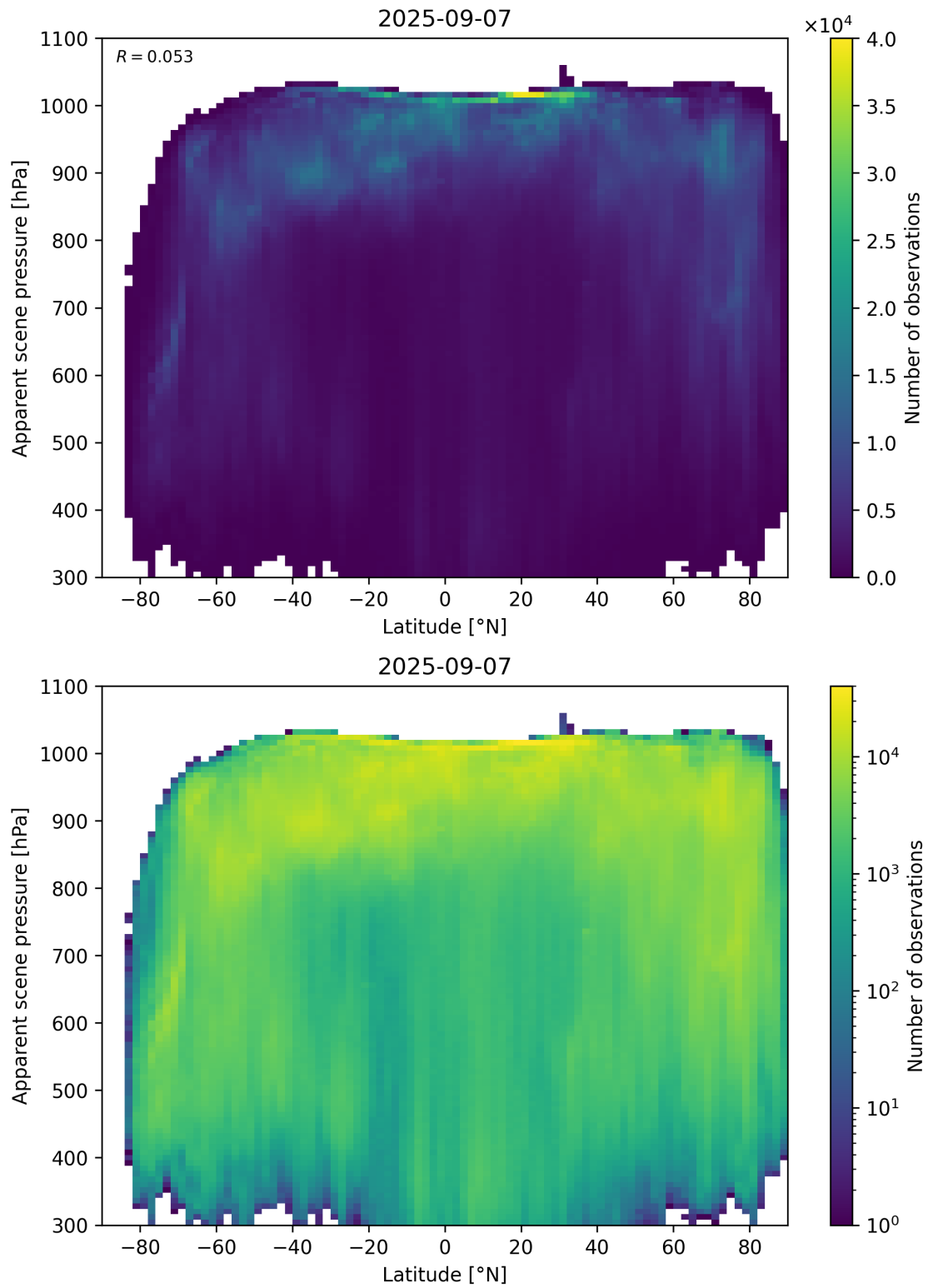
Figure 88: Scatter density plot of “Latitude” against “Apparent scene pressure” for 2025-09-06 to 2025-09-08.
