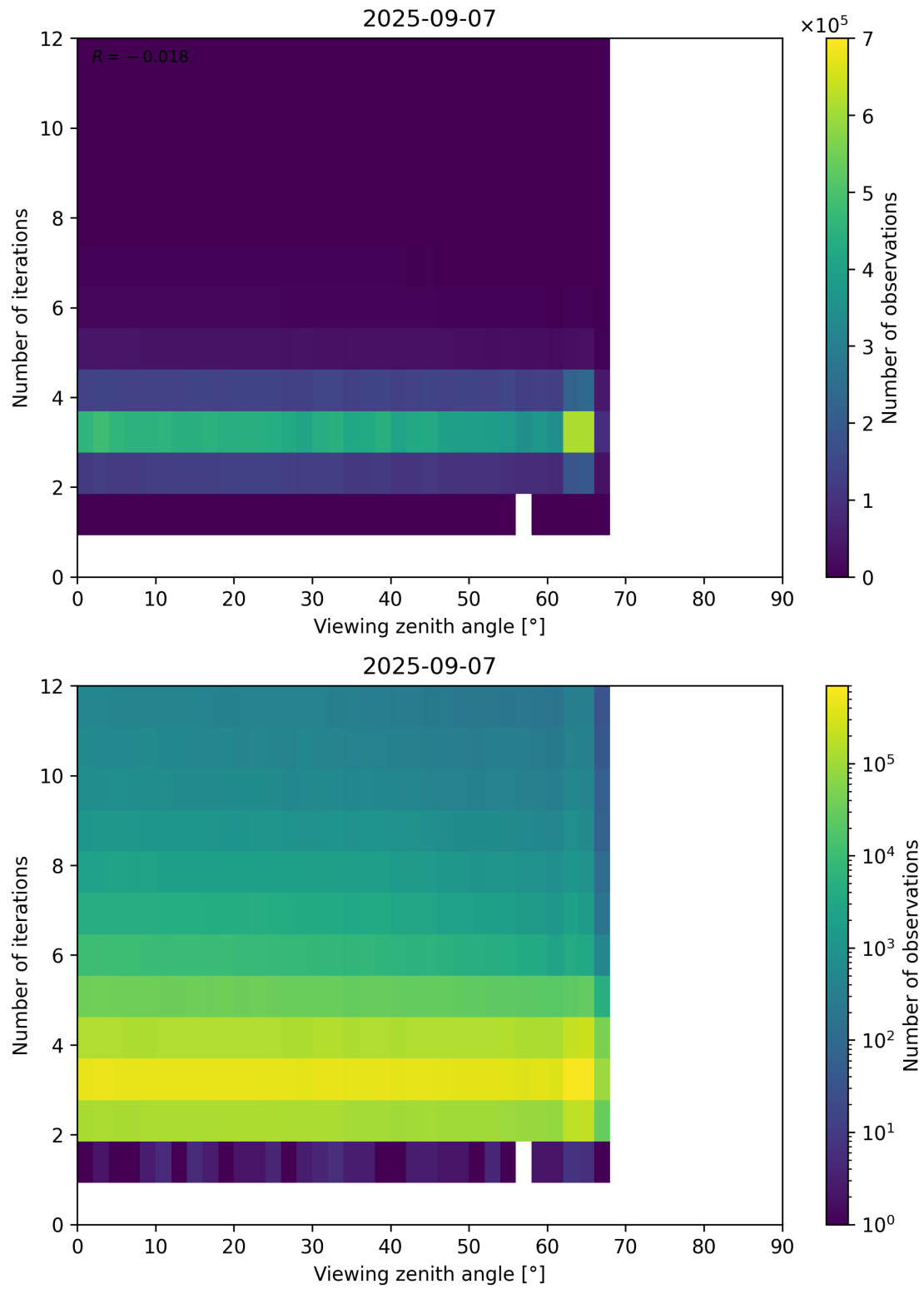
Figure 124: Scatter density plot of “Viewing zenith angle” against “Number of iterations” for 2025-09-06 to 2025-09-08.
