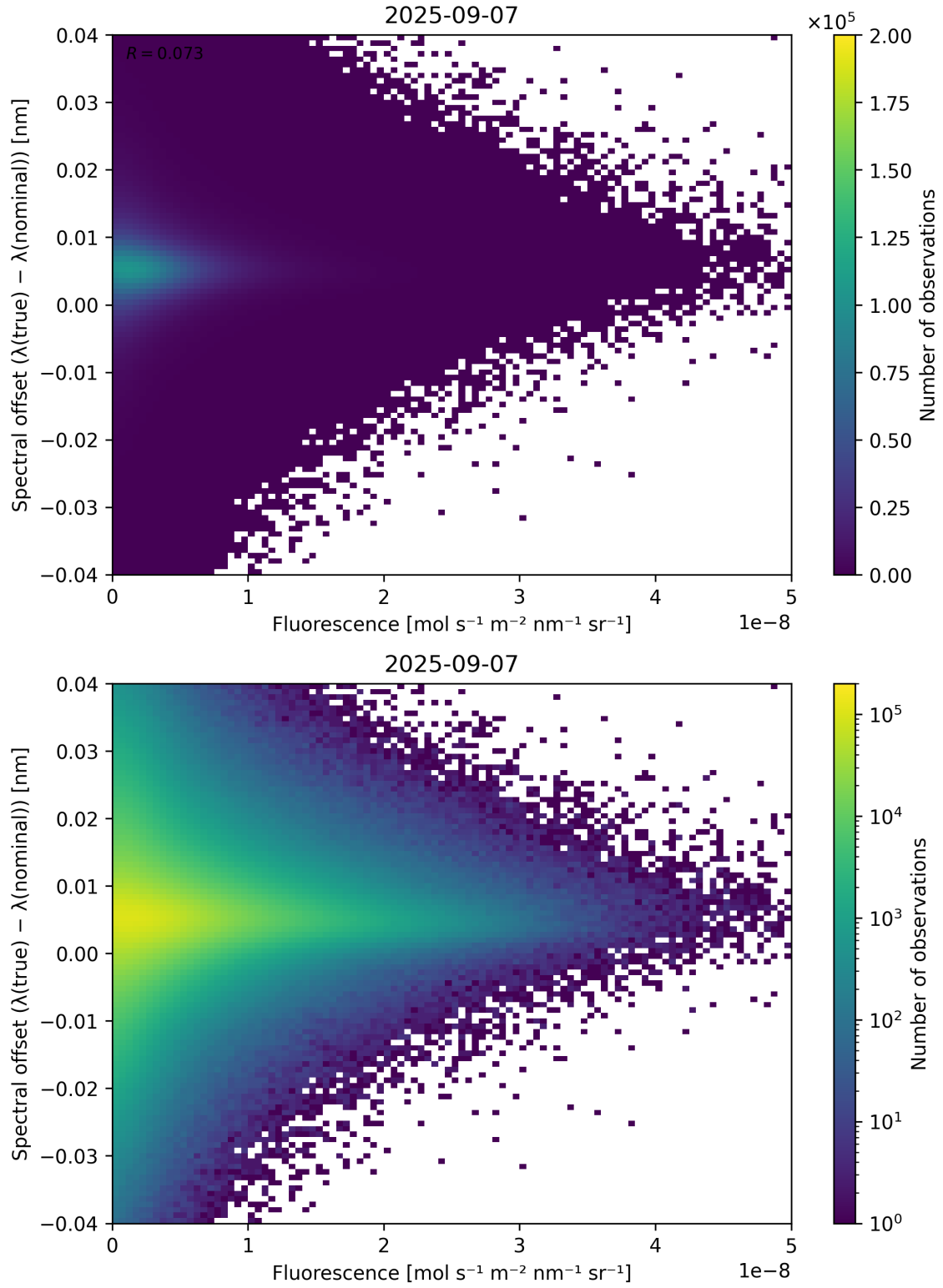
Figure 87: Scatter density plot of “Fluorescence” against “Spectral offset ( \lambda_{\text{true}} - \lambda_{\text{nominal}} )” for 2025-09-06 to 2025-09-08.
