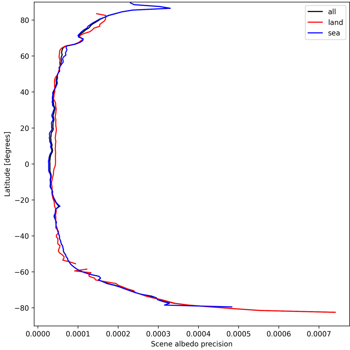
Figure 18: Zonal average of “Scene albedo precision” for 2025-09-06 to 2025-09-08.
