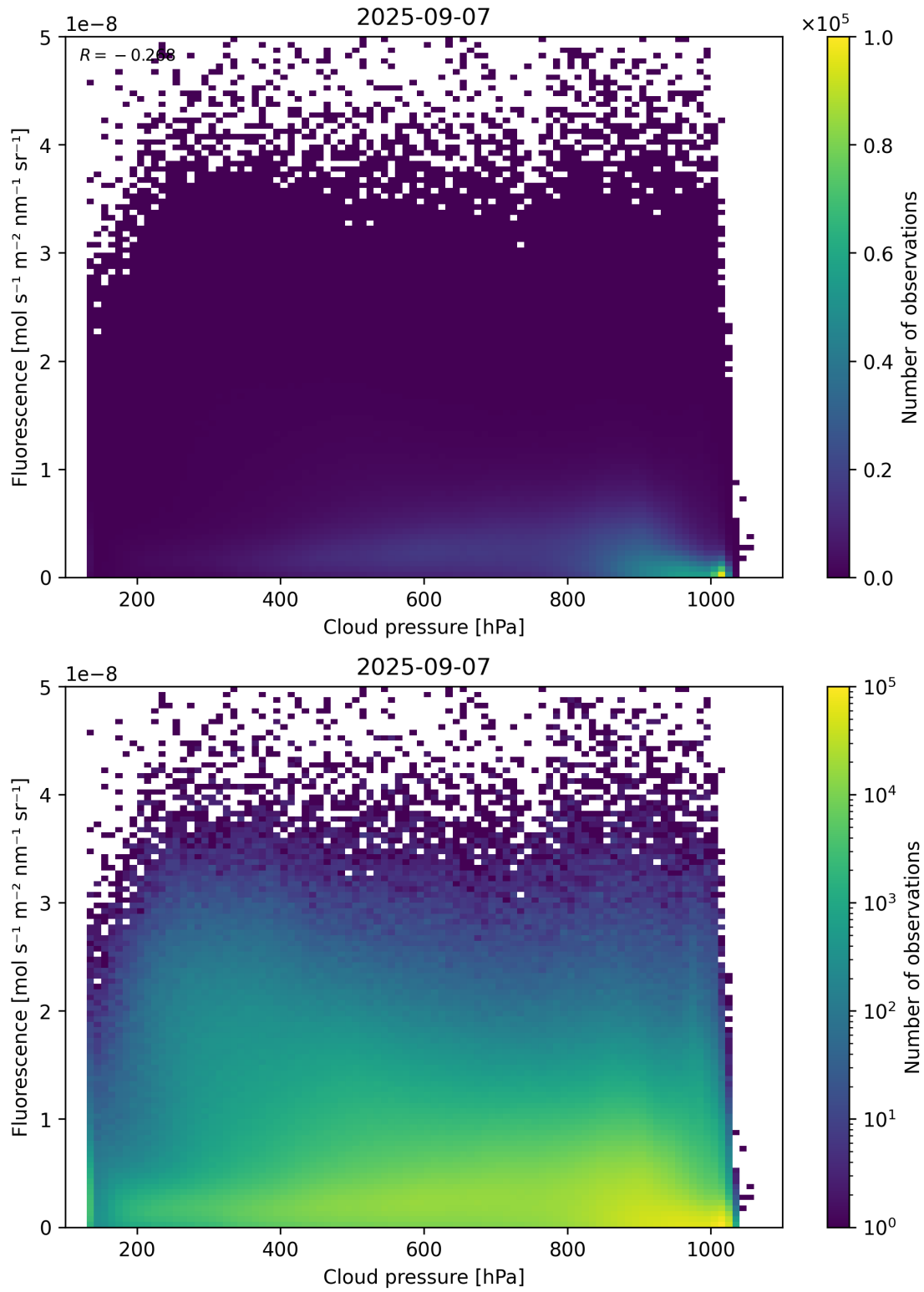
Figure 80: Scatter density plot of “Cloud pressure” against “Fluorescence” for 2025-09-06 to 2025-09-08.
