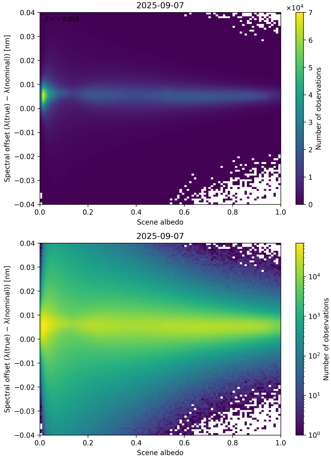
Figure 107: Scatter density plot of “Scene albedo” against “Spectral offset ( \lambda_{\text{true}} - \lambda_{\text{nominal}} )” for 2025-09-06 to 2025-09-08.
