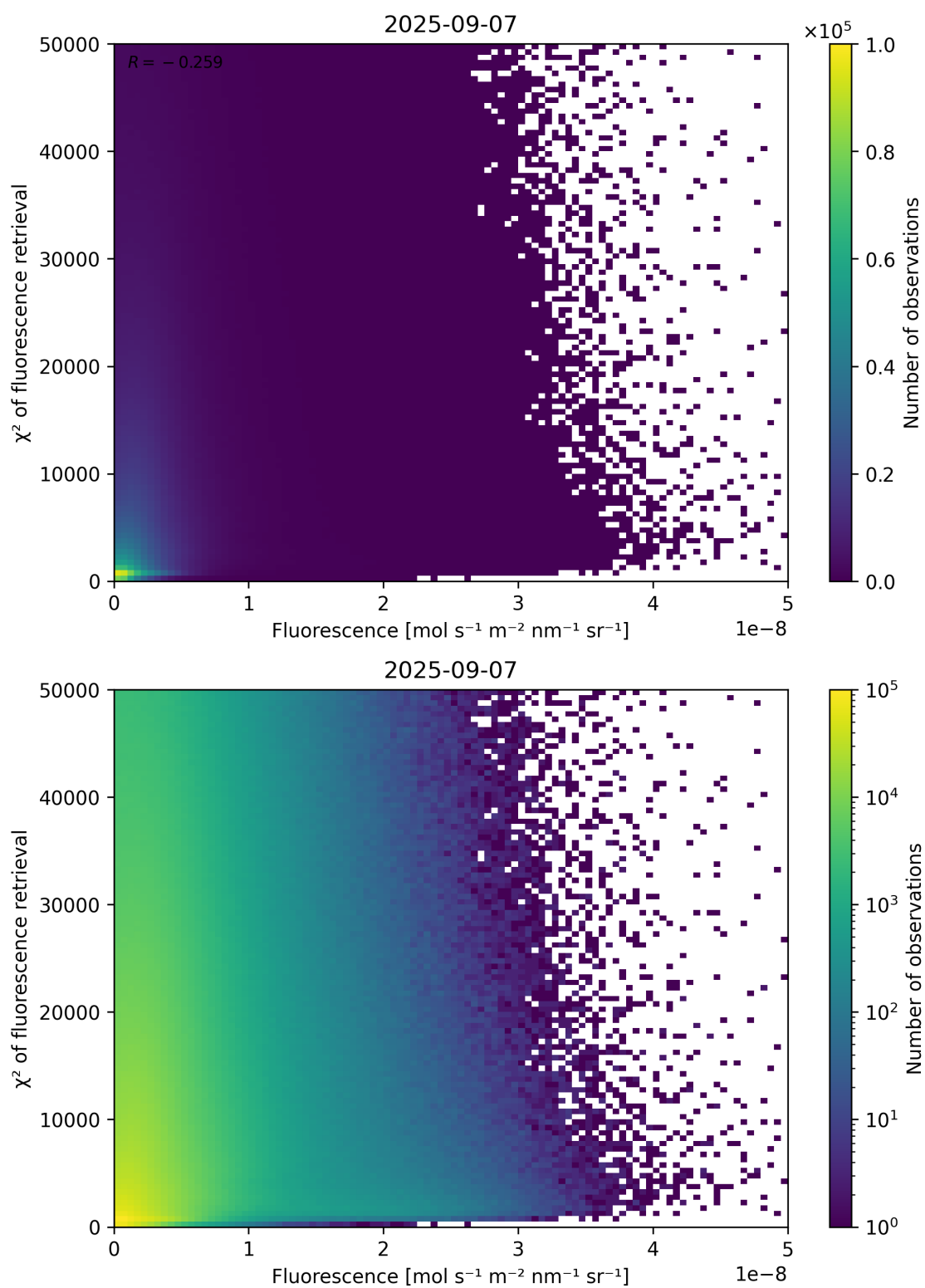
Figure 85: Scatter density plot of “Fluorescence” against “ \chi^2 of fluorescence retrieval” for 2025-09-06 to 2025-09-08.
