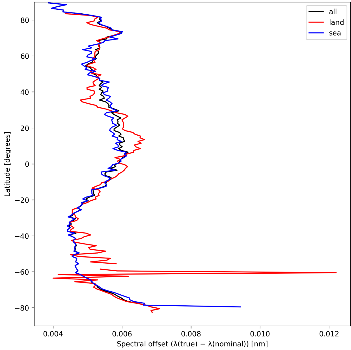
Figure 28: Zonal average of “Spectral offset ( \lambda_{\text{true}} - \lambda_{\text{nominal}} )” for 2025-09-06 to 2025-09-08.
