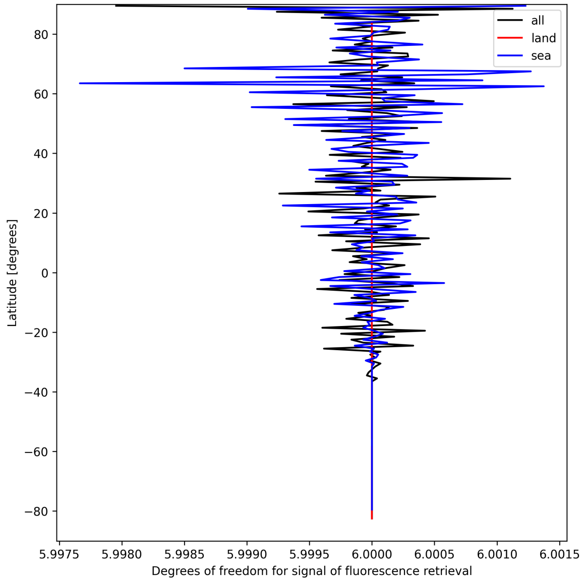
Figure 26: Zonal average of “Degrees of freedom for signal of fluorescence retrieval” for 2025-09-06 to 2025-09-08.
