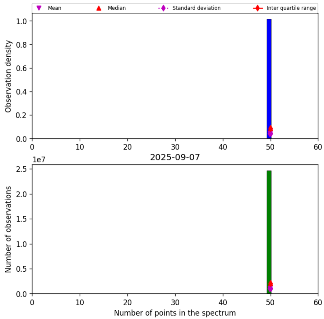
Figure 44: Histogram of "Number of points in the spectrum" for 2025-09-06 to 2025-09-08
