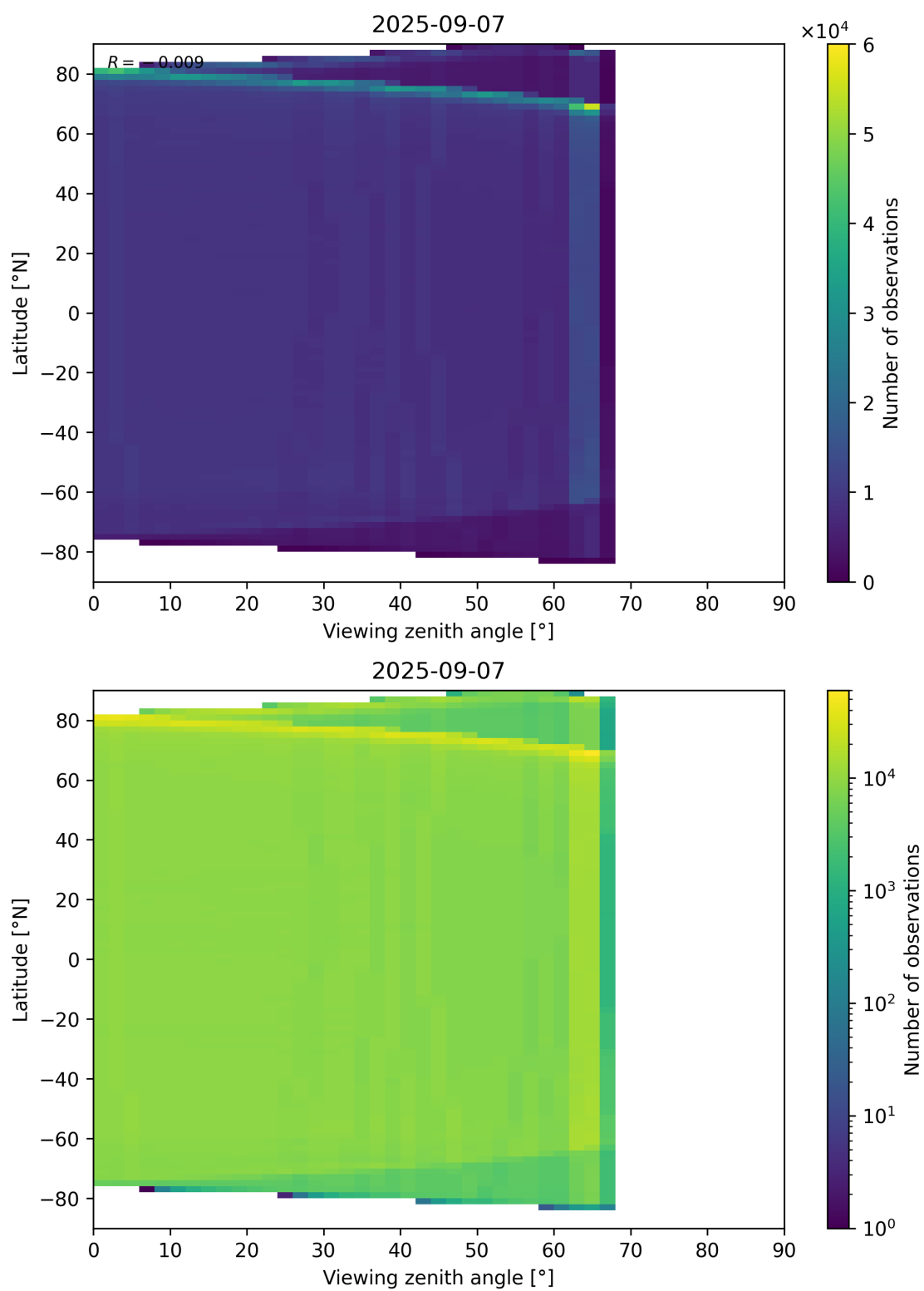
Figure 123: Scatter density plot of “Viewing zenith angle” against “Latitude” for 2025-09-06 to 2025-09-08.
