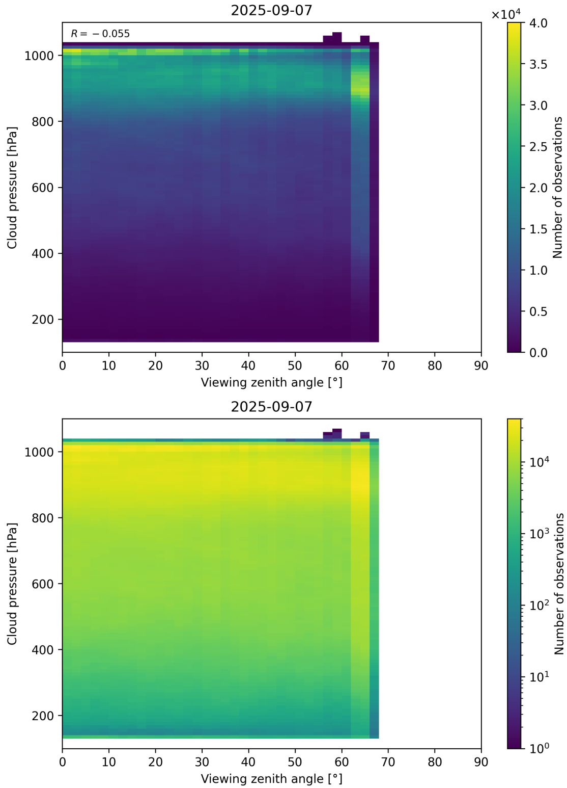
Figure 121: Scatter density plot of “Viewing zenith angle” against “Cloud pressure” for 2025-09-06 to 2025-09-08.
