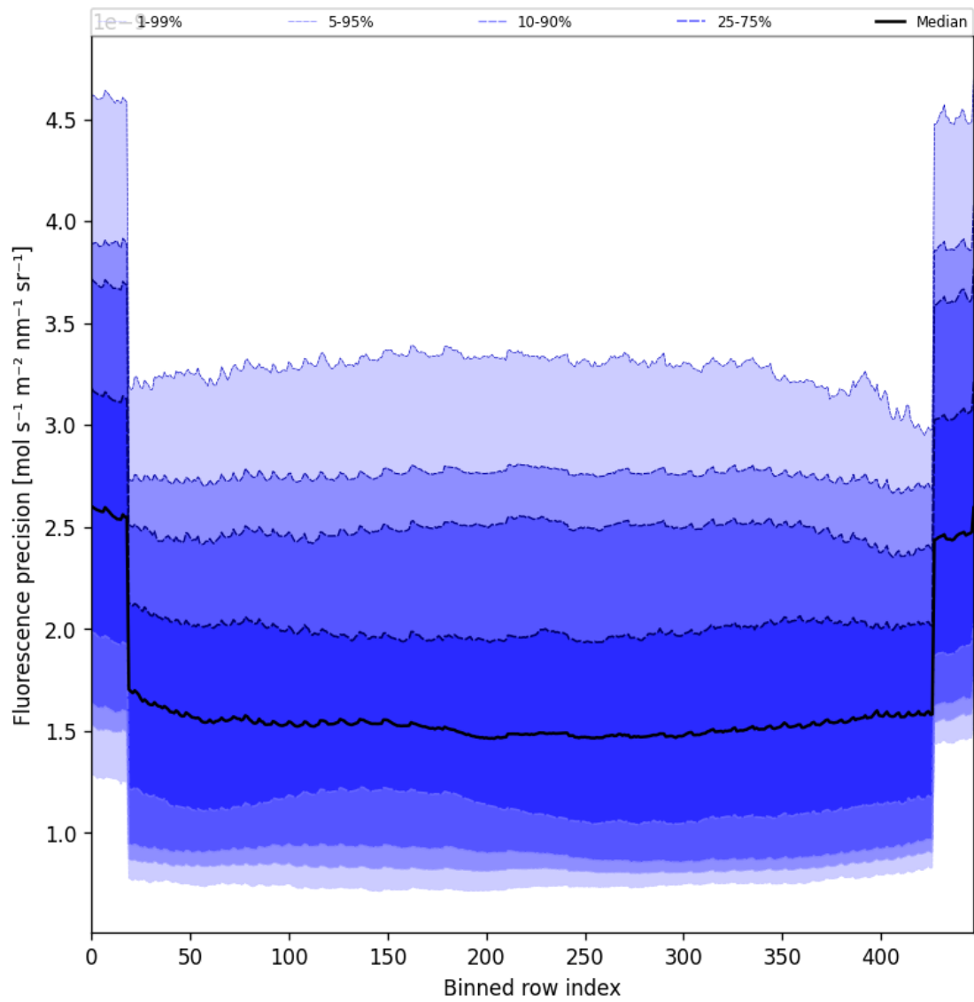
Figure 58: Along track statistics of “Fluorescence precision” for 2025-09-06 to 2025-09-08
