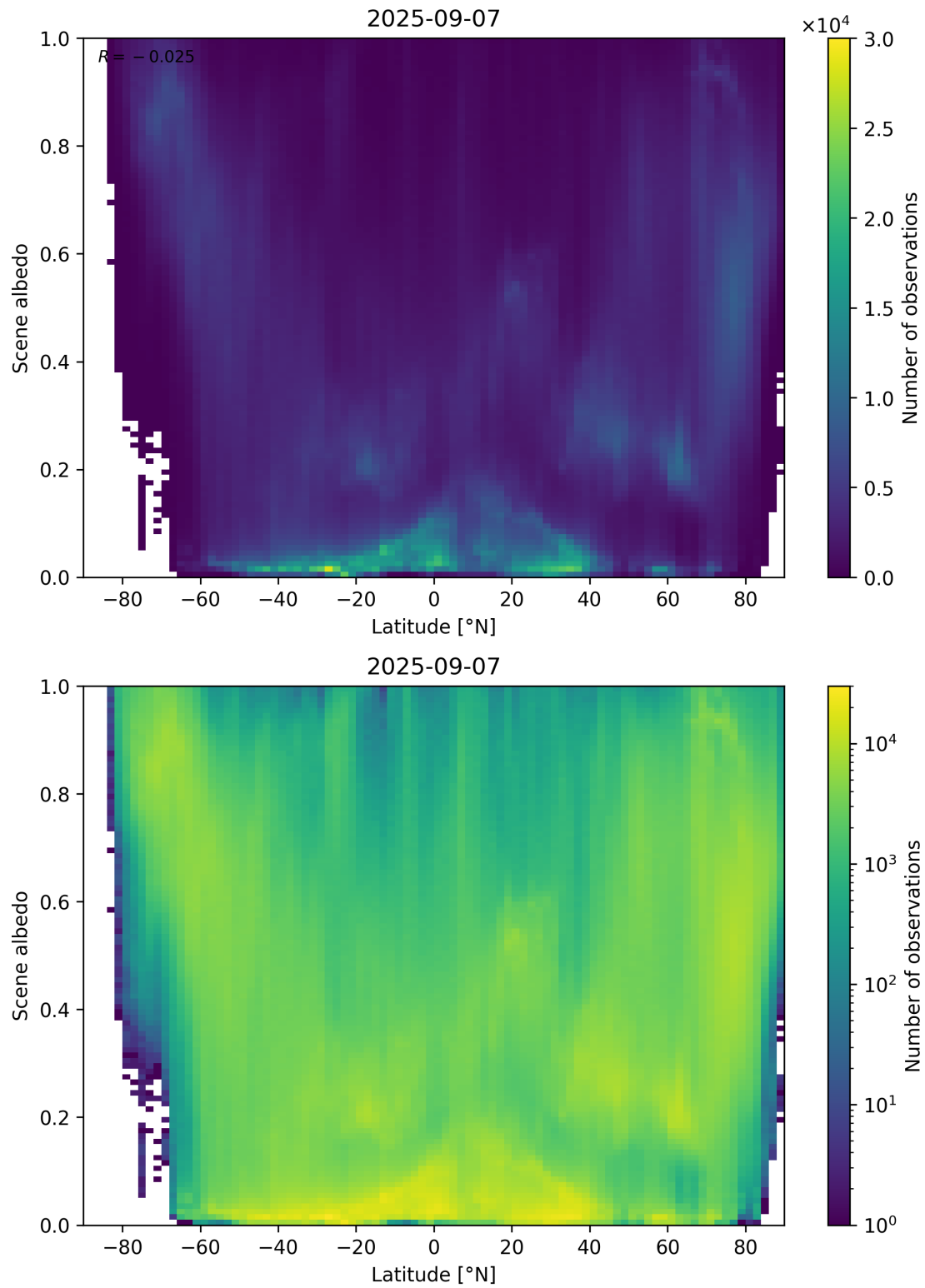
Figure 95: Scatter density plot of “Latitude” against “Scene albedo” for 2025-09-06 to 2025-09-08.
