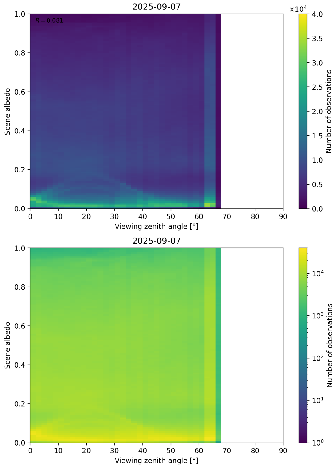
Figure 126: Scatter density plot of “Viewing zenith angle” against “Scene albedo” for 2025-09-06 to 2025-09-08.
