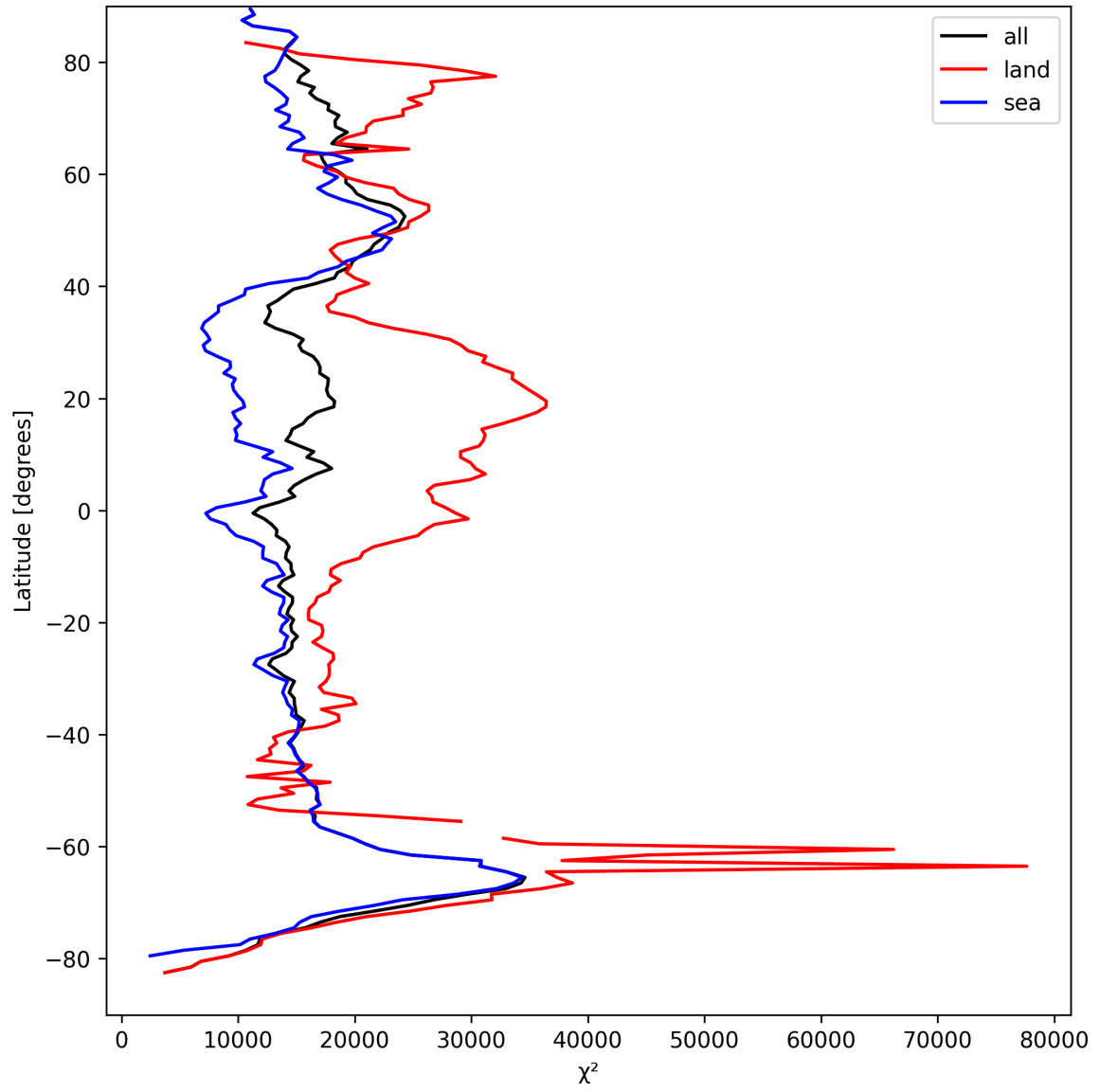
Figure 21: Zonal average of “ \chi^2 ” for 2025-09-06 to 2025-09-08.
