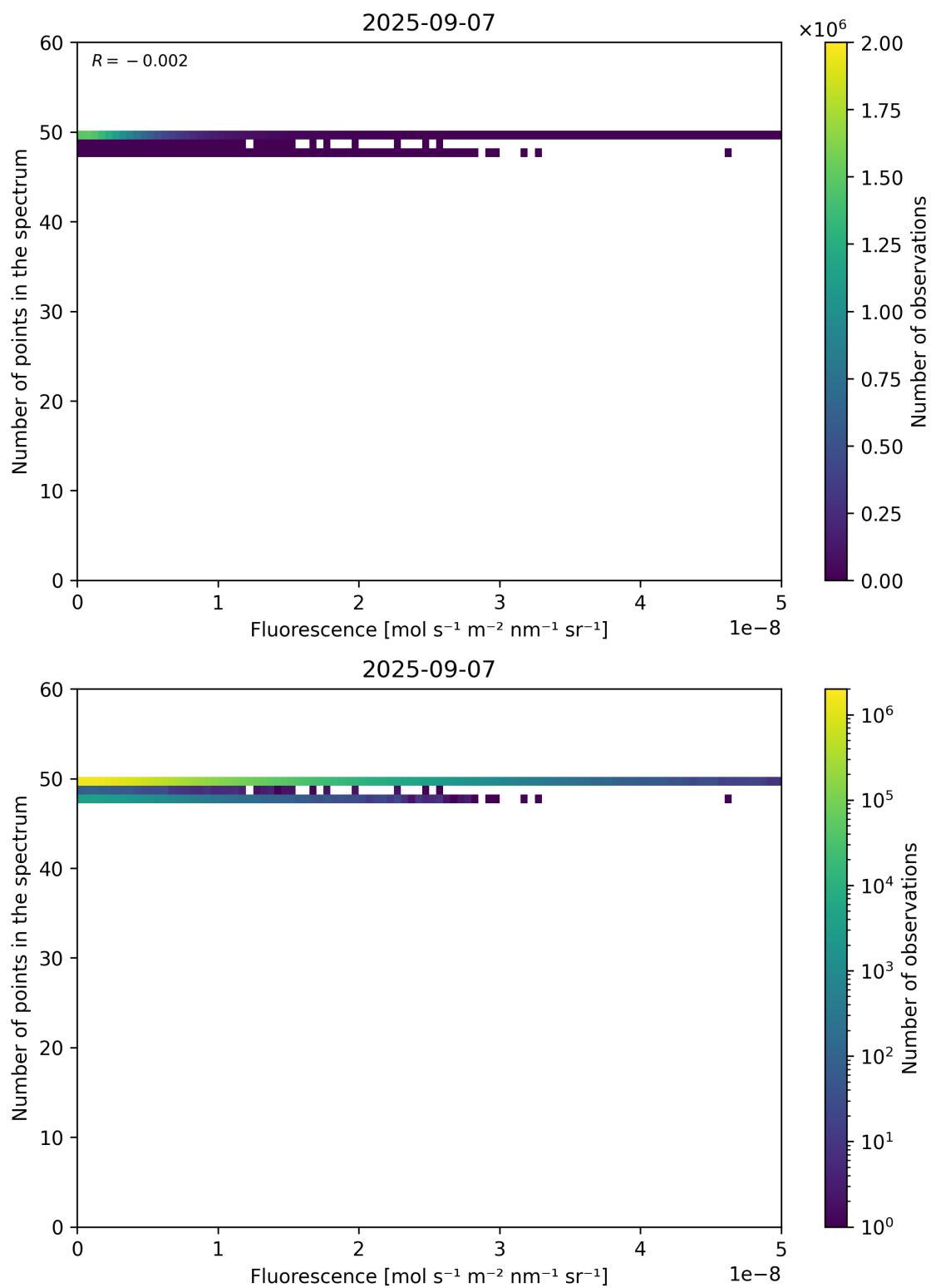
Figure 86: Scatter density plot of “Fluorescence” against “Number of points in the spectrum” for 2025-09-06 to 2025-09-08.
