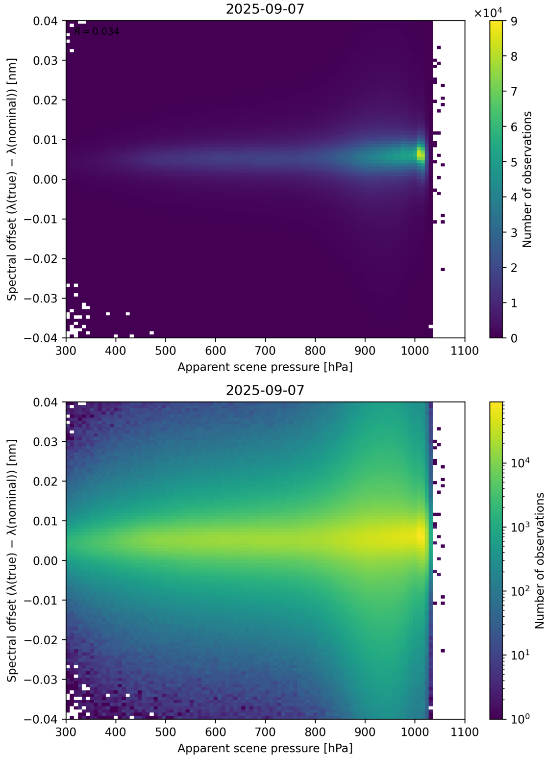
Figure 67: Scatter density plot of “Apparent scene pressure” against “Spectral offset ( \lambda_{\text{true}} - \lambda_{\text{nominal}} )” for 2025-09-06 to 2025-09-08.
