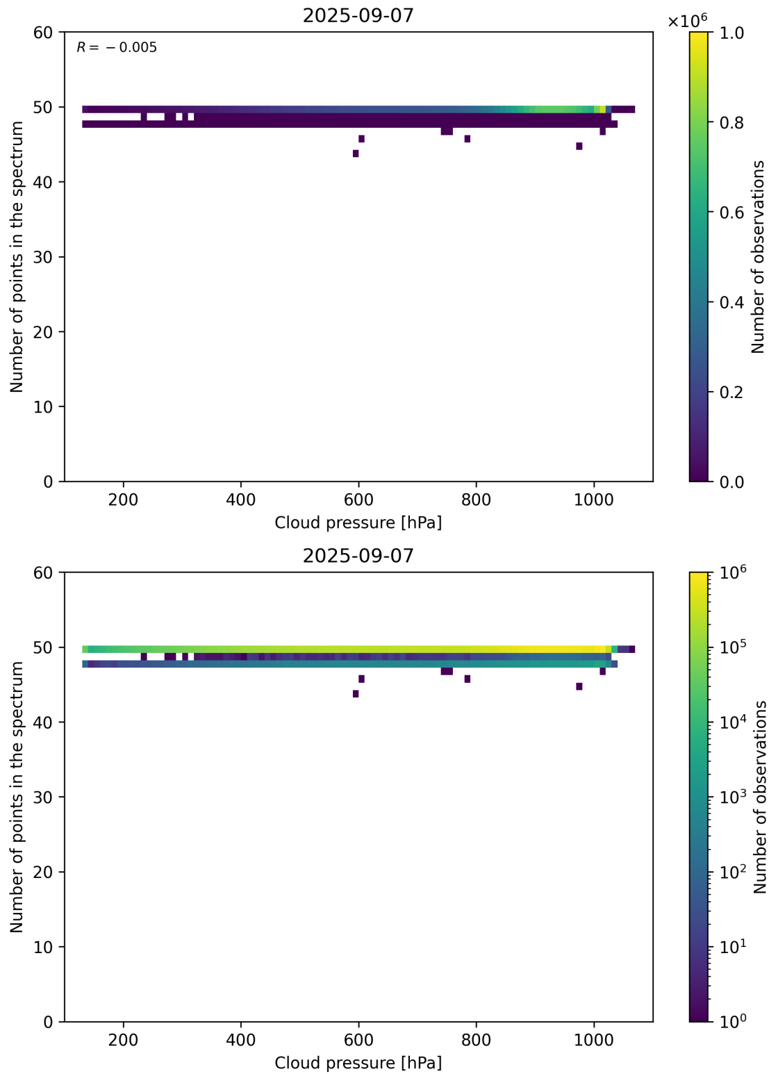
Figure 82: Scatter density plot of “Cloud pressure” against “Number of points in the spectrum” for 2025-09-06 to 2025-09-08.
