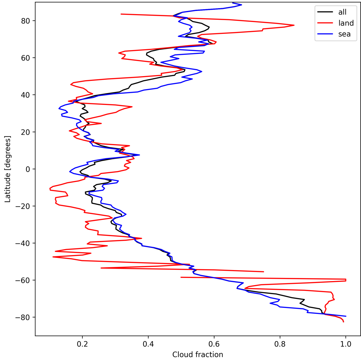
Figure 15: Zonal average of “Cloud fraction” for 2025-09-06 to 2025-09-08.
