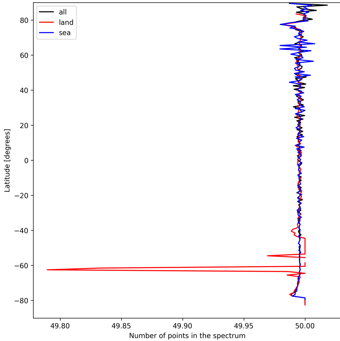
Figure 27: Zonal average of “Number of points in the spectrum” for 2025-09-06 to 2025-09-08.
