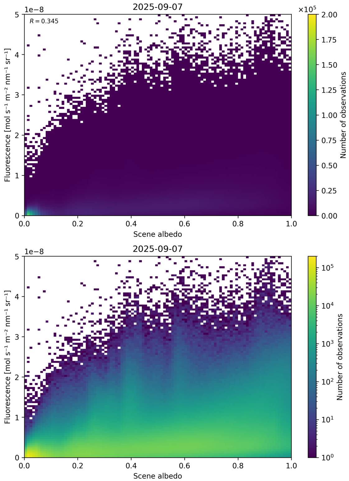
Figure 104: Scatter density plot of “Scene albedo” against “Fluorescence” for 2025-09-06 to 2025-09-08.
