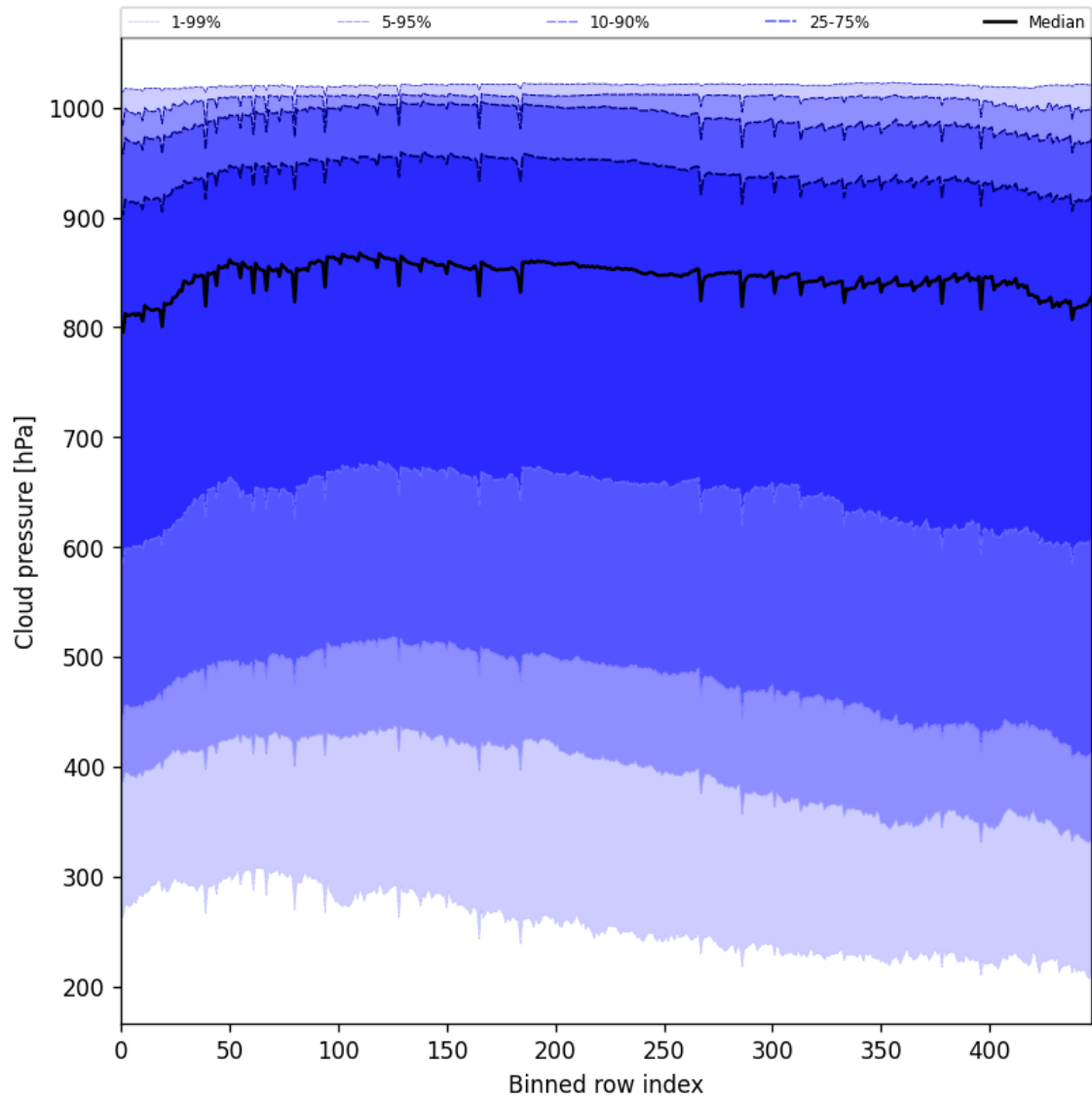
Figure 47: Along track statistics of “Cloud pressure” for 2025-09-06 to 2025-09-08
