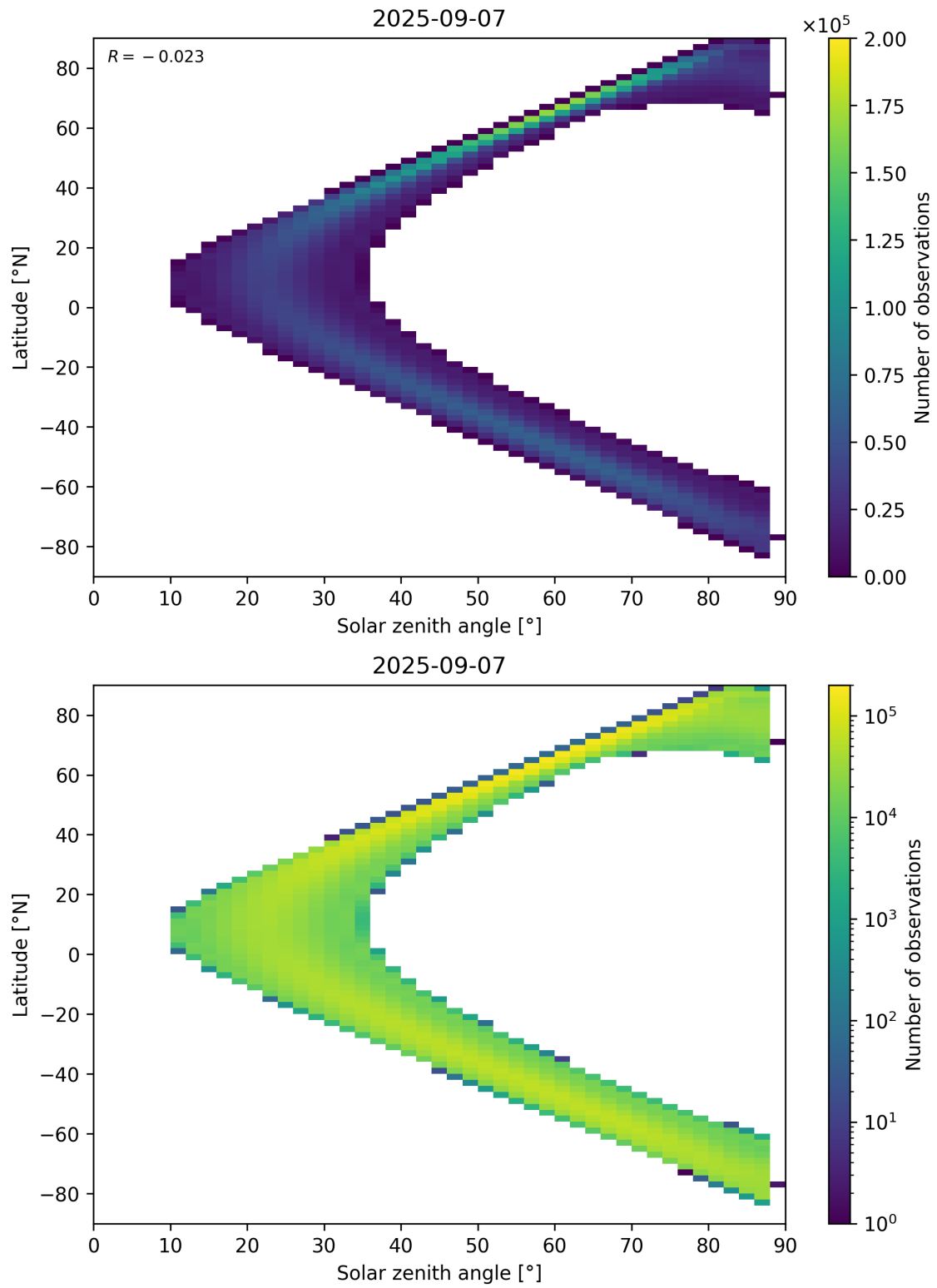
Figure 113: Scatter density plot of “Solar zenith angle” against “Latitude” for 2025-09-06 to 2025-09-08.
