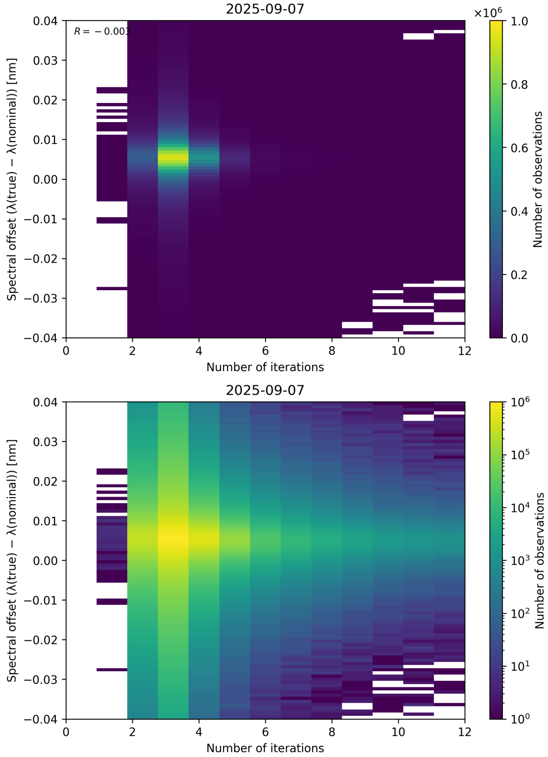
Figure 100: Scatter density plot of “Number of iterations” against “Spectral offset ( \lambda_{\text{true}} - \lambda_{\text{nominal}} )” for 2025-09-06 to 2025-09-08.
