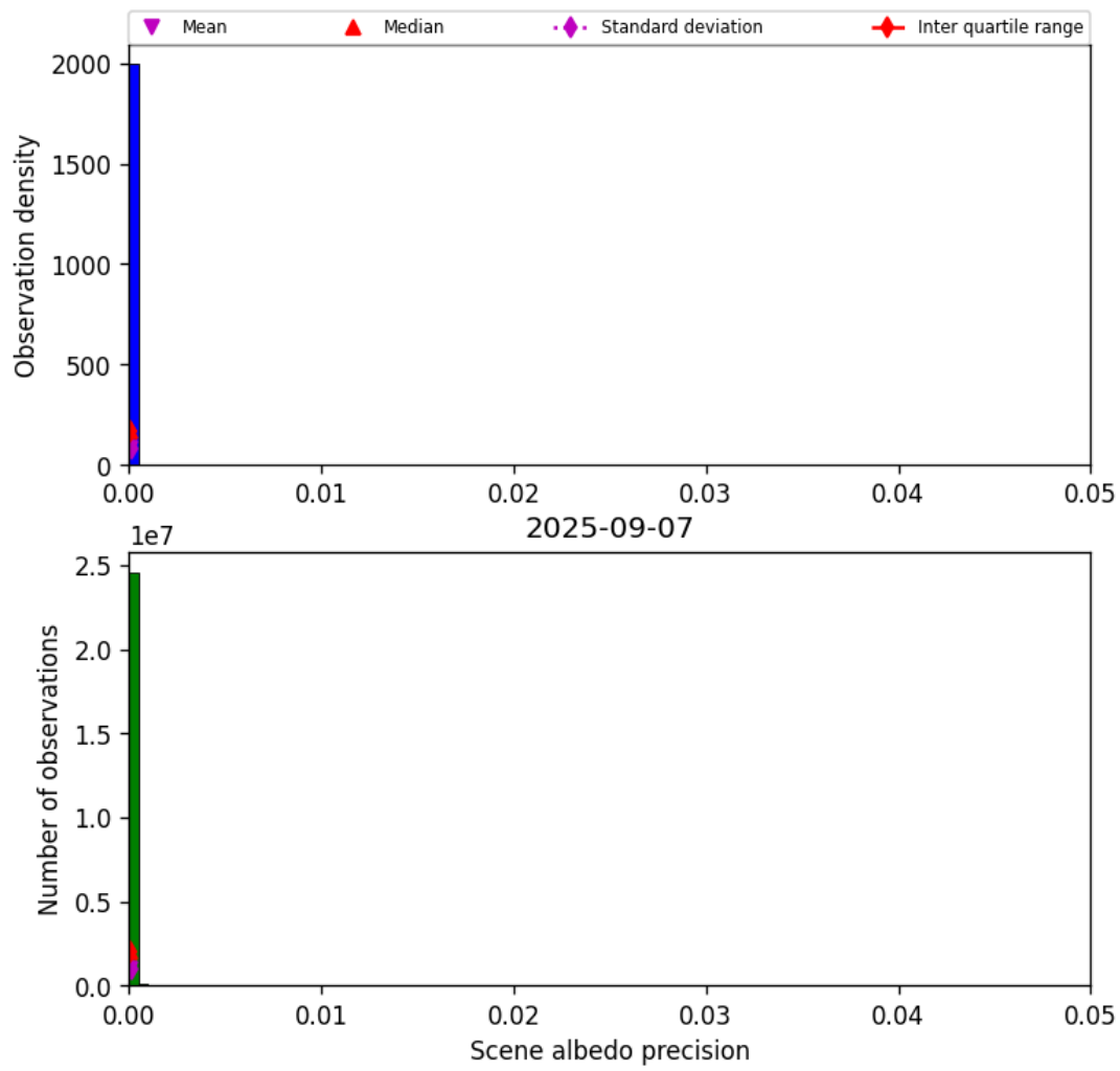
Figure 35: Histogram of “Scene albedo precision” for 2025-09-06 to 2025-09-08
