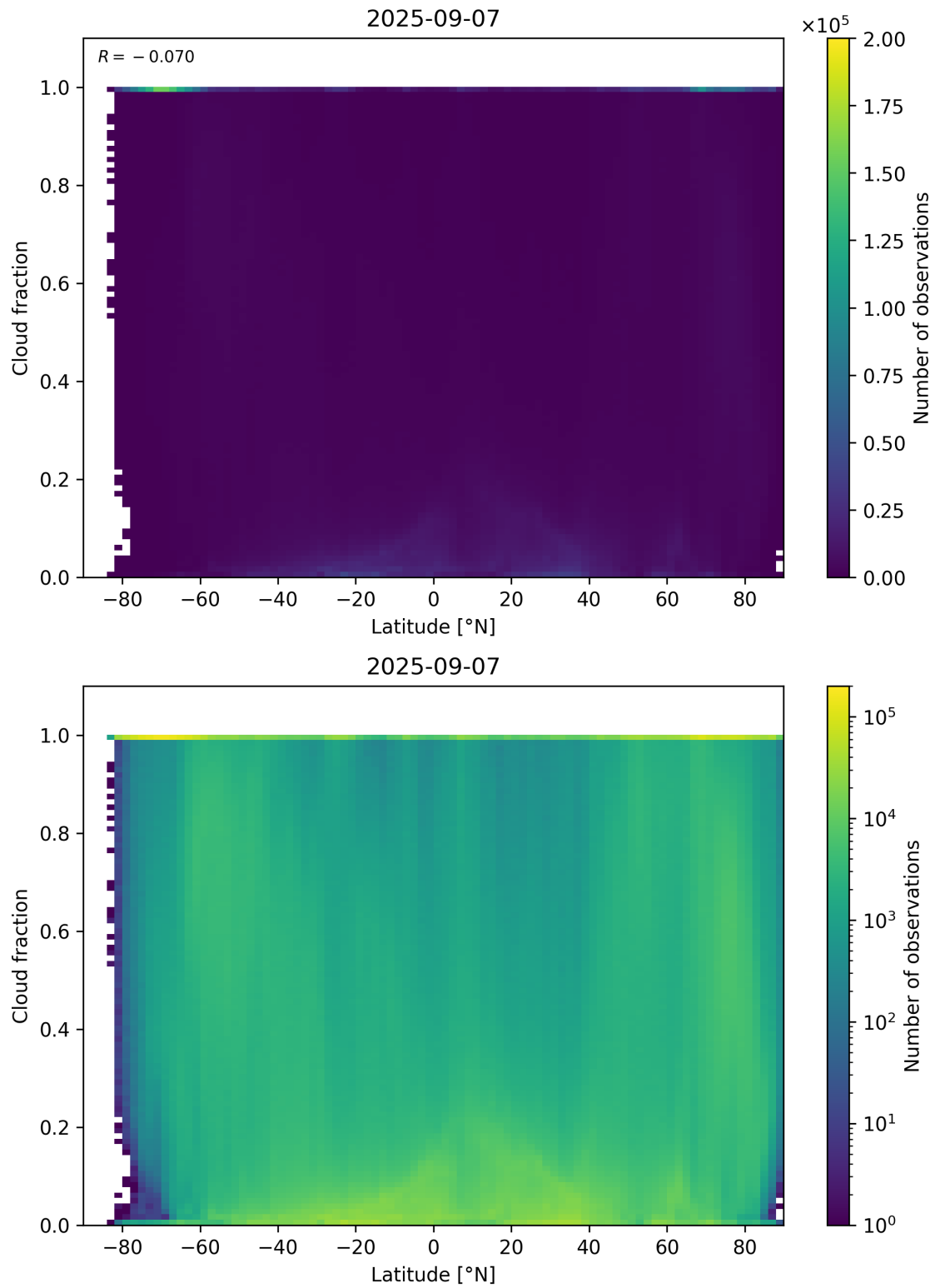
Figure 90: Scatter density plot of “Latitude” against “Cloud fraction” for 2025-09-06 to 2025-09-08.
