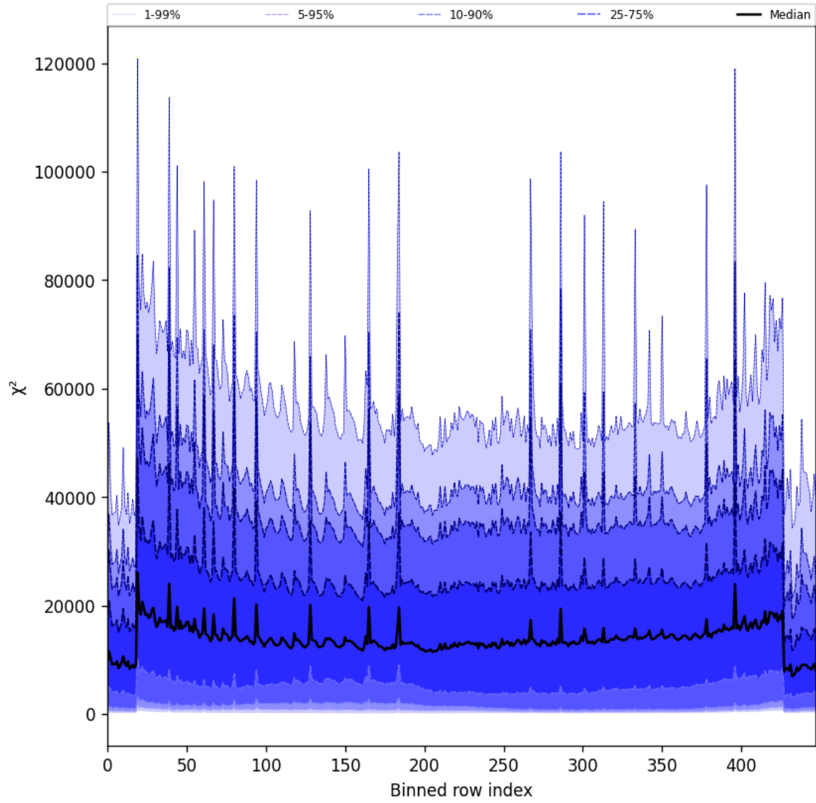
Figure 55: Along track statistics of “ \chi^2 ” for 2025-09-06 to 2025-09-08
