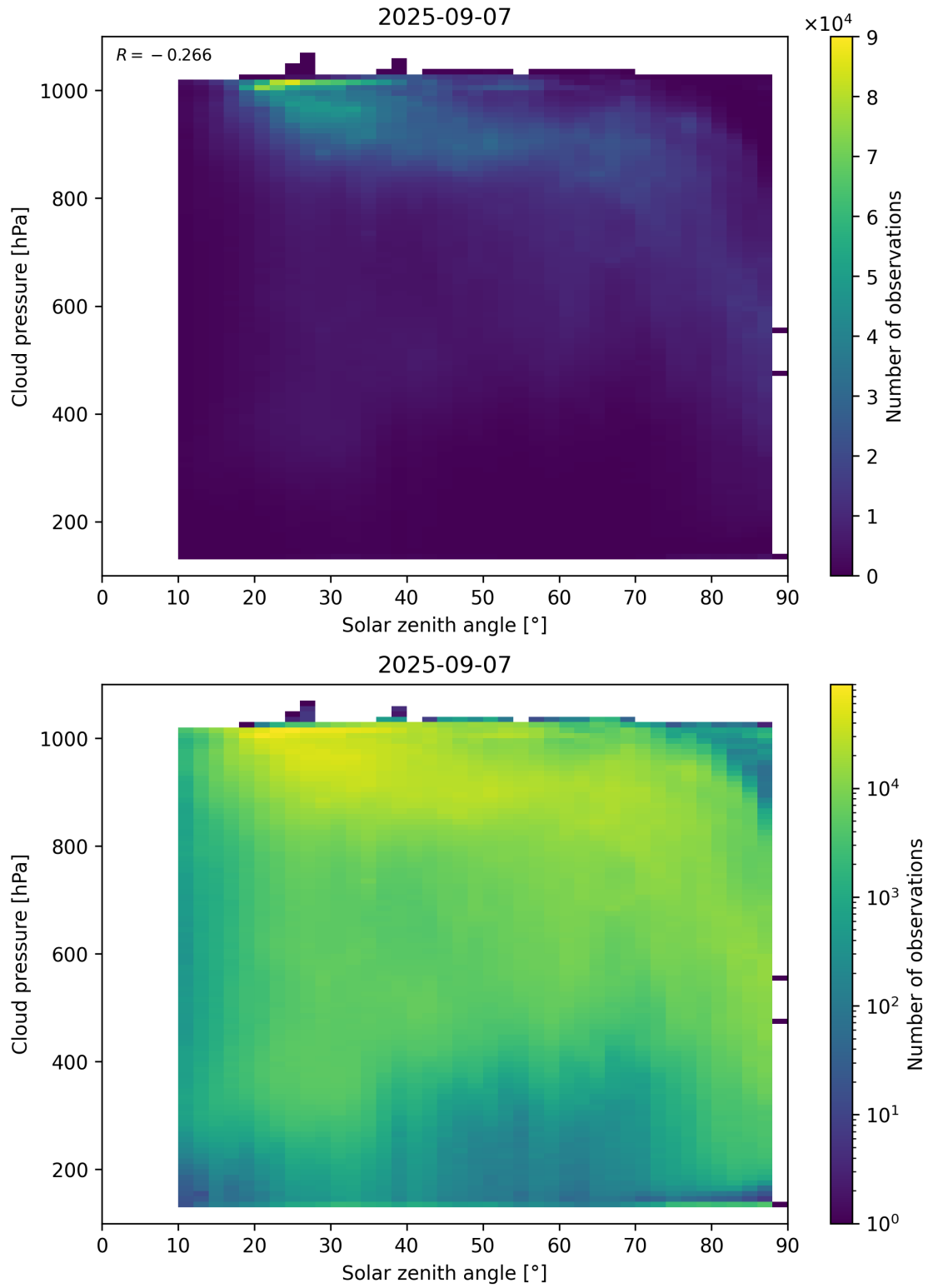
Figure 111: Scatter density plot of “Solar zenith angle” against “Cloud pressure” for 2025-09-06 to 2025-09-08.
