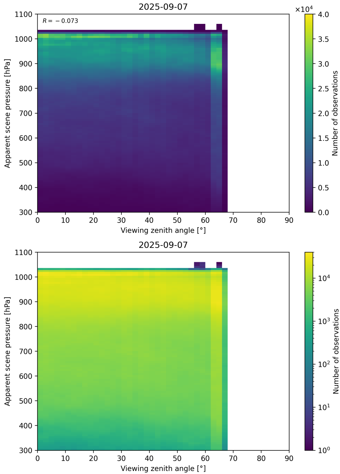
Figure 118: Scatter density plot of “Viewing zenith angle” against “Apparent scene pressure” for 2025-09-06 to 2025-09-08.
