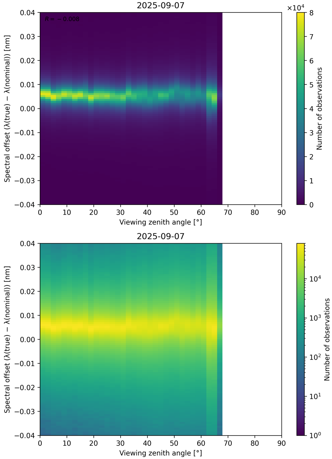
Figure 128: Scatter density plot of “Viewing zenith angle” against “Spectral offset ( \lambda_{\text{true}} - \lambda_{\text{nominal}} )” for 2025-09-06 to 2025-09-08.
