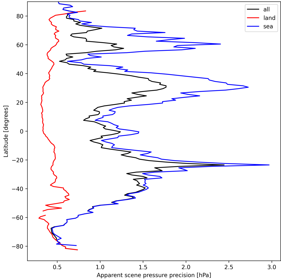
Figure 20: Zonal average of “Apparent scene pressure precision” for 2025-09-06 to 2025-09-08.
