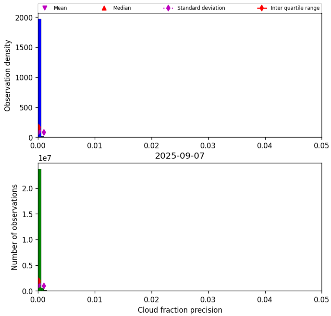
Figure 33: Histogram of “Cloud fraction precision” for 2025-09-06 to 2025-09-08
