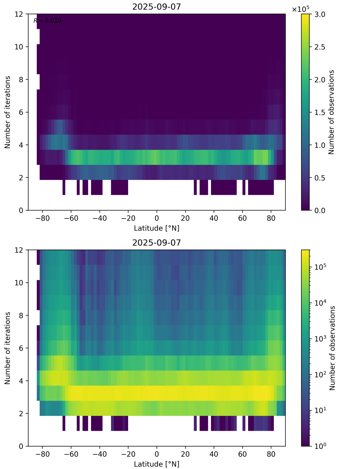
Figure 93: Scatter density plot of “Latitude” against “Number of iterations” for 2025-09-06 to 2025-09-08.
