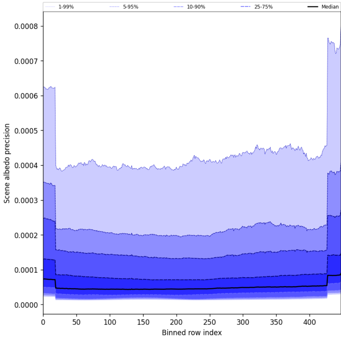
Figure 52: Along track statistics of “Scene albedo precision” for 2025-09-06 to 2025-09-08
