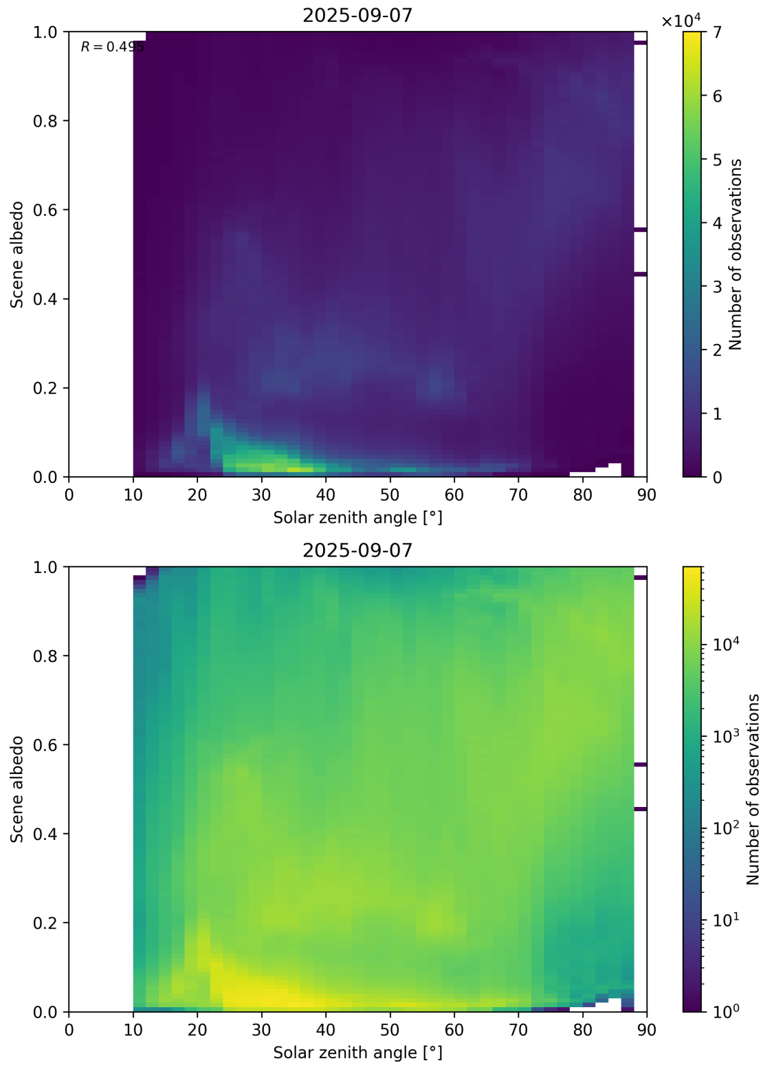
Figure 116: Scatter density plot of “Solar zenith angle” against “Scene albedo” for 2025-09-06 to 2025-09-08.
