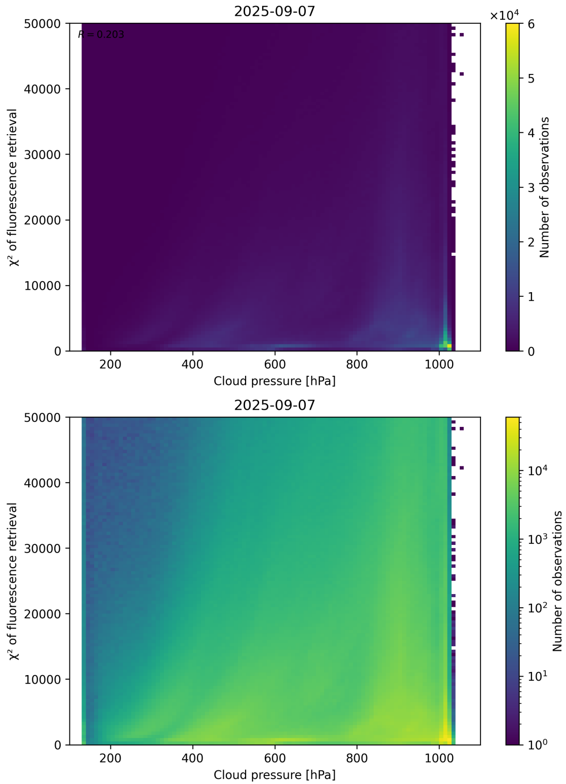
Figure 78: Scatter density plot of “Cloud pressure” against “ \chi^2 of fluorescence retrieval” for 2025-09-06 to 2025-09-08.
