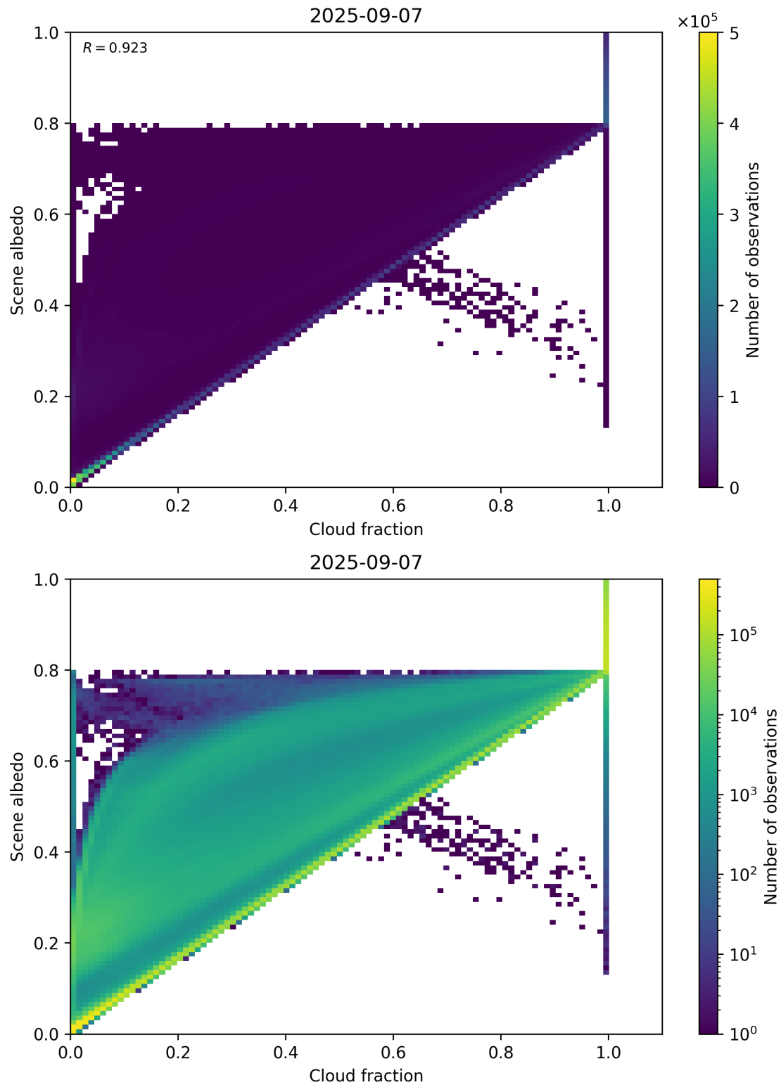
Figure 75: Scatter density plot of “Cloud fraction” against “Scene albedo” for 2025-09-06 to 2025-09-08.
