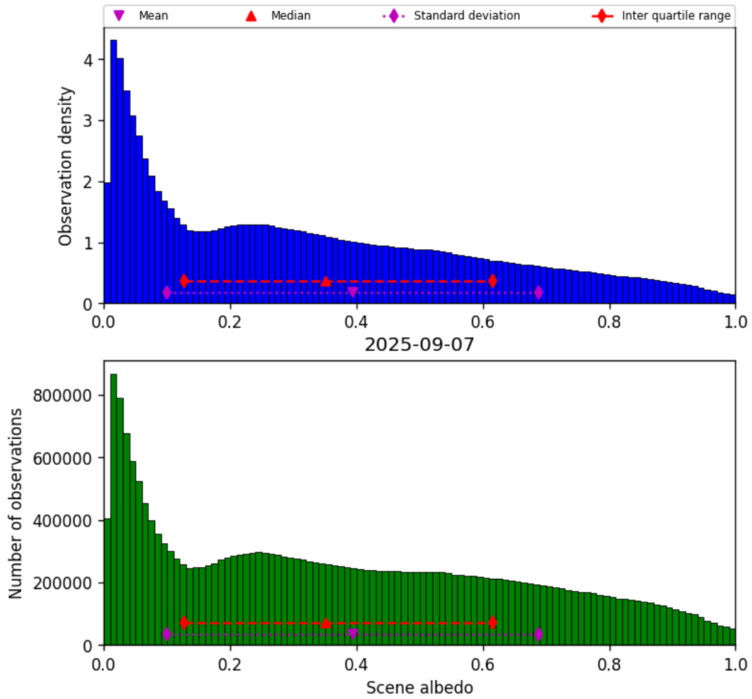
Figure 34: Histogram of “Scene albedo” for 2025-09-06 to 2025-09-08
