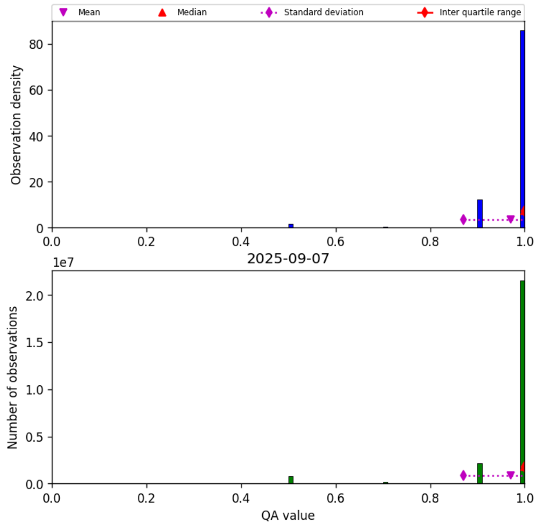
Figure 29: Histogram of “QA value” for 2025-09-06 to 2025-09-08
