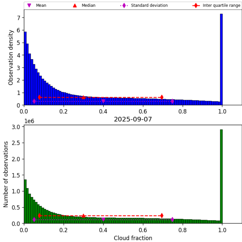
Figure 32: Histogram of “Cloud fraction” for 2025-09-06 to 2025-09-08
