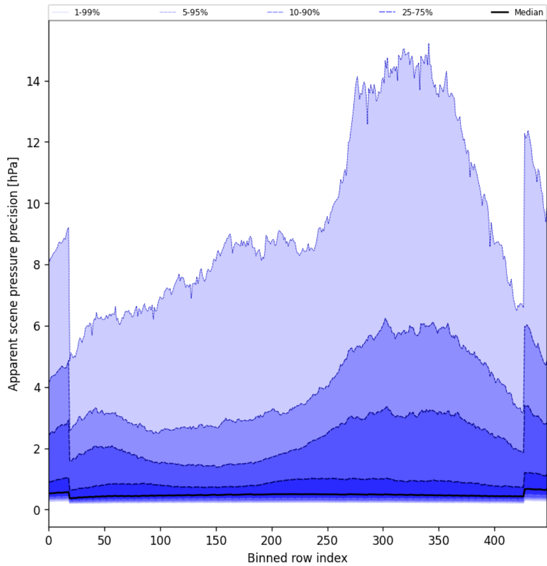
Figure 54: Along track statistics of “Apparent scene pressure precision” for 2025-09-06 to 2025-09-08
