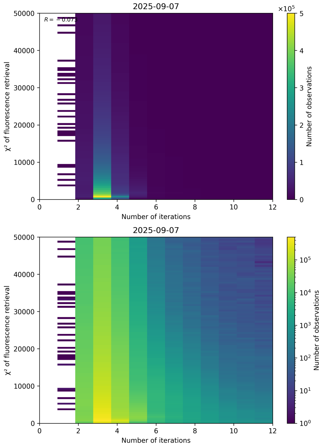
Figure 97: Scatter density plot of “Number of iterations” against “ \chi^2 of fluorescence retrieval” for 2025-09-06 to 2025-09-08.
