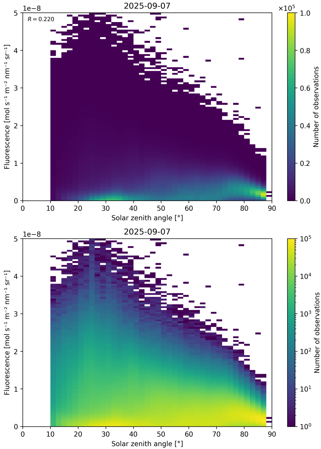
Figure 112: Scatter density plot of “Solar zenith angle” against “Fluorescence” for 2025-09-06 to 2025-09-08.
