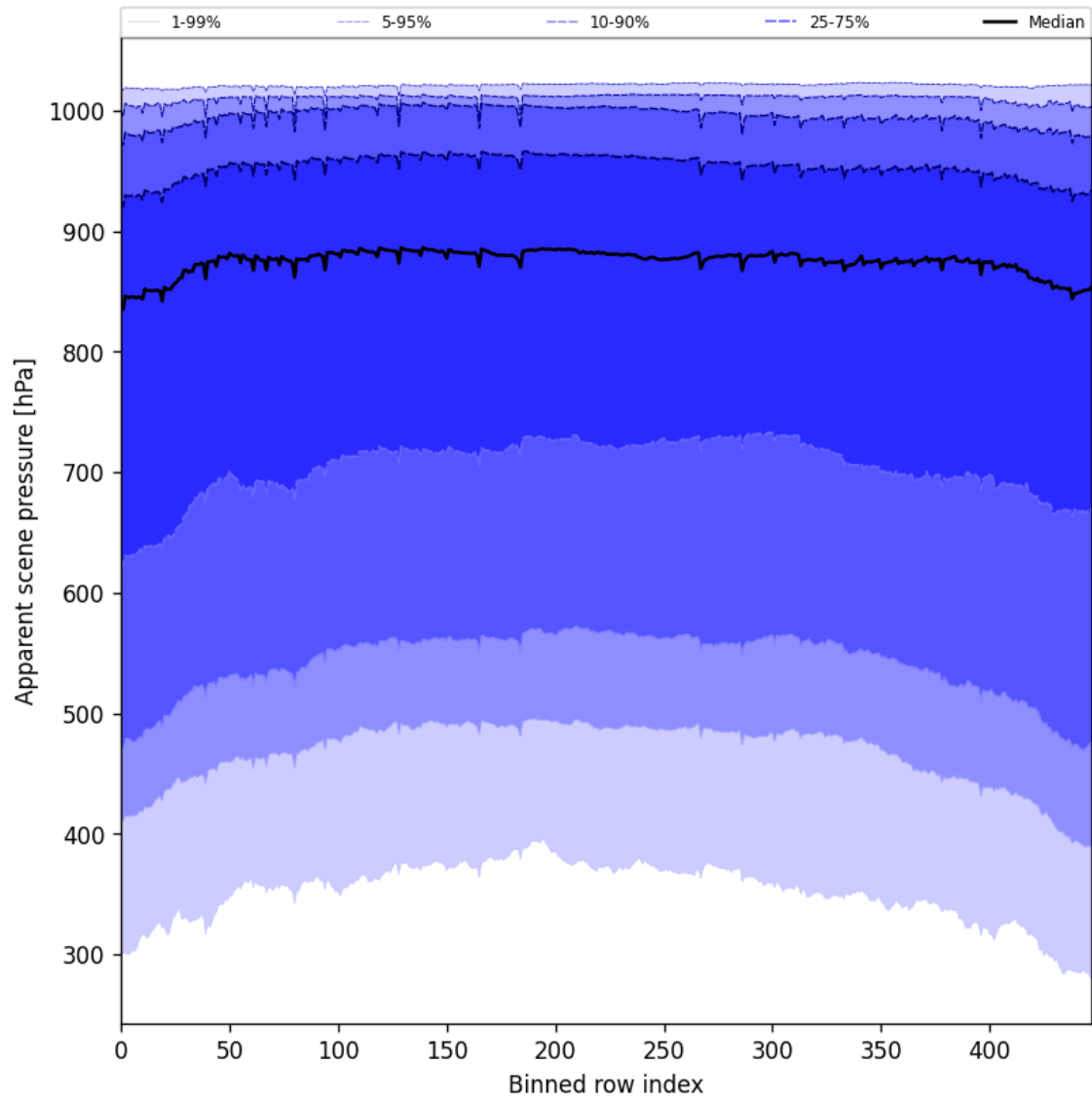
Figure 53: Along track statistics of “Apparent scene pressure” for 2025-09-06 to 2025-09-08
