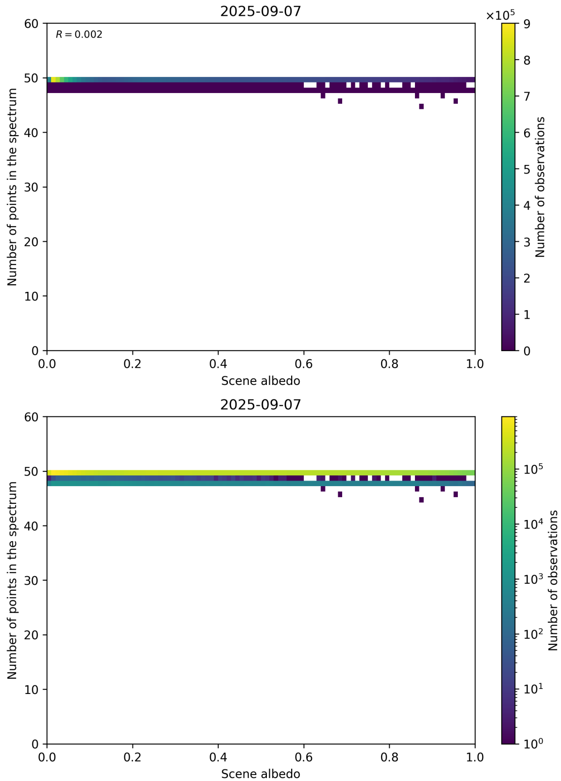
Figure 106: Scatter density plot of “Scene albedo” against “Number of points in the spectrum” for 2025-09-06 to 2025-09-08.
