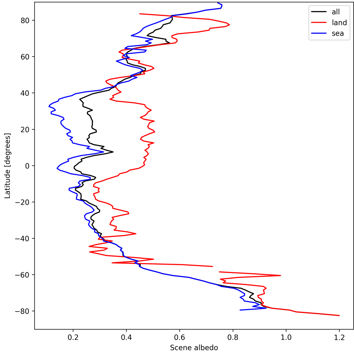
Figure 17: Zonal average of “Scene albedo” for 2025-09-06 to 2025-09-08.
