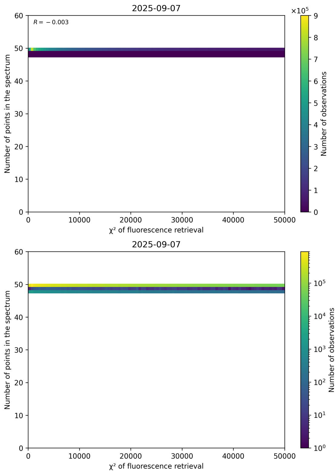
Figure 68: Scatter density plot of “ \chi^2 of fluorescence retrieval” against “Number of points in the spectrum” for 2025-09-06 to 2025-09-08.
