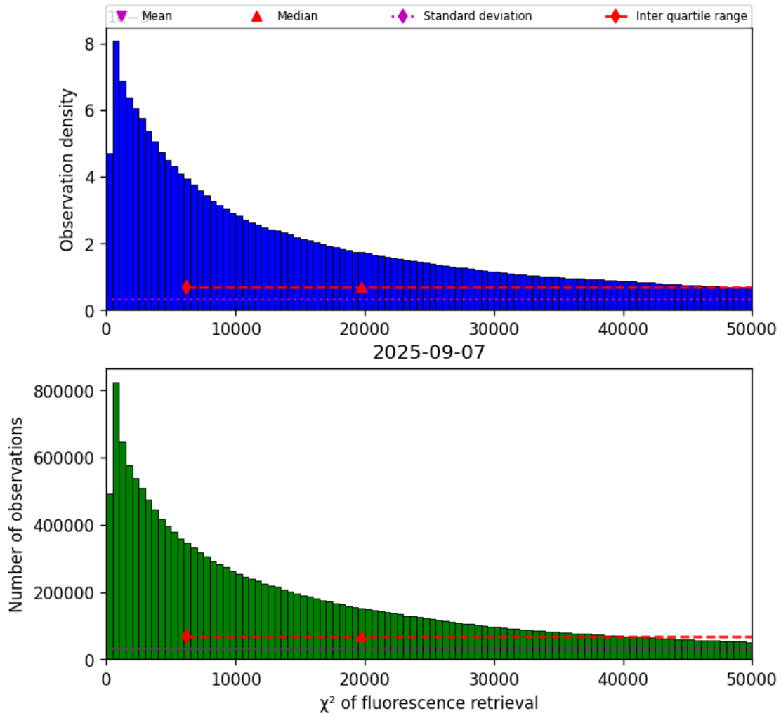
Figure 42: Histogram of “ \chi^2 of fluorescence retrieval” for 2025-09-06 to 2025-09-08
