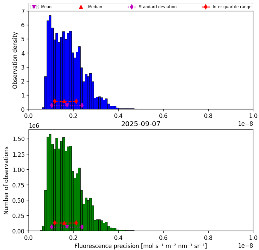
Figure 41: Histogram of “Fluorescence precision” for 2025-09-06 to 2025-09-08
