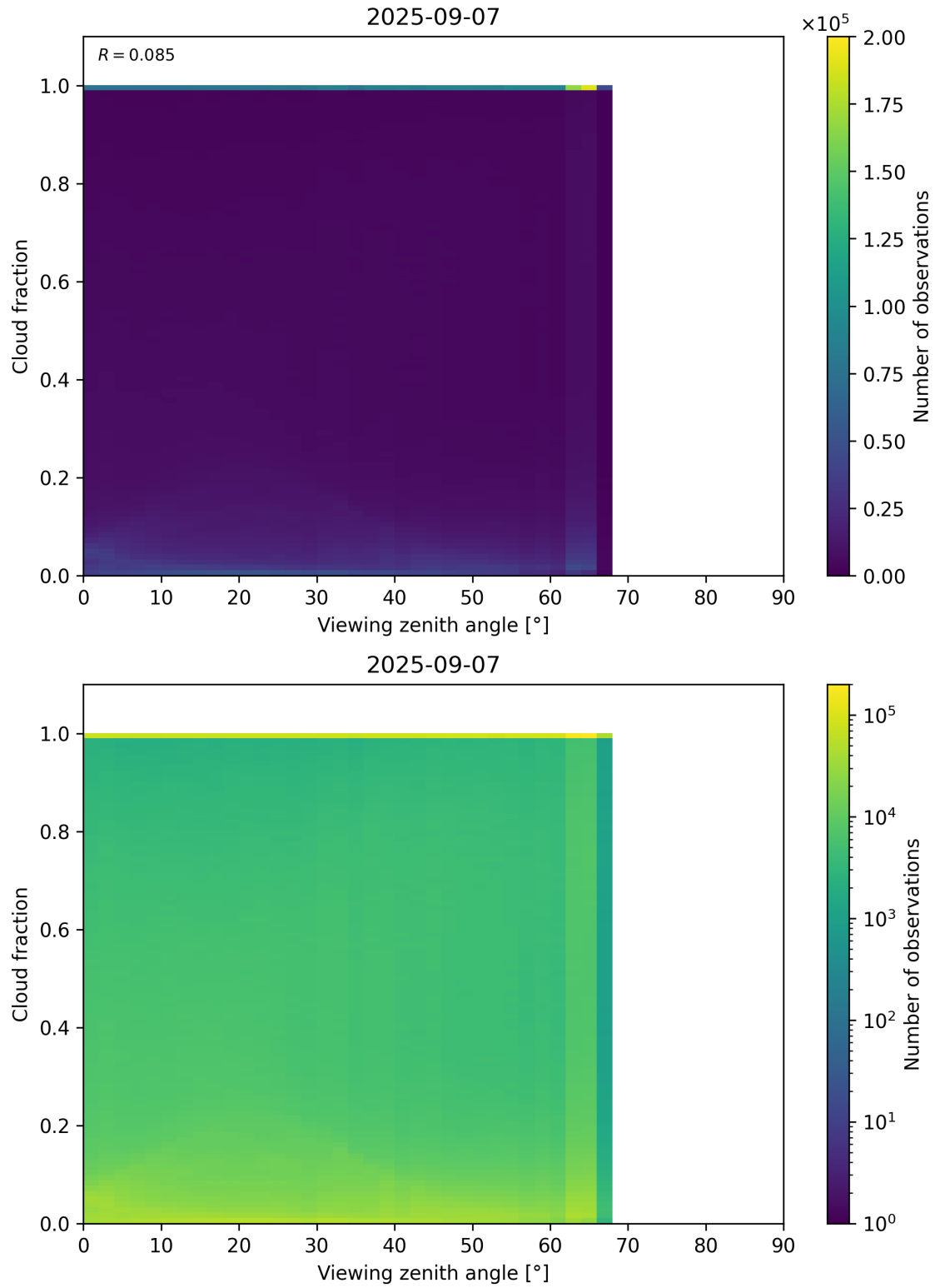
Figure 120: Scatter density plot of “Viewing zenith angle” against “Cloud fraction” for 2025-09-06 to 2025-09-08.
