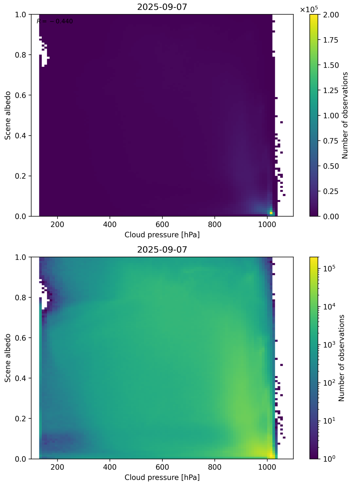
Figure 83: Scatter density plot of “Cloud pressure” against “Scene albedo” for 2025-09-06 to 2025-09-08.
