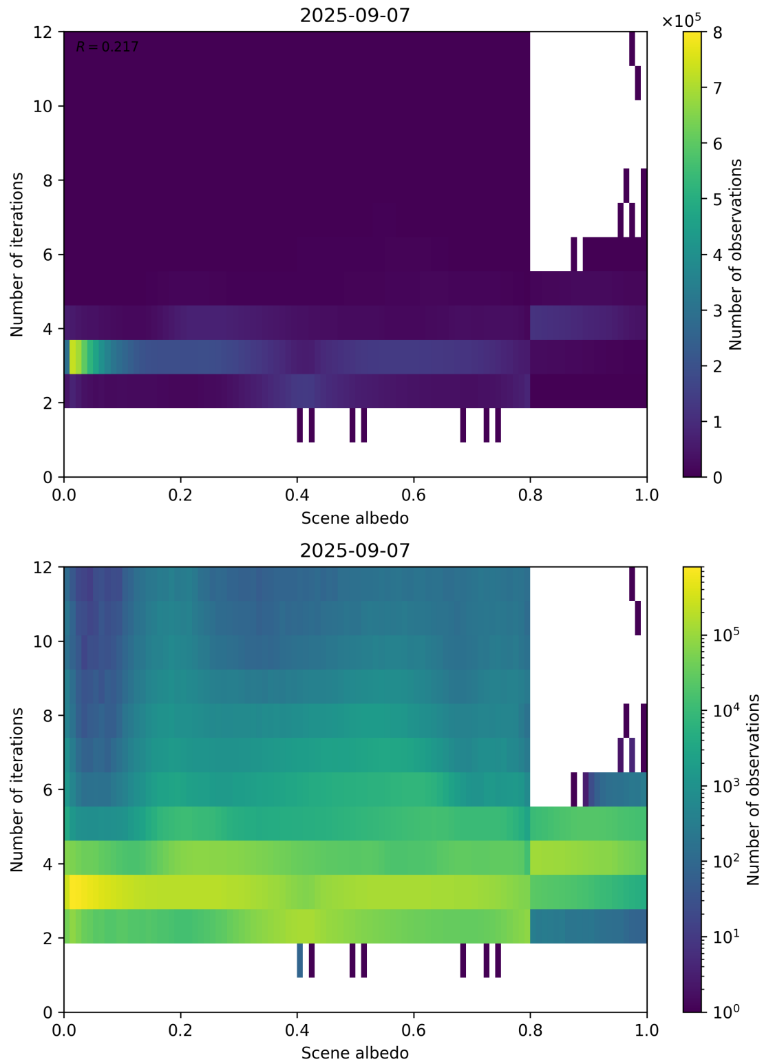
Figure 105: Scatter density plot of “Scene albedo” against “Number of iterations” for 2025-09-06 to 2025-09-08.
