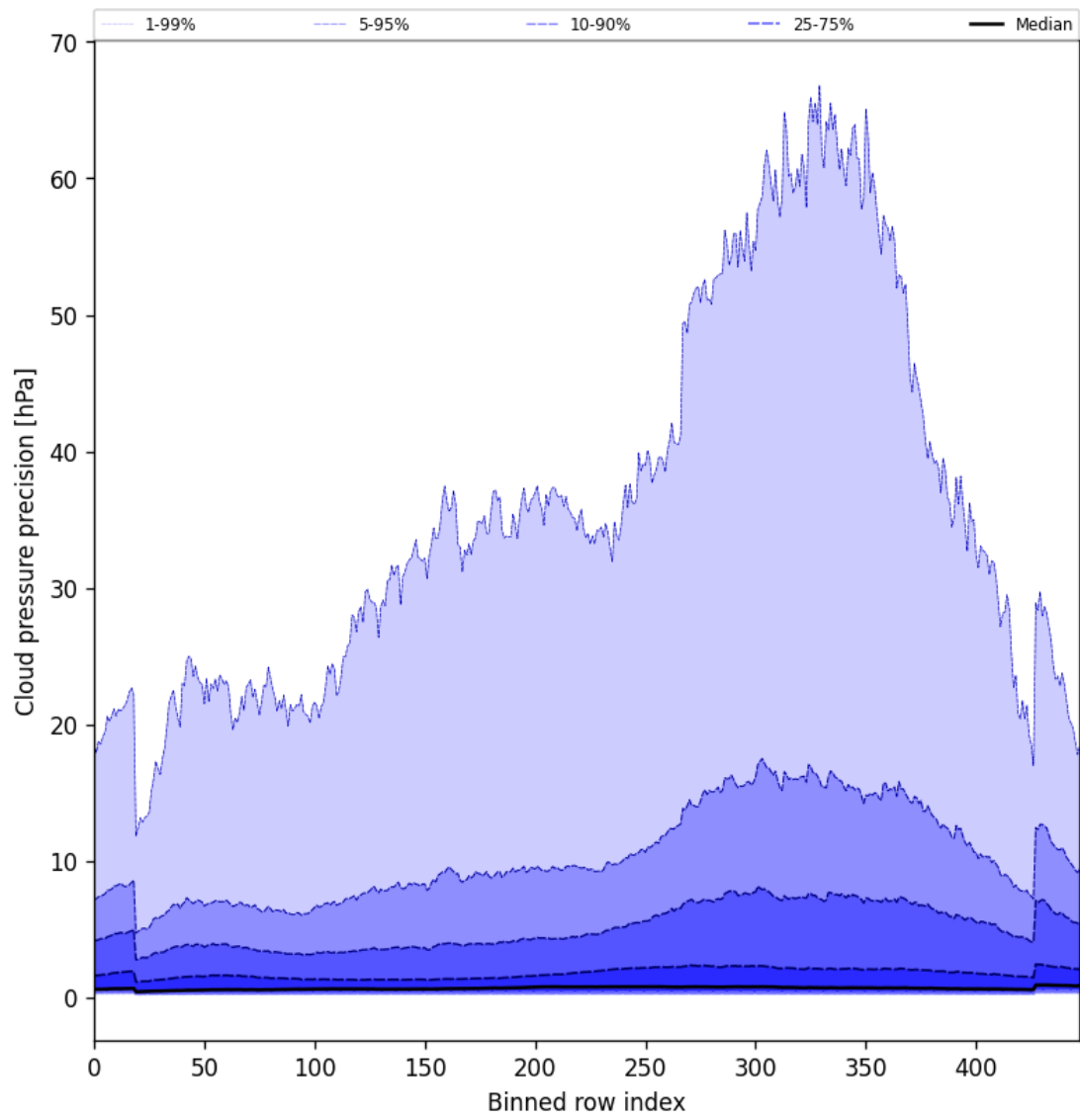
Figure 48: Along track statistics of “Cloud pressure precision” for 2025-09-06 to 2025-09-08
