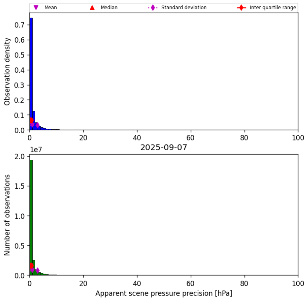
Figure 37: Histogram of “Apparent scene pressure precision” for 2025-09-06 to 2025-09-08
