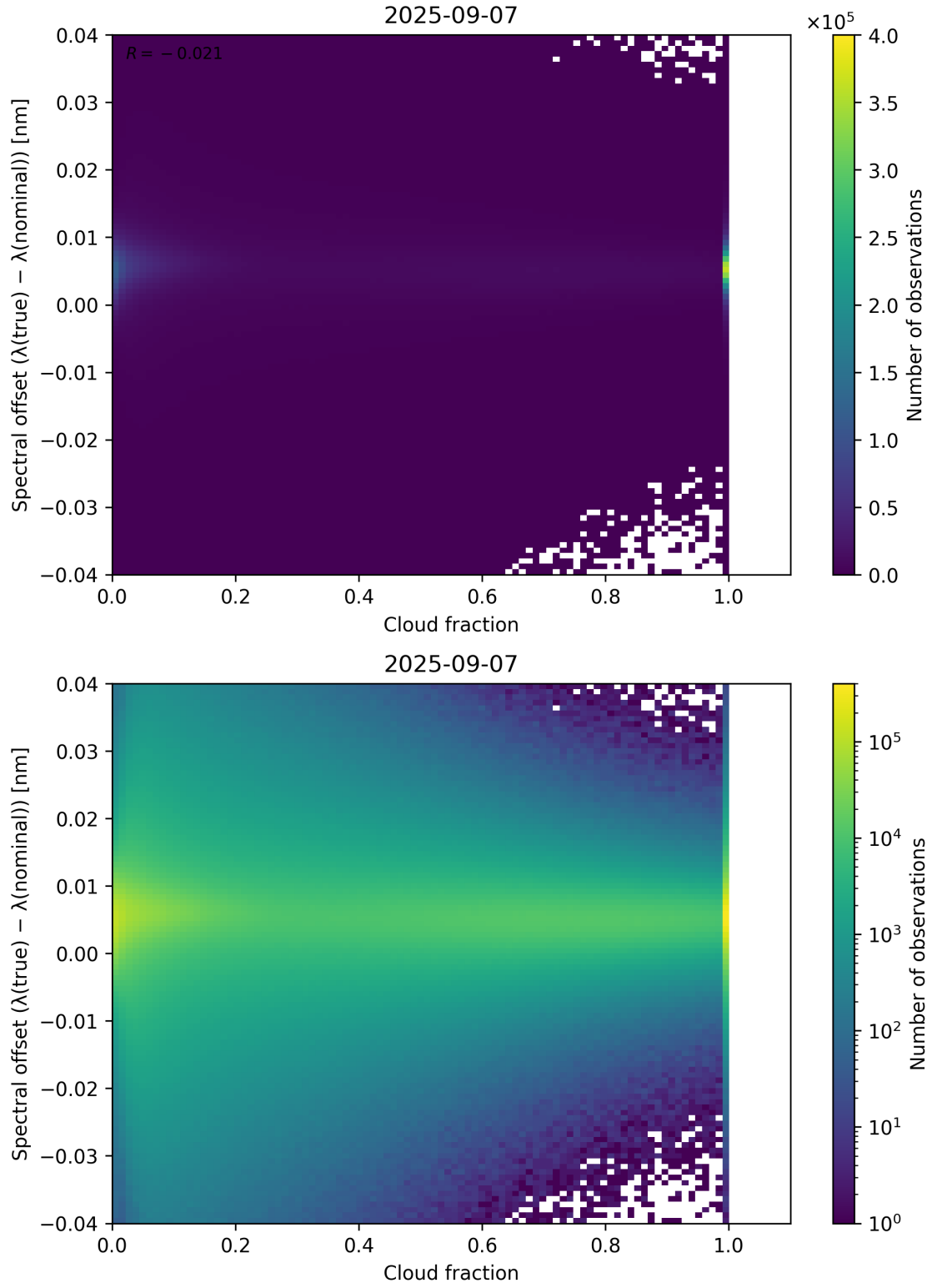
Figure 76: Scatter density plot of “Cloud fraction” against “Spectral offset ( \lambda_{\text{true}} - \lambda_{\text{nominal}} )” for 2025-09-06 to 2025-09-08.
