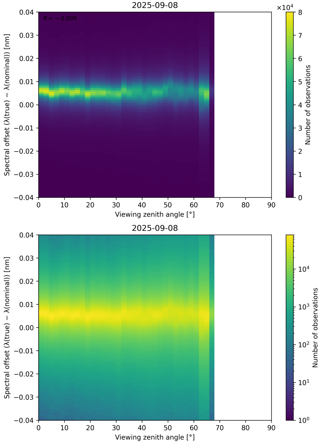
Figure 128: Scatter density plot of “Viewing zenith angle” against “Spectral offset ( \lambda_{\text{true}} - \lambda_{\text{nominal}} )” for 2025-09-07 to 2025-09-09.
