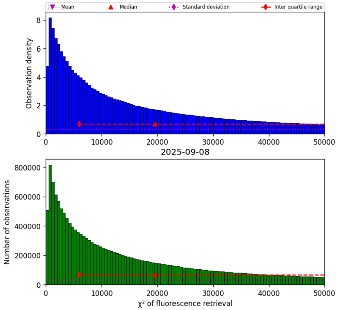
Figure 42: Histogram of “ \chi^2 of fluorescence retrieval” for 2025-09-07 to 2025-09-09
