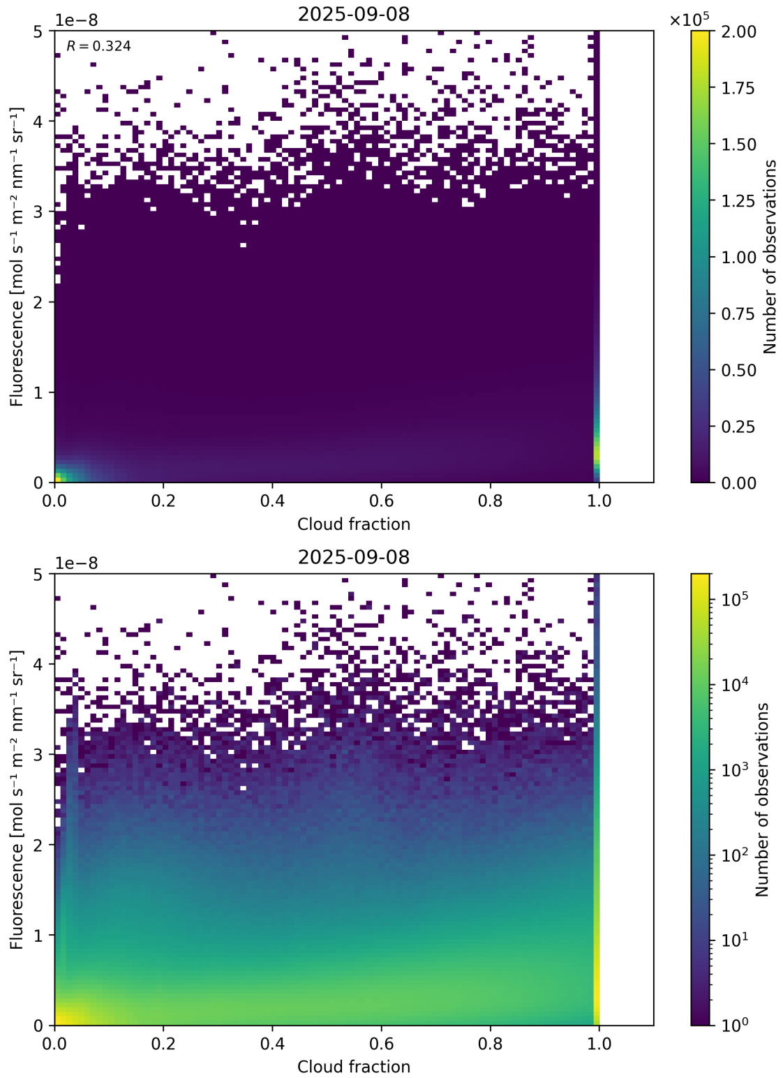
Figure 72: Scatter density plot of “Cloud fraction” against “Fluorescence” for 2025-09-07 to 2025-09-09.
