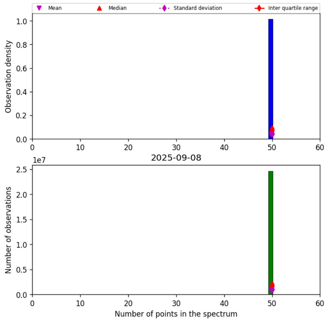
Figure 44: Histogram of "Number of points in the spectrum" for 2025-09-07 to 2025-09-09
