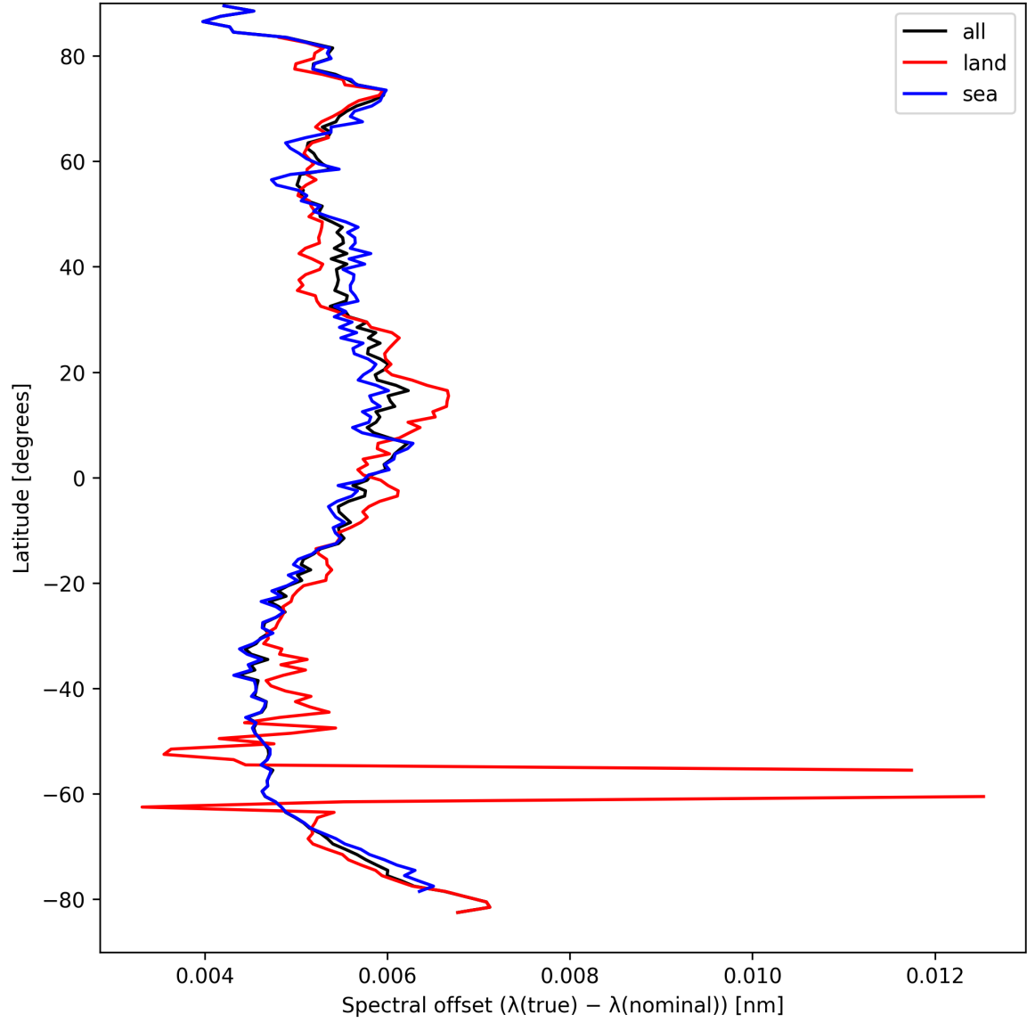
Figure 28: Zonal average of “Spectral offset ( \lambda_{\text{true}} - \lambda_{\text{nominal}} )” for 2025-09-07 to 2025-09-09.
