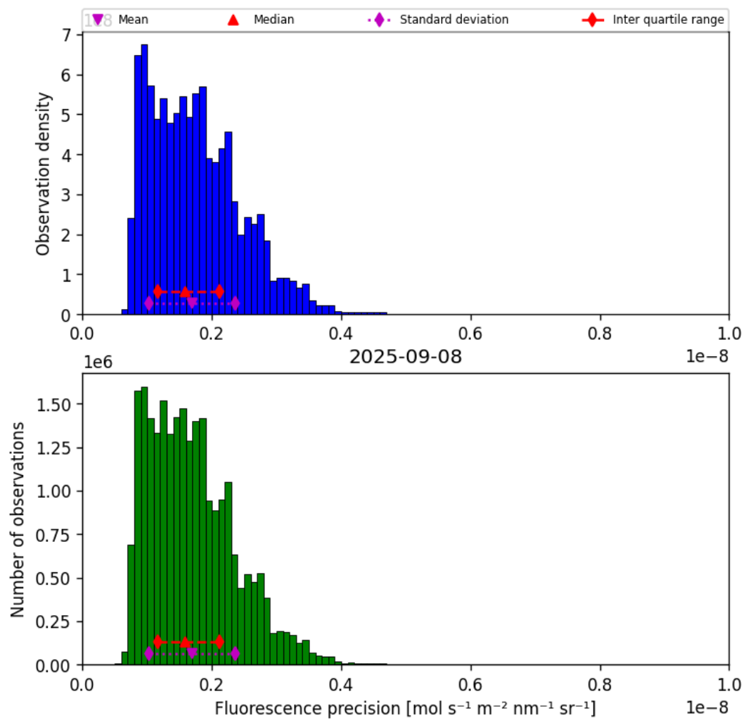
Figure 41: Histogram of “Fluorescence precision” for 2025-09-07 to 2025-09-09
