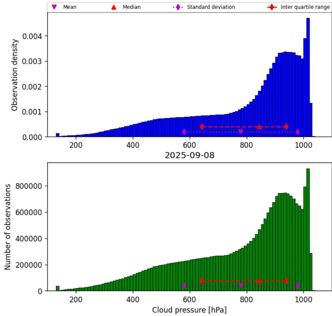
Figure 30: Histogram of “Cloud pressure” for 2025-09-07 to 2025-09-09
