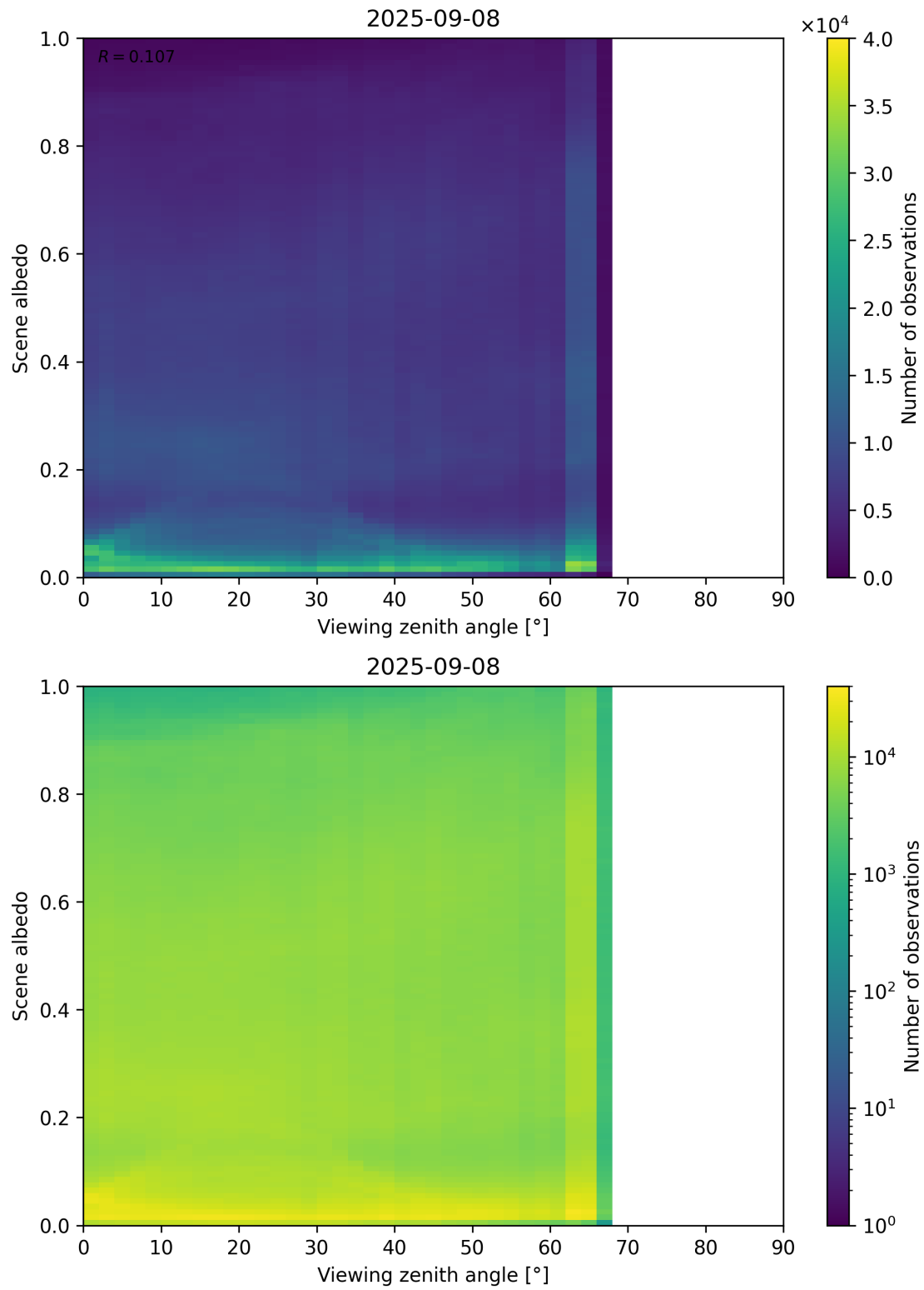
Figure 126: Scatter density plot of “Viewing zenith angle” against “Scene albedo” for 2025-09-07 to 2025-09-09.
