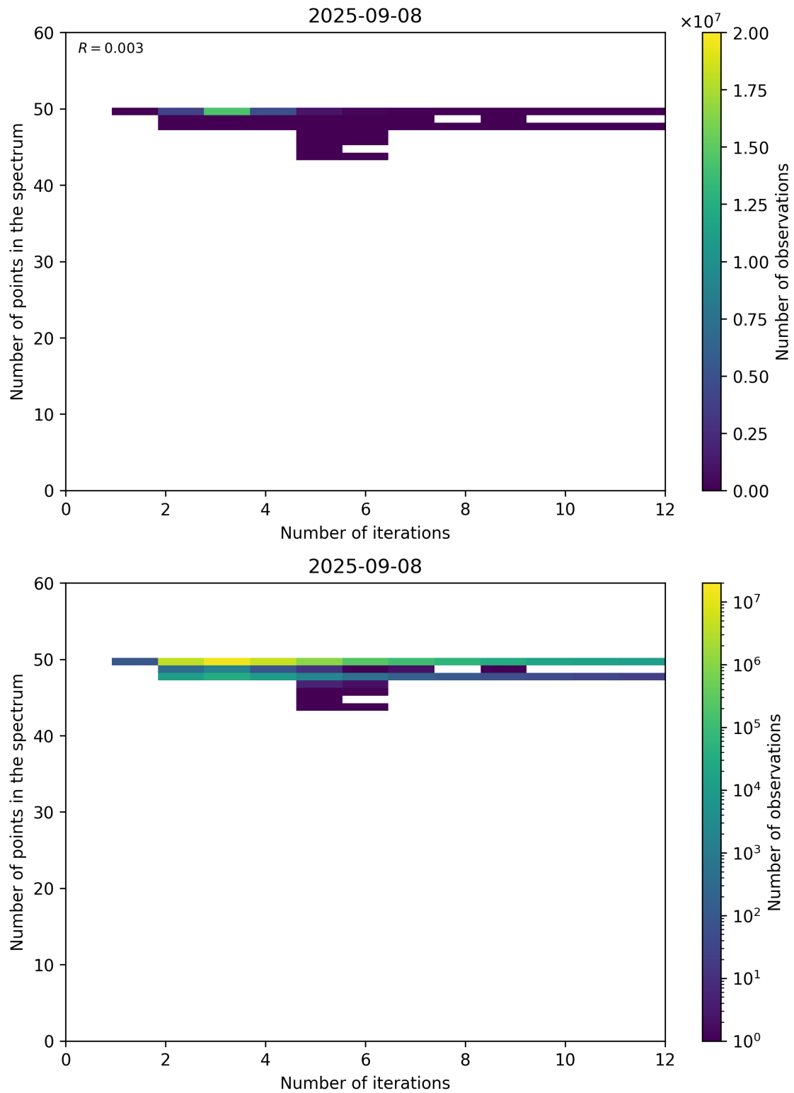
Figure 99: Scatter density plot of “Number of iterations” against “Number of points in the spectrum” for 2025-09-07 to 2025-09-09.
