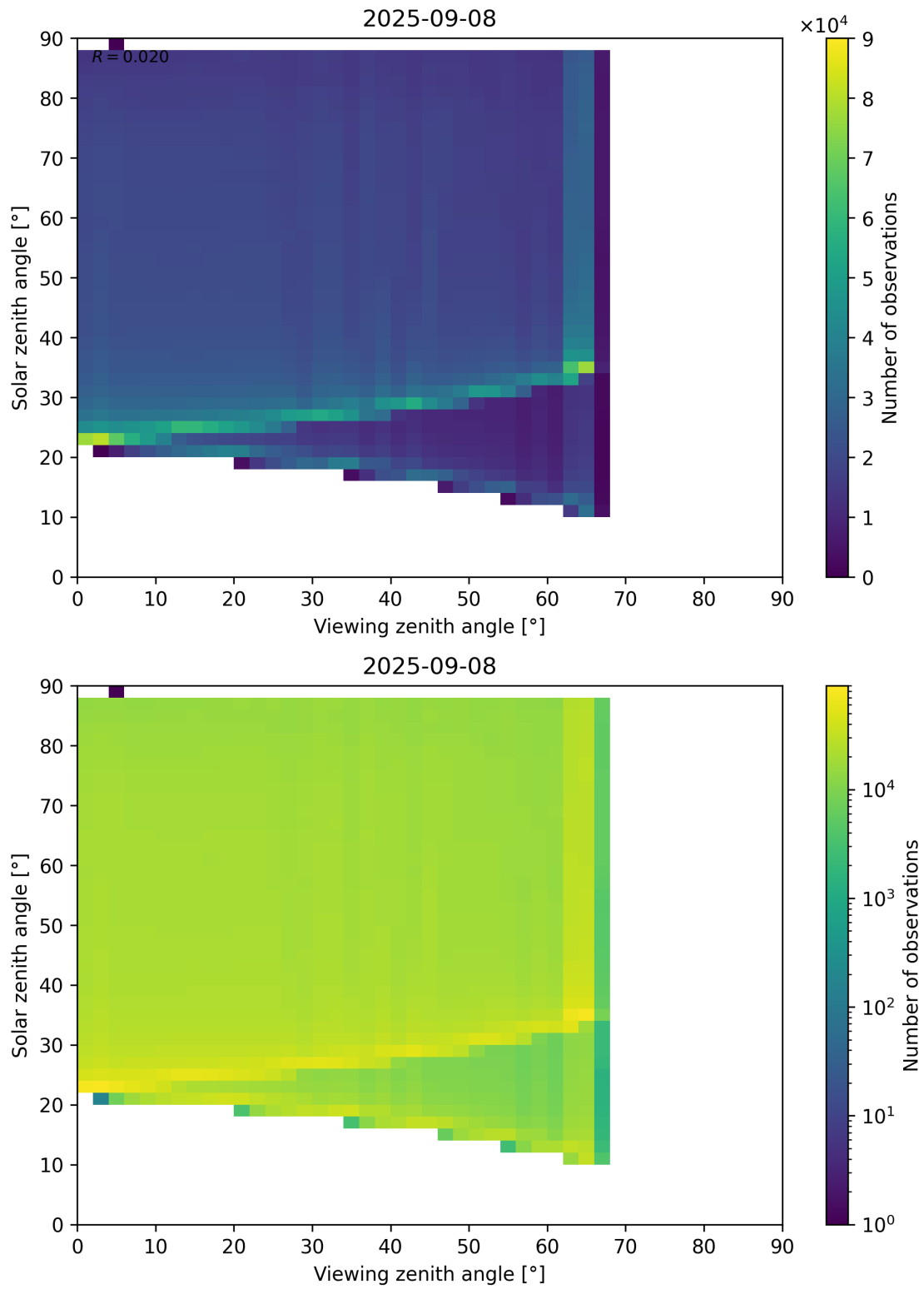
Figure 127: Scatter density plot of “Viewing zenith angle” against “Solar zenith angle” for 2025-09-07 to 2025-09-09.
