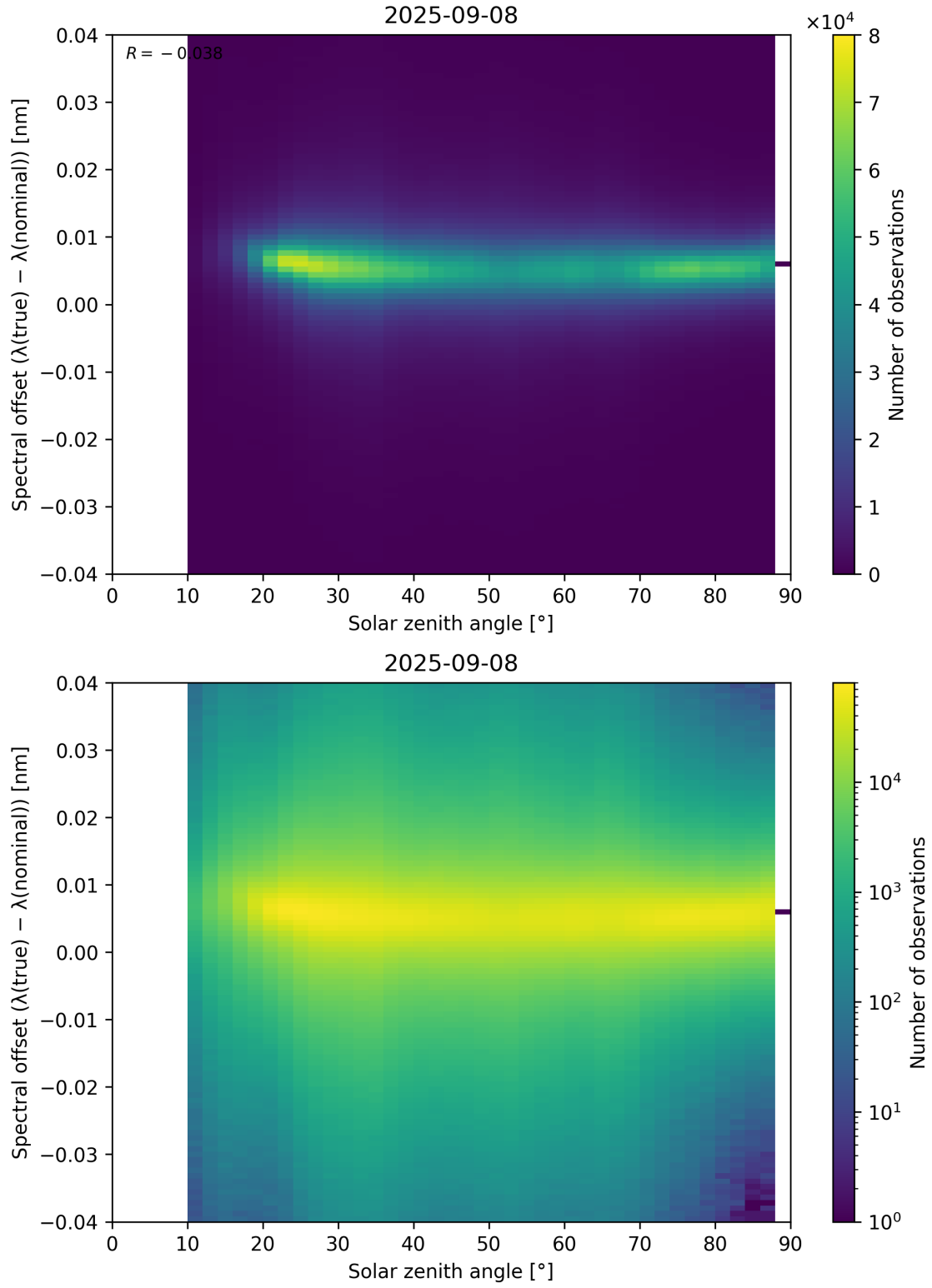
Figure 117: Scatter density plot of “Solar zenith angle” against “Spectral offset ( \lambda_{\text{true}} - \lambda_{\text{nominal}} )” for 2025-09-07 to 2025-09-09.
