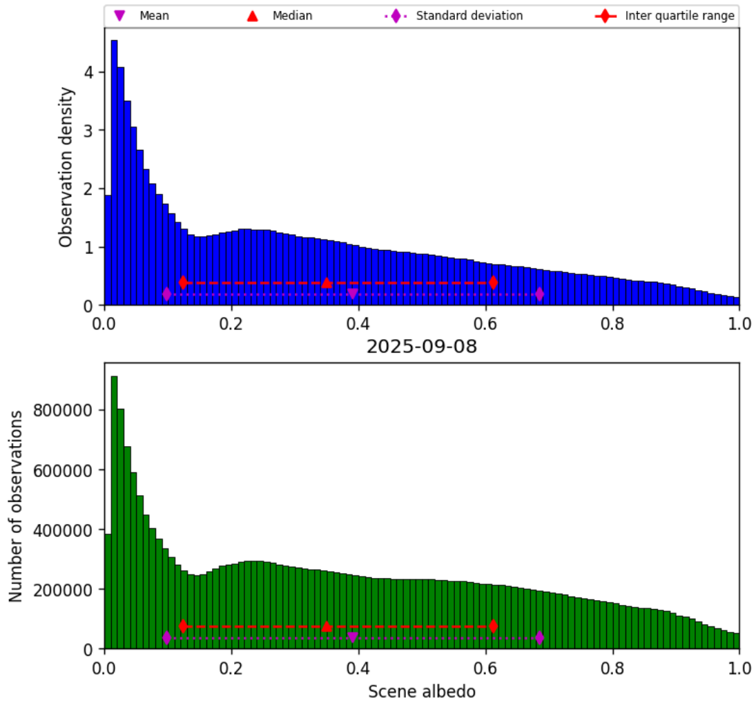
Figure 34: Histogram of “Scene albedo” for 2025-09-07 to 2025-09-09
