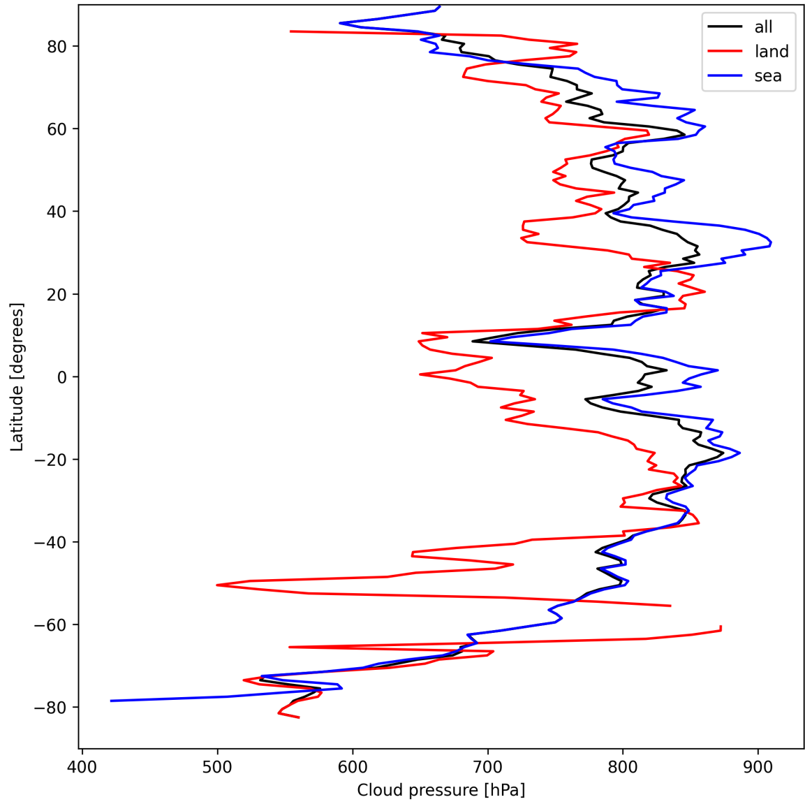
Figure 13: Zonal average of “Cloud pressure” for 2025-09-07 to 2025-09-09.
