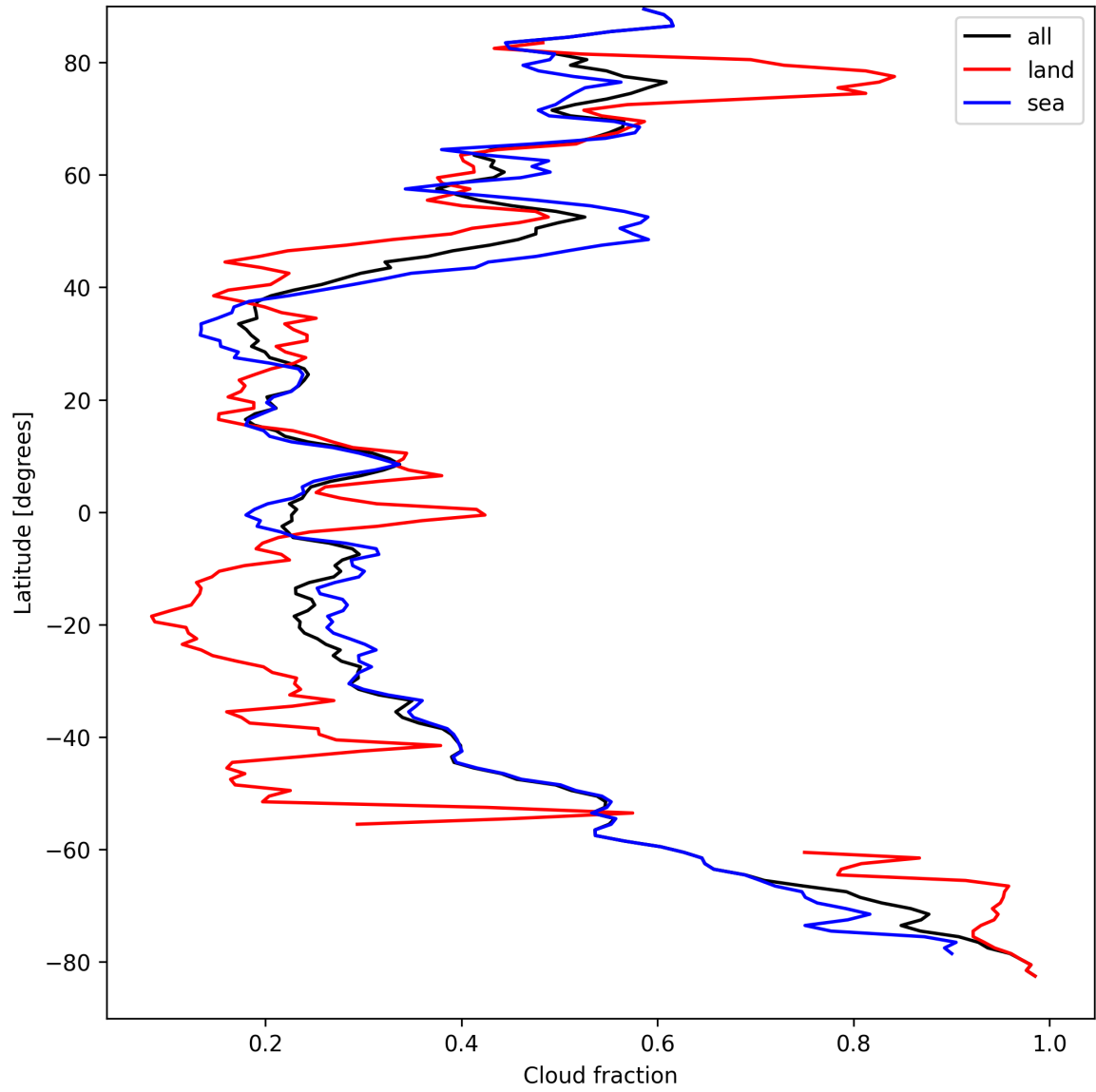
Figure 15: Zonal average of “Cloud fraction” for 2025-09-07 to 2025-09-09.
