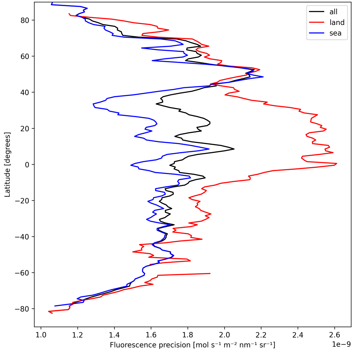
Figure 24: Zonal average of “Fluorescence precision” for 2025-09-07 to 2025-09-09.
