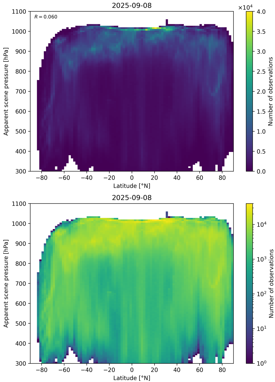
Figure 88: Scatter density plot of “Latitude” against “Apparent scene pressure” for 2025-09-07 to 2025-09-09.
