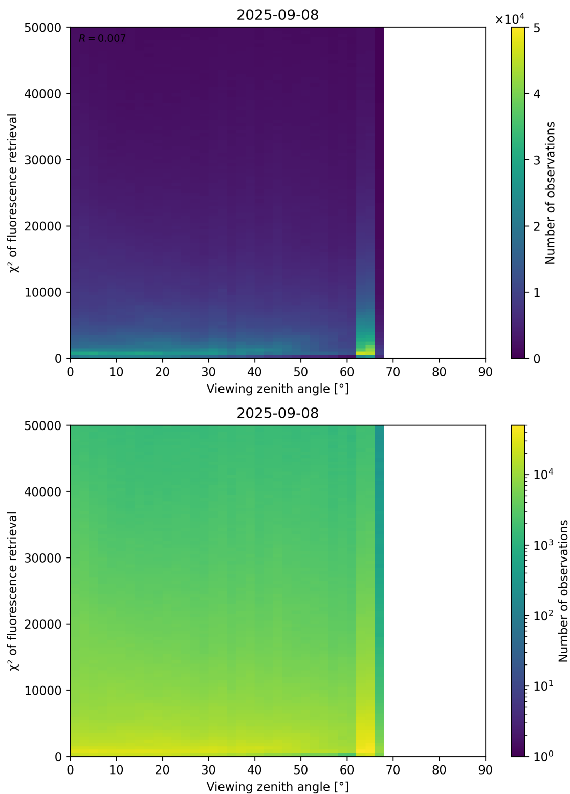
Figure 119: Scatter density plot of “Viewing zenith angle” against “ \chi^2 of fluorescence retrieval” for 2025-09-07 to 2025-09-09.
