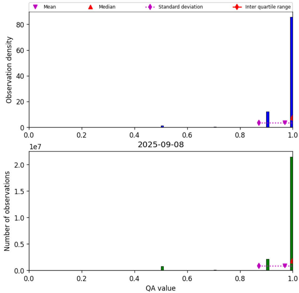
Figure 29: Histogram of “QA value” for 2025-09-07 to 2025-09-09
