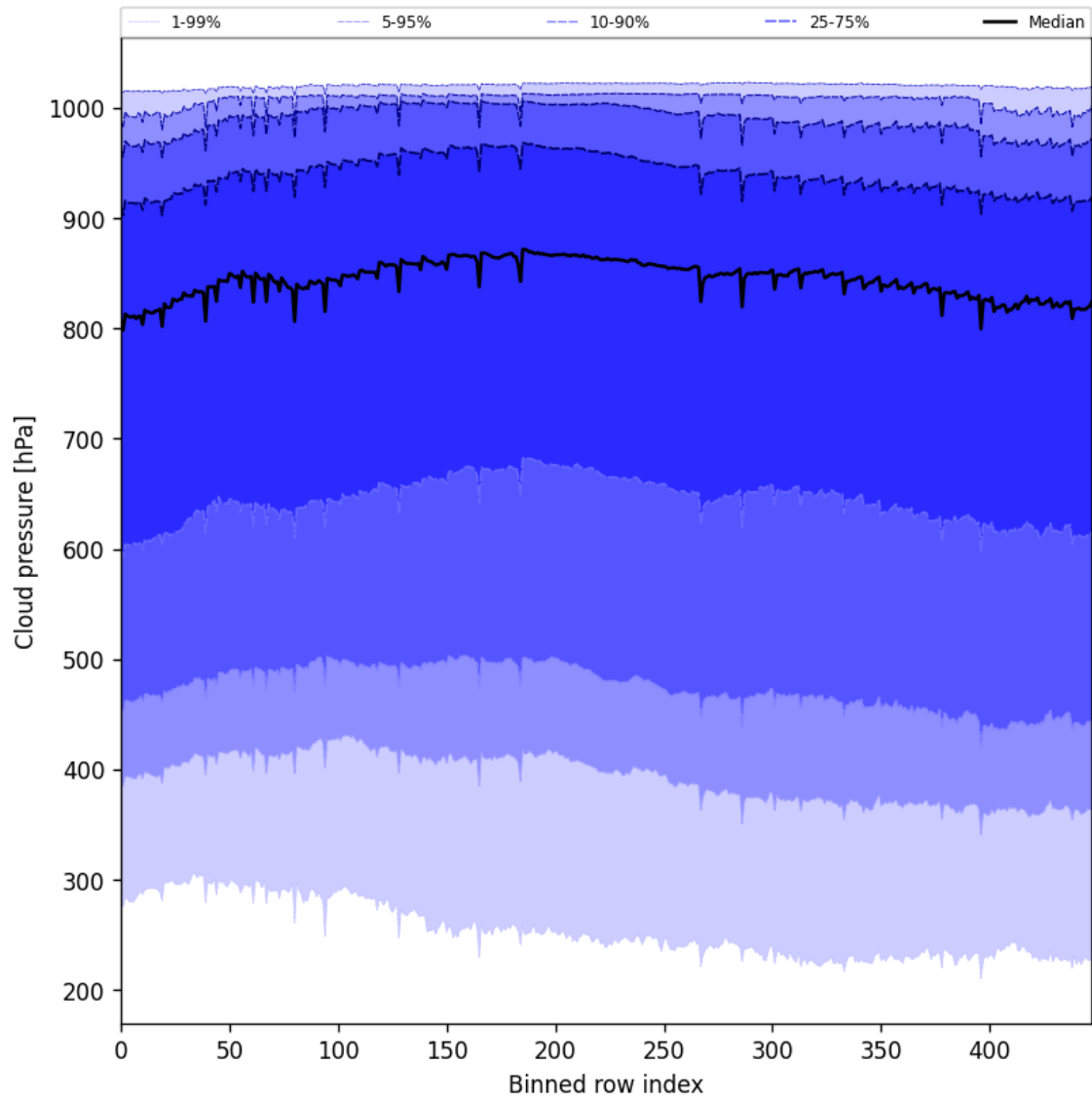
Figure 47: Along track statistics of “Cloud pressure” for 2025-09-07 to 2025-09-09
