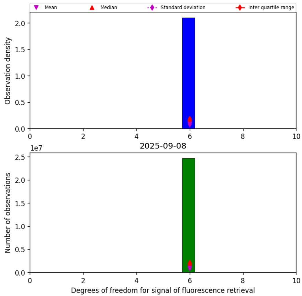
Figure 43: Histogram of "Degrees of freedom for signal of fluorescence retrieval" for 2025-09-07 to 2025-09-09
