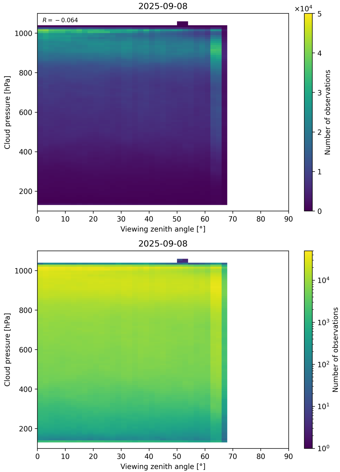
Figure 121: Scatter density plot of “Viewing zenith angle” against “Cloud pressure” for 2025-09-07 to 2025-09-09.
