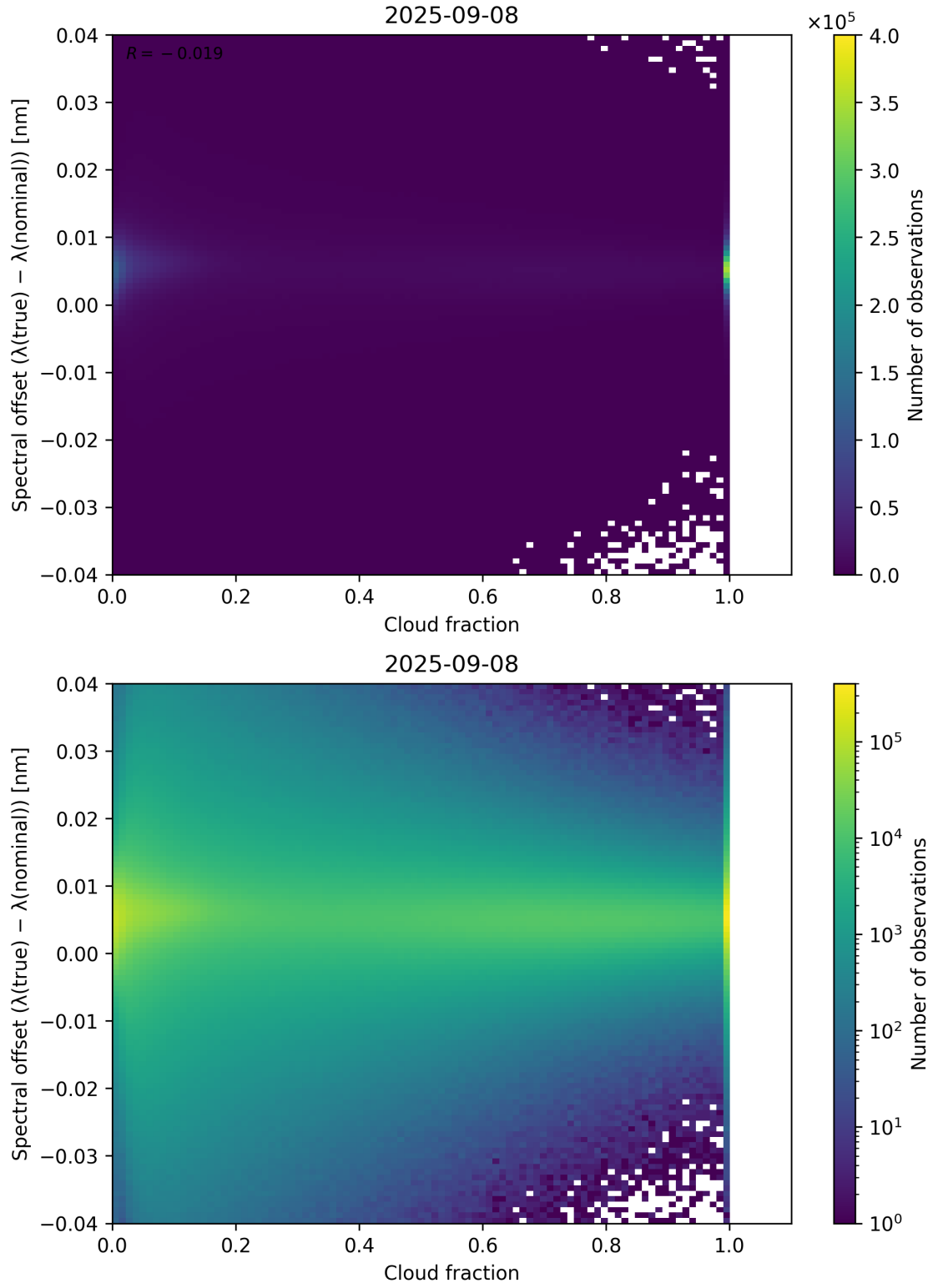
Figure 76: Scatter density plot of “Cloud fraction” against “Spectral offset ( \lambda_{\text{true}} - \lambda_{\text{nominal}} )” for 2025-09-07 to 2025-09-09.
