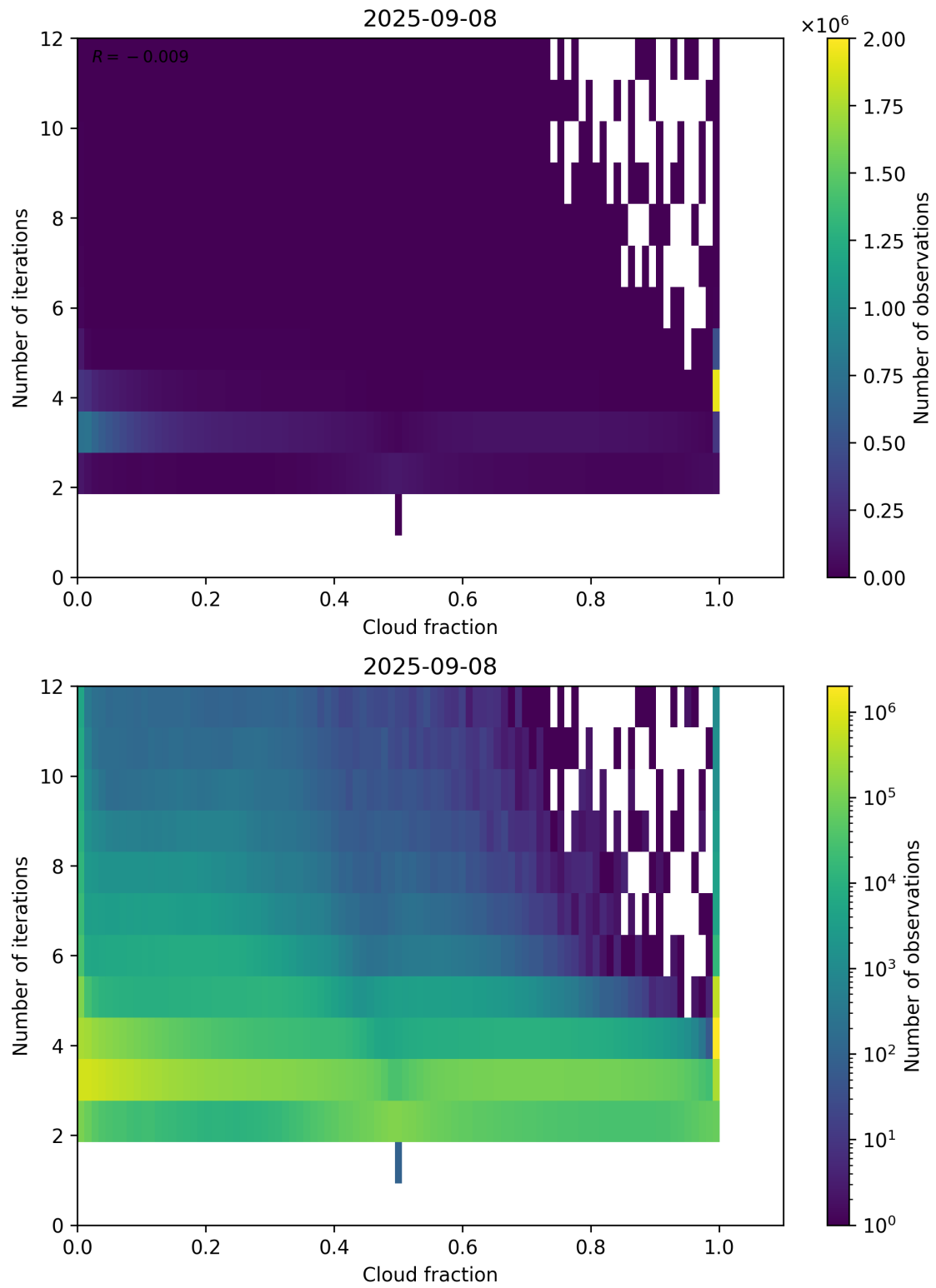
Figure 73: Scatter density plot of “Cloud fraction” against “Number of iterations” for 2025-09-07 to 2025-09-09.
