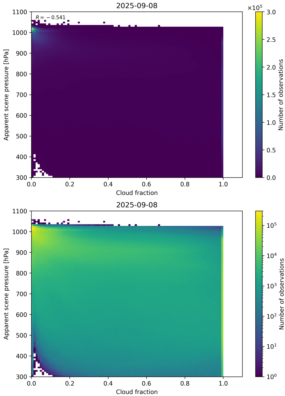
Figure 70: Scatter density plot of “Cloud fraction” against “Apparent scene pressure” for 2025-09-07 to 2025-09-09.
