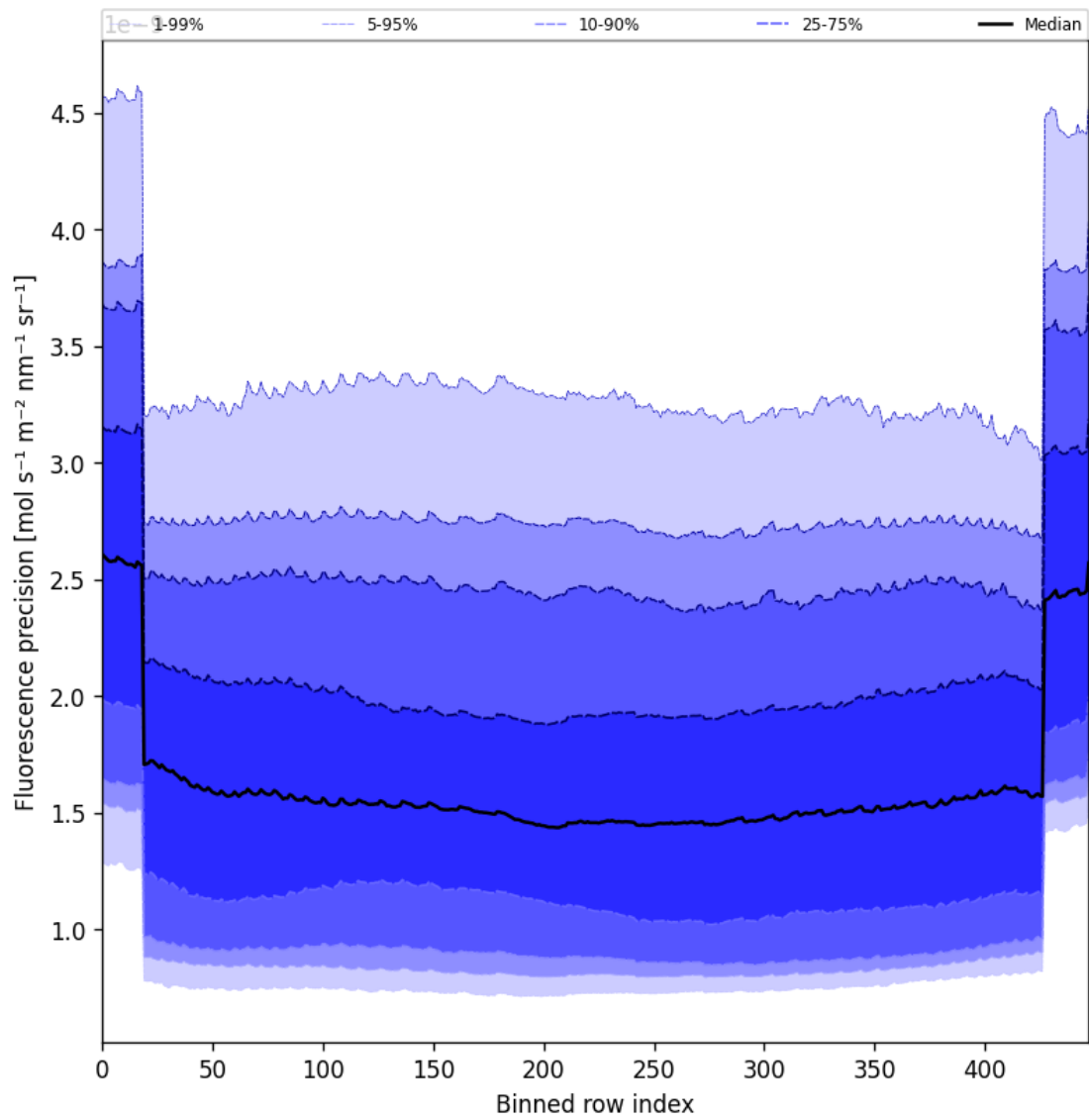
Figure 58: Along track statistics of “Fluorescence precision” for 2025-09-07 to 2025-09-09
