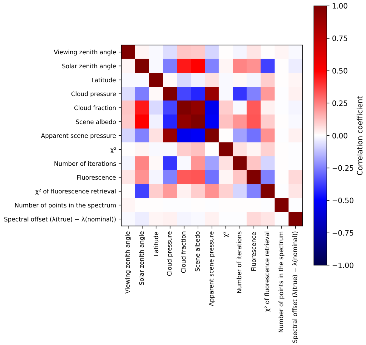
Figure 2: Map of correlation matrix for 2025-09-07 to 2025-09-09.
