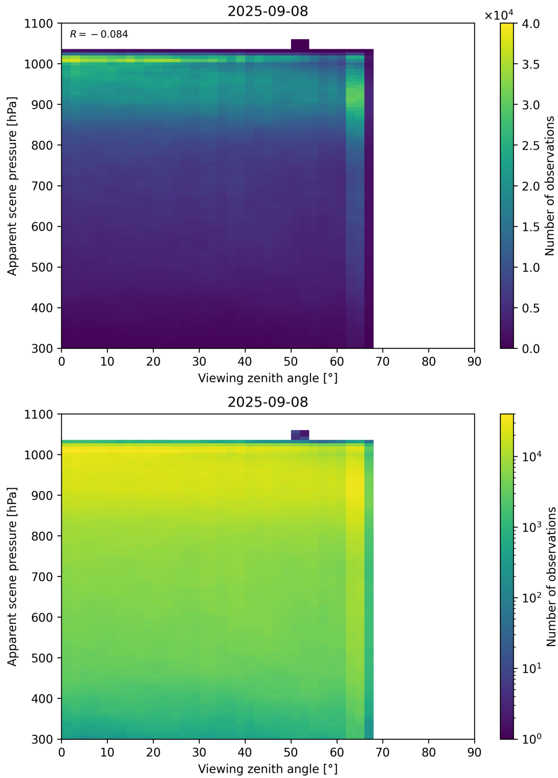
Figure 118: Scatter density plot of “Viewing zenith angle” against “Apparent scene pressure” for 2025-09-07 to 2025-09-09.
