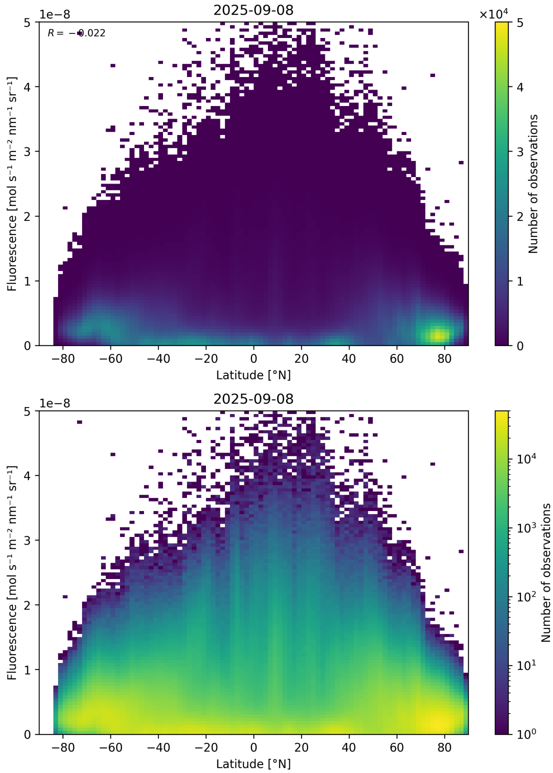
Figure 92: Scatter density plot of “Latitude” against “Fluorescence” for 2025-09-07 to 2025-09-09.
