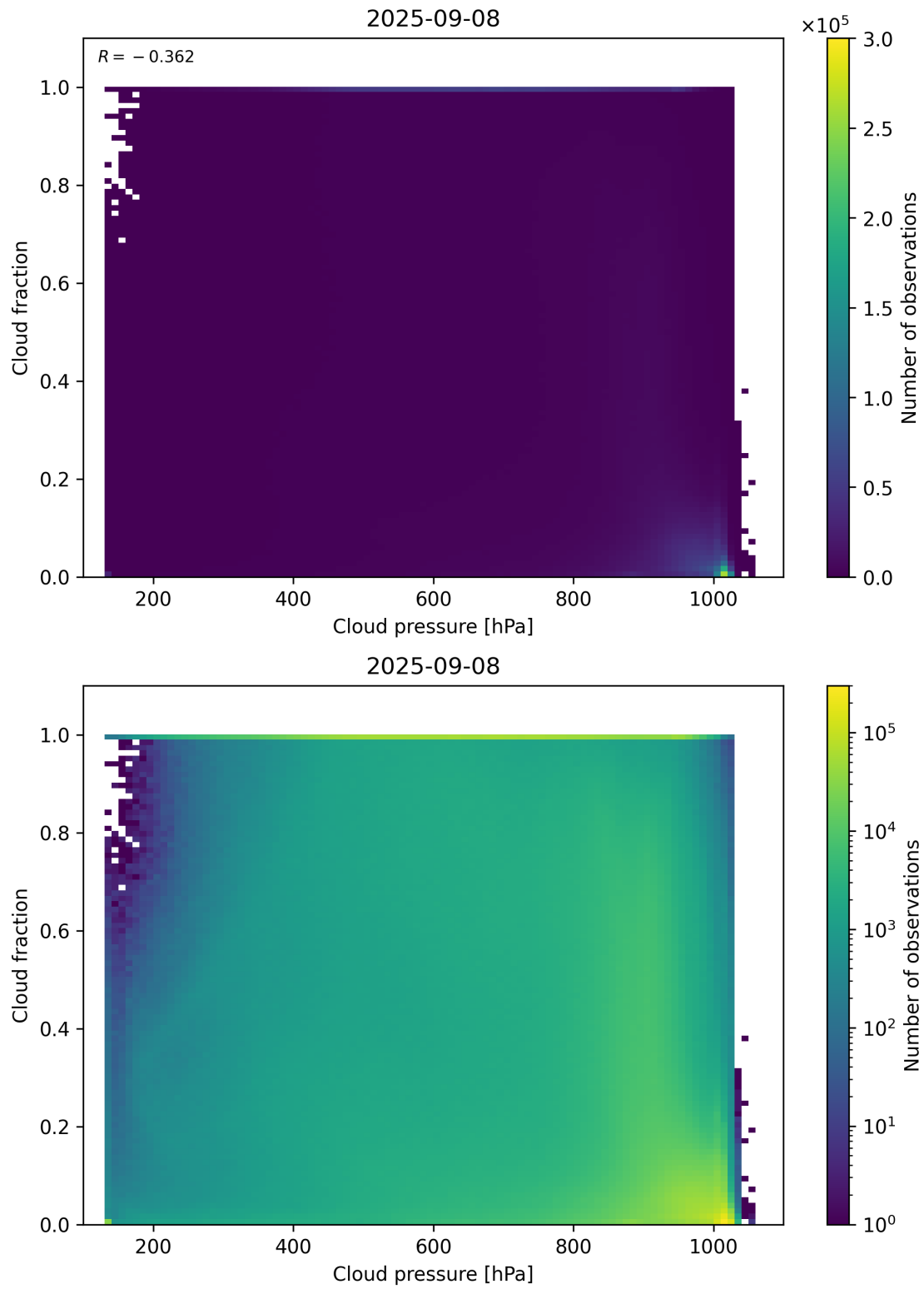
Figure 79: Scatter density plot of “Cloud pressure” against “Cloud fraction” for 2025-09-07 to 2025-09-09.
