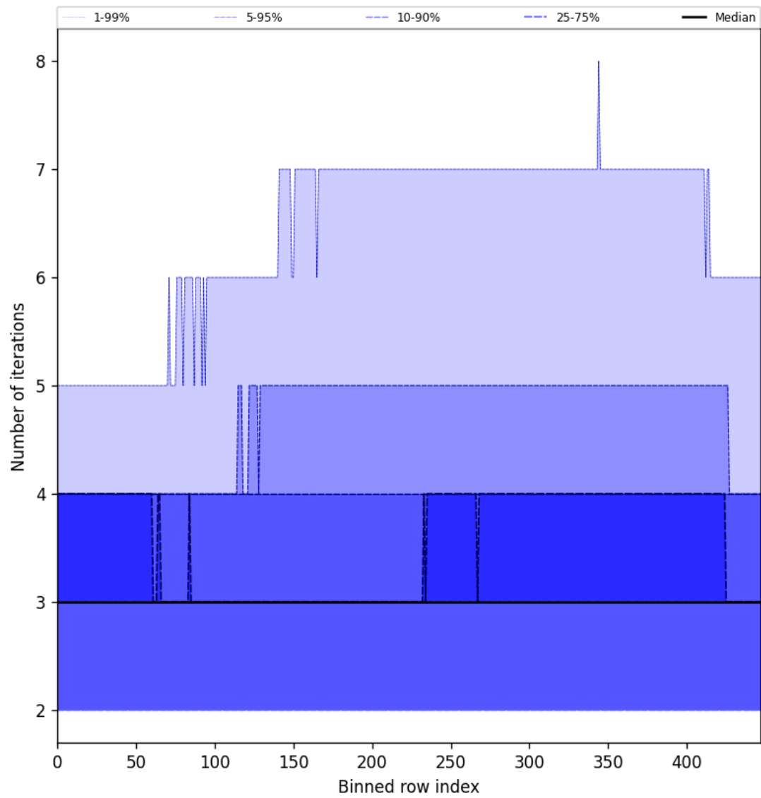
Figure 56: Along track statistics of “Number of iterations” for 2025-09-07 to 2025-09-09
