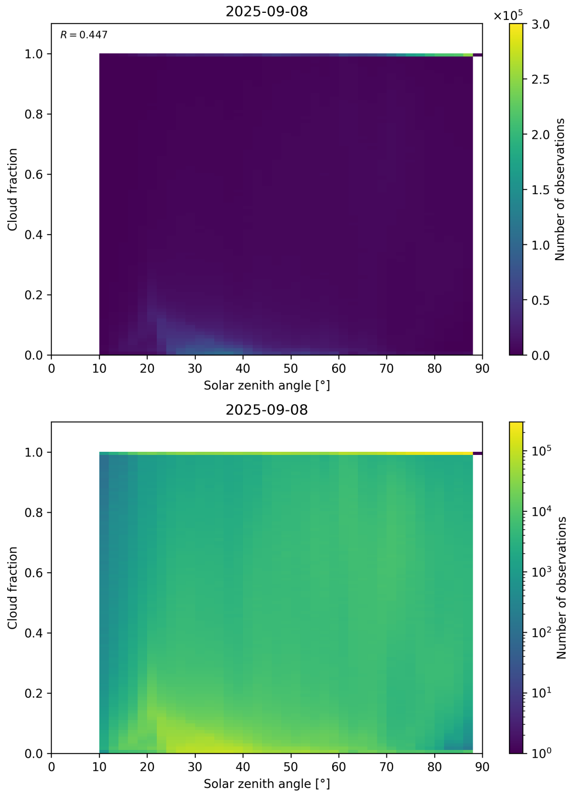
Figure 110: Scatter density plot of “Solar zenith angle” against “Cloud fraction” for 2025-09-07 to 2025-09-09.
