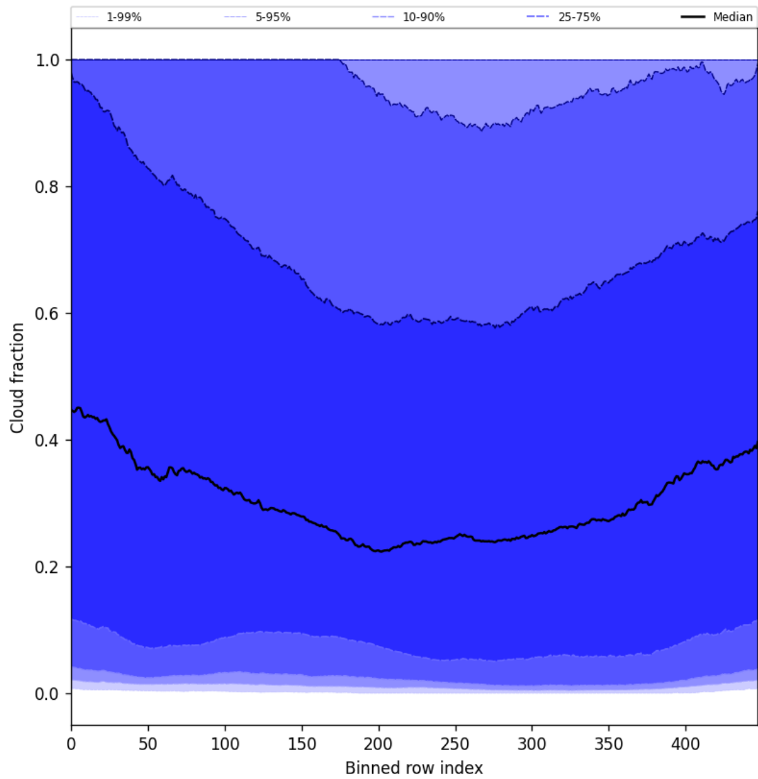
Figure 49: Along track statistics of “Cloud fraction” for 2025-09-07 to 2025-09-09
