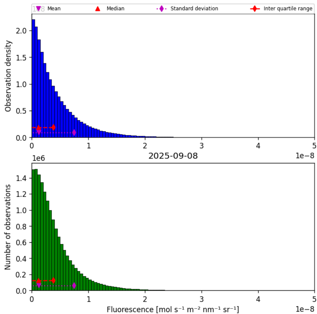
Figure 40: Histogram of “Fluorescence” for 2025-09-07 to 2025-09-09
