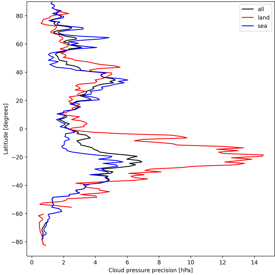
Figure 14: Zonal average of “Cloud pressure precision” for 2025-09-07 to 2025-09-09.
