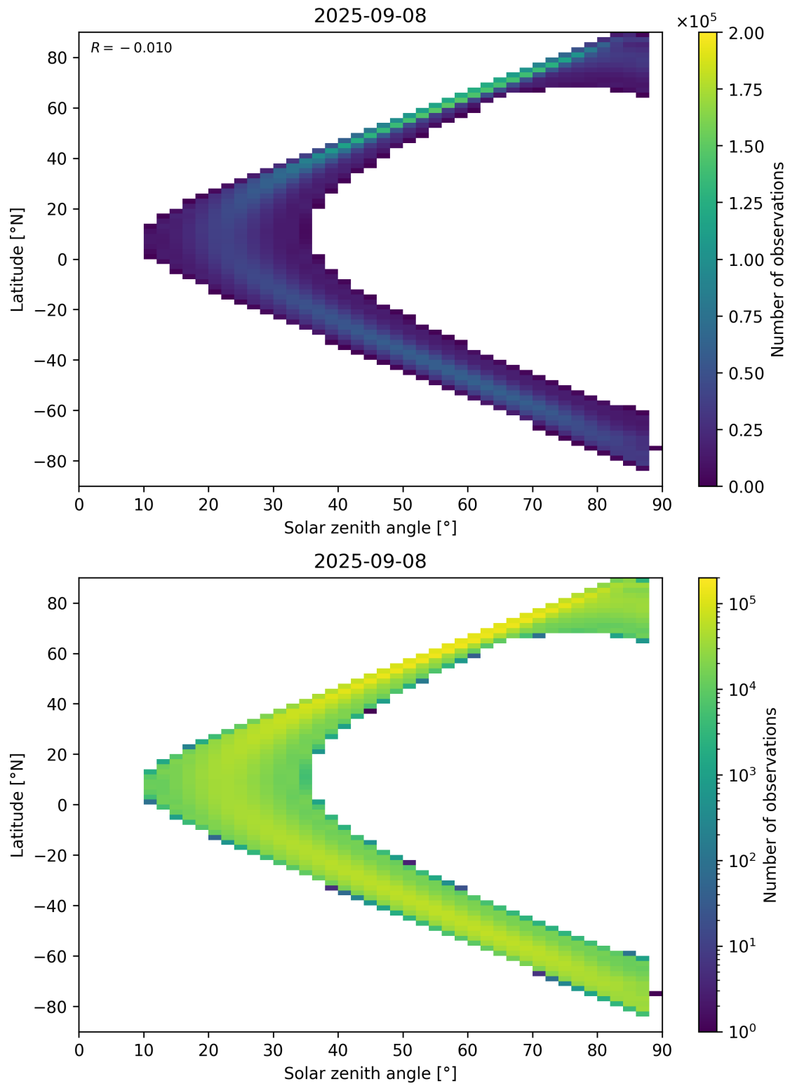
Figure 113: Scatter density plot of “Solar zenith angle” against “Latitude” for 2025-09-07 to 2025-09-09.
