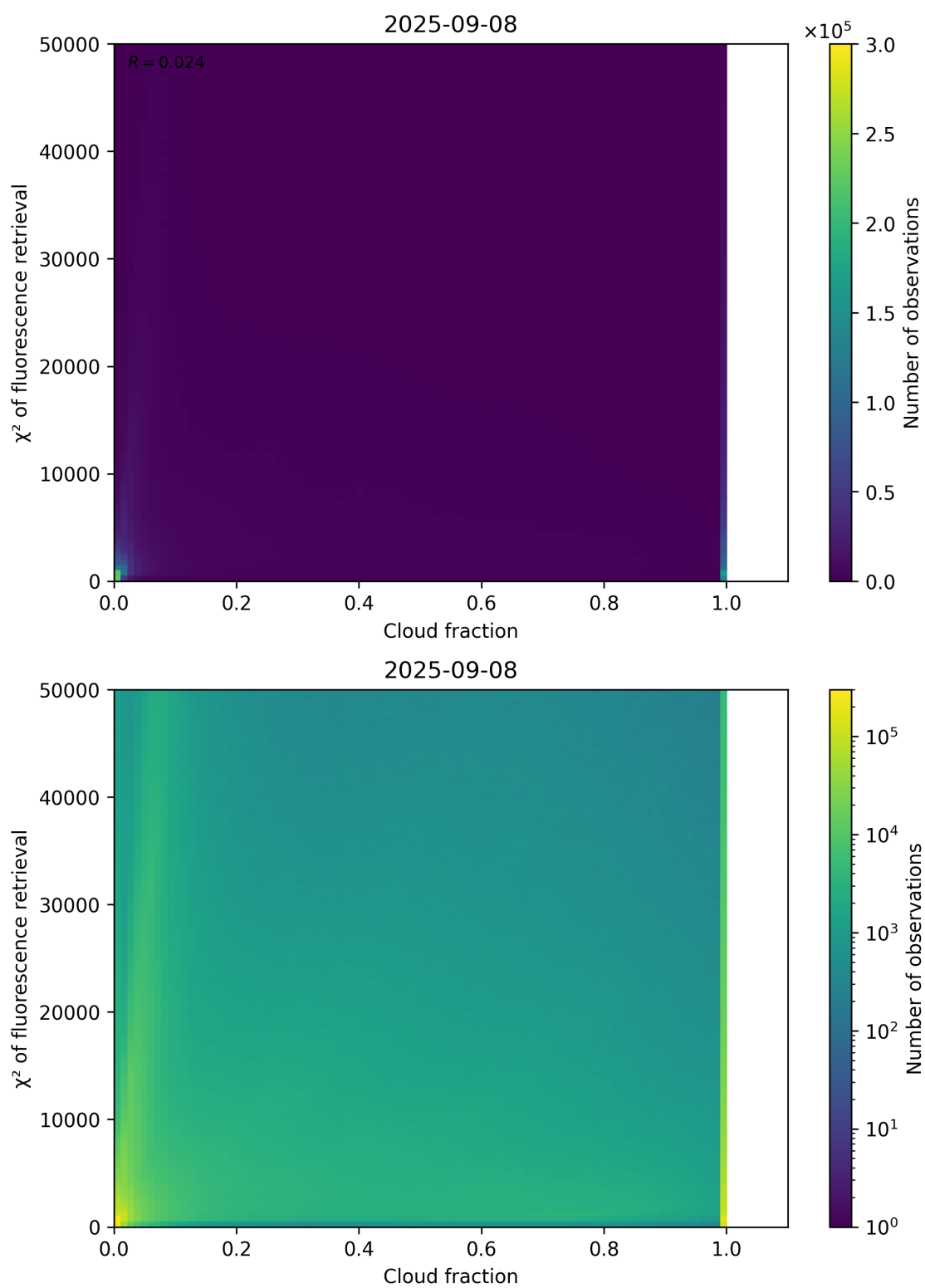
Figure 71: Scatter density plot of “Cloud fraction” against “ \chi^2 of fluorescence retrieval” for 2025-09-07 to 2025-09-09.
