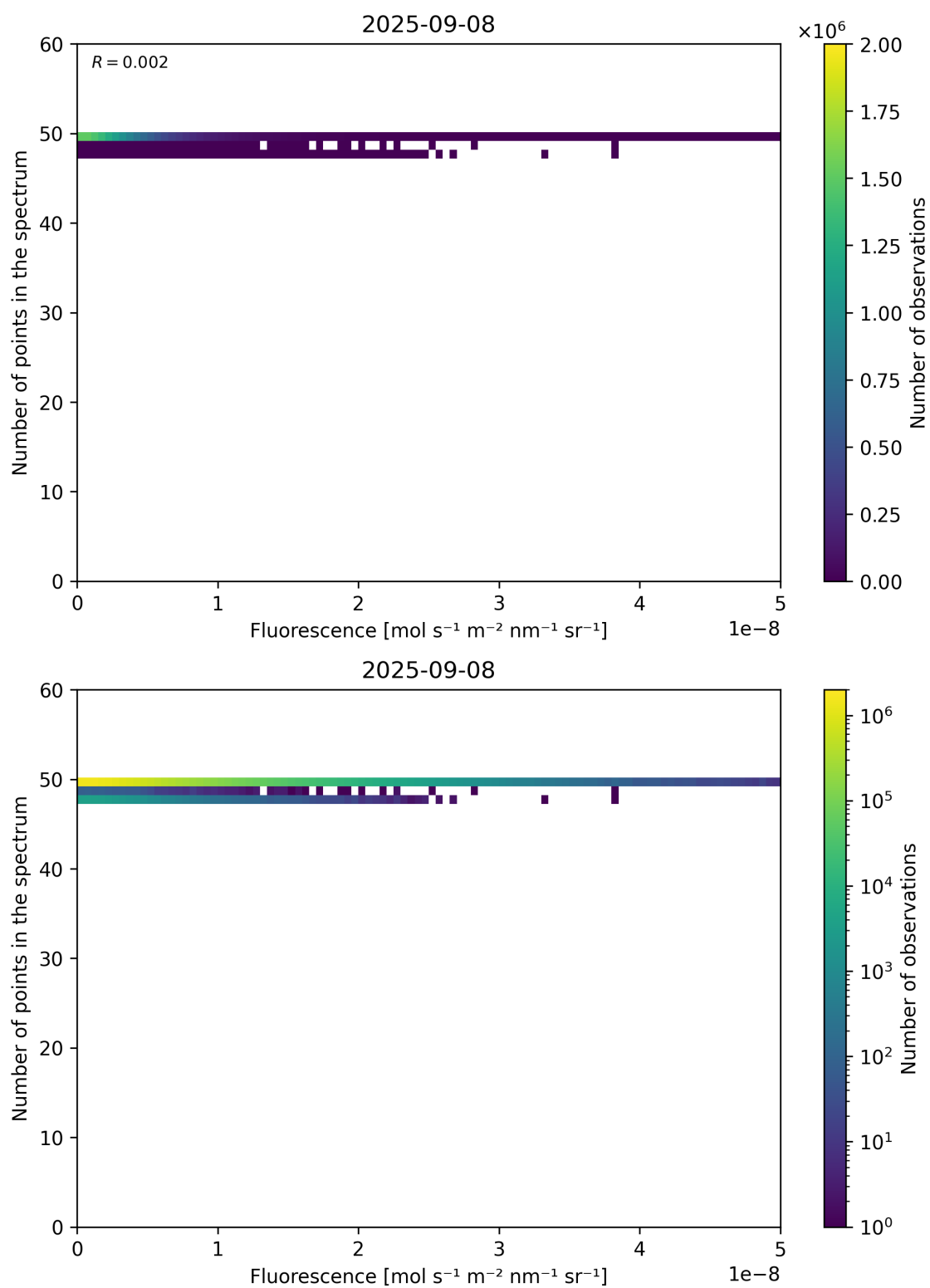
Figure 86: Scatter density plot of “Fluorescence” against “Number of points in the spectrum” for 2025-09-07 to 2025-09-09.
