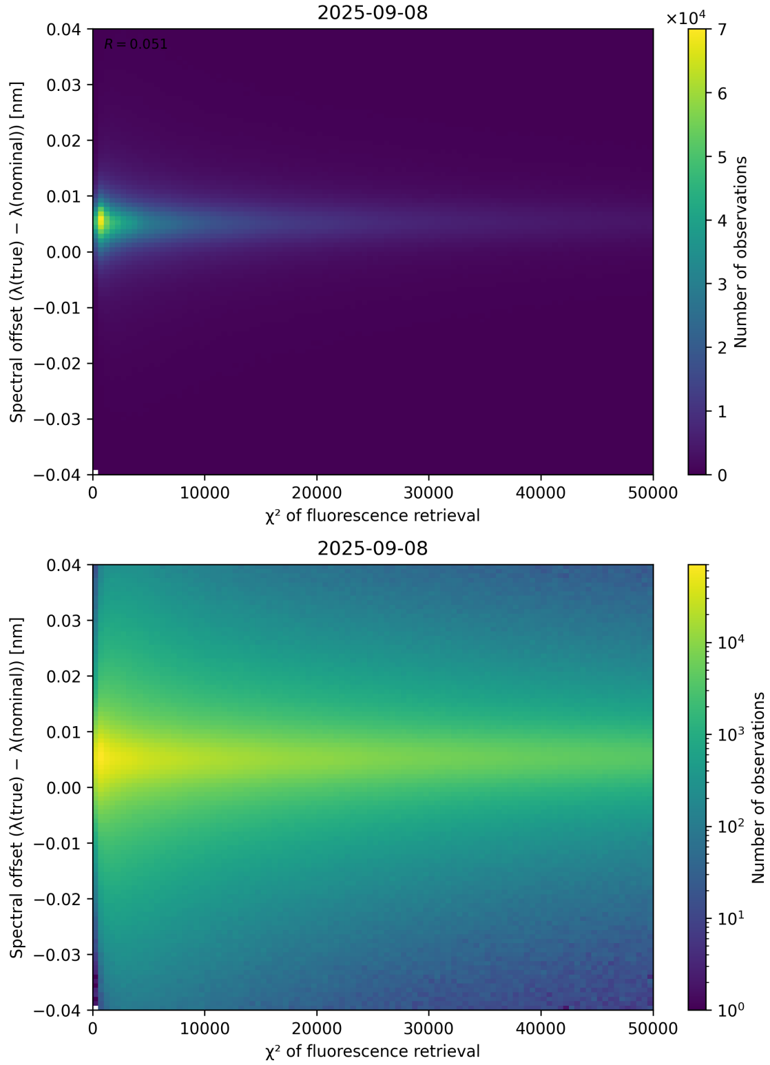
Figure 69: Scatter density plot of “ \chi^2 of fluorescence retrieval” against “Spectral offset ( \lambda_{\text{true}} - \lambda_{\text{nominal}} )” for 2025-09-07 to 2025-09-09.
