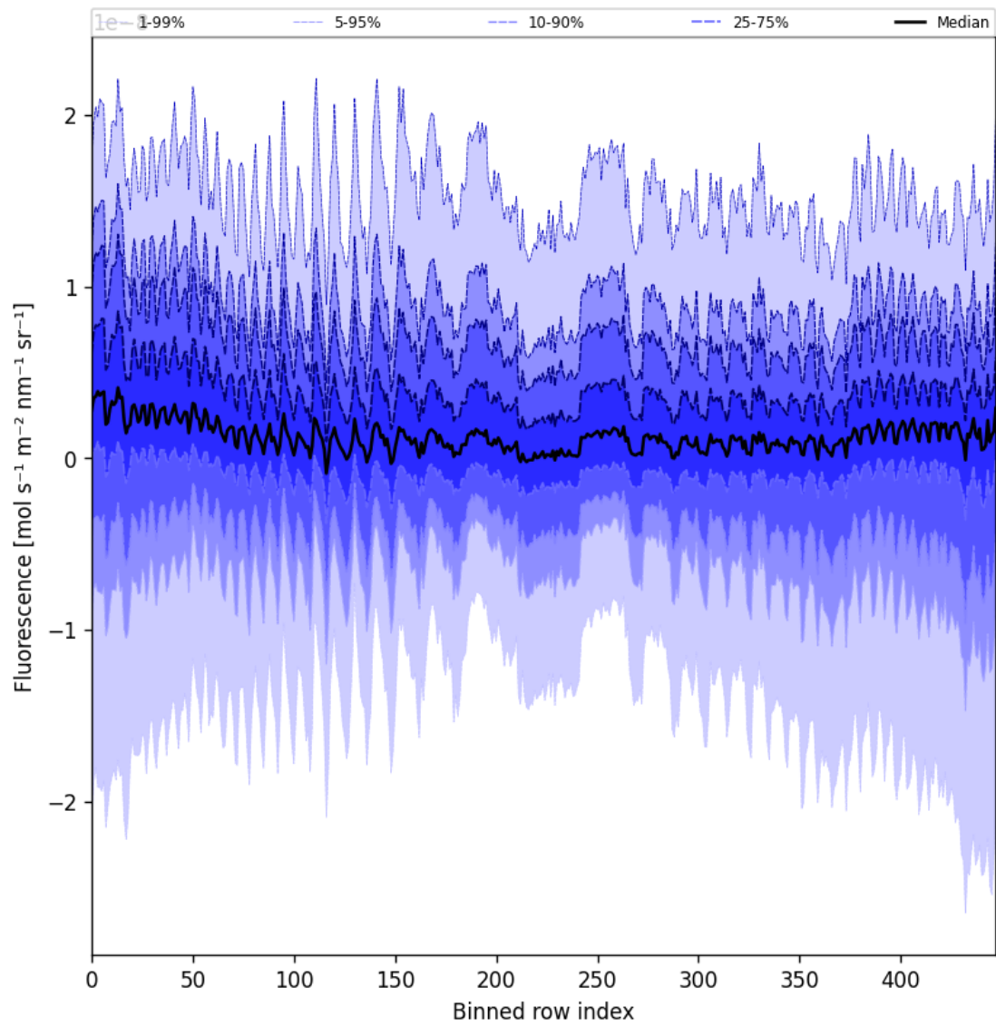
Figure 57: Along track statistics of “Fluorescence” for 2025-09-07 to 2025-09-09
