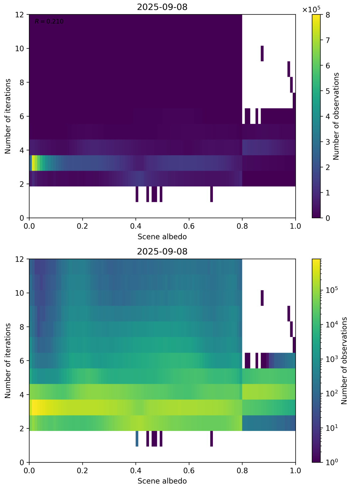
Figure 105: Scatter density plot of “Scene albedo” against “Number of iterations” for 2025-09-07 to 2025-09-09.
