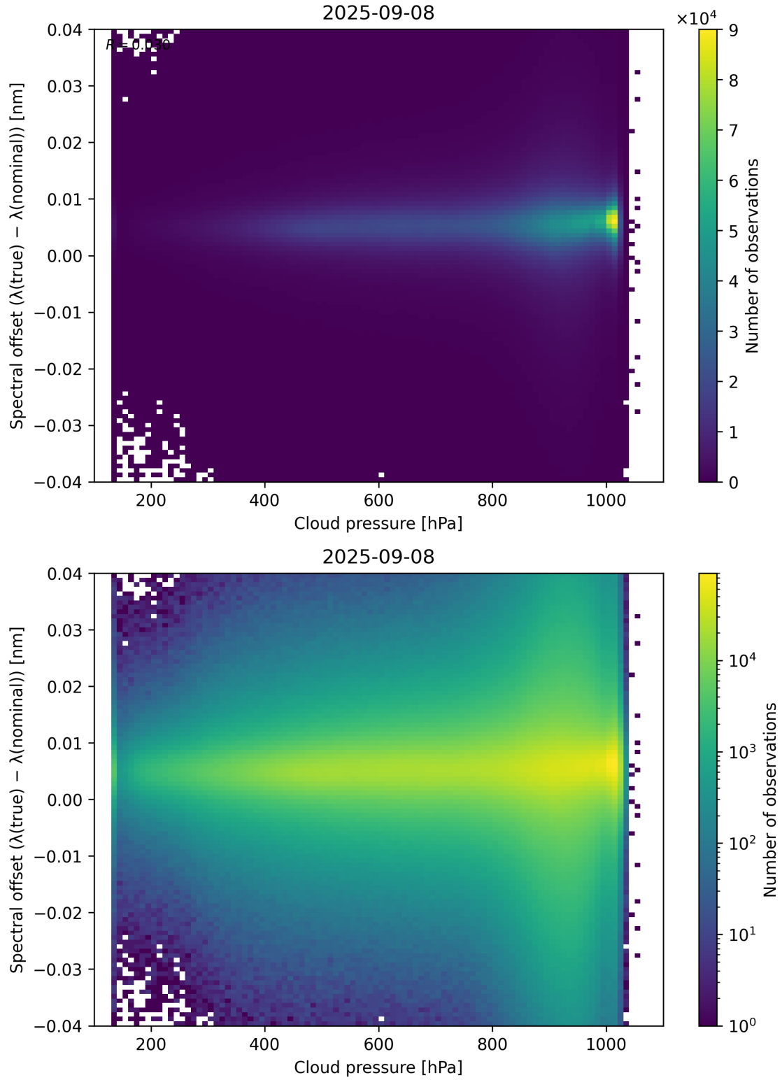
Figure 84: Scatter density plot of “Cloud pressure” against “Spectral offset ( \lambda_{\text{true}} - \lambda_{\text{nominal}} )” for 2025-09-07 to 2025-09-09.
