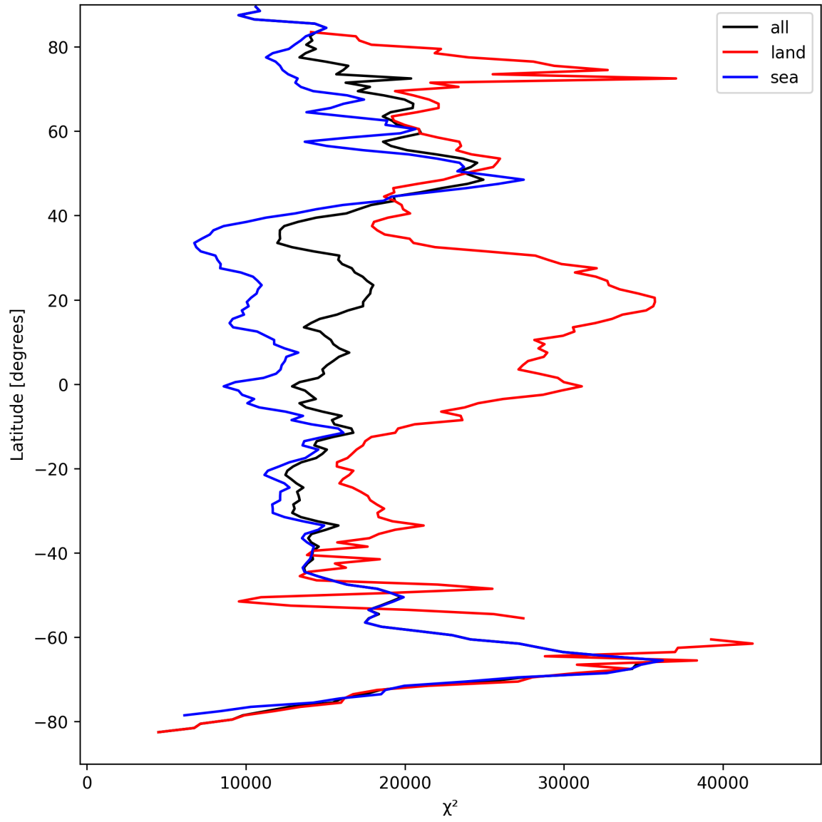
Figure 21: Zonal average of “ \chi^2 ” for 2025-09-07 to 2025-09-09.
