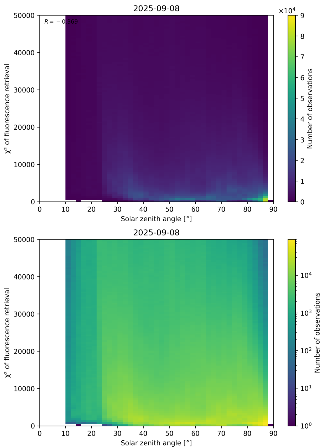
Figure 109: Scatter density plot of “Solar zenith angle” against “ \chi^2 of fluorescence retrieval” for 2025-09-07 to 2025-09-09.
