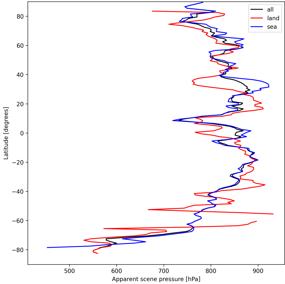
Figure 19: Zonal average of “Apparent scene pressure” for 2025-09-07 to 2025-09-09.
