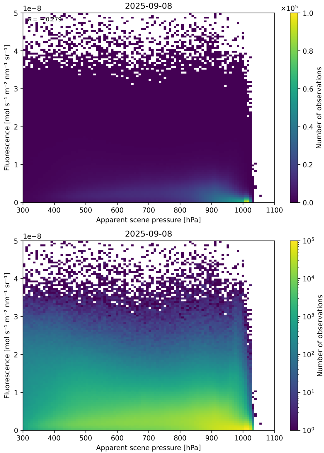
Figure 64: Scatter density plot of “Apparent scene pressure” against “Fluorescence” for 2025-09-07 to 2025-09-09.
