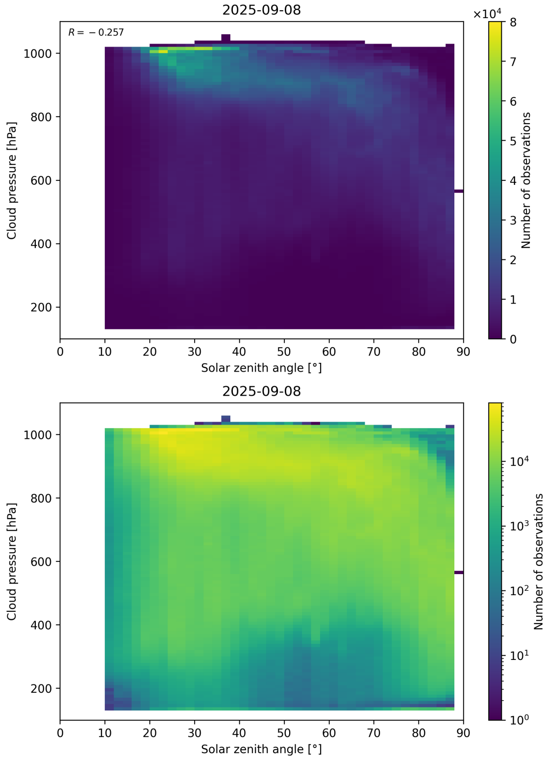
Figure 111: Scatter density plot of “Solar zenith angle” against “Cloud pressure” for 2025-09-07 to 2025-09-09.
