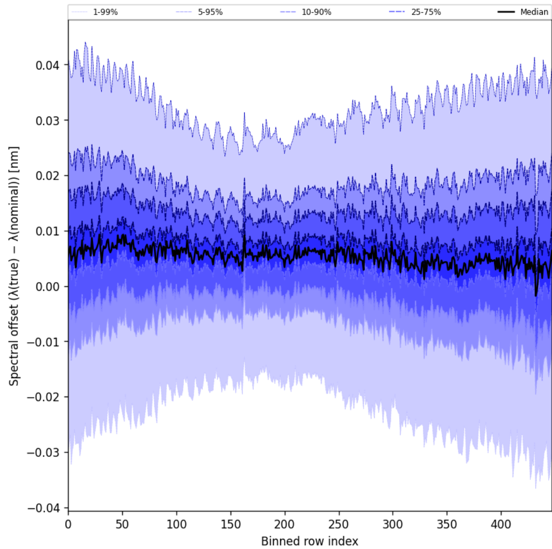
Figure 62: Along track statistics of “Spectral offset ( \lambda_{\text{true}} - \lambda_{\text{nominal}} )” for 2025-09-07 to 2025-09-09
