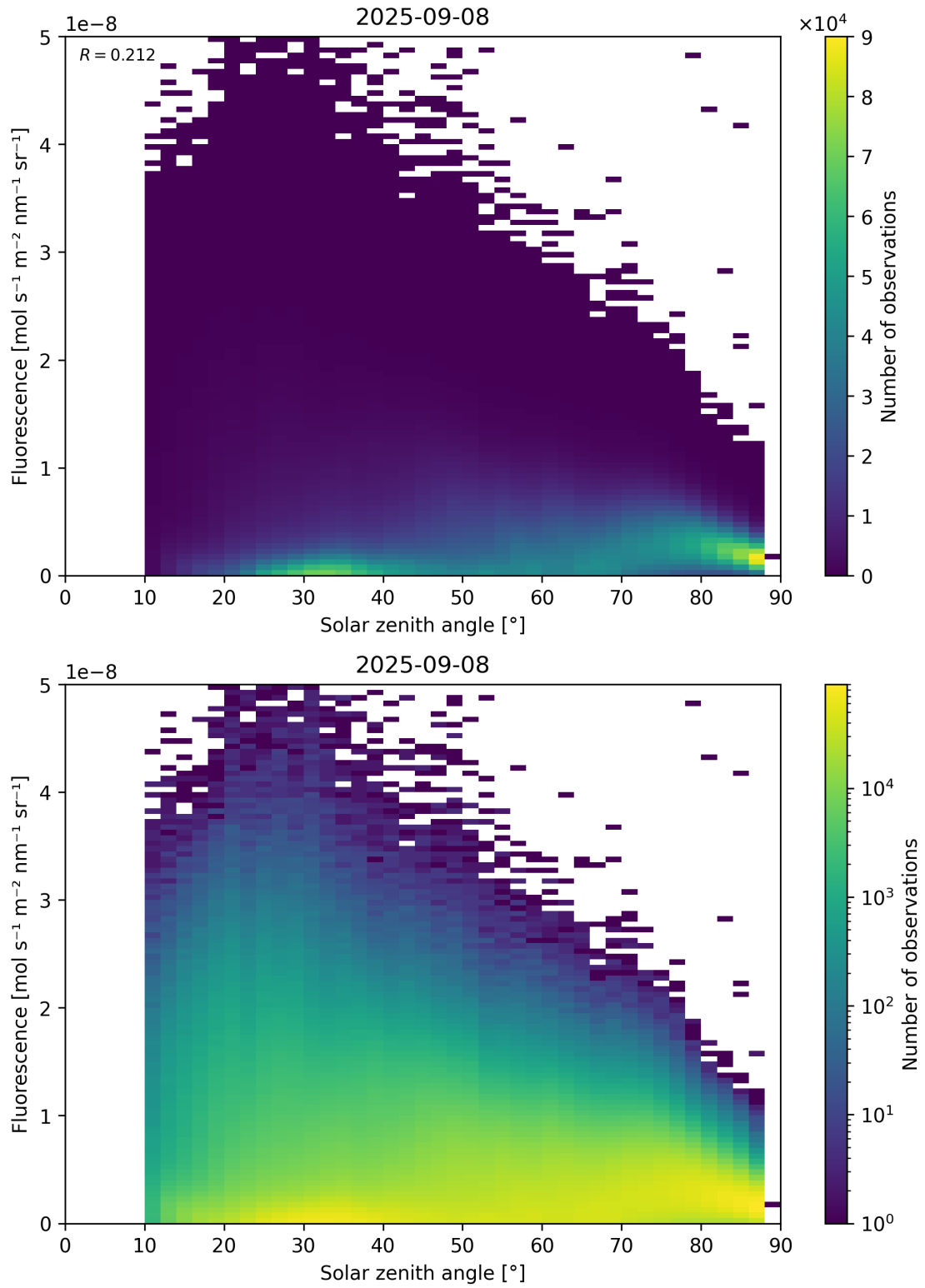
Figure 112: Scatter density plot of “Solar zenith angle” against “Fluorescence” for 2025-09-07 to 2025-09-09.
