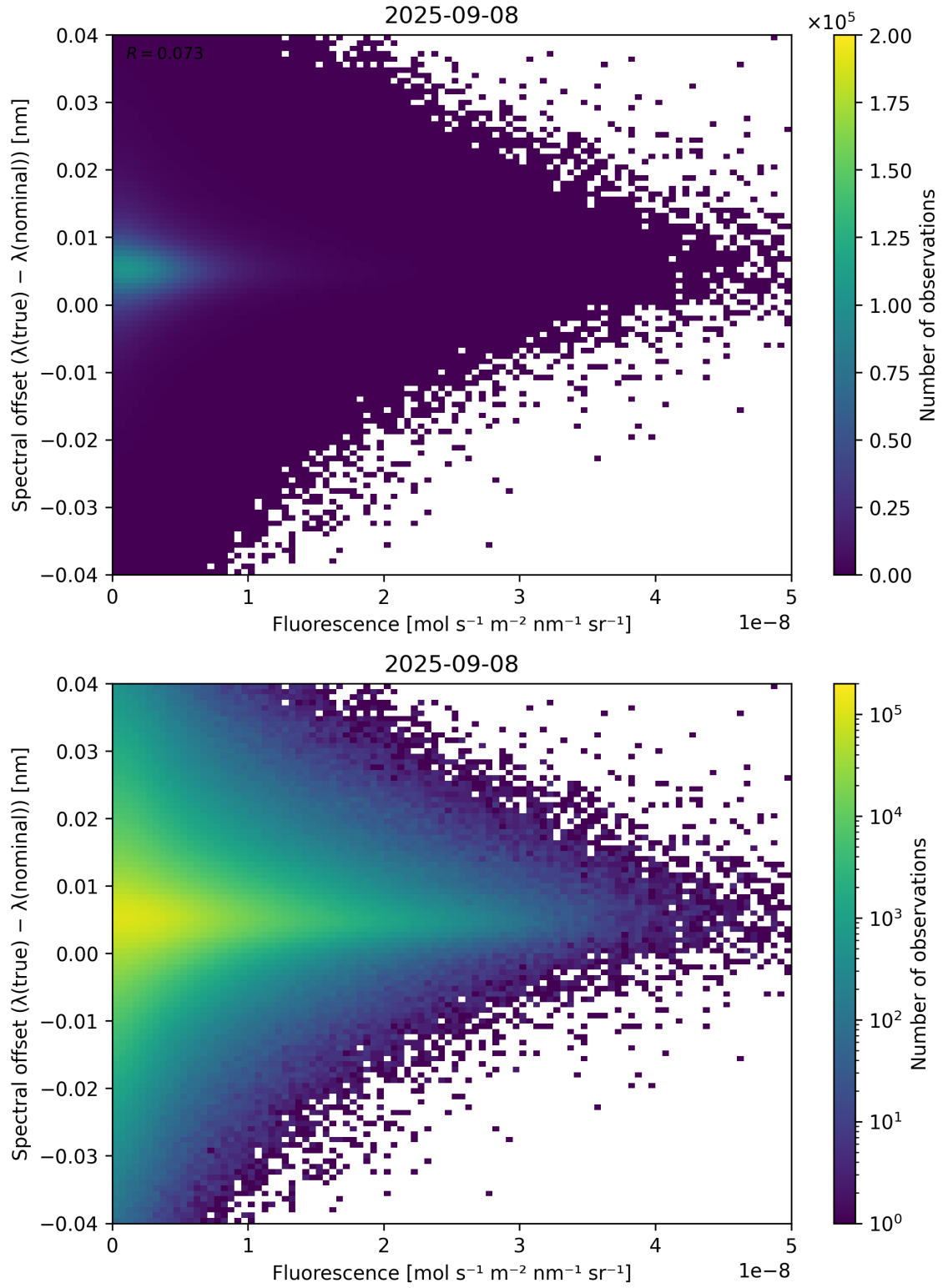
Figure 87: Scatter density plot of “Fluorescence” against “Spectral offset ( \lambda_{\text{true}} - \lambda_{\text{nominal}} )” for 2025-09-07 to 2025-09-09.
