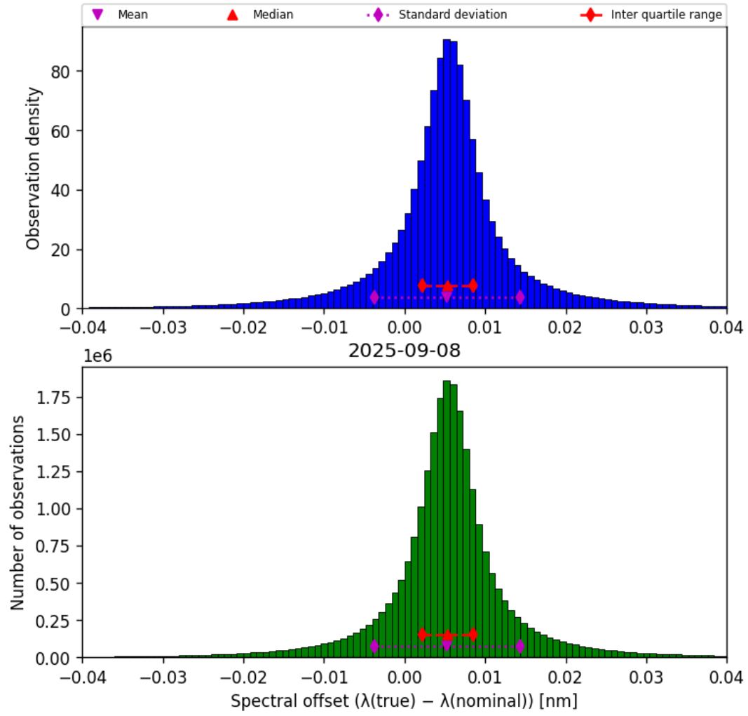
Figure 45: Histogram of “Spectral offset ( \lambda_{\text{true}} - \lambda_{\text{nominal}} )” for 2025-09-07 to 2025-09-09
