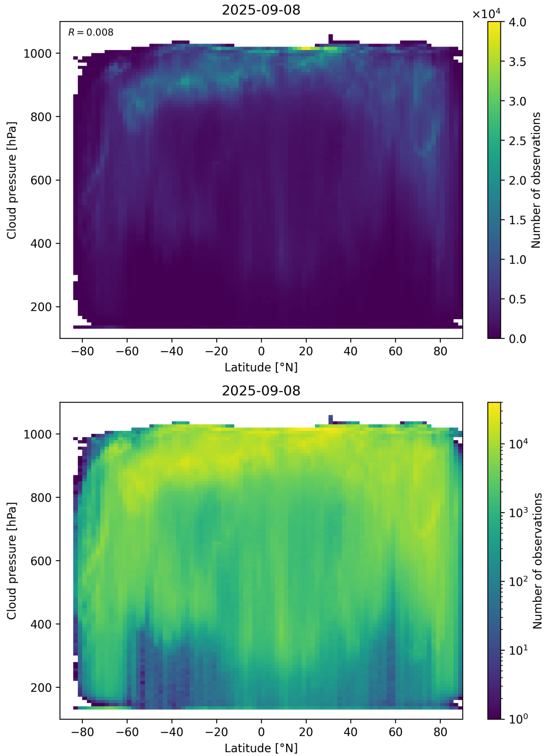
Figure 91: Scatter density plot of “Latitude” against “Cloud pressure” for 2025-09-07 to 2025-09-09.
