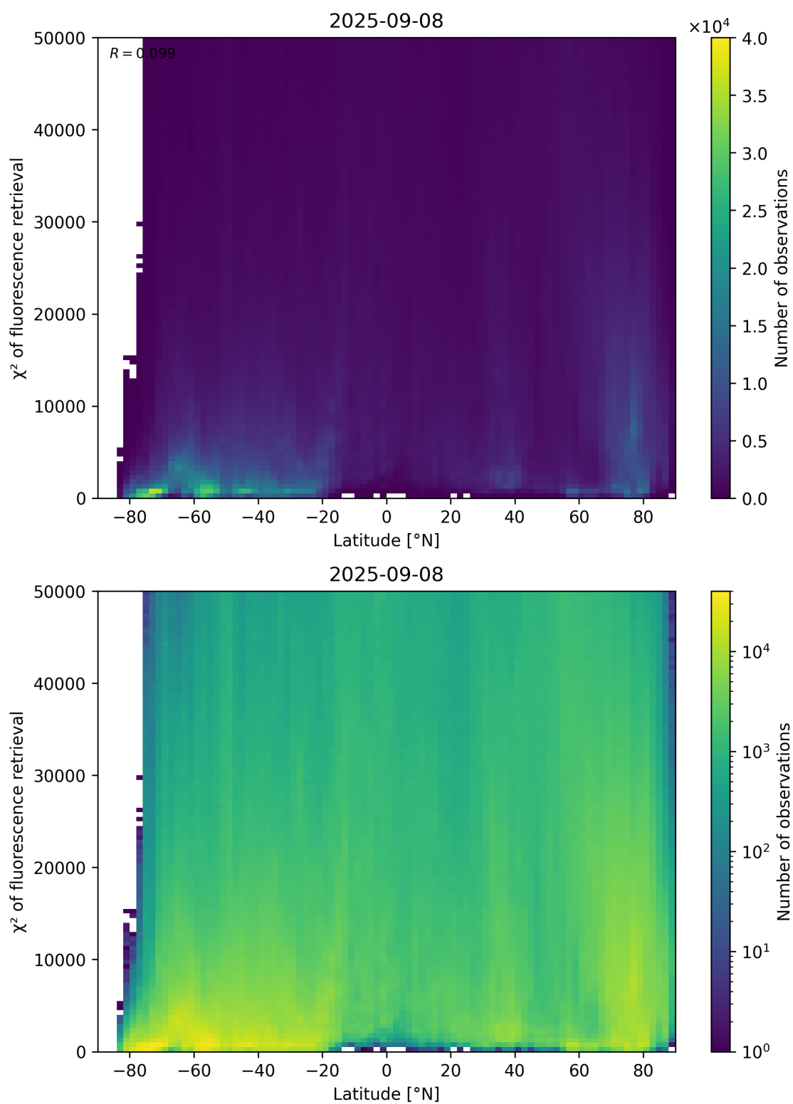
Figure 89: Scatter density plot of “Latitude” against “ \chi^2 of fluorescence retrieval” for 2025-09-07 to 2025-09-09.
