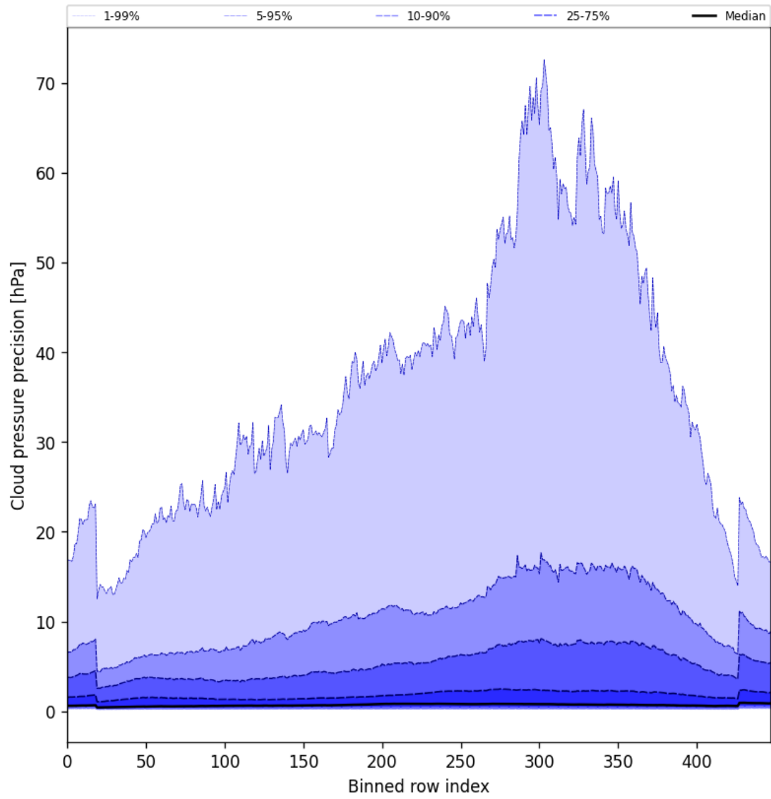
Figure 48: Along track statistics of “Cloud pressure precision” for 2025-09-07 to 2025-09-09
