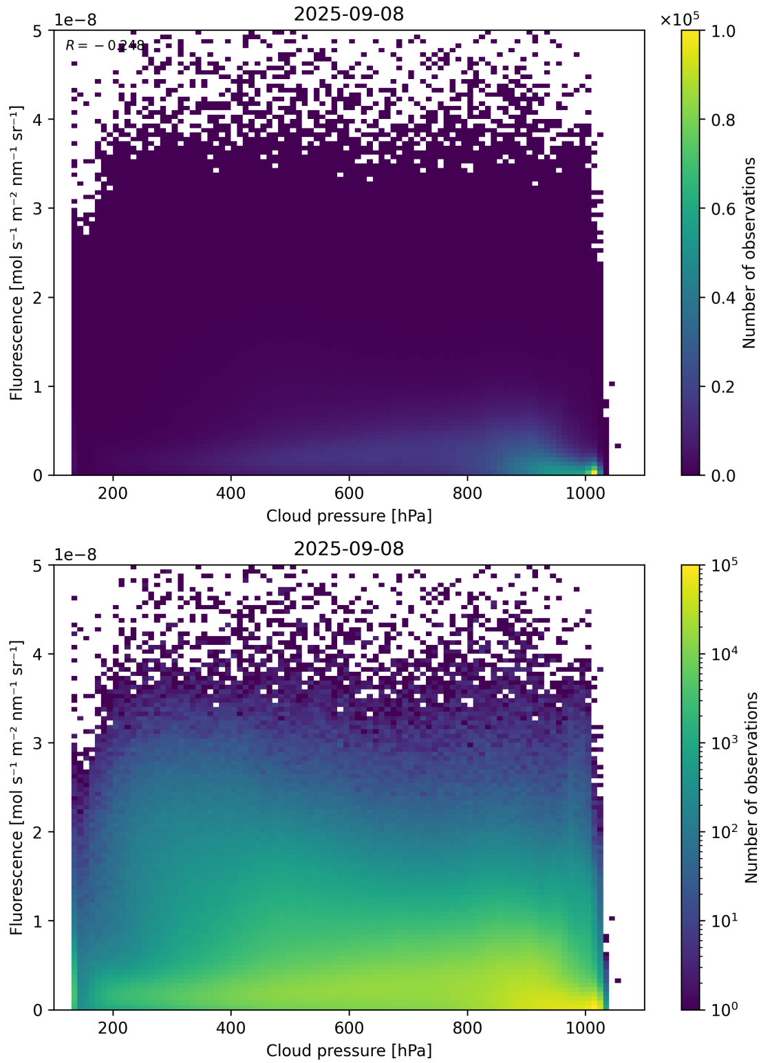
Figure 80: Scatter density plot of “Cloud pressure” against “Fluorescence” for 2025-09-07 to 2025-09-09.
