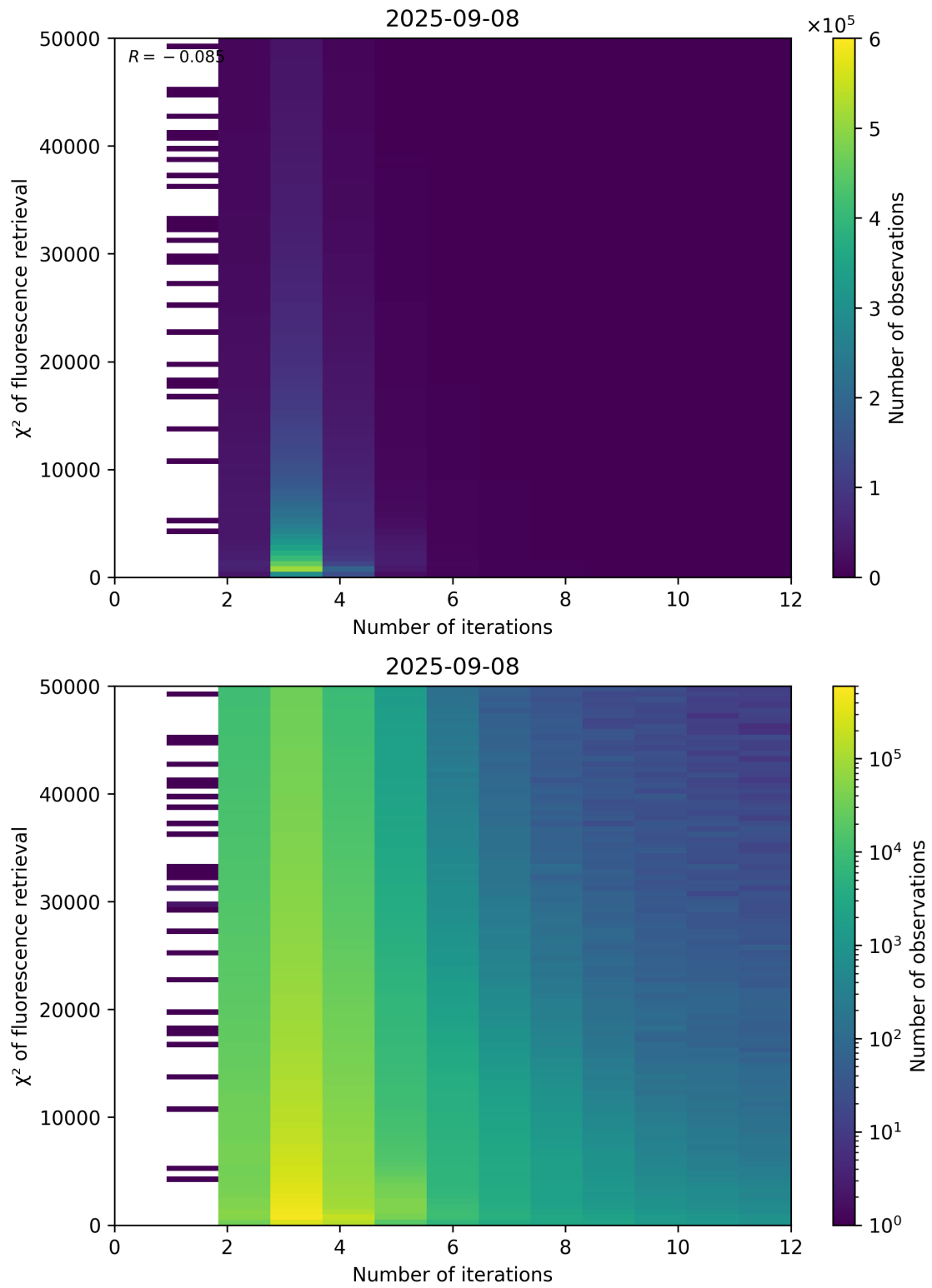
Figure 97: Scatter density plot of “Number of iterations” against “ \chi^2 of fluorescence retrieval” for 2025-09-07 to 2025-09-09.
