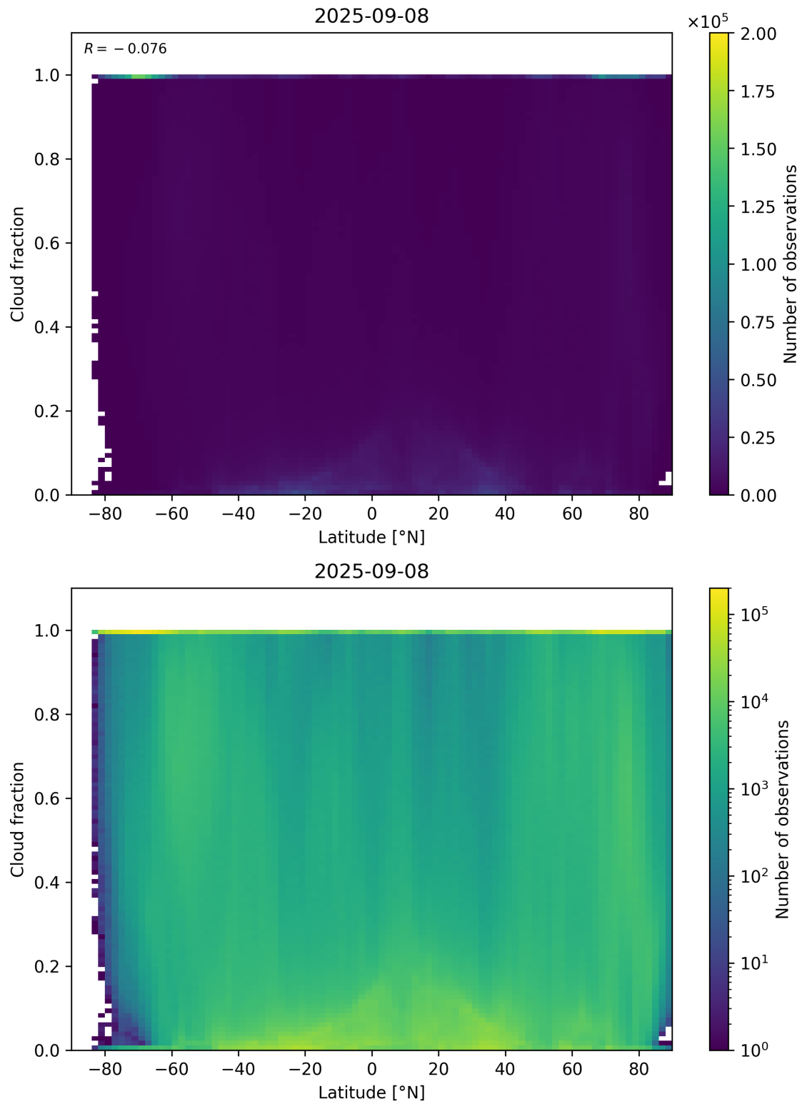
Figure 90: Scatter density plot of “Latitude” against “Cloud fraction” for 2025-09-07 to 2025-09-09.
