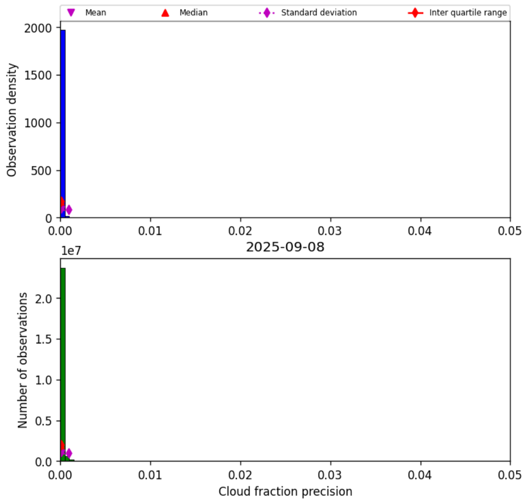
Figure 33: Histogram of “Cloud fraction precision” for 2025-09-07 to 2025-09-09
