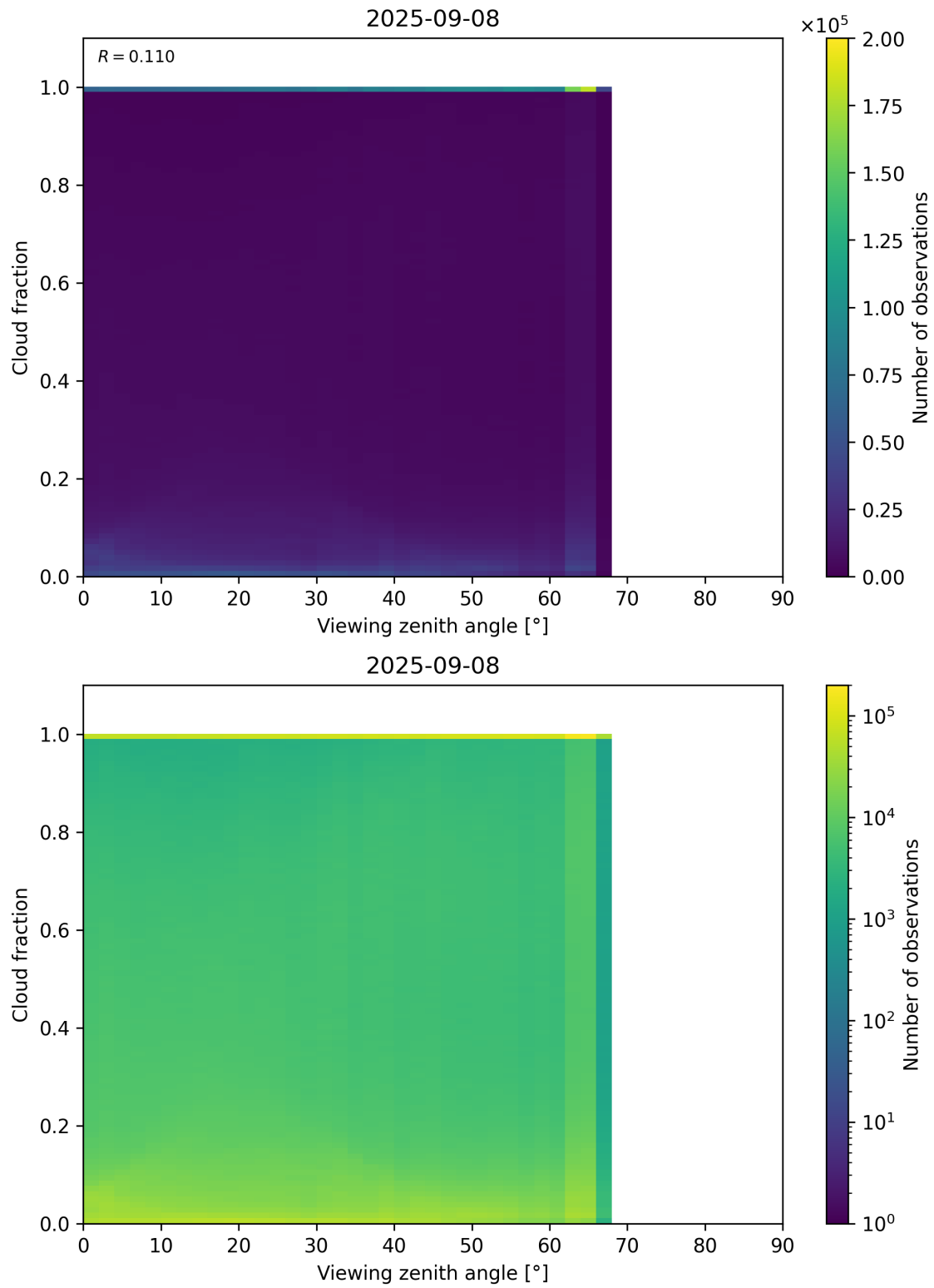
Figure 120: Scatter density plot of “Viewing zenith angle” against “Cloud fraction” for 2025-09-07 to 2025-09-09.
