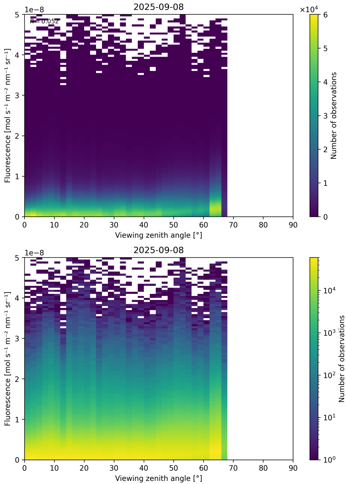
Figure 122: Scatter density plot of “Viewing zenith angle” against “Fluorescence” for 2025-09-07 to 2025-09-09.
