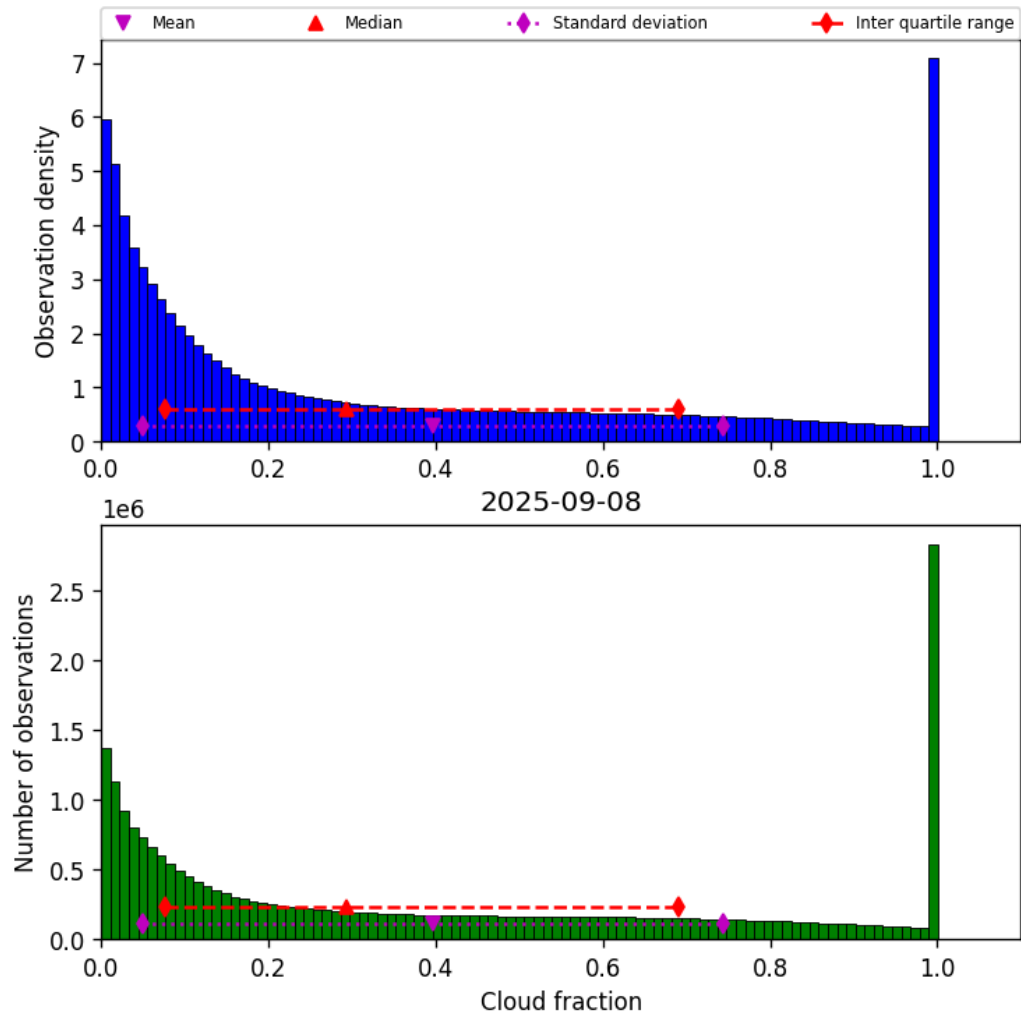
Figure 32: Histogram of “Cloud fraction” for 2025-09-07 to 2025-09-09
