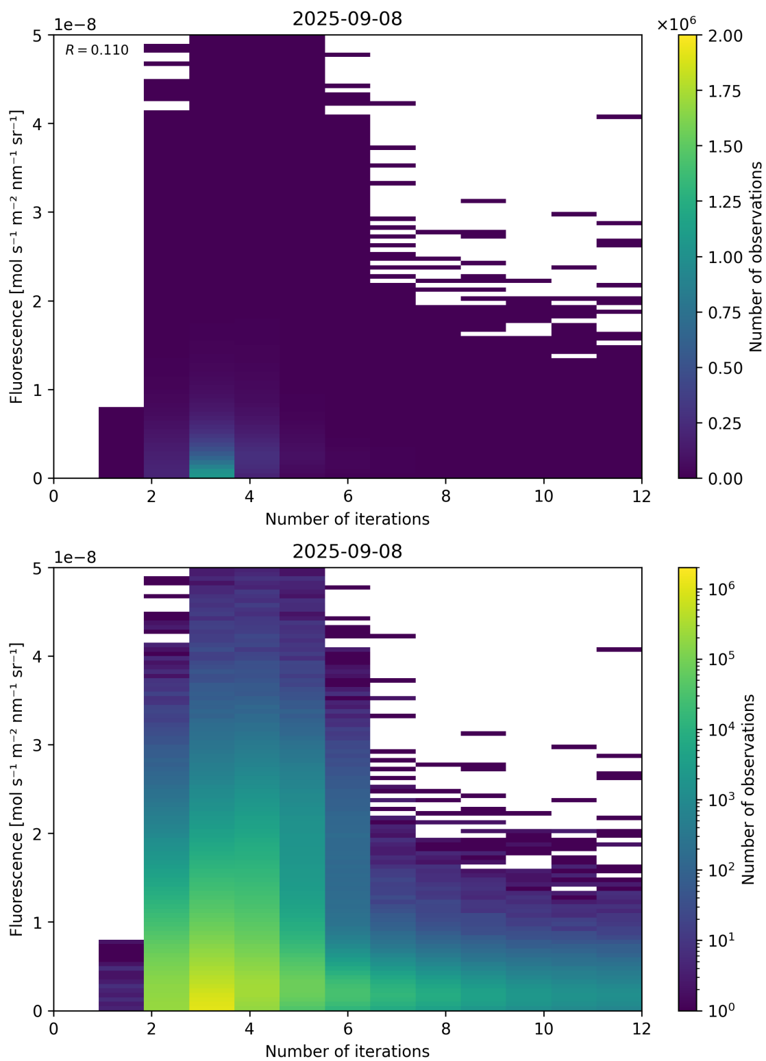
Figure 98: Scatter density plot of “Number of iterations” against “Fluorescence” for 2025-09-07 to 2025-09-09.
