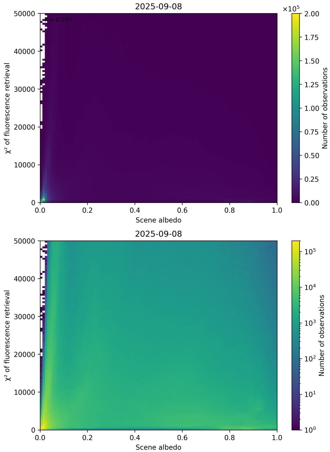
Figure 103: Scatter density plot of “Scene albedo” against “ \chi^2 of fluorescence retrieval” for 2025-09-07 to 2025-09-09.
