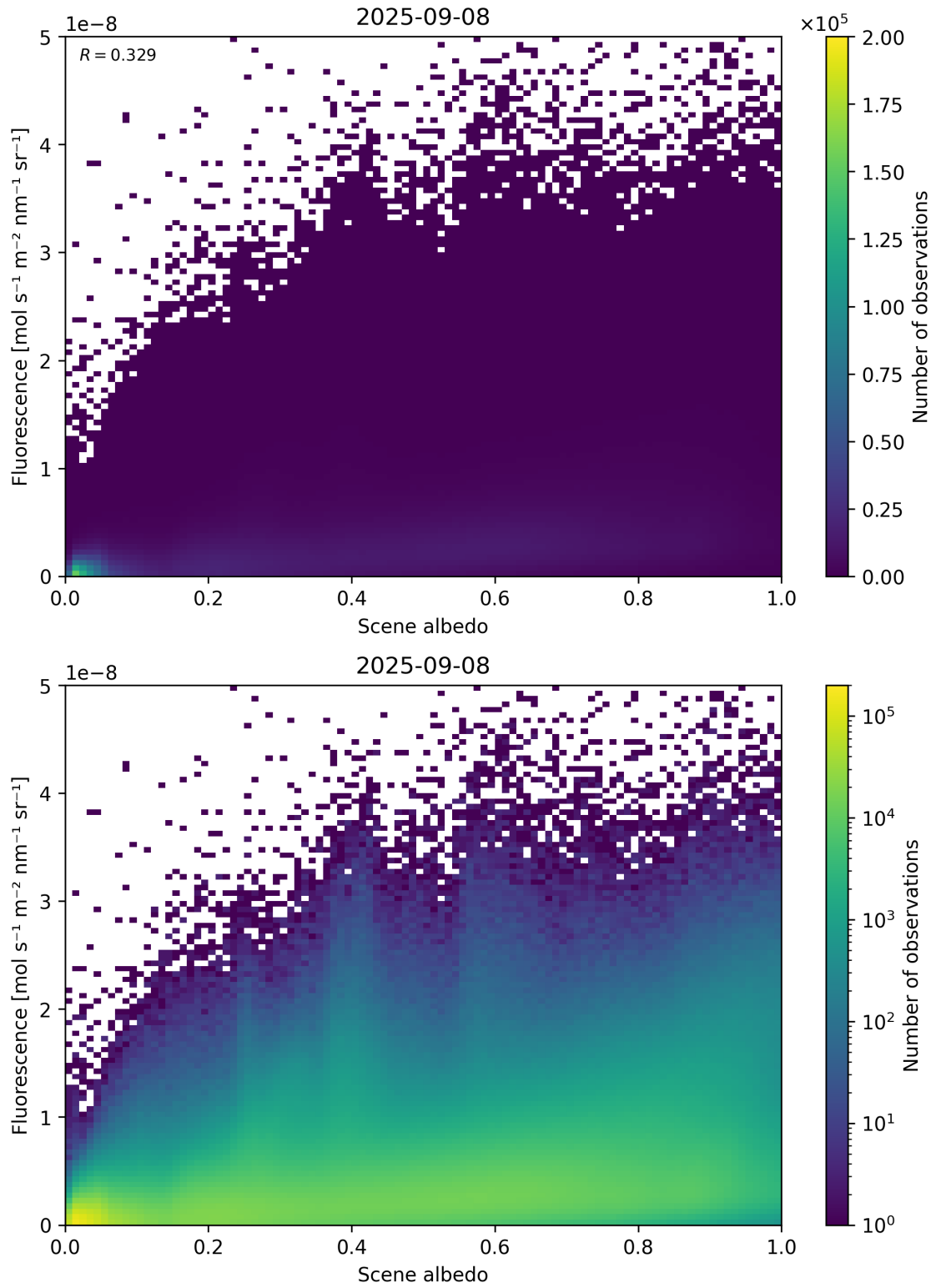
Figure 104: Scatter density plot of “Scene albedo” against “Fluorescence” for 2025-09-07 to 2025-09-09.
