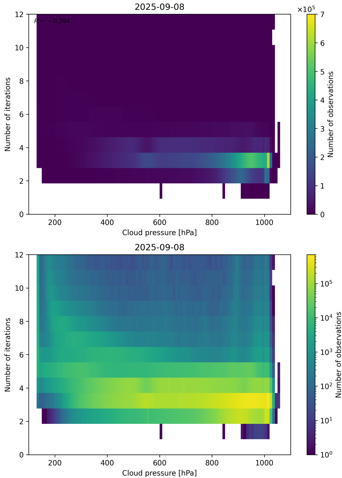
Figure 81: Scatter density plot of “Cloud pressure” against “Number of iterations” for 2025-09-07 to 2025-09-09.
