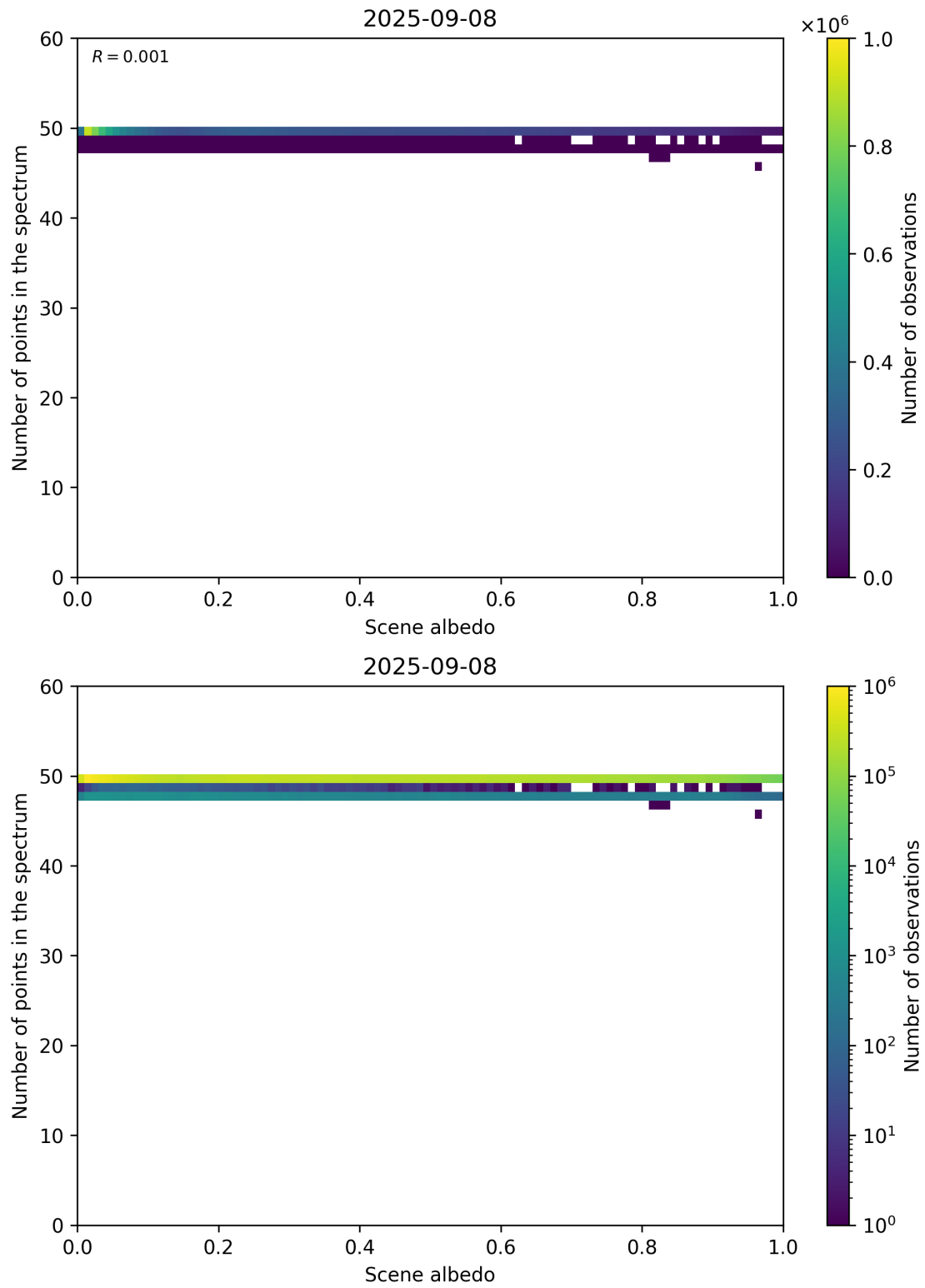
Figure 106: Scatter density plot of “Scene albedo” against “Number of points in the spectrum” for 2025-09-07 to 2025-09-09.
