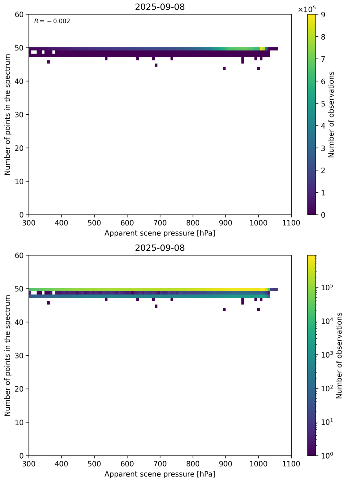
Figure 66: Scatter density plot of “Apparent scene pressure” against “Number of points in the spectrum” for 2025-09-07 to 2025-09-09.
