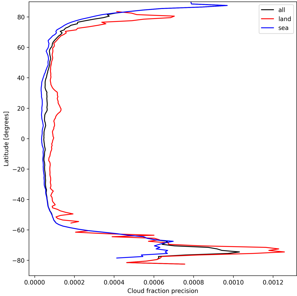
Figure 16: Zonal average of “Cloud fraction precision” for 2025-09-07 to 2025-09-09.
