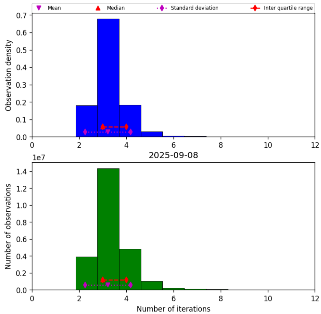
Figure 39: Histogram of “Number of iterations” for 2025-09-07 to 2025-09-09
