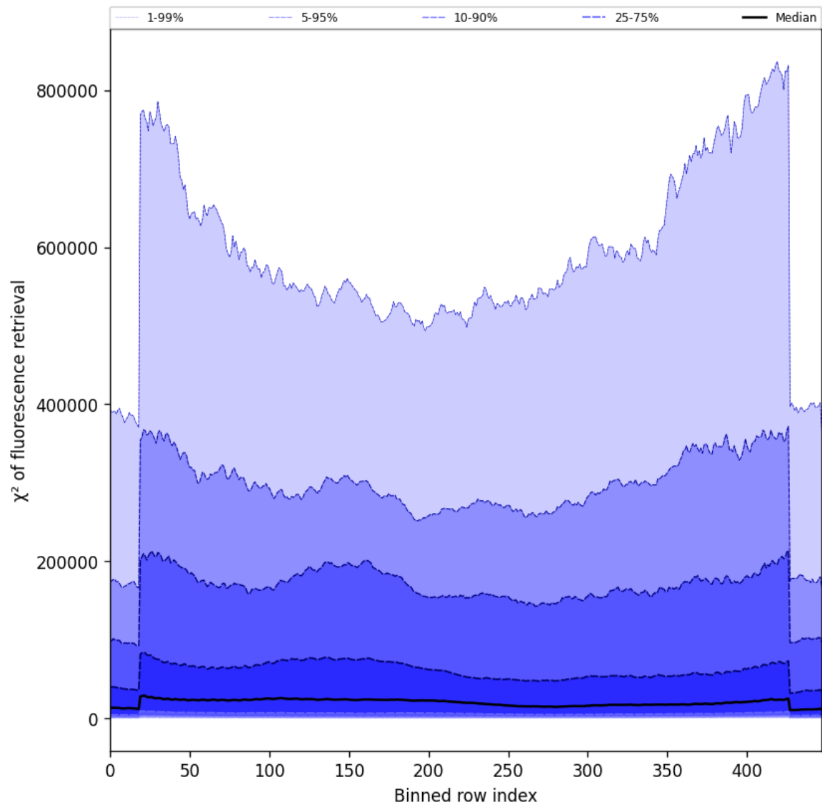
Figure 59: Along track statistics of “ \chi^2 of fluorescence retrieval” for 2025-09-07 to 2025-09-09
