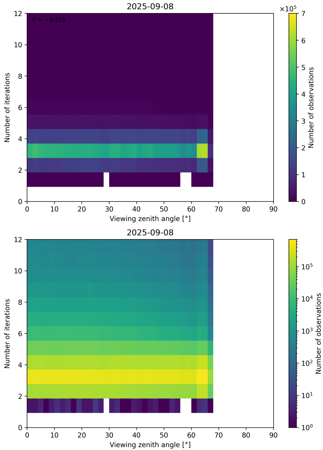
Figure 124: Scatter density plot of “Viewing zenith angle” against “Number of iterations” for 2025-09-07 to 2025-09-09.
