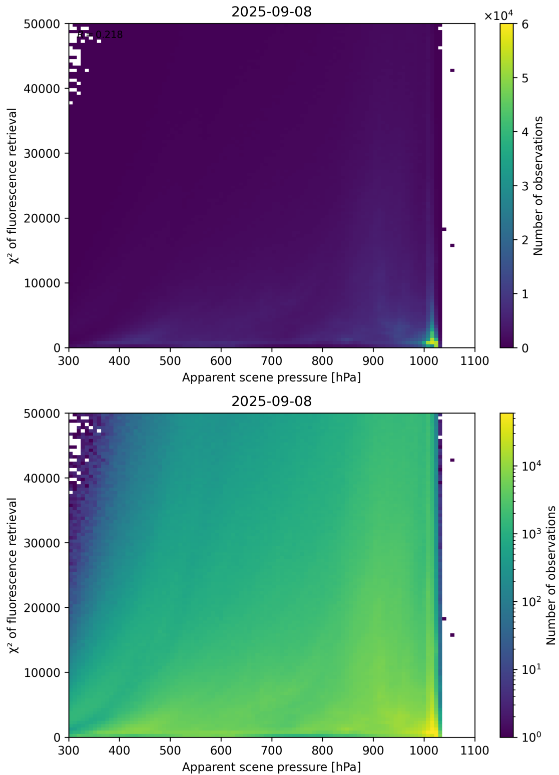
Figure 63: Scatter density plot of “Apparent scene pressure” against “ \chi^2 of fluorescence retrieval” for 2025-09-07 to 2025-09-09.
