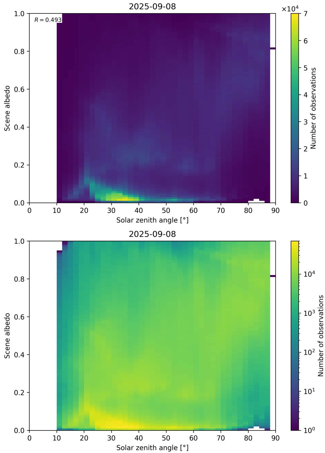
Figure 116: Scatter density plot of “Solar zenith angle” against “Scene albedo” for 2025-09-07 to 2025-09-09.
