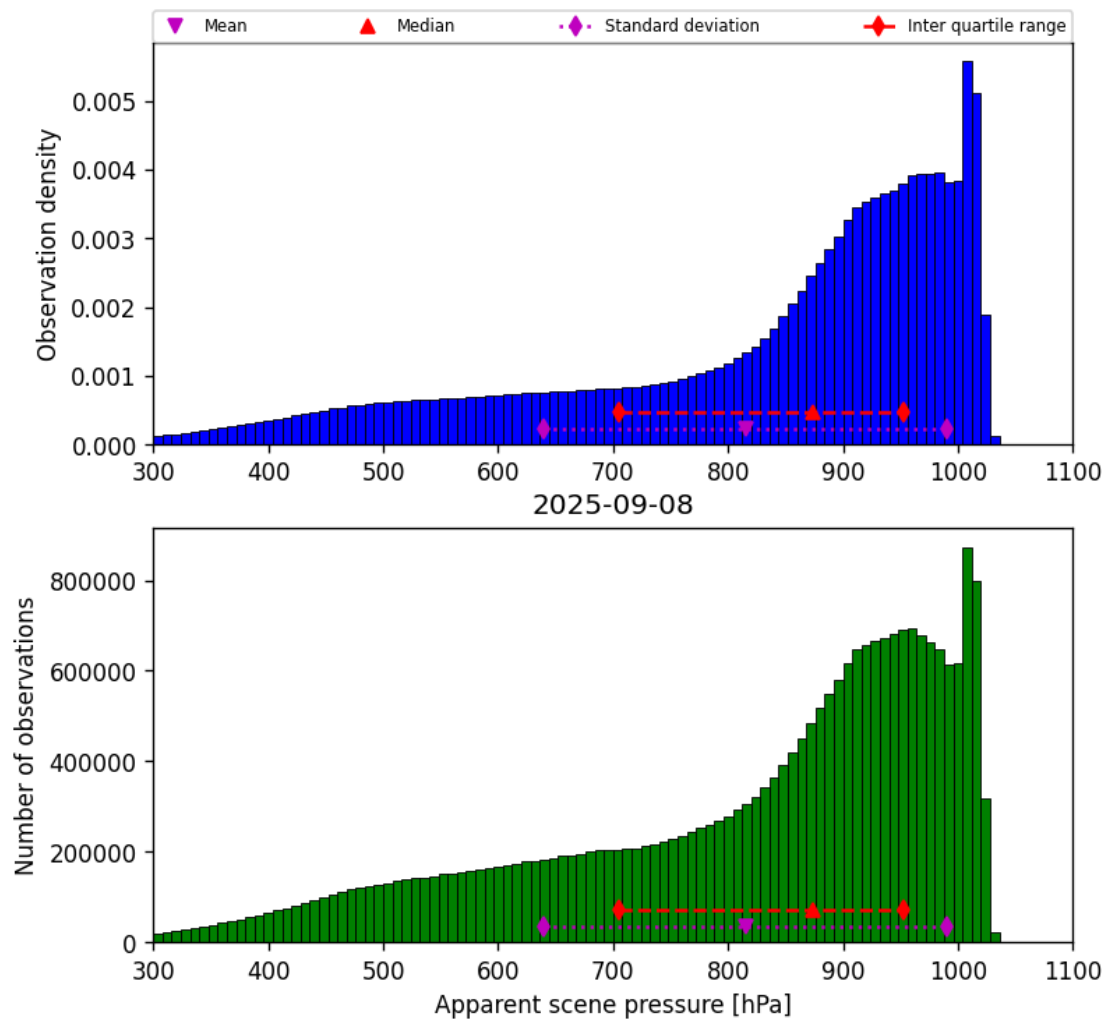
Figure 36: Histogram of “Apparent scene pressure” for 2025-09-07 to 2025-09-09
