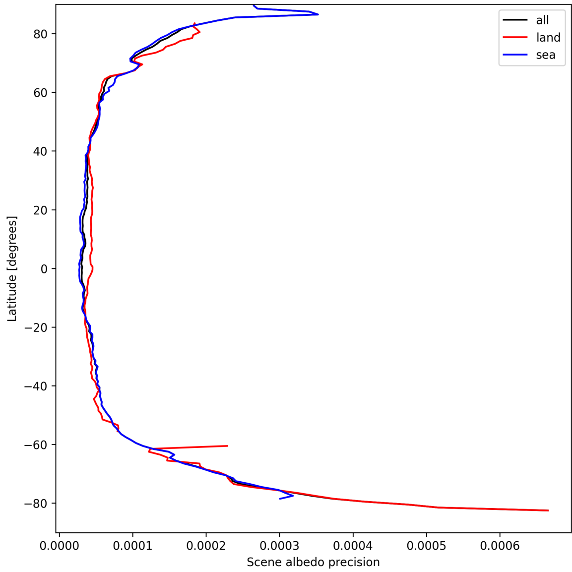
Figure 18: Zonal average of “Scene albedo precision” for 2025-09-07 to 2025-09-09.
