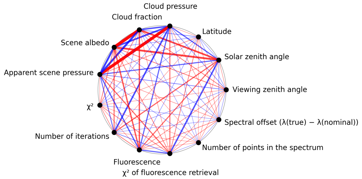
Figure 1: Map of correlation graph for 2025-09-07 to 2025-09-09.
