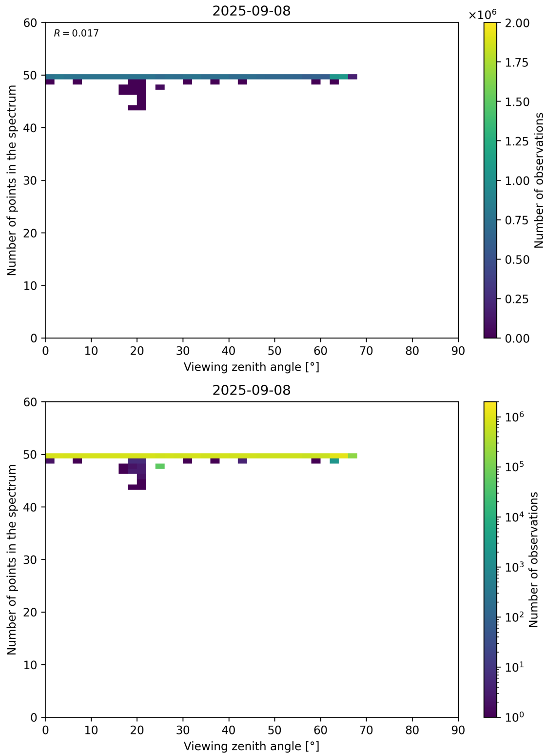
Figure 125: Scatter density plot of “Viewing zenith angle” against “Number of points in the spectrum” for 2025-09-07 to 2025-09-09.
