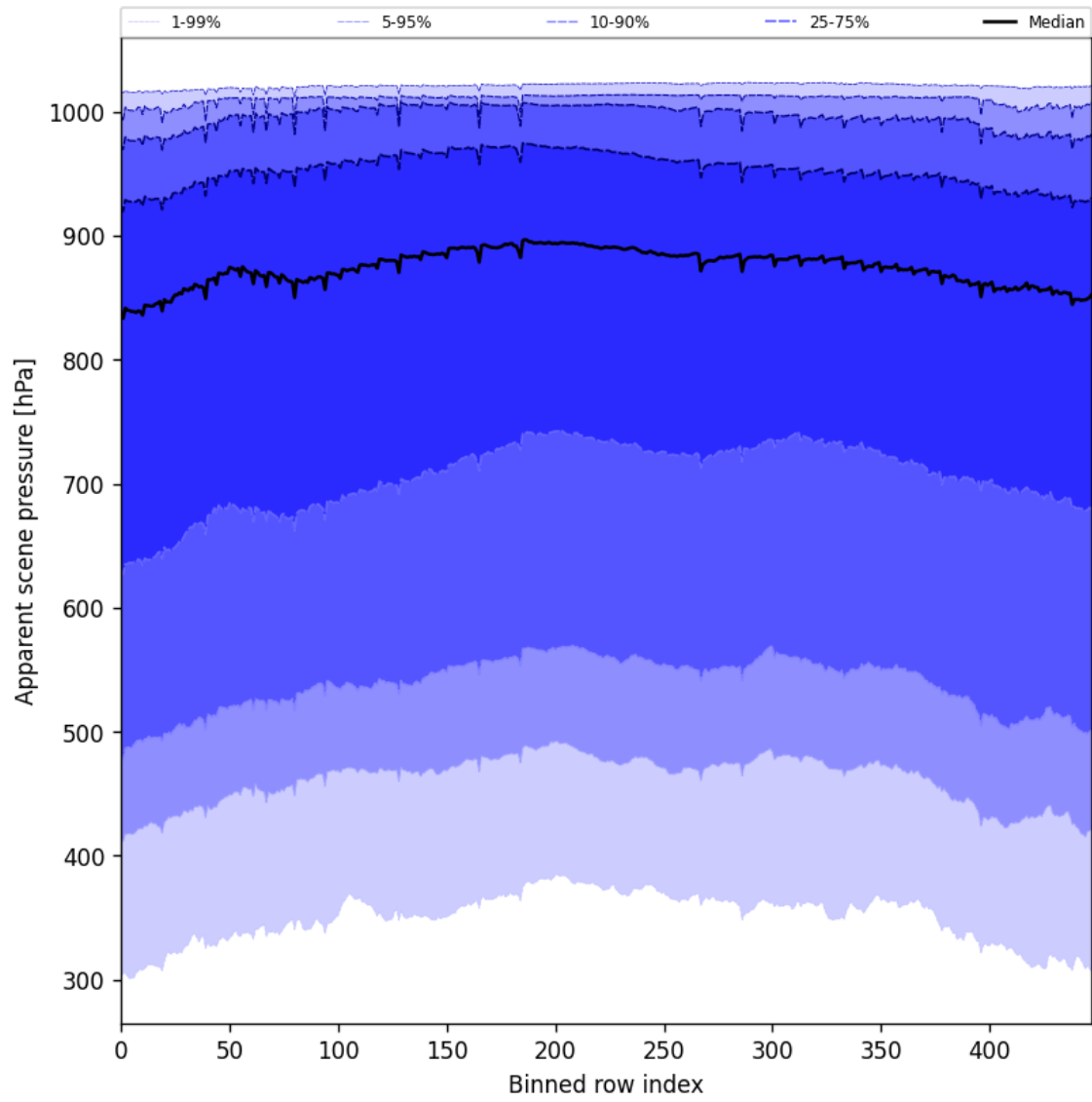
Figure 53: Along track statistics of “Apparent scene pressure” for 2025-09-07 to 2025-09-09
