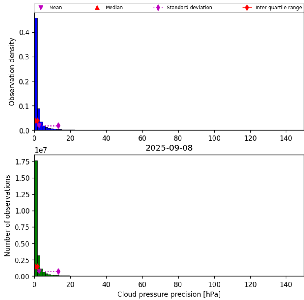
Figure 31: Histogram of “Cloud pressure precision” for 2025-09-07 to 2025-09-09
