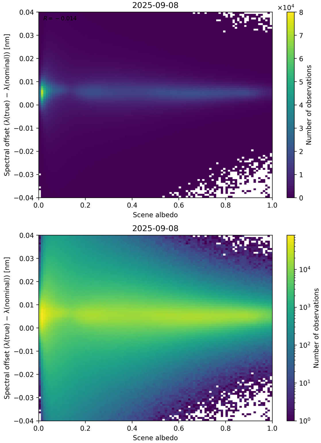
Figure 107: Scatter density plot of “Scene albedo” against “Spectral offset ( \lambda_{\text{true}} - \lambda_{\text{nominal}} )” for 2025-09-07 to 2025-09-09.
