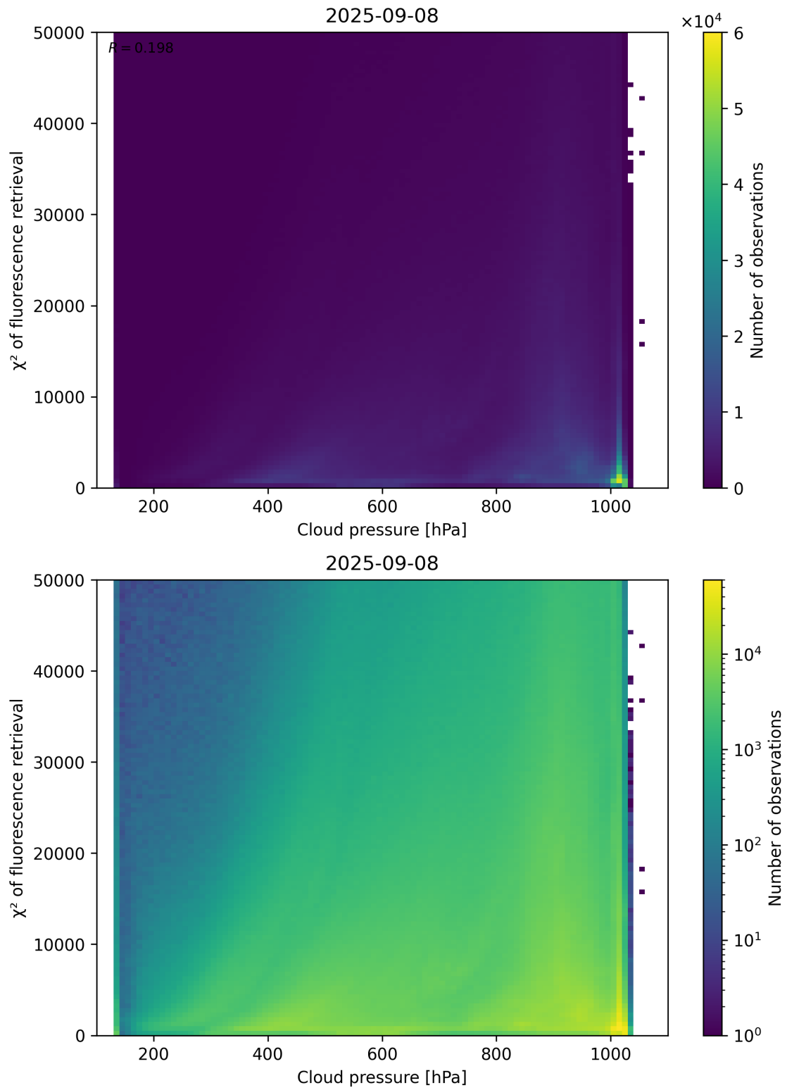
Figure 78: Scatter density plot of “Cloud pressure” against “ \chi^2 of fluorescence retrieval” for 2025-09-07 to 2025-09-09.
