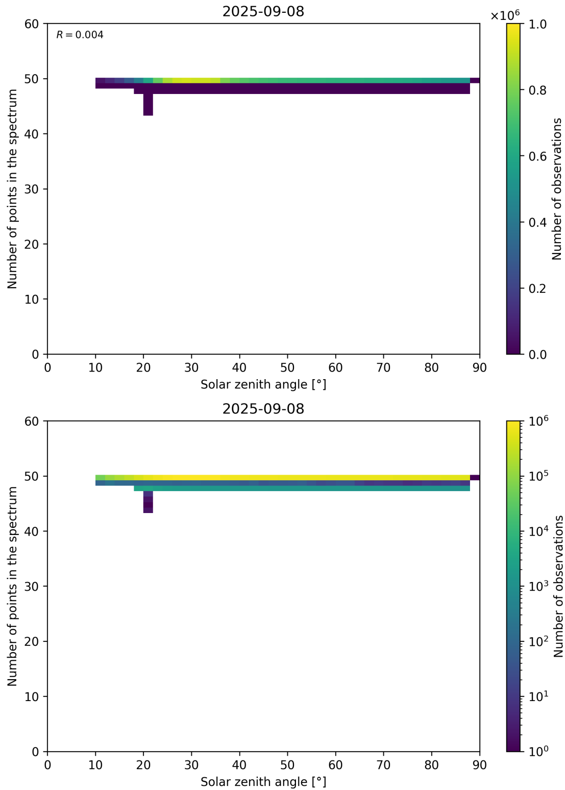
Figure 115: Scatter density plot of “Solar zenith angle” against “Number of points in the spectrum” for 2025-09-07 to 2025-09-09.
