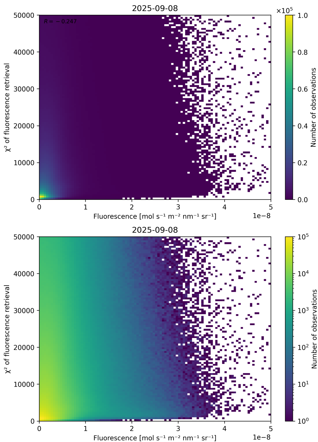
Figure 85: Scatter density plot of “Fluorescence” against “ \chi^2 of fluorescence retrieval” for 2025-09-07 to 2025-09-09.
