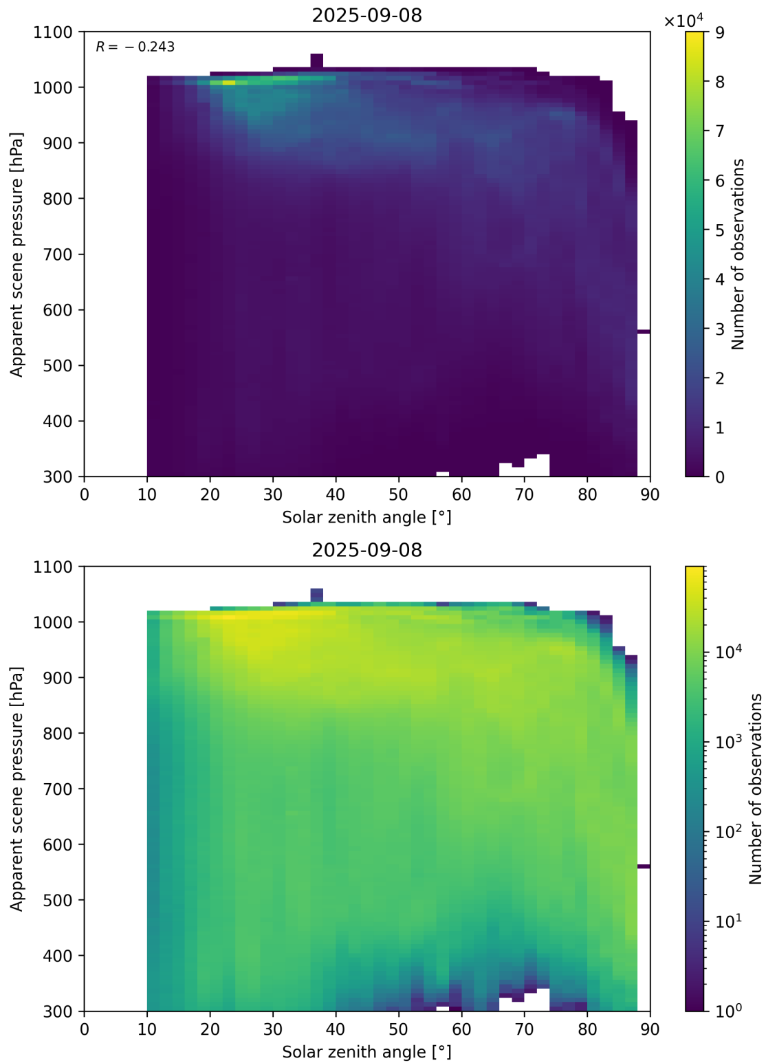
Figure 108: Scatter density plot of “Solar zenith angle” against “Apparent scene pressure” for 2025-09-07 to 2025-09-09.
