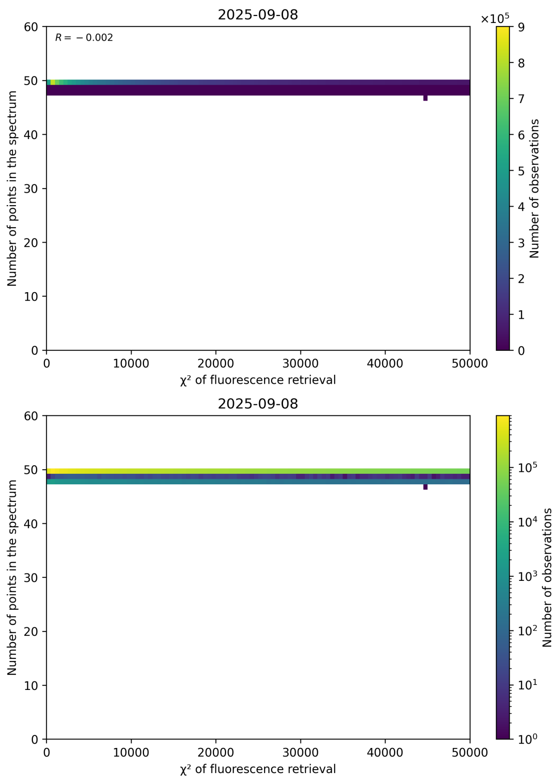
Figure 68: Scatter density plot of " \chi^2 of fluorescence retrieval" against "Number of points in the spectrum" for 2025-09-07 to 2025-09-09.
