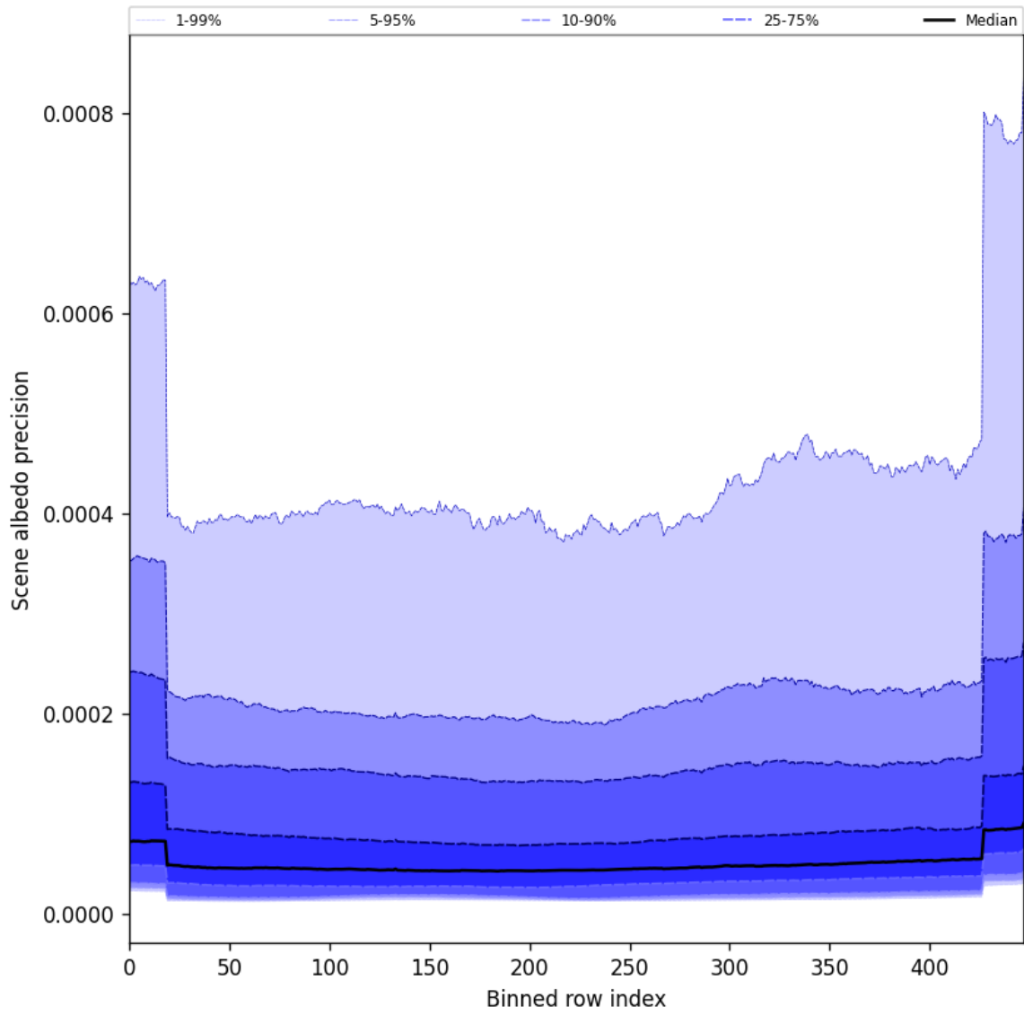
Figure 52: Along track statistics of “Scene albedo precision” for 2025-09-07 to 2025-09-09
