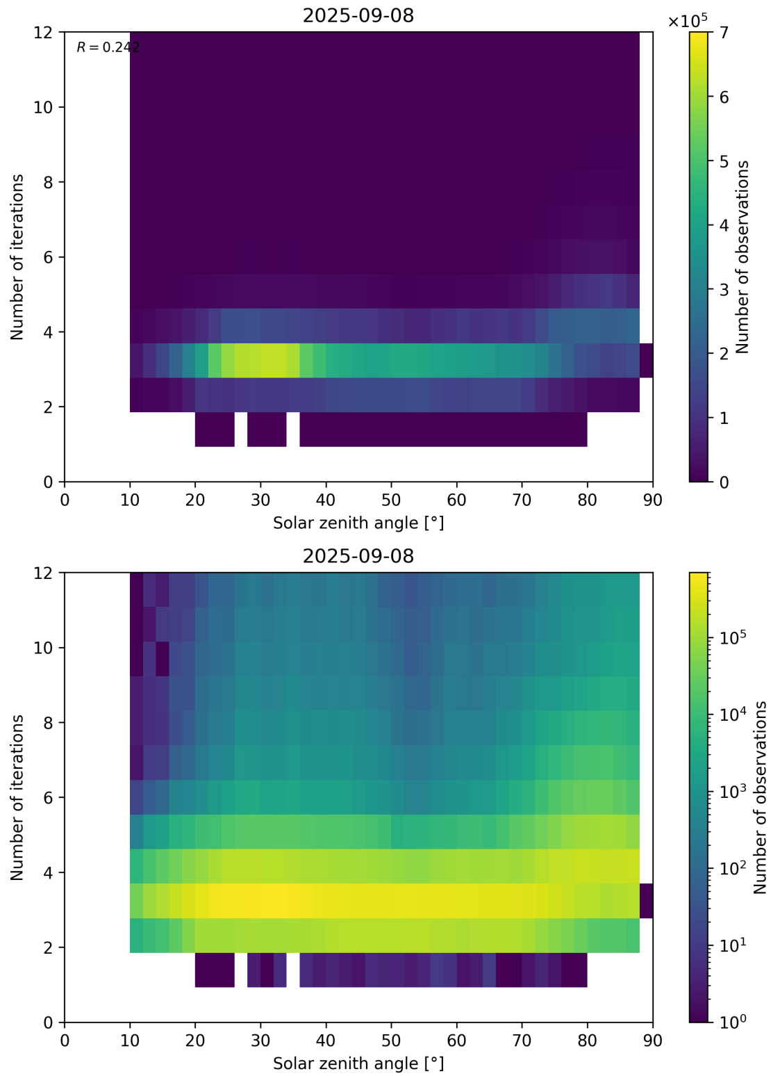
Figure 114: Scatter density plot of “Solar zenith angle” against “Number of iterations” for 2025-09-07 to 2025-09-09.
