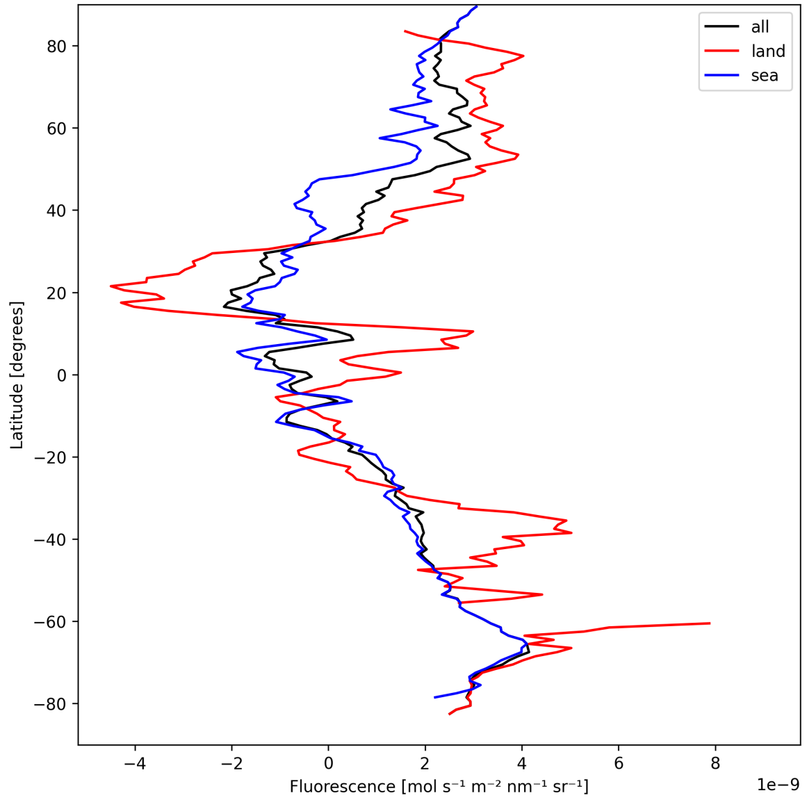
Figure 23: Zonal average of “Fluorescence” for 2025-09-07 to 2025-09-09.
