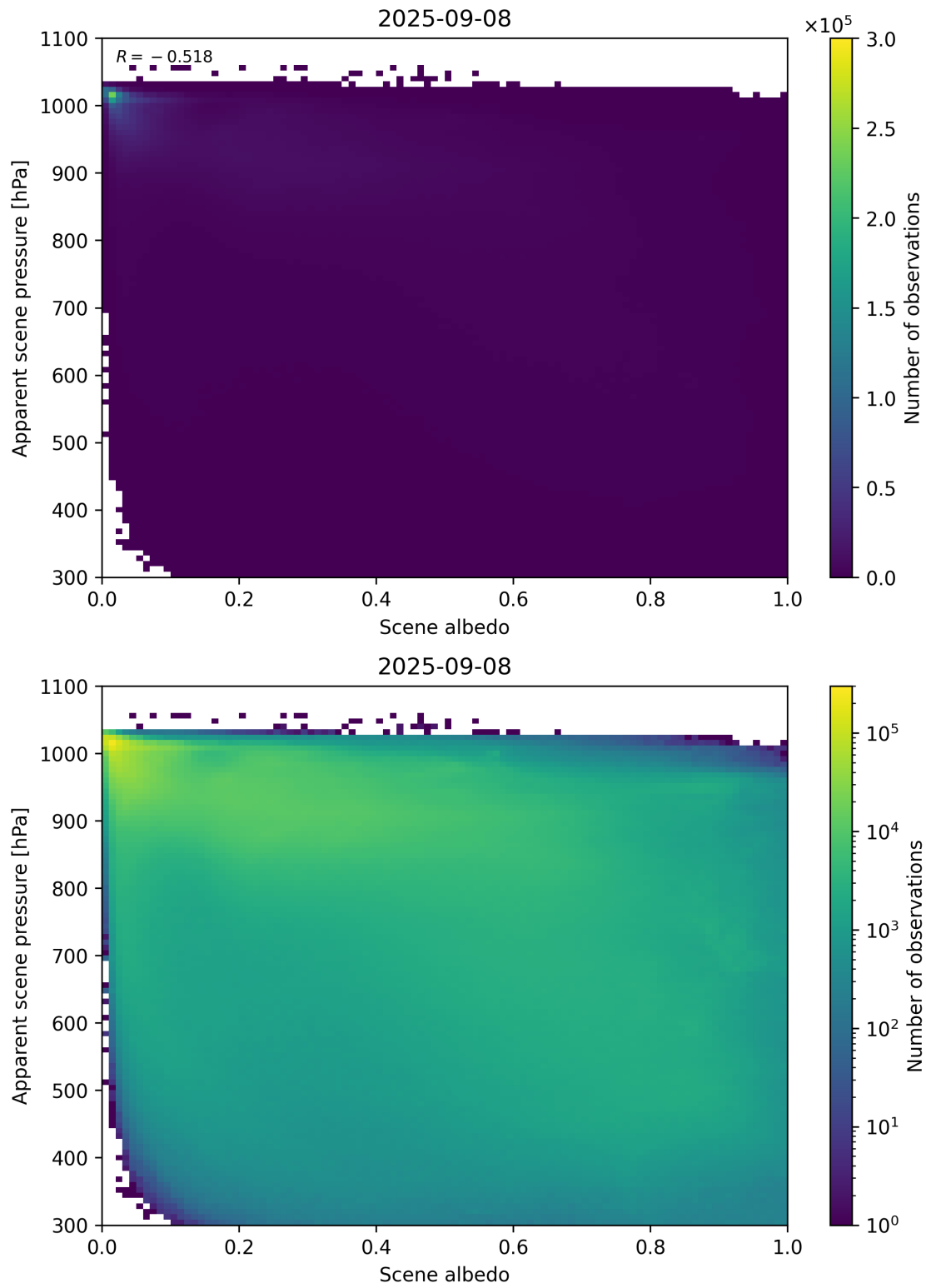
Figure 102: Scatter density plot of “Scene albedo” against “Apparent scene pressure” for 2025-09-07 to 2025-09-09.
