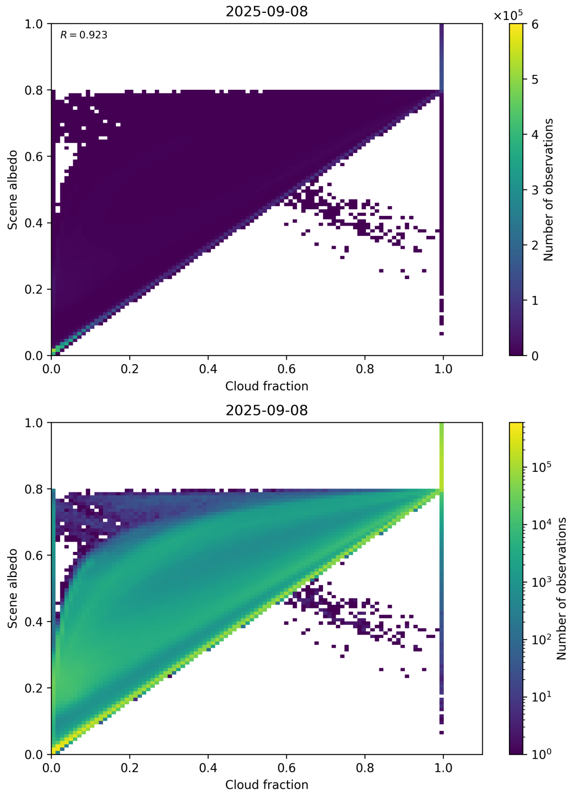
Figure 75: Scatter density plot of “Cloud fraction” against “Scene albedo” for 2025-09-07 to 2025-09-09.
