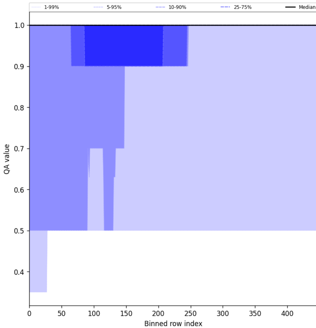
Figure 46: Along track statistics of “QA value” for 2025-09-07 to 2025-09-09
