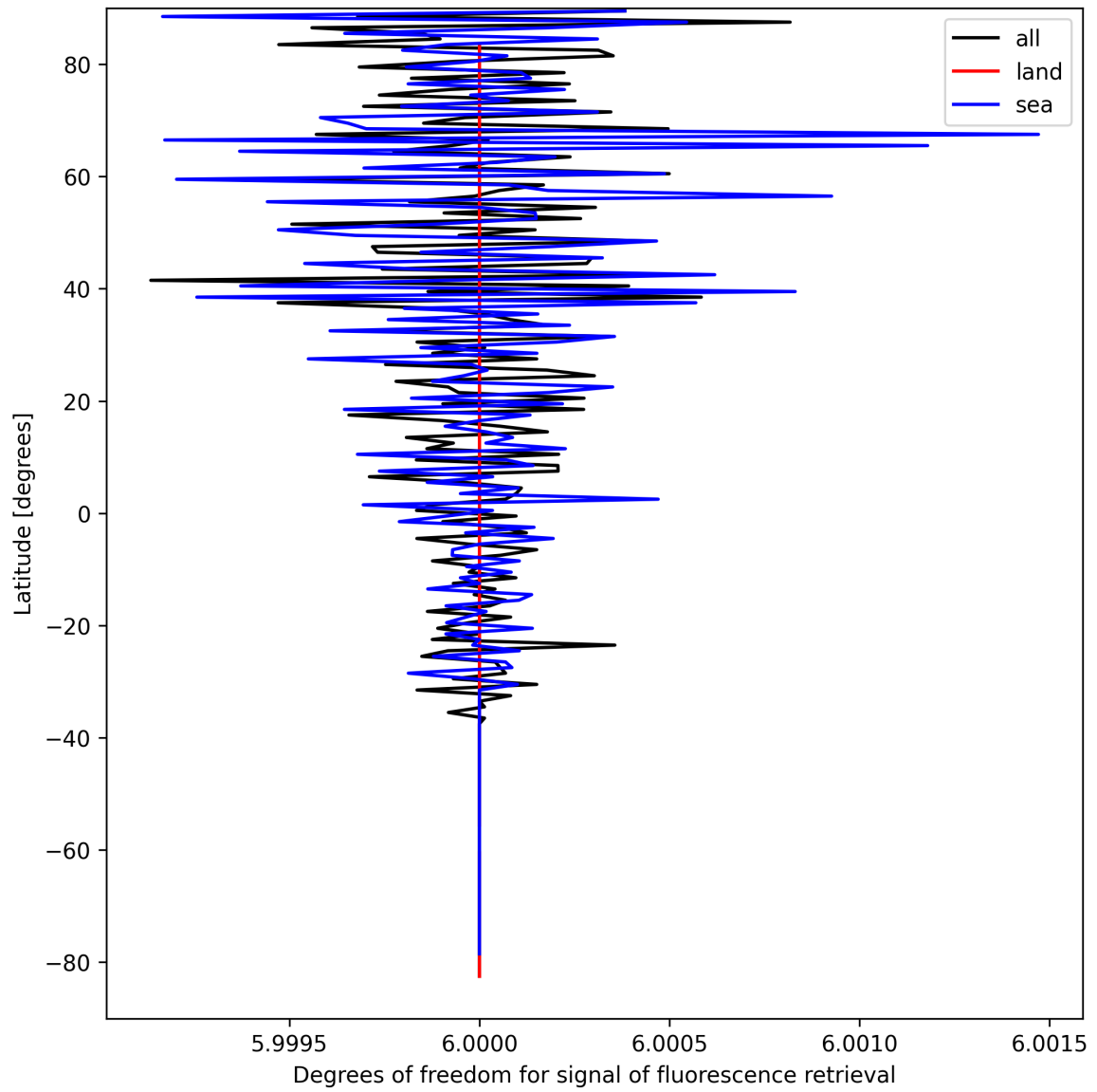
Figure 26: Zonal average of “Degrees of freedom for signal of fluorescence retrieval” for 2025-09-07 to 2025-09-09.
