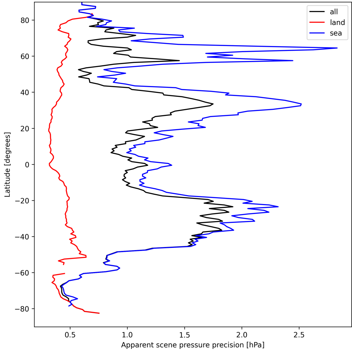
Figure 20: Zonal average of “Apparent scene pressure precision” for 2025-09-07 to 2025-09-09.
