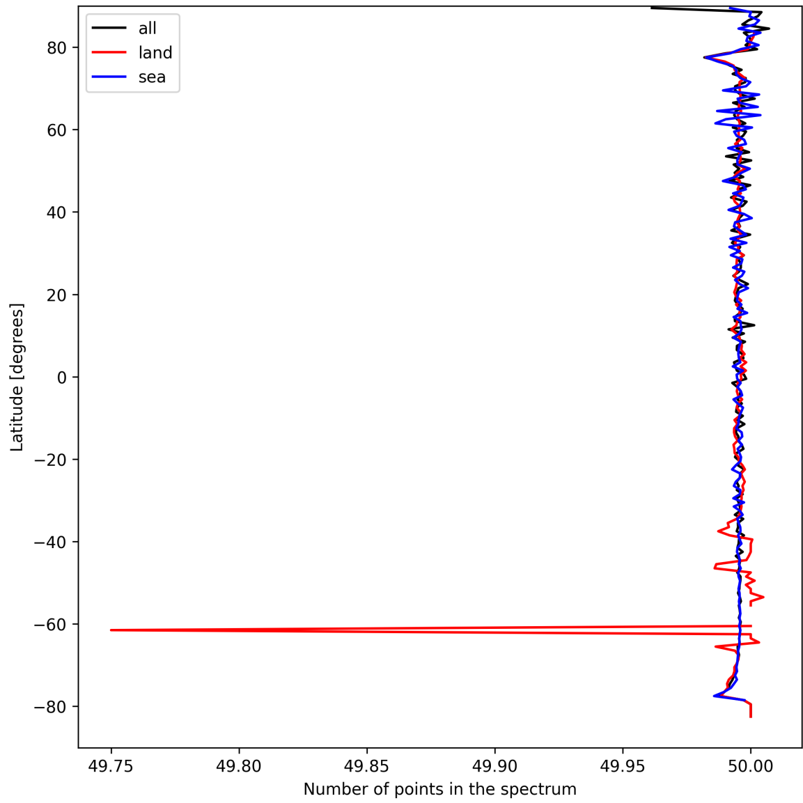
Figure 27: Zonal average of “Number of points in the spectrum” for 2025-09-07 to 2025-09-09.
