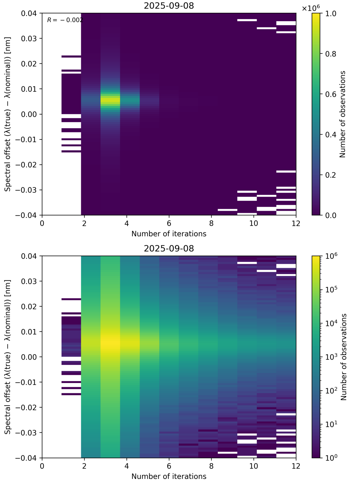
Figure 100: Scatter density plot of “Number of iterations” against “Spectral offset ( \lambda_{\text{true}} - \lambda_{\text{nominal}} )” for 2025-09-07 to 2025-09-09.
