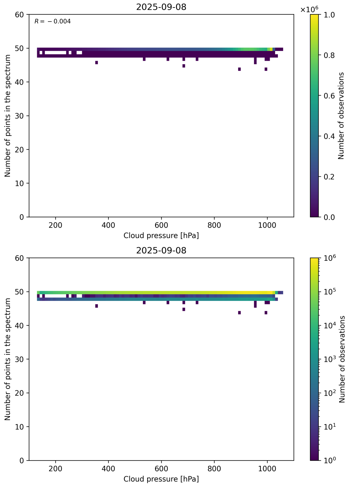
Figure 82: Scatter density plot of “Cloud pressure” against “Number of points in the spectrum” for 2025-09-07 to 2025-09-09.
