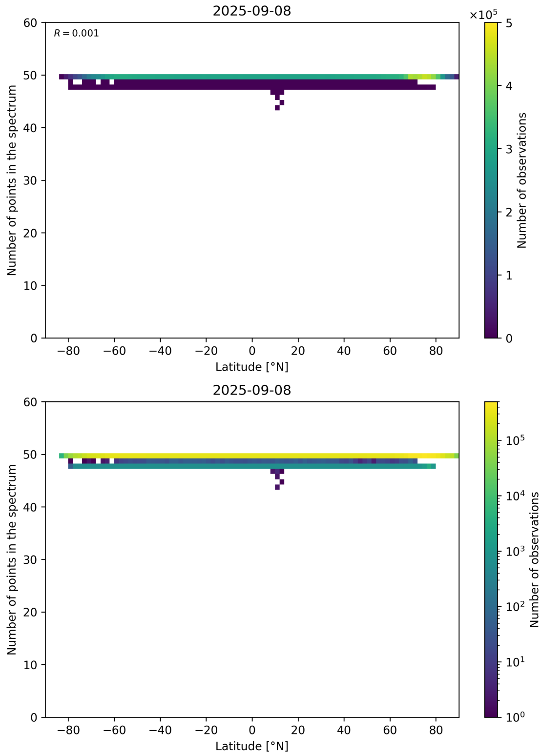
Figure 94: Scatter density plot of “Latitude” against “Number of points in the spectrum” for 2025-09-07 to 2025-09-09.
