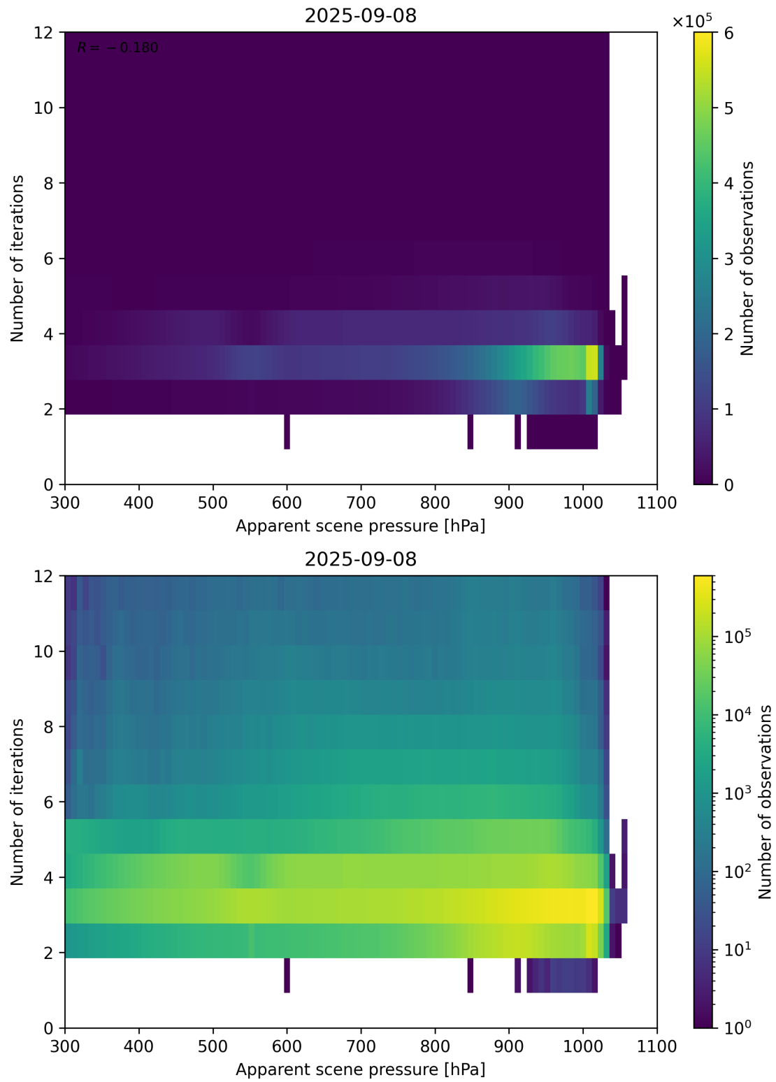
Figure 65: Scatter density plot of “Apparent scene pressure” against “Number of iterations” for 2025-09-07 to 2025-09-09.
