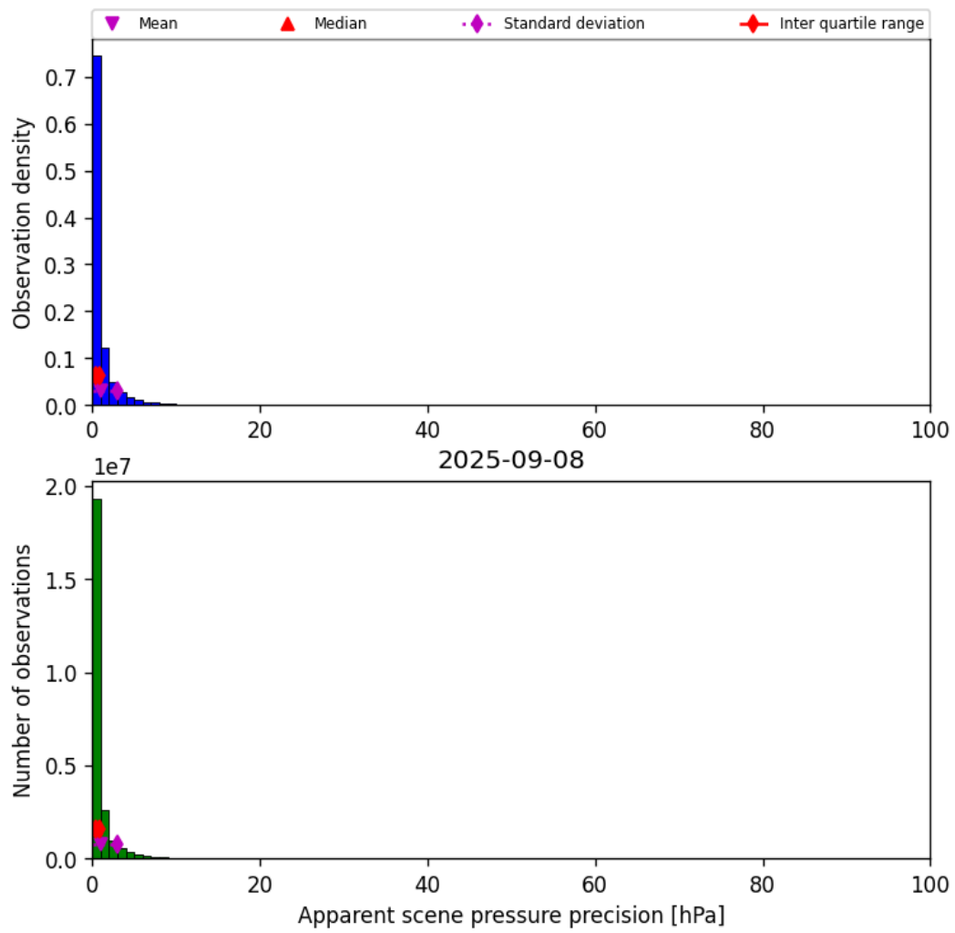
Figure 37: Histogram of “Apparent scene pressure precision” for 2025-09-07 to 2025-09-09
