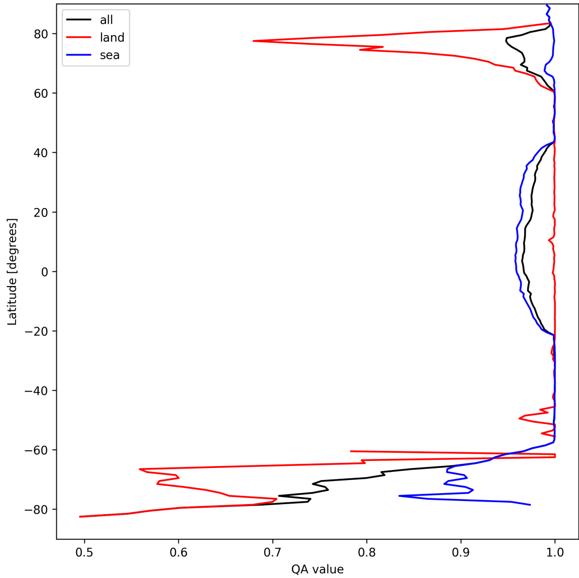
Figure 12: Zonal average of “QA value” for 2025-09-07 to 2025-09-09.
