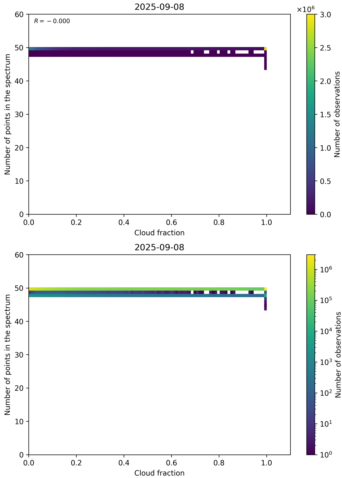
Figure 74: Scatter density plot of “Cloud fraction” against “Number of points in the spectrum” for 2025-09-07 to 2025-09-09.
