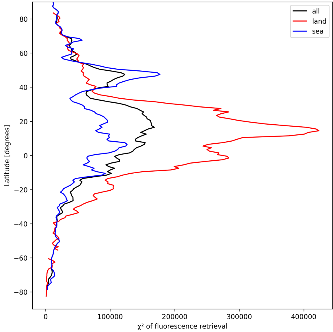
Figure 25: Zonal average of “ \chi^2 of fluorescence retrieval” for 2025-09-07 to 2025-09-09.
