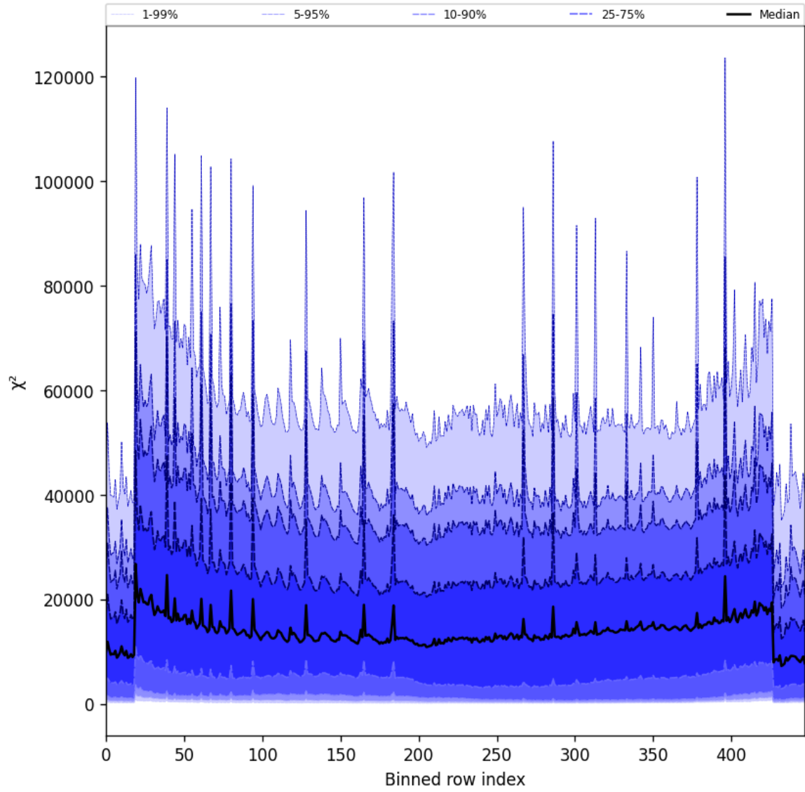
Figure 55: Along track statistics of “ \chi^2 ” for 2025-09-07 to 2025-09-09
