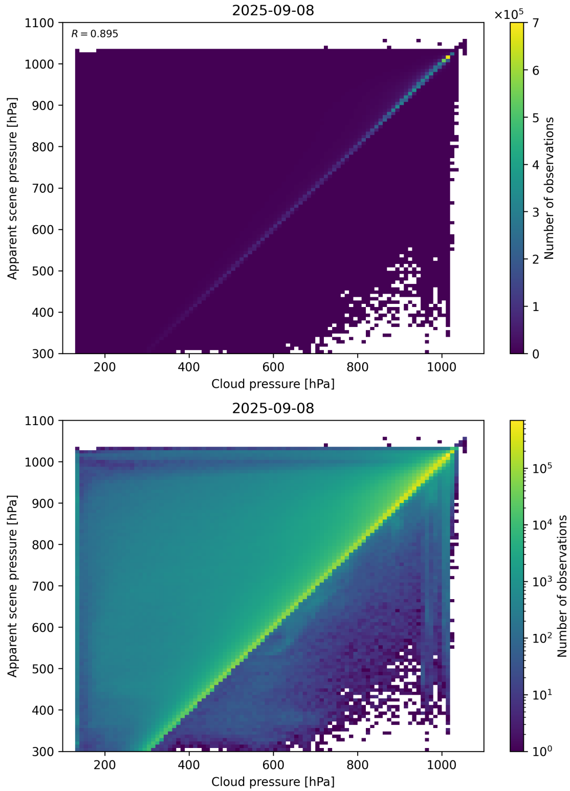
Figure 77: Scatter density plot of “Cloud pressure” against “Apparent scene pressure” for 2025-09-07 to 2025-09-09.
