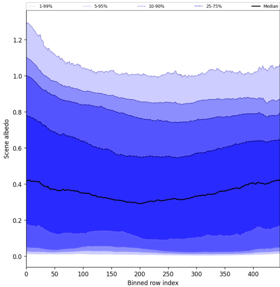
Figure 51: Along track statistics of “Scene albedo” for 2025-09-07 to 2025-09-09
