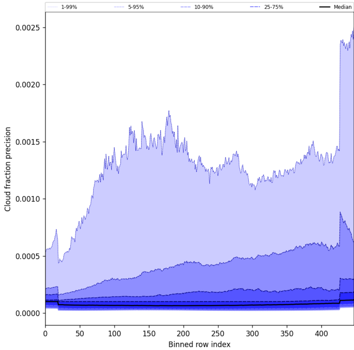
Figure 50: Along track statistics of “Cloud fraction precision” for 2025-09-07 to 2025-09-09
