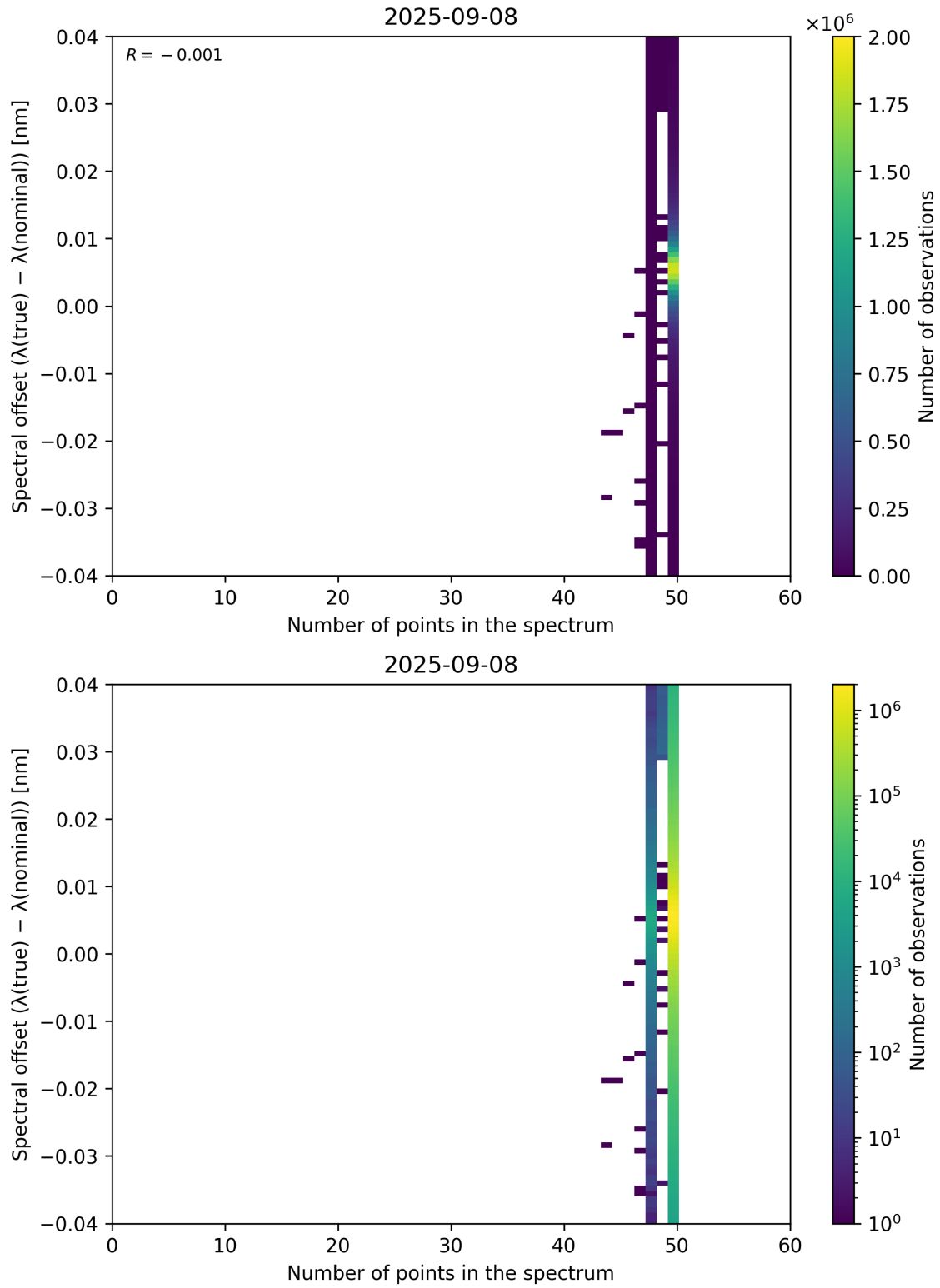
Figure 101: Scatter density plot of “Number of points in the spectrum” against “Spectral offset ( \lambda_{\text{true}} - \lambda_{\text{nominal}} )” for 2025-09-07 to 2025-09-09.
