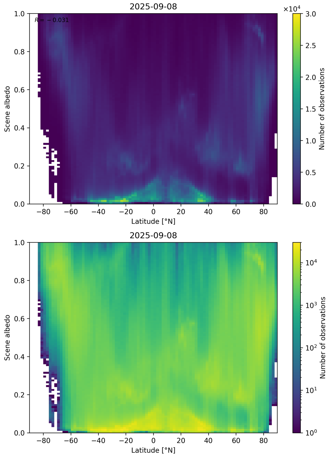
Figure 95: Scatter density plot of “Latitude” against “Scene albedo” for 2025-09-07 to 2025-09-09.
