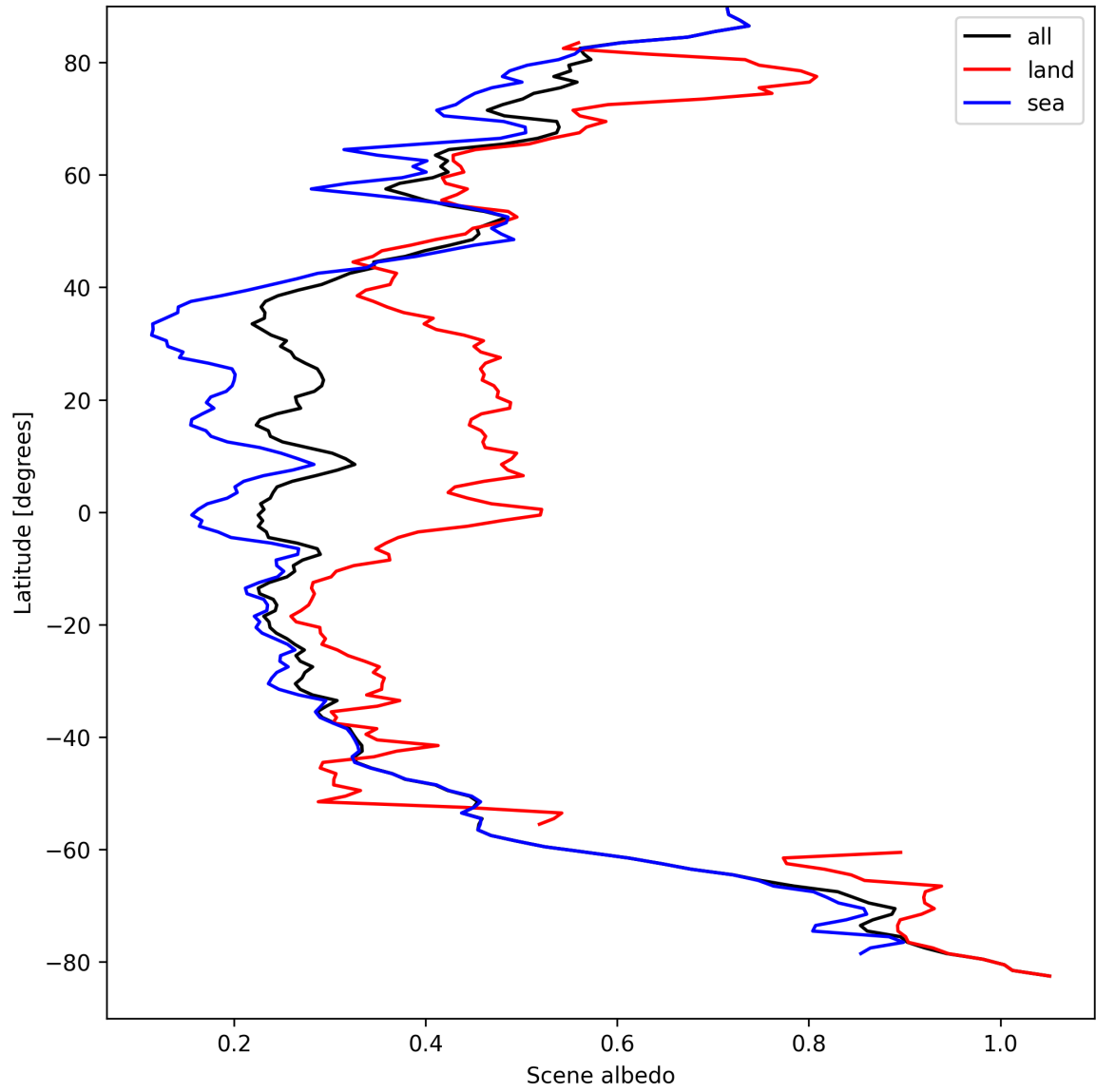
Figure 17: Zonal average of “Scene albedo” for 2025-09-07 to 2025-09-09.
