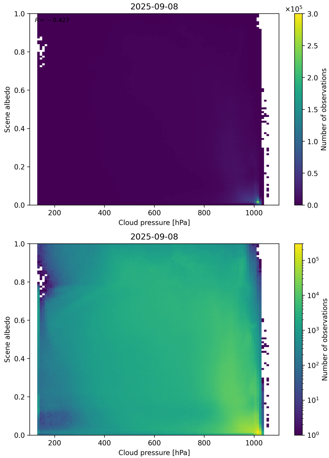
Figure 83: Scatter density plot of “Cloud pressure” against “Scene albedo” for 2025-09-07 to 2025-09-09.
