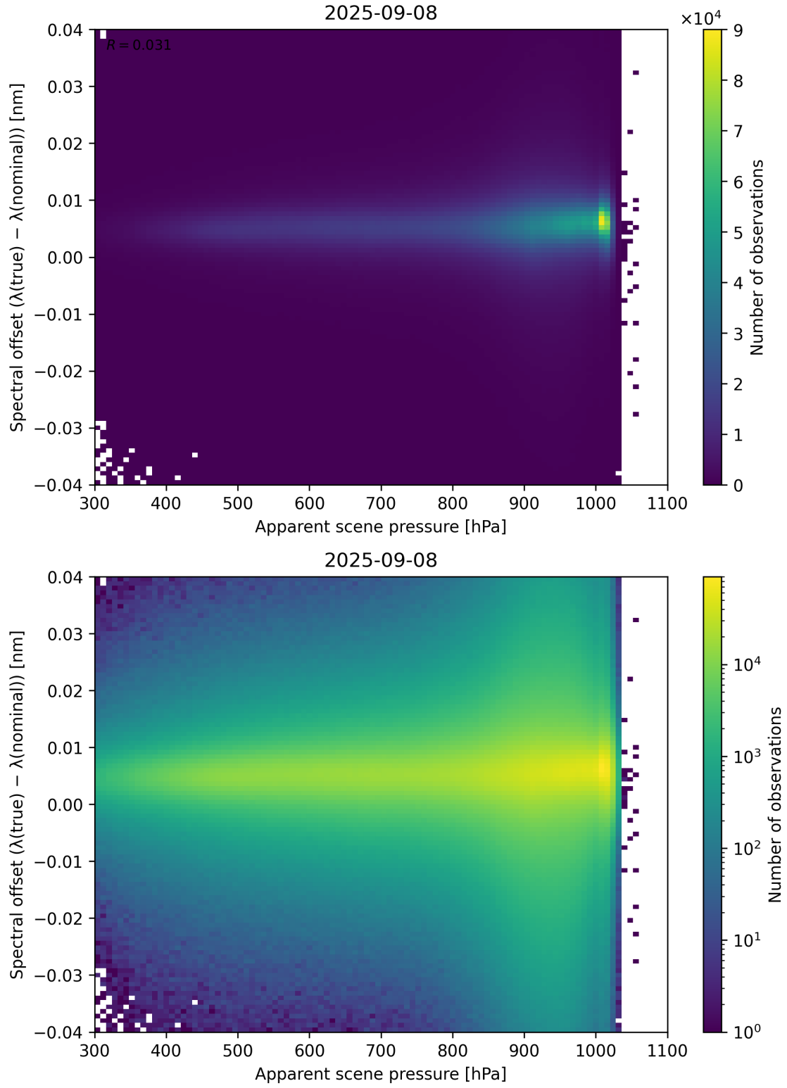
Figure 67: Scatter density plot of “Apparent scene pressure” against “Spectral offset ( \lambda_{\text{true}} - \lambda_{\text{nominal}} )” for 2025-09-07 to 2025-09-09.
