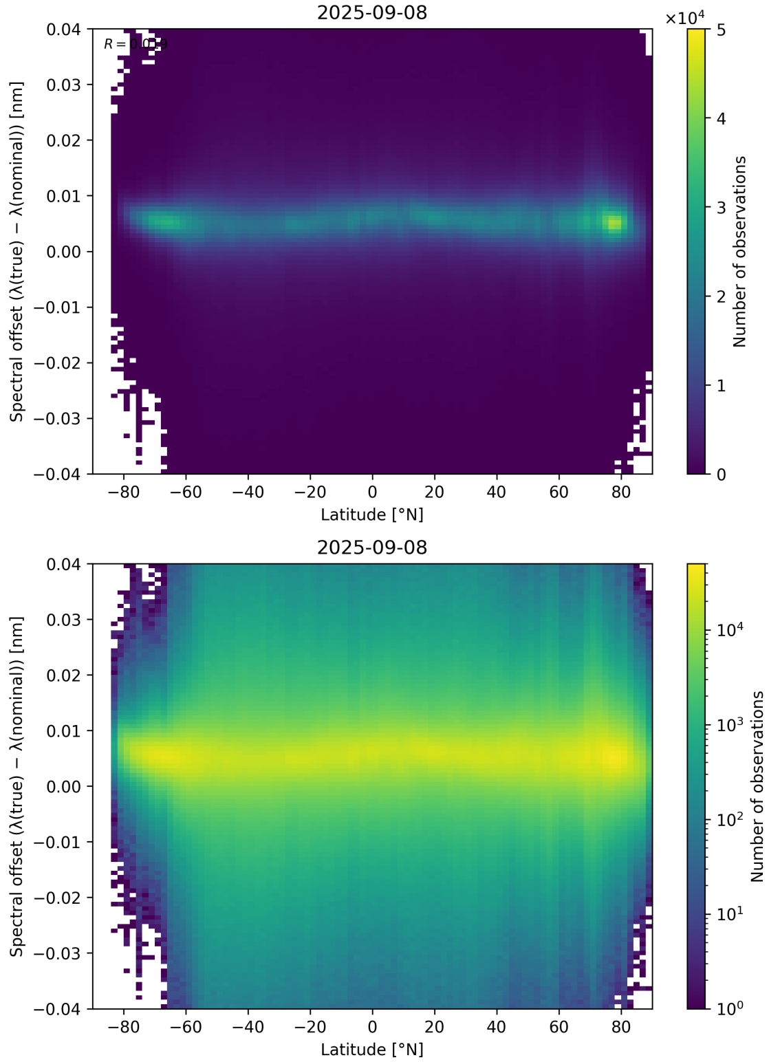
Figure 96: Scatter density plot of “Latitude” against “Spectral offset ( \lambda_{\text{true}} - \lambda_{\text{nominal}} )” for 2025-09-07 to 2025-09-09.
