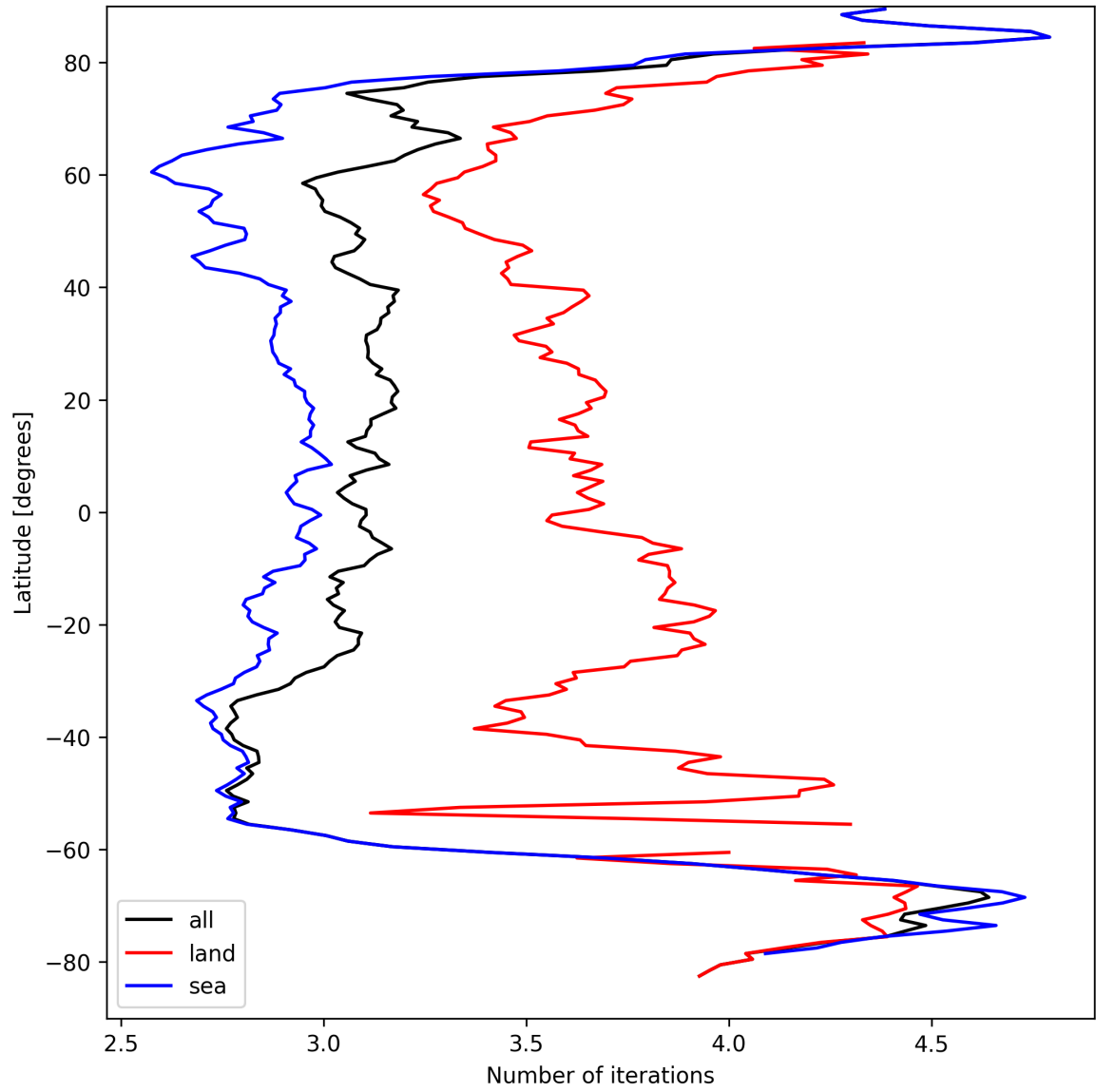
Figure 22: Zonal average of “Number of iterations” for 2025-09-07 to 2025-09-09.
