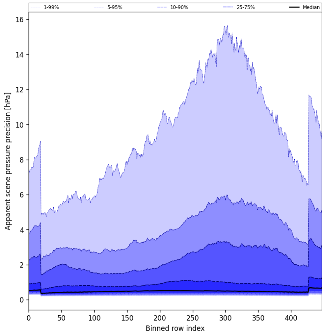
Figure 54: Along track statistics of “Apparent scene pressure precision” for 2025-09-07 to 2025-09-09
