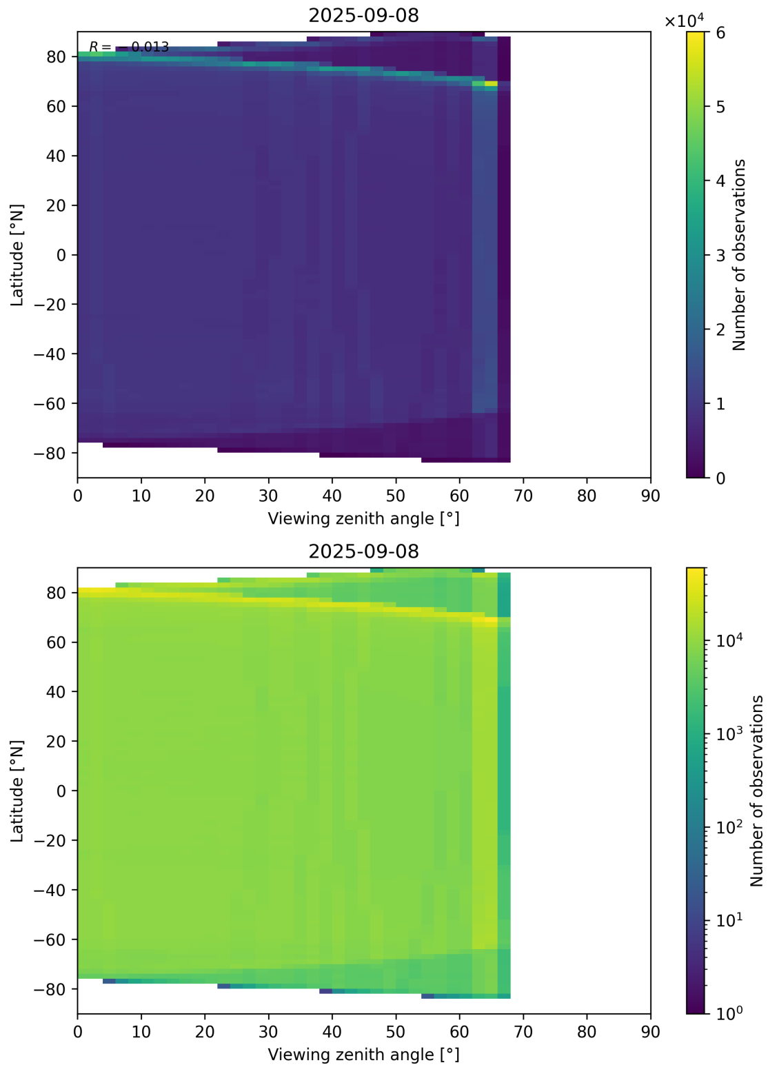
Figure 123: Scatter density plot of “Viewing zenith angle” against “Latitude” for 2025-09-07 to 2025-09-09.
