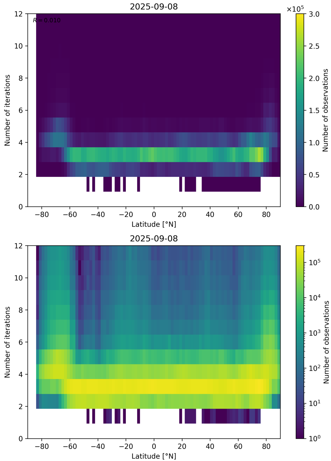
Figure 93: Scatter density plot of “Latitude” against “Number of iterations” for 2025-09-07 to 2025-09-09.
