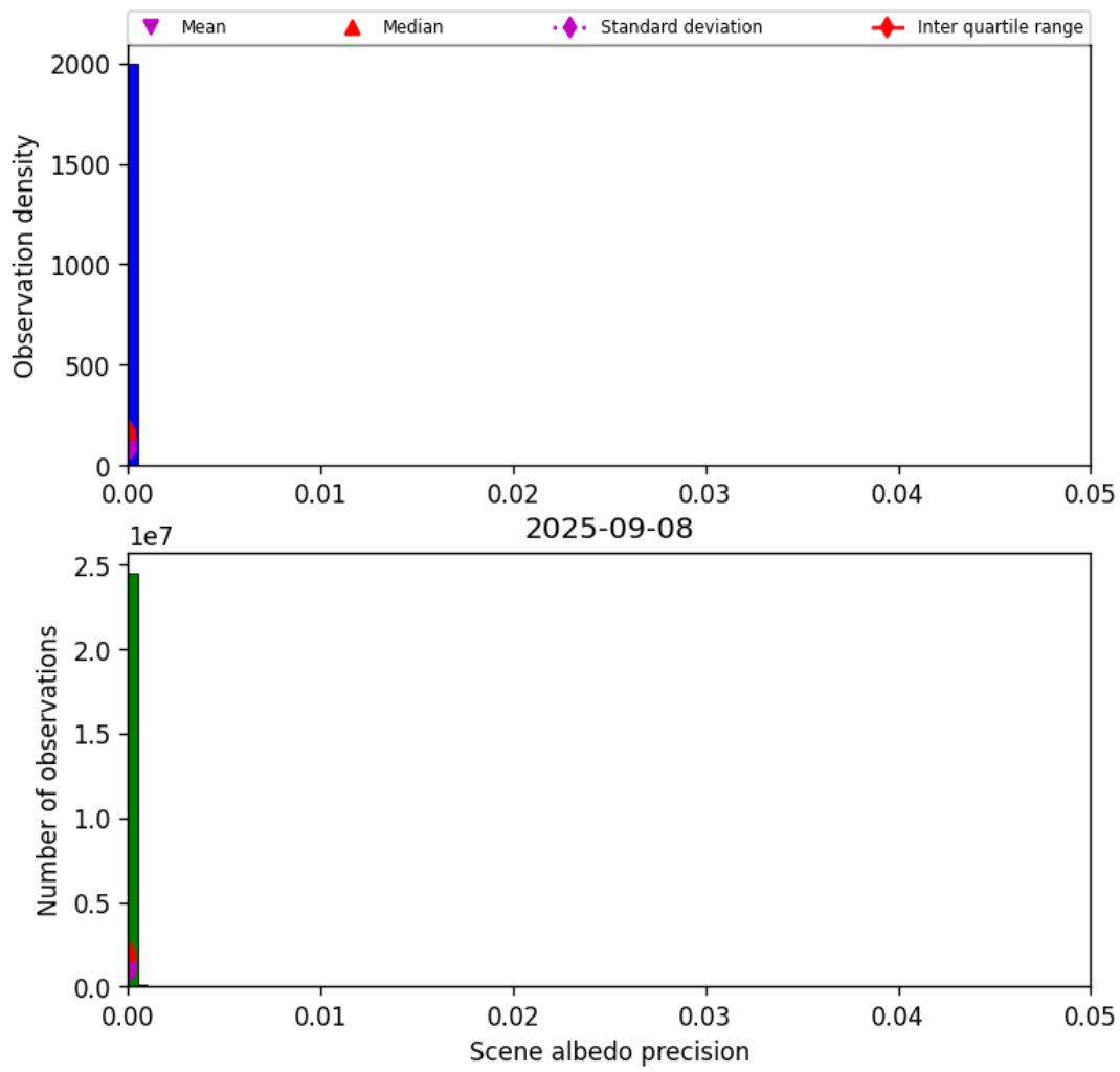
Figure 35: Histogram of “Scene albedo precision” for 2025-09-07 to 2025-09-09
