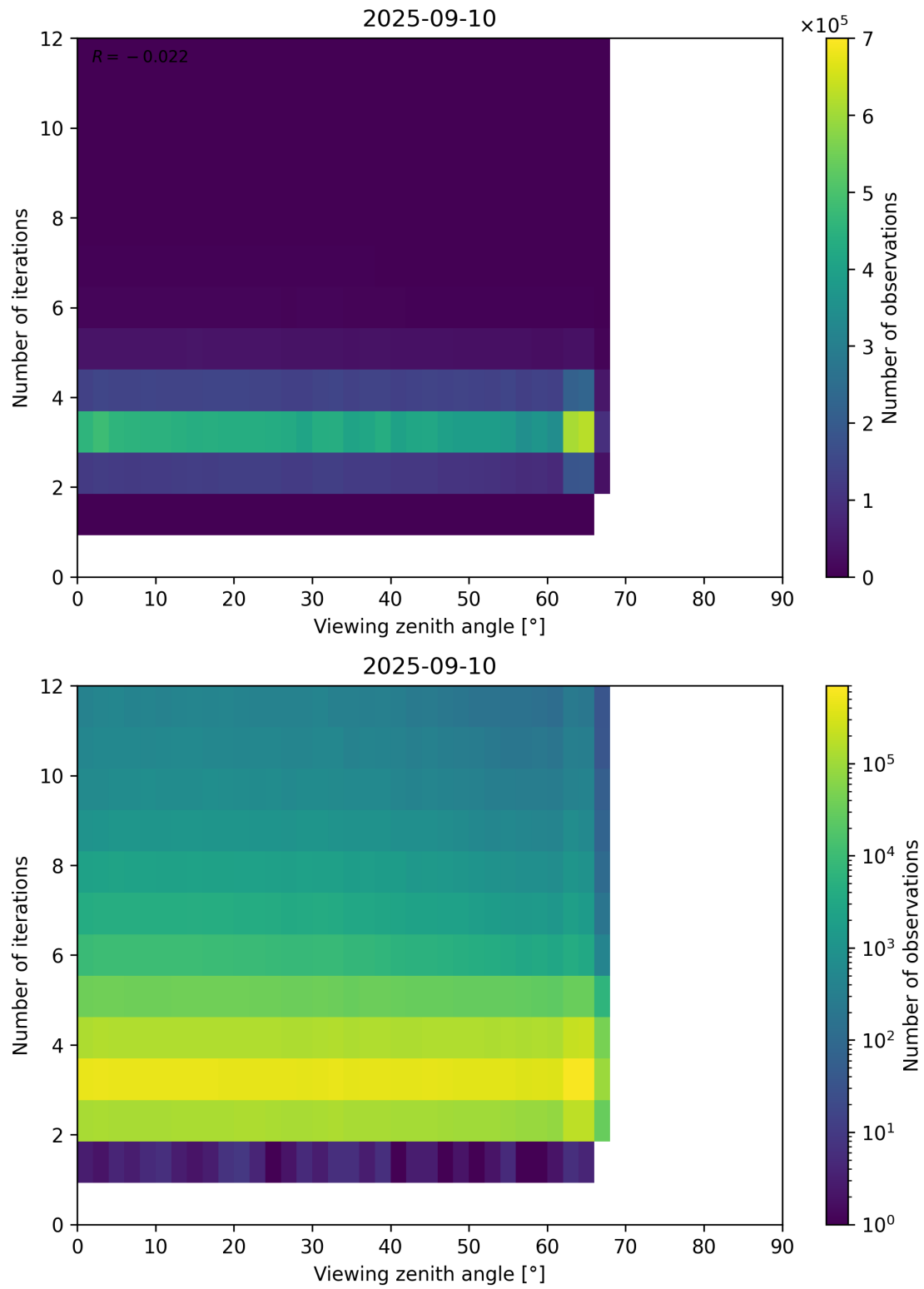
Figure 124: Scatter density plot of “Viewing zenith angle” against “Number of iterations” for 2025-09-10 to 2025-09-11.
