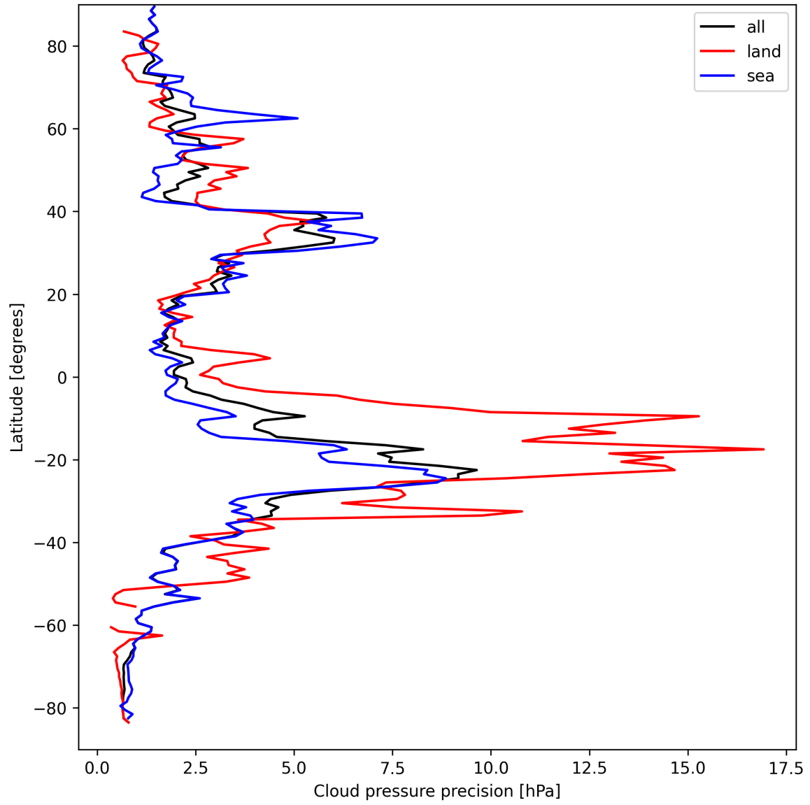
Figure 14: Zonal average of “Cloud pressure precision” for 2025-09-10 to 2025-09-11.
