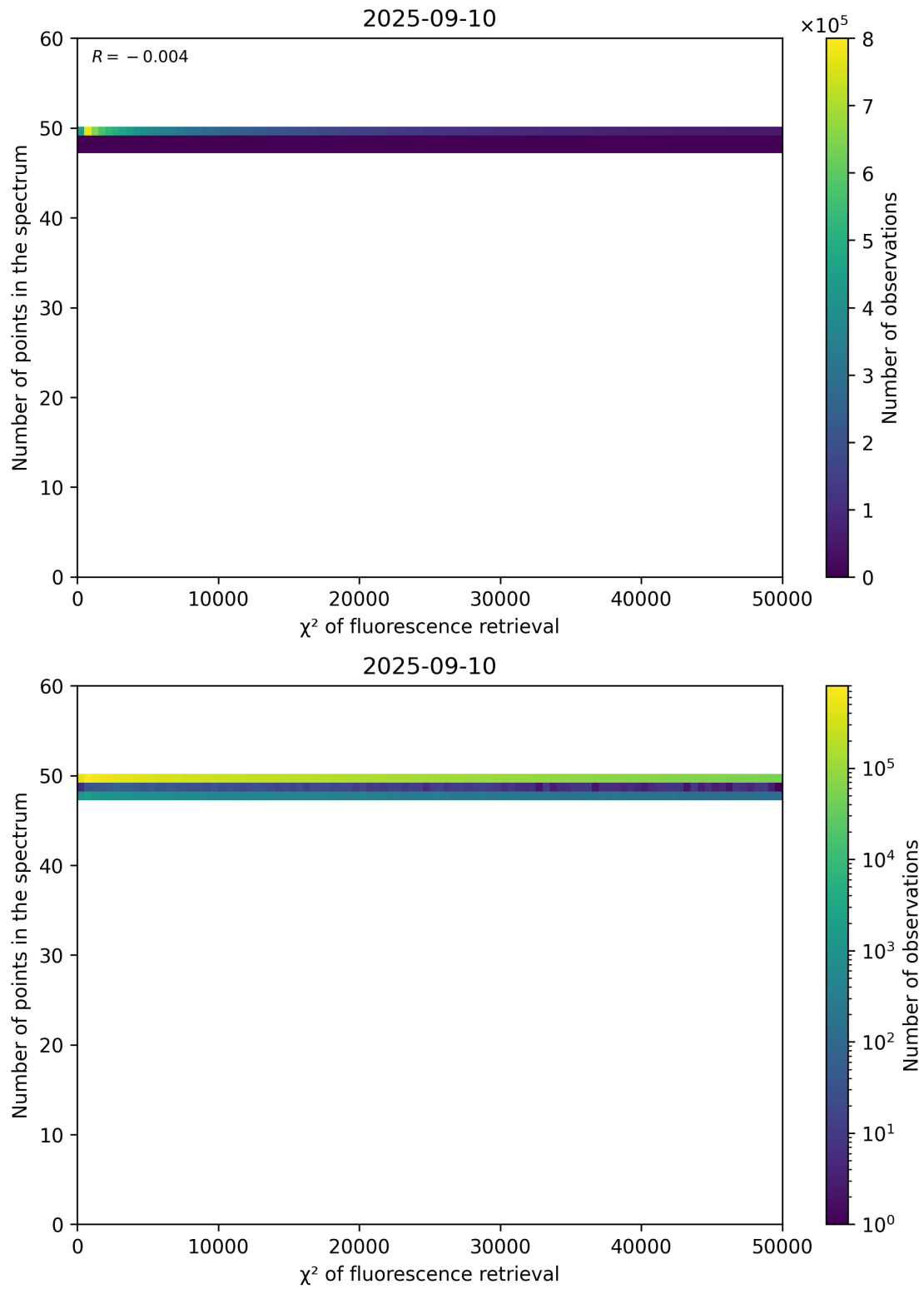
Figure 68: Scatter density plot of “ \chi^2 of fluorescence retrieval” against “Number of points in the spectrum” for 2025-09-10 to 2025-09-11.
