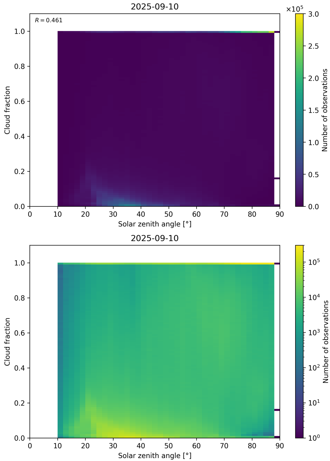
Figure 110: Scatter density plot of “Solar zenith angle” against “Cloud fraction” for 2025-09-10 to 2025-09-11.
