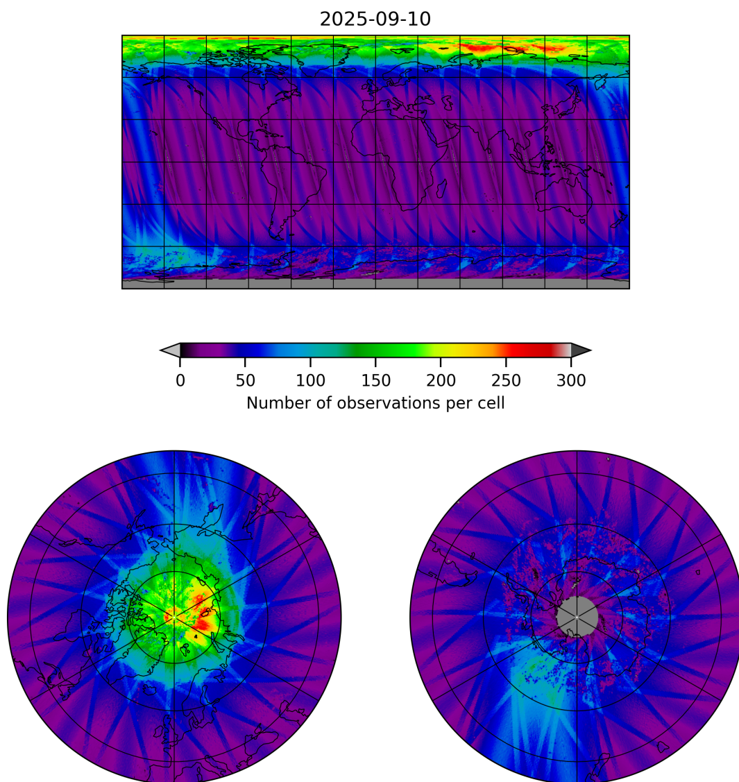
Figure 11: Map of the number of observations for 2025-09-10 to 2025-09-11
