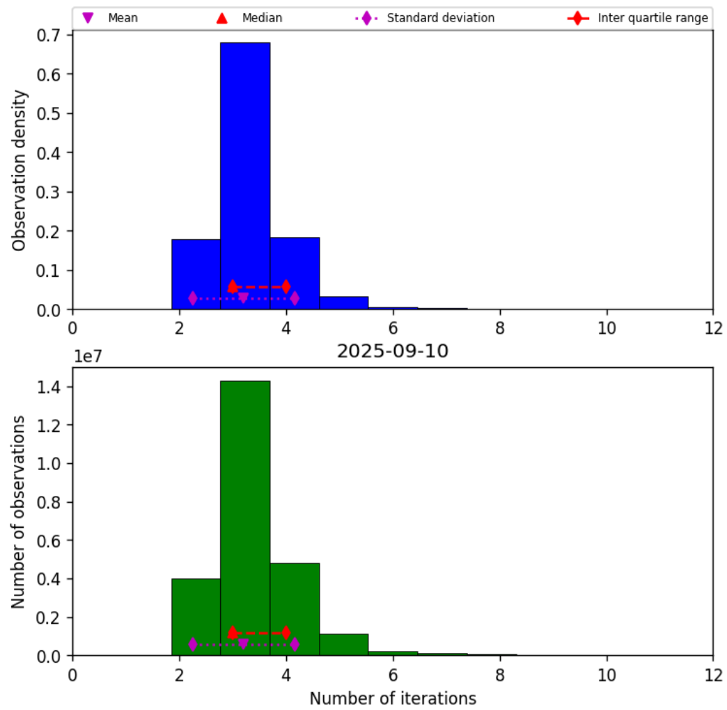
Figure 39: Histogram of “Number of iterations” for 2025-09-10 to 2025-09-11
