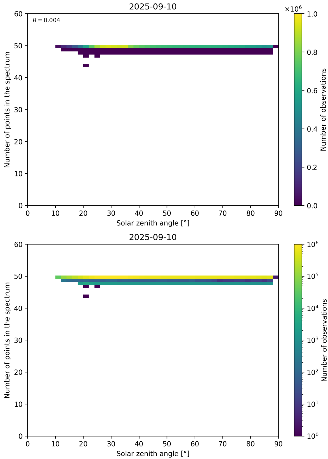
Figure 115: Scatter density plot of “Solar zenith angle” against “Number of points in the spectrum” for 2025-09-10 to 2025-09-11.
