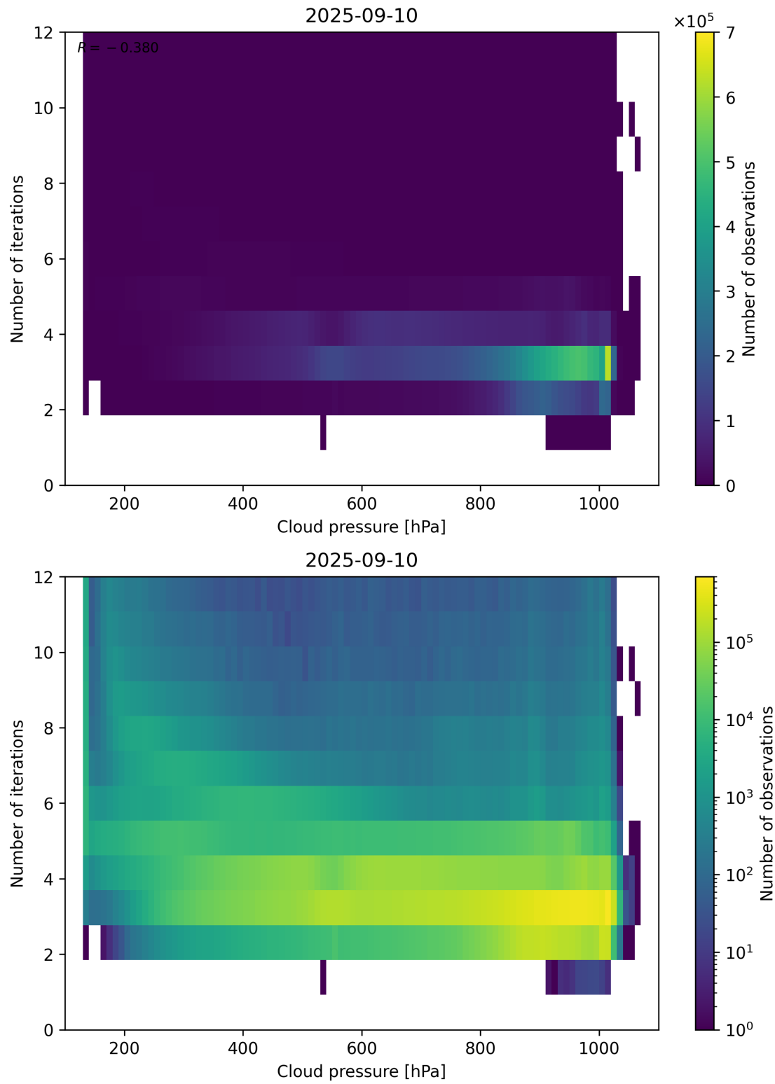
Figure 81: Scatter density plot of “Cloud pressure” against “Number of iterations” for 2025-09-10 to 2025-09-11.
