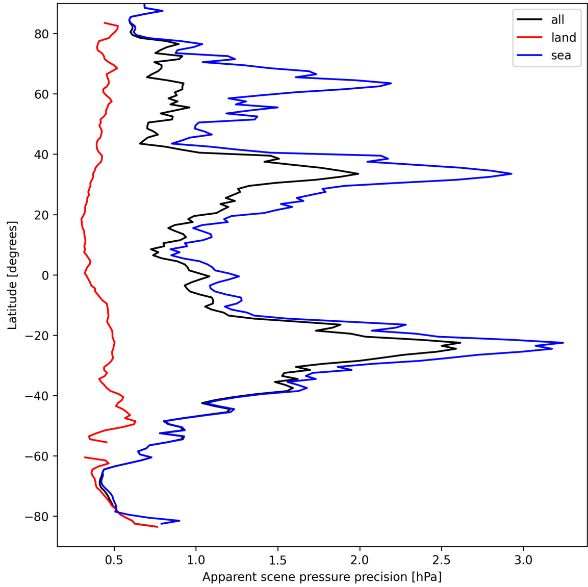
Figure 20: Zonal average of “Apparent scene pressure precision” for 2025-09-10 to 2025-09-11.
