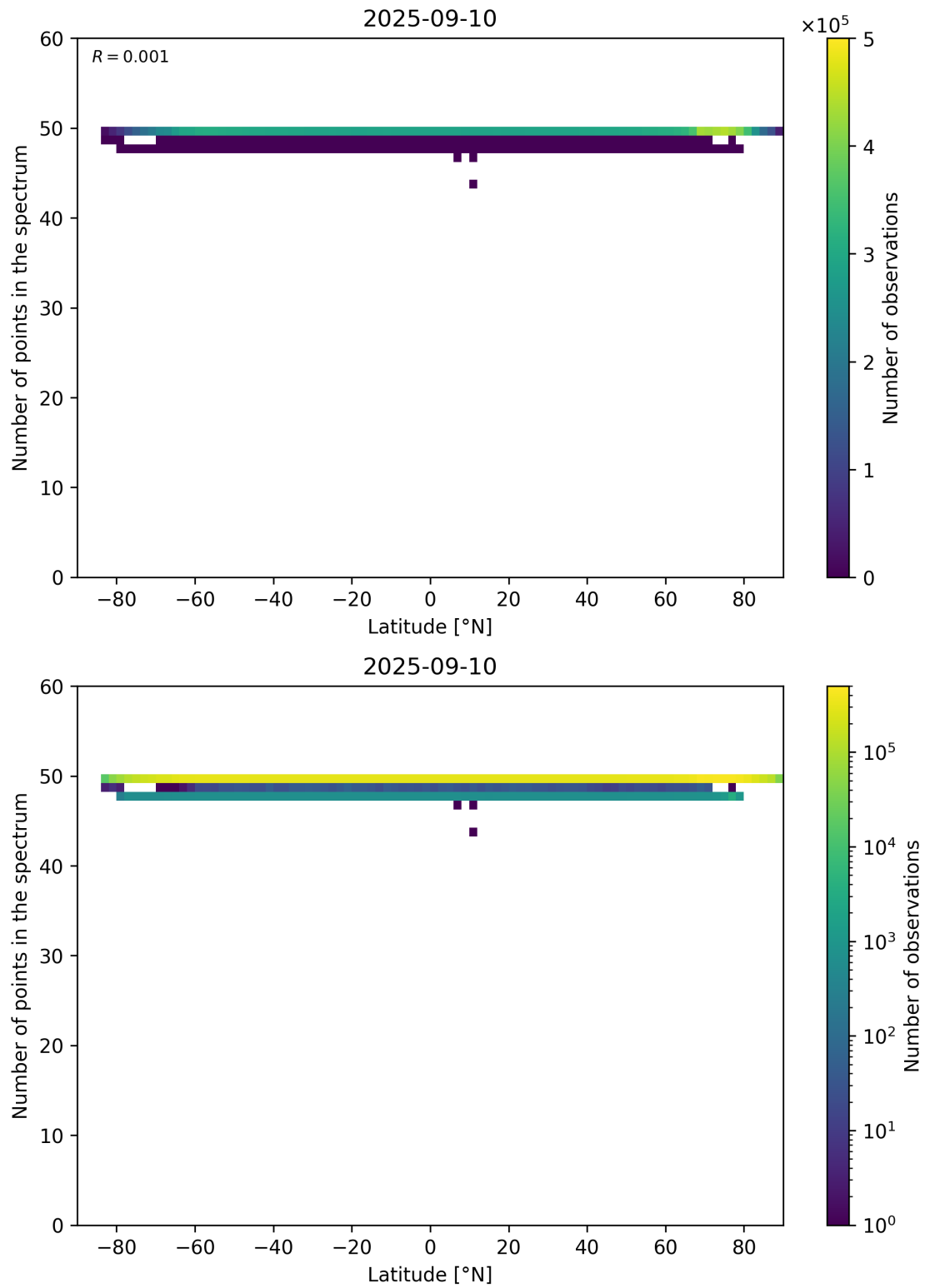
Figure 94: Scatter density plot of “Latitude” against “Number of points in the spectrum” for 2025-09-10 to 2025-09-11.
