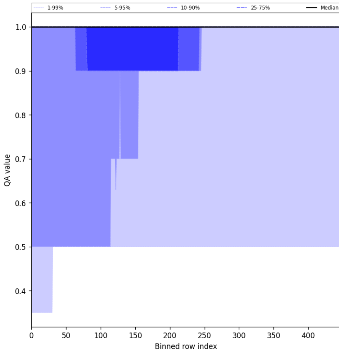
Figure 46: Along track statistics of “QA value” for 2025-09-10 to 2025-09-11
