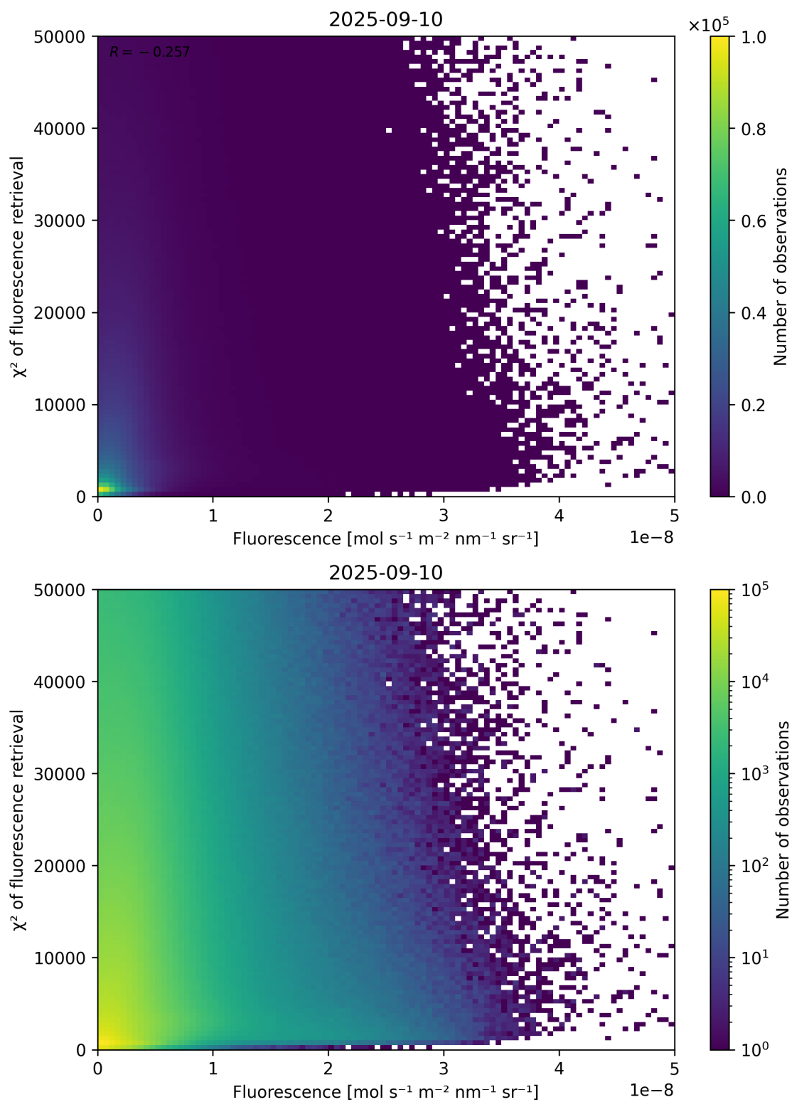
Figure 85: Scatter density plot of “Fluorescence” against “ \chi^2 of fluorescence retrieval” for 2025-09-10 to 2025-09-11.
