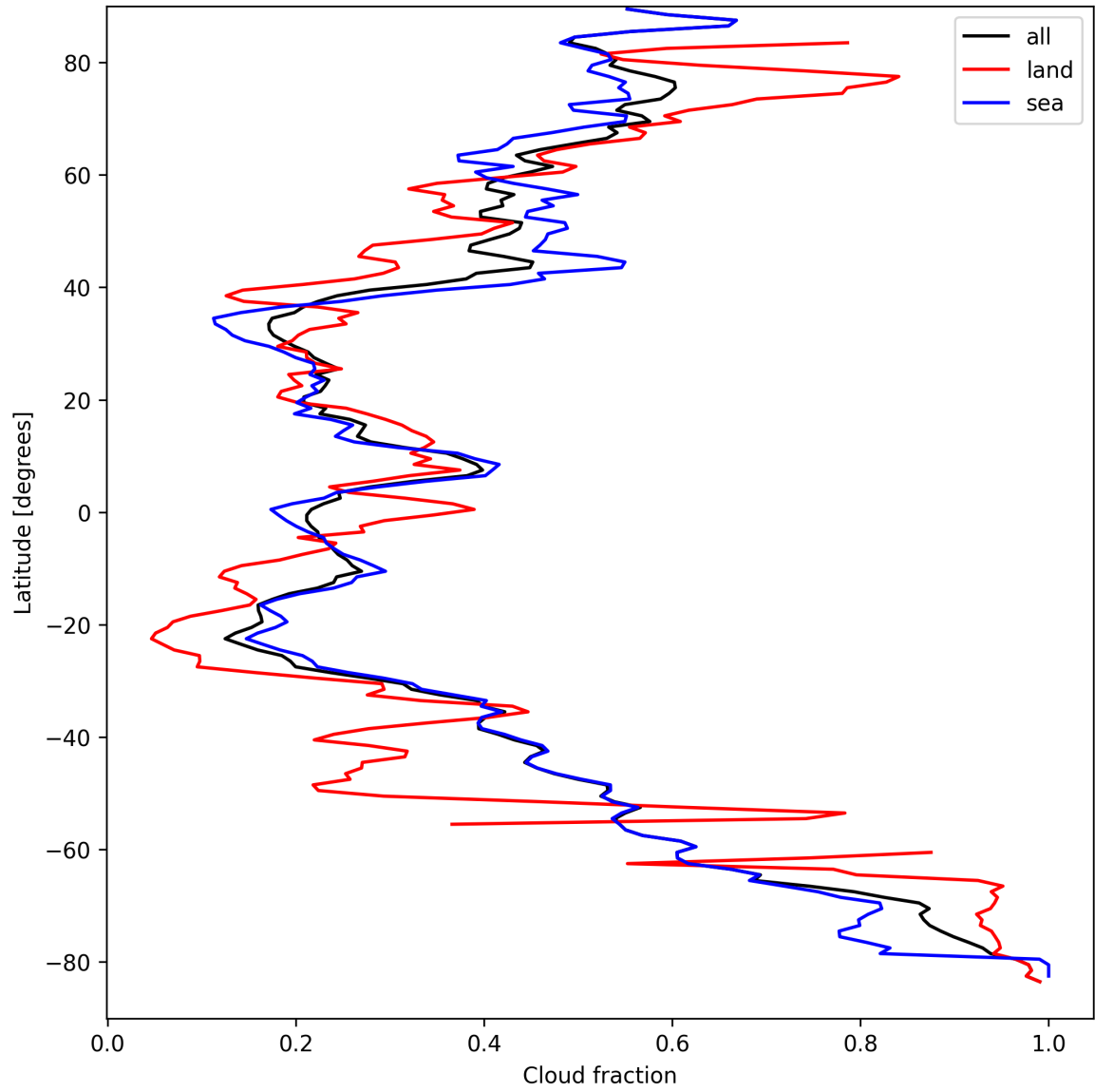
Figure 15: Zonal average of “Cloud fraction” for 2025-09-10 to 2025-09-11.
