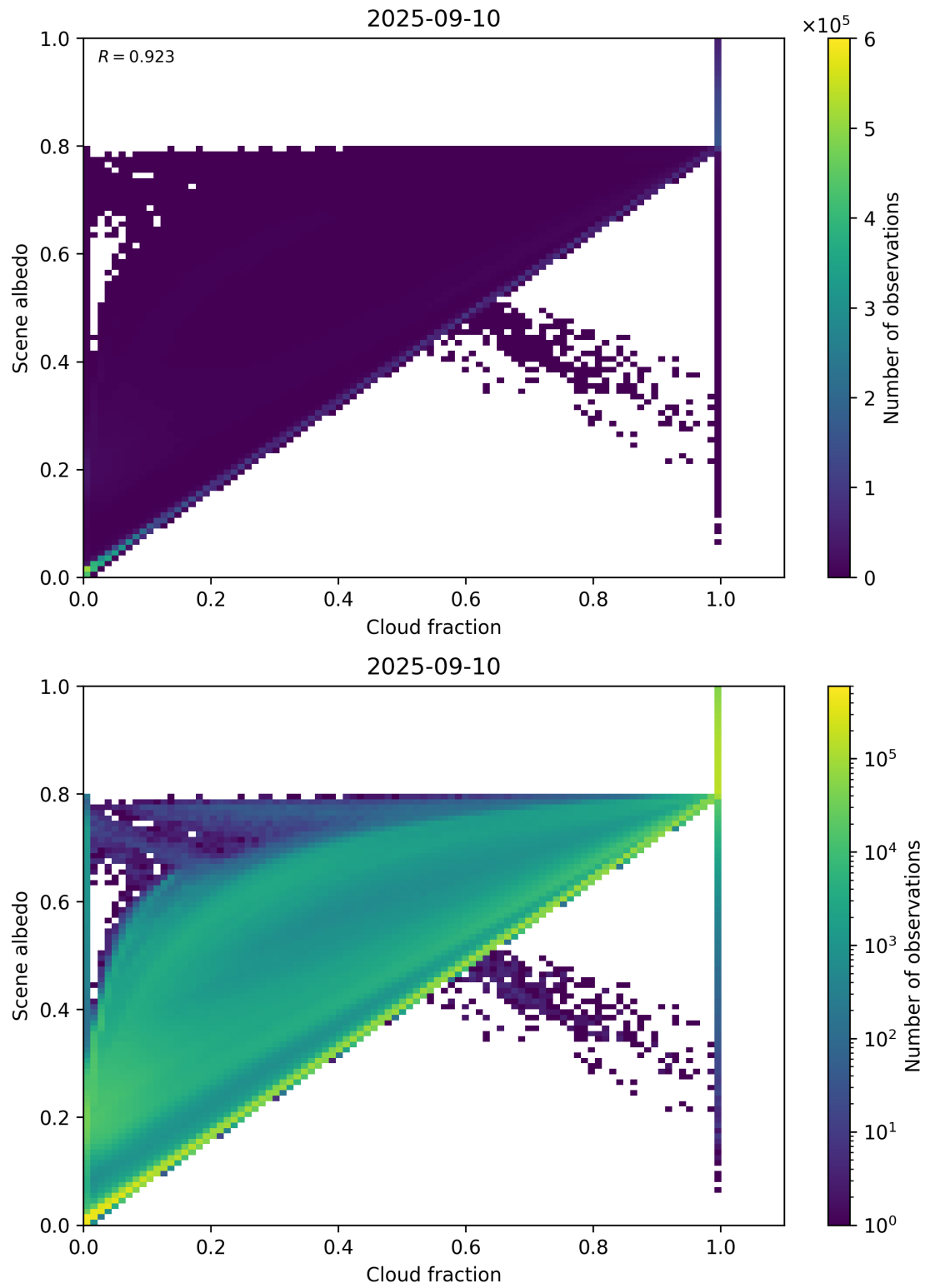
Figure 75: Scatter density plot of “Cloud fraction” against “Scene albedo” for 2025-09-10 to 2025-09-11.
