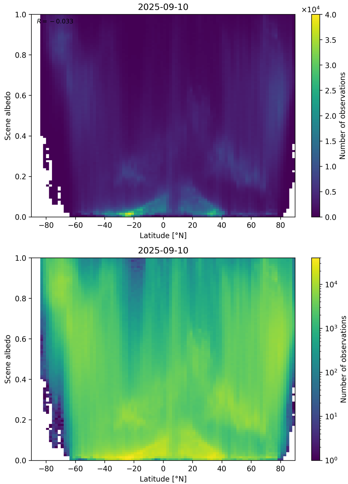
Figure 95: Scatter density plot of “Latitude” against “Scene albedo” for 2025-09-10 to 2025-09-11.
