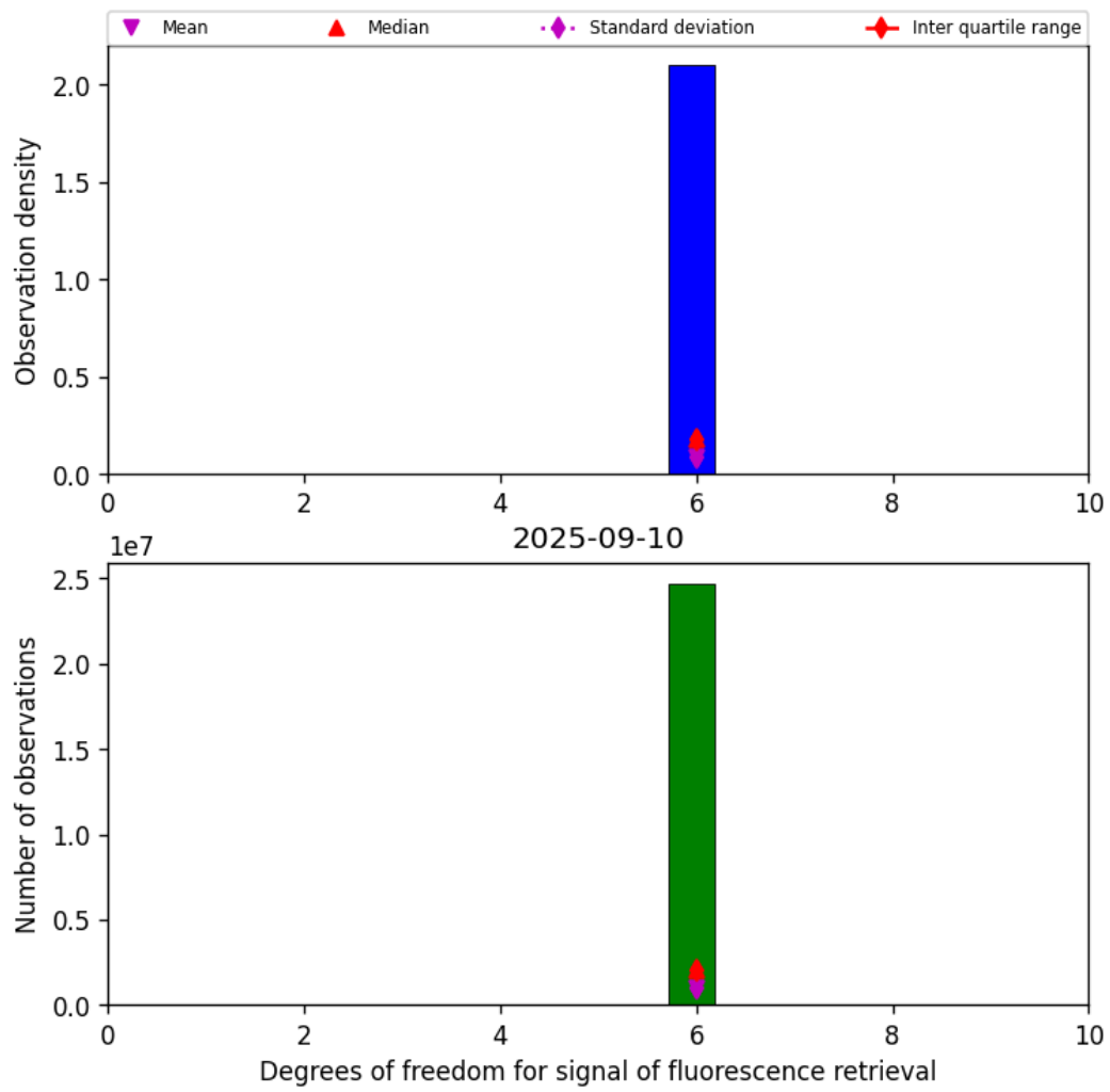
Figure 43: Histogram of “Degrees of freedom for signal of fluorescence retrieval” for 2025-09-10 to 2025-09-11
