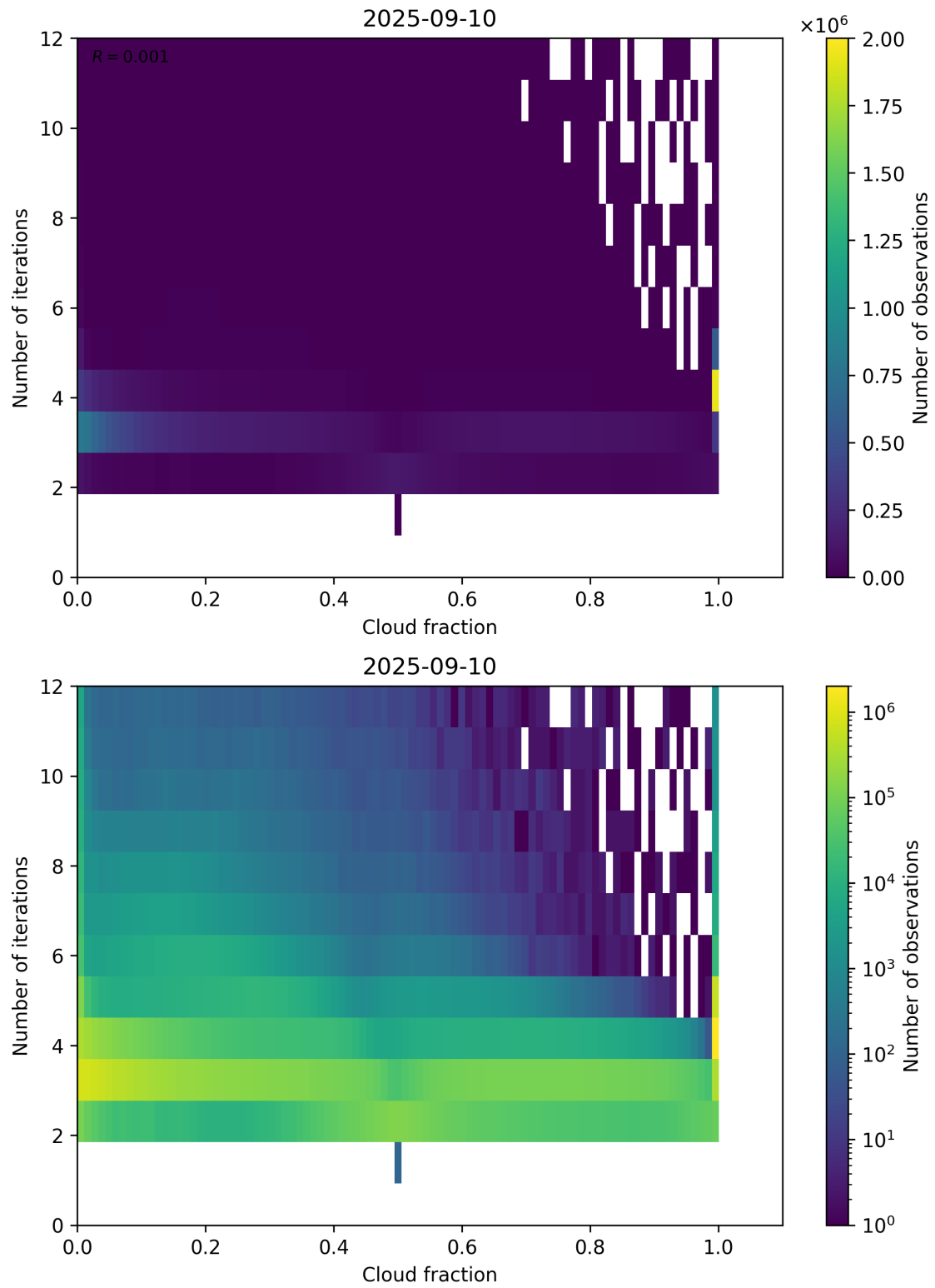
Figure 73: Scatter density plot of “Cloud fraction” against “Number of iterations” for 2025-09-10 to 2025-09-11.
