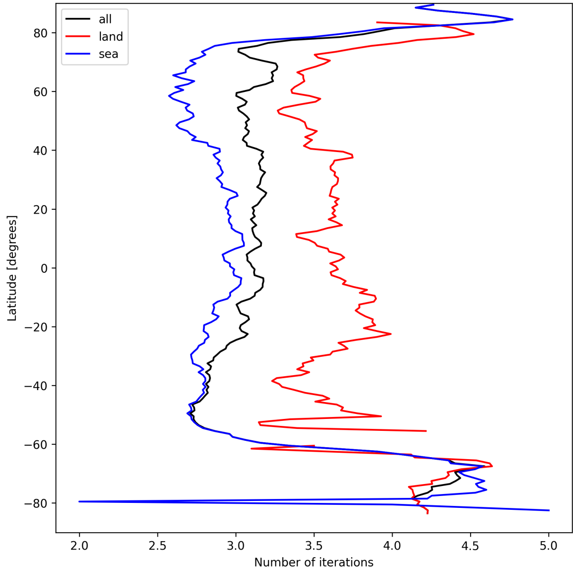
Figure 22: Zonal average of “Number of iterations” for 2025-09-10 to 2025-09-11.
