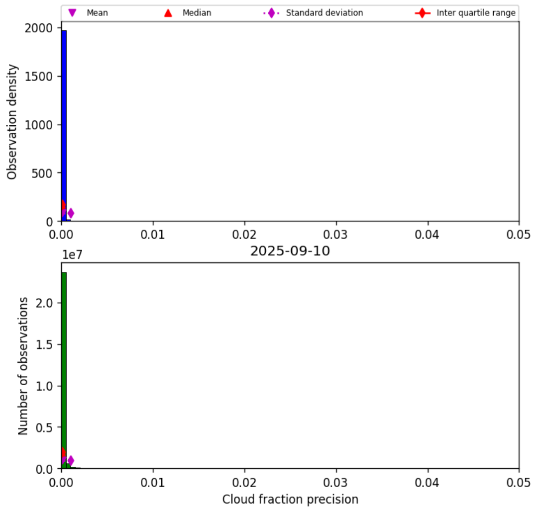
Figure 33: Histogram of “Cloud fraction precision” for 2025-09-10 to 2025-09-11
