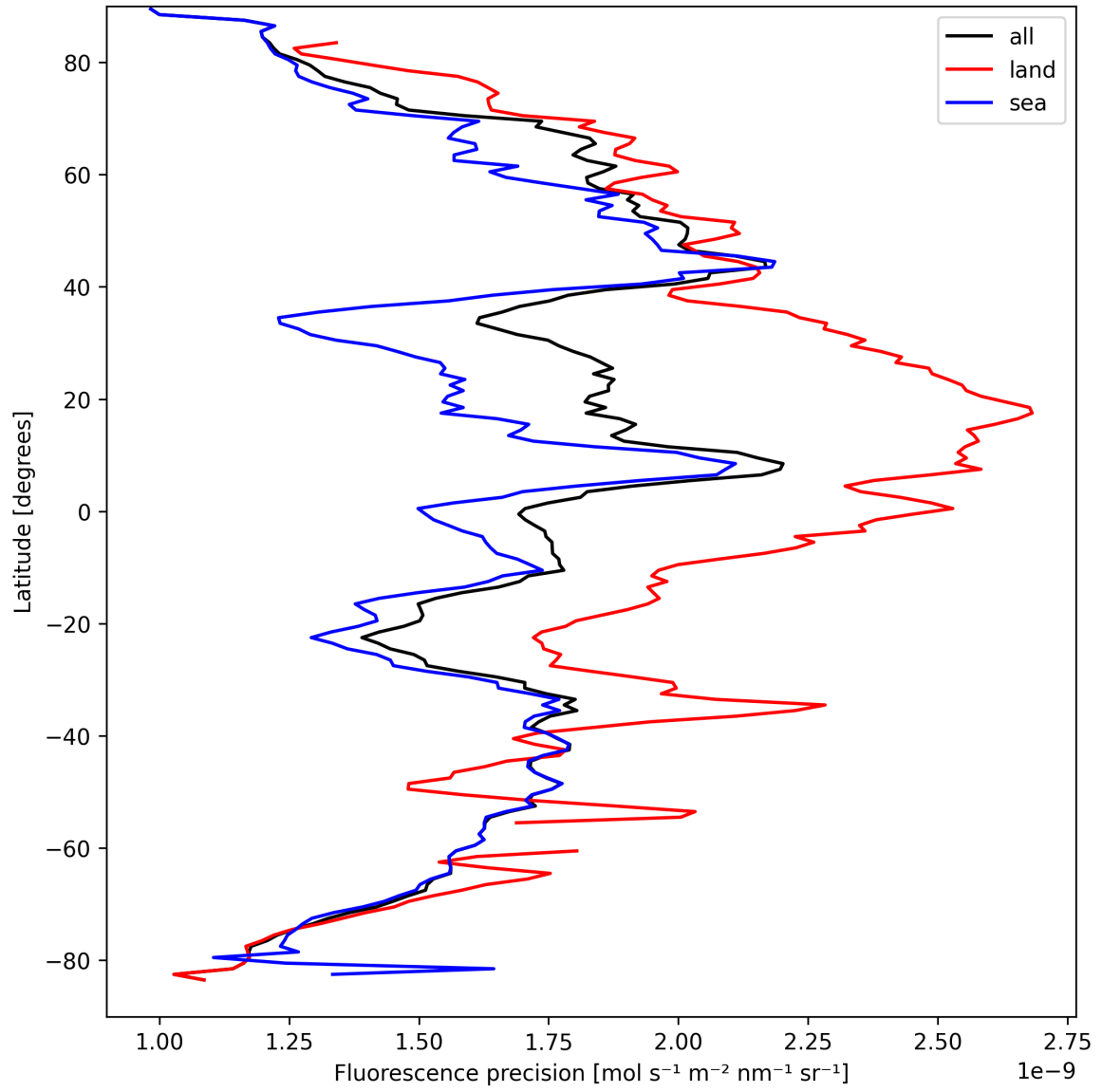
Figure 24: Zonal average of “Fluorescence precision” for 2025-09-10 to 2025-09-11.
