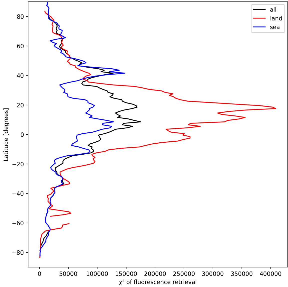
Figure 25: Zonal average of “ \chi^2 of fluorescence retrieval” for 2025-09-10 to 2025-09-11.
