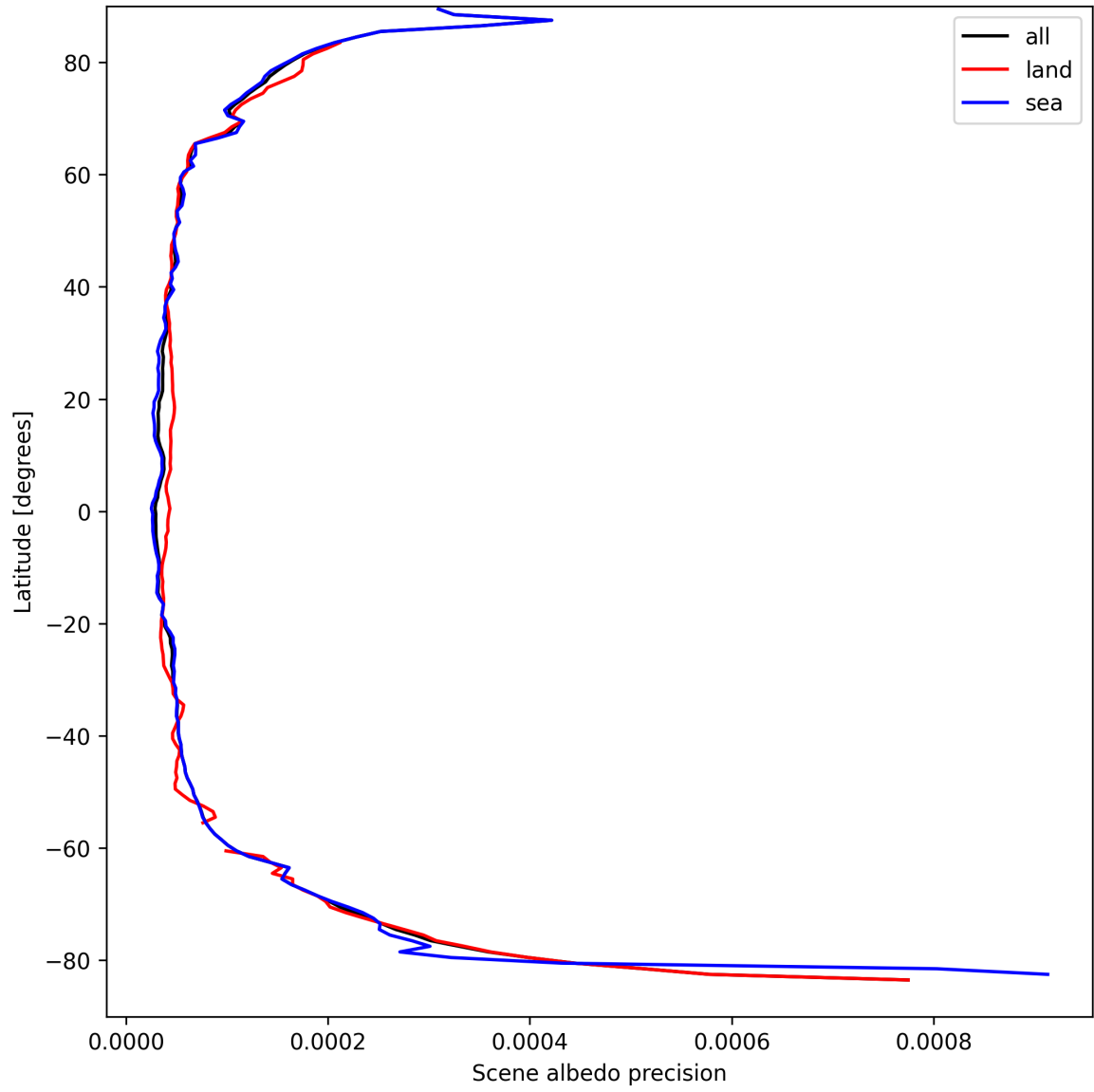
Figure 18: Zonal average of “Scene albedo precision” for 2025-09-10 to 2025-09-11.
