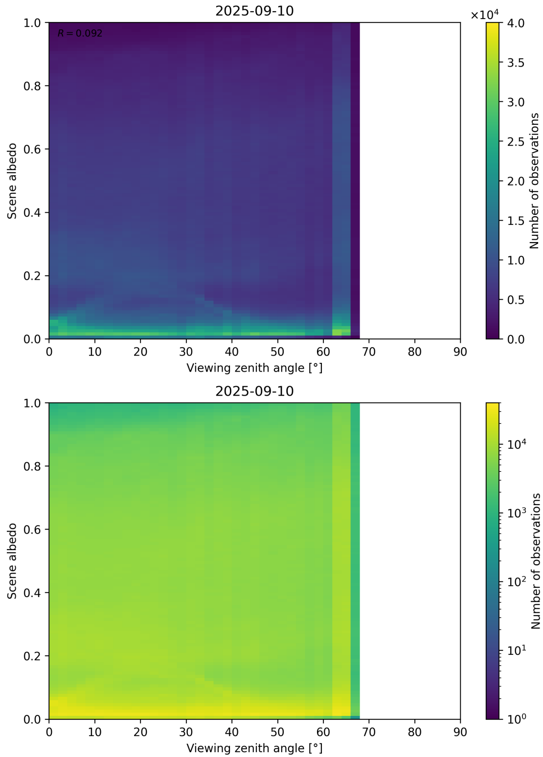
Figure 126: Scatter density plot of “Viewing zenith angle” against “Scene albedo” for 2025-09-10 to 2025-09-11.
