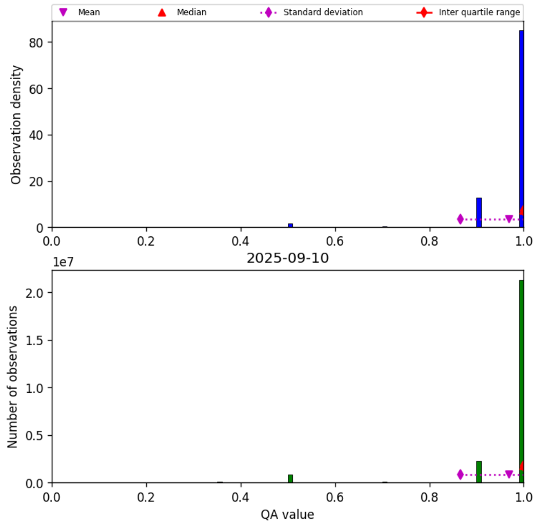
Figure 29: Histogram of “QA value” for 2025-09-10 to 2025-09-11
