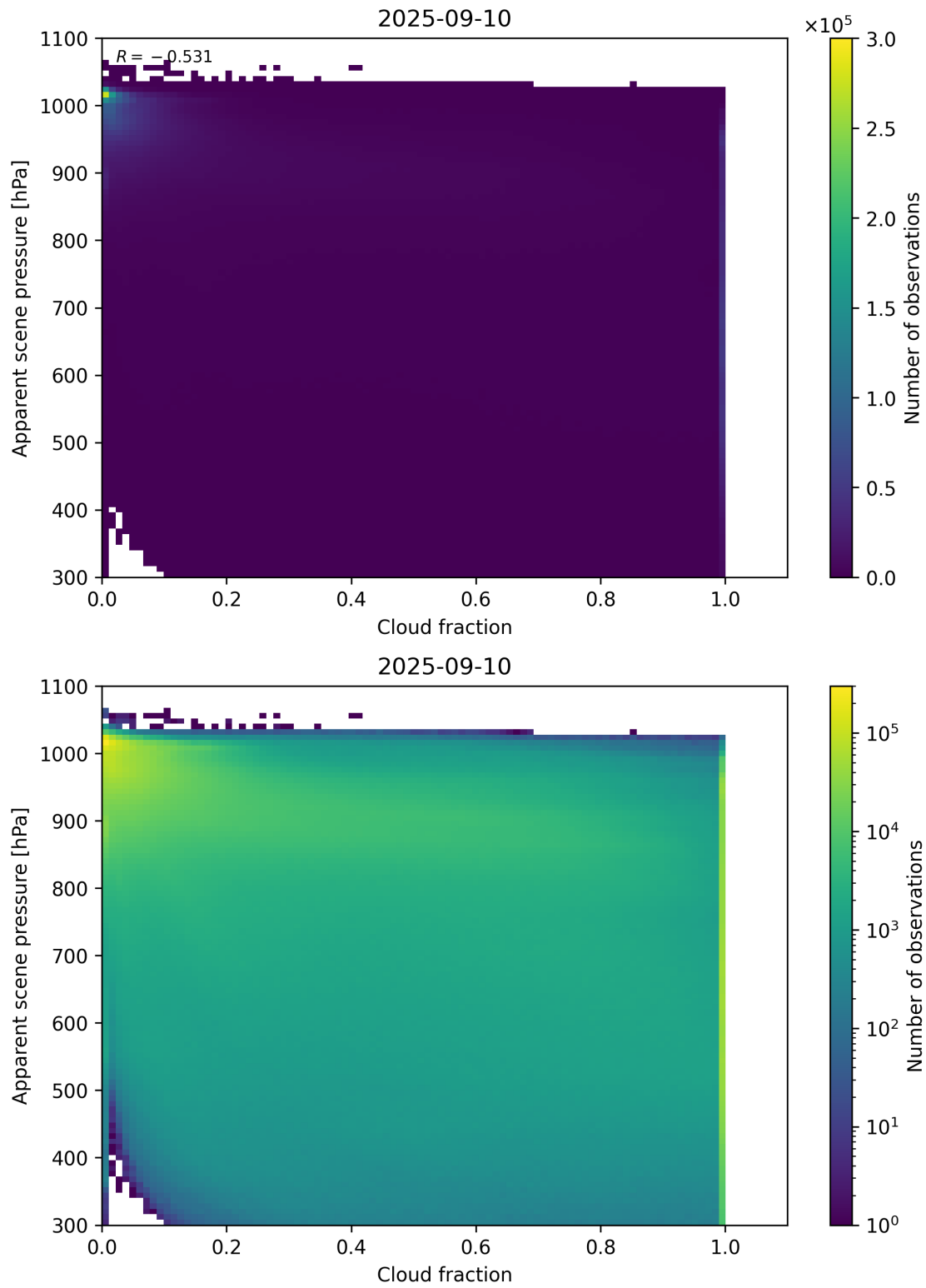
Figure 70: Scatter density plot of “Cloud fraction” against “Apparent scene pressure” for 2025-09-10 to 2025-09-11.
