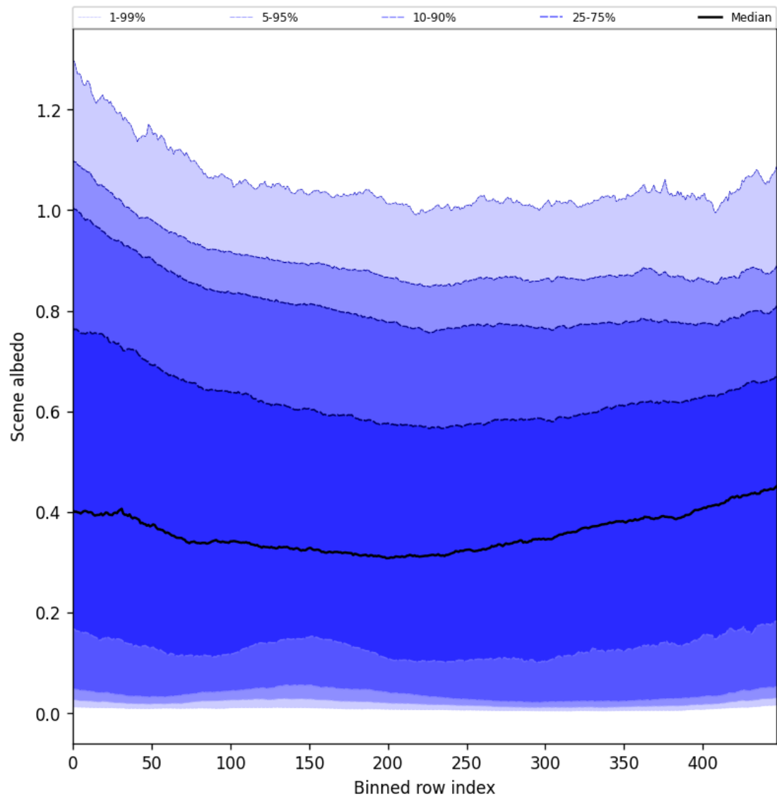
Figure 51: Along track statistics of “Scene albedo” for 2025-09-10 to 2025-09-11
