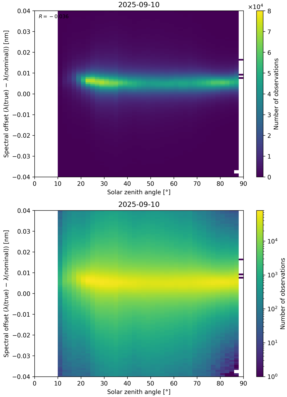
Figure 117: Scatter density plot of “Solar zenith angle” against “Spectral offset ( \lambda_{\text{true}} - \lambda_{\text{nominal}} )” for 2025-09-10 to 2025-09-11.
