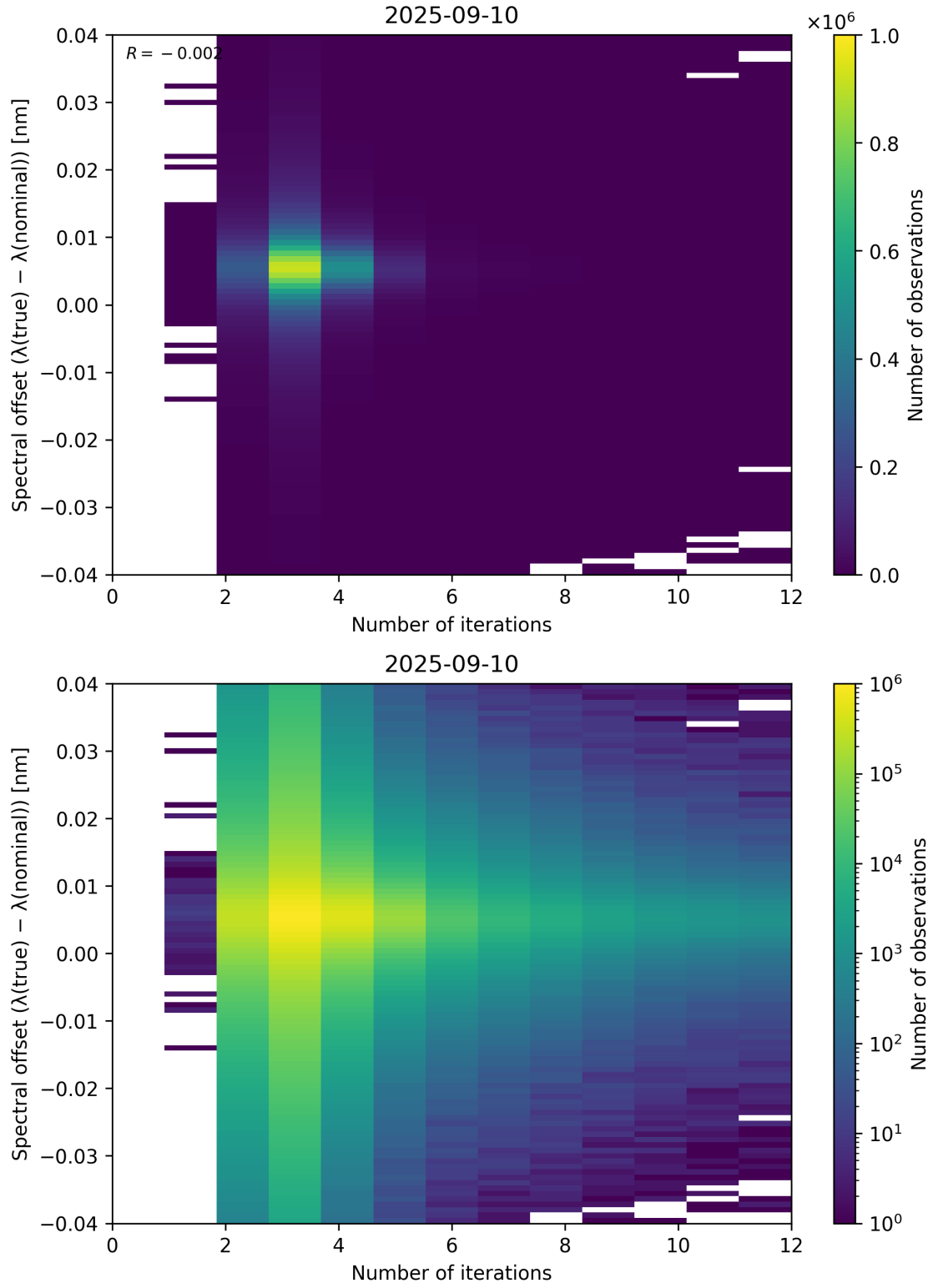
Figure 100: Scatter density plot of “Number of iterations” against “Spectral offset ( \lambda_{\text{true}} - \lambda_{\text{nominal}} )” for 2025-09-10 to 2025-09-11.
