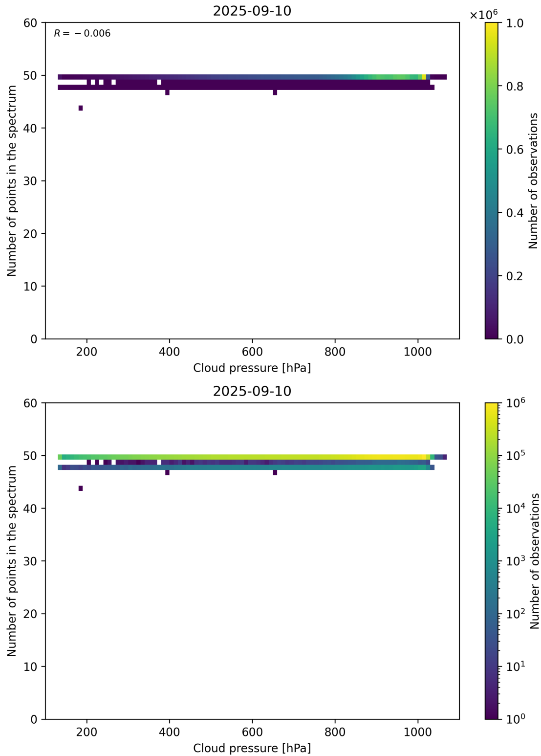
Figure 82: Scatter density plot of “Cloud pressure” against “Number of points in the spectrum” for 2025-09-10 to 2025-09-11.
