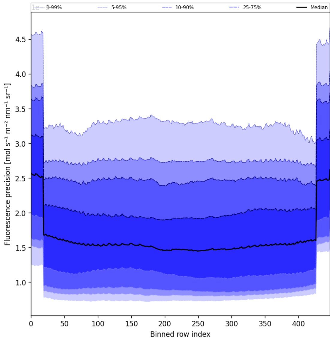
Figure 58: Along track statistics of “Fluorescence precision” for 2025-09-10 to 2025-09-11
