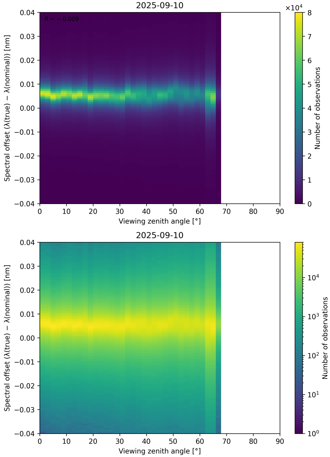
Figure 128: Scatter density plot of “Viewing zenith angle” against “Spectral offset ( \lambda_{\text{true}} - \lambda_{\text{nominal}} )” for 2025-09-10 to 2025-09-11.
