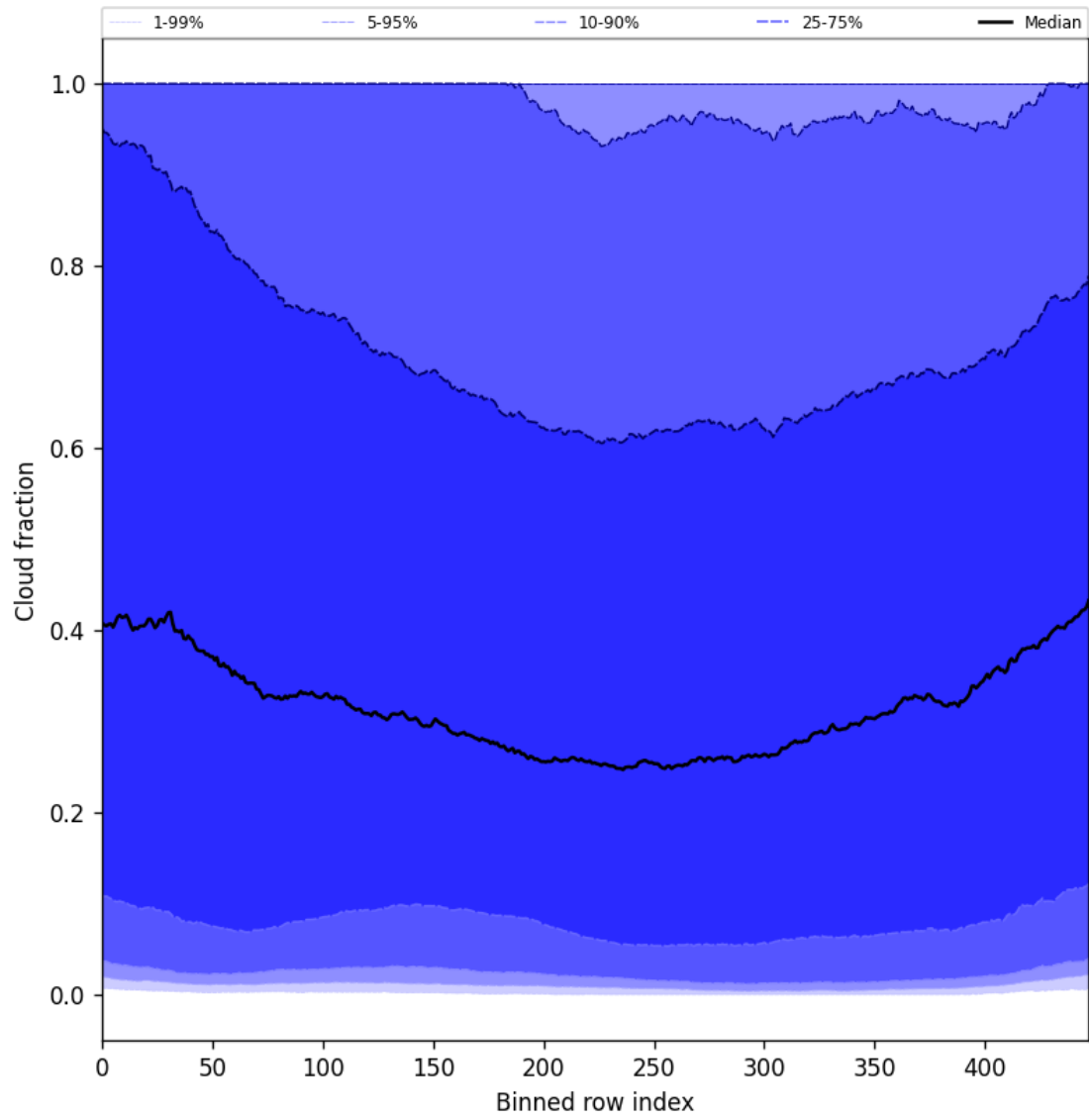
Figure 49: Along track statistics of “Cloud fraction” for 2025-09-10 to 2025-09-11
