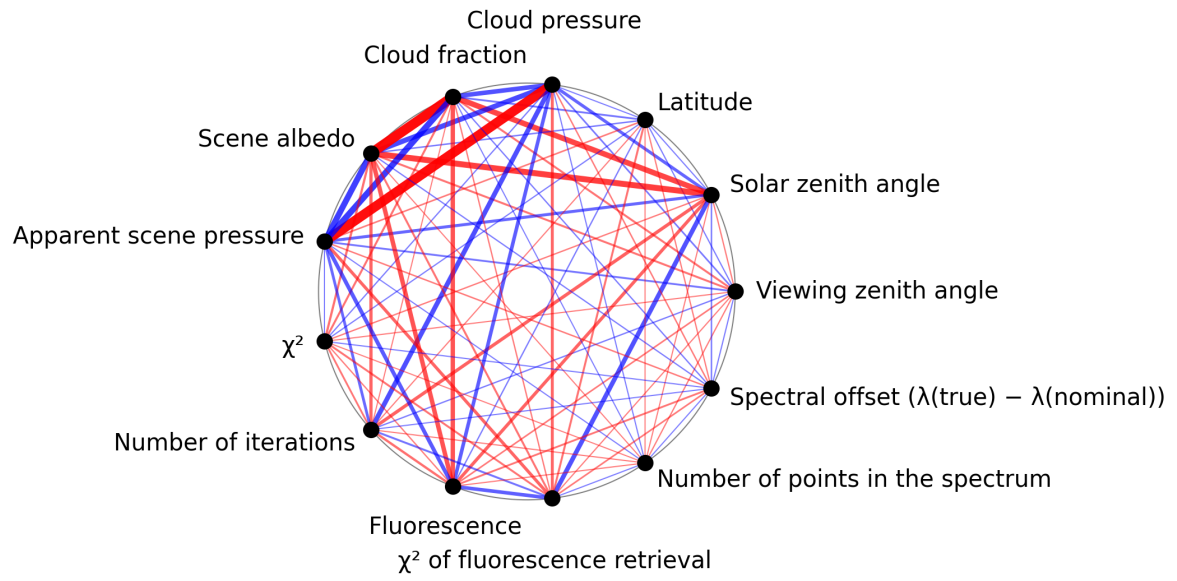
Figure 1: Map of correlation graph for 2025-09-10 to 2025-09-11.
