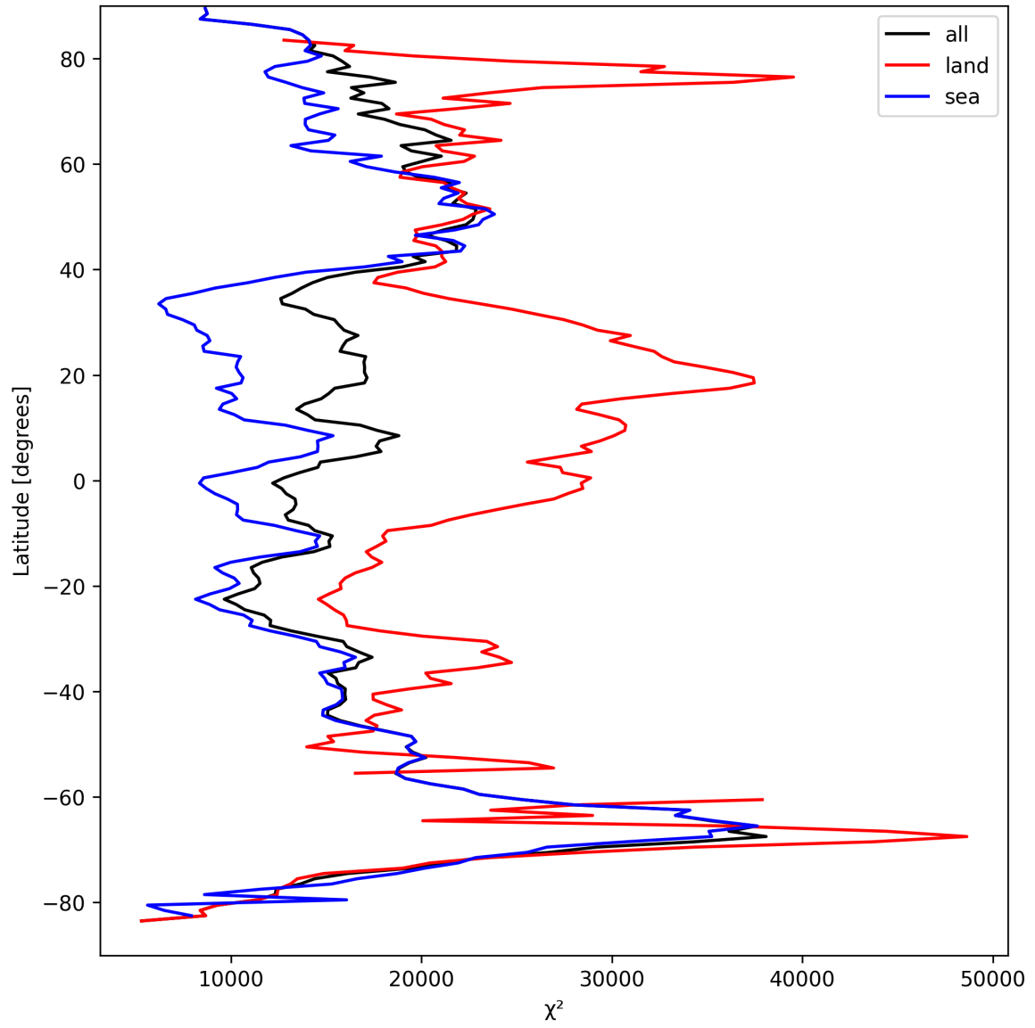
Figure 21: Zonal average of “ \chi^2 ” for 2025-09-10 to 2025-09-11.
