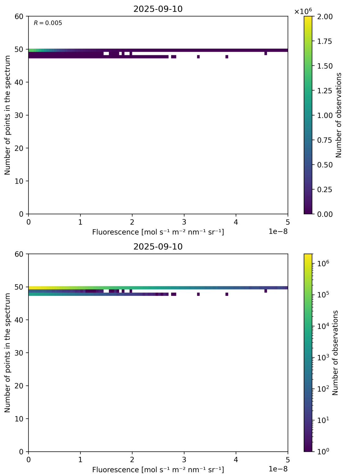
Figure 86: Scatter density plot of “Fluorescence” against “Number of points in the spectrum” for 2025-09-10 to 2025-09-11.
