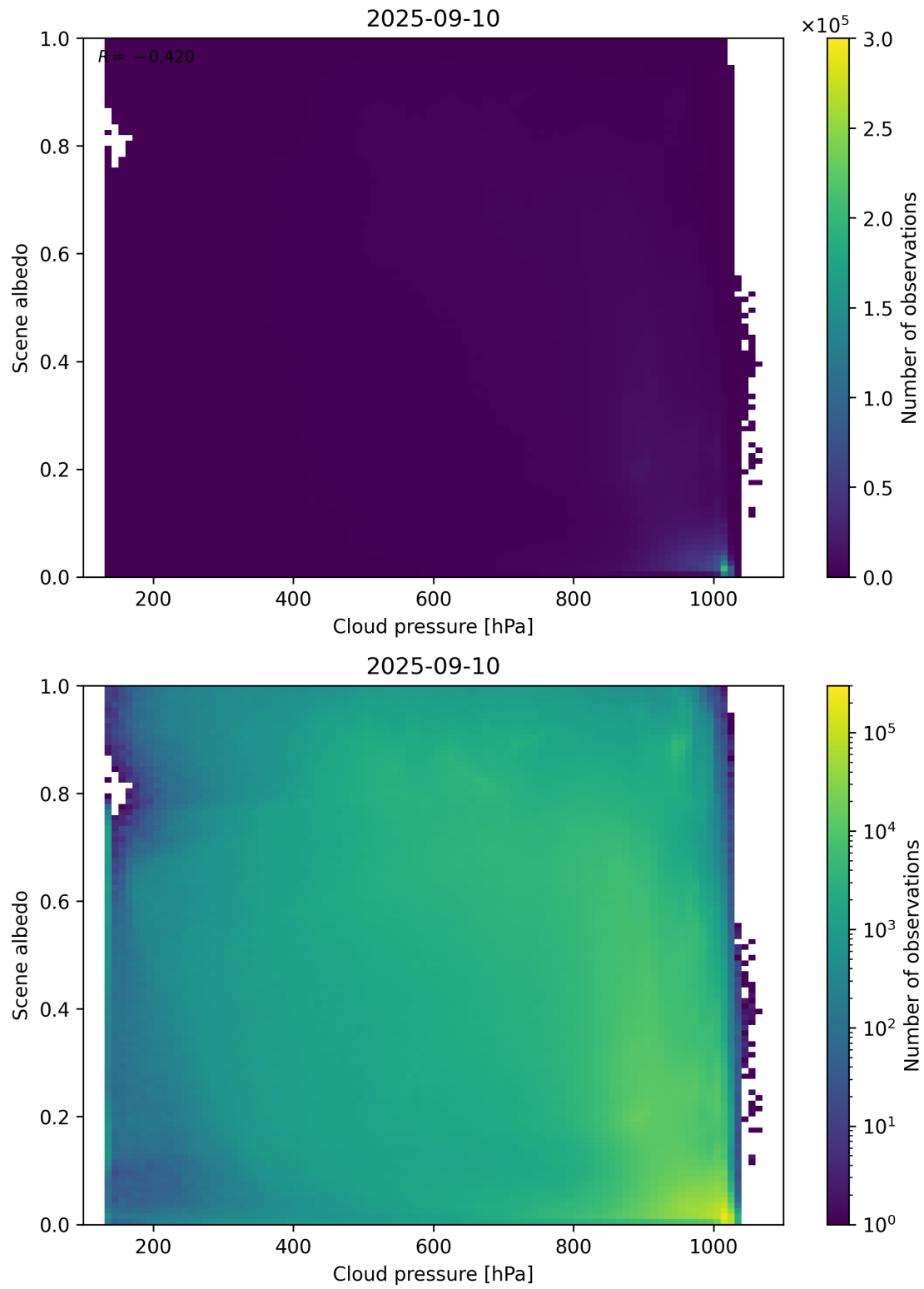
Figure 83: Scatter density plot of “Cloud pressure” against “Scene albedo” for 2025-09-10 to 2025-09-11.
