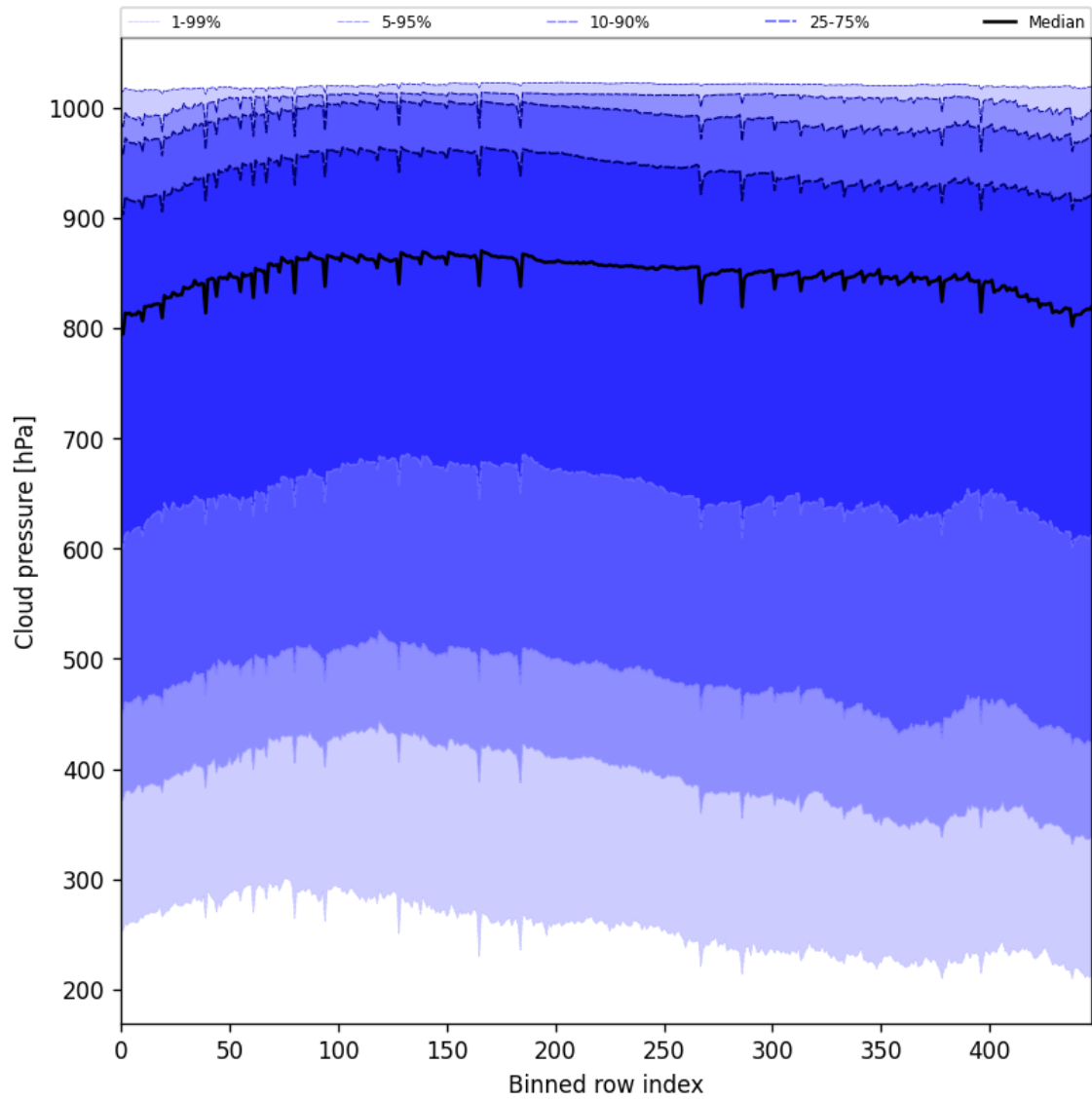
Figure 47: Along track statistics of “Cloud pressure” for 2025-09-10 to 2025-09-11
