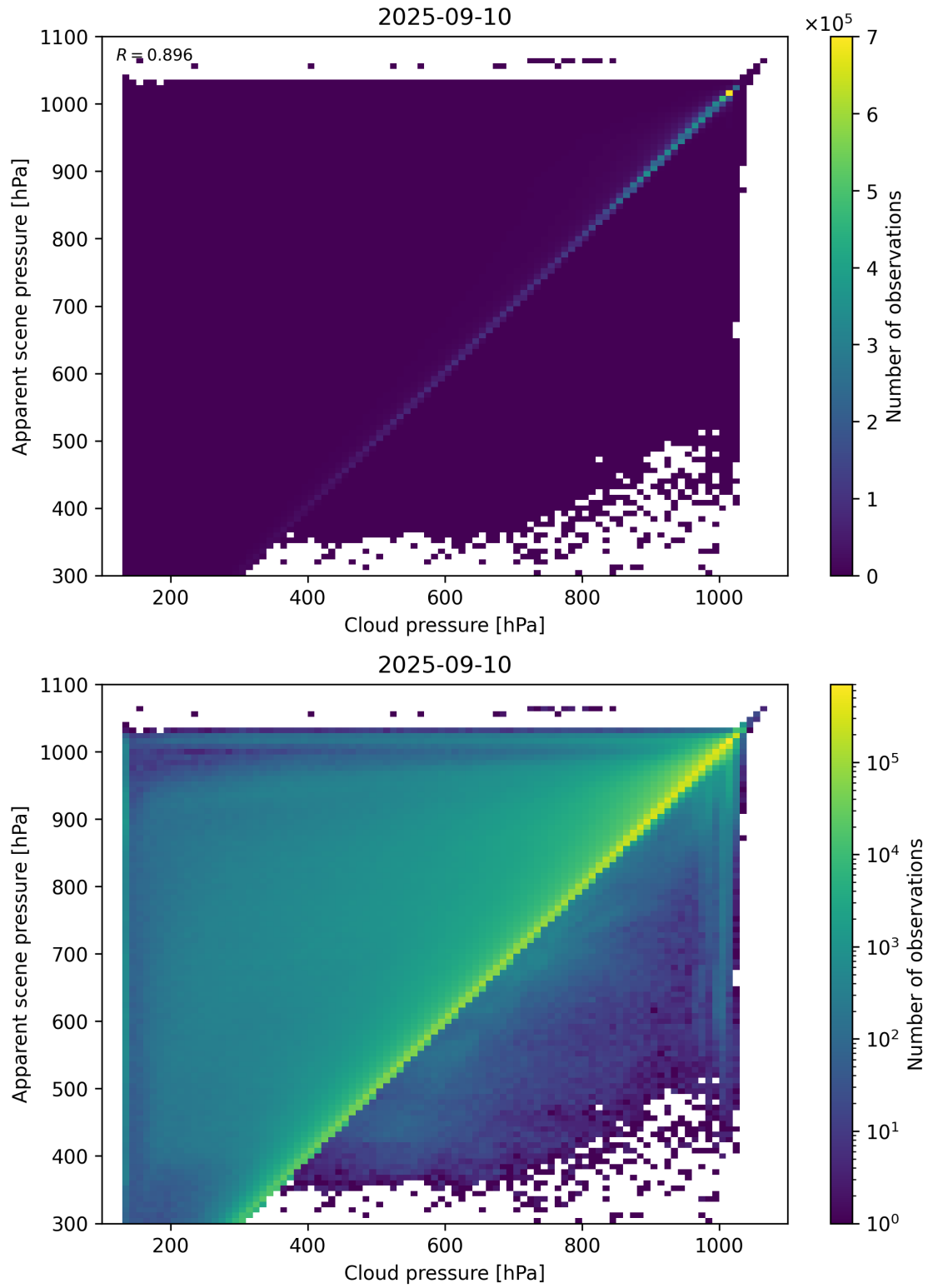
Figure 77: Scatter density plot of “Cloud pressure” against “Apparent scene pressure” for 2025-09-10 to 2025-09-11.
