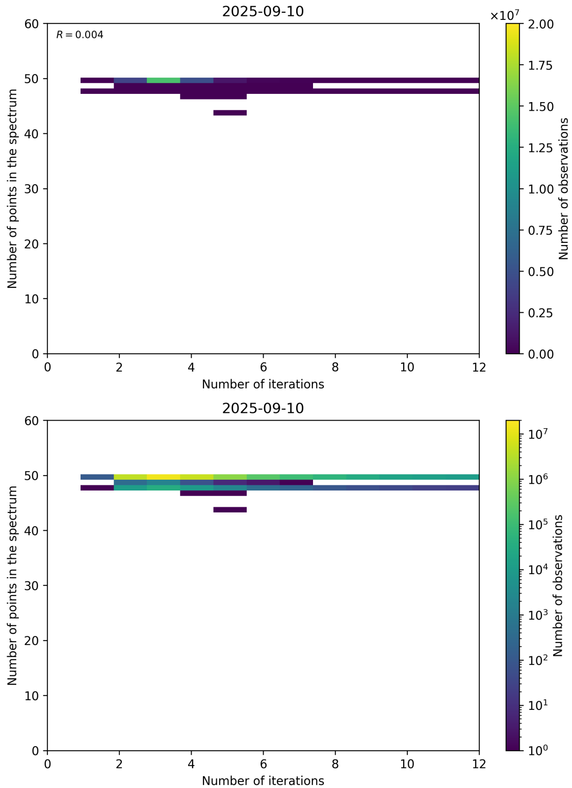
Figure 99: Scatter density plot of “Number of iterations” against “Number of points in the spectrum” for 2025-09-10 to 2025-09-11.
