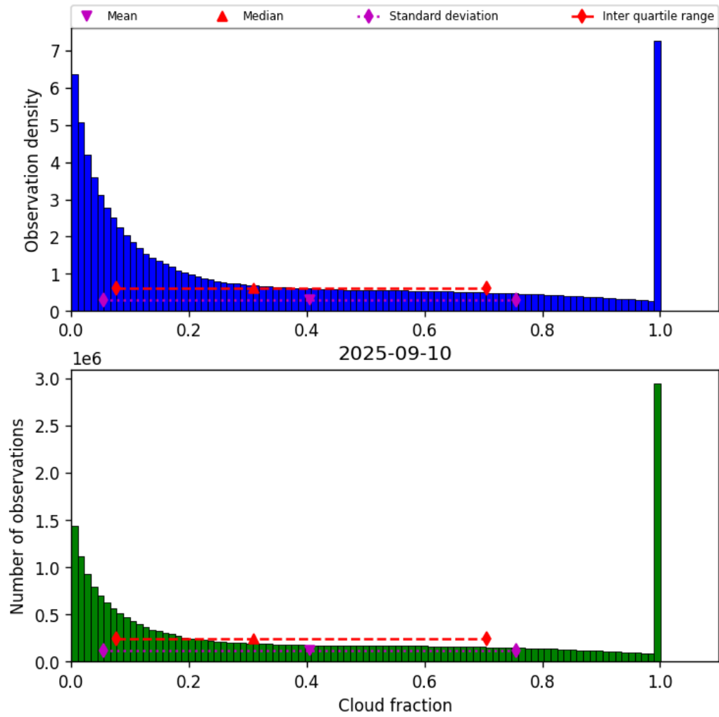
Figure 32: Histogram of “Cloud fraction” for 2025-09-10 to 2025-09-11
