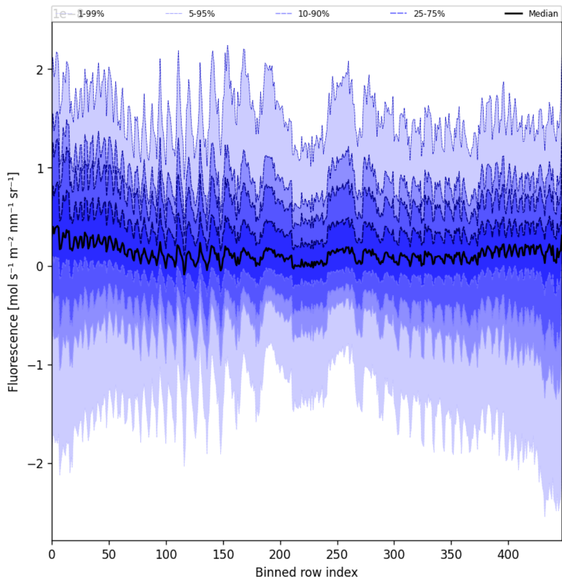
Figure 57: Along track statistics of "Fluorescence" for 2025-09-10 to 2025-09-11
