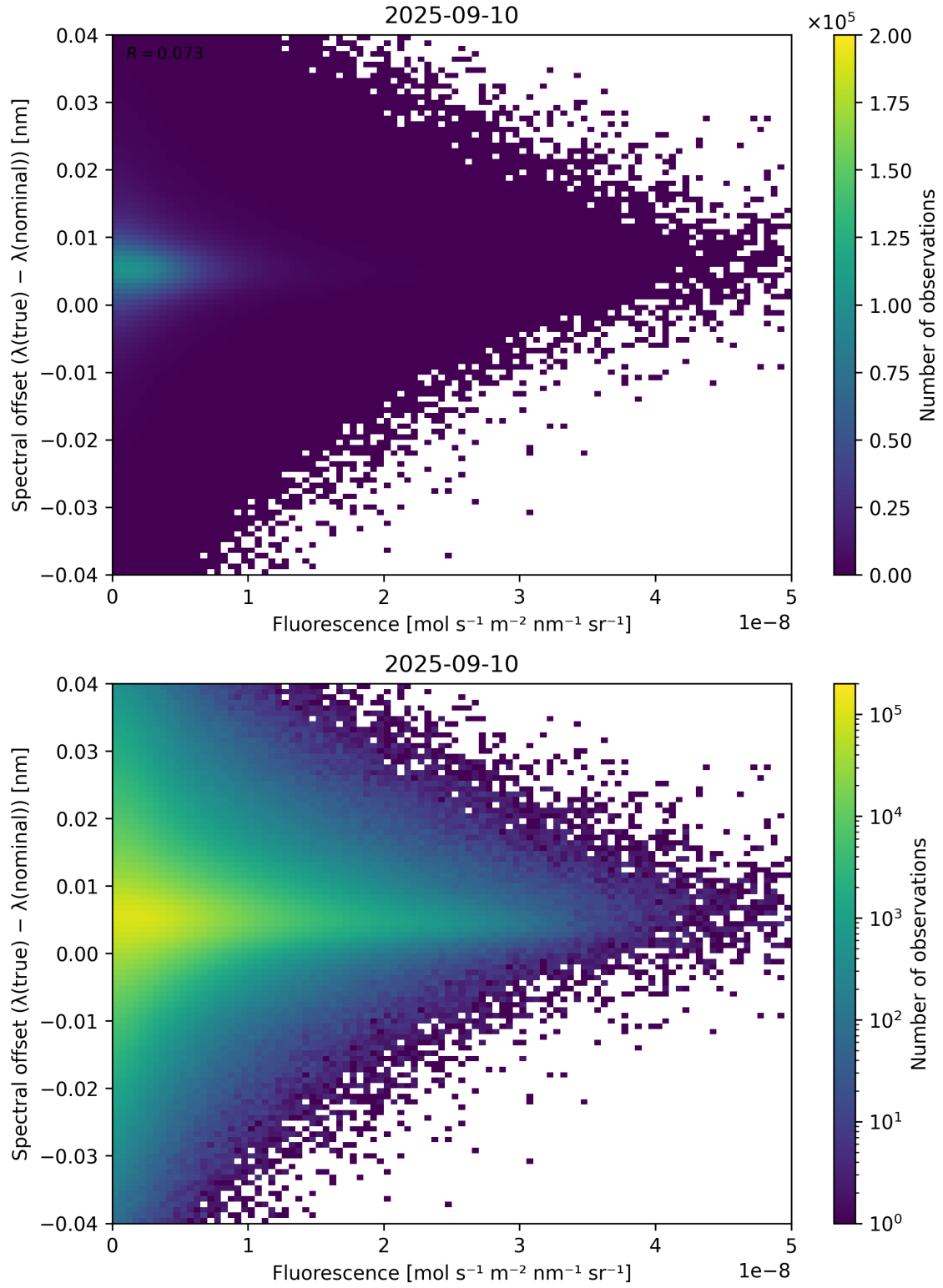
Figure 87: Scatter density plot of “Fluorescence” against “Spectral offset ( \lambda_{\text{true}} - \lambda_{\text{nominal}} )” for 2025-09-10 to 2025-09-11.
