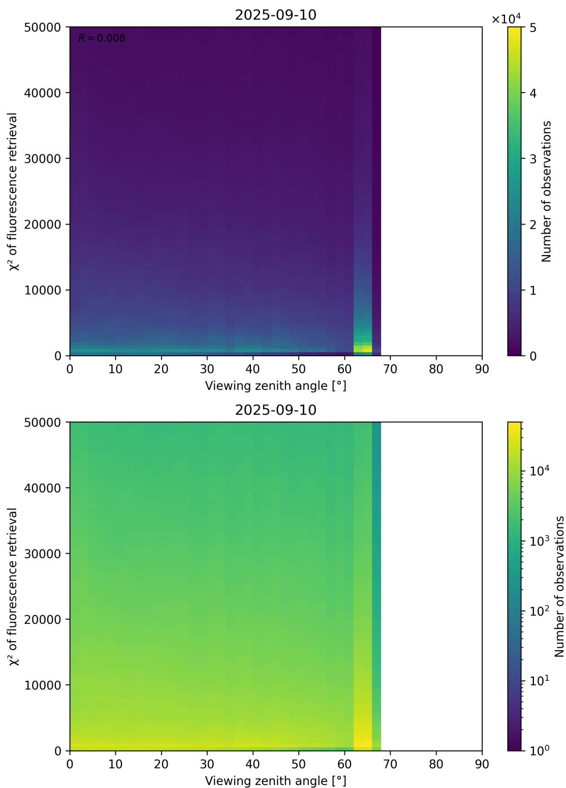
Figure 119: Scatter density plot of “Viewing zenith angle” against “ \chi^2 of fluorescence retrieval” for 2025-09-10 to 2025-09-11.
