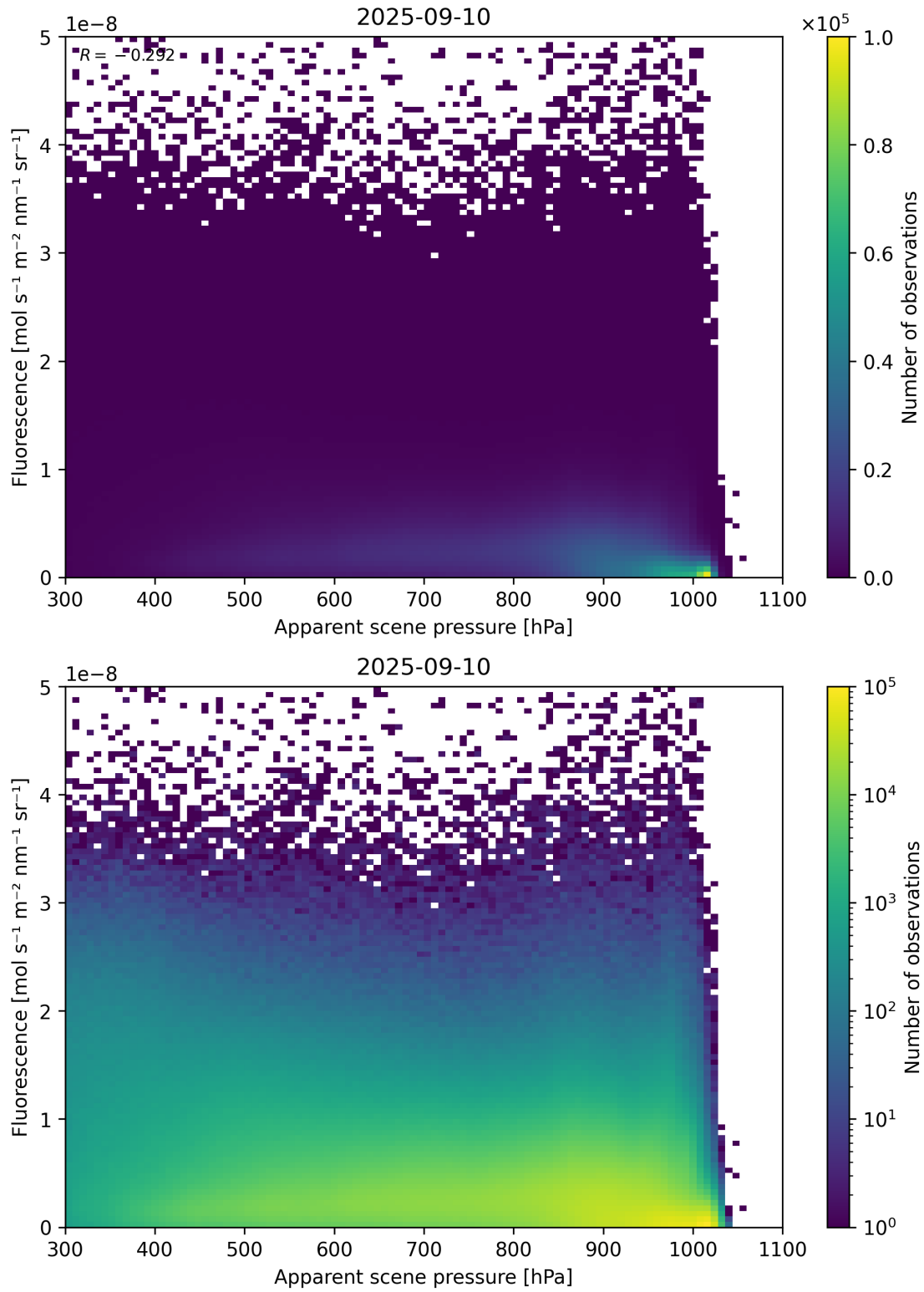
Figure 64: Scatter density plot of “Apparent scene pressure” against “Fluorescence” for 2025-09-10 to 2025-09-11.
