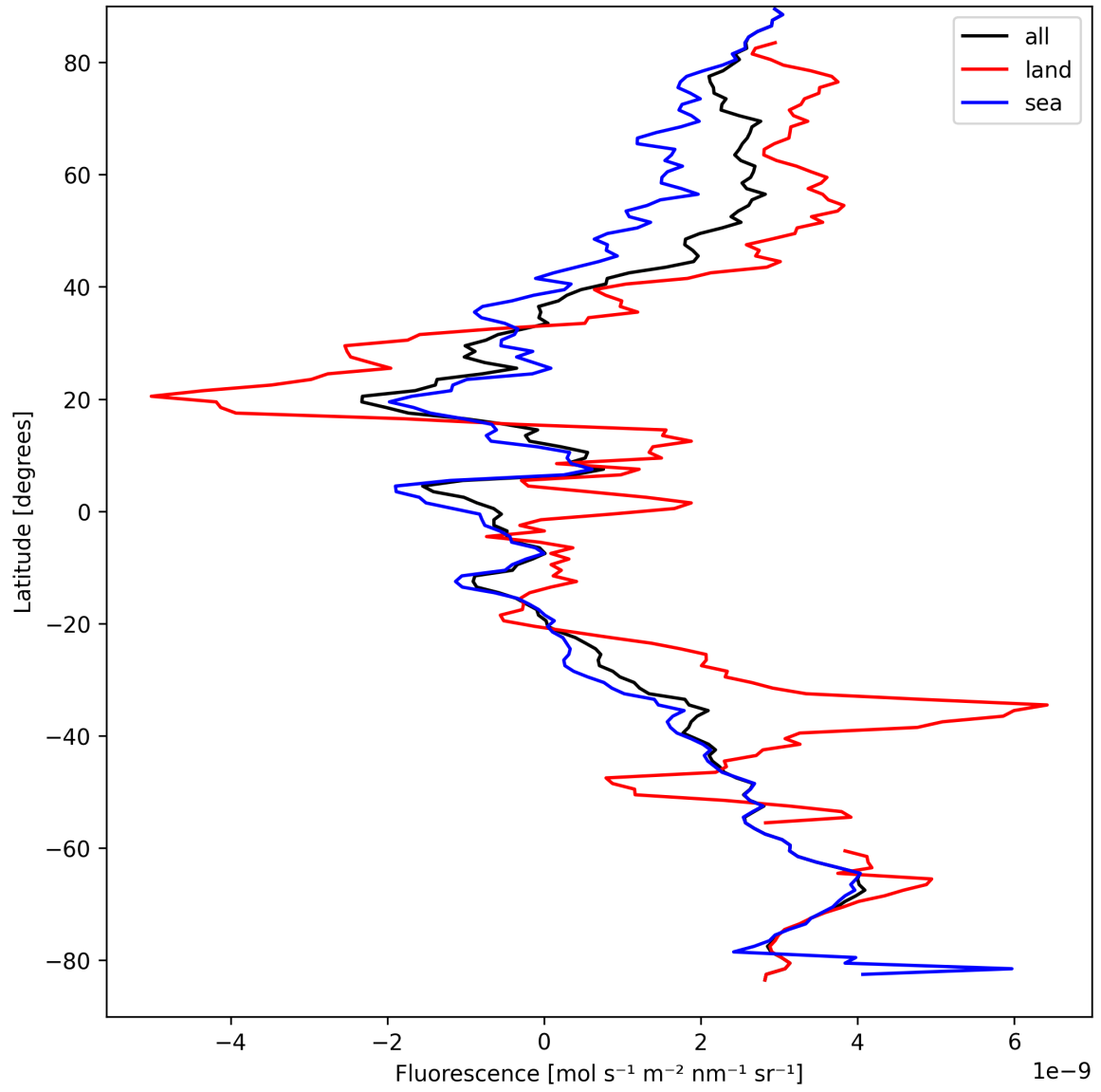
Figure 23: Zonal average of “Fluorescence” for 2025-09-10 to 2025-09-11.
