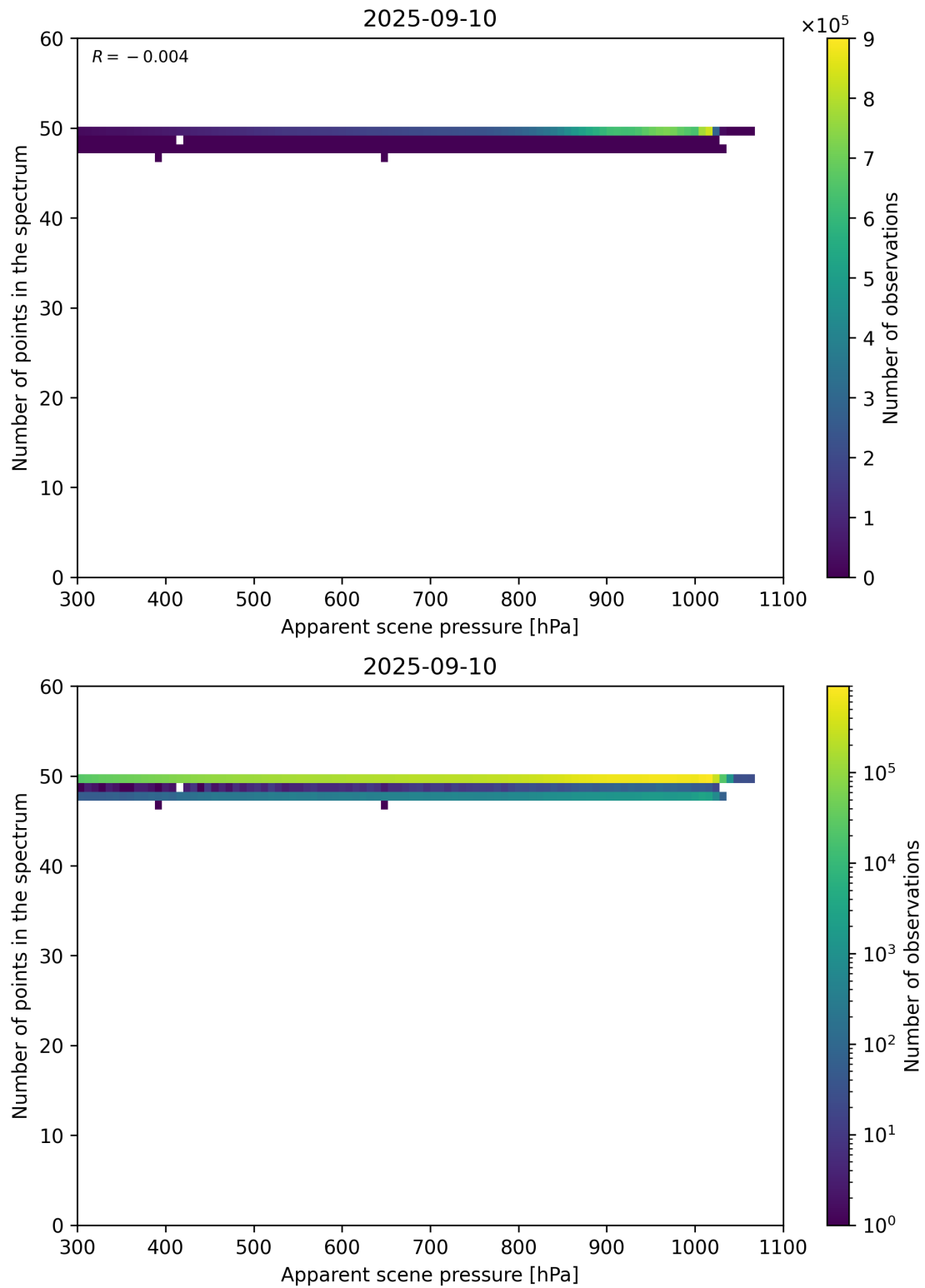
Figure 66: Scatter density plot of “Apparent scene pressure” against “Number of points in the spectrum” for 2025-09-10 to 2025-09-11.
