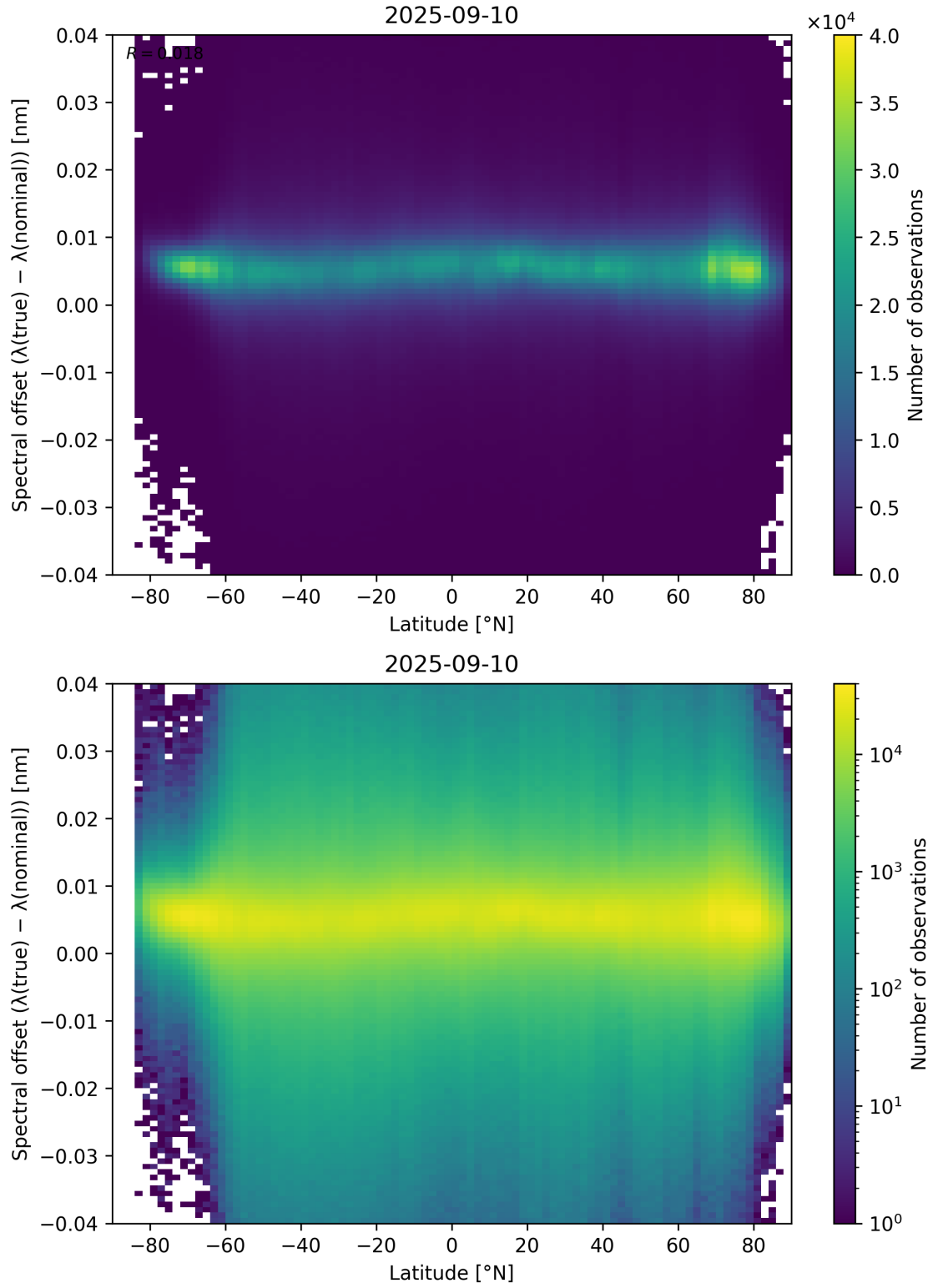
Figure 96: Scatter density plot of “Latitude” against “Spectral offset ( \lambda_{\text{true}} - \lambda_{\text{nominal}} )” for 2025-09-10 to 2025-09-11.
