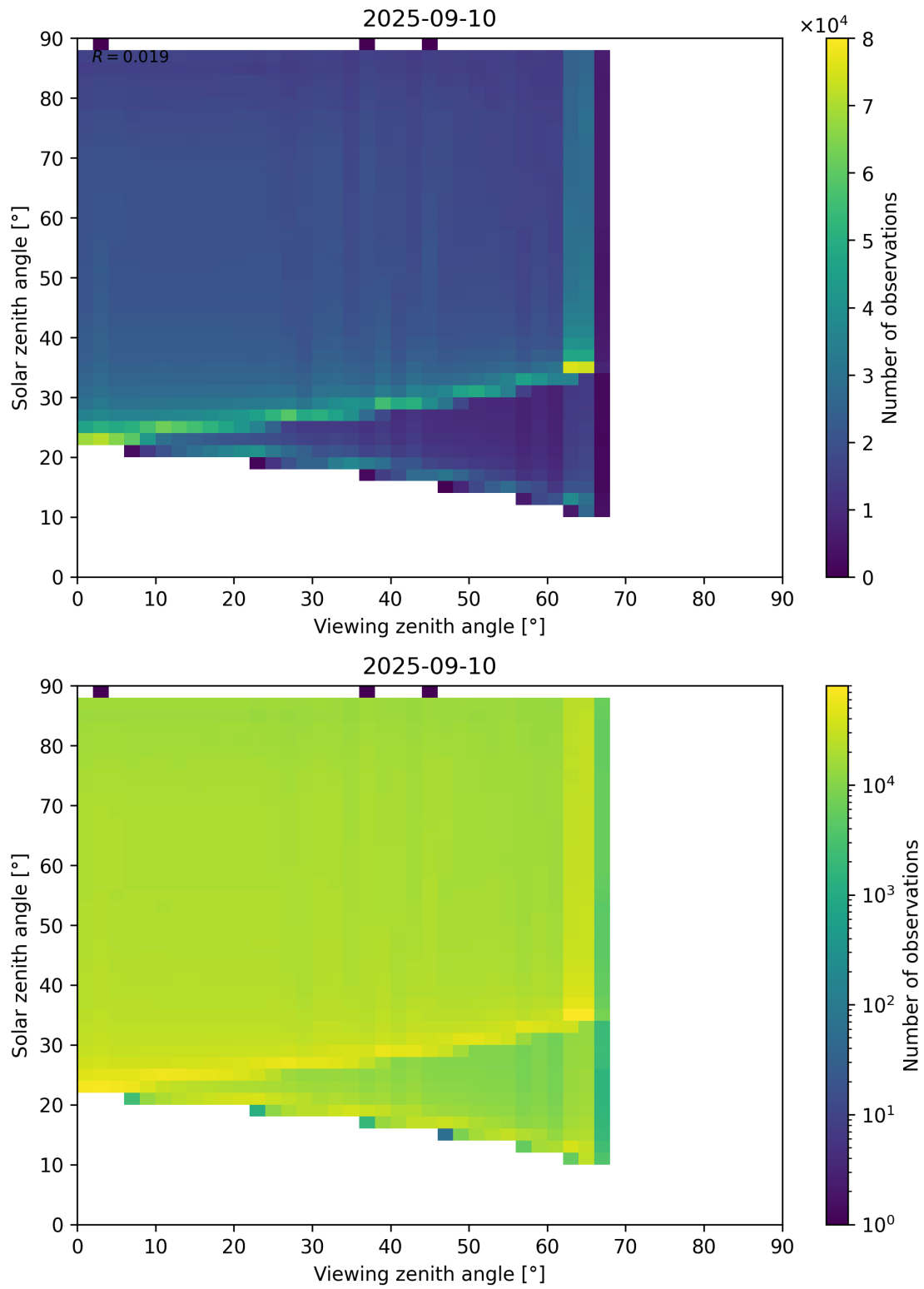
Figure 127: Scatter density plot of “Viewing zenith angle” against “Solar zenith angle” for 2025-09-10 to 2025-09-11.
