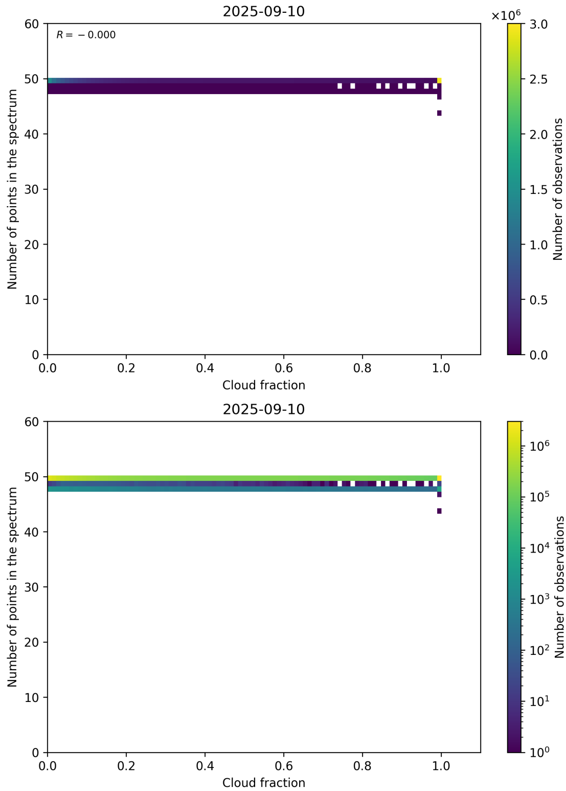
Figure 74: Scatter density plot of “Cloud fraction” against “Number of points in the spectrum” for 2025-09-10 to 2025-09-11.
