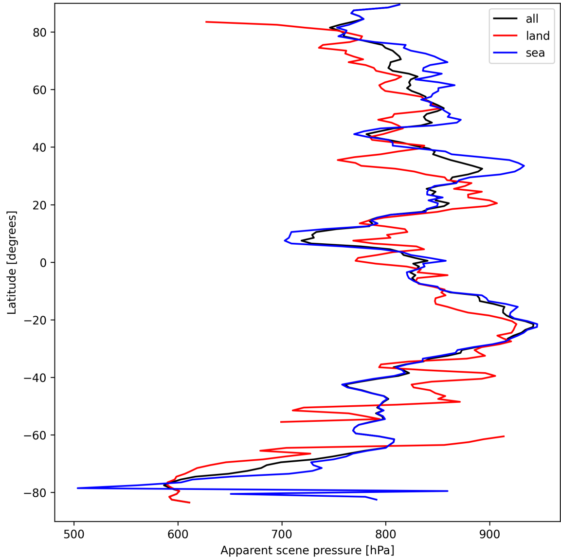
Figure 19: Zonal average of “Apparent scene pressure” for 2025-09-10 to 2025-09-11.
