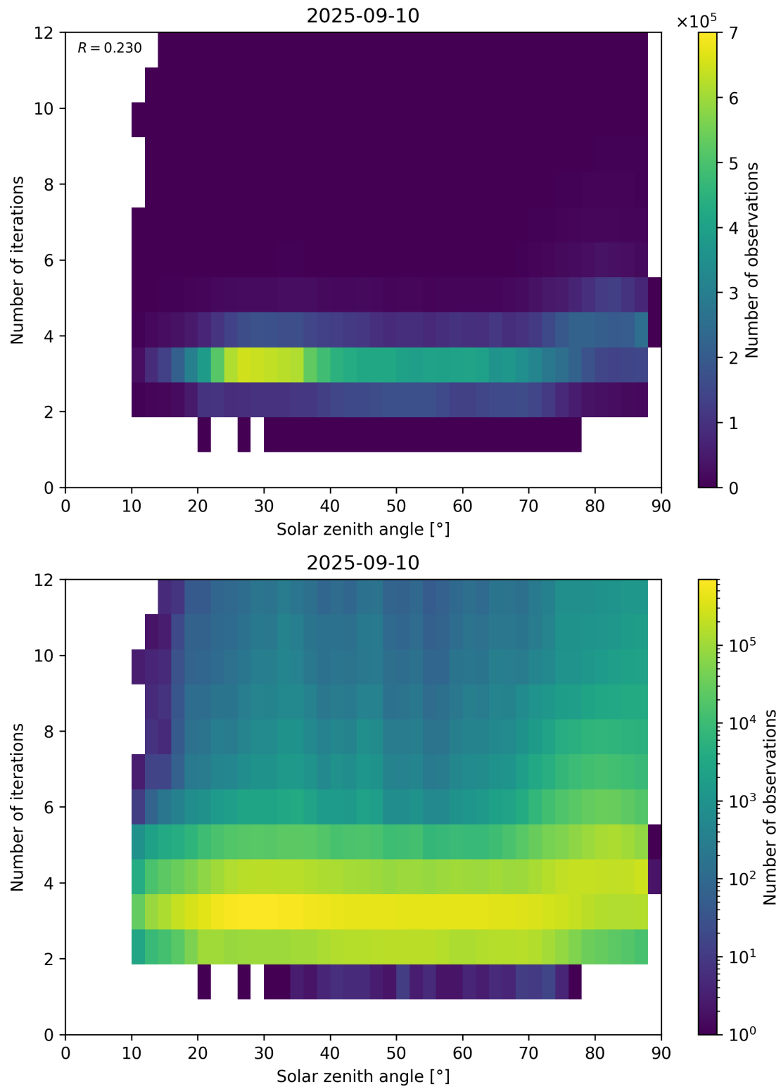
Figure 114: Scatter density plot of “Solar zenith angle” against “Number of iterations” for 2025-09-10 to 2025-09-11.
