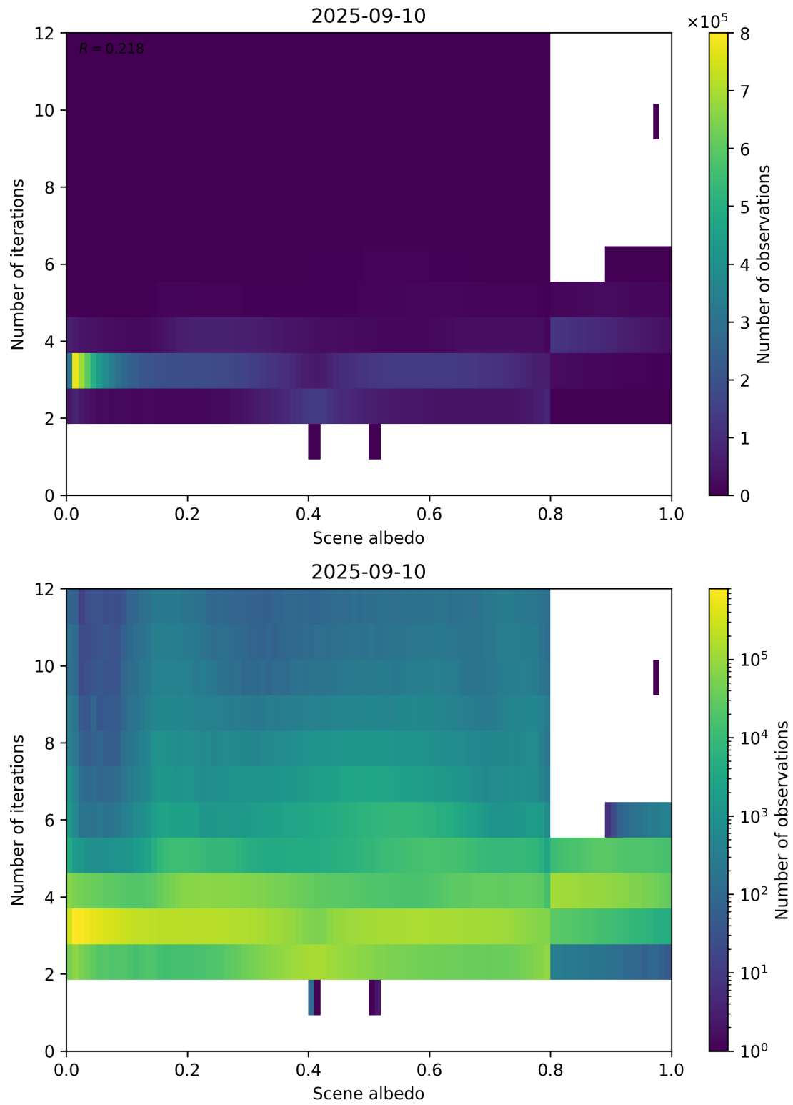
Figure 105: Scatter density plot of “Scene albedo” against “Number of iterations” for 2025-09-10 to 2025-09-11.
