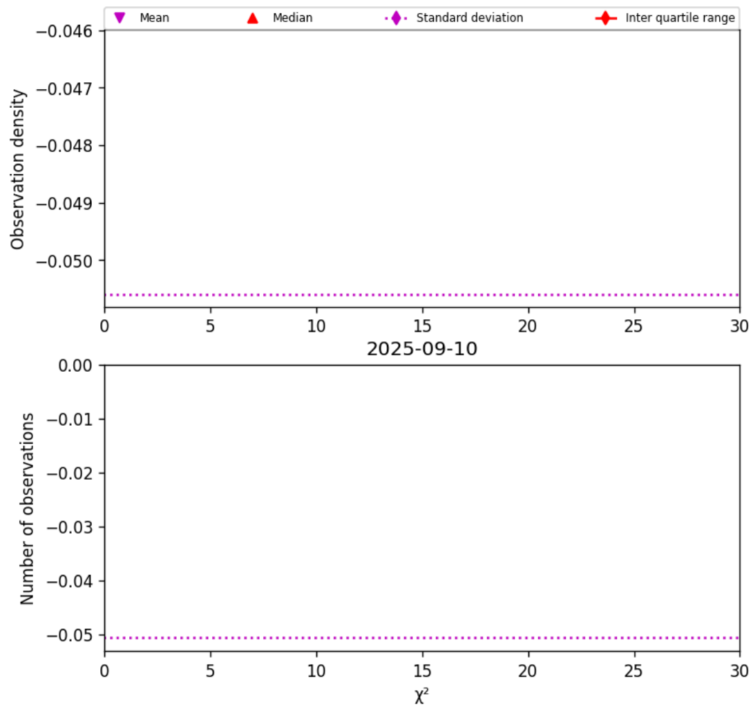
Figure 38: Histogram of " \chi^2 " for 2025-09-10 to 2025-09-11
