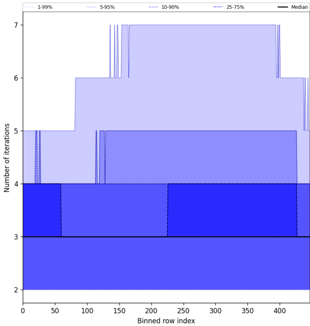
Figure 56: Along track statistics of “Number of iterations” for 2025-09-10 to 2025-09-11
