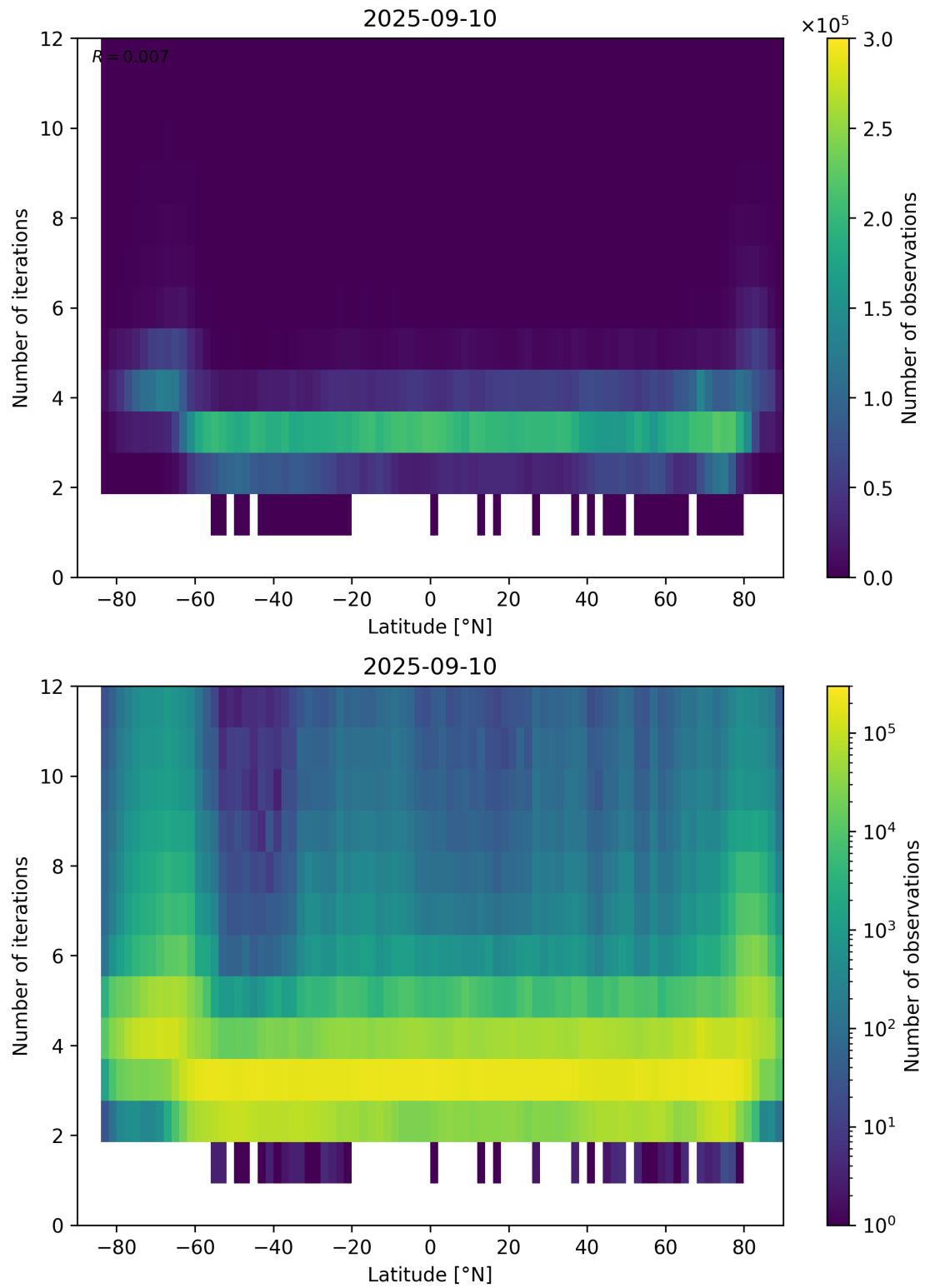
Figure 93: Scatter density plot of “Latitude” against “Number of iterations” for 2025-09-10 to 2025-09-11.
