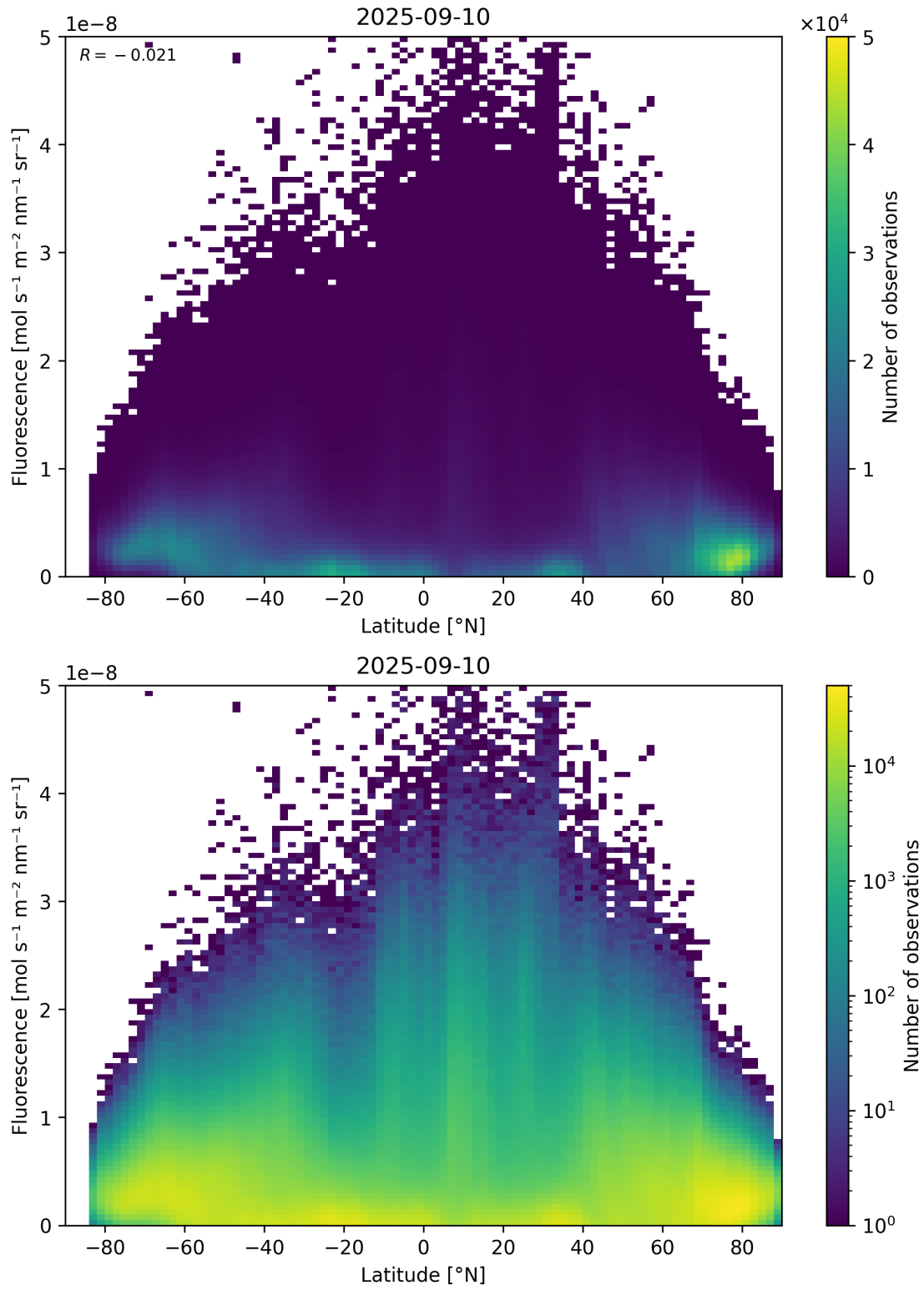
Figure 92: Scatter density plot of “Latitude” against “Fluorescence” for 2025-09-10 to 2025-09-11.
