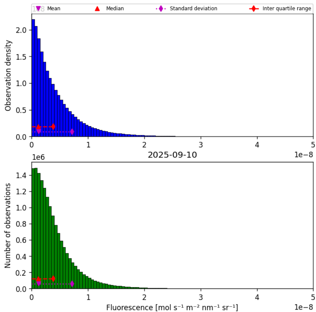
Figure 40: Histogram of “Fluorescence” for 2025-09-10 to 2025-09-11
