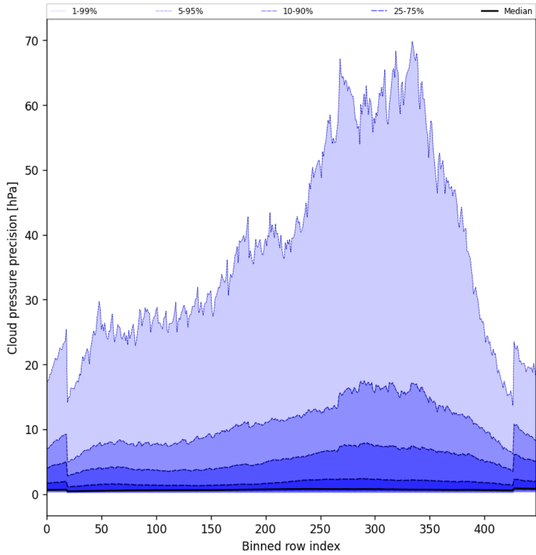
Figure 48: Along track statistics of “Cloud pressure precision” for 2025-09-10 to 2025-09-11
