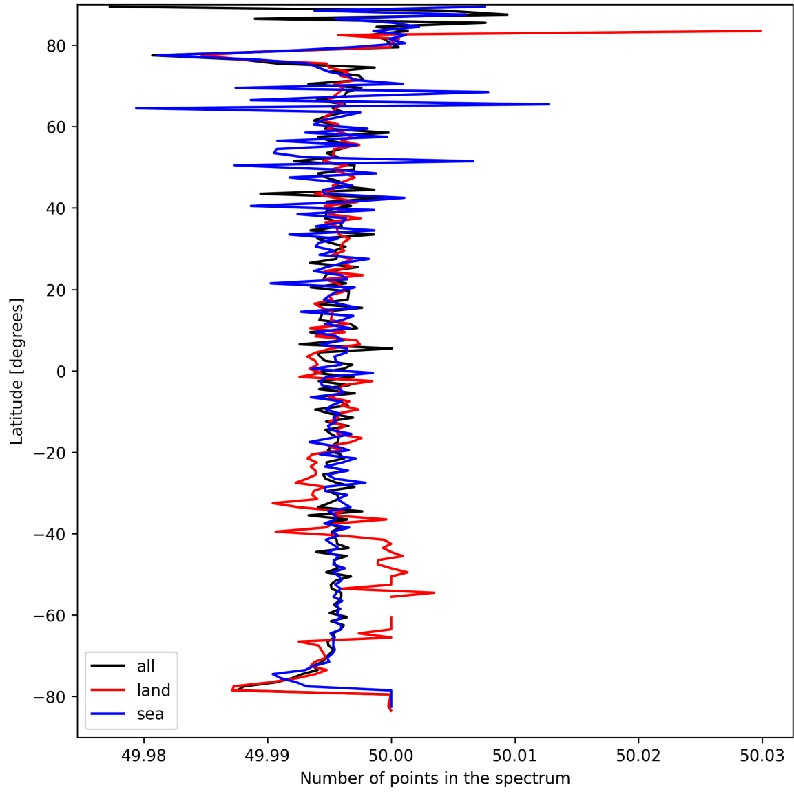
Figure 27: Zonal average of “Number of points in the spectrum” for 2025-09-10 to 2025-09-11.
