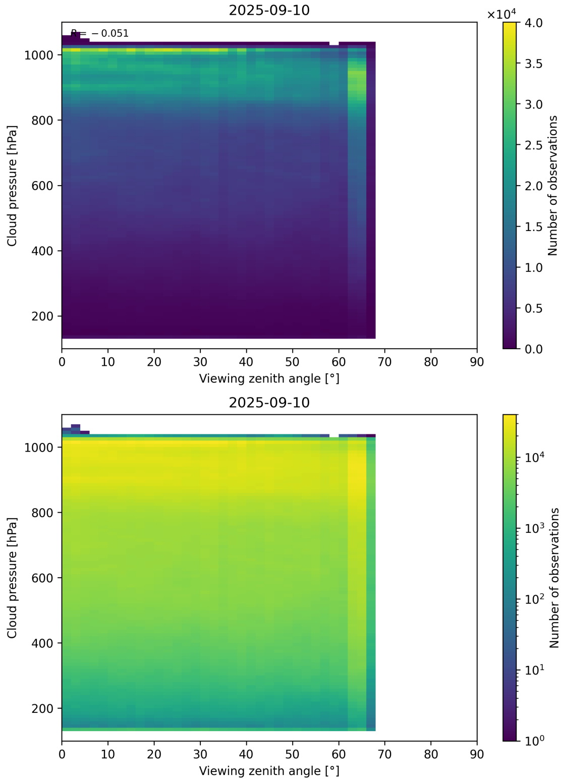
Figure 121: Scatter density plot of “Viewing zenith angle” against “Cloud pressure” for 2025-09-10 to 2025-09-11.
