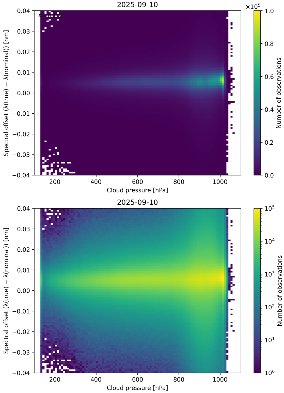
Figure 84: Scatter density plot of “Cloud pressure” against “Spectral offset ( \lambda_{\text{true}} - \lambda_{\text{nominal}} )” for 2025-09-10 to 2025-09-11.
