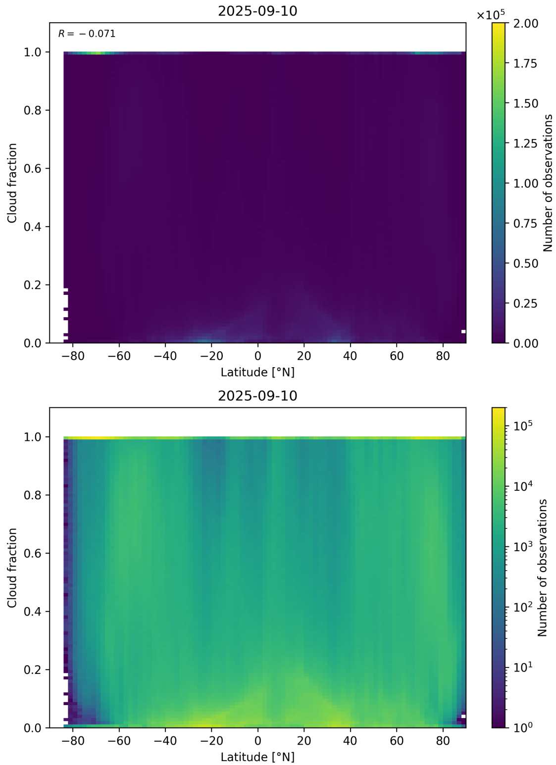
Figure 90: Scatter density plot of “Latitude” against “Cloud fraction” for 2025-09-10 to 2025-09-11.
