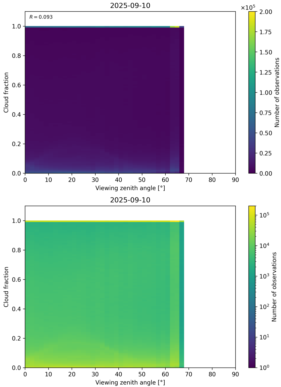
Figure 120: Scatter density plot of “Viewing zenith angle” against “Cloud fraction” for 2025-09-10 to 2025-09-11.
