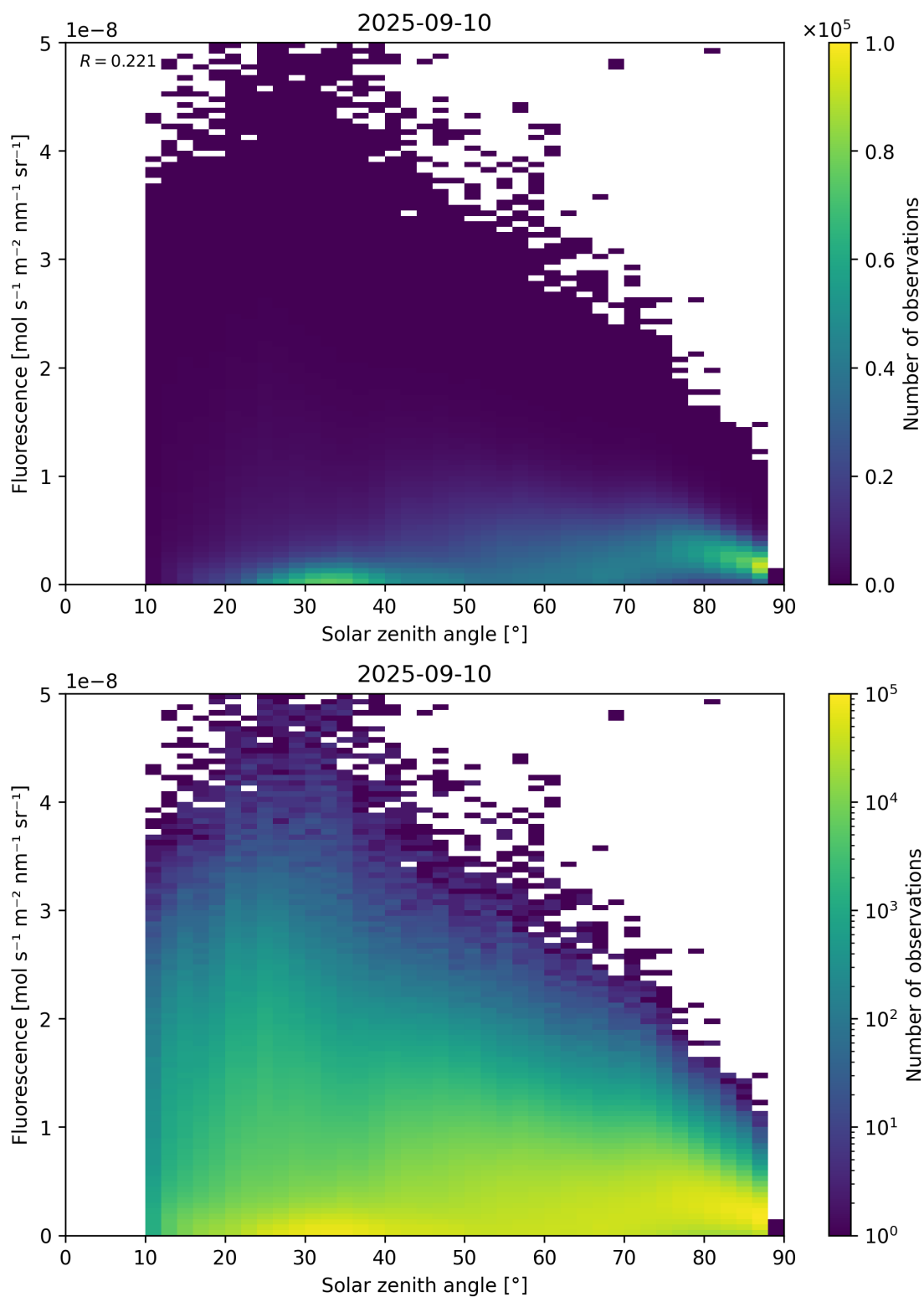
Figure 112: Scatter density plot of “Solar zenith angle” against “Fluorescence” for 2025-09-10 to 2025-09-11.
