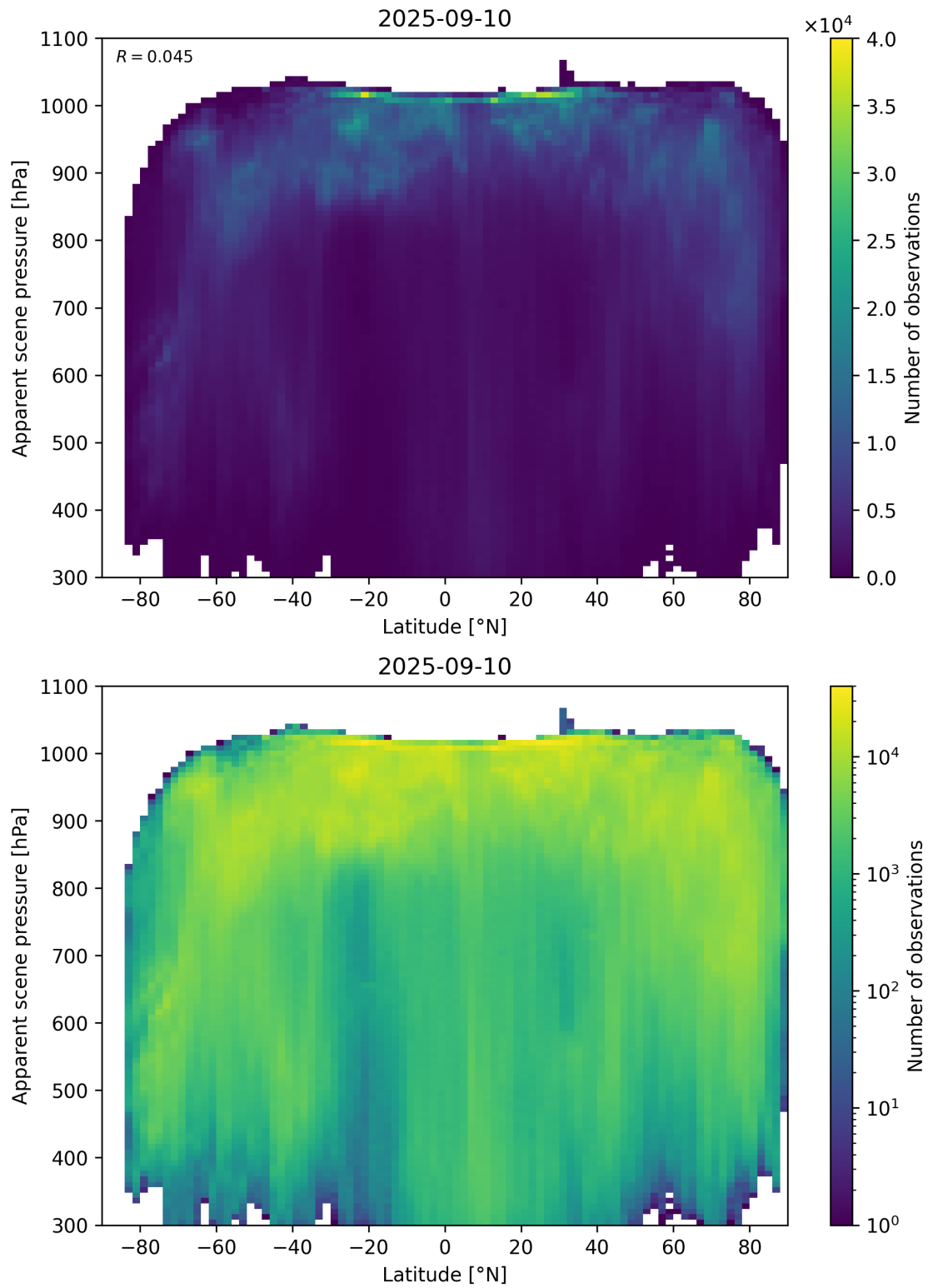
Figure 88: Scatter density plot of “Latitude” against “Apparent scene pressure” for 2025-09-10 to 2025-09-11.
