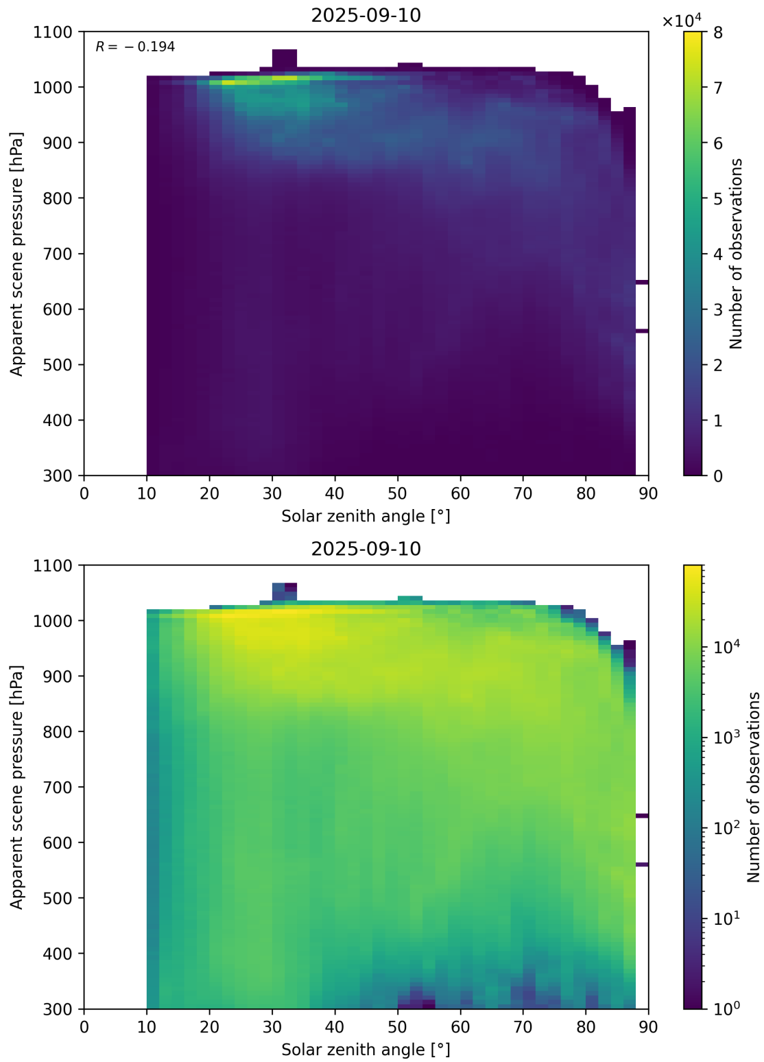
Figure 108: Scatter density plot of “Solar zenith angle” against “Apparent scene pressure” for 2025-09-10 to 2025-09-11.
