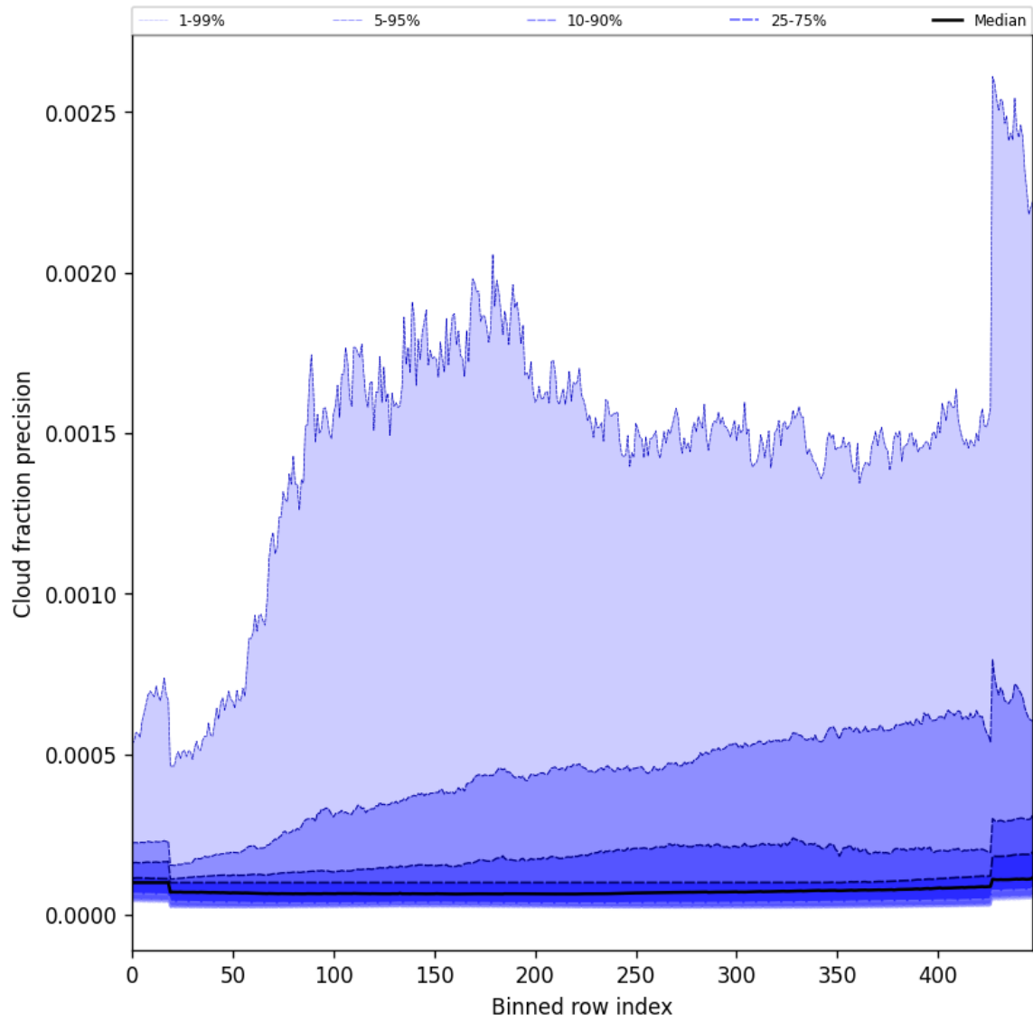
Figure 50: Along track statistics of “Cloud fraction precision” for 2025-09-10 to 2025-09-11
