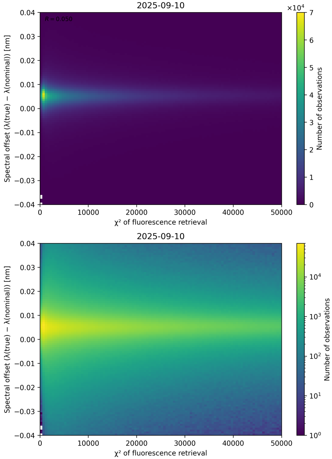
Figure 69: Scatter density plot of “ \chi^2 of fluorescence retrieval” against “Spectral offset ( \lambda_{\text{true}} - \lambda_{\text{nominal}} )” for 2025-09-10 to 2025-09-11.
