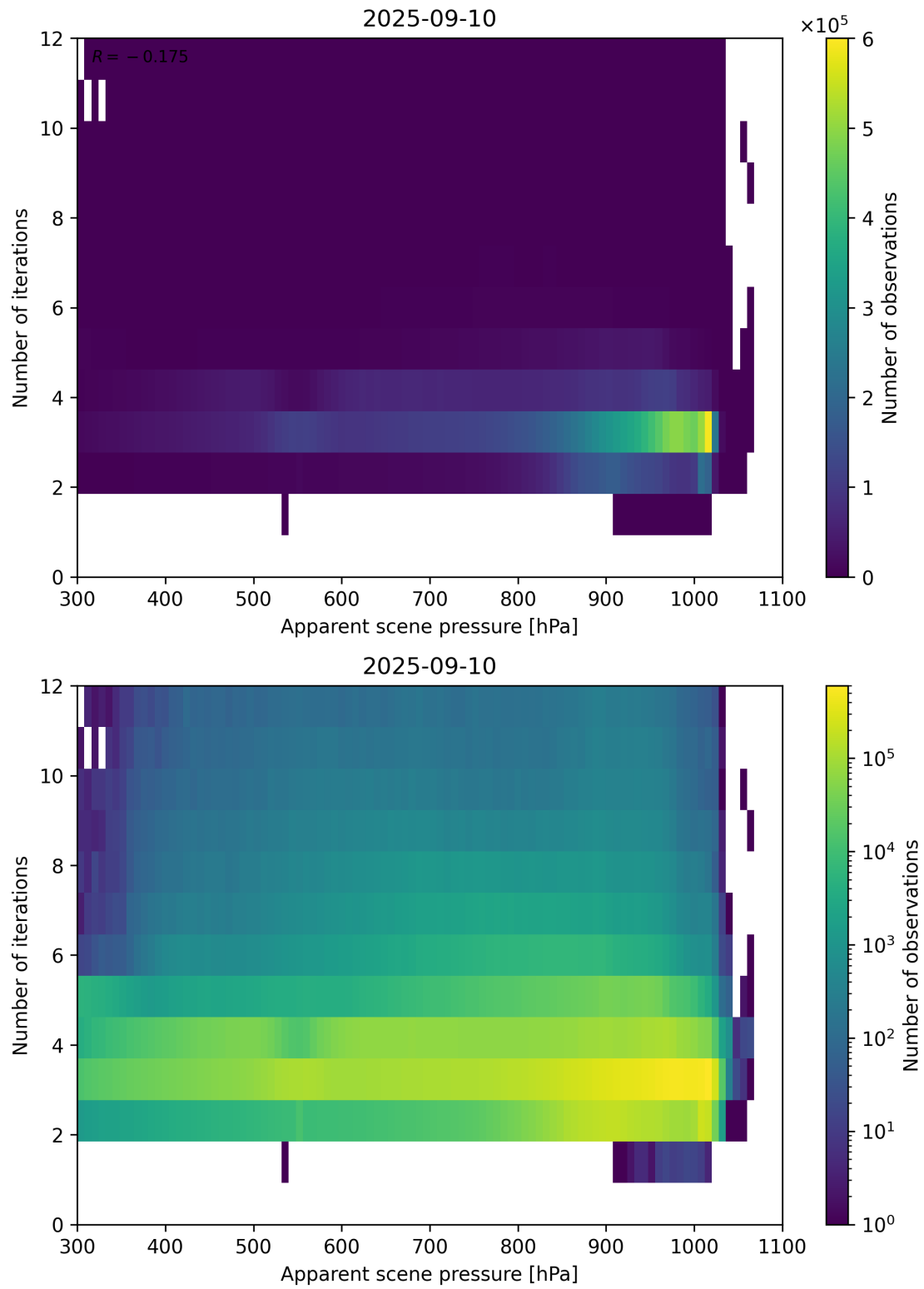
Figure 65: Scatter density plot of “Apparent scene pressure” against “Number of iterations” for 2025-09-10 to 2025-09-11.
