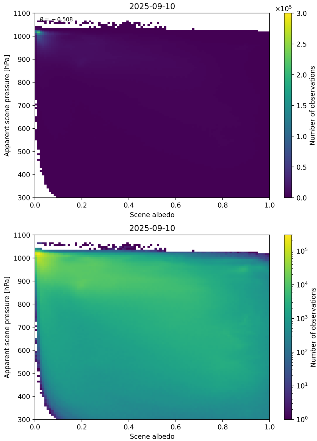
Figure 102: Scatter density plot of “Scene albedo” against “Apparent scene pressure” for 2025-09-10 to 2025-09-11.
