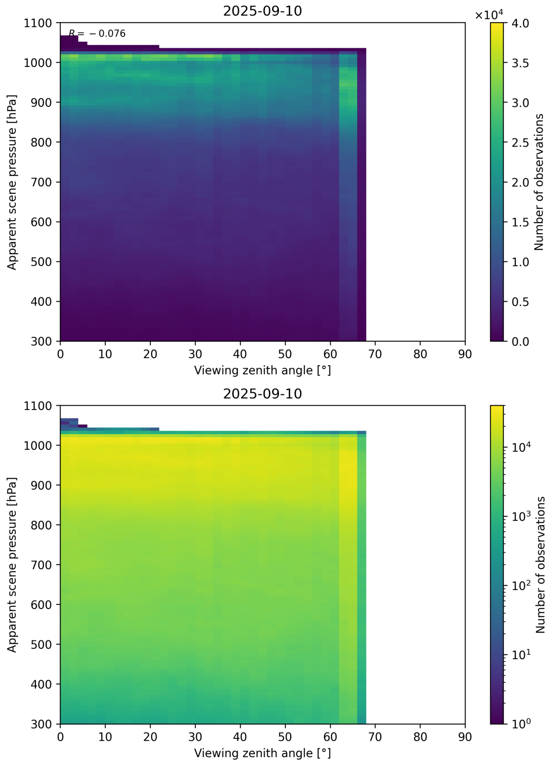
Figure 118: Scatter density plot of “Viewing zenith angle” against “Apparent scene pressure” for 2025-09-10 to 2025-09-11.
