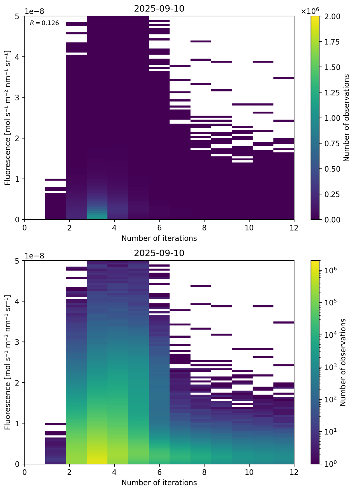
Figure 98: Scatter density plot of “Number of iterations” against “Fluorescence” for 2025-09-10 to 2025-09-11.
