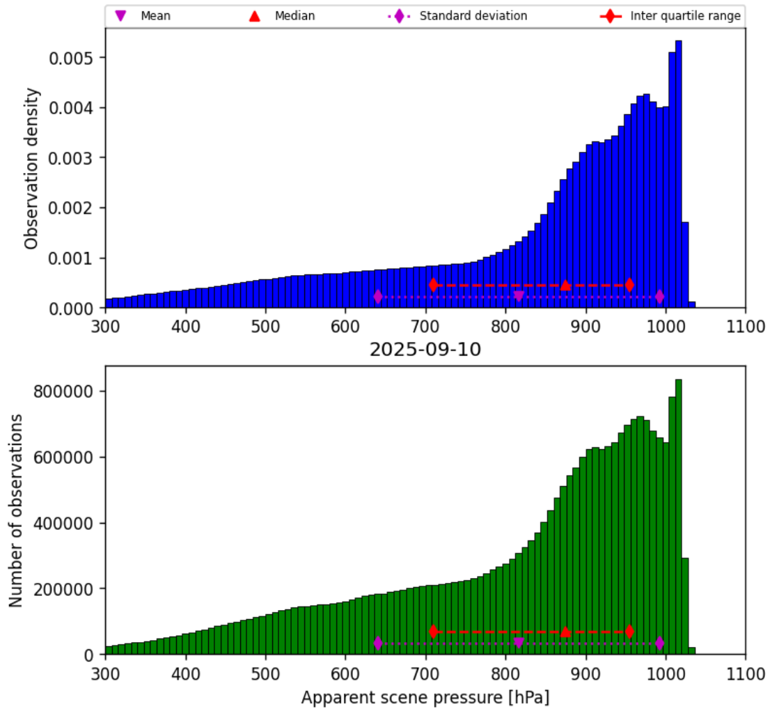
Figure 36: Histogram of “Apparent scene pressure” for 2025-09-10 to 2025-09-11
