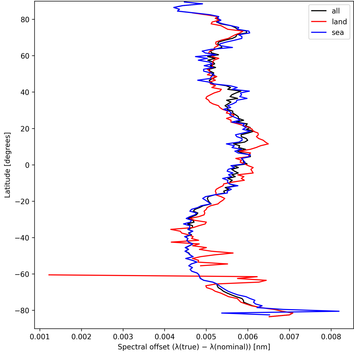
Figure 28: Zonal average of “Spectral offset ( \lambda_{\text{true}} - \lambda_{\text{nominal}} )” for 2025-09-10 to 2025-09-11.
