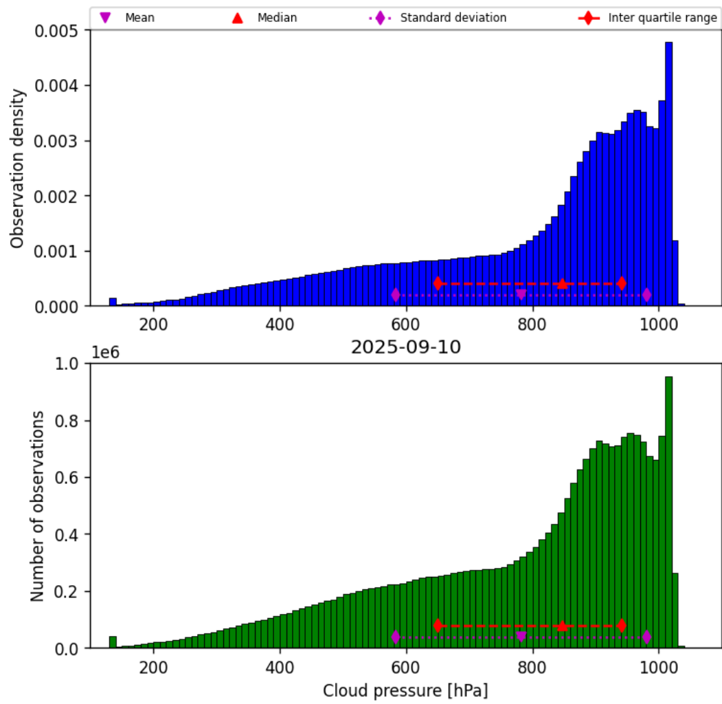
Figure 30: Histogram of “Cloud pressure” for 2025-09-10 to 2025-09-11
