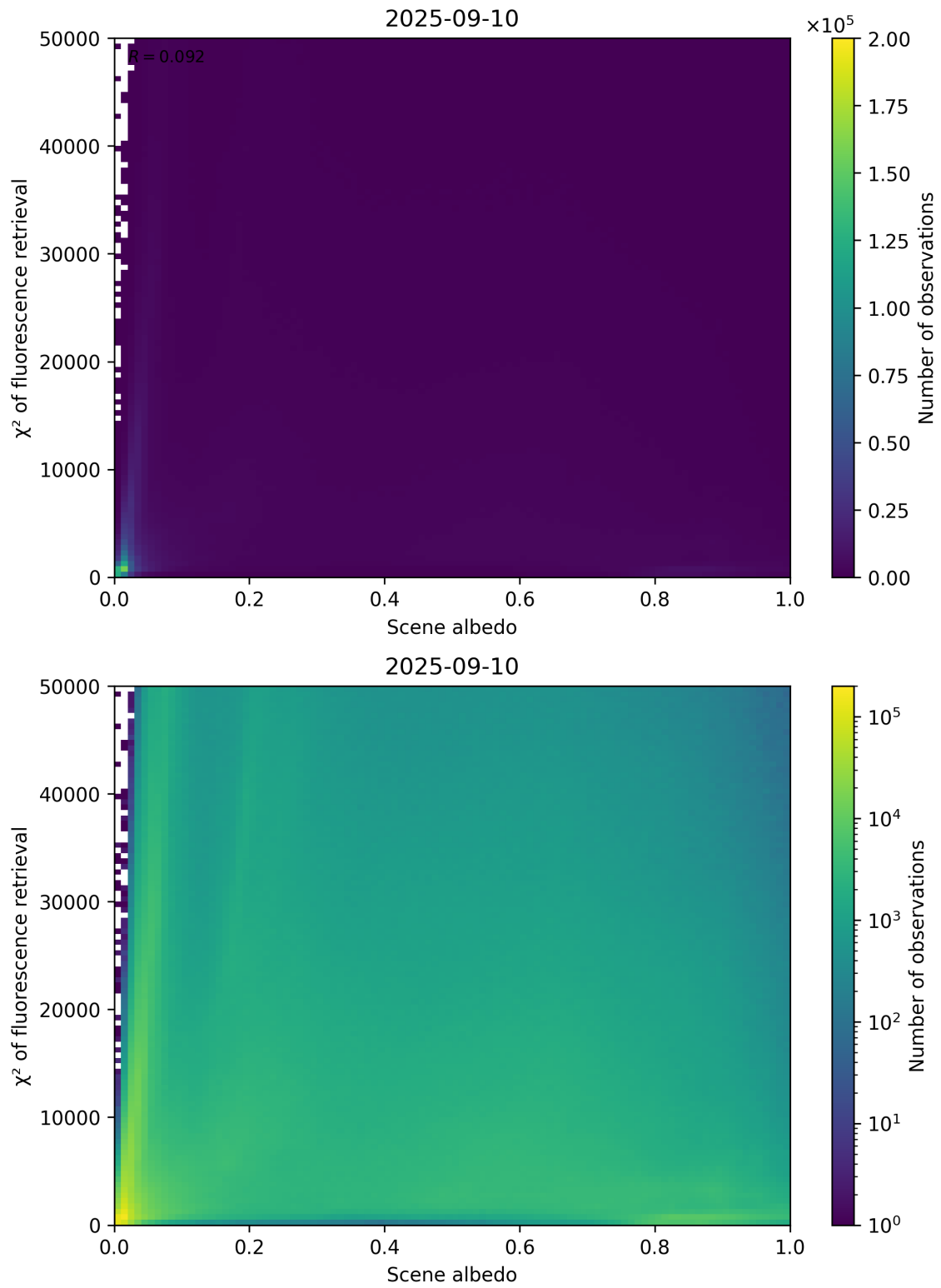
Figure 103: Scatter density plot of “Scene albedo” against “ \chi^2 of fluorescence retrieval” for 2025-09-10 to 2025-09-11.
