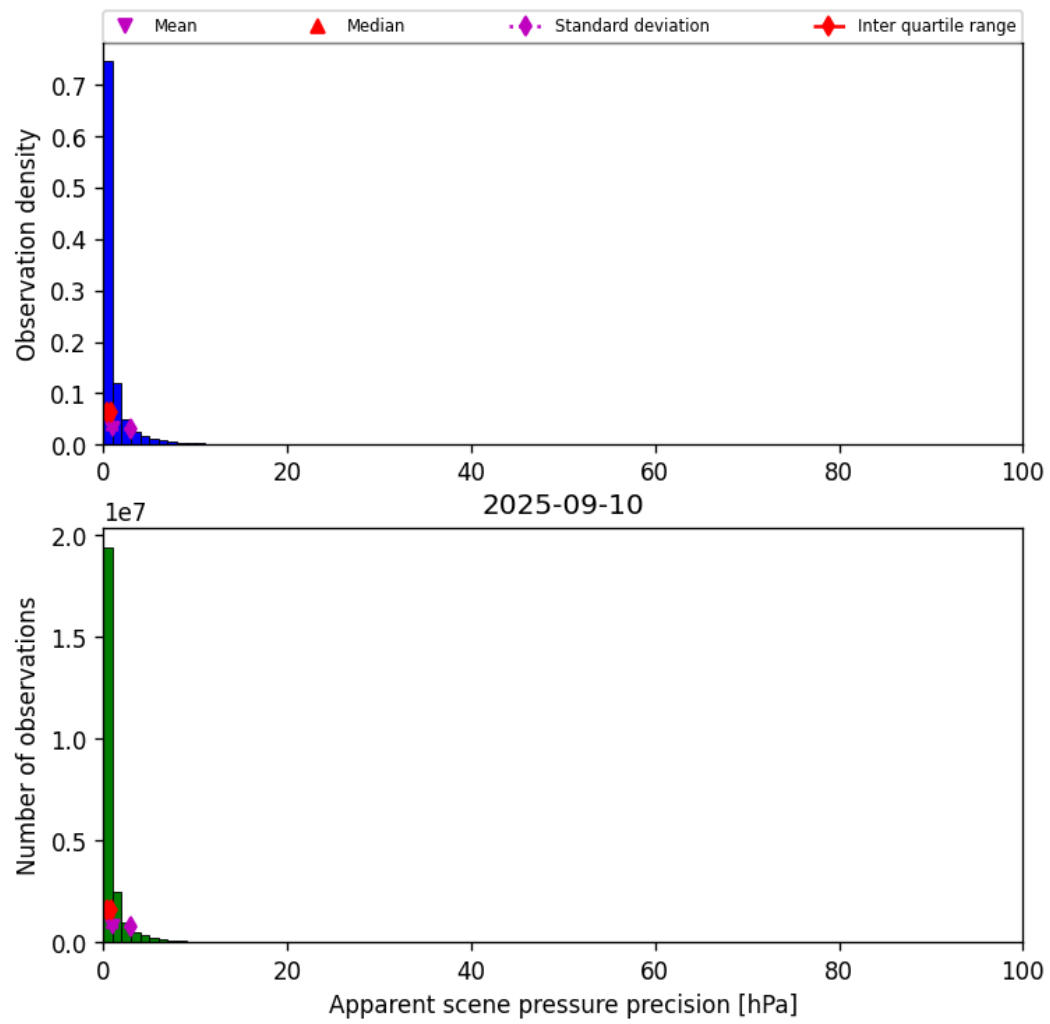
Figure 37: Histogram of “Apparent scene pressure precision” for 2025-09-10 to 2025-09-11
