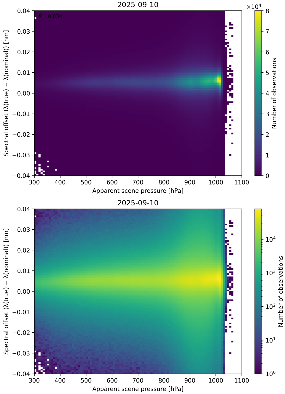
Figure 67: Scatter density plot of “Apparent scene pressure” against “Spectral offset ( \lambda_{\text{true}} - \lambda_{\text{nominal}} )” for 2025-09-10 to 2025-09-11.
