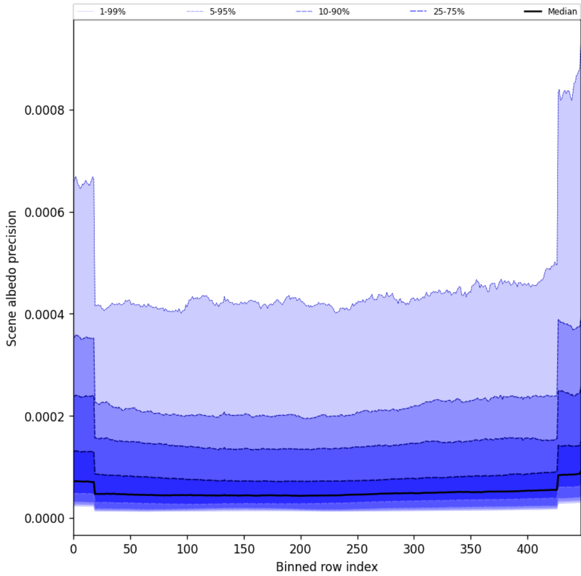
Figure 52: Along track statistics of “Scene albedo precision” for 2025-09-10 to 2025-09-11
