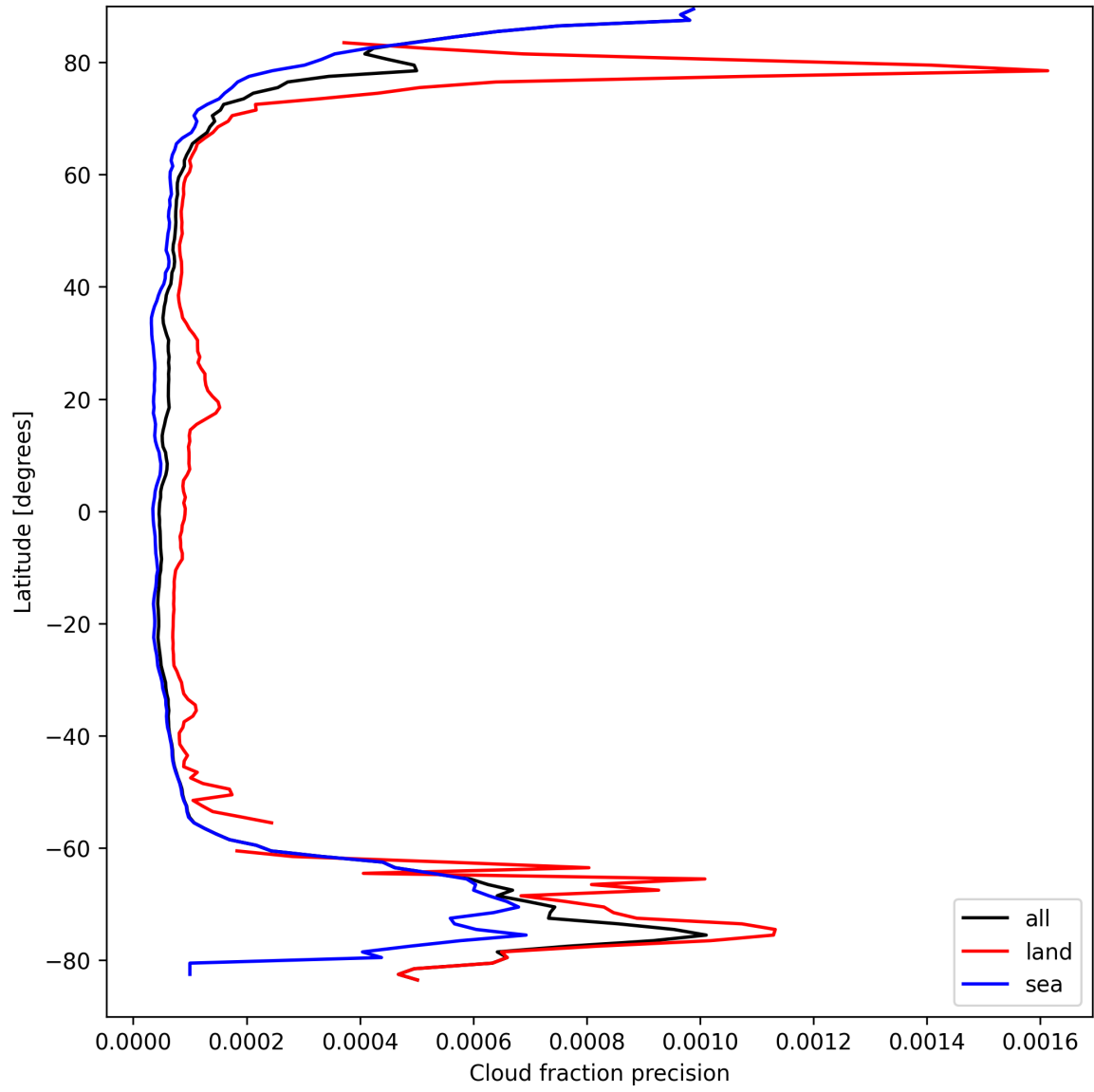
Figure 16: Zonal average of “Cloud fraction precision” for 2025-09-10 to 2025-09-11.
