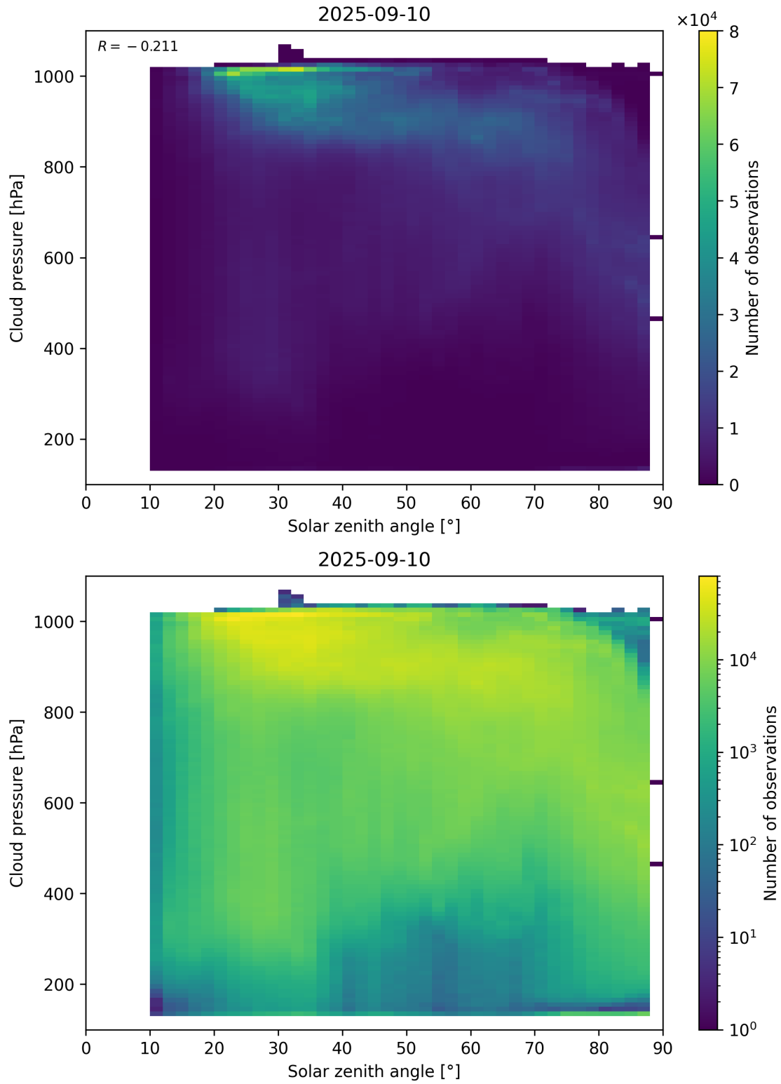
Figure 111: Scatter density plot of “Solar zenith angle” against “Cloud pressure” for 2025-09-10 to 2025-09-11.
