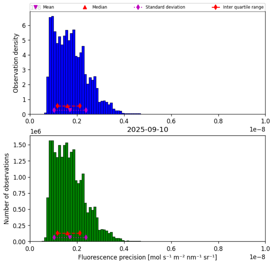
Figure 41: Histogram of “Fluorescence precision” for 2025-09-10 to 2025-09-11
