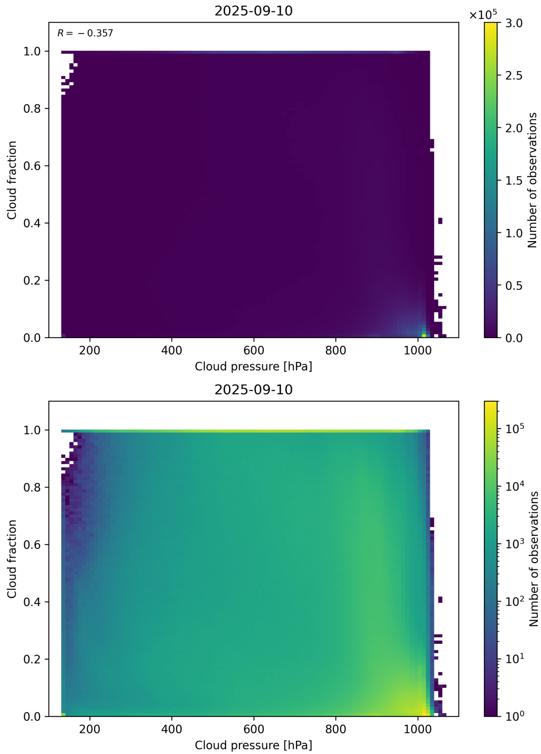
Figure 79: Scatter density plot of “Cloud pressure” against “Cloud fraction” for 2025-09-10 to 2025-09-11.
