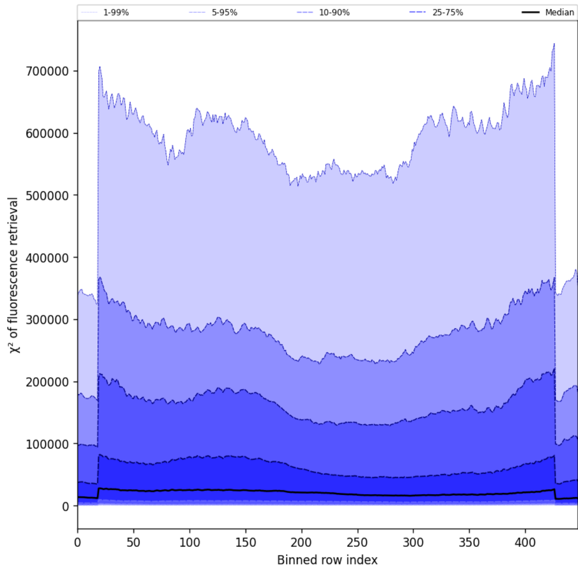
Figure 59: Along track statistics of “ \chi^2 of fluorescence retrieval” for 2025-09-10 to 2025-09-11
