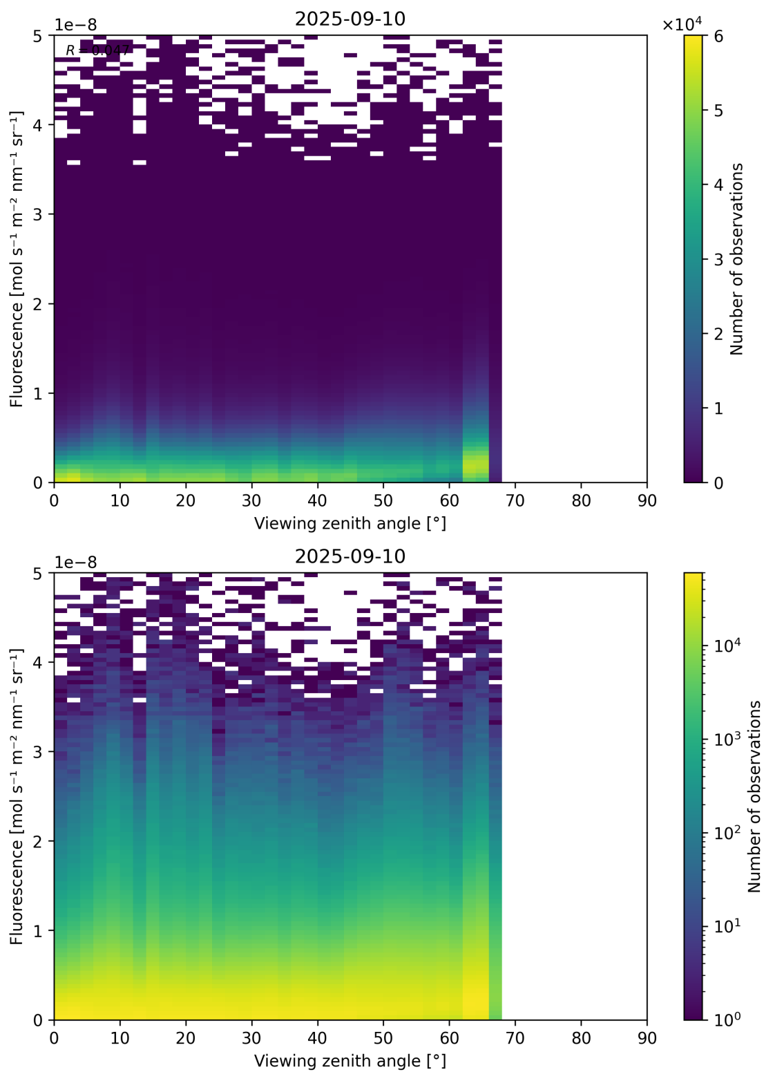
Figure 122: Scatter density plot of "Viewing zenith angle" against "Fluorescence" for 2025-09-10 to 2025-09-11.
