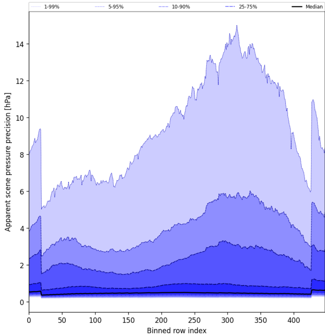
Figure 54: Along track statistics of “Apparent scene pressure precision” for 2025-09-10 to 2025-09-11
