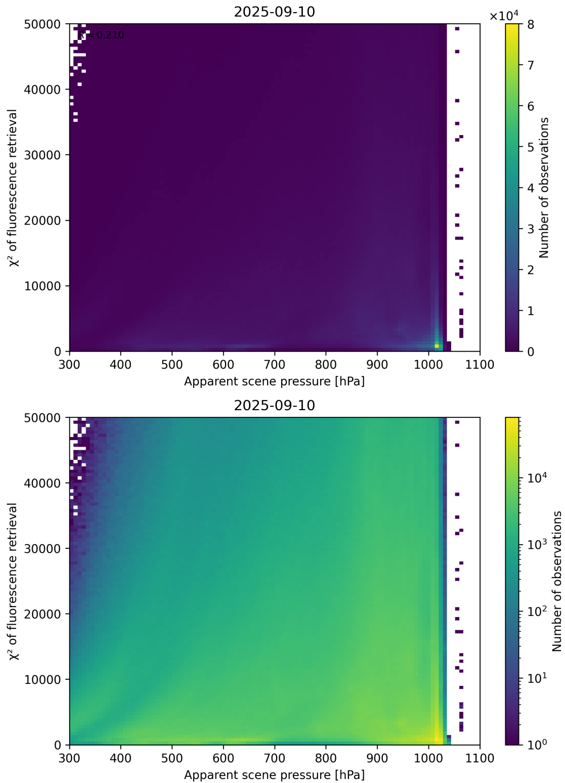
Figure 63: Scatter density plot of “Apparent scene pressure” against “ \chi^2 of fluorescence retrieval” for 2025-09-10 to 2025-09-11.
