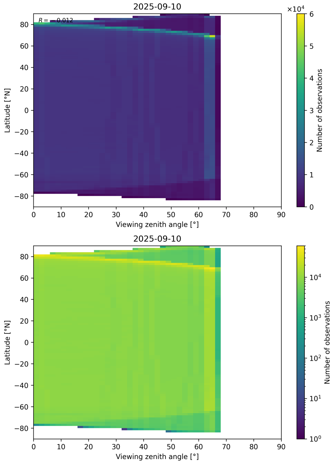
Figure 123: Scatter density plot of “Viewing zenith angle” against “Latitude” for 2025-09-10 to 2025-09-11.
