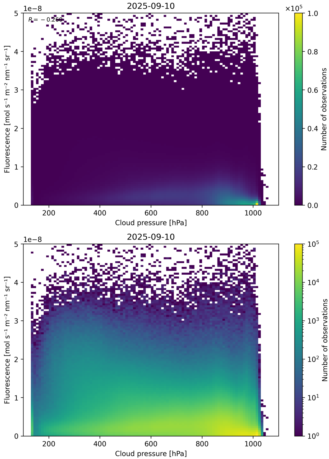
Figure 80: Scatter density plot of “Cloud pressure” against “Fluorescence” for 2025-09-10 to 2025-09-11.
