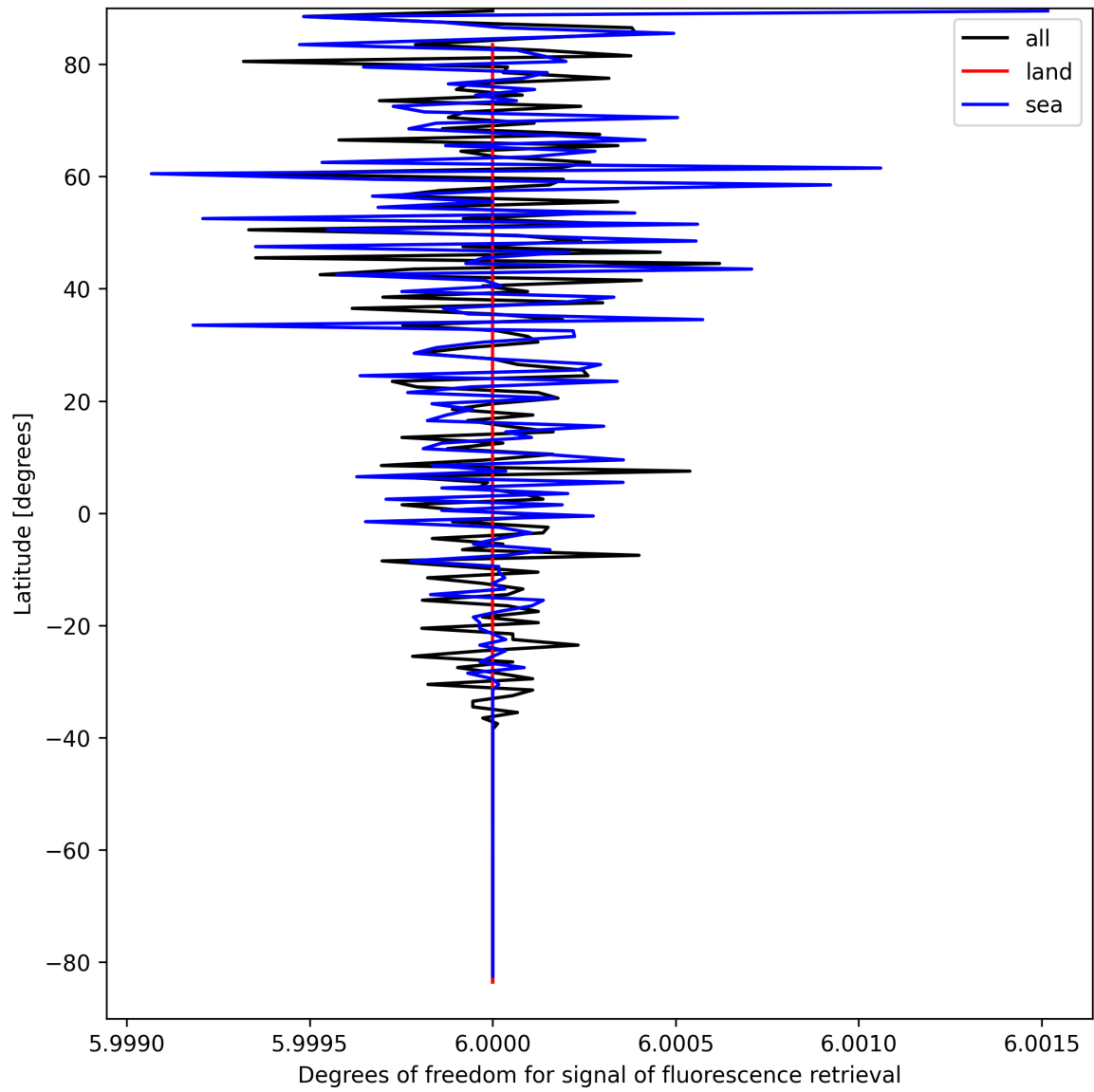
Figure 26: Zonal average of “Degrees of freedom for signal of fluorescence retrieval” for 2025-09-10 to 2025-09-11.
