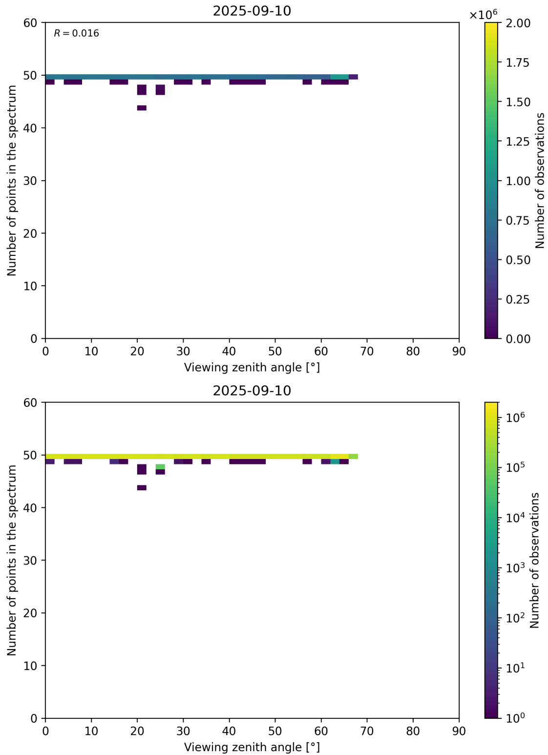
Figure 125: Scatter density plot of “Viewing zenith angle” against “Number of points in the spectrum” for 2025-09-10 to 2025-09-11.
