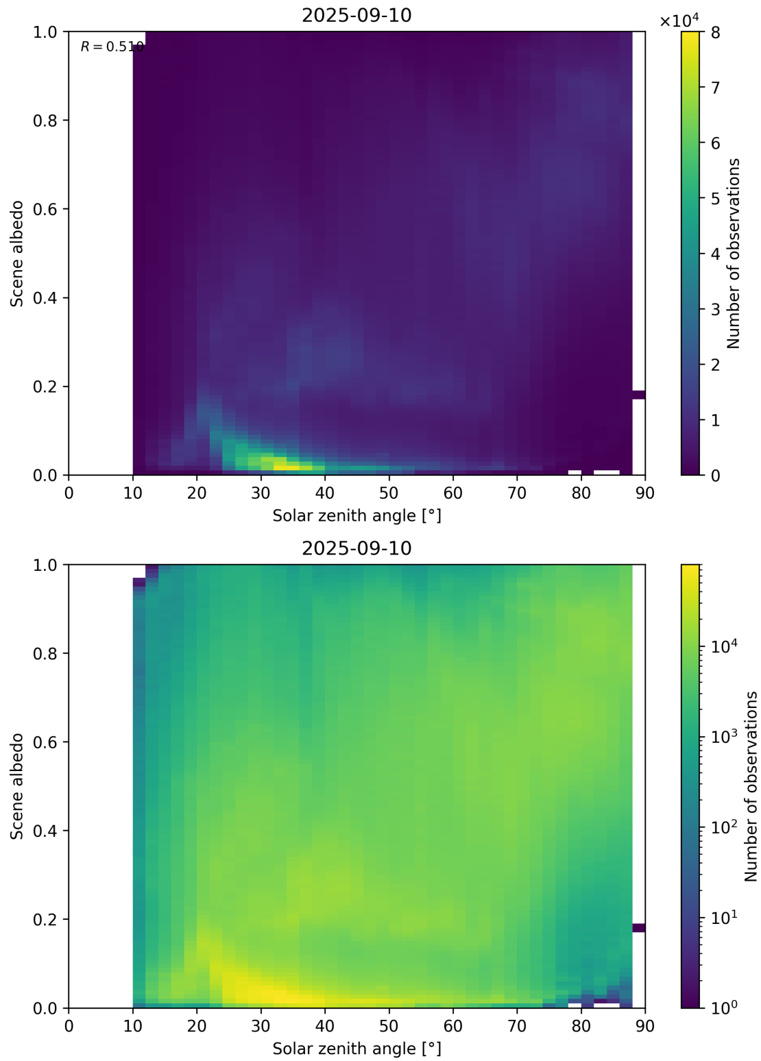
Figure 116: Scatter density plot of “Solar zenith angle” against “Scene albedo” for 2025-09-10 to 2025-09-11.
