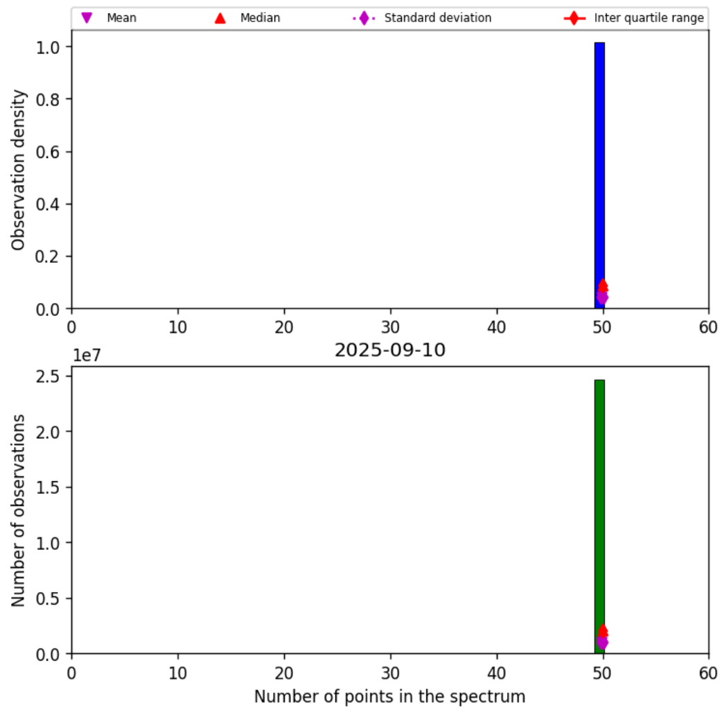
Figure 44: Histogram of “Number of points in the spectrum” for 2025-09-10 to 2025-09-11
