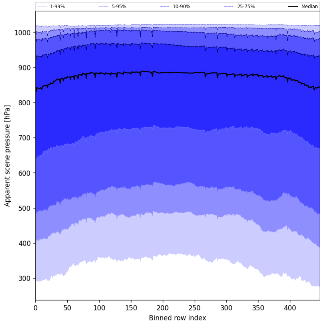
Figure 53: Along track statistics of “Apparent scene pressure” for 2025-09-10 to 2025-09-11
