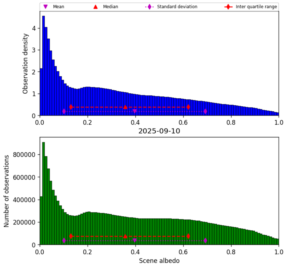
Figure 34: Histogram of “Scene albedo” for 2025-09-10 to 2025-09-11
