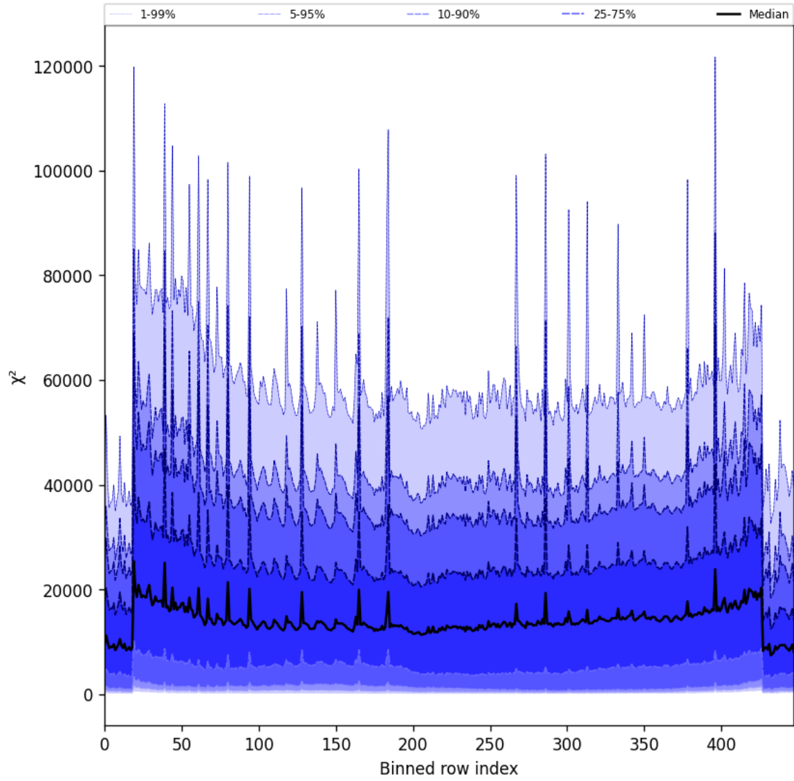
Figure 55: Along track statistics of “ \chi^2 ” for 2025-09-10 to 2025-09-11
