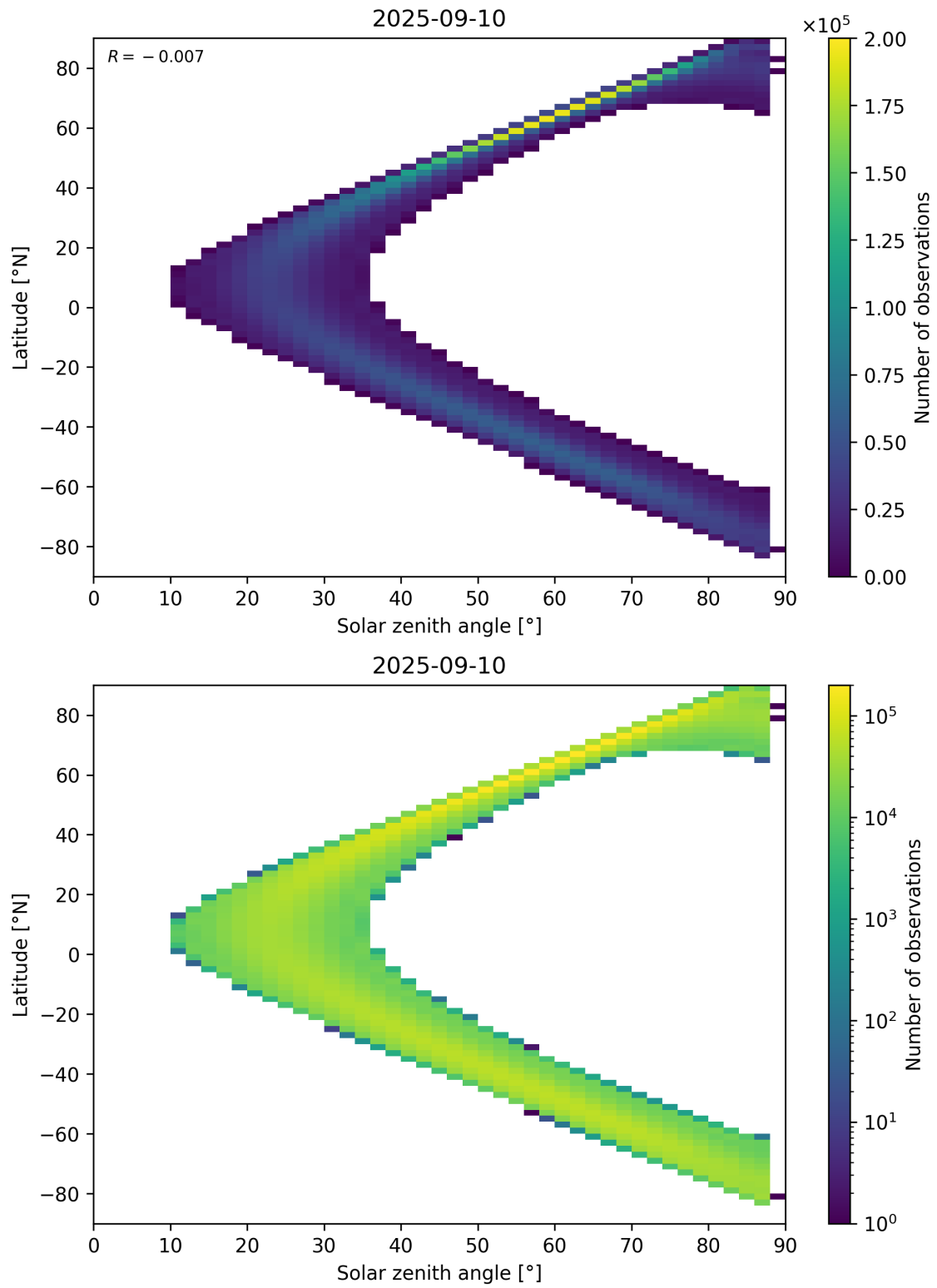
Figure 113: Scatter density plot of “Solar zenith angle” against “Latitude” for 2025-09-10 to 2025-09-11.
