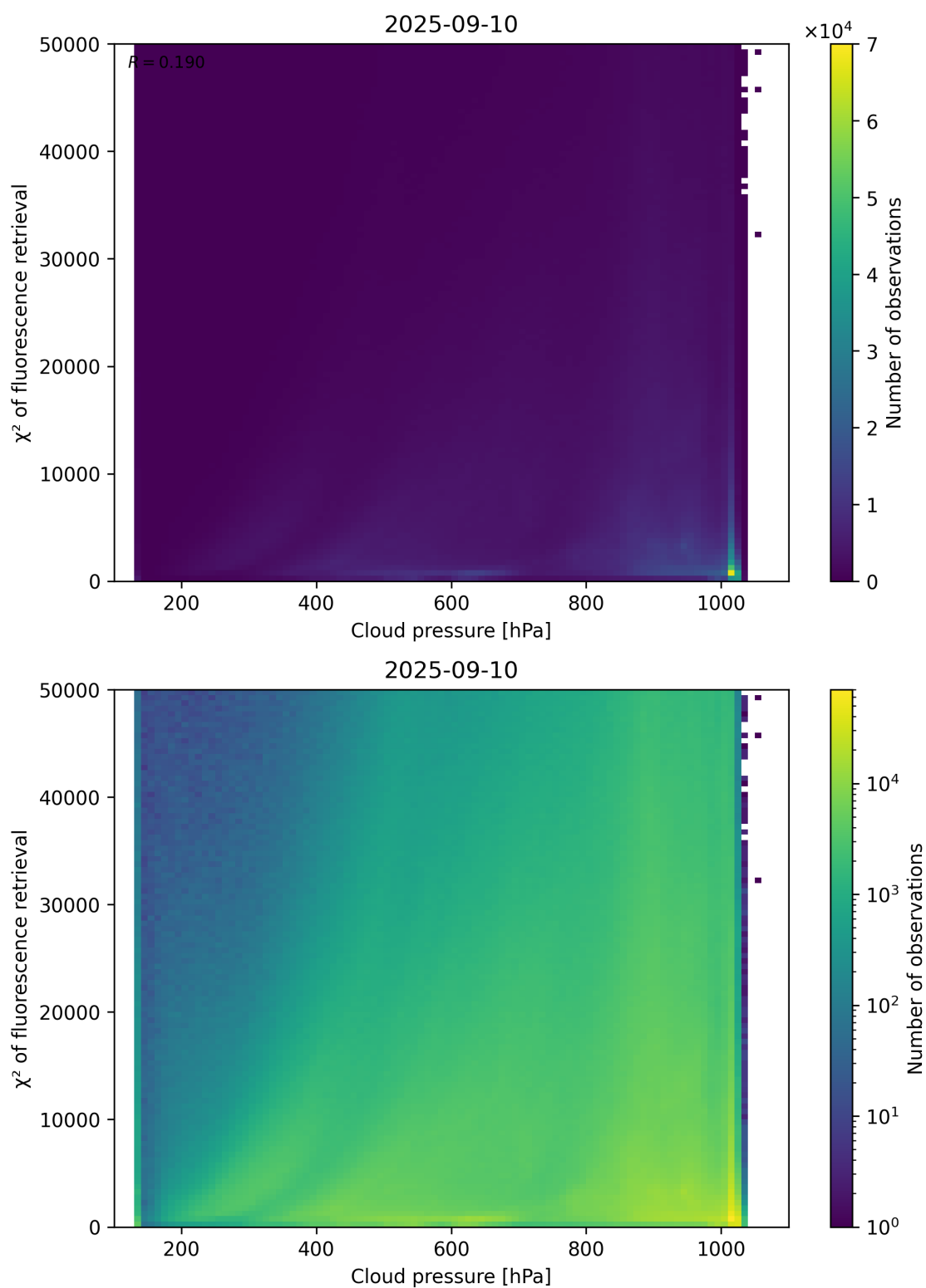
Figure 78: Scatter density plot of “Cloud pressure” against “ \chi^2 of fluorescence retrieval” for 2025-09-10 to 2025-09-11.
