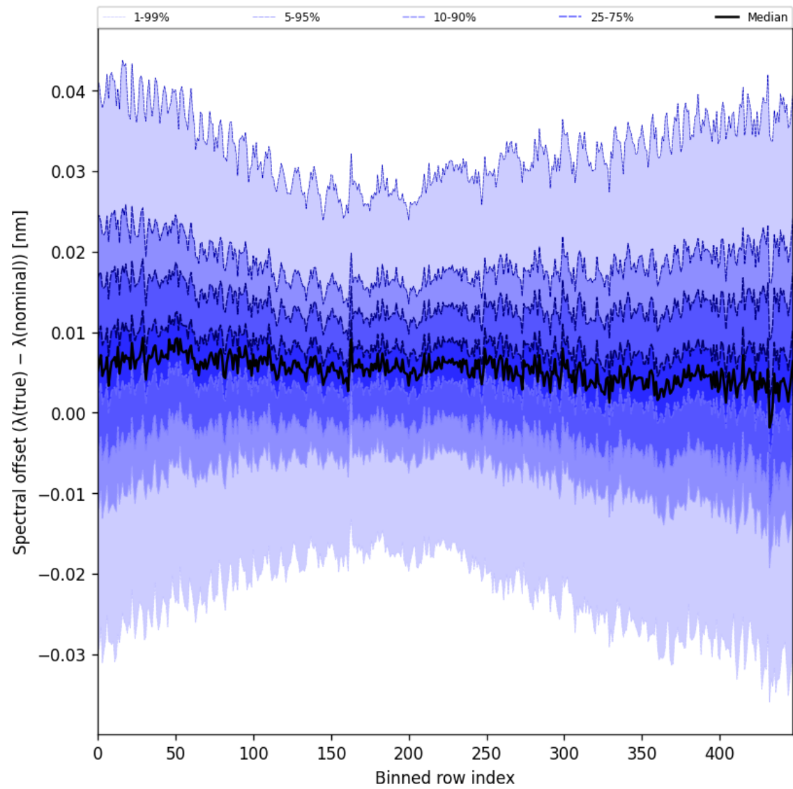
Figure 62: Along track statistics of “Spectral offset ( \lambda_{\text{true}} - \lambda_{\text{nominal}} )” for 2025-09-10 to 2025-09-11
