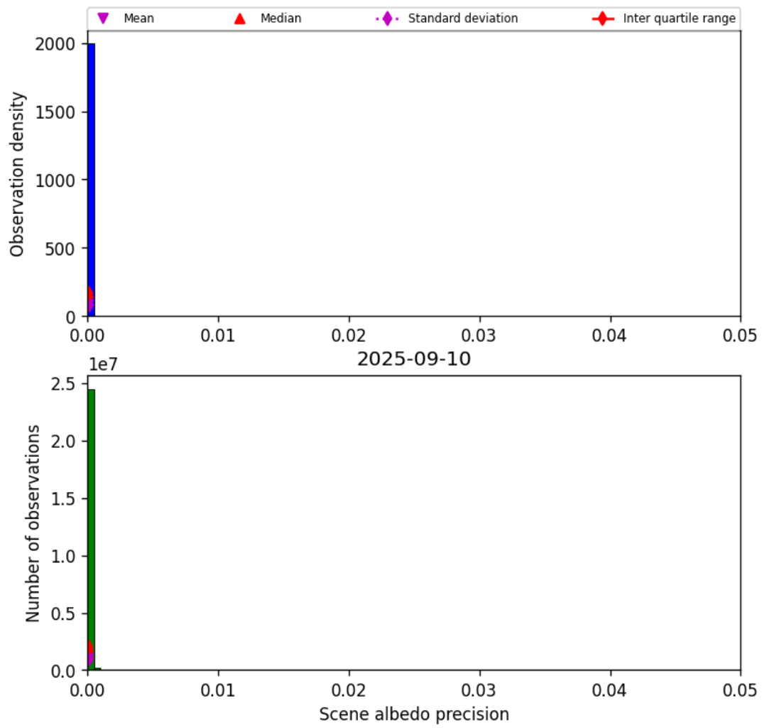
Figure 35: Histogram of “Scene albedo precision” for 2025-09-10 to 2025-09-11
