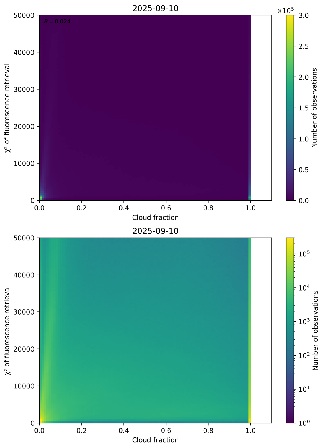
Figure 71: Scatter density plot of “Cloud fraction” against “ \chi^2 of fluorescence retrieval” for 2025-09-10 to 2025-09-11.
