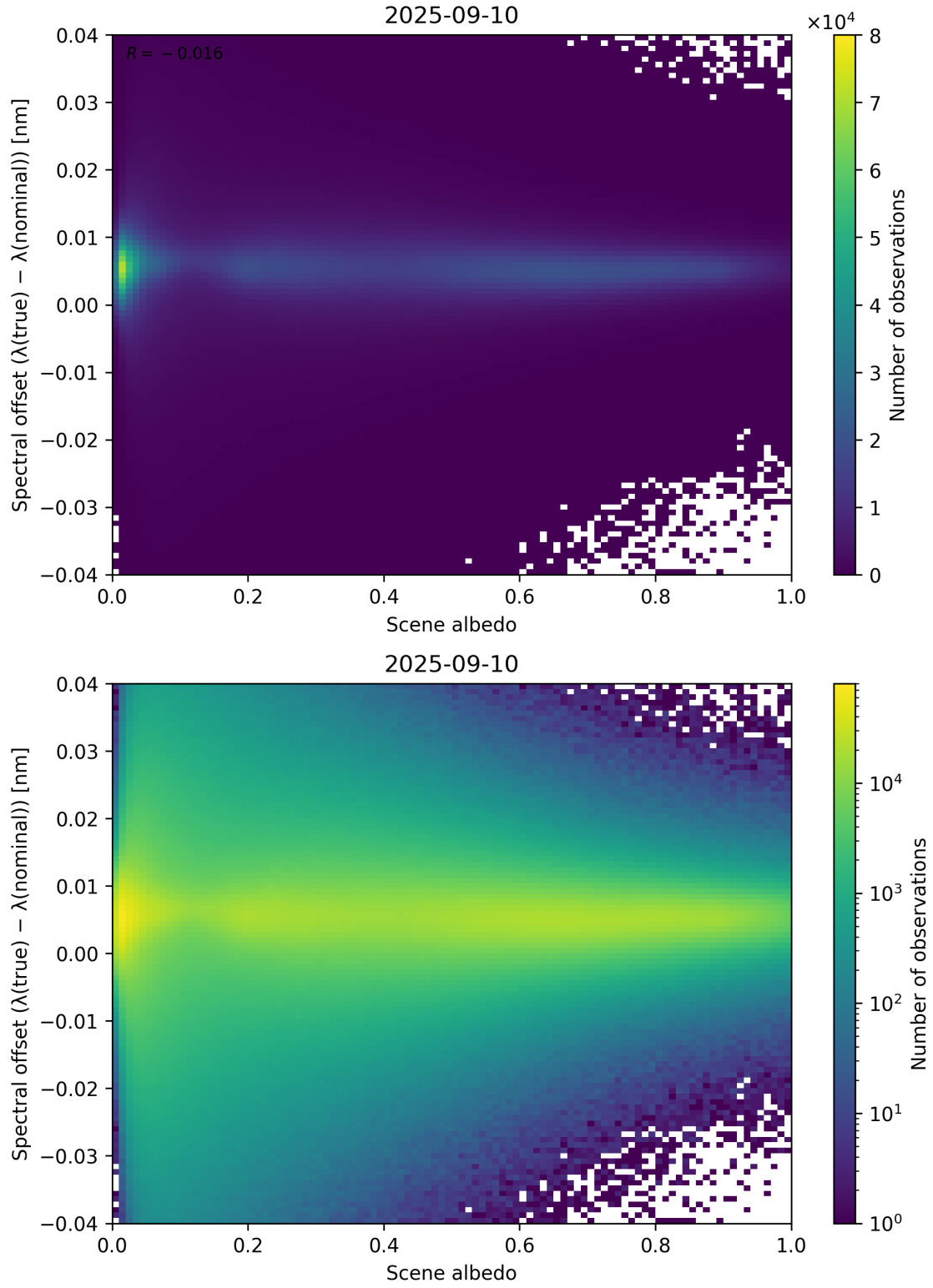
Figure 107: Scatter density plot of “Scene albedo” against “Spectral offset ( \lambda_{\text{true}} - \lambda_{\text{nominal}} )” for 2025-09-10 to 2025-09-11.
