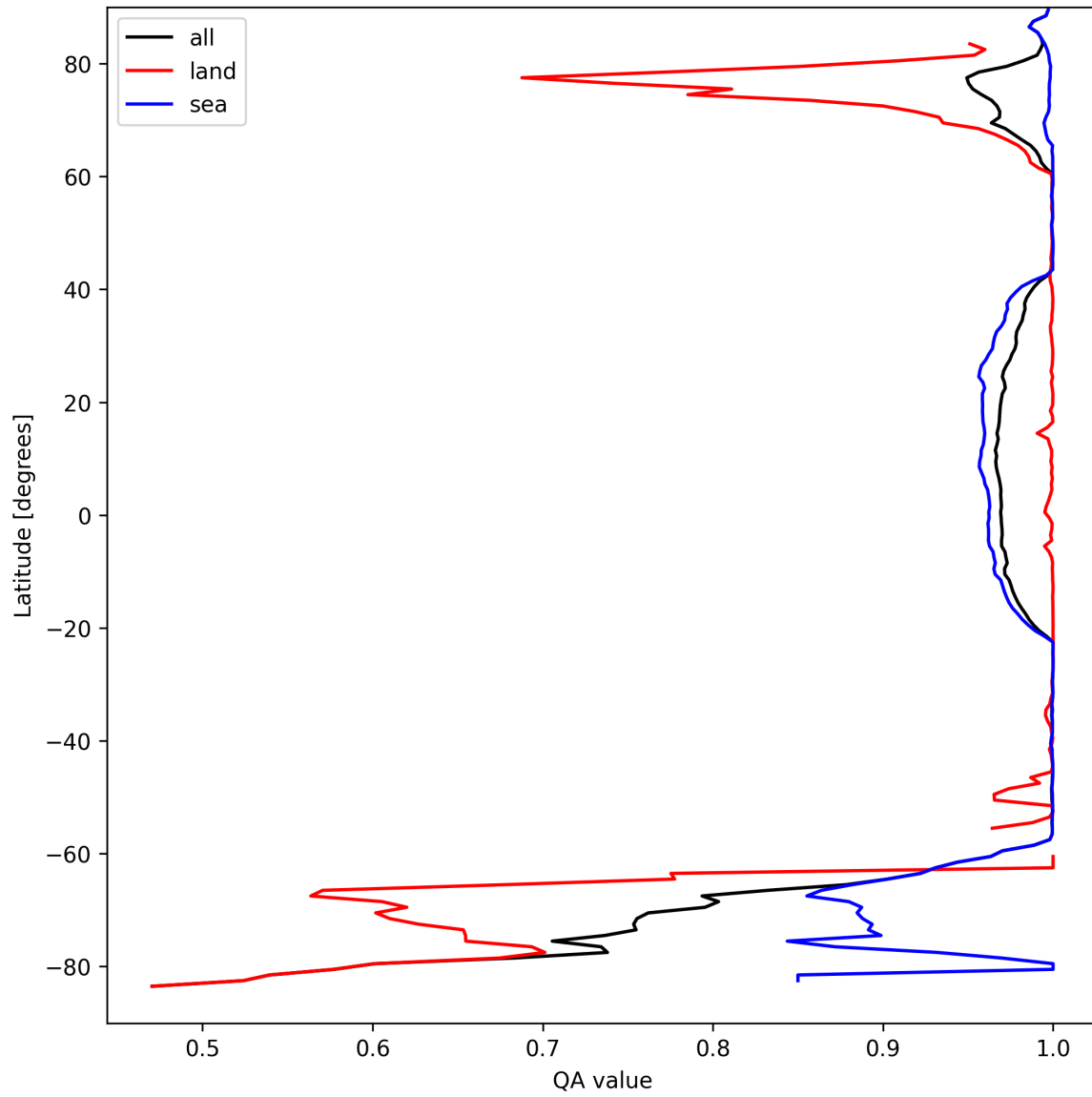
Figure 12: Zonal average of “QA value” for 2025-09-10 to 2025-09-11.
