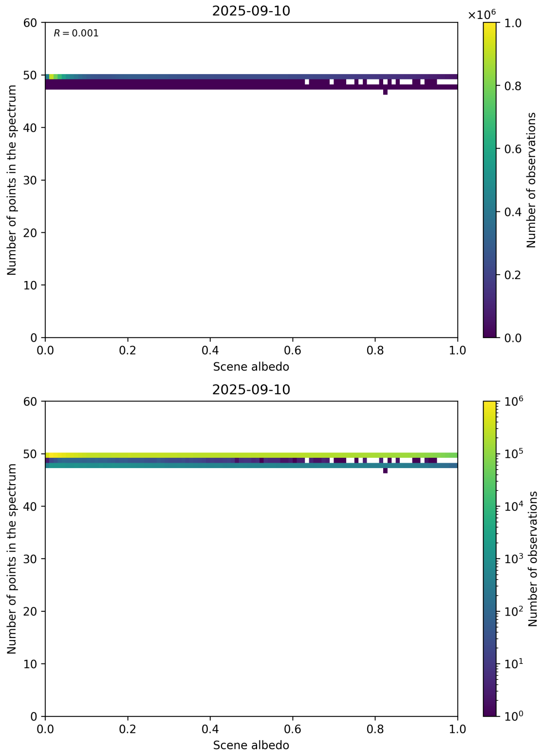
Figure 106: Scatter density plot of “Scene albedo” against “Number of points in the spectrum” for 2025-09-10 to 2025-09-11.
