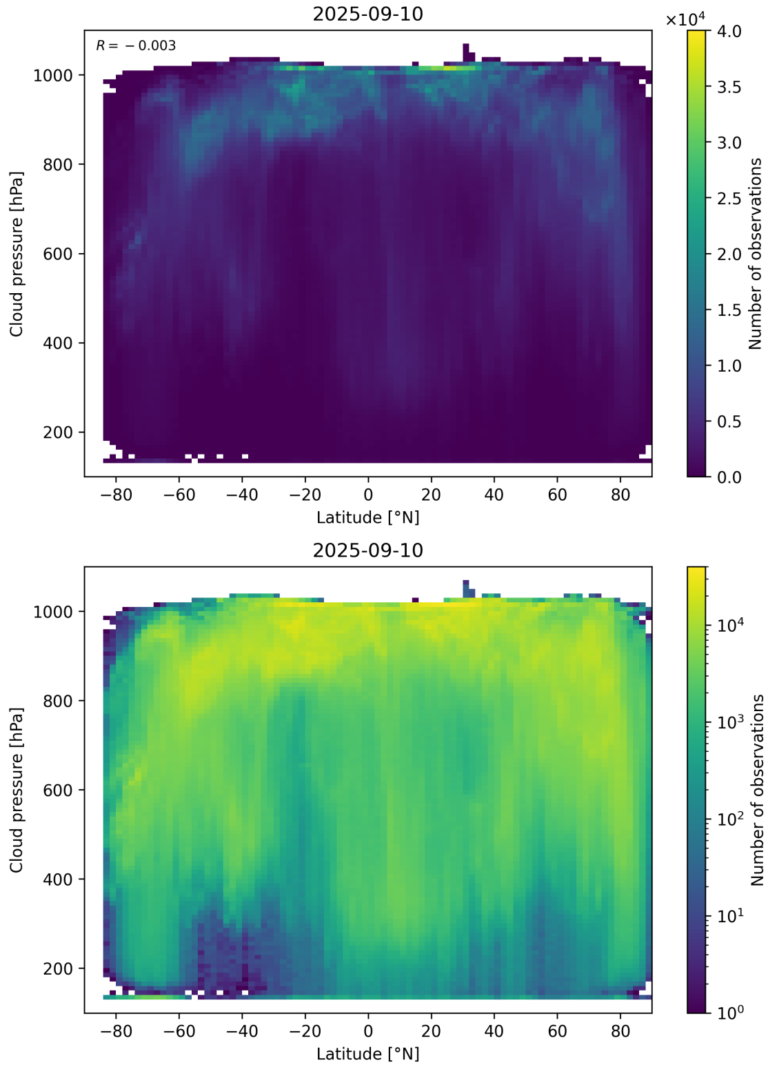
Figure 91: Scatter density plot of “Latitude” against “Cloud pressure” for 2025-09-10 to 2025-09-11.
