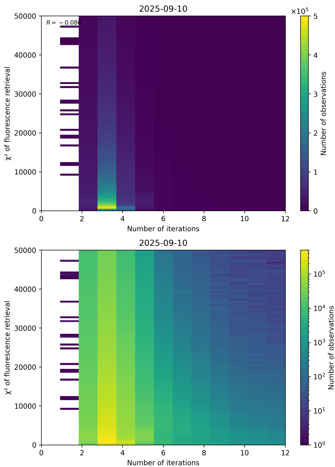
Figure 97: Scatter density plot of “Number of iterations” against “ \chi^2 of fluorescence retrieval” for 2025-09-10 to 2025-09-11.
