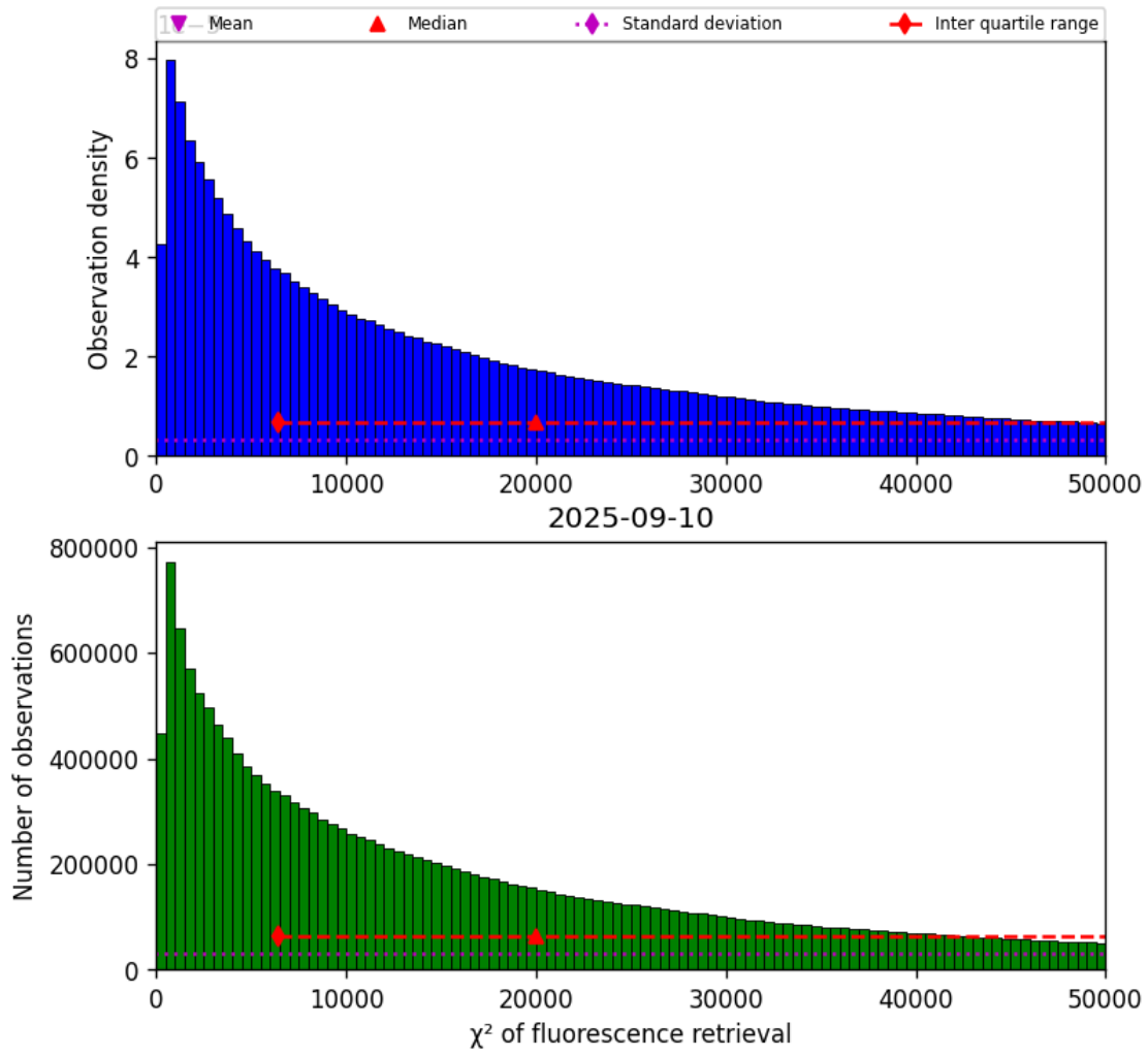
Figure 42: Histogram of “ \chi^2 of fluorescence retrieval” for 2025-09-10 to 2025-09-11
