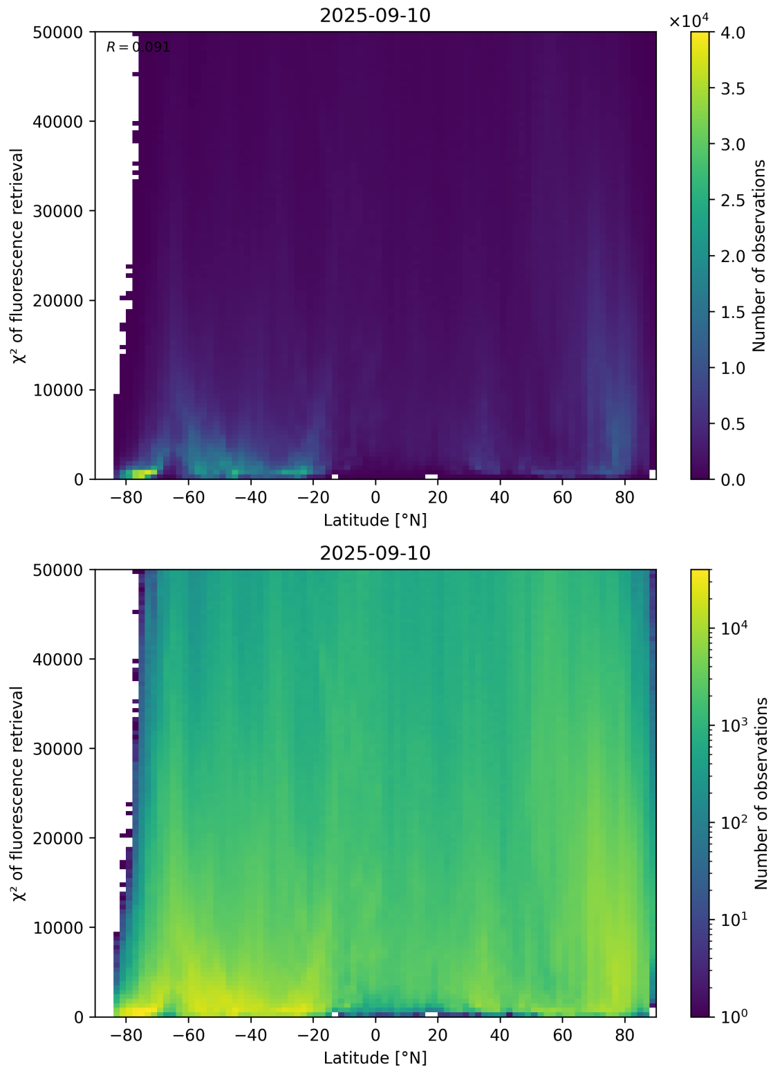
Figure 89: Scatter density plot of “Latitude” against “ \chi^2 of fluorescence retrieval” for 2025-09-10 to 2025-09-11.
