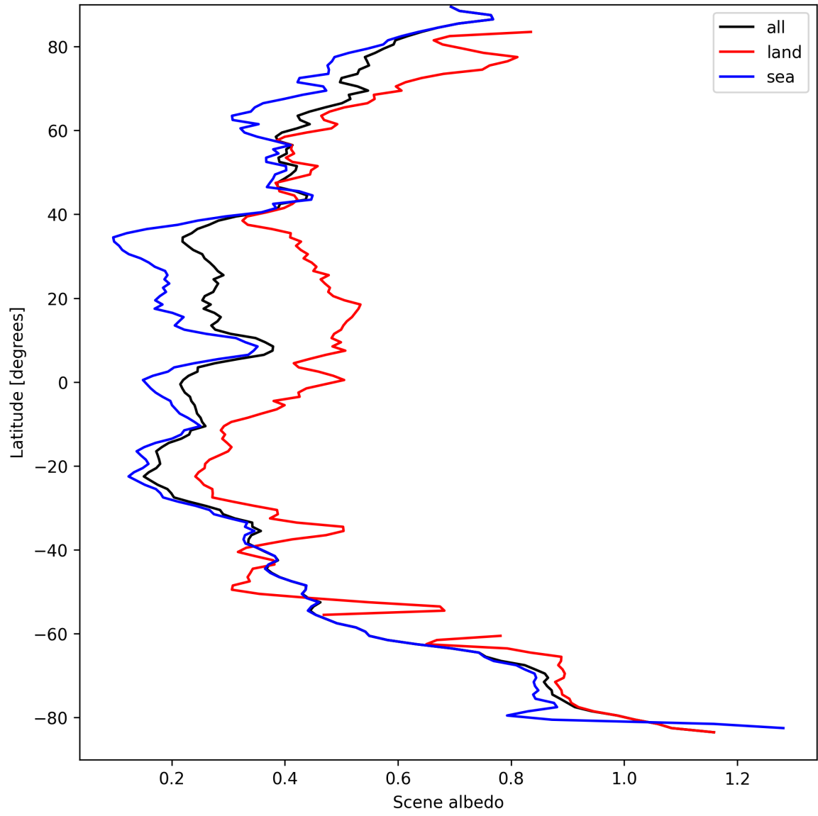
Figure 17: Zonal average of “Scene albedo” for 2025-09-10 to 2025-09-11.
