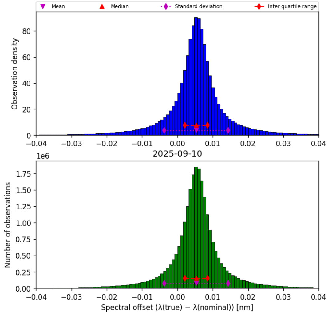
Figure 45: Histogram of “Spectral offset ( \lambda_{\text{true}} - \lambda_{\text{nominal}} )” for 2025-09-10 to 2025-09-11
