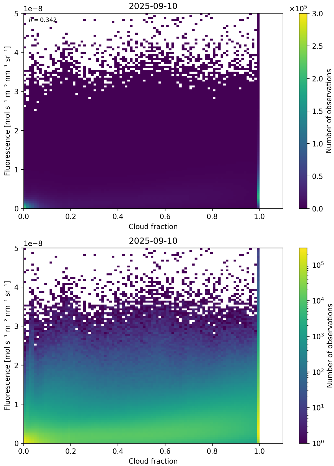
Figure 72: Scatter density plot of “Cloud fraction” against “Fluorescence” for 2025-09-10 to 2025-09-11.
