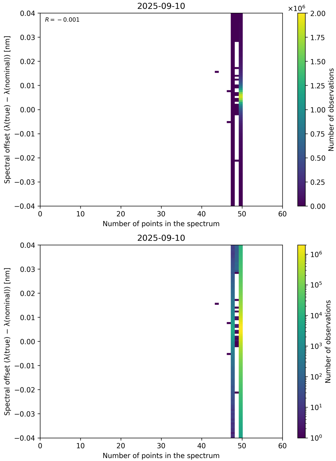
Figure 101: Scatter density plot of “Number of points in the spectrum” against “Spectral offset ( \lambda_{\text{true}} - \lambda_{\text{nominal}} )” for 2025-09-10 to 2025-09-11.
