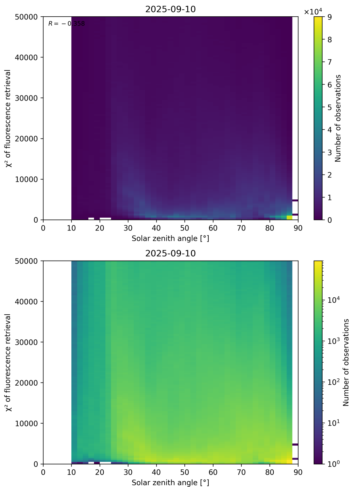
Figure 109: Scatter density plot of “Solar zenith angle” against “ \chi^2 of fluorescence retrieval” for 2025-09-10 to 2025-09-11.
