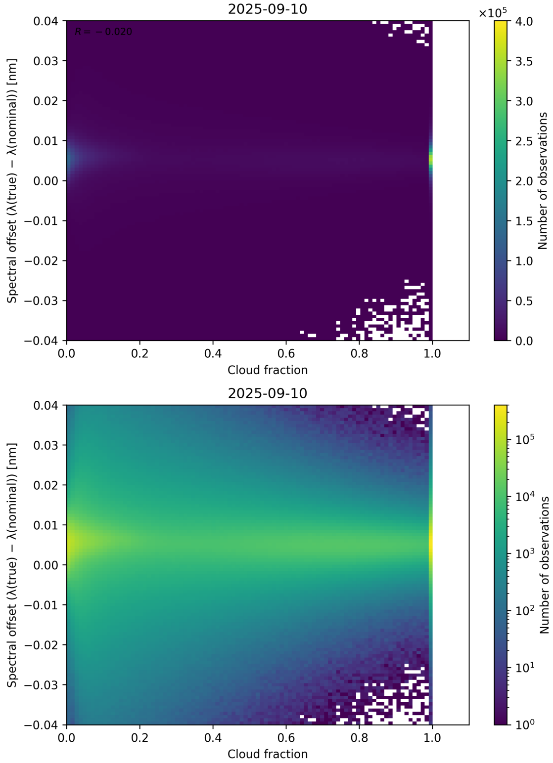
Figure 76: Scatter density plot of “Cloud fraction” against “Spectral offset ( \lambda_{\text{true}} - \lambda_{\text{nominal}} )” for 2025-09-10 to 2025-09-11.
