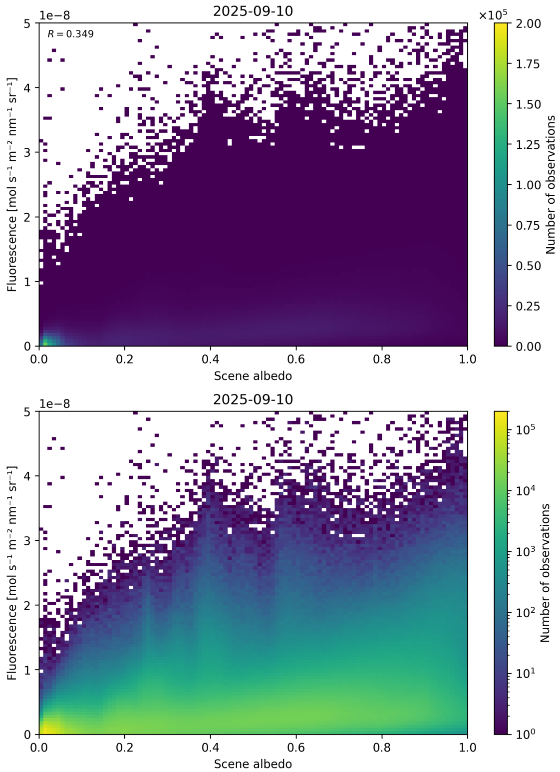
Figure 104: Scatter density plot of “Scene albedo” against “Fluorescence” for 2025-09-10 to 2025-09-11.
