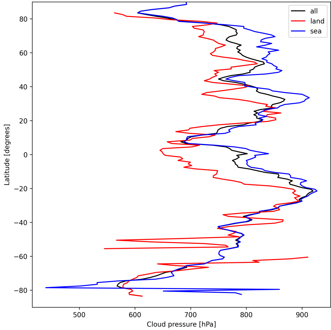
Figure 13: Zonal average of “Cloud pressure” for 2025-09-10 to 2025-09-11.
