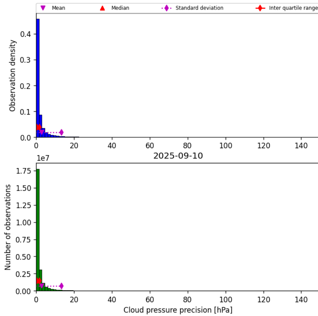
Figure 31: Histogram of “Cloud pressure precision” for 2025-09-10 to 2025-09-11
