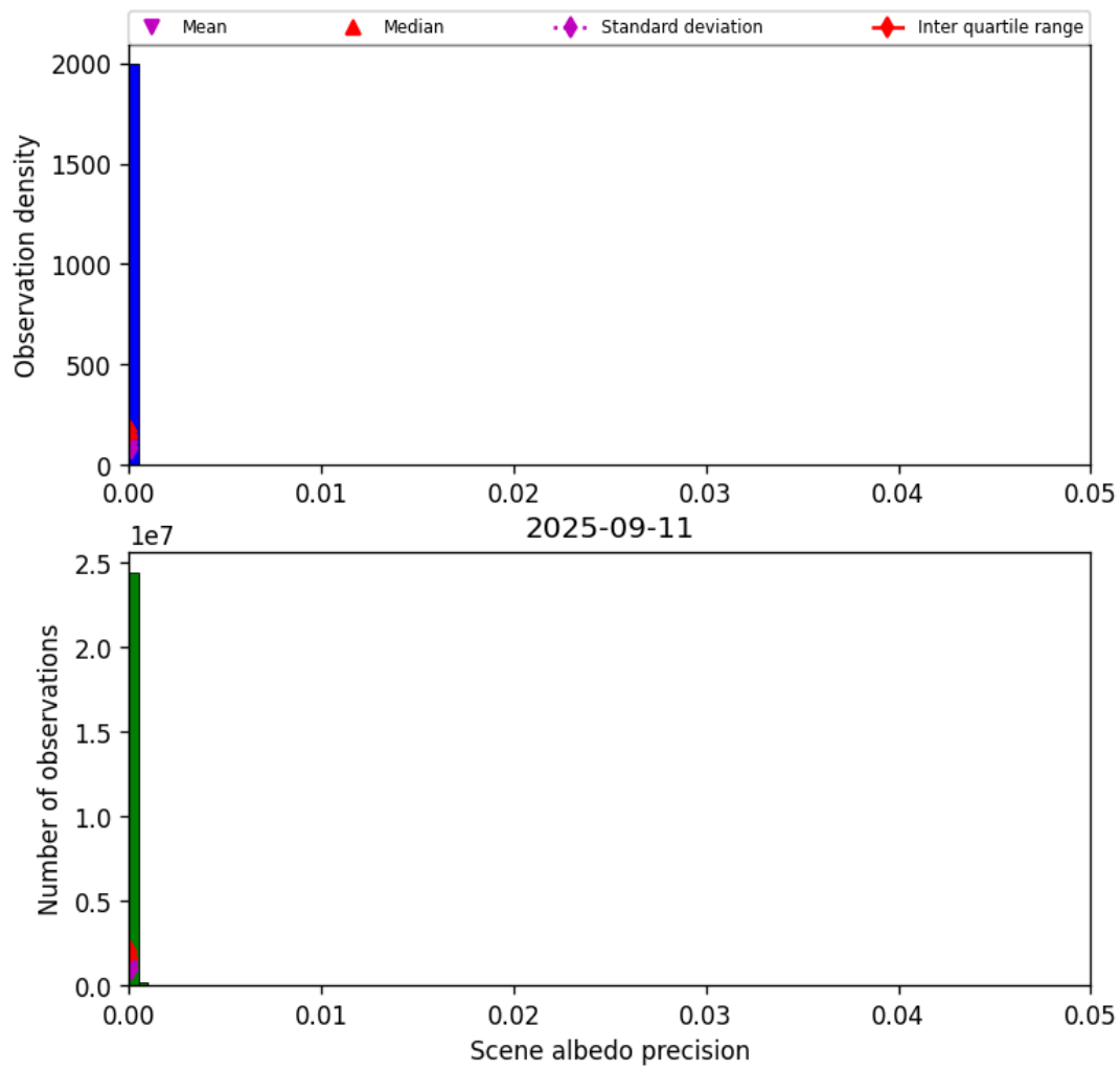
Figure 35: Histogram of “Scene albedo precision” for 2025-09-10 to 2025-09-12
