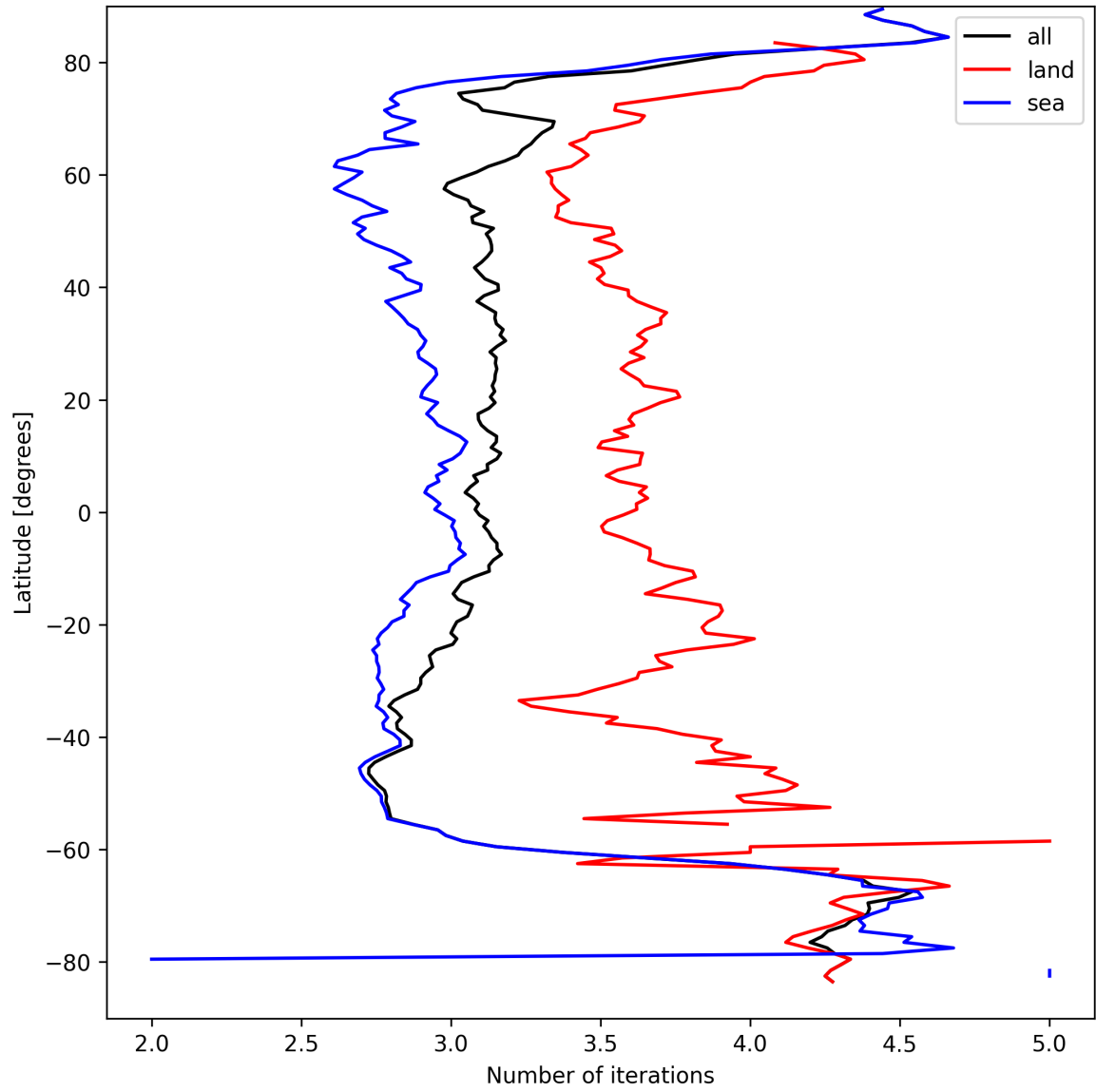
Figure 22: Zonal average of “Number of iterations” for 2025-09-10 to 2025-09-12.
