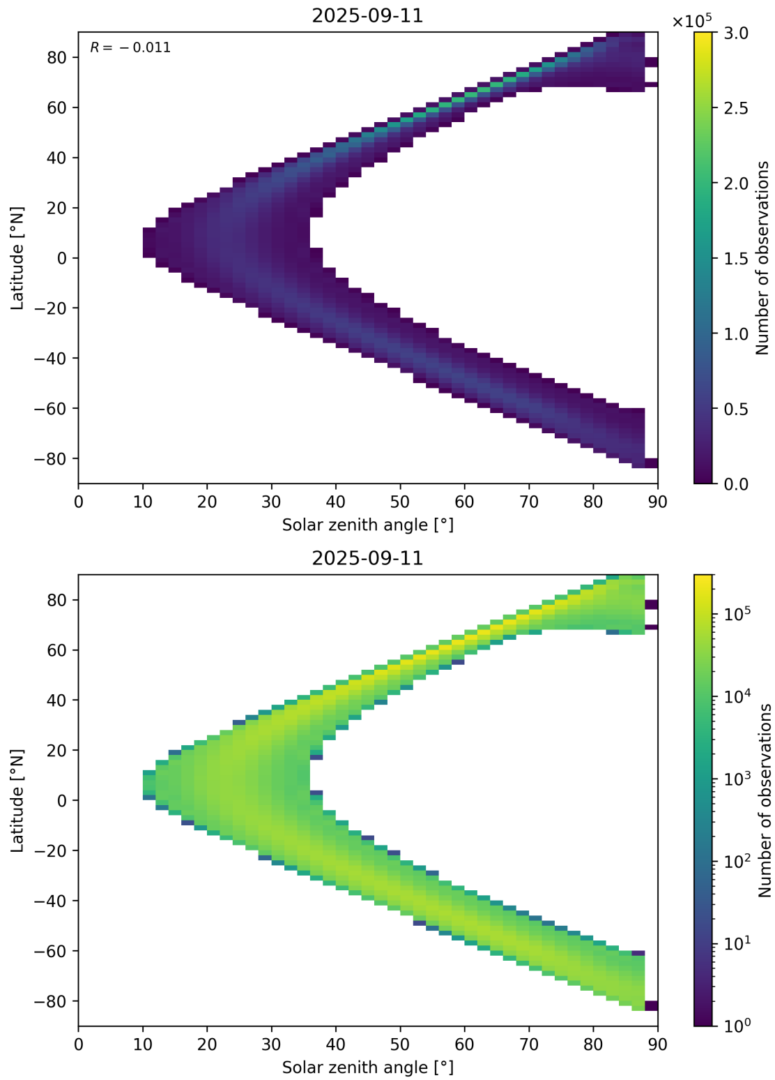
Figure 113: Scatter density plot of “Solar zenith angle” against “Latitude” for 2025-09-10 to 2025-09-12.
