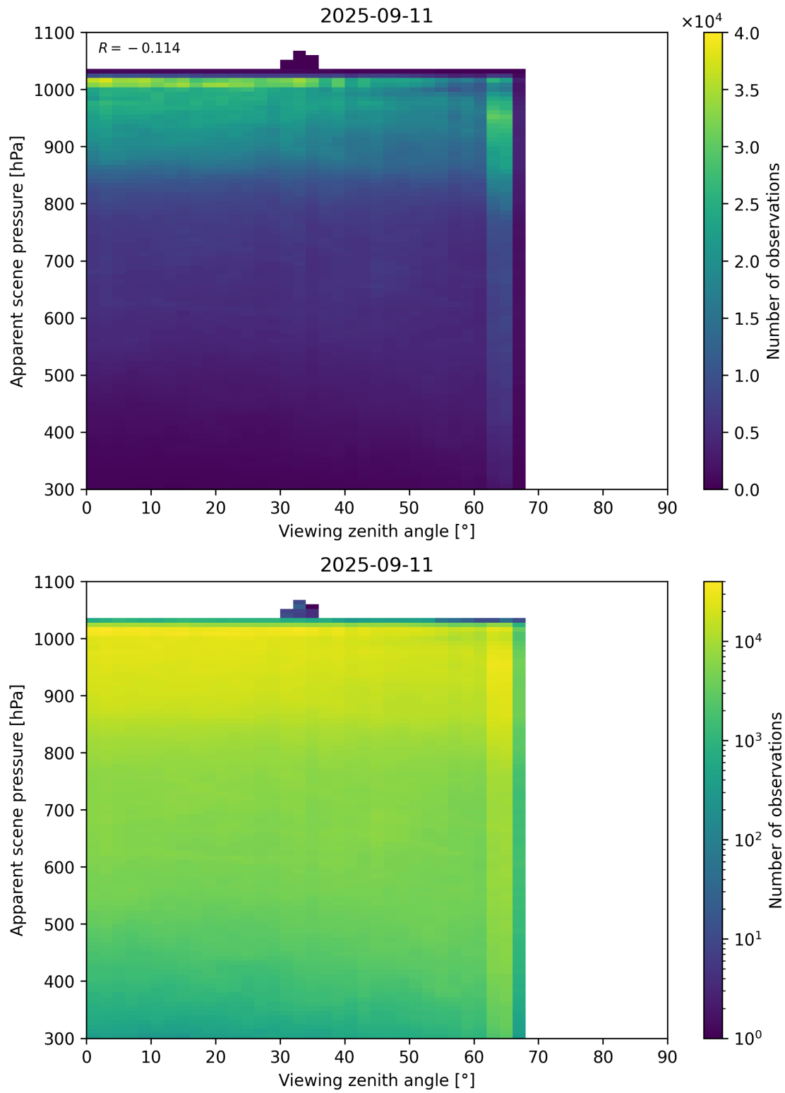
Figure 118: Scatter density plot of “Viewing zenith angle” against “Apparent scene pressure” for 2025-09-10 to 2025-09-12.
