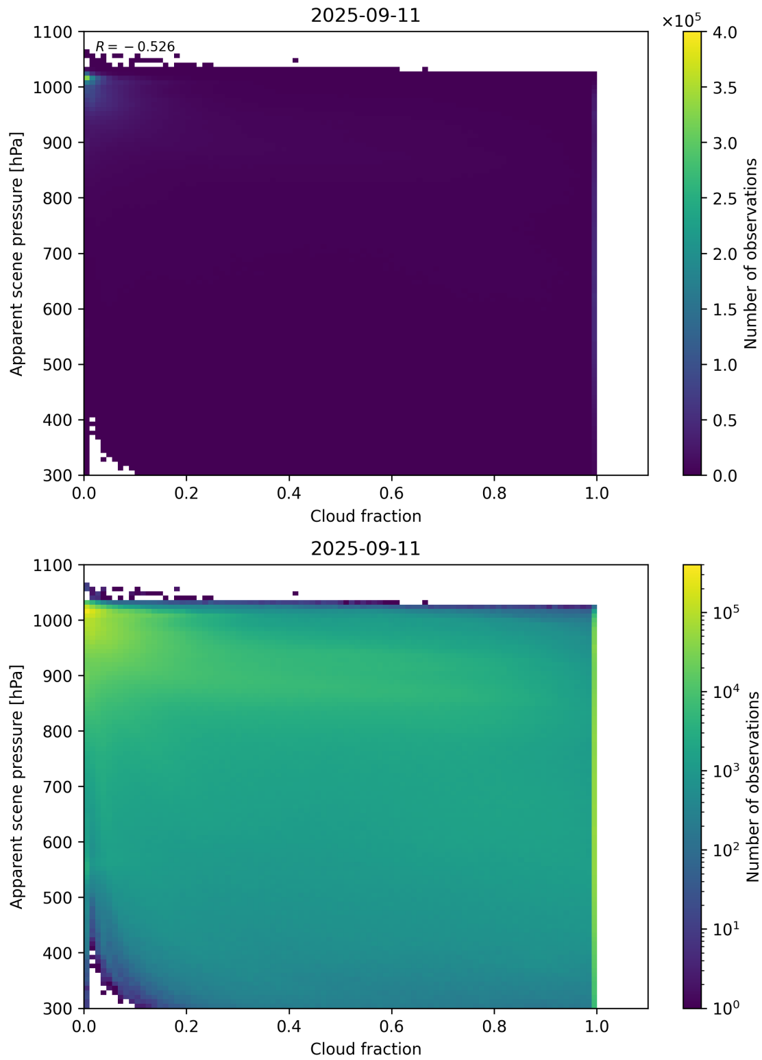
Figure 70: Scatter density plot of “Cloud fraction” against “Apparent scene pressure” for 2025-09-10 to 2025-09-12.
