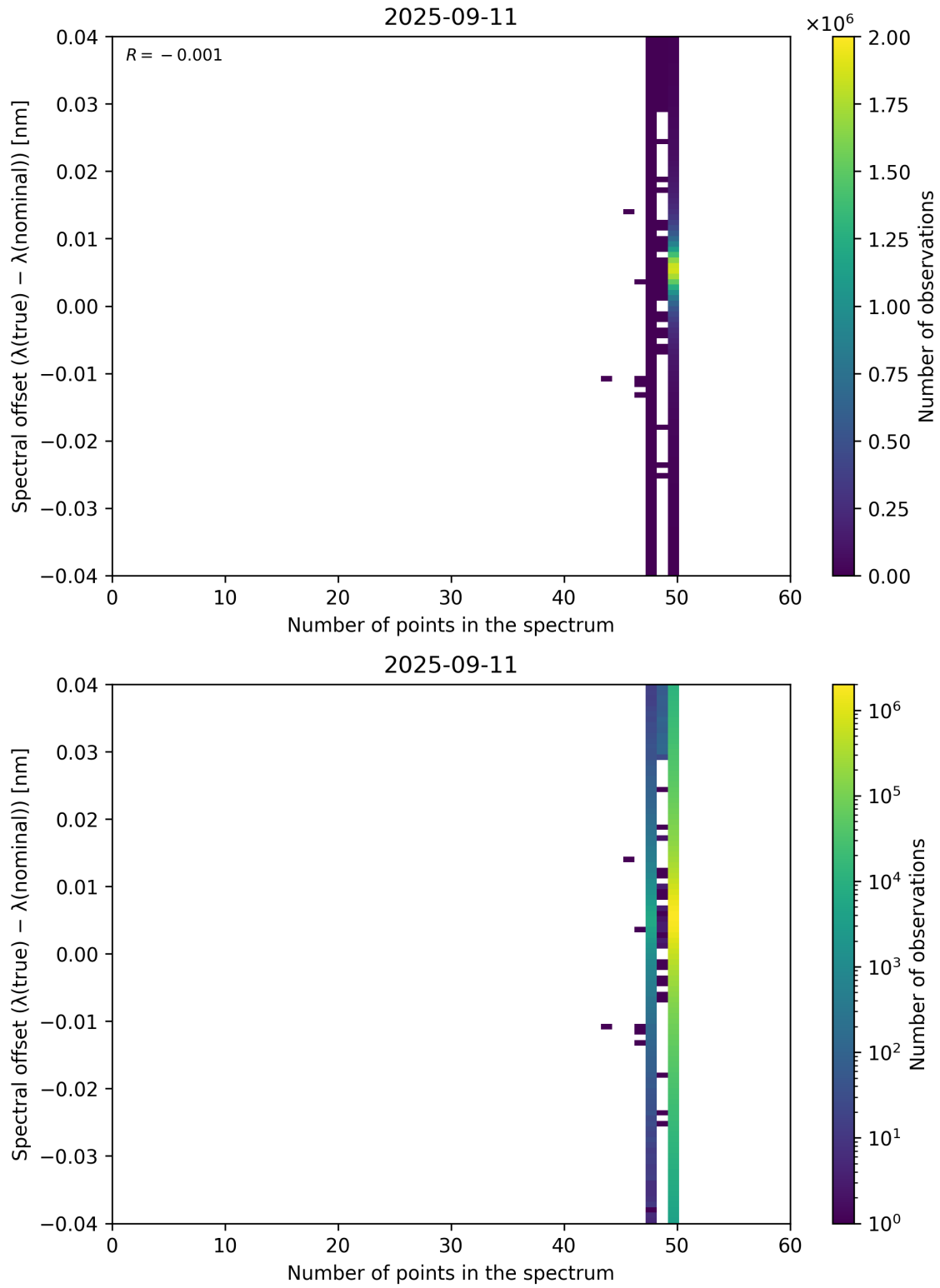
Figure 101: Scatter density plot of “Number of points in the spectrum” against “Spectral offset ( \lambda_{\text{true}} - \lambda_{\text{nominal}} )” for 2025-09-10 to 2025-09-12.
