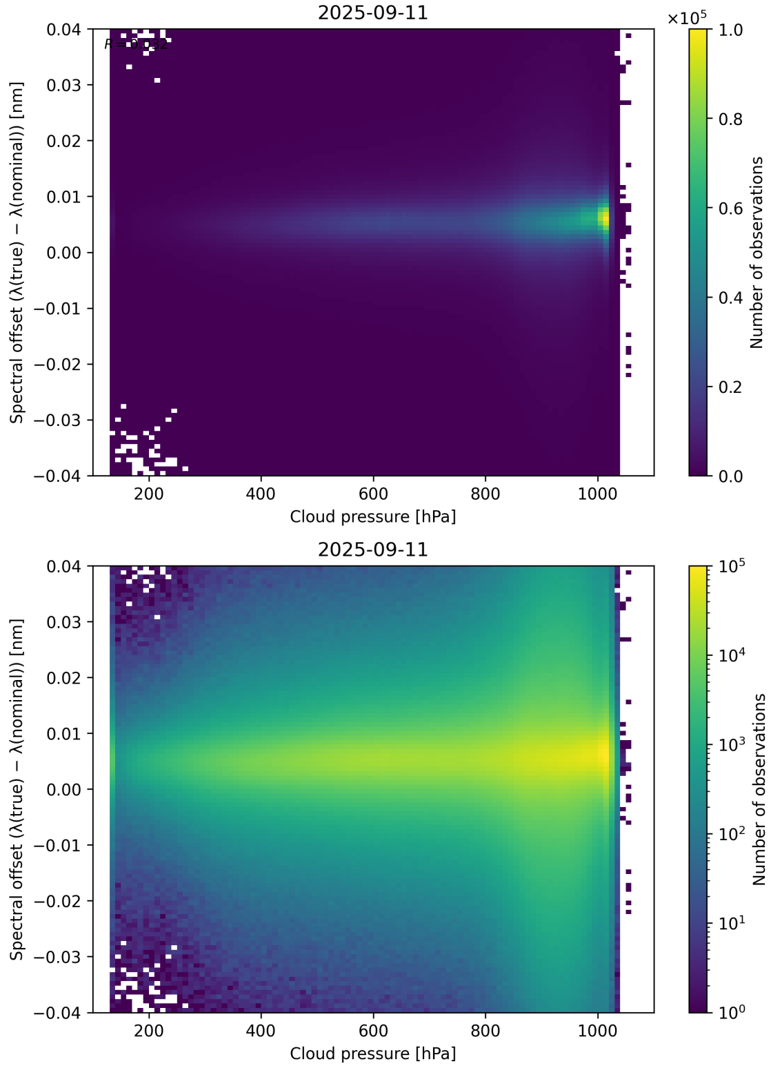
Figure 84: Scatter density plot of “Cloud pressure” against “Spectral offset ( \lambda_{\text{true}} - \lambda_{\text{nominal}} )” for 2025-09-10 to 2025-09-12.
