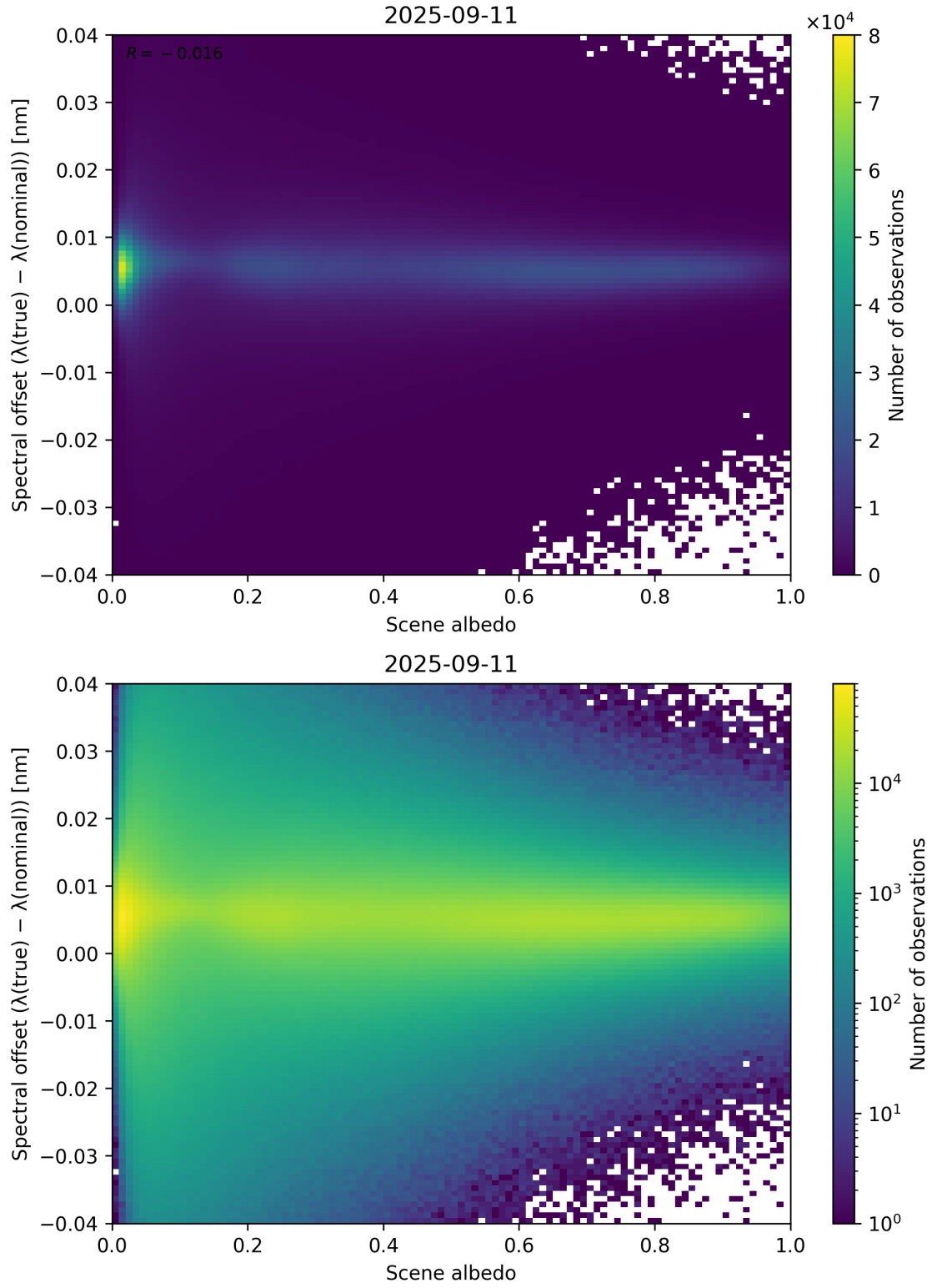
Figure 107: Scatter density plot of “Scene albedo” against “Spectral offset ( \lambda_{\text{true}} - \lambda_{\text{nominal}} )” for 2025-09-10 to 2025-09-12.
