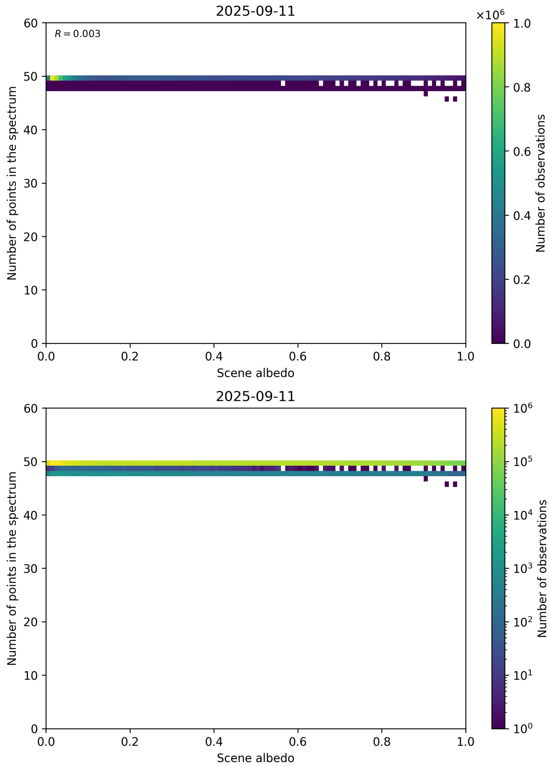
Figure 106: Scatter density plot of “Scene albedo” against “Number of points in the spectrum” for 2025-09-10 to 2025-09-12.
