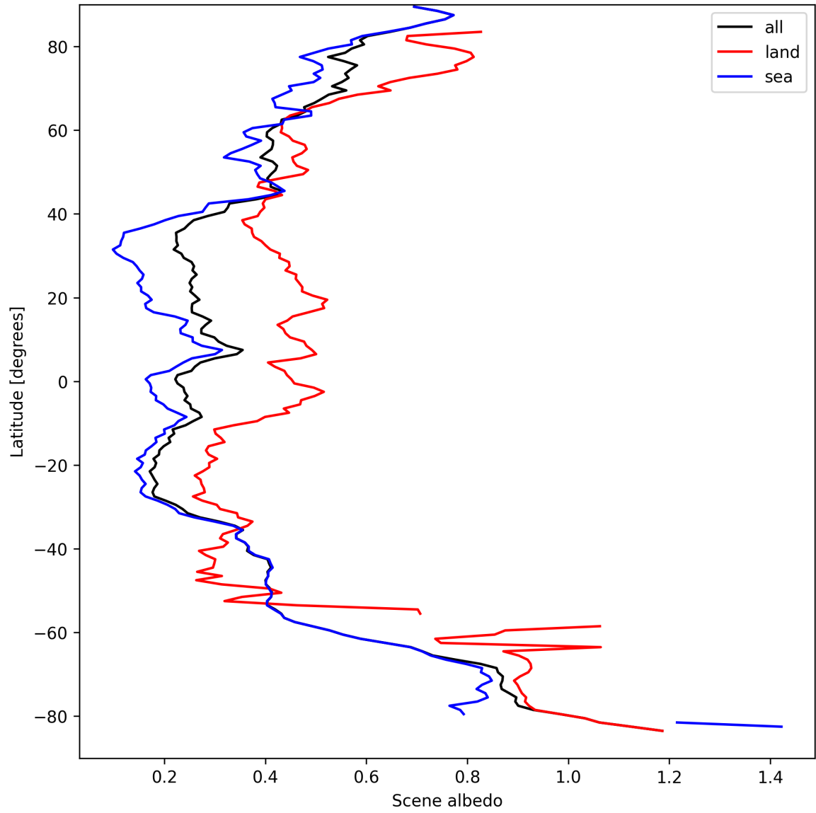
Figure 17: Zonal average of “Scene albedo” for 2025-09-10 to 2025-09-12.
