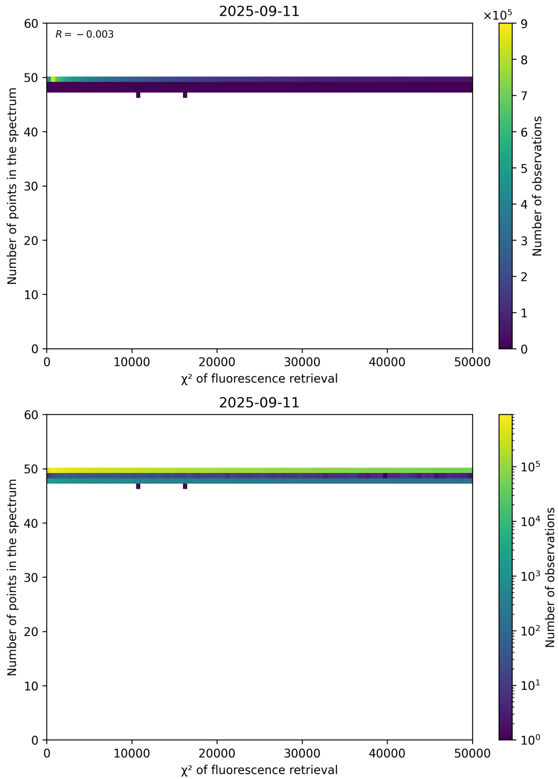
Figure 68: Scatter density plot of “ \chi^2 of fluorescence retrieval” against “Number of points in the spectrum” for 2025-09-10 to 2025-09-12.
