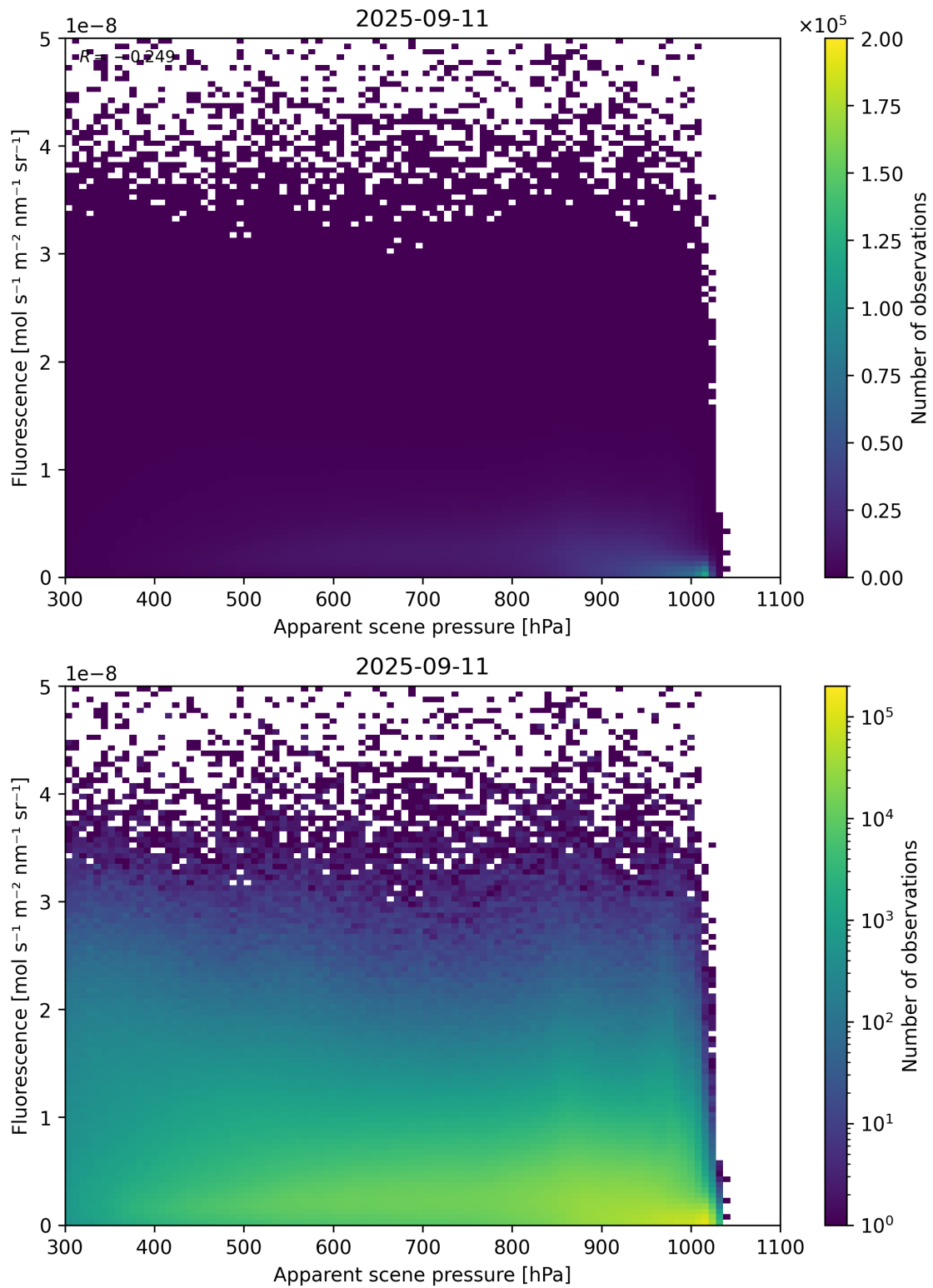
Figure 64: Scatter density plot of “Apparent scene pressure” against “Fluorescence” for 2025-09-10 to 2025-09-12.
