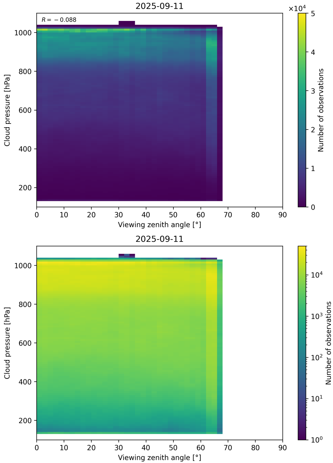
Figure 121: Scatter density plot of “Viewing zenith angle” against “Cloud pressure” for 2025-09-10 to 2025-09-12.
