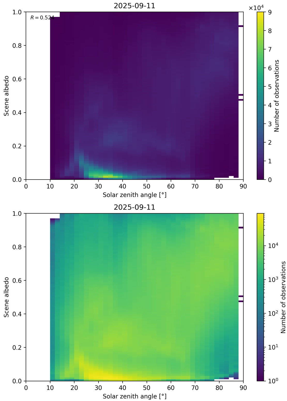
Figure 116: Scatter density plot of “Solar zenith angle” against “Scene albedo” for 2025-09-10 to 2025-09-12.
