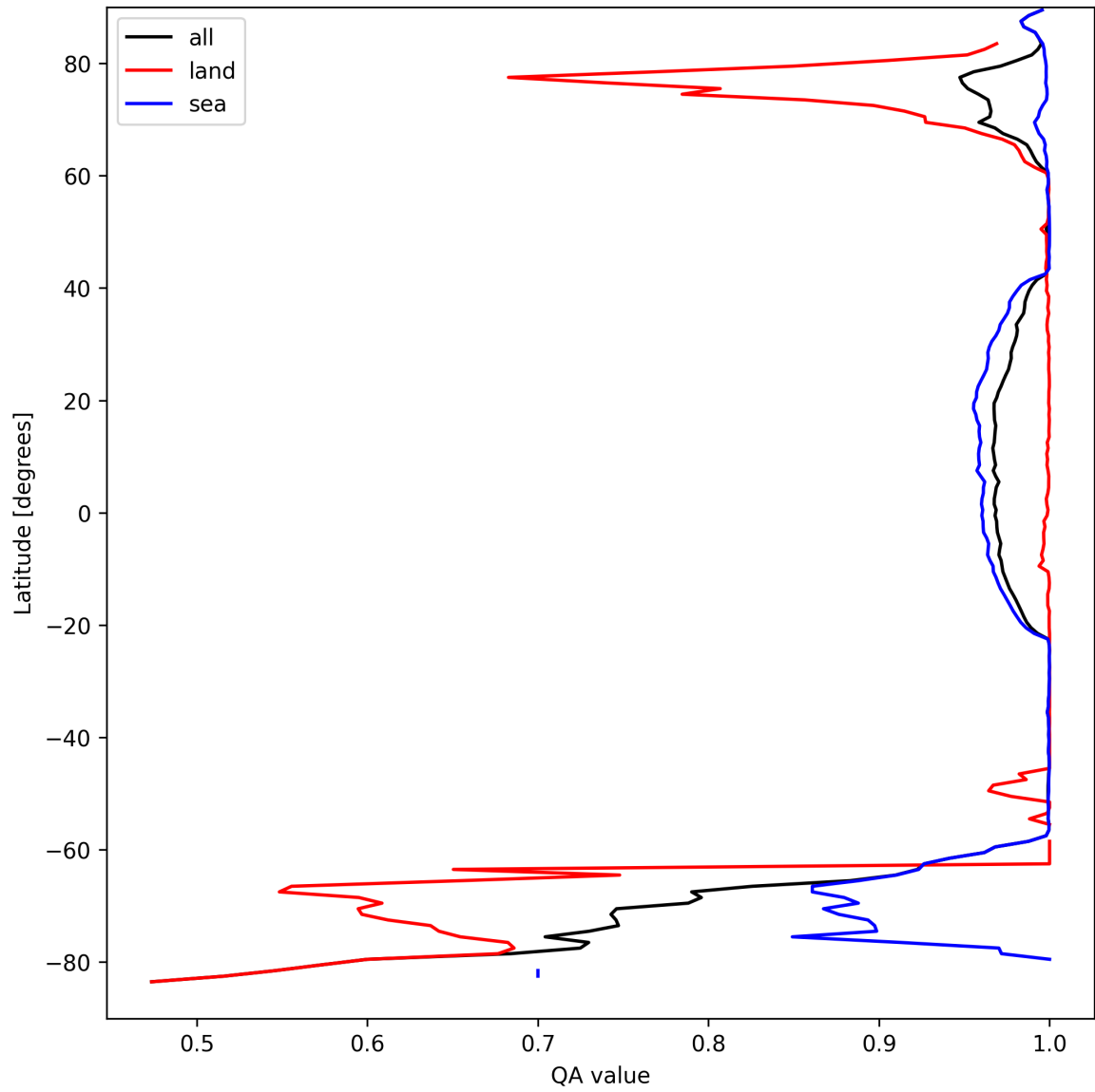
Figure 12: Zonal average of “QA value” for 2025-09-10 to 2025-09-12.
