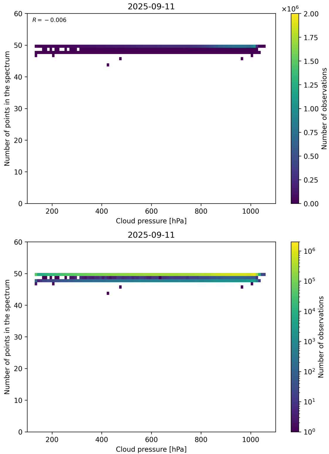
Figure 82: Scatter density plot of “Cloud pressure” against “Number of points in the spectrum” for 2025-09-10 to 2025-09-12.
