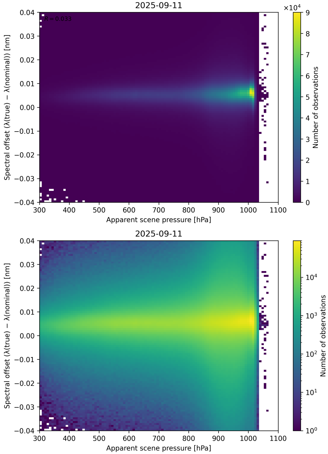
Figure 67: Scatter density plot of “Apparent scene pressure” against “Spectral offset ( \lambda_{\text{true}} - \lambda_{\text{nominal}} )” for 2025-09-10 to 2025-09-12.
