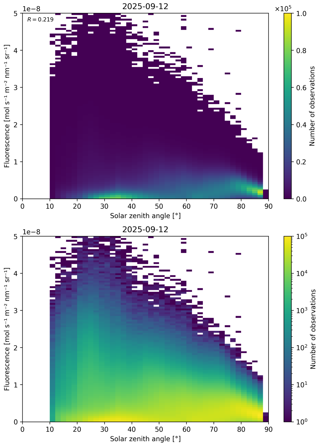
Figure 112: Scatter density plot of “Solar zenith angle” against “Fluorescence” for 2025-09-11 to 2025-09-13.
