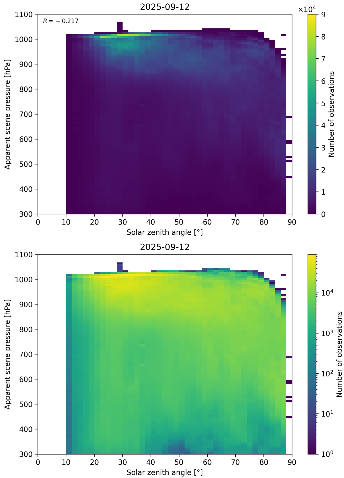
Figure 108: Scatter density plot of “Solar zenith angle” against “Apparent scene pressure” for 2025-09-11 to 2025-09-13.
