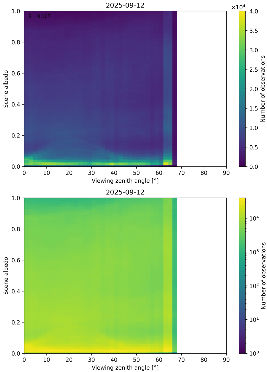
Figure 126: Scatter density plot of “Viewing zenith angle” against “Scene albedo” for 2025-09-11 to 2025-09-13.
