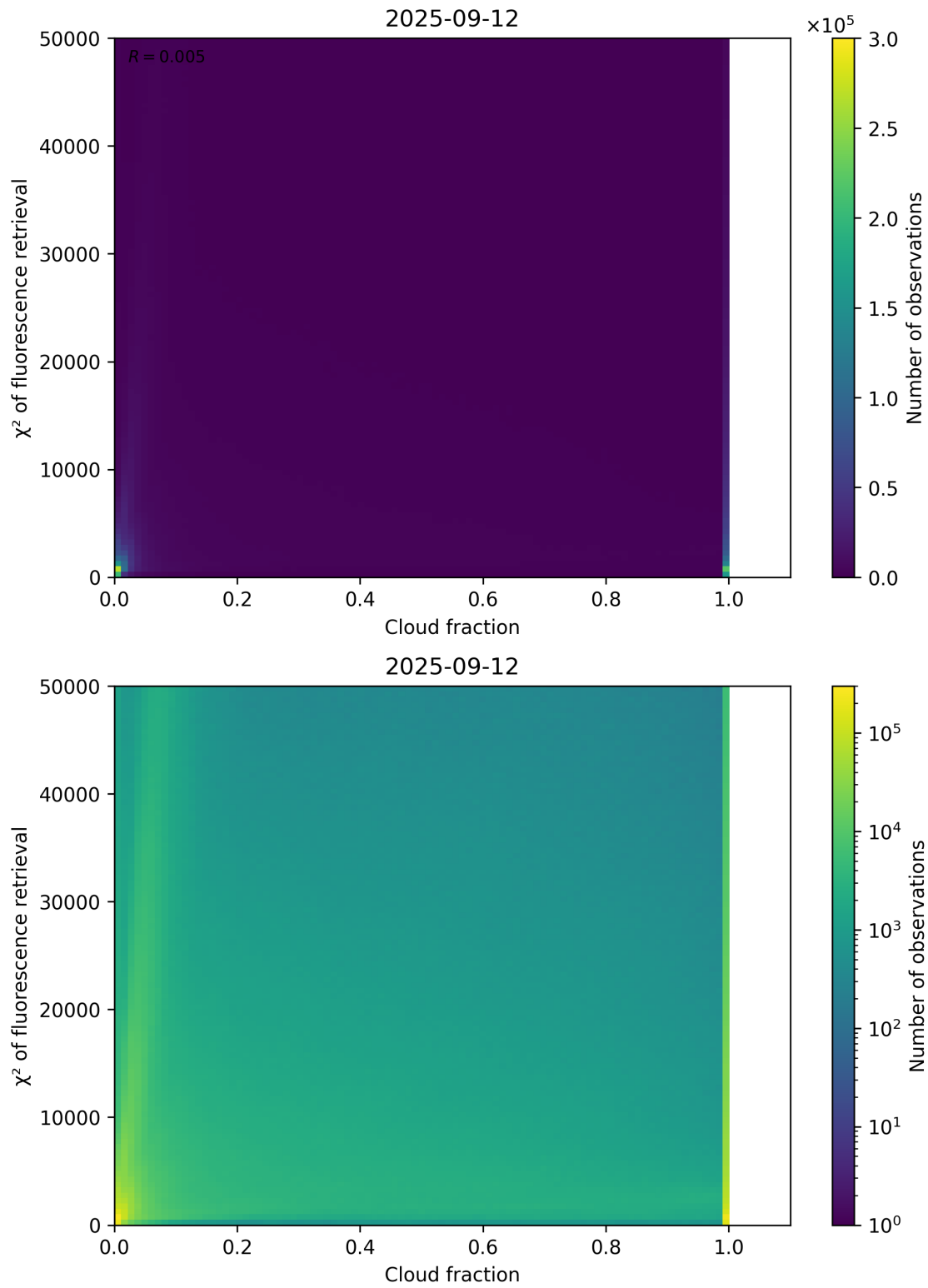
Figure 71: Scatter density plot of “Cloud fraction” against “ \chi^2 of fluorescence retrieval” for 2025-09-11 to 2025-09-13.
