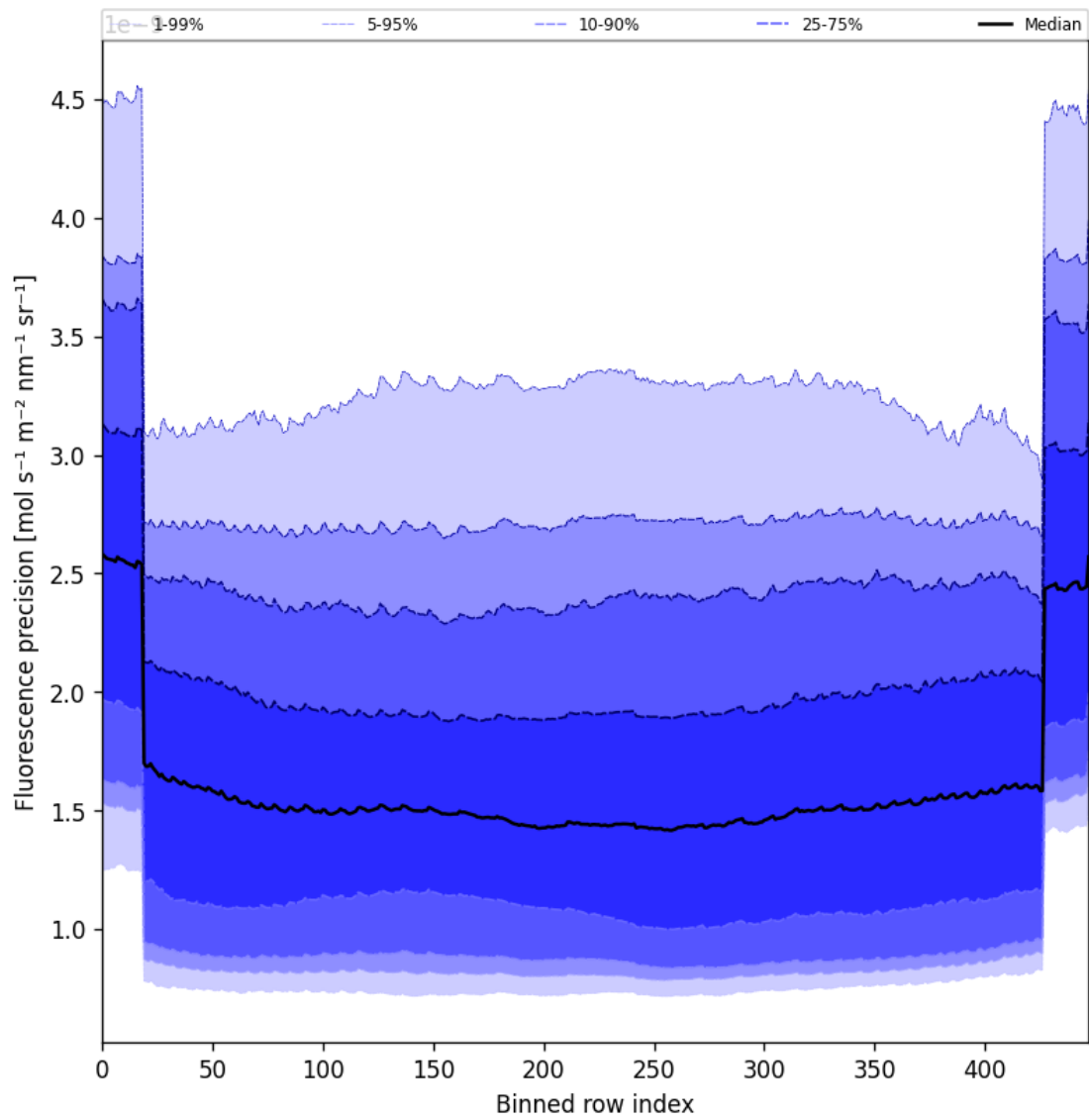
Figure 58: Along track statistics of “Fluorescence precision” for 2025-09-11 to 2025-09-13
