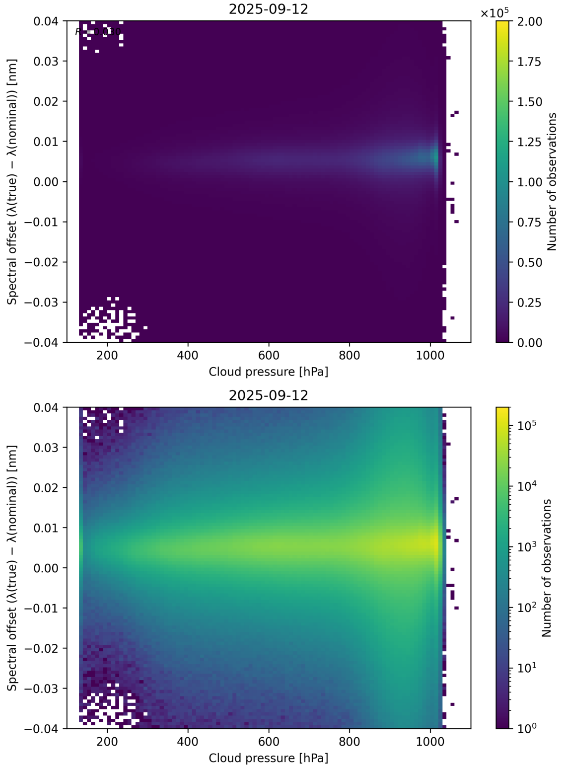
Figure 84: Scatter density plot of “Cloud pressure” against “Spectral offset ( \lambda_{\text{true}} - \lambda_{\text{nominal}} )” for 2025-09-11 to 2025-09-13.
