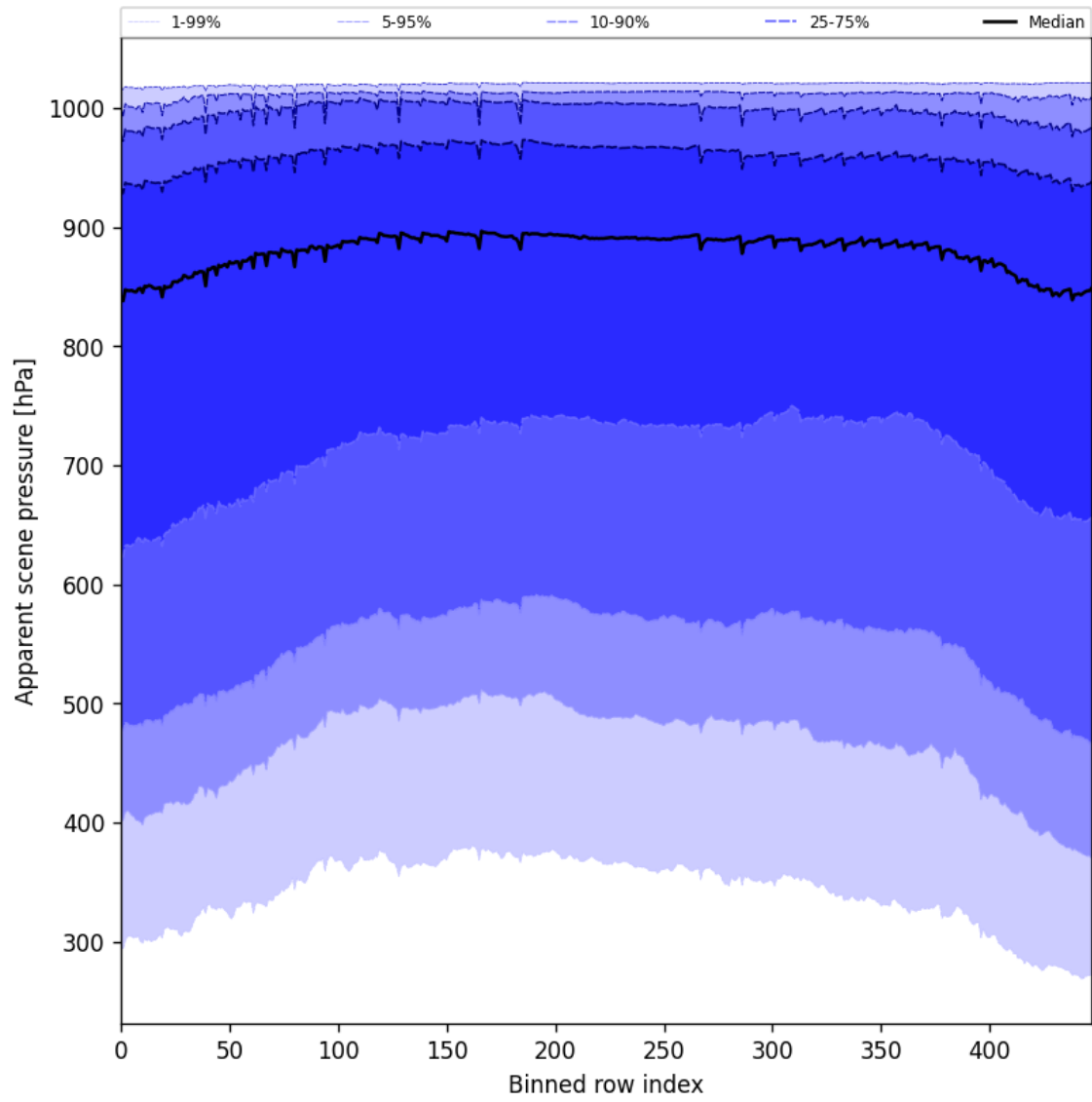
Figure 53: Along track statistics of “Apparent scene pressure” for 2025-09-11 to 2025-09-13
