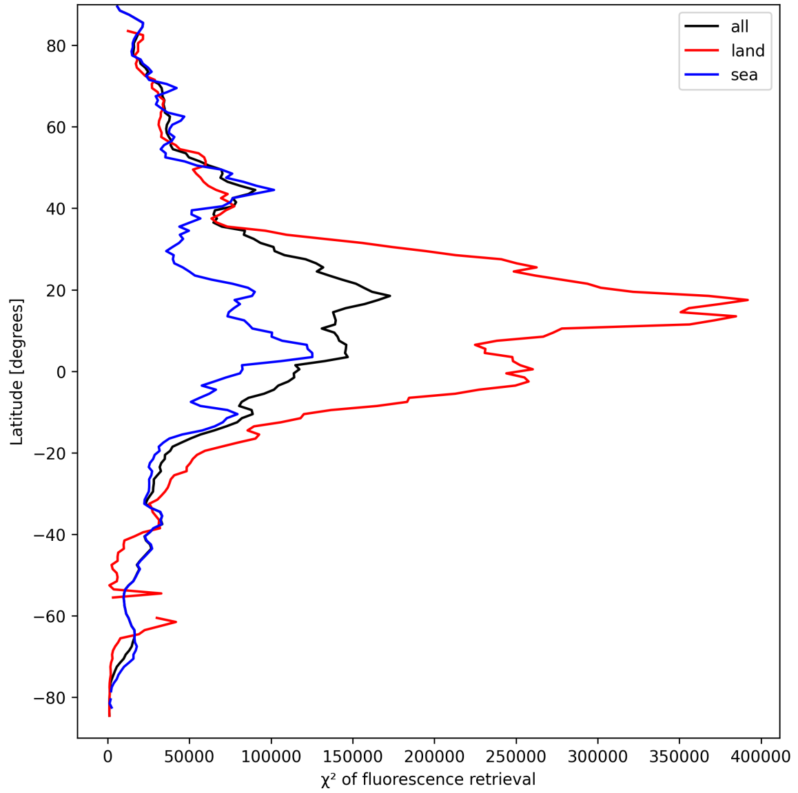
Figure 25: Zonal average of “ \chi^2 of fluorescence retrieval” for 2025-09-11 to 2025-09-13.
