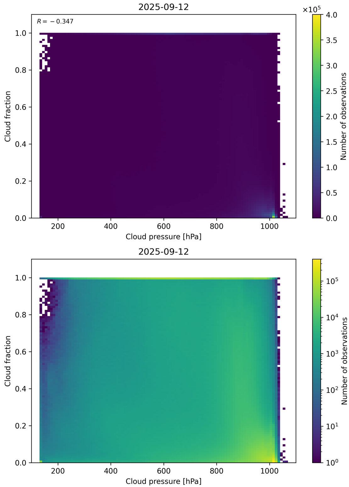
Figure 79: Scatter density plot of “Cloud pressure” against “Cloud fraction” for 2025-09-11 to 2025-09-13.
