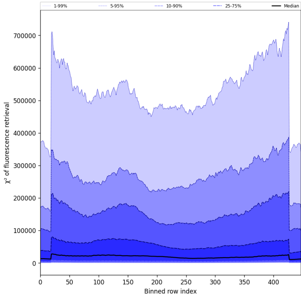
Figure 59: Along track statistics of “ \chi^2 of fluorescence retrieval” for 2025-09-11 to 2025-09-13
