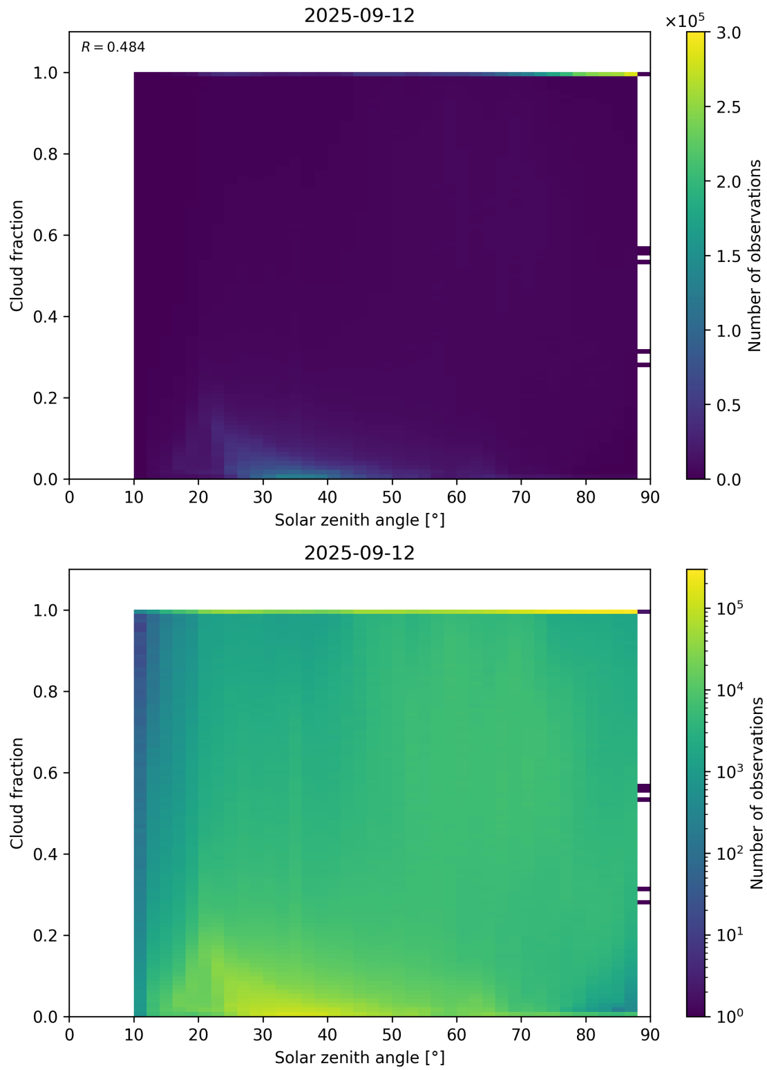
Figure 110: Scatter density plot of “Solar zenith angle” against “Cloud fraction” for 2025-09-11 to 2025-09-13.
