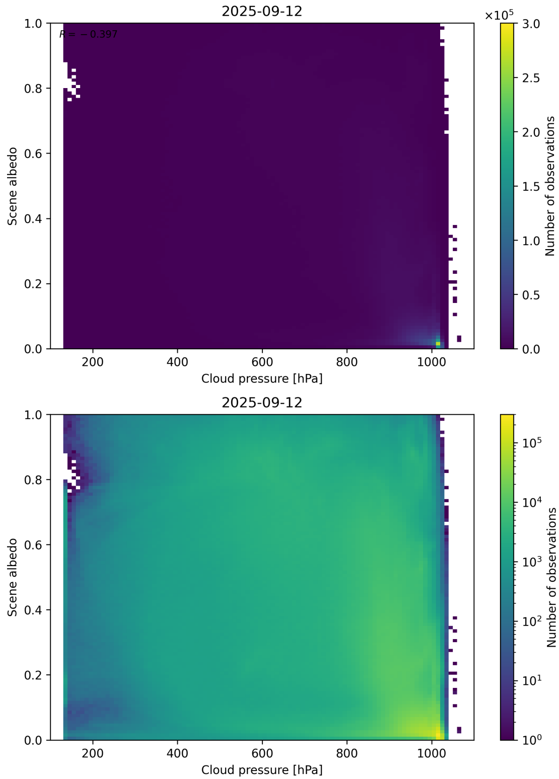
Figure 83: Scatter density plot of “Cloud pressure” against “Scene albedo” for 2025-09-11 to 2025-09-13.
