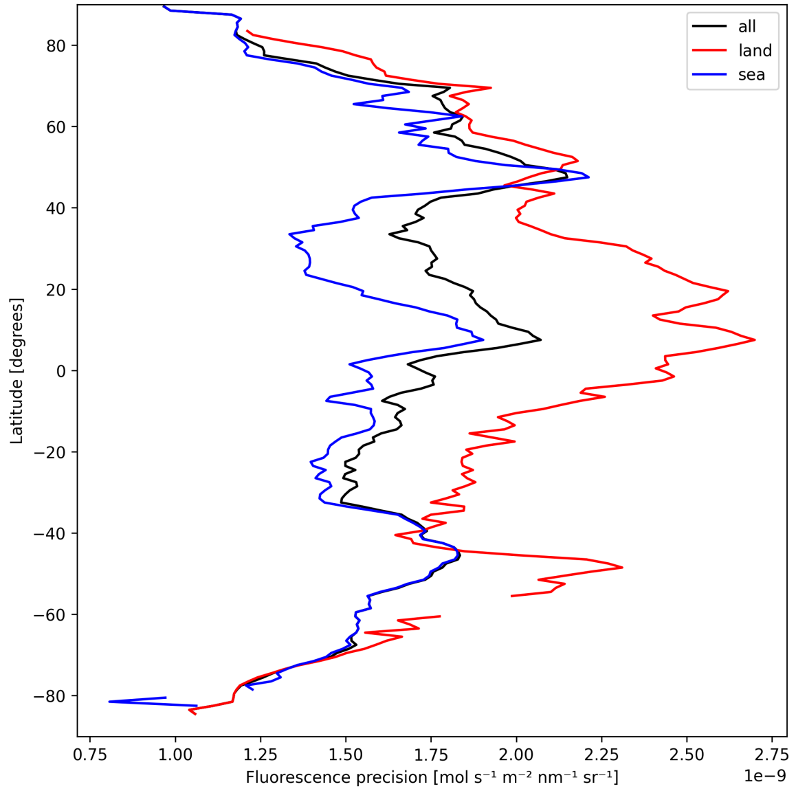
Figure 24: Zonal average of “Fluorescence precision” for 2025-09-11 to 2025-09-13.
