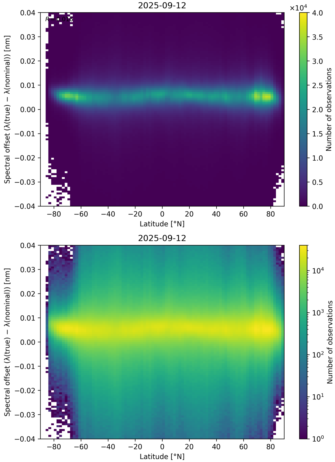
Figure 96: Scatter density plot of “Latitude” against “Spectral offset ( \lambda_{\text{true}} - \lambda_{\text{nominal}} )” for 2025-09-11 to 2025-09-13.
