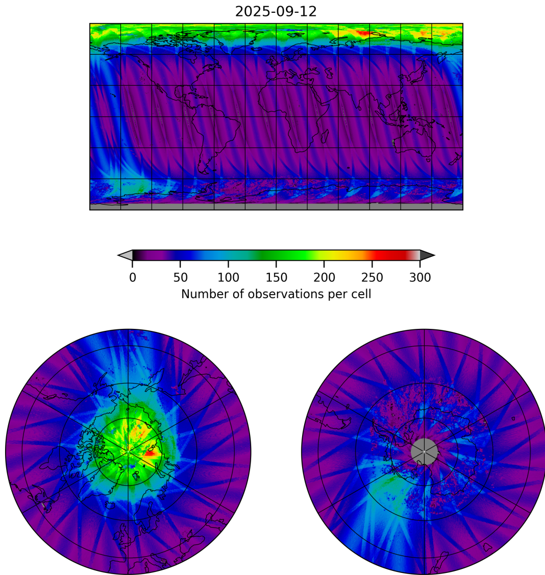
Figure 11: Map of the number of observations for 2025-09-11 to 2025-09-13
