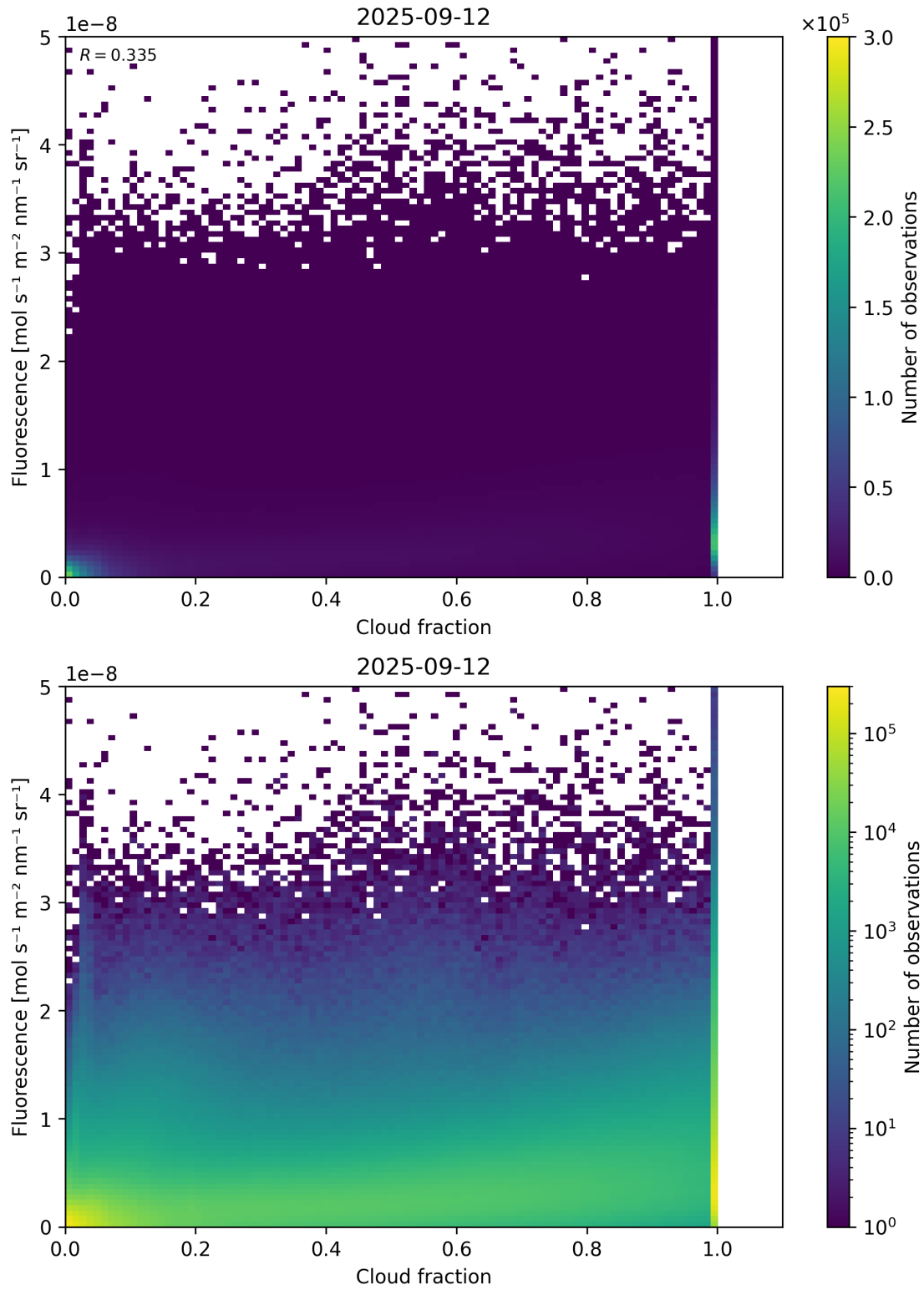
Figure 72: Scatter density plot of “Cloud fraction” against “Fluorescence” for 2025-09-11 to 2025-09-13.
