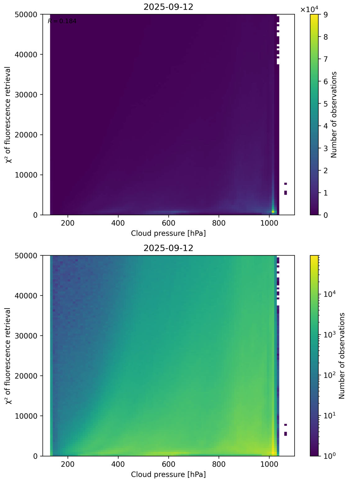
Figure 78: Scatter density plot of “Cloud pressure” against “ \chi^2 of fluorescence retrieval” for 2025-09-11 to 2025-09-13.
