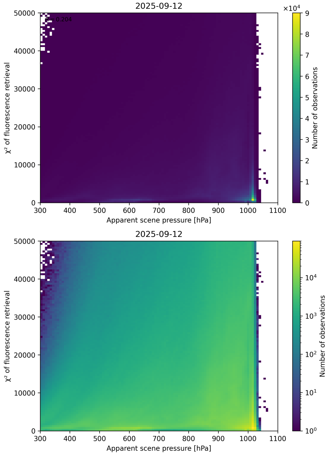
Figure 63: Scatter density plot of “Apparent scene pressure” against “ \chi^2 of fluorescence retrieval” for 2025-09-11 to 2025-09-13.
