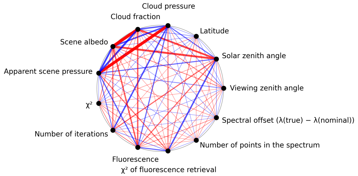
Figure 1: Map of correlation graph for 2025-09-11 to 2025-09-13.
