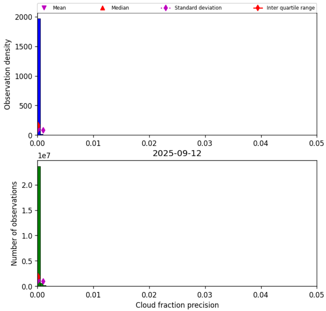
Figure 33: Histogram of “Cloud fraction precision” for 2025-09-11 to 2025-09-13
