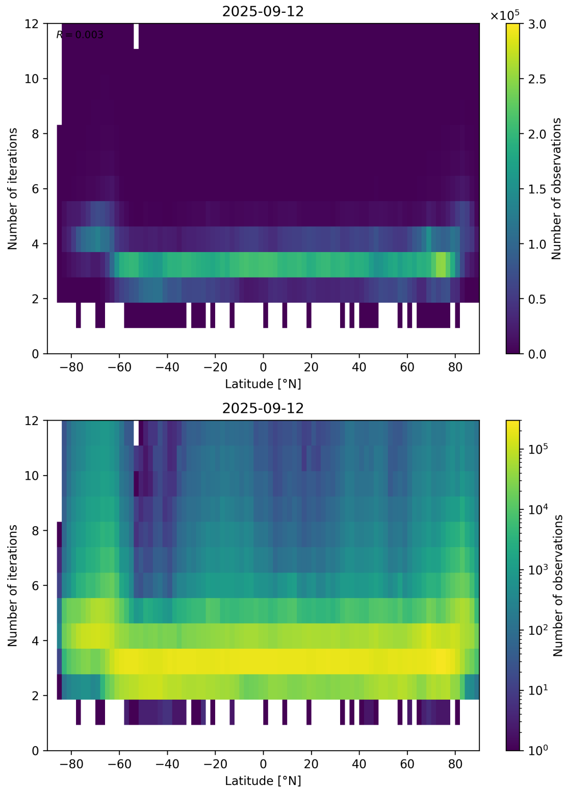
Figure 93: Scatter density plot of “Latitude” against “Number of iterations” for 2025-09-11 to 2025-09-13.
