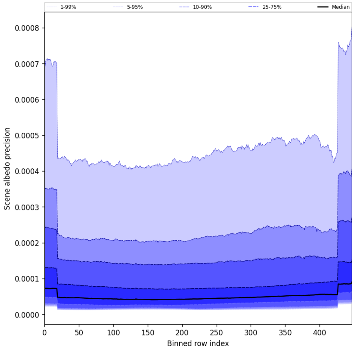
Figure 52: Along track statistics of “Scene albedo precision” for 2025-09-11 to 2025-09-13
