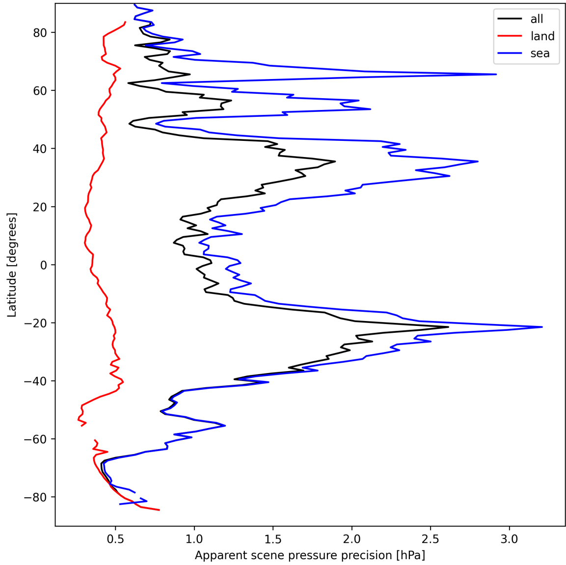
Figure 20: Zonal average of “Apparent scene pressure precision” for 2025-09-11 to 2025-09-13.
