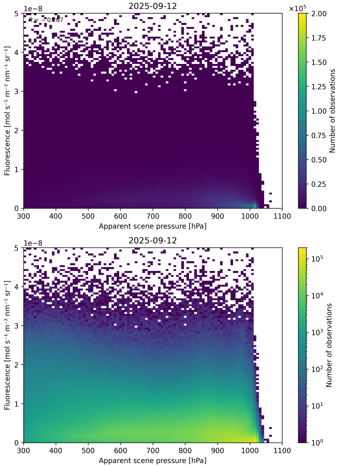
Figure 64: Scatter density plot of “Apparent scene pressure” against “Fluorescence” for 2025-09-11 to 2025-09-13.
