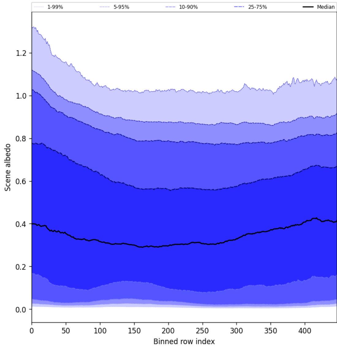
Figure 51: Along track statistics of “Scene albedo” for 2025-09-11 to 2025-09-13
