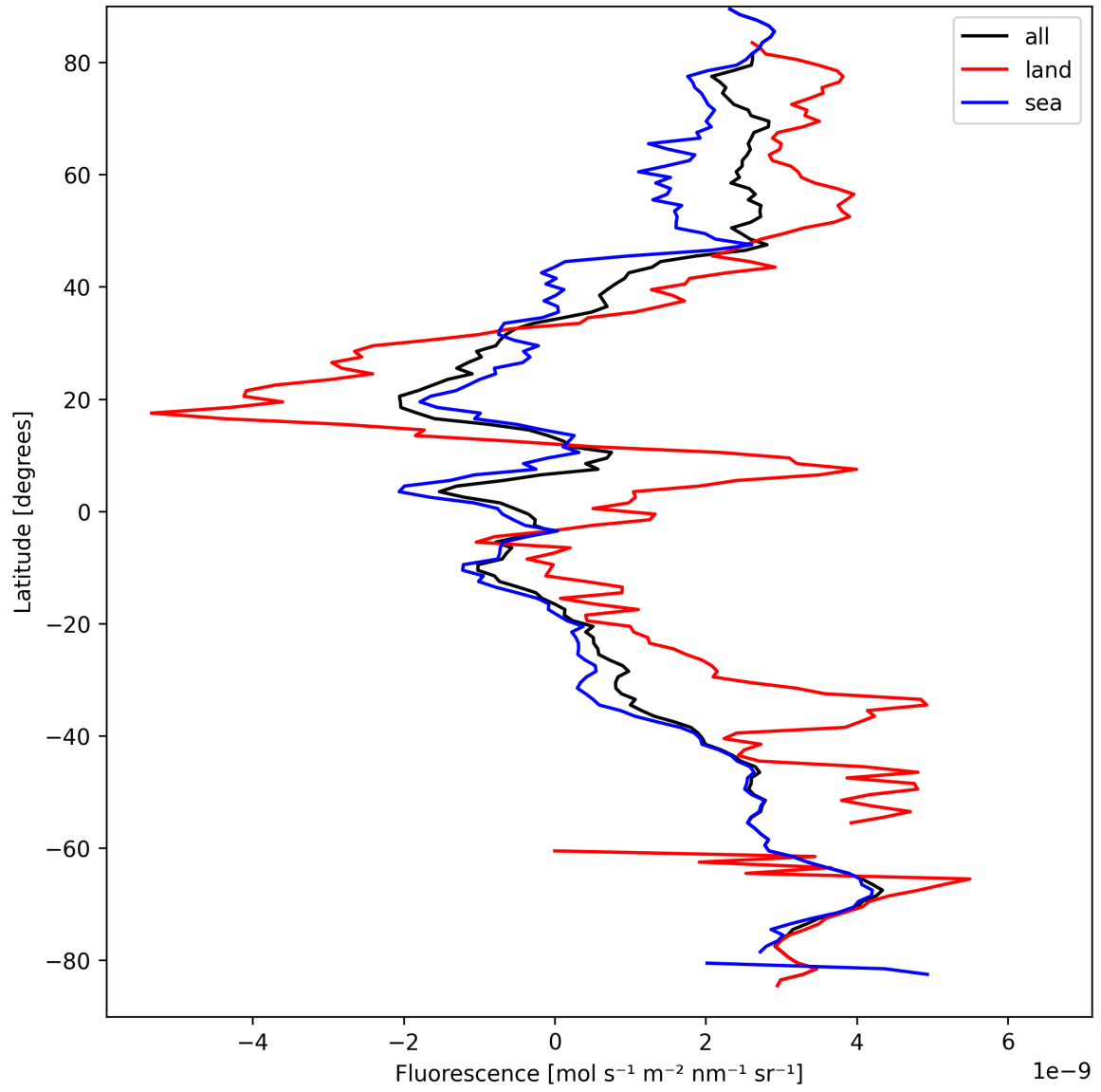
Figure 23: Zonal average of “Fluorescence” for 2025-09-11 to 2025-09-13.
