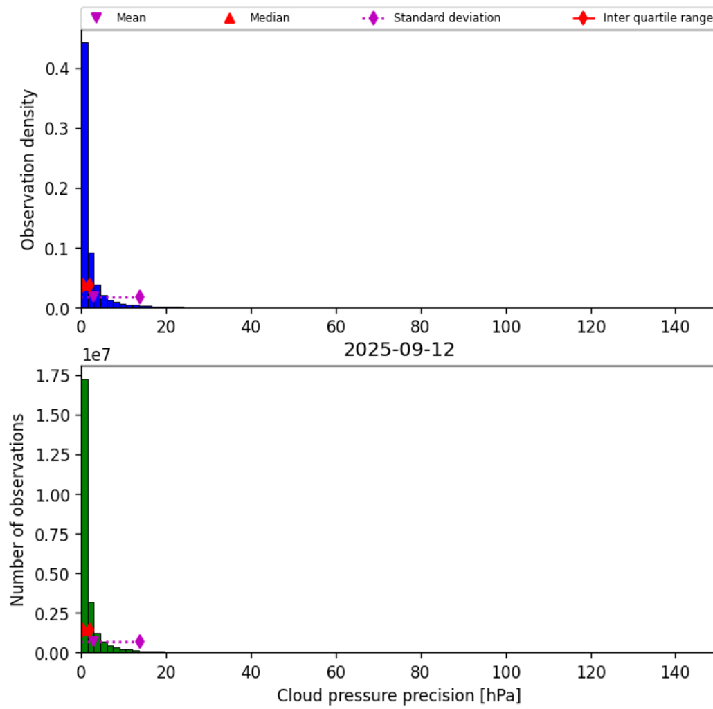
Figure 31: Histogram of “Cloud pressure precision” for 2025-09-11 to 2025-09-13
