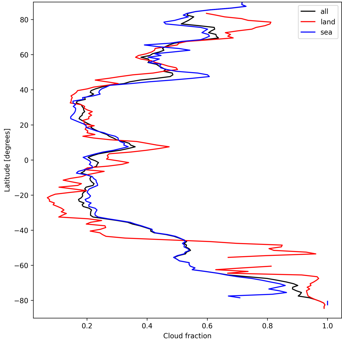
Figure 15: Zonal average of “Cloud fraction” for 2025-09-11 to 2025-09-13.
