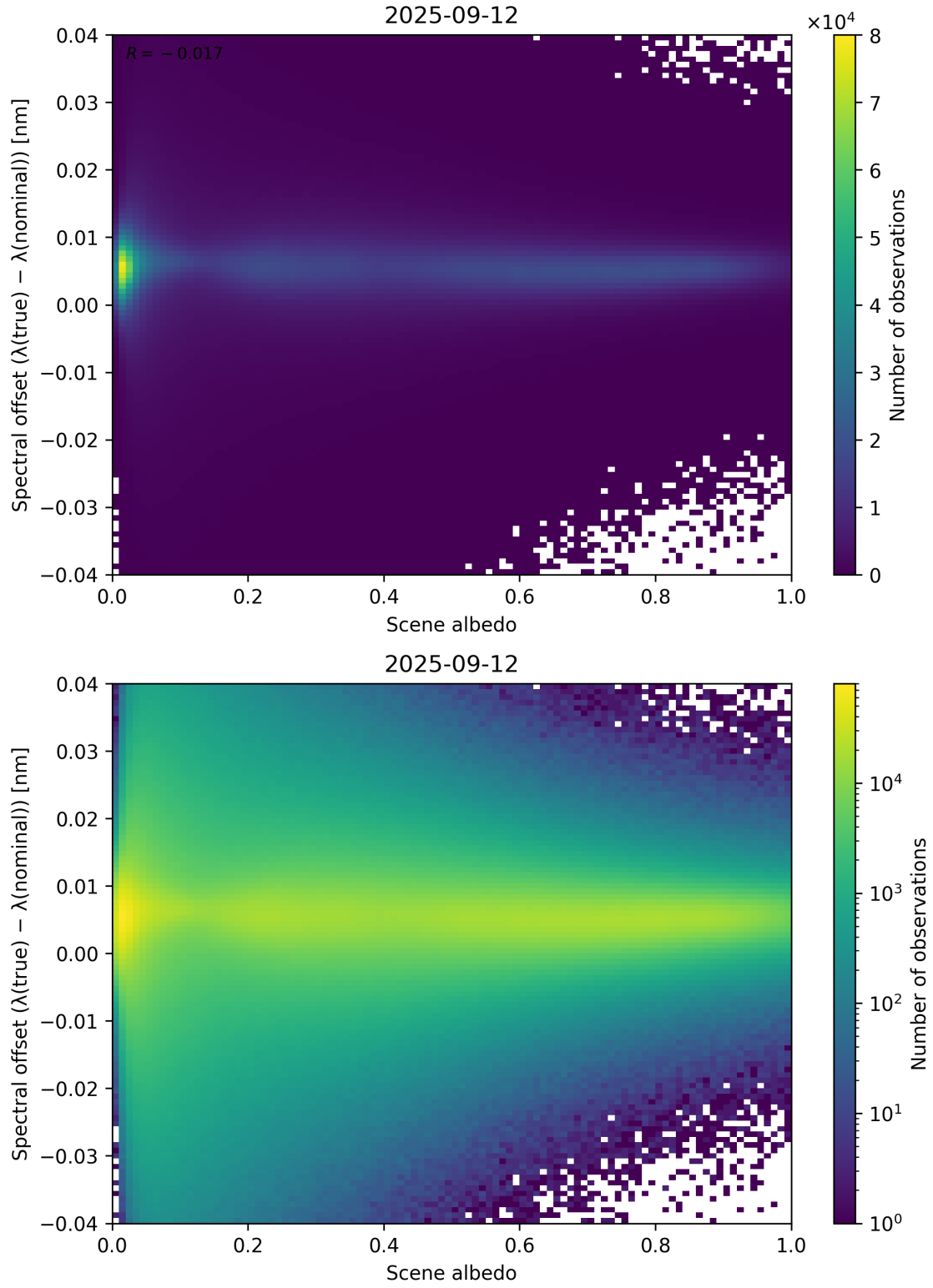
Figure 107: Scatter density plot of “Scene albedo” against “Spectral offset ( \lambda_{\text{true}} - \lambda_{\text{nominal}} )” for 2025-09-11 to 2025-09-13.
