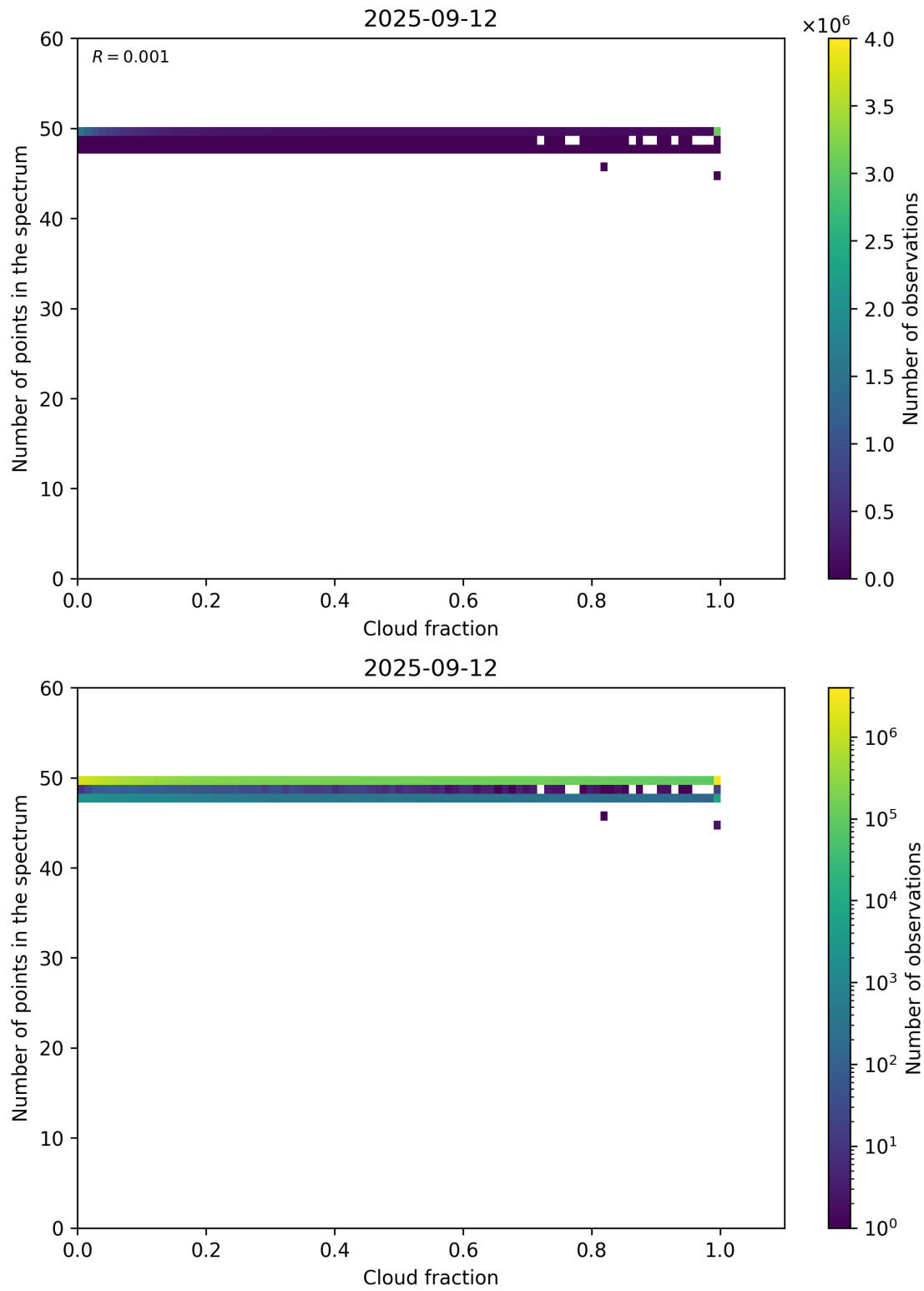
Figure 74: Scatter density plot of “Cloud fraction” against “Number of points in the spectrum” for 2025-09-11 to 2025-09-13.
