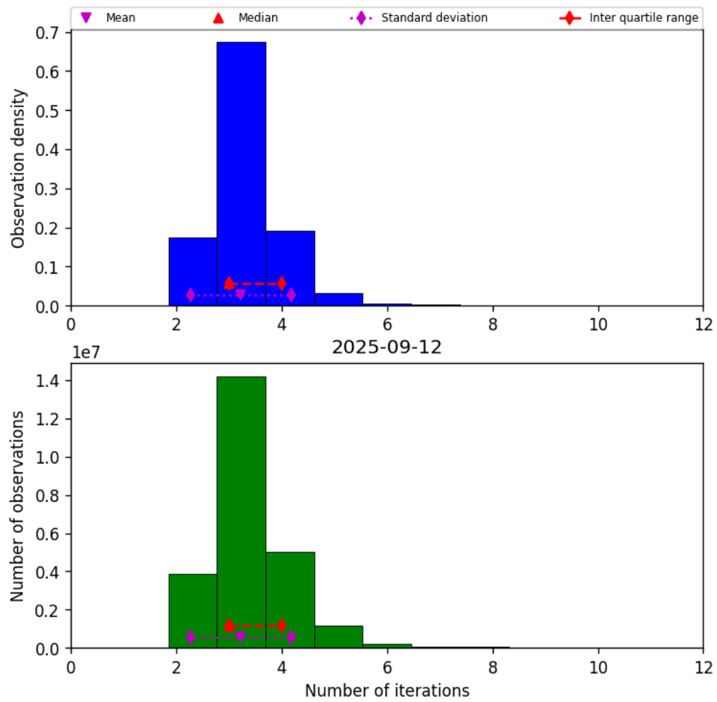
Figure 39: Histogram of “Number of iterations” for 2025-09-11 to 2025-09-13
