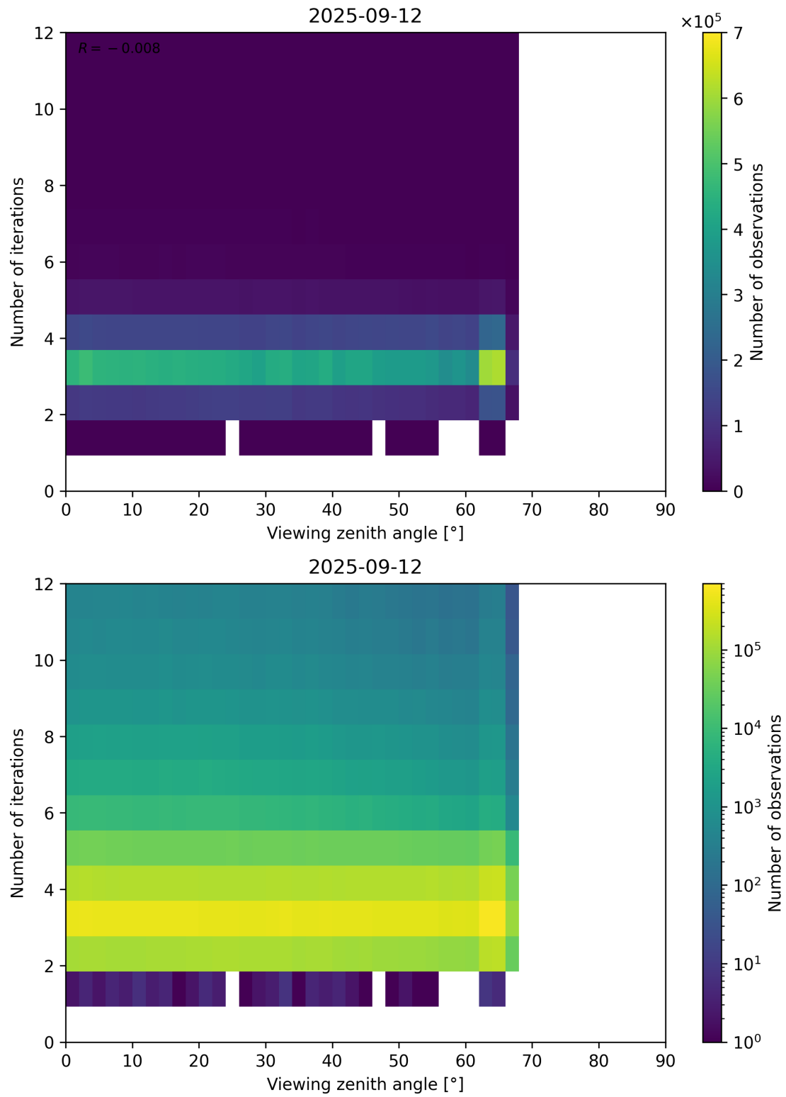
Figure 124: Scatter density plot of “Viewing zenith angle” against “Number of iterations” for 2025-09-11 to 2025-09-13.
