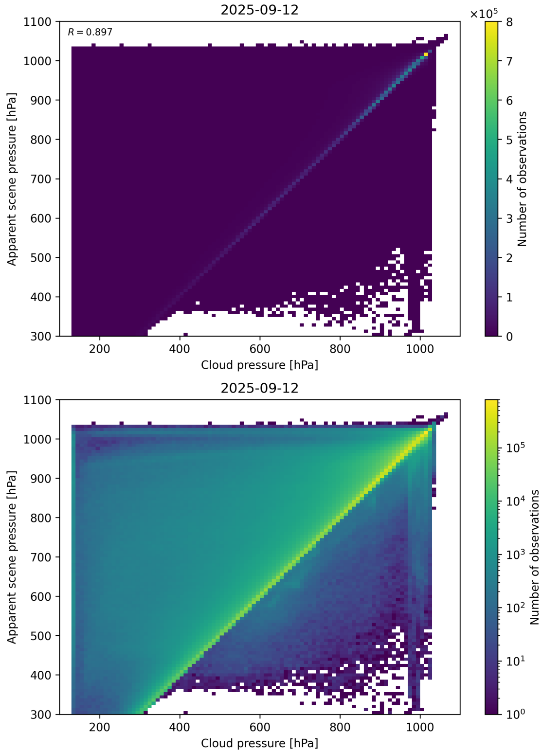
Figure 77: Scatter density plot of “Cloud pressure” against “Apparent scene pressure” for 2025-09-11 to 2025-09-13.
