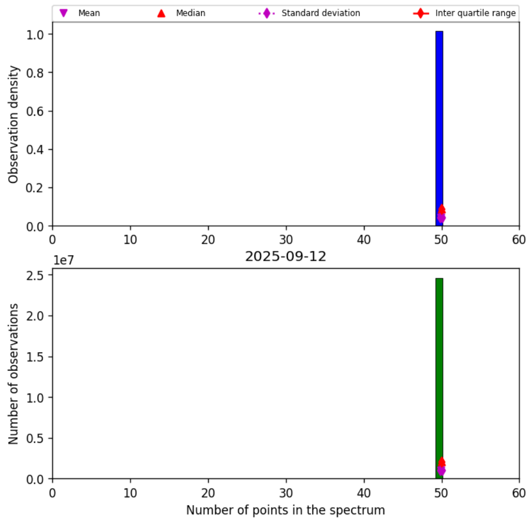
Figure 44: Histogram of "Number of points in the spectrum" for 2025-09-11 to 2025-09-13
