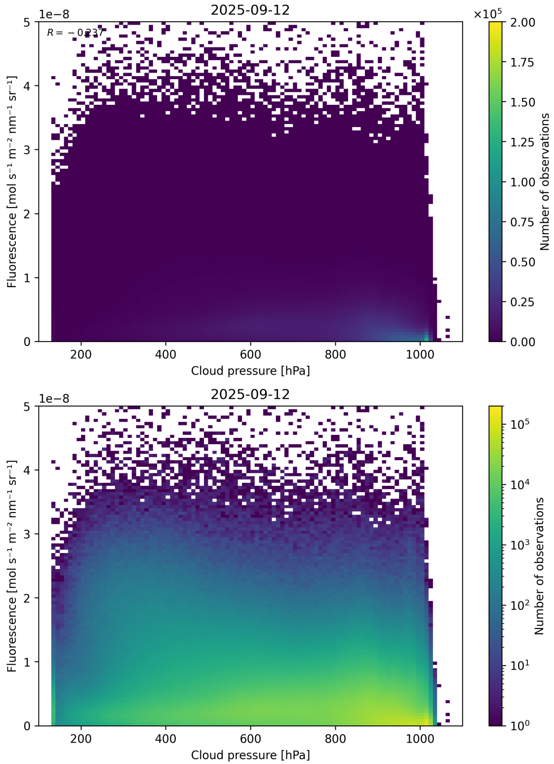
Figure 80: Scatter density plot of “Cloud pressure” against “Fluorescence” for 2025-09-11 to 2025-09-13.
