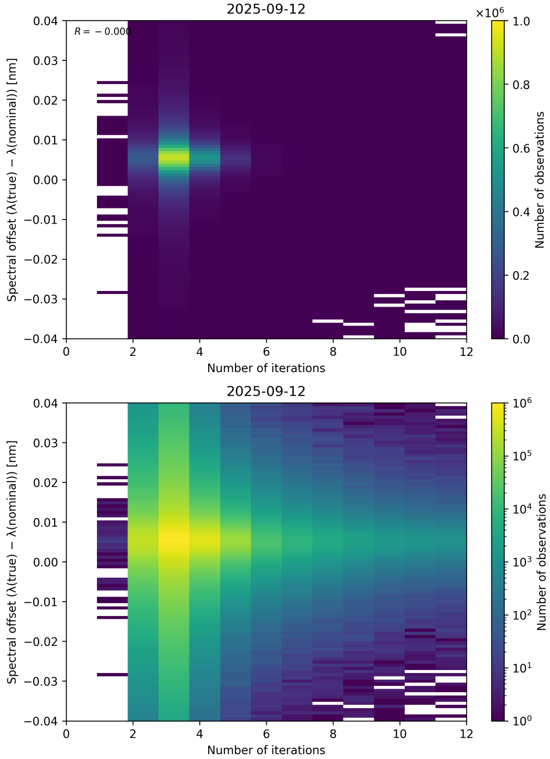
Figure 100: Scatter density plot of “Number of iterations” against “Spectral offset ( \lambda_{\text{true}} - \lambda_{\text{nominal}} )” for 2025-09-11 to 2025-09-13.
