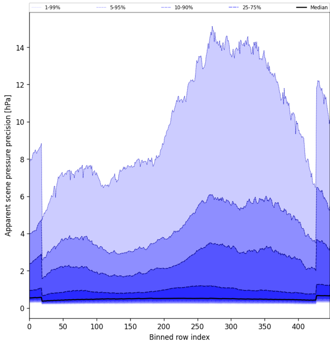
Figure 54: Along track statistics of “Apparent scene pressure precision” for 2025-09-11 to 2025-09-13
