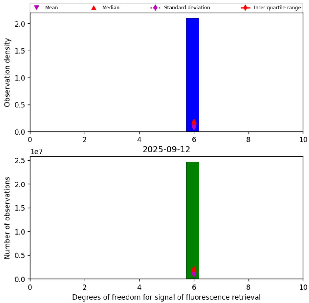
Figure 43: Histogram of “Degrees of freedom for signal of fluorescence retrieval” for 2025-09-11 to 2025-09-13
