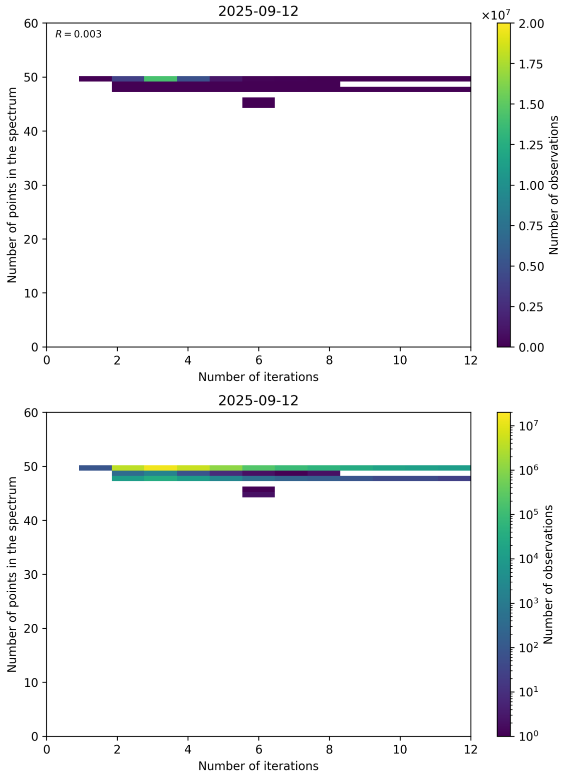
Figure 99: Scatter density plot of “Number of iterations” against “Number of points in the spectrum” for 2025-09-11 to 2025-09-13.
