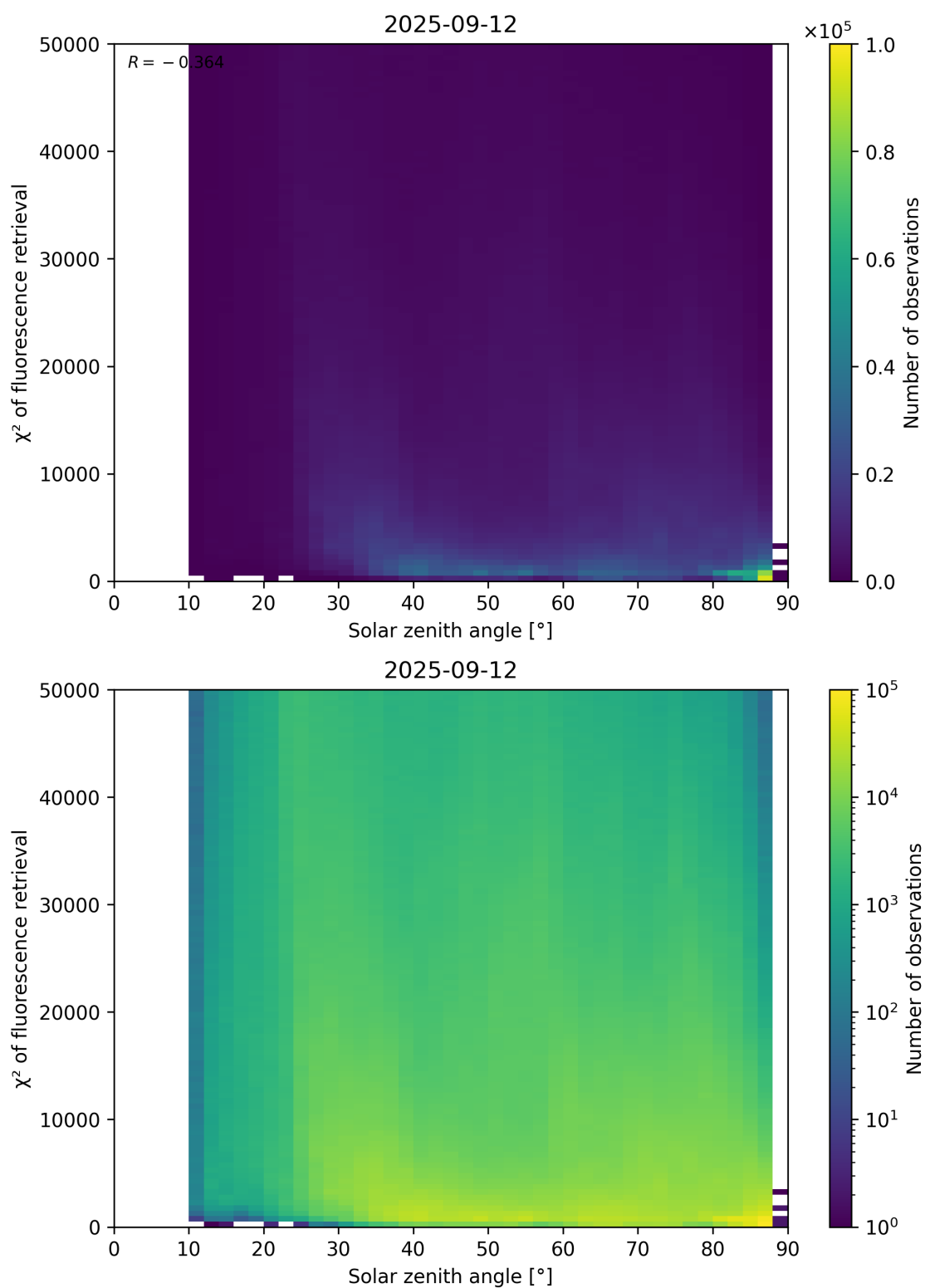
Figure 109: Scatter density plot of “Solar zenith angle” against “ \chi^2 of fluorescence retrieval” for 2025-09-11 to 2025-09-13.
