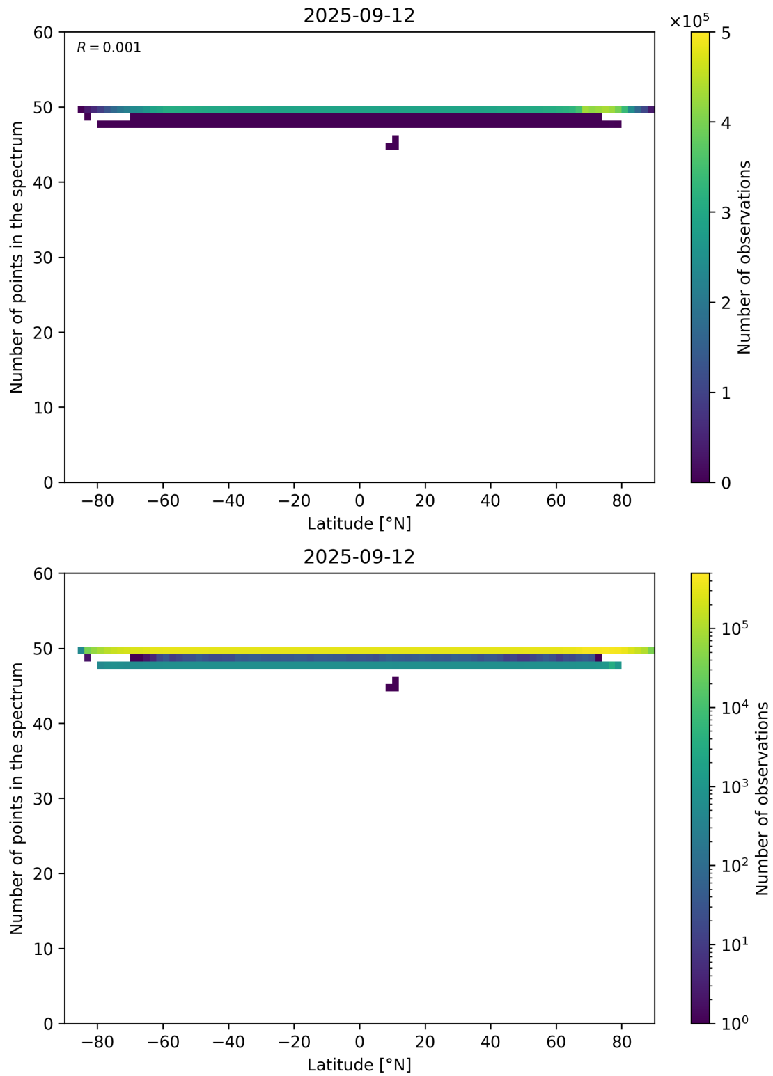
Figure 94: Scatter density plot of “Latitude” against “Number of points in the spectrum” for 2025-09-11 to 2025-09-13.
