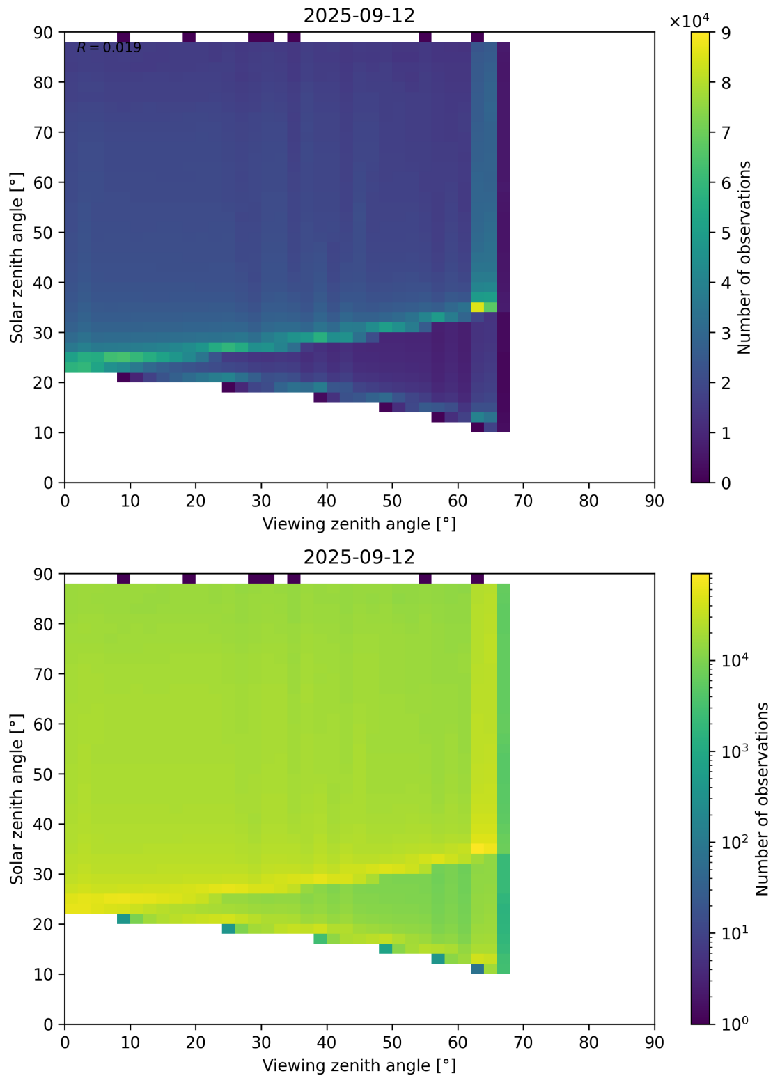
Figure 127: Scatter density plot of “Viewing zenith angle” against “Solar zenith angle” for 2025-09-11 to 2025-09-13.
