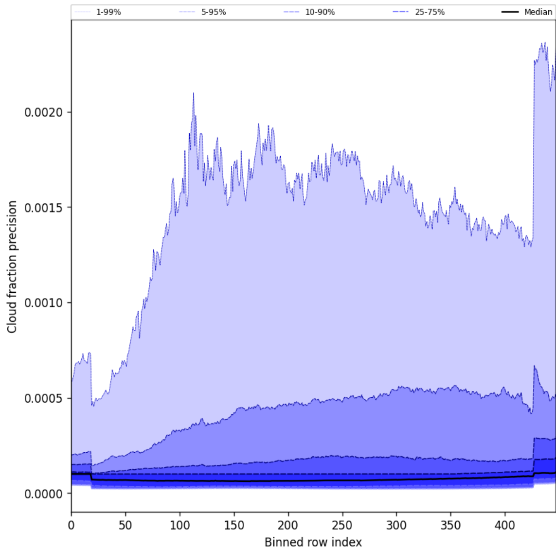
Figure 50: Along track statistics of “Cloud fraction precision” for 2025-09-11 to 2025-09-13
