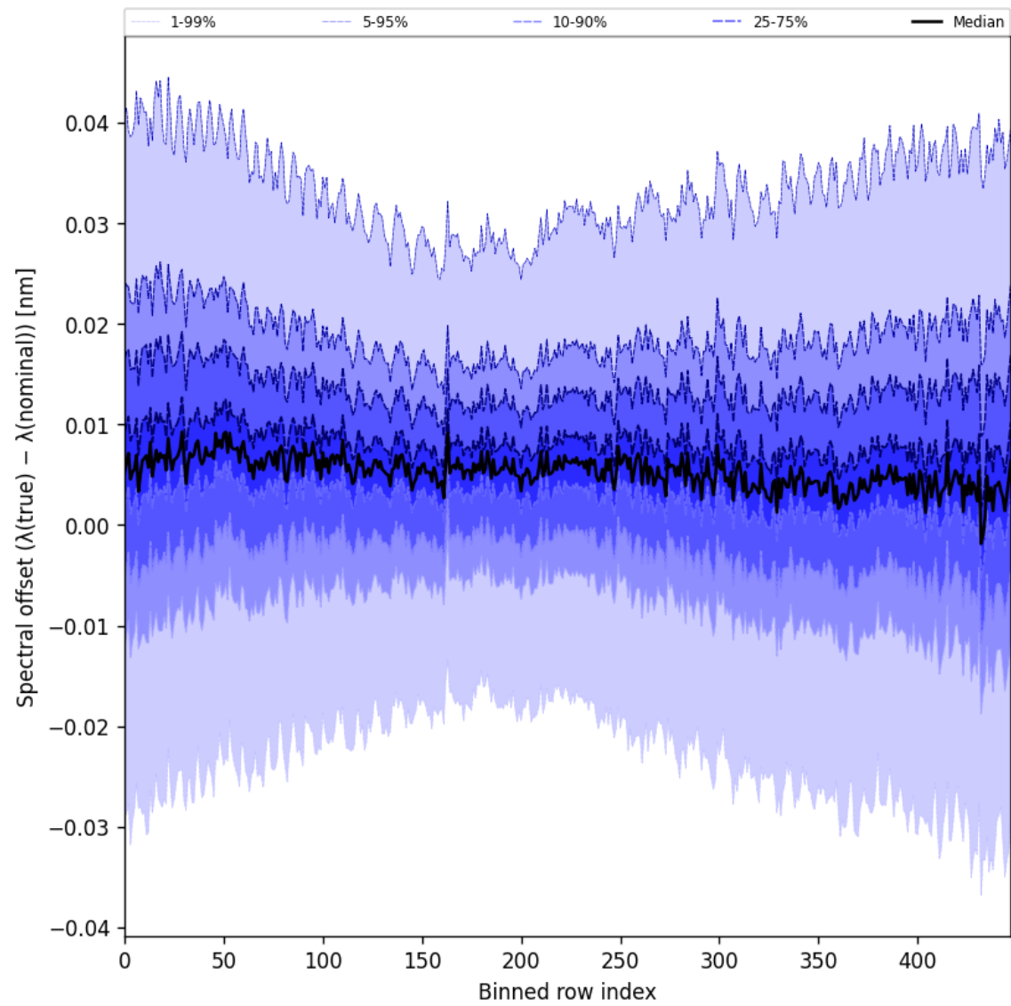
Figure 62: Along track statistics of “Spectral offset ( \lambda_{\text{true}} - \lambda_{\text{nominal}} )” for 2025-09-11 to 2025-09-13
