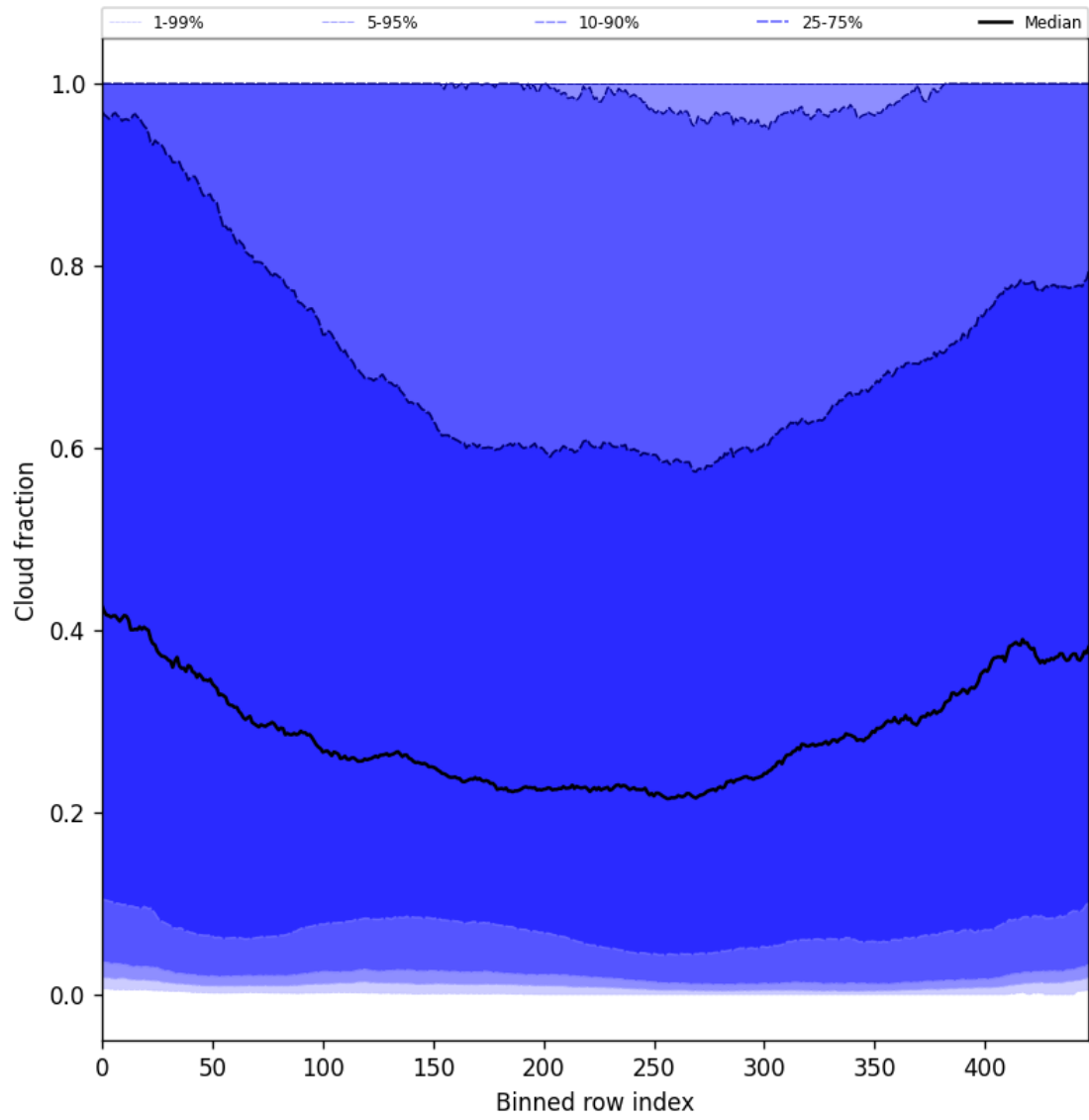
Figure 49: Along track statistics of “Cloud fraction” for 2025-09-11 to 2025-09-13
