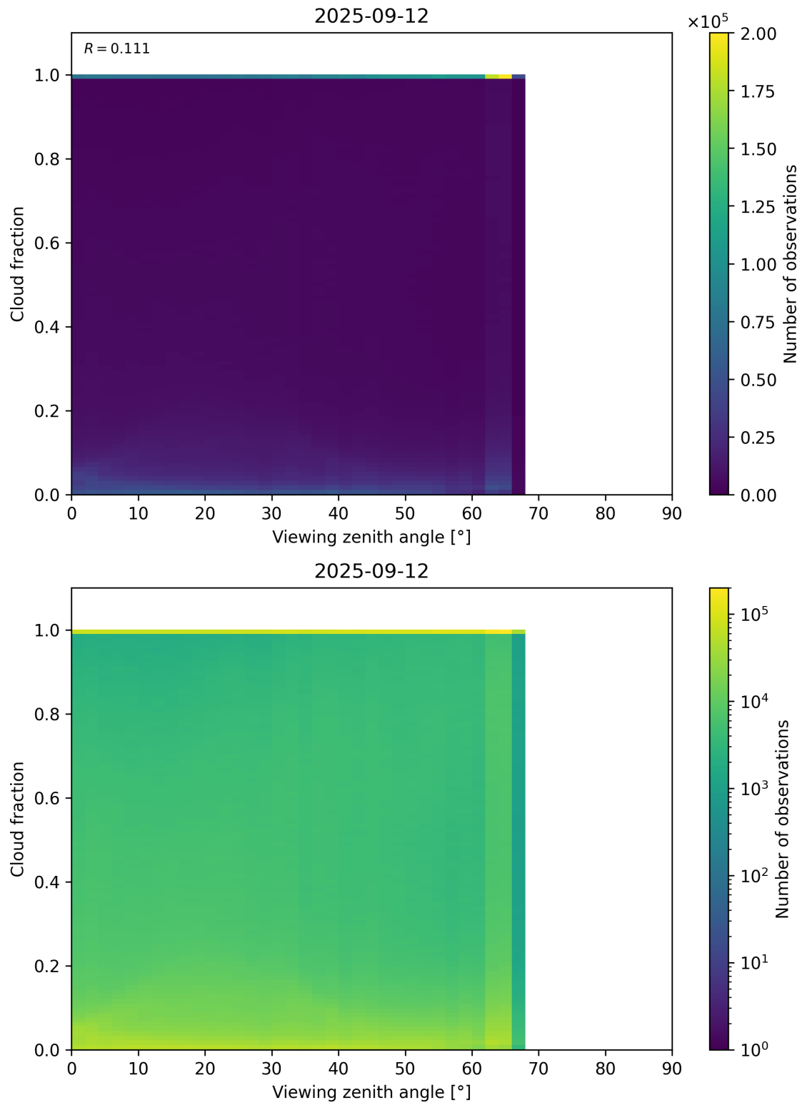
Figure 120: Scatter density plot of “Viewing zenith angle” against “Cloud fraction” for 2025-09-11 to 2025-09-13.
