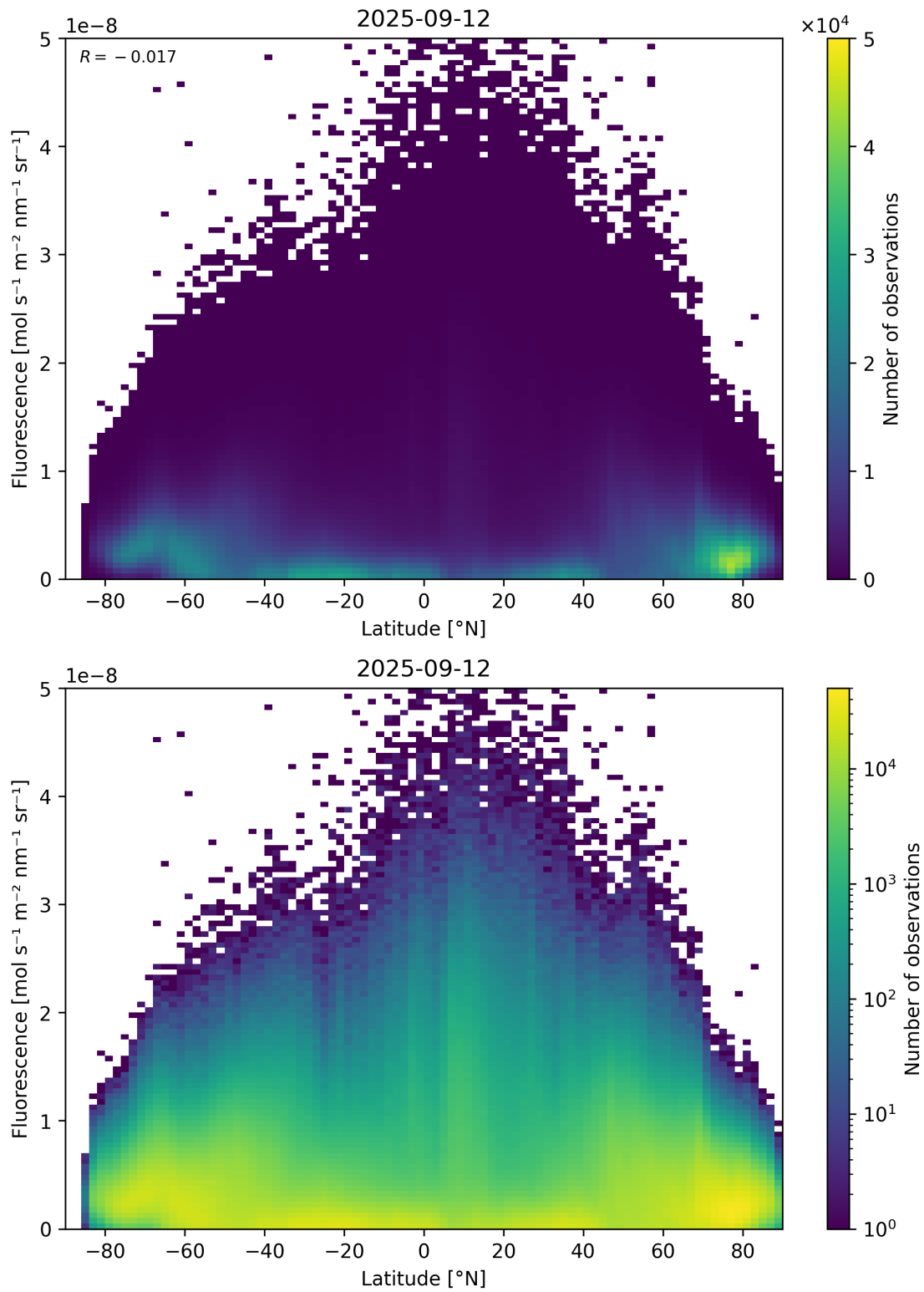
Figure 92: Scatter density plot of “Latitude” against “Fluorescence” for 2025-09-11 to 2025-09-13.
