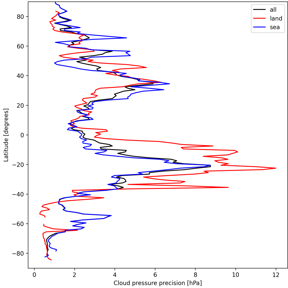
Figure 14: Zonal average of “Cloud pressure precision” for 2025-09-11 to 2025-09-13.
