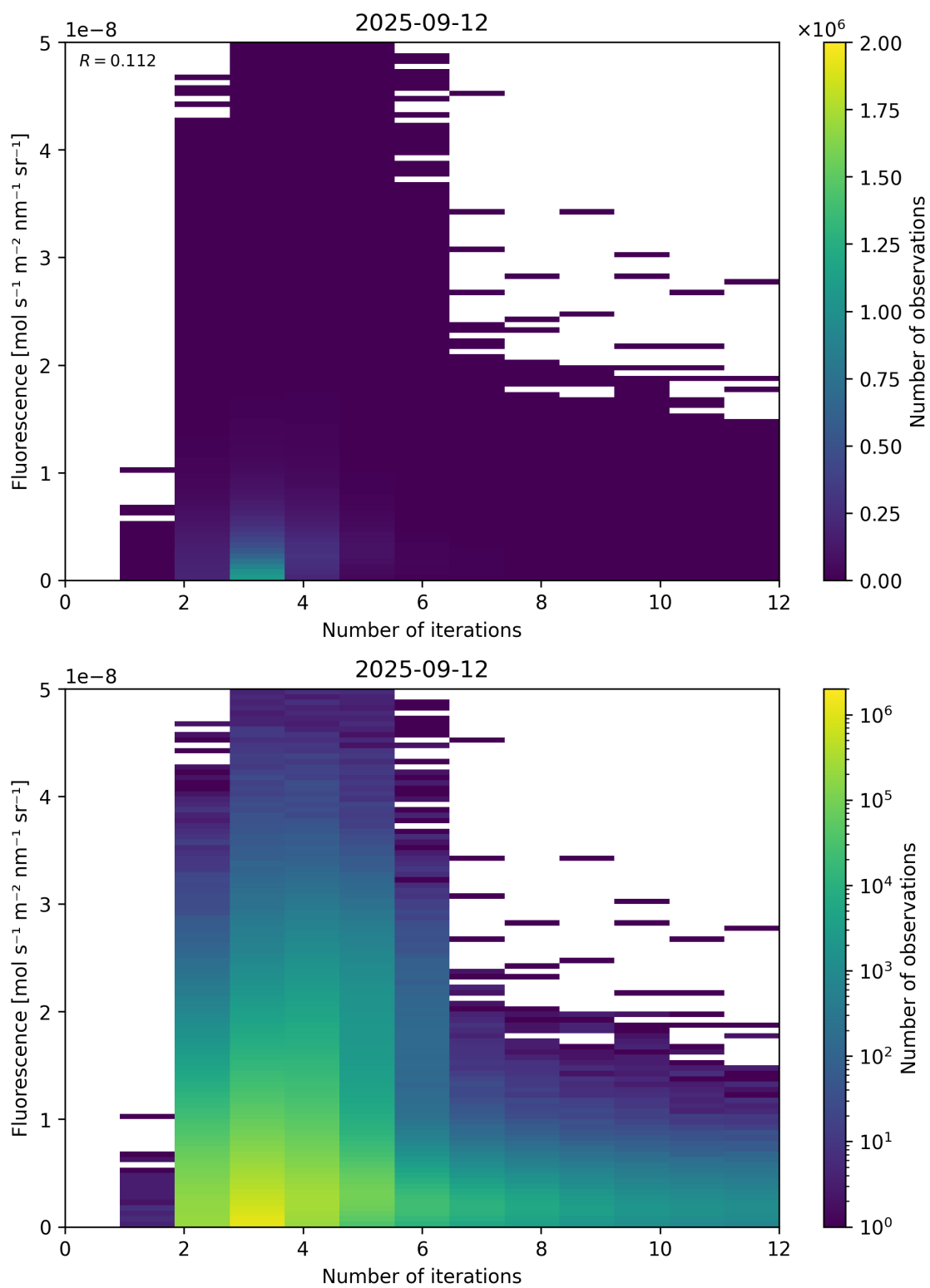
Figure 98: Scatter density plot of “Number of iterations” against “Fluorescence” for 2025-09-11 to 2025-09-13.
