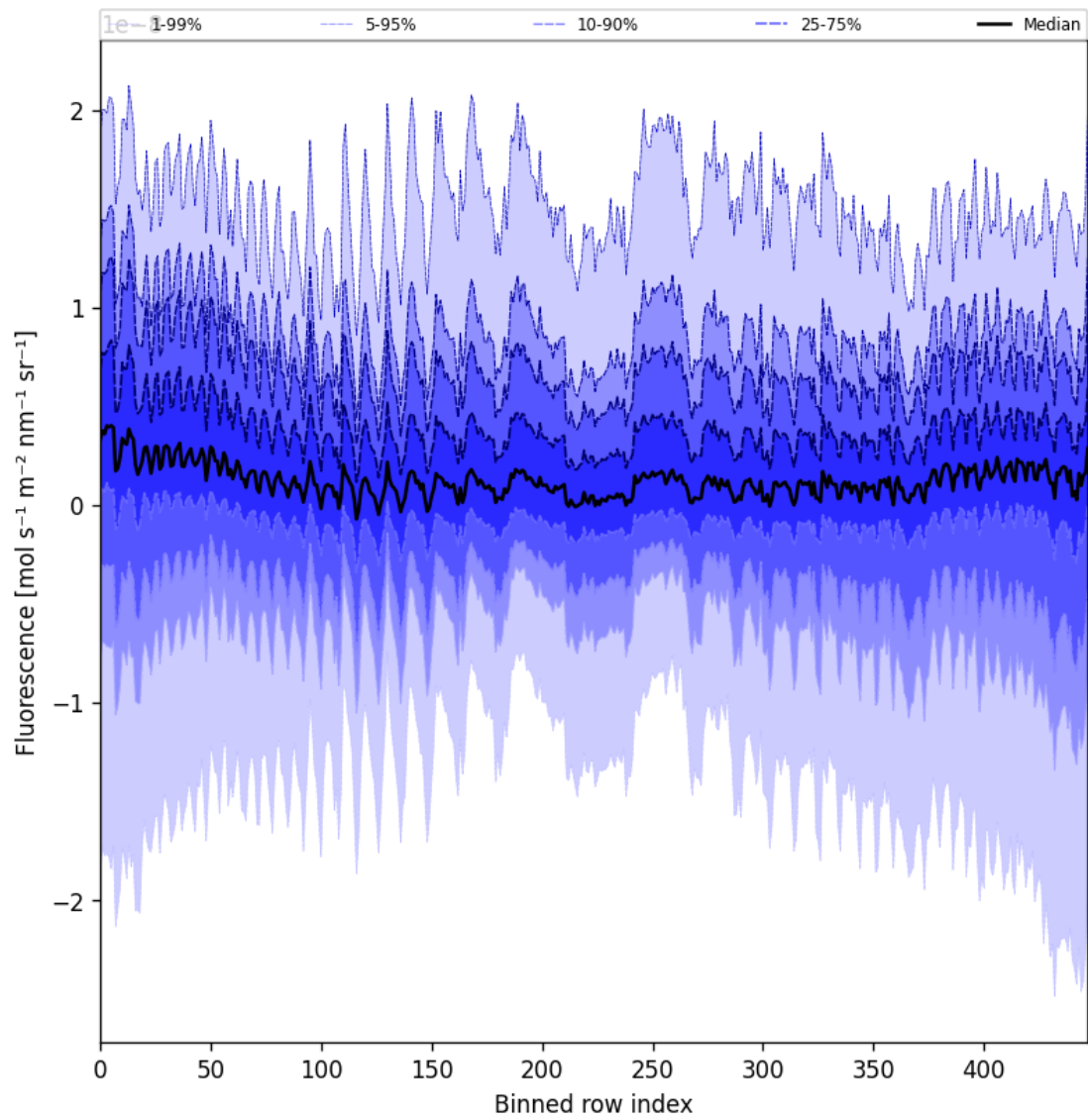
Figure 57: Along track statistics of “Fluorescence” for 2025-09-11 to 2025-09-13
