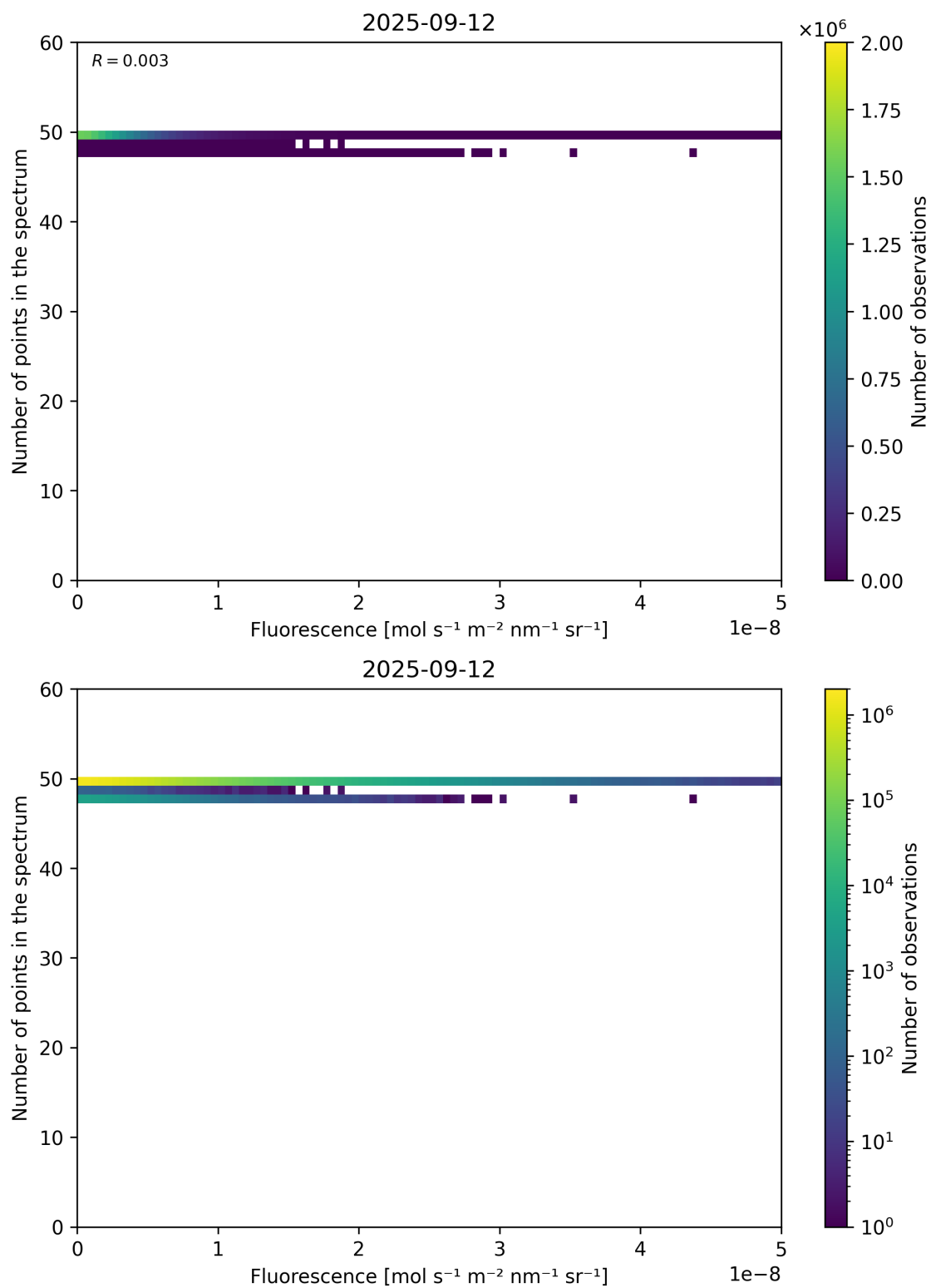
Figure 86: Scatter density plot of “Fluorescence” against “Number of points in the spectrum” for 2025-09-11 to 2025-09-13.
