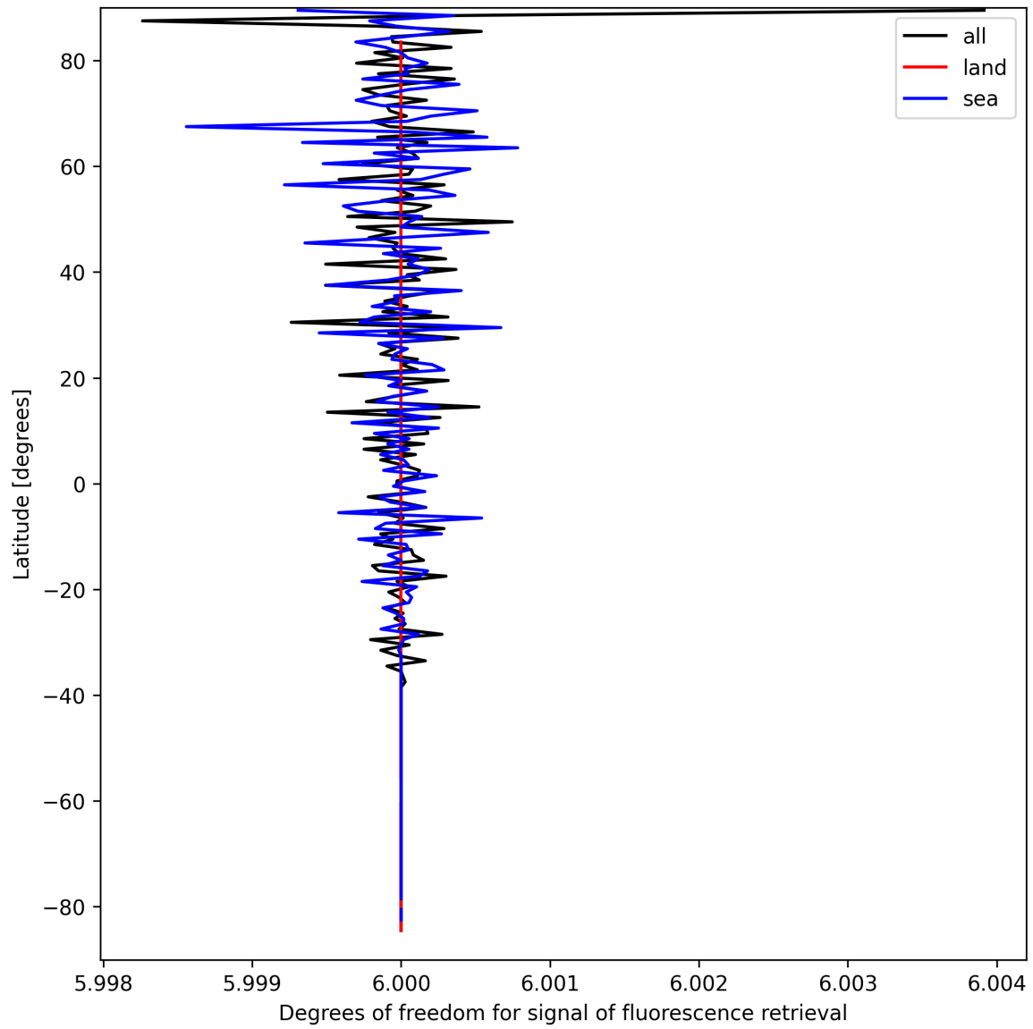
Figure 26: Zonal average of “Degrees of freedom for signal of fluorescence retrieval” for 2025-09-11 to 2025-09-13.
