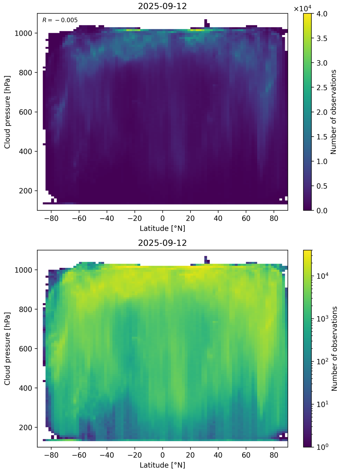
Figure 91: Scatter density plot of “Latitude” against “Cloud pressure” for 2025-09-11 to 2025-09-13.
