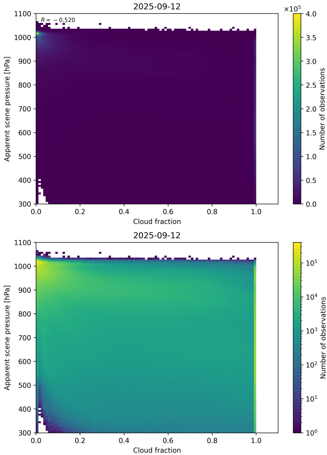
Figure 70: Scatter density plot of “Cloud fraction” against “Apparent scene pressure” for 2025-09-11 to 2025-09-13.
