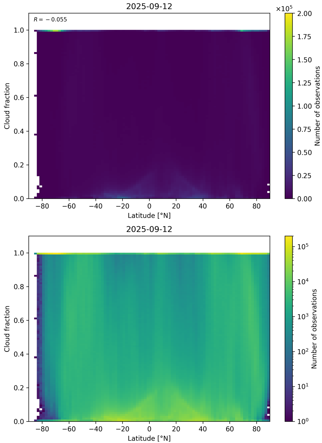
Figure 90: Scatter density plot of “Latitude” against “Cloud fraction” for 2025-09-11 to 2025-09-13.
