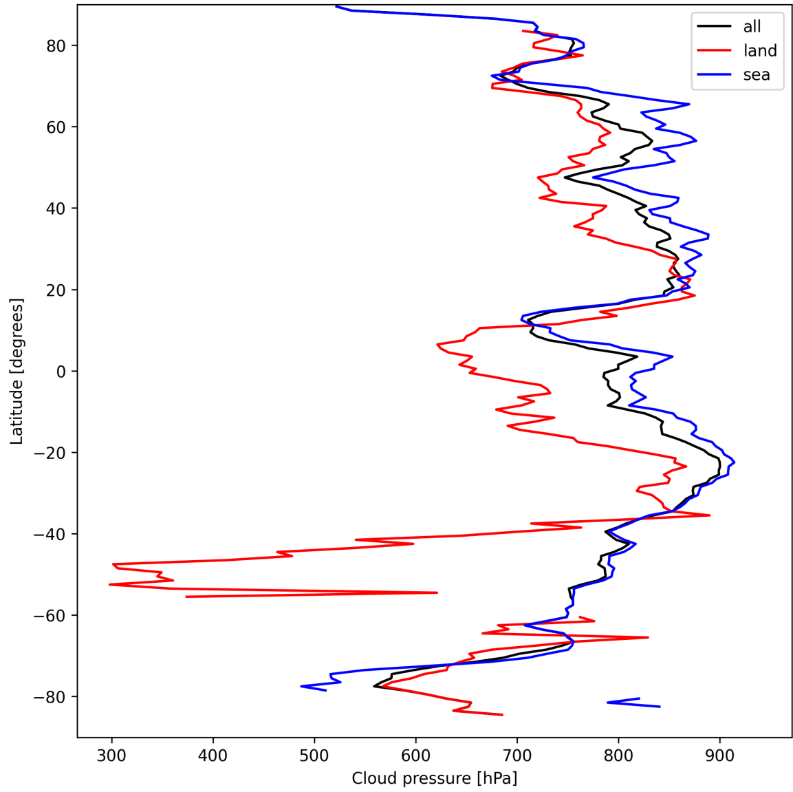
Figure 13: Zonal average of “Cloud pressure” for 2025-09-11 to 2025-09-13.
