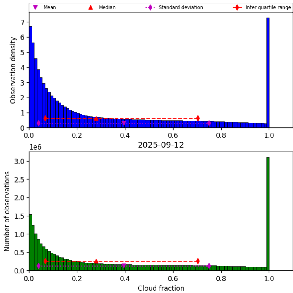
Figure 32: Histogram of “Cloud fraction” for 2025-09-11 to 2025-09-13
