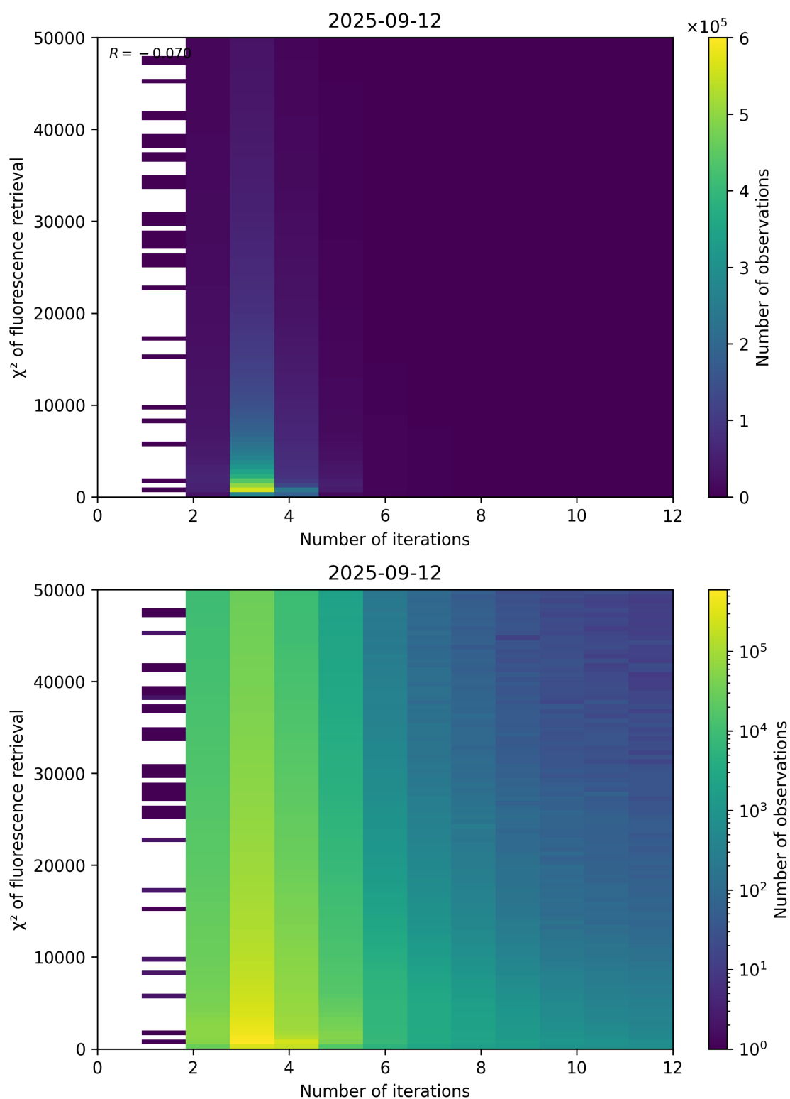
Figure 97: Scatter density plot of “Number of iterations” against “ \chi^2 of fluorescence retrieval” for 2025-09-11 to 2025-09-13.
