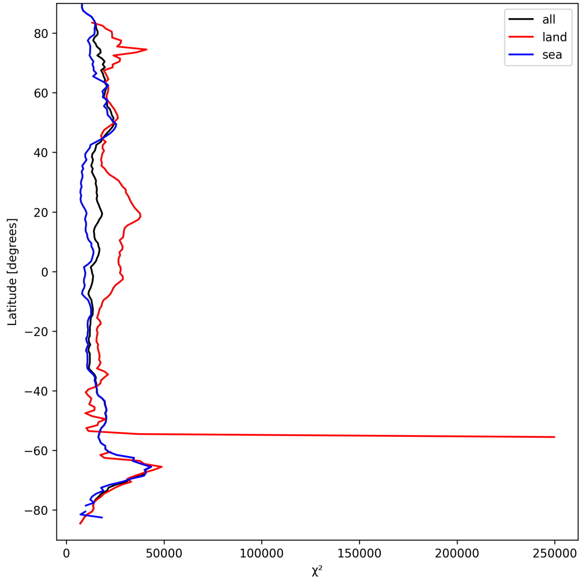
Figure 21: Zonal average of “ \chi^2 ” for 2025-09-11 to 2025-09-13.
