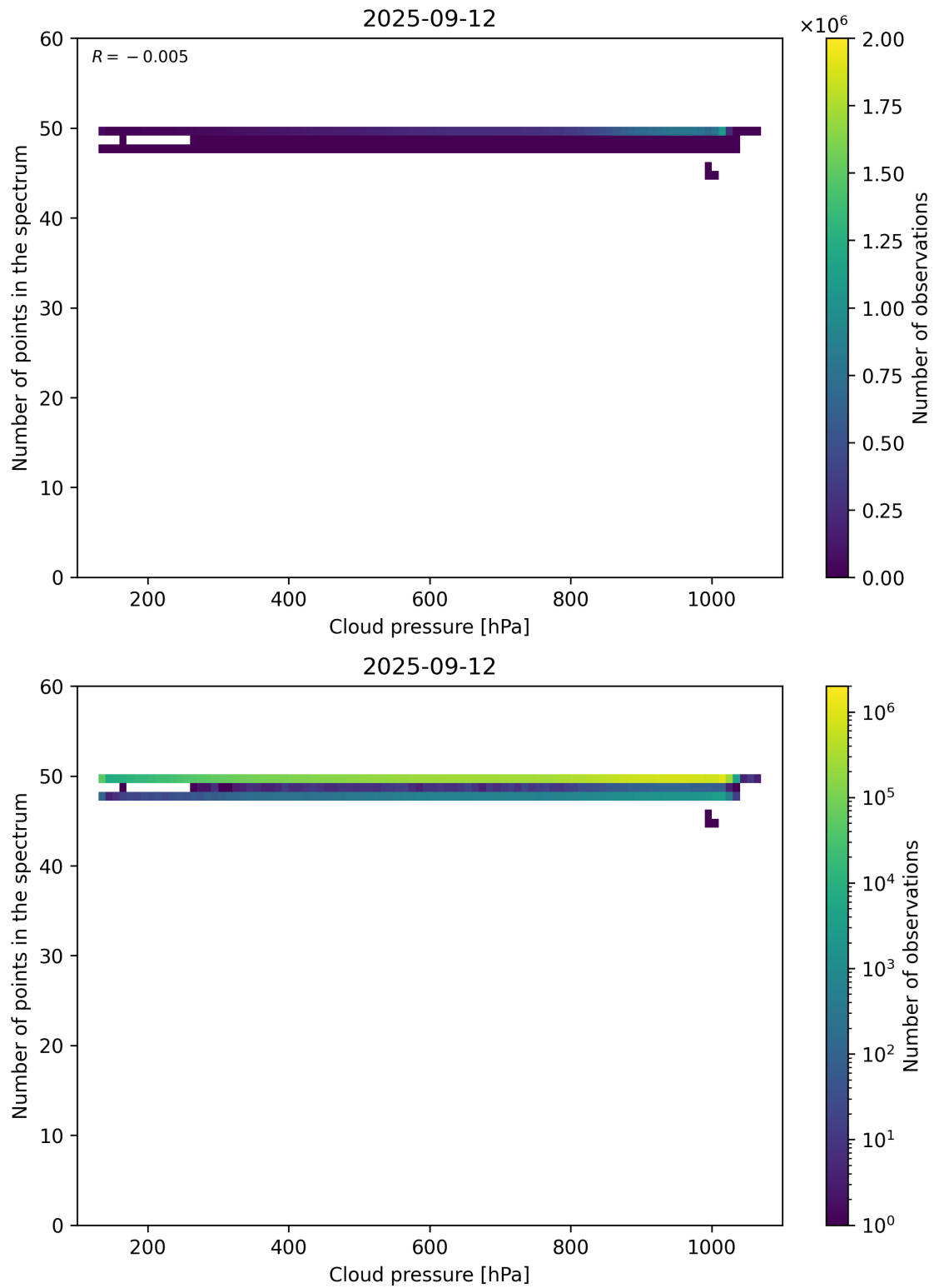
Figure 82: Scatter density plot of “Cloud pressure” against “Number of points in the spectrum” for 2025-09-11 to 2025-09-13.
