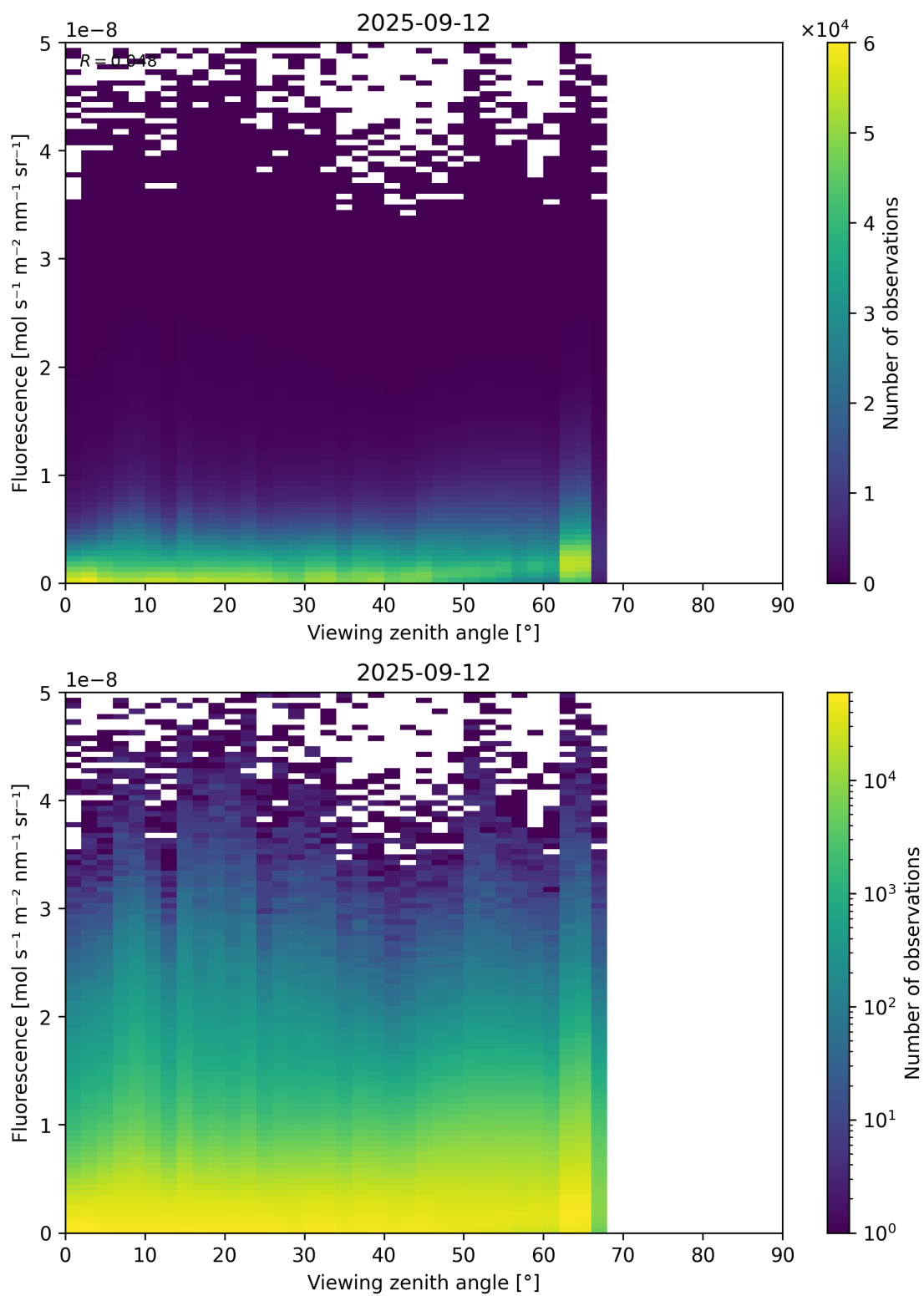
Figure 122: Scatter density plot of “Viewing zenith angle” against “Fluorescence” for 2025-09-11 to 2025-09-13.
