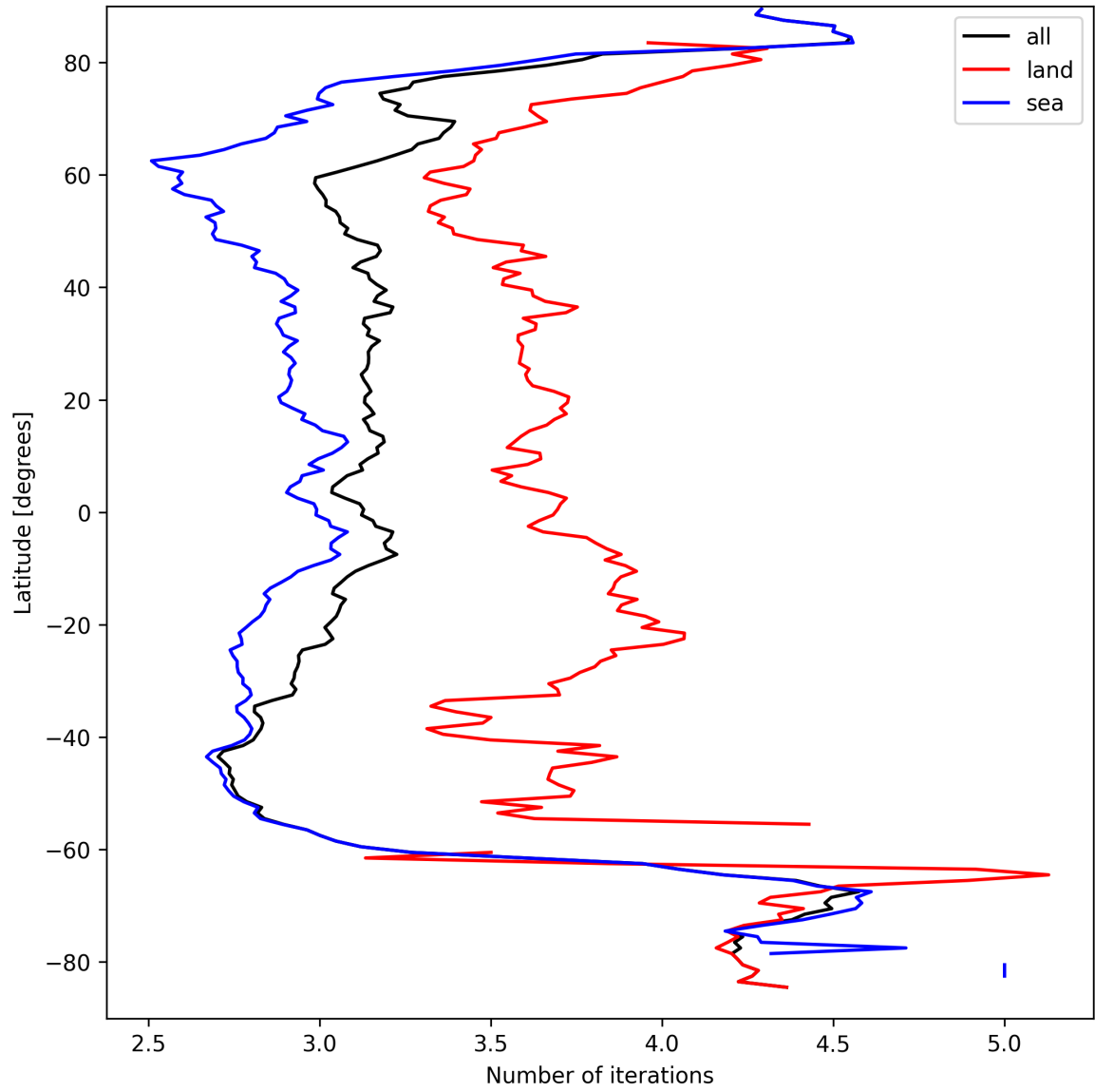
Figure 22: Zonal average of “Number of iterations” for 2025-09-11 to 2025-09-13.
