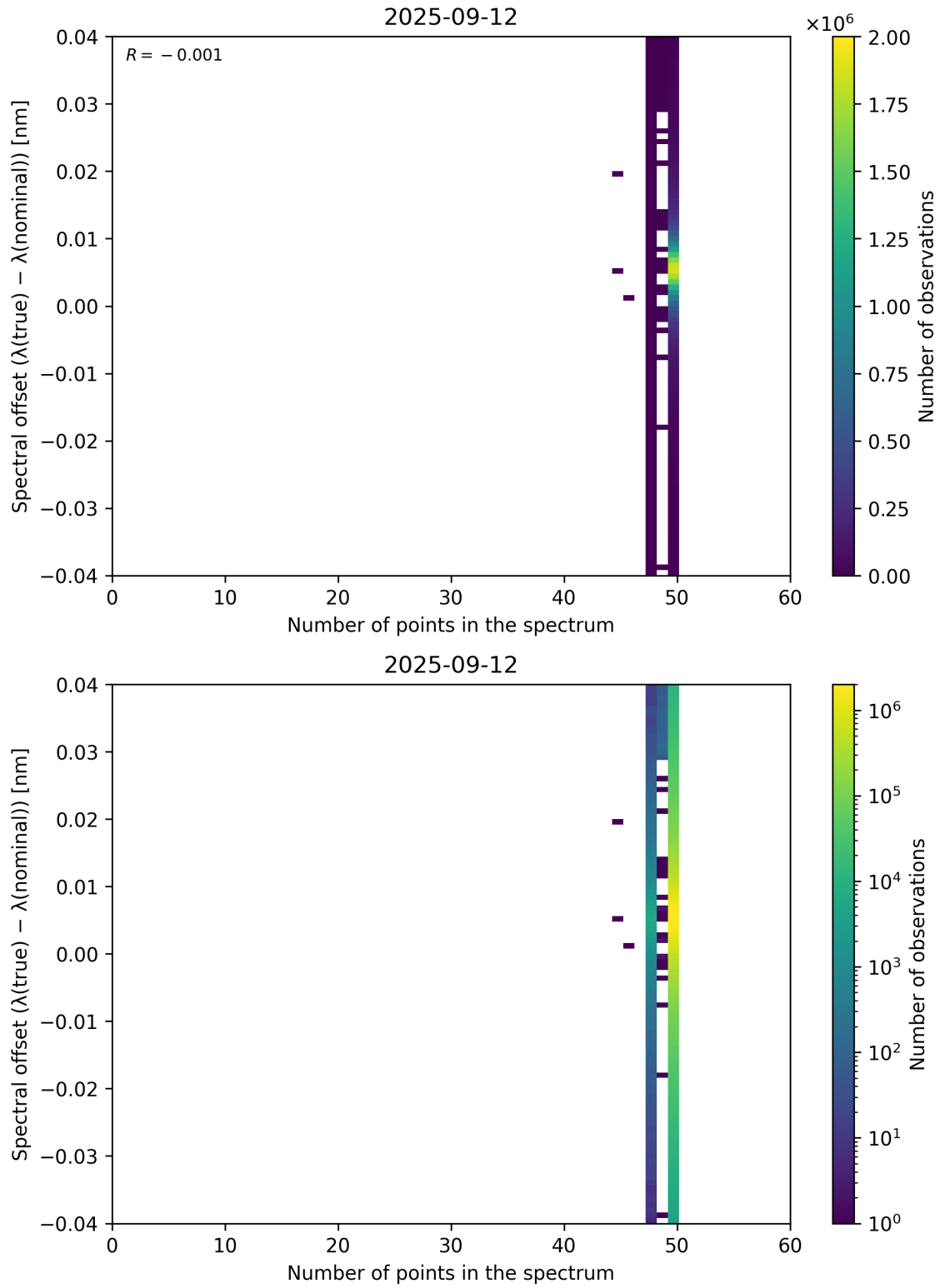
Figure 101: Scatter density plot of “Number of points in the spectrum” against “Spectral offset ( \lambda_{\text{true}} - \lambda_{\text{nominal}} )” for 2025-09-11 to 2025-09-13.
