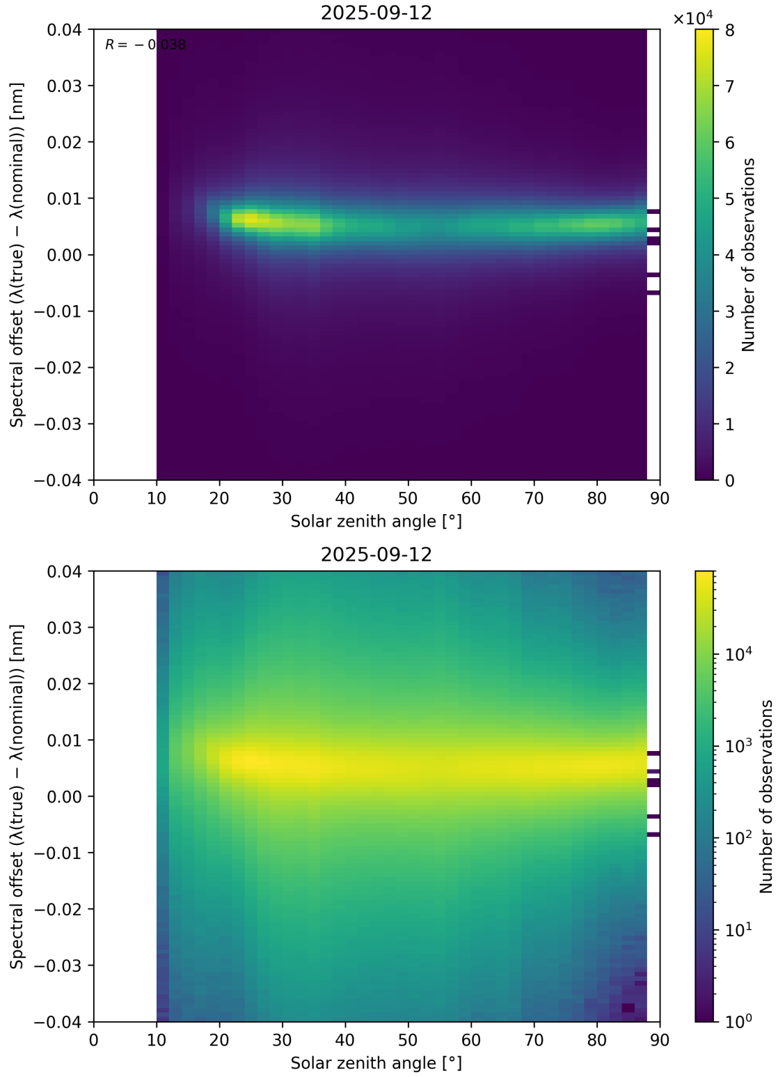
Figure 117: Scatter density plot of “Solar zenith angle” against “Spectral offset ( \lambda_{\text{true}} - \lambda_{\text{nominal}} )” for 2025-09-11 to 2025-09-13.
