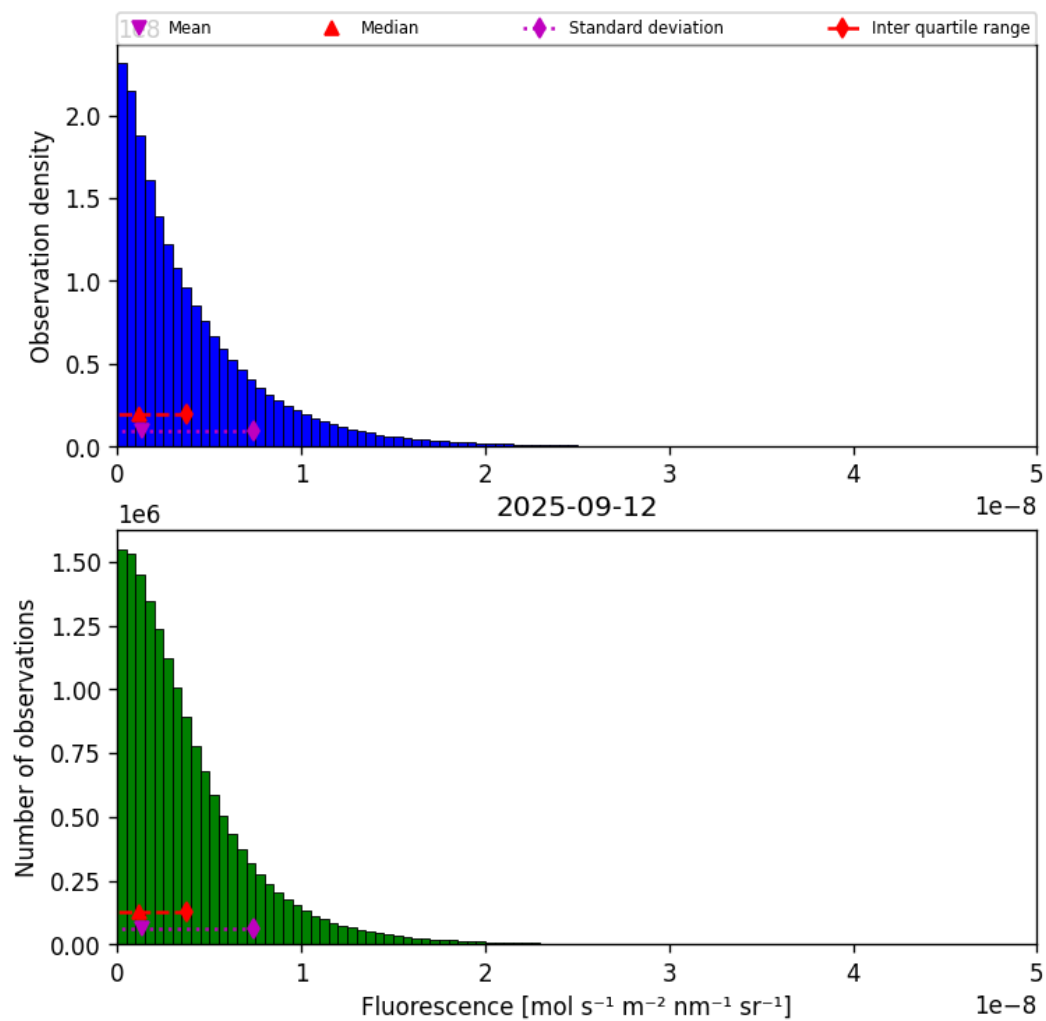
Figure 40: Histogram of “Fluorescence” for 2025-09-11 to 2025-09-13
