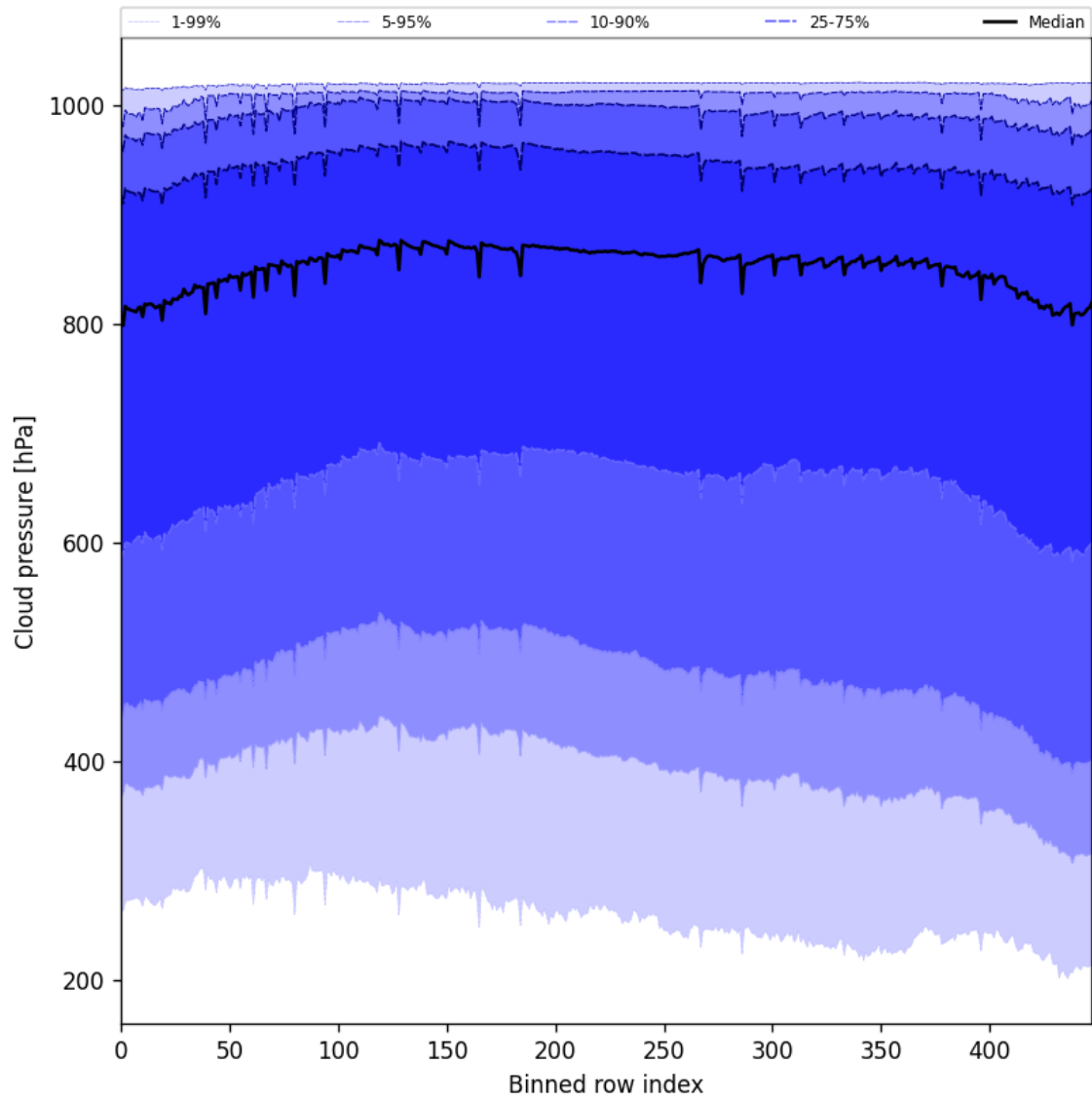
Figure 47: Along track statistics of “Cloud pressure” for 2025-09-11 to 2025-09-13
