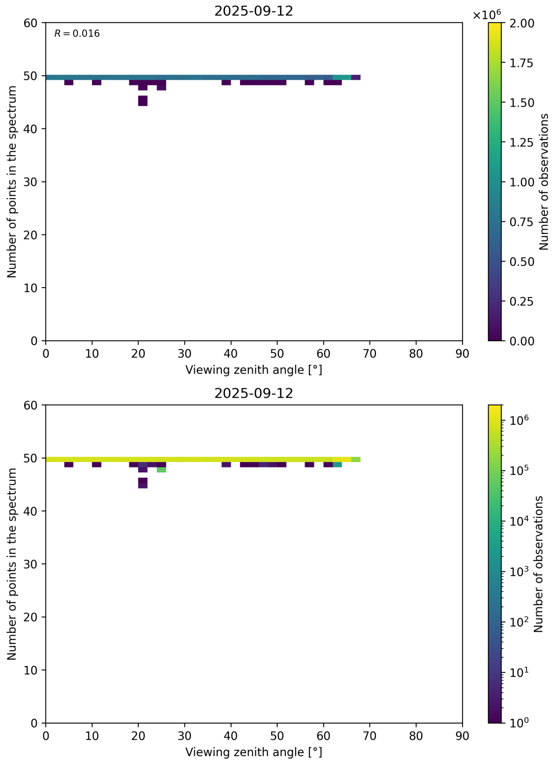
Figure 125: Scatter density plot of “Viewing zenith angle” against “Number of points in the spectrum” for 2025-09-11 to 2025-09-13.
