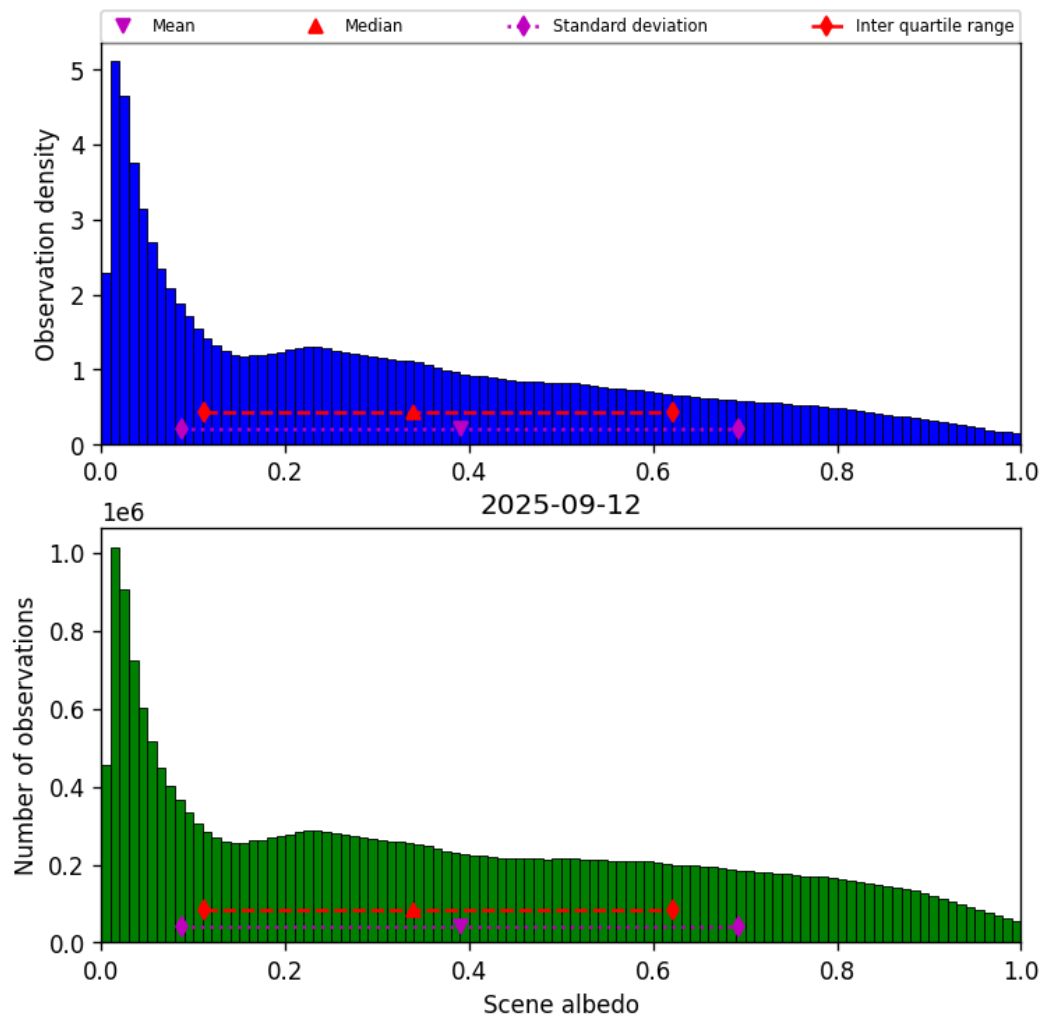
Figure 34: Histogram of “Scene albedo” for 2025-09-11 to 2025-09-13
