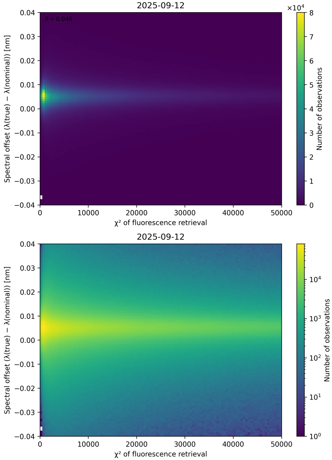
Figure 69: Scatter density plot of “ \chi^2 of fluorescence retrieval” against “Spectral offset ( \lambda_{\text{true}} - \lambda_{\text{nominal}} )” for 2025-09-11 to 2025-09-13.
