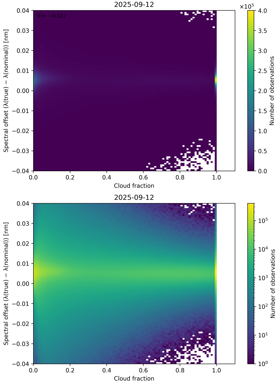
Figure 76: Scatter density plot of “Cloud fraction” against “Spectral offset ( \lambda_{\text{true}} - \lambda_{\text{nominal}} )” for 2025-09-11 to 2025-09-13.
