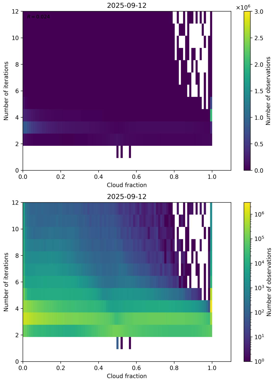
Figure 73: Scatter density plot of “Cloud fraction” against “Number of iterations” for 2025-09-11 to 2025-09-13.
