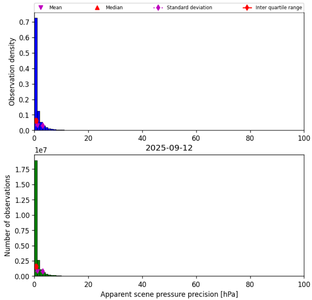
Figure 37: Histogram of “Apparent scene pressure precision” for 2025-09-11 to 2025-09-13
