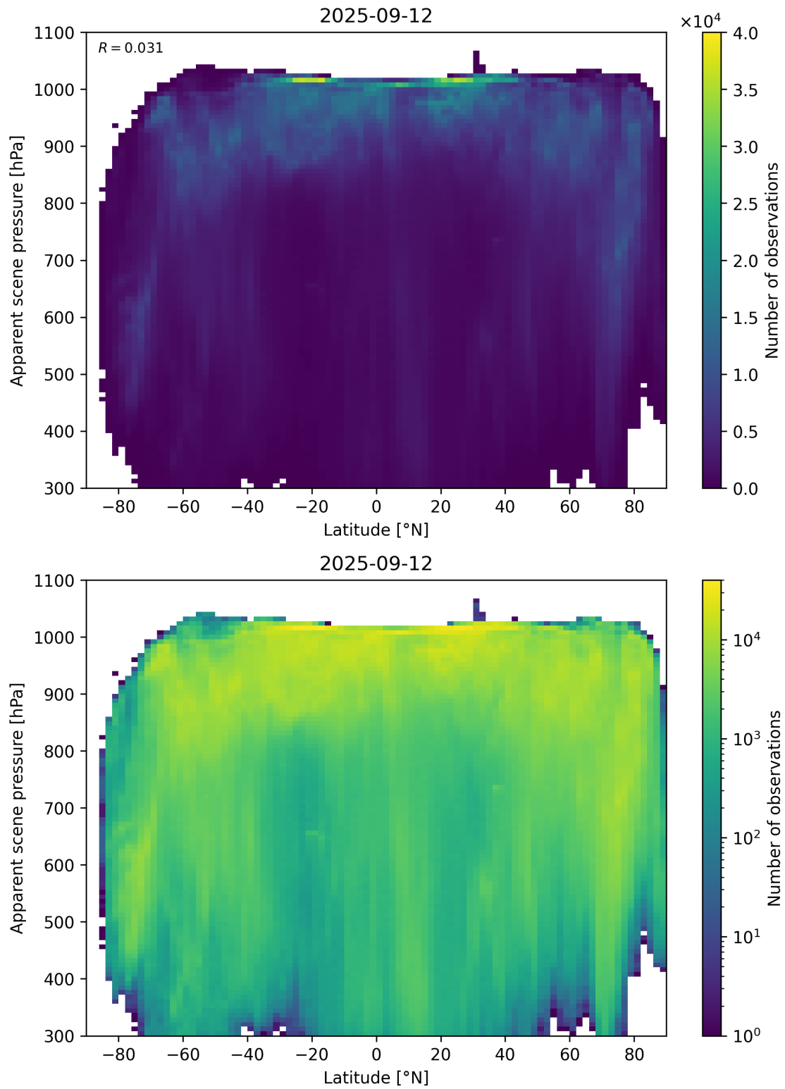
Figure 88: Scatter density plot of “Latitude” against “Apparent scene pressure” for 2025-09-11 to 2025-09-13.
