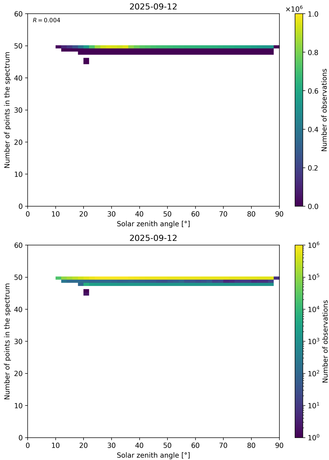
Figure 115: Scatter density plot of “Solar zenith angle” against “Number of points in the spectrum” for 2025-09-11 to 2025-09-13.
