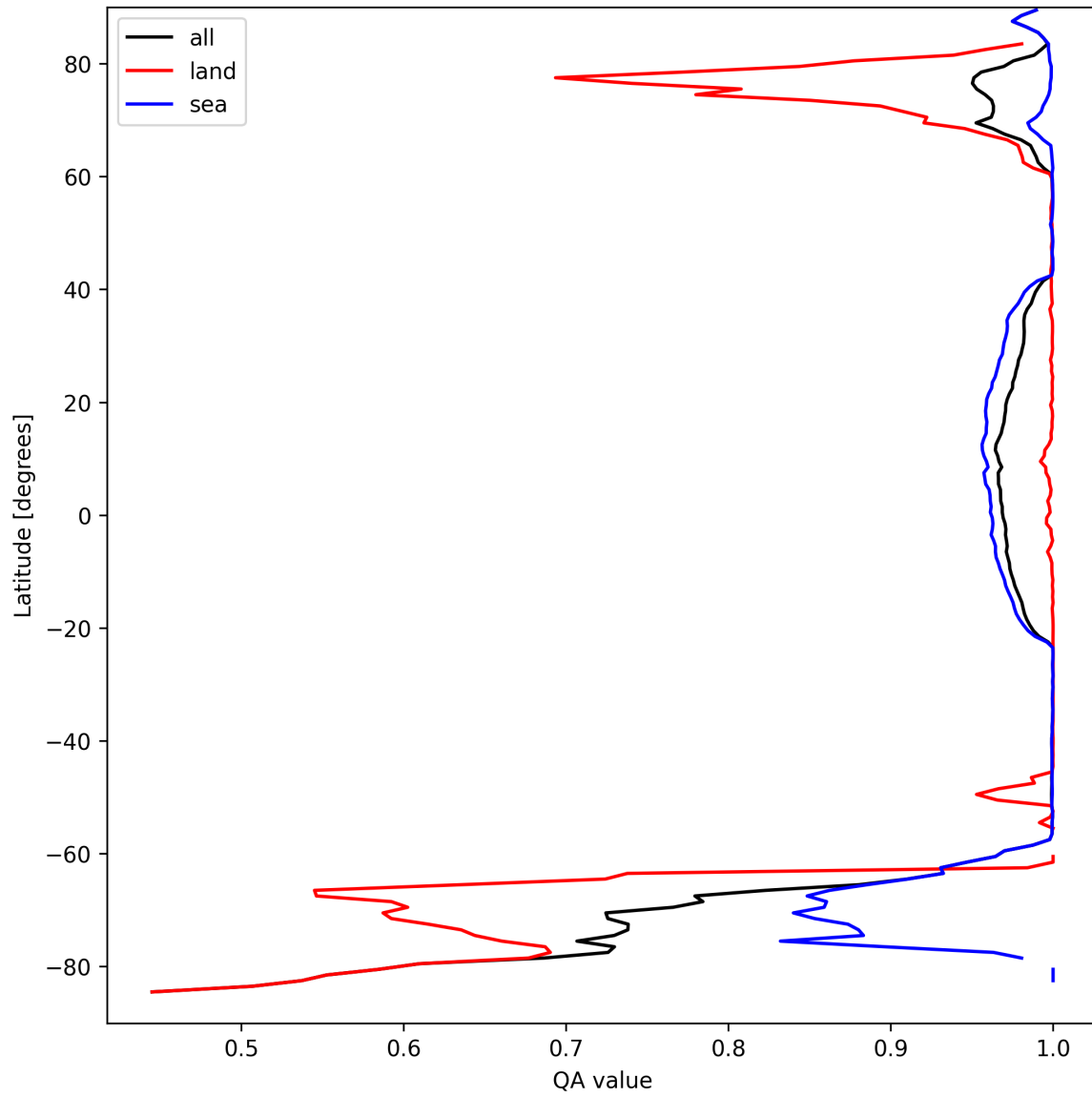
Figure 12: Zonal average of “QA value” for 2025-09-11 to 2025-09-13.
