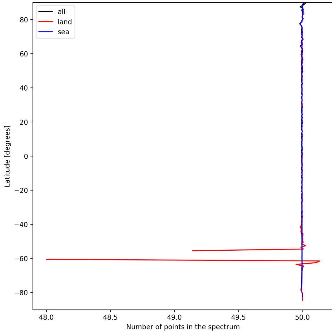
Figure 27: Zonal average of “Number of points in the spectrum” for 2025-09-11 to 2025-09-13.
