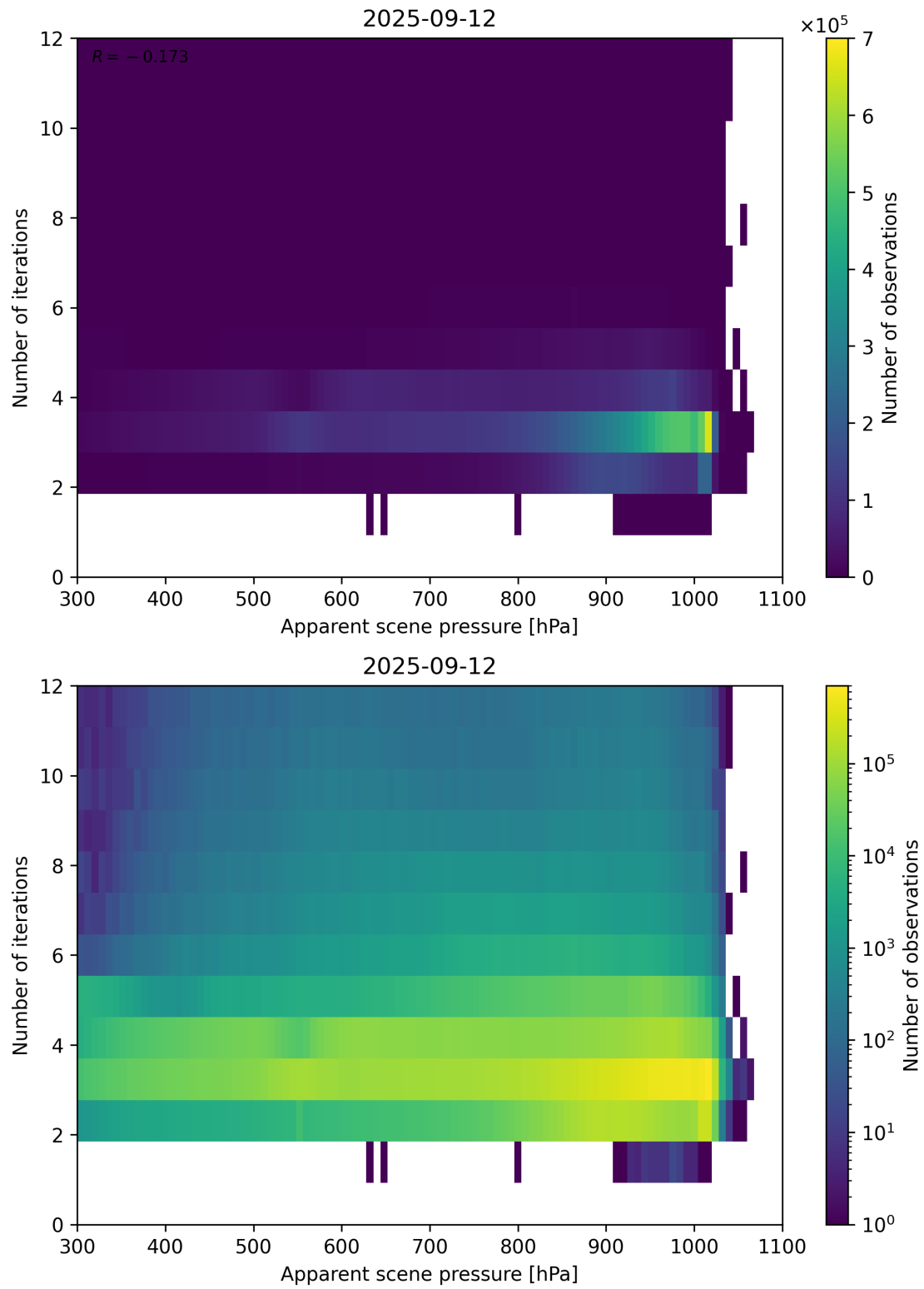
Figure 65: Scatter density plot of “Apparent scene pressure” against “Number of iterations” for 2025-09-11 to 2025-09-13.
