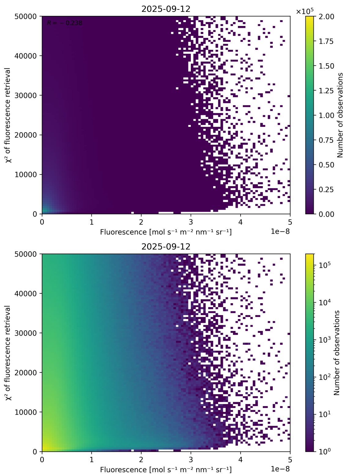
Figure 85: Scatter density plot of “Fluorescence” against “ \chi^2 of fluorescence retrieval” for 2025-09-11 to 2025-09-13.
