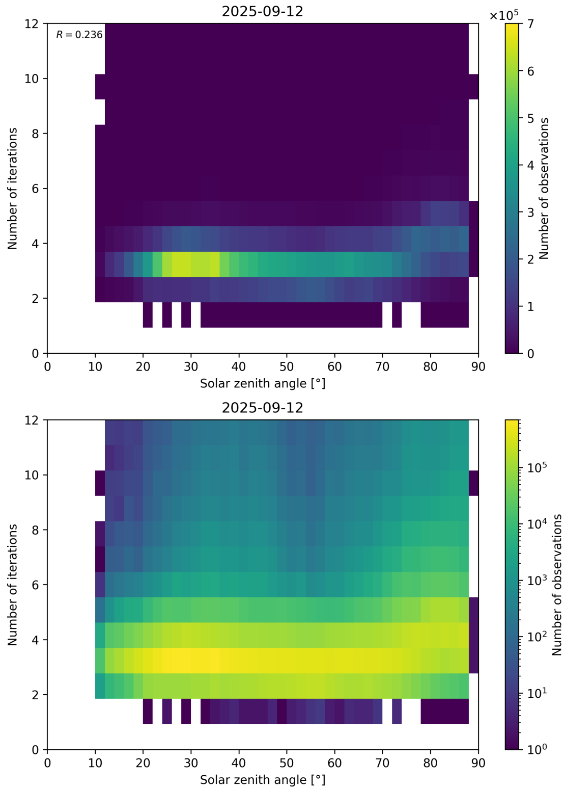
Figure 114: Scatter density plot of “Solar zenith angle” against “Number of iterations” for 2025-09-11 to 2025-09-13.
