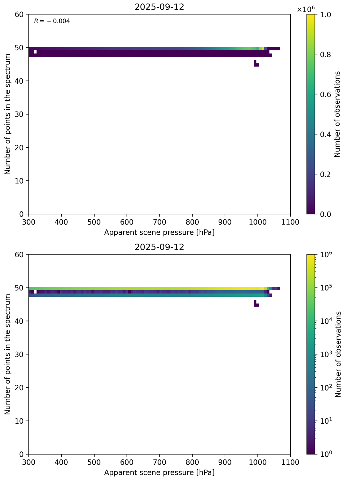
Figure 66: Scatter density plot of “Apparent scene pressure” against “Number of points in the spectrum” for 2025-09-11 to 2025-09-13.
