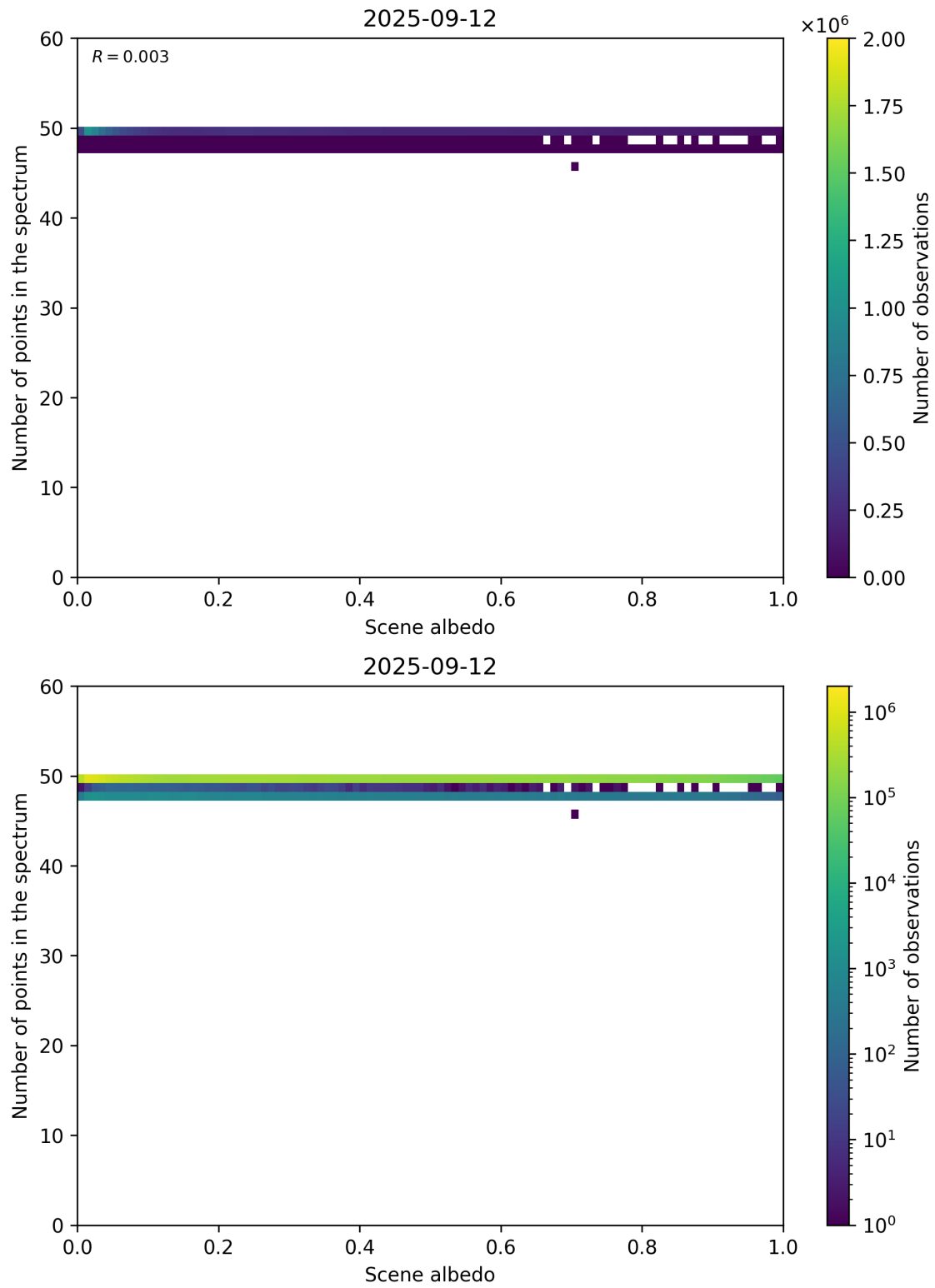
Figure 106: Scatter density plot of “Scene albedo” against “Number of points in the spectrum” for 2025-09-11 to 2025-09-13.
