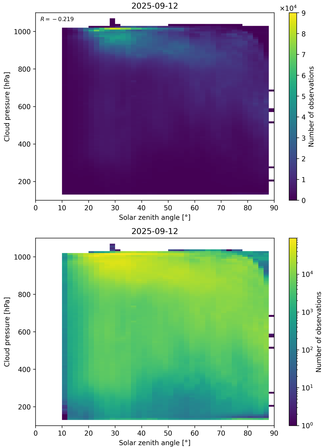
Figure 111: Scatter density plot of “Solar zenith angle” against “Cloud pressure” for 2025-09-11 to 2025-09-13.
