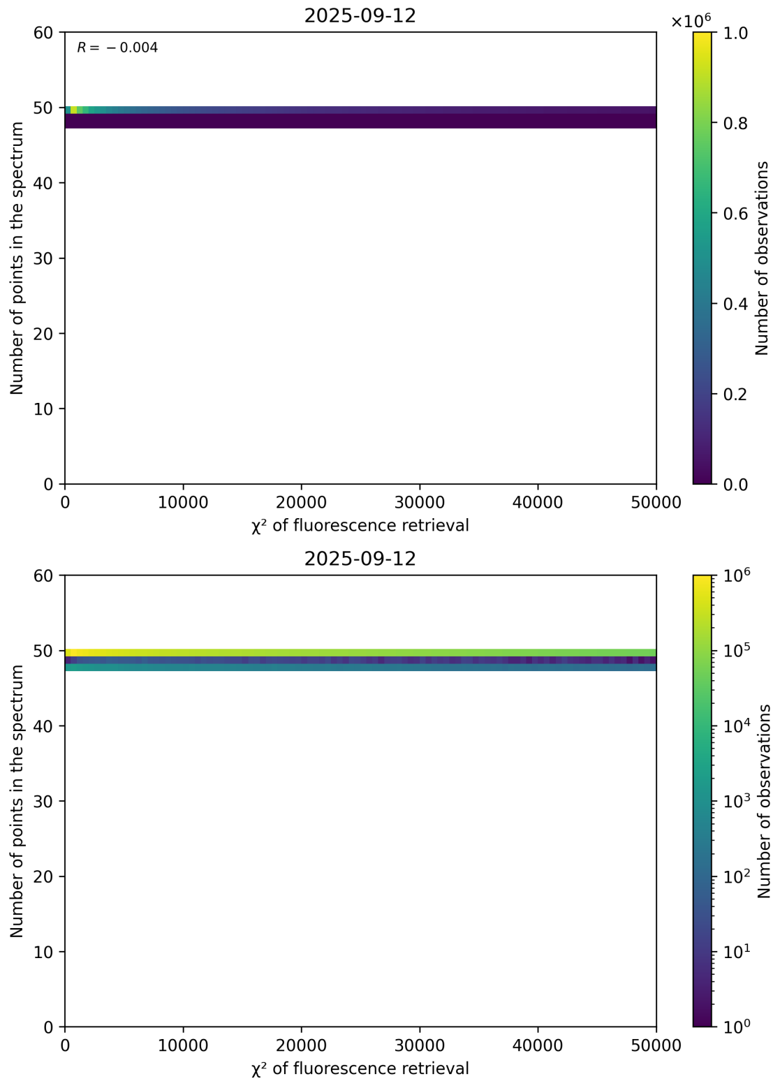
Figure 68: Scatter density plot of " \chi^2 of fluorescence retrieval" against "Number of points in the spectrum" for 2025-09-11 to 2025-09-13.
