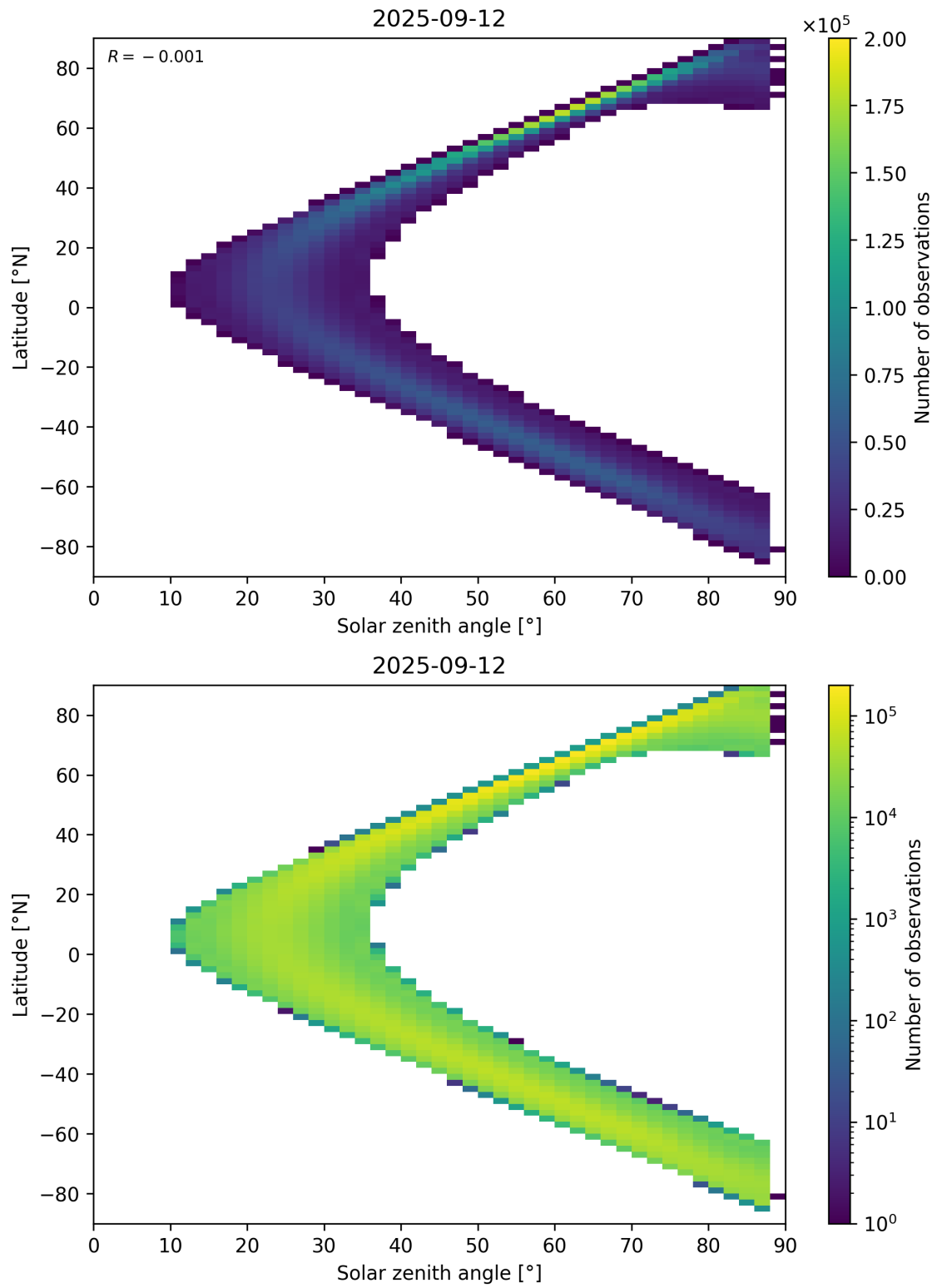
Figure 113: Scatter density plot of “Solar zenith angle” against “Latitude” for 2025-09-11 to 2025-09-13.
