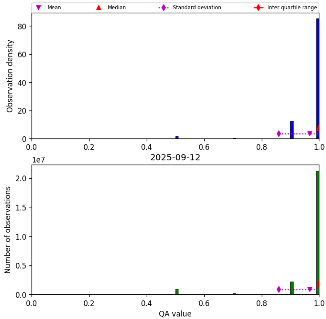
Figure 29: Histogram of “QA value” for 2025-09-11 to 2025-09-13
