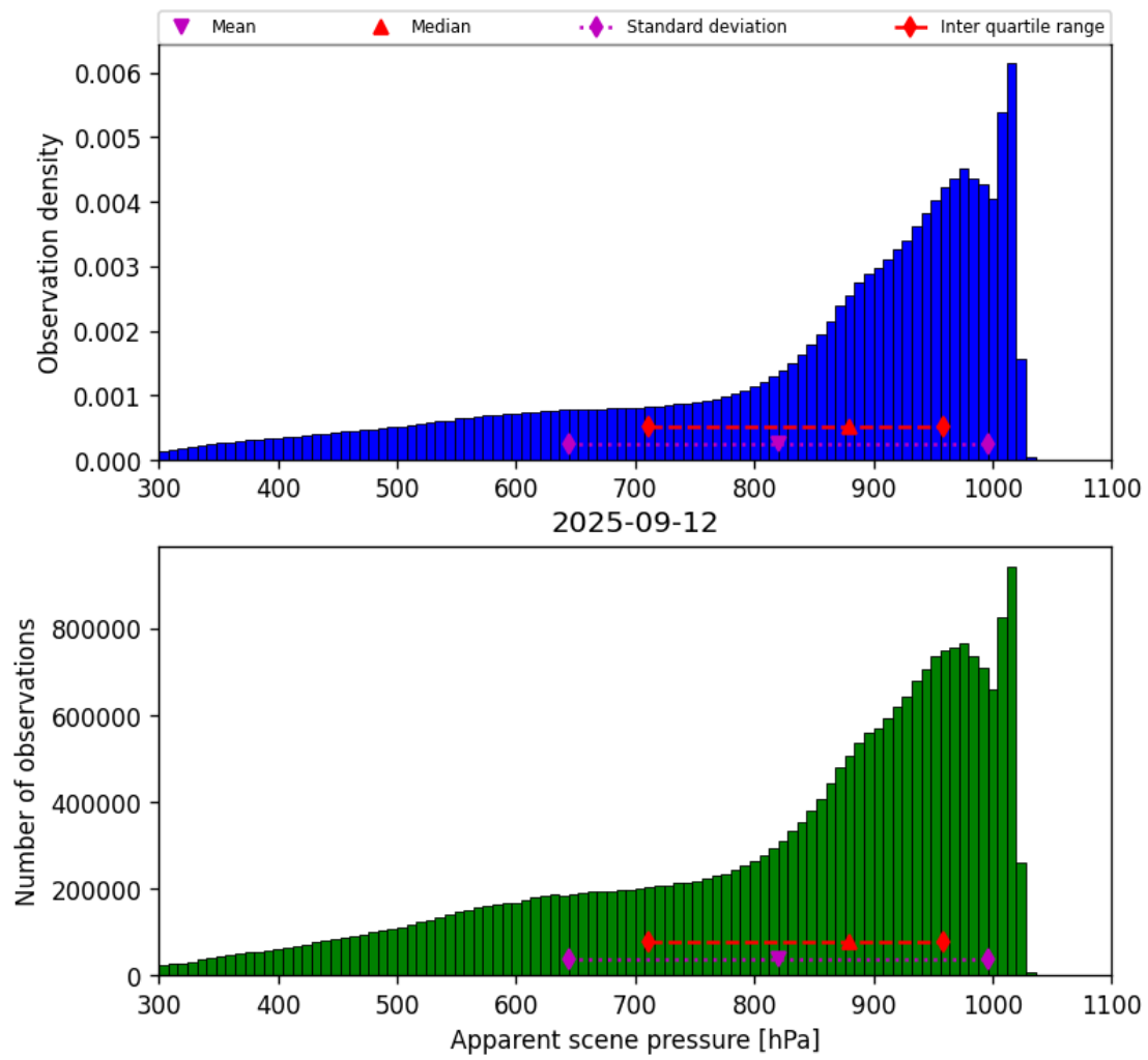
Figure 36: Histogram of “Apparent scene pressure” for 2025-09-11 to 2025-09-13
