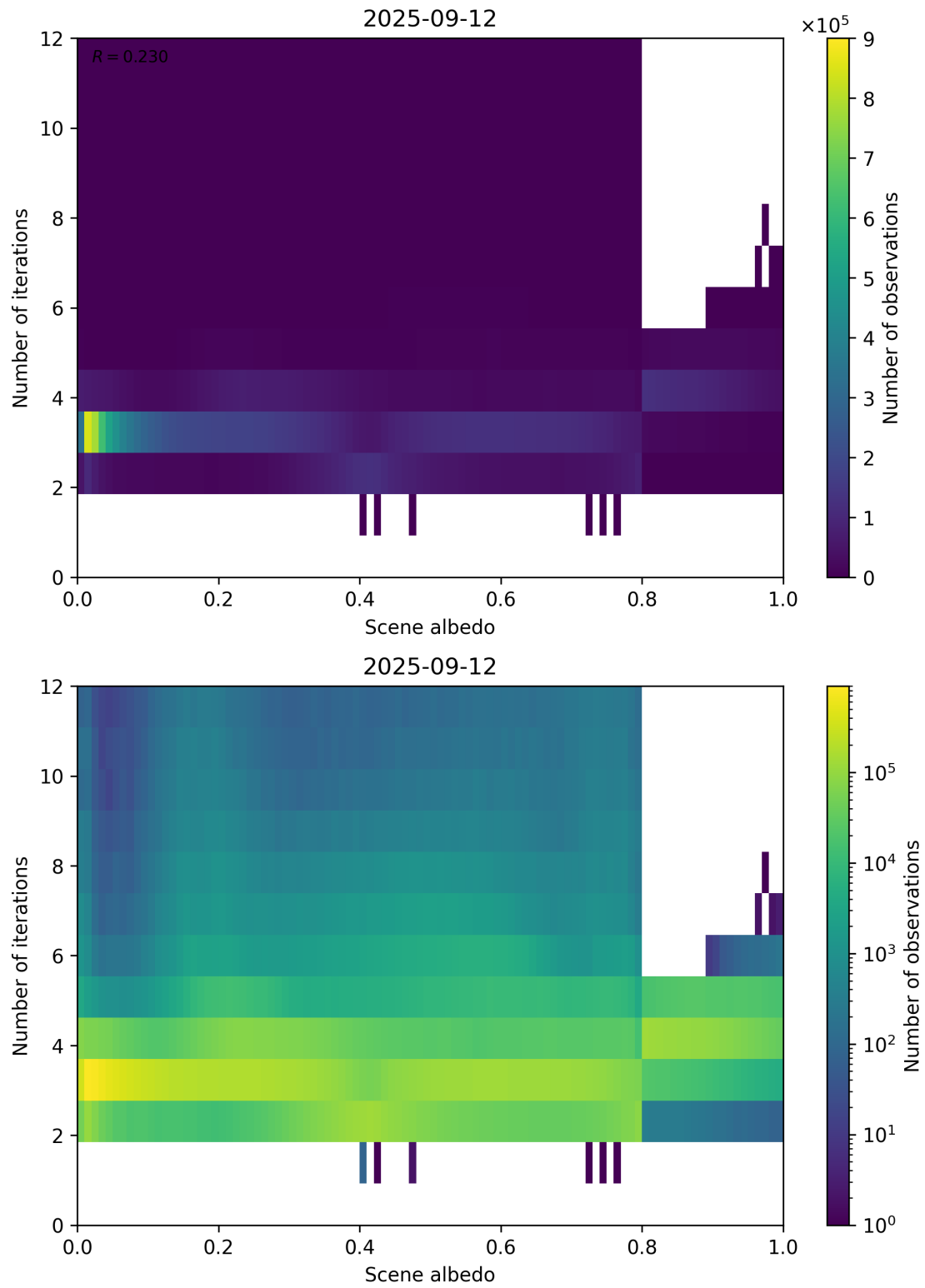
Figure 105: Scatter density plot of “Scene albedo” against “Number of iterations” for 2025-09-11 to 2025-09-13.
