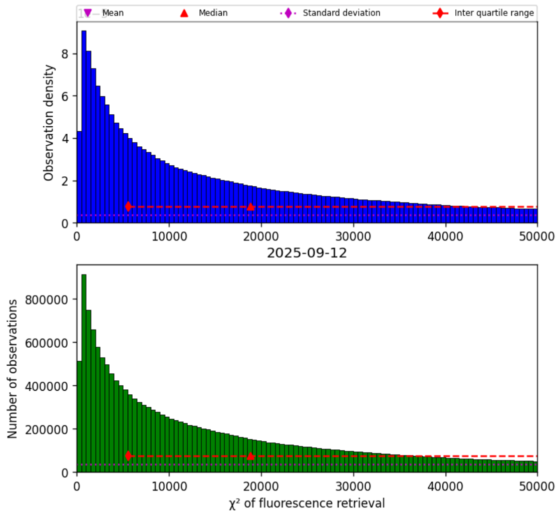
Figure 42: Histogram of “ \chi^2 of fluorescence retrieval” for 2025-09-11 to 2025-09-13
