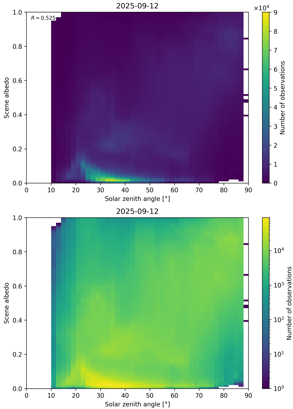
Figure 116: Scatter density plot of “Solar zenith angle” against “Scene albedo” for 2025-09-11 to 2025-09-13.
