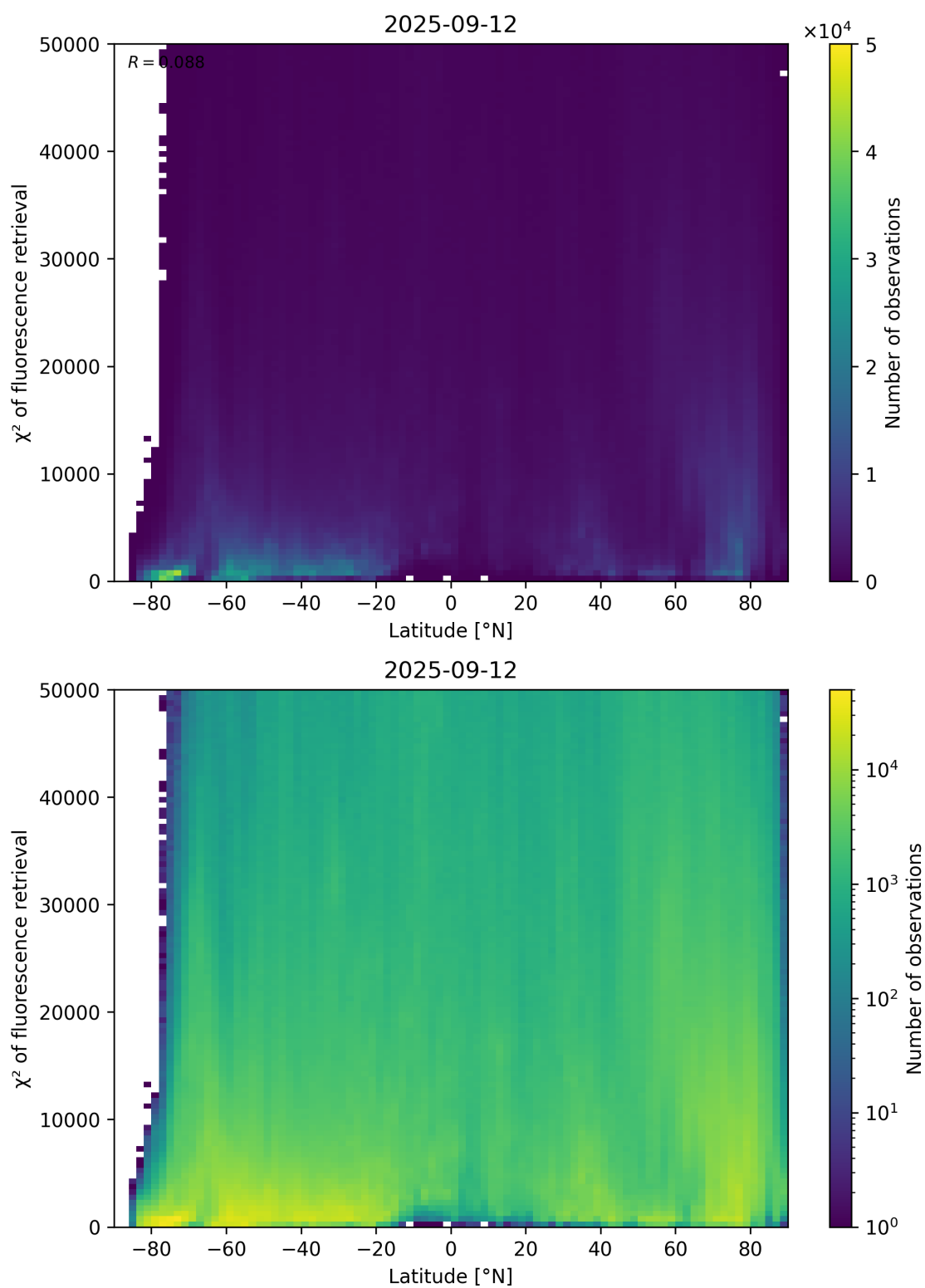
Figure 89: Scatter density plot of “Latitude” against “ \chi^2 of fluorescence retrieval” for 2025-09-11 to 2025-09-13.
