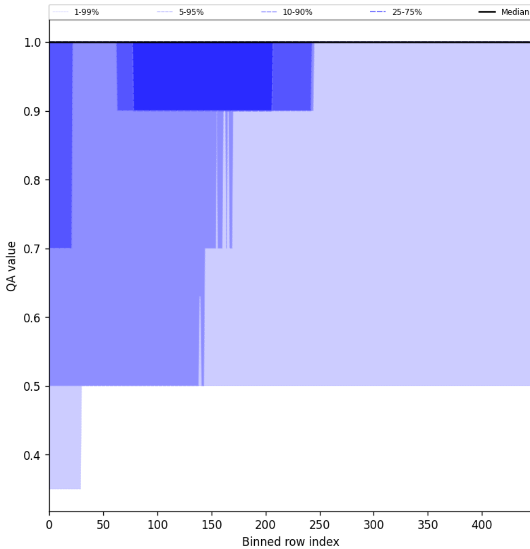
Figure 46: Along track statistics of “QA value” for 2025-09-11 to 2025-09-13
