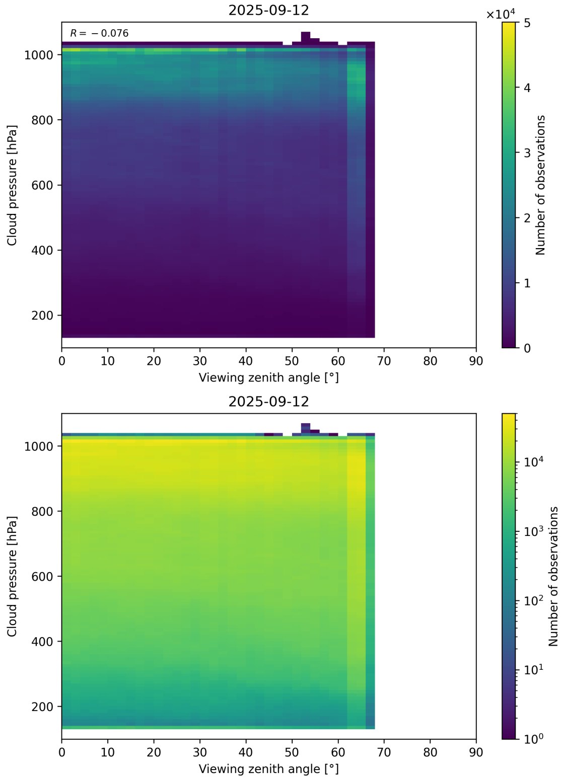
Figure 121: Scatter density plot of “Viewing zenith angle” against “Cloud pressure” for 2025-09-11 to 2025-09-13.
