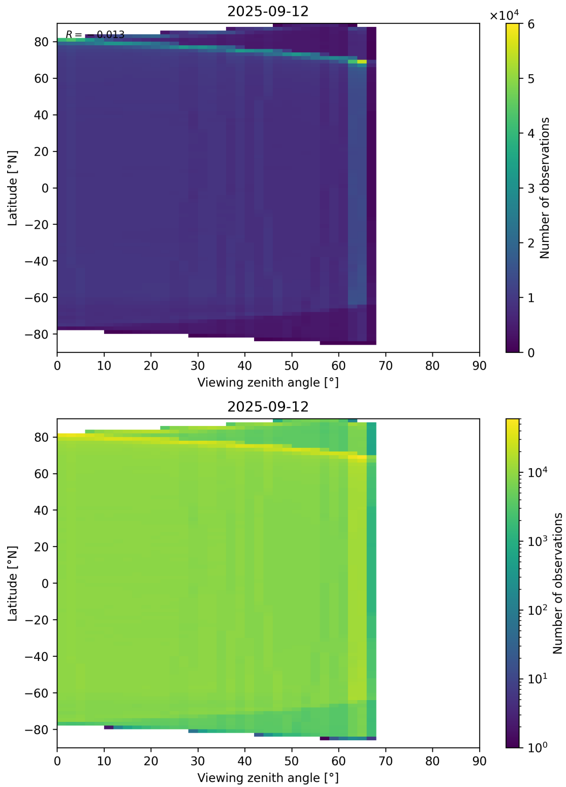
Figure 123: Scatter density plot of “Viewing zenith angle” against “Latitude” for 2025-09-11 to 2025-09-13.
