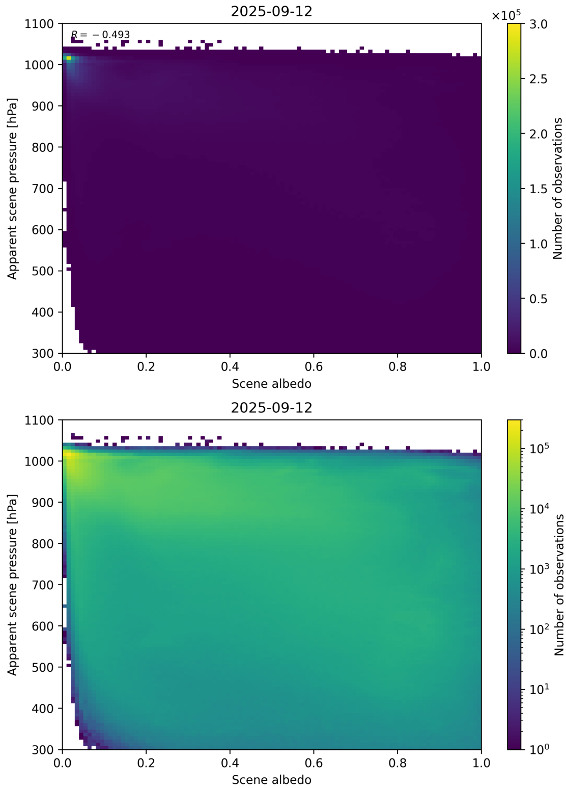
Figure 102: Scatter density plot of “Scene albedo” against “Apparent scene pressure” for 2025-09-11 to 2025-09-13.
