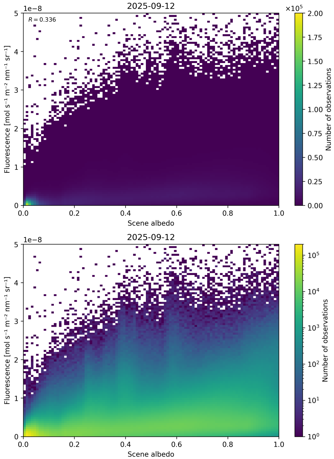
Figure 104: Scatter density plot of “Scene albedo” against “Fluorescence” for 2025-09-11 to 2025-09-13.
