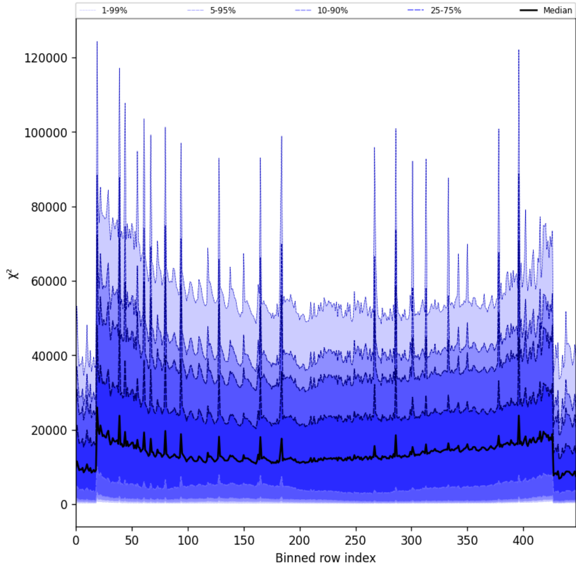
Figure 55: Along track statistics of “ \chi^2 ” for 2025-09-11 to 2025-09-13
