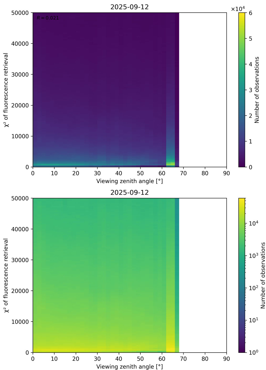
Figure 119: Scatter density plot of “Viewing zenith angle” against “ \chi^2 of fluorescence retrieval” for 2025-09-11 to 2025-09-13.
