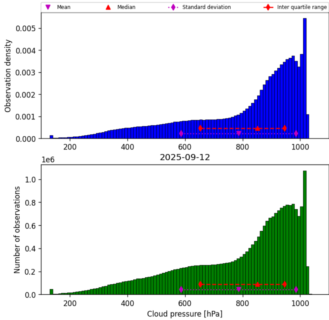
Figure 30: Histogram of “Cloud pressure” for 2025-09-11 to 2025-09-13
