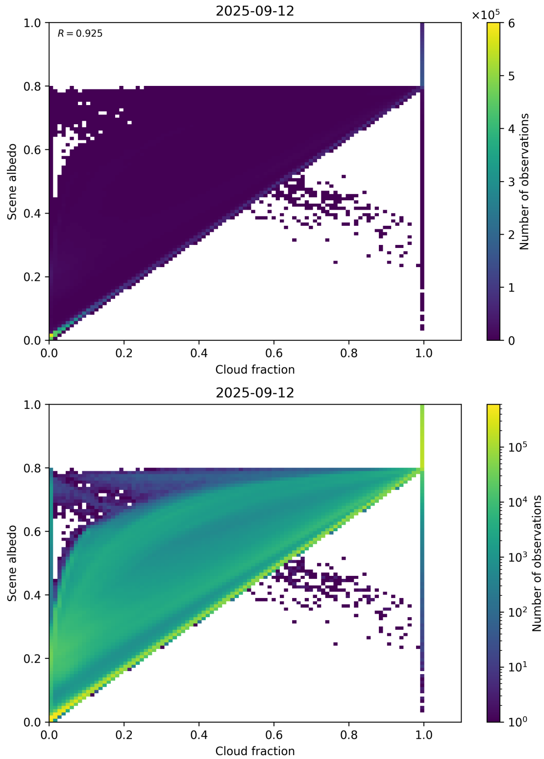
Figure 75: Scatter density plot of “Cloud fraction” against “Scene albedo” for 2025-09-11 to 2025-09-13.
