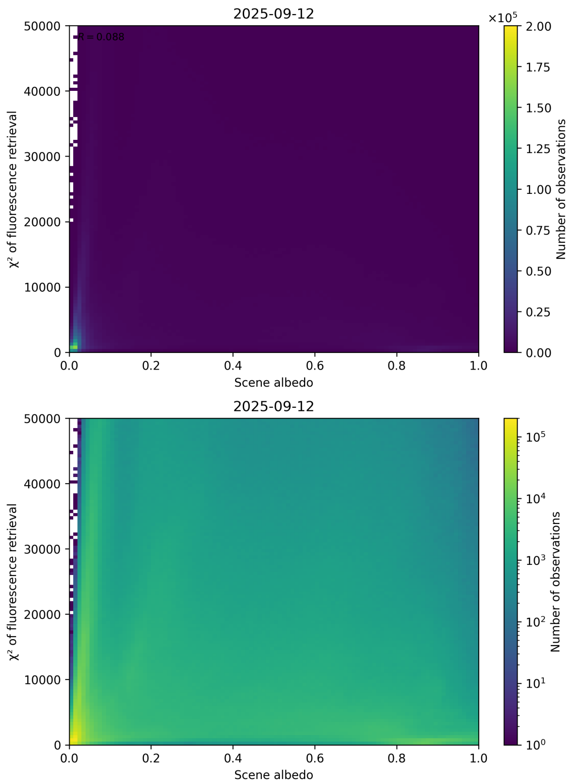
Figure 103: Scatter density plot of “Scene albedo” against “ \chi^2 of fluorescence retrieval” for 2025-09-11 to 2025-09-13.
