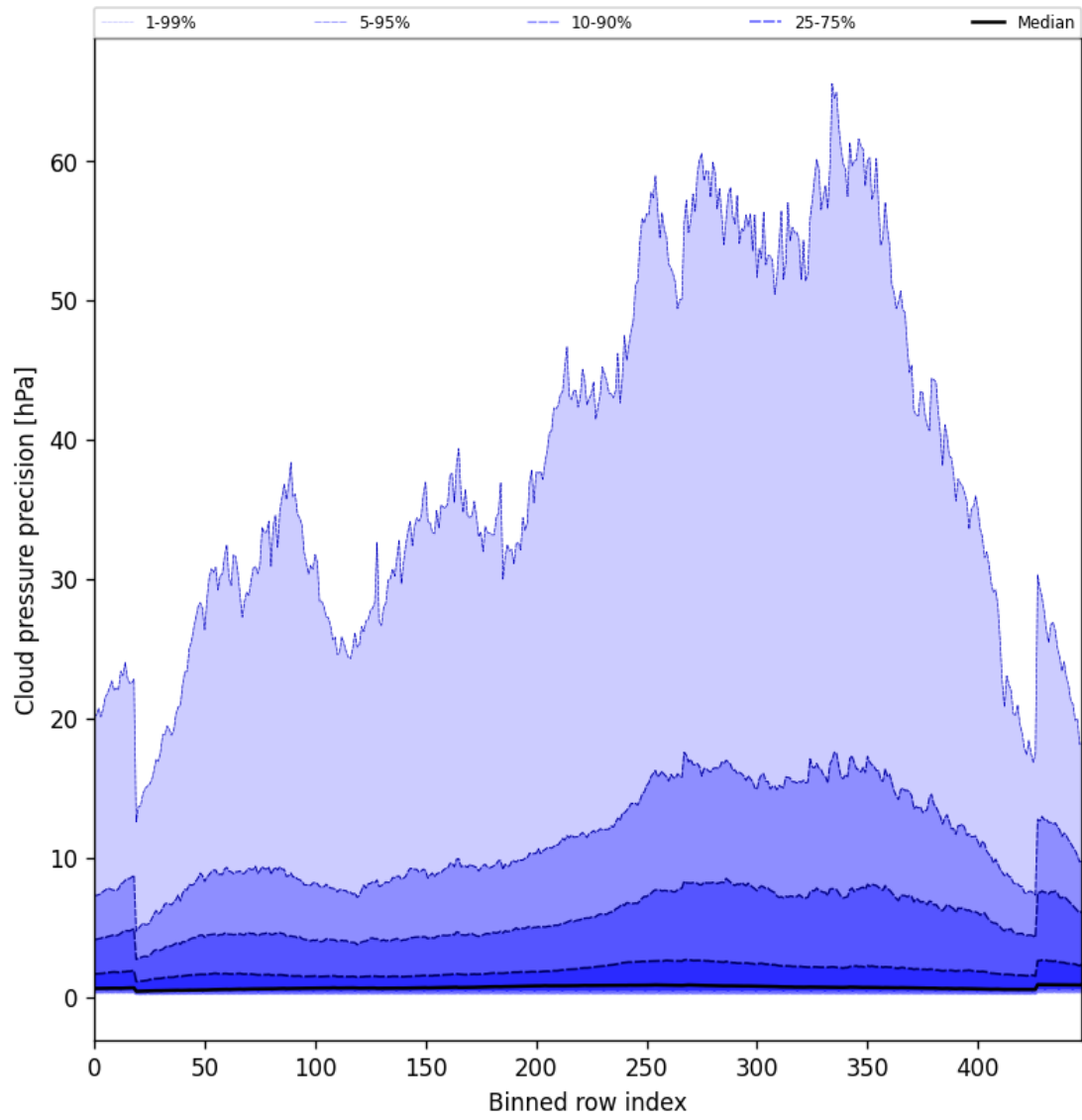
Figure 48: Along track statistics of “Cloud pressure precision” for 2025-09-11 to 2025-09-13
