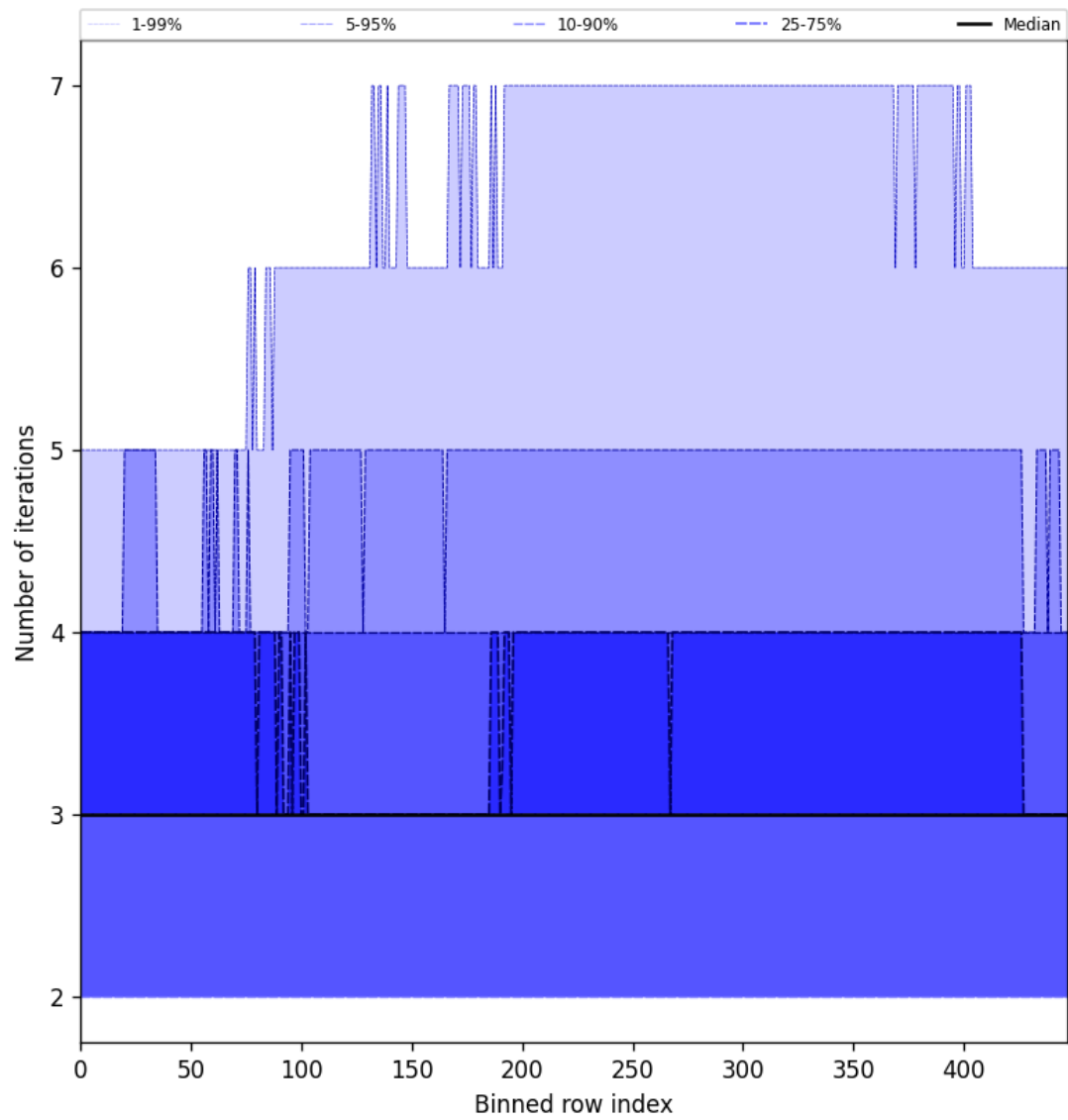
Figure 56: Along track statistics of “Number of iterations” for 2025-09-11 to 2025-09-13
