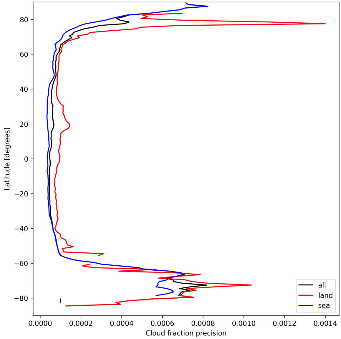
Figure 16: Zonal average of “Cloud fraction precision” for 2025-09-11 to 2025-09-13.
