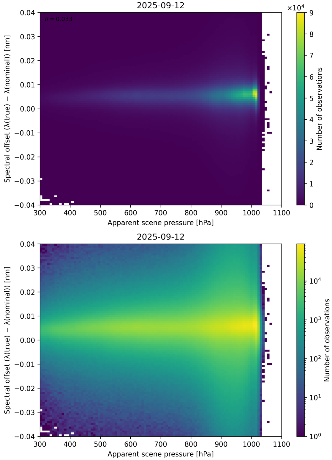
Figure 67: Scatter density plot of “Apparent scene pressure” against “Spectral offset ( \lambda_{\text{true}} - \lambda_{\text{nominal}} )” for 2025-09-11 to 2025-09-13.
