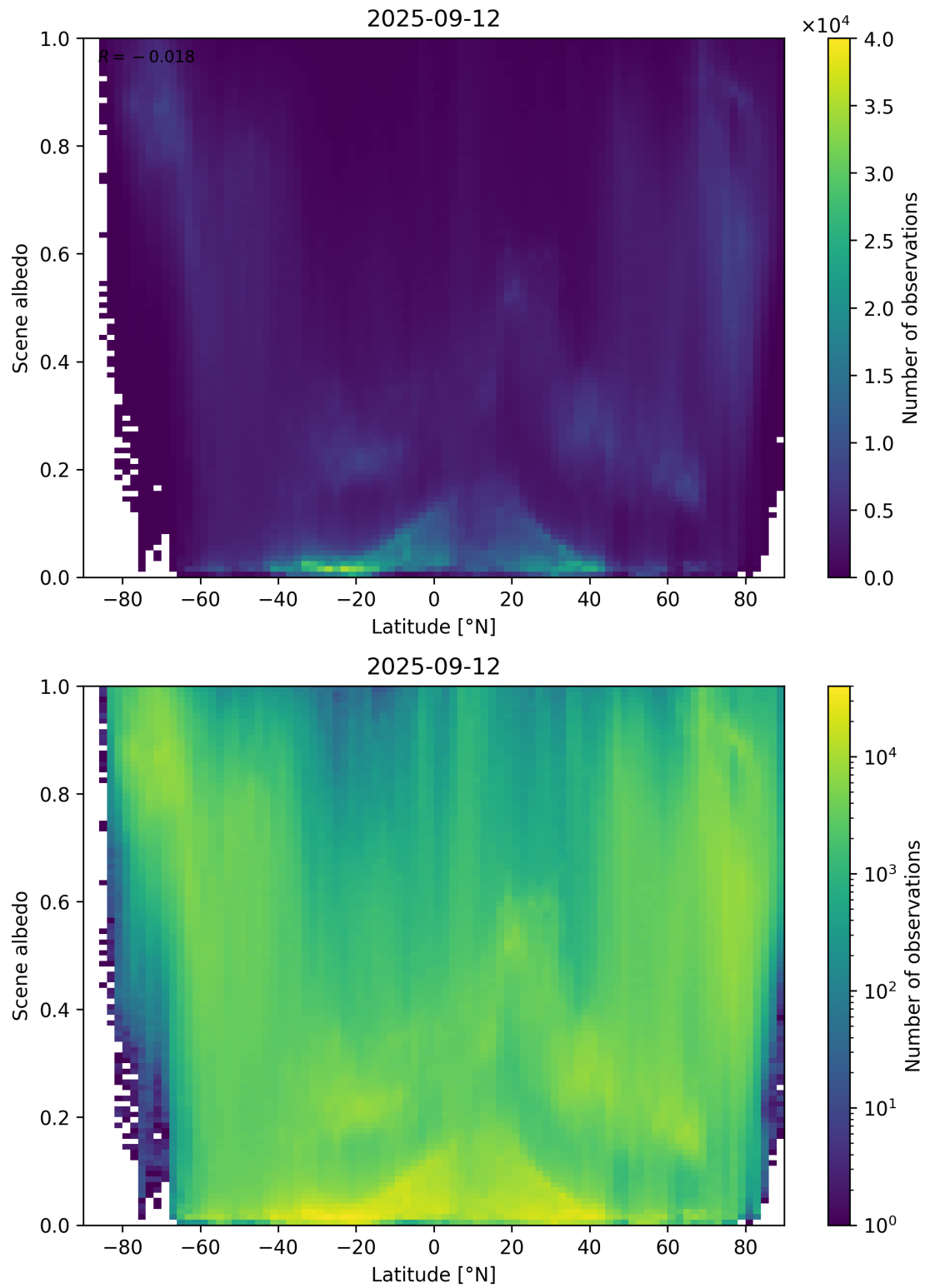
Figure 95: Scatter density plot of “Latitude” against “Scene albedo” for 2025-09-11 to 2025-09-13.
