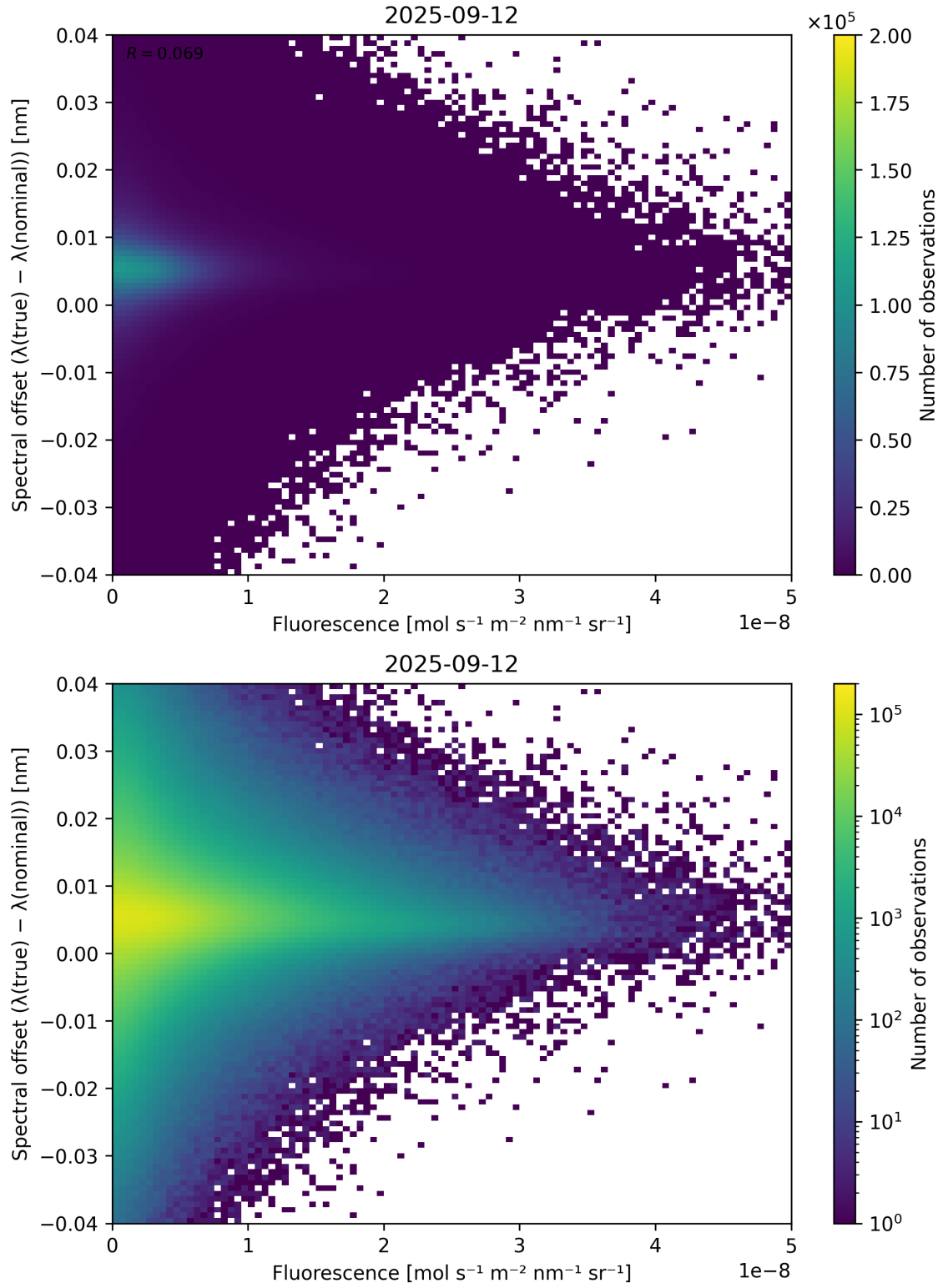
Figure 87: Scatter density plot of “Fluorescence” against “Spectral offset ( \lambda_{\text{true}} - \lambda_{\text{nominal}} )” for 2025-09-11 to 2025-09-13.
