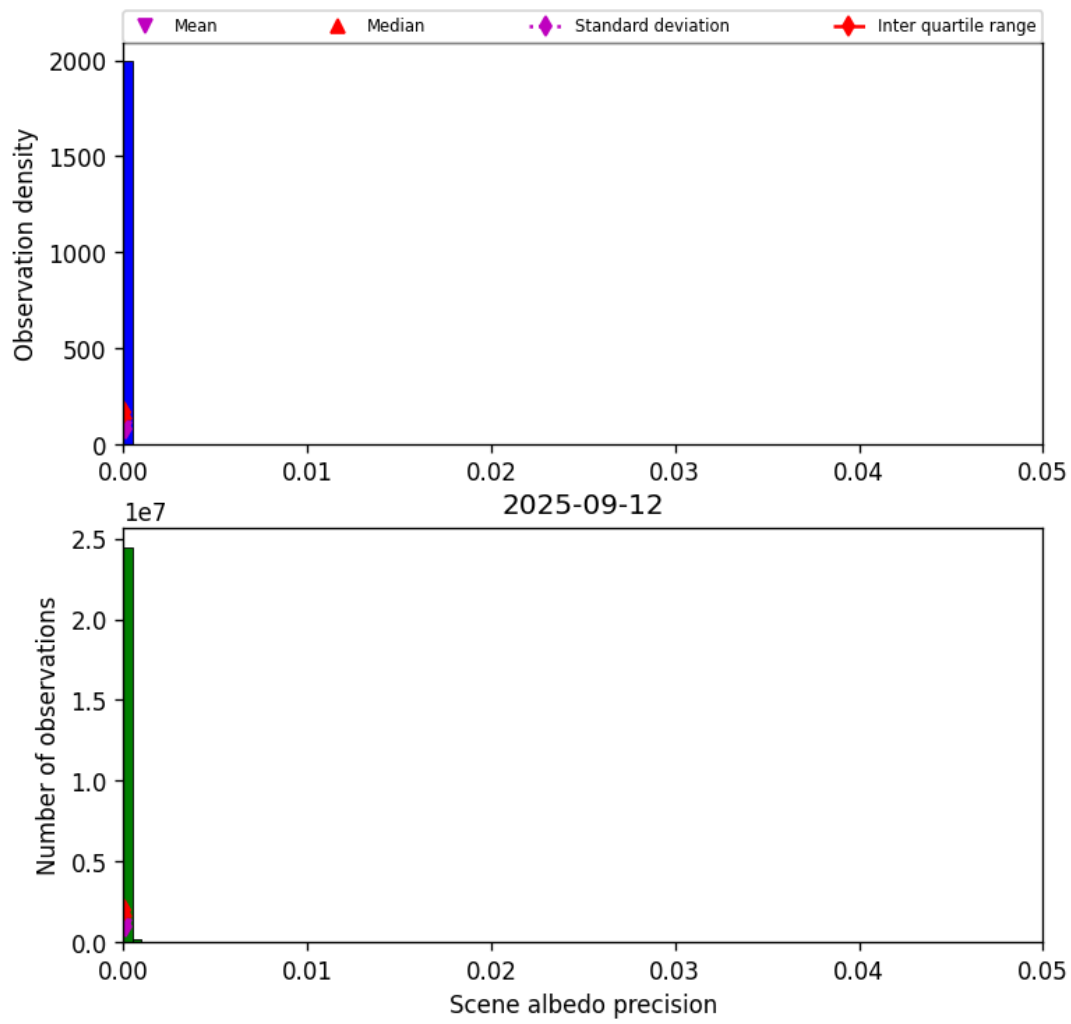
Figure 35: Histogram of “Scene albedo precision” for 2025-09-11 to 2025-09-13
