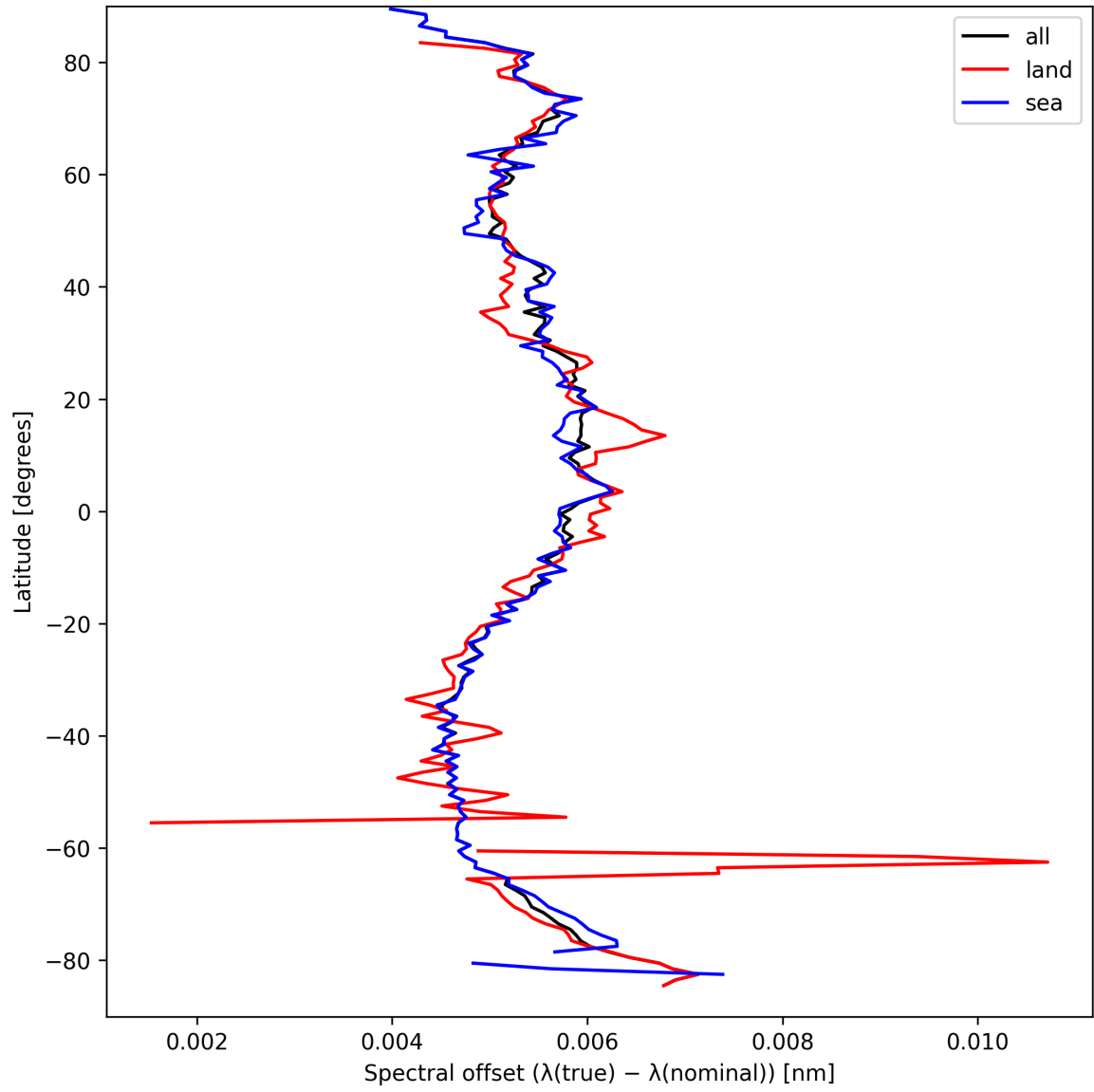
Figure 28: Zonal average of “Spectral offset ( \lambda_{\text{true}} - \lambda_{\text{nominal}} )” for 2025-09-11 to 2025-09-13.
