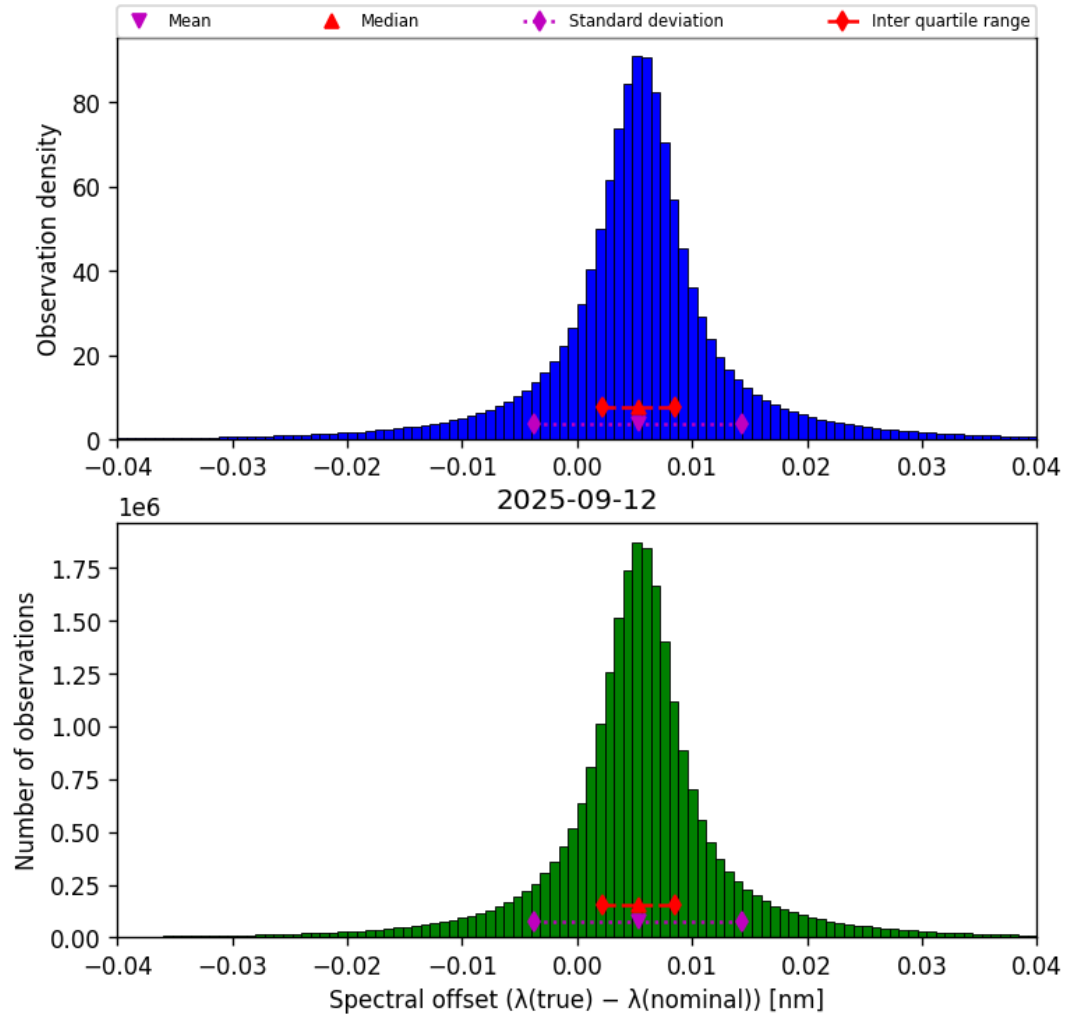
Figure 45: Histogram of “Spectral offset ( \lambda_{\text{true}} - \lambda_{\text{nominal}} )” for 2025-09-11 to 2025-09-13
