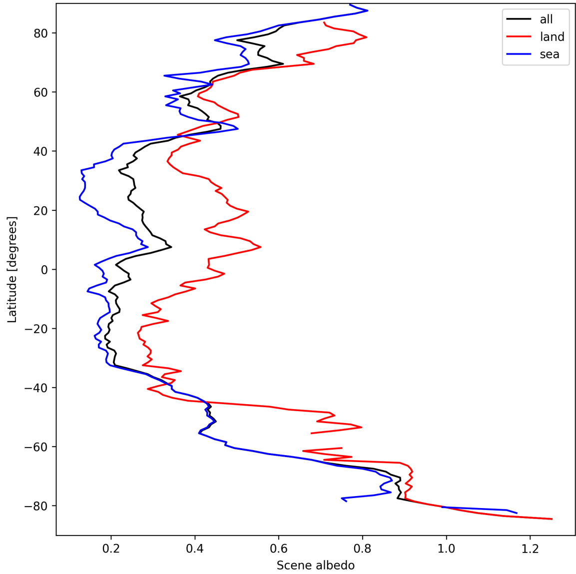
Figure 17: Zonal average of “Scene albedo” for 2025-09-11 to 2025-09-13.
