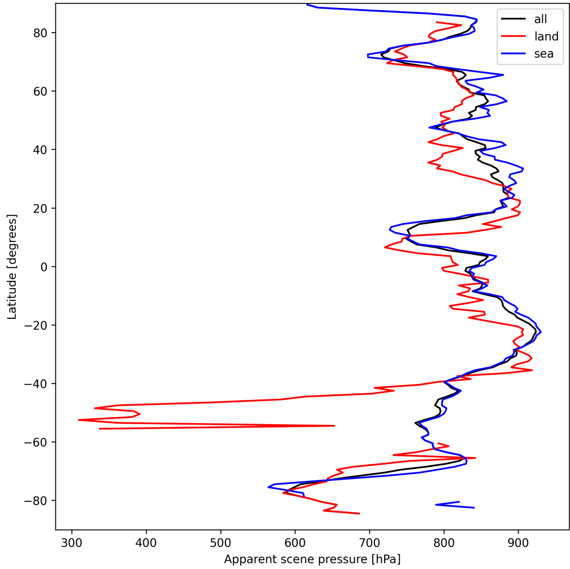
Figure 19: Zonal average of “Apparent scene pressure” for 2025-09-11 to 2025-09-13.
