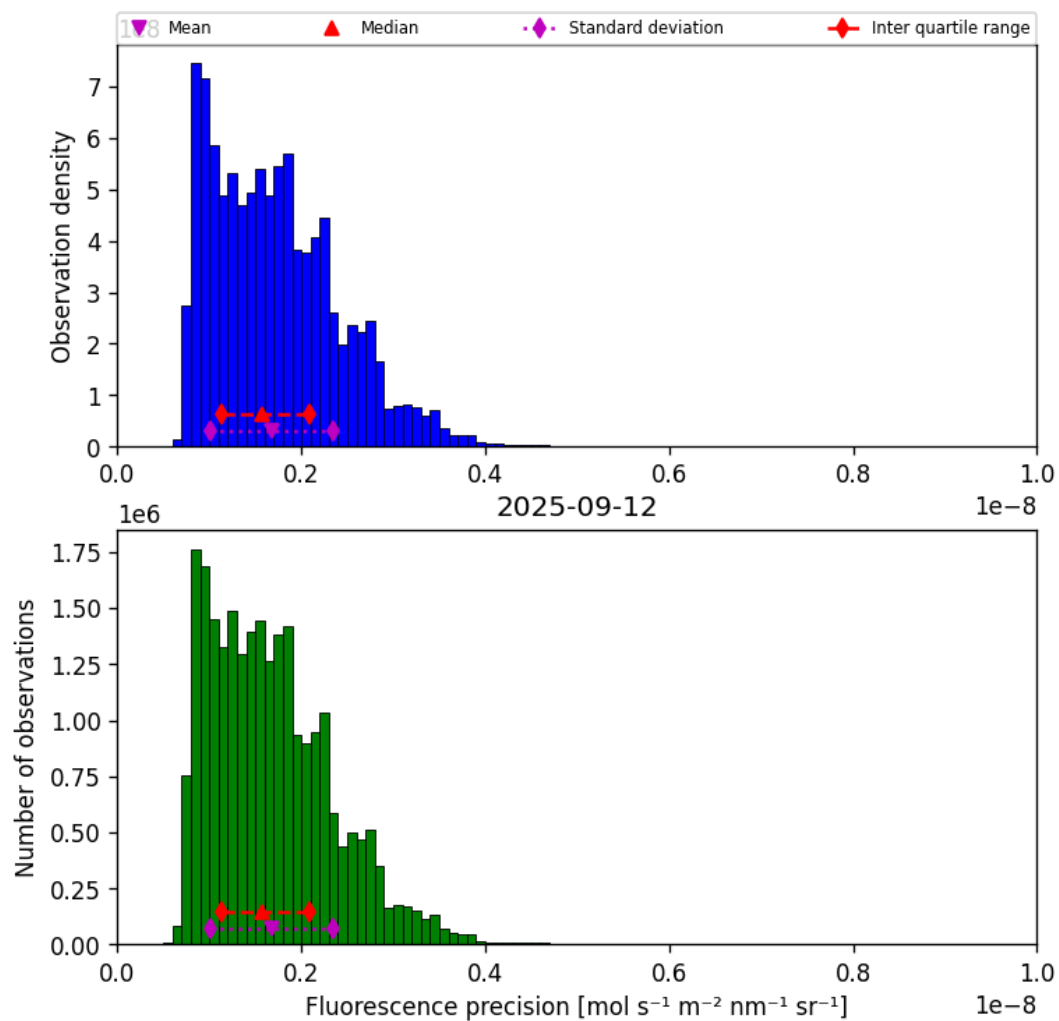
Figure 41: Histogram of “Fluorescence precision” for 2025-09-11 to 2025-09-13
