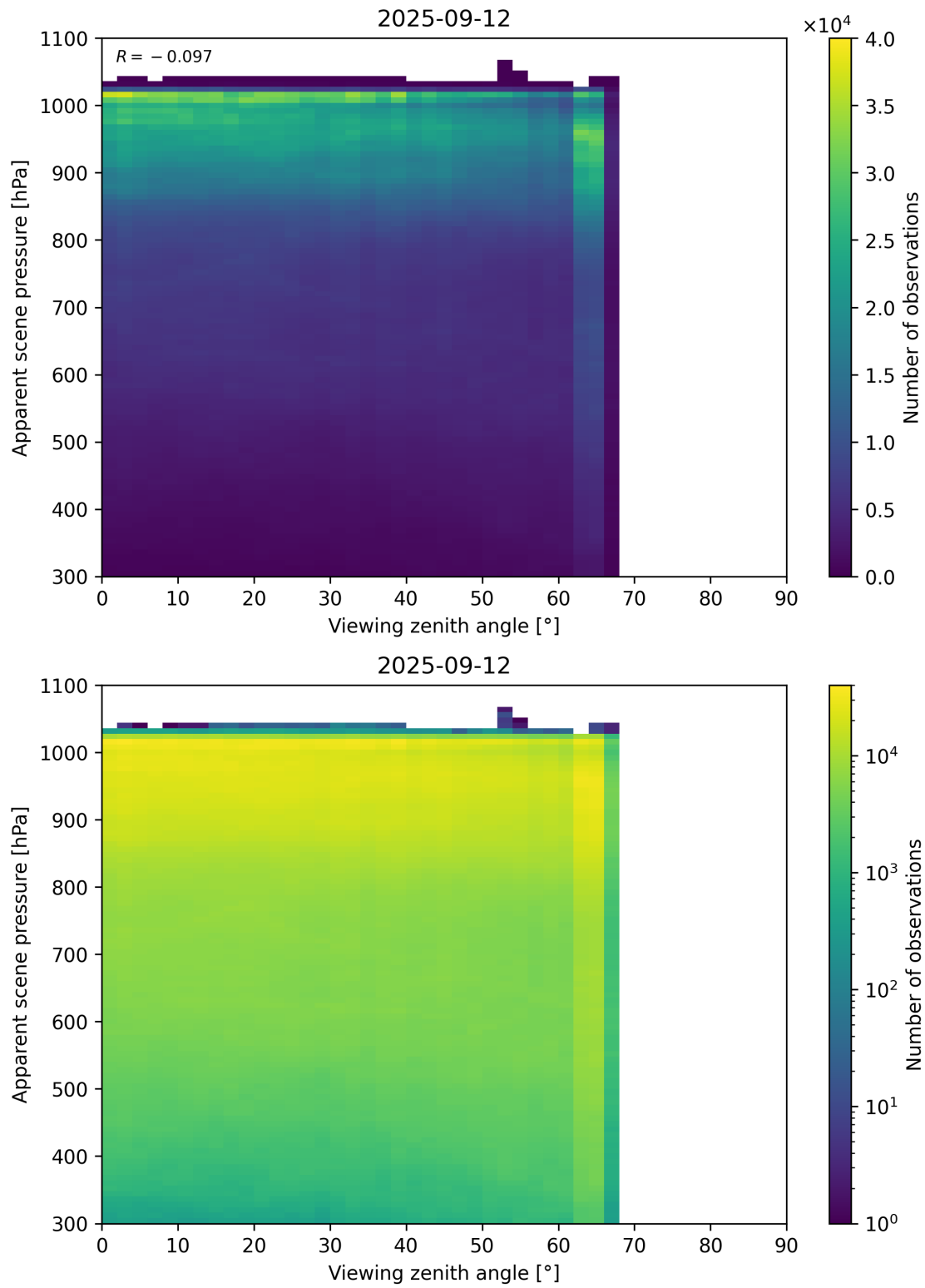
Figure 118: Scatter density plot of “Viewing zenith angle” against “Apparent scene pressure” for 2025-09-11 to 2025-09-13.
