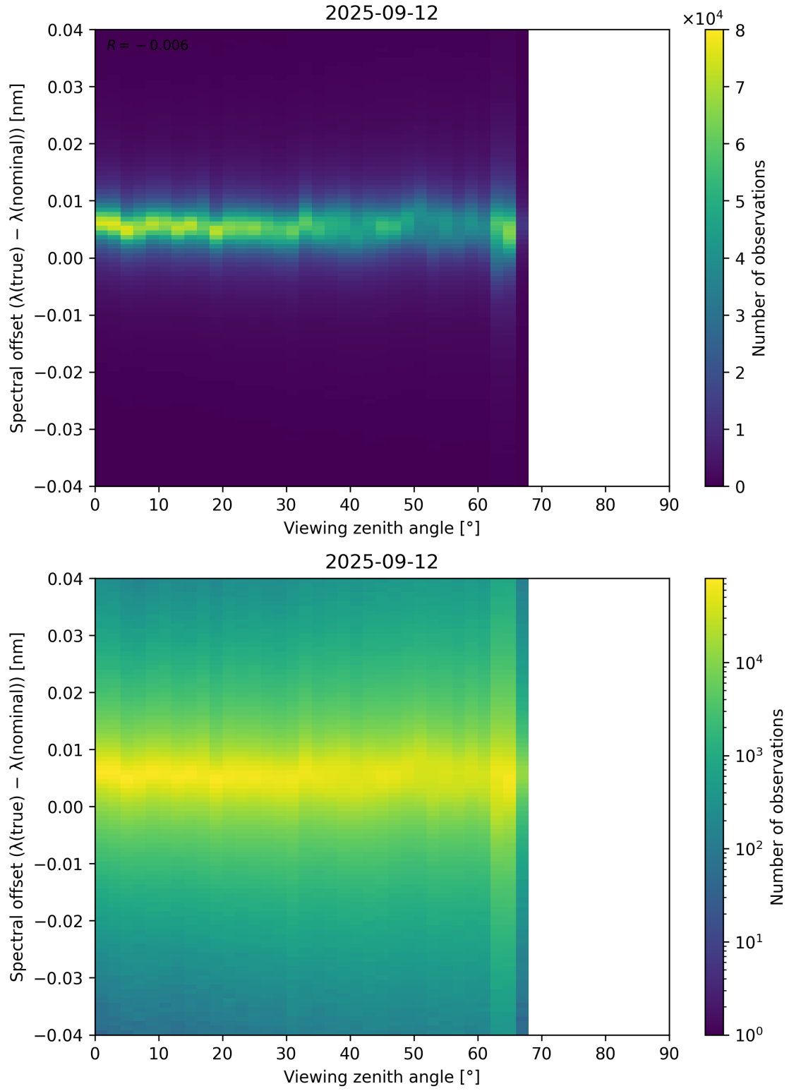
Figure 128: Scatter density plot of “Viewing zenith angle” against “Spectral offset ( \lambda_{\text{true}} - \lambda_{\text{nominal}} )” for 2025-09-11 to 2025-09-13.
