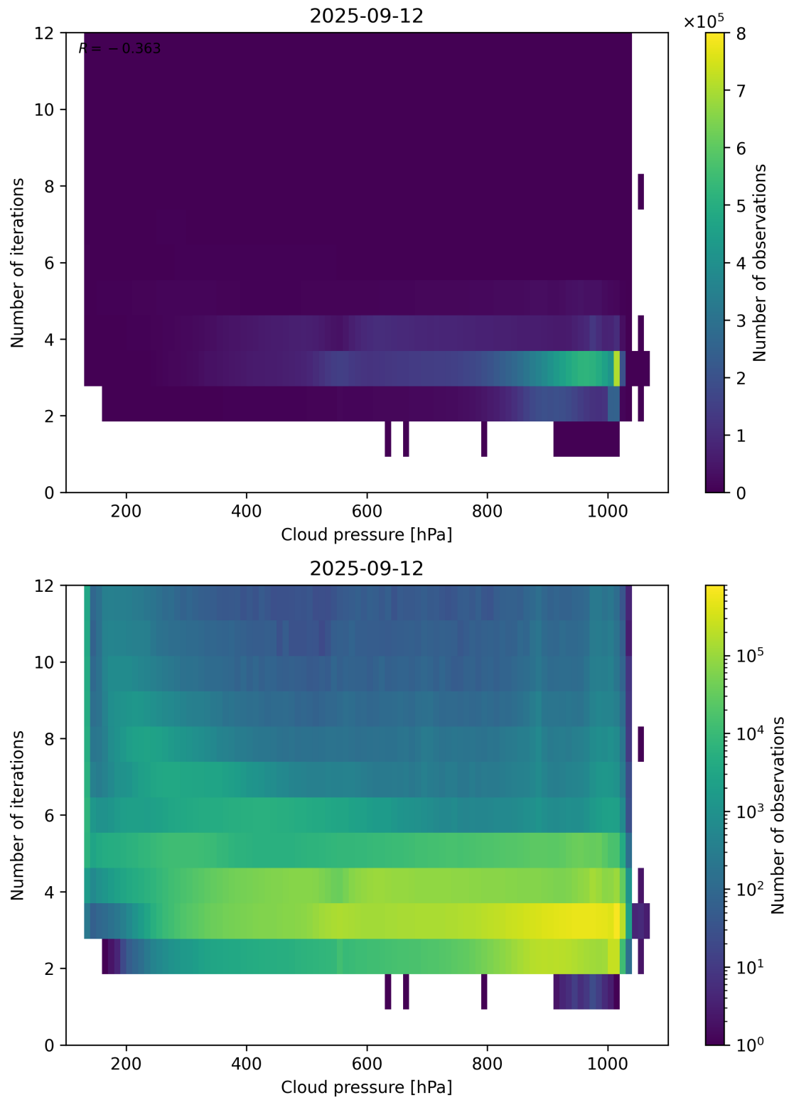
Figure 81: Scatter density plot of “Cloud pressure” against “Number of iterations” for 2025-09-11 to 2025-09-13.
