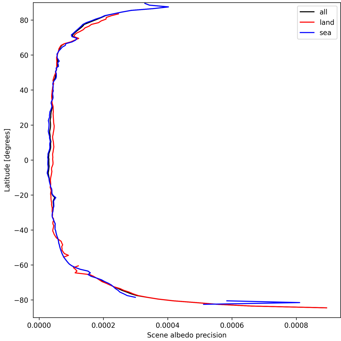
Figure 18: Zonal average of “Scene albedo precision” for 2025-09-11 to 2025-09-13.
