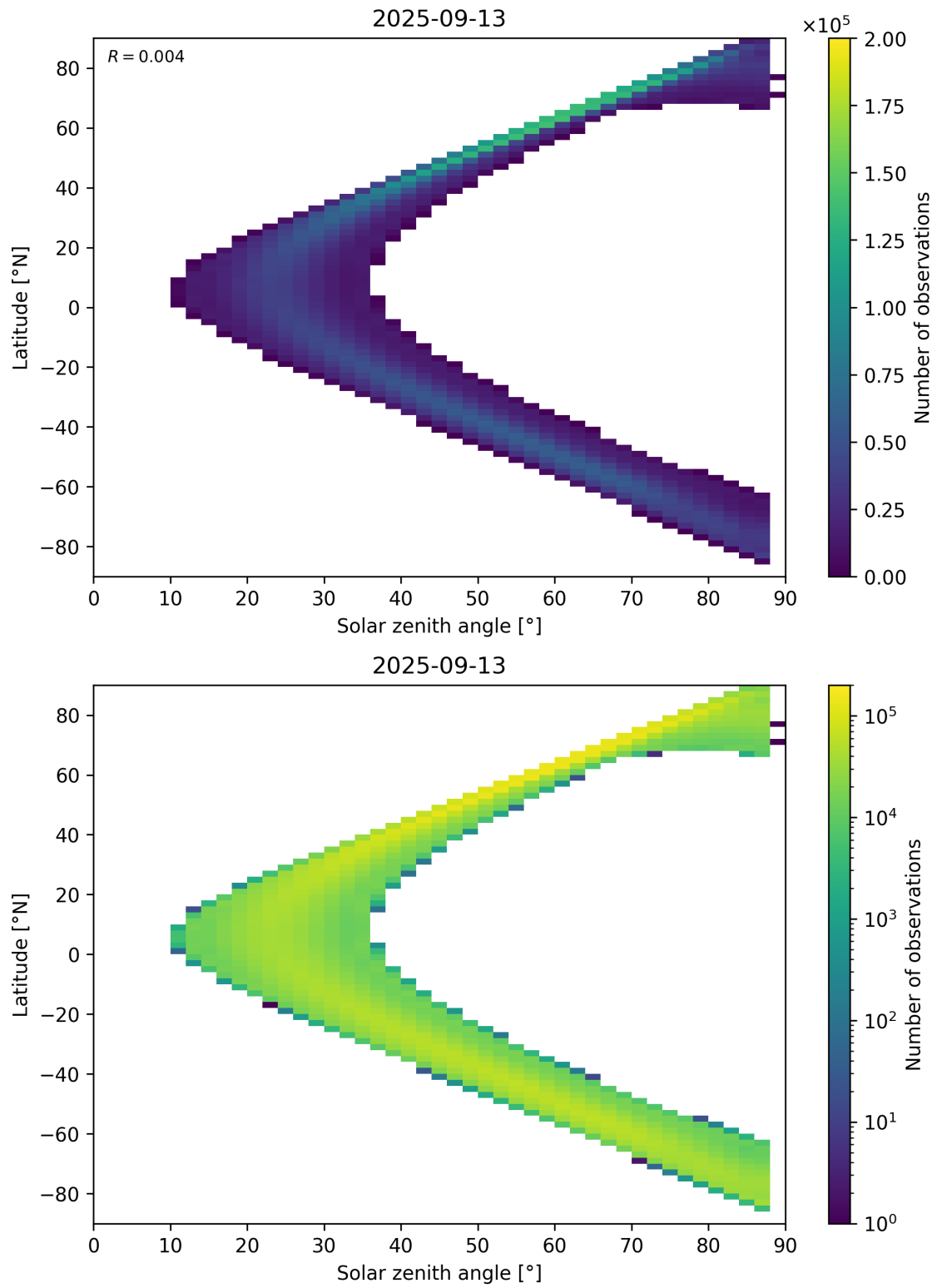
Figure 113: Scatter density plot of “Solar zenith angle” against “Latitude” for 2025-09-12 to 2025-09-14.
