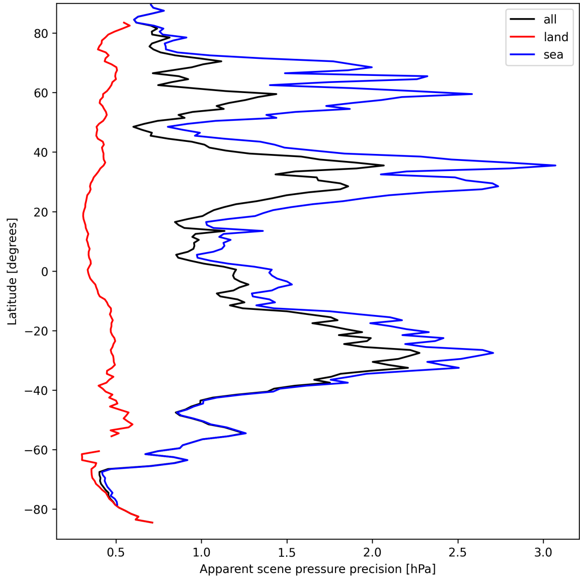
Figure 20: Zonal average of “Apparent scene pressure precision” for 2025-09-12 to 2025-09-14.
