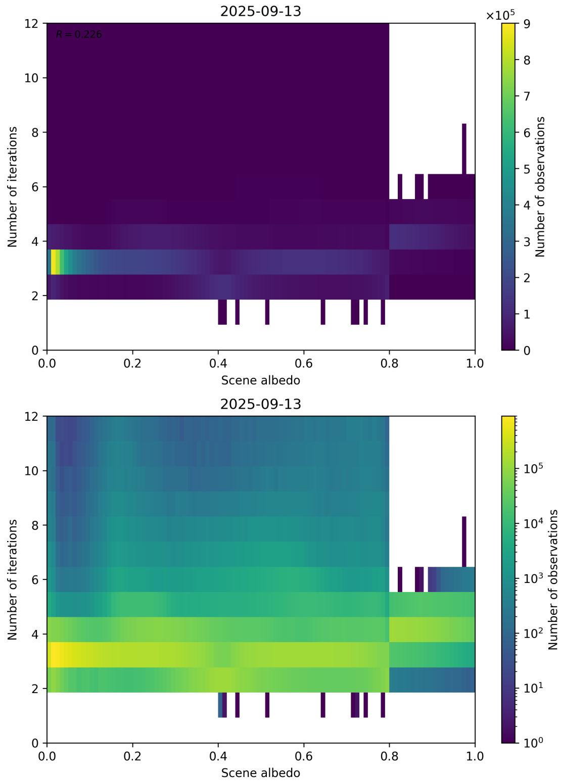
Figure 105: Scatter density plot of “Scene albedo” against “Number of iterations” for 2025-09-12 to 2025-09-14.
