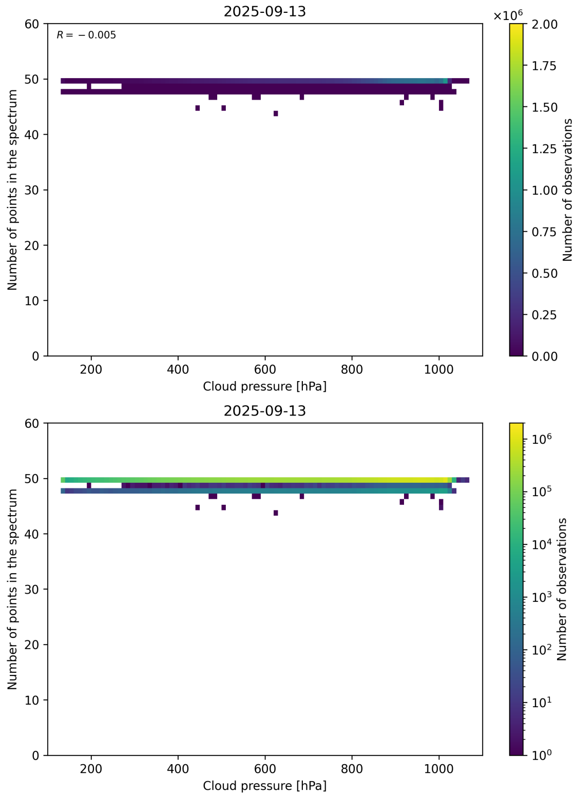
Figure 82: Scatter density plot of “Cloud pressure” against “Number of points in the spectrum” for 2025-09-12 to 2025-09-14.
