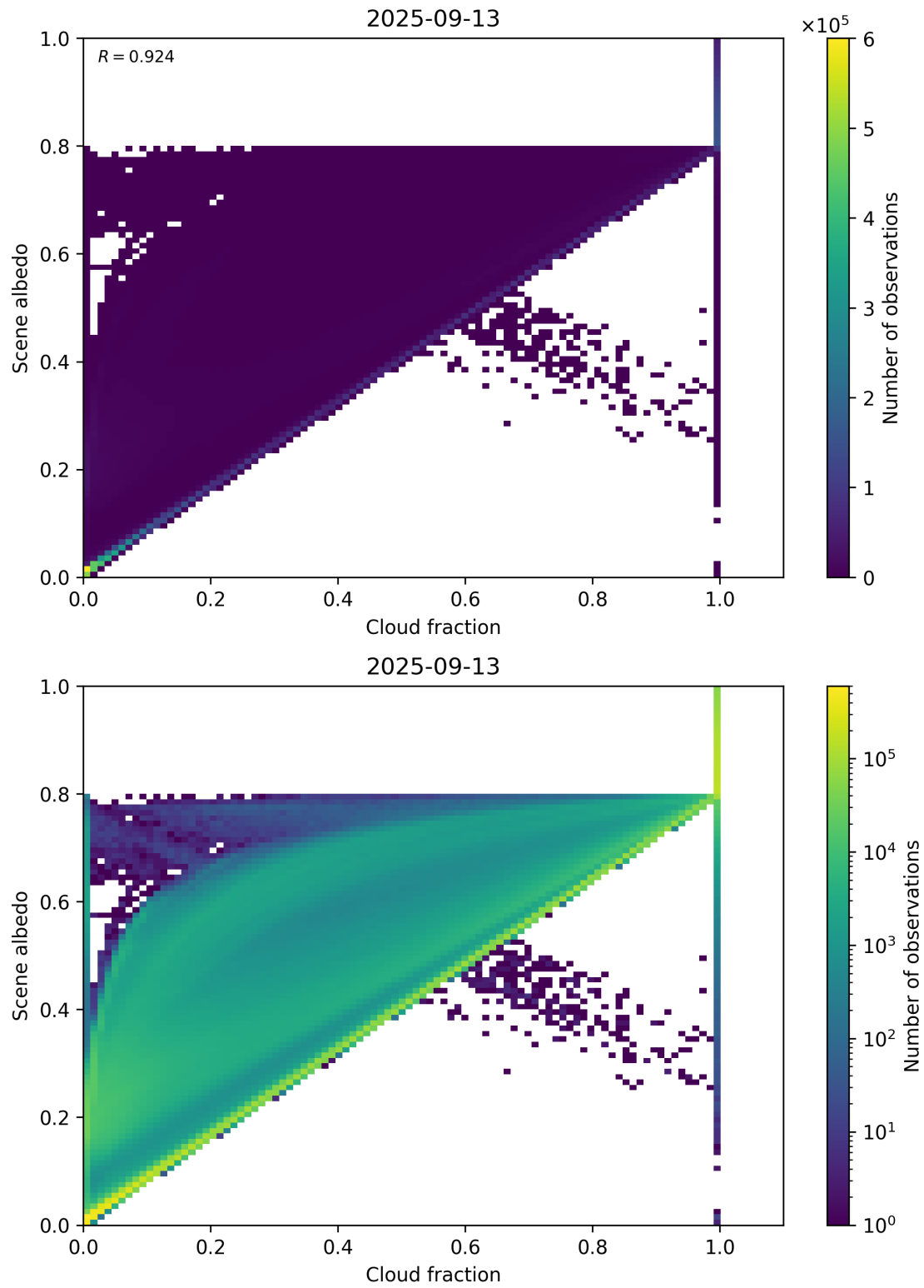
Figure 75: Scatter density plot of “Cloud fraction” against “Scene albedo” for 2025-09-12 to 2025-09-14.
