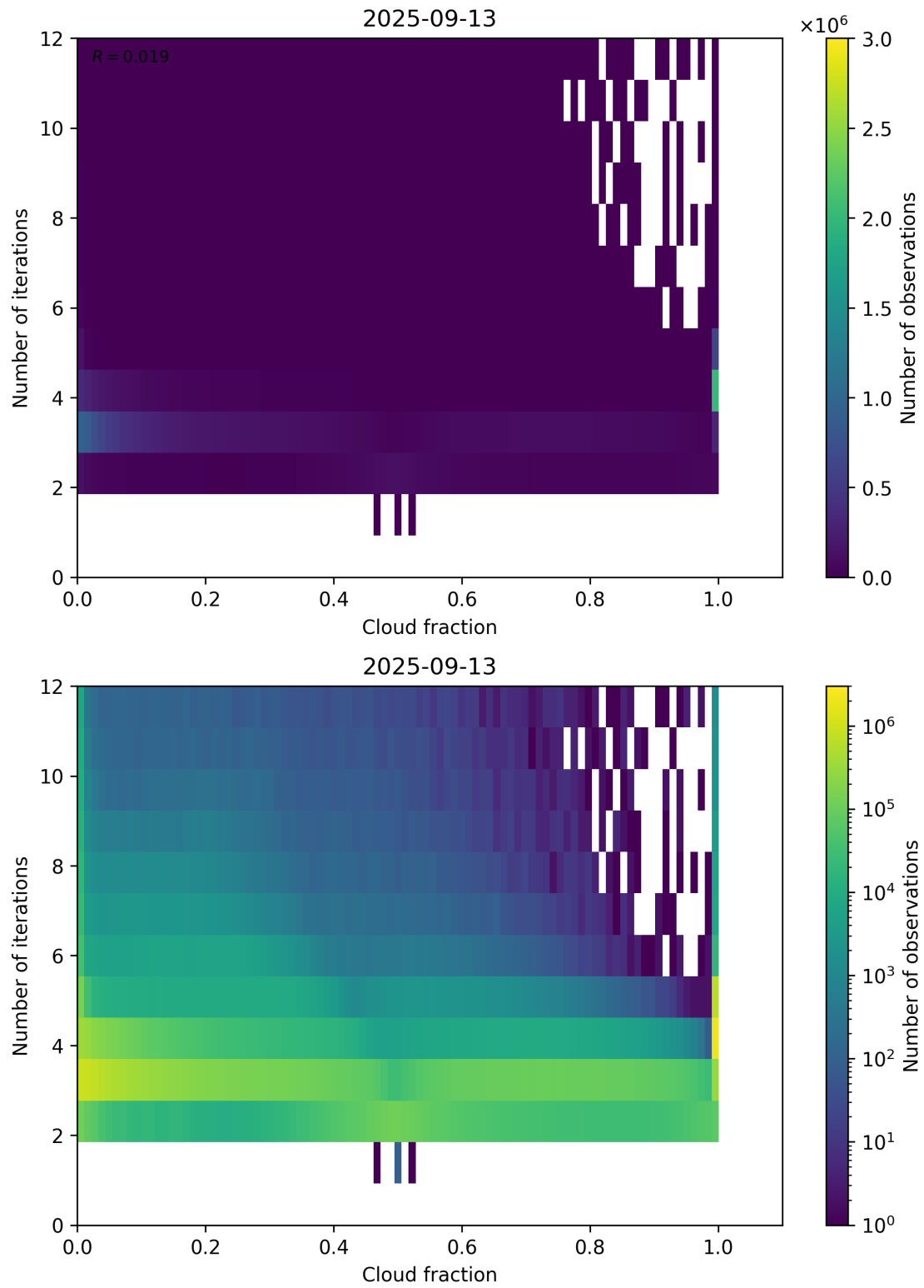
Figure 73: Scatter density plot of “Cloud fraction” against “Number of iterations” for 2025-09-12 to 2025-09-14.
