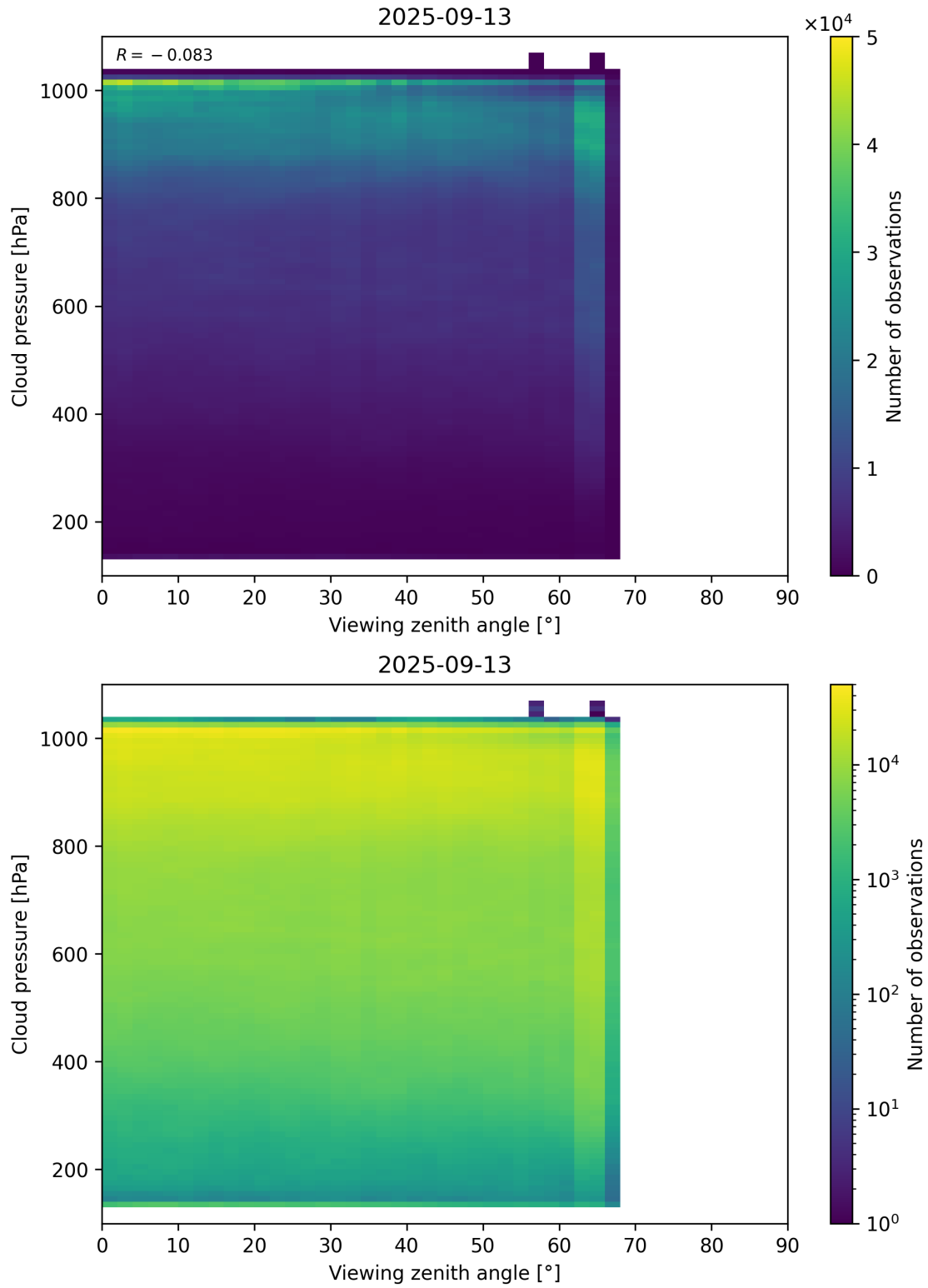
Figure 121: Scatter density plot of “Viewing zenith angle” against “Cloud pressure” for 2025-09-12 to 2025-09-14.
