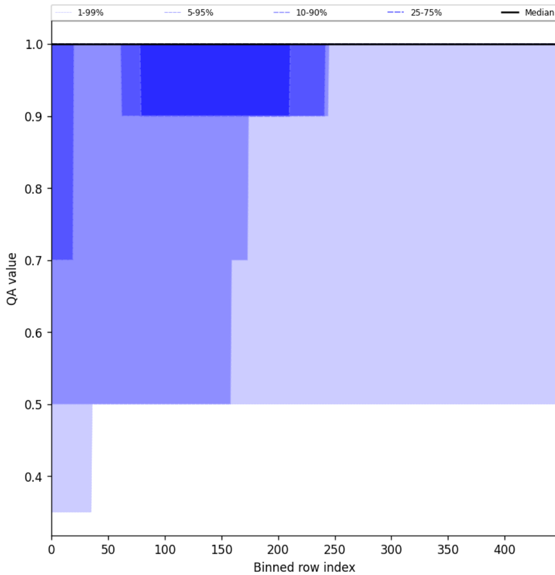
Figure 46: Along track statistics of “QA value” for 2025-09-12 to 2025-09-14
