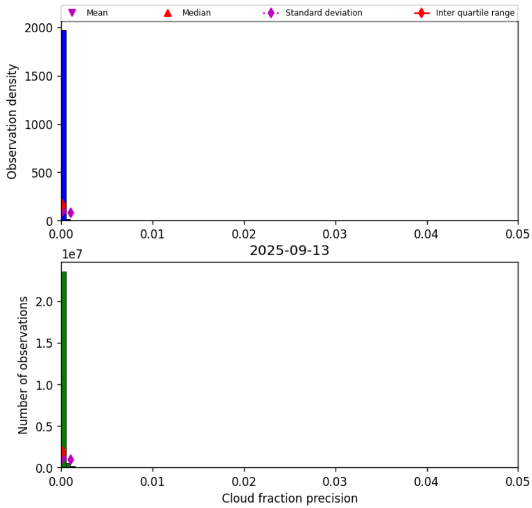
Figure 33: Histogram of “Cloud fraction precision” for 2025-09-12 to 2025-09-14
