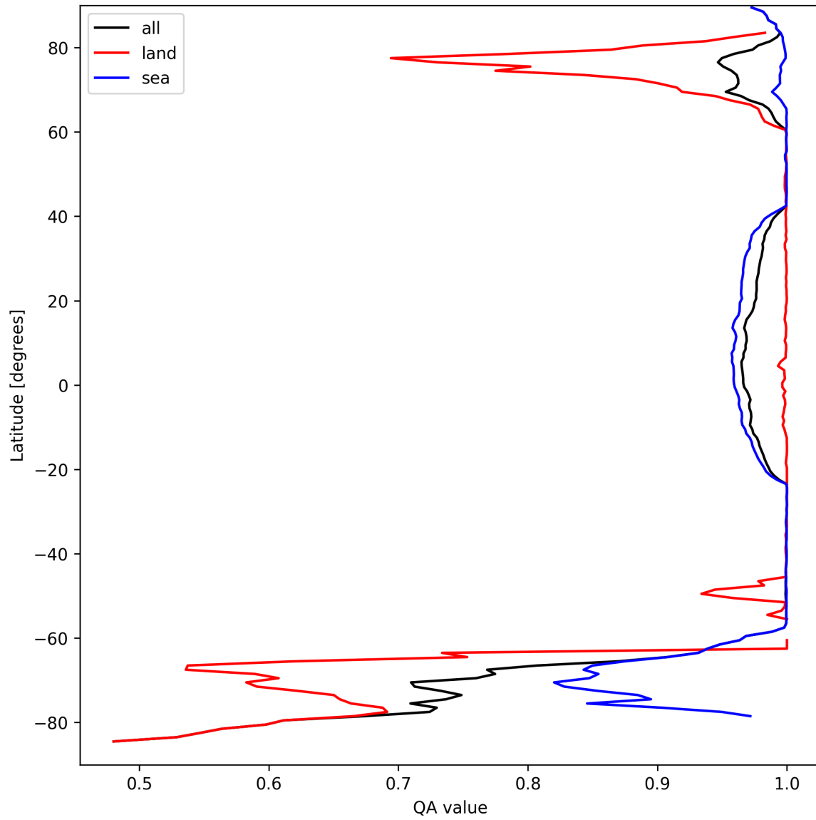
Figure 12: Zonal average of "QA value" for 2025-09-12 to 2025-09-14.
