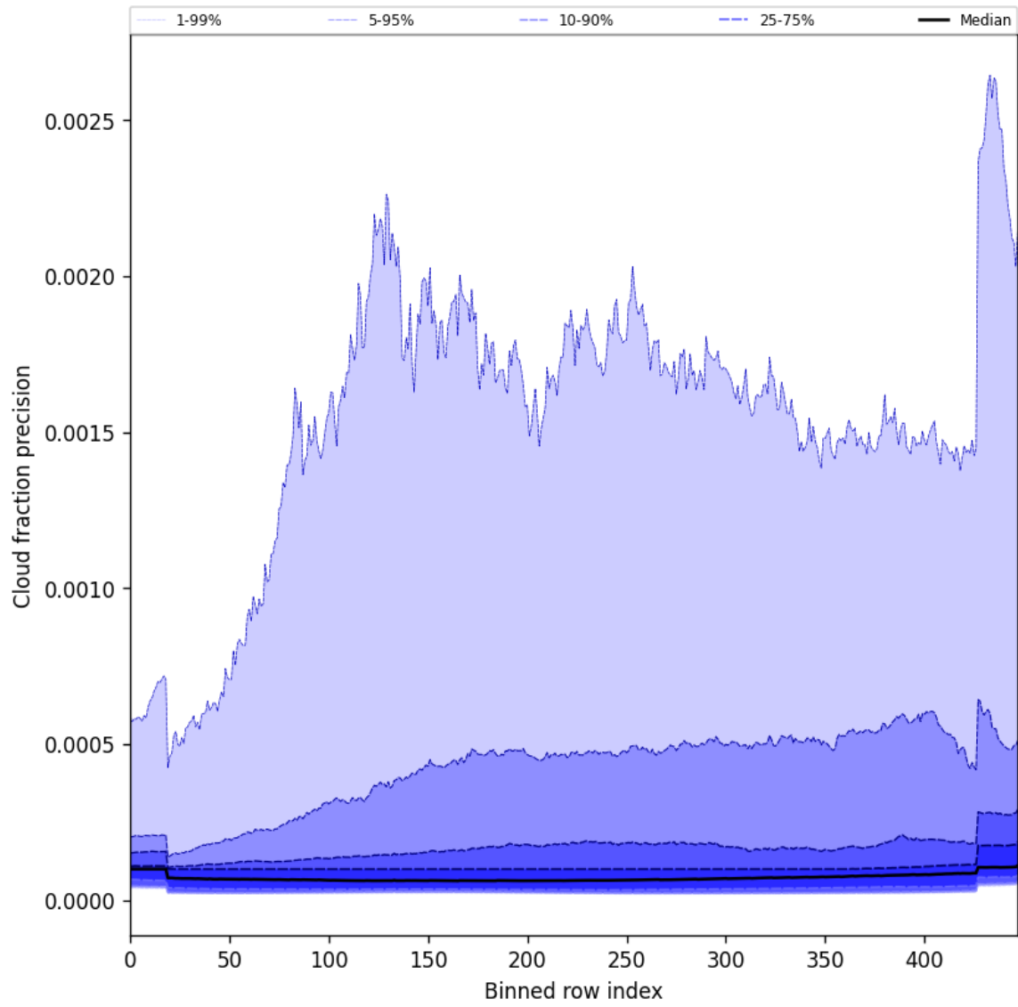
Figure 50: Along track statistics of “Cloud fraction precision” for 2025-09-12 to 2025-09-14
