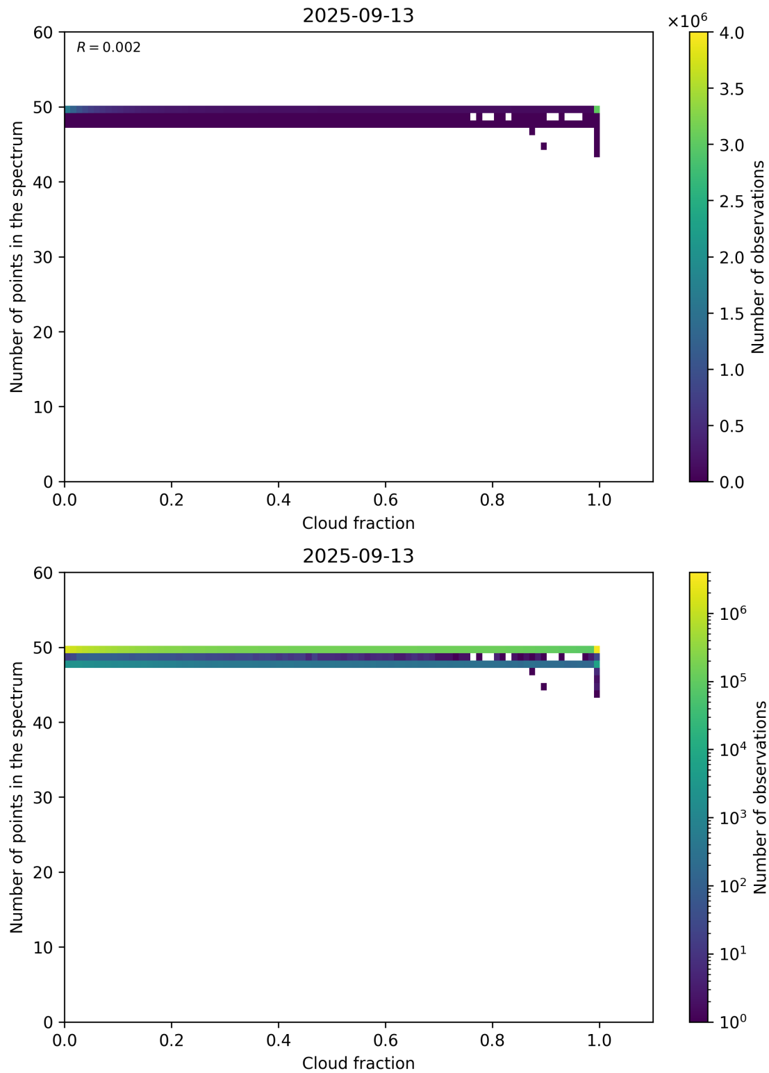
Figure 74: Scatter density plot of “Cloud fraction” against “Number of points in the spectrum” for 2025-09-12 to 2025-09-14.
