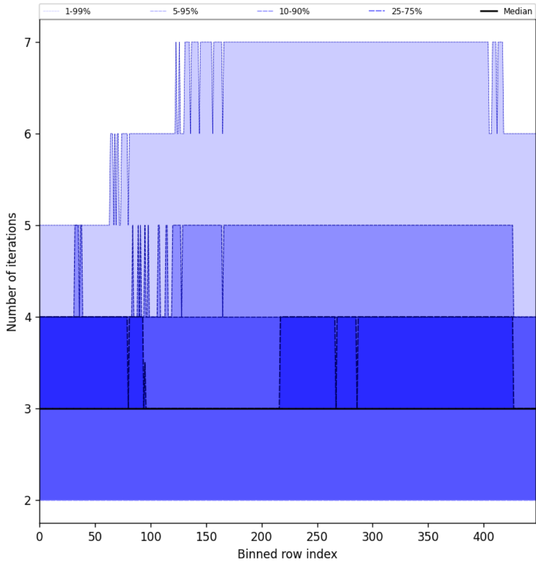
Figure 56: Along track statistics of “Number of iterations” for 2025-09-12 to 2025-09-14
