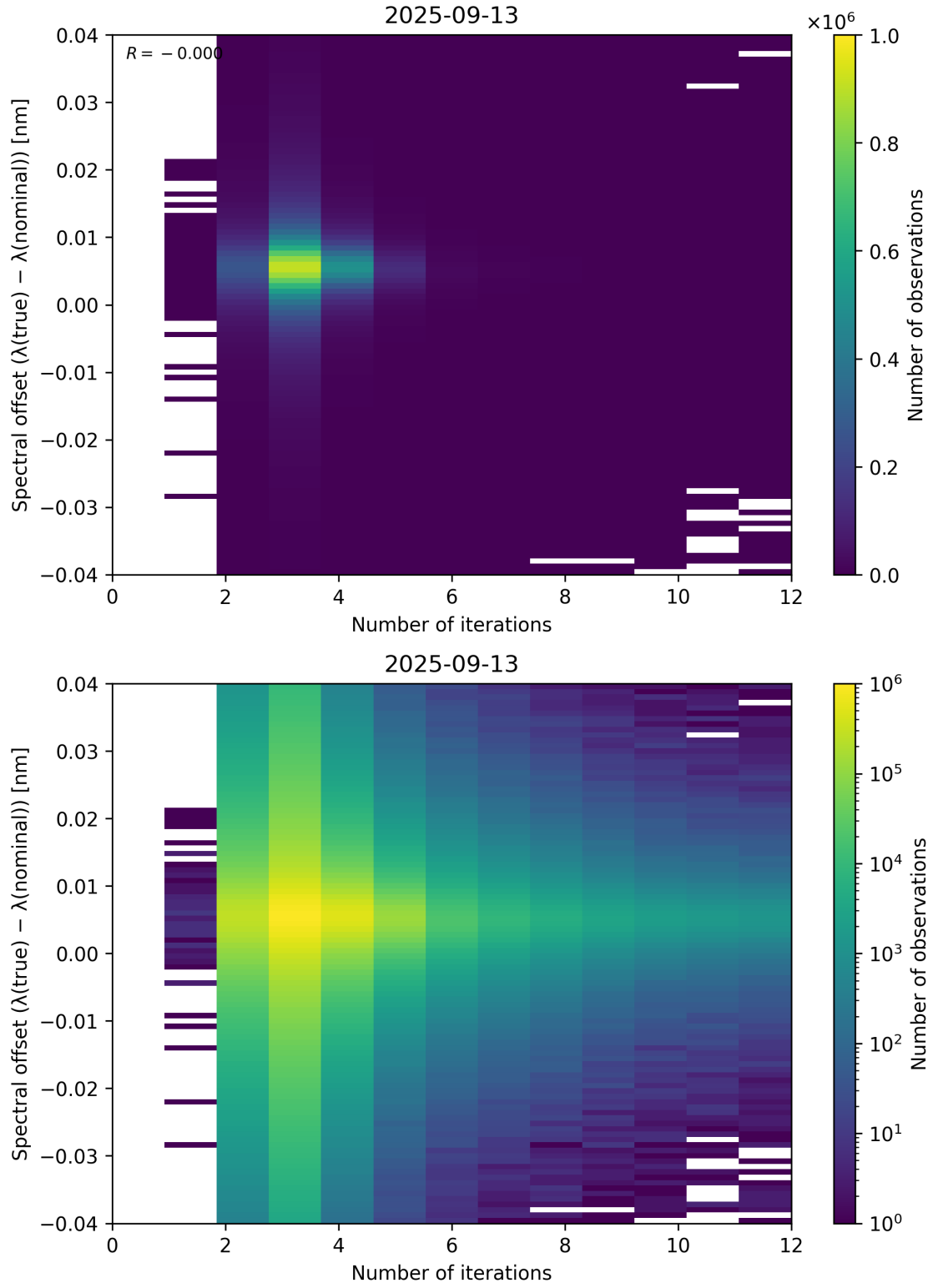
Figure 100: Scatter density plot of “Number of iterations” against “Spectral offset ( \lambda_{\text{true}} - \lambda_{\text{nominal}} )” for 2025-09-12 to 2025-09-14.
