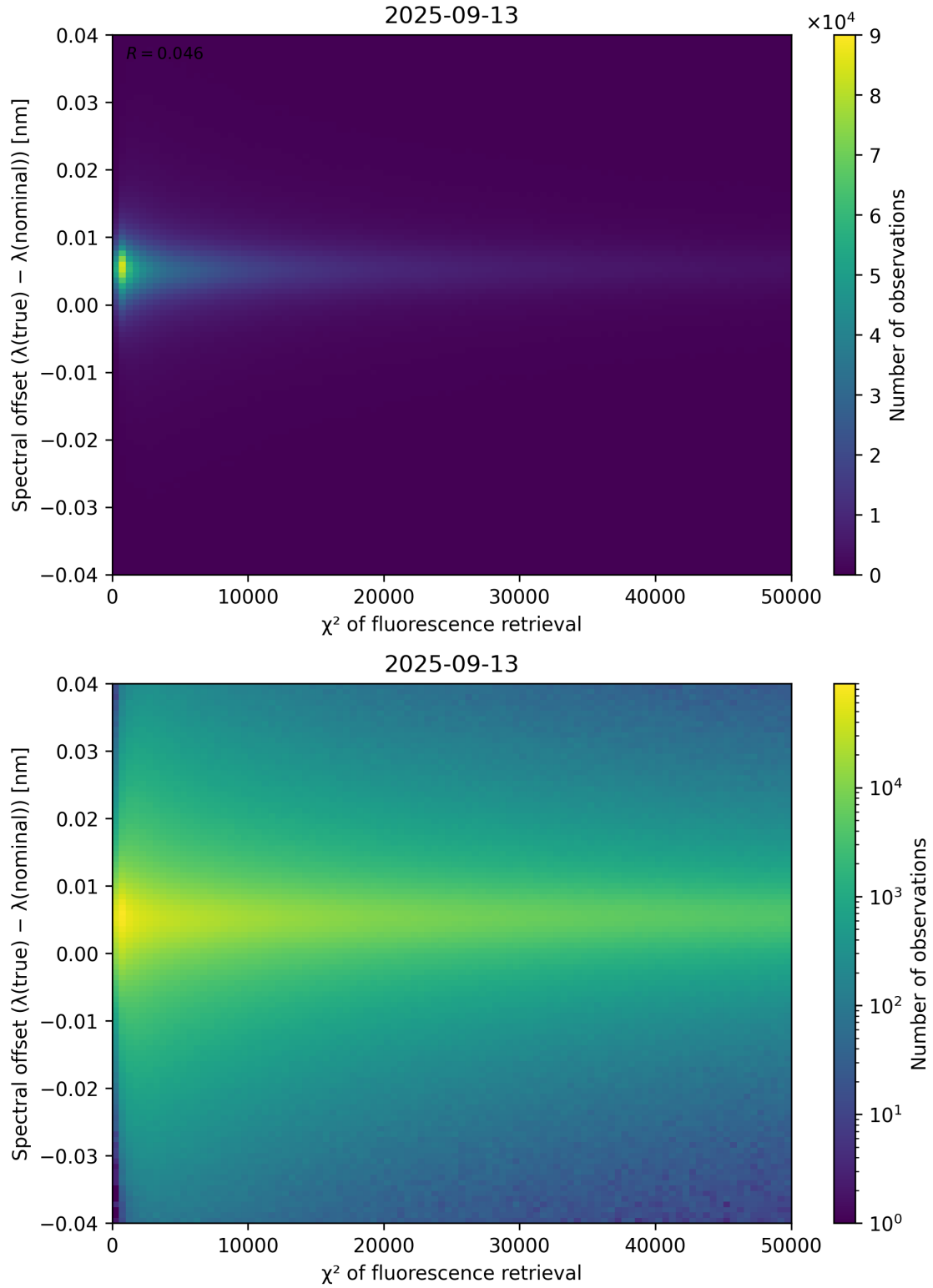
Figure 69: Scatter density plot of “ \chi^2 of fluorescence retrieval” against “Spectral offset ( \lambda_{\text{true}} - \lambda_{\text{nominal}} )” for 2025-09-12 to 2025-09-14.
