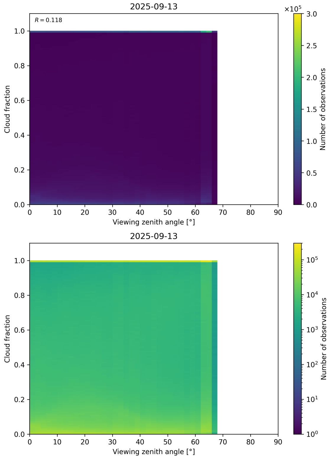
Figure 120: Scatter density plot of “Viewing zenith angle” against “Cloud fraction” for 2025-09-12 to 2025-09-14.
