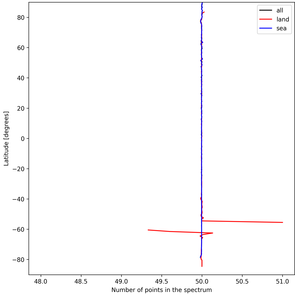
Figure 27: Zonal average of “Number of points in the spectrum” for 2025-09-12 to 2025-09-14.
