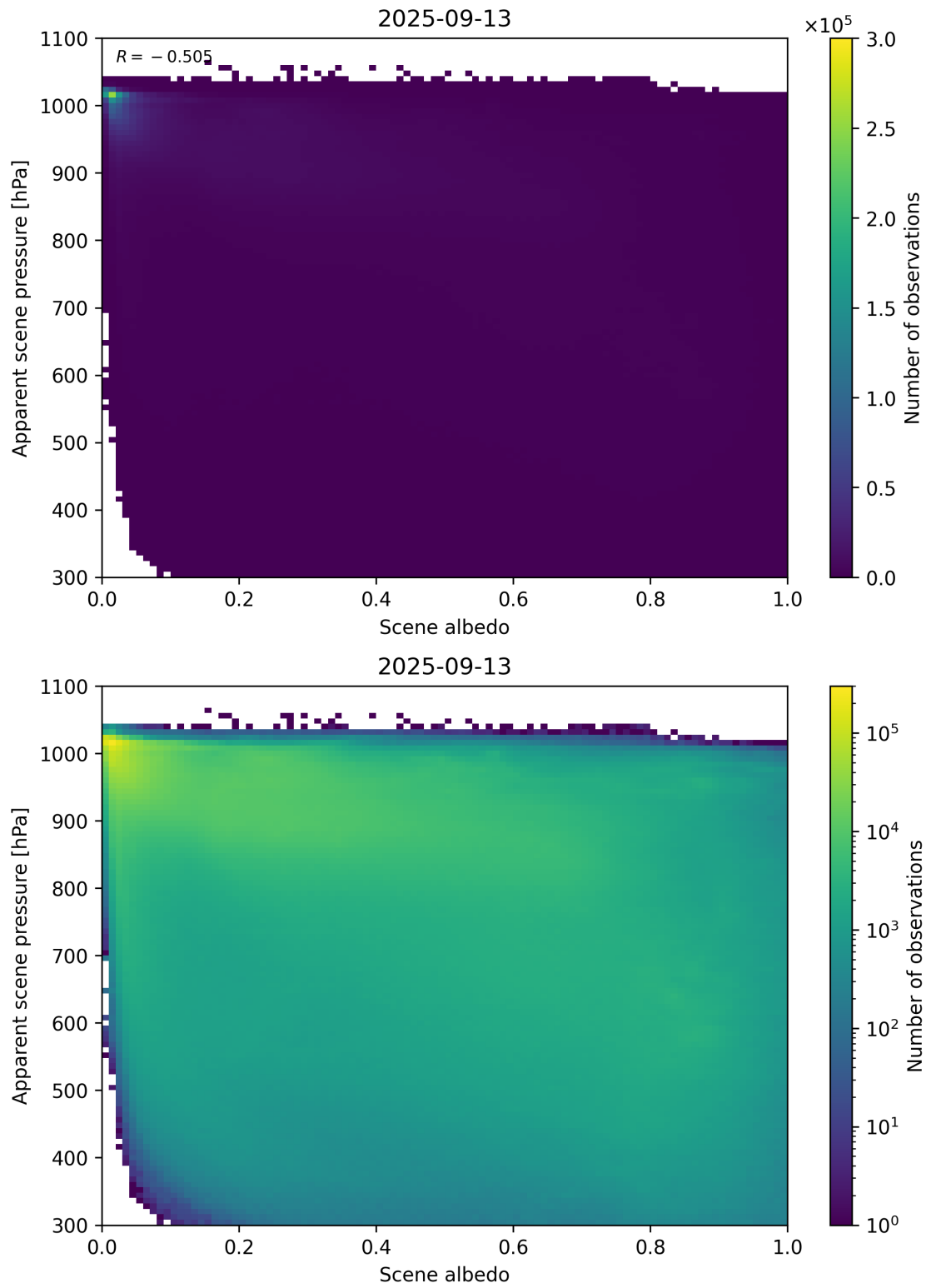
Figure 102: Scatter density plot of “Scene albedo” against “Apparent scene pressure” for 2025-09-12 to 2025-09-14.
