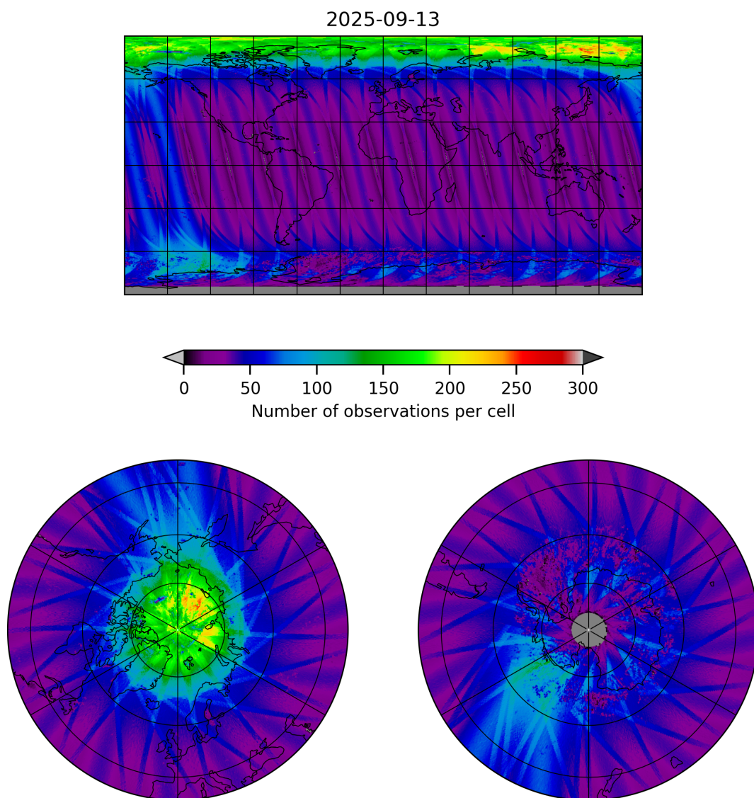
Figure 11: Map of the number of observations for 2025-09-12 to 2025-09-14
