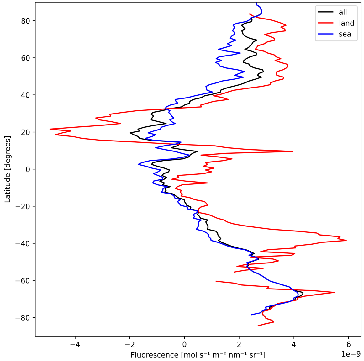
Figure 23: Zonal average of “Fluorescence” for 2025-09-12 to 2025-09-14.
