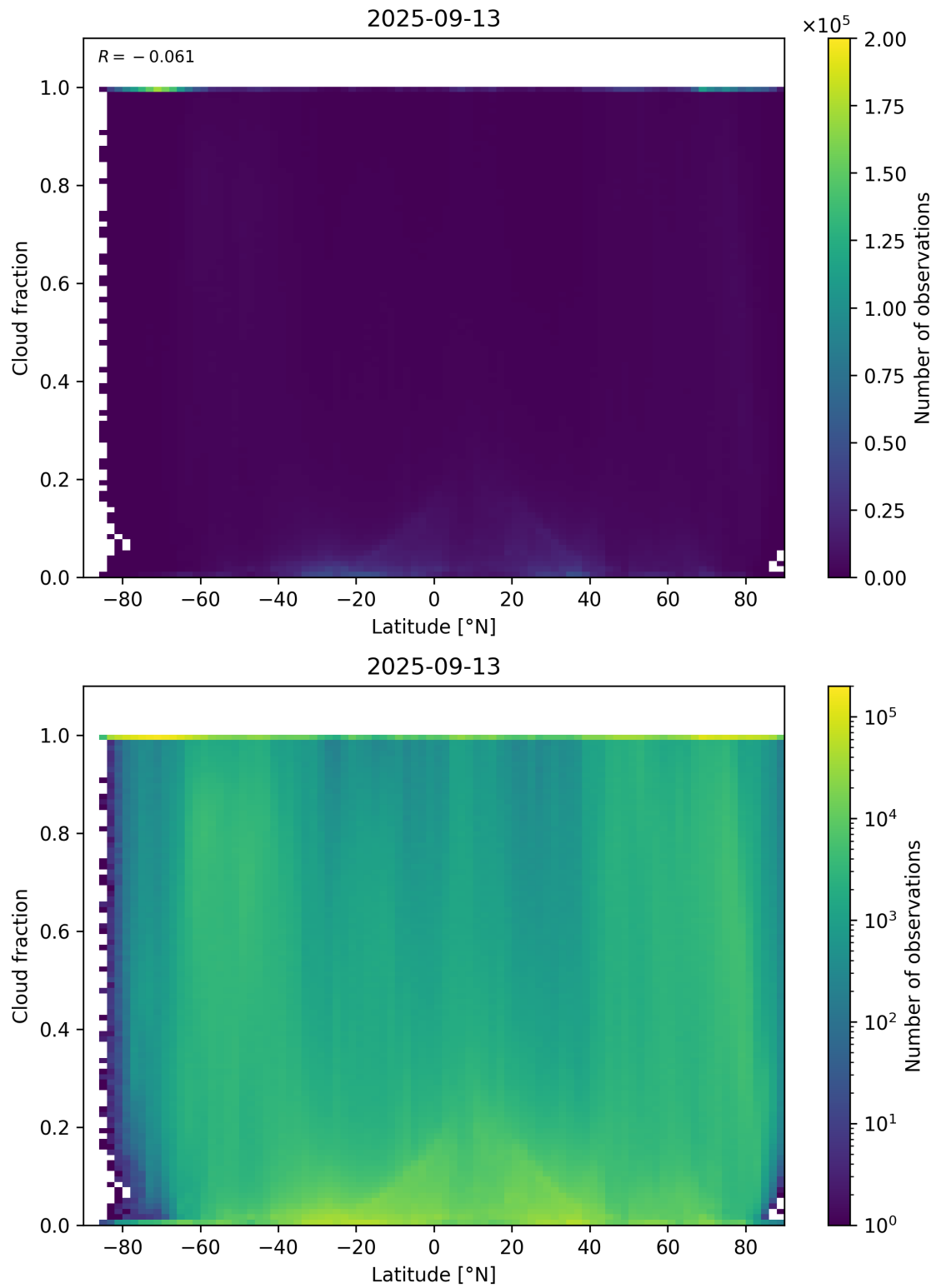
Figure 90: Scatter density plot of “Latitude” against “Cloud fraction” for 2025-09-12 to 2025-09-14.
