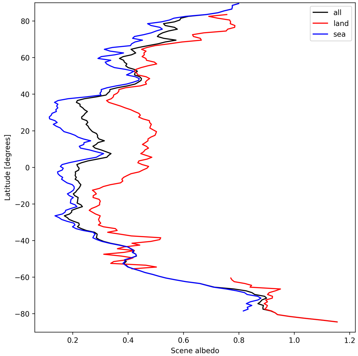
Figure 17: Zonal average of “Scene albedo” for 2025-09-12 to 2025-09-14.
