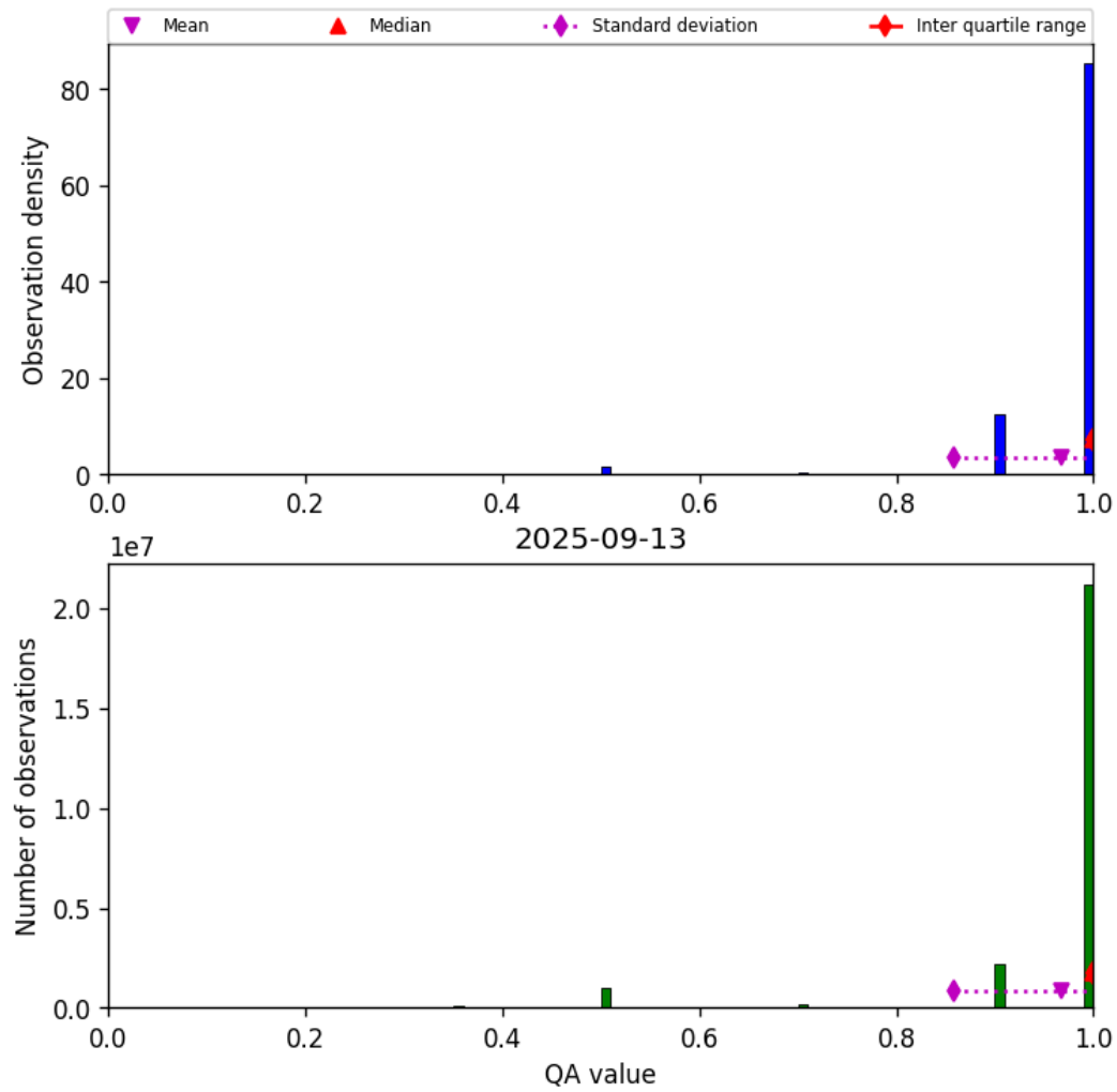
Figure 29: Histogram of “QA value” for 2025-09-12 to 2025-09-14
