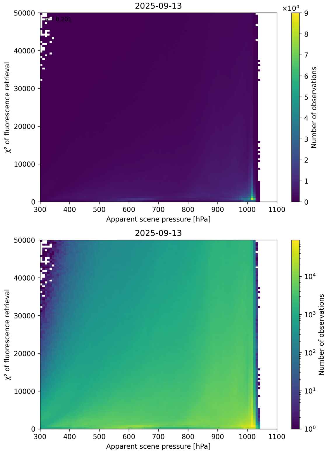
Figure 63: Scatter density plot of “Apparent scene pressure” against “ \chi^2 of fluorescence retrieval” for 2025-09-12 to 2025-09-14.
