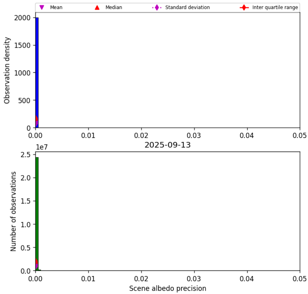
Figure 35: Histogram of “Scene albedo precision” for 2025-09-12 to 2025-09-14
