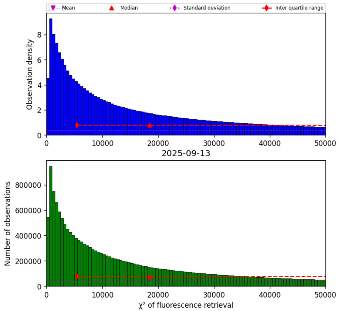
Figure 42: Histogram of “ \chi^2 of fluorescence retrieval” for 2025-09-12 to 2025-09-14
