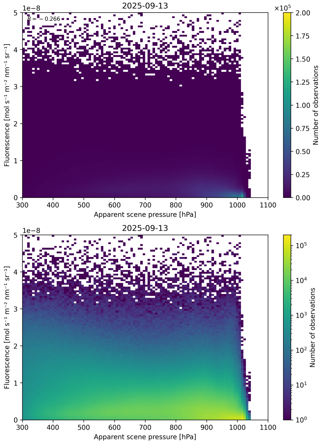
Figure 64: Scatter density plot of “Apparent scene pressure” against “Fluorescence” for 2025-09-12 to 2025-09-14.
