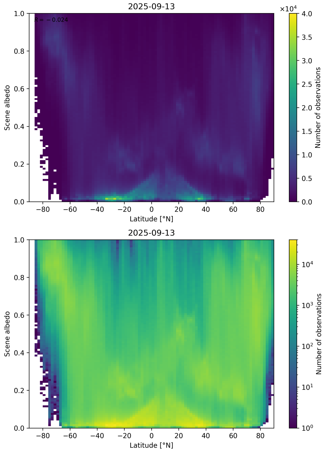
Figure 95: Scatter density plot of “Latitude” against “Scene albedo” for 2025-09-12 to 2025-09-14.
