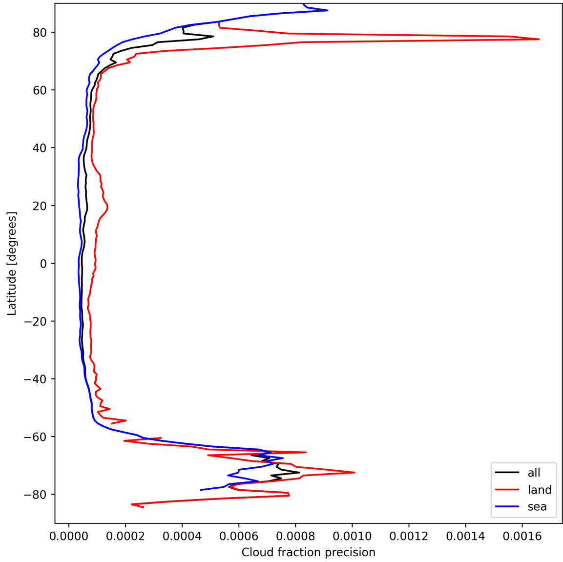
Figure 16: Zonal average of “Cloud fraction precision” for 2025-09-12 to 2025-09-14.
