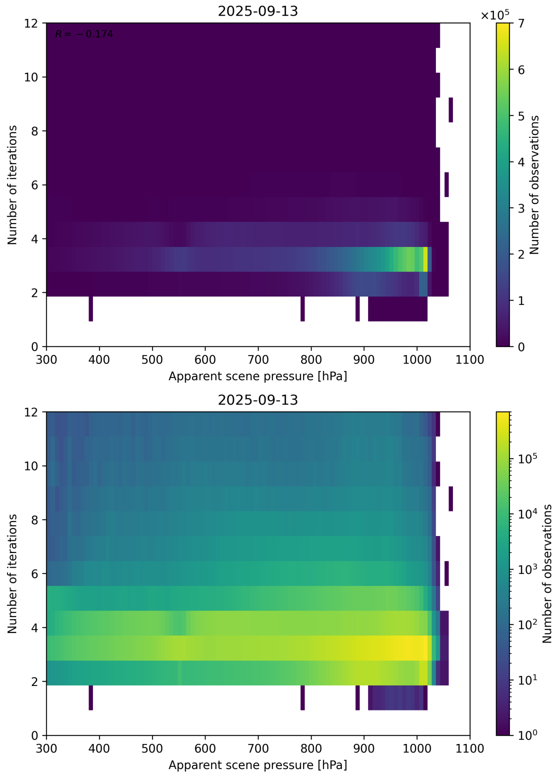
Figure 65: Scatter density plot of “Apparent scene pressure” against “Number of iterations” for 2025-09-12 to 2025-09-14.
