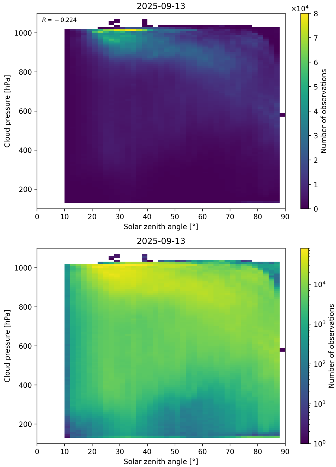
Figure 111: Scatter density plot of “Solar zenith angle” against “Cloud pressure” for 2025-09-12 to 2025-09-14.
