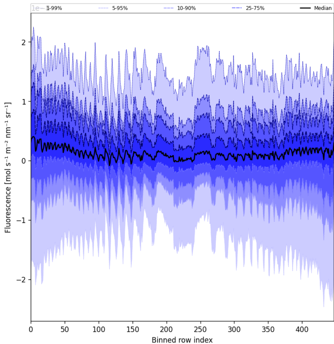
Figure 57: Along track statistics of “Fluorescence” for 2025-09-12 to 2025-09-14
