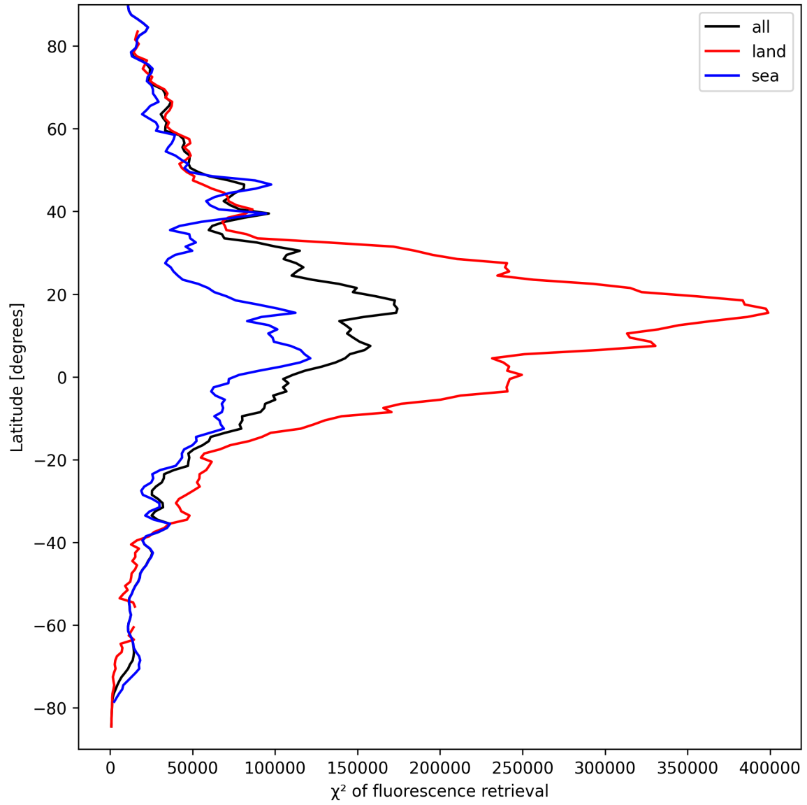
Figure 25: Zonal average of “ \chi^2 of fluorescence retrieval” for 2025-09-12 to 2025-09-14.
