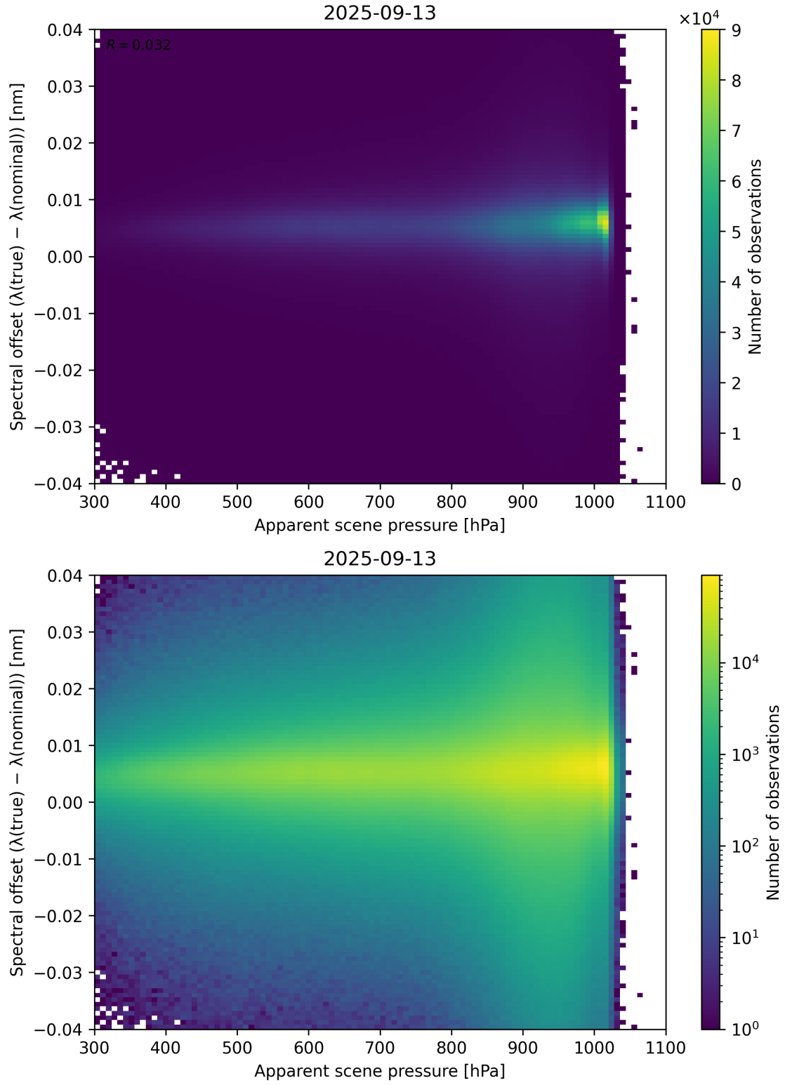
Figure 67: Scatter density plot of “Apparent scene pressure” against “Spectral offset ( \lambda_{\text{true}} - \lambda_{\text{nominal}} )” for 2025-09-12 to 2025-09-14.
