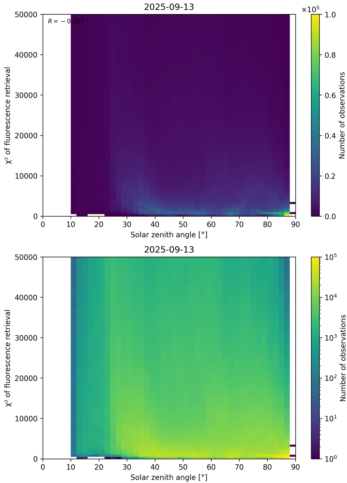
Figure 109: Scatter density plot of “Solar zenith angle” against “ \chi^2 of fluorescence retrieval” for 2025-09-12 to 2025-09-14.
