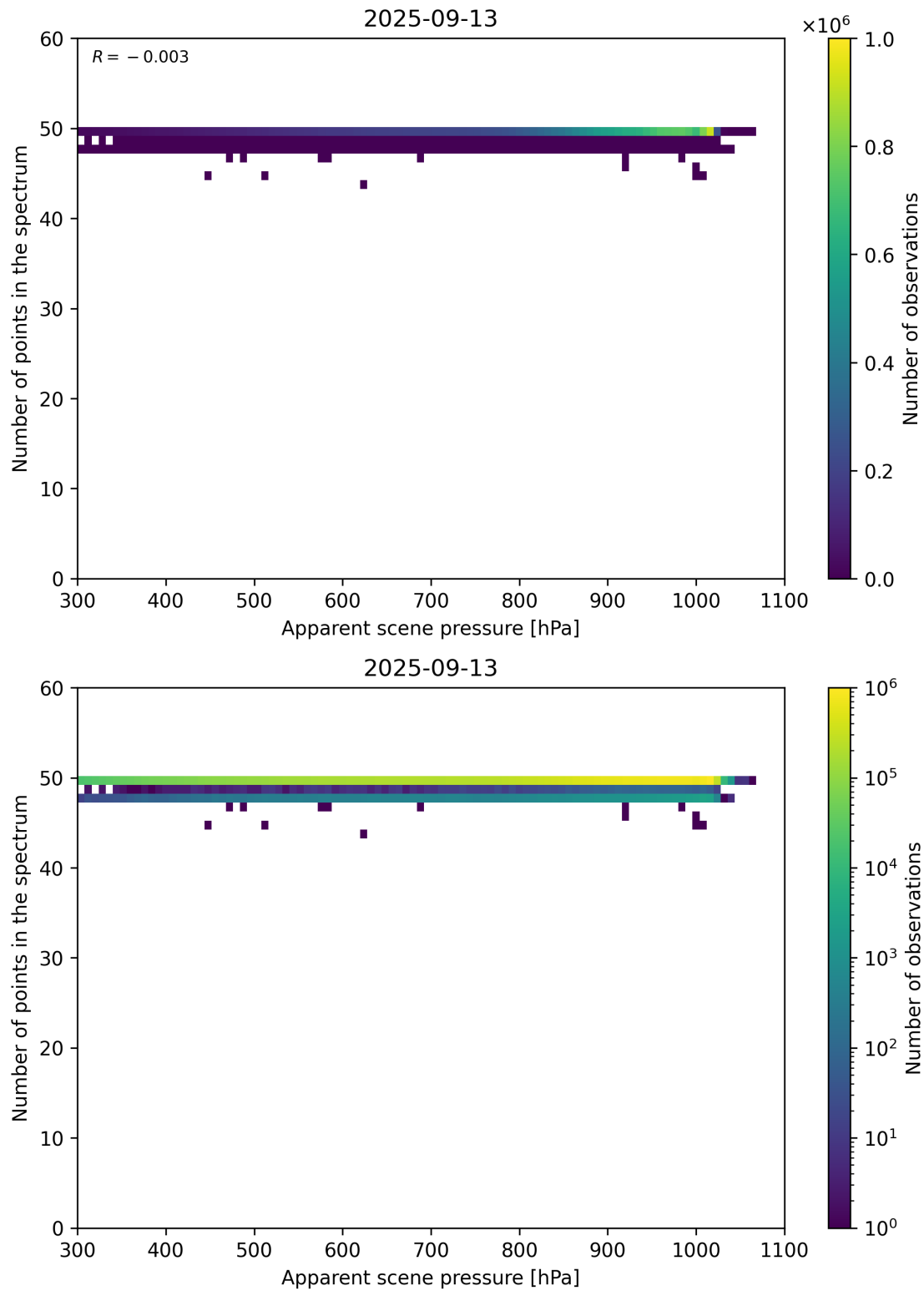
Figure 66: Scatter density plot of “Apparent scene pressure” against “Number of points in the spectrum” for 2025-09-12 to 2025-09-14.
