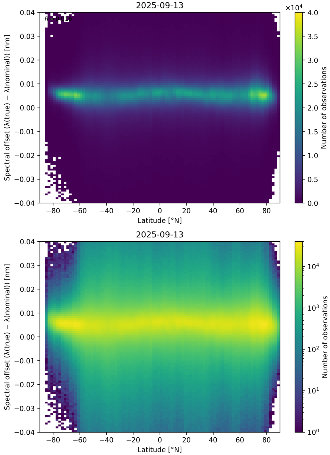
Figure 96: Scatter density plot of “Latitude” against “Spectral offset ( \lambda_{\text{true}} - \lambda_{\text{nominal}} )” for 2025-09-12 to 2025-09-14.
