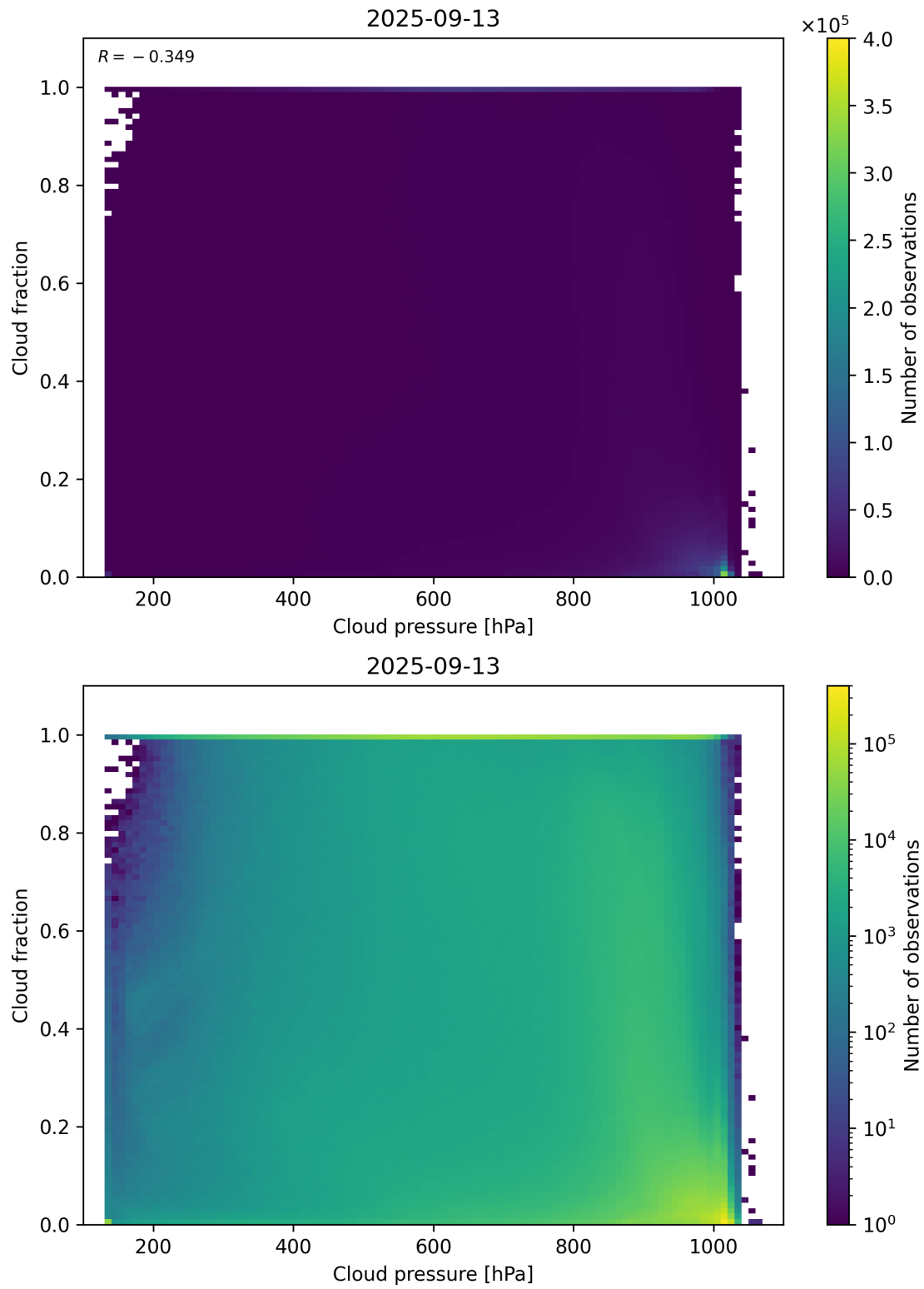
Figure 79: Scatter density plot of “Cloud pressure” against “Cloud fraction” for 2025-09-12 to 2025-09-14.
