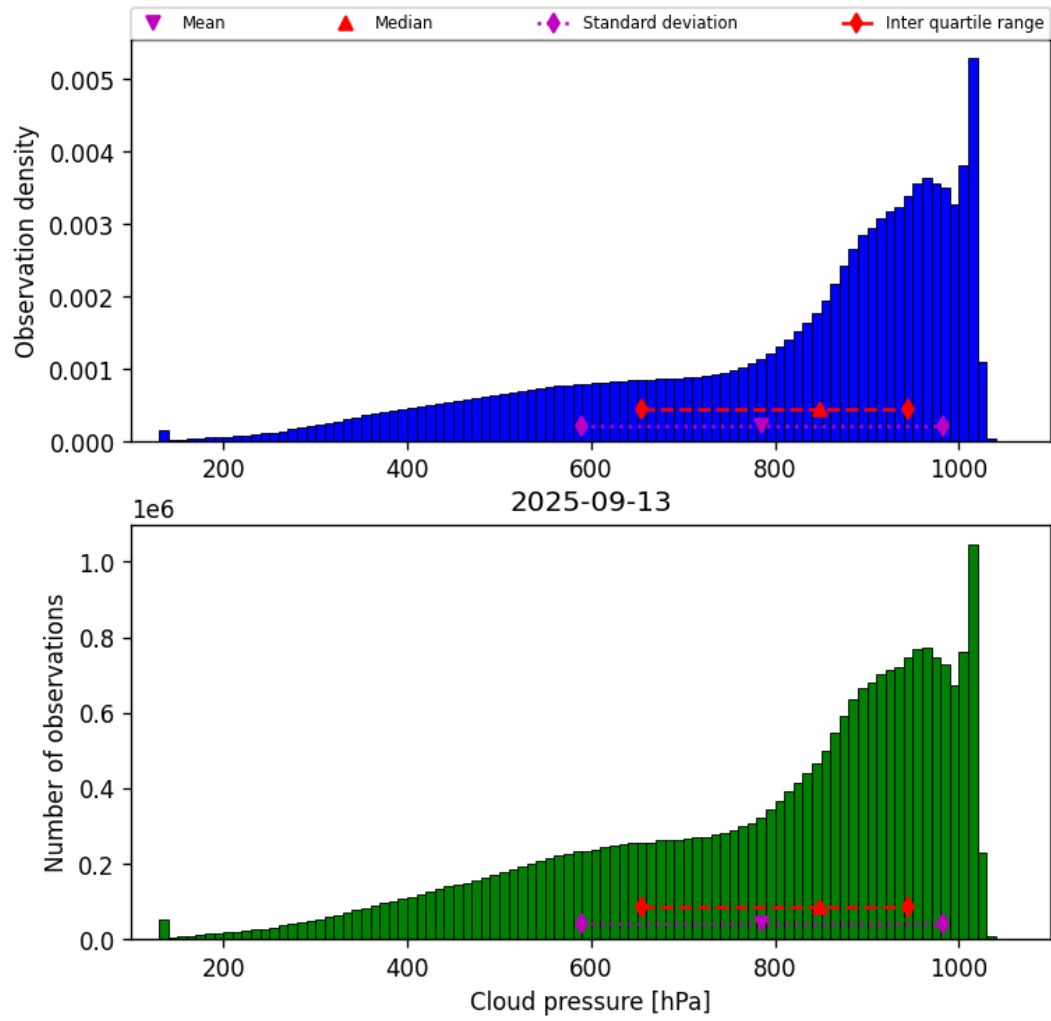
Figure 30: Histogram of “Cloud pressure” for 2025-09-12 to 2025-09-14
