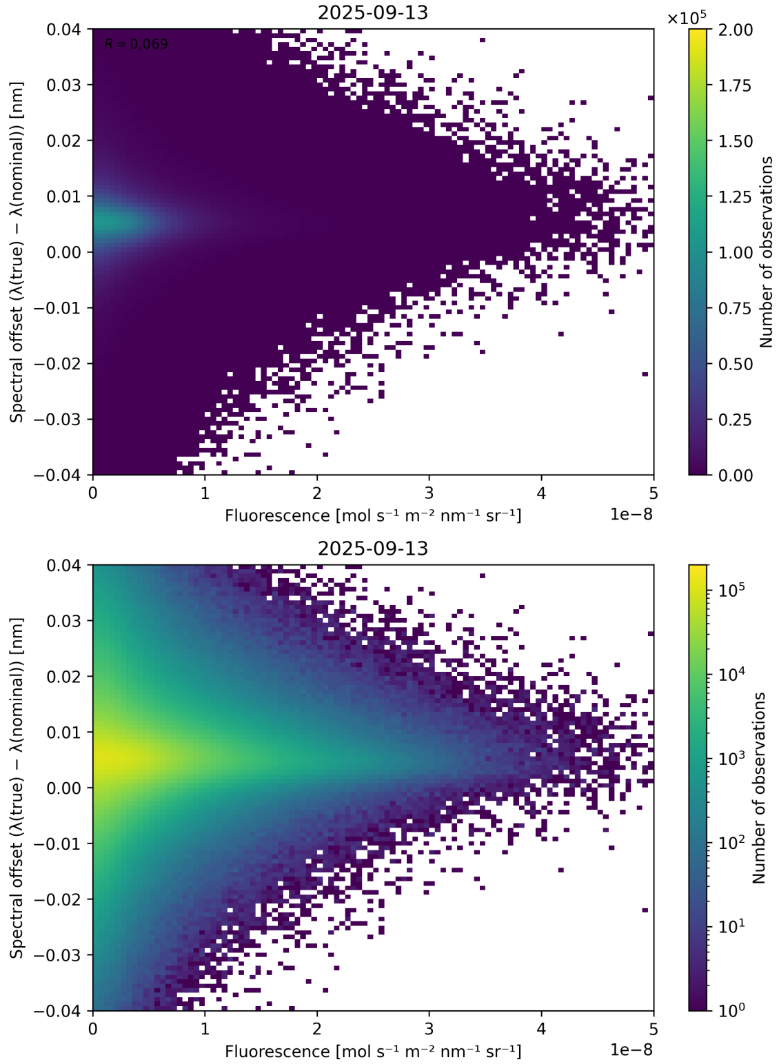
Figure 87: Scatter density plot of “Fluorescence” against “Spectral offset ( \lambda_{\text{true}} - \lambda_{\text{nominal}} )” for 2025-09-12 to 2025-09-14.
