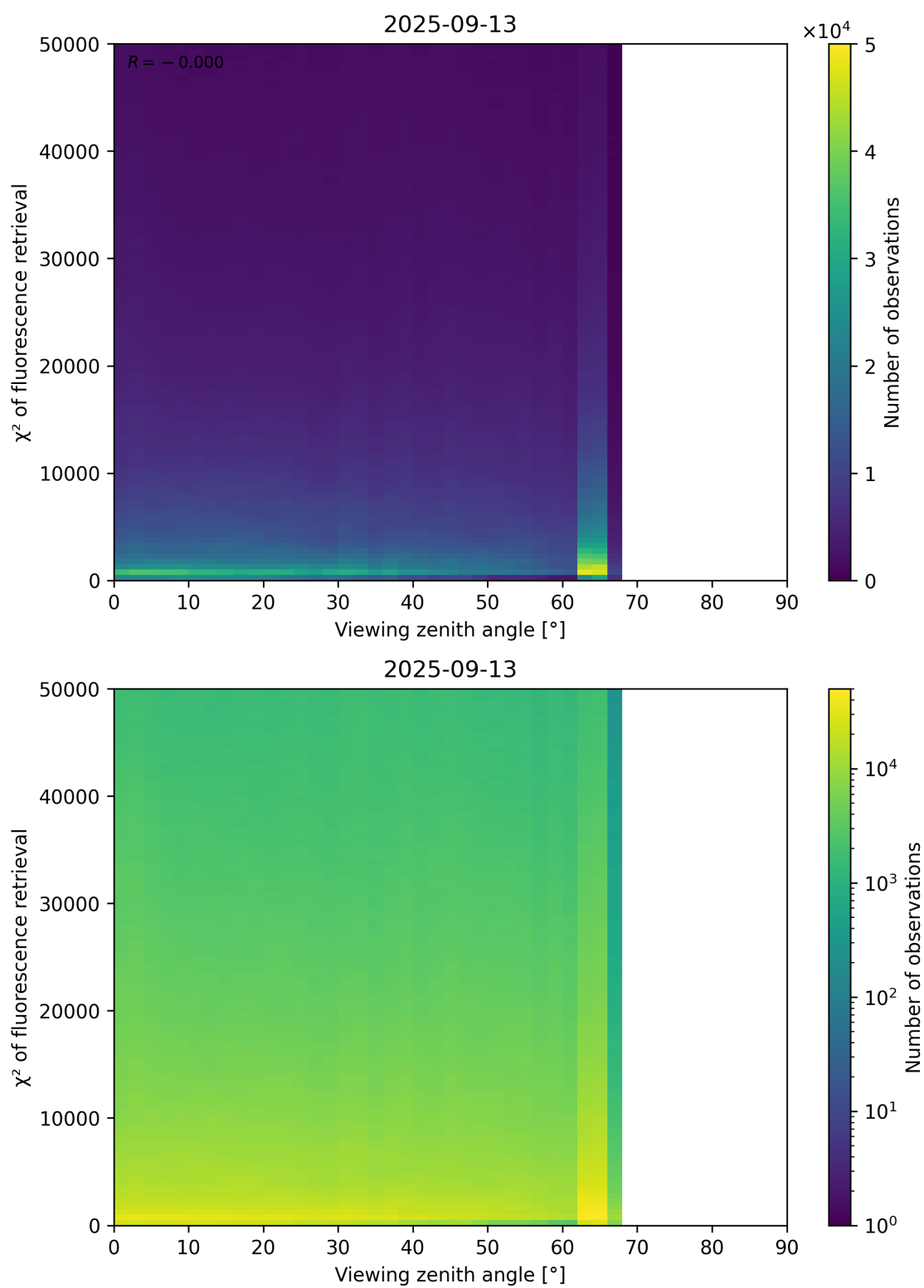
Figure 119: Scatter density plot of “Viewing zenith angle” against “ \chi^2 of fluorescence retrieval” for 2025-09-12 to 2025-09-14.
