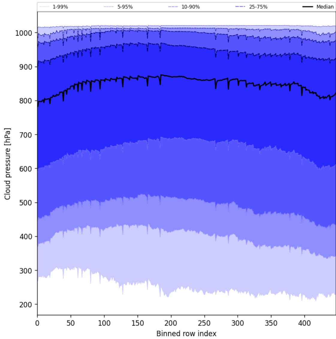
Figure 47: Along track statistics of “Cloud pressure” for 2025-09-12 to 2025-09-14
