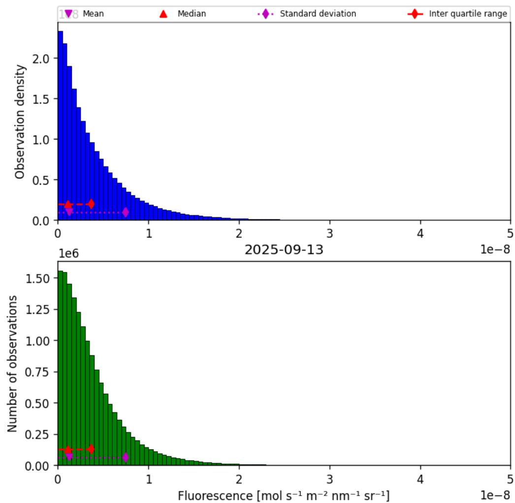
Figure 40: Histogram of “Fluorescence” for 2025-09-12 to 2025-09-14
