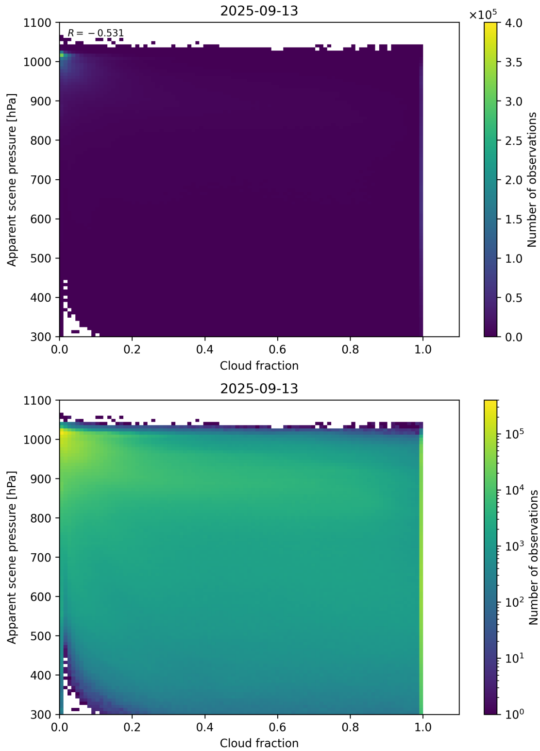
Figure 70: Scatter density plot of “Cloud fraction” against “Apparent scene pressure” for 2025-09-12 to 2025-09-14.
