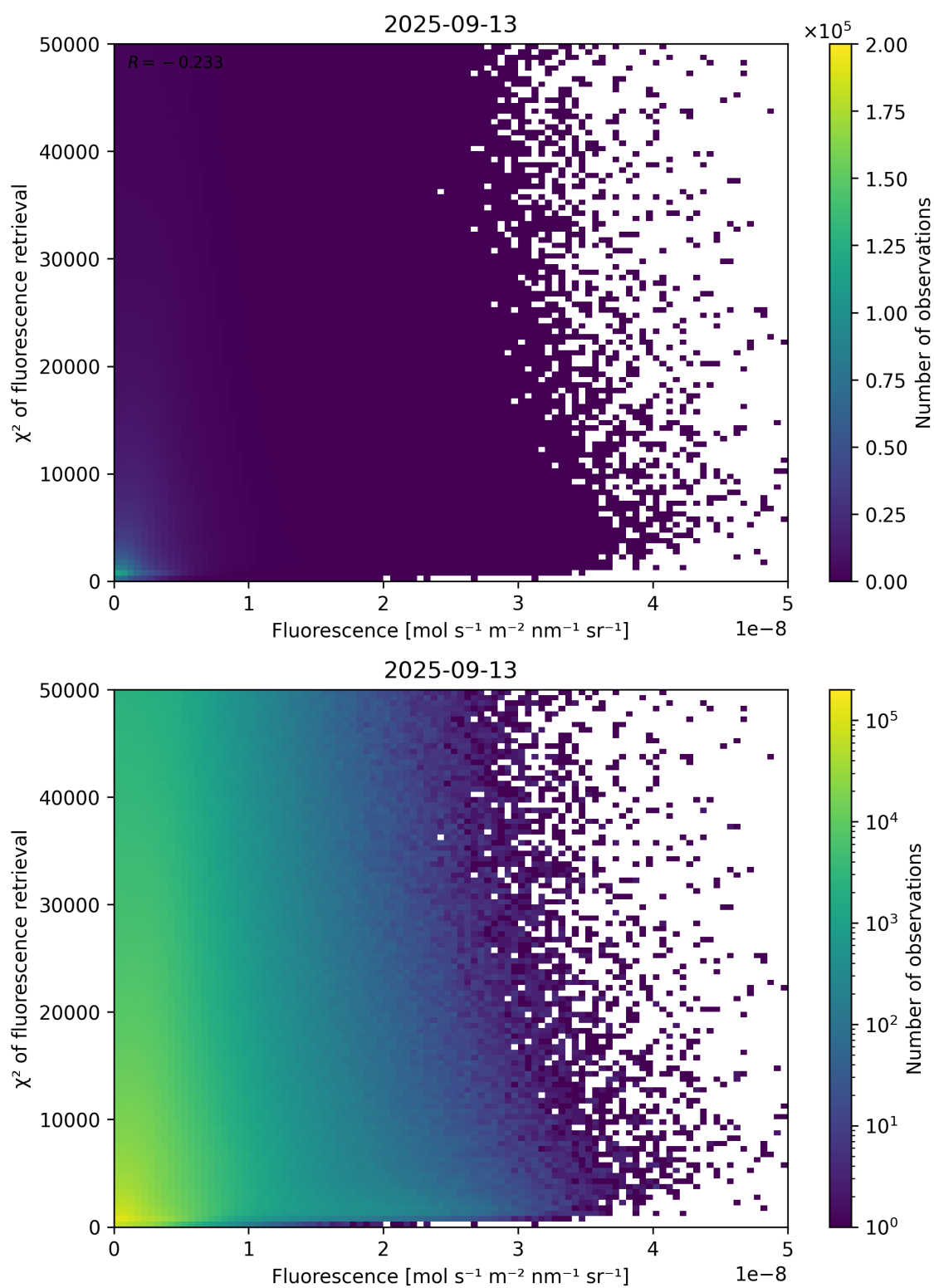
Figure 85: Scatter density plot of “Fluorescence” against “ \chi^2 of fluorescence retrieval” for 2025-09-12 to 2025-09-14.
