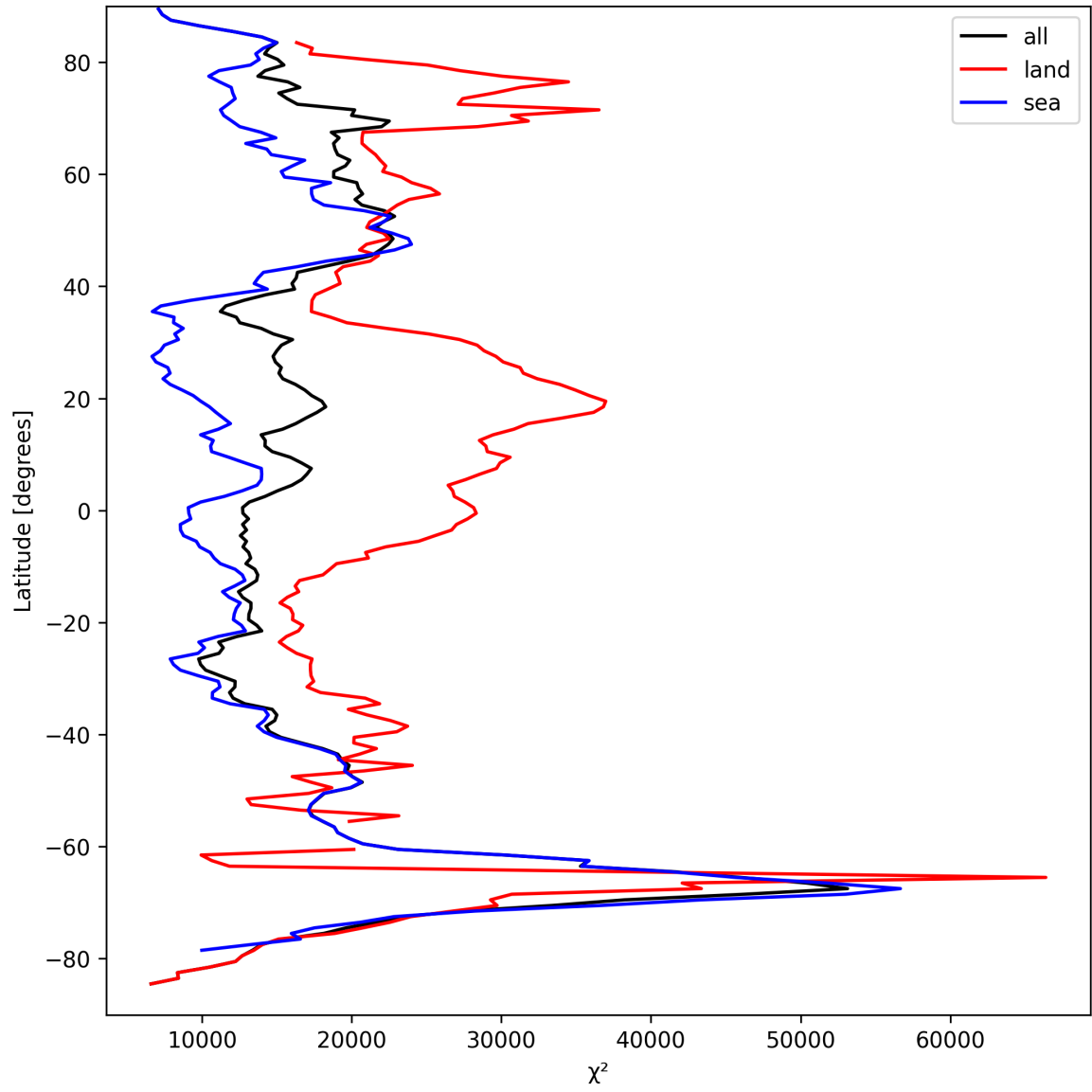
Figure 21: Zonal average of “ \chi^2 ” for 2025-09-12 to 2025-09-14.
