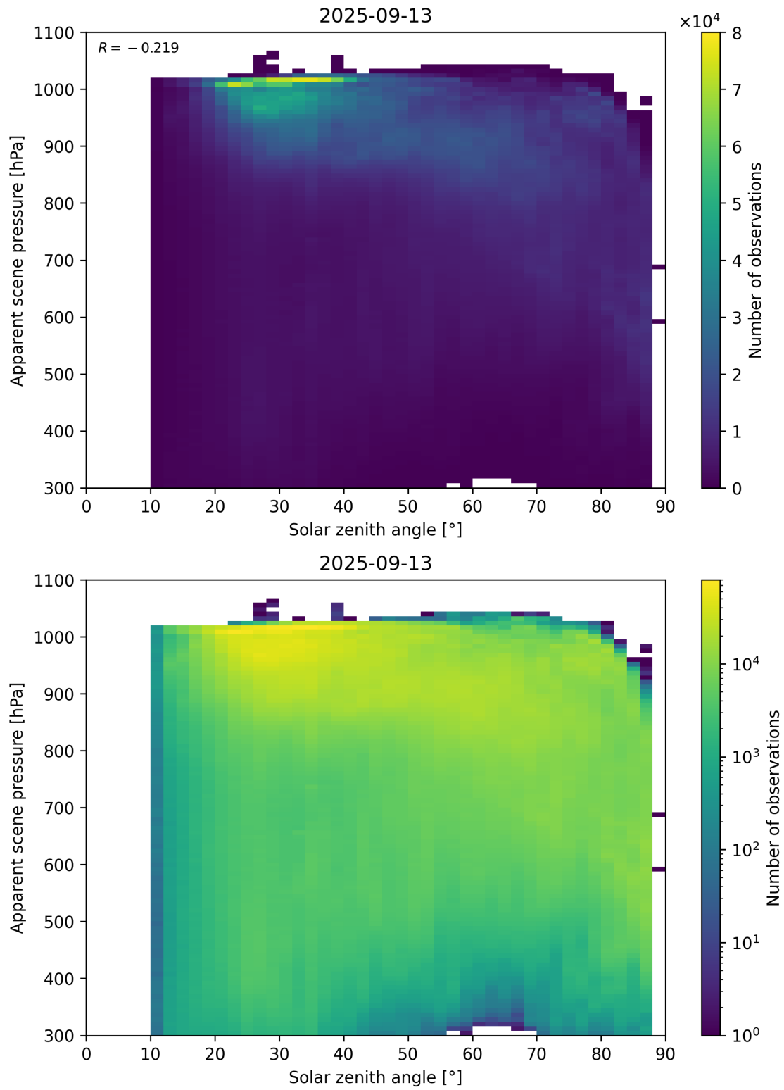
Figure 108: Scatter density plot of “Solar zenith angle” against “Apparent scene pressure” for 2025-09-12 to 2025-09-14.
