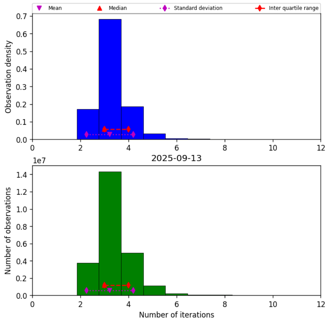
Figure 39: Histogram of “Number of iterations” for 2025-09-12 to 2025-09-14
