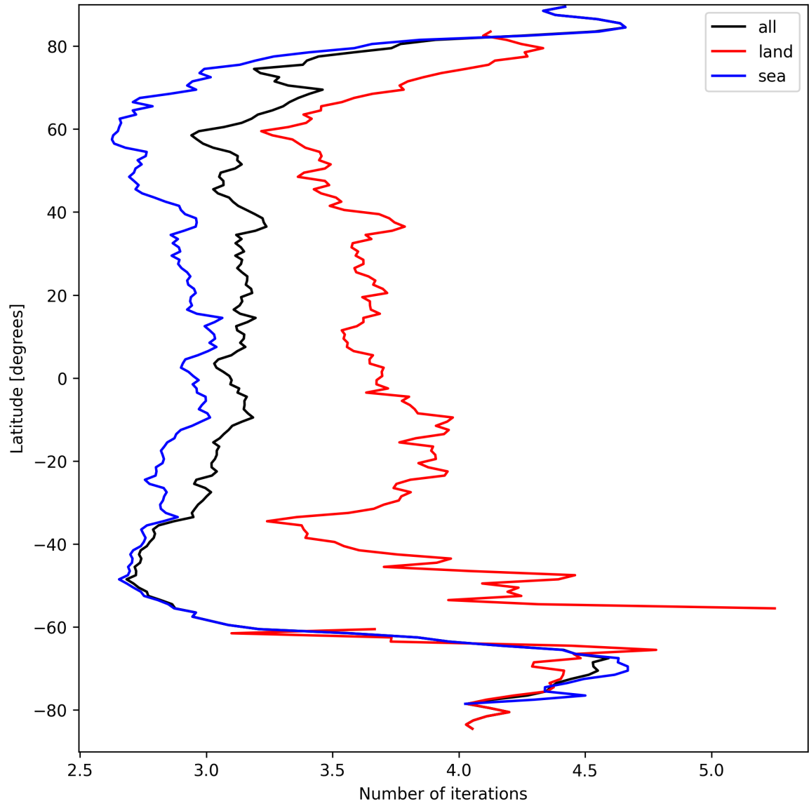
Figure 22: Zonal average of “Number of iterations” for 2025-09-12 to 2025-09-14.
