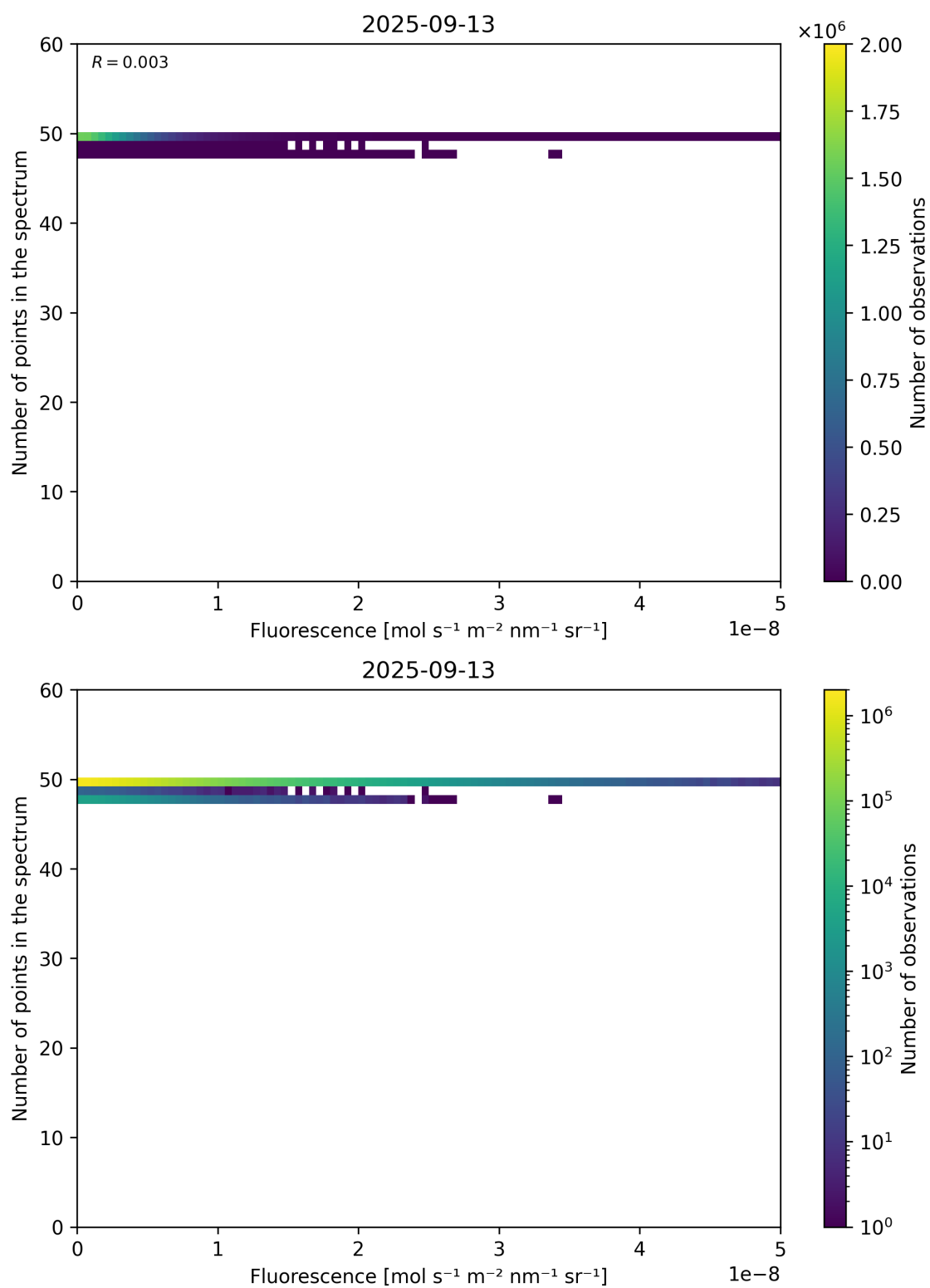
Figure 86: Scatter density plot of “Fluorescence” against “Number of points in the spectrum” for 2025-09-12 to 2025-09-14.
