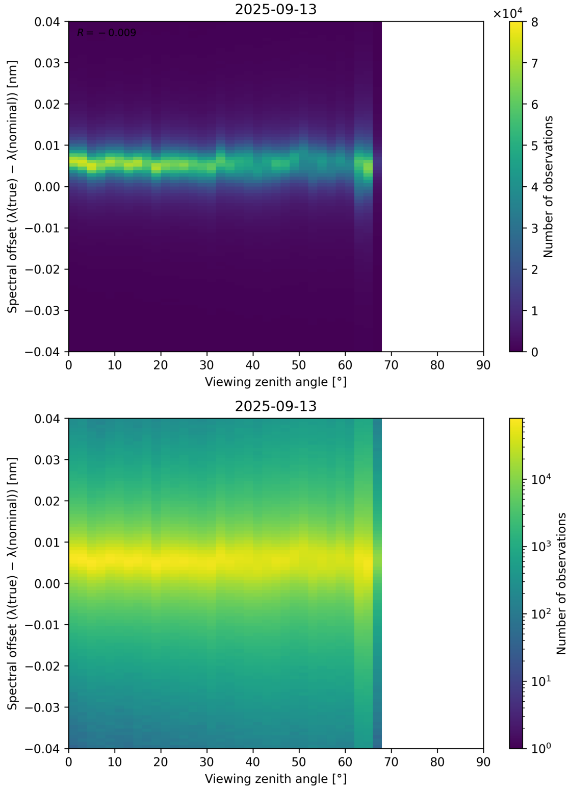
Figure 128: Scatter density plot of “Viewing zenith angle” against “Spectral offset ( \lambda_{\text{true}} - \lambda_{\text{nominal}} )” for 2025-09-12 to 2025-09-14.
