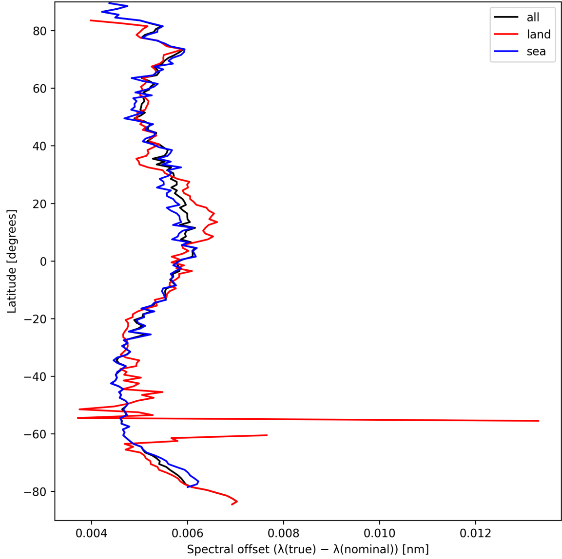
Figure 28: Zonal average of “Spectral offset ( \lambda_{\text{true}} - \lambda_{\text{nominal}} )” for 2025-09-12 to 2025-09-14.
