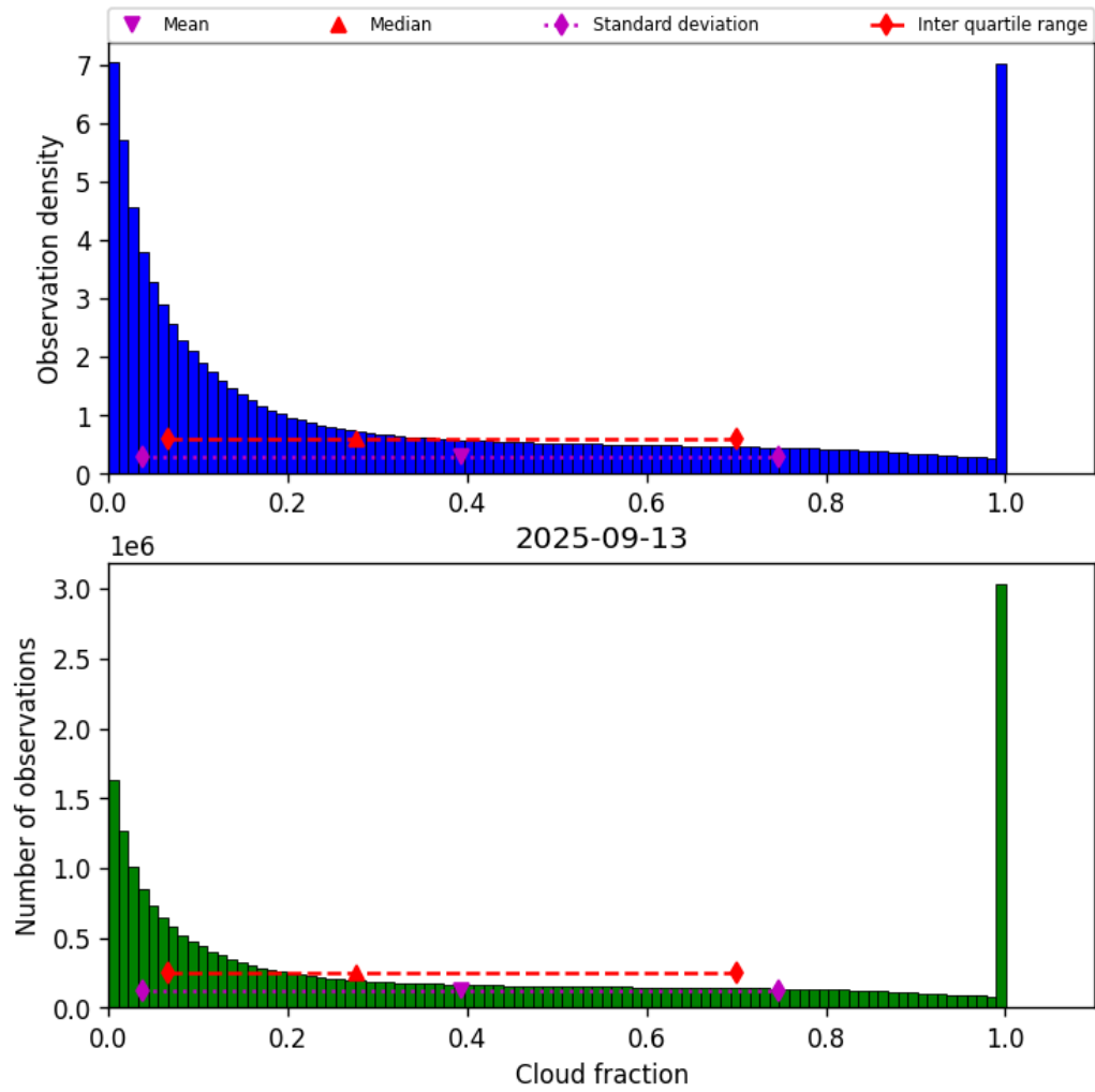
Figure 32: Histogram of “Cloud fraction” for 2025-09-12 to 2025-09-14
