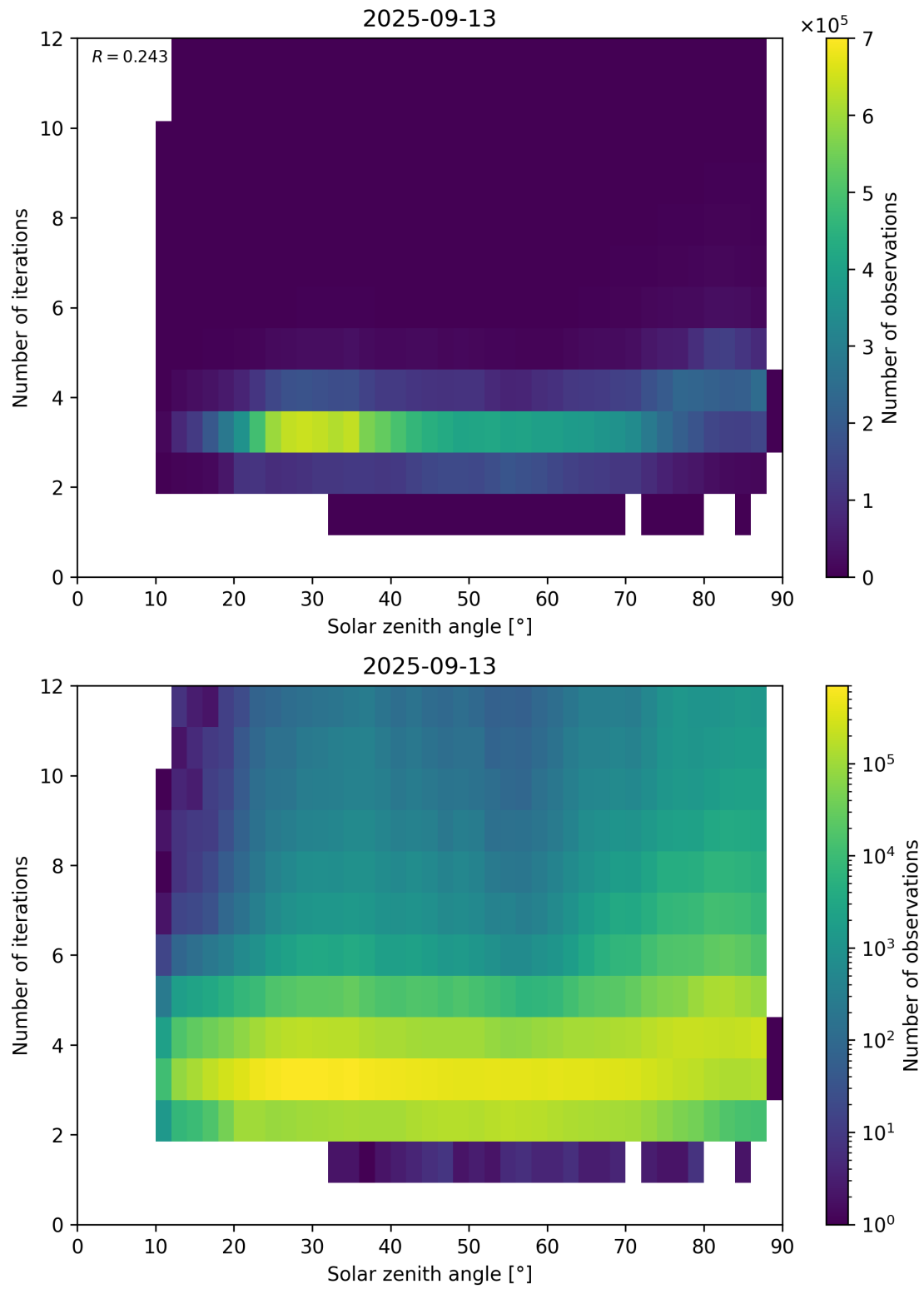
Figure 114: Scatter density plot of “Solar zenith angle” against “Number of iterations” for 2025-09-12 to 2025-09-14.
