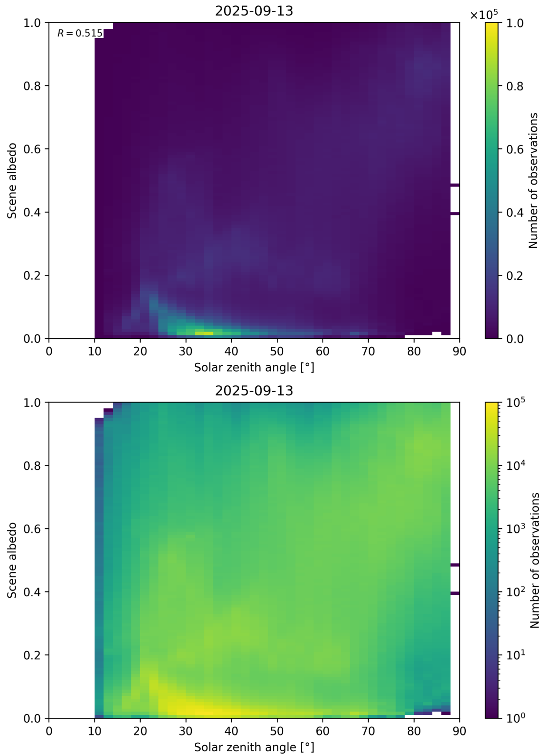
Figure 116: Scatter density plot of “Solar zenith angle” against “Scene albedo” for 2025-09-12 to 2025-09-14.
