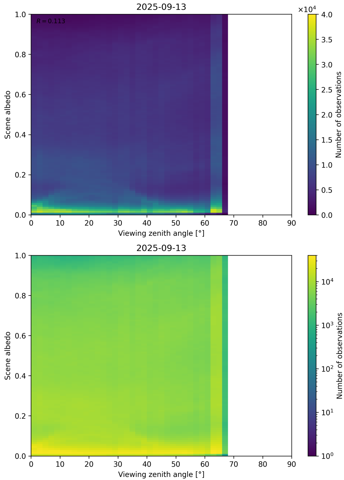
Figure 126: Scatter density plot of “Viewing zenith angle” against “Scene albedo” for 2025-09-12 to 2025-09-14.
