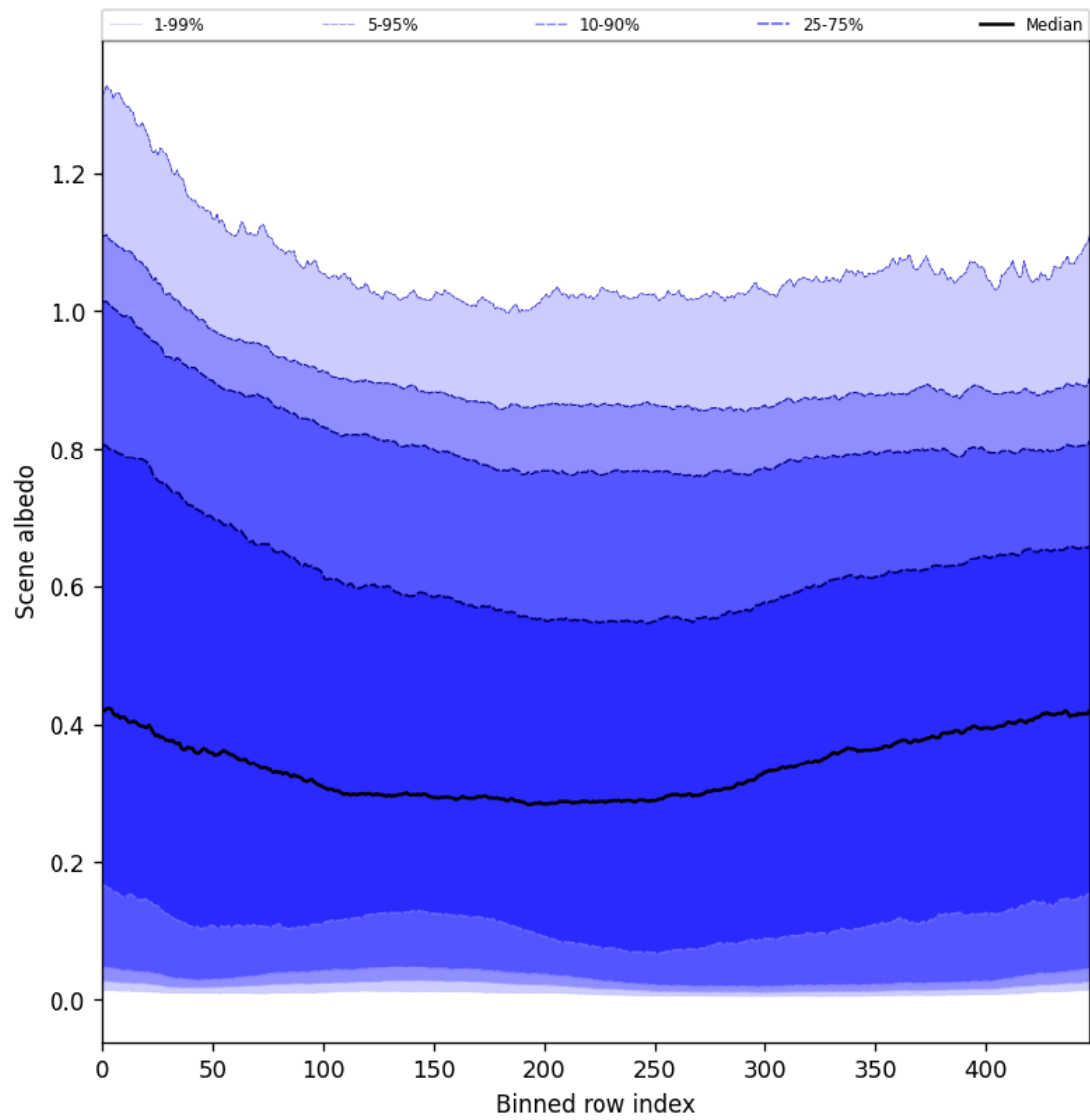
Figure 51: Along track statistics of “Scene albedo” for 2025-09-12 to 2025-09-14
