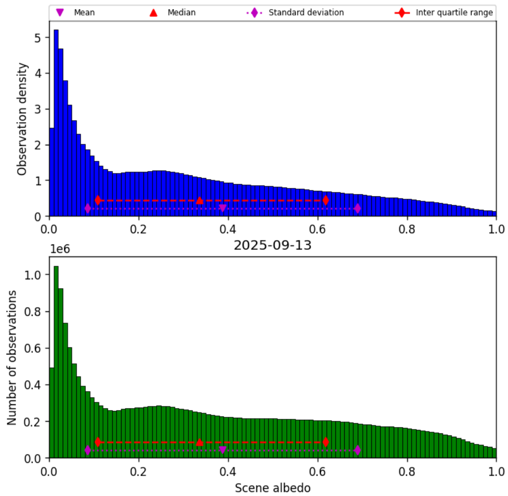
Figure 34: Histogram of “Scene albedo” for 2025-09-12 to 2025-09-14
