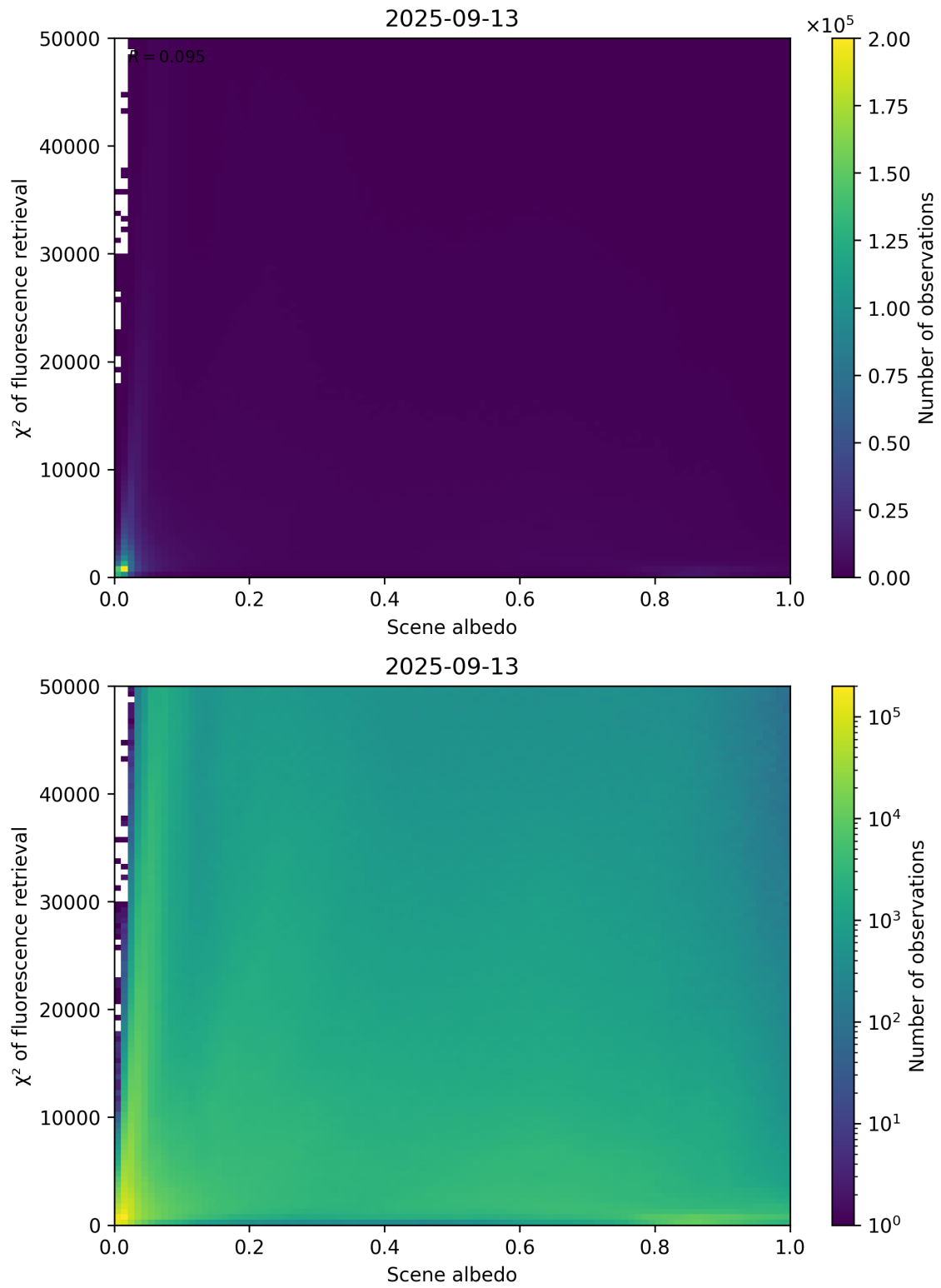
Figure 103: Scatter density plot of “Scene albedo” against “ \chi^2 of fluorescence retrieval” for 2025-09-12 to 2025-09-14.
