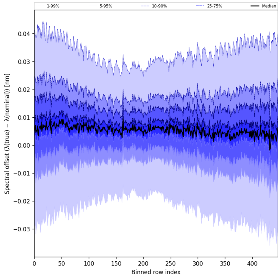
Figure 62: Along track statistics of “Spectral offset ( \lambda_{\text{true}} - \lambda_{\text{nominal}} )” for 2025-09-12 to 2025-09-14
