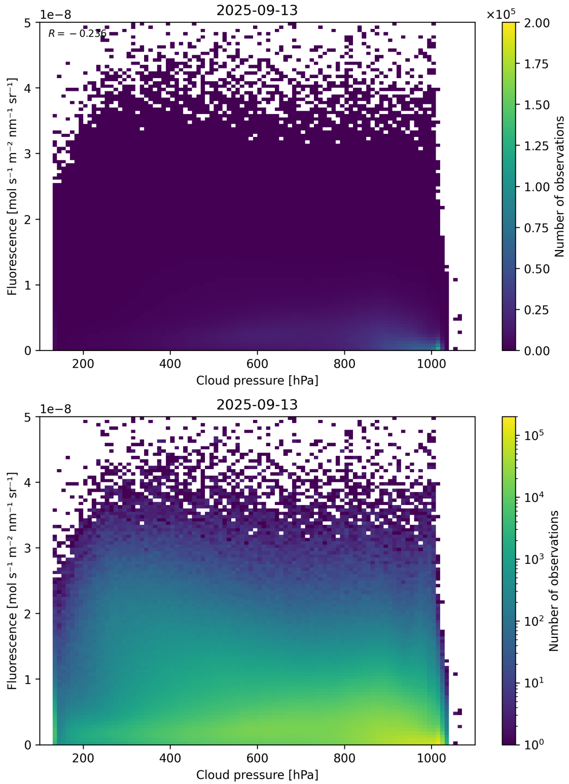
Figure 80: Scatter density plot of “Cloud pressure” against “Fluorescence” for 2025-09-12 to 2025-09-14.
