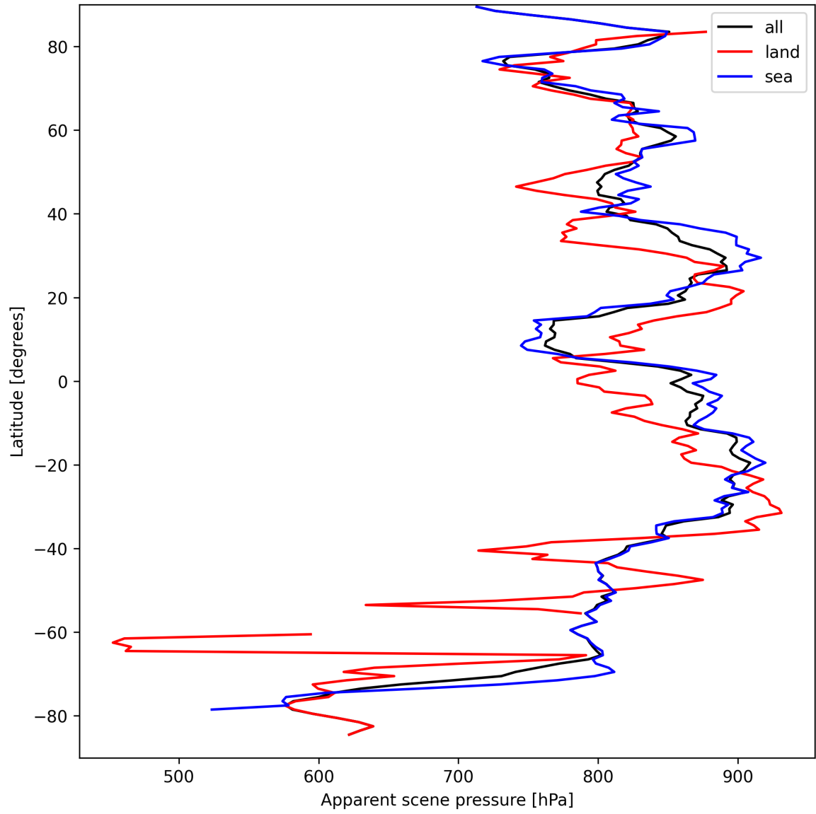
Figure 19: Zonal average of “Apparent scene pressure” for 2025-09-12 to 2025-09-14.
