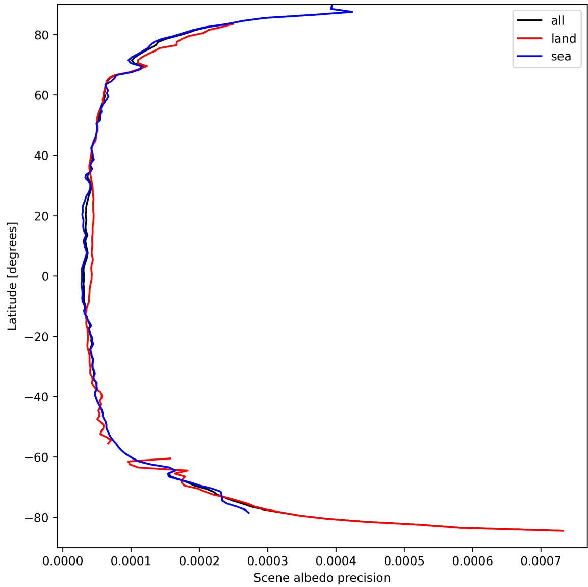
Figure 18: Zonal average of “Scene albedo precision” for 2025-09-12 to 2025-09-14.
