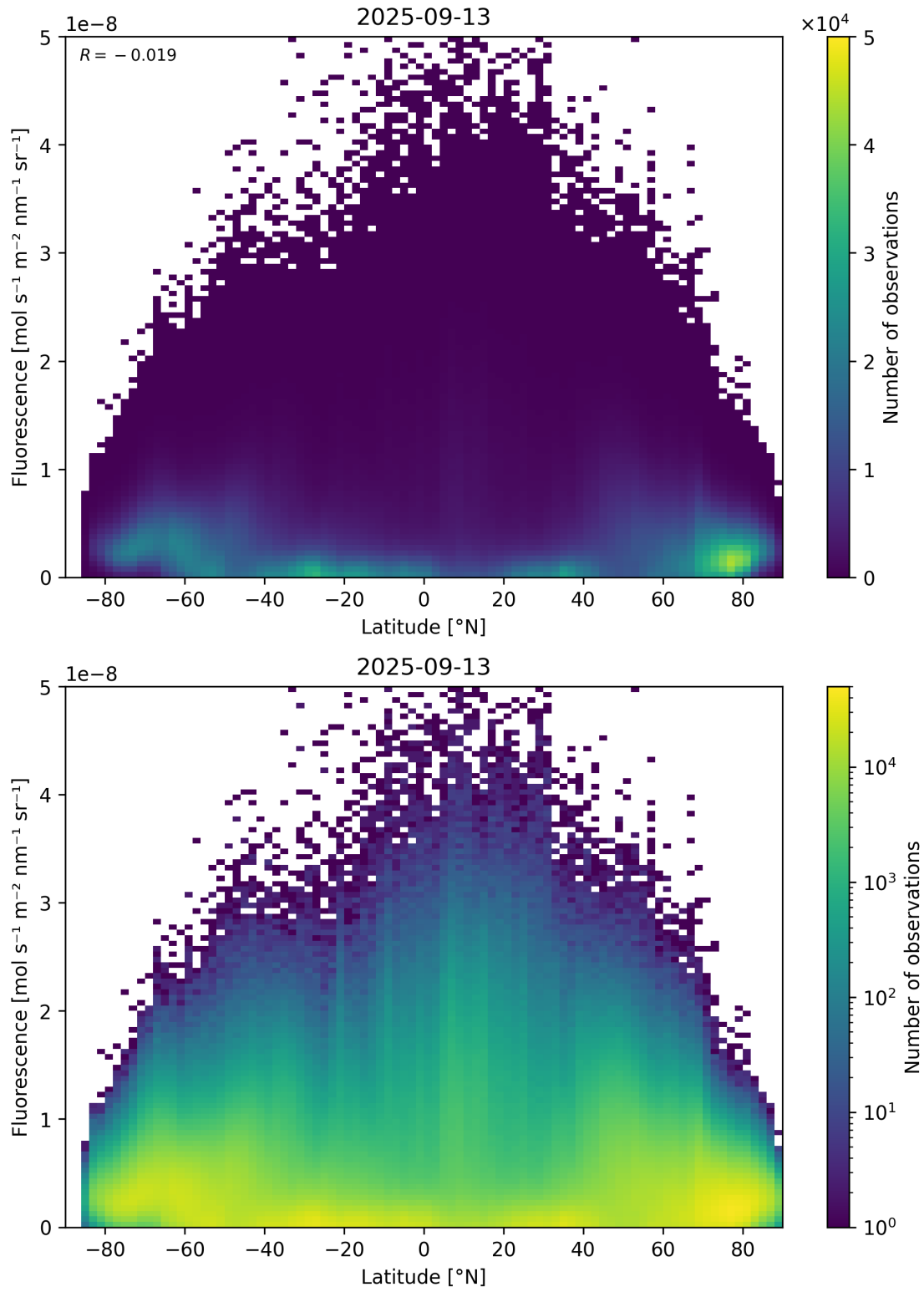
Figure 92: Scatter density plot of “Latitude” against “Fluorescence” for 2025-09-12 to 2025-09-14.
