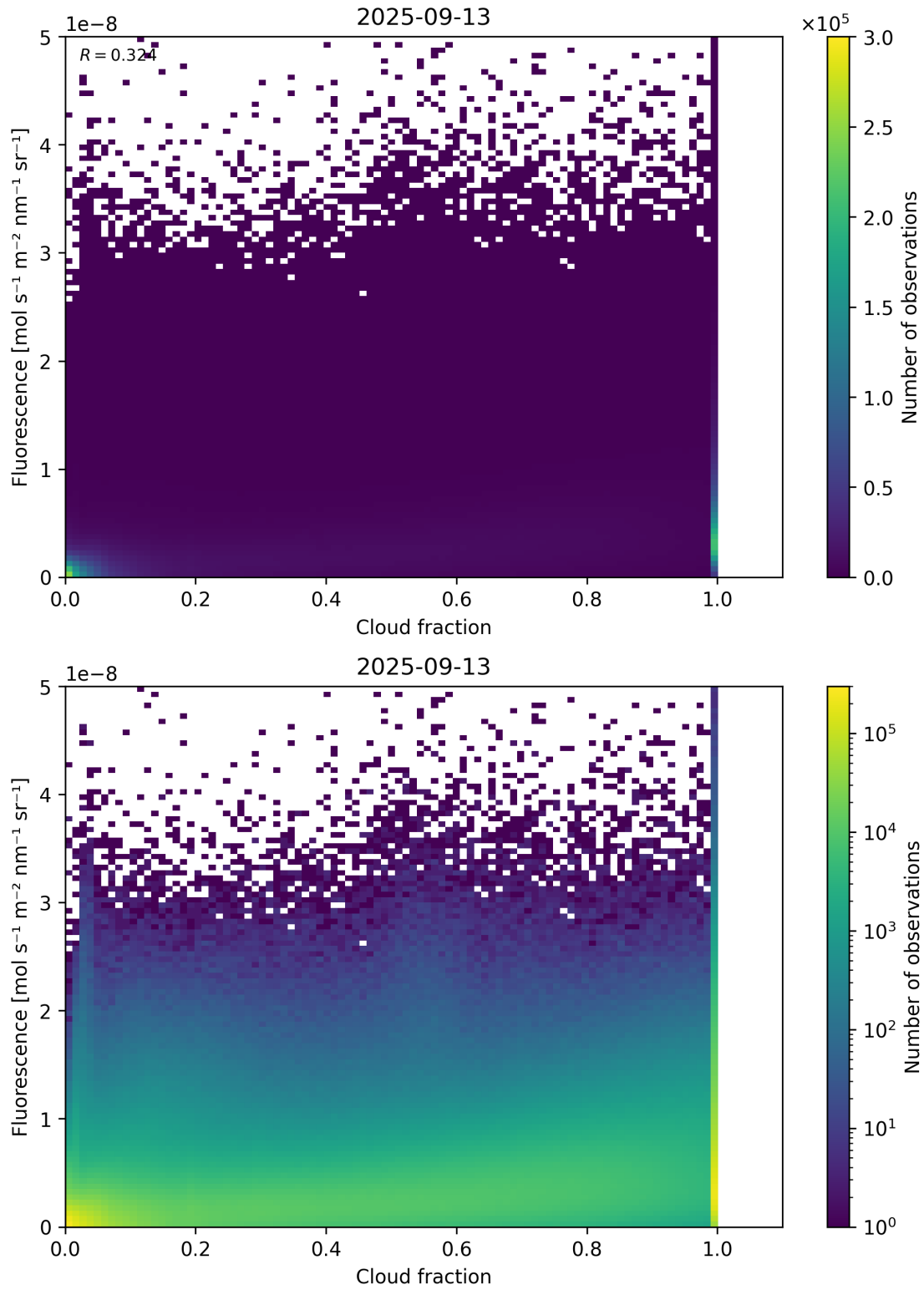
Figure 72: Scatter density plot of “Cloud fraction” against “Fluorescence” for 2025-09-12 to 2025-09-14.
