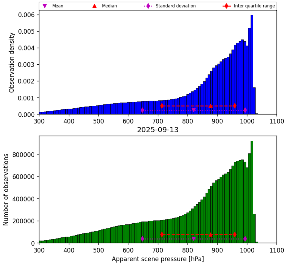
Figure 36: Histogram of “Apparent scene pressure” for 2025-09-12 to 2025-09-14
