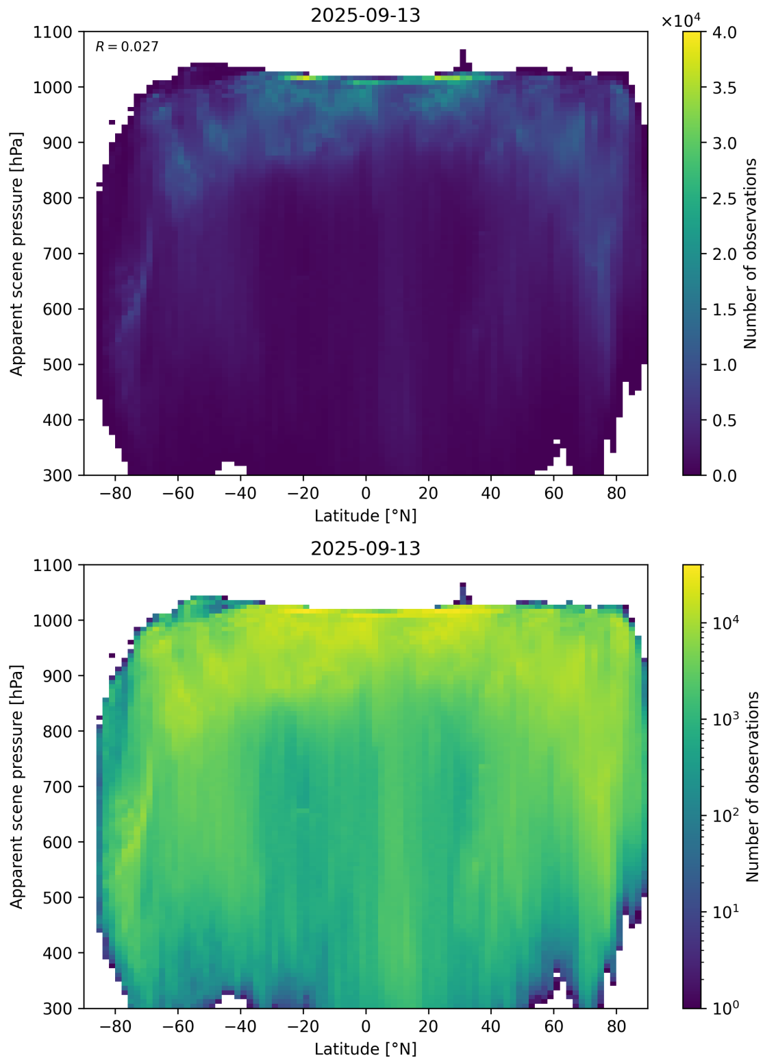
Figure 88: Scatter density plot of “Latitude” against “Apparent scene pressure” for 2025-09-12 to 2025-09-14.
