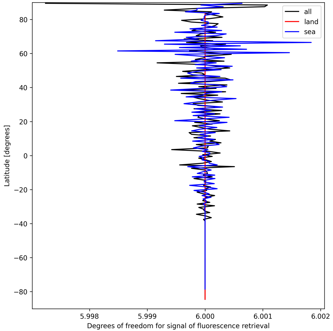
Figure 26: Zonal average of “Degrees of freedom for signal of fluorescence retrieval” for 2025-09-12 to 2025-09-14.
