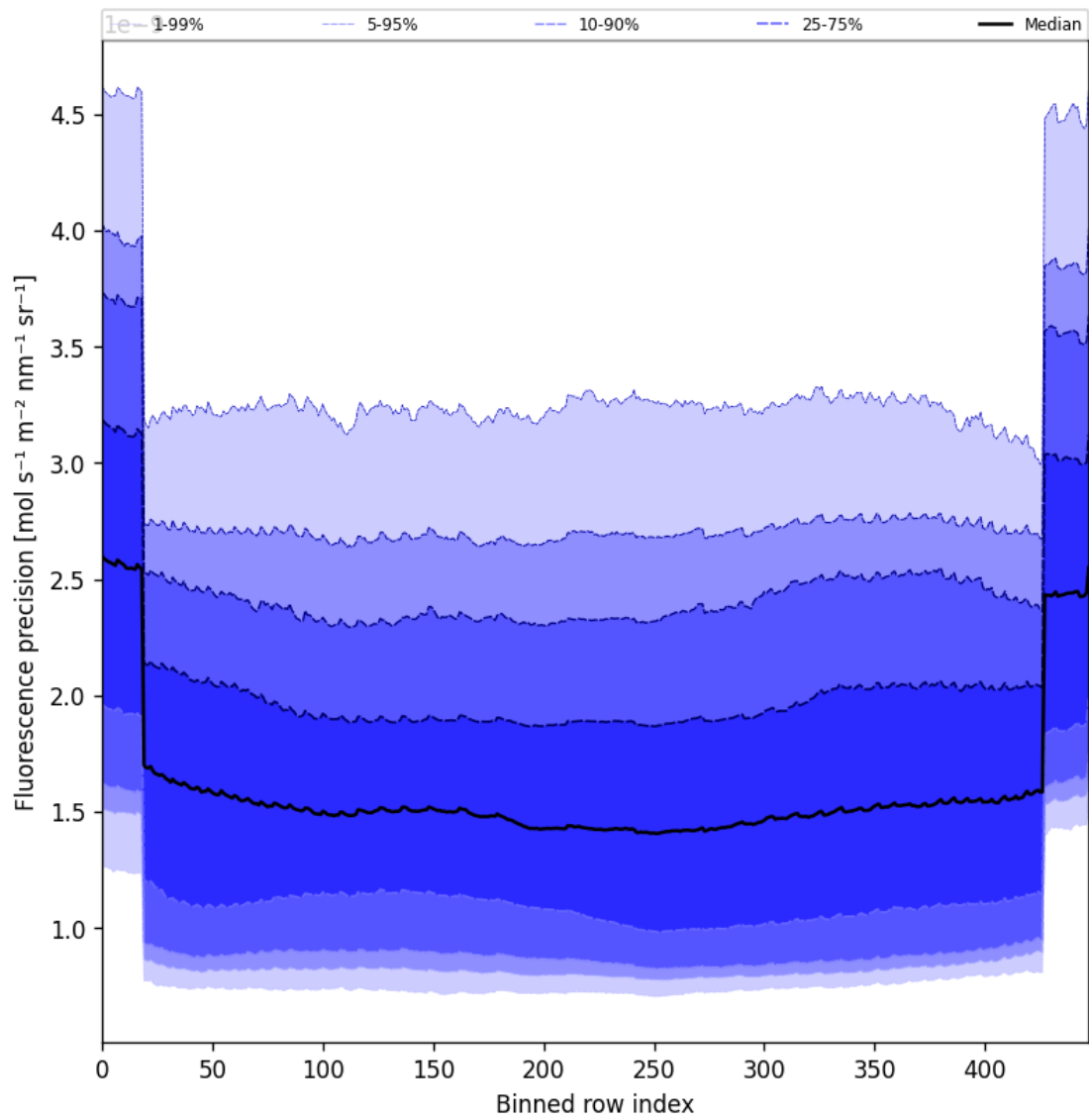
Figure 58: Along track statistics of “Fluorescence precision” for 2025-09-12 to 2025-09-14
