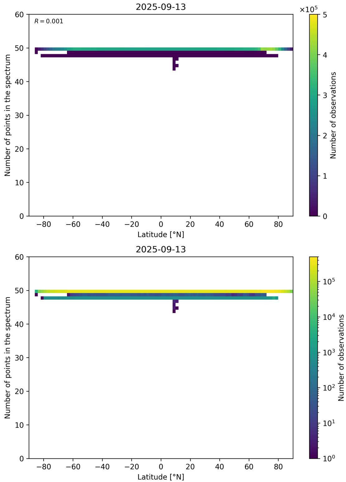
Figure 94: Scatter density plot of “Latitude” against “Number of points in the spectrum” for 2025-09-12 to 2025-09-14.
