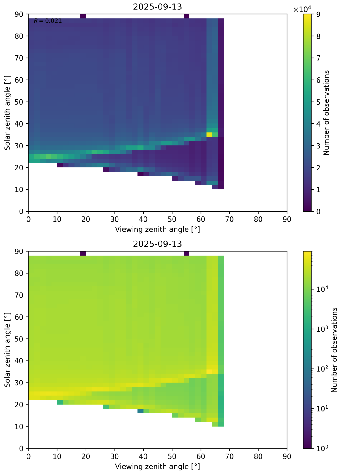
Figure 127: Scatter density plot of “Viewing zenith angle” against “Solar zenith angle” for 2025-09-12 to 2025-09-14.
