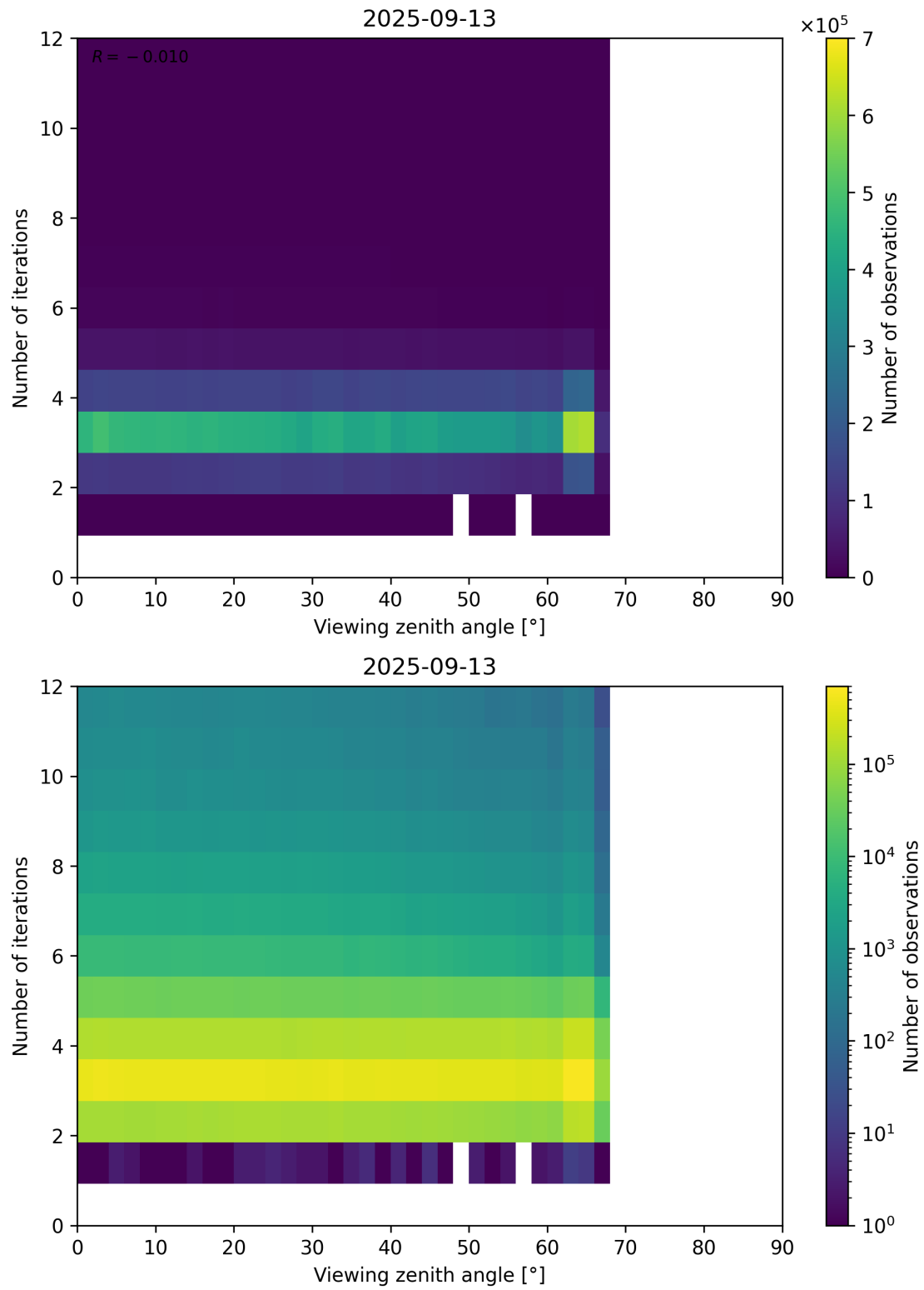
Figure 124: Scatter density plot of “Viewing zenith angle” against “Number of iterations” for 2025-09-12 to 2025-09-14.
