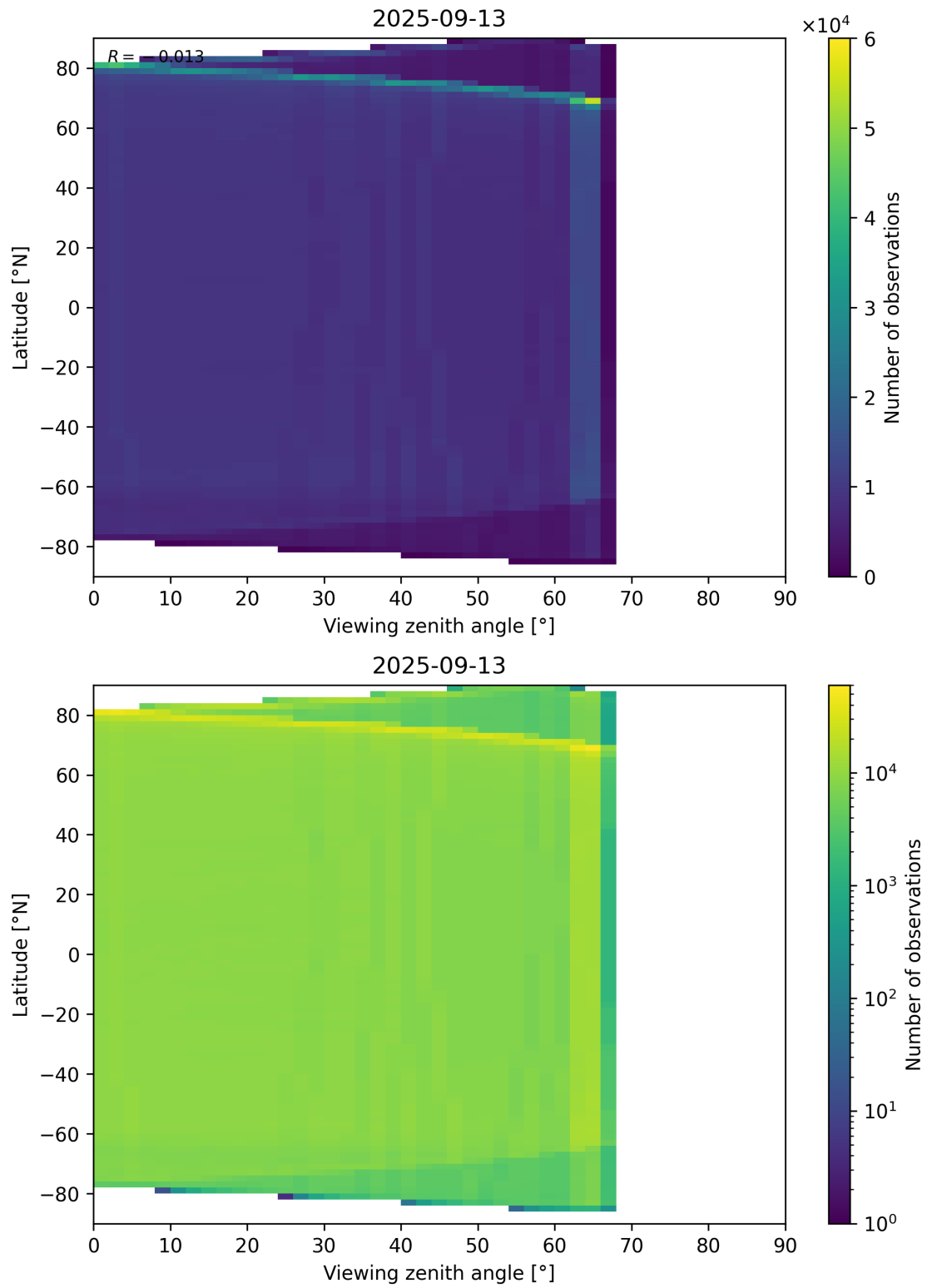
Figure 123: Scatter density plot of “Viewing zenith angle” against “Latitude” for 2025-09-12 to 2025-09-14.
