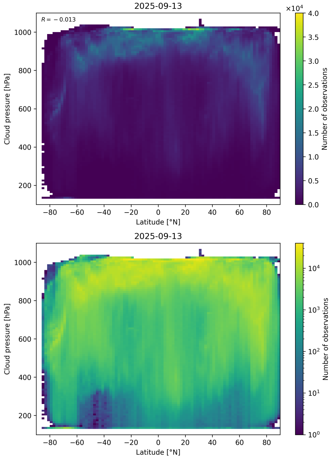
Figure 91: Scatter density plot of “Latitude” against “Cloud pressure” for 2025-09-12 to 2025-09-14.
