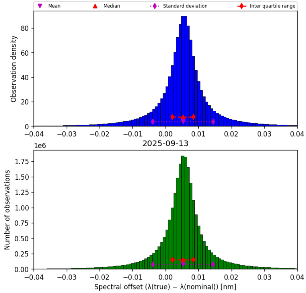
Figure 45: Histogram of “Spectral offset ( \lambda_{\text{true}} - \lambda_{\text{nominal}} )” for 2025-09-12 to 2025-09-14
