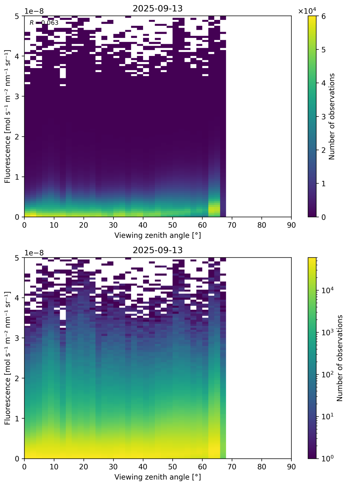
Figure 122: Scatter density plot of “Viewing zenith angle” against “Fluorescence” for 2025-09-12 to 2025-09-14.
