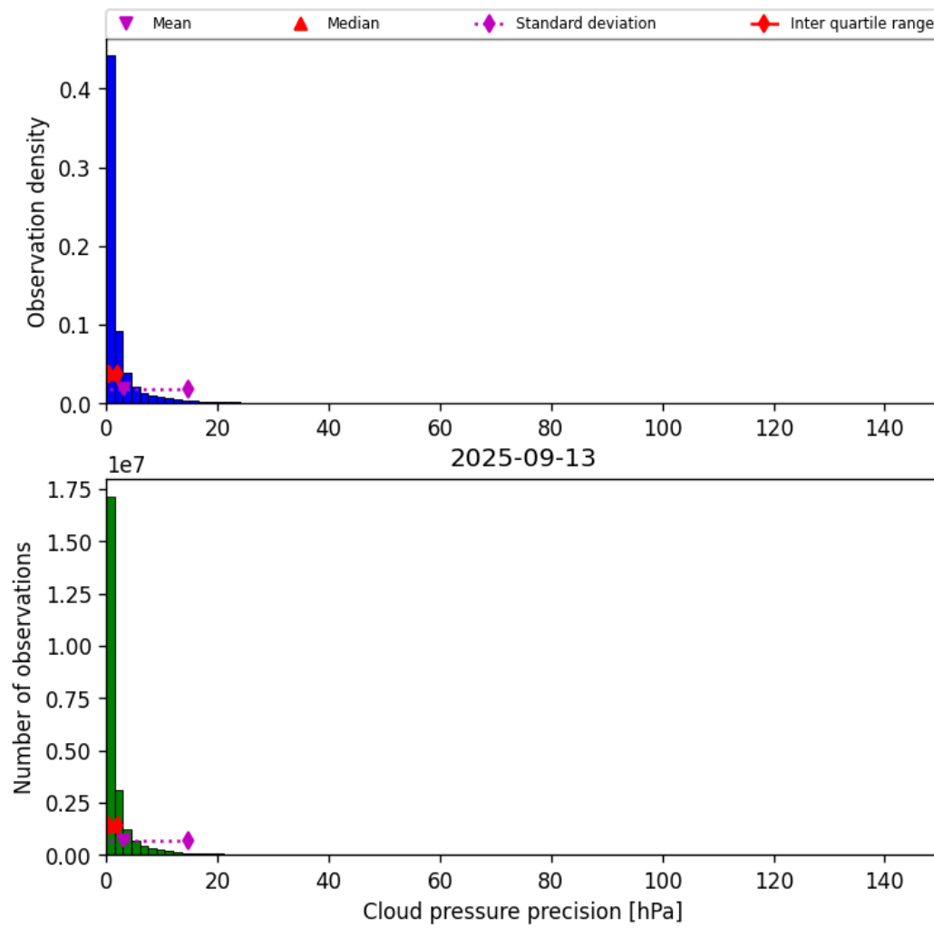
Figure 31: Histogram of “Cloud pressure precision” for 2025-09-12 to 2025-09-14
