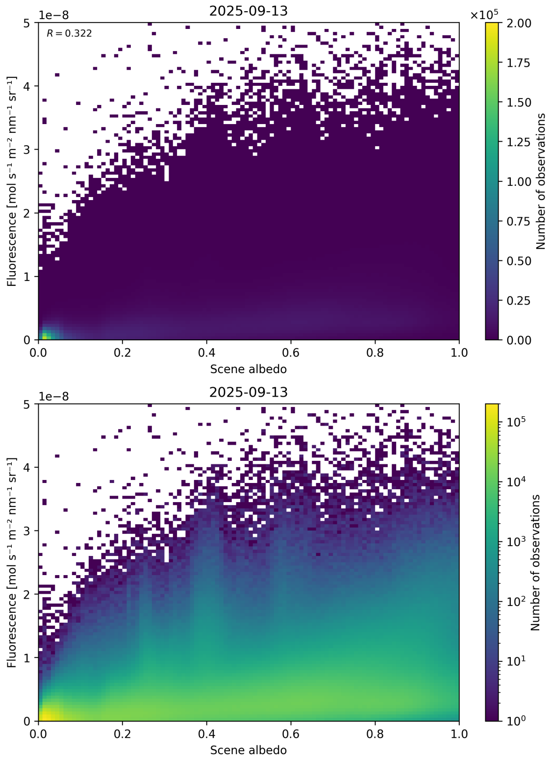
Figure 104: Scatter density plot of “Scene albedo” against “Fluorescence” for 2025-09-12 to 2025-09-14.
