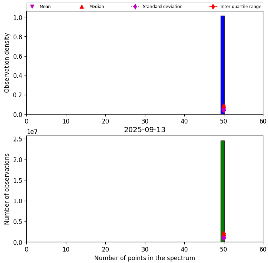
Figure 44: Histogram of “Number of points in the spectrum” for 2025-09-12 to 2025-09-14
