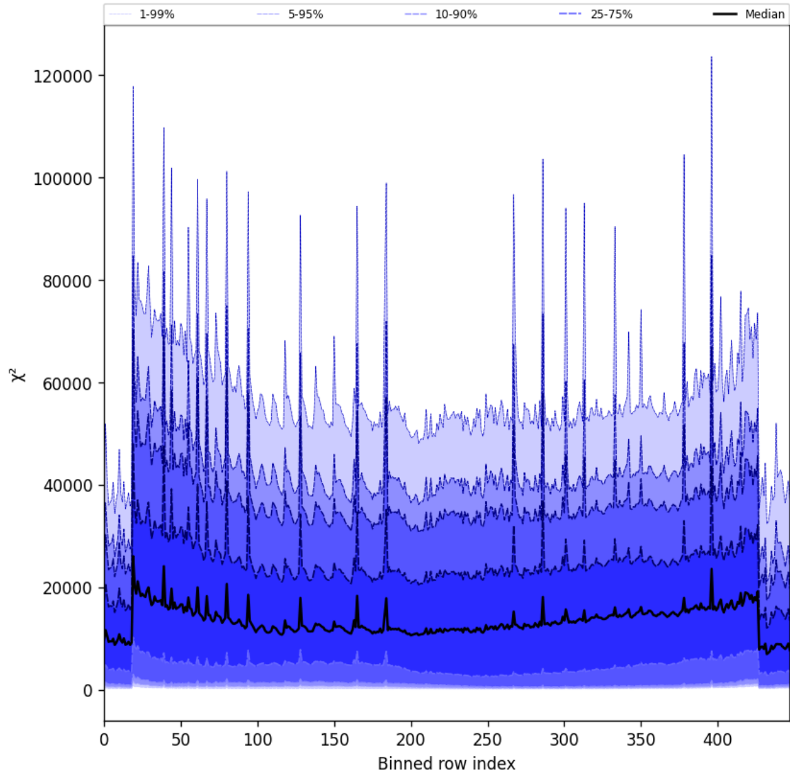
Figure 55: Along track statistics of “ \chi^2 ” for 2025-09-12 to 2025-09-14
