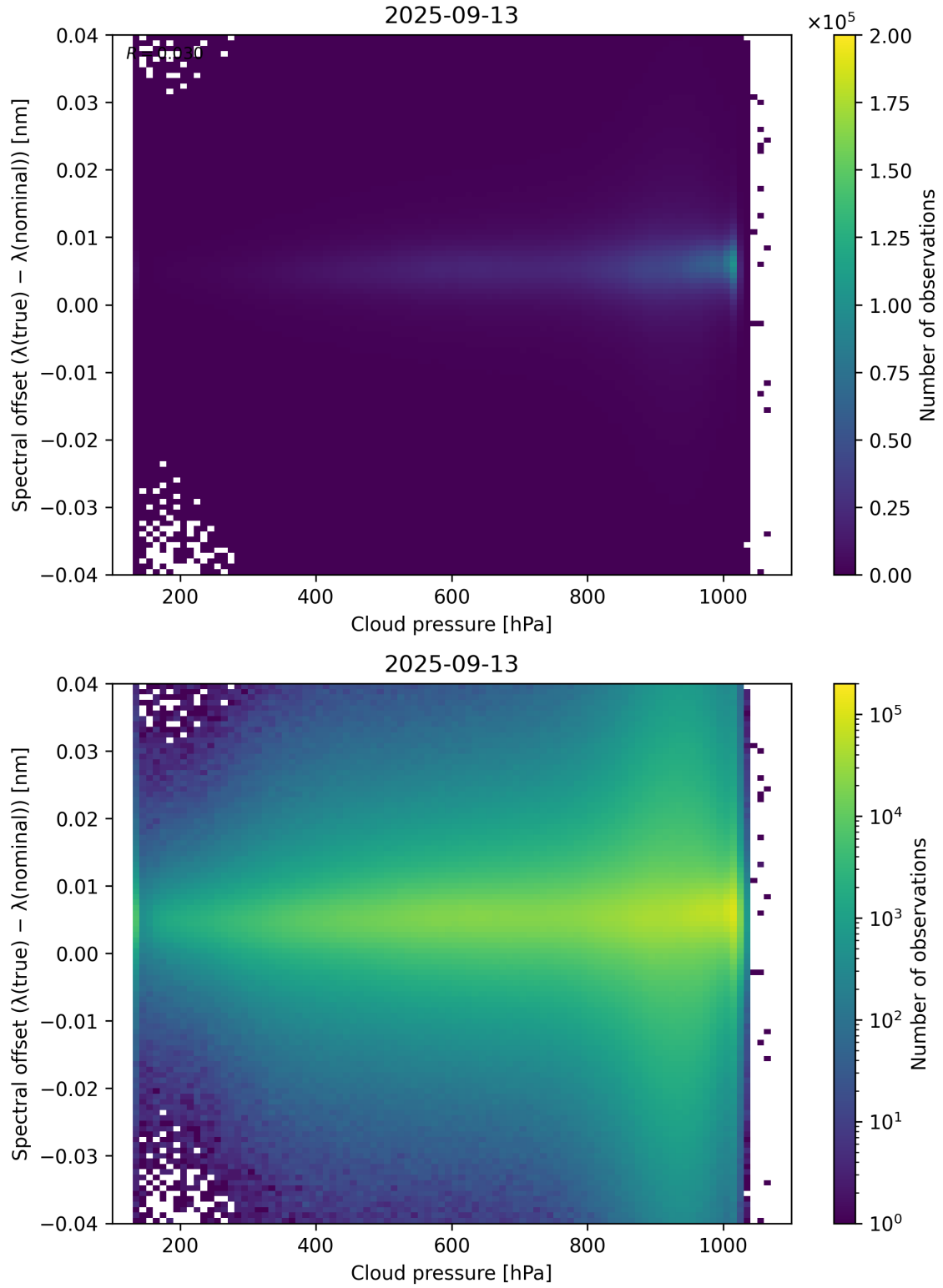
Figure 84: Scatter density plot of “Cloud pressure” against “Spectral offset ( \lambda_{\text{true}} - \lambda_{\text{nominal}} )” for 2025-09-12 to 2025-09-14.
