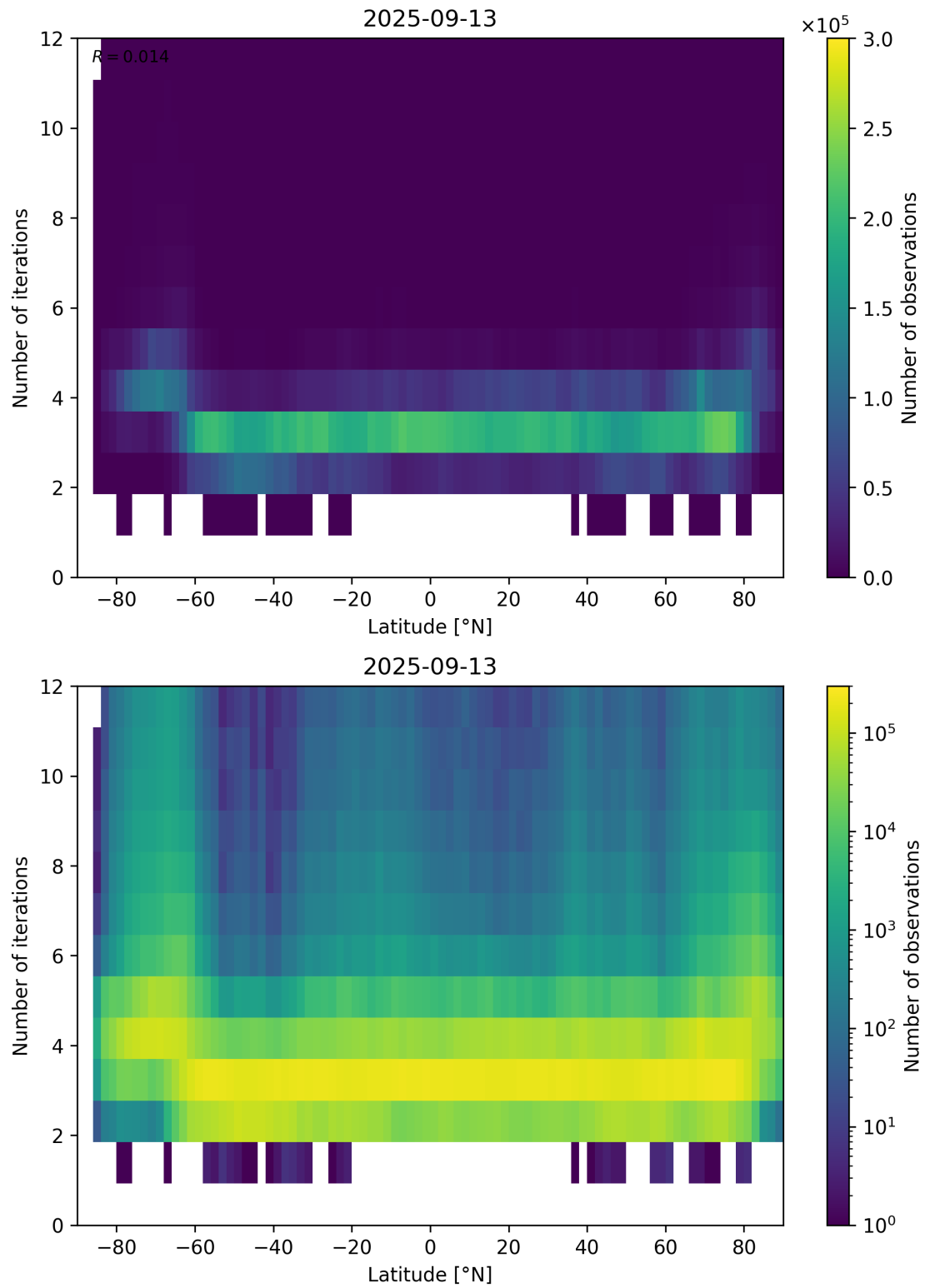
Figure 93: Scatter density plot of “Latitude” against “Number of iterations” for 2025-09-12 to 2025-09-14.
