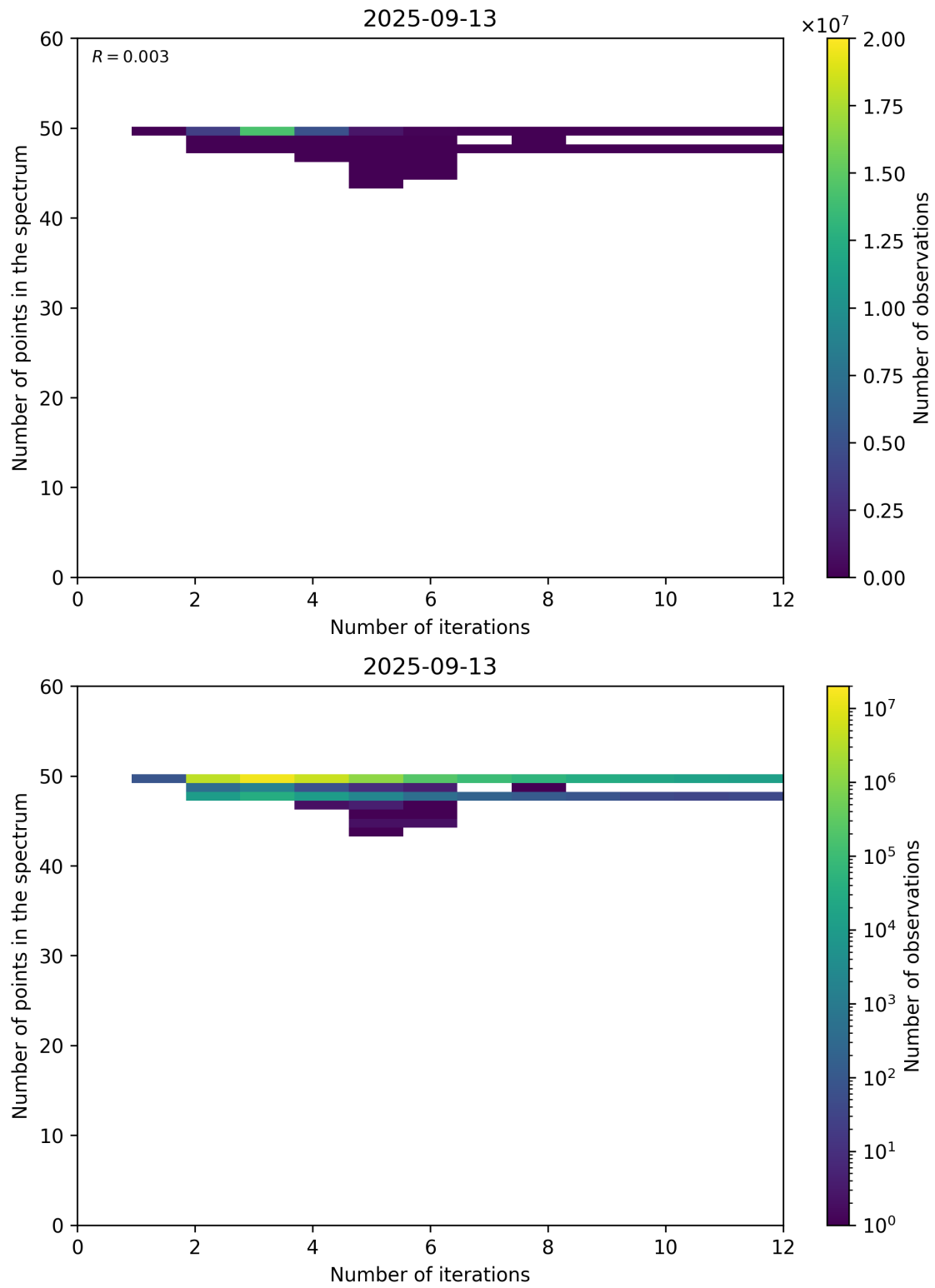
Figure 99: Scatter density plot of “Number of iterations” against “Number of points in the spectrum” for 2025-09-12 to 2025-09-14.
