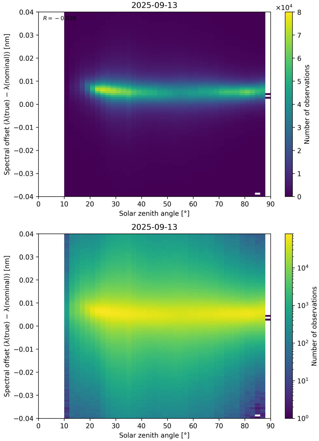
Figure 117: Scatter density plot of “Solar zenith angle” against “Spectral offset ( \lambda_{\text{true}} - \lambda_{\text{nominal}} )” for 2025-09-12 to 2025-09-14.
