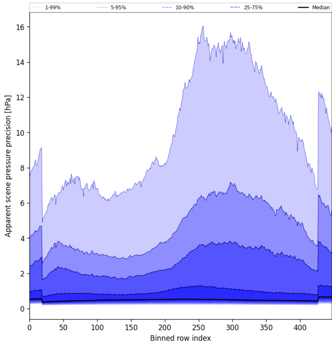
Figure 54: Along track statistics of “Apparent scene pressure precision” for 2025-09-12 to 2025-09-14
