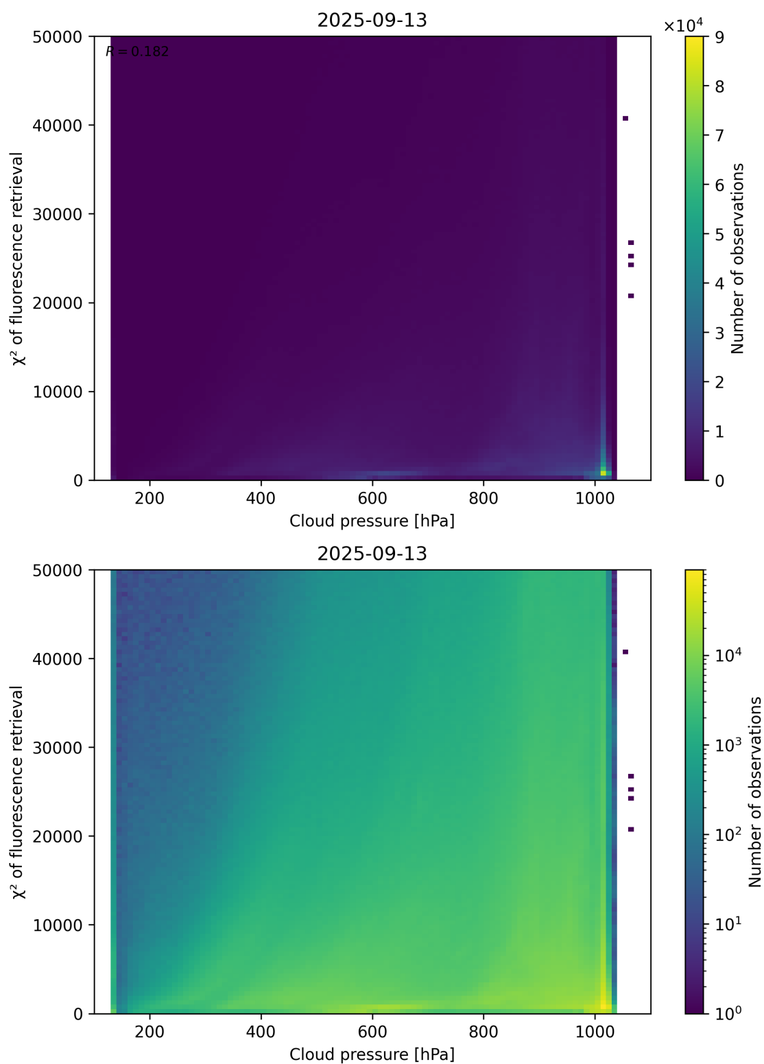
Figure 78: Scatter density plot of “Cloud pressure” against “ \chi^2 of fluorescence retrieval” for 2025-09-12 to 2025-09-14.
