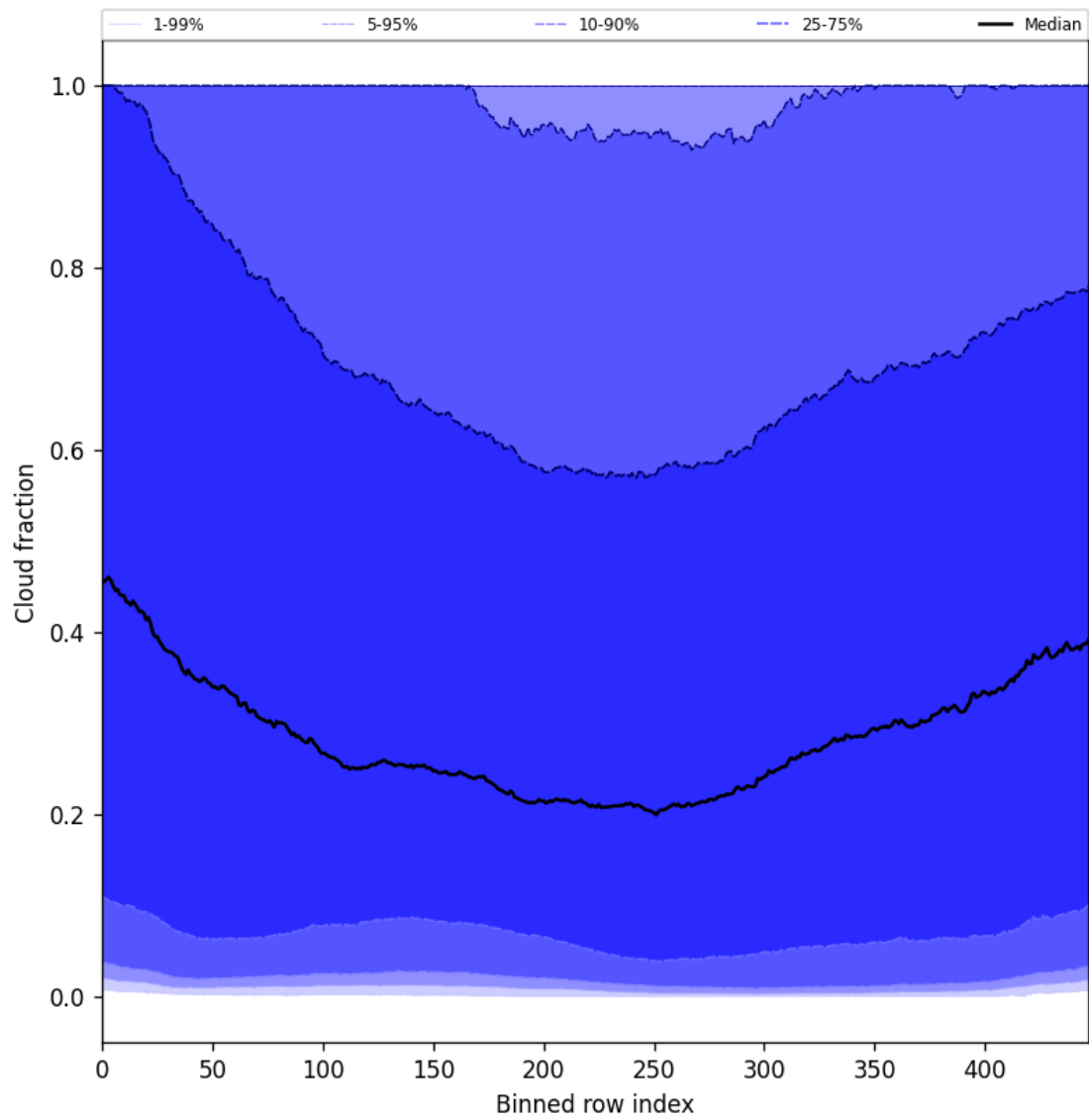
Figure 49: Along track statistics of “Cloud fraction” for 2025-09-12 to 2025-09-14
