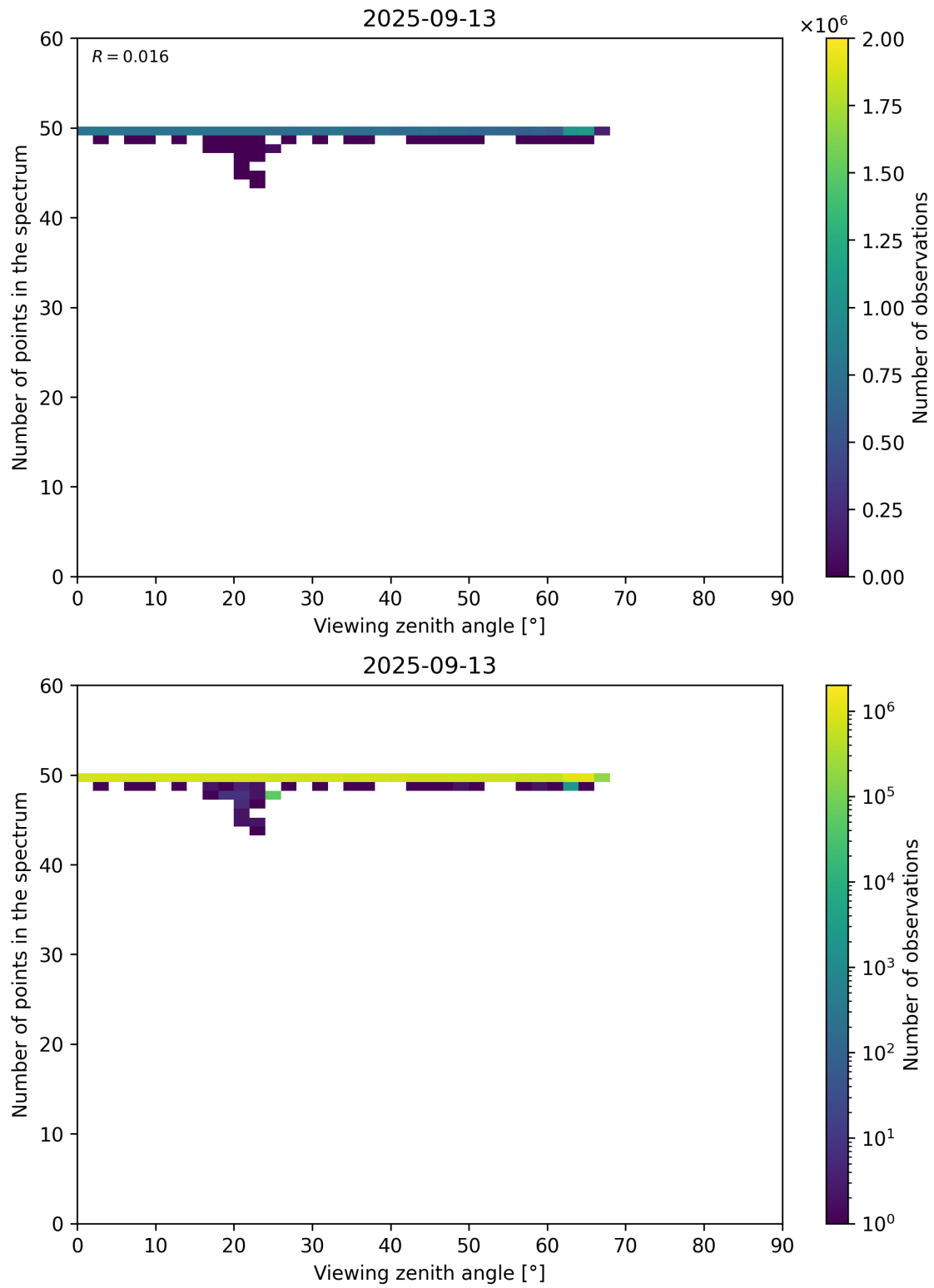
Figure 125: Scatter density plot of “Viewing zenith angle” against “Number of points in the spectrum” for 2025-09-12 to 2025-09-14.
