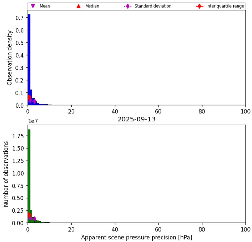
Figure 37: Histogram of “Apparent scene pressure precision” for 2025-09-12 to 2025-09-14
