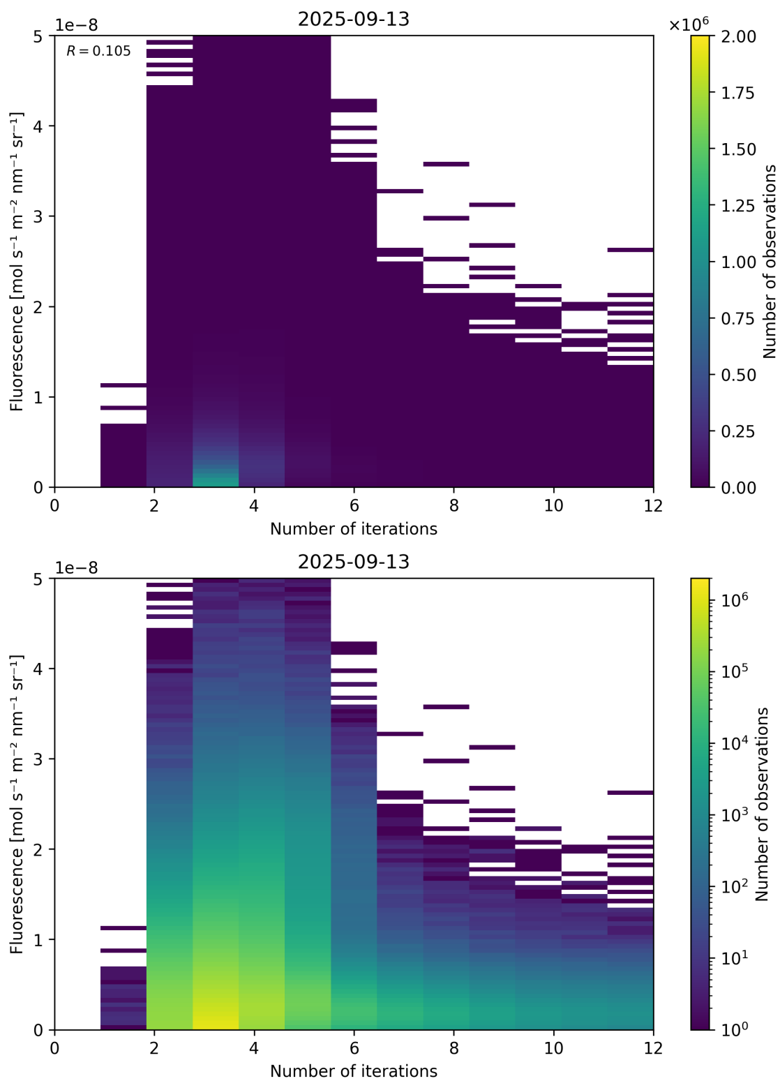
Figure 98: Scatter density plot of “Number of iterations” against “Fluorescence” for 2025-09-12 to 2025-09-14.
