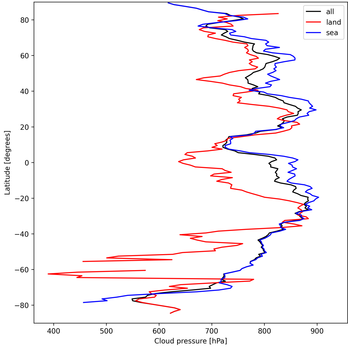
Figure 13: Zonal average of “Cloud pressure” for 2025-09-12 to 2025-09-14.
