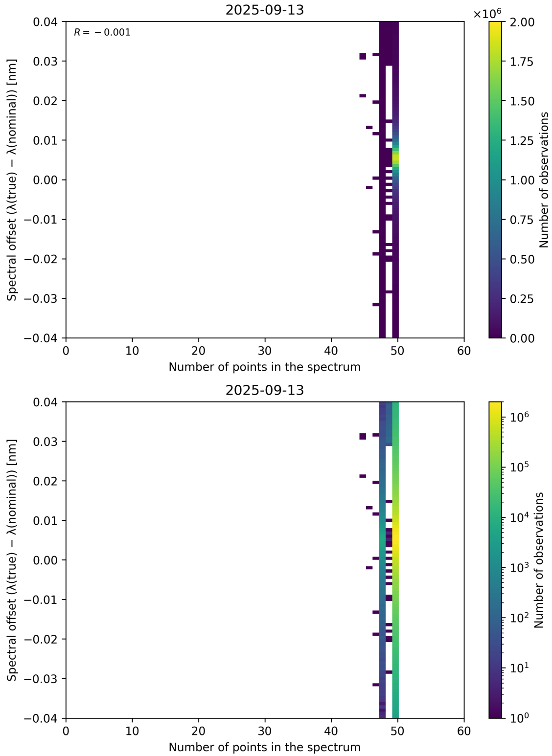
Figure 101: Scatter density plot of “Number of points in the spectrum” against “Spectral offset ( \lambda_{\text{true}} - \lambda_{\text{nominal}} )” for 2025-09-12 to 2025-09-14.
