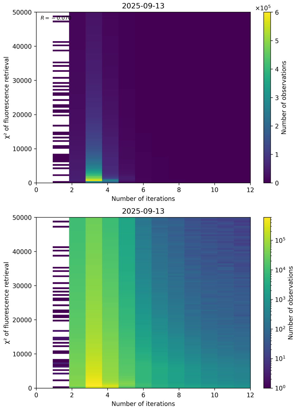
Figure 97: Scatter density plot of “Number of iterations” against “ \chi^2 of fluorescence retrieval” for 2025-09-12 to 2025-09-14.
