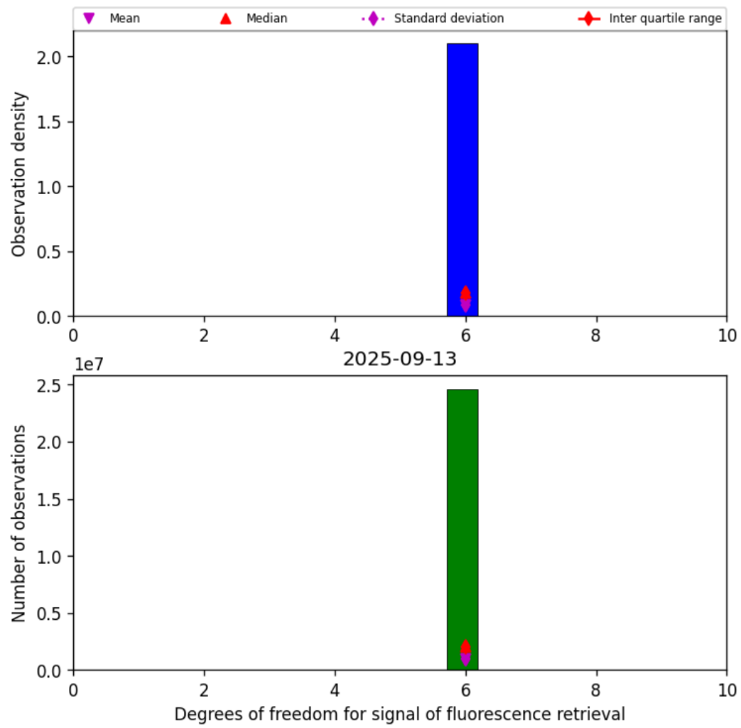
Figure 43: Histogram of “Degrees of freedom for signal of fluorescence retrieval” for 2025-09-12 to 2025-09-14
