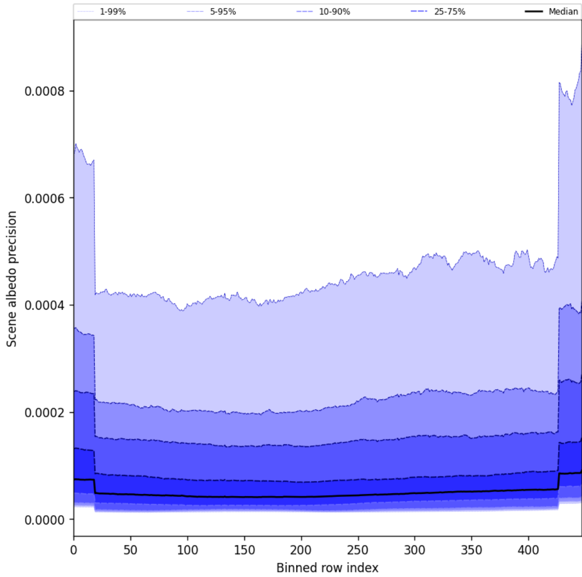
Figure 52: Along track statistics of “Scene albedo precision” for 2025-09-12 to 2025-09-14
