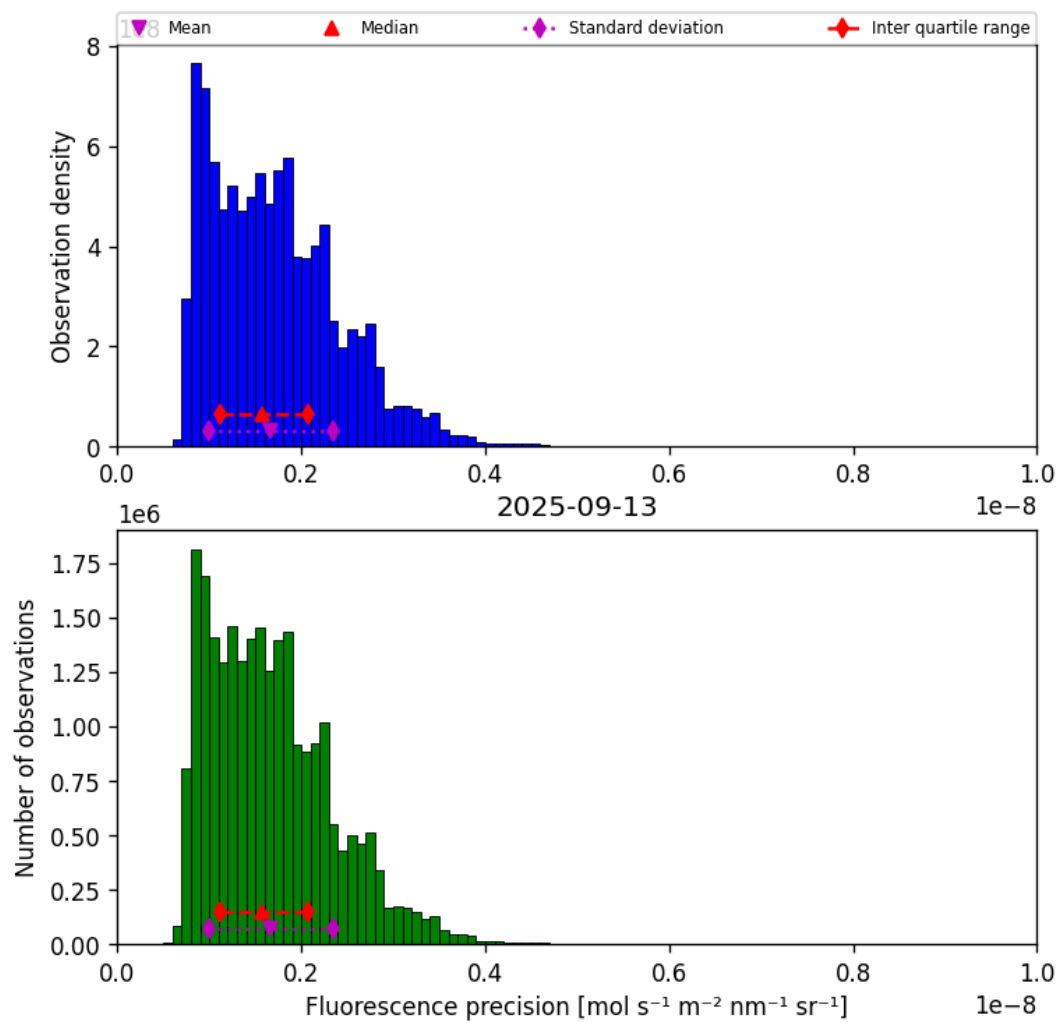
Figure 41: Histogram of “Fluorescence precision” for 2025-09-12 to 2025-09-14
