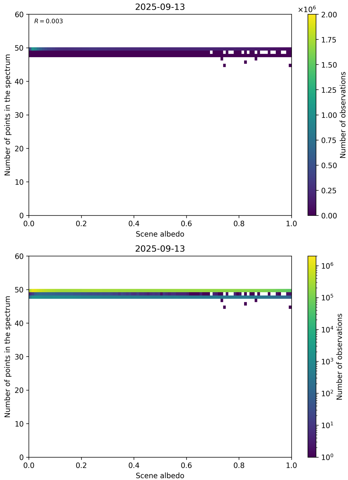
Figure 106: Scatter density plot of “Scene albedo” against “Number of points in the spectrum” for 2025-09-12 to 2025-09-14.
