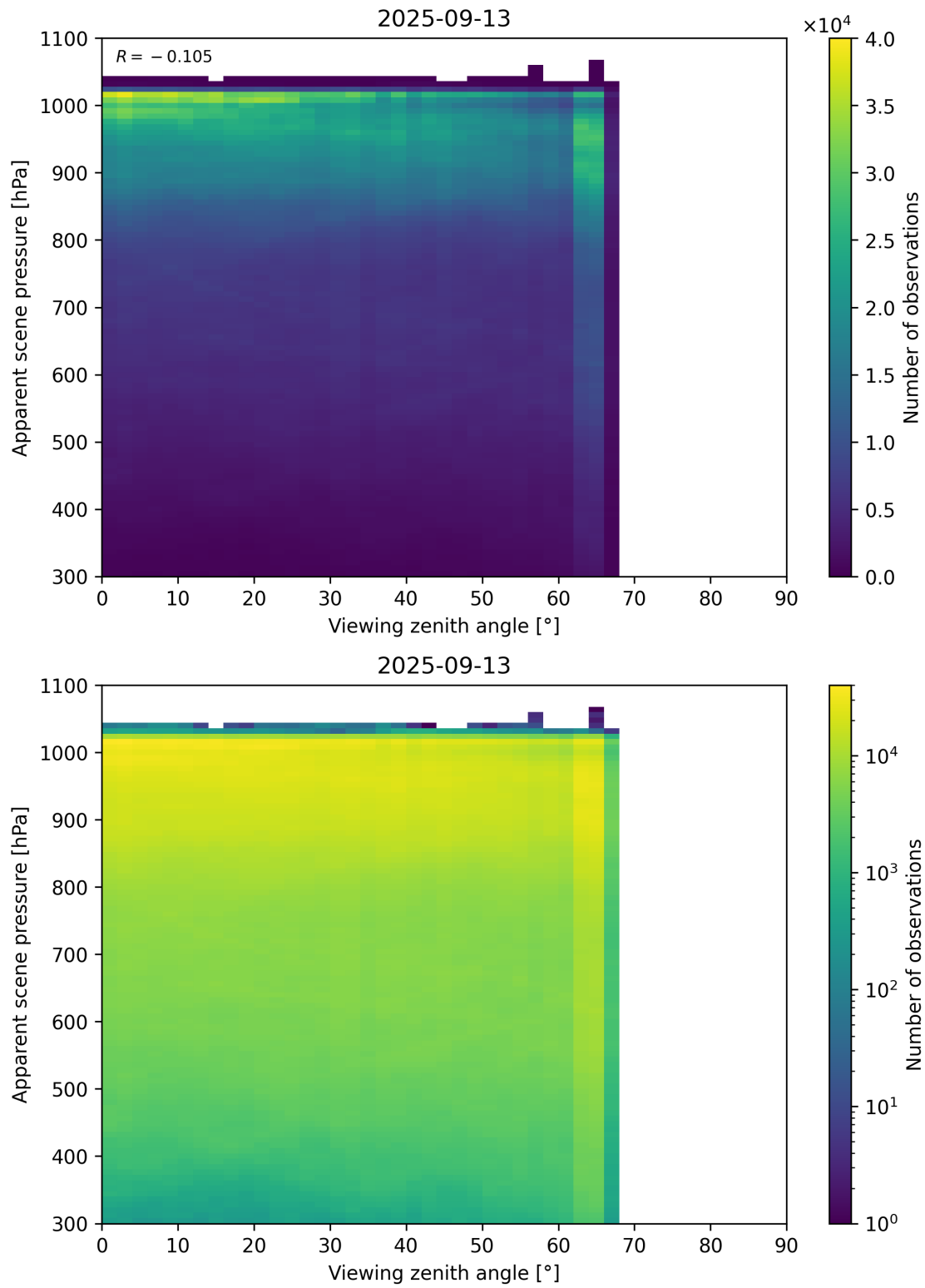
Figure 118: Scatter density plot of “Viewing zenith angle” against “Apparent scene pressure” for 2025-09-12 to 2025-09-14.
