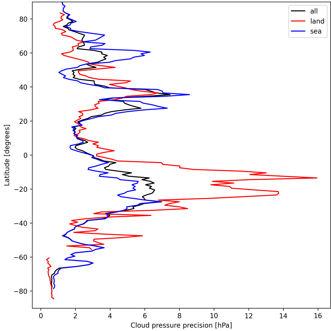
Figure 14: Zonal average of “Cloud pressure precision” for 2025-09-12 to 2025-09-14.
