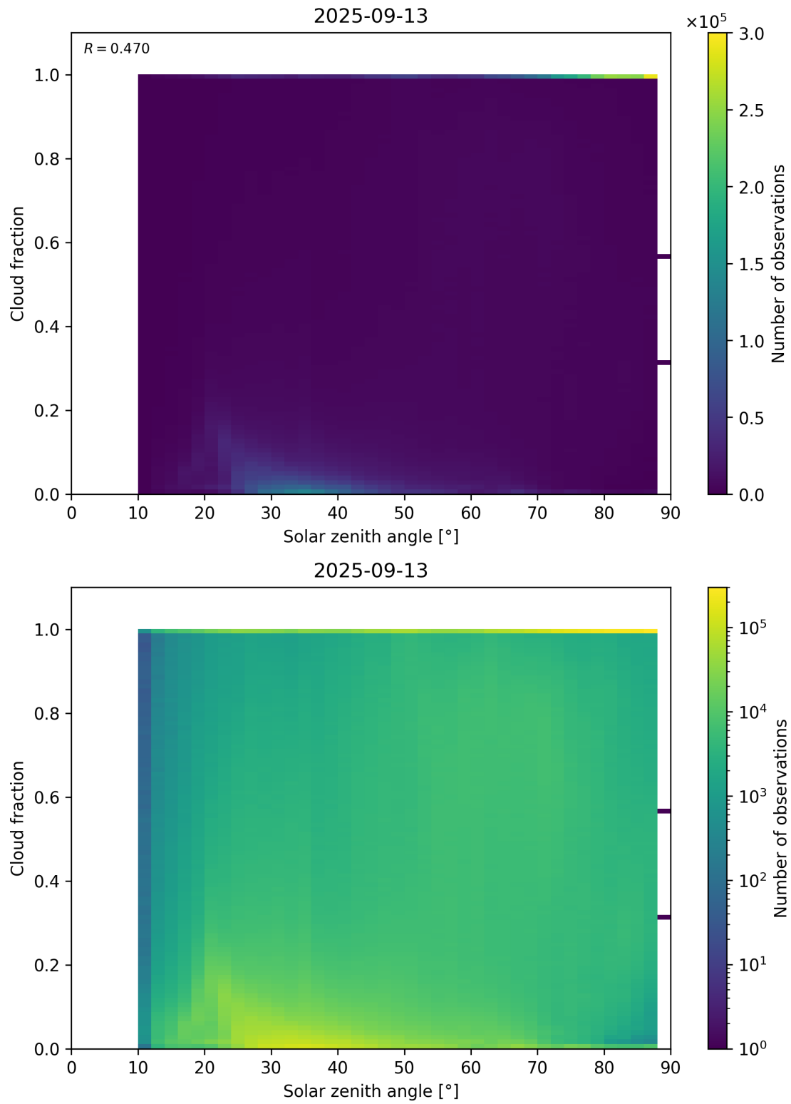
Figure 110: Scatter density plot of “Solar zenith angle” against “Cloud fraction” for 2025-09-12 to 2025-09-14.
