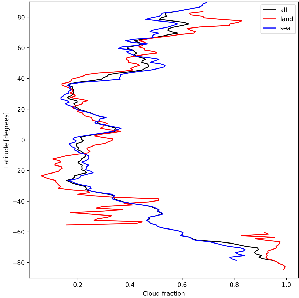
Figure 15: Zonal average of “Cloud fraction” for 2025-09-12 to 2025-09-14.
