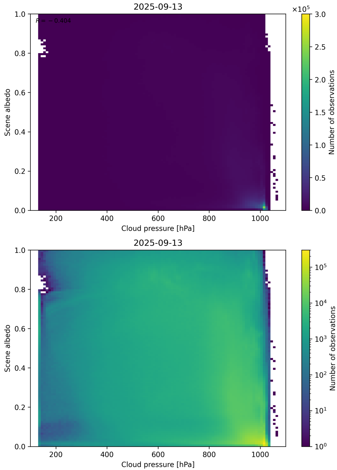
Figure 83: Scatter density plot of “Cloud pressure” against “Scene albedo” for 2025-09-12 to 2025-09-14.
