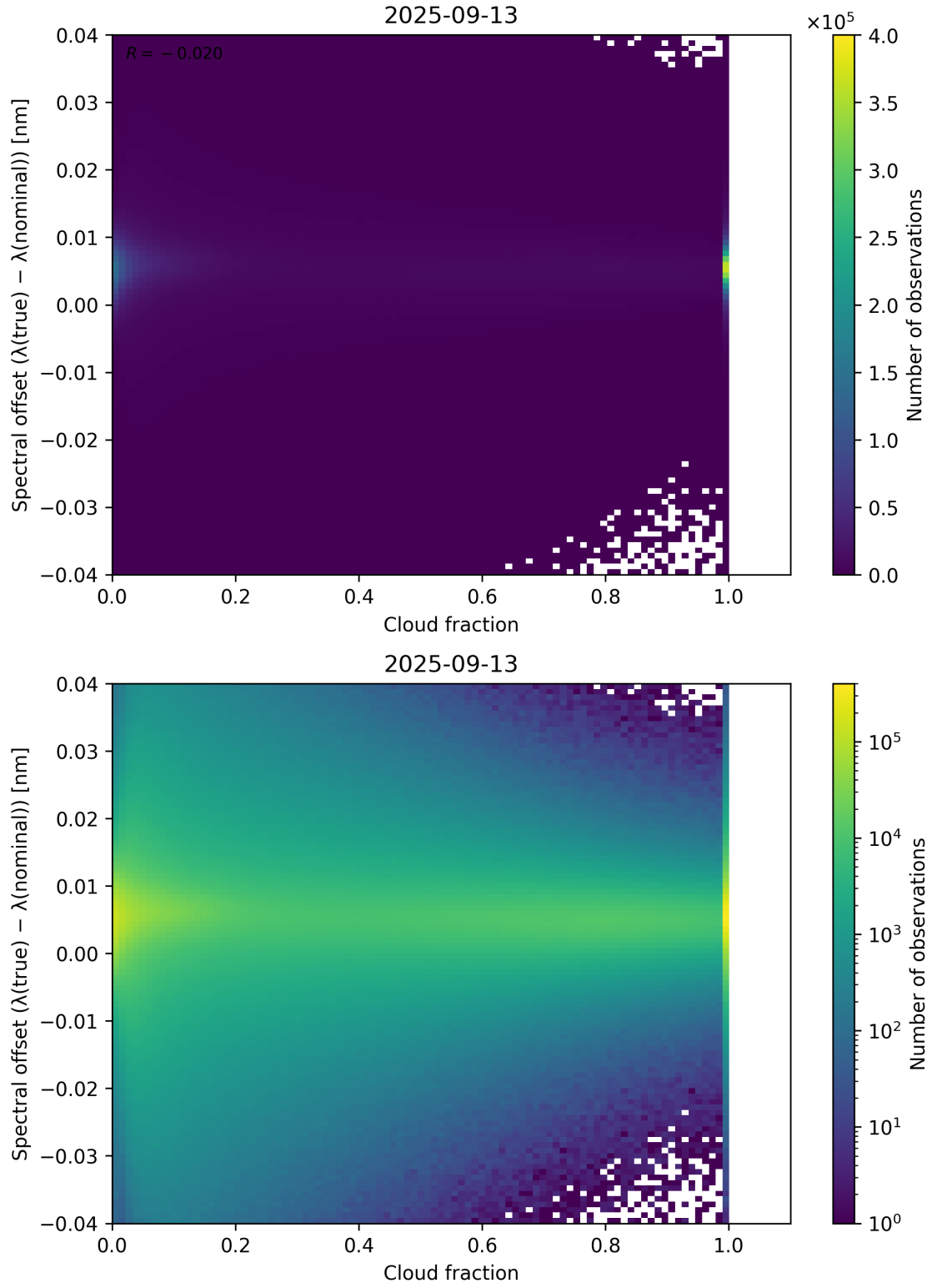
Figure 76: Scatter density plot of “Cloud fraction” against “Spectral offset ( \lambda_{\text{true}} - \lambda_{\text{nominal}} )” for 2025-09-12 to 2025-09-14.
