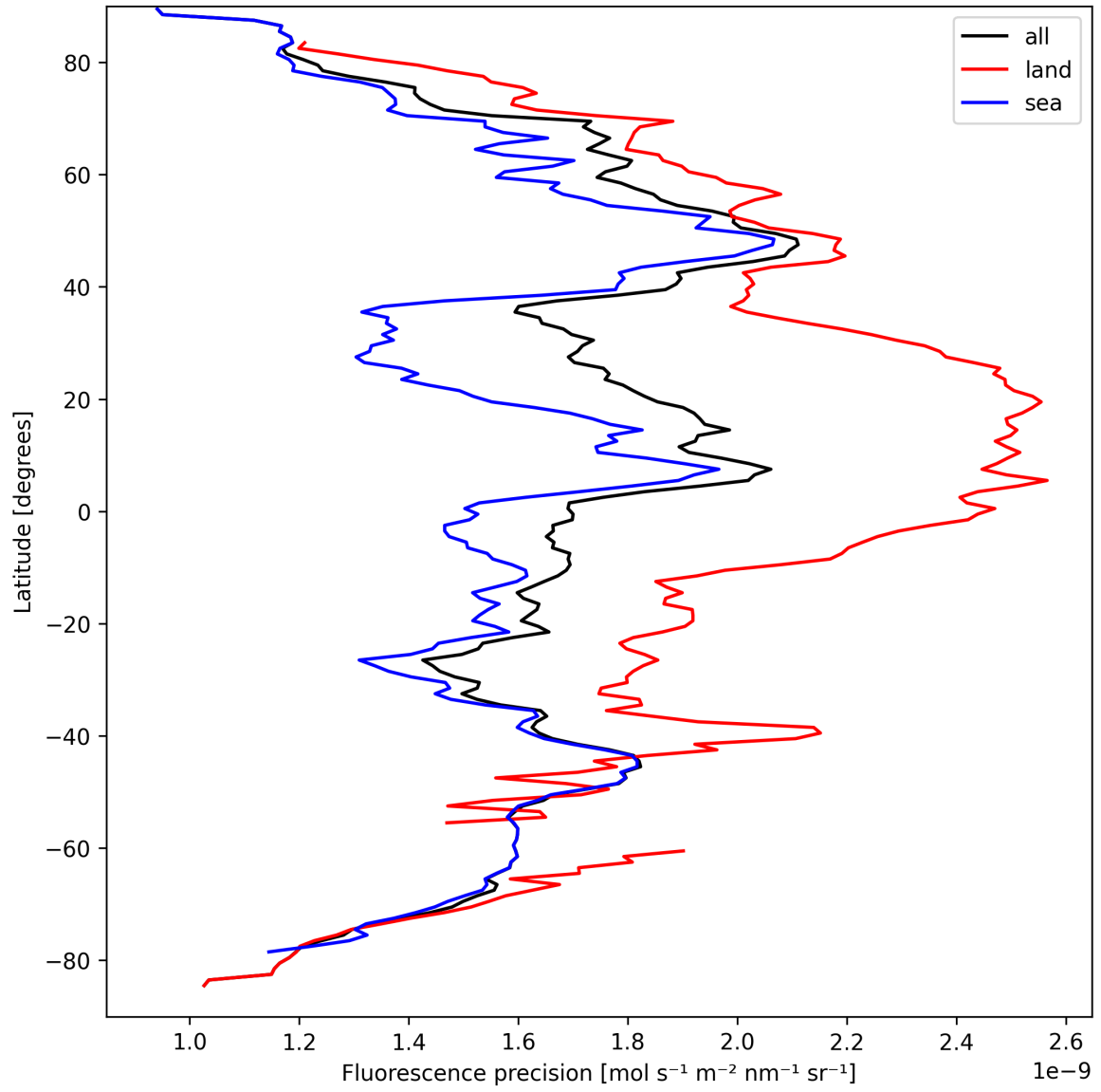
Figure 24: Zonal average of “Fluorescence precision” for 2025-09-12 to 2025-09-14.
