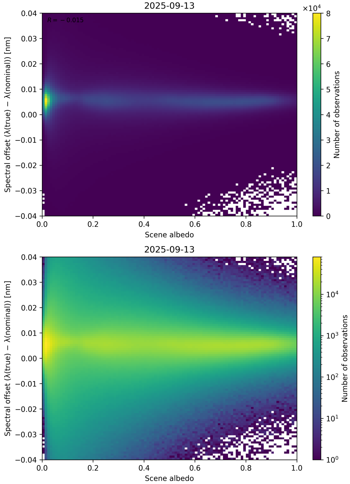
Figure 107: Scatter density plot of “Scene albedo” against “Spectral offset ( \lambda_{\text{true}} - \lambda_{\text{nominal}} )” for 2025-09-12 to 2025-09-14.
