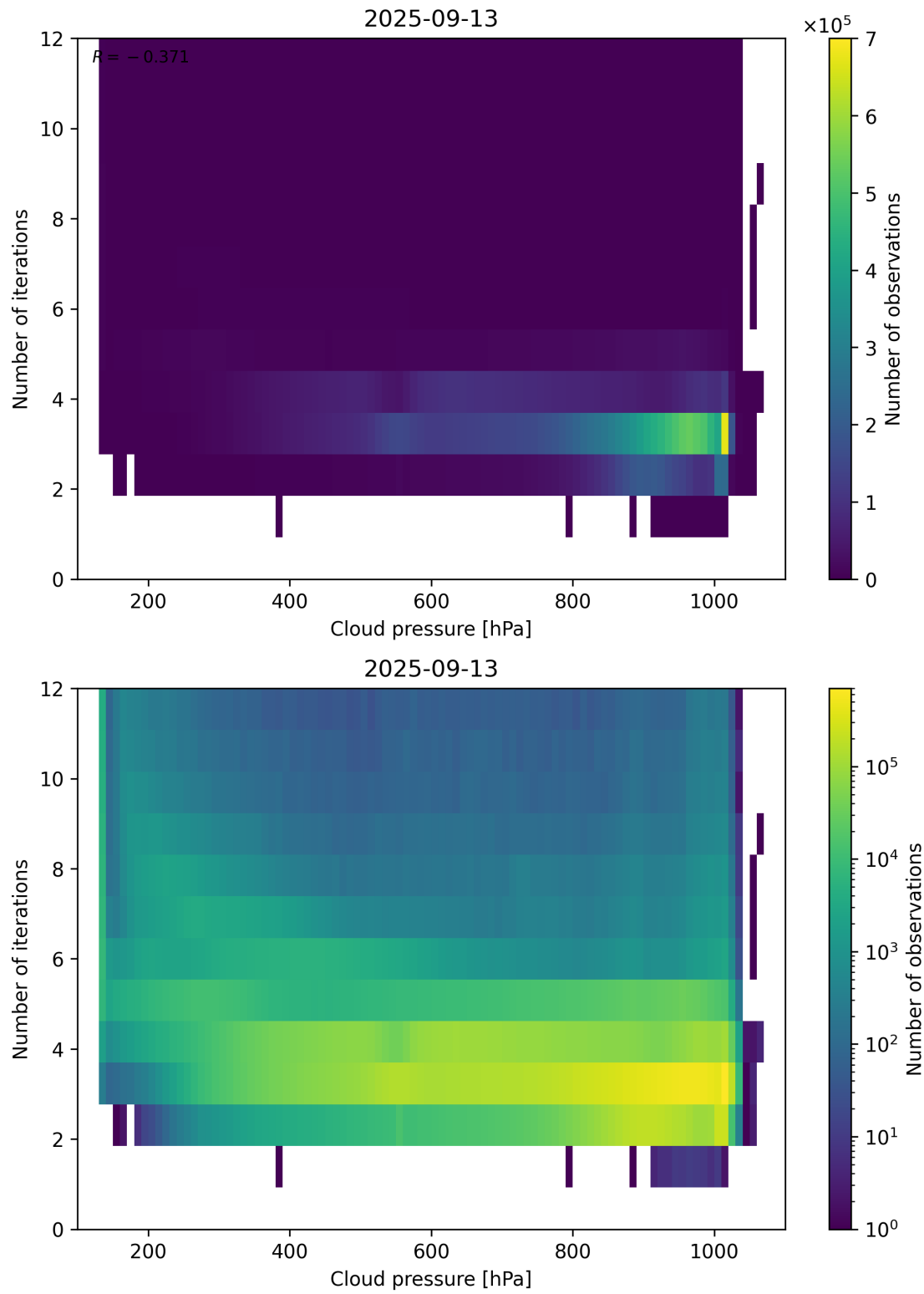
Figure 81: Scatter density plot of “Cloud pressure” against “Number of iterations” for 2025-09-12 to 2025-09-14.
