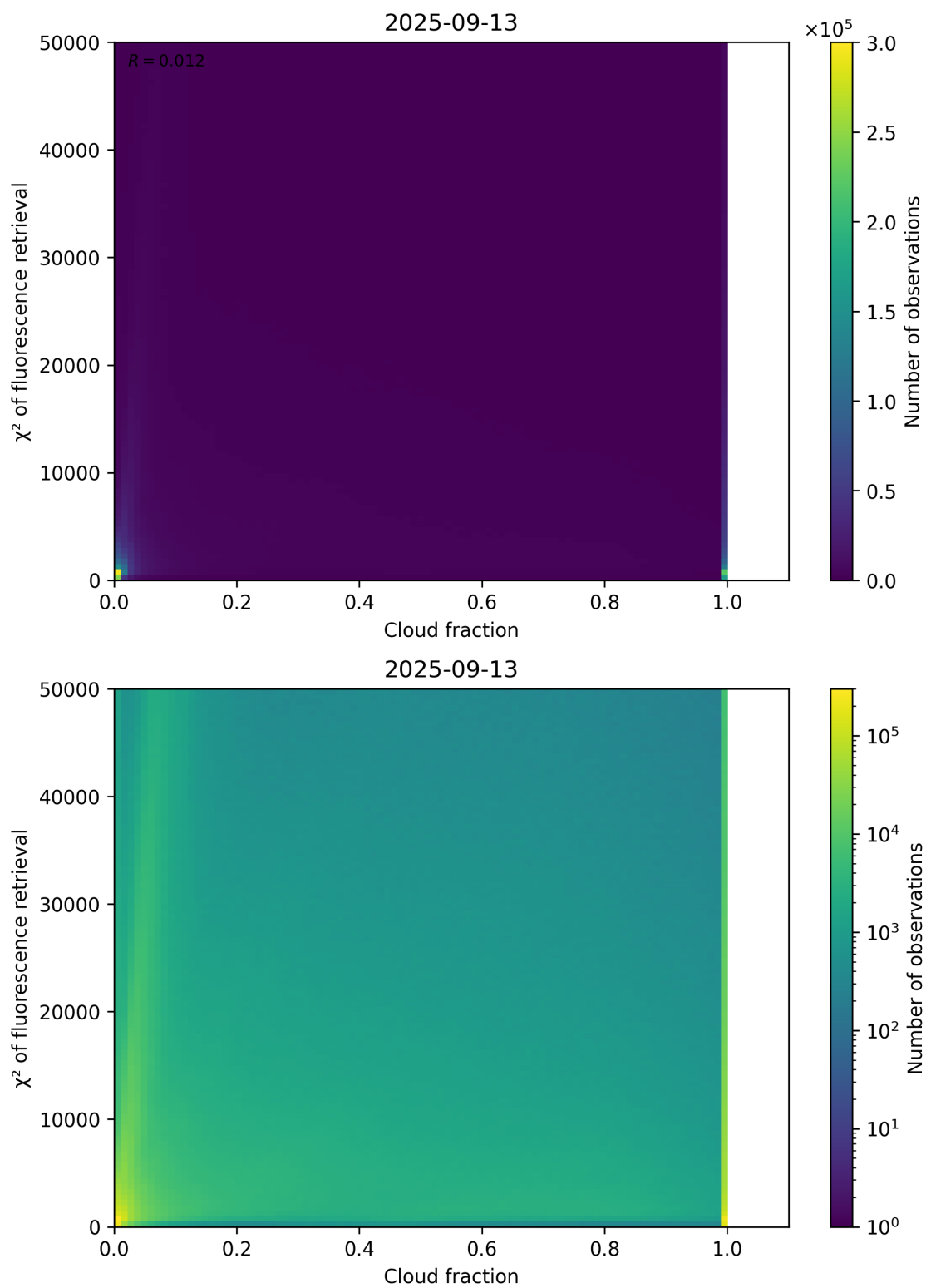
Figure 71: Scatter density plot of “Cloud fraction” against “ \chi^2 of fluorescence retrieval” for 2025-09-12 to 2025-09-14.
