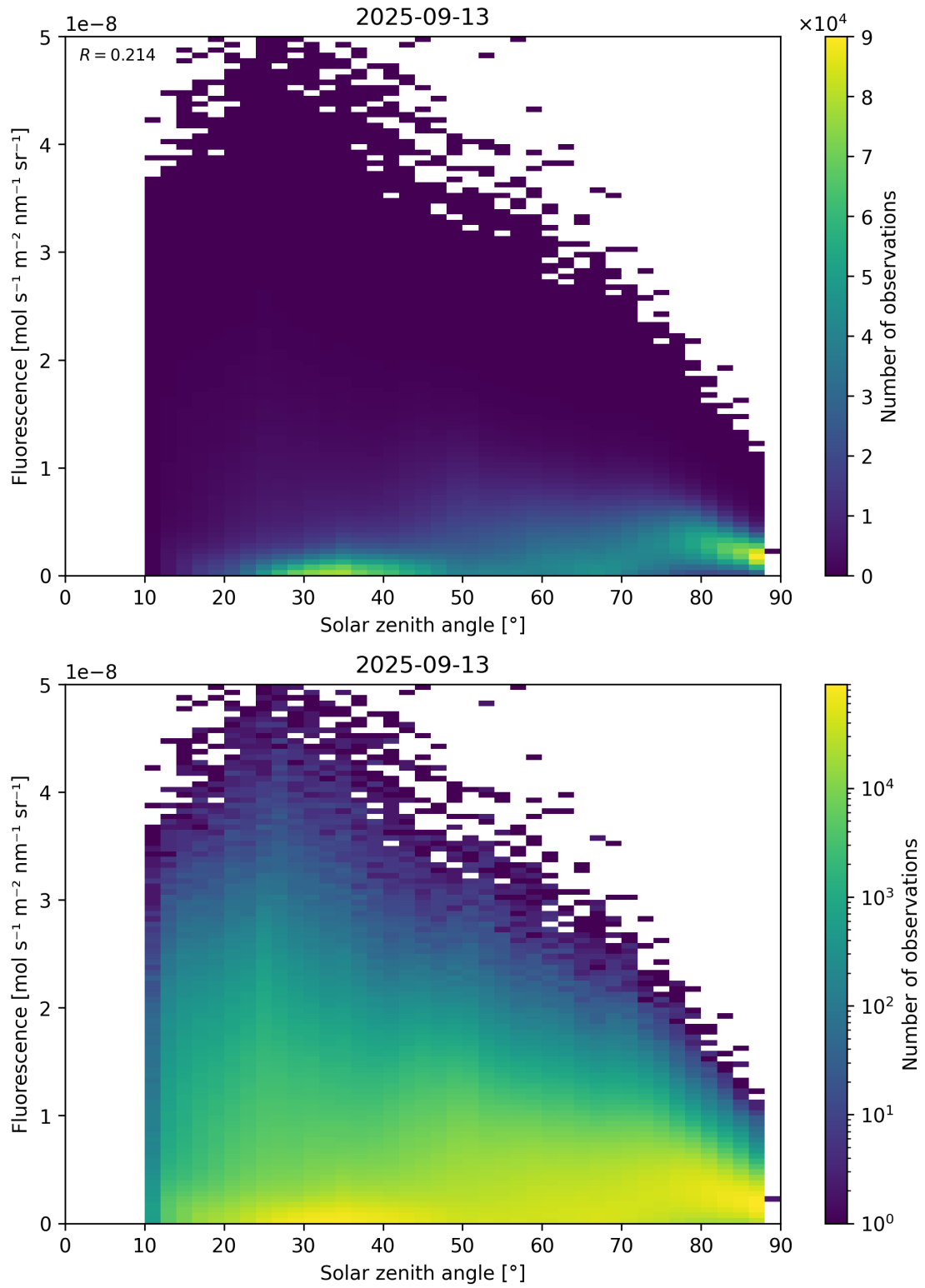
Figure 112: Scatter density plot of “Solar zenith angle” against “Fluorescence” for 2025-09-12 to 2025-09-14.
