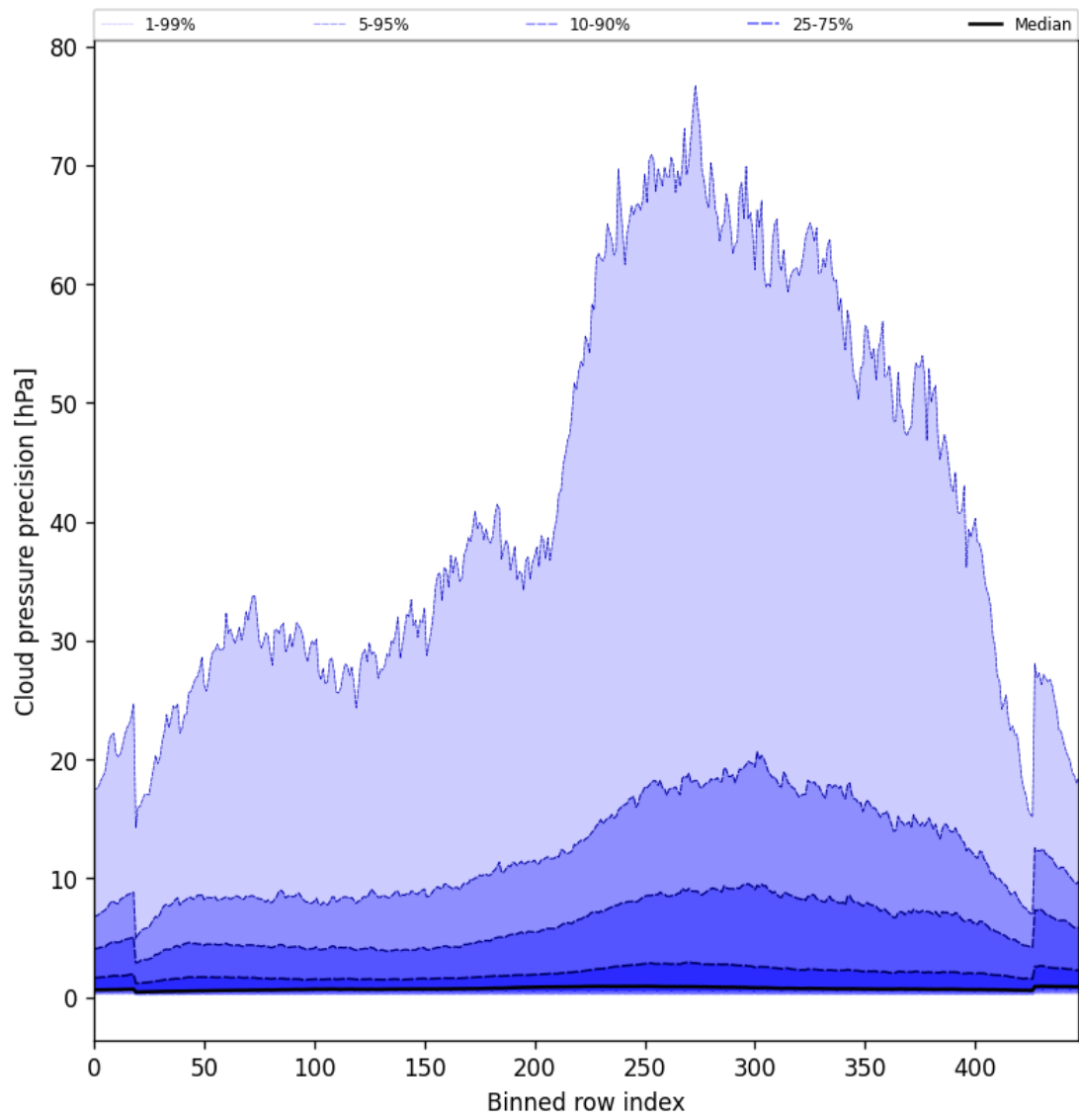
Figure 48: Along track statistics of “Cloud pressure precision” for 2025-09-12 to 2025-09-14
