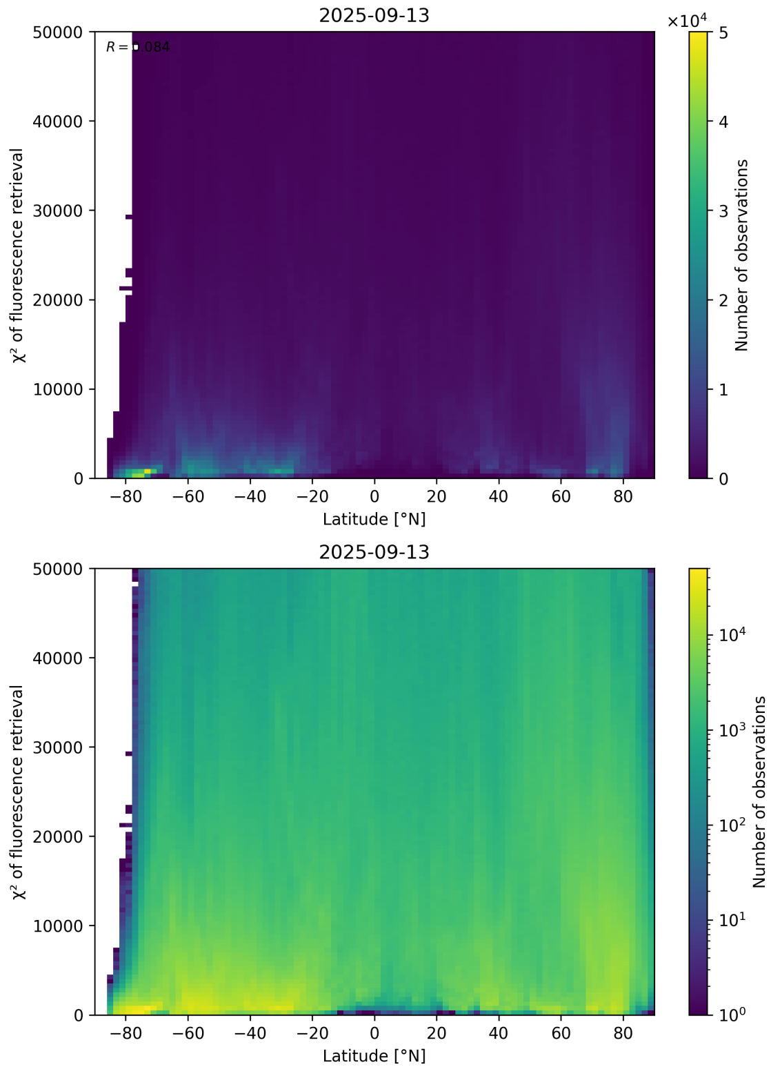
Figure 89: Scatter density plot of “Latitude” against “ \chi^2 of fluorescence retrieval” for 2025-09-12 to 2025-09-14.
