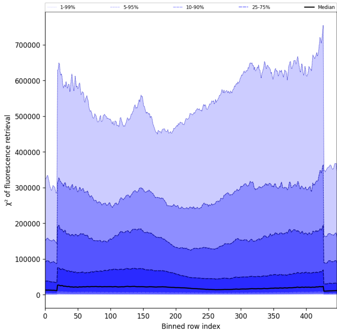
Figure 59: Along track statistics of “ \chi^2 of fluorescence retrieval” for 2025-09-12 to 2025-09-14
