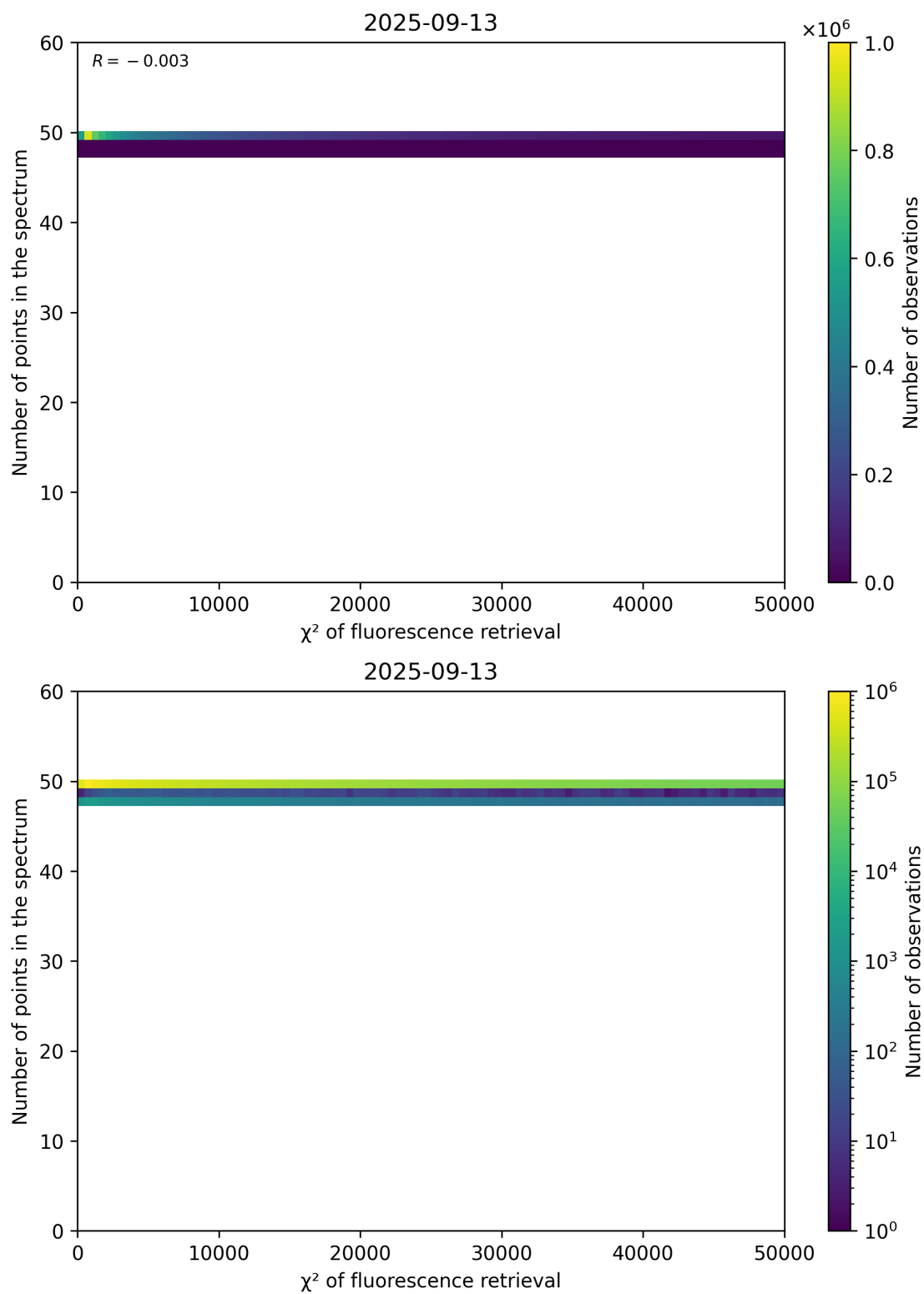
Figure 68: Scatter density plot of " \chi^2 of fluorescence retrieval" against "Number of points in the spectrum" for 2025-09-12 to 2025-09-14.
