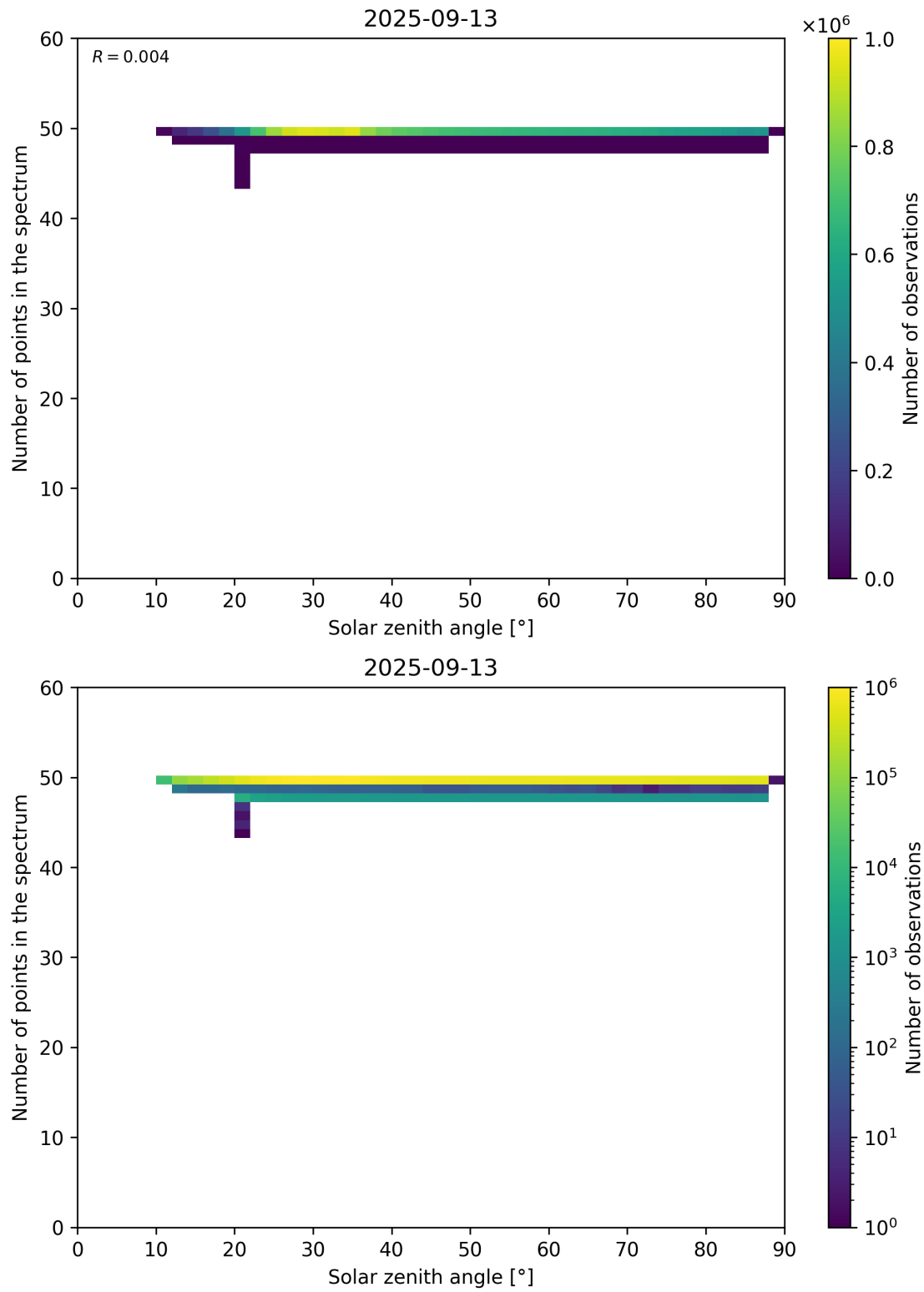
Figure 115: Scatter density plot of “Solar zenith angle” against “Number of points in the spectrum” for 2025-09-12 to 2025-09-14.
