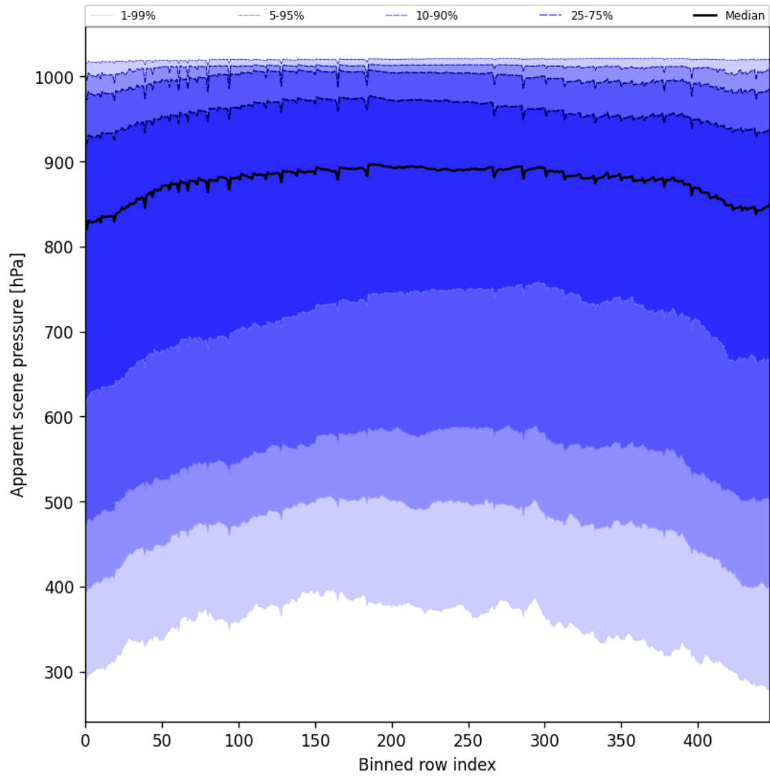
Figure 53: Along track statistics of “Apparent scene pressure” for 2025-09-12 to 2025-09-14
