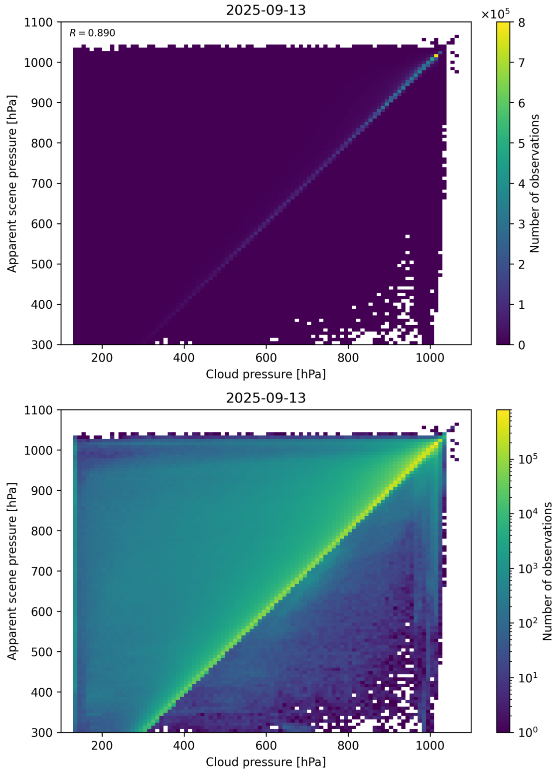
Figure 77: Scatter density plot of “Cloud pressure” against “Apparent scene pressure” for 2025-09-12 to 2025-09-14.
