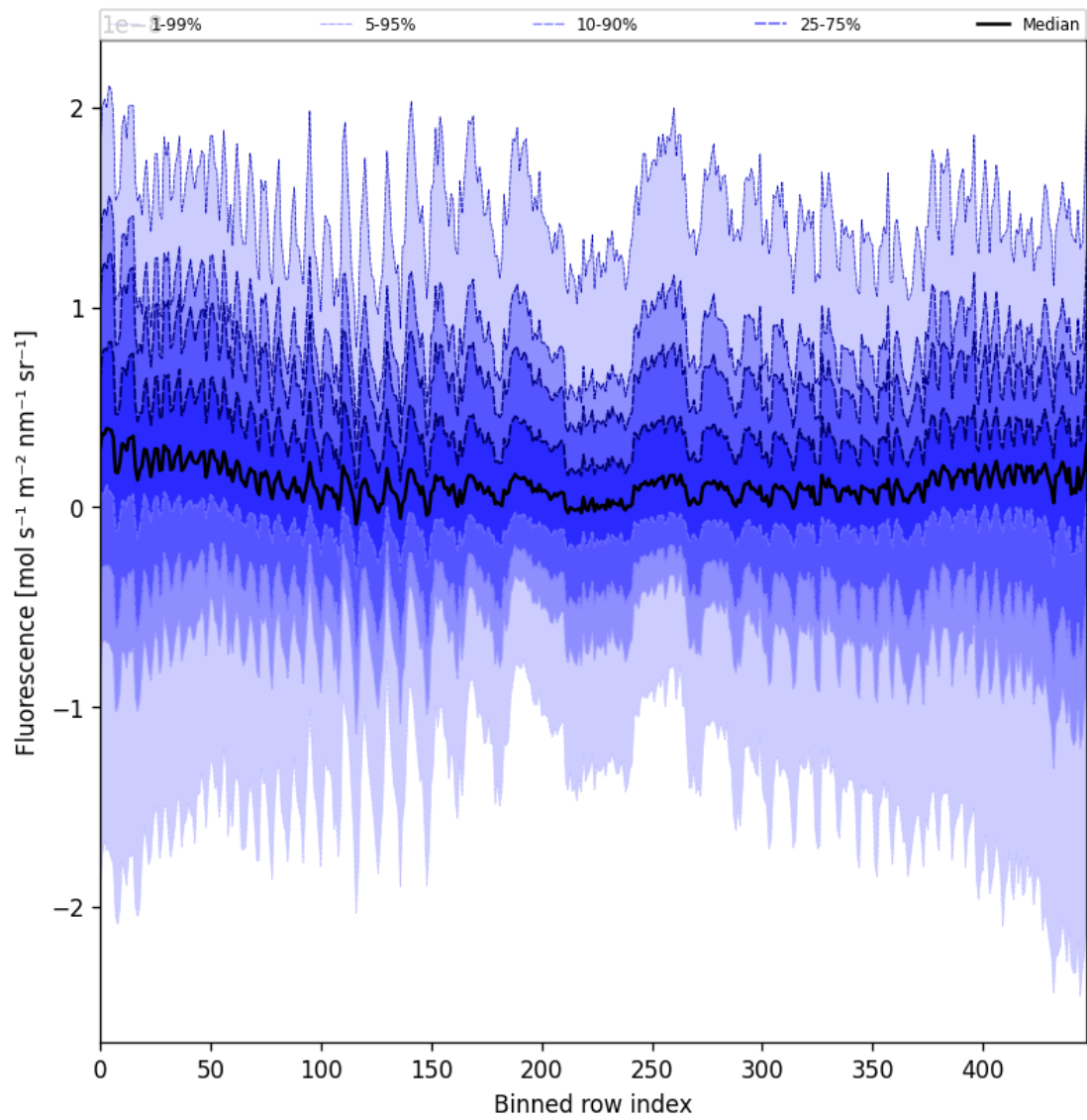
Figure 57: Along track statistics of “Fluorescence” for 2025-09-13 to 2025-09-15
