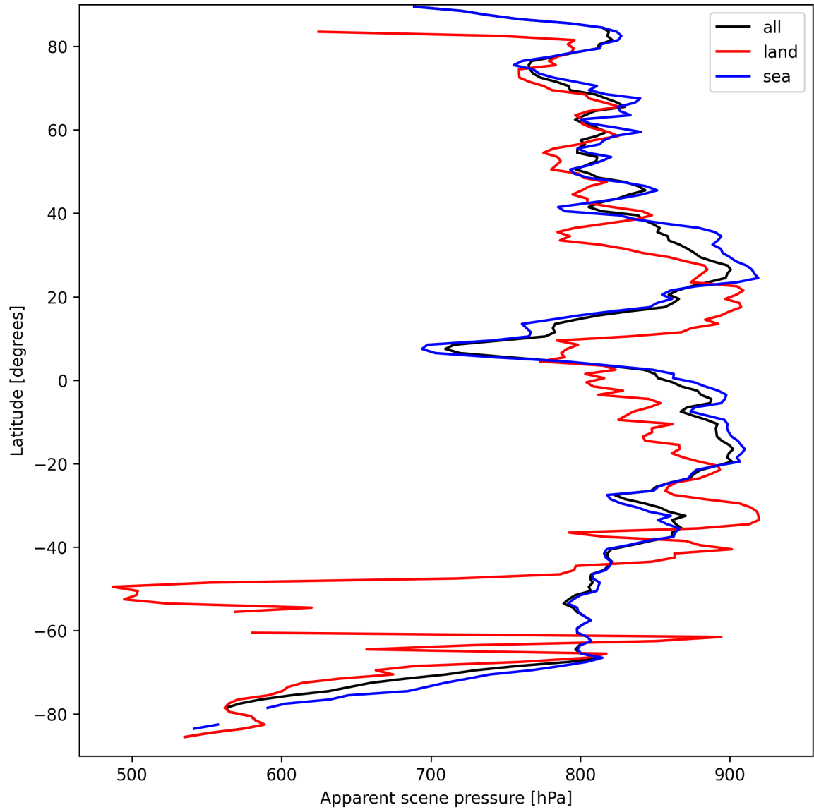
Figure 19: Zonal average of “Apparent scene pressure” for 2025-09-13 to 2025-09-15.
