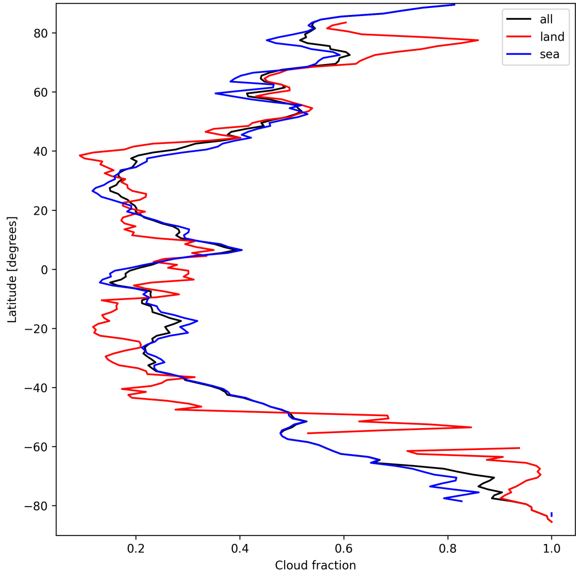
Figure 15: Zonal average of “Cloud fraction” for 2025-09-13 to 2025-09-15.
