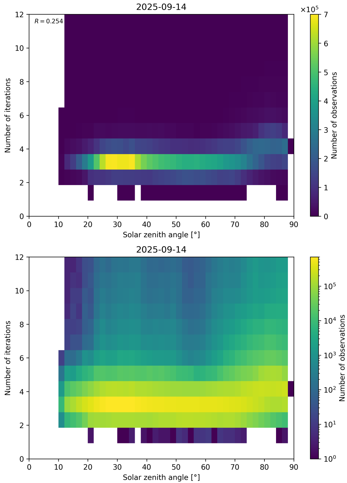
Figure 114: Scatter density plot of “Solar zenith angle” against “Number of iterations” for 2025-09-13 to 2025-09-15.
