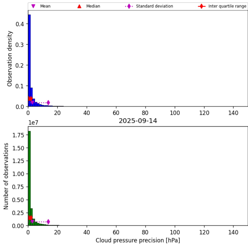
Figure 31: Histogram of “Cloud pressure precision” for 2025-09-13 to 2025-09-15
