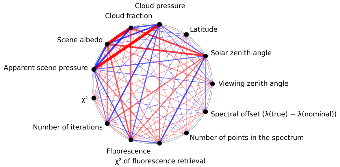
Figure 1: Map of correlation graph for 2025-09-13 to 2025-09-15.
