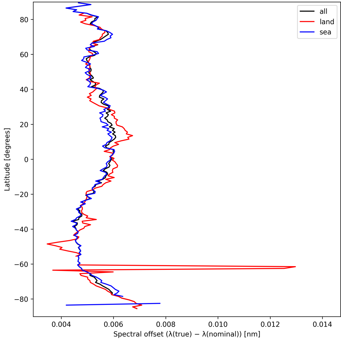
Figure 28: Zonal average of “Spectral offset ( \lambda_{\text{true}} - \lambda_{\text{nominal}} )” for 2025-09-13 to 2025-09-15.
