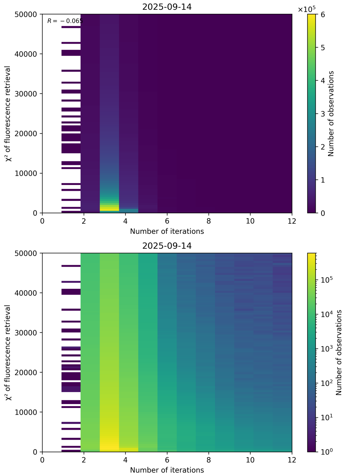
Figure 97: Scatter density plot of “Number of iterations” against “ \chi^2 of fluorescence retrieval” for 2025-09-13 to 2025-09-15.
