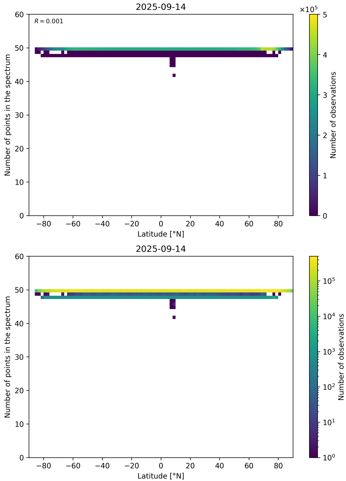
Figure 94: Scatter density plot of “Latitude” against “Number of points in the spectrum” for 2025-09-13 to 2025-09-15.
