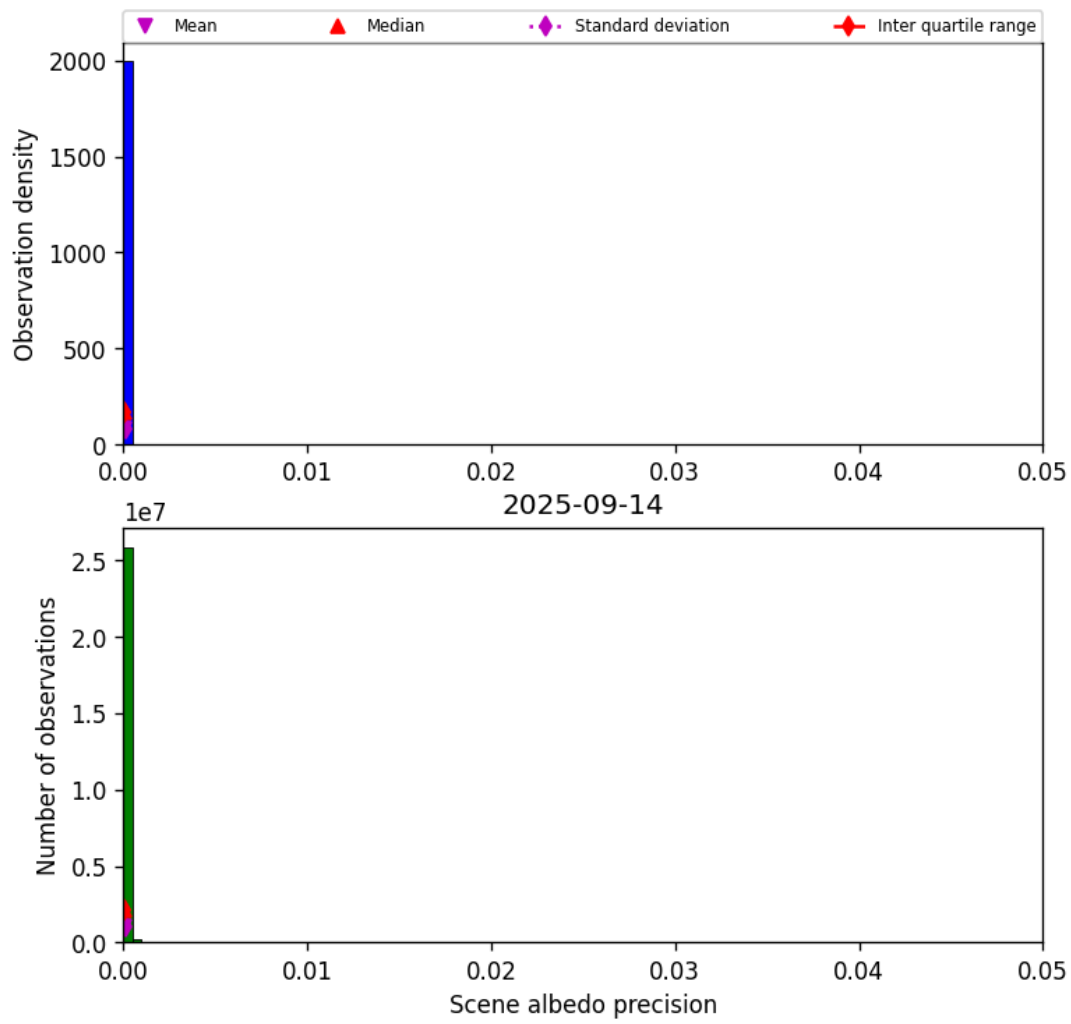
Figure 35: Histogram of “Scene albedo precision” for 2025-09-13 to 2025-09-15
