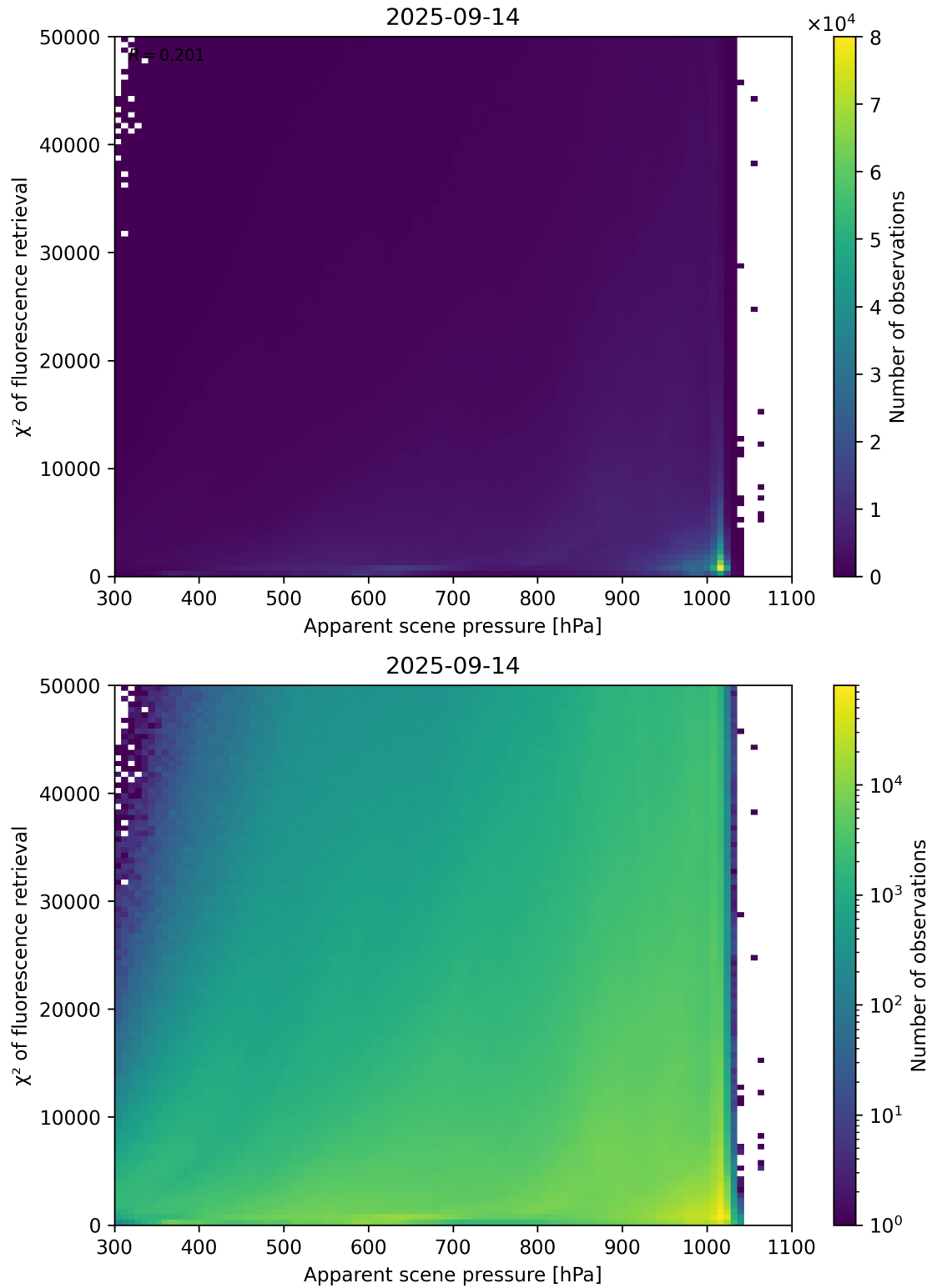
Figure 63: Scatter density plot of “Apparent scene pressure” against “ \chi^2 of fluorescence retrieval” for 2025-09-13 to 2025-09-15.
