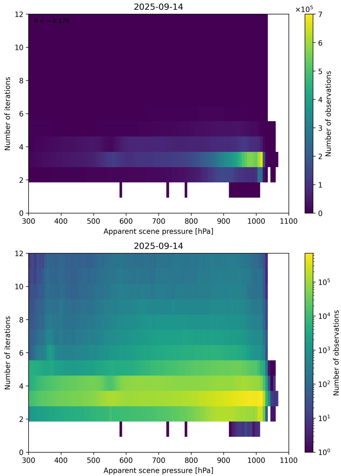
Figure 65: Scatter density plot of “Apparent scene pressure” against “Number of iterations” for 2025-09-13 to 2025-09-15.
