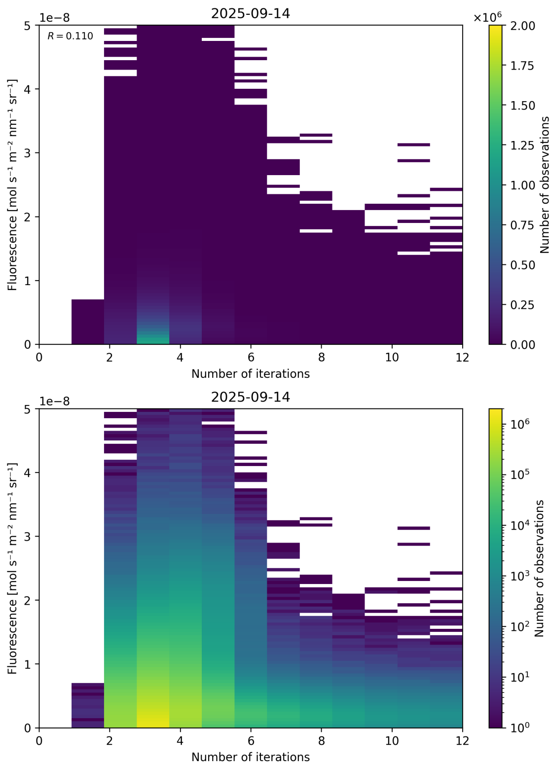
Figure 98: Scatter density plot of “Number of iterations” against “Fluorescence” for 2025-09-13 to 2025-09-15.
