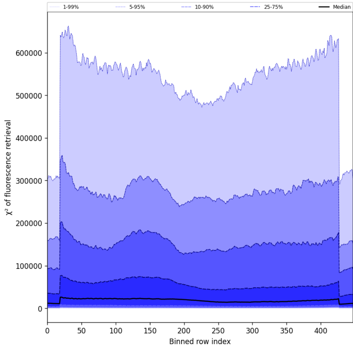
Figure 59: Along track statistics of “ \chi^2 of fluorescence retrieval” for 2025-09-13 to 2025-09-15
