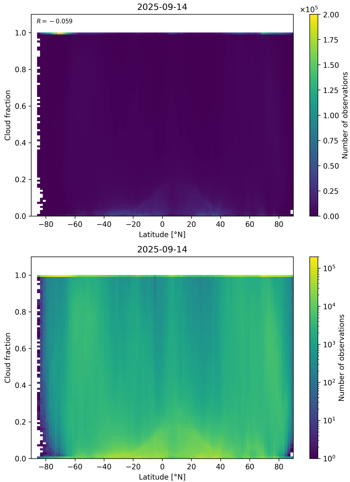
Figure 90: Scatter density plot of “Latitude” against “Cloud fraction” for 2025-09-13 to 2025-09-15.
