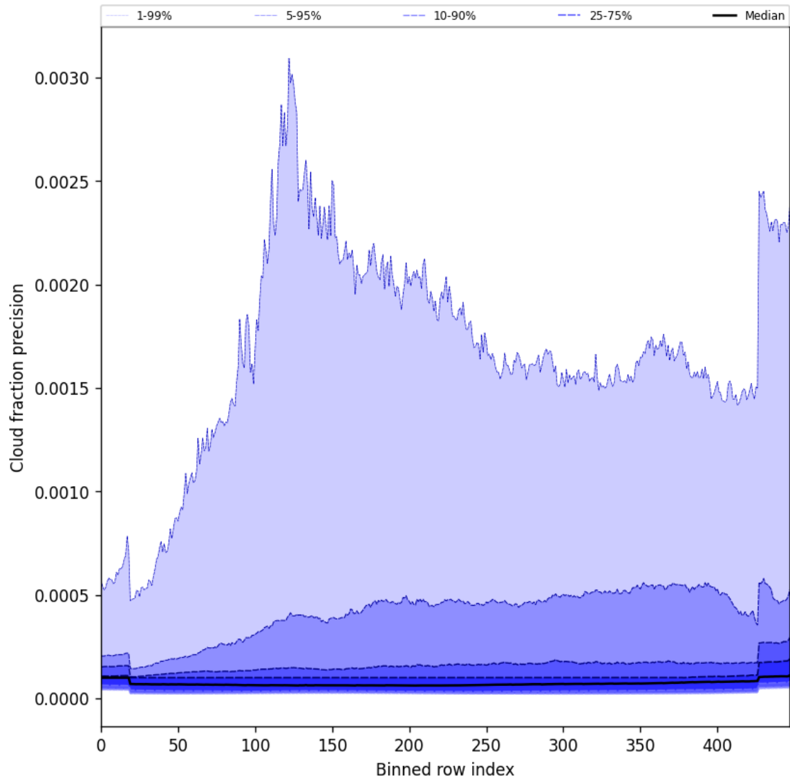
Figure 50: Along track statistics of “Cloud fraction precision” for 2025-09-13 to 2025-09-15
