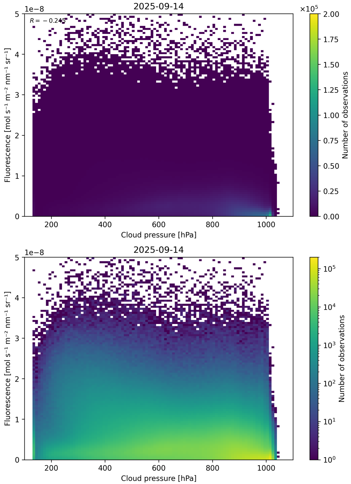
Figure 80: Scatter density plot of “Cloud pressure” against “Fluorescence” for 2025-09-13 to 2025-09-15.
