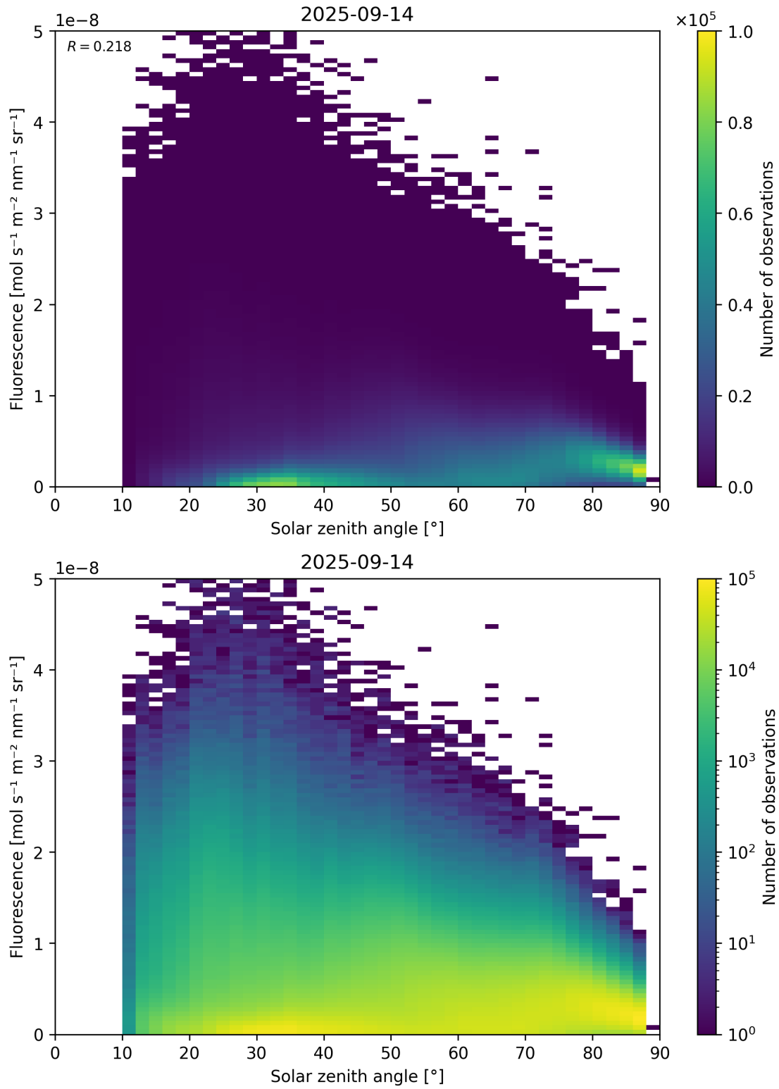
Figure 112: Scatter density plot of “Solar zenith angle” against “Fluorescence” for 2025-09-13 to 2025-09-15.
