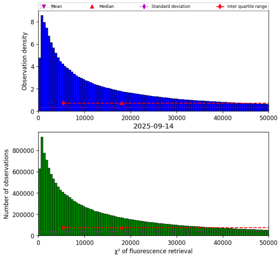
Figure 42: Histogram of “ \chi^2 of fluorescence retrieval” for 2025-09-13 to 2025-09-15
