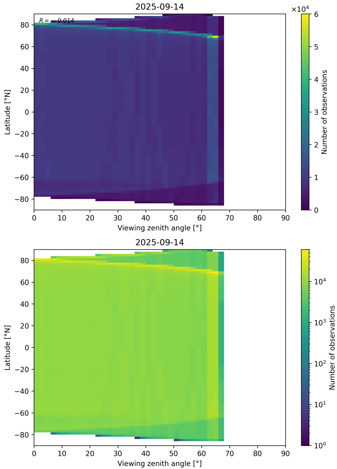
Figure 123: Scatter density plot of “Viewing zenith angle” against “Latitude” for 2025-09-13 to 2025-09-15.
