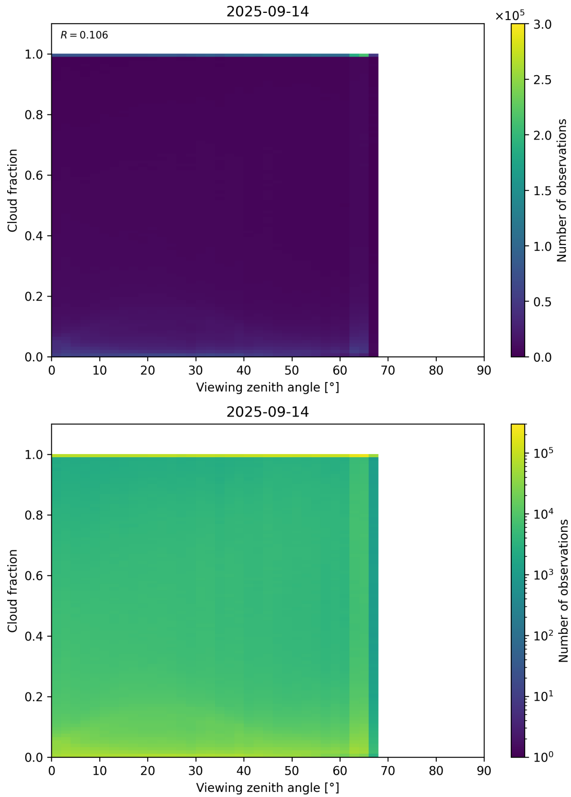
Figure 120: Scatter density plot of “Viewing zenith angle” against “Cloud fraction” for 2025-09-13 to 2025-09-15.
