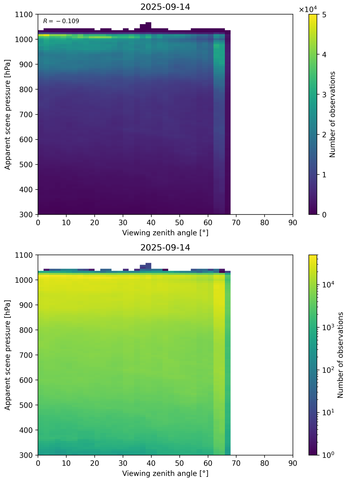
Figure 118: Scatter density plot of “Viewing zenith angle” against “Apparent scene pressure” for 2025-09-13 to 2025-09-15.
