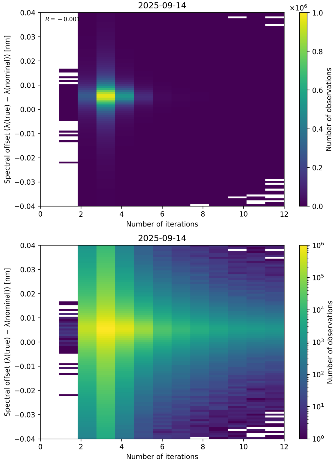
Figure 100: Scatter density plot of “Number of iterations” against “Spectral offset ( \lambda_{\text{true}} - \lambda_{\text{nominal}} )” for 2025-09-13 to 2025-09-15.
