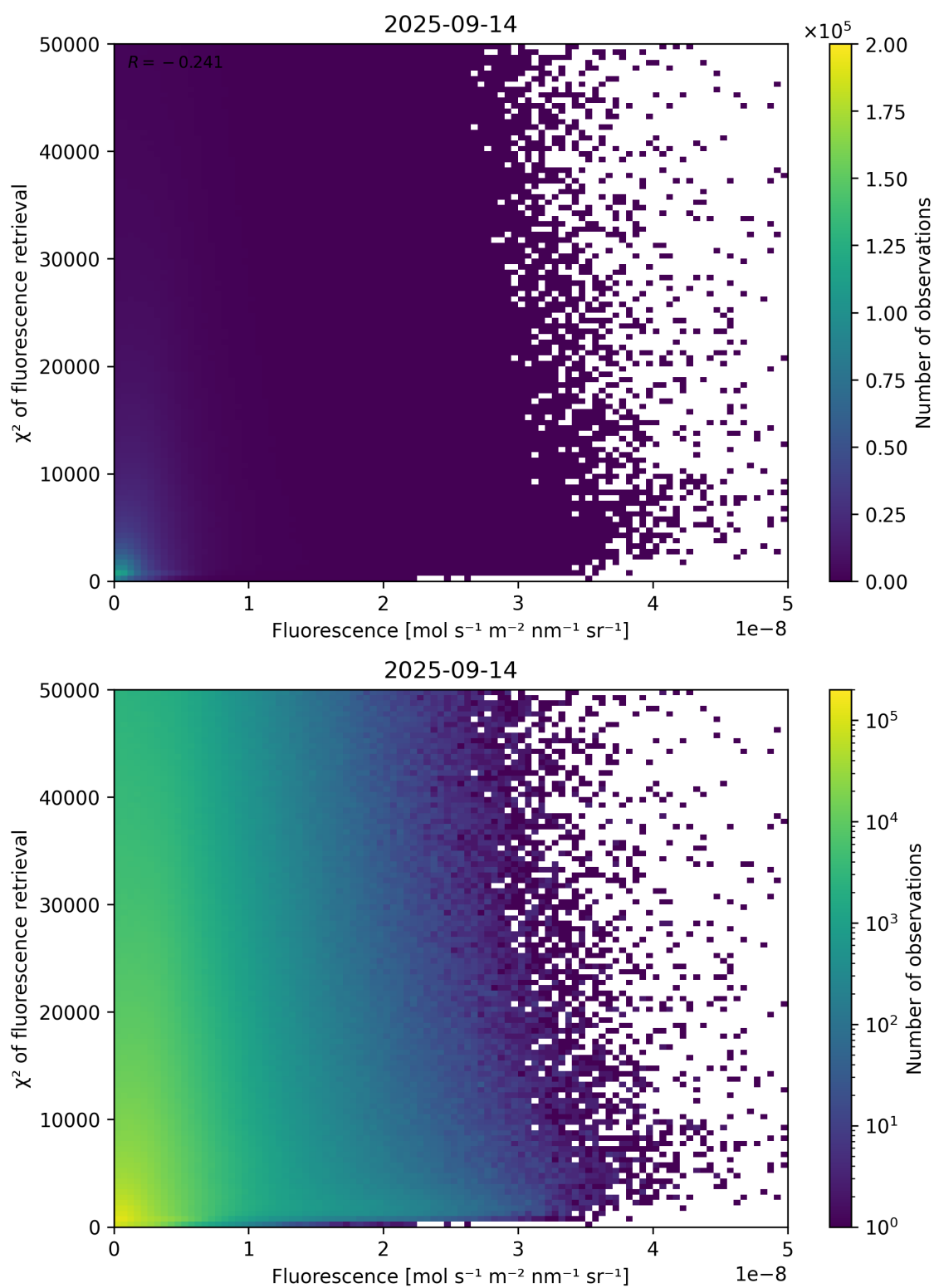
Figure 85: Scatter density plot of “Fluorescence” against “ \chi^2 of fluorescence retrieval” for 2025-09-13 to 2025-09-15.
