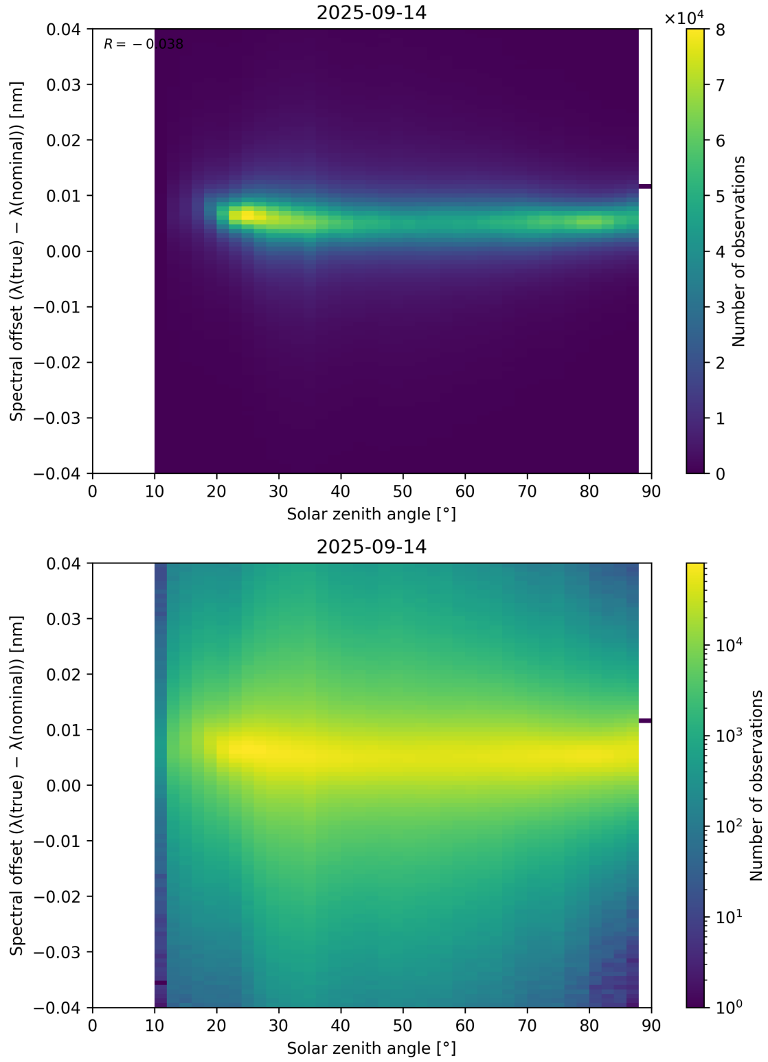
Figure 117: Scatter density plot of “Solar zenith angle” against “Spectral offset ( \lambda_{\text{true}} - \lambda_{\text{nominal}} )” for 2025-09-13 to 2025-09-15.
