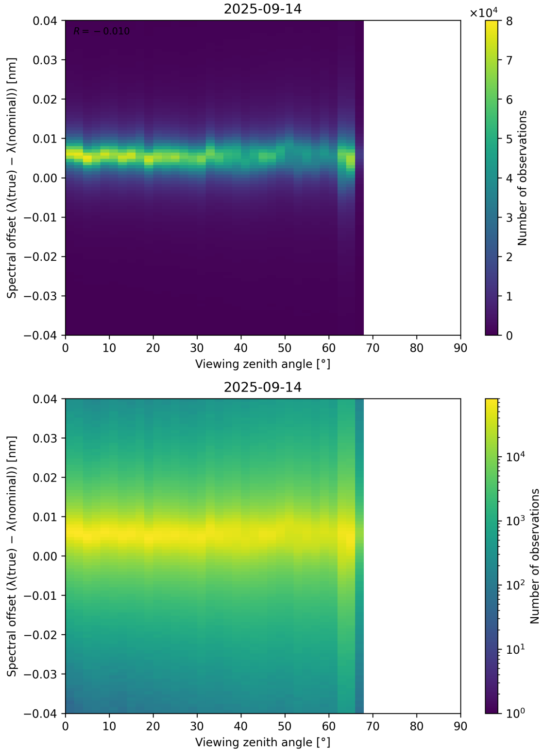
Figure 128: Scatter density plot of “Viewing zenith angle” against “Spectral offset ( \lambda_{\text{true}} - \lambda_{\text{nominal}} )” for 2025-09-13 to 2025-09-15.
