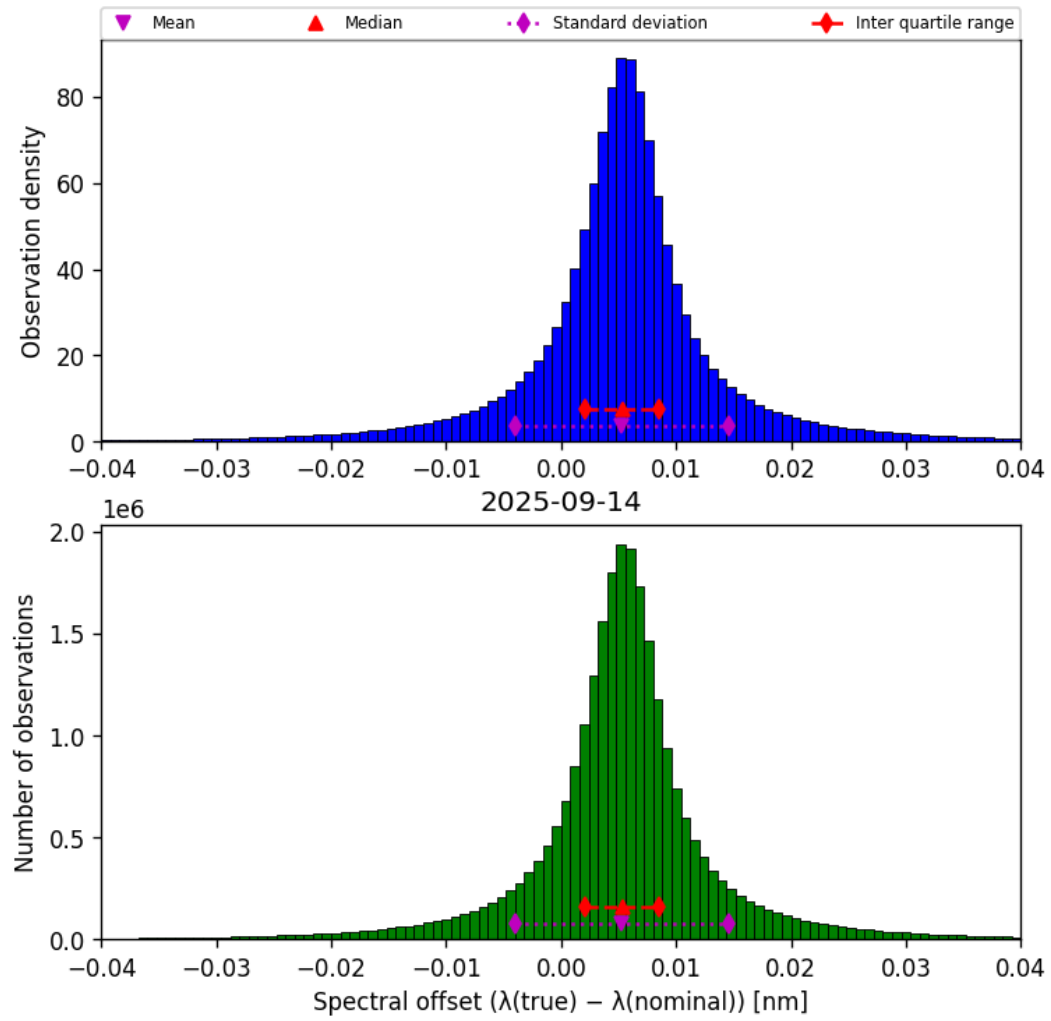
Figure 45: Histogram of “Spectral offset ( \lambda_{\text{true}} - \lambda_{\text{nominal}} )” for 2025-09-13 to 2025-09-15
