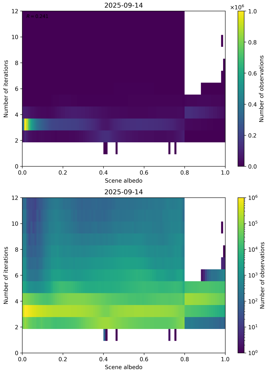
Figure 105: Scatter density plot of “Scene albedo” against “Number of iterations” for 2025-09-13 to 2025-09-15.
