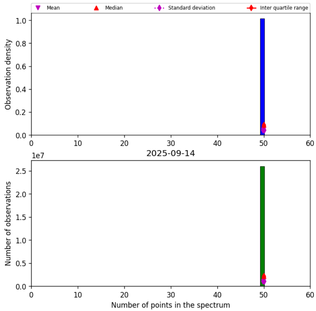
Figure 44: Histogram of “Number of points in the spectrum” for 2025-09-13 to 2025-09-15
