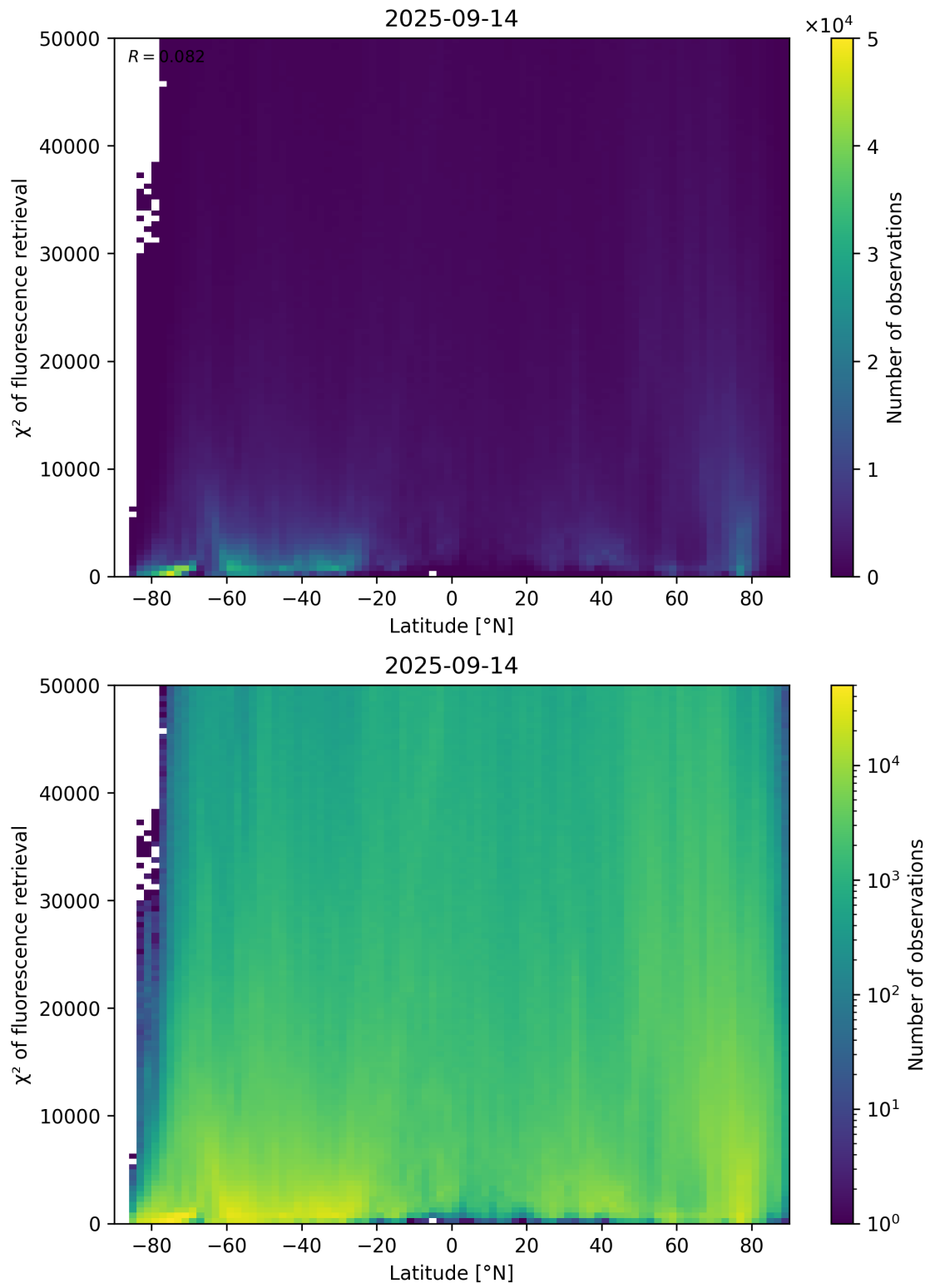
Figure 89: Scatter density plot of “Latitude” against “ \chi^2 of fluorescence retrieval” for 2025-09-13 to 2025-09-15.
