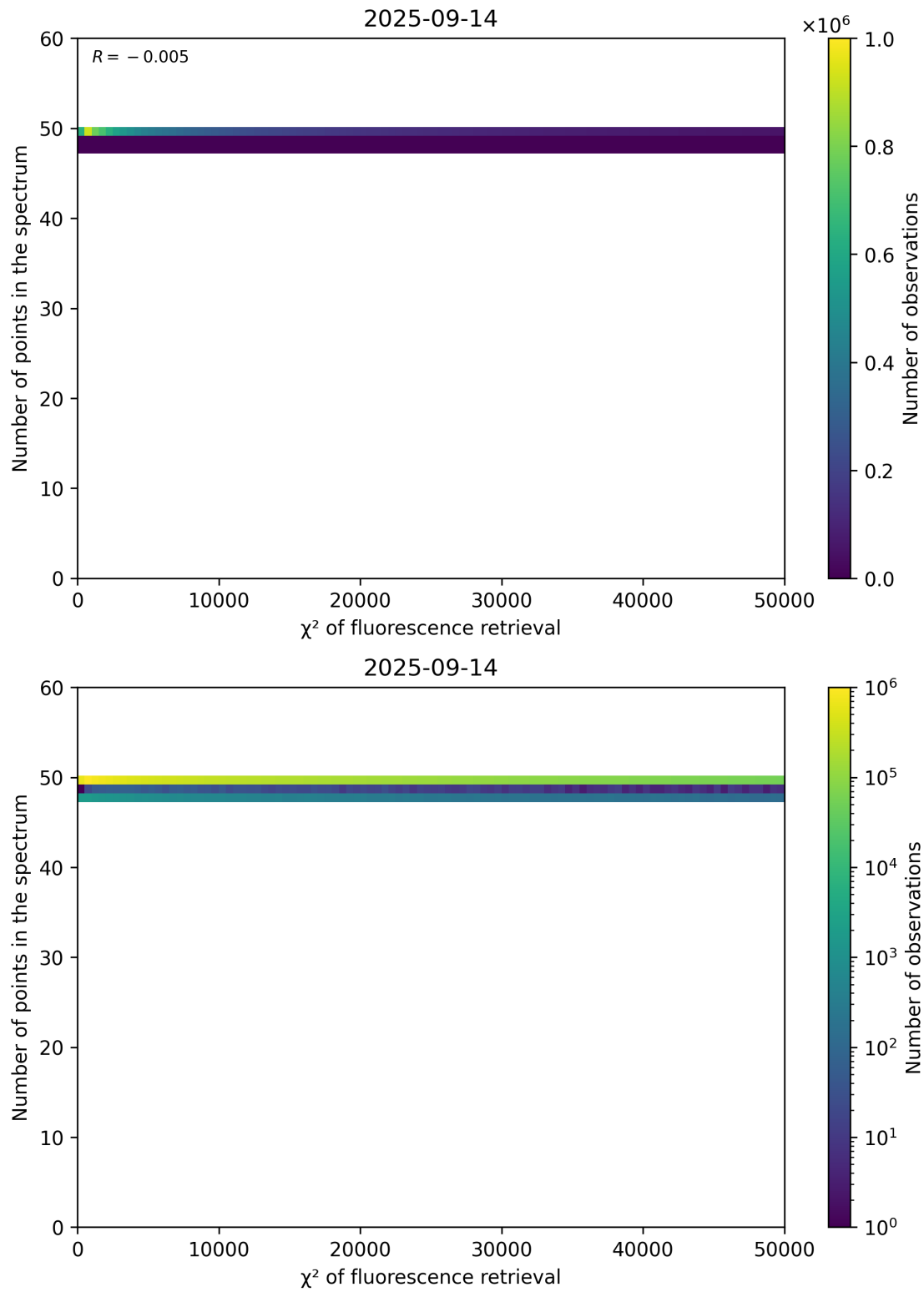
Figure 68: Scatter density plot of “ \chi^2 of fluorescence retrieval” against “Number of points in the spectrum” for 2025-09-13 to 2025-09-15.
