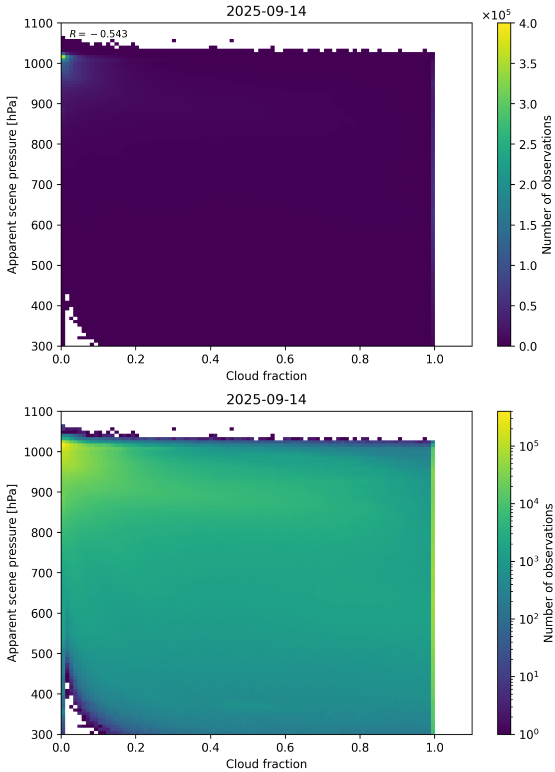
Figure 70: Scatter density plot of “Cloud fraction” against “Apparent scene pressure” for 2025-09-13 to 2025-09-15.
