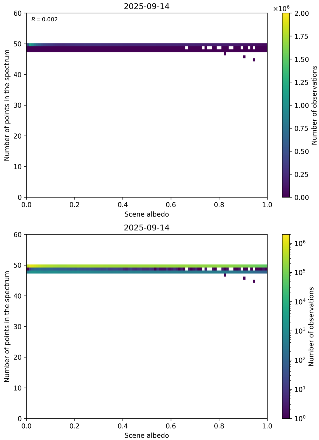
Figure 106: Scatter density plot of “Scene albedo” against “Number of points in the spectrum” for 2025-09-13 to 2025-09-15.
