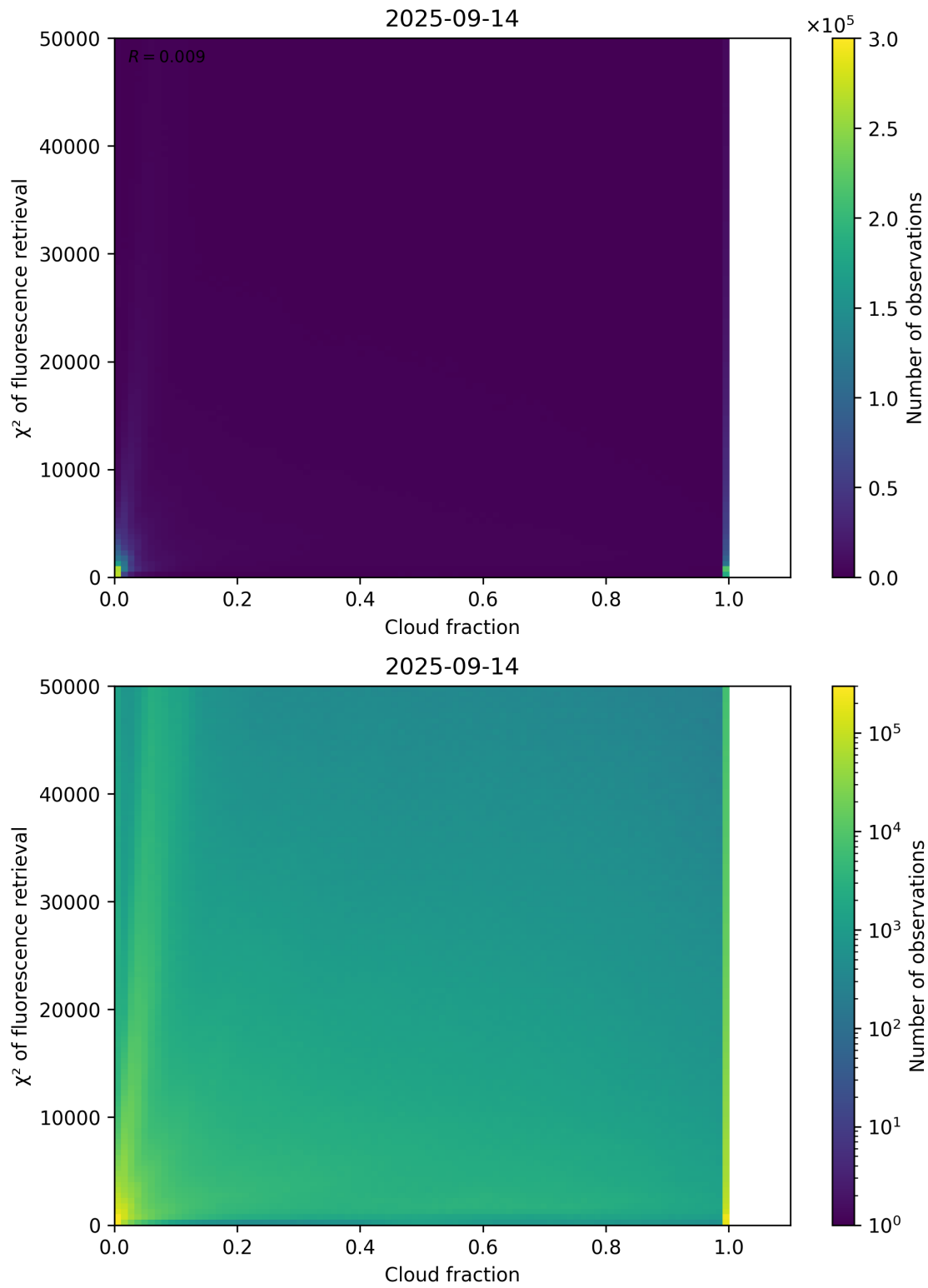
Figure 71: Scatter density plot of “Cloud fraction” against “ \chi^2 of fluorescence retrieval” for 2025-09-13 to 2025-09-15.
