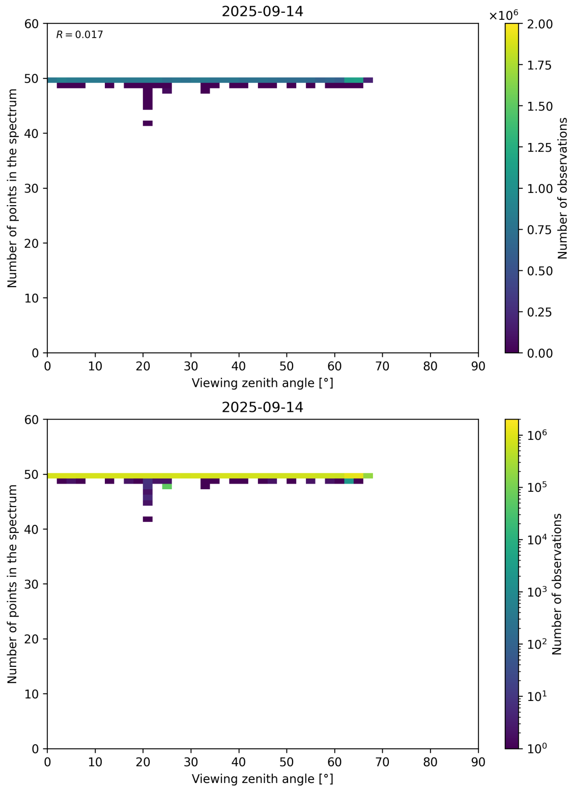
Figure 125: Scatter density plot of “Viewing zenith angle” against “Number of points in the spectrum” for 2025-09-13 to 2025-09-15.
