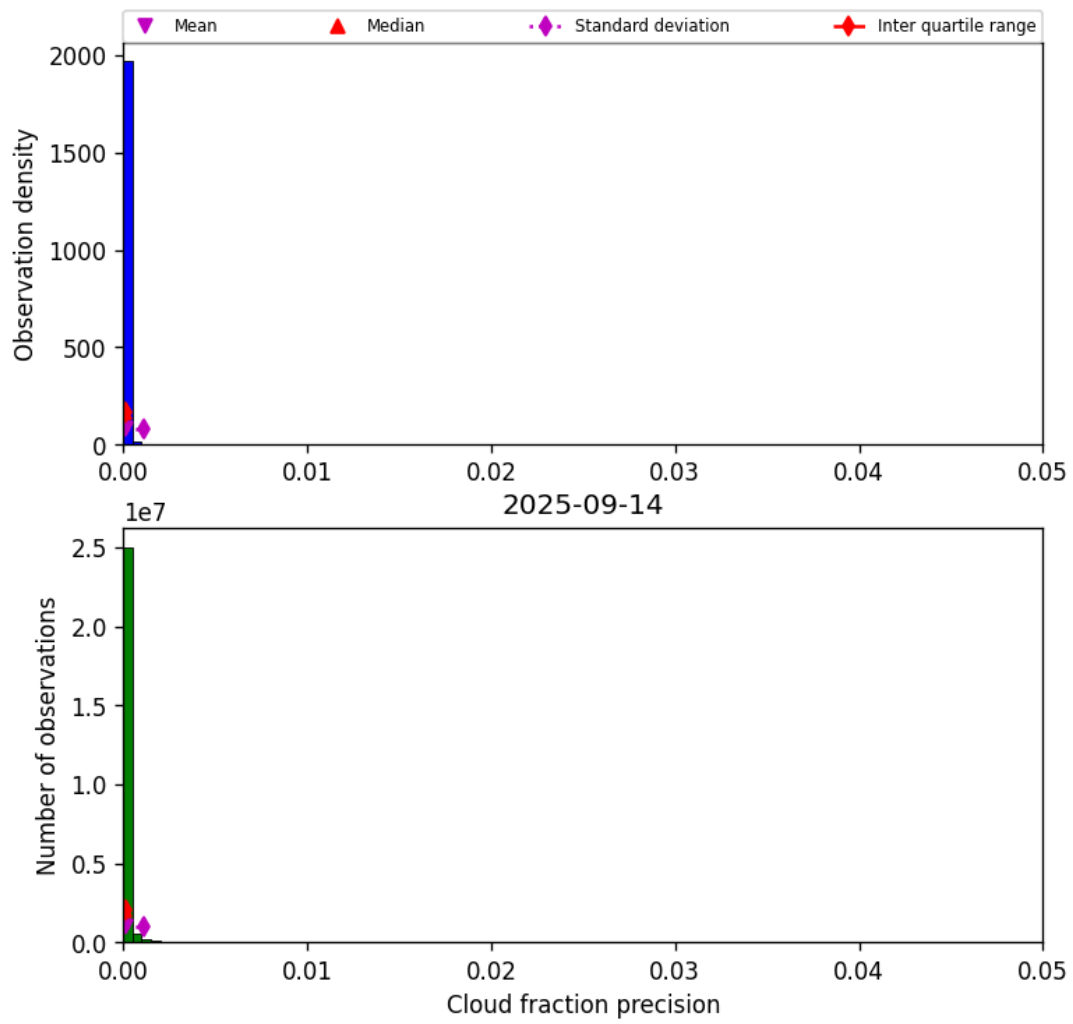
Figure 33: Histogram of “Cloud fraction precision” for 2025-09-13 to 2025-09-15
