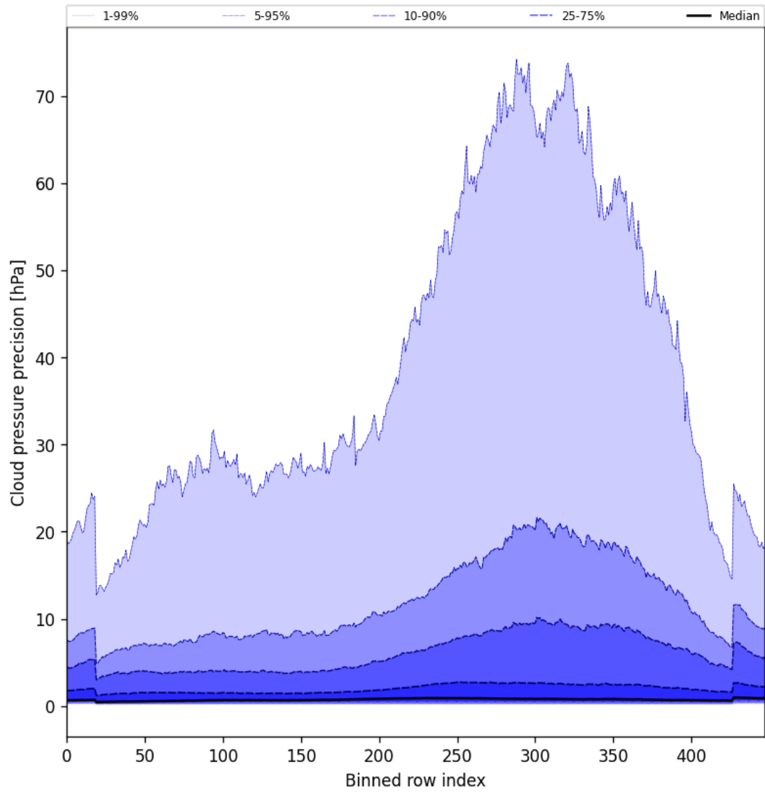
Figure 48: Along track statistics of “Cloud pressure precision” for 2025-09-13 to 2025-09-15
