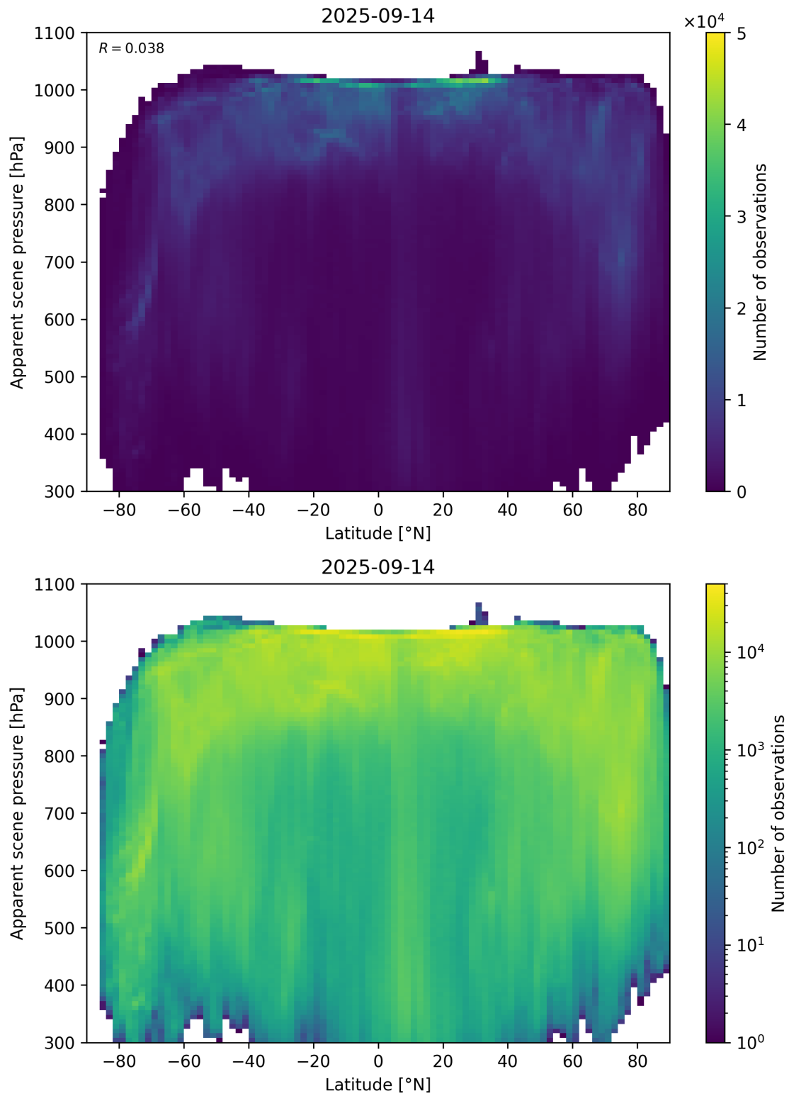
Figure 88: Scatter density plot of “Latitude” against “Apparent scene pressure” for 2025-09-13 to 2025-09-15.
