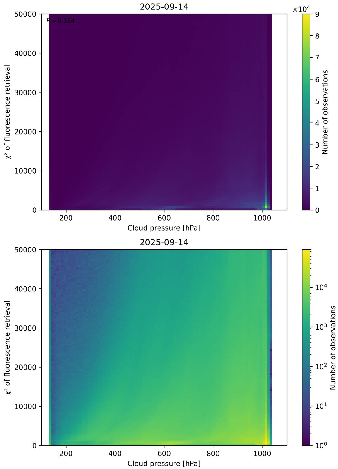
Figure 78: Scatter density plot of “Cloud pressure” against “ \chi^2 of fluorescence retrieval” for 2025-09-13 to 2025-09-15.
