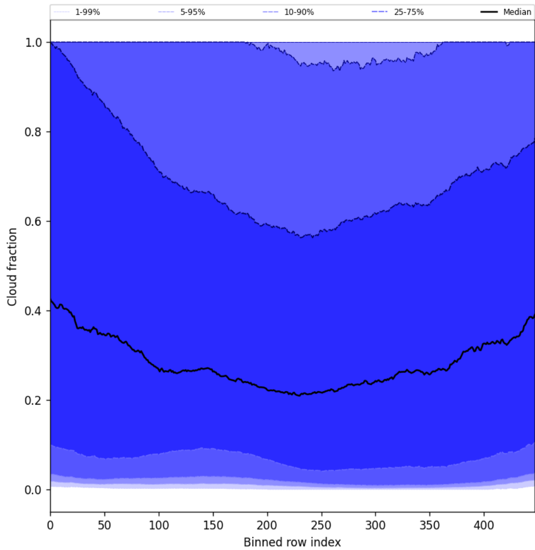
Figure 49: Along track statistics of “Cloud fraction” for 2025-09-13 to 2025-09-15
