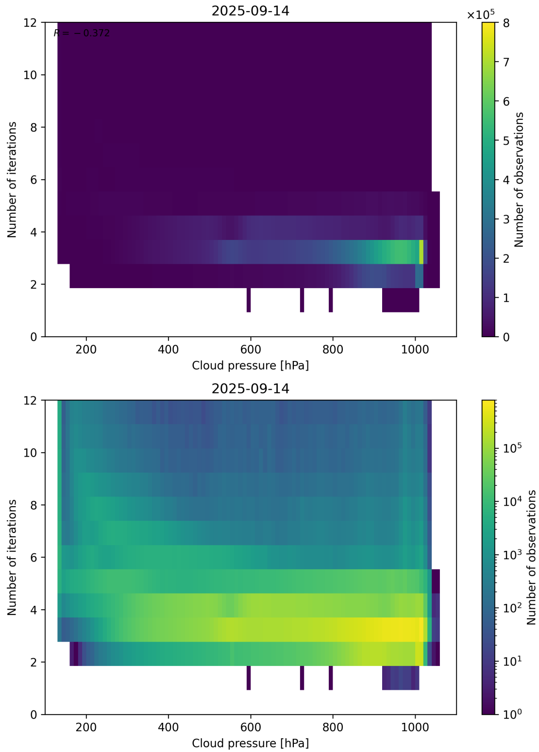
Figure 81: Scatter density plot of “Cloud pressure” against “Number of iterations” for 2025-09-13 to 2025-09-15.
