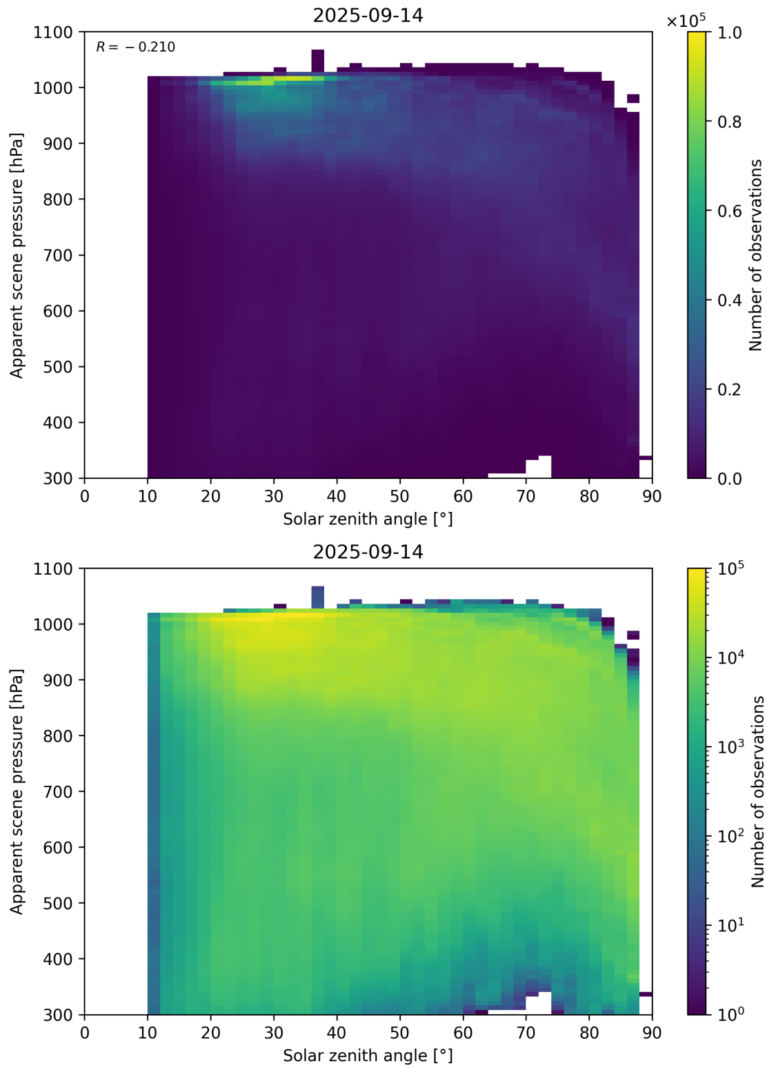
Figure 108: Scatter density plot of “Solar zenith angle” against “Apparent scene pressure” for 2025-09-13 to 2025-09-15.
