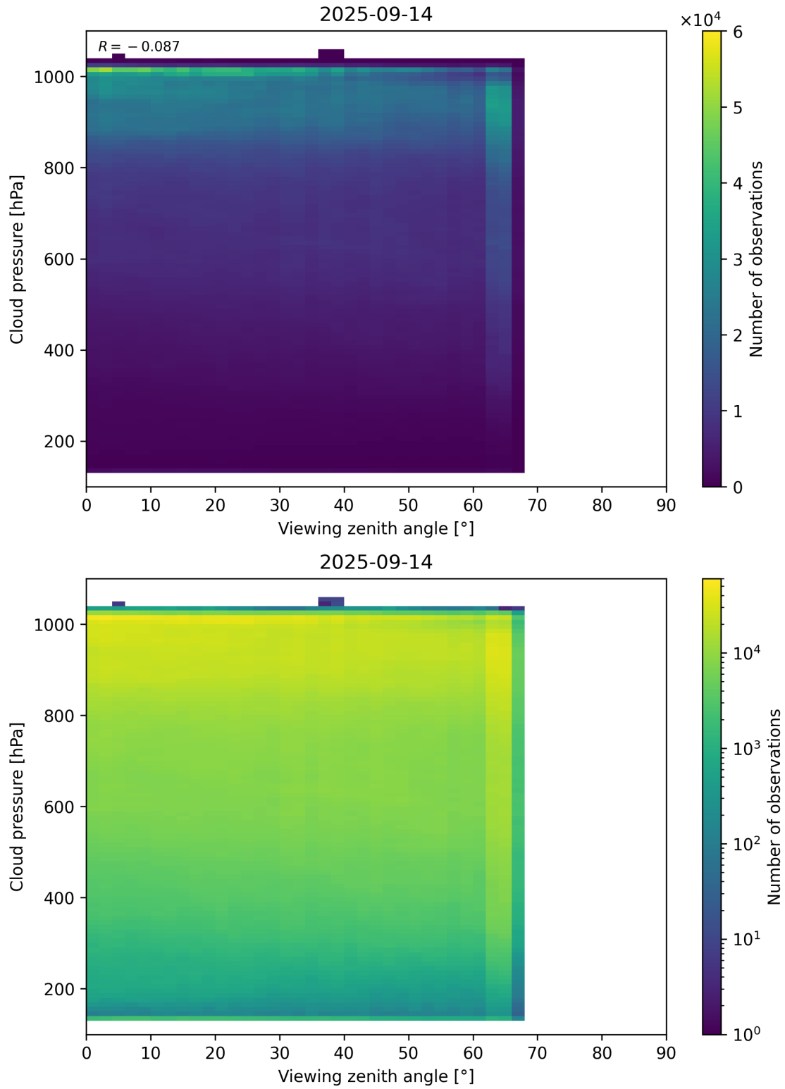
Figure 121: Scatter density plot of “Viewing zenith angle” against “Cloud pressure” for 2025-09-13 to 2025-09-15.
