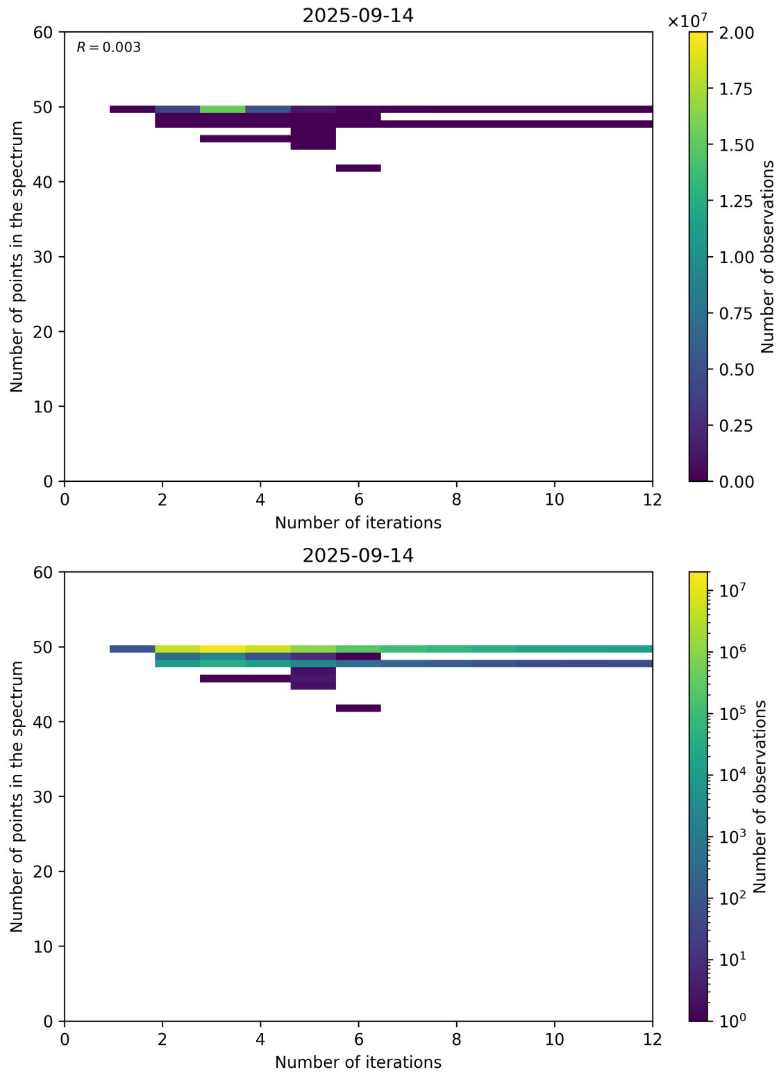
Figure 99: Scatter density plot of “Number of iterations” against “Number of points in the spectrum” for 2025-09-13 to 2025-09-15.
