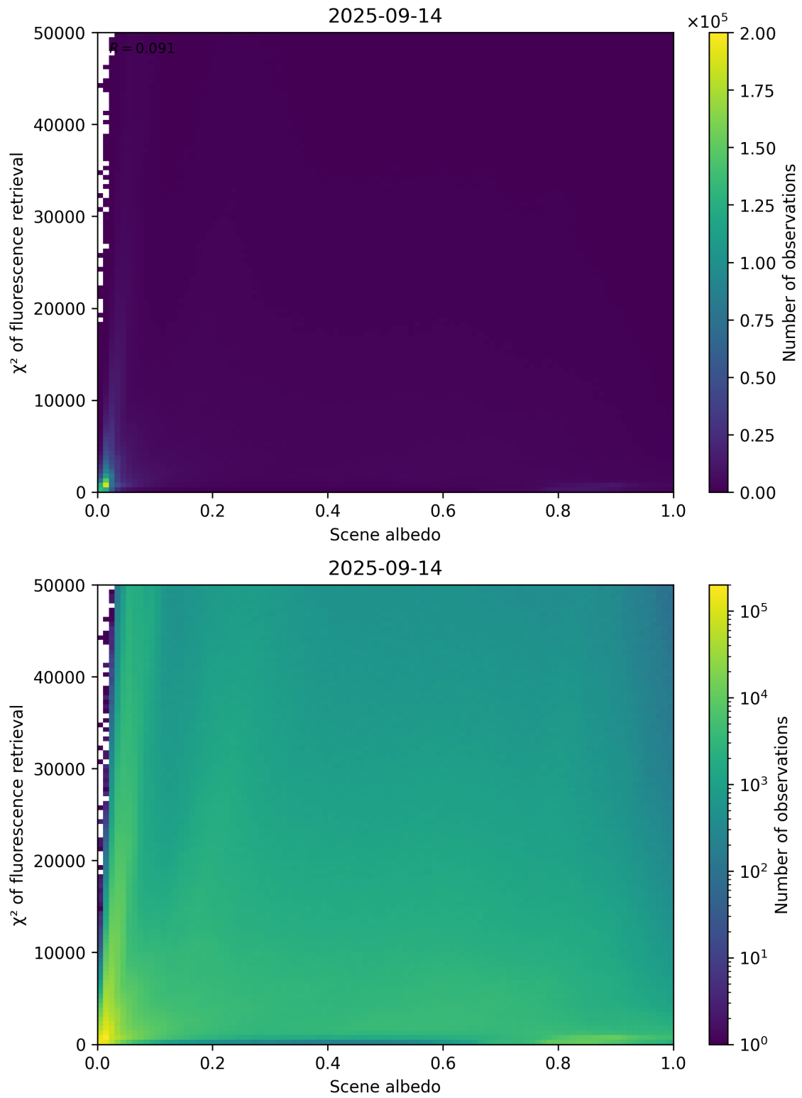
Figure 103: Scatter density plot of “Scene albedo” against “ \chi^2 of fluorescence retrieval” for 2025-09-13 to 2025-09-15.
