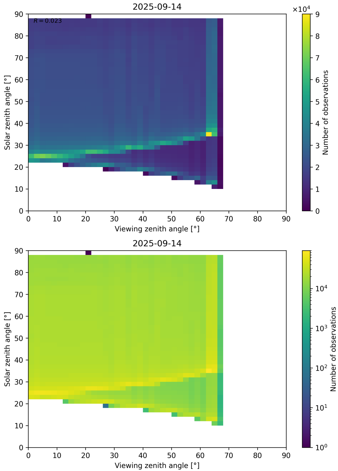
Figure 127: Scatter density plot of “Viewing zenith angle” against “Solar zenith angle” for 2025-09-13 to 2025-09-15.
