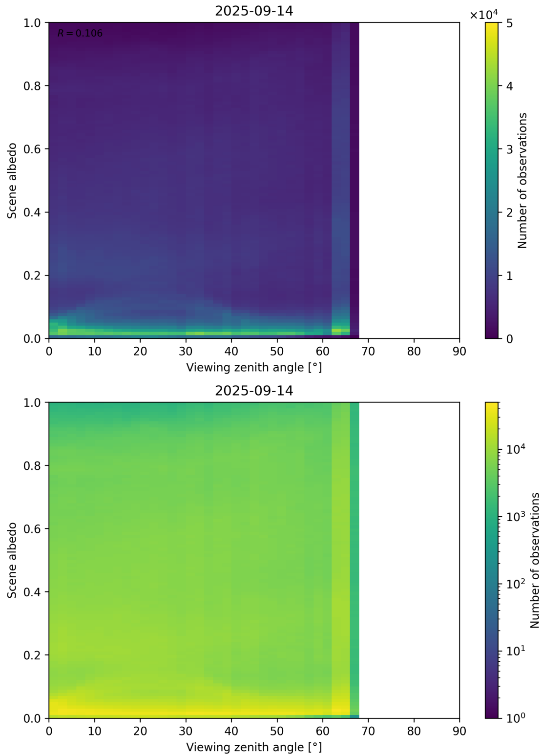
Figure 126: Scatter density plot of “Viewing zenith angle” against “Scene albedo” for 2025-09-13 to 2025-09-15.
