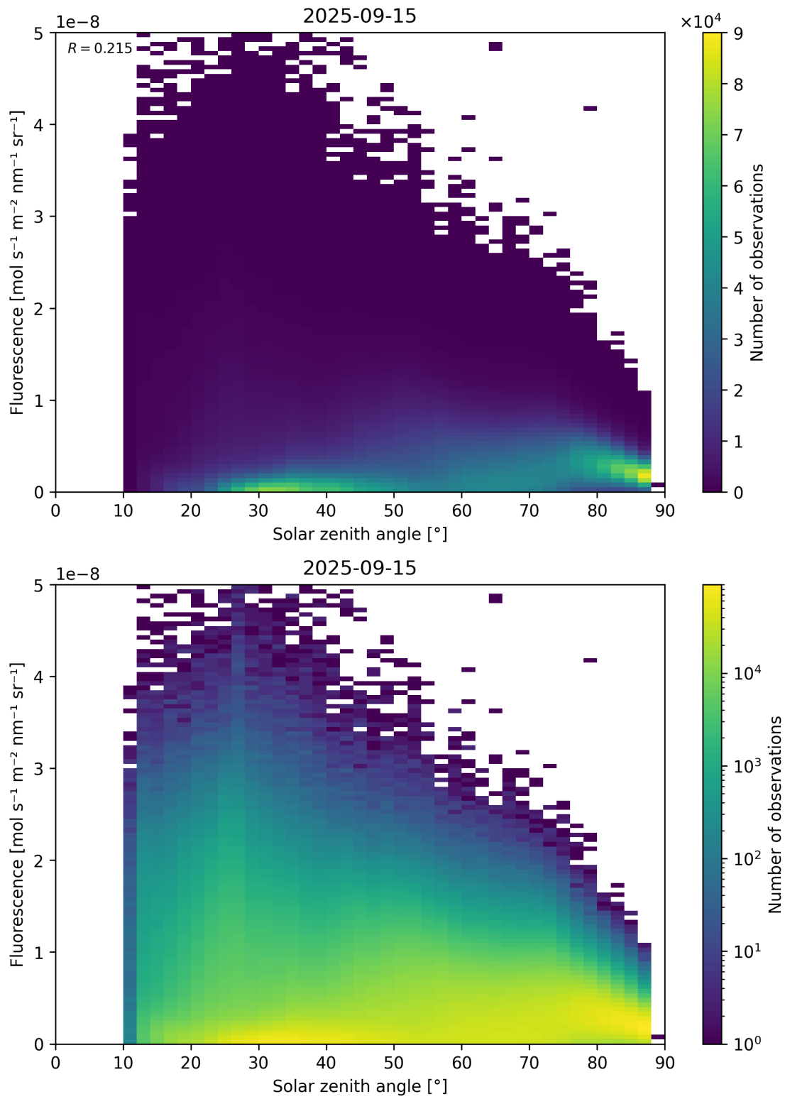
Figure 112: Scatter density plot of “Solar zenith angle” against “Fluorescence” for 2025-09-15 to 2025-09-16.
