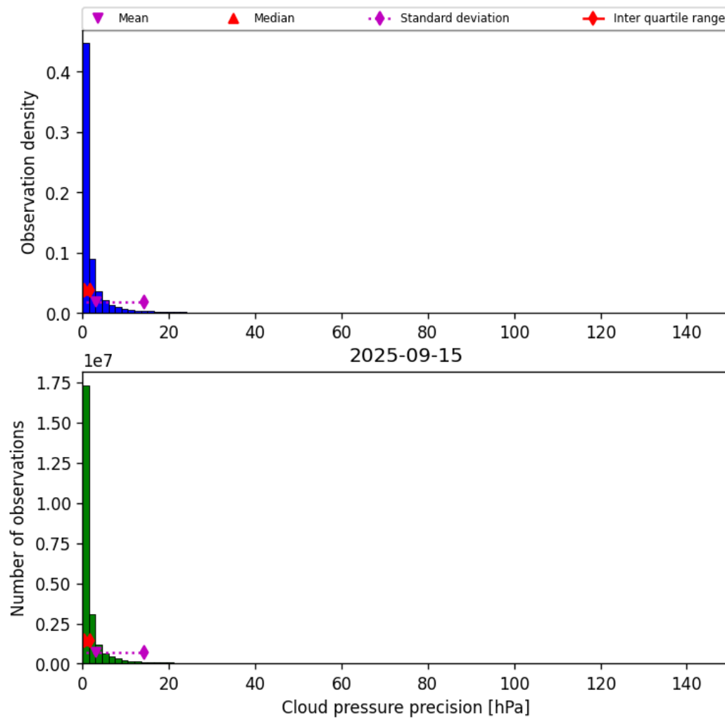
Figure 31: Histogram of “Cloud pressure precision” for 2025-09-15 to 2025-09-16
