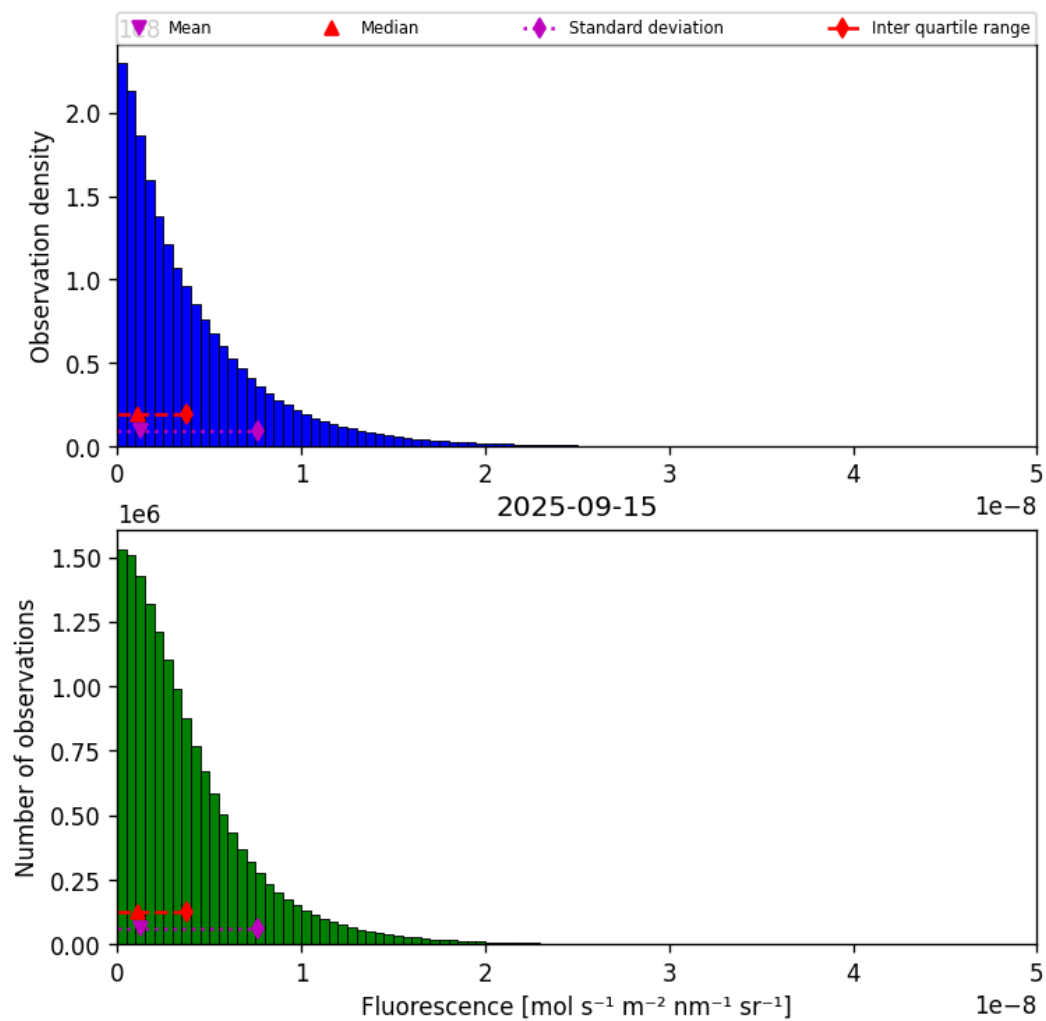
Figure 40: Histogram of “Fluorescence” for 2025-09-15 to 2025-09-16
