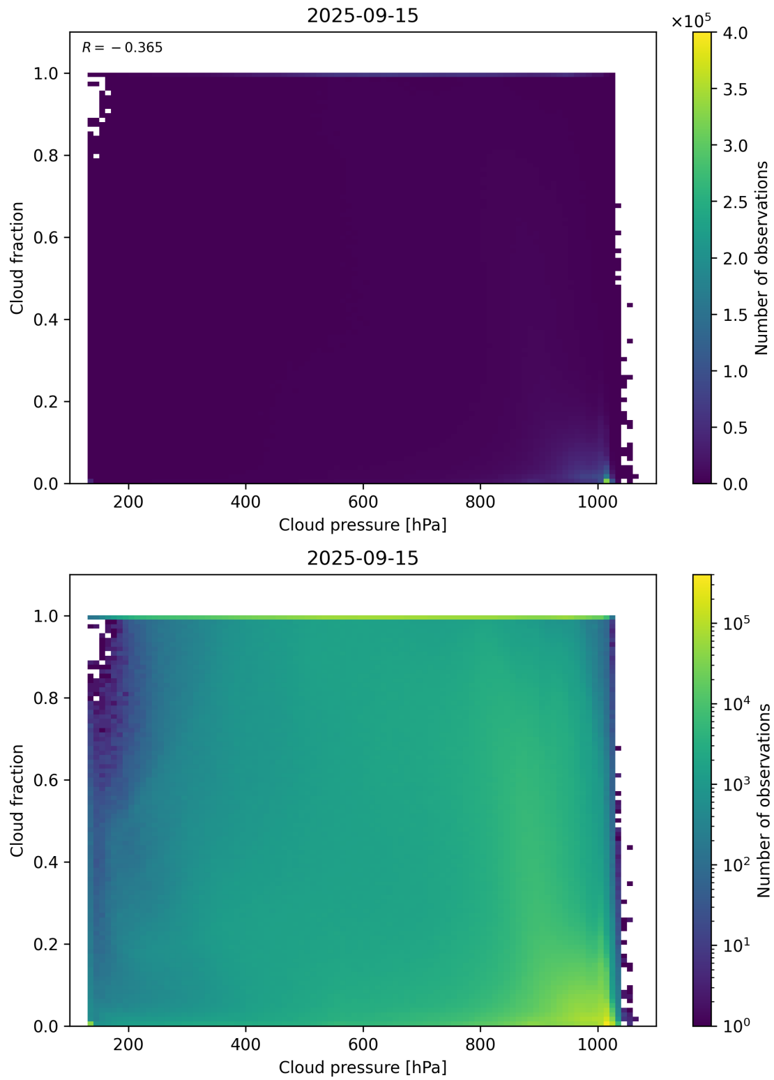
Figure 79: Scatter density plot of “Cloud pressure” against “Cloud fraction” for 2025-09-15 to 2025-09-16.
