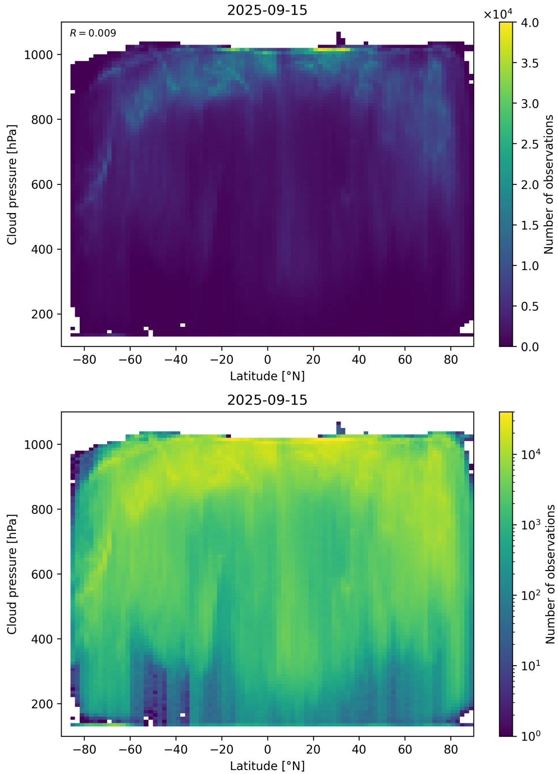
Figure 91: Scatter density plot of “Latitude” against “Cloud pressure” for 2025-09-15 to 2025-09-16.
