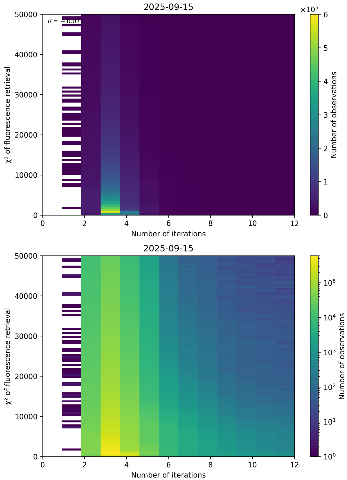
Figure 97: Scatter density plot of “Number of iterations” against “ \chi^2 of fluorescence retrieval” for 2025-09-15 to 2025-09-16.
