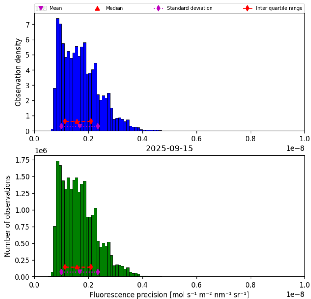
Figure 41: Histogram of “Fluorescence precision” for 2025-09-15 to 2025-09-16
