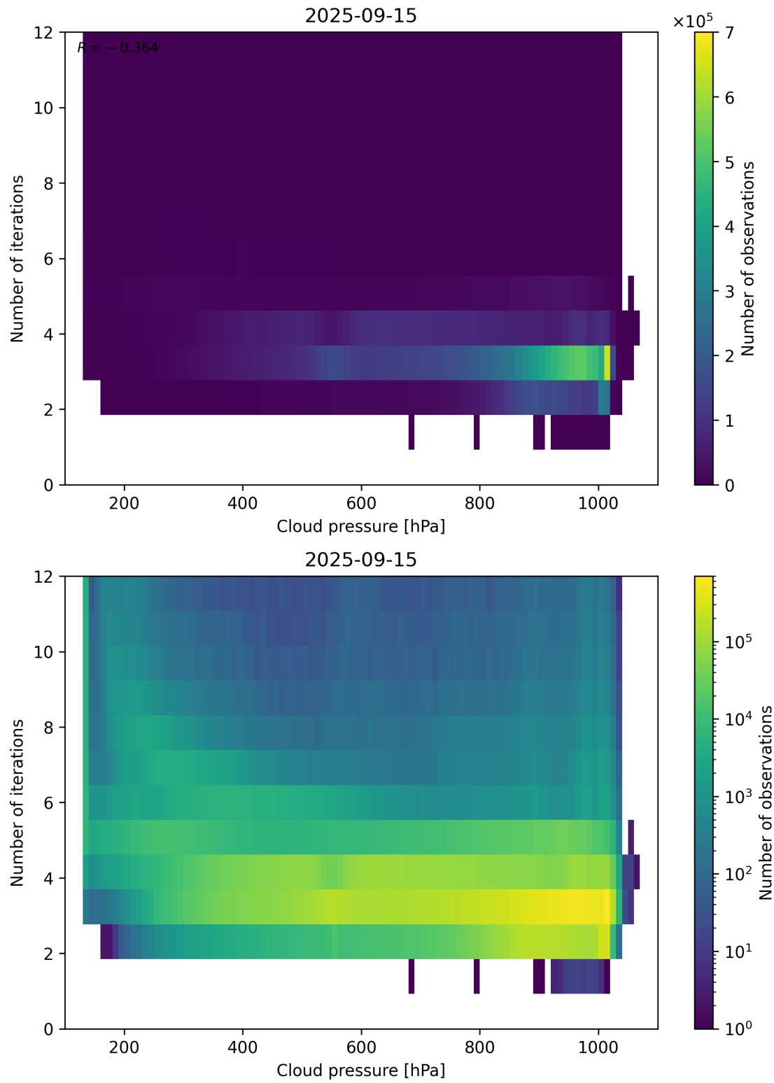
Figure 81: Scatter density plot of “Cloud pressure” against “Number of iterations” for 2025-09-15 to 2025-09-16.
