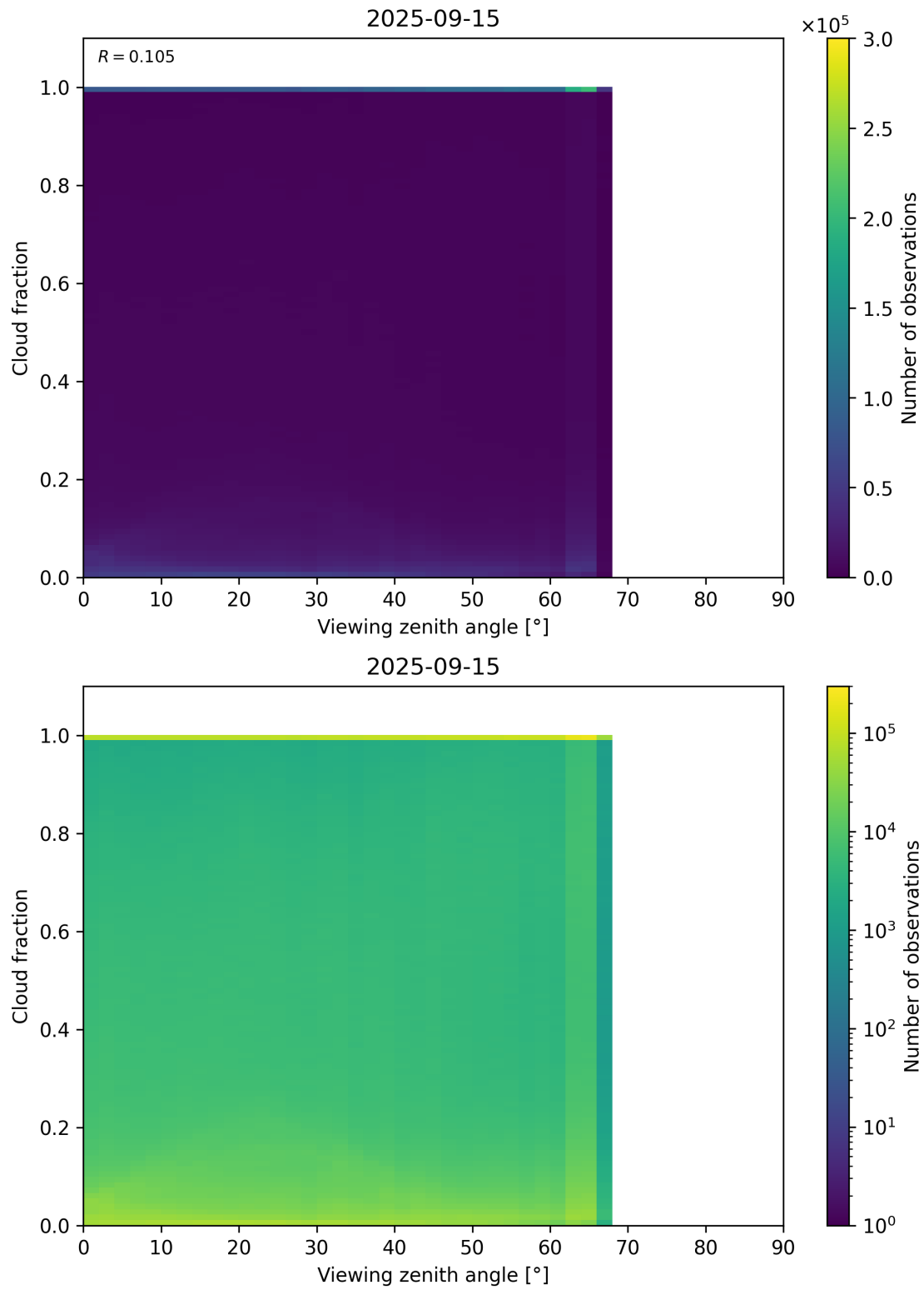
Figure 120: Scatter density plot of “Viewing zenith angle” against “Cloud fraction” for 2025-09-15 to 2025-09-16.
