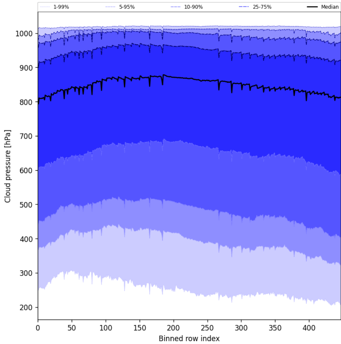
Figure 47: Along track statistics of “Cloud pressure” for 2025-09-15 to 2025-09-16
