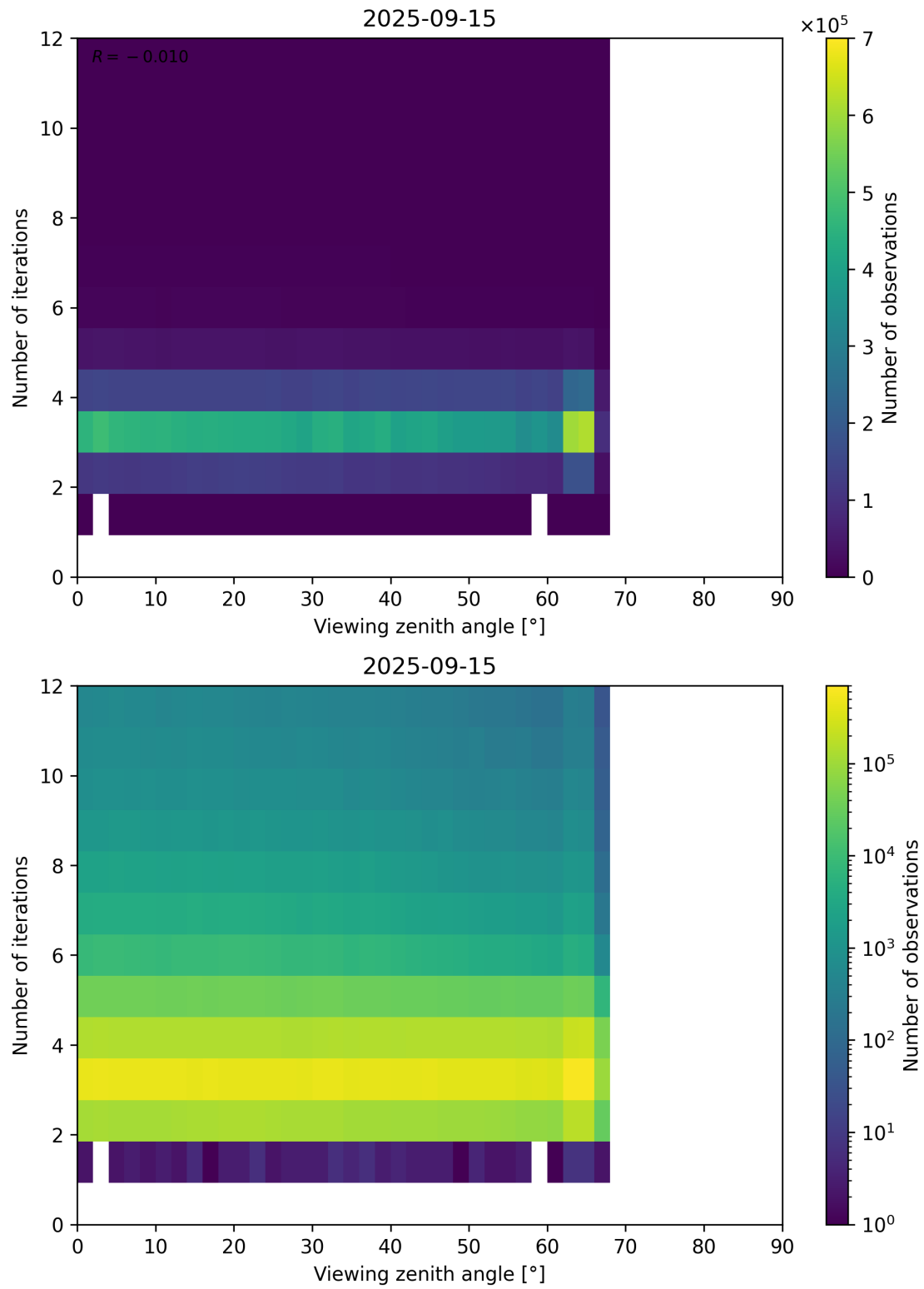
Figure 124: Scatter density plot of “Viewing zenith angle” against “Number of iterations” for 2025-09-15 to 2025-09-16.
