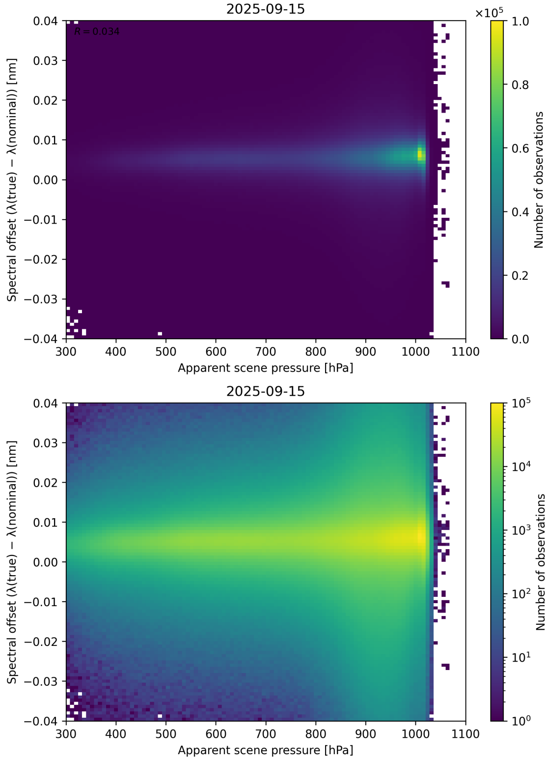
Figure 67: Scatter density plot of “Apparent scene pressure” against “Spectral offset ( \lambda_{\text{true}} - \lambda_{\text{nominal}} )” for 2025-09-15 to 2025-09-16.
