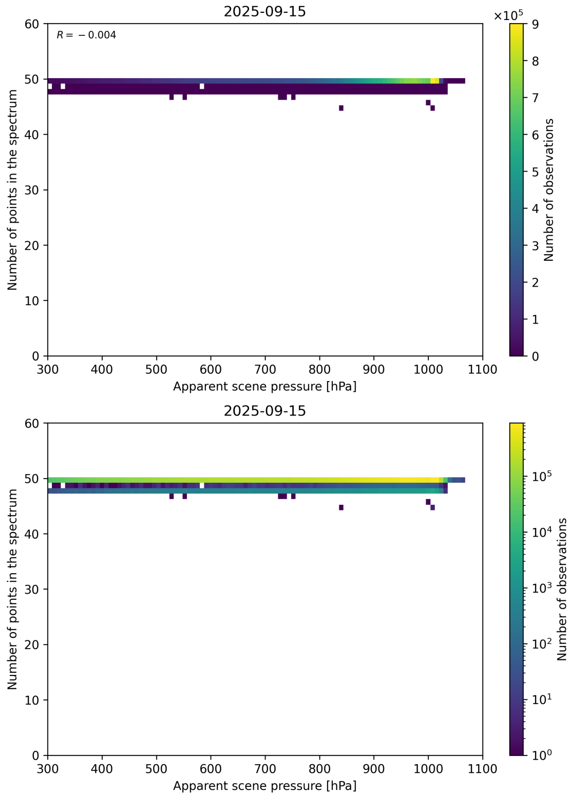
Figure 66: Scatter density plot of “Apparent scene pressure” against “Number of points in the spectrum” for 2025-09-15 to 2025-09-16.
