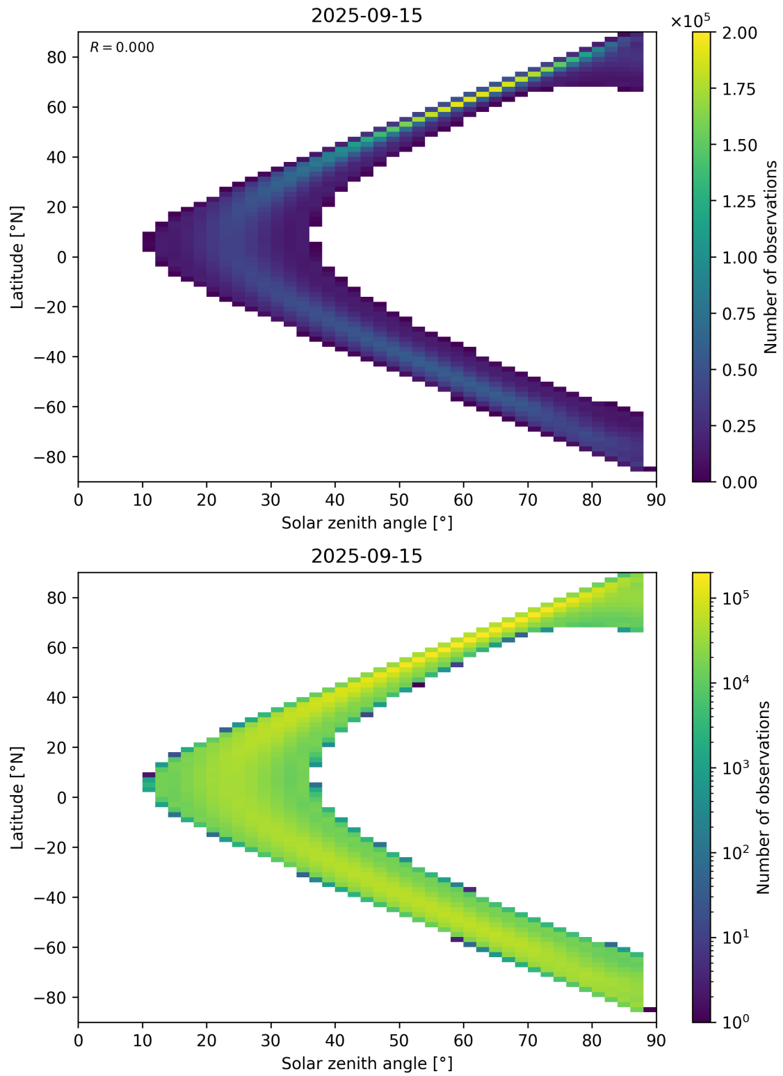
Figure 113: Scatter density plot of “Solar zenith angle” against “Latitude” for 2025-09-15 to 2025-09-16.
