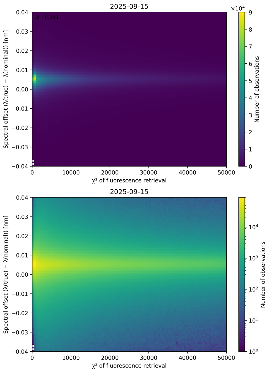
Figure 69: Scatter density plot of “ \chi^2 of fluorescence retrieval” against “Spectral offset ( \lambda_{\text{true}} - \lambda_{\text{nominal}} )” for 2025-09-15 to 2025-09-16.
