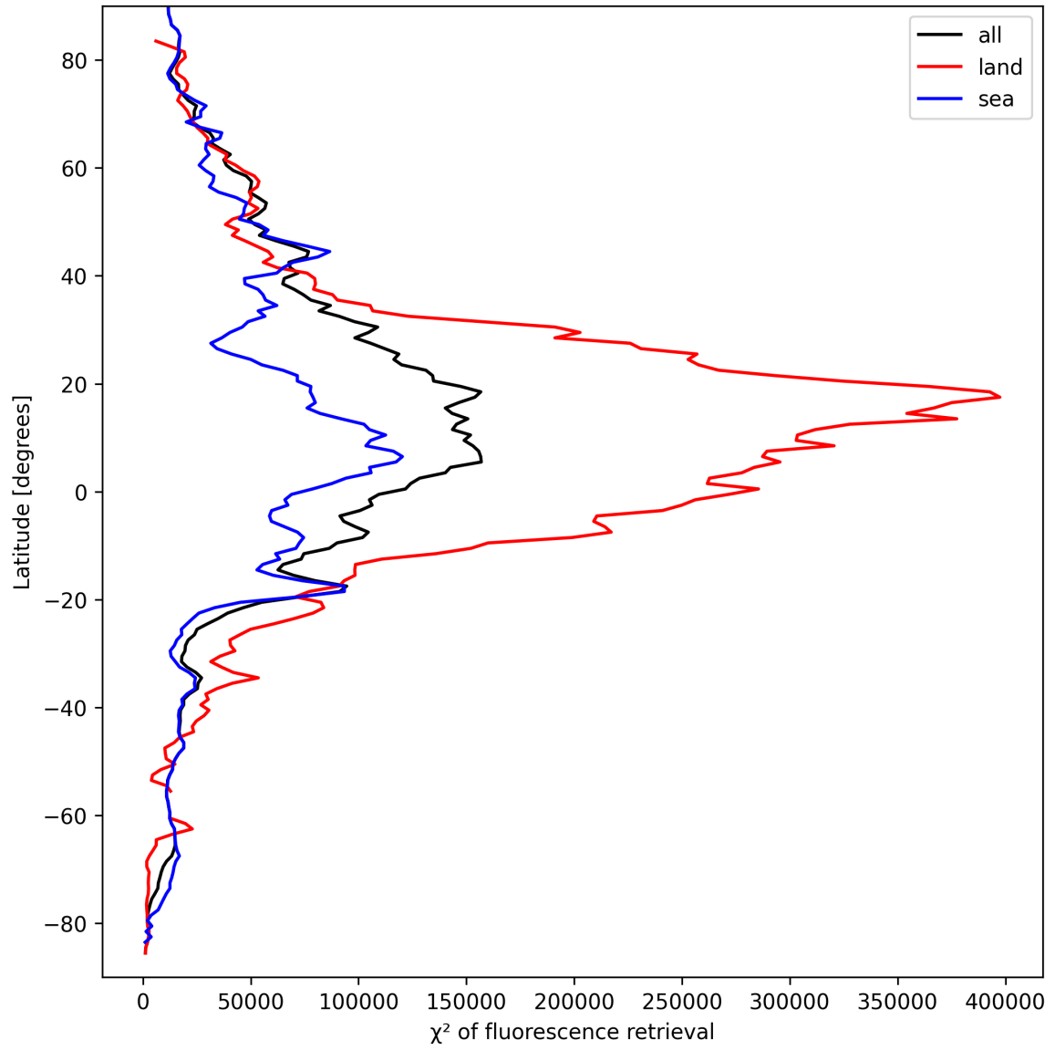
Figure 25: Zonal average of “ \chi^2 of fluorescence retrieval” for 2025-09-15 to 2025-09-16.
