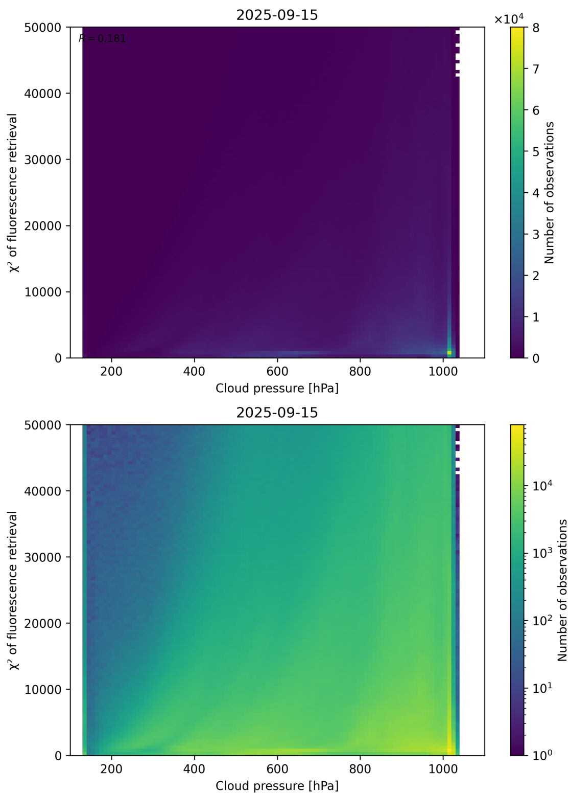
Figure 78: Scatter density plot of “Cloud pressure” against “ \chi^2 of fluorescence retrieval” for 2025-09-15 to 2025-09-16.
