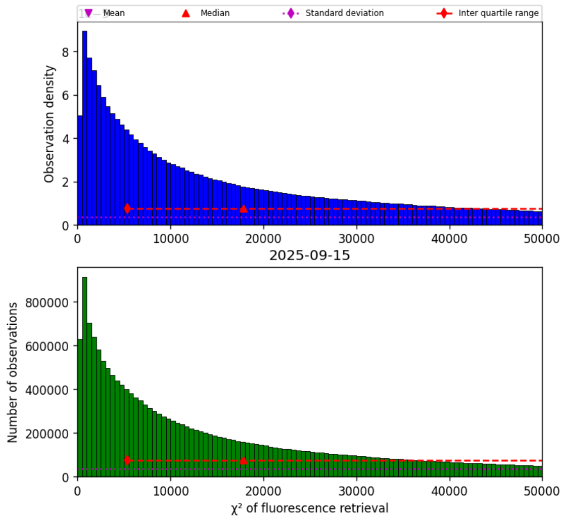
Figure 42: Histogram of “ \chi^2 of fluorescence retrieval” for 2025-09-15 to 2025-09-16
