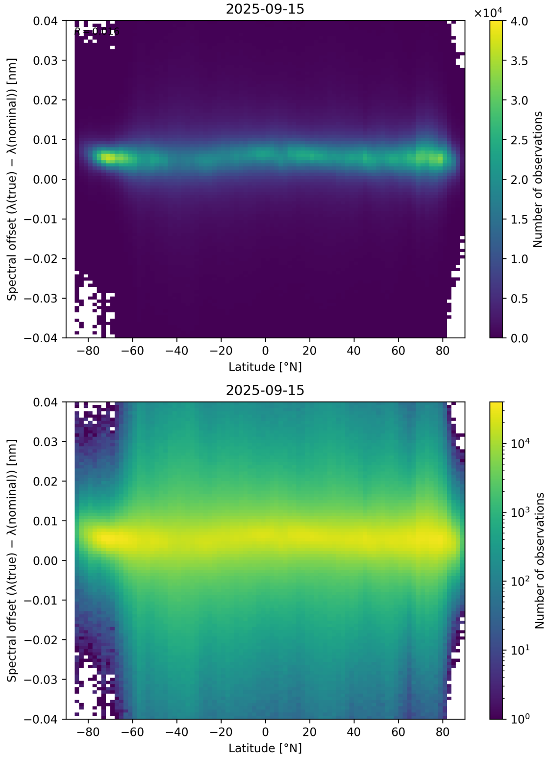
Figure 96: Scatter density plot of “Latitude” against “Spectral offset ( \lambda_{\text{true}} - \lambda_{\text{nominal}} )” for 2025-09-15 to 2025-09-16.
