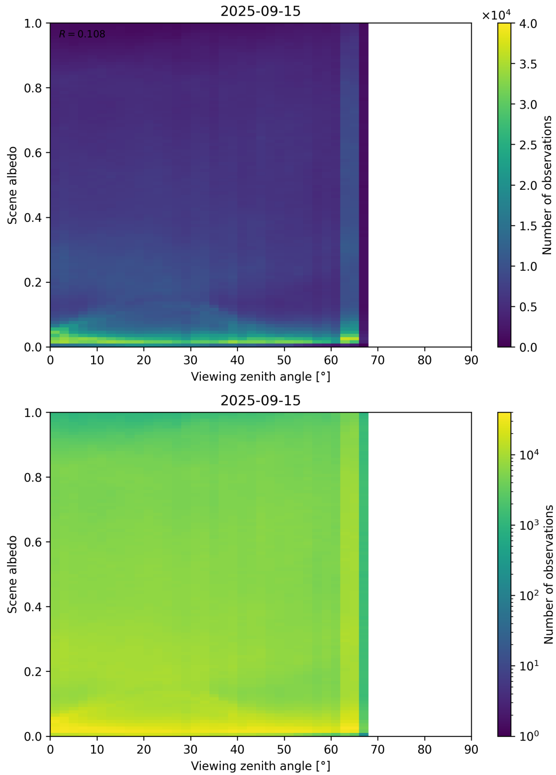
Figure 126: Scatter density plot of “Viewing zenith angle” against “Scene albedo” for 2025-09-15 to 2025-09-16.
