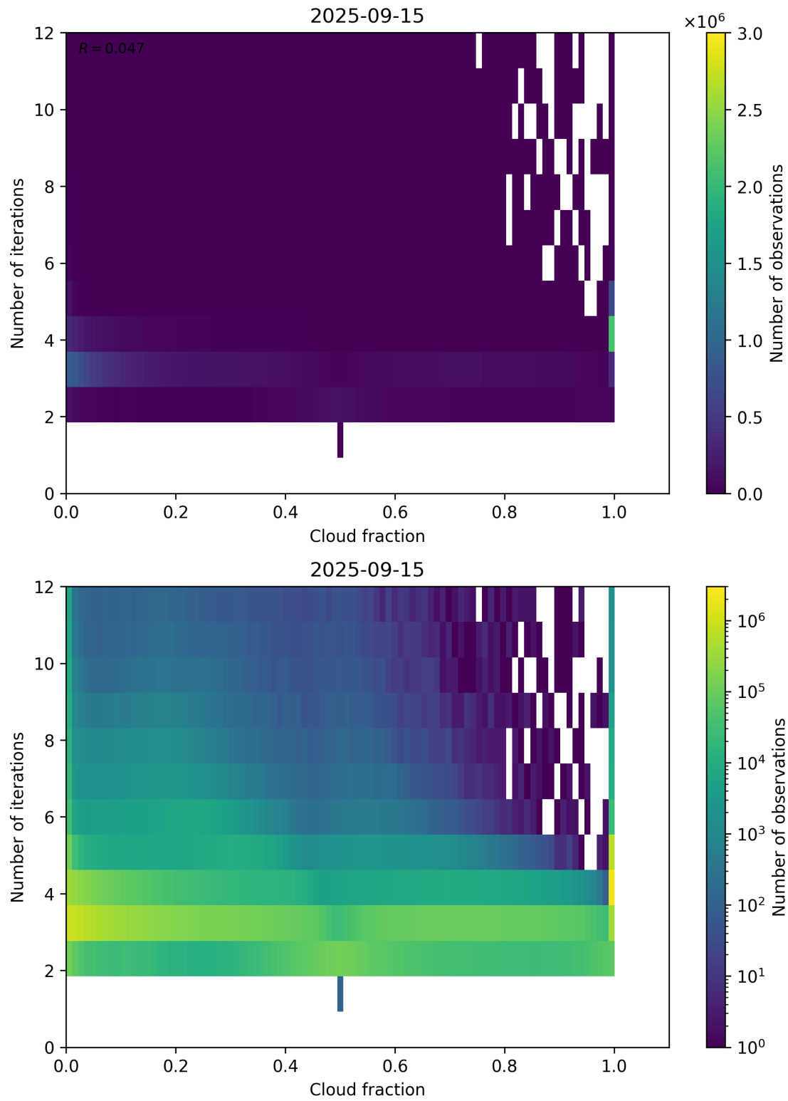
Figure 73: Scatter density plot of “Cloud fraction” against “Number of iterations” for 2025-09-15 to 2025-09-16.
