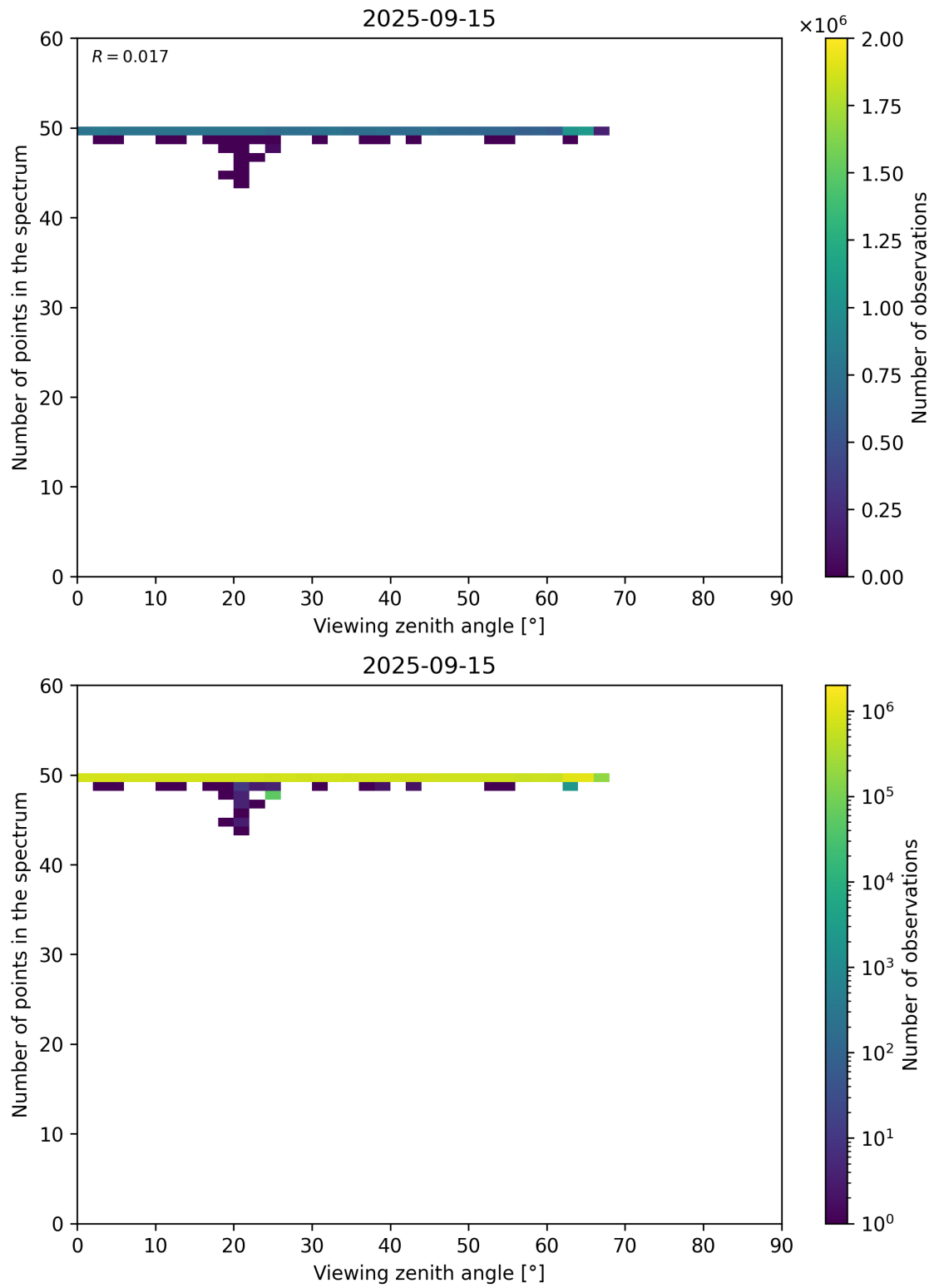
Figure 125: Scatter density plot of “Viewing zenith angle” against “Number of points in the spectrum” for 2025-09-15 to 2025-09-16.
