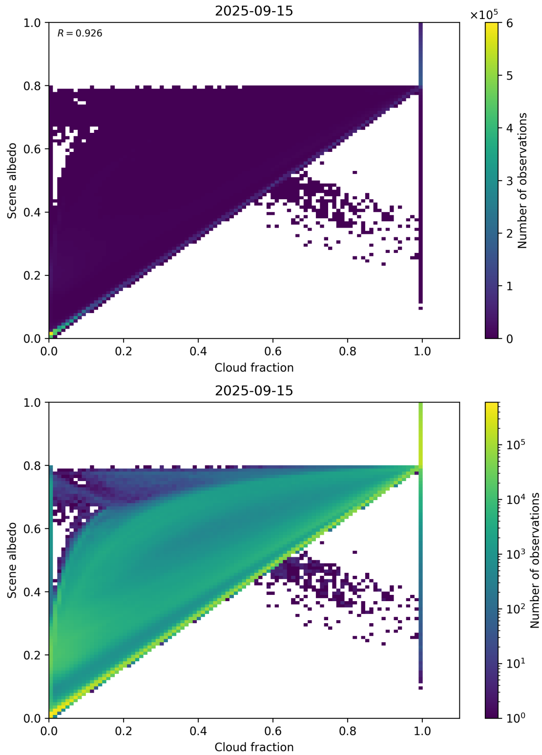
Figure 75: Scatter density plot of “Cloud fraction” against “Scene albedo” for 2025-09-15 to 2025-09-16.
