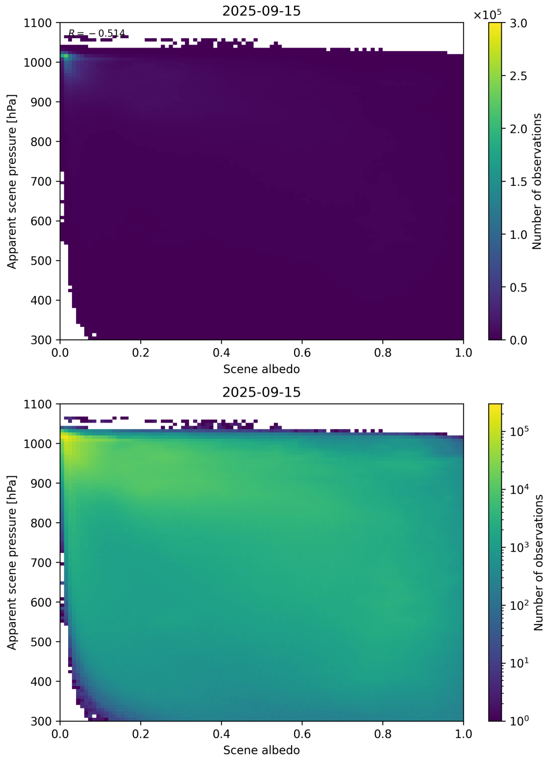
Figure 102: Scatter density plot of “Scene albedo” against “Apparent scene pressure” for 2025-09-15 to 2025-09-16.
