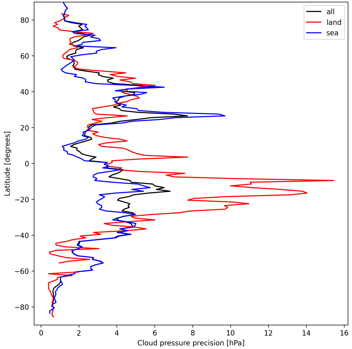
Figure 14: Zonal average of “Cloud pressure precision” for 2025-09-15 to 2025-09-16.
