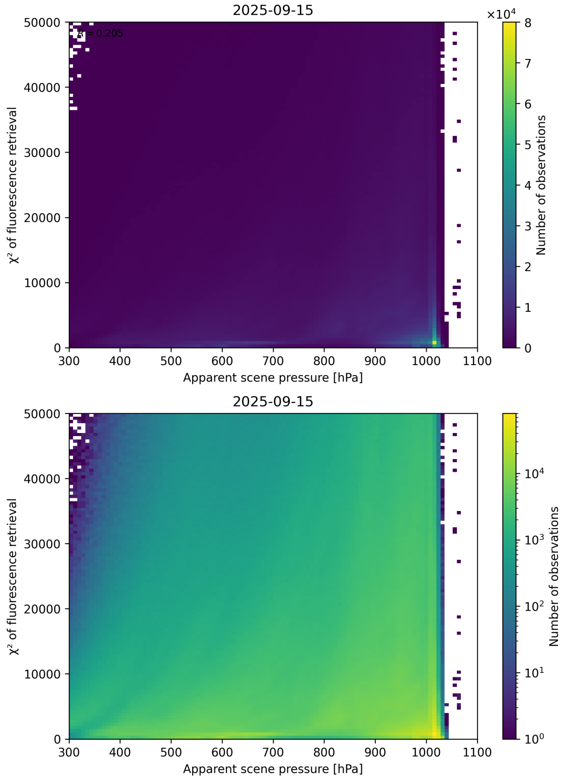
Figure 63: Scatter density plot of “Apparent scene pressure” against “ \chi^2 of fluorescence retrieval” for 2025-09-15 to 2025-09-16.
