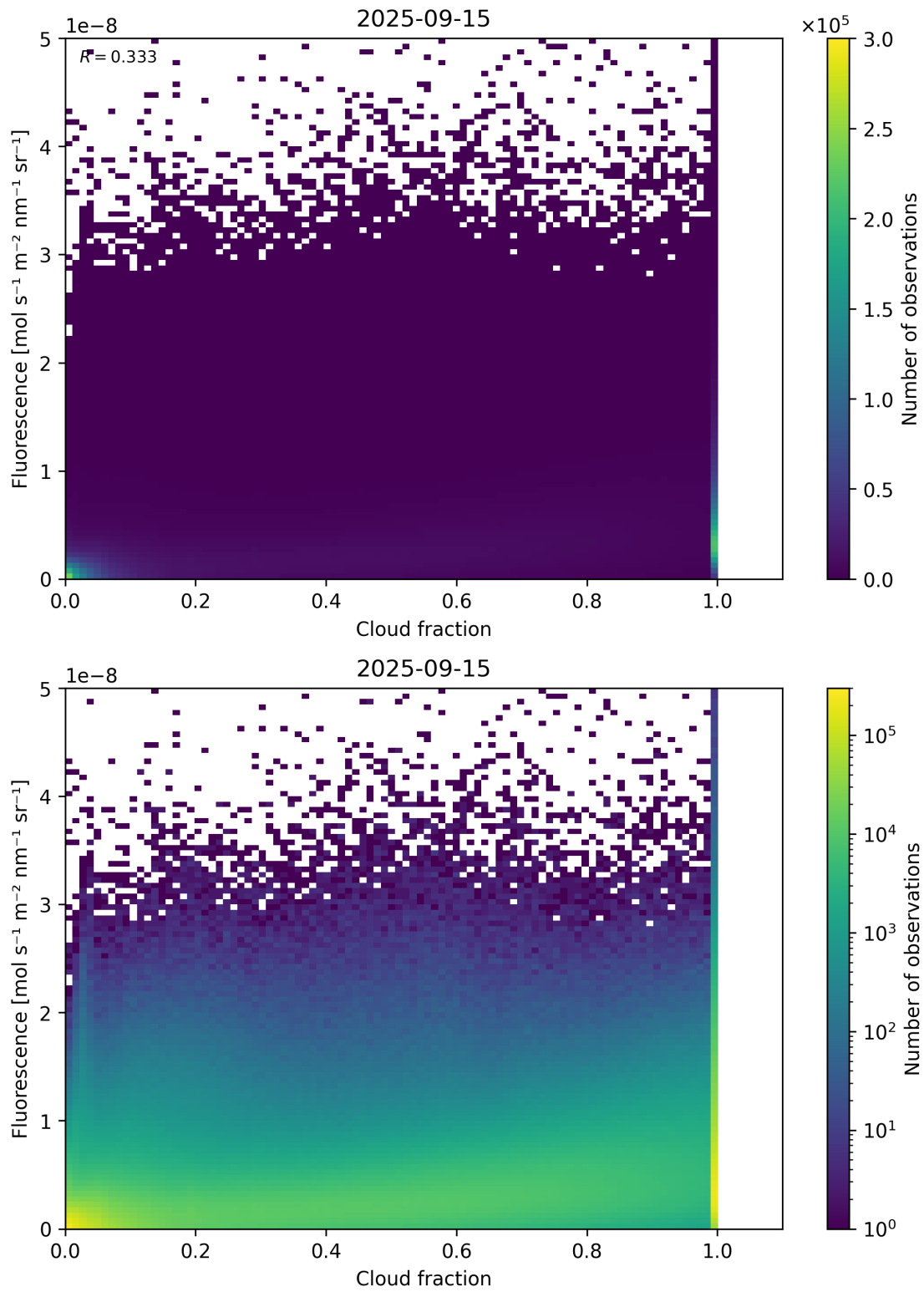
Figure 72: Scatter density plot of “Cloud fraction” against “Fluorescence” for 2025-09-15 to 2025-09-16.
