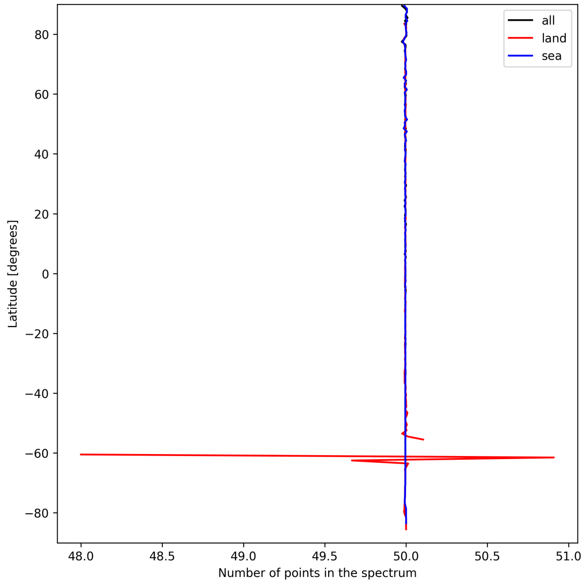
Figure 27: Zonal average of “Number of points in the spectrum” for 2025-09-15 to 2025-09-16.
