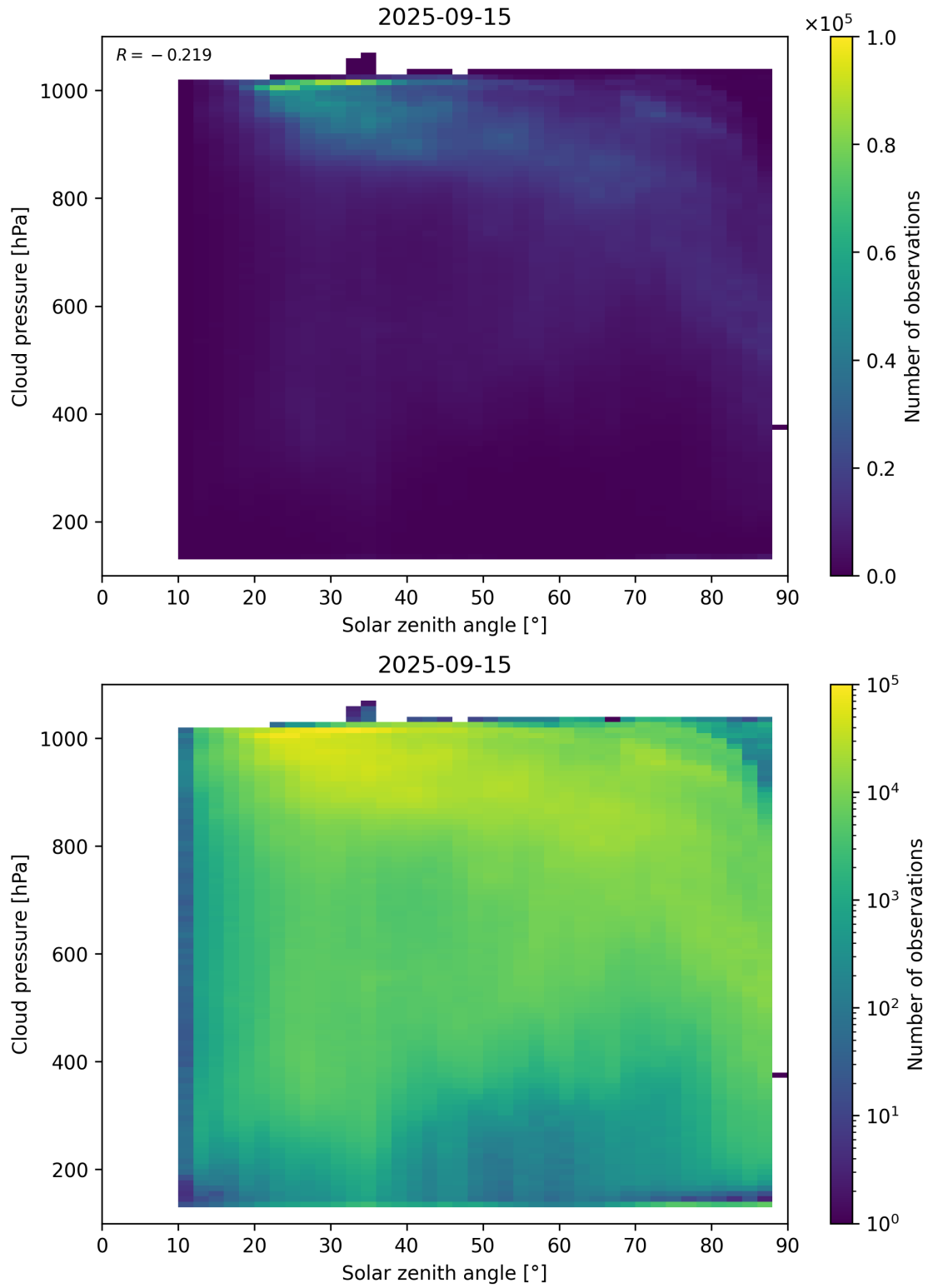
Figure 111: Scatter density plot of “Solar zenith angle” against “Cloud pressure” for 2025-09-15 to 2025-09-16.
