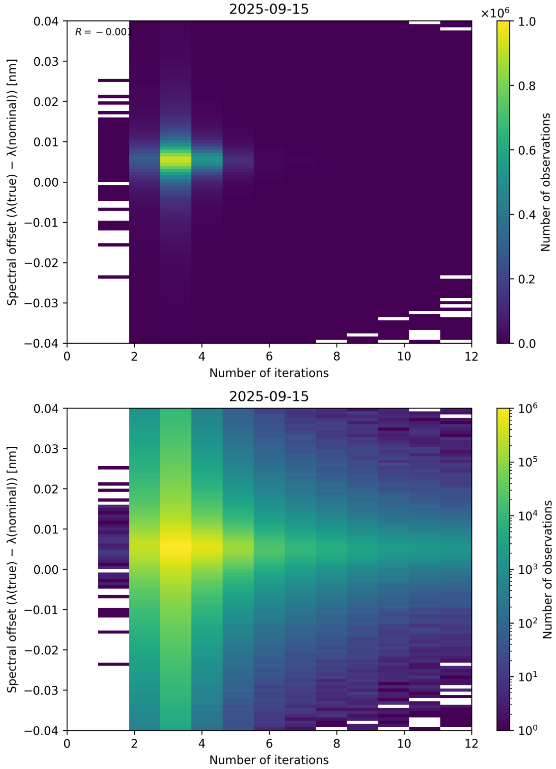
Figure 100: Scatter density plot of “Number of iterations” against “Spectral offset ( \lambda_{\text{true}} - \lambda_{\text{nominal}} )” for 2025-09-15 to 2025-09-16.
