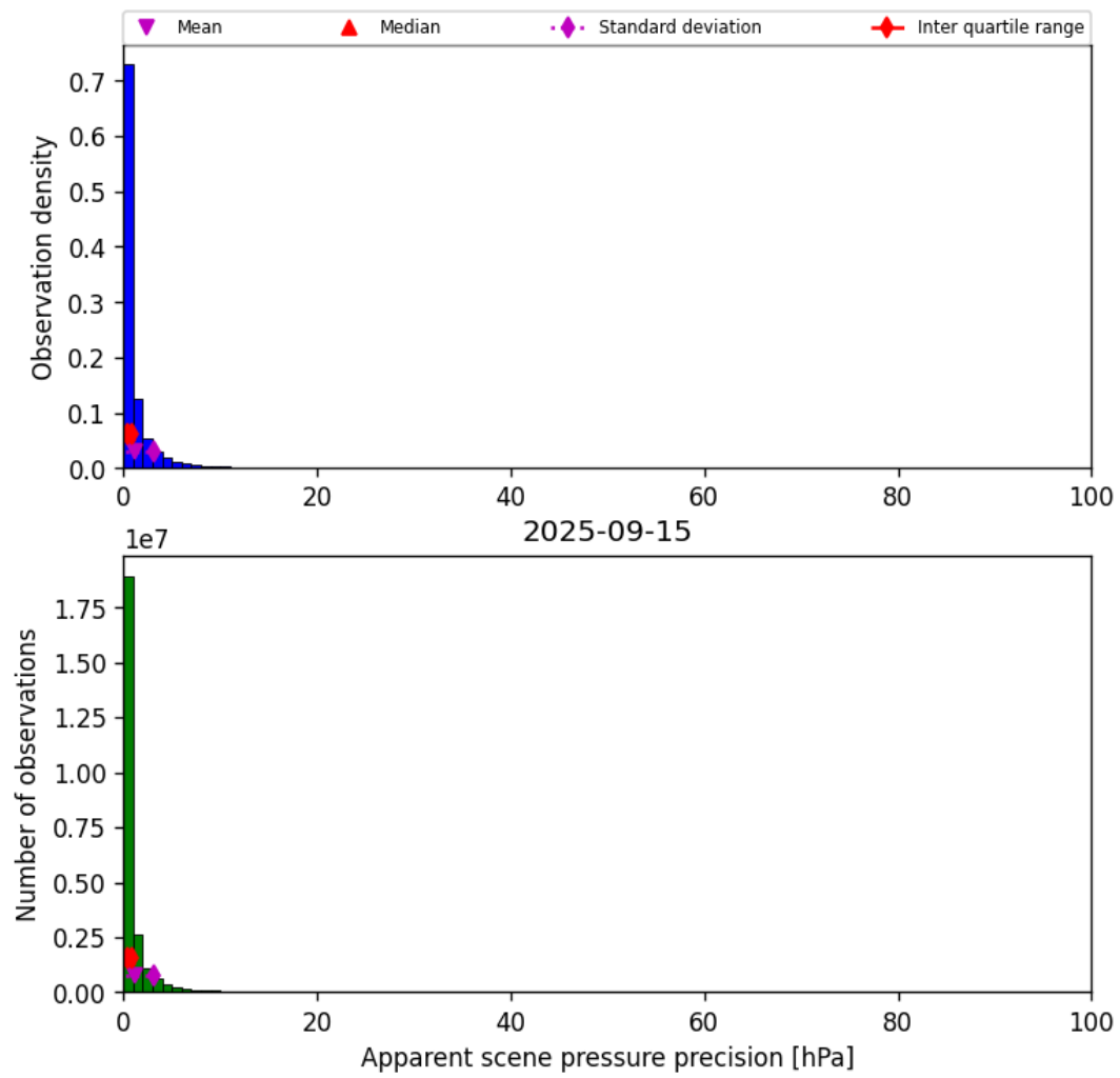
Figure 37: Histogram of “Apparent scene pressure precision” for 2025-09-15 to 2025-09-16
