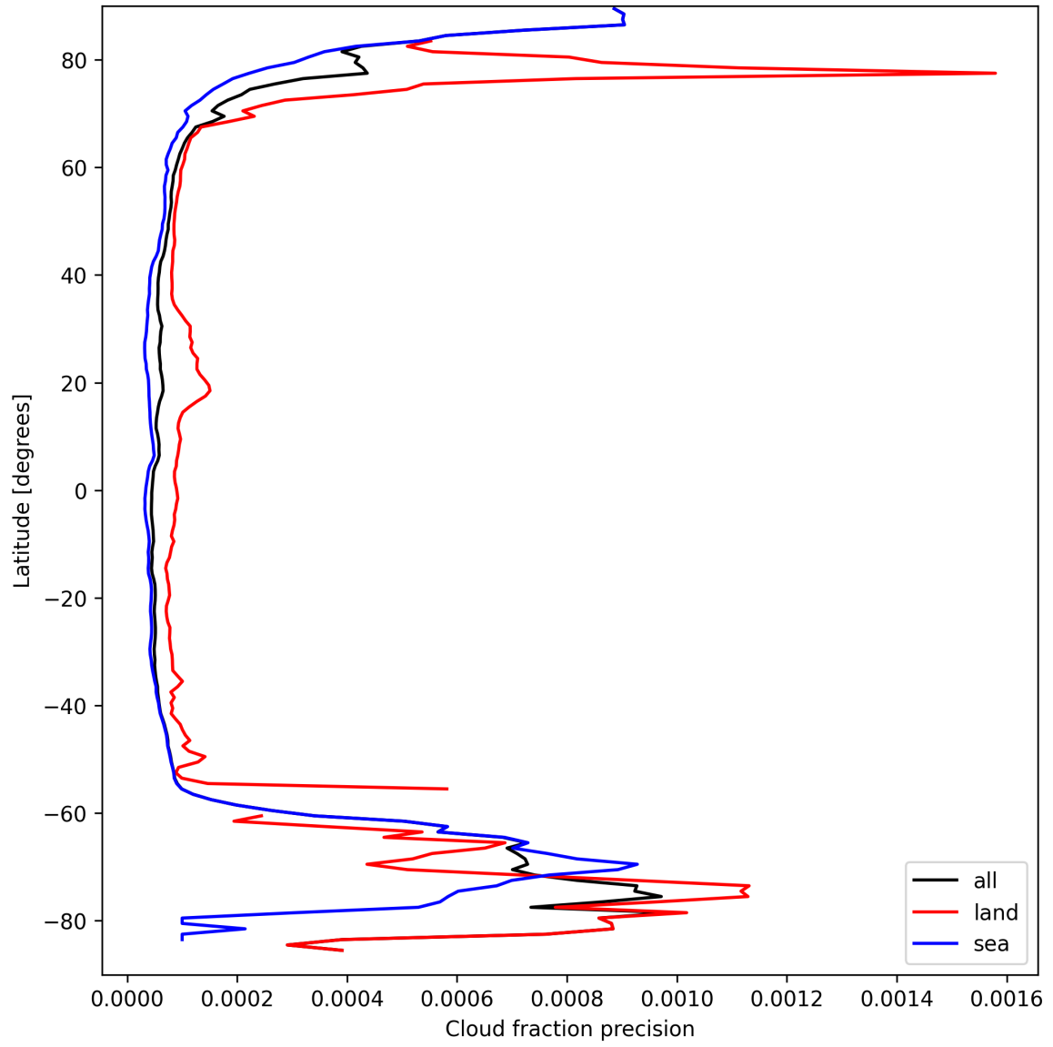
Figure 16: Zonal average of “Cloud fraction precision” for 2025-09-15 to 2025-09-16.
