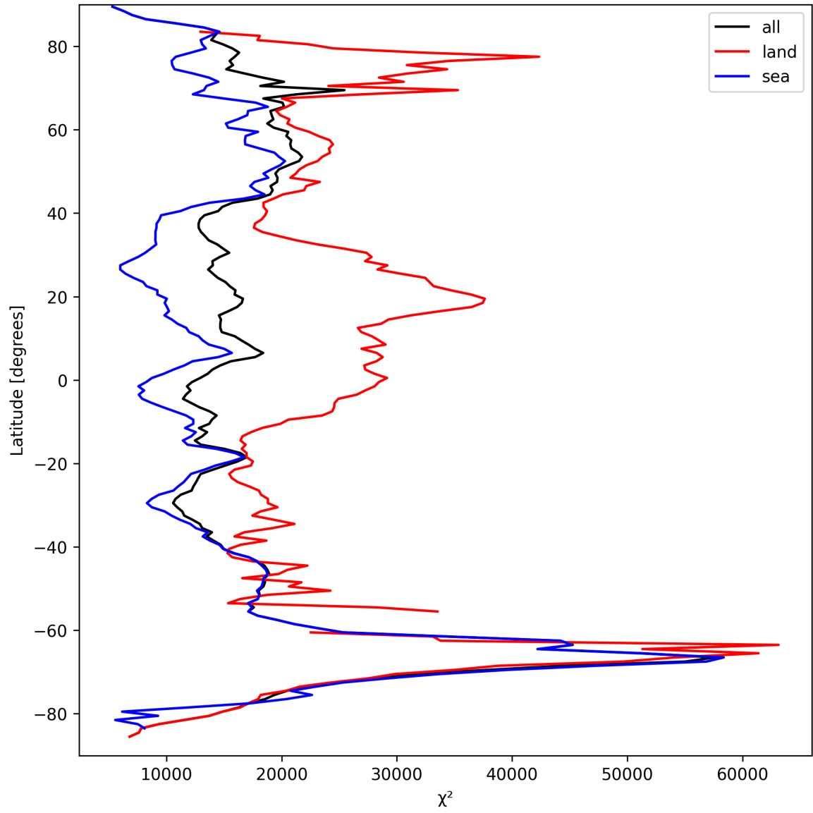
Figure 21: Zonal average of “ \chi^2 ” for 2025-09-15 to 2025-09-16.
