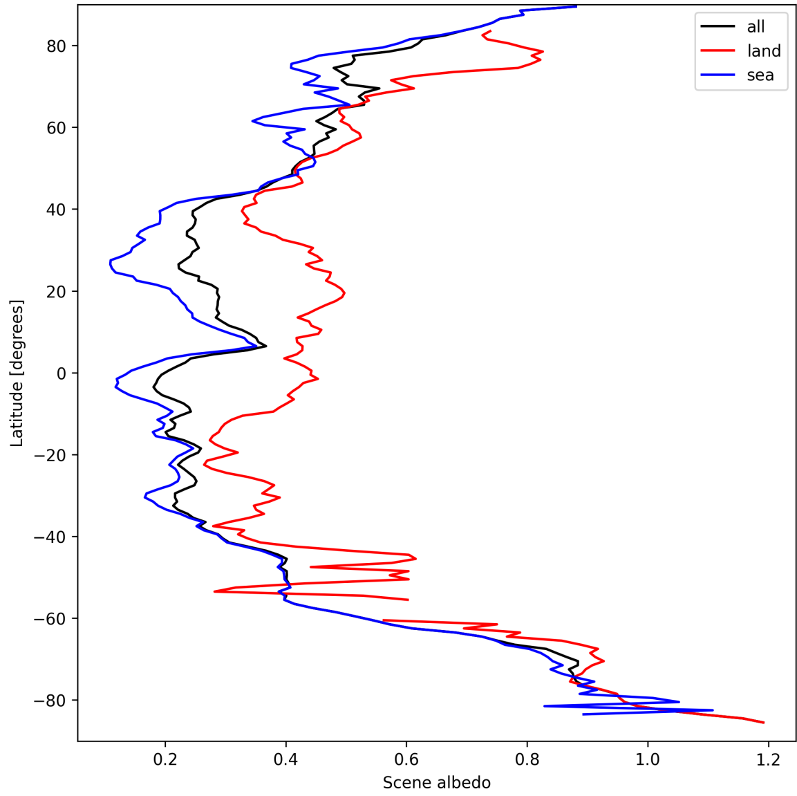
Figure 17: Zonal average of “Scene albedo” for 2025-09-15 to 2025-09-16.
