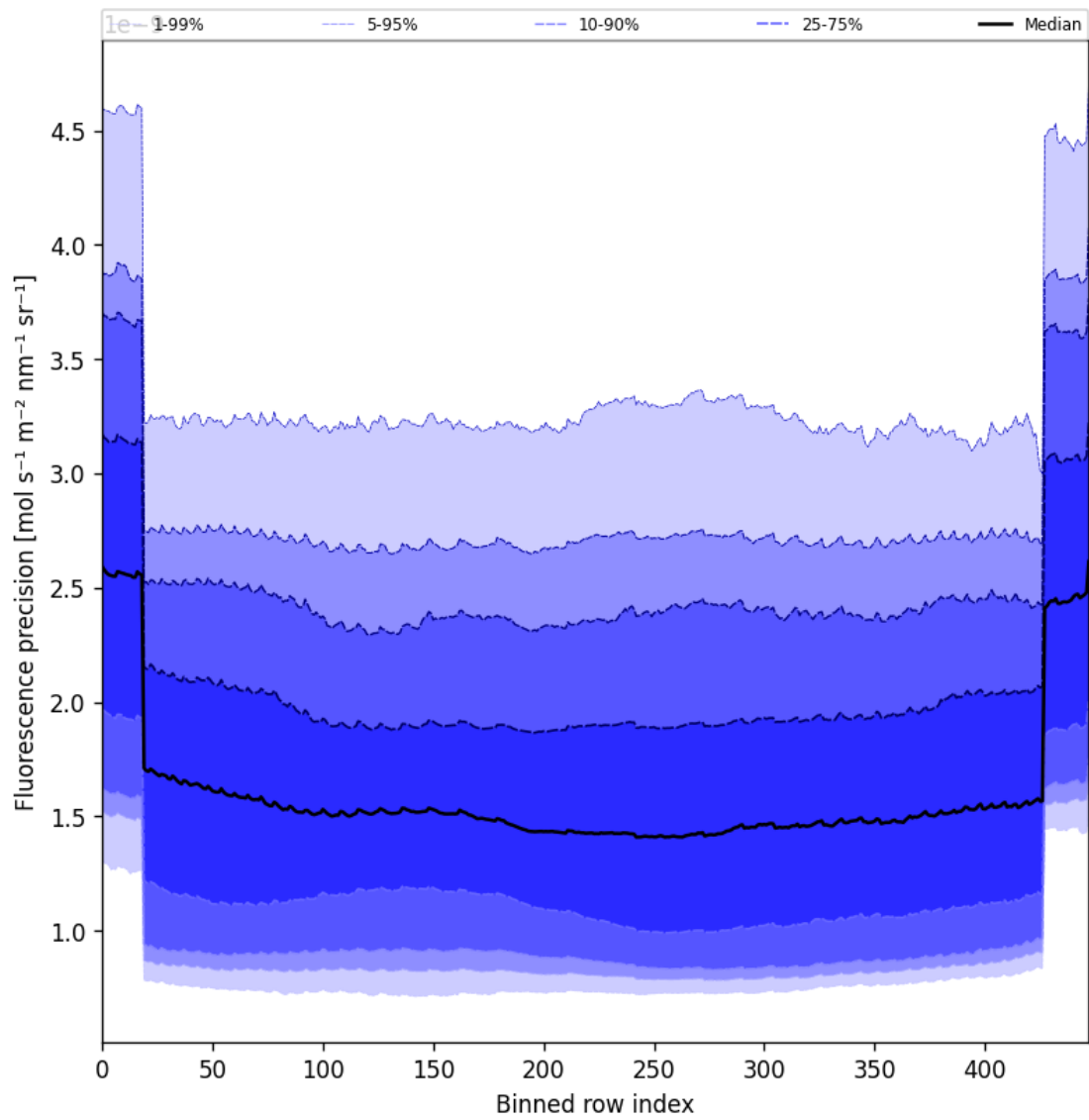
Figure 58: Along track statistics of “Fluorescence precision” for 2025-09-15 to 2025-09-16
