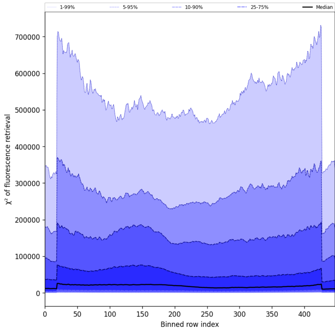
Figure 59: Along track statistics of “ \chi^2 of fluorescence retrieval” for 2025-09-15 to 2025-09-16
