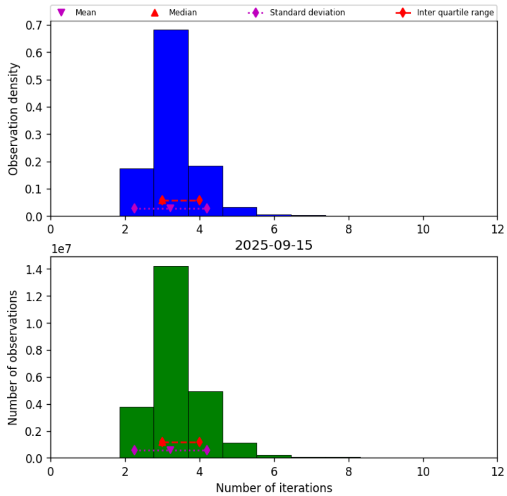
Figure 39: Histogram of “Number of iterations” for 2025-09-15 to 2025-09-16
