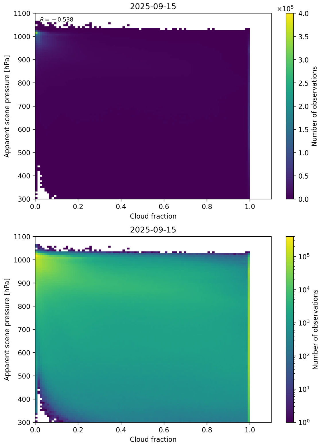
Figure 70: Scatter density plot of “Cloud fraction” against “Apparent scene pressure” for 2025-09-15 to 2025-09-16.
