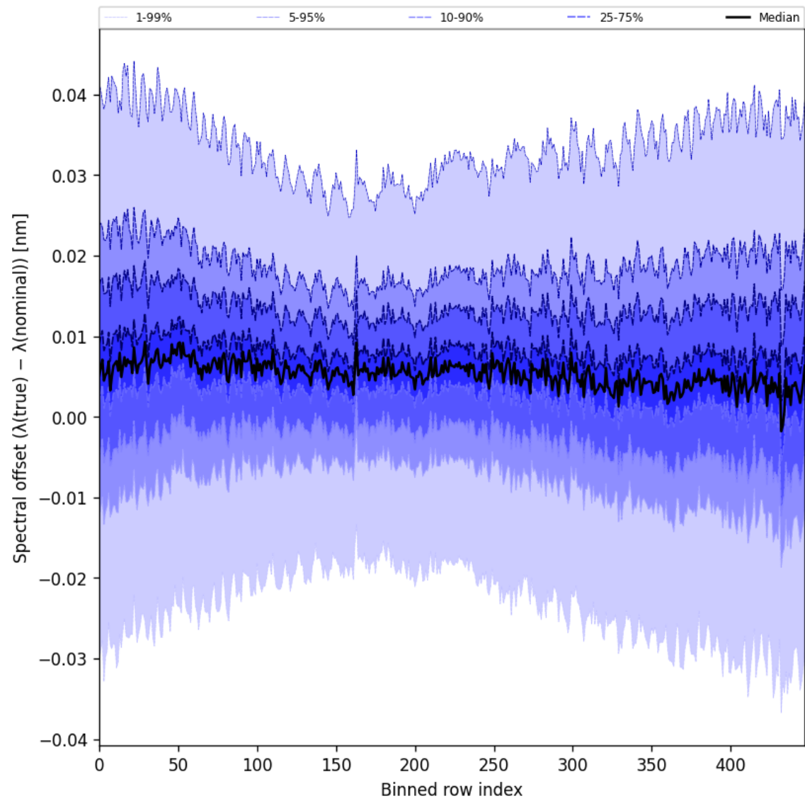
Figure 62: Along track statistics of “Spectral offset ( \lambda_{\text{true}} - \lambda_{\text{nominal}} )” for 2025-09-15 to 2025-09-16
