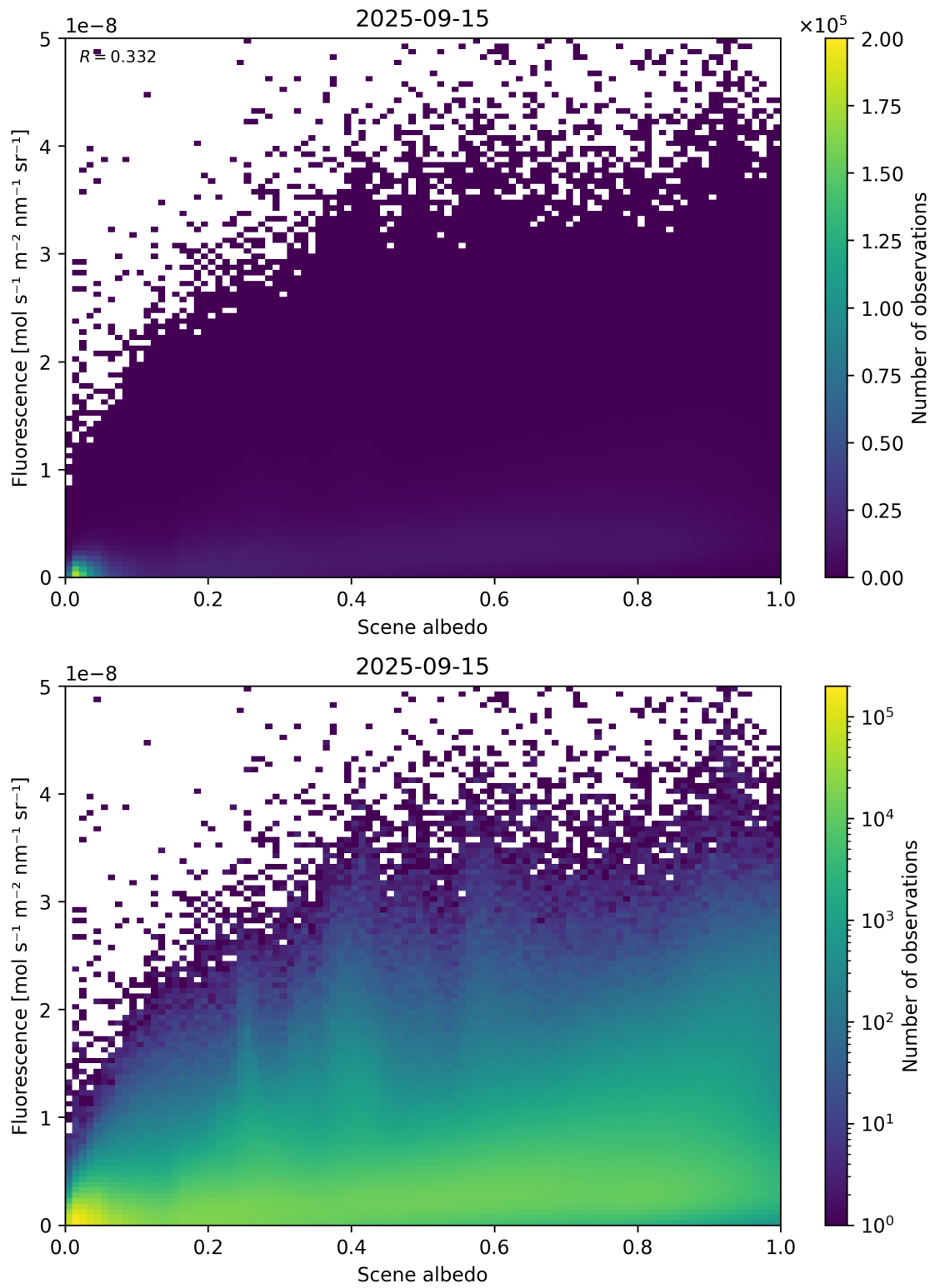
Figure 104: Scatter density plot of “Scene albedo” against “Fluorescence” for 2025-09-15 to 2025-09-16.
