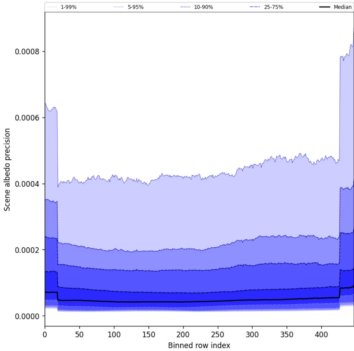
Figure 52: Along track statistics of “Scene albedo precision” for 2025-09-15 to 2025-09-16
