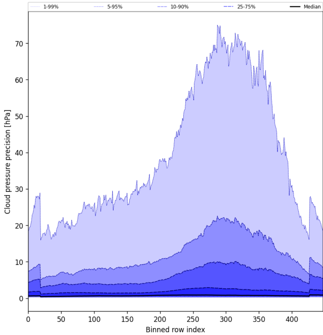
Figure 48: Along track statistics of “Cloud pressure precision” for 2025-09-15 to 2025-09-16
