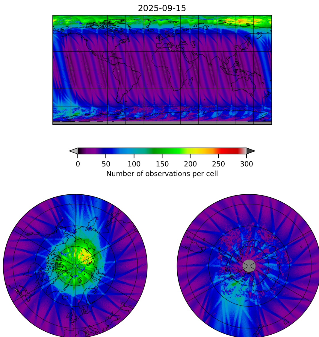
Figure 11: Map of the number of observations for 2025-09-15 to 2025-09-16
