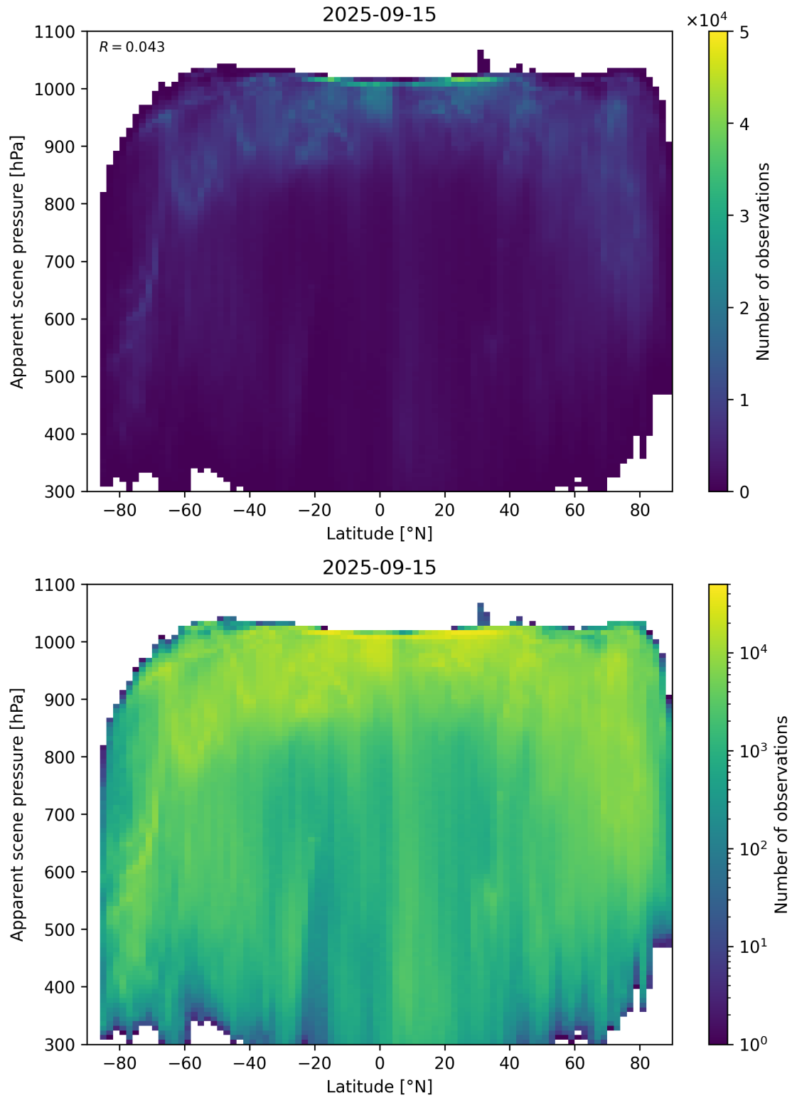
Figure 88: Scatter density plot of “Latitude” against “Apparent scene pressure” for 2025-09-15 to 2025-09-16.
