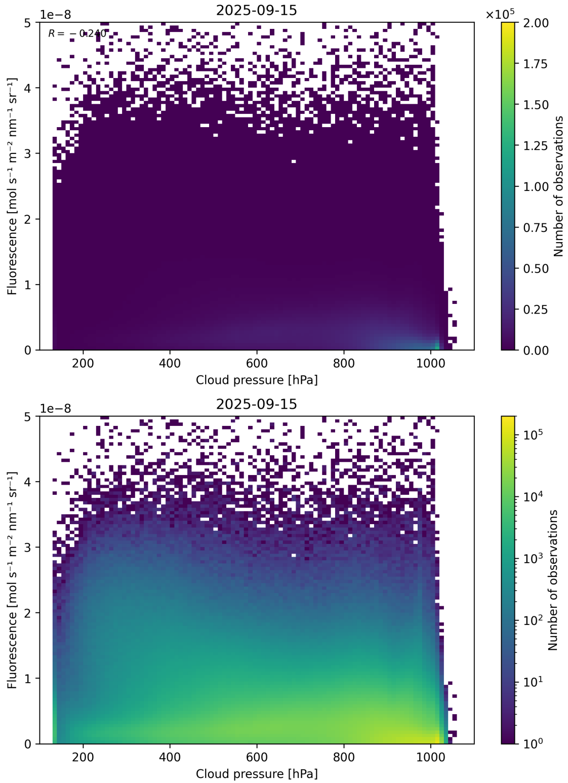
Figure 80: Scatter density plot of “Cloud pressure” against “Fluorescence” for 2025-09-15 to 2025-09-16.
