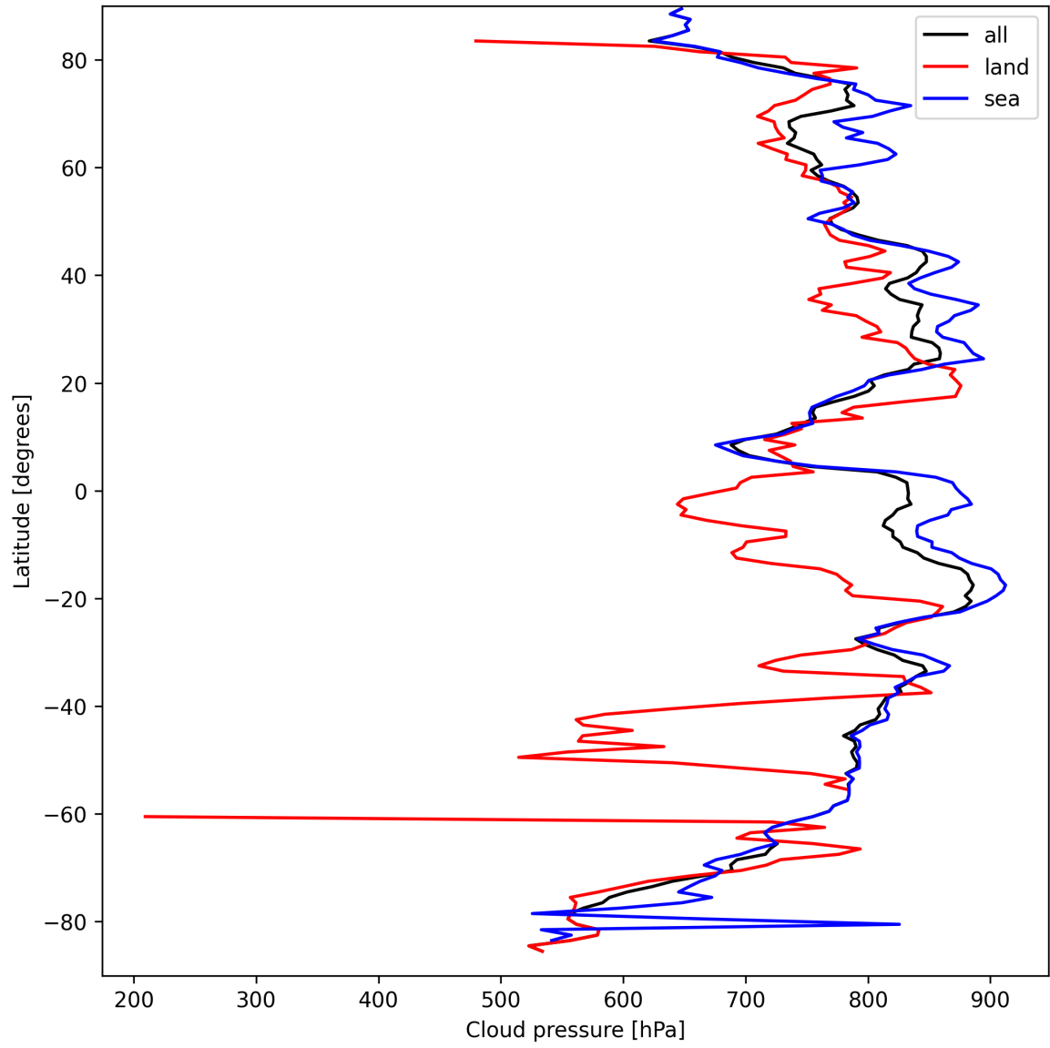
Figure 13: Zonal average of “Cloud pressure” for 2025-09-15 to 2025-09-16.
