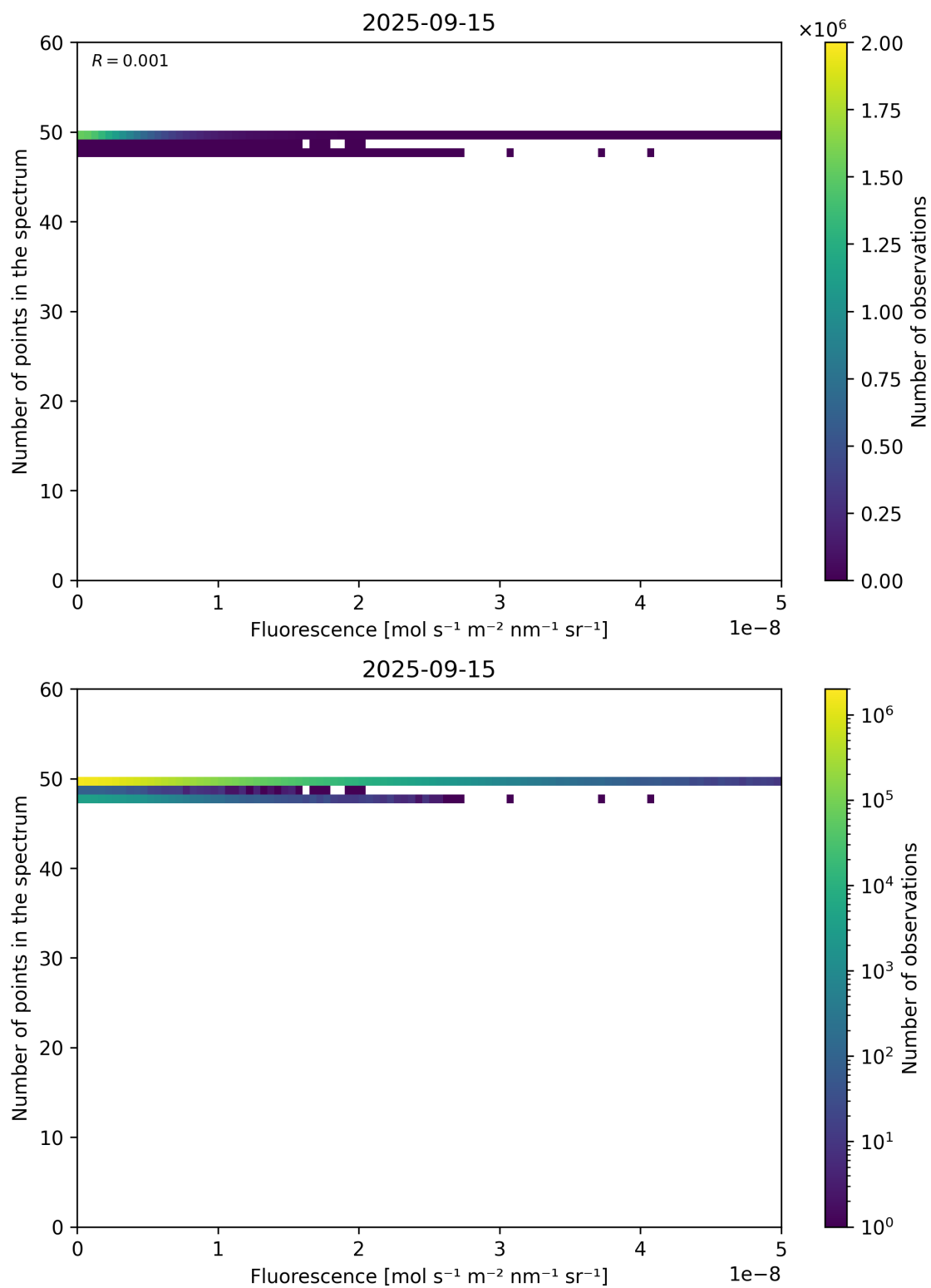
Figure 86: Scatter density plot of “Fluorescence” against “Number of points in the spectrum” for 2025-09-15 to 2025-09-16.
