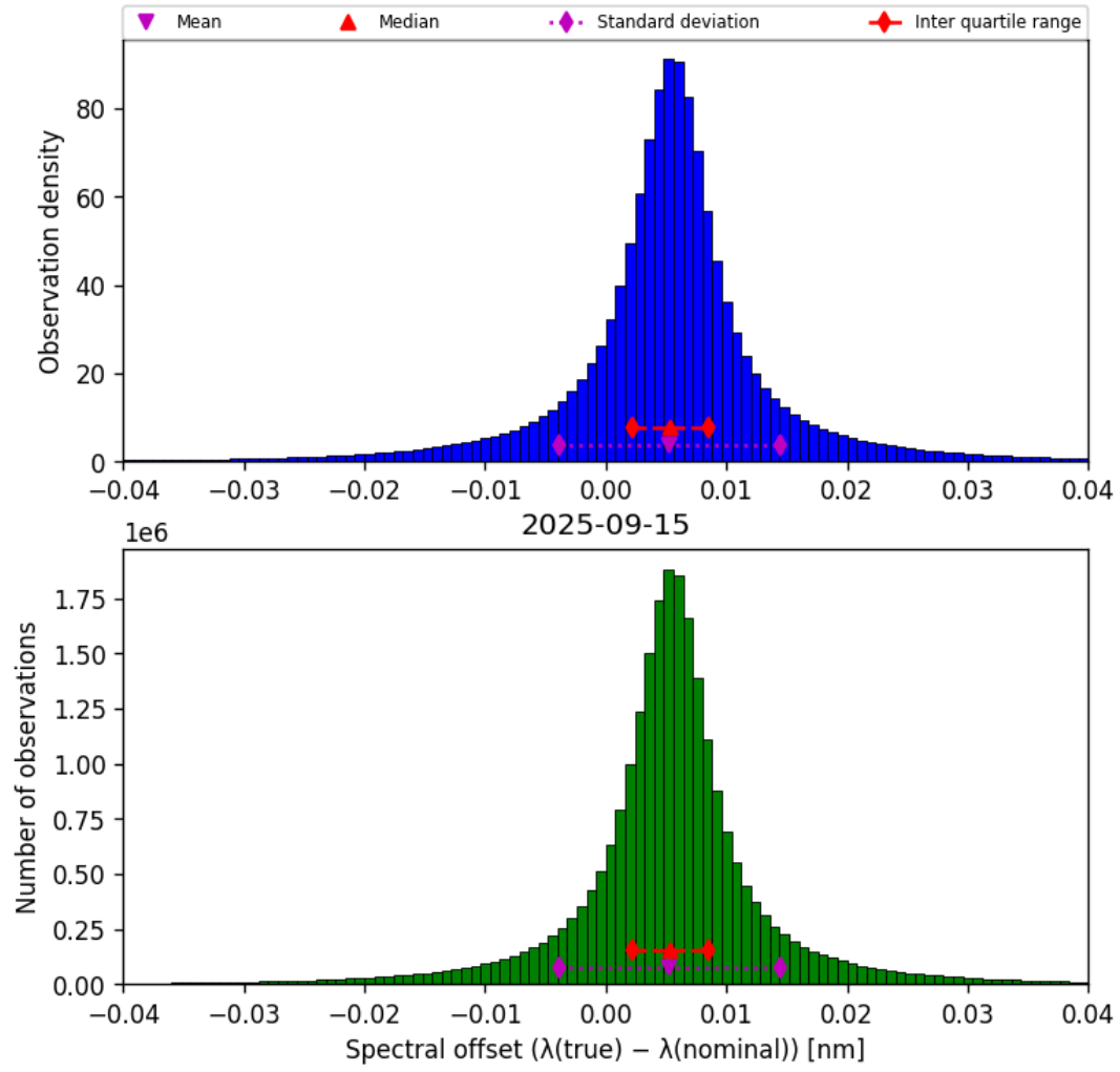
Figure 45: Histogram of “Spectral offset ( \lambda_{\text{true}} - \lambda_{\text{nominal}} )” for 2025-09-15 to 2025-09-16
