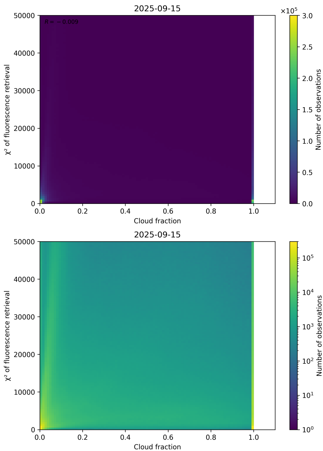
Figure 71: Scatter density plot of “Cloud fraction” against “ \chi^2 of fluorescence retrieval” for 2025-09-15 to 2025-09-16.
