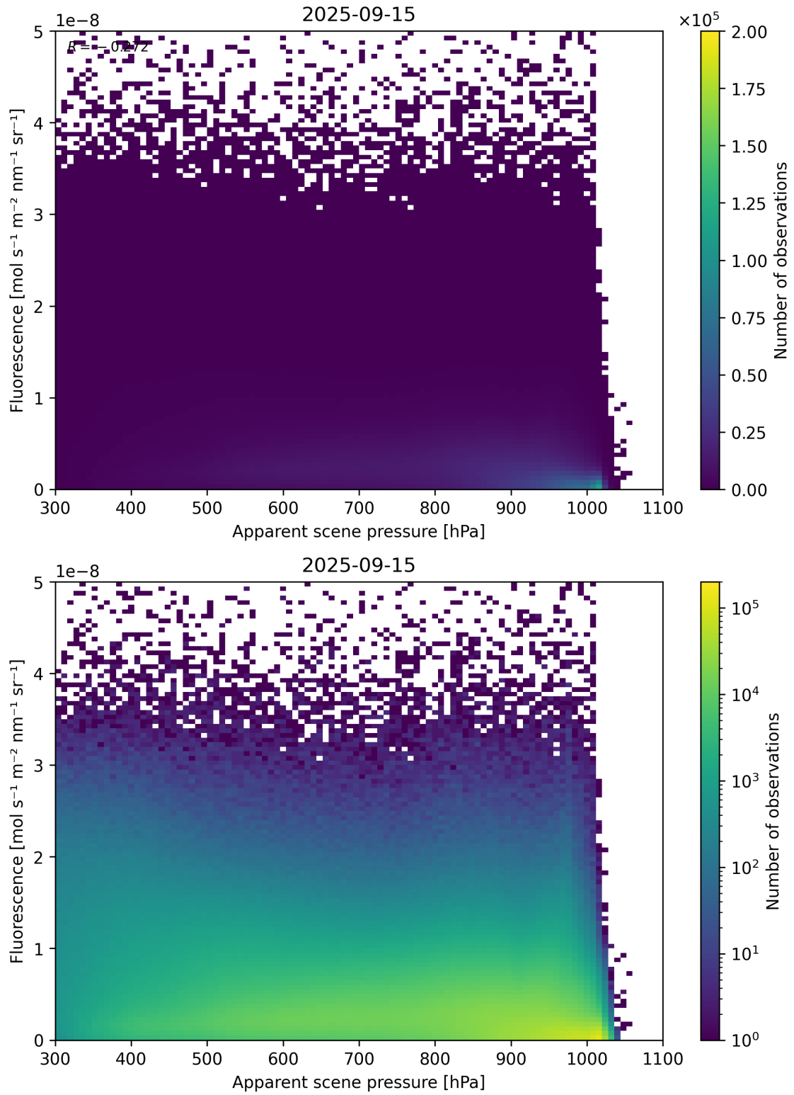
Figure 64: Scatter density plot of “Apparent scene pressure” against “Fluorescence” for 2025-09-15 to 2025-09-16.
