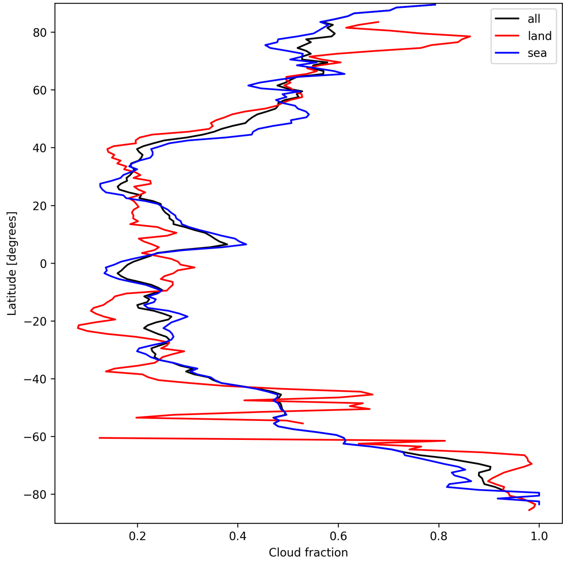
Figure 15: Zonal average of “Cloud fraction” for 2025-09-15 to 2025-09-16.
