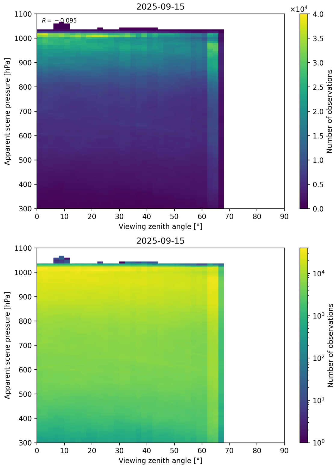
Figure 118: Scatter density plot of “Viewing zenith angle” against “Apparent scene pressure” for 2025-09-15 to 2025-09-16.
