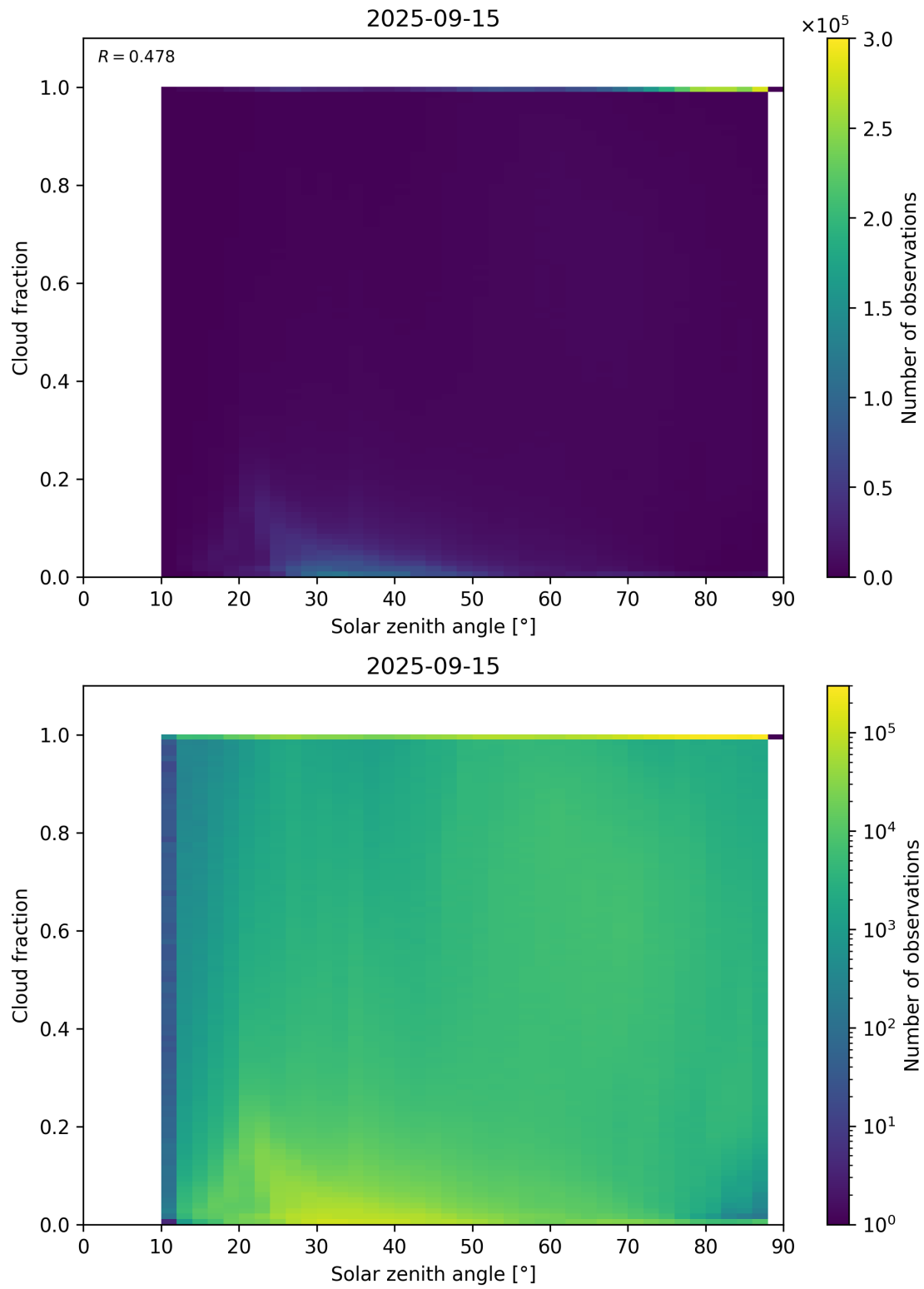
Figure 110: Scatter density plot of “Solar zenith angle” against “Cloud fraction” for 2025-09-15 to 2025-09-16.
