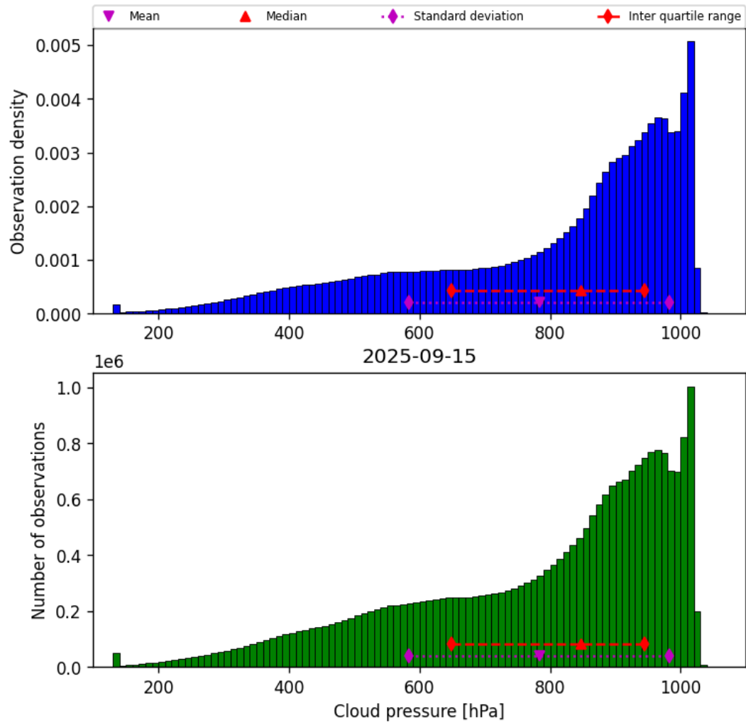
Figure 30: Histogram of “Cloud pressure” for 2025-09-15 to 2025-09-16
