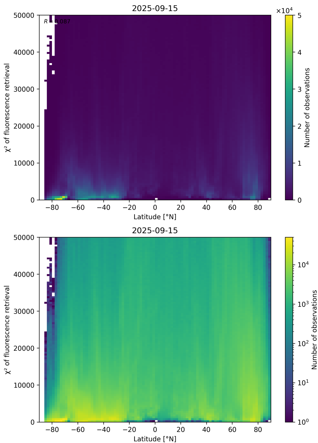
Figure 89: Scatter density plot of “Latitude” against “ \chi^2 of fluorescence retrieval” for 2025-09-15 to 2025-09-16.
