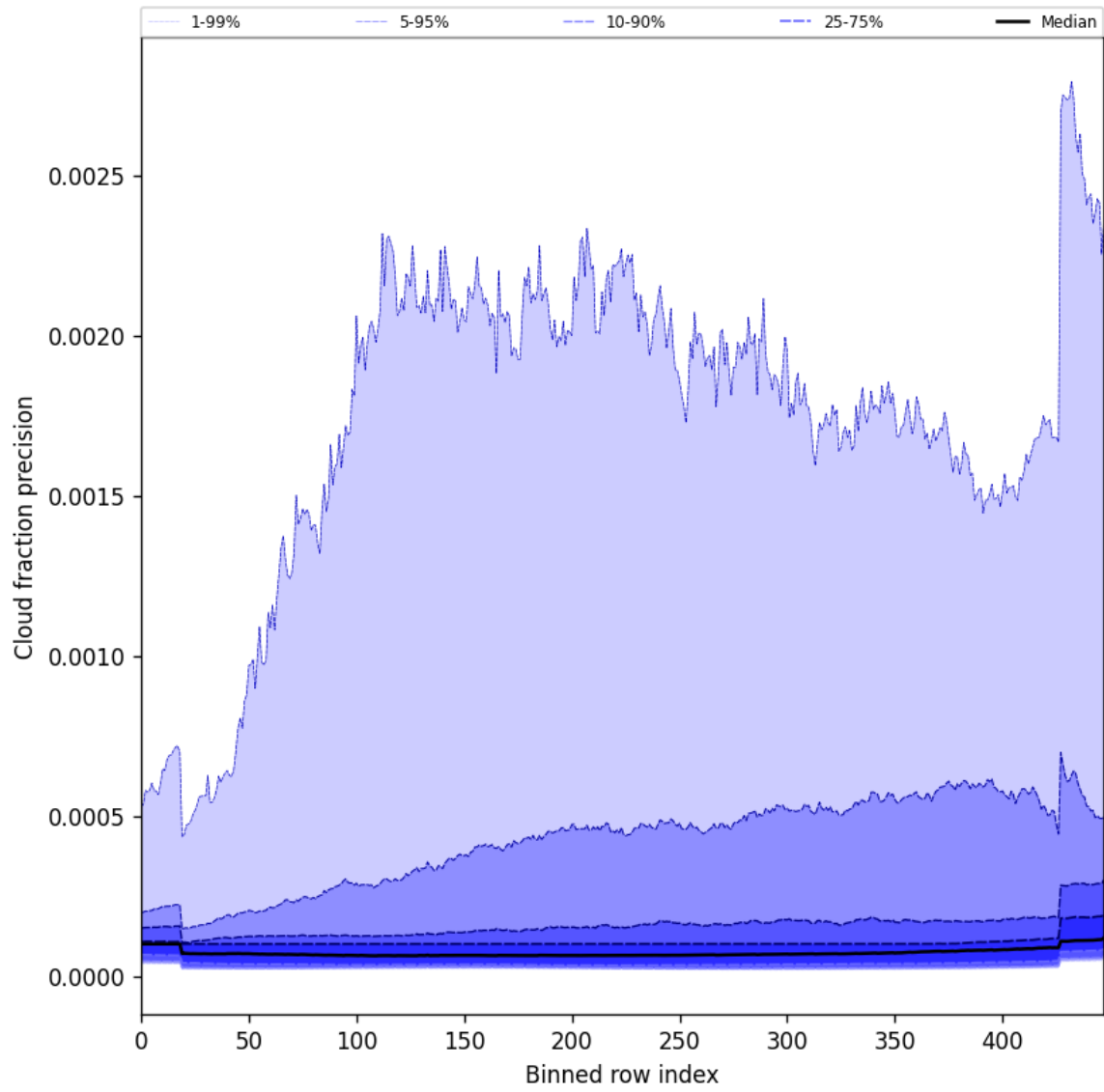
Figure 50: Along track statistics of “Cloud fraction precision” for 2025-09-15 to 2025-09-16
