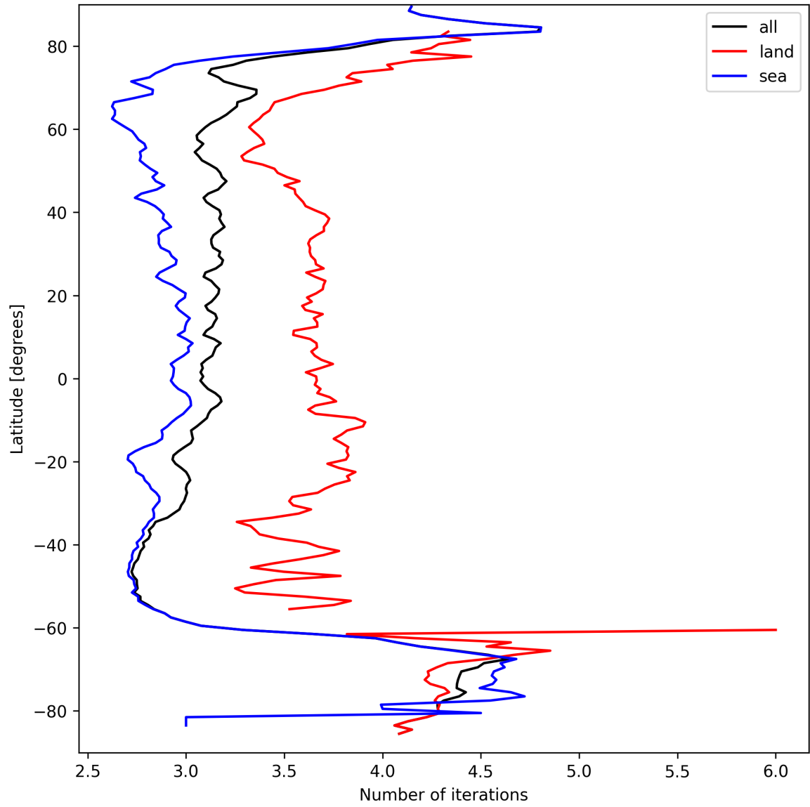
Figure 22: Zonal average of “Number of iterations” for 2025-09-15 to 2025-09-16.
