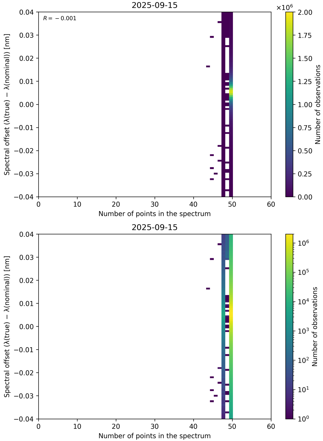
Figure 101: Scatter density plot of “Number of points in the spectrum” against “Spectral offset ( \lambda_{\text{true}} - \lambda_{\text{nominal}} )” for 2025-09-15 to 2025-09-16.
