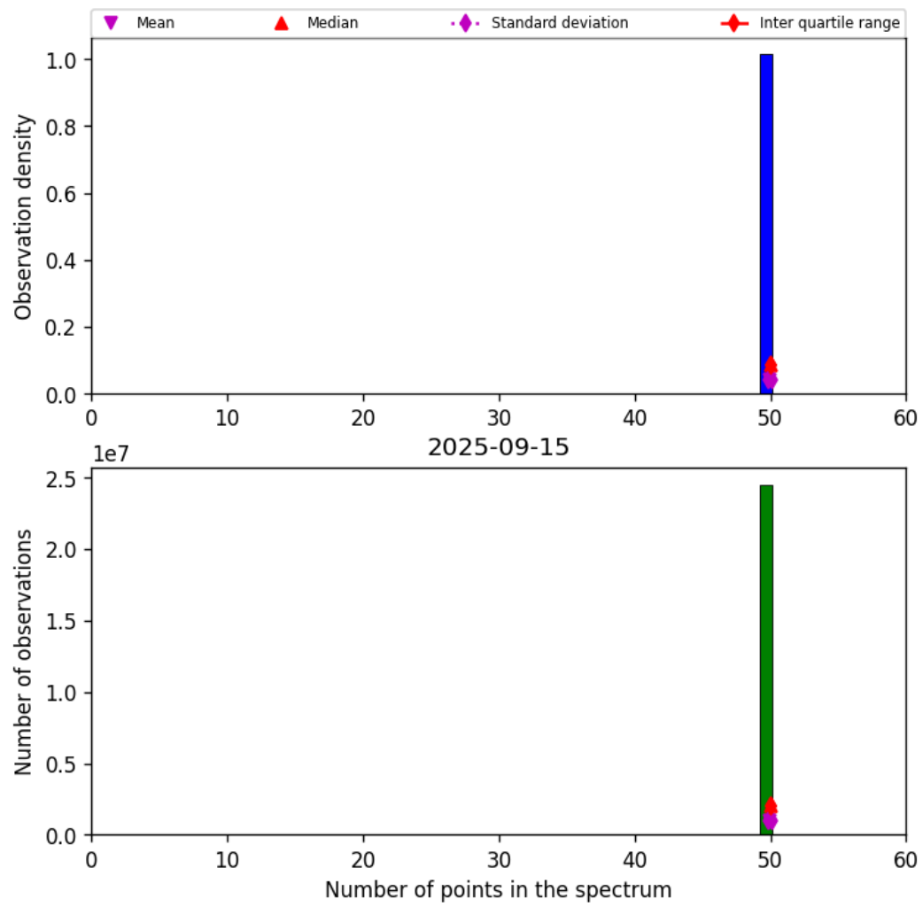
Figure 44: Histogram of “Number of points in the spectrum” for 2025-09-15 to 2025-09-16
