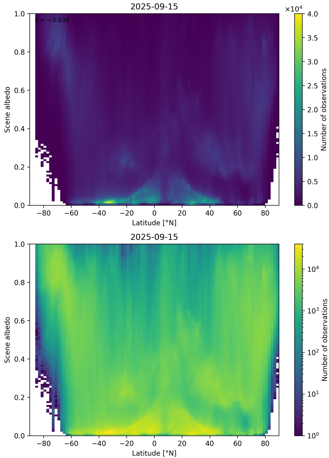
Figure 95: Scatter density plot of “Latitude” against “Scene albedo” for 2025-09-15 to 2025-09-16.
