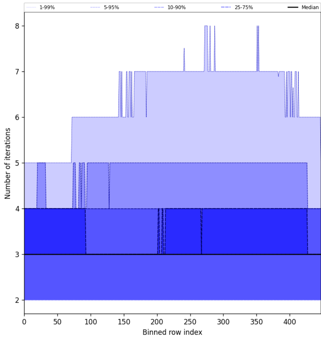
Figure 56: Along track statistics of “Number of iterations” for 2025-09-15 to 2025-09-16
