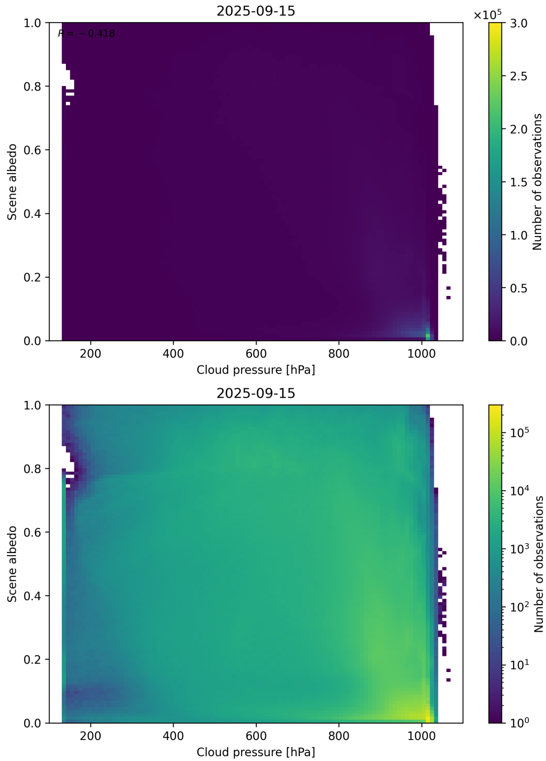
Figure 83: Scatter density plot of “Cloud pressure” against “Scene albedo” for 2025-09-15 to 2025-09-16.
