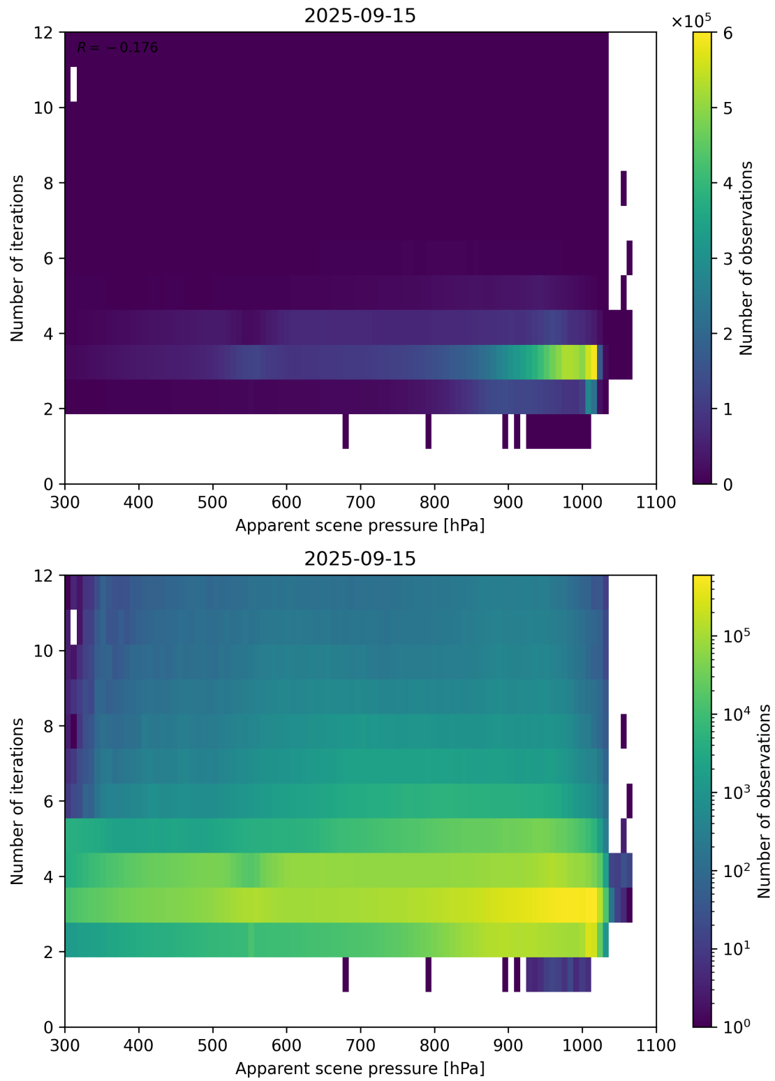
Figure 65: Scatter density plot of “Apparent scene pressure” against “Number of iterations” for 2025-09-15 to 2025-09-16.
