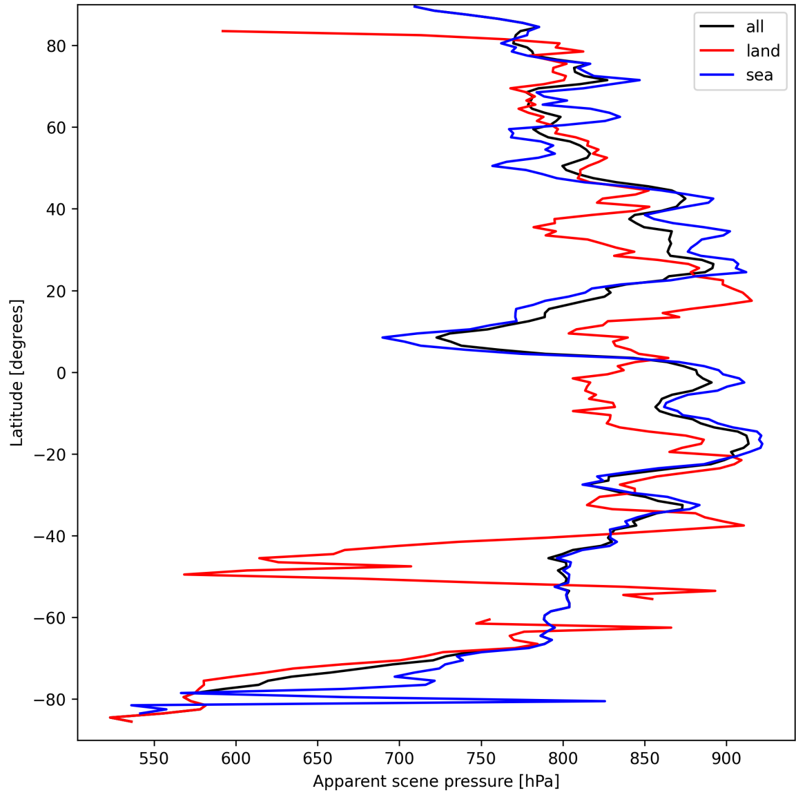
Figure 19: Zonal average of “Apparent scene pressure” for 2025-09-15 to 2025-09-16.
