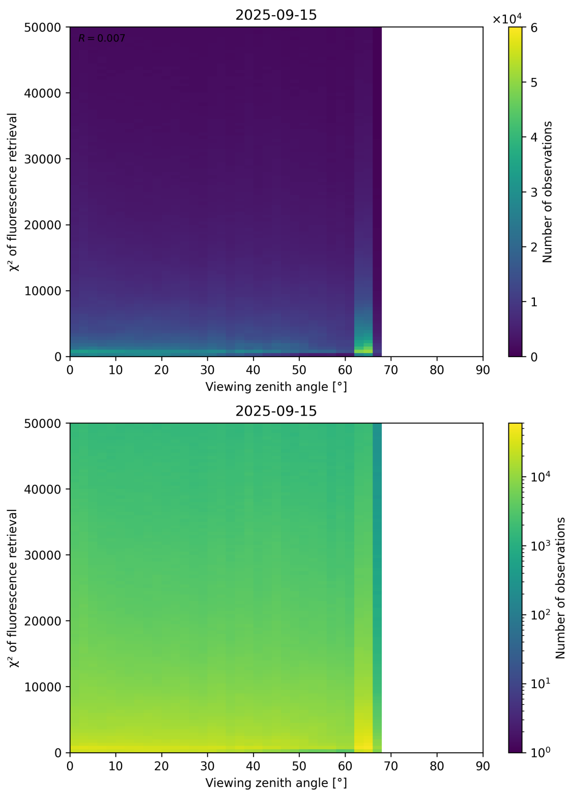
Figure 119: Scatter density plot of “Viewing zenith angle” against “ \chi^2 of fluorescence retrieval” for 2025-09-15 to 2025-09-16.
