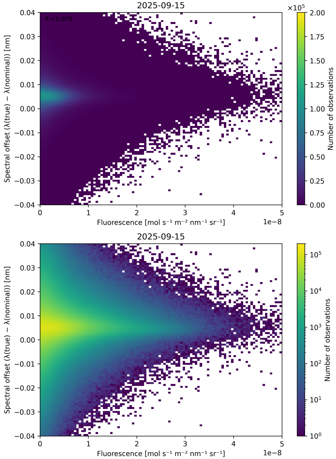
Figure 87: Scatter density plot of “Fluorescence” against “Spectral offset ( \lambda_{\text{true}} - \lambda_{\text{nominal}} )” for 2025-09-15 to 2025-09-16.
