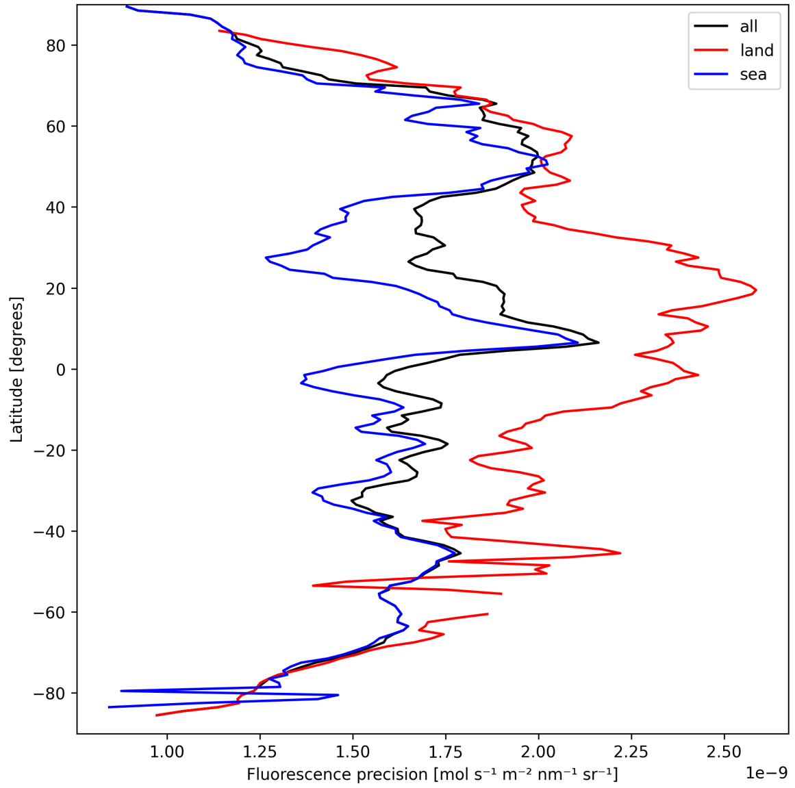
Figure 24: Zonal average of “Fluorescence precision” for 2025-09-15 to 2025-09-16.
