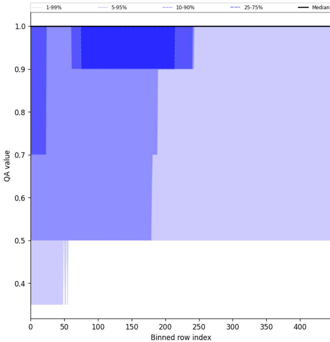
Figure 46: Along track statistics of “QA value” for 2025-09-15 to 2025-09-16
