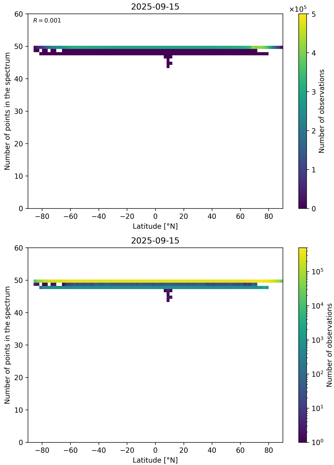
Figure 94: Scatter density plot of “Latitude” against “Number of points in the spectrum” for 2025-09-15 to 2025-09-16.
