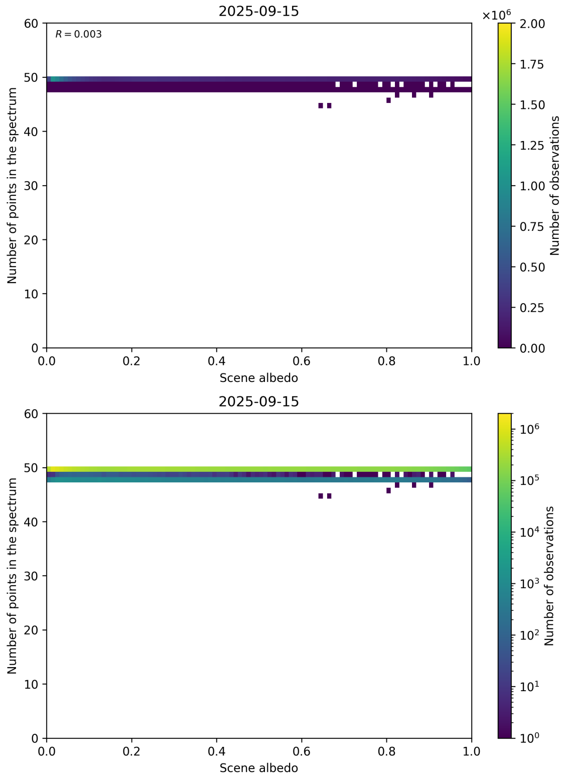
Figure 106: Scatter density plot of “Scene albedo” against “Number of points in the spectrum” for 2025-09-15 to 2025-09-16.
