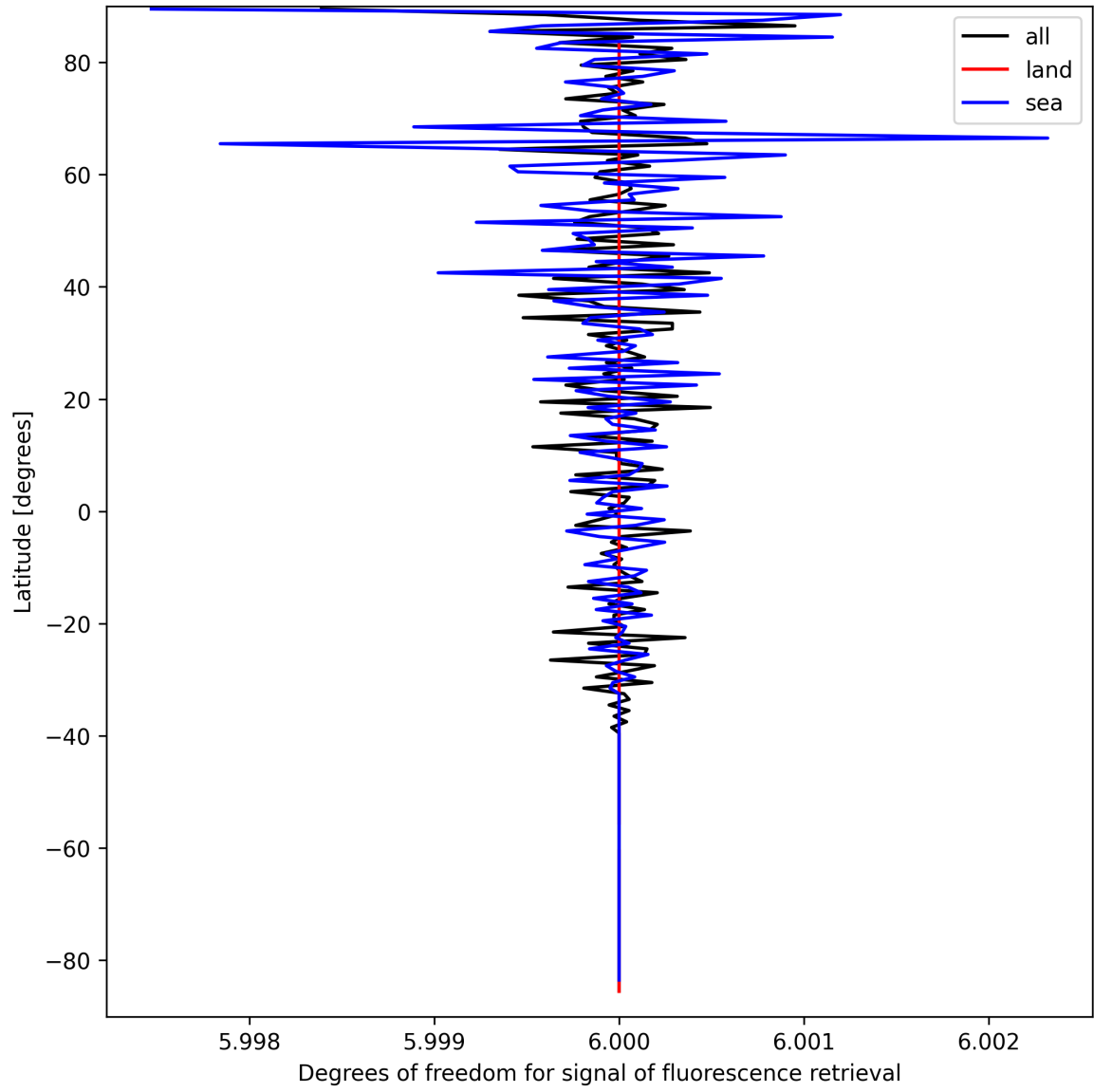
Figure 26: Zonal average of “Degrees of freedom for signal of fluorescence retrieval” for 2025-09-15 to 2025-09-16.
