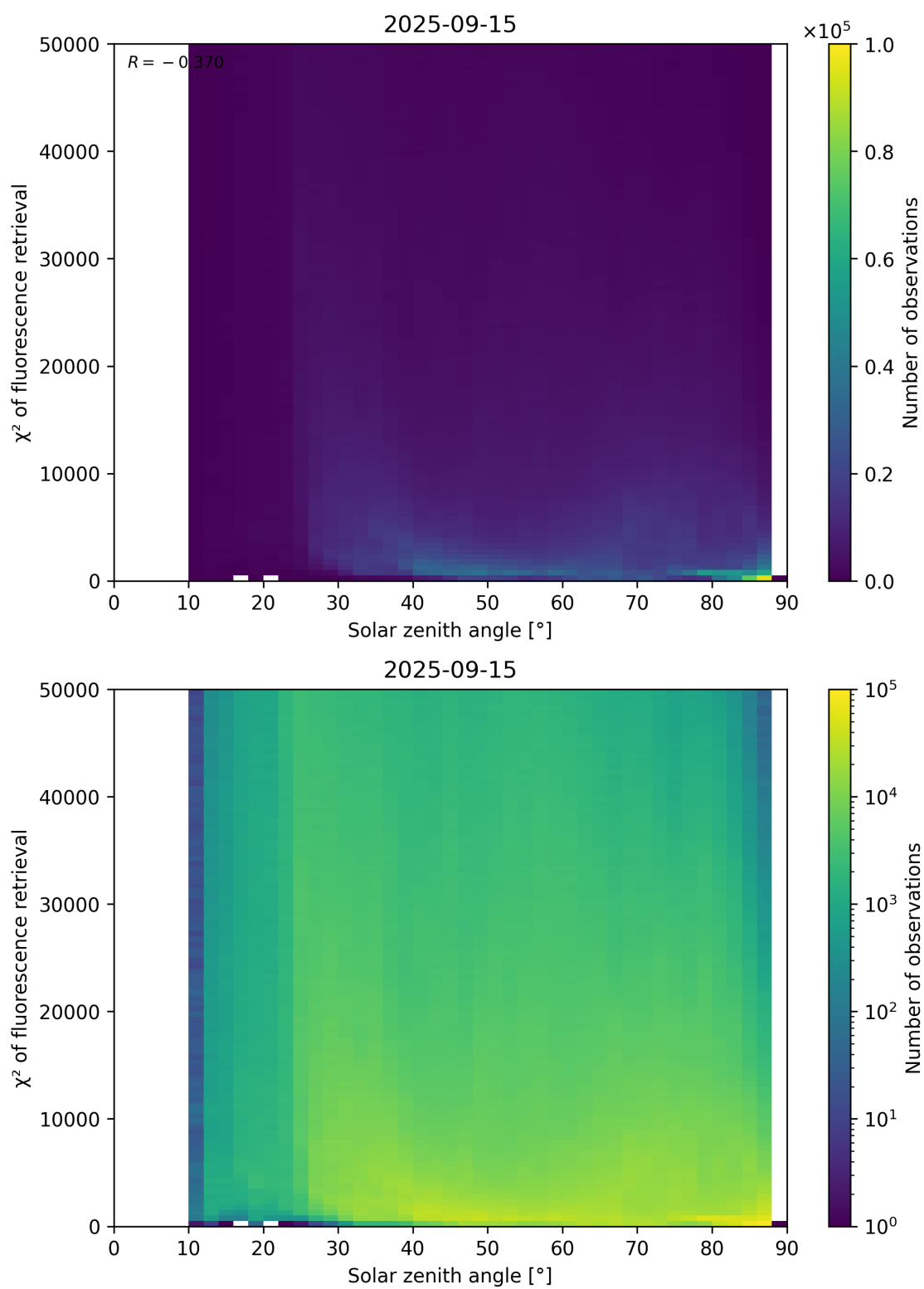
Figure 109: Scatter density plot of “Solar zenith angle” against “ \chi^2 of fluorescence retrieval” for 2025-09-15 to 2025-09-16.
