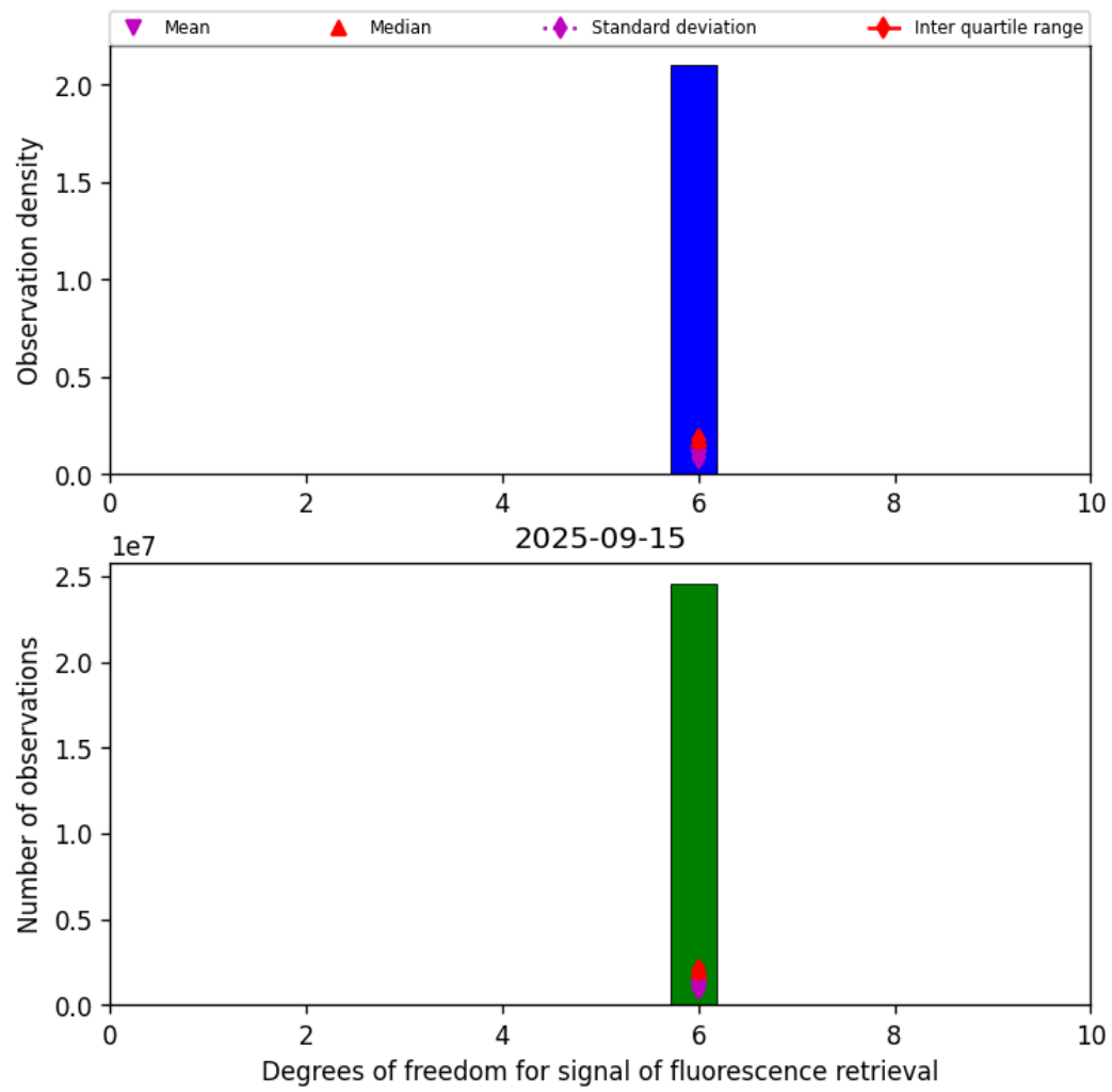
Figure 43: Histogram of “Degrees of freedom for signal of fluorescence retrieval” for 2025-09-15 to 2025-09-16
