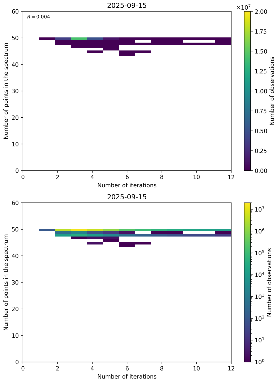
Figure 99: Scatter density plot of “Number of iterations” against “Number of points in the spectrum” for 2025-09-15 to 2025-09-16.
