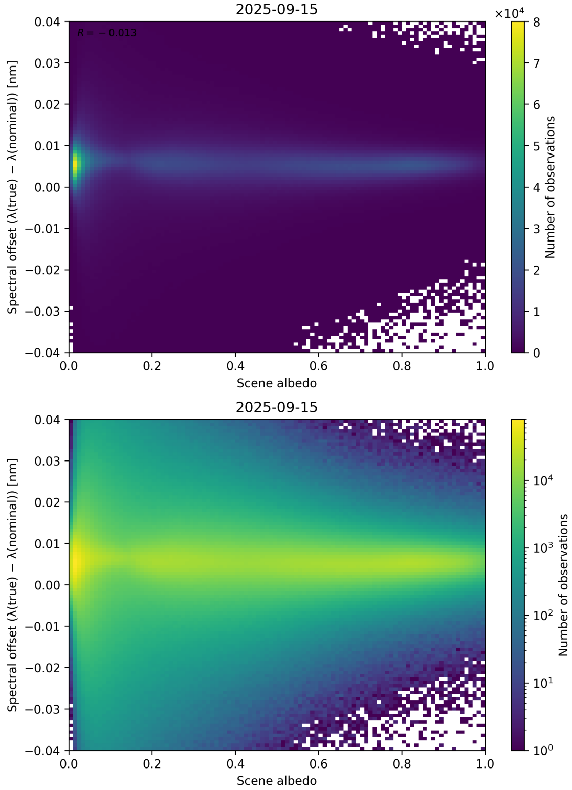
Figure 107: Scatter density plot of “Scene albedo” against “Spectral offset ( \lambda_{\text{true}} - \lambda_{\text{nominal}} )” for 2025-09-15 to 2025-09-16.
