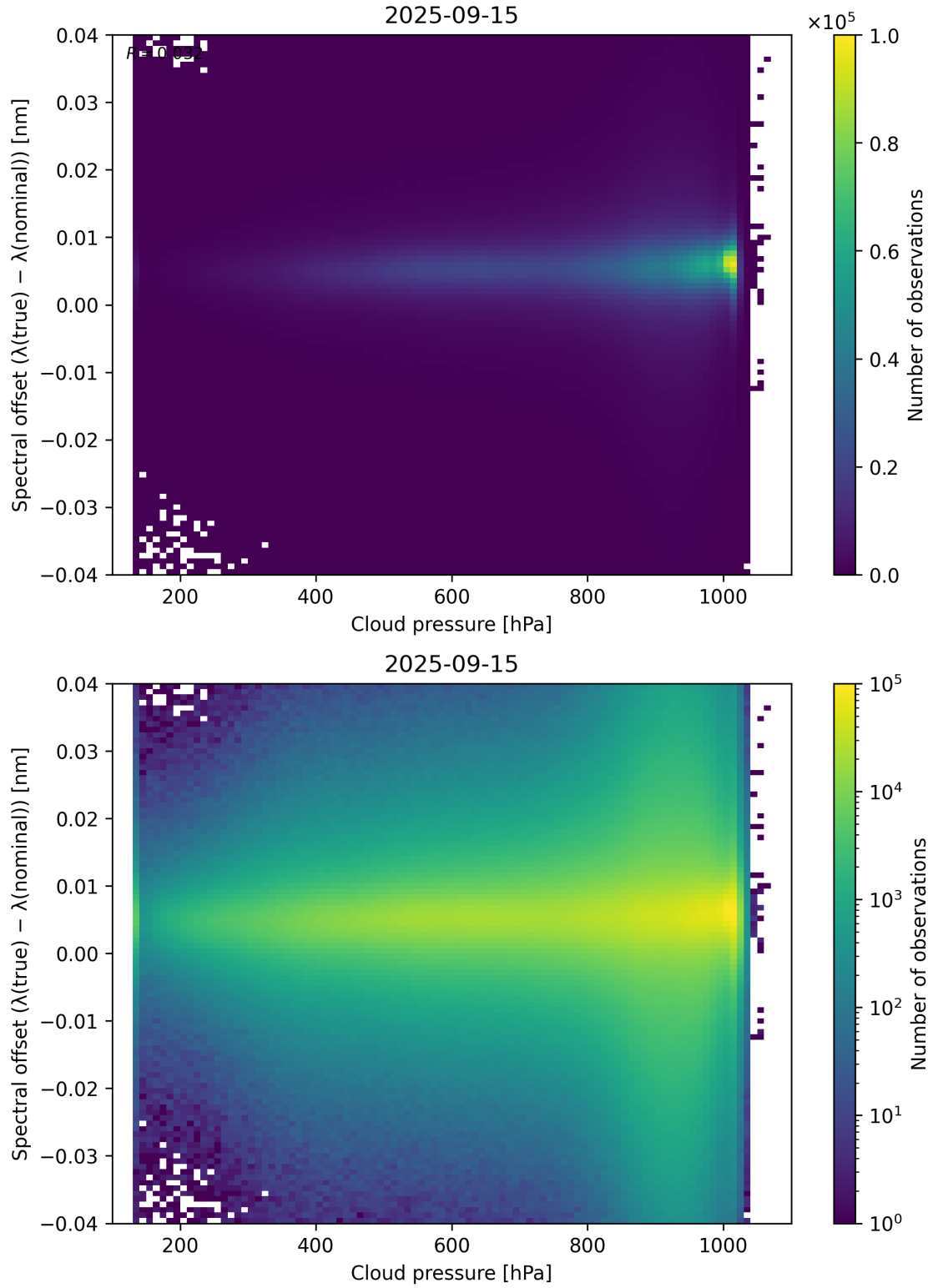
Figure 84: Scatter density plot of “Cloud pressure” against “Spectral offset ( \lambda_{\text{true}} - \lambda_{\text{nominal}} )” for 2025-09-15 to 2025-09-16.
