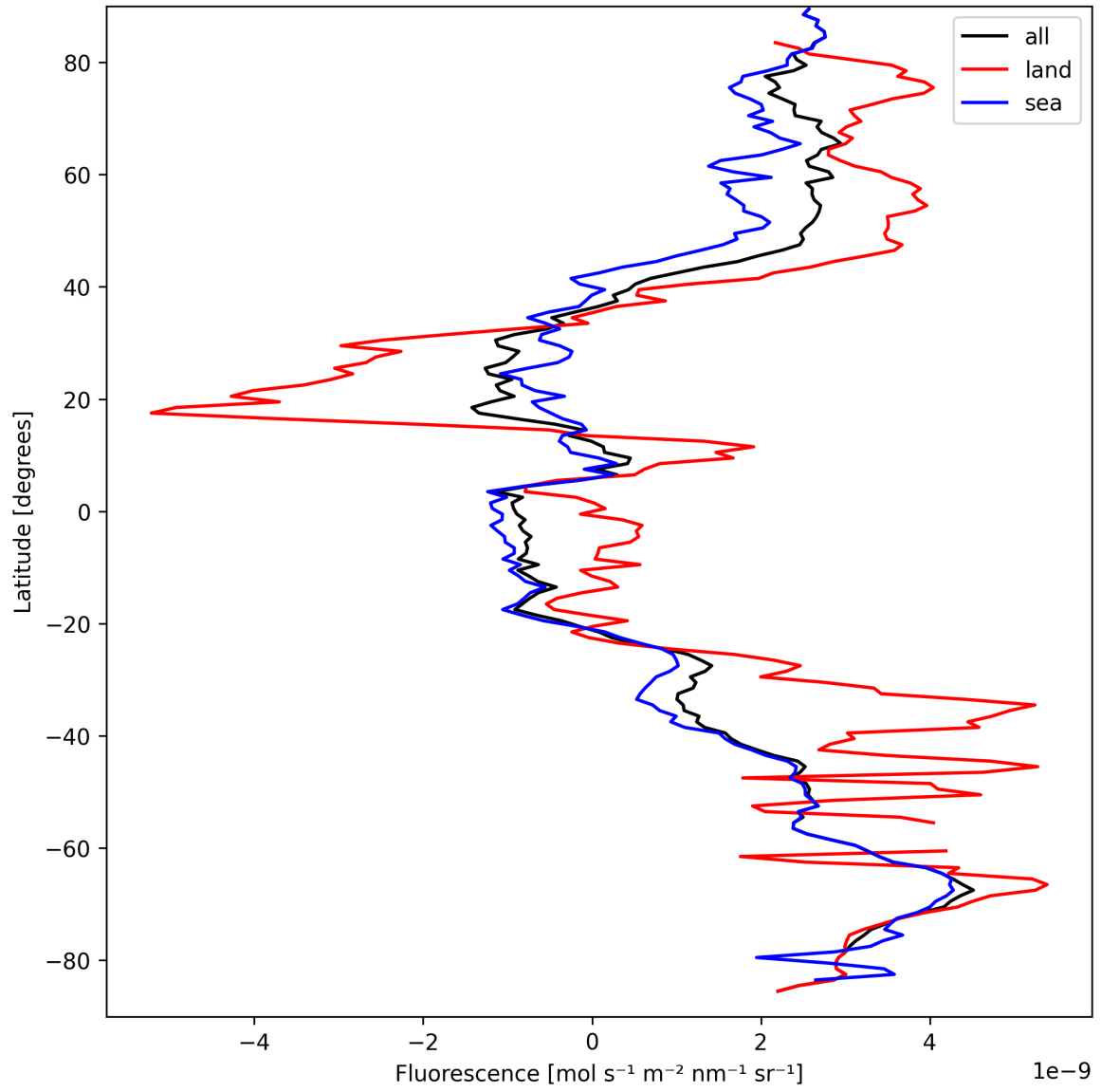
Figure 23: Zonal average of “Fluorescence” for 2025-09-15 to 2025-09-16.
