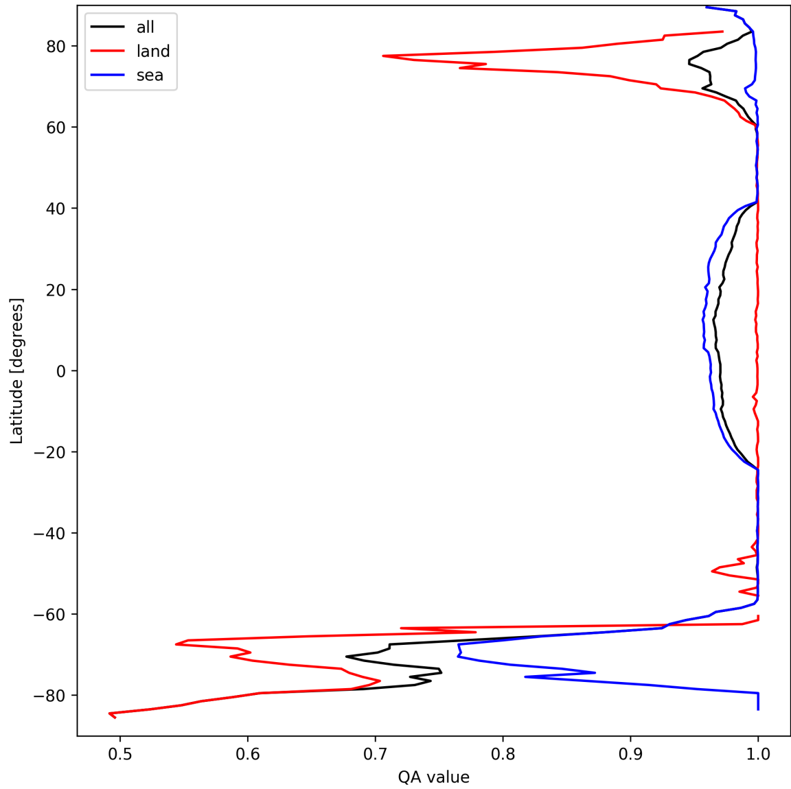
Figure 12: Zonal average of “QA value” for 2025-09-15 to 2025-09-16.
