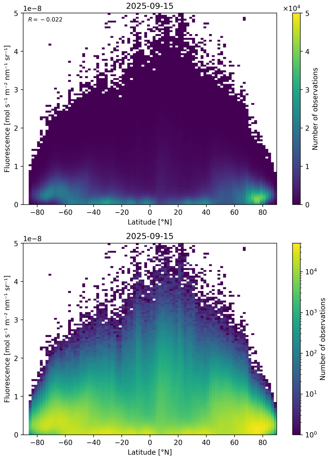
Figure 92: Scatter density plot of “Latitude” against “Fluorescence” for 2025-09-15 to 2025-09-16.
