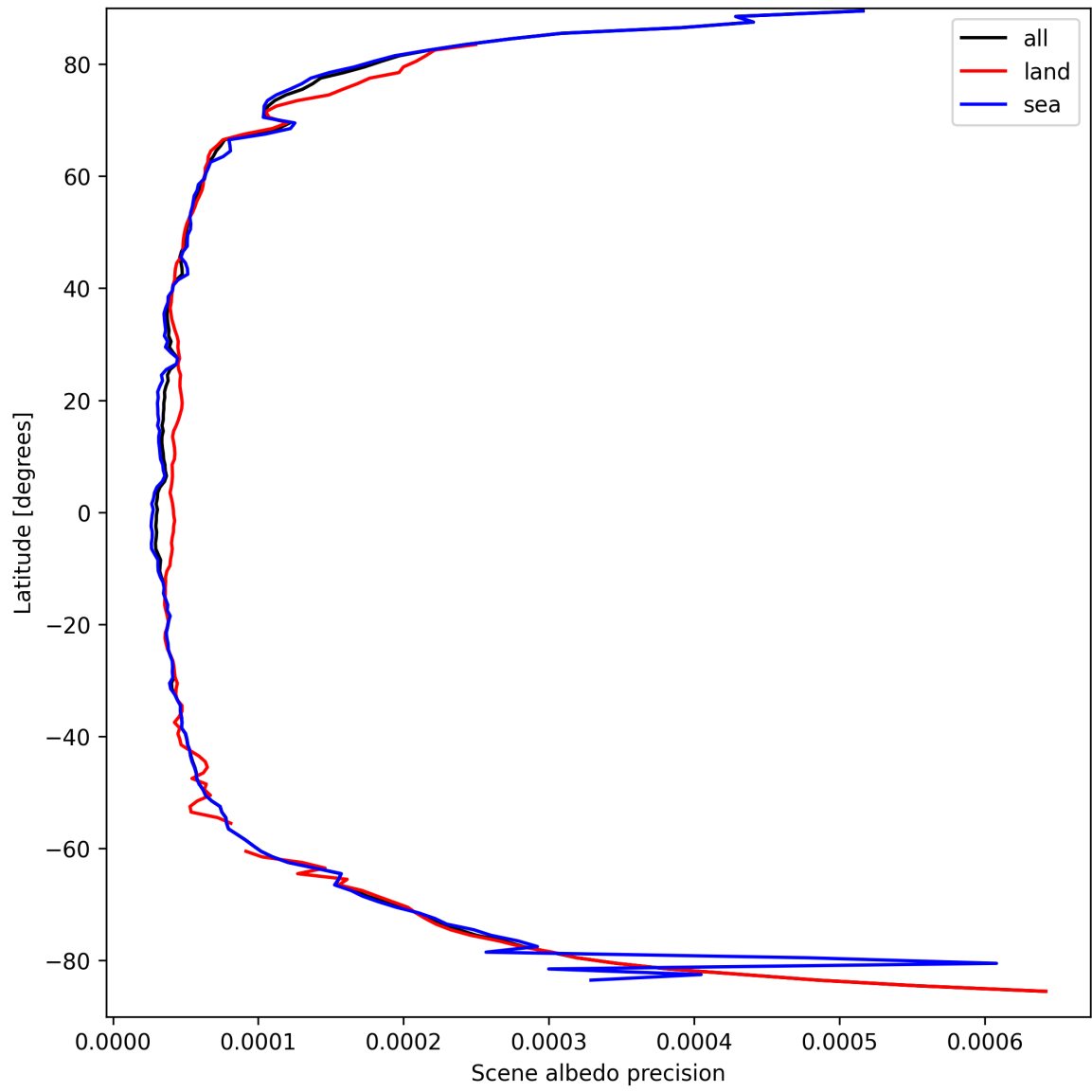
Figure 18: Zonal average of “Scene albedo precision” for 2025-09-15 to 2025-09-16.
