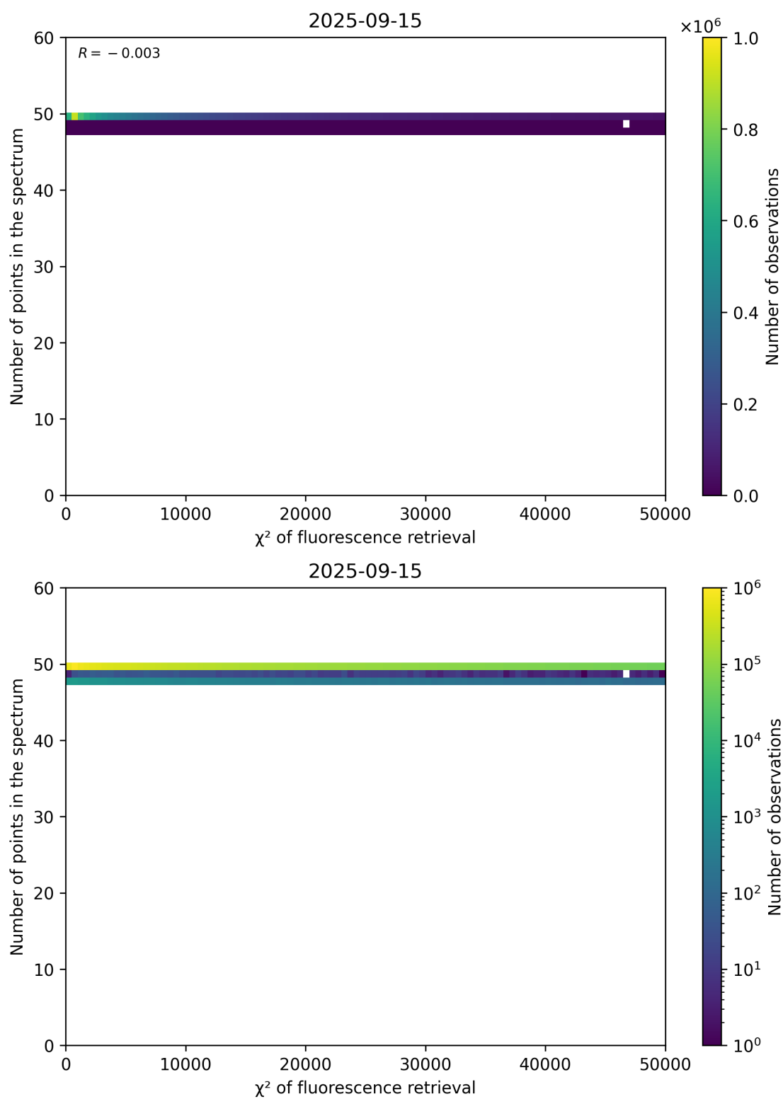
Figure 68: Scatter density plot of " \chi^2 of fluorescence retrieval" against "Number of points in the spectrum" for 2025-09-15 to 2025-09-16.
