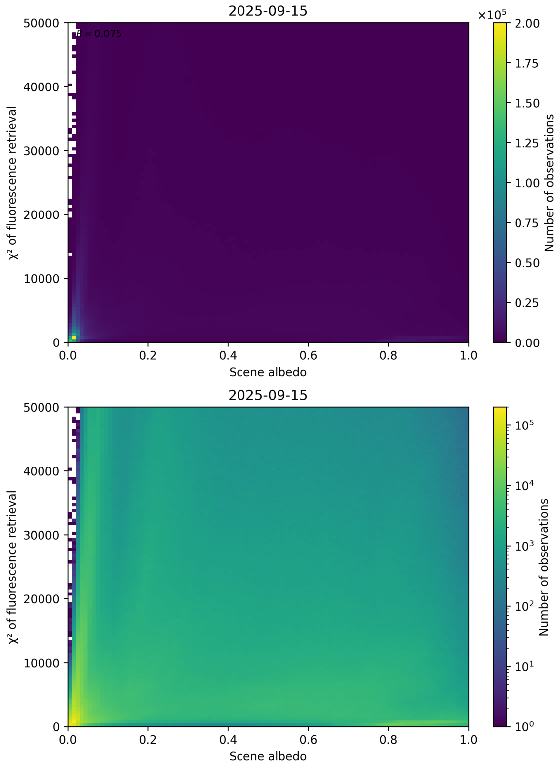
Figure 103: Scatter density plot of “Scene albedo” against “ \chi^2 of fluorescence retrieval” for 2025-09-15 to 2025-09-16.
