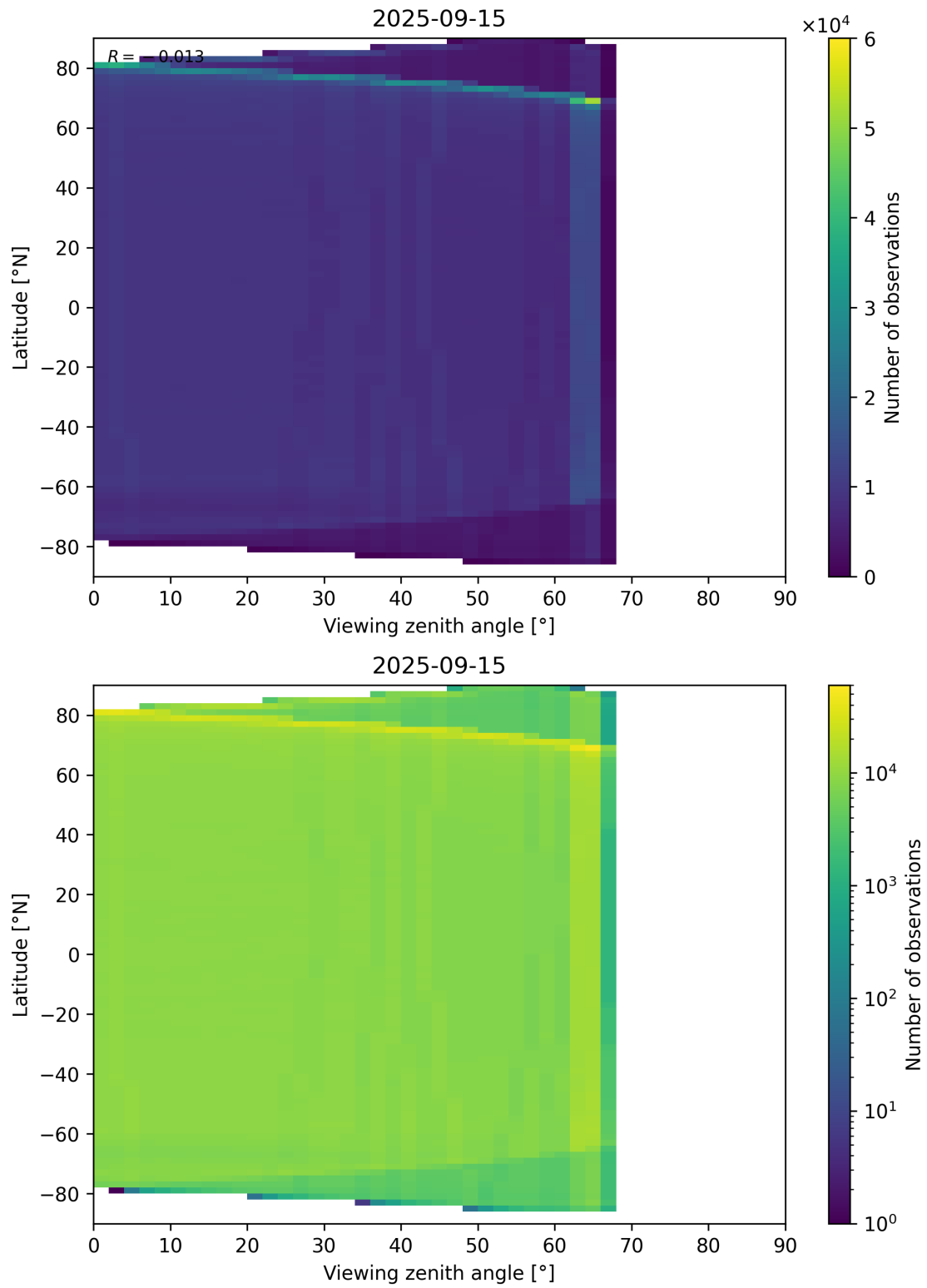
Figure 123: Scatter density plot of “Viewing zenith angle” against “Latitude” for 2025-09-15 to 2025-09-16.
