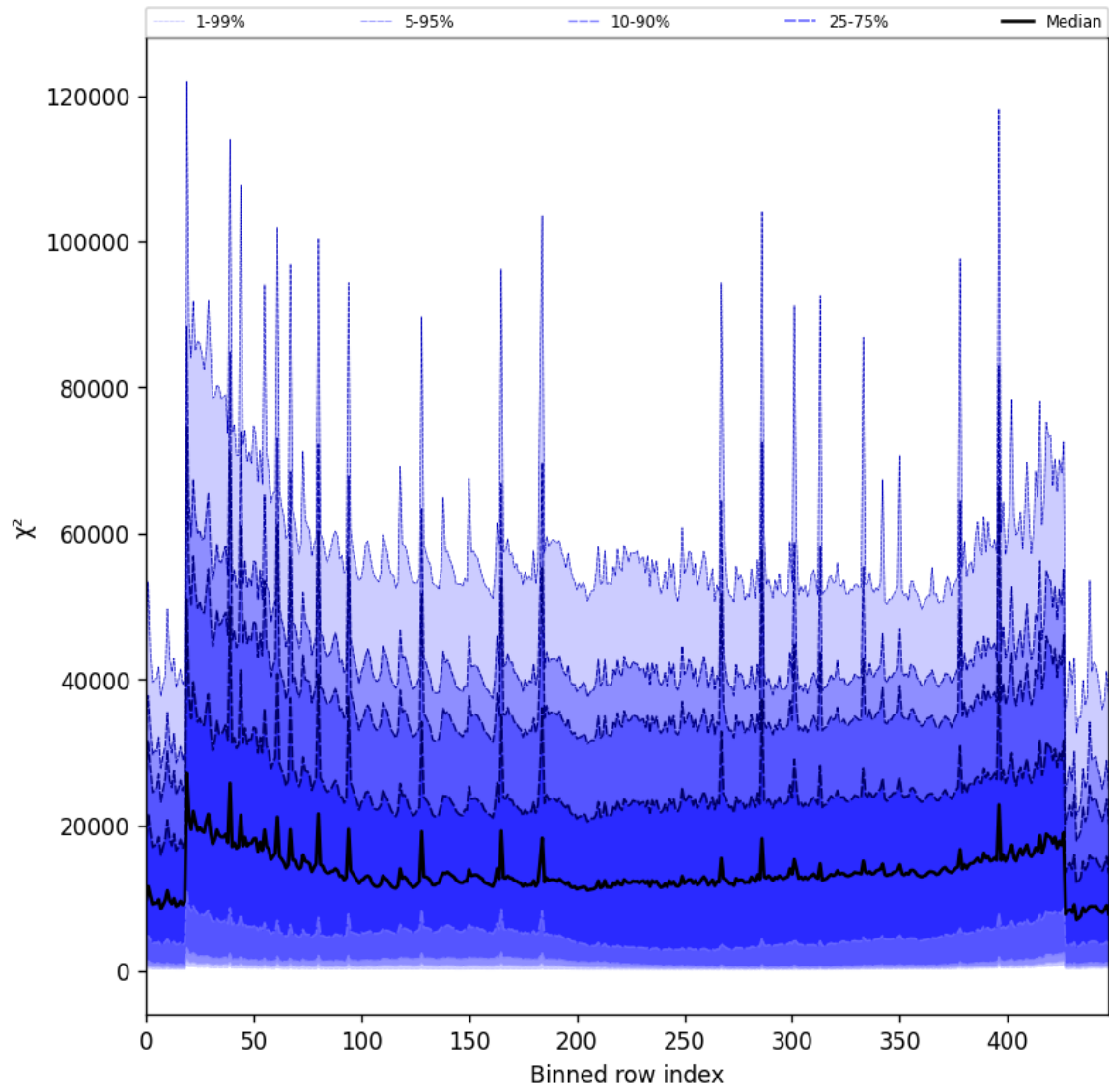
Figure 55: Along track statistics of “ \chi^2 ” for 2025-09-15 to 2025-09-16
