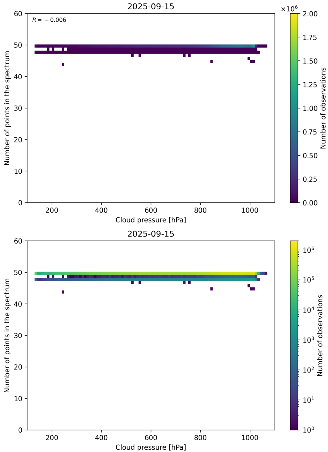
Figure 82: Scatter density plot of “Cloud pressure” against “Number of points in the spectrum” for 2025-09-15 to 2025-09-16.
