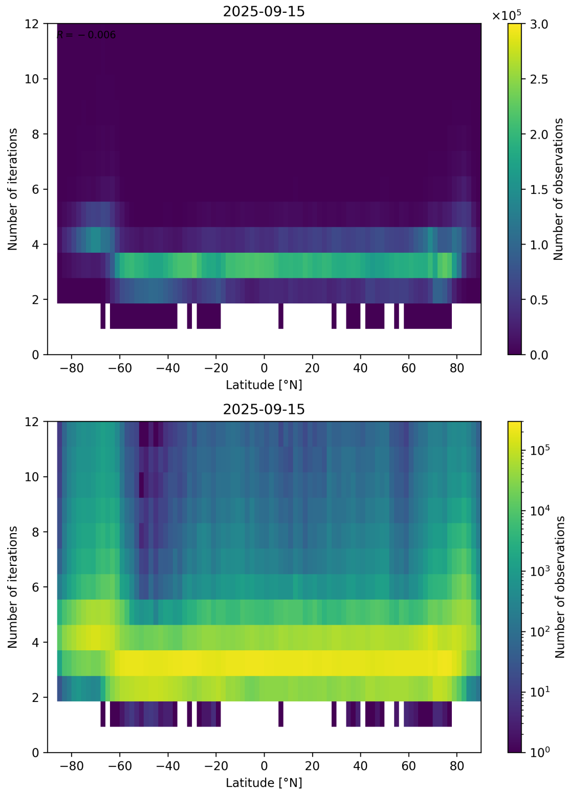
Figure 93: Scatter density plot of “Latitude” against “Number of iterations” for 2025-09-15 to 2025-09-16.
