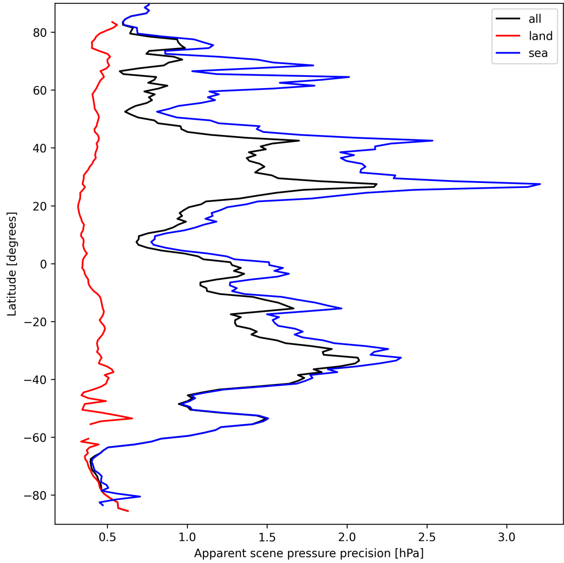
Figure 20: Zonal average of “Apparent scene pressure precision” for 2025-09-15 to 2025-09-16.
