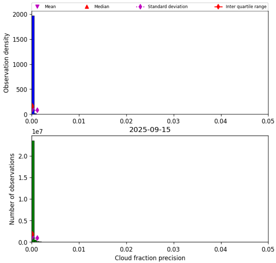
Figure 33: Histogram of “Cloud fraction precision” for 2025-09-15 to 2025-09-16
