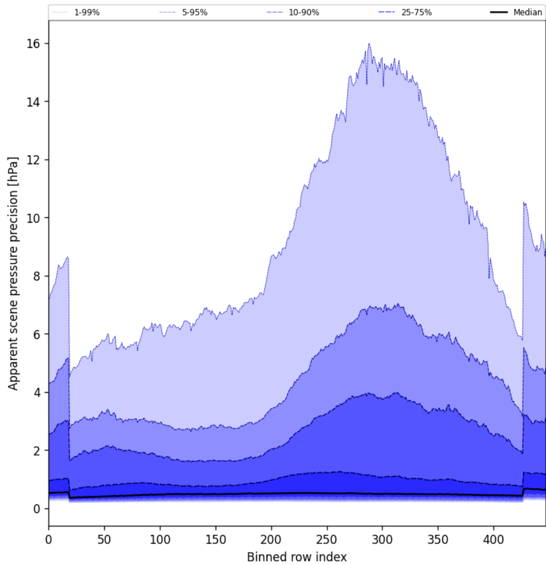
Figure 54: Along track statistics of “Apparent scene pressure precision” for 2025-09-15 to 2025-09-16
