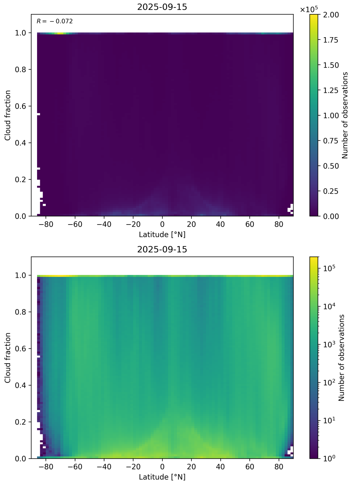
Figure 90: Scatter density plot of “Latitude” against “Cloud fraction” for 2025-09-15 to 2025-09-16.
