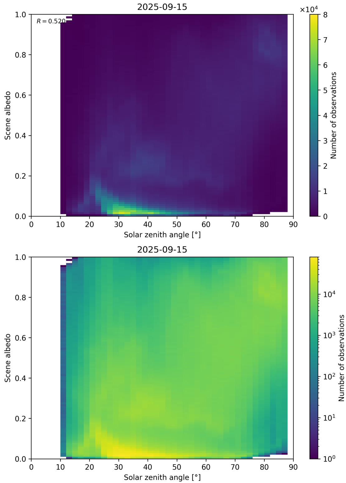
Figure 116: Scatter density plot of “Solar zenith angle” against “Scene albedo” for 2025-09-15 to 2025-09-16.
