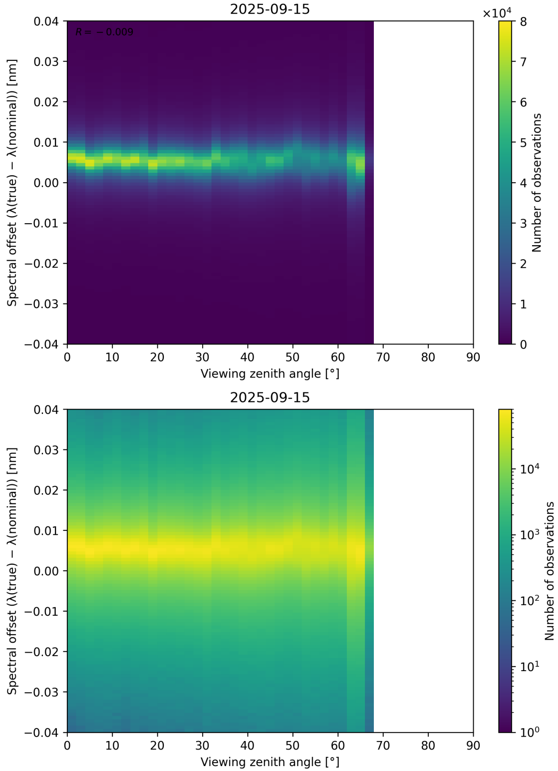
Figure 128: Scatter density plot of “Viewing zenith angle” against “Spectral offset ( \lambda_{\text{true}} - \lambda_{\text{nominal}} )” for 2025-09-15 to 2025-09-16.
