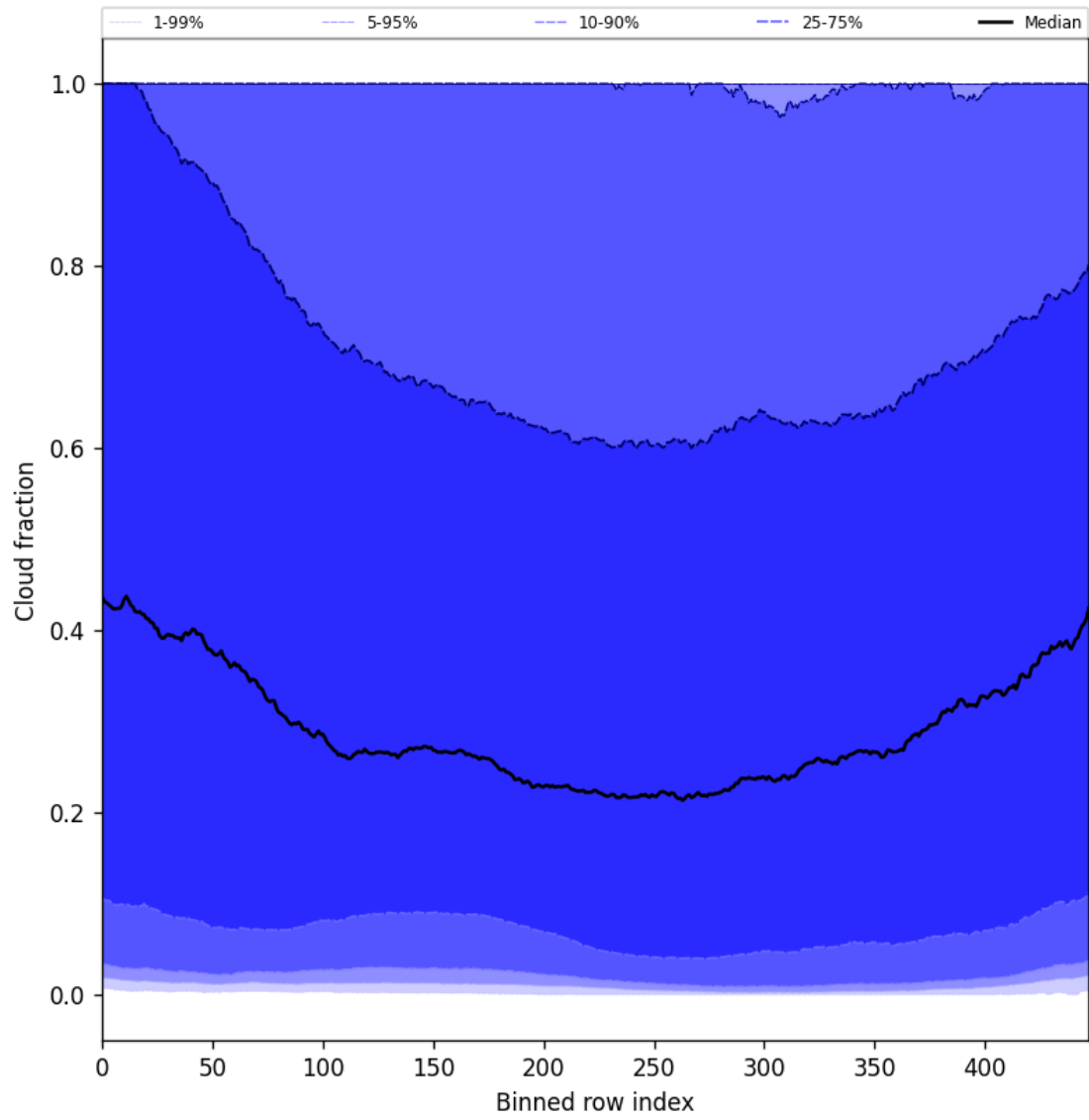
Figure 49: Along track statistics of “Cloud fraction” for 2025-09-15 to 2025-09-16
