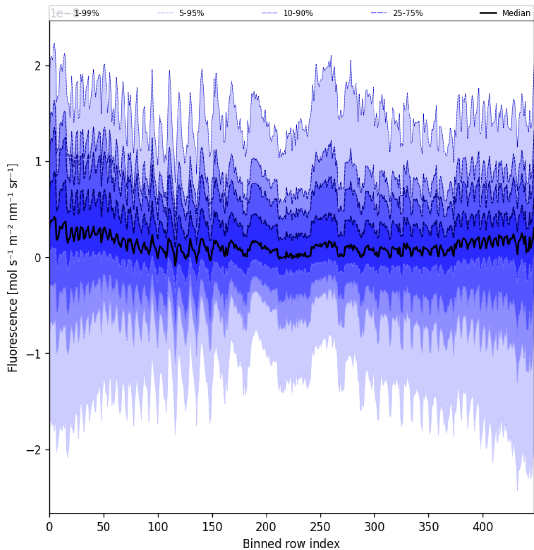
Figure 57: Along track statistics of “Fluorescence” for 2025-09-15 to 2025-09-16
