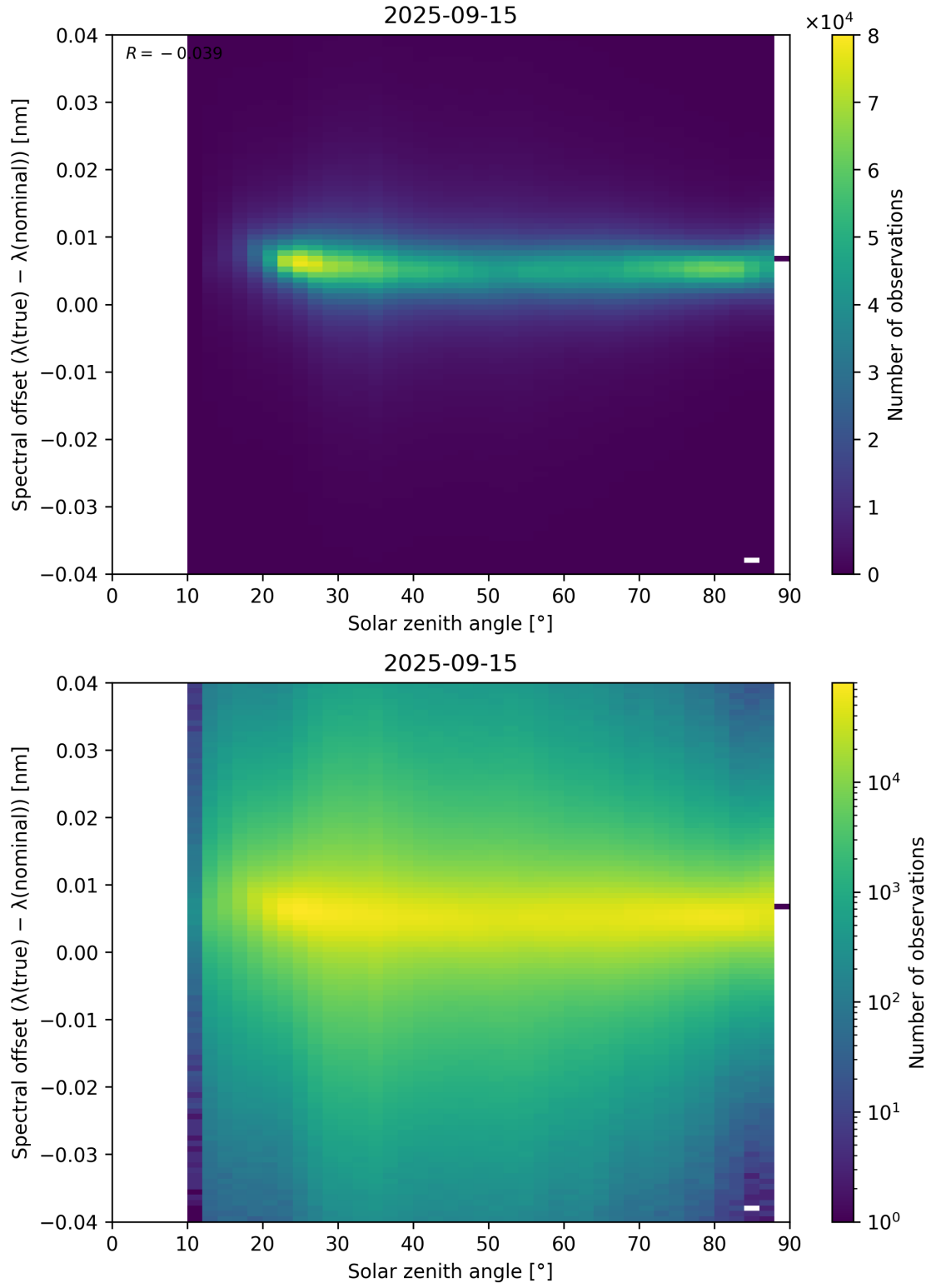
Figure 117: Scatter density plot of “Solar zenith angle” against “Spectral offset ( \lambda_{\text{true}} - \lambda_{\text{nominal}} )” for 2025-09-15 to 2025-09-16.
