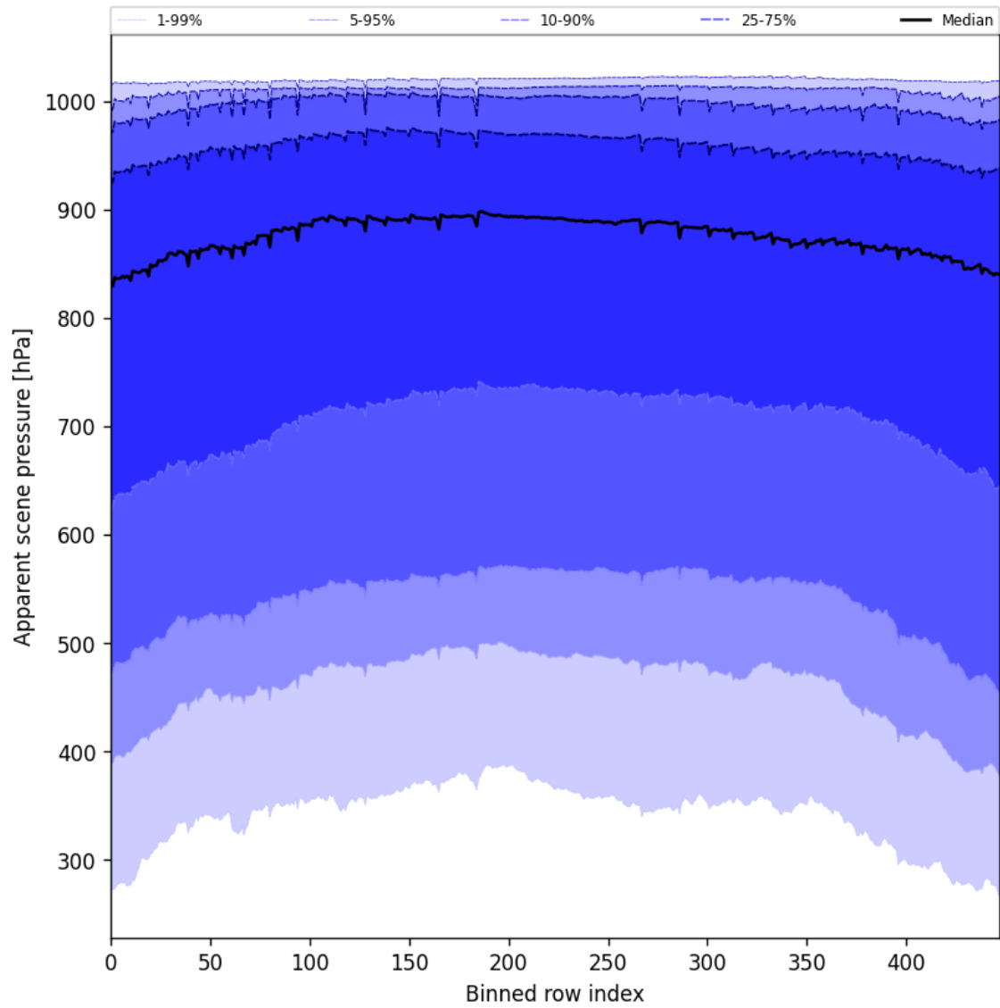
Figure 53: Along track statistics of “Apparent scene pressure” for 2025-09-15 to 2025-09-16
