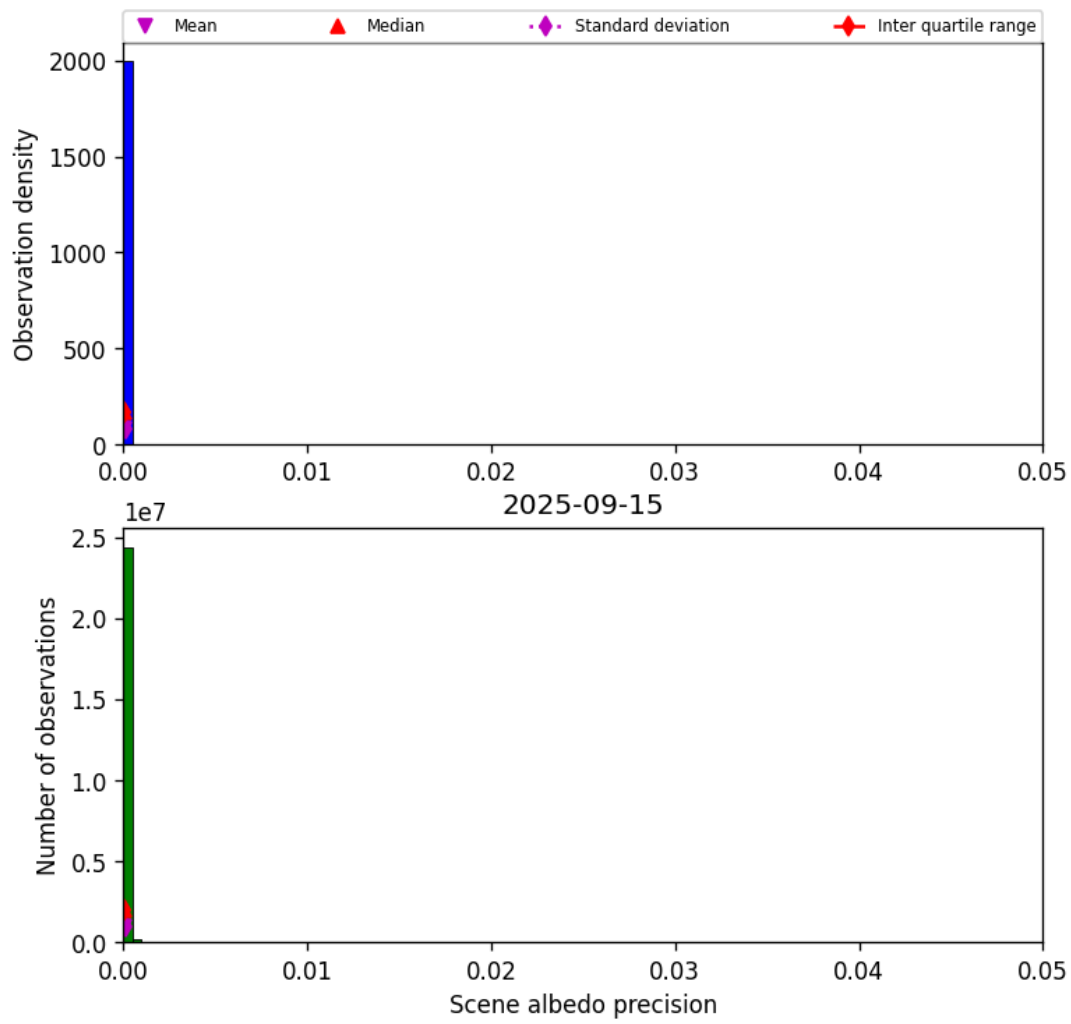
Figure 35: Histogram of “Scene albedo precision” for 2025-09-15 to 2025-09-16
