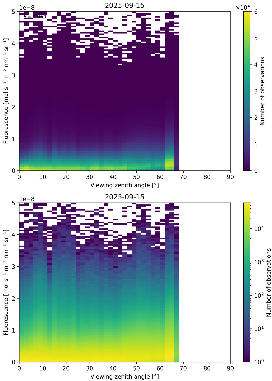
Figure 122: Scatter density plot of "Viewing zenith angle" against "Fluorescence" for 2025-09-15 to 2025-09-16.
