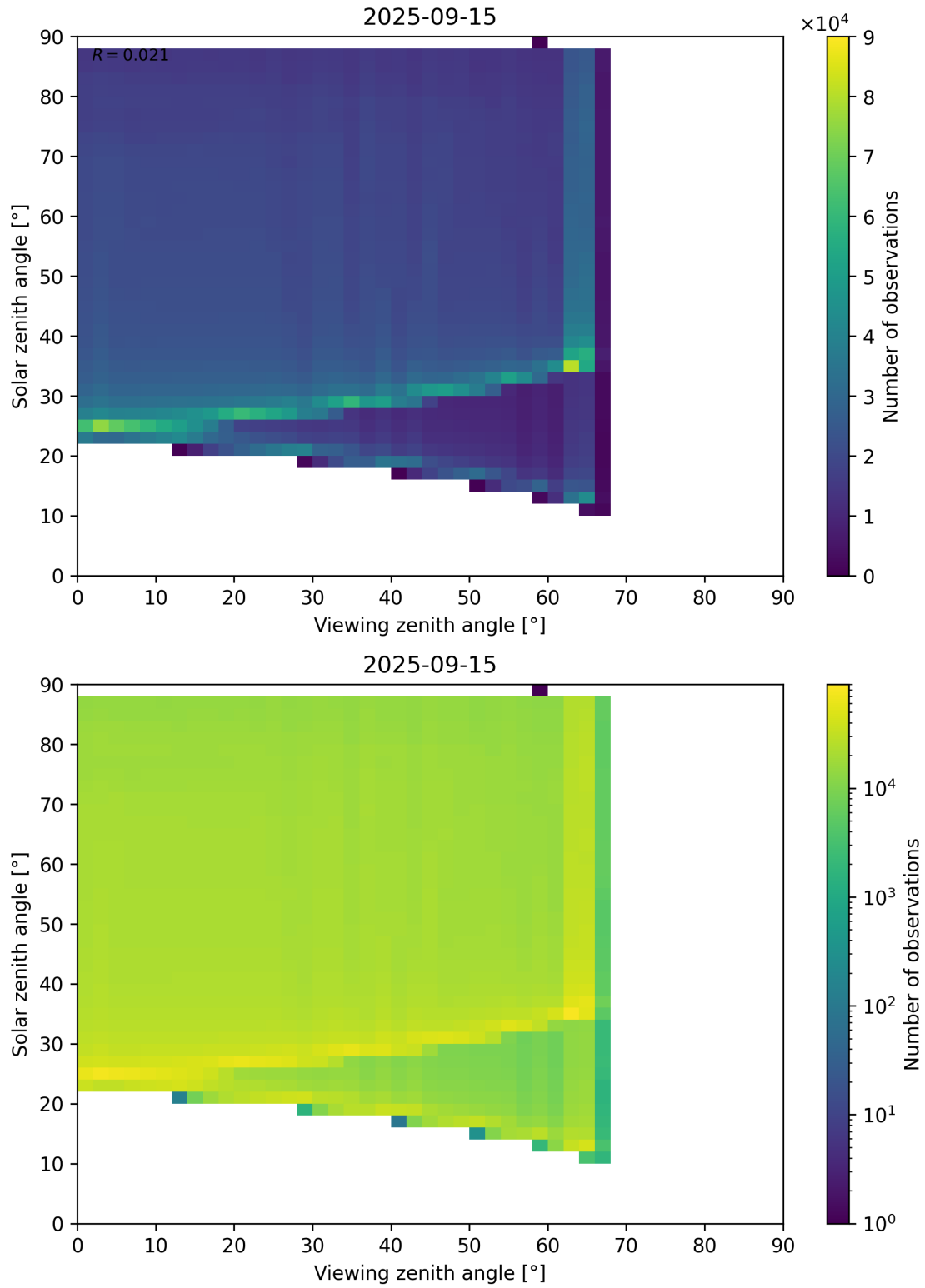
Figure 127: Scatter density plot of “Viewing zenith angle” against “Solar zenith angle” for 2025-09-15 to 2025-09-16.
