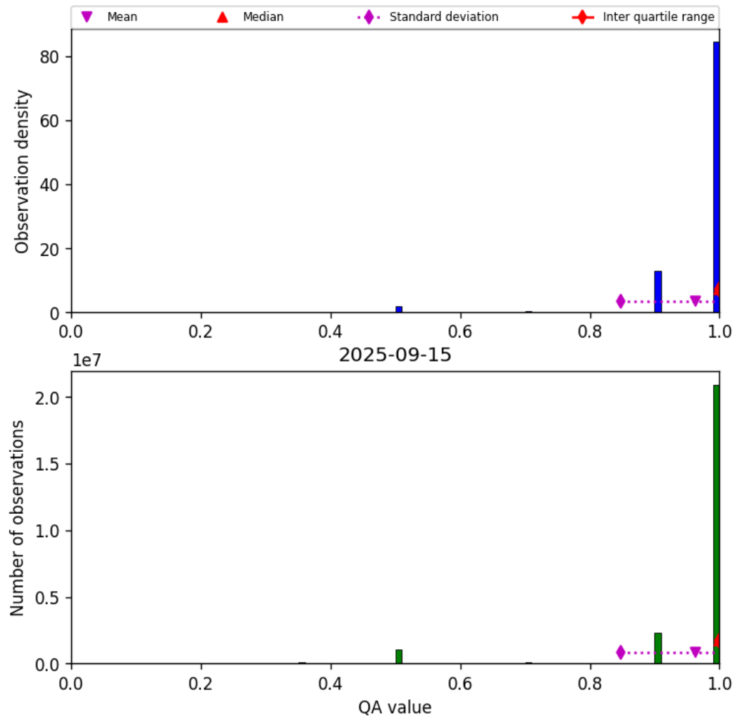
Figure 29: Histogram of “QA value” for 2025-09-15 to 2025-09-16
