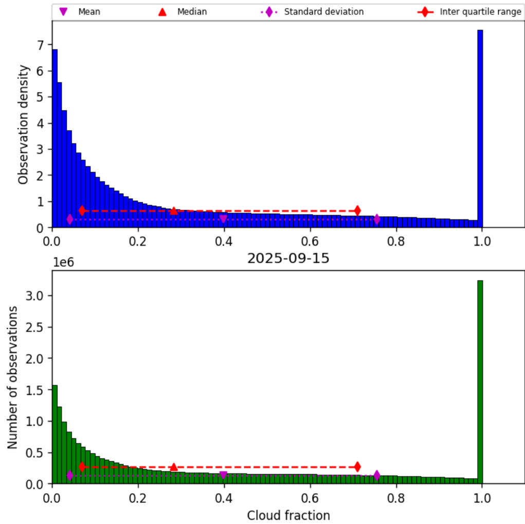
Figure 32: Histogram of “Cloud fraction” for 2025-09-15 to 2025-09-16
