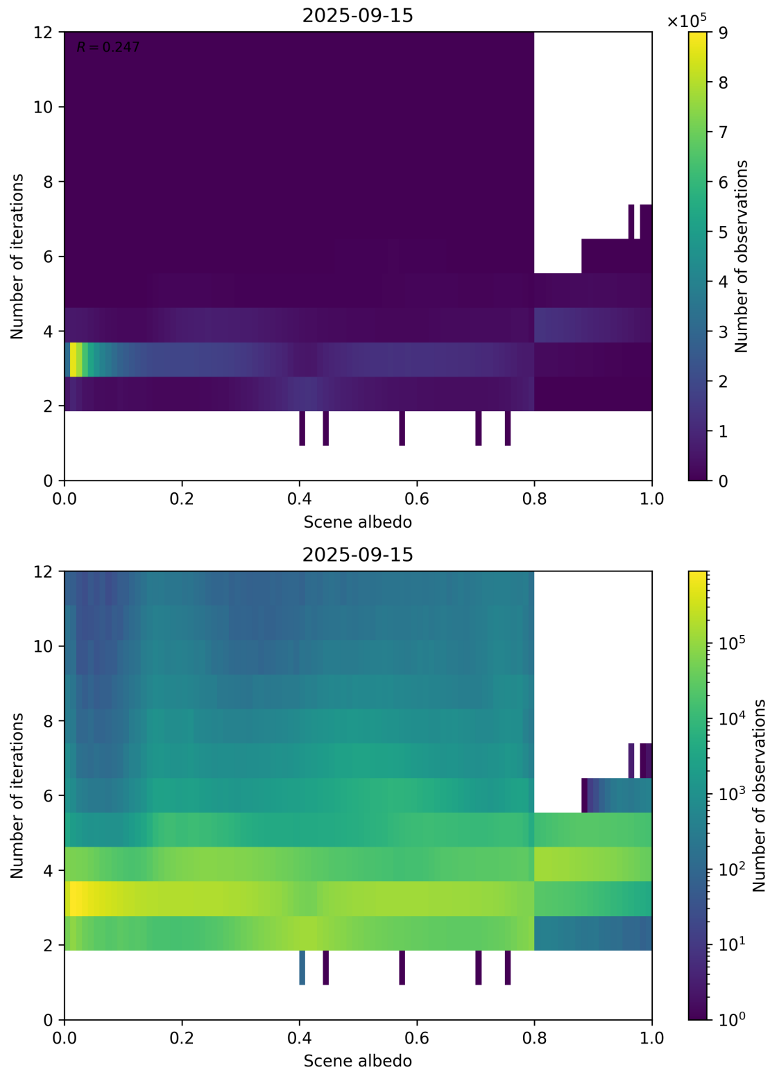
Figure 105: Scatter density plot of “Scene albedo” against “Number of iterations” for 2025-09-15 to 2025-09-16.
