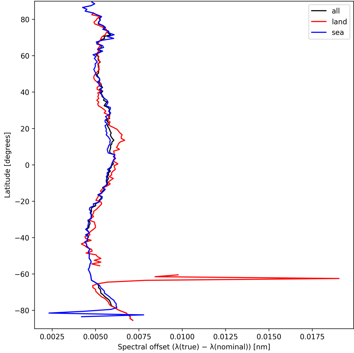
Figure 28: Zonal average of “Spectral offset ( \lambda_{\text{true}} - \lambda_{\text{nominal}} )” for 2025-09-15 to 2025-09-16.
