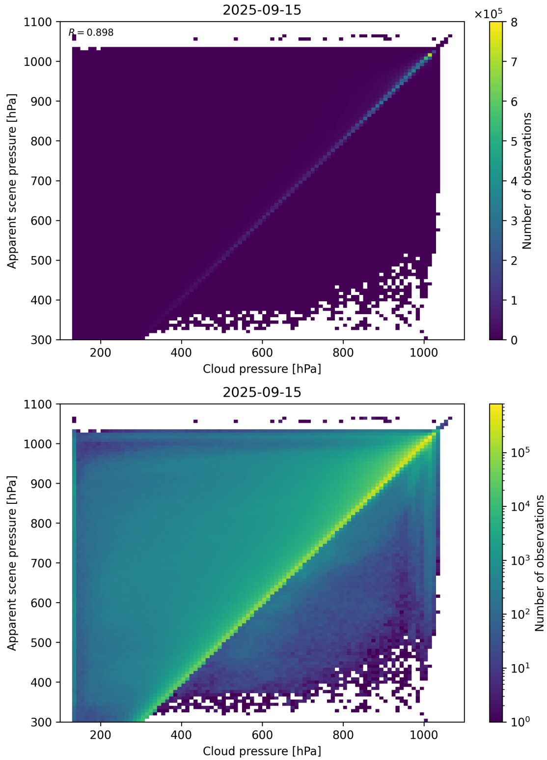
Figure 77: Scatter density plot of “Cloud pressure” against “Apparent scene pressure” for 2025-09-15 to 2025-09-16.
