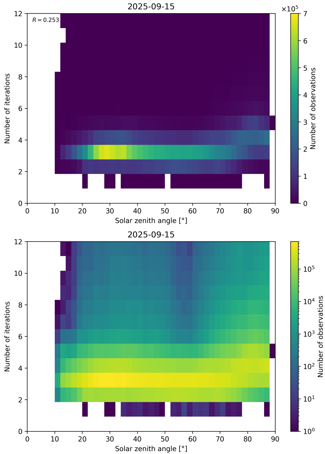
Figure 114: Scatter density plot of “Solar zenith angle” against “Number of iterations” for 2025-09-15 to 2025-09-16.
