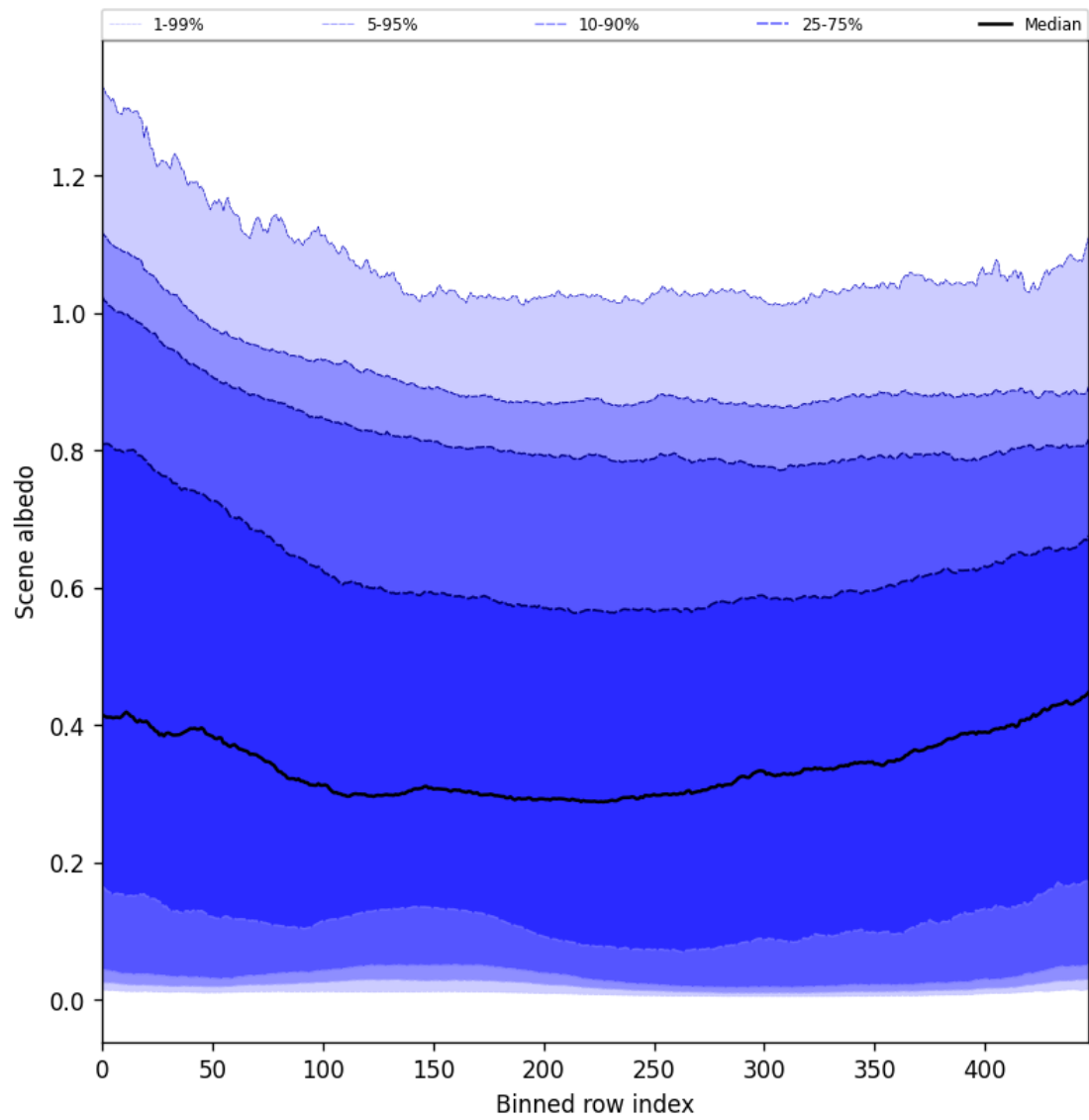
Figure 51: Along track statistics of “Scene albedo” for 2025-09-15 to 2025-09-16
