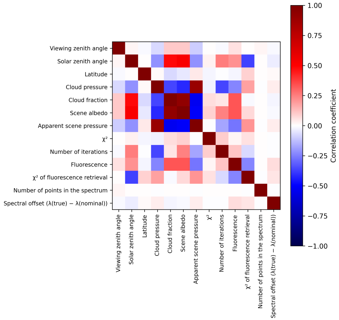
Figure 2: Map of correlation matrix for 2025-09-15 to 2025-09-16.
