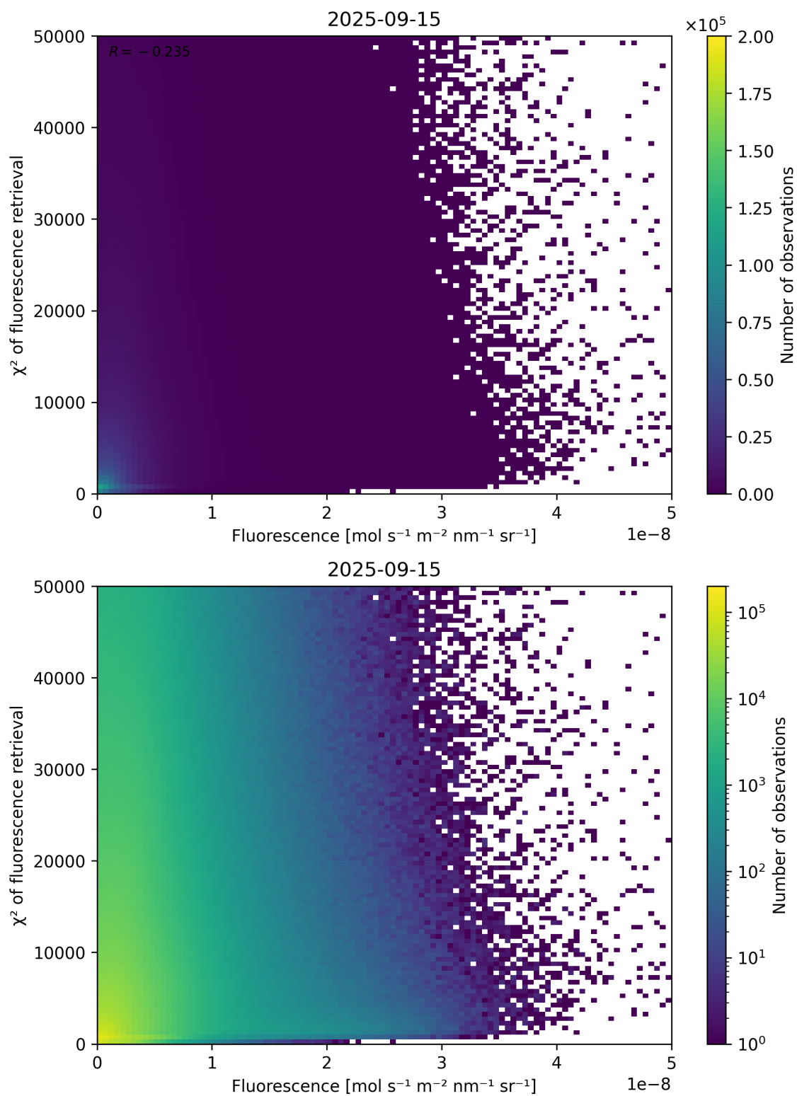
Figure 85: Scatter density plot of “Fluorescence” against “ \chi^2 of fluorescence retrieval” for 2025-09-15 to 2025-09-16.
