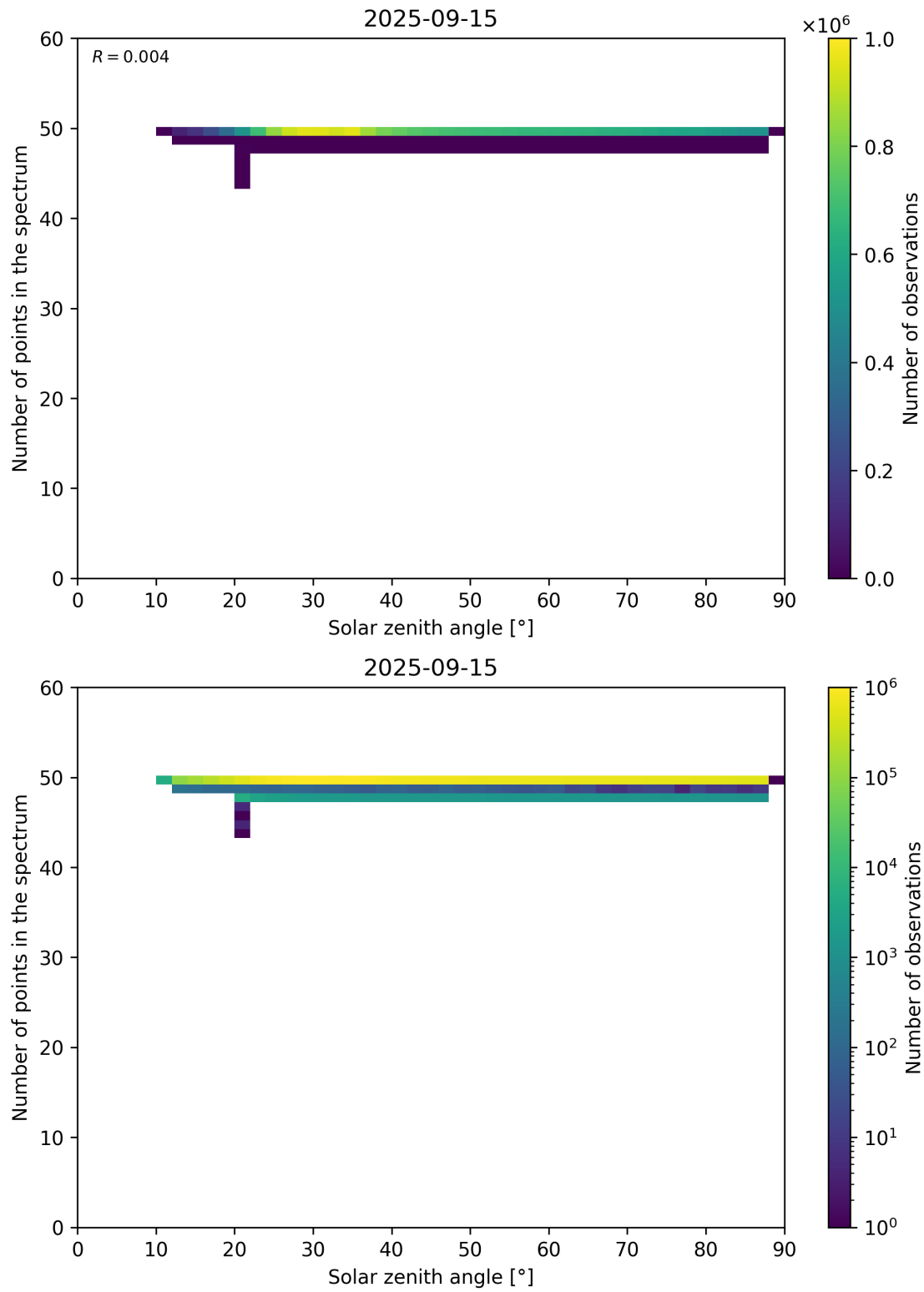
Figure 115: Scatter density plot of “Solar zenith angle” against “Number of points in the spectrum” for 2025-09-15 to 2025-09-16.
