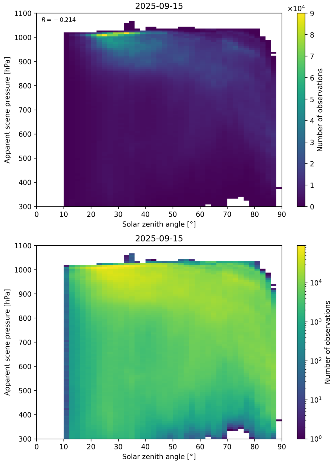
Figure 108: Scatter density plot of “Solar zenith angle” against “Apparent scene pressure” for 2025-09-15 to 2025-09-16.
