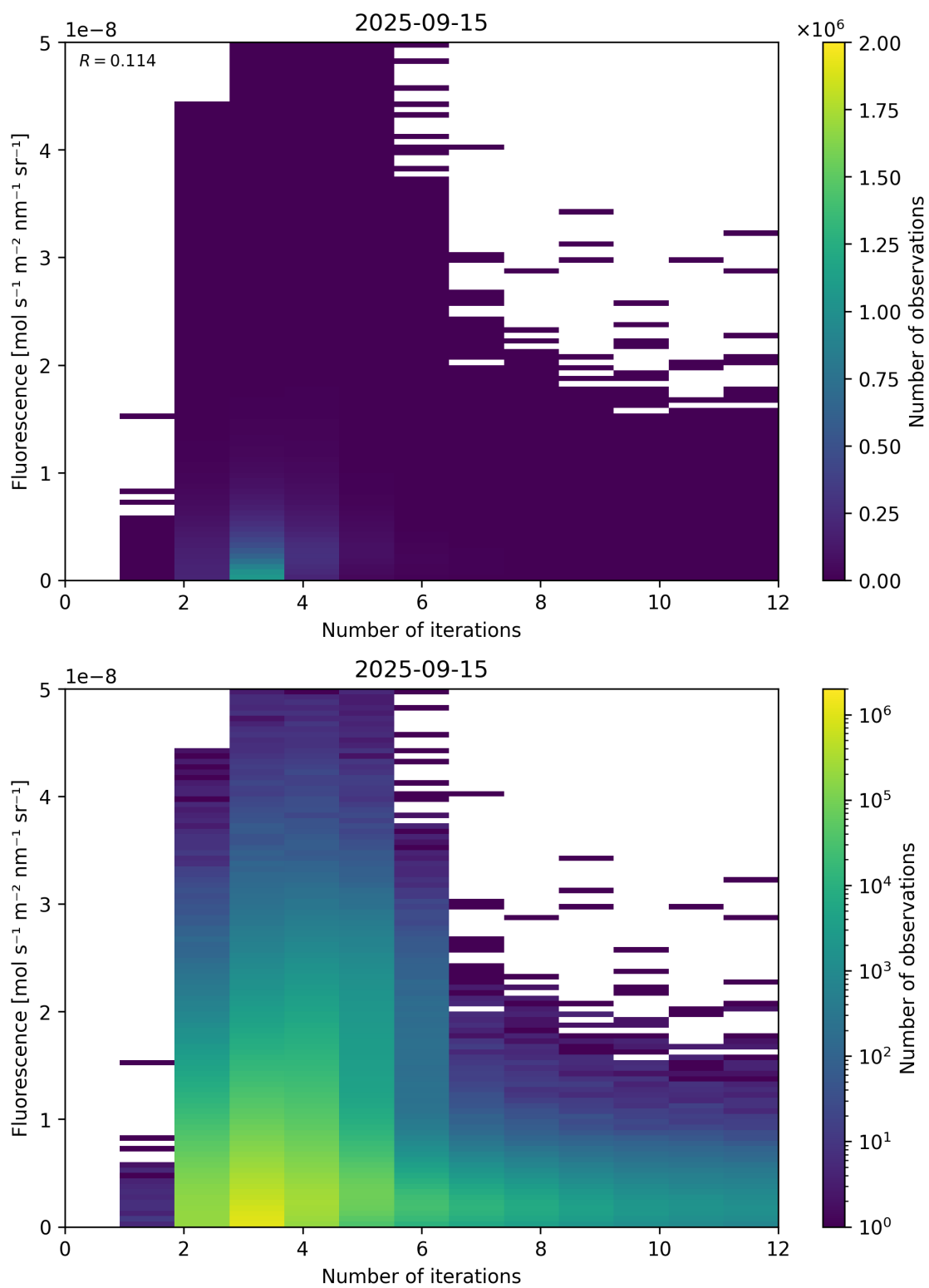
Figure 98: Scatter density plot of “Number of iterations” against “Fluorescence” for 2025-09-15 to 2025-09-16.
