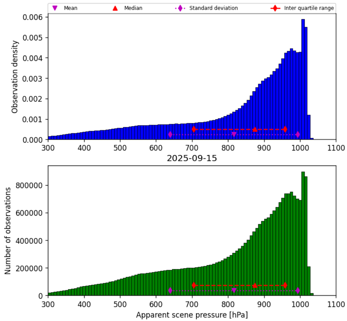
Figure 36: Histogram of “Apparent scene pressure” for 2025-09-15 to 2025-09-16
