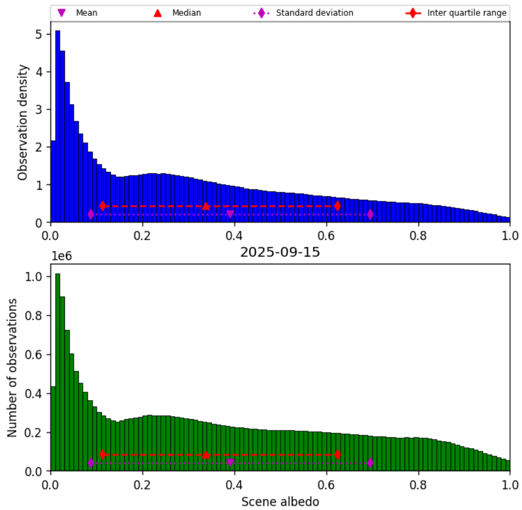
Figure 34: Histogram of “Scene albedo” for 2025-09-15 to 2025-09-16
