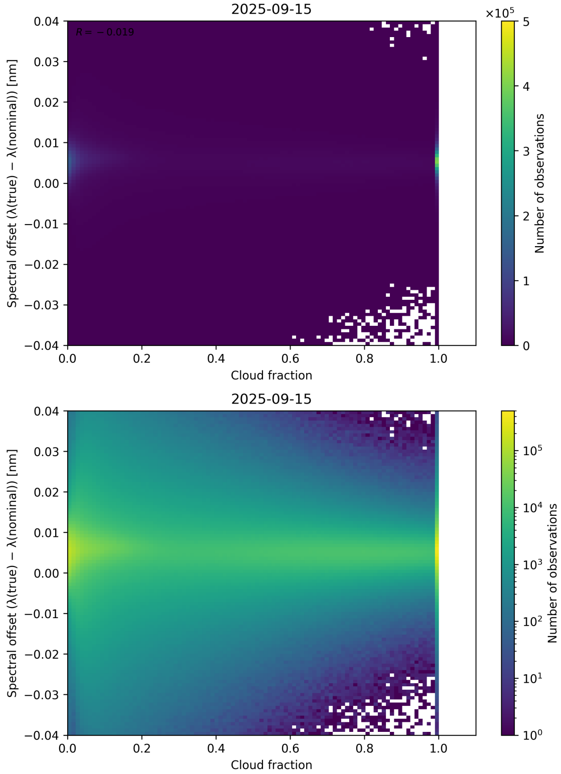
Figure 76: Scatter density plot of “Cloud fraction” against “Spectral offset ( \lambda_{\text{true}} - \lambda_{\text{nominal}} )” for 2025-09-15 to 2025-09-16.
