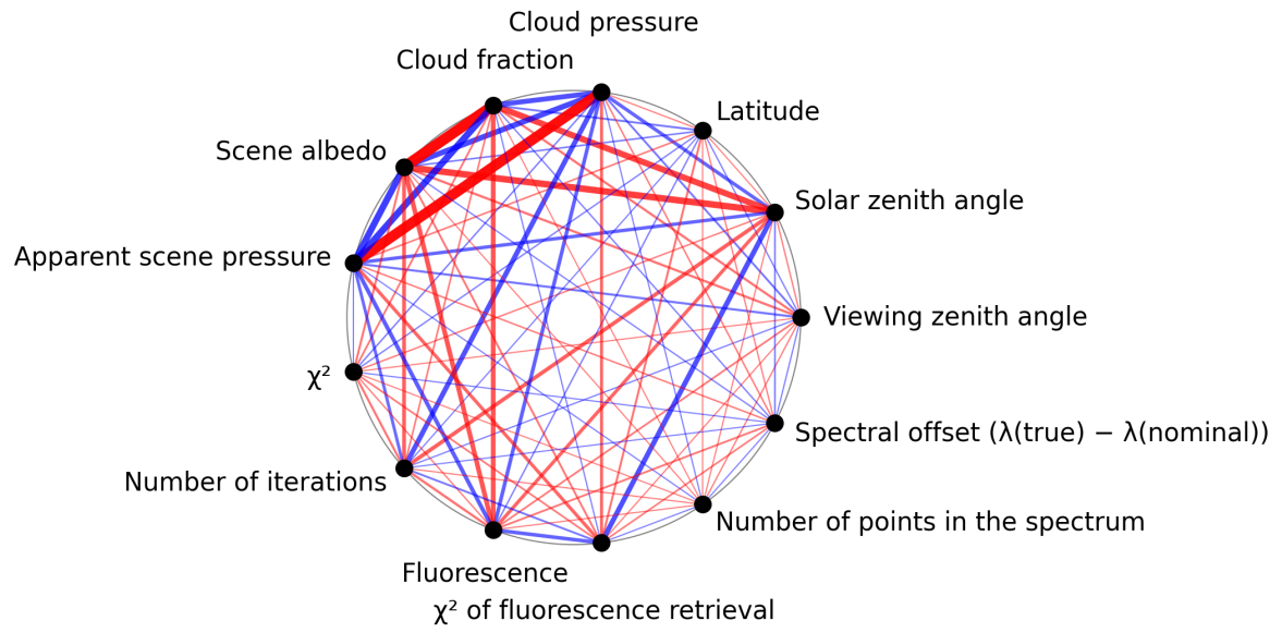
Figure 1: Map of correlation graph for 2025-09-15 to 2025-09-16.
