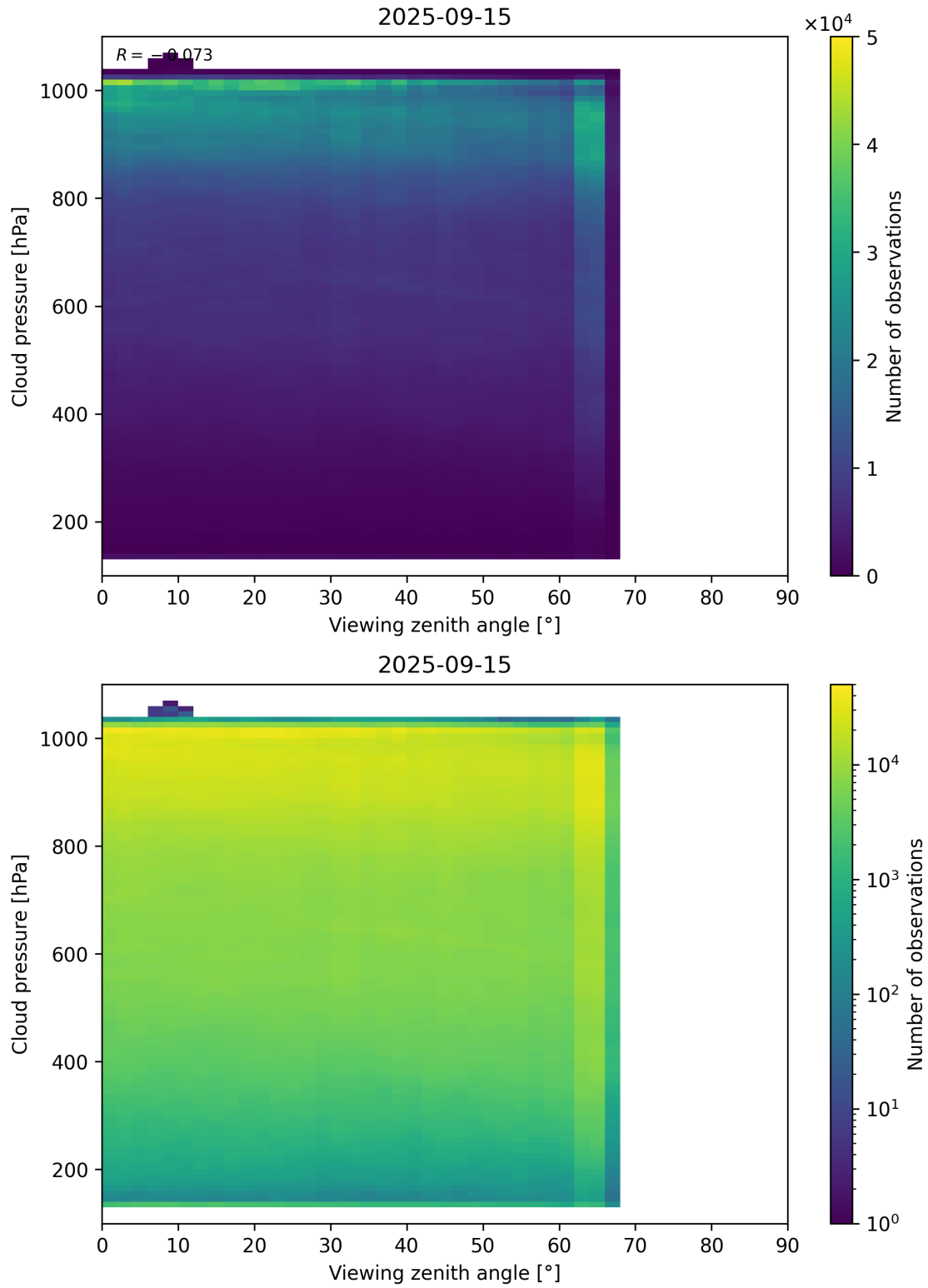
Figure 121: Scatter density plot of “Viewing zenith angle” against “Cloud pressure” for 2025-09-15 to 2025-09-16.
