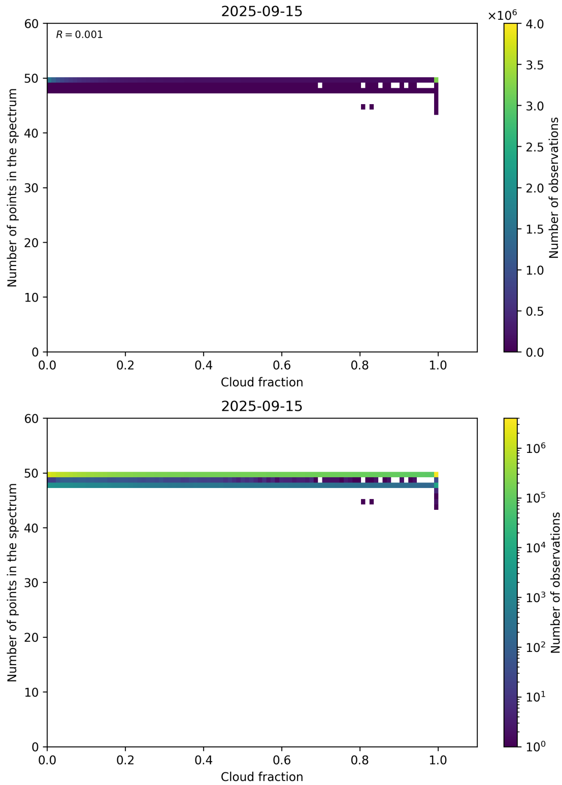
Figure 74: Scatter density plot of “Cloud fraction” against “Number of points in the spectrum” for 2025-09-15 to 2025-09-16.
