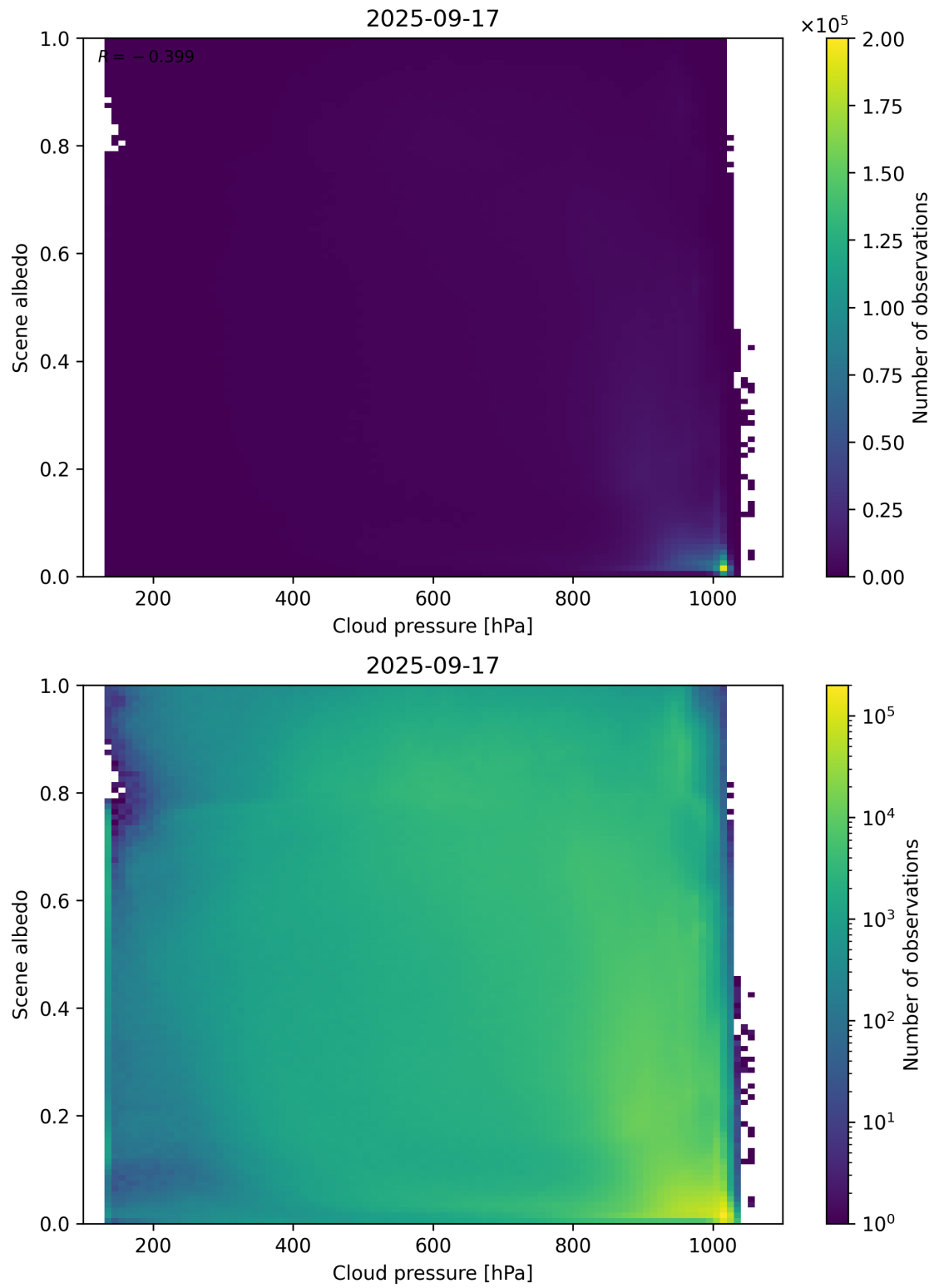
Figure 83: Scatter density plot of “Cloud pressure” against “Scene albedo” for 2025-09-16 to 2025-09-18.
