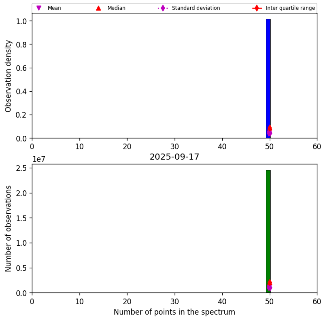
Figure 44: Histogram of “Number of points in the spectrum” for 2025-09-16 to 2025-09-18
