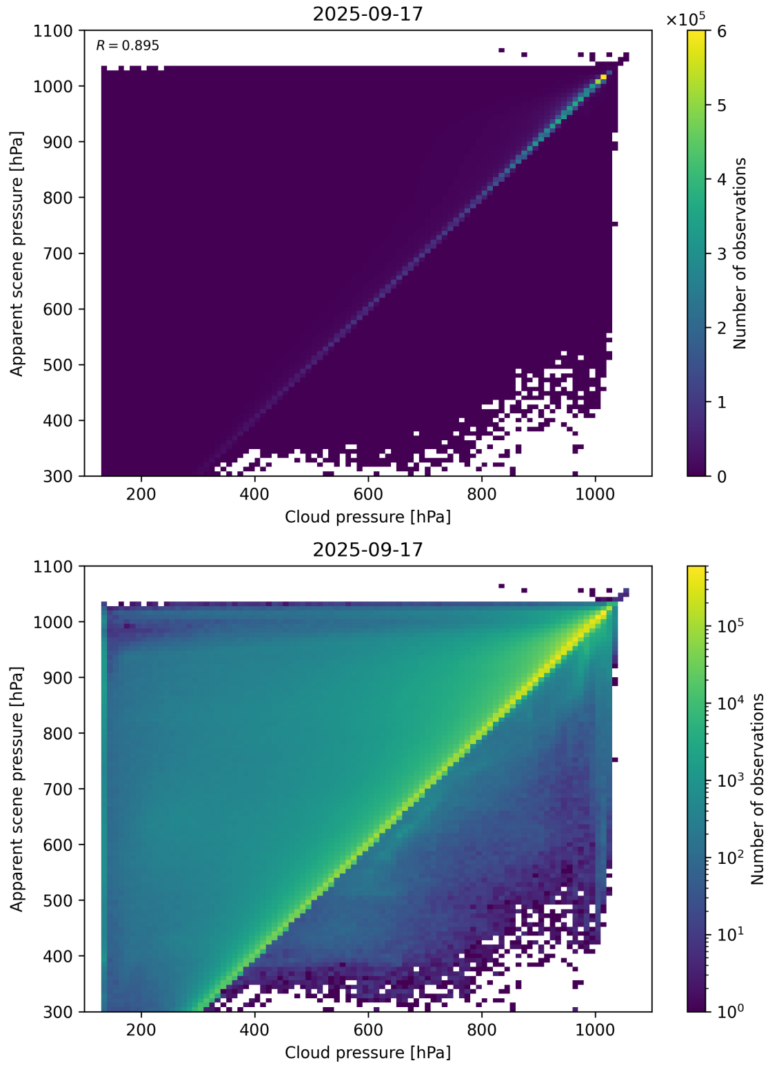
Figure 77: Scatter density plot of “Cloud pressure” against “Apparent scene pressure” for 2025-09-16 to 2025-09-18.
