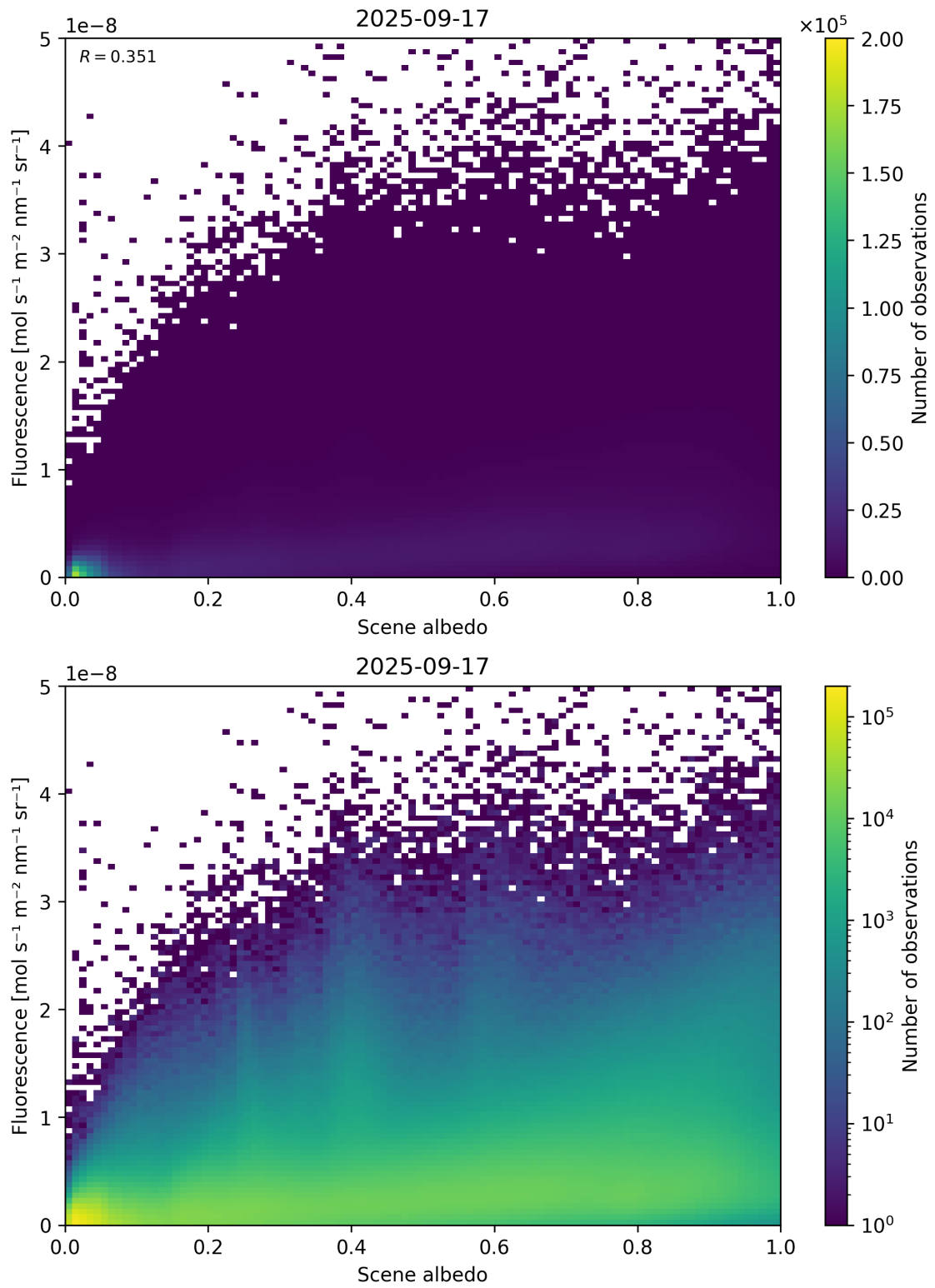
Figure 104: Scatter density plot of “Scene albedo” against “Fluorescence” for 2025-09-16 to 2025-09-18.
