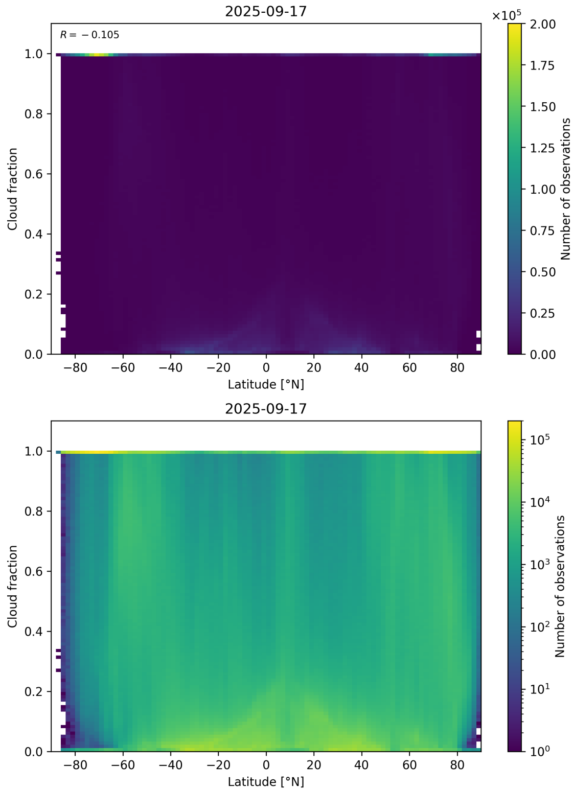
Figure 90: Scatter density plot of “Latitude” against “Cloud fraction” for 2025-09-16 to 2025-09-18.
