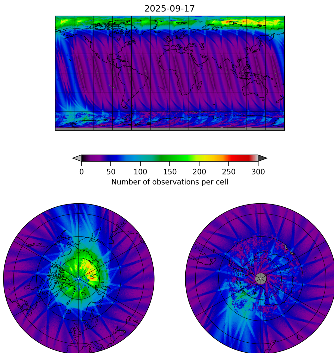
Figure 11: Map of the number of observations for 2025-09-16 to 2025-09-18
