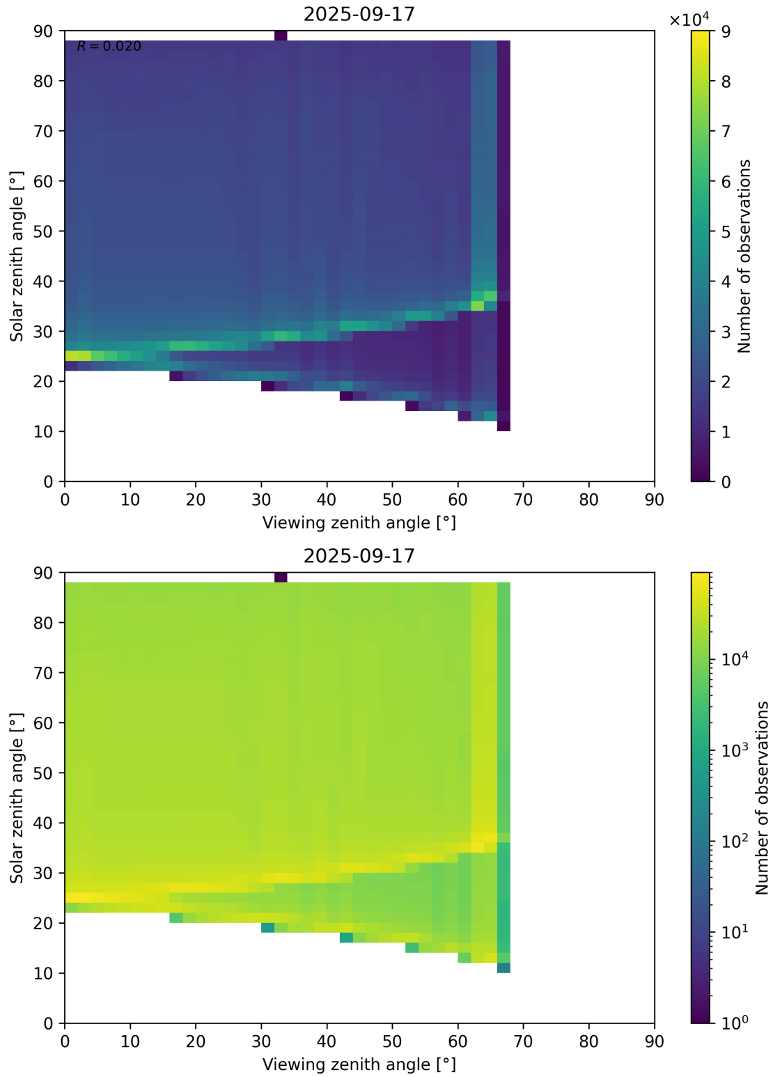
Figure 127: Scatter density plot of “Viewing zenith angle” against “Solar zenith angle” for 2025-09-16 to 2025-09-18.
