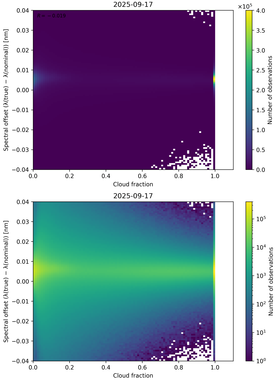
Figure 76: Scatter density plot of “Cloud fraction” against “Spectral offset ( \lambda_{\text{true}} - \lambda_{\text{nominal}} )” for 2025-09-16 to 2025-09-18.
