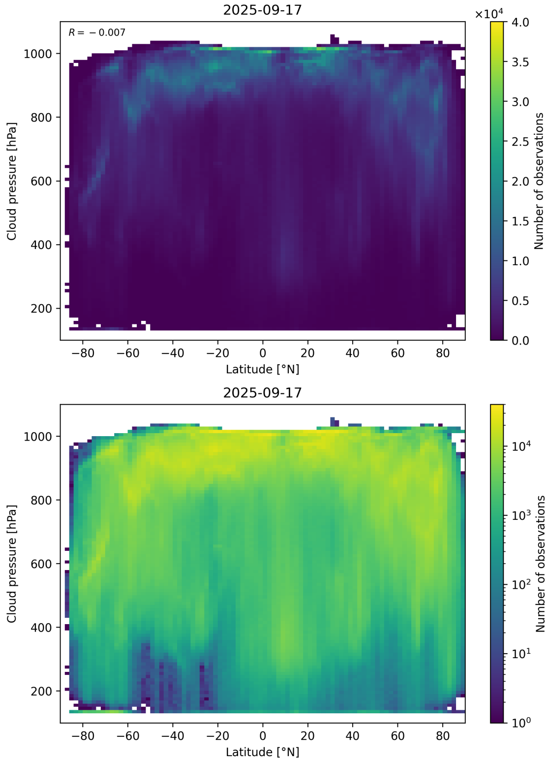
Figure 91: Scatter density plot of “Latitude” against “Cloud pressure” for 2025-09-16 to 2025-09-18.
