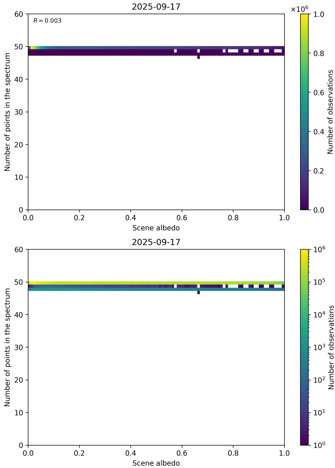
Figure 106: Scatter density plot of “Scene albedo” against “Number of points in the spectrum” for 2025-09-16 to 2025-09-18.
