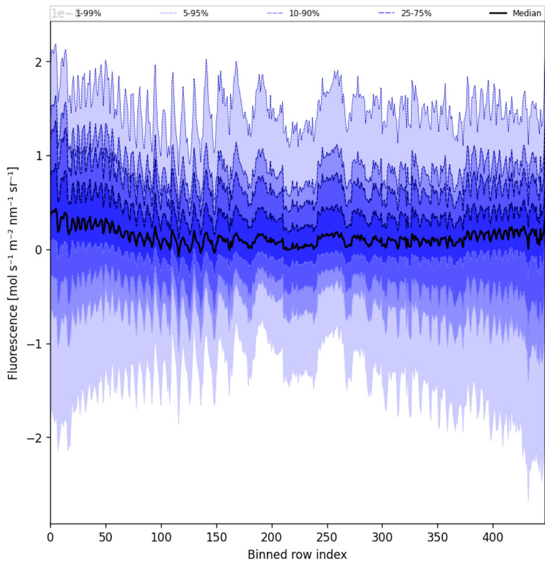
Figure 57: Along track statistics of “Fluorescence” for 2025-09-16 to 2025-09-18
