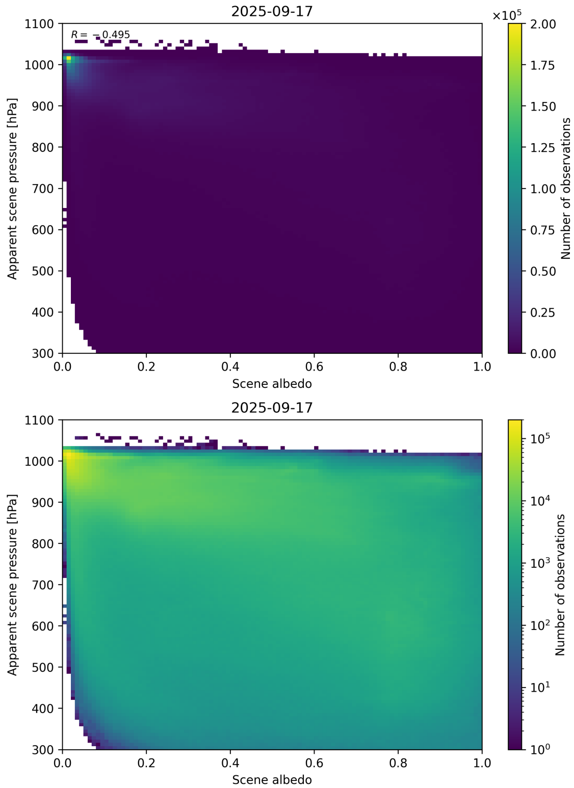
Figure 102: Scatter density plot of “Scene albedo” against “Apparent scene pressure” for 2025-09-16 to 2025-09-18.
