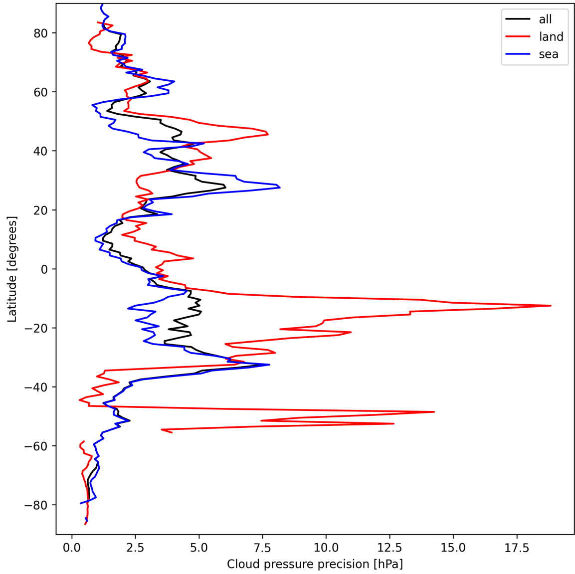
Figure 14: Zonal average of “Cloud pressure precision” for 2025-09-16 to 2025-09-18.
