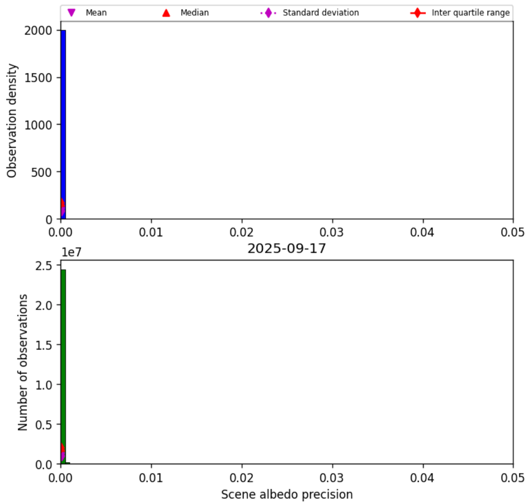
Figure 35: Histogram of “Scene albedo precision” for 2025-09-16 to 2025-09-18
