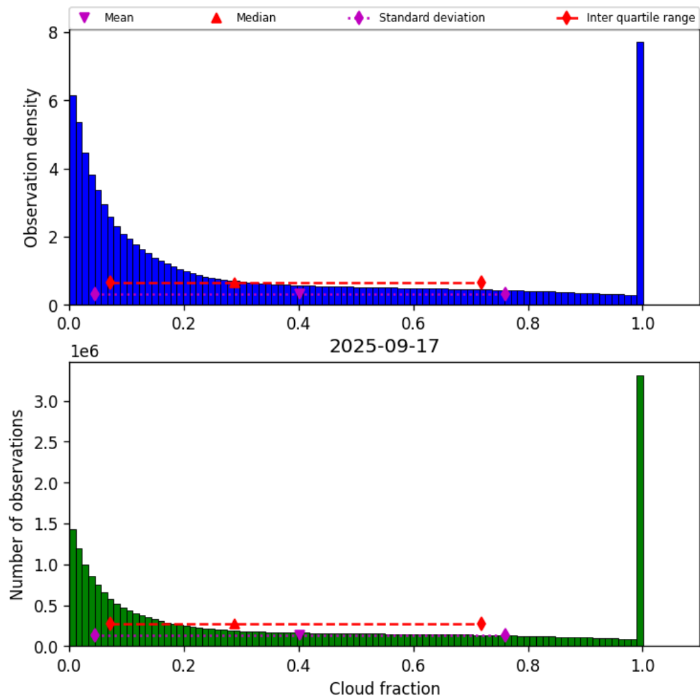
Figure 32: Histogram of “Cloud fraction” for 2025-09-16 to 2025-09-18
