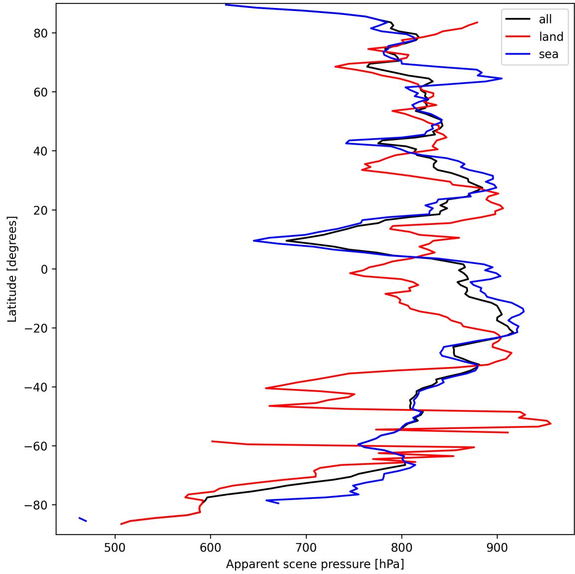
Figure 19: Zonal average of “Apparent scene pressure” for 2025-09-16 to 2025-09-18.
