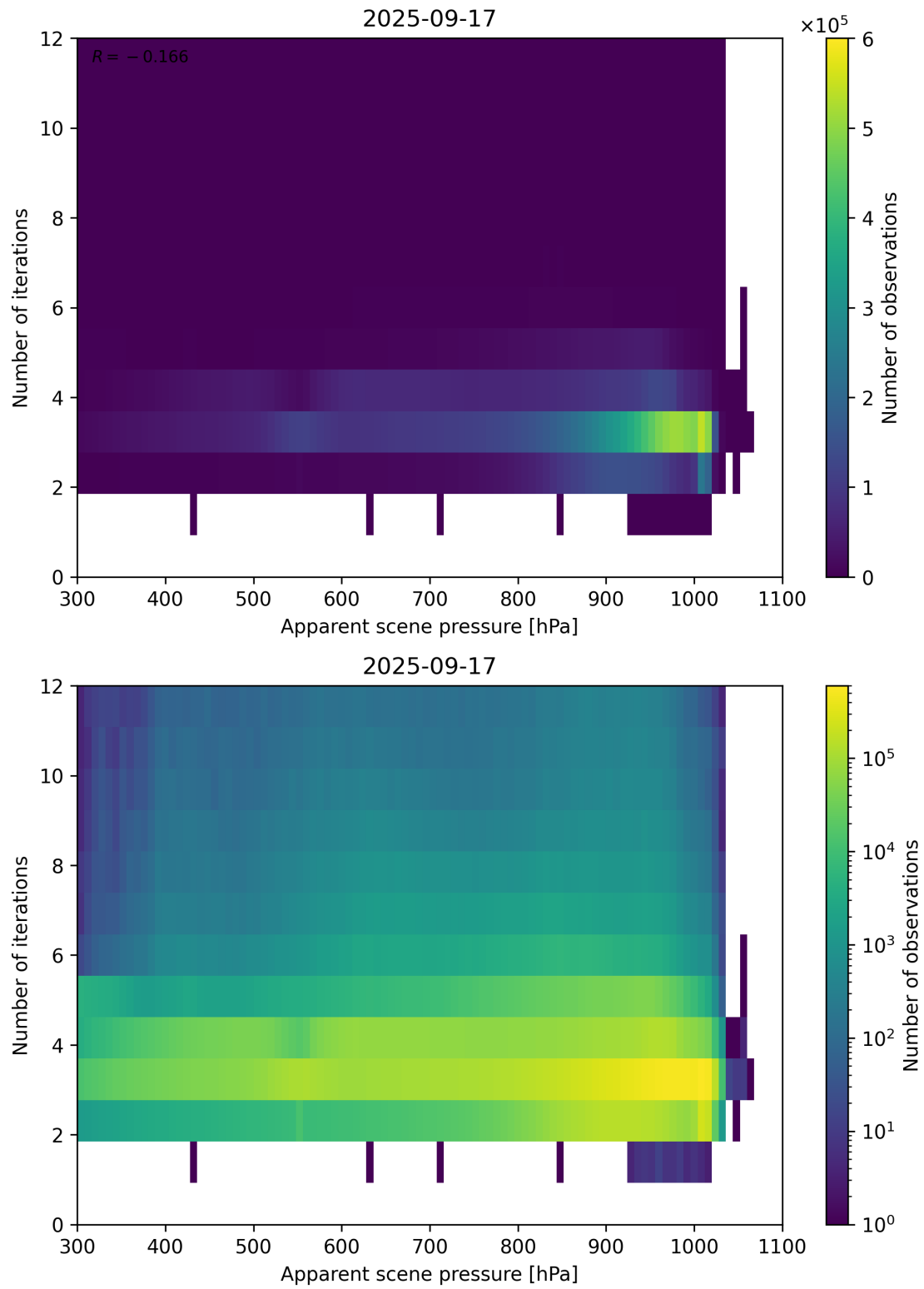
Figure 65: Scatter density plot of “Apparent scene pressure” against “Number of iterations” for 2025-09-16 to 2025-09-18.
