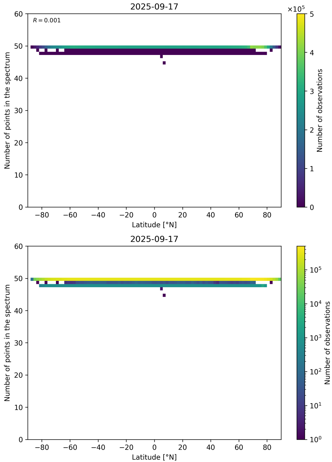
Figure 94: Scatter density plot of “Latitude” against “Number of points in the spectrum” for 2025-09-16 to 2025-09-18.
