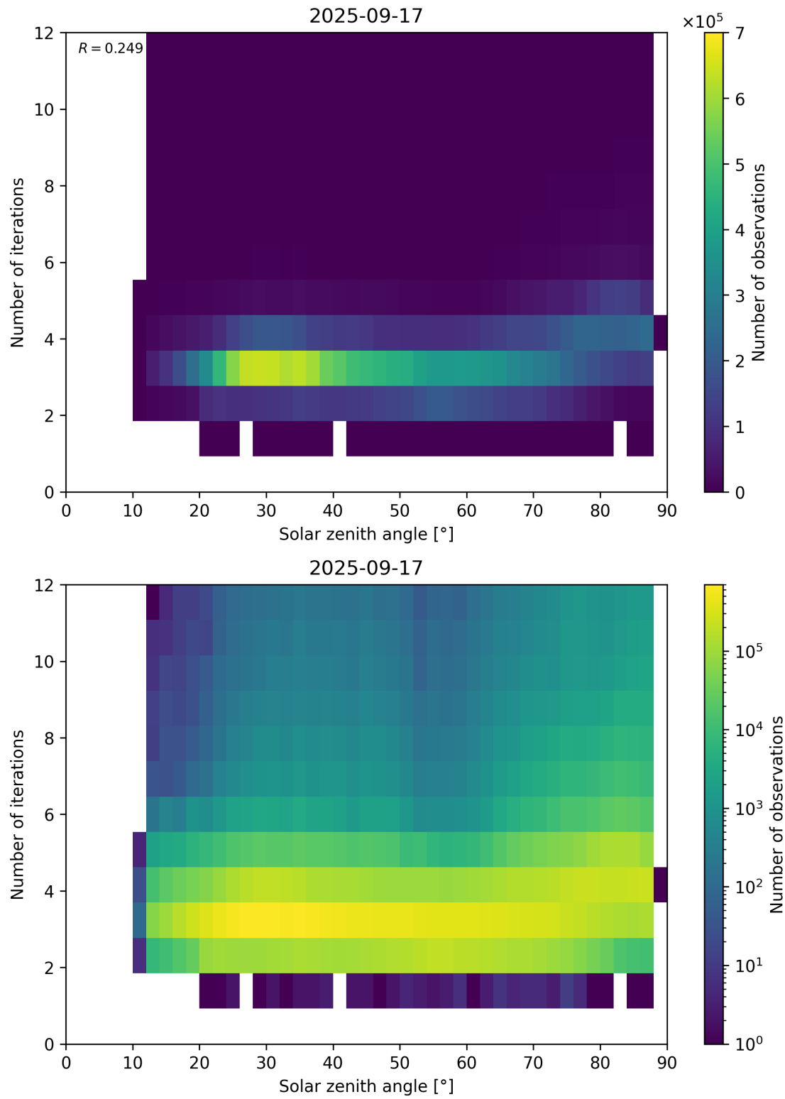
Figure 114: Scatter density plot of “Solar zenith angle” against “Number of iterations” for 2025-09-16 to 2025-09-18.
