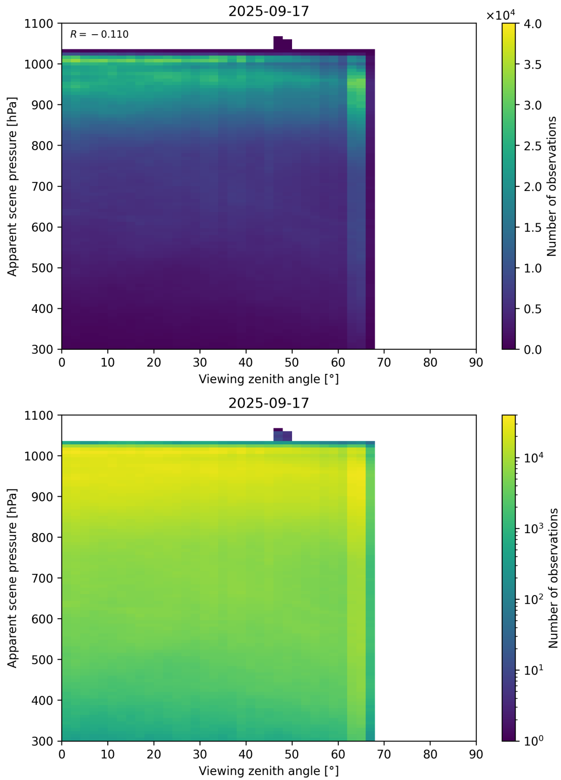
Figure 118: Scatter density plot of “Viewing zenith angle” against “Apparent scene pressure” for 2025-09-16 to 2025-09-18.
