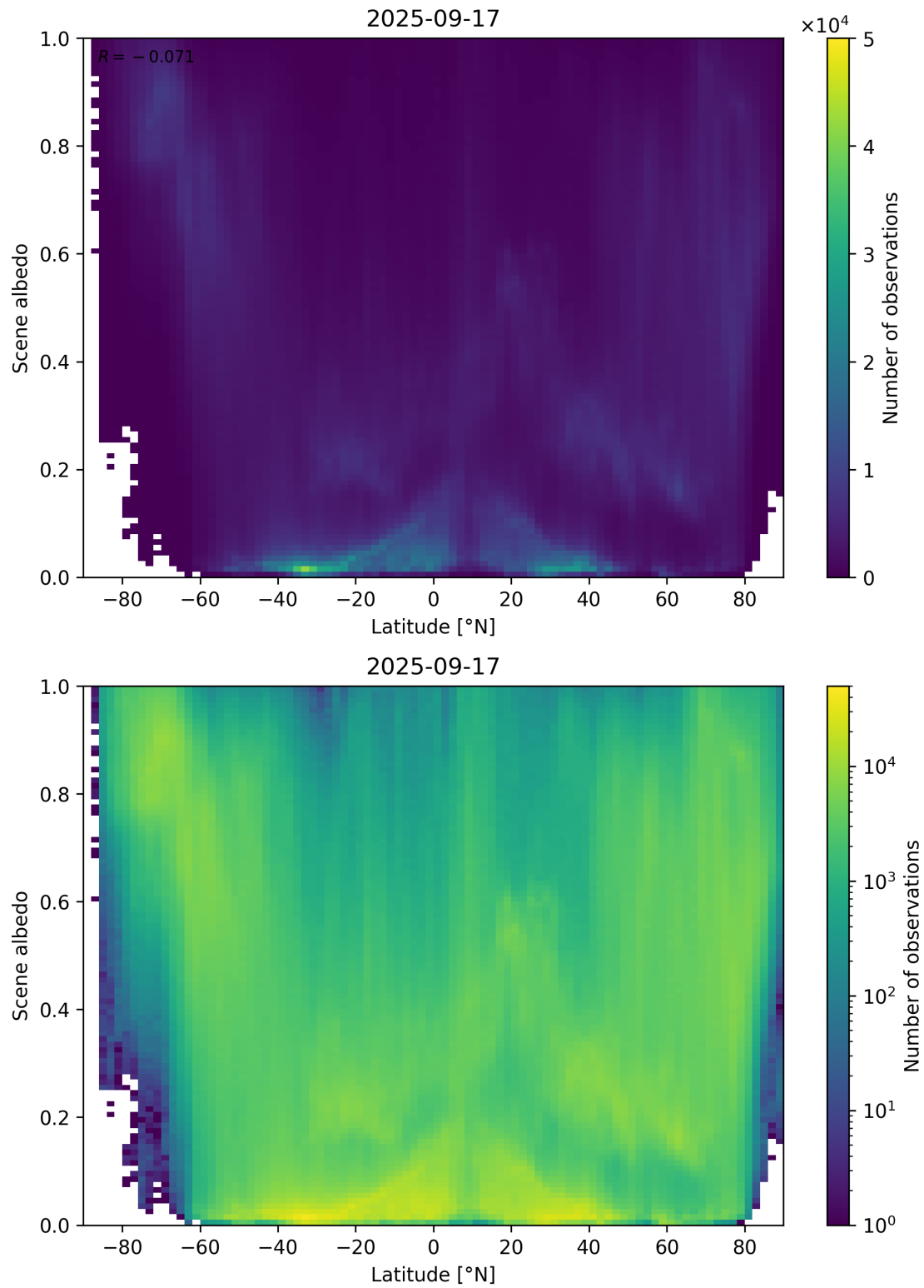
Figure 95: Scatter density plot of “Latitude” against “Scene albedo” for 2025-09-16 to 2025-09-18.
