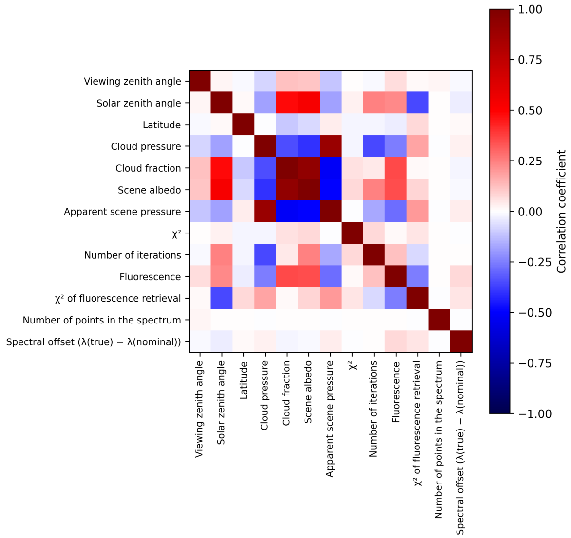
Figure 2: Map of correlation matrix for 2025-09-16 to 2025-09-18.
