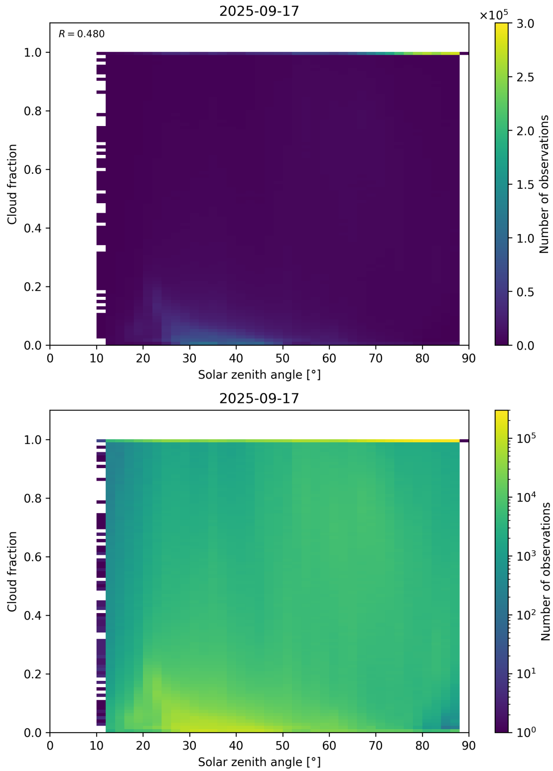
Figure 110: Scatter density plot of “Solar zenith angle” against “Cloud fraction” for 2025-09-16 to 2025-09-18.
