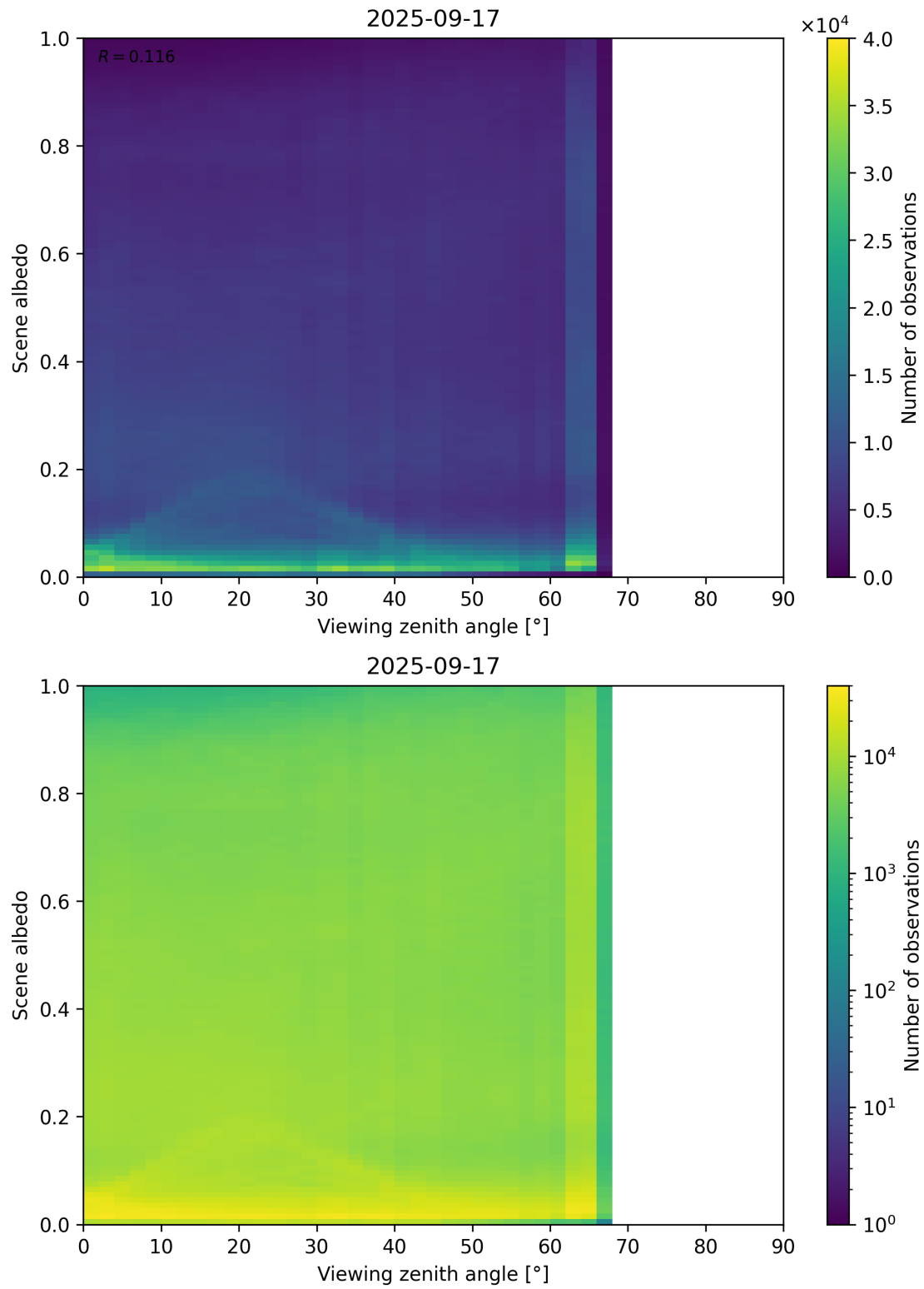
Figure 126: Scatter density plot of “Viewing zenith angle” against “Scene albedo” for 2025-09-16 to 2025-09-18.
