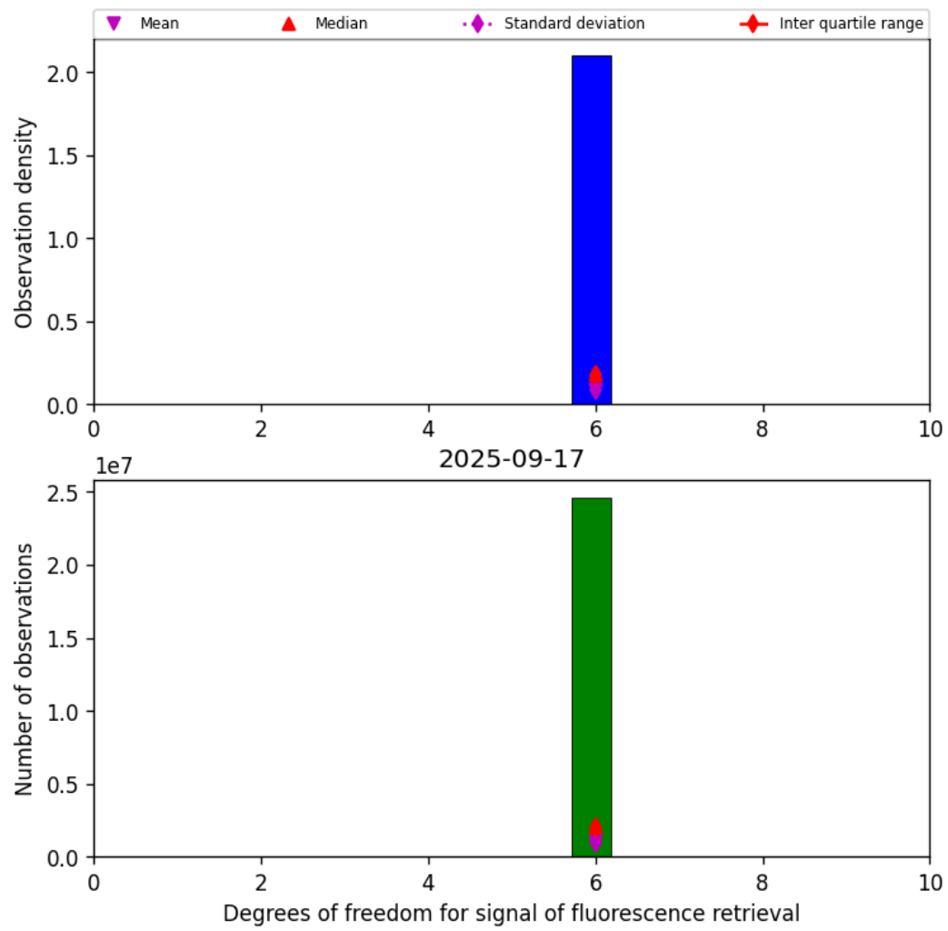
Figure 43: Histogram of "Degrees of freedom for signal of fluorescence retrieval" for 2025-09-16 to 2025-09-18
