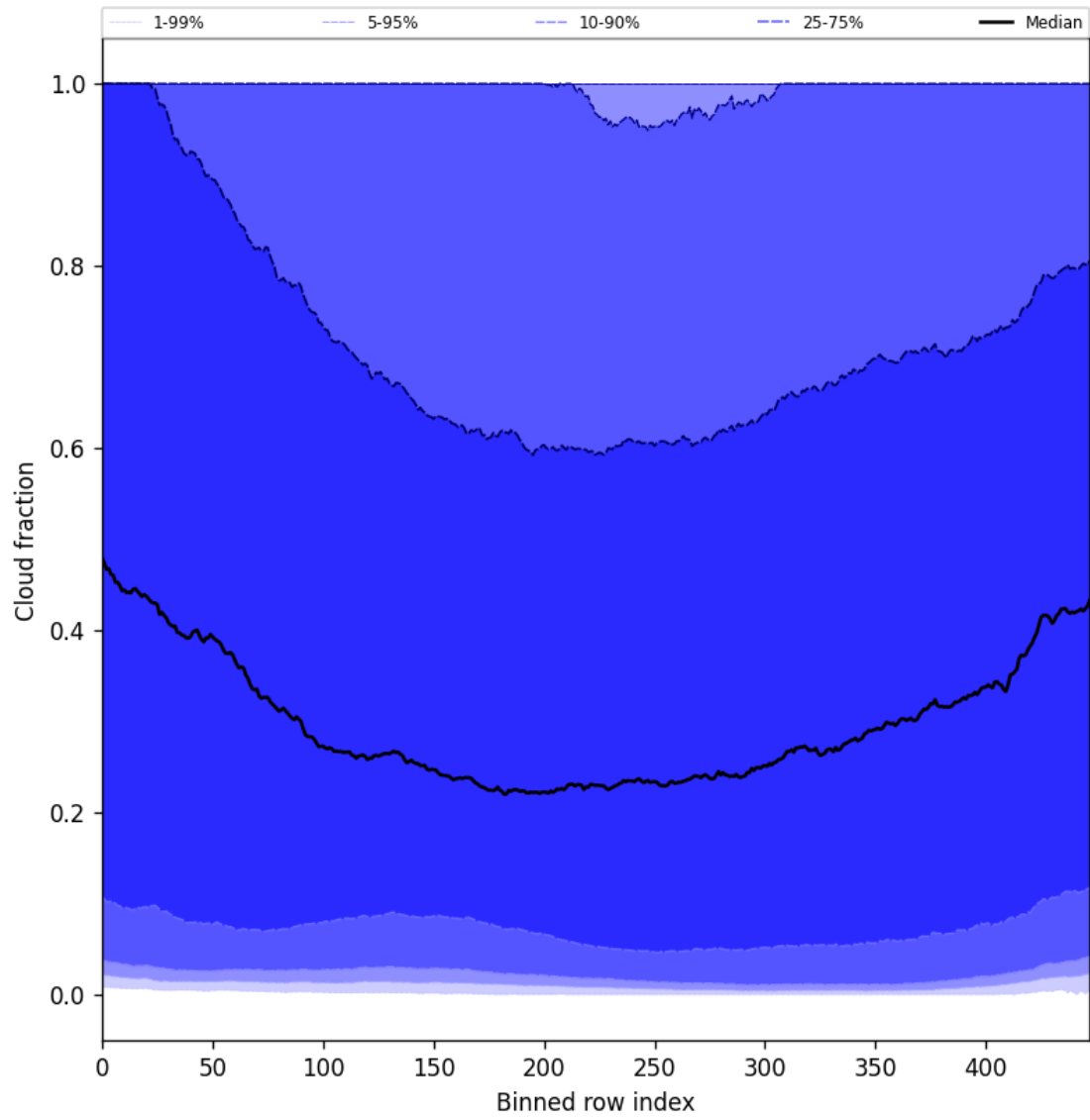
Figure 49: Along track statistics of “Cloud fraction” for 2025-09-16 to 2025-09-18
