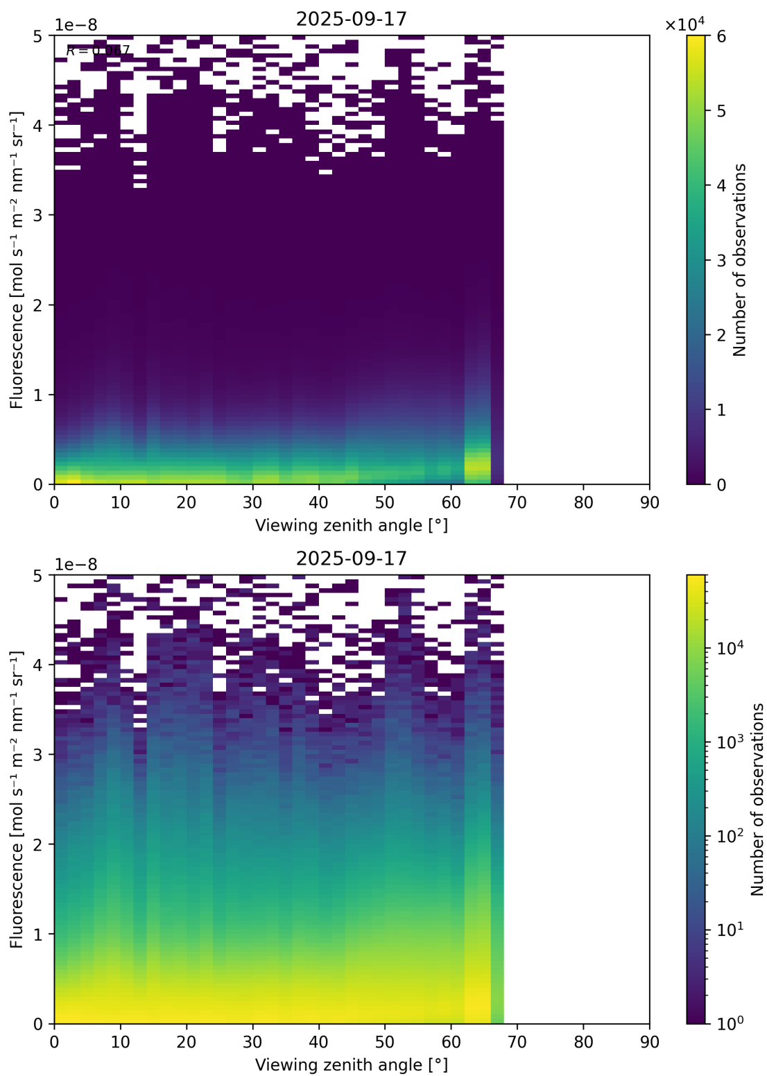
Figure 122: Scatter density plot of "Viewing zenith angle" against "Fluorescence" for 2025-09-16 to 2025-09-18.
