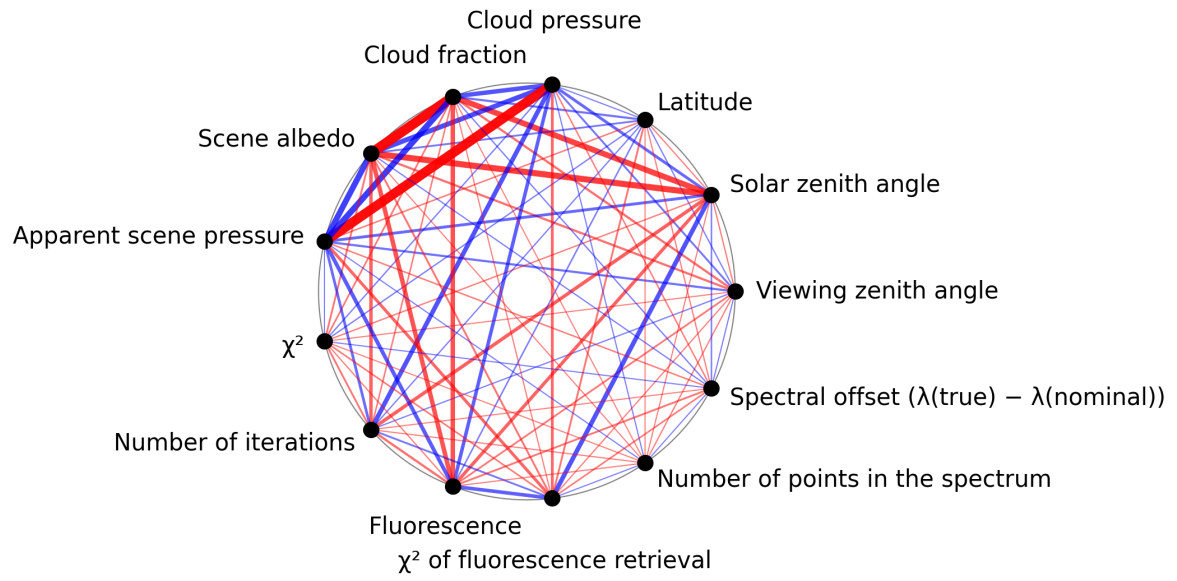
Figure 1: Map of correlation graph for 2025-09-16 to 2025-09-18.
