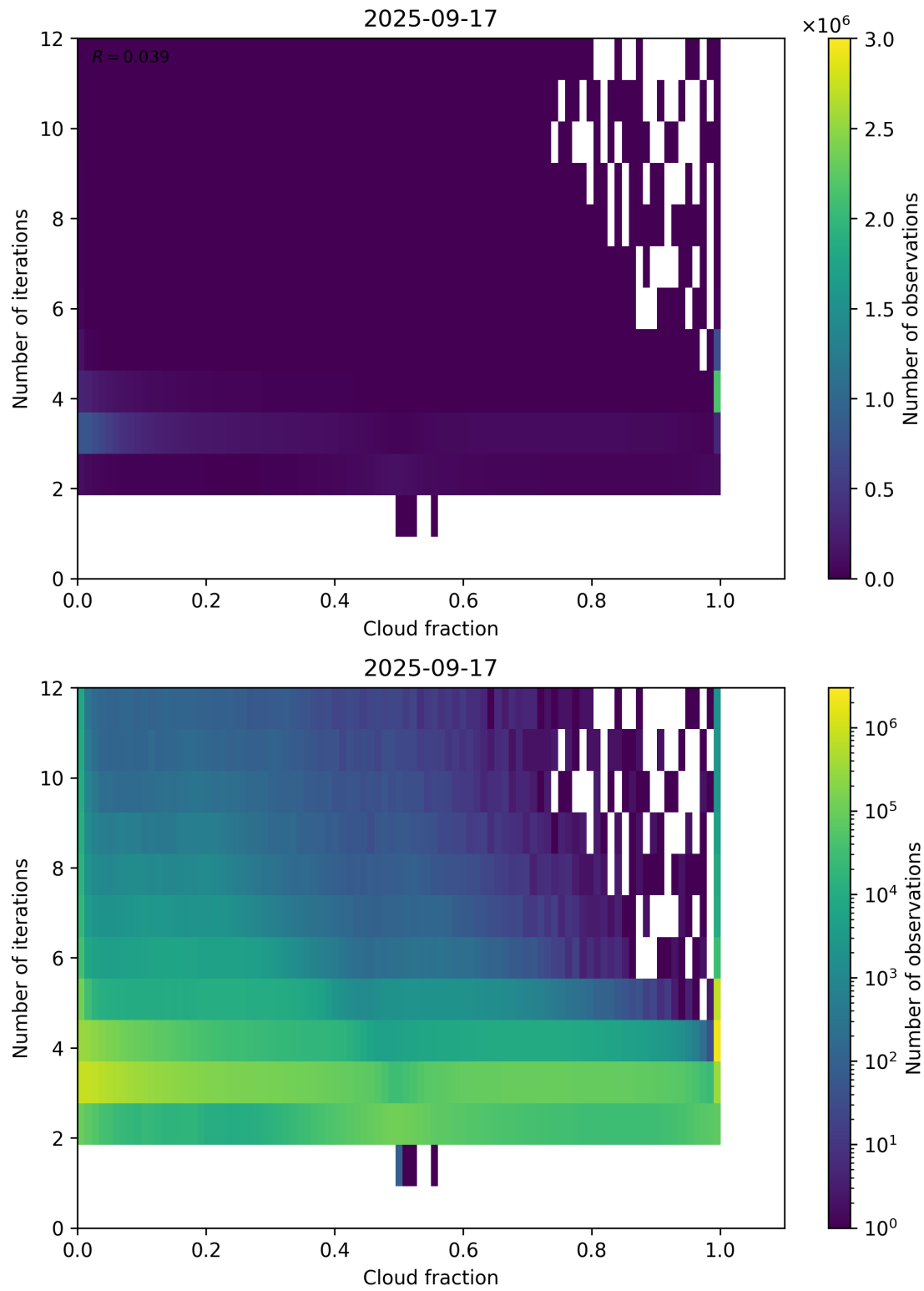
Figure 73: Scatter density plot of “Cloud fraction” against “Number of iterations” for 2025-09-16 to 2025-09-18.
