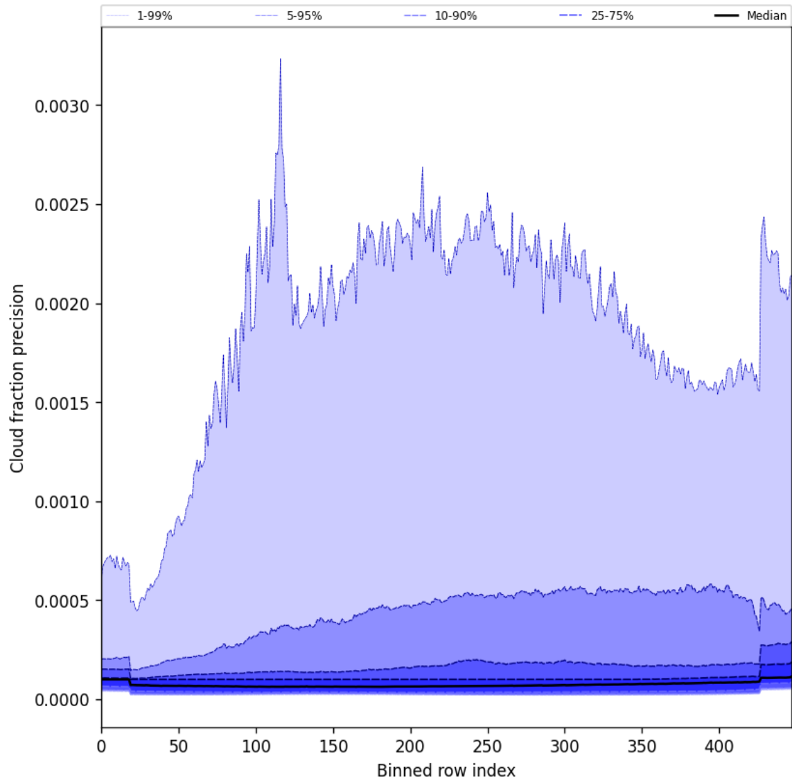
Figure 50: Along track statistics of “Cloud fraction precision” for 2025-09-16 to 2025-09-18
