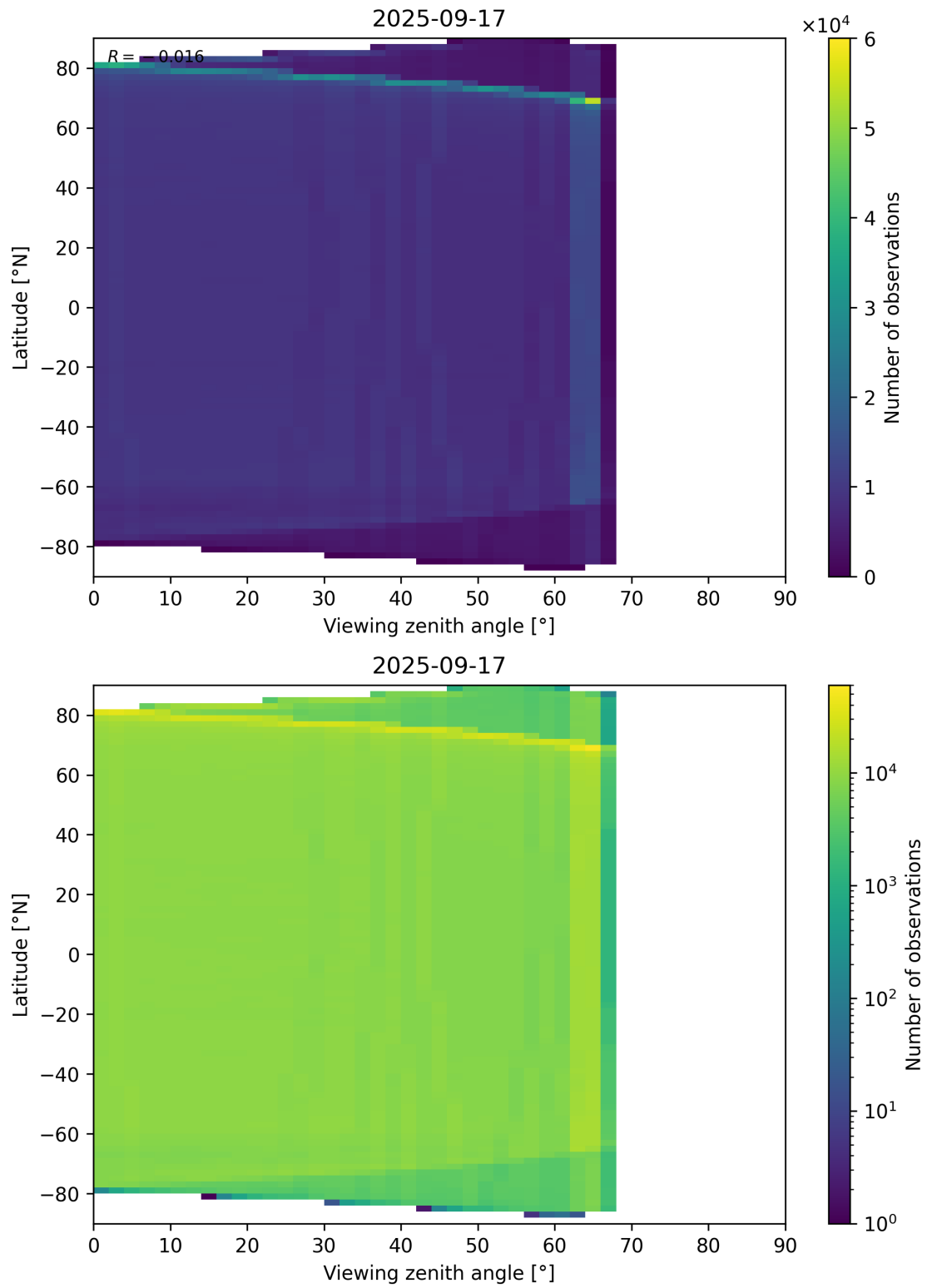
Figure 123: Scatter density plot of “Viewing zenith angle” against “Latitude” for 2025-09-16 to 2025-09-18.
