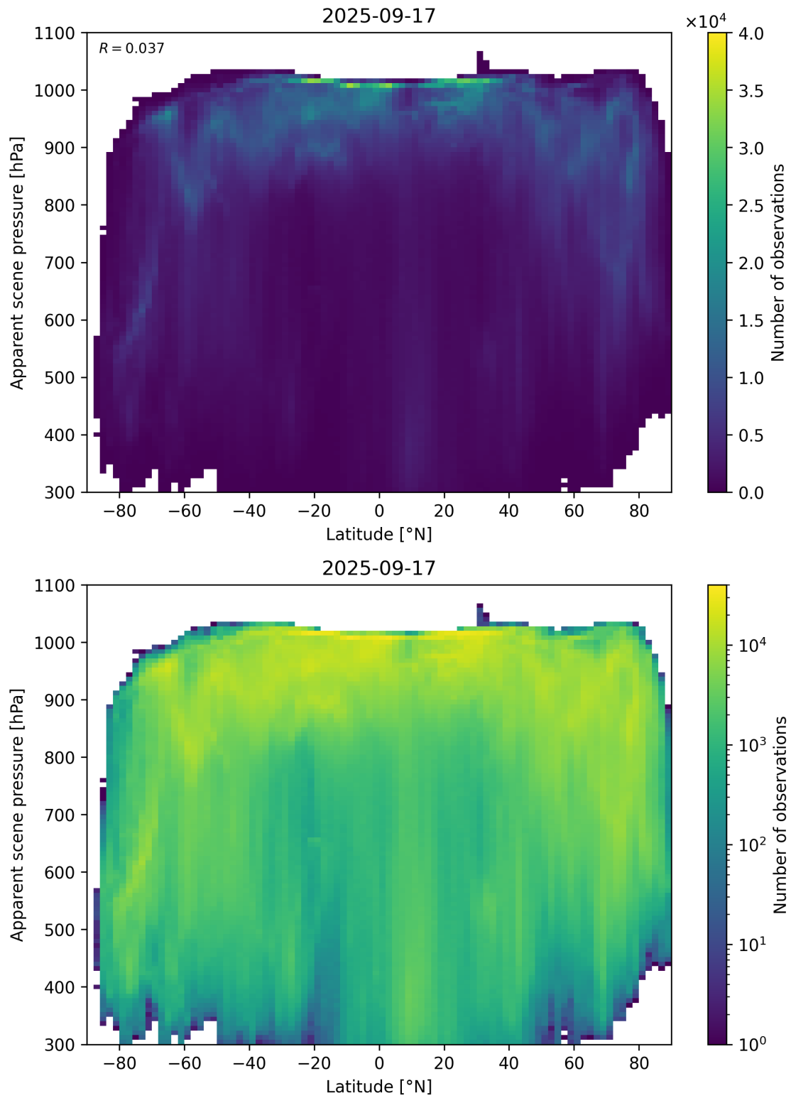
Figure 88: Scatter density plot of “Latitude” against “Apparent scene pressure” for 2025-09-16 to 2025-09-18.
