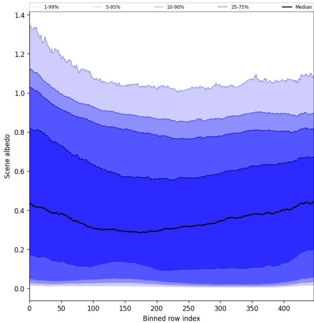
Figure 51: Along track statistics of “Scene albedo” for 2025-09-16 to 2025-09-18
