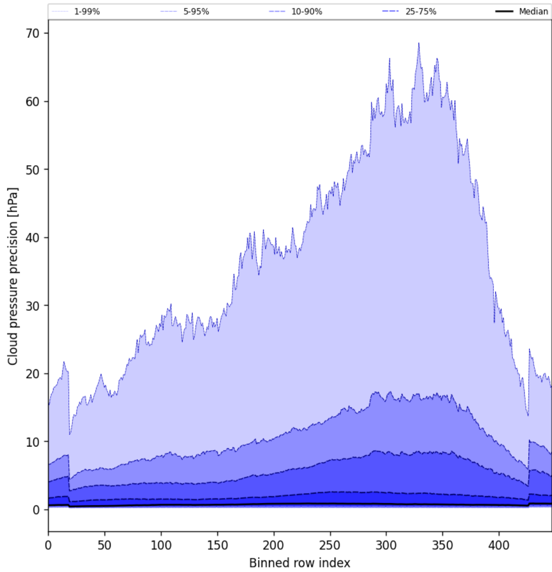
Figure 48: Along track statistics of “Cloud pressure precision” for 2025-09-16 to 2025-09-18
