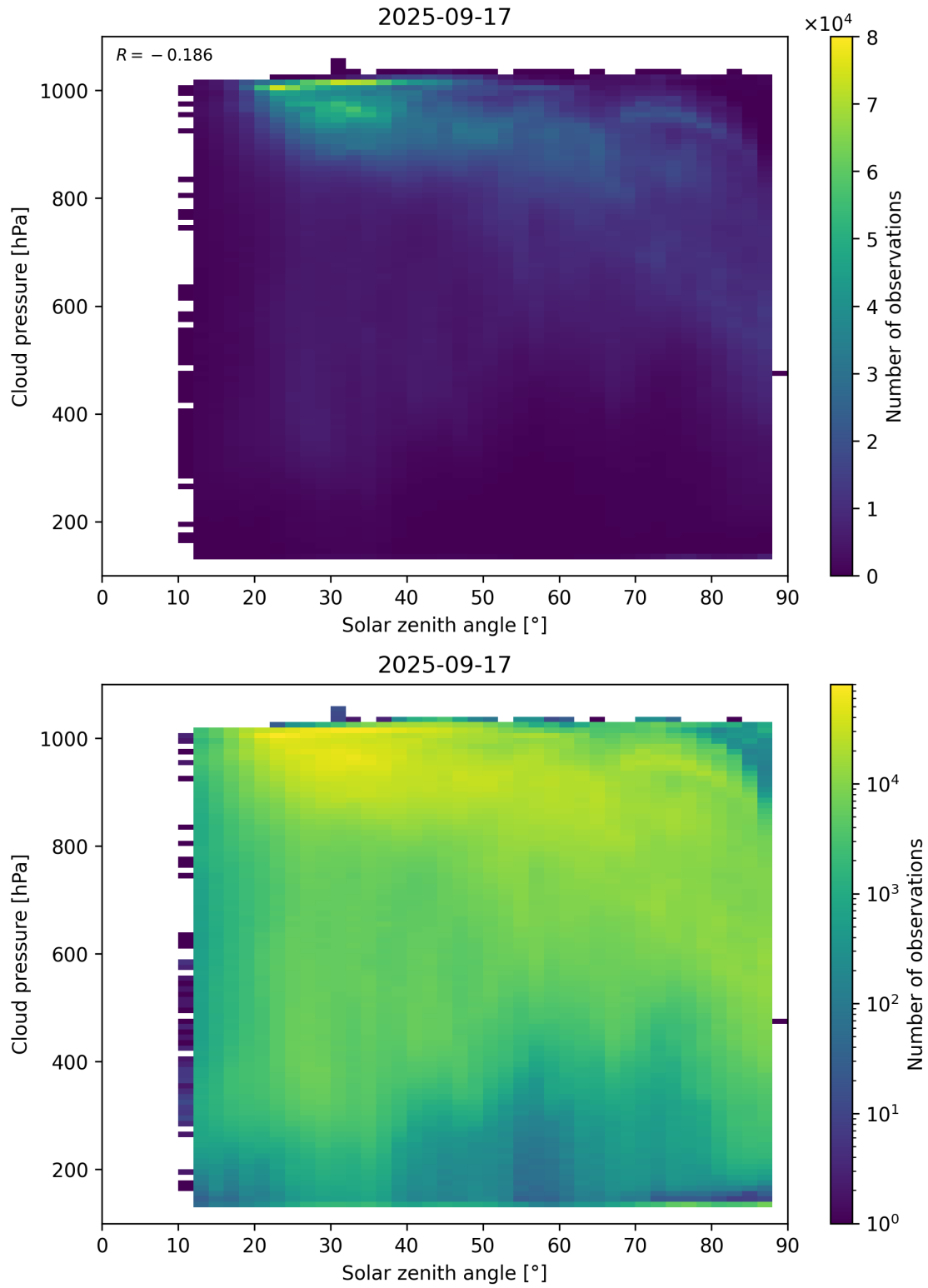
Figure 111: Scatter density plot of “Solar zenith angle” against “Cloud pressure” for 2025-09-16 to 2025-09-18.
