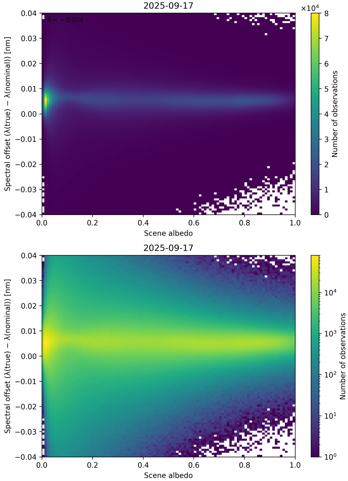
Figure 107: Scatter density plot of “Scene albedo” against “Spectral offset ( \lambda_{\text{true}} - \lambda_{\text{nominal}} )” for 2025-09-16 to 2025-09-18.
