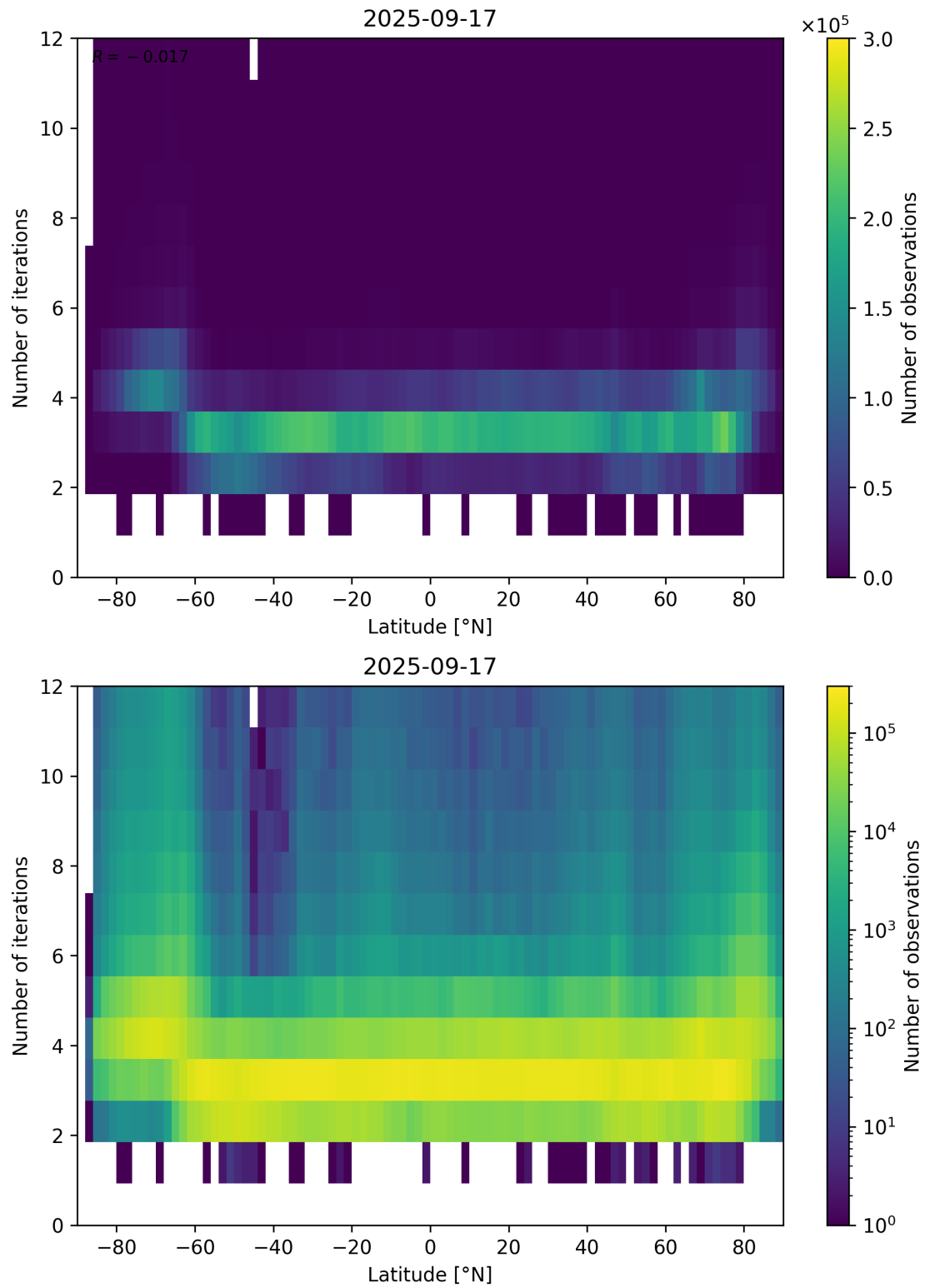
Figure 93: Scatter density plot of “Latitude” against “Number of iterations” for 2025-09-16 to 2025-09-18.
