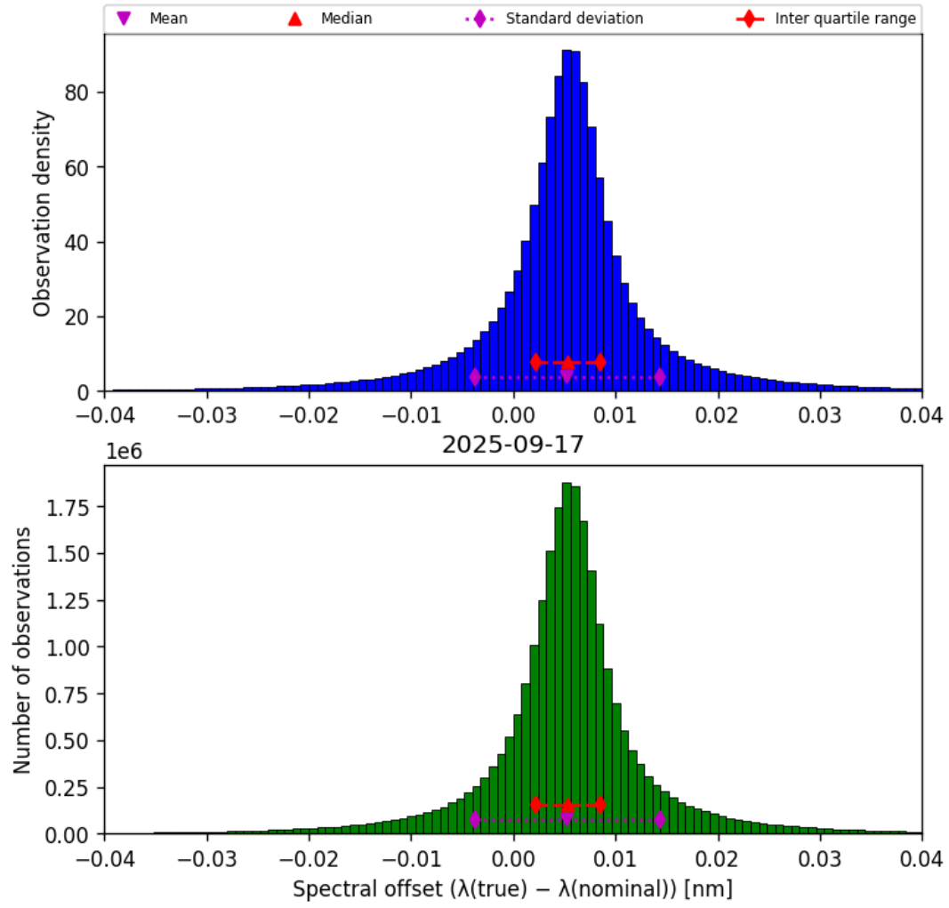
Figure 45: Histogram of “Spectral offset ( \lambda_{\text{true}} - \lambda_{\text{nominal}} )” for 2025-09-16 to 2025-09-18
