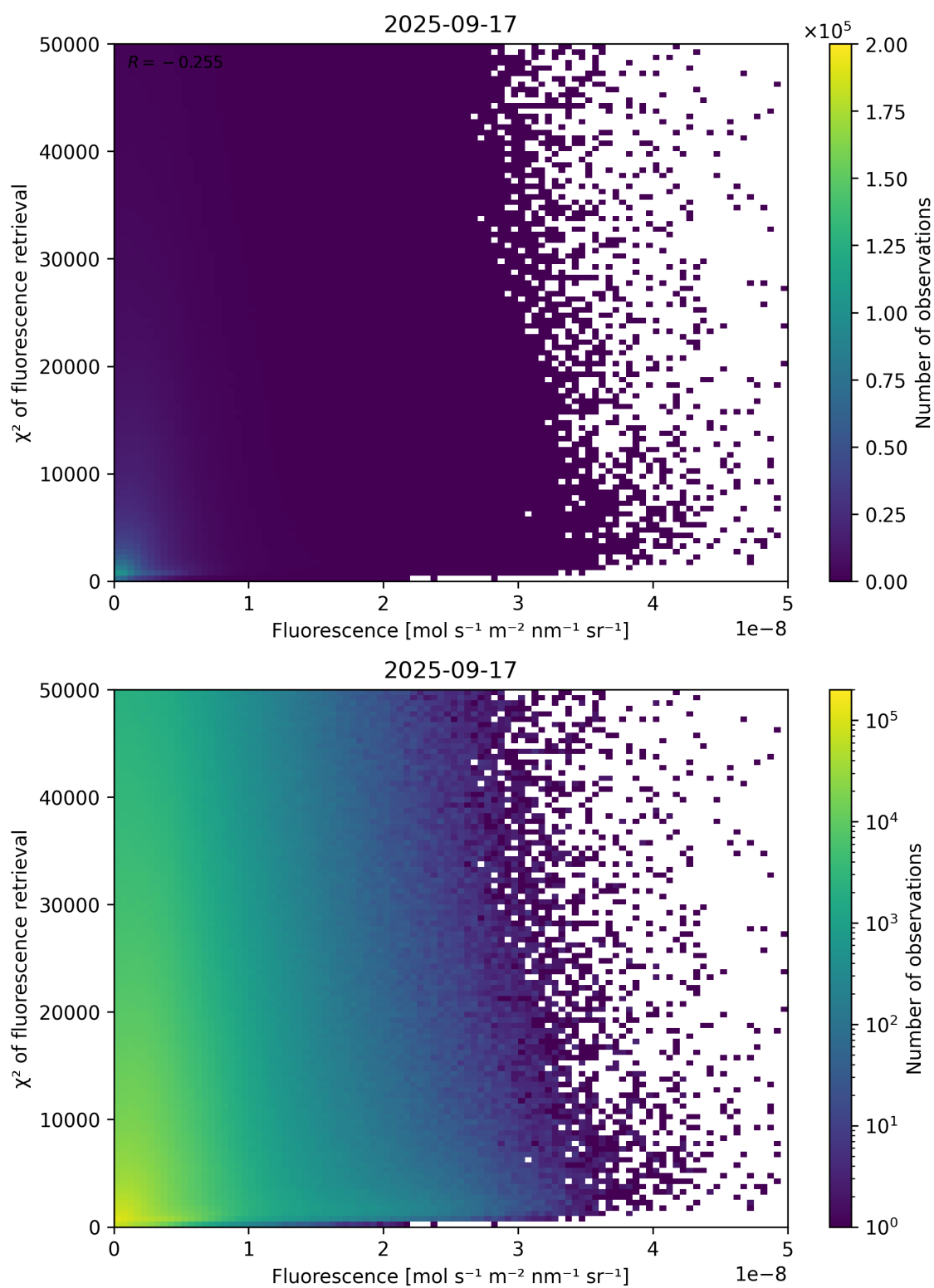
Figure 85: Scatter density plot of “Fluorescence” against “ \chi^2 of fluorescence retrieval” for 2025-09-16 to 2025-09-18.
