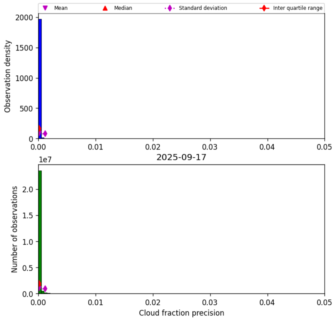
Figure 33: Histogram of “Cloud fraction precision” for 2025-09-16 to 2025-09-18
