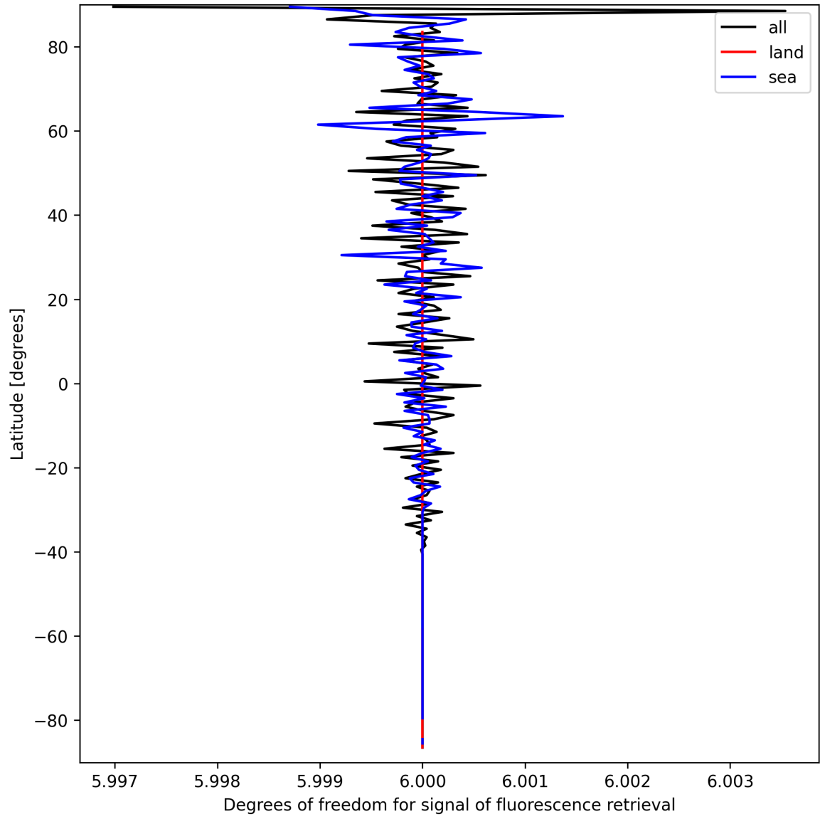
Figure 26: Zonal average of “Degrees of freedom for signal of fluorescence retrieval” for 2025-09-16 to 2025-09-18.
