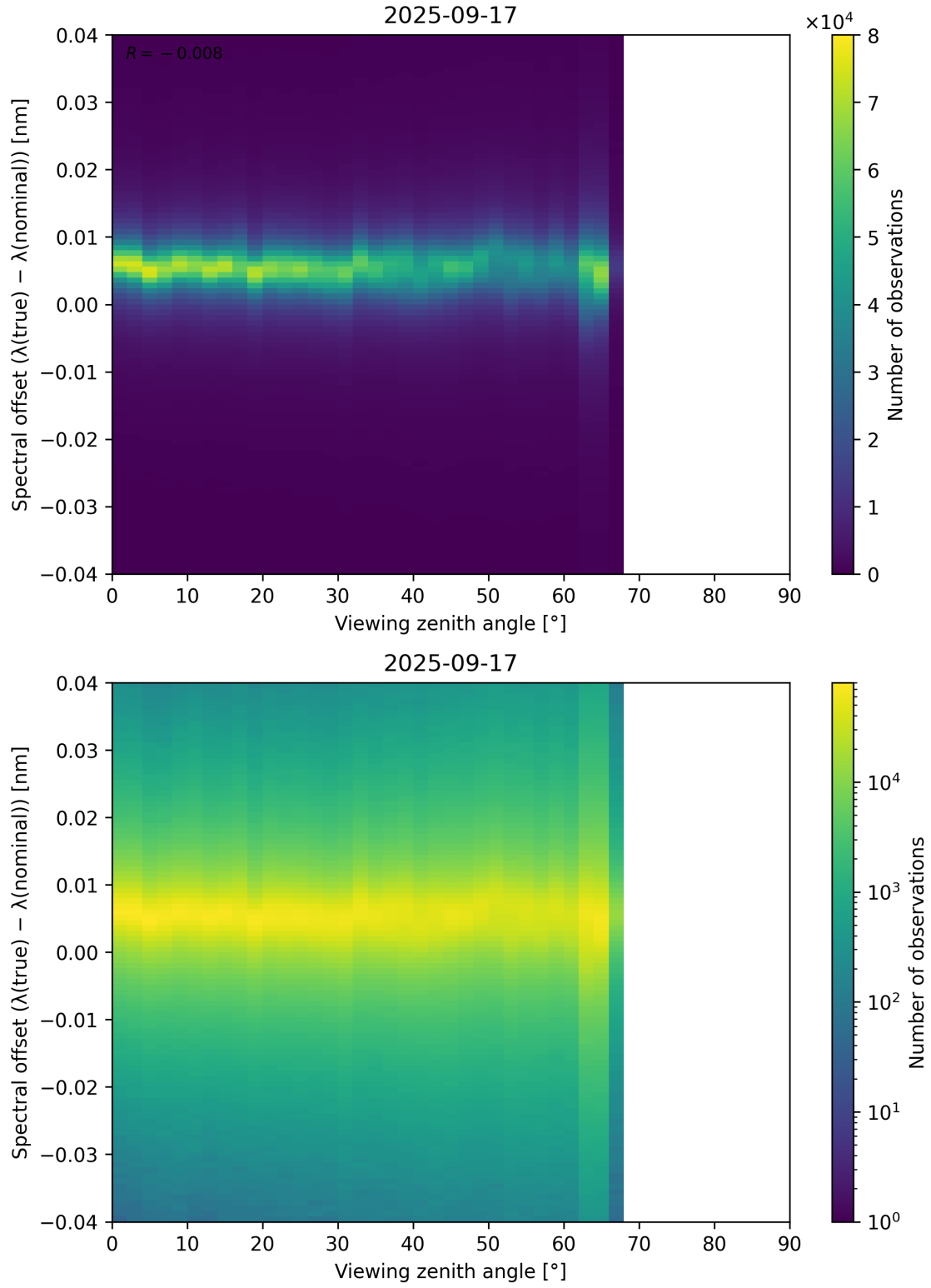
Figure 128: Scatter density plot of “Viewing zenith angle” against “Spectral offset ( \lambda_{\text{true}} - \lambda_{\text{nominal}} )” for 2025-09-16 to 2025-09-18.
