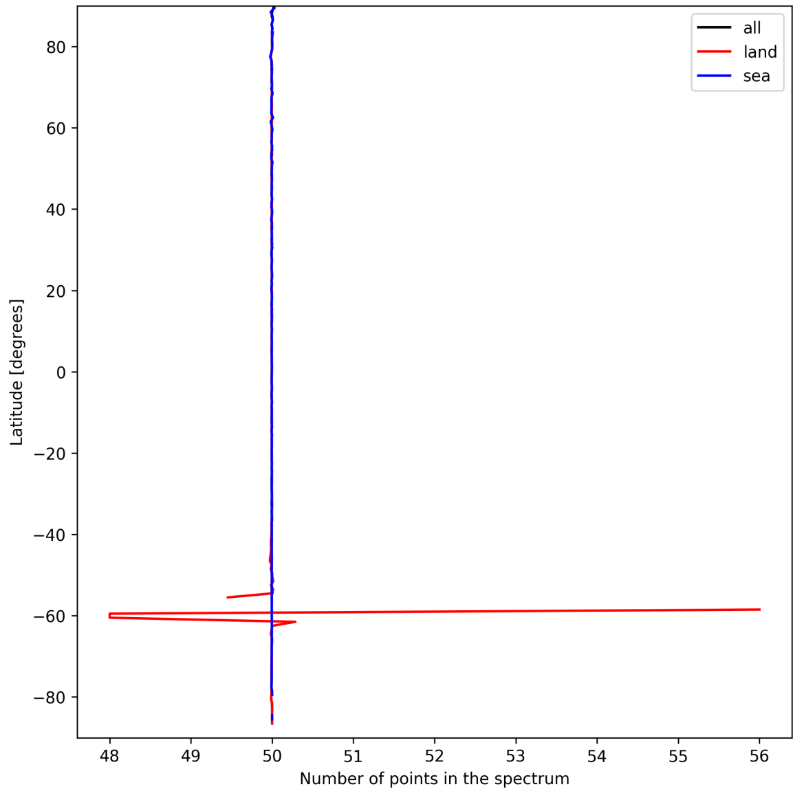
Figure 27: Zonal average of “Number of points in the spectrum” for 2025-09-16 to 2025-09-18.
