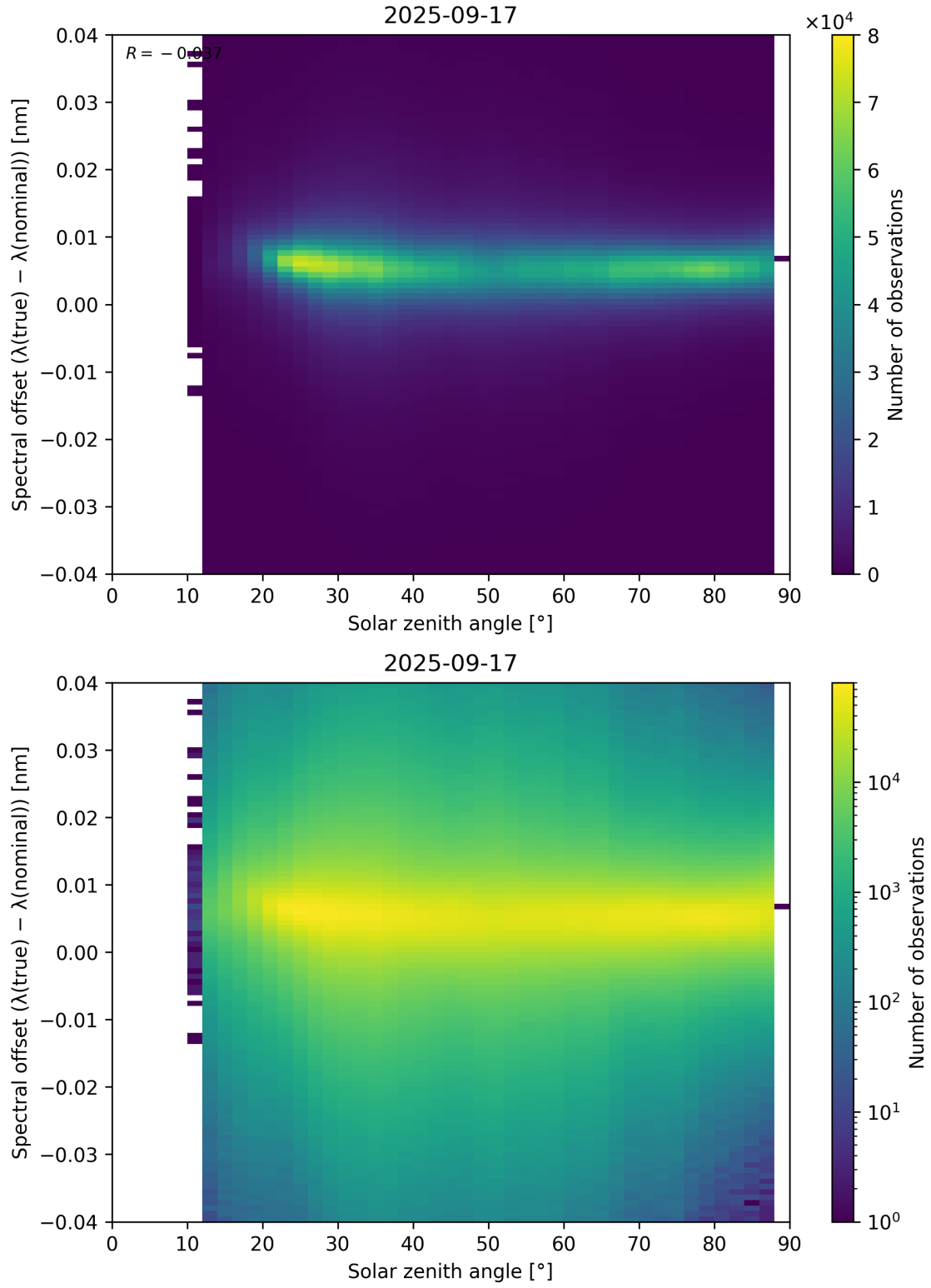
Figure 117: Scatter density plot of “Solar zenith angle” against “Spectral offset ( \lambda_{\text{true}} - \lambda_{\text{nominal}} )” for 2025-09-16 to 2025-09-18.
