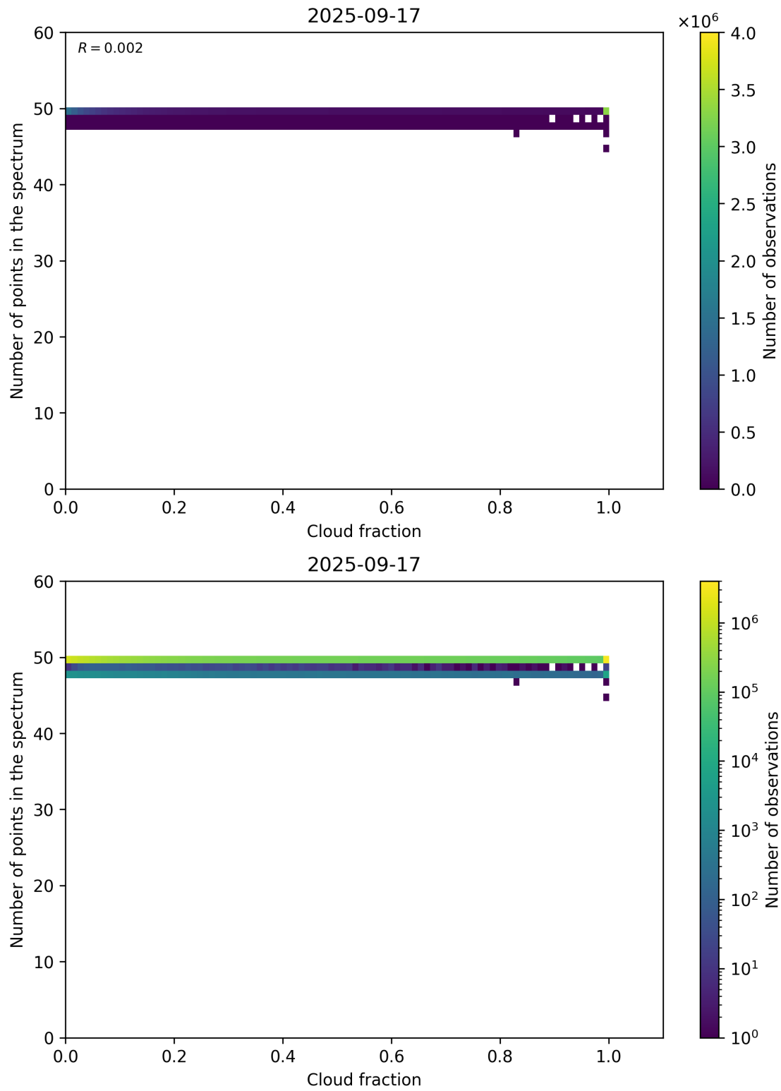
Figure 74: Scatter density plot of “Cloud fraction” against “Number of points in the spectrum” for 2025-09-16 to 2025-09-18.
