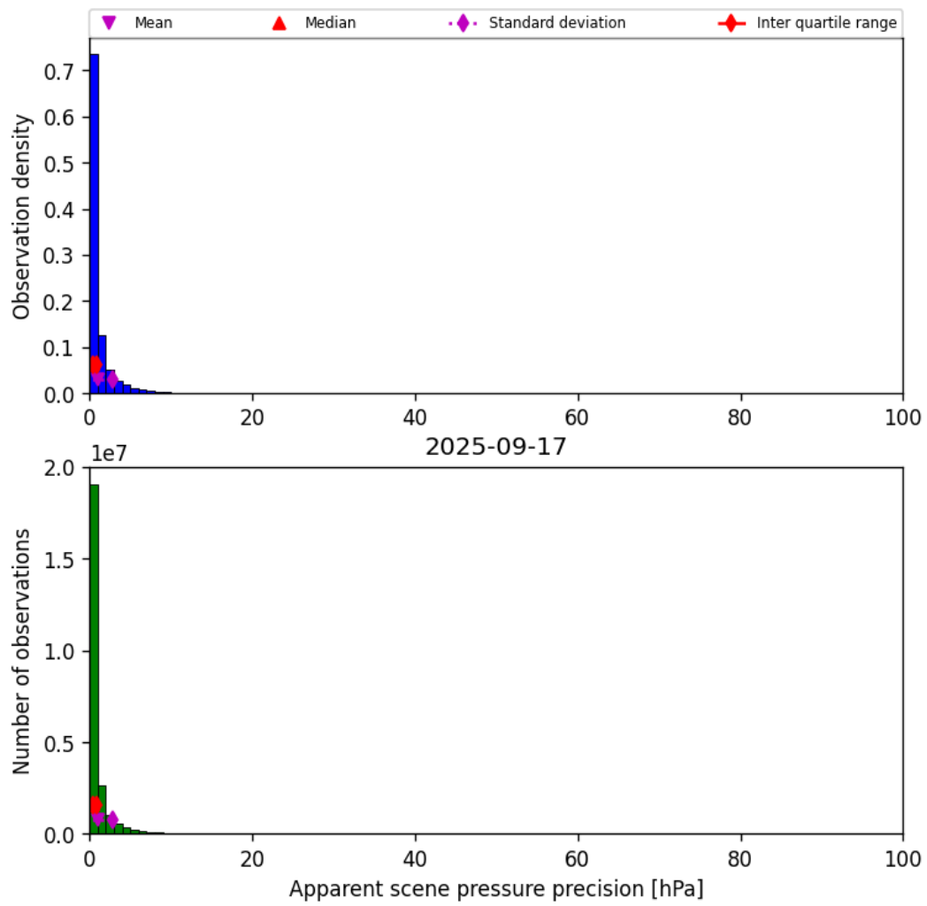
Figure 37: Histogram of “Apparent scene pressure precision” for 2025-09-16 to 2025-09-18
