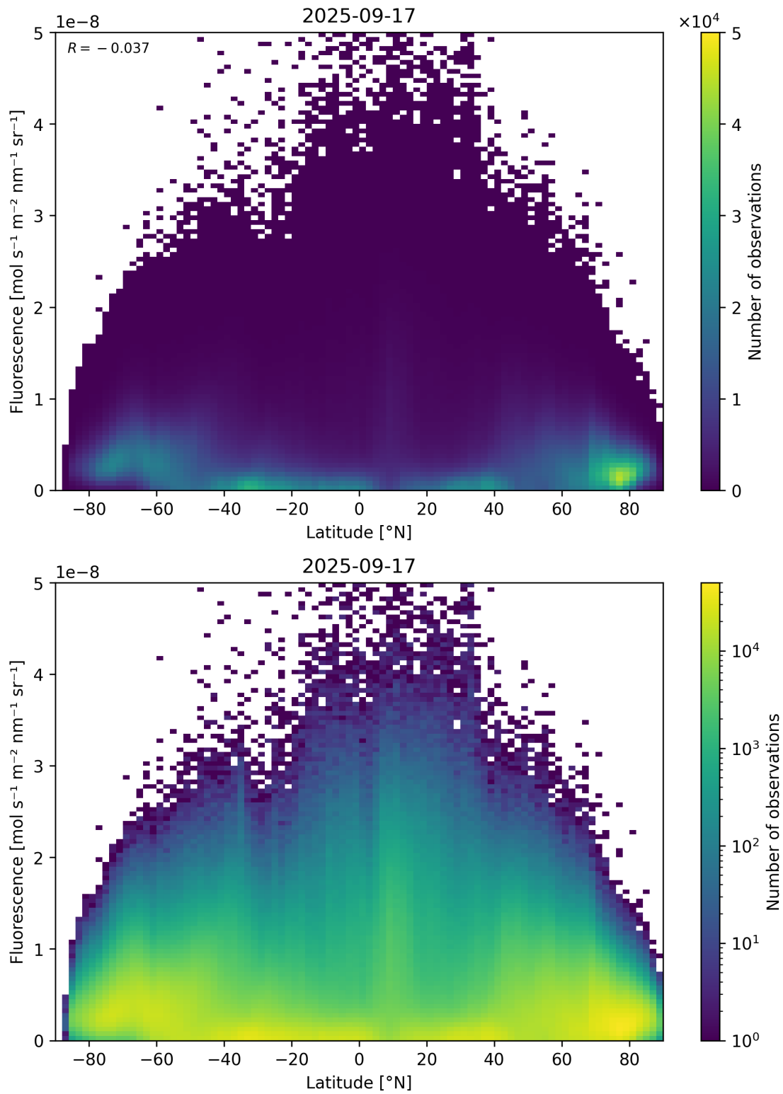
Figure 92: Scatter density plot of “Latitude” against “Fluorescence” for 2025-09-16 to 2025-09-18.
