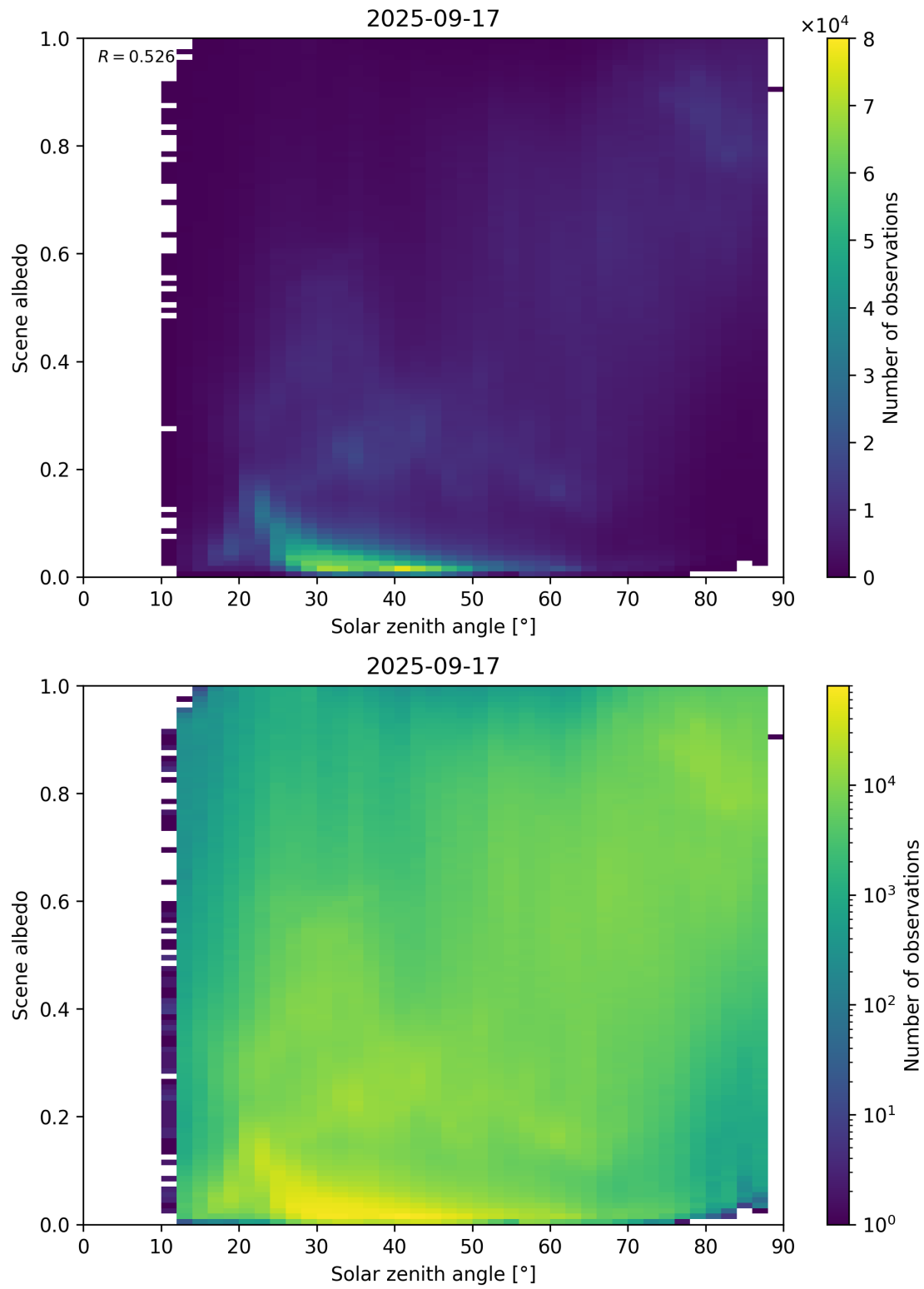
Figure 116: Scatter density plot of “Solar zenith angle” against “Scene albedo” for 2025-09-16 to 2025-09-18.
