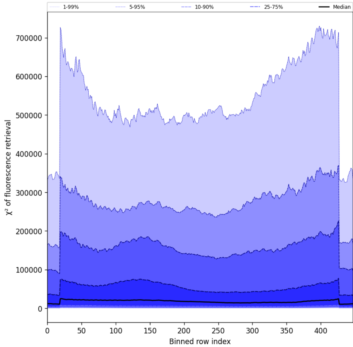
Figure 59: Along track statistics of “ \chi^2 of fluorescence retrieval” for 2025-09-16 to 2025-09-18
