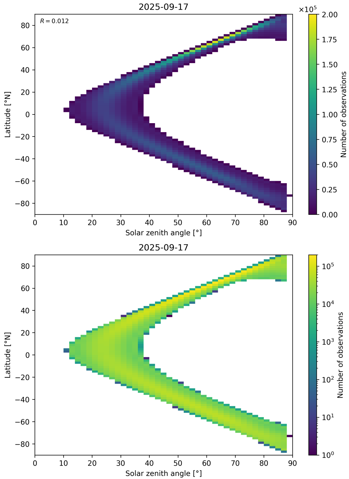
Figure 113: Scatter density plot of “Solar zenith angle” against “Latitude” for 2025-09-16 to 2025-09-18.
