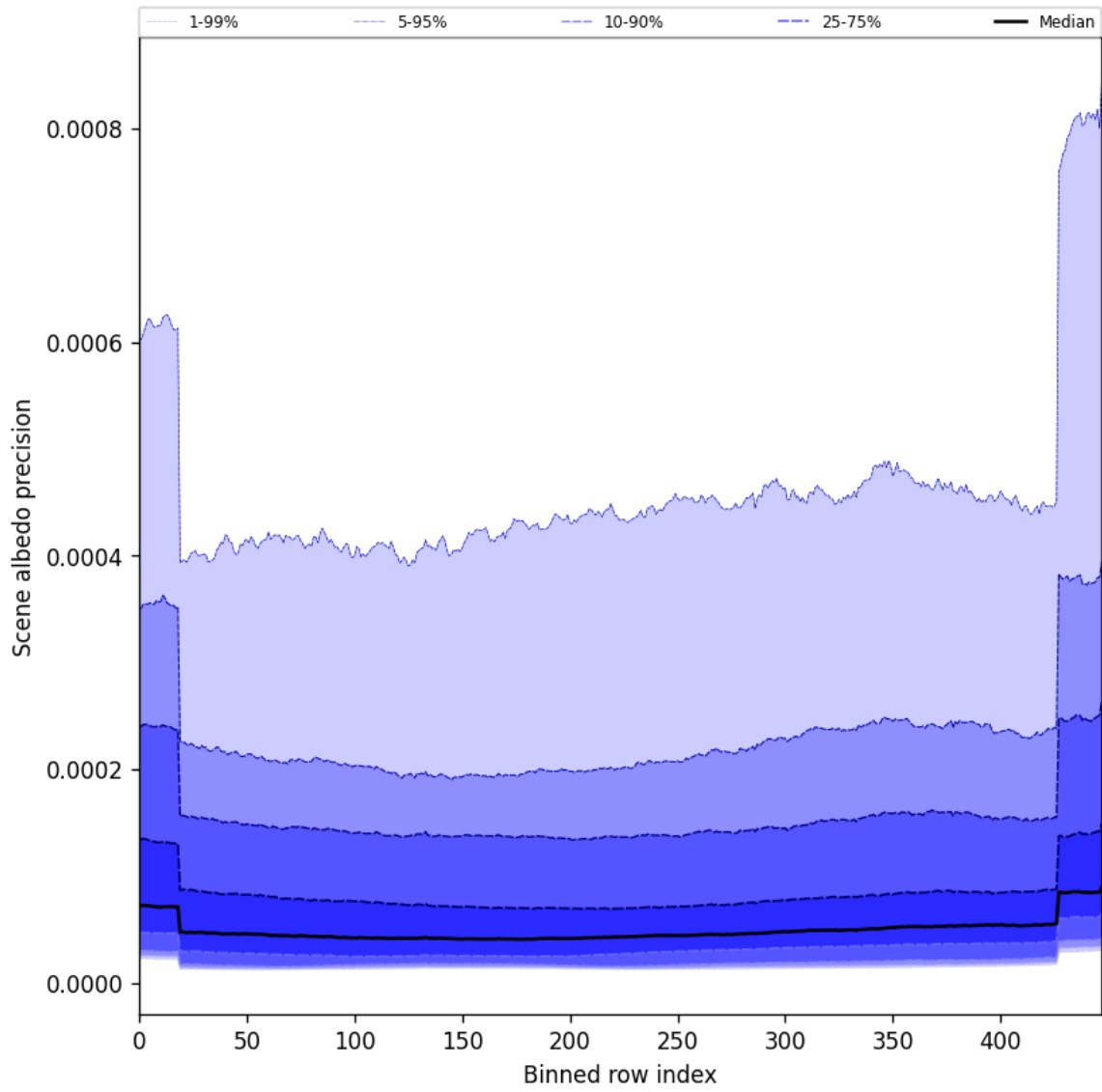
Figure 52: Along track statistics of “Scene albedo precision” for 2025-09-16 to 2025-09-18
