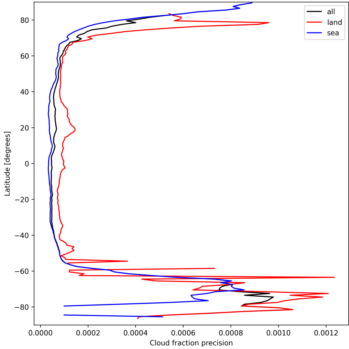
Figure 16: Zonal average of “Cloud fraction precision” for 2025-09-16 to 2025-09-18.
