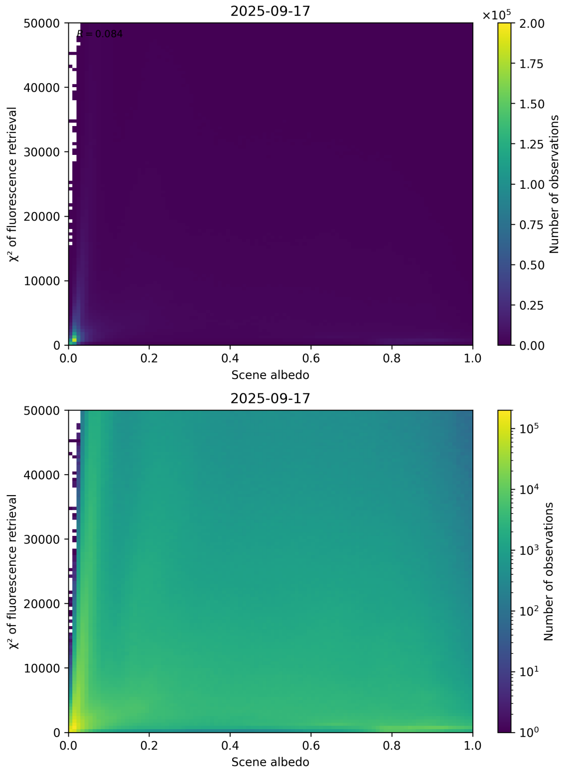
Figure 103: Scatter density plot of “Scene albedo” against “ \chi^2 of fluorescence retrieval” for 2025-09-16 to 2025-09-18.
