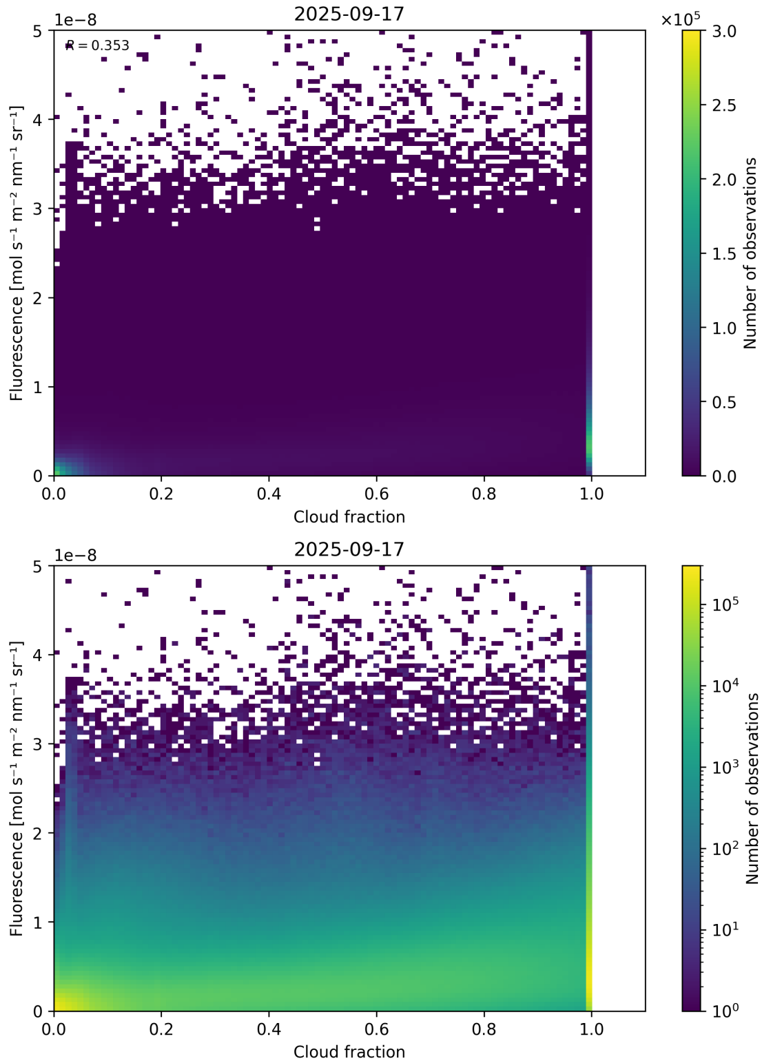
Figure 72: Scatter density plot of “Cloud fraction” against “Fluorescence” for 2025-09-16 to 2025-09-18.
