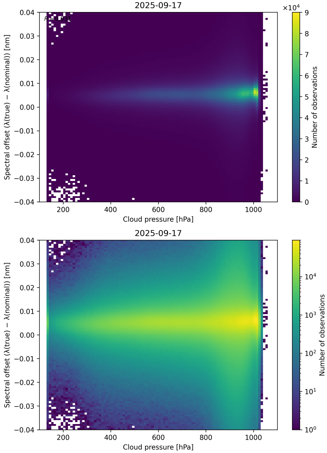
Figure 84: Scatter density plot of “Cloud pressure” against “Spectral offset ( \lambda_{\text{true}} - \lambda_{\text{nominal}} )” for 2025-09-16 to 2025-09-18.
