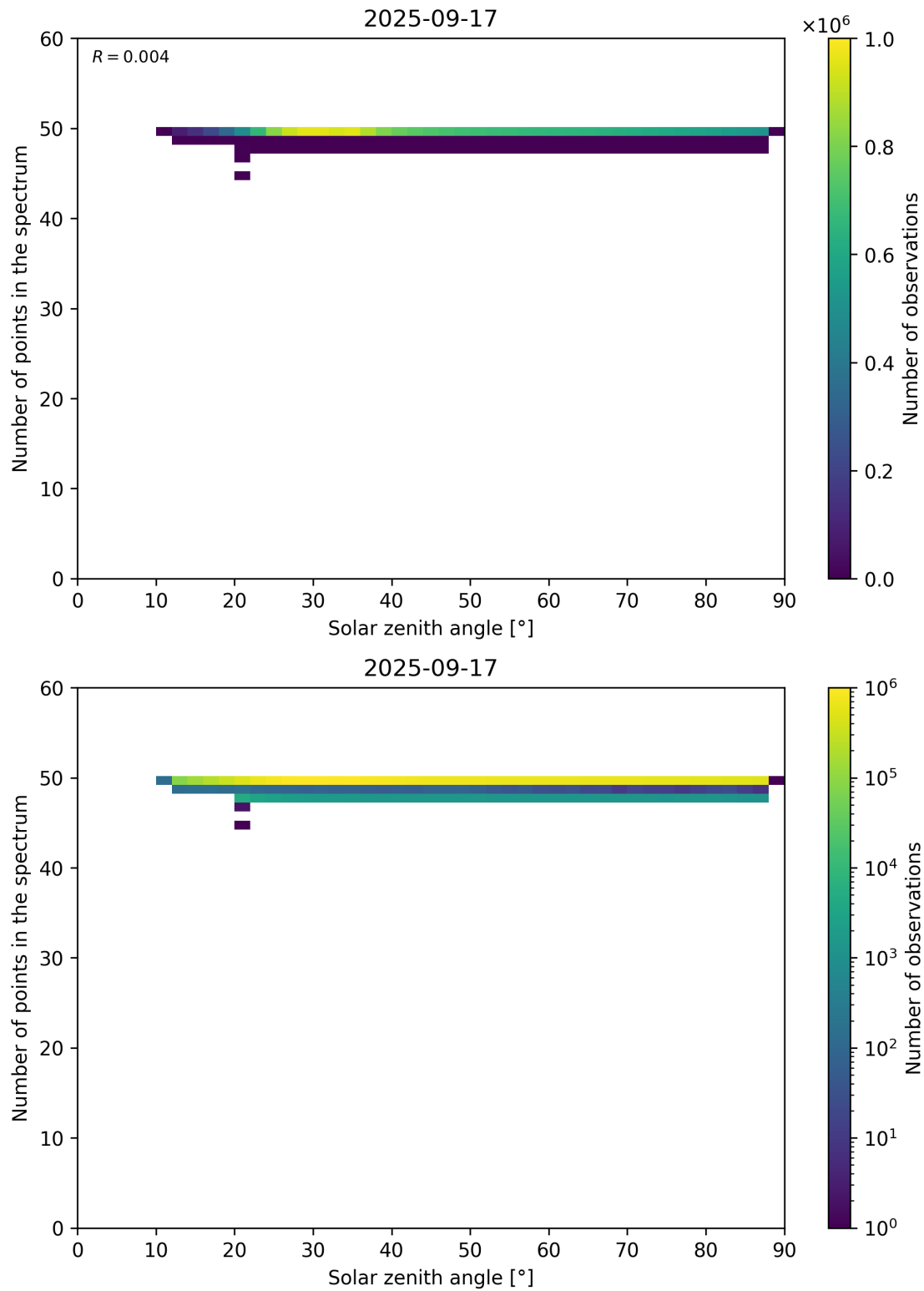
Figure 115: Scatter density plot of “Solar zenith angle” against “Number of points in the spectrum” for 2025-09-16 to 2025-09-18.
