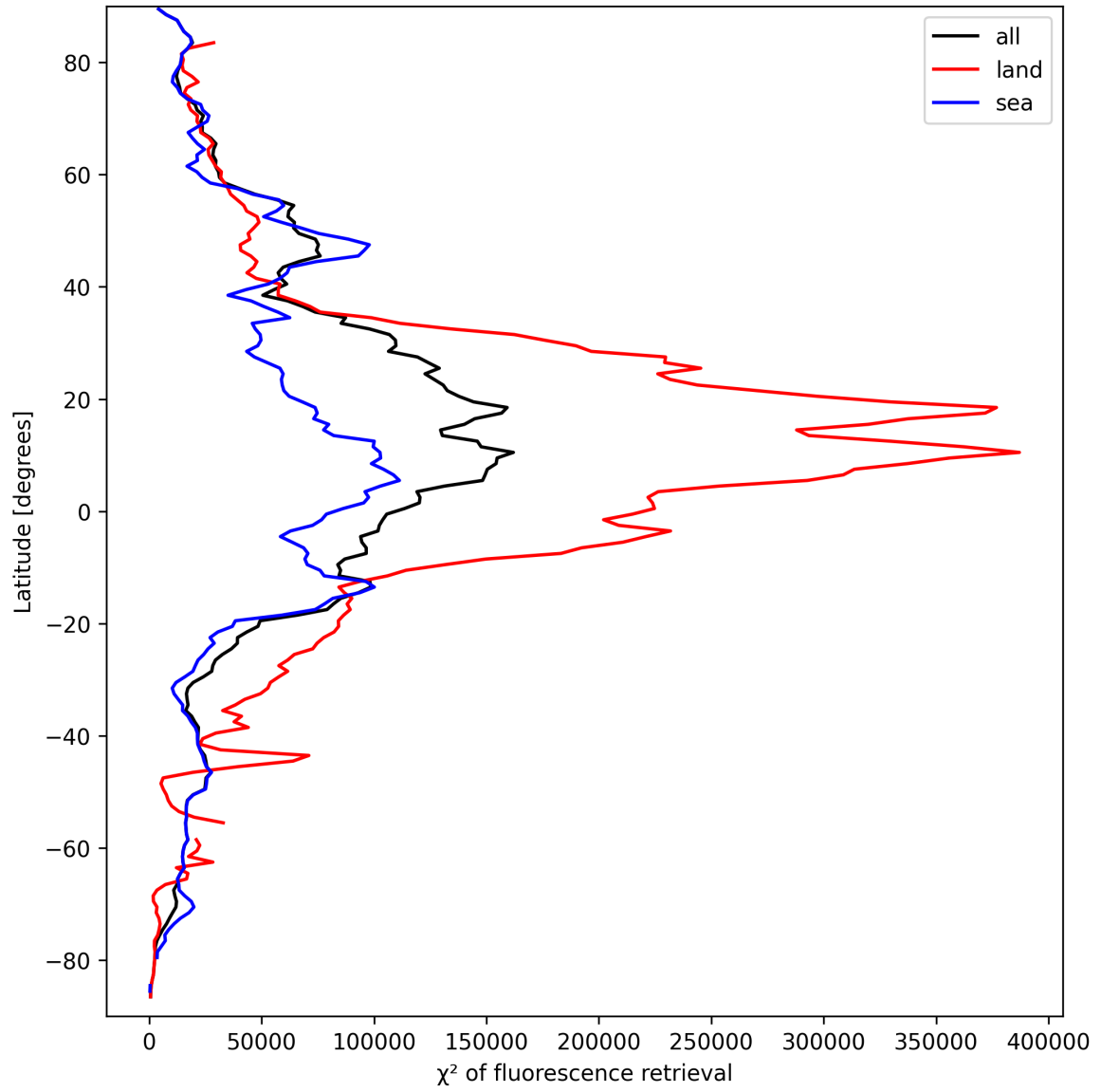
Figure 25: Zonal average of “ \chi^2 of fluorescence retrieval” for 2025-09-16 to 2025-09-18.
