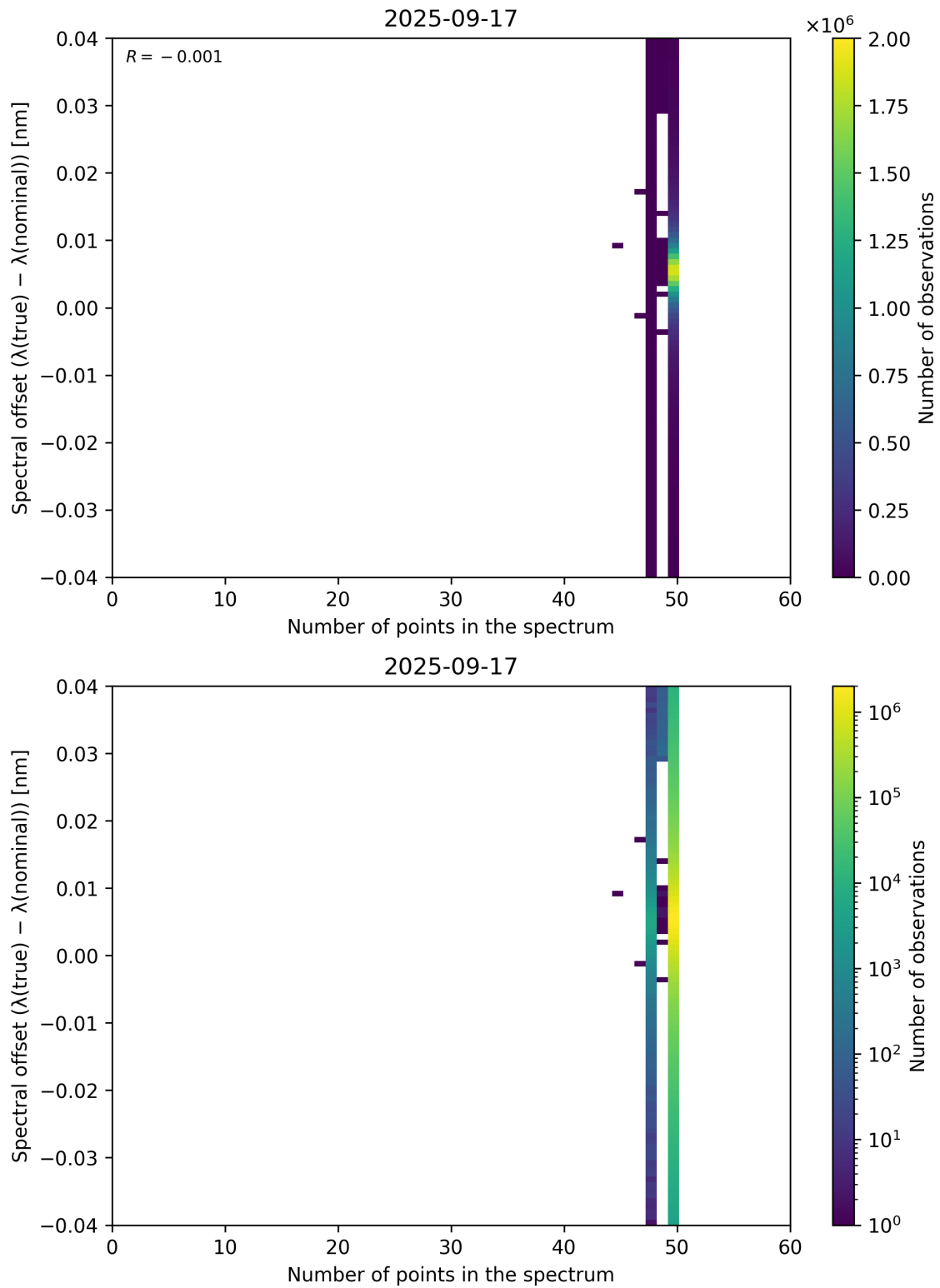
Figure 101: Scatter density plot of “Number of points in the spectrum” against “Spectral offset ( \lambda_{\text{true}} - \lambda_{\text{nominal}} )” for 2025-09-16 to 2025-09-18.
