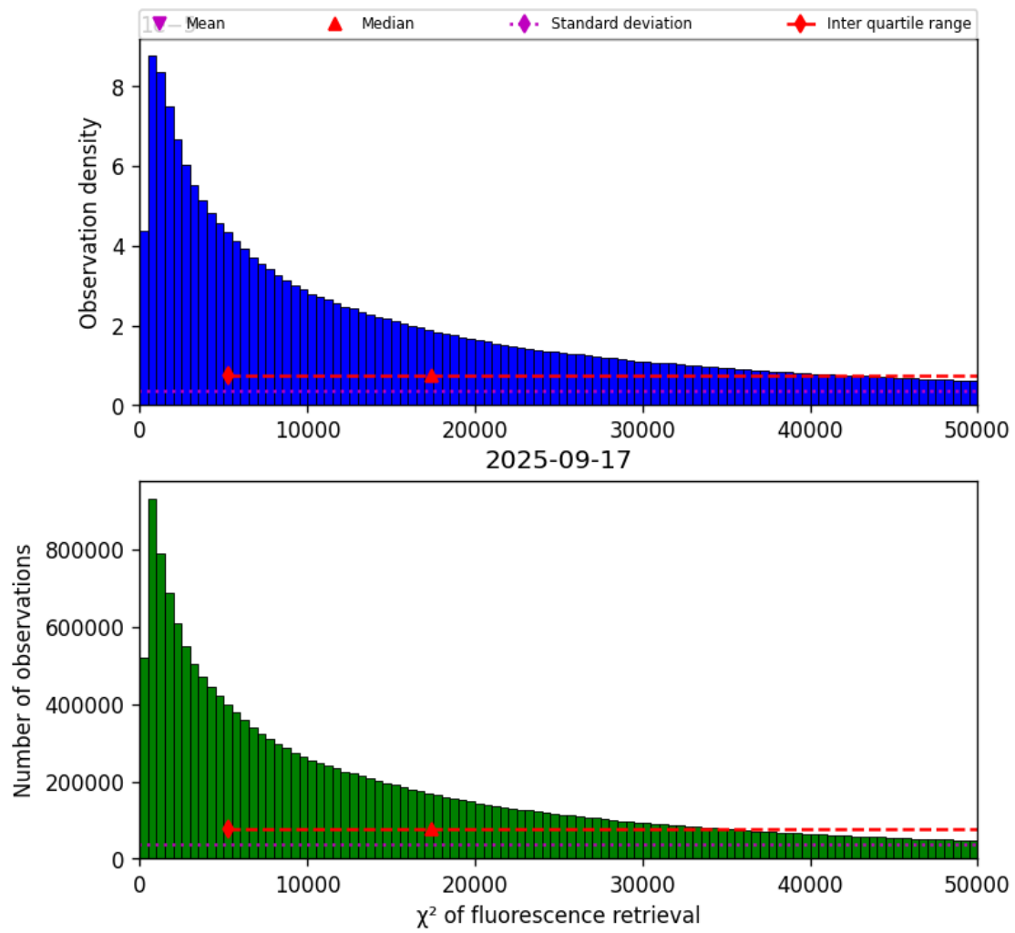
Figure 42: Histogram of “ \chi^2 of fluorescence retrieval” for 2025-09-16 to 2025-09-18
