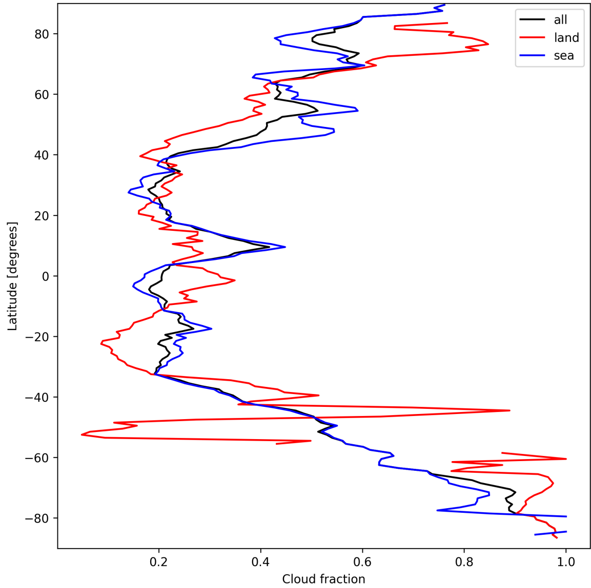
Figure 15: Zonal average of “Cloud fraction” for 2025-09-16 to 2025-09-18.
