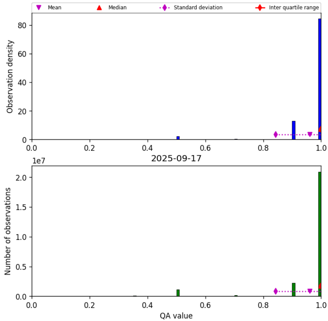
Figure 29: Histogram of “QA value” for 2025-09-16 to 2025-09-18
