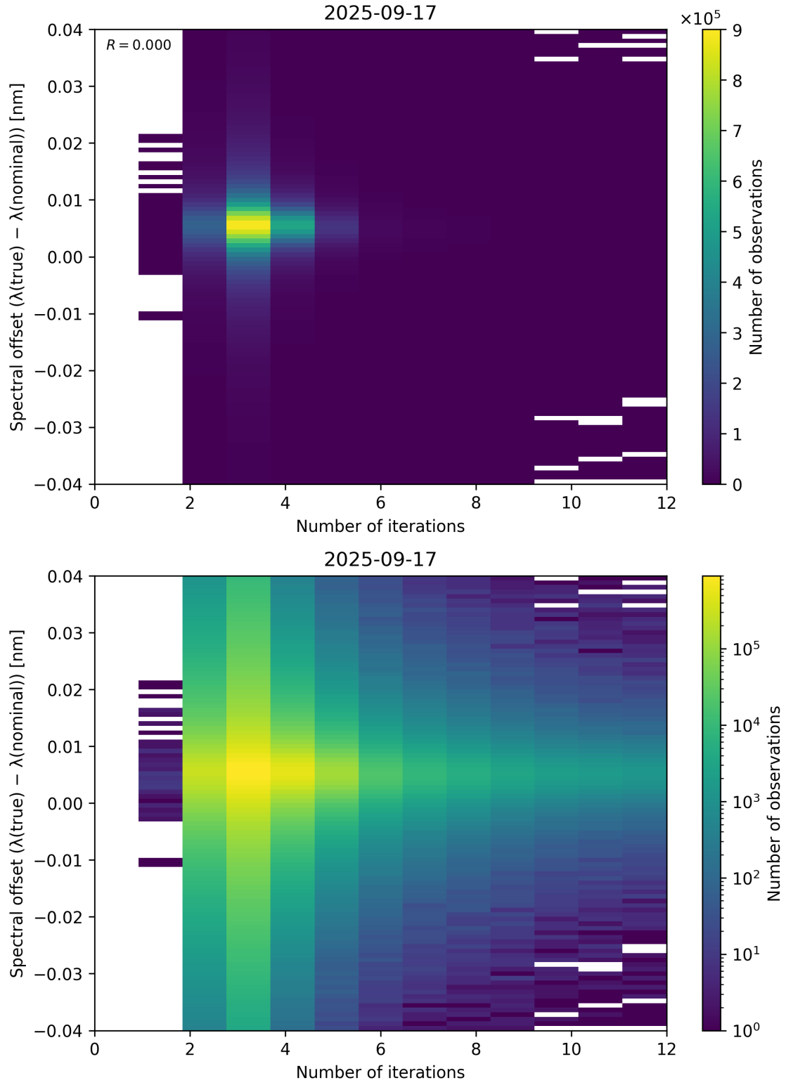
Figure 100: Scatter density plot of “Number of iterations” against “Spectral offset ( \lambda_{\text{true}} - \lambda_{\text{nominal}} )” for 2025-09-16 to 2025-09-18.
