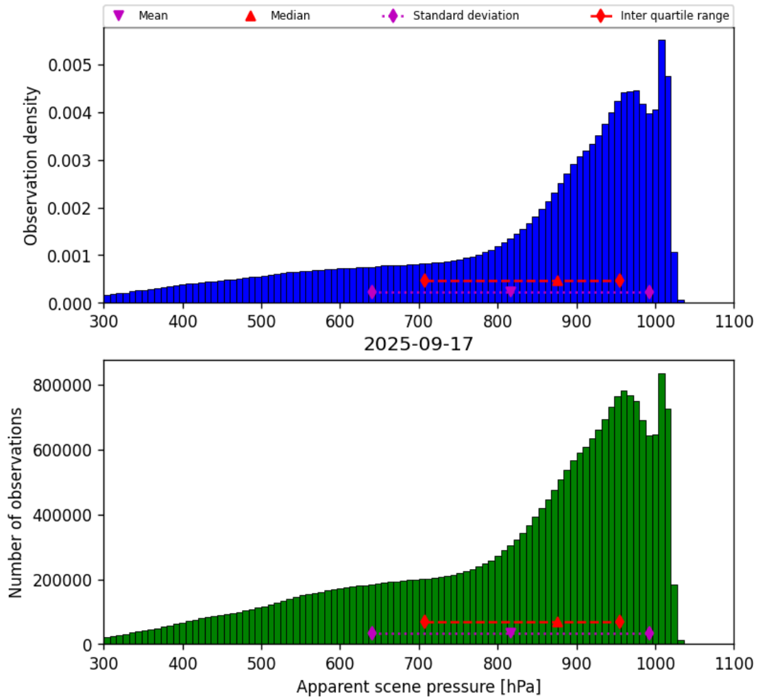
Figure 36: Histogram of “Apparent scene pressure” for 2025-09-16 to 2025-09-18
