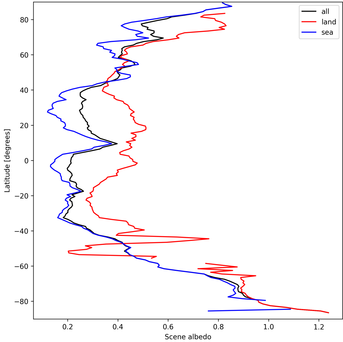
Figure 17: Zonal average of “Scene albedo” for 2025-09-16 to 2025-09-18.
