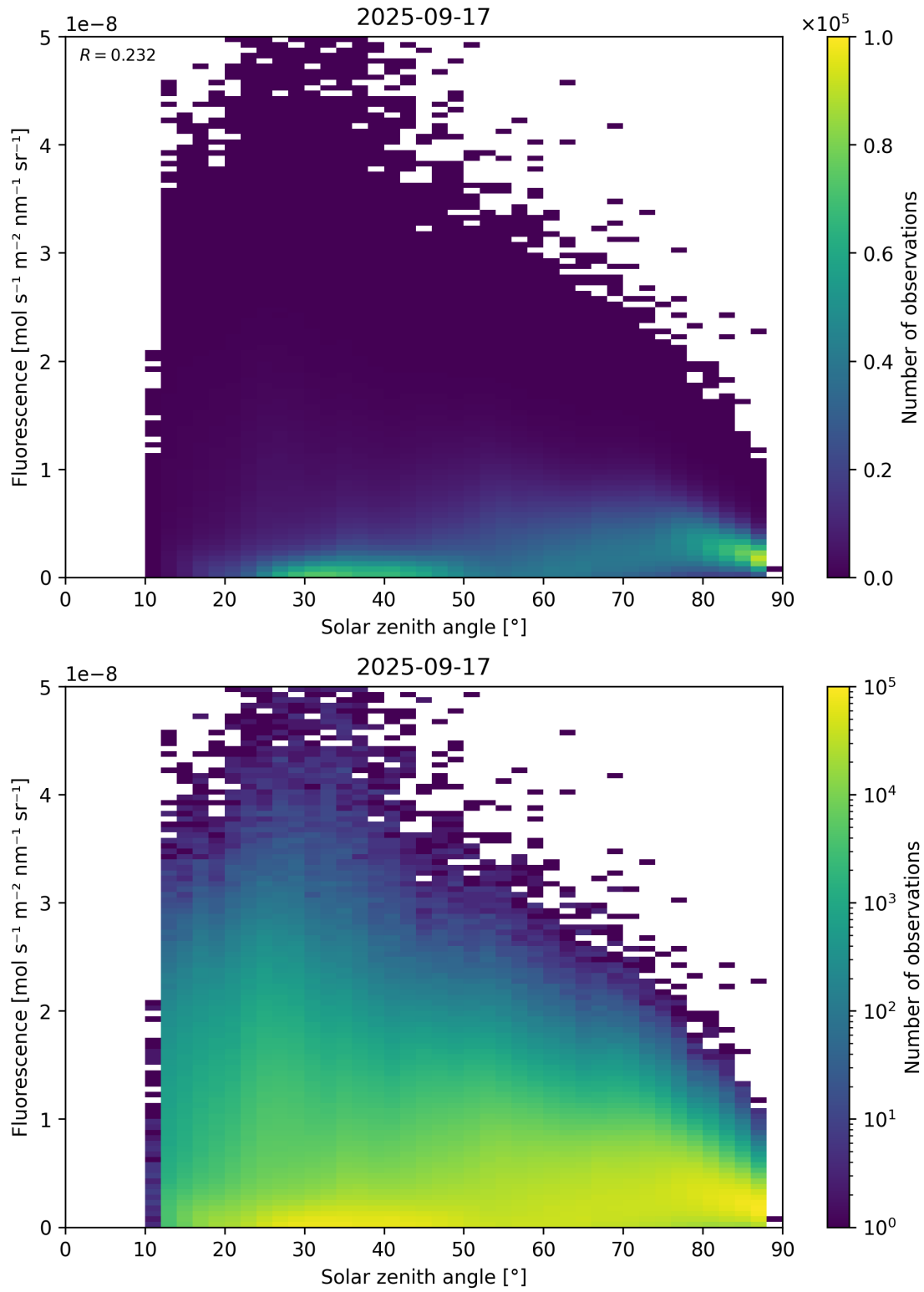
Figure 112: Scatter density plot of “Solar zenith angle” against “Fluorescence” for 2025-09-16 to 2025-09-18.
