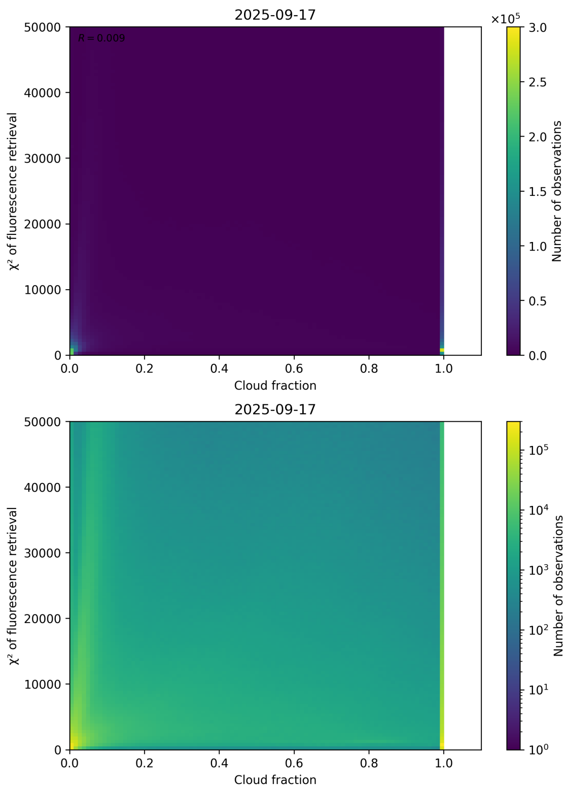
Figure 71: Scatter density plot of “Cloud fraction” against “ \chi^2 of fluorescence retrieval” for 2025-09-16 to 2025-09-18.
