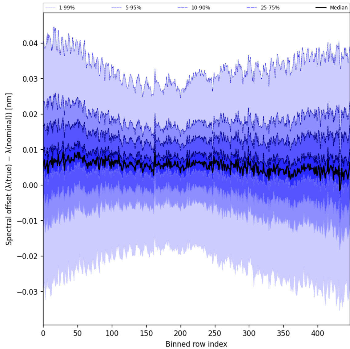
Figure 62: Along track statistics of “Spectral offset ( \lambda_{\text{true}} - \lambda_{\text{nominal}} )” for 2025-09-16 to 2025-09-18
