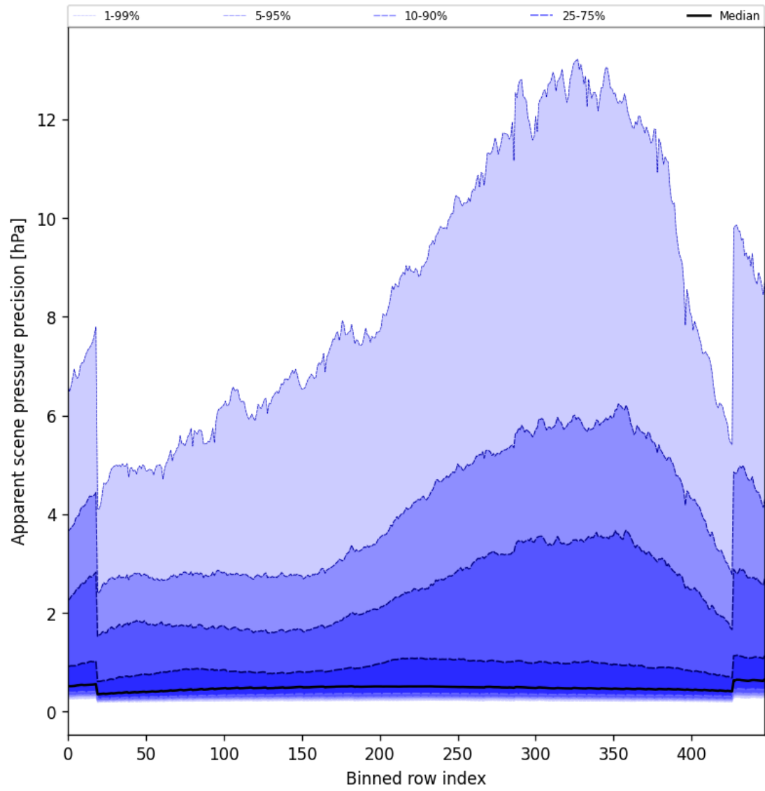
Figure 54: Along track statistics of “Apparent scene pressure precision” for 2025-09-16 to 2025-09-18
