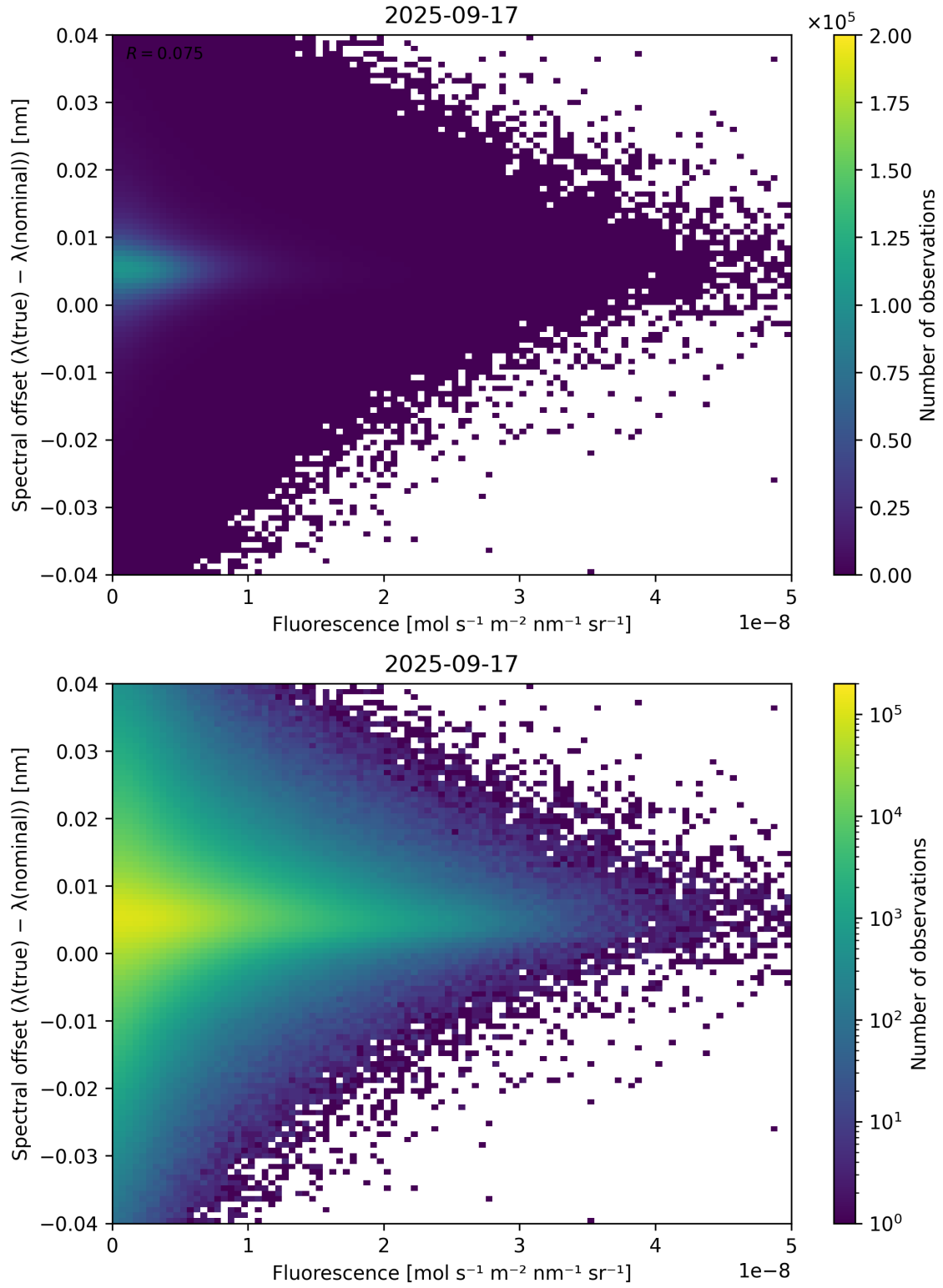
Figure 87: Scatter density plot of “Fluorescence” against “Spectral offset ( \lambda_{\text{true}} - \lambda_{\text{nominal}} )” for 2025-09-16 to 2025-09-18.
