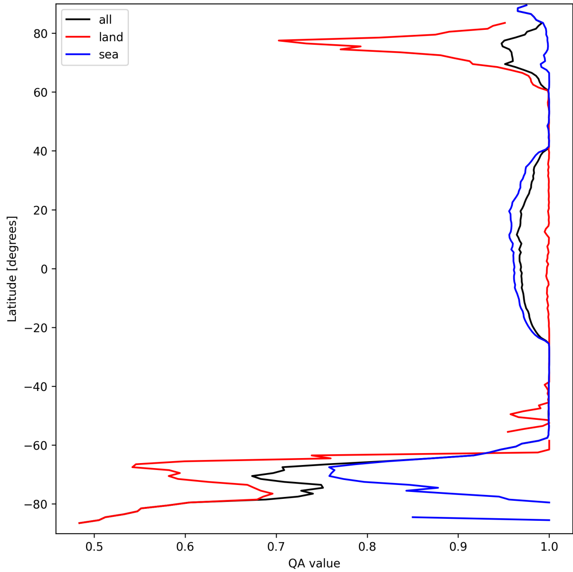
Figure 12: Zonal average of “QA value” for 2025-09-16 to 2025-09-18.
