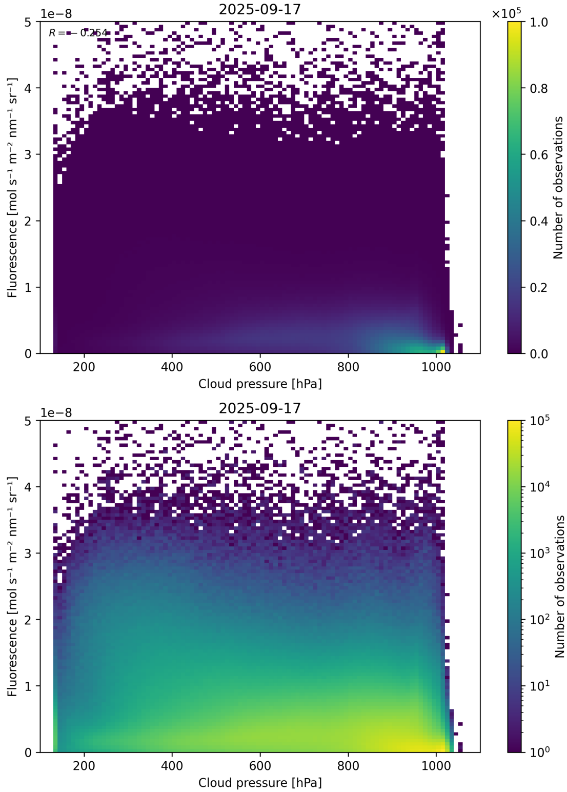
Figure 80: Scatter density plot of “Cloud pressure” against “Fluorescence” for 2025-09-16 to 2025-09-18.
