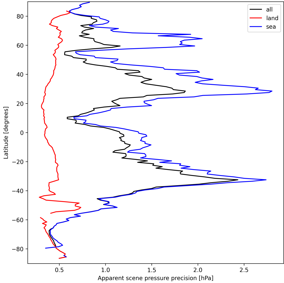
Figure 20: Zonal average of “Apparent scene pressure precision” for 2025-09-16 to 2025-09-18.
