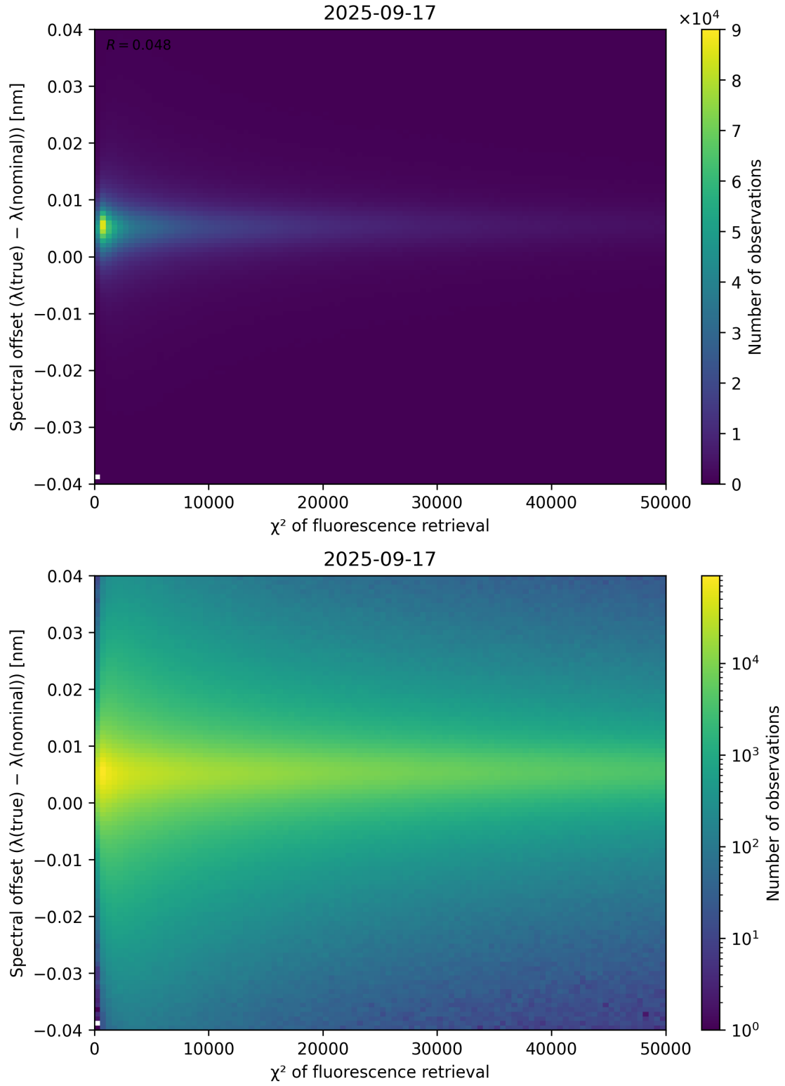
Figure 69: Scatter density plot of “ \chi^2 of fluorescence retrieval” against “Spectral offset ( \lambda_{\text{true}} - \lambda_{\text{nominal}} )” for 2025-09-16 to 2025-09-18.
