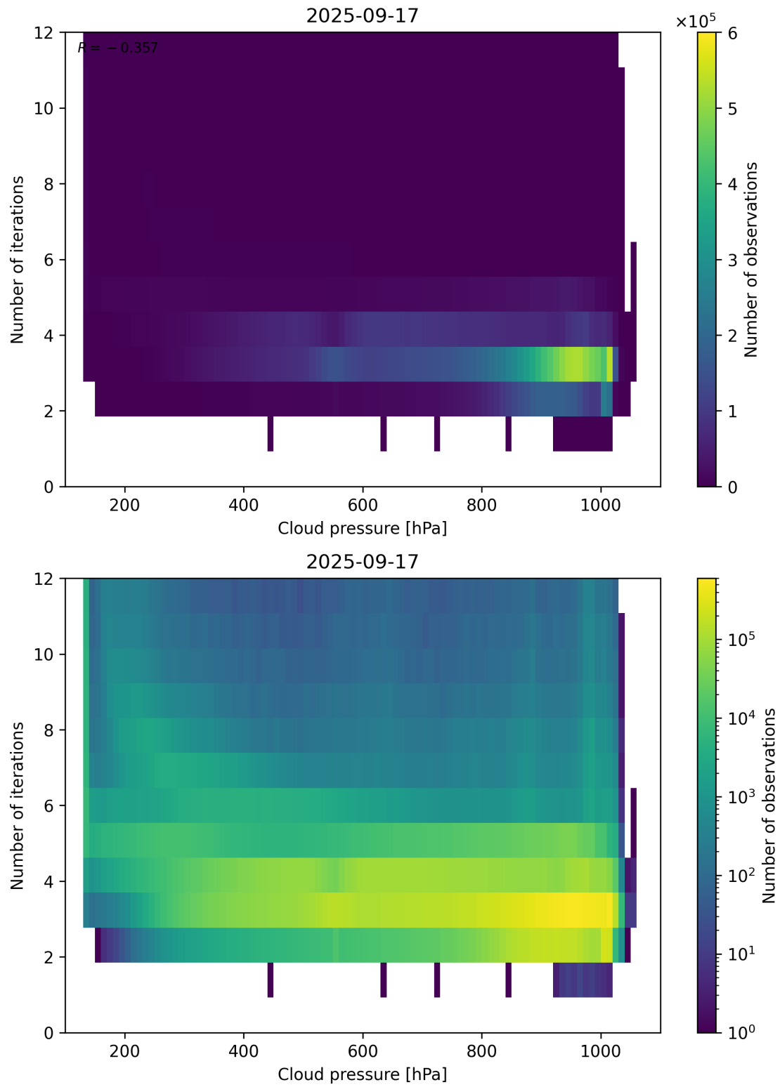
Figure 81: Scatter density plot of “Cloud pressure” against “Number of iterations” for 2025-09-16 to 2025-09-18.
