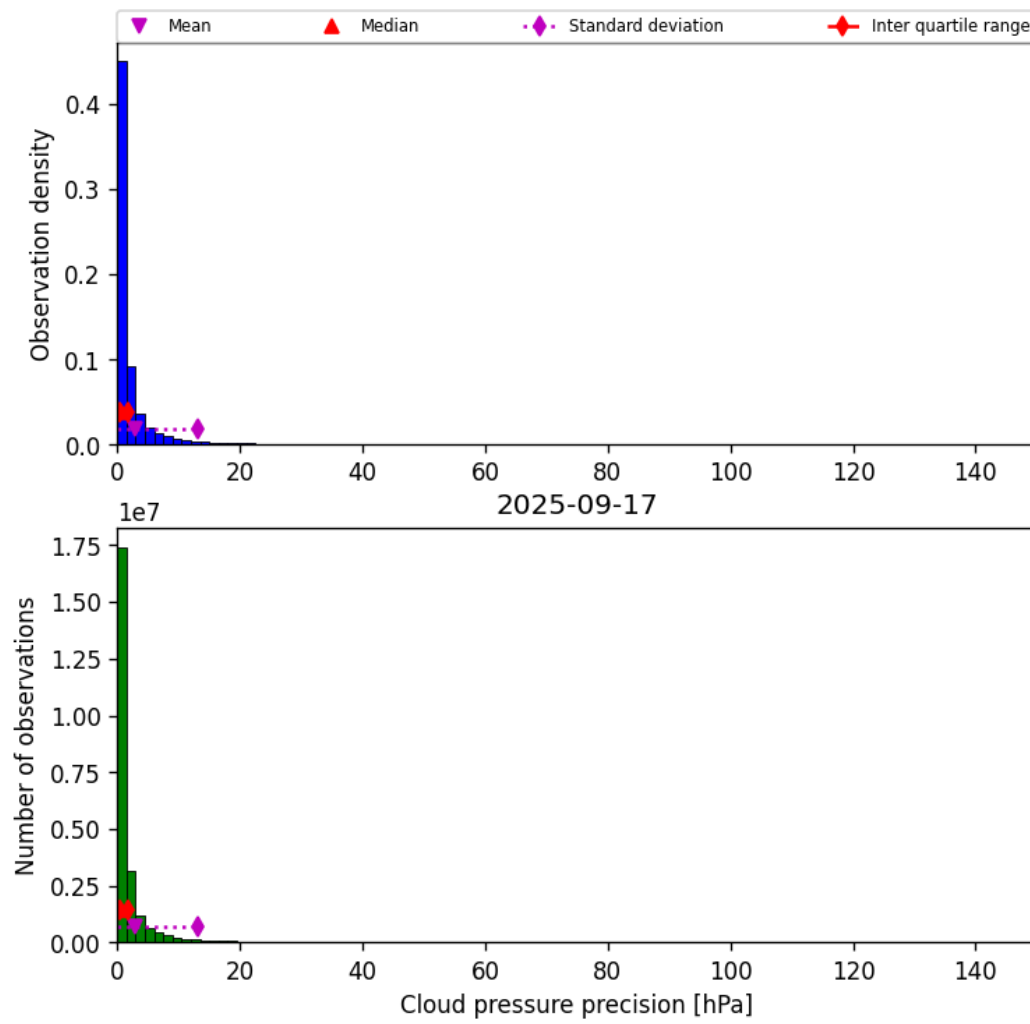
Figure 31: Histogram of “Cloud pressure precision” for 2025-09-16 to 2025-09-18
