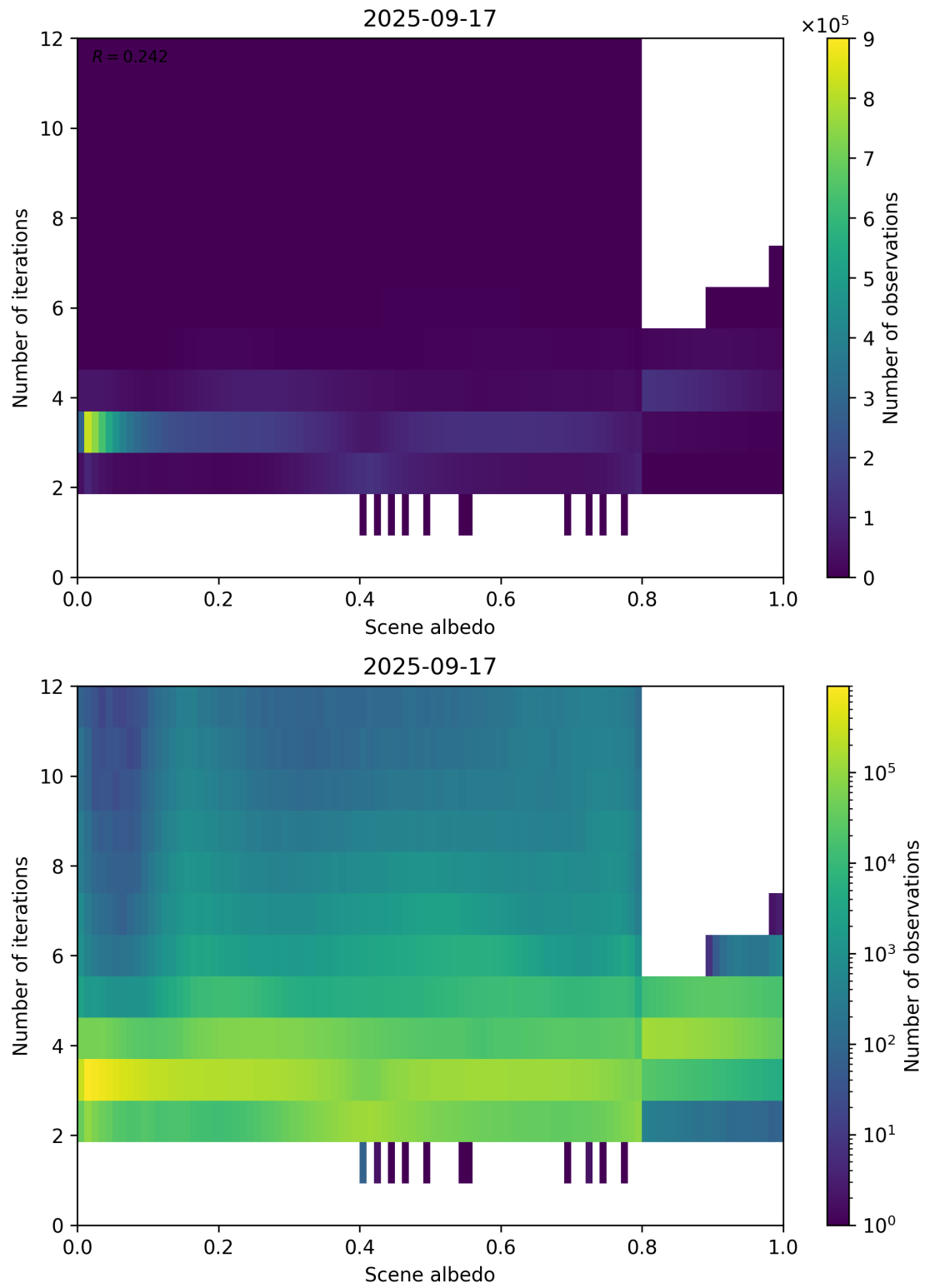
Figure 105: Scatter density plot of “Scene albedo” against “Number of iterations” for 2025-09-16 to 2025-09-18.
