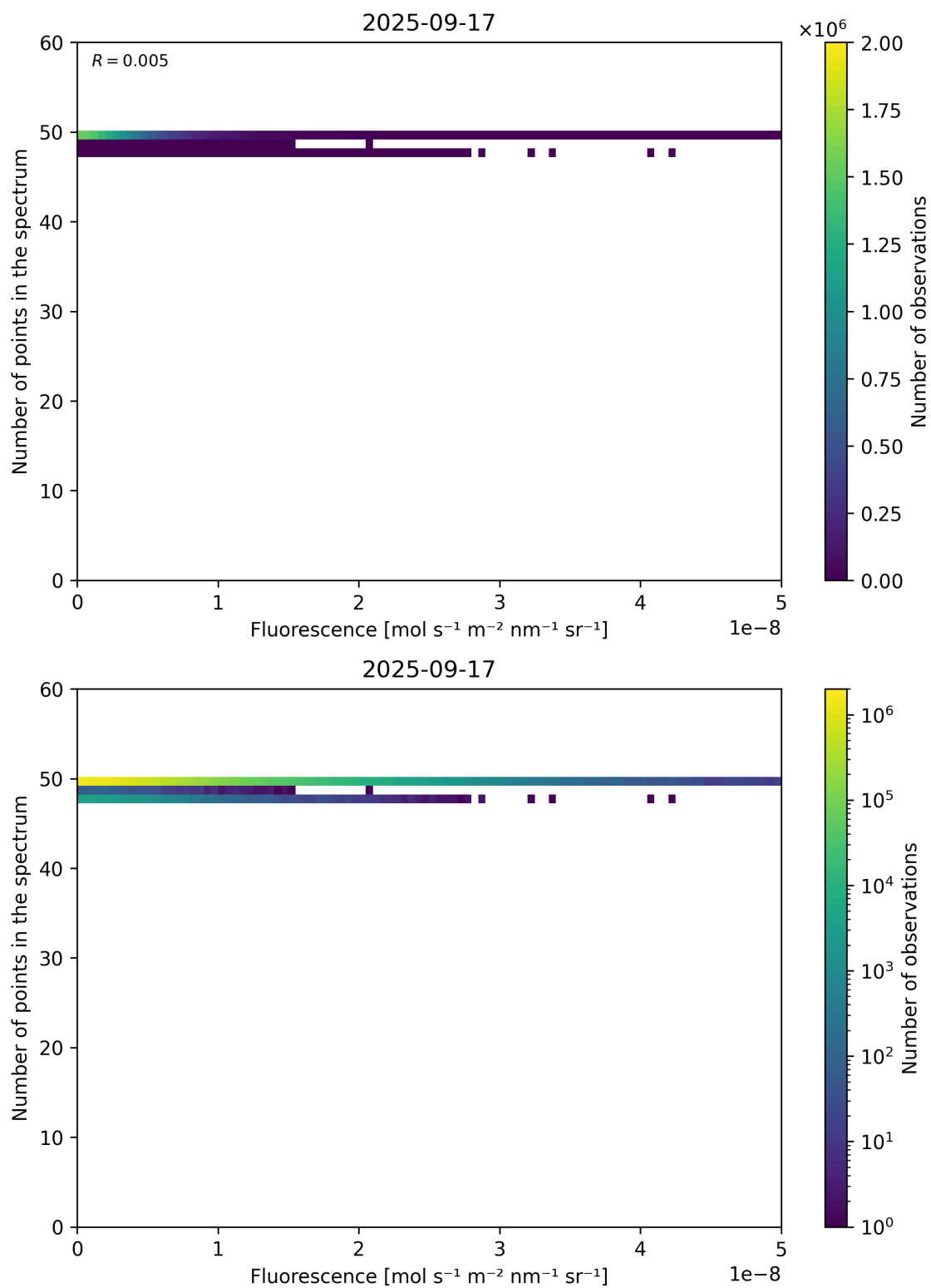
Figure 86: Scatter density plot of “Fluorescence” against “Number of points in the spectrum” for 2025-09-16 to 2025-09-18.
