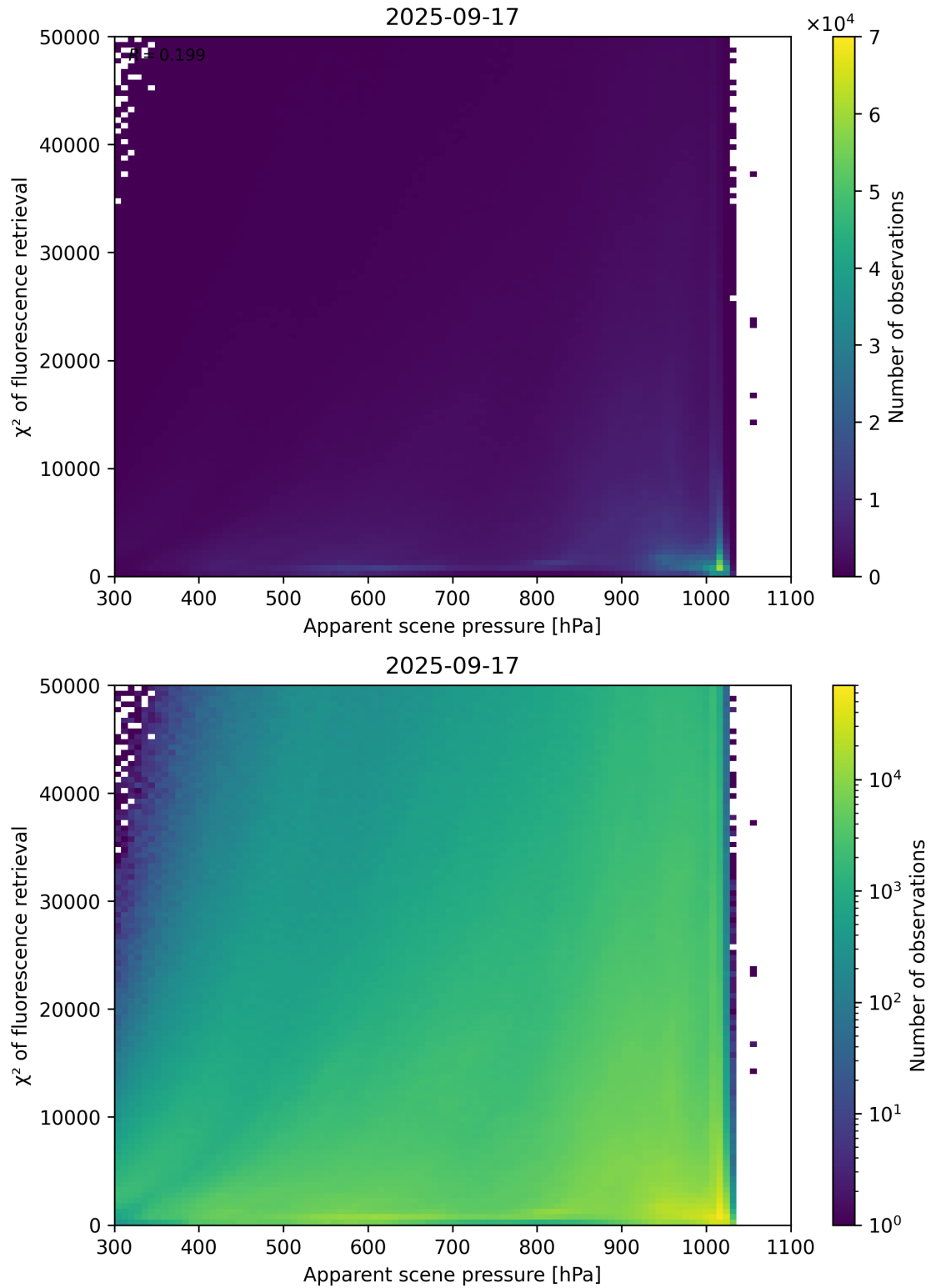
Figure 63: Scatter density plot of “Apparent scene pressure” against “ \chi^2 of fluorescence retrieval” for 2025-09-16 to 2025-09-18.
