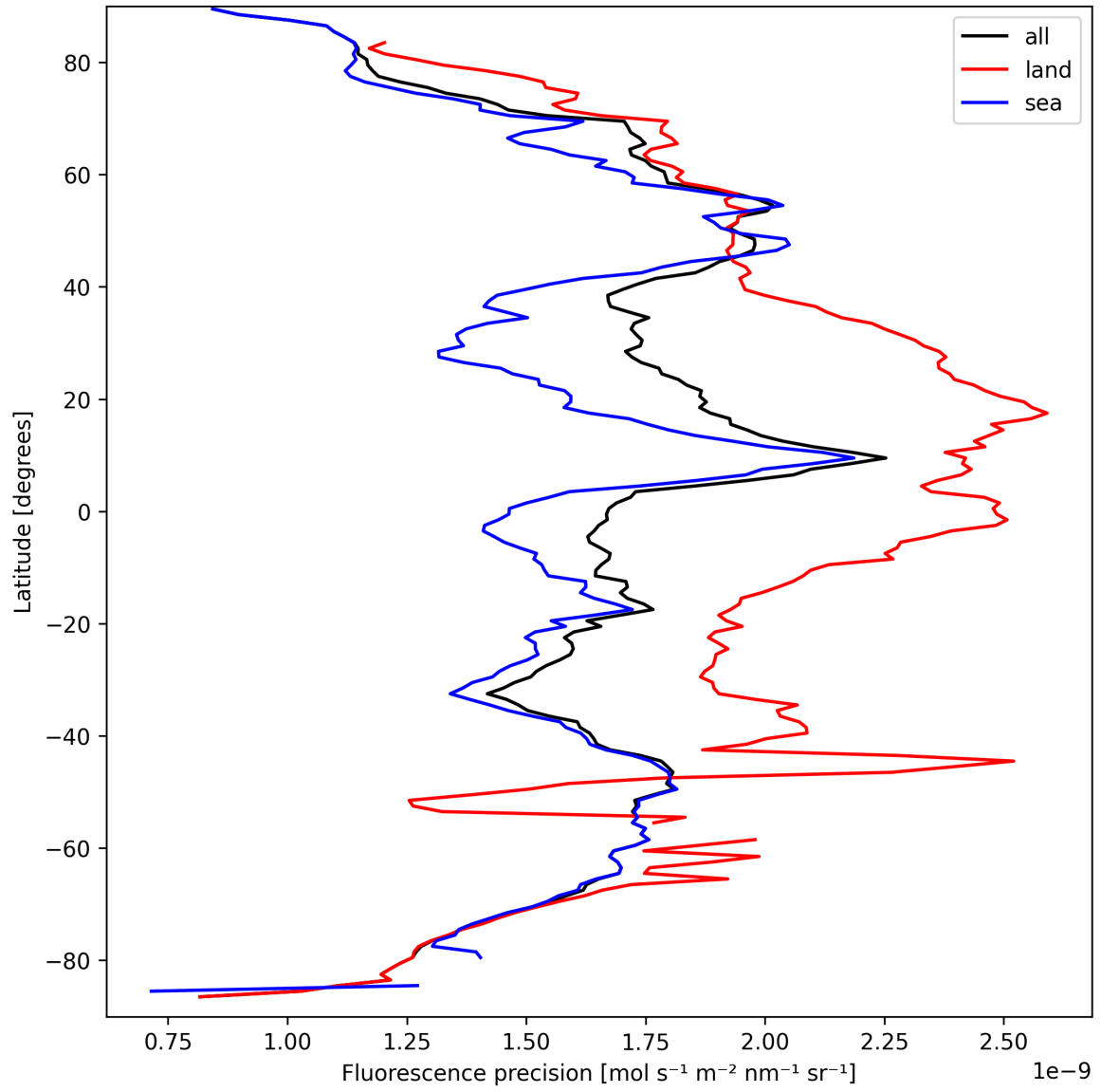
Figure 24: Zonal average of “Fluorescence precision” for 2025-09-16 to 2025-09-18.
