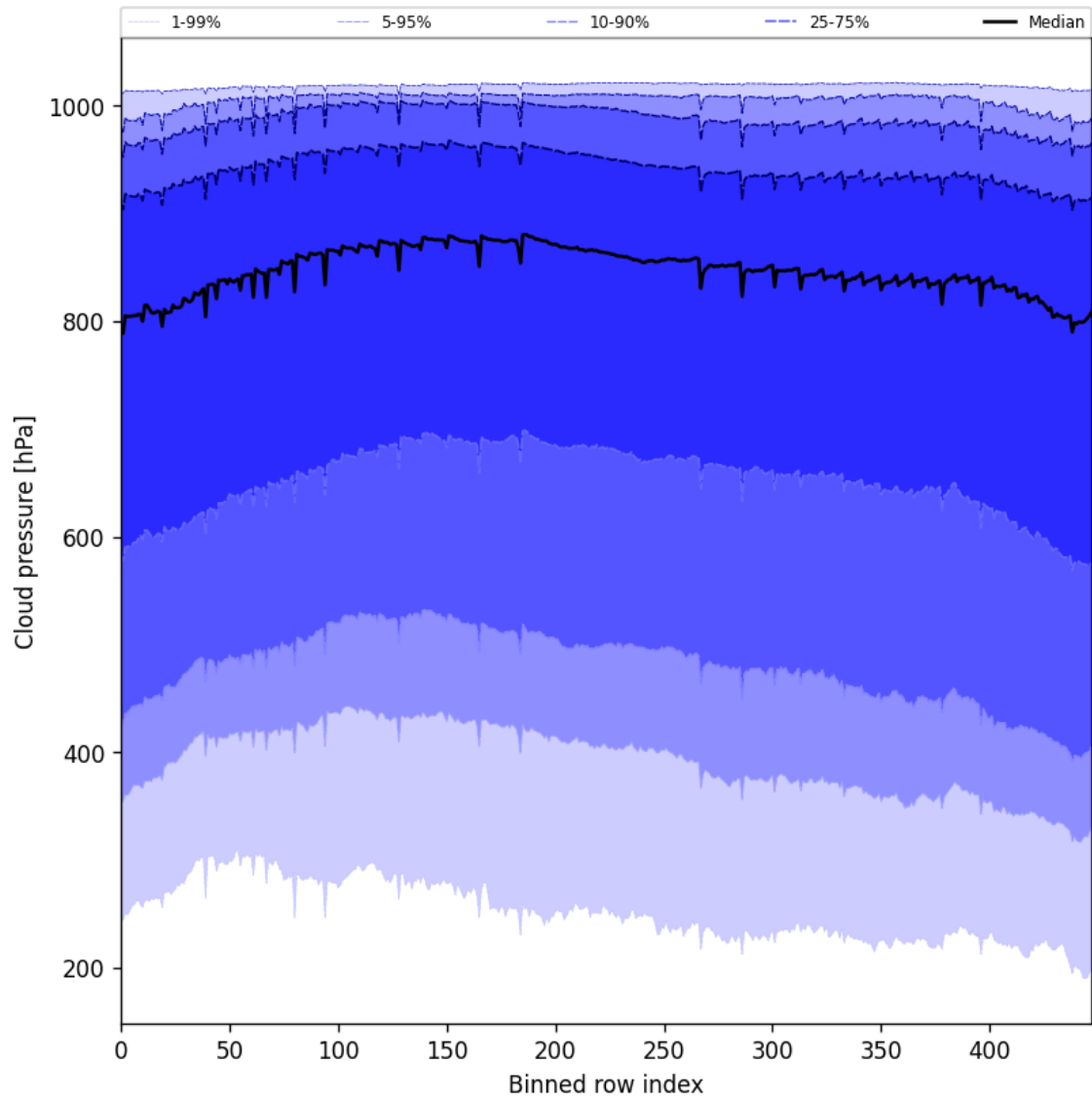
Figure 47: Along track statistics of “Cloud pressure” for 2025-09-16 to 2025-09-18
