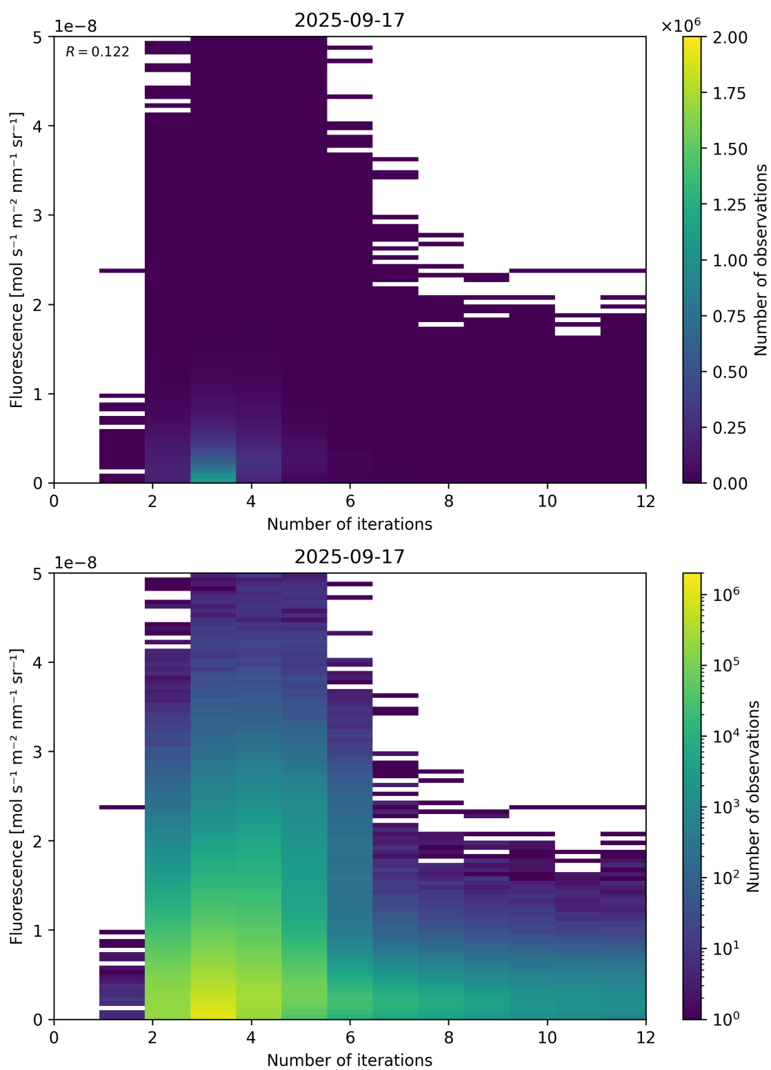
Figure 98: Scatter density plot of “Number of iterations” against “Fluorescence” for 2025-09-16 to 2025-09-18.
