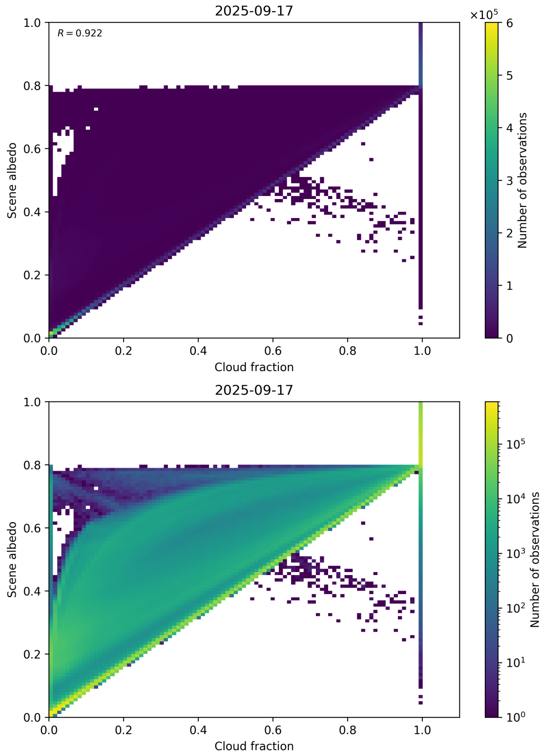
Figure 75: Scatter density plot of “Cloud fraction” against “Scene albedo” for 2025-09-16 to 2025-09-18.
