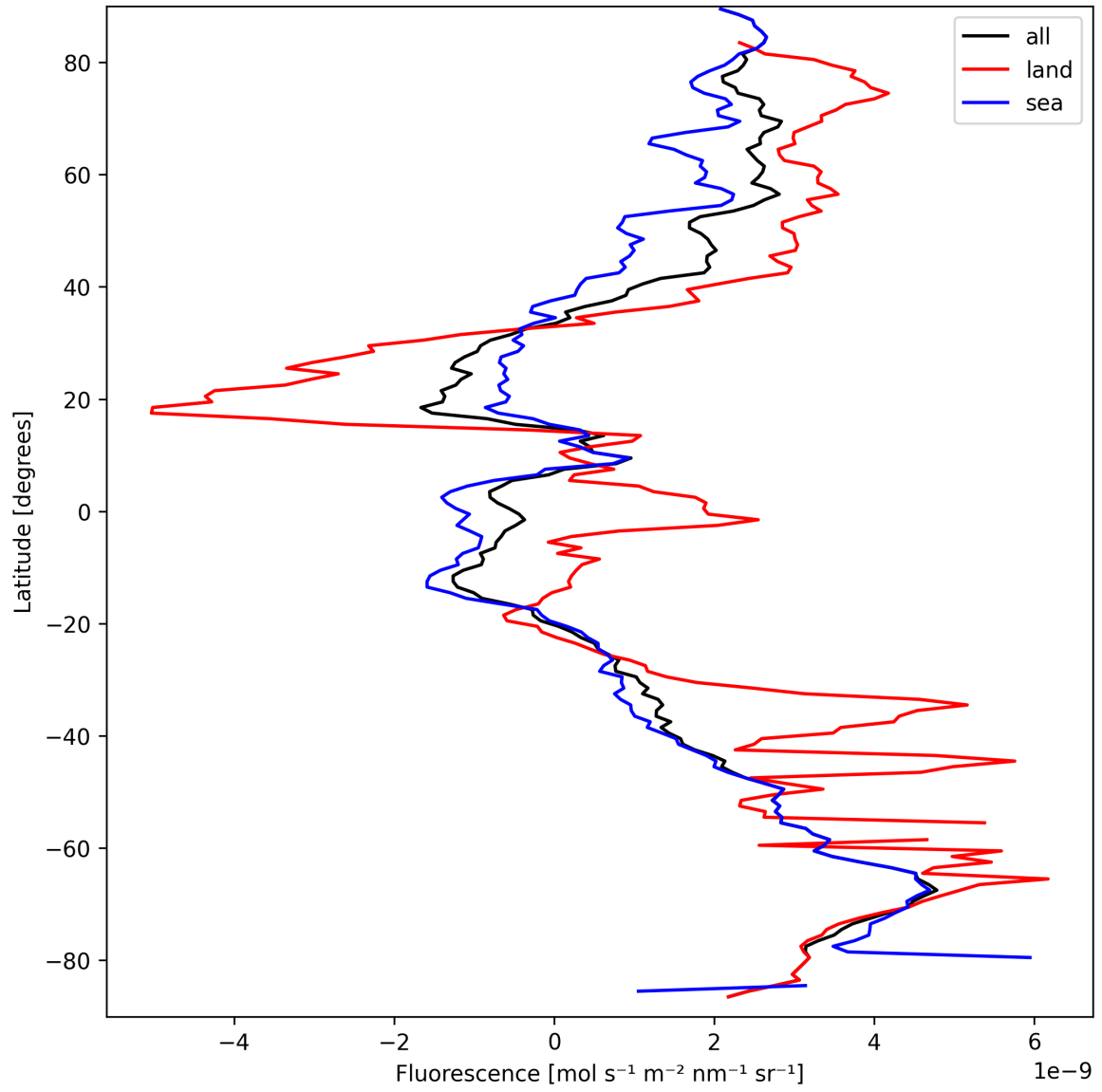
Figure 23: Zonal average of “Fluorescence” for 2025-09-16 to 2025-09-18.
