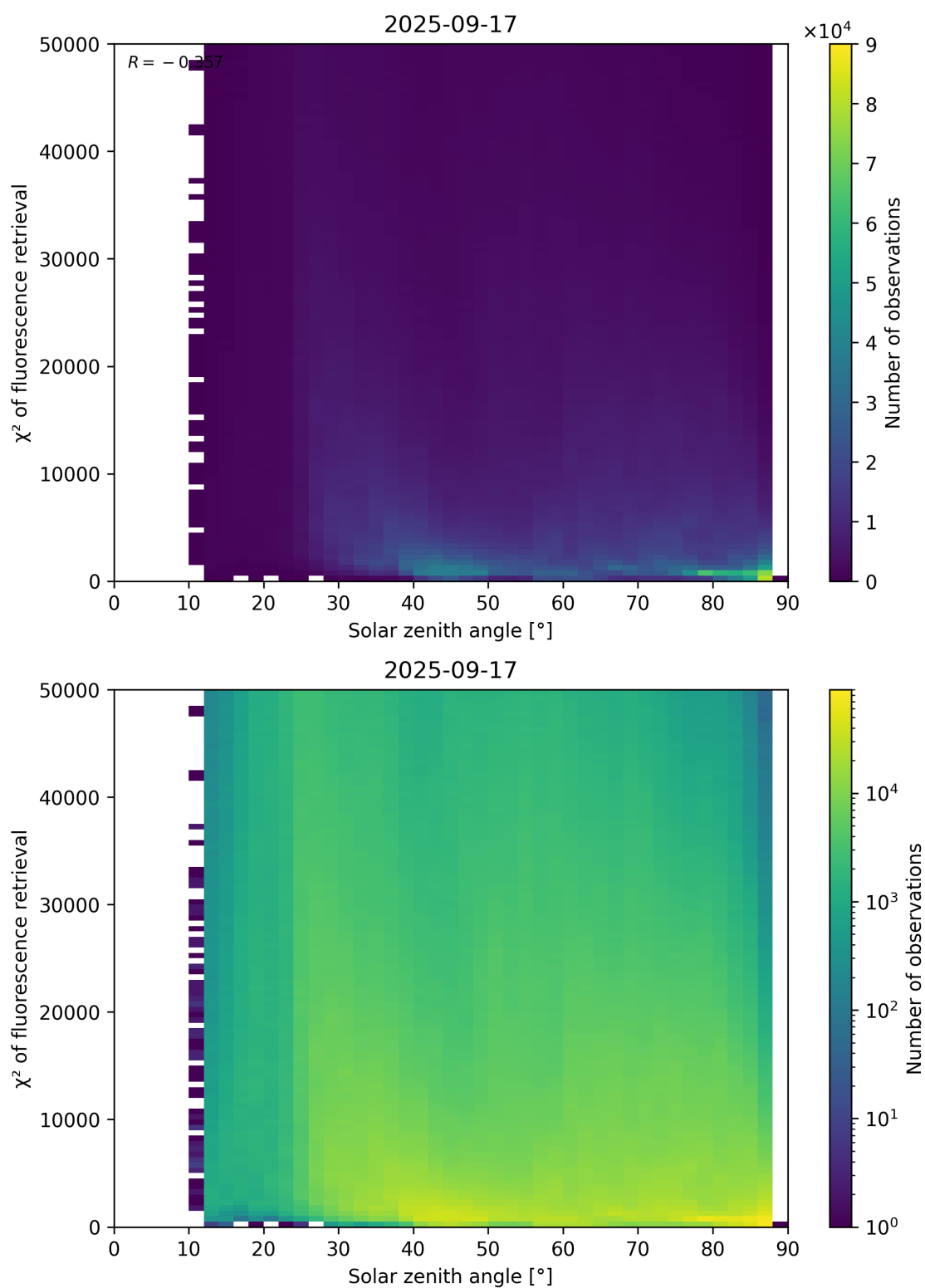
Figure 109: Scatter density plot of “Solar zenith angle” against “ \chi^2 of fluorescence retrieval” for 2025-09-16 to 2025-09-18.
