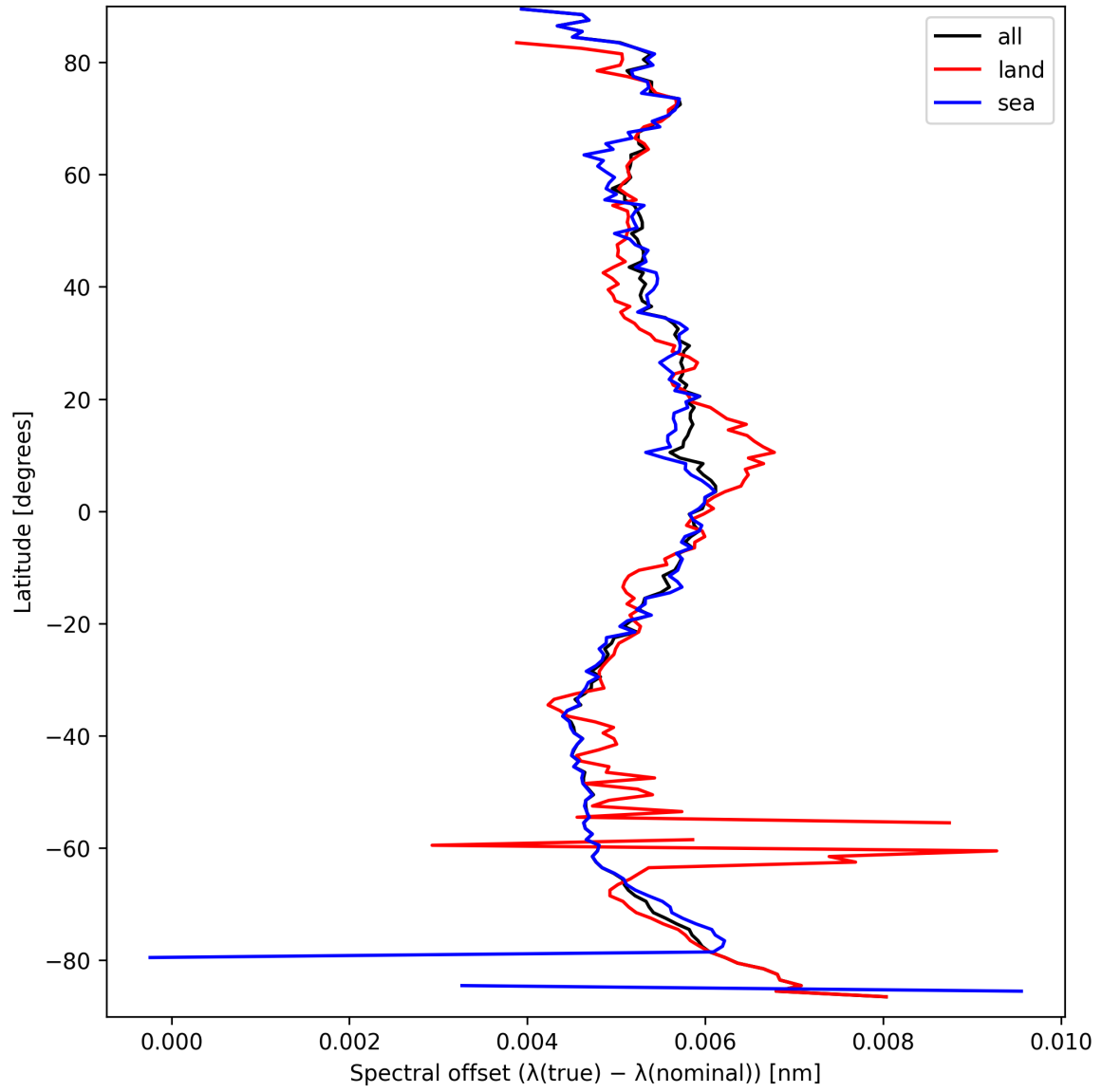
Figure 28: Zonal average of “Spectral offset ( \lambda_{\text{true}} - \lambda_{\text{nominal}} )” for 2025-09-16 to 2025-09-18.
