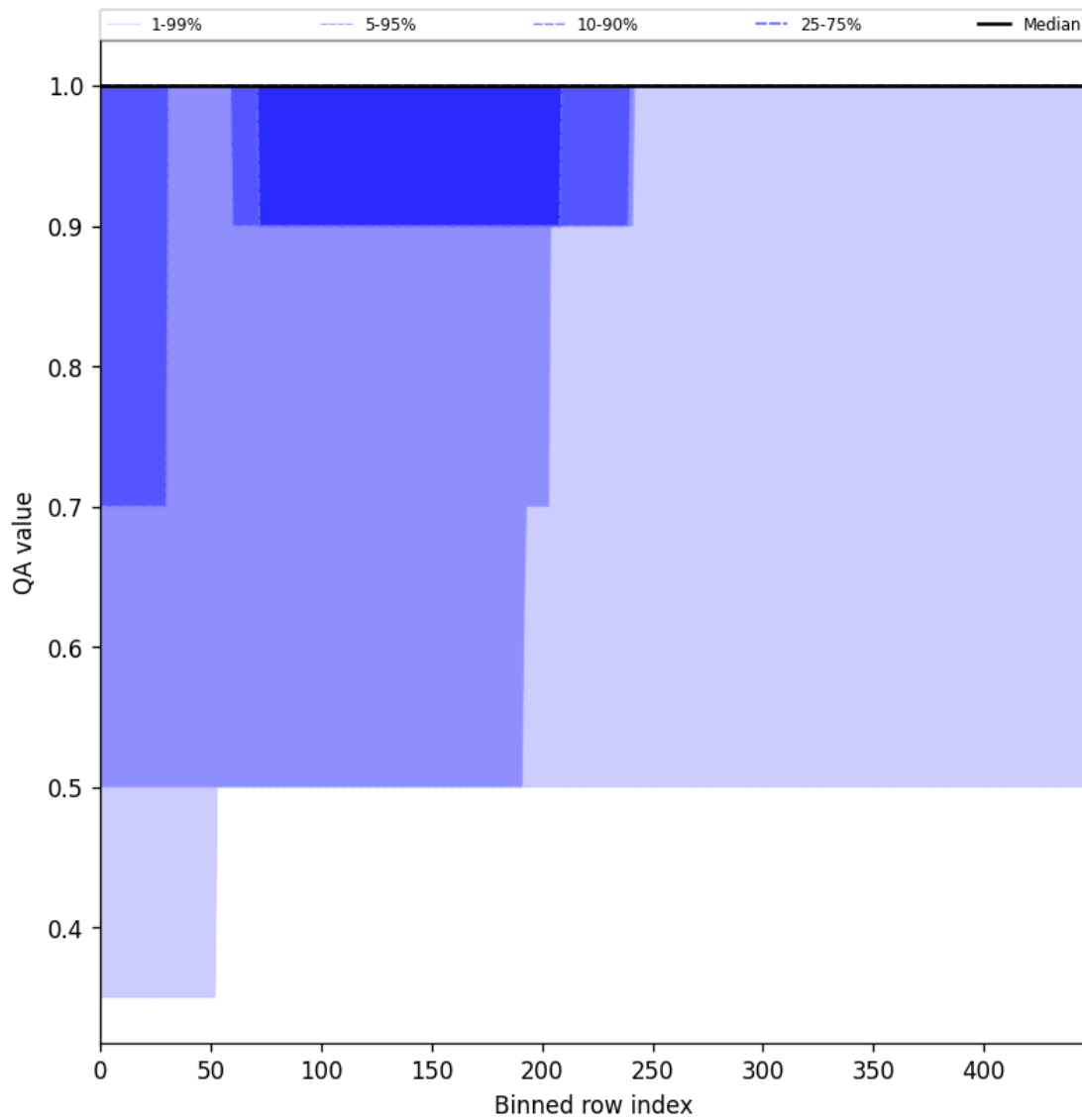
Figure 46: Along track statistics of “QA value” for 2025-09-16 to 2025-09-18
