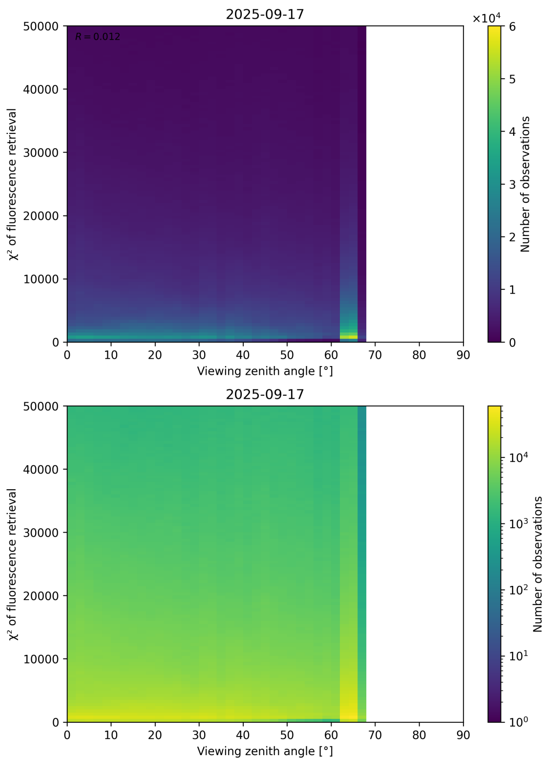
Figure 119: Scatter density plot of “Viewing zenith angle” against “ \chi^2 of fluorescence retrieval” for 2025-09-16 to 2025-09-18.
