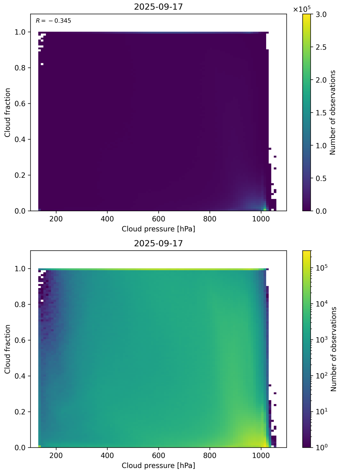
Figure 79: Scatter density plot of “Cloud pressure” against “Cloud fraction” for 2025-09-16 to 2025-09-18.
