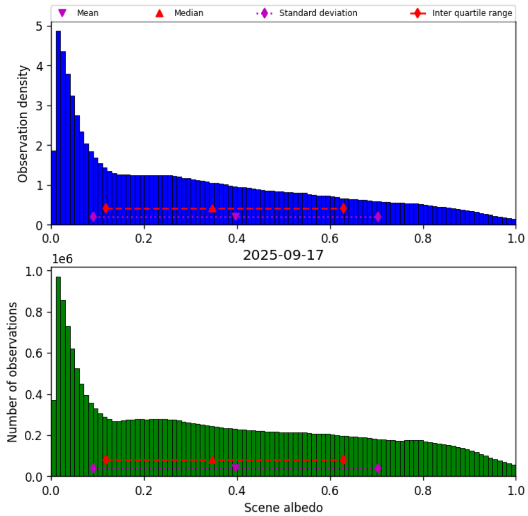
Figure 34: Histogram of “Scene albedo” for 2025-09-16 to 2025-09-18
