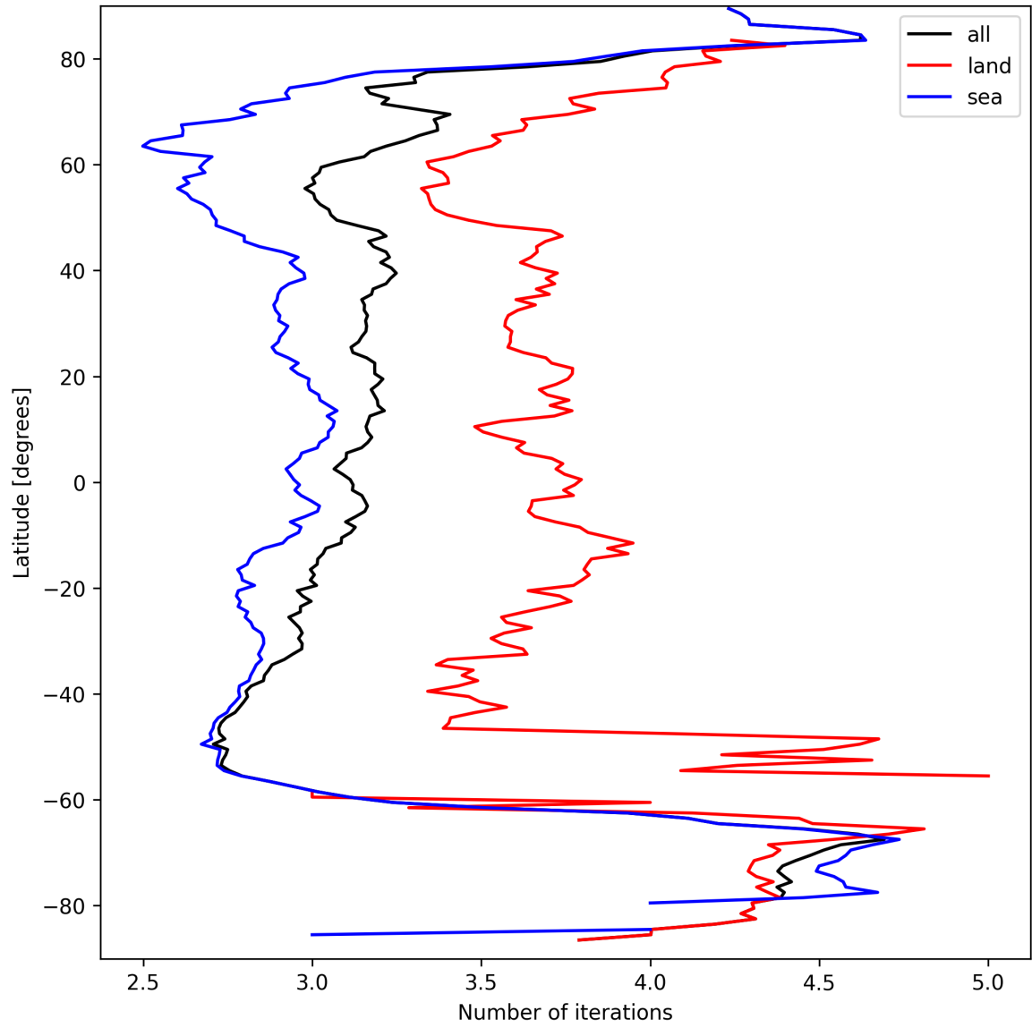
Figure 22: Zonal average of “Number of iterations” for 2025-09-16 to 2025-09-18.
