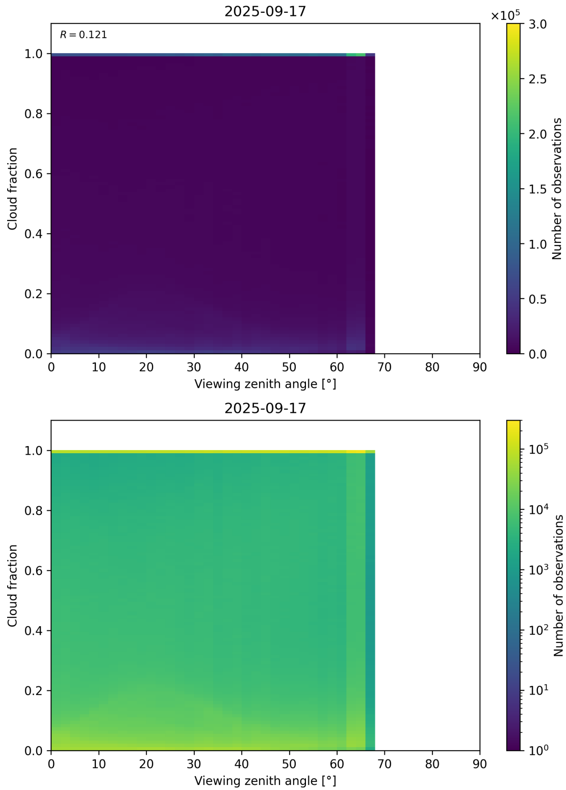
Figure 120: Scatter density plot of “Viewing zenith angle” against “Cloud fraction” for 2025-09-16 to 2025-09-18.
