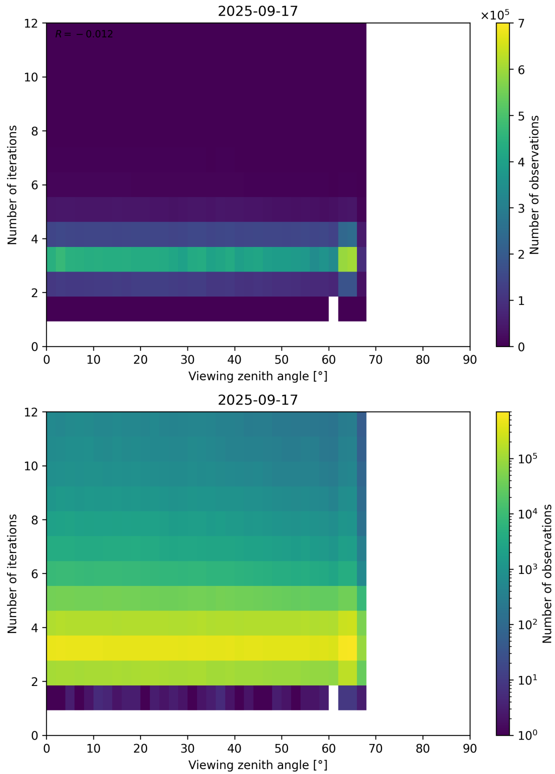
Figure 124: Scatter density plot of “Viewing zenith angle” against “Number of iterations” for 2025-09-16 to 2025-09-18.
