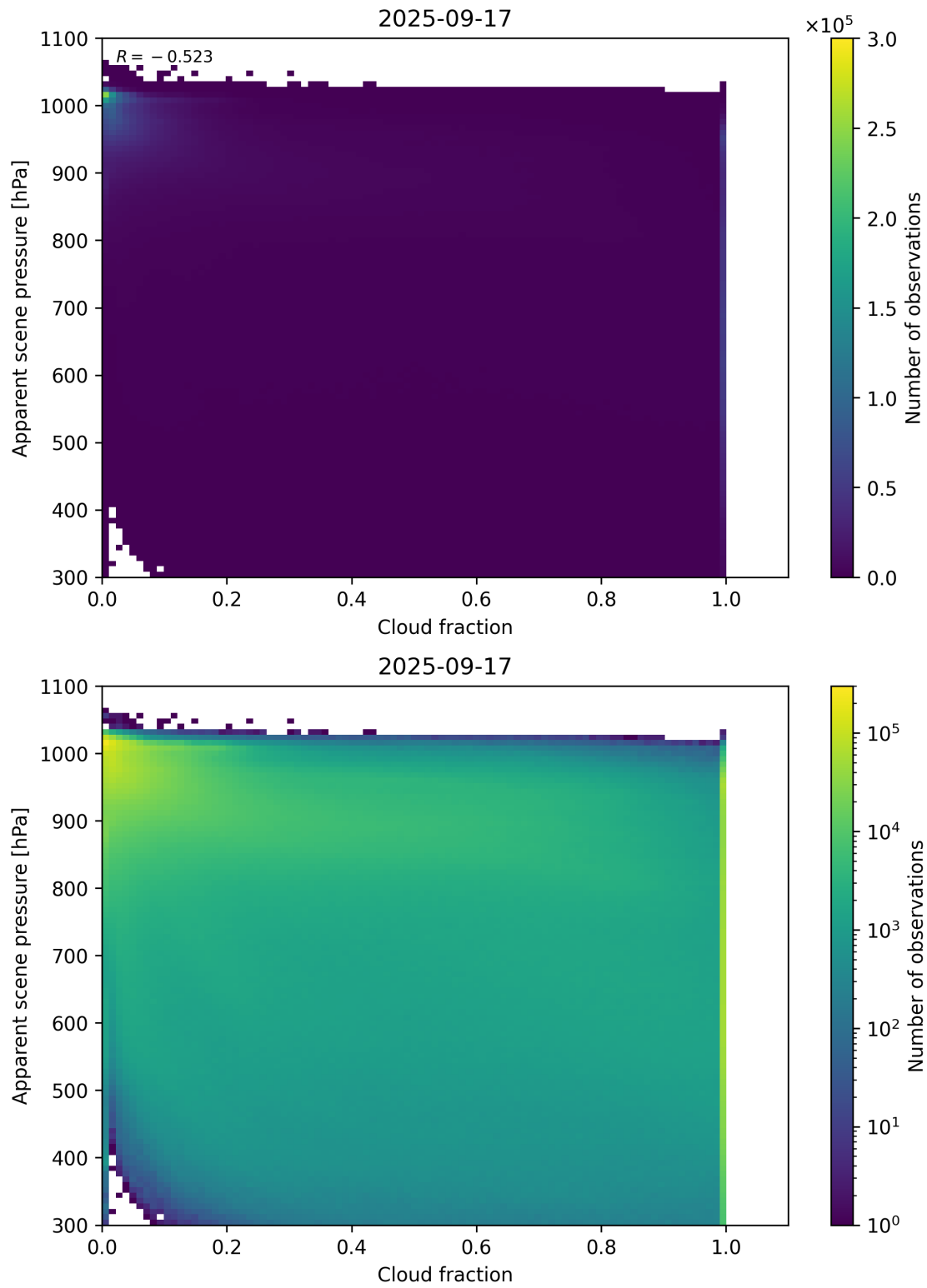
Figure 70: Scatter density plot of “Cloud fraction” against “Apparent scene pressure” for 2025-09-16 to 2025-09-18.
