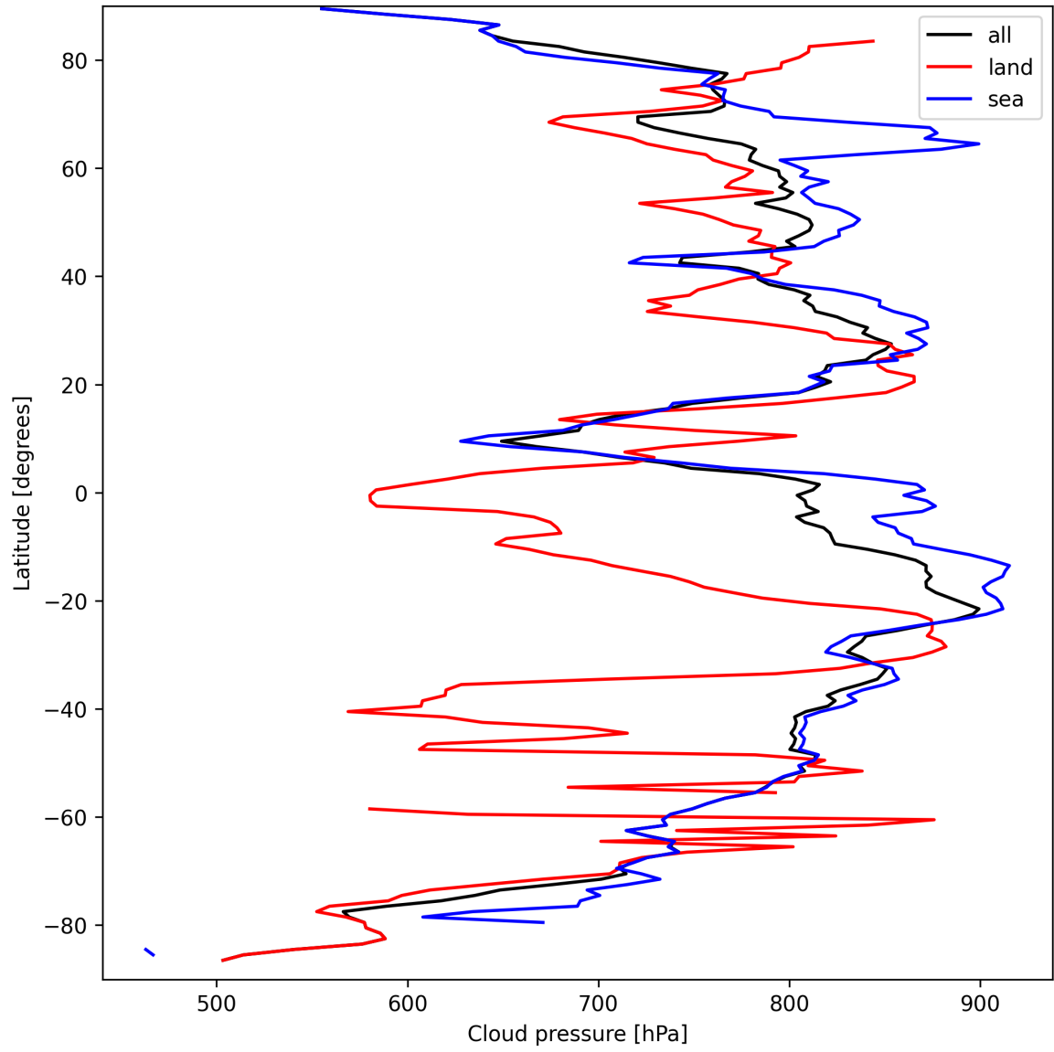
Figure 13: Zonal average of “Cloud pressure” for 2025-09-16 to 2025-09-18.
