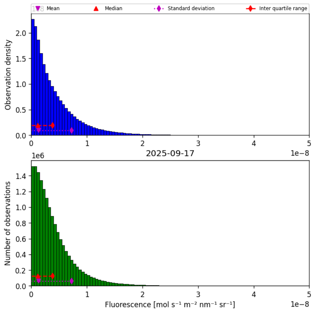
Figure 40: Histogram of “Fluorescence” for 2025-09-16 to 2025-09-18
