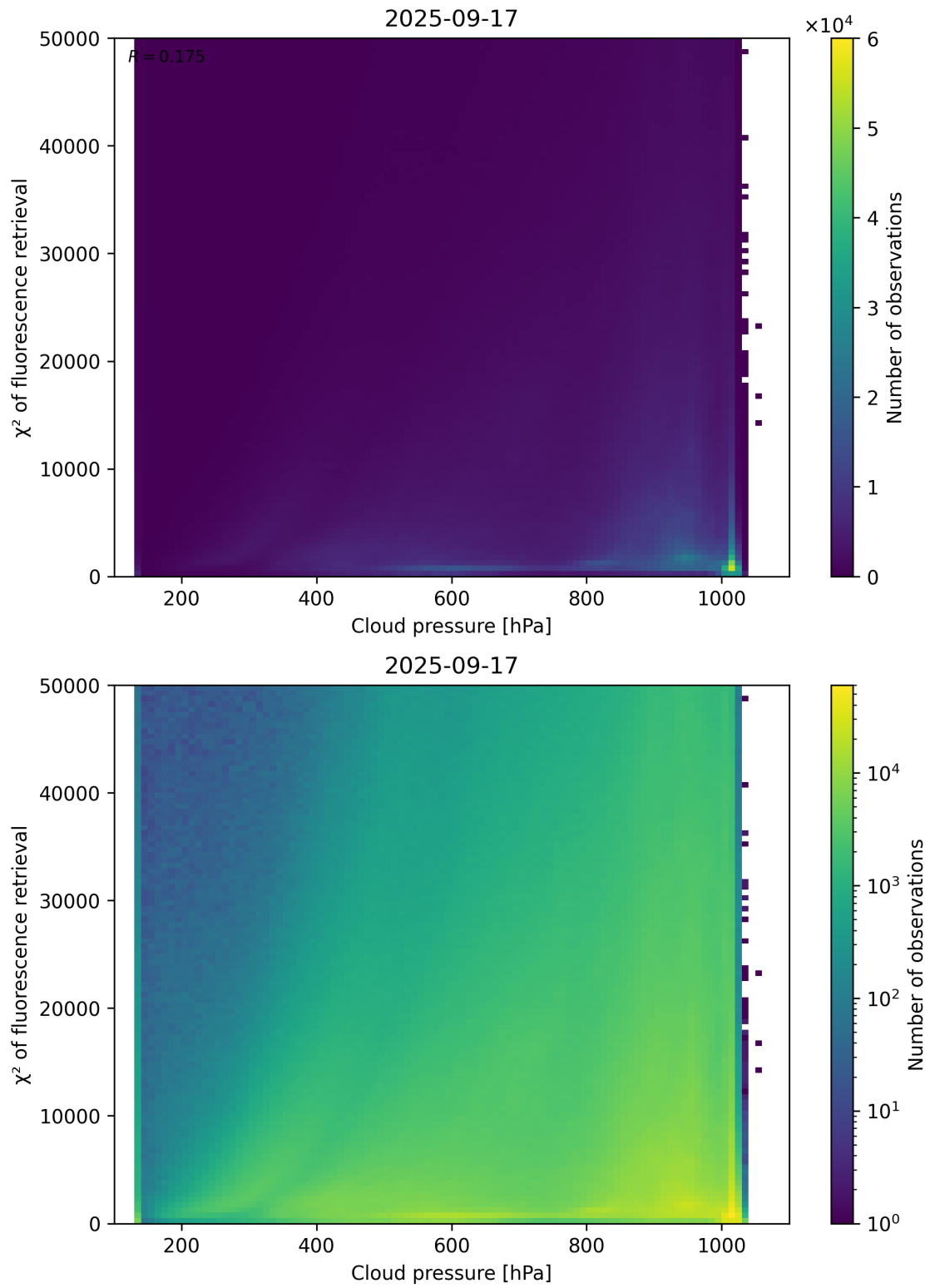
Figure 78: Scatter density plot of “Cloud pressure” against “ \chi^2 of fluorescence retrieval” for 2025-09-16 to 2025-09-18.
