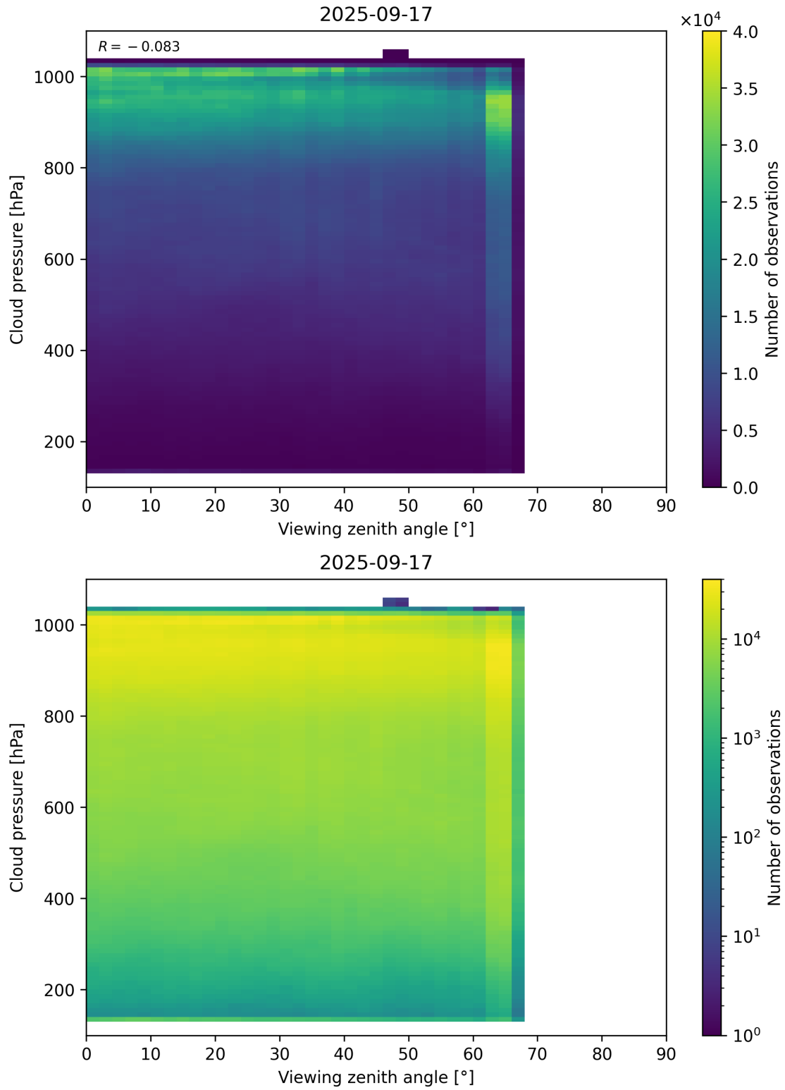
Figure 121: Scatter density plot of “Viewing zenith angle” against “Cloud pressure” for 2025-09-16 to 2025-09-18.
