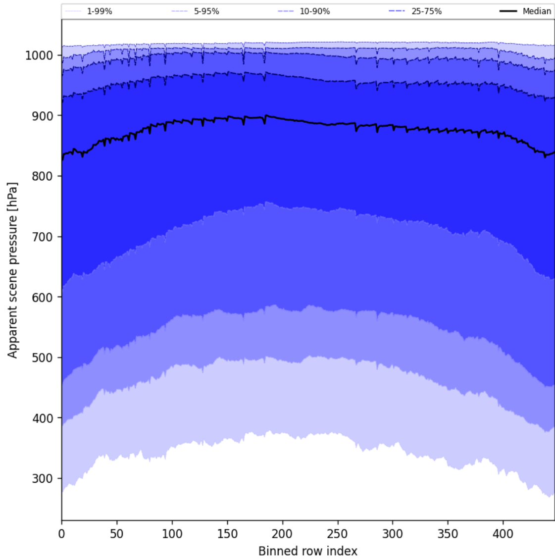
Figure 53: Along track statistics of “Apparent scene pressure” for 2025-09-16 to 2025-09-18
