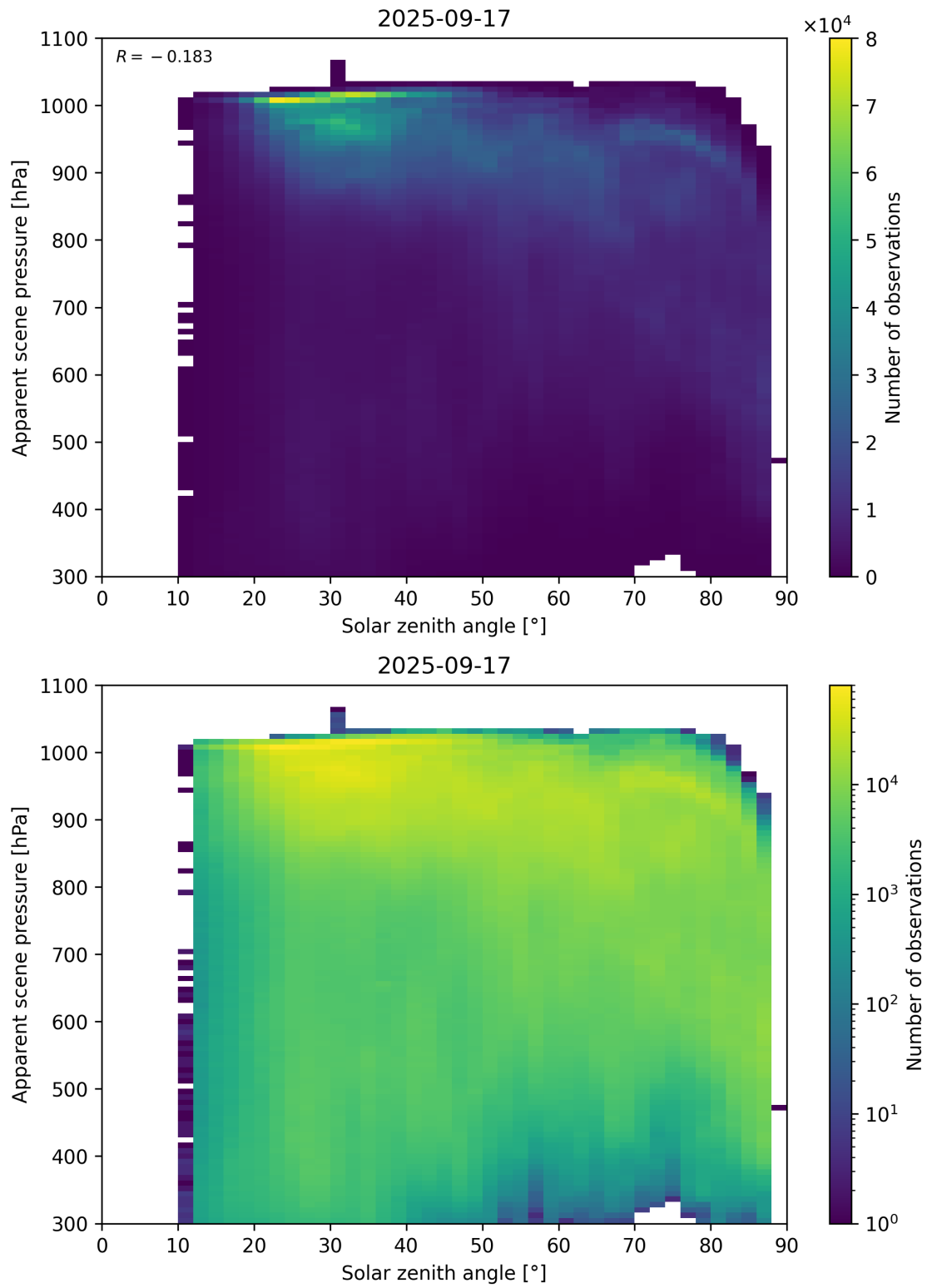
Figure 108: Scatter density plot of “Solar zenith angle” against “Apparent scene pressure” for 2025-09-16 to 2025-09-18.
