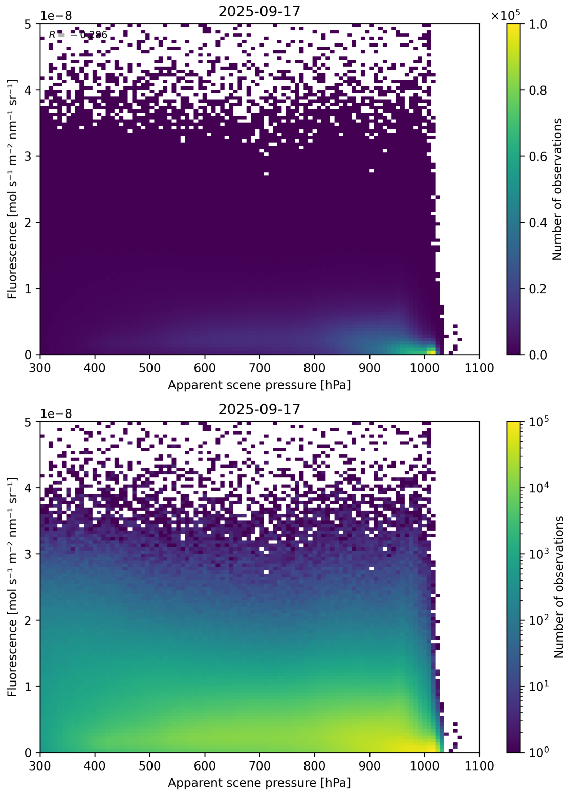
Figure 64: Scatter density plot of “Apparent scene pressure” against “Fluorescence” for 2025-09-16 to 2025-09-18.
