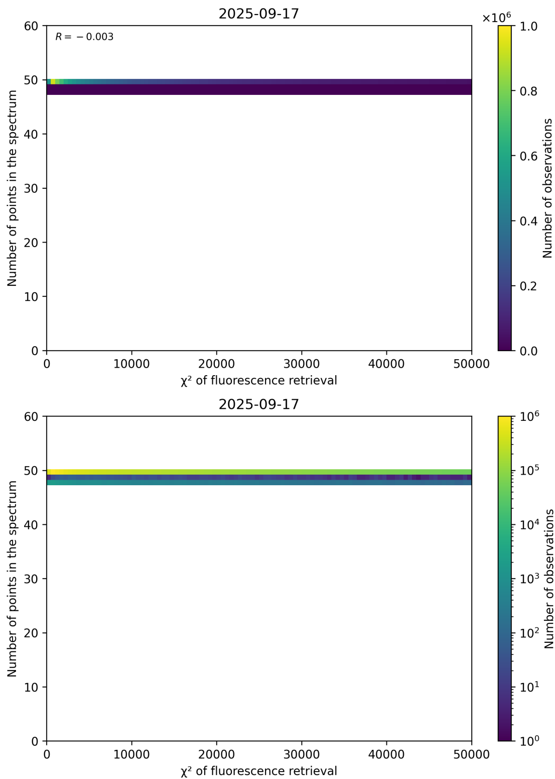
Figure 68: Scatter density plot of " \chi^2 of fluorescence retrieval" against "Number of points in the spectrum" for 2025-09-16 to 2025-09-18.
