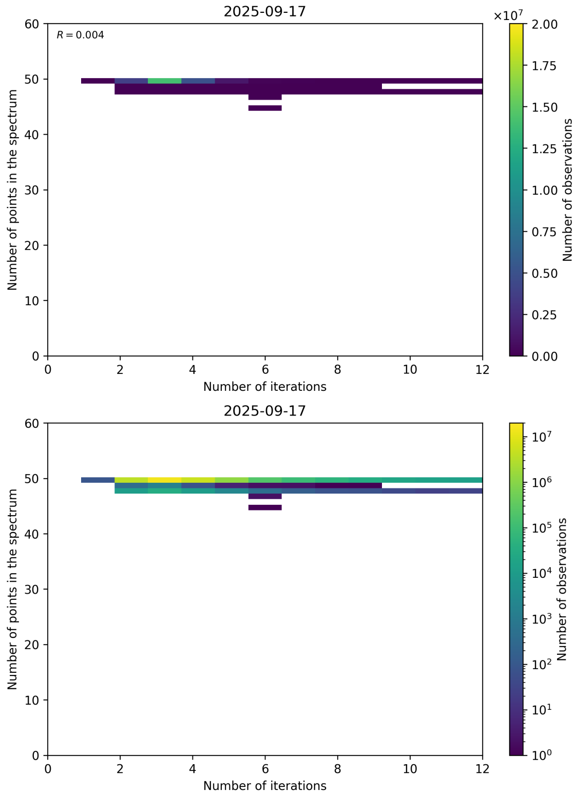
Figure 99: Scatter density plot of “Number of iterations” against “Number of points in the spectrum” for 2025-09-16 to 2025-09-18.
