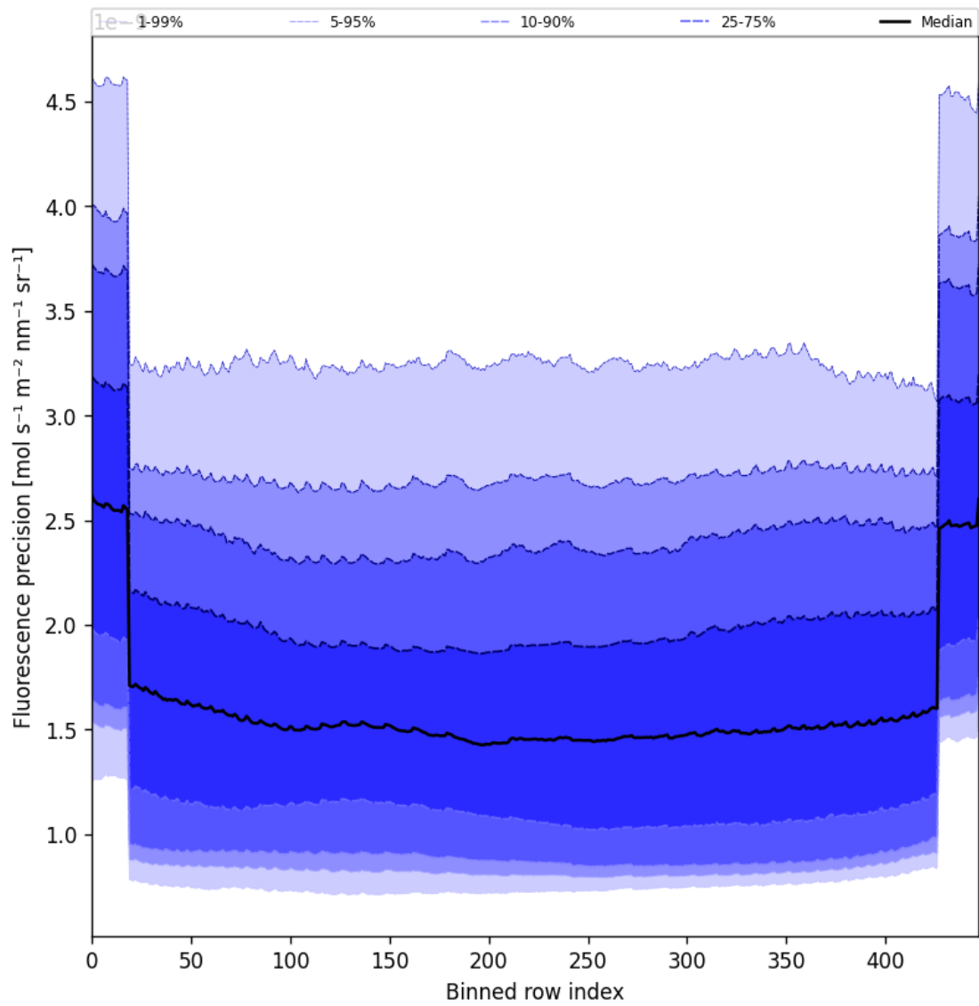
Figure 58: Along track statistics of “Fluorescence precision” for 2025-09-16 to 2025-09-18
