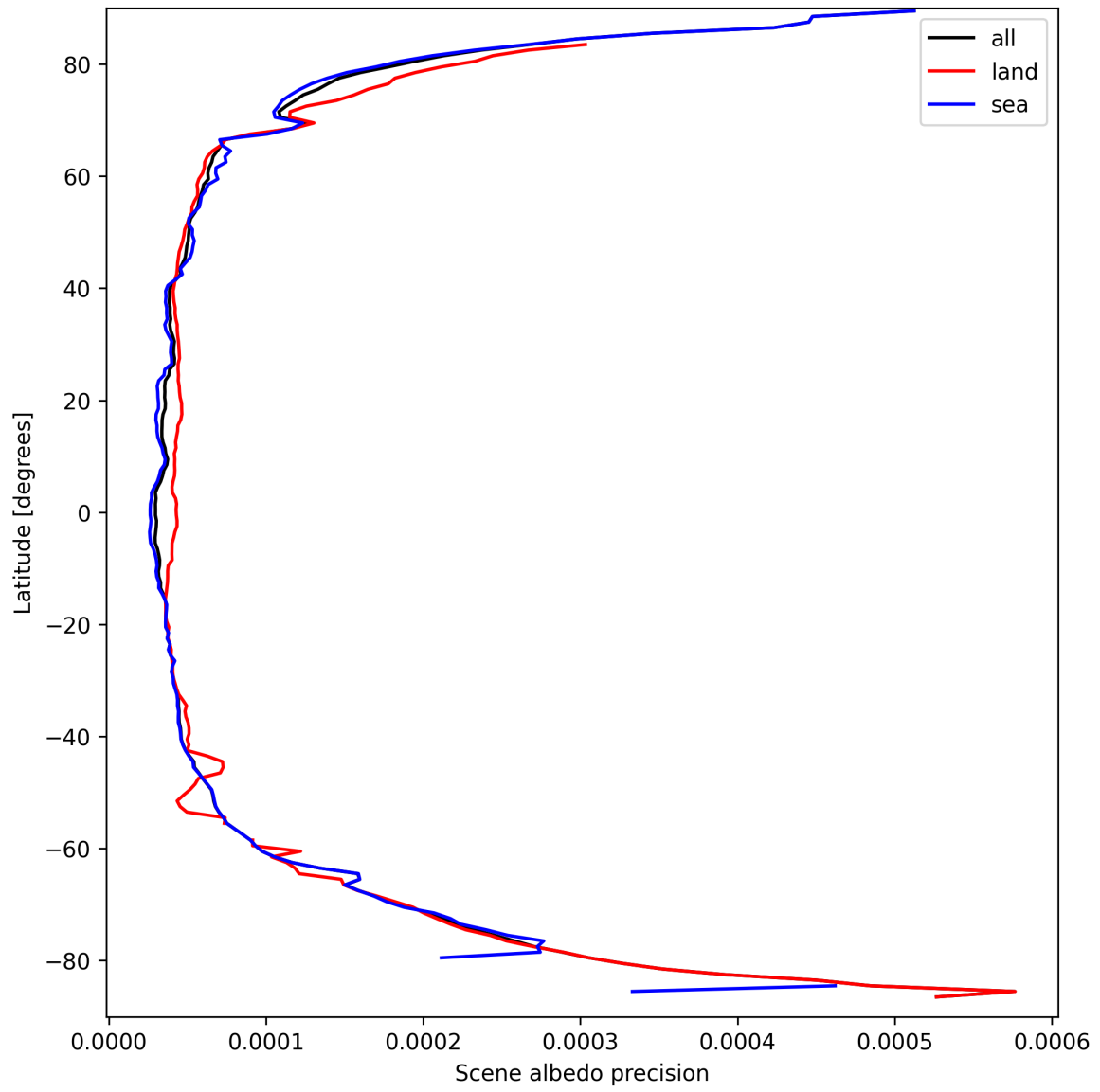
Figure 18: Zonal average of “Scene albedo precision” for 2025-09-16 to 2025-09-18.
