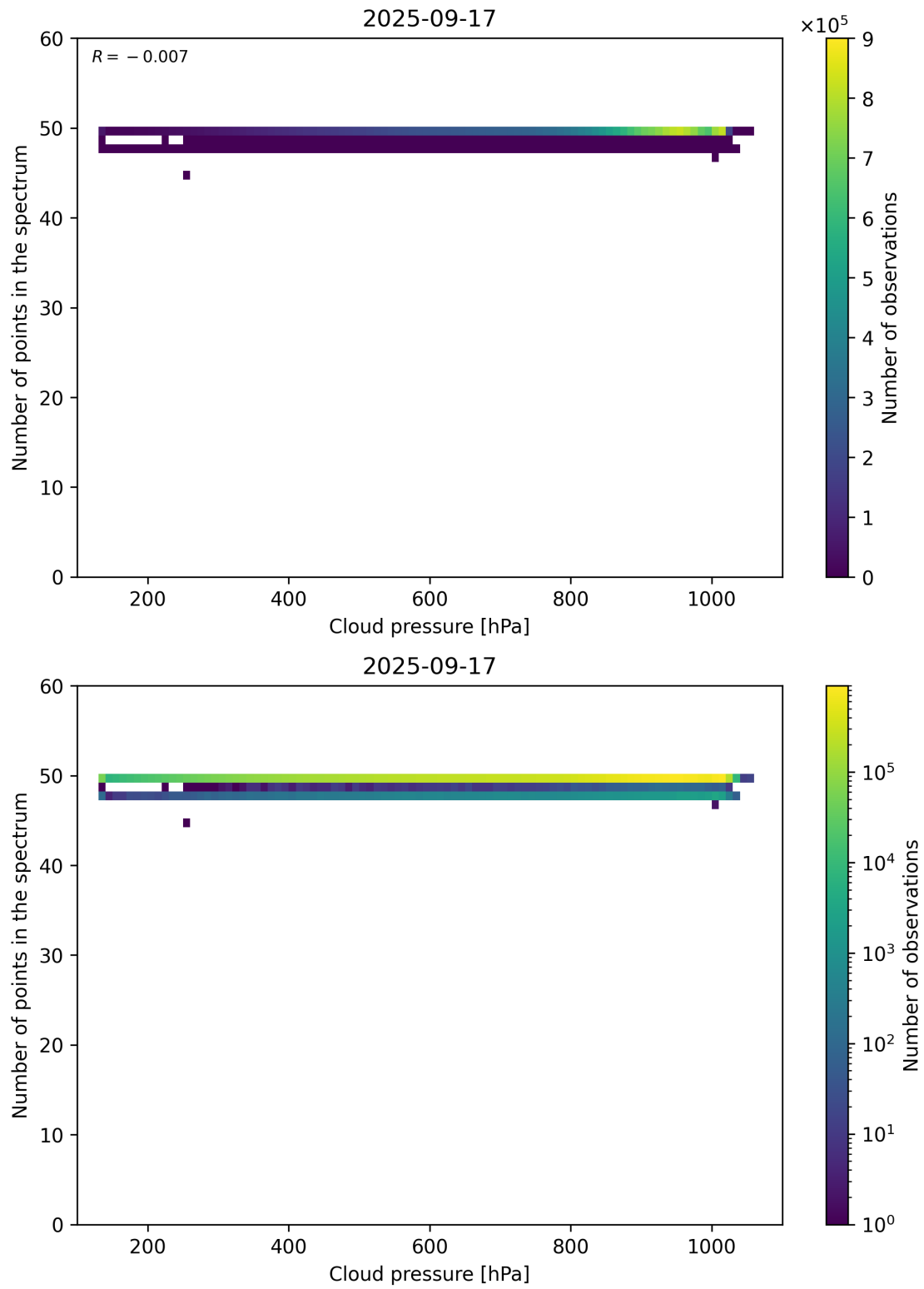
Figure 82: Scatter density plot of “Cloud pressure” against “Number of points in the spectrum” for 2025-09-16 to 2025-09-18.
