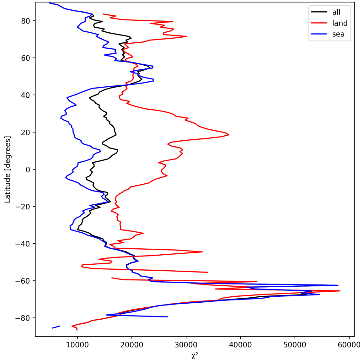
Figure 21: Zonal average of “ \chi^2 ” for 2025-09-16 to 2025-09-18.
