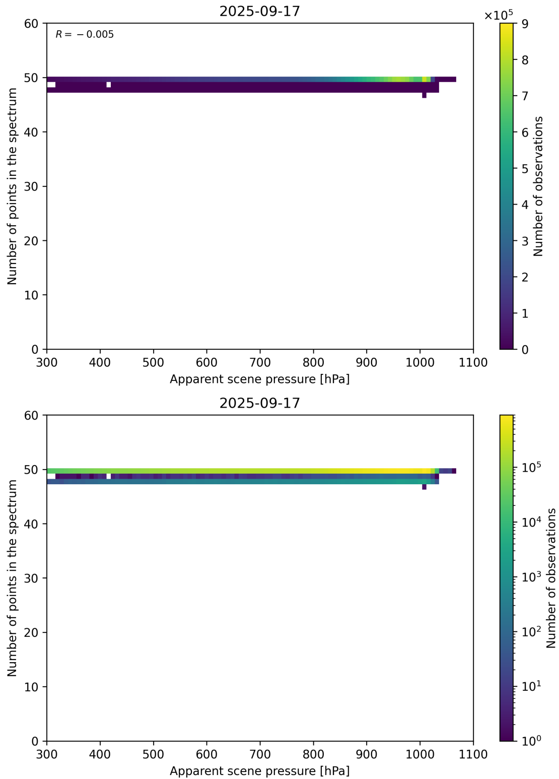
Figure 66: Scatter density plot of “Apparent scene pressure” against “Number of points in the spectrum” for 2025-09-16 to 2025-09-18.
