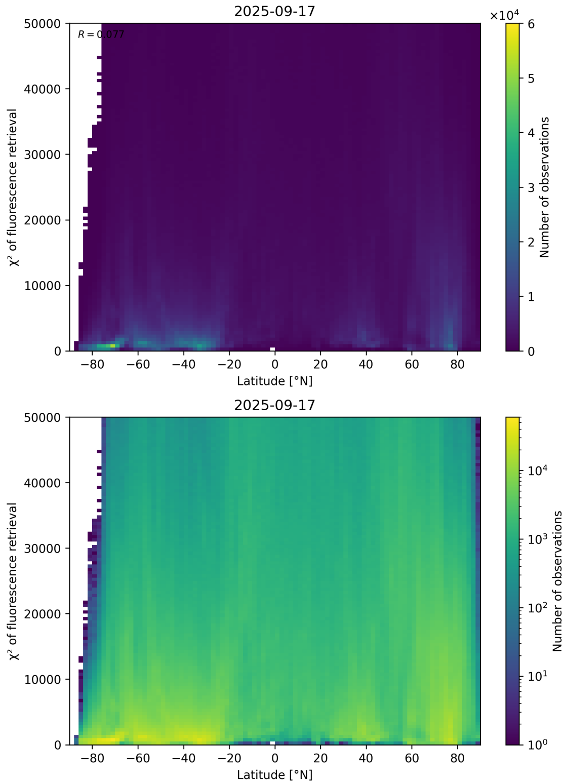
Figure 89: Scatter density plot of “Latitude” against “ \chi^2 of fluorescence retrieval” for 2025-09-16 to 2025-09-18.
