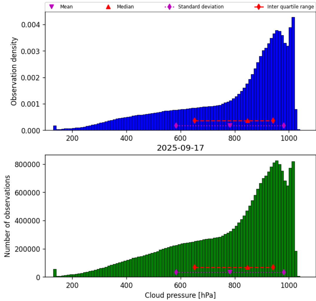
Figure 30: Histogram of “Cloud pressure” for 2025-09-16 to 2025-09-18
