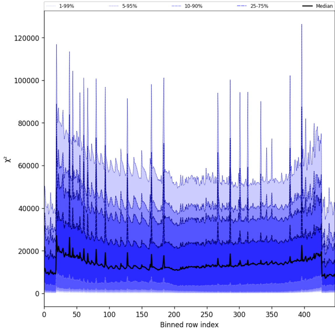
Figure 55: Along track statistics of “ \chi^2 ” for 2025-09-16 to 2025-09-18
