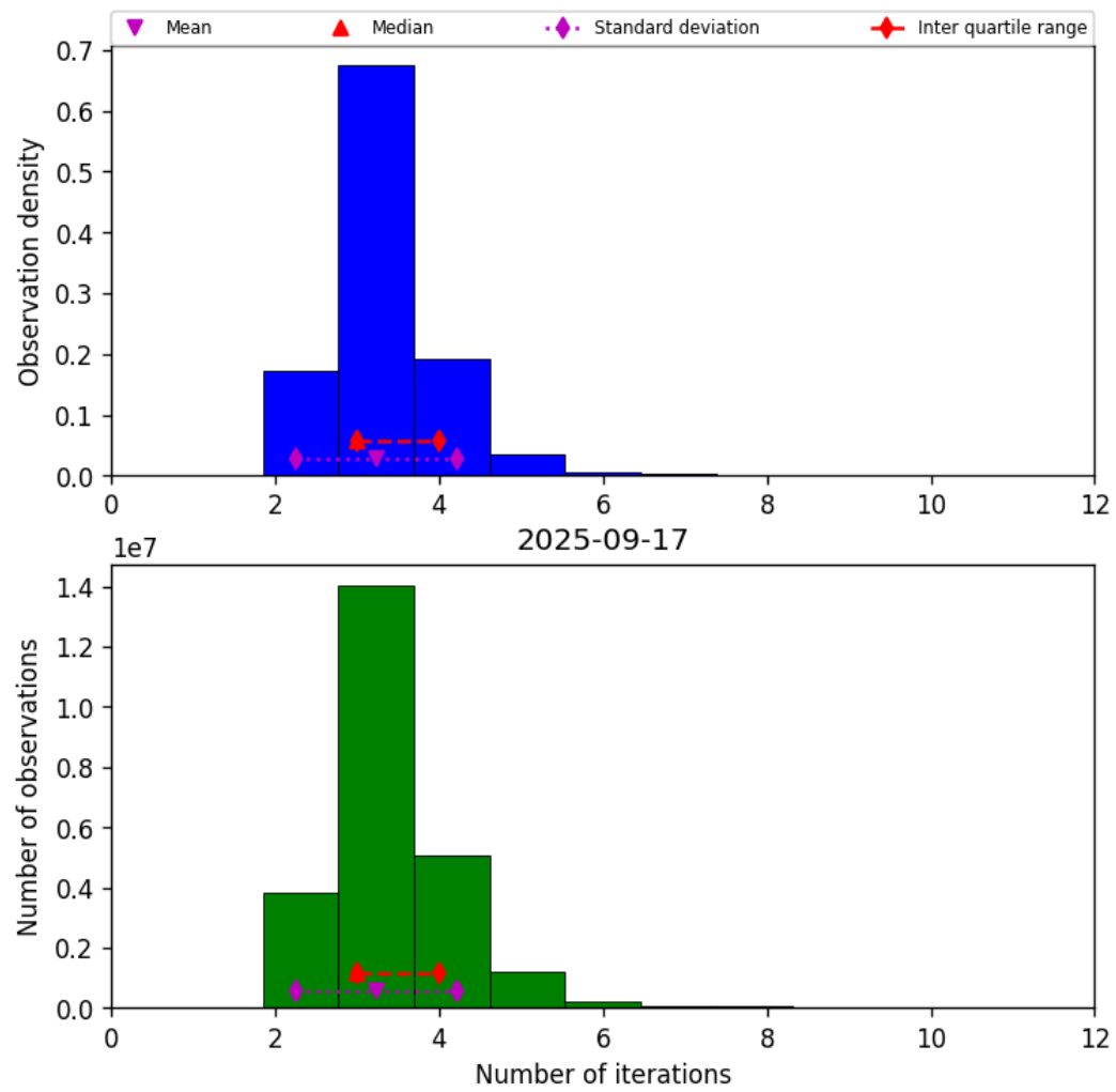
Figure 39: Histogram of “Number of iterations” for 2025-09-16 to 2025-09-18
