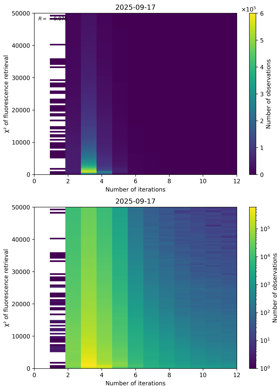
Figure 97: Scatter density plot of “Number of iterations” against “ \chi^2 of fluorescence retrieval” for 2025-09-16 to 2025-09-18.
