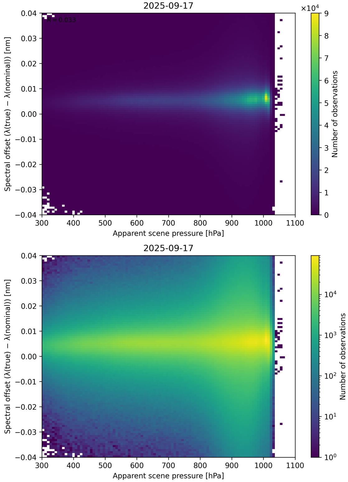
Figure 67: Scatter density plot of “Apparent scene pressure” against “Spectral offset ( \lambda_{\text{true}} - \lambda_{\text{nominal}} )” for 2025-09-16 to 2025-09-18.
