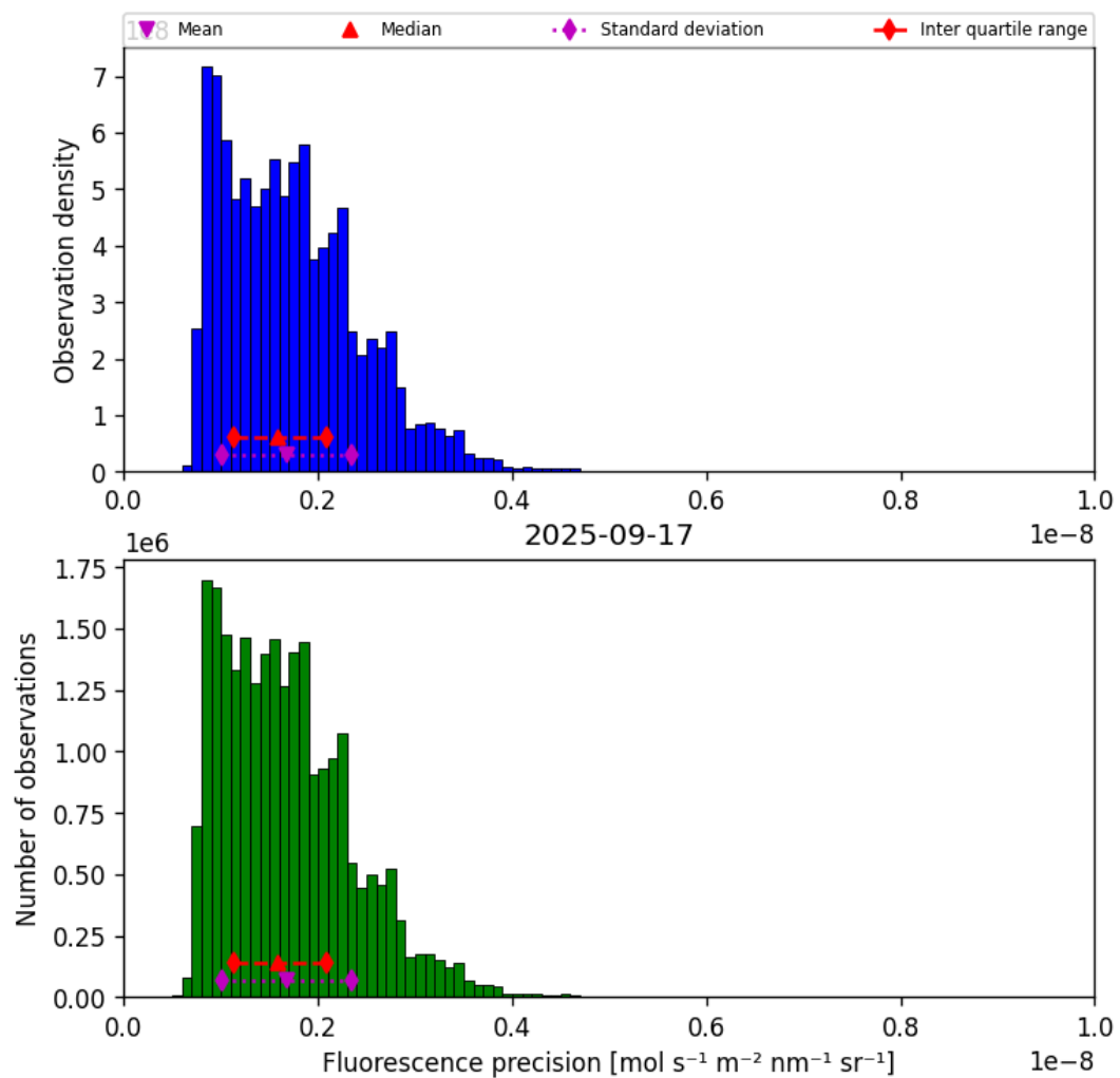
Figure 41: Histogram of “Fluorescence precision” for 2025-09-16 to 2025-09-18
