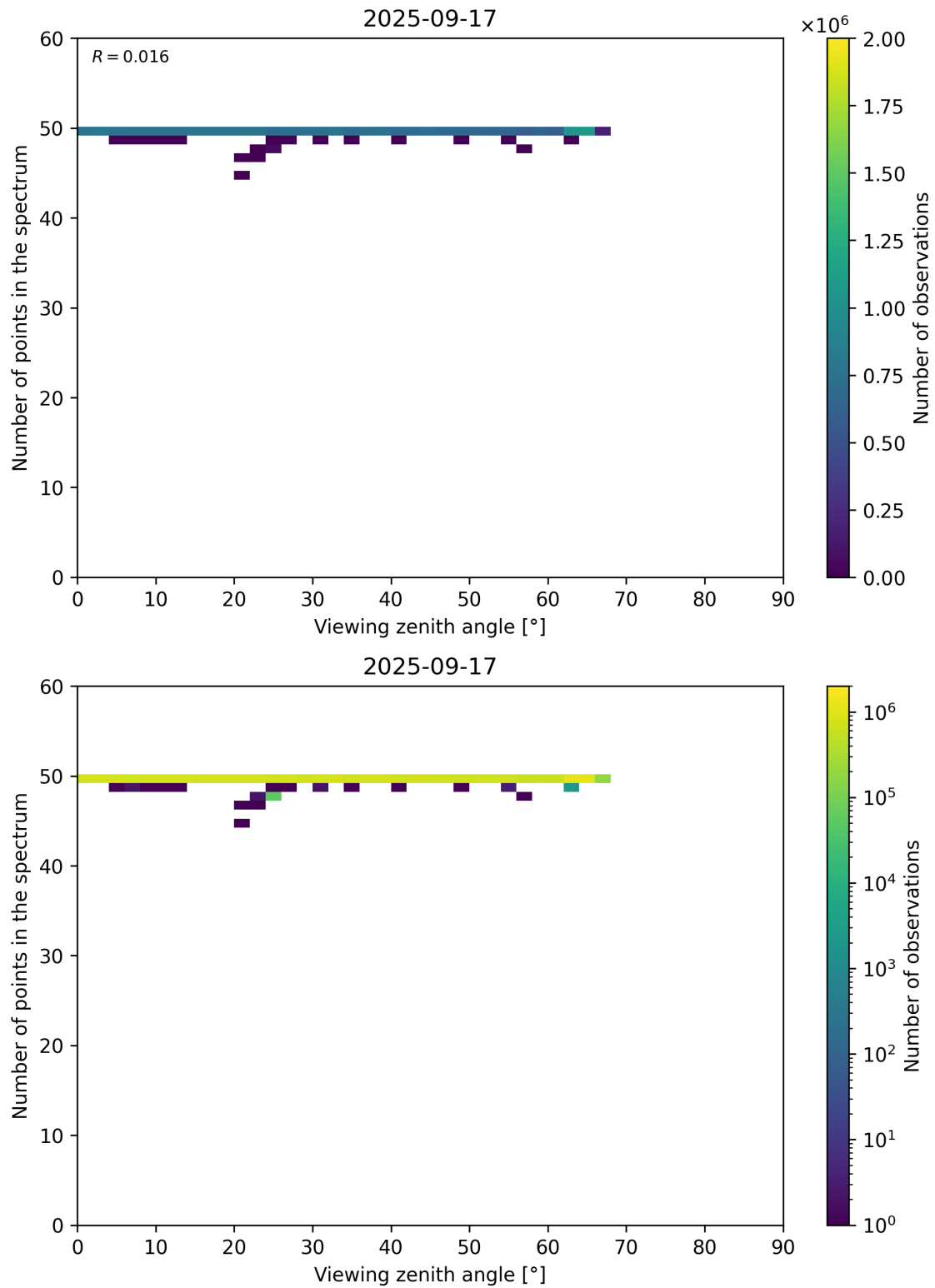
Figure 125: Scatter density plot of “Viewing zenith angle” against “Number of points in the spectrum” for 2025-09-16 to 2025-09-18.
