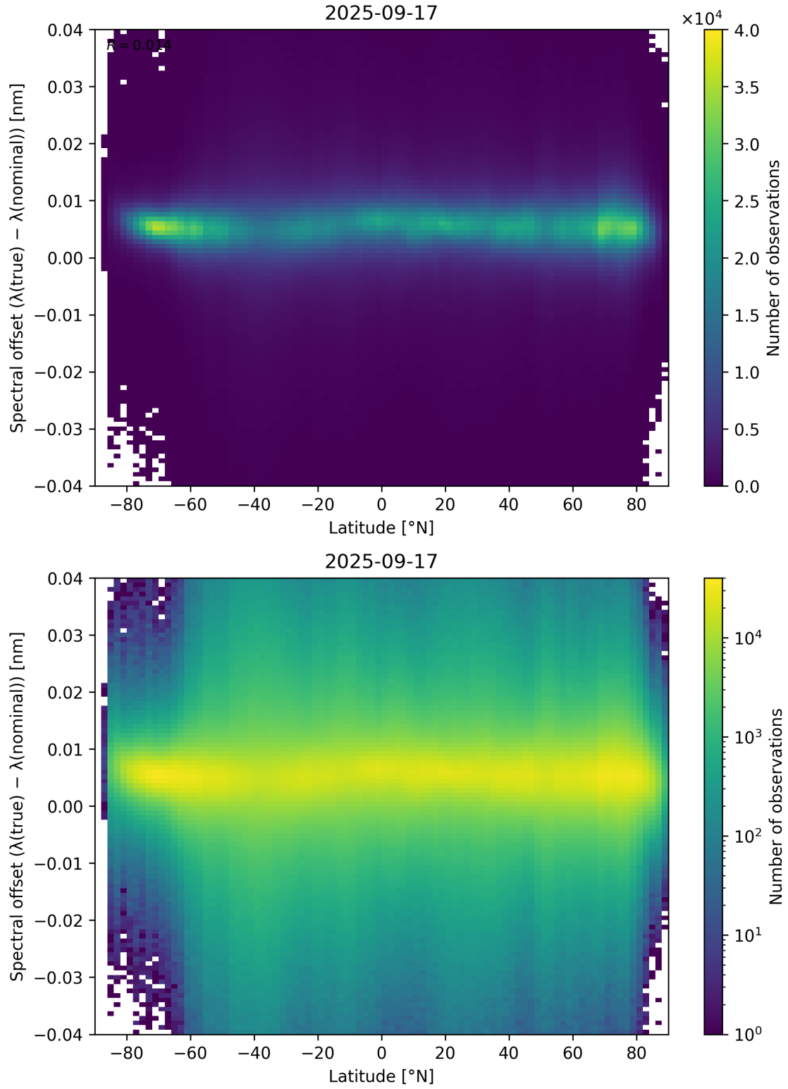
Figure 96: Scatter density plot of “Latitude” against “Spectral offset ( \lambda_{\text{true}} - \lambda_{\text{nominal}} )” for 2025-09-16 to 2025-09-18.
