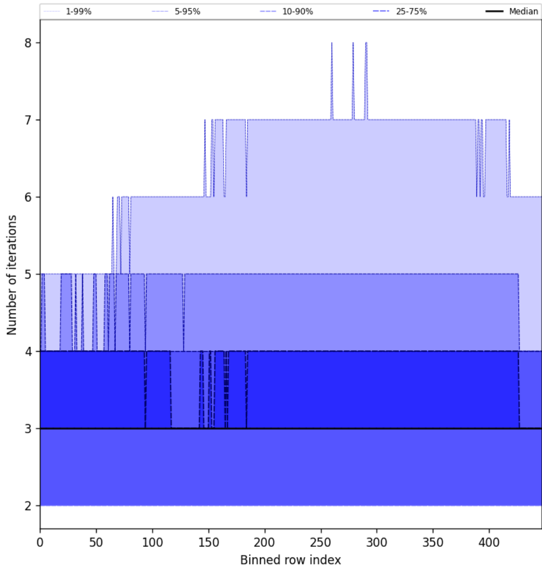
Figure 56: Along track statistics of “Number of iterations” for 2025-09-16 to 2025-09-18
