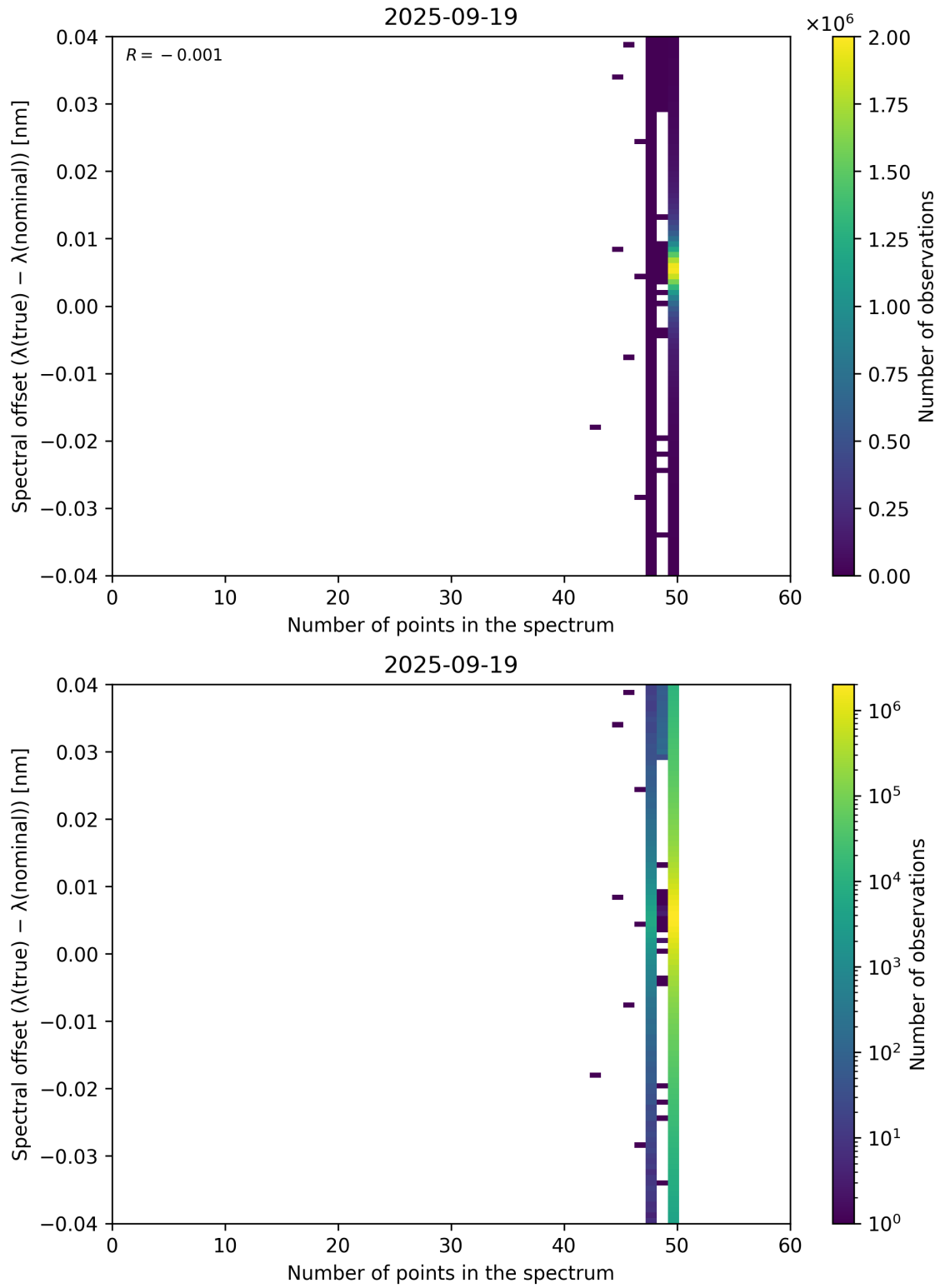
Figure 101: Scatter density plot of “Number of points in the spectrum” against “Spectral offset ( \lambda_{\text{true}} - \lambda_{\text{nominal}} )” for 2025-09-18 to 2025-09-20.
