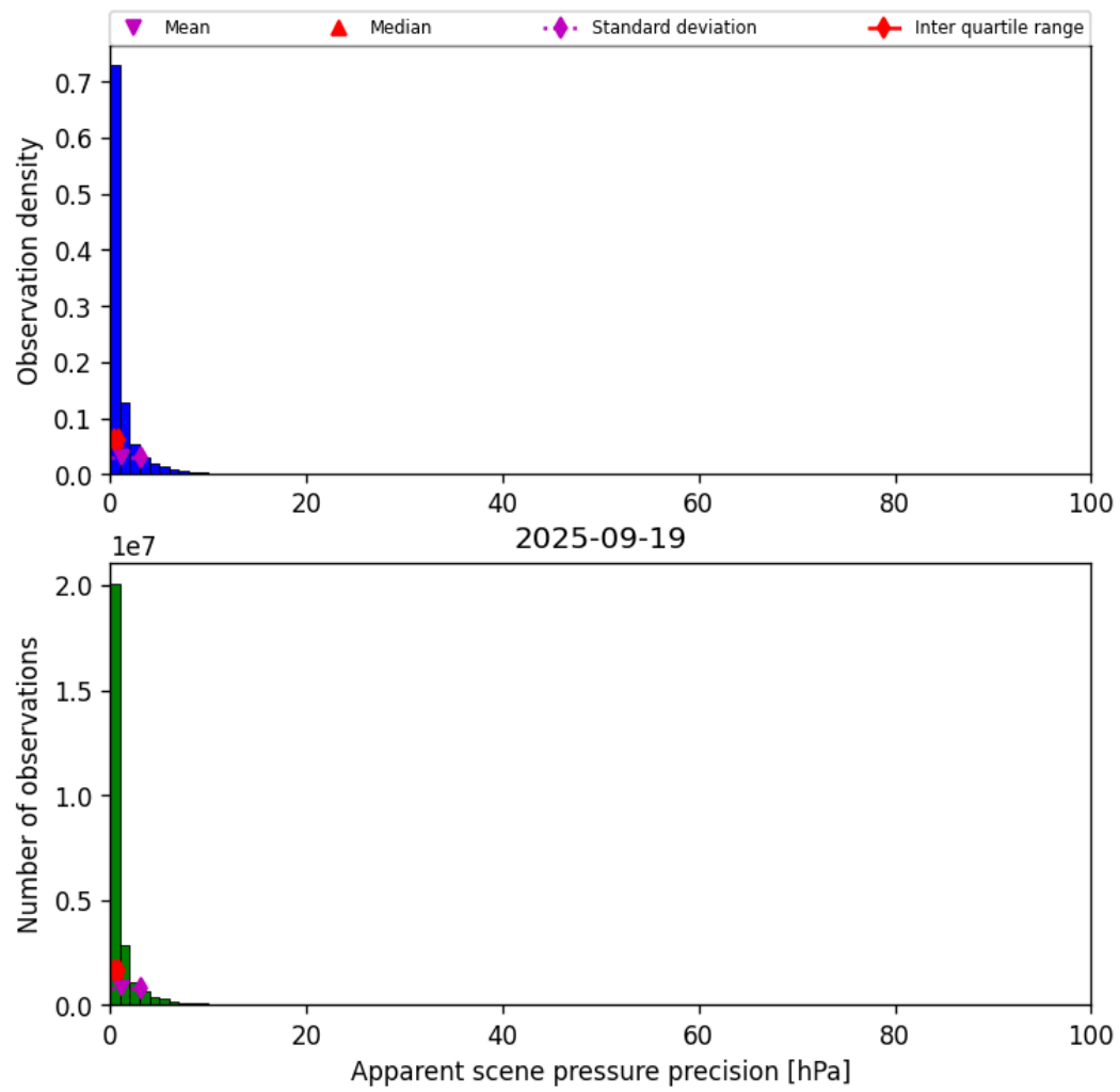
Figure 37: Histogram of “Apparent scene pressure precision” for 2025-09-18 to 2025-09-20
