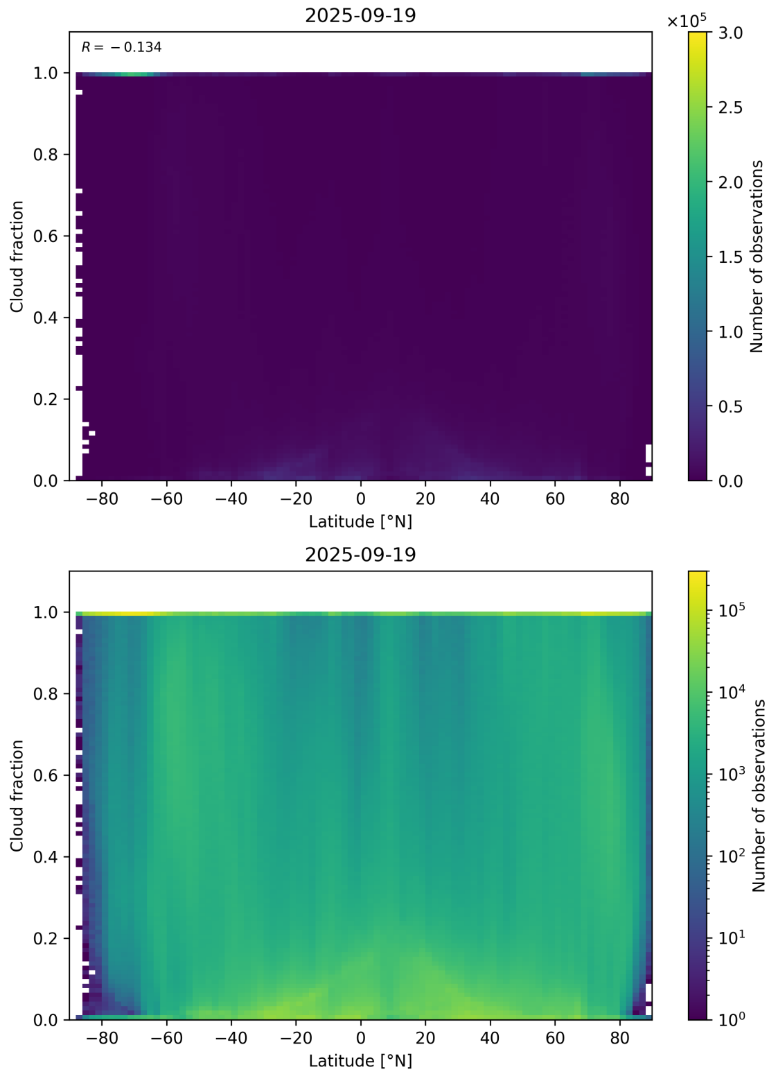
Figure 90: Scatter density plot of “Latitude” against “Cloud fraction” for 2025-09-18 to 2025-09-20.
