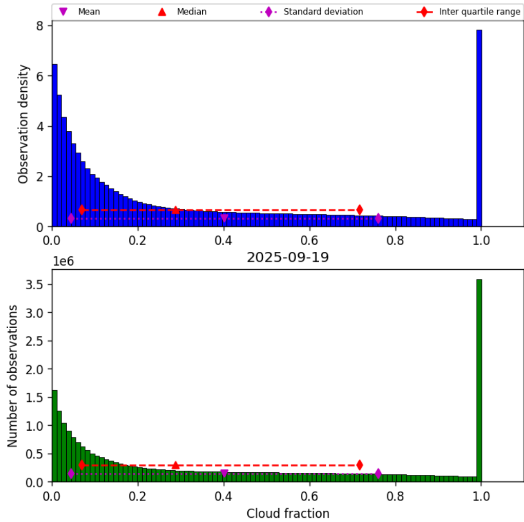
Figure 32: Histogram of “Cloud fraction” for 2025-09-18 to 2025-09-20
