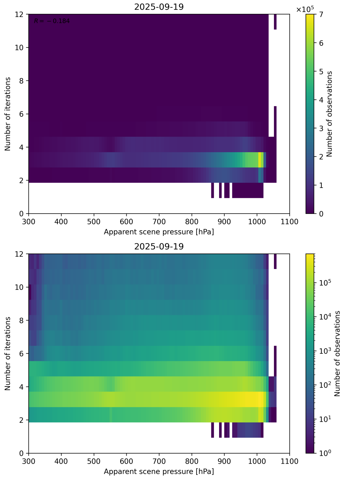
Figure 65: Scatter density plot of “Apparent scene pressure” against “Number of iterations” for 2025-09-18 to 2025-09-20.
