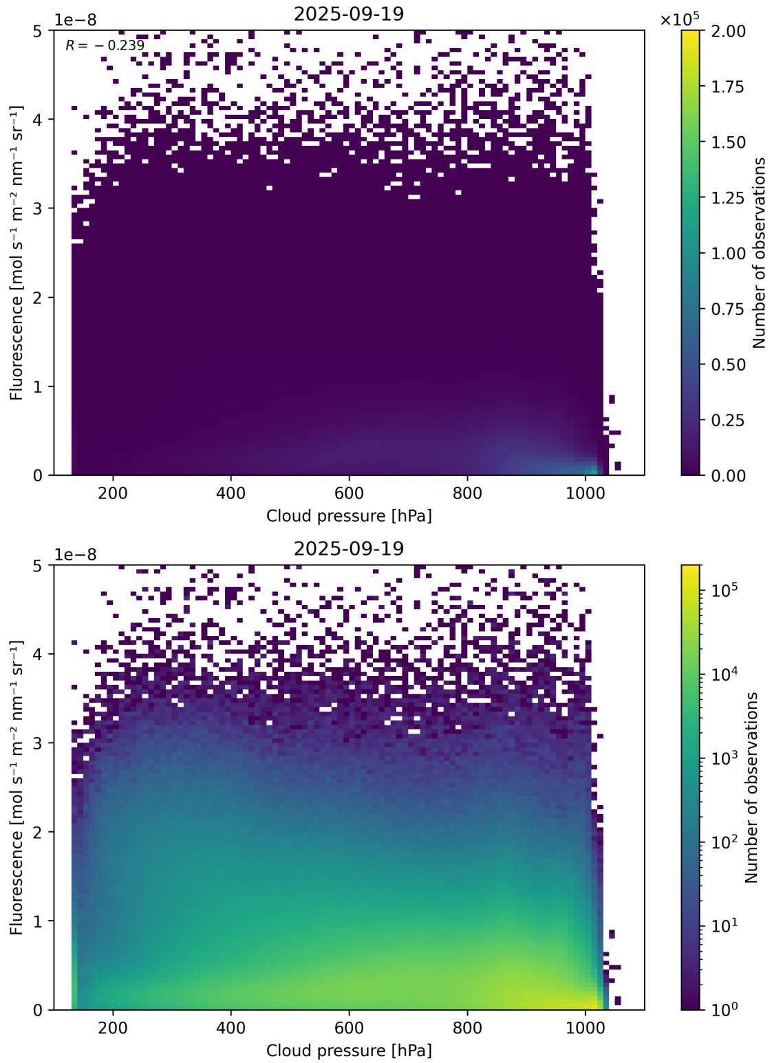
Figure 80: Scatter density plot of “Cloud pressure” against “Fluorescence” for 2025-09-18 to 2025-09-20.
