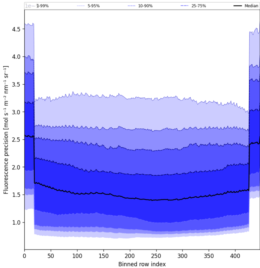
Figure 58: Along track statistics of “Fluorescence precision” for 2025-09-18 to 2025-09-20
