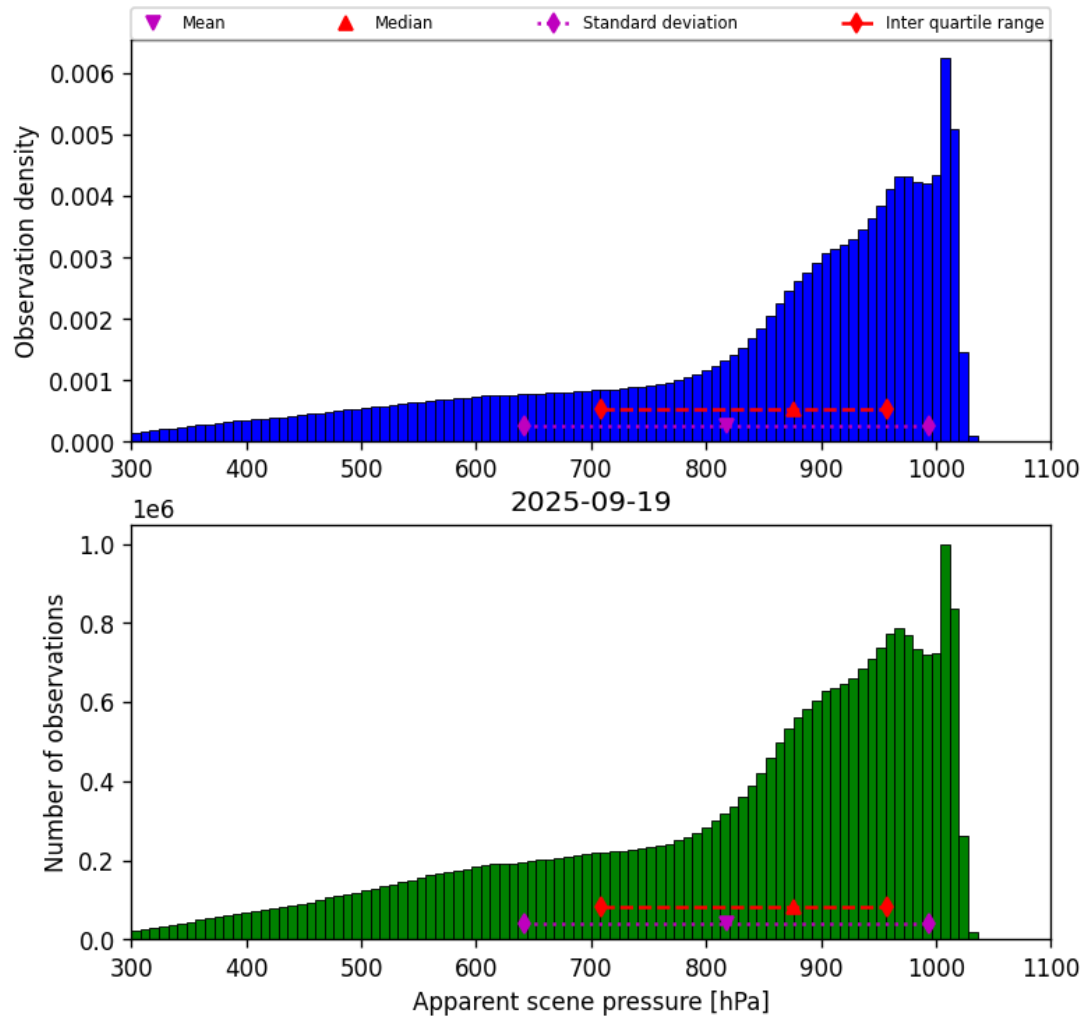
Figure 36: Histogram of “Apparent scene pressure” for 2025-09-18 to 2025-09-20
