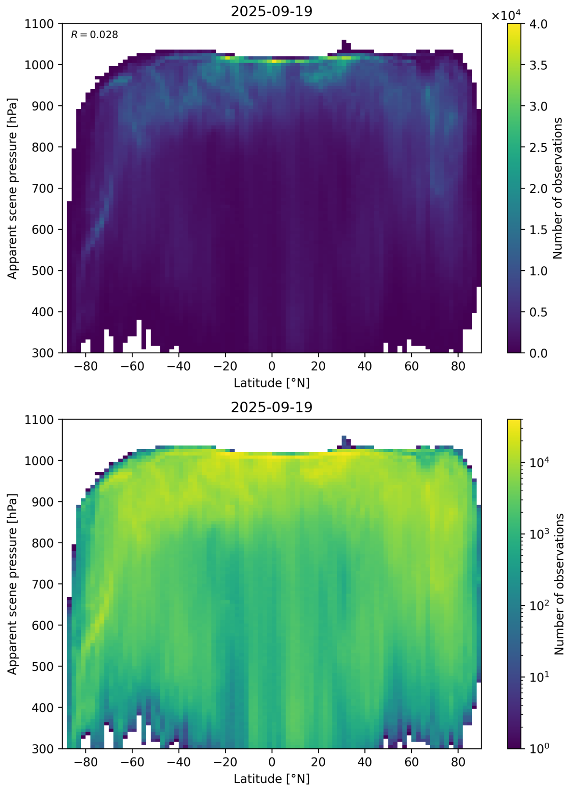
Figure 88: Scatter density plot of “Latitude” against “Apparent scene pressure” for 2025-09-18 to 2025-09-20.
