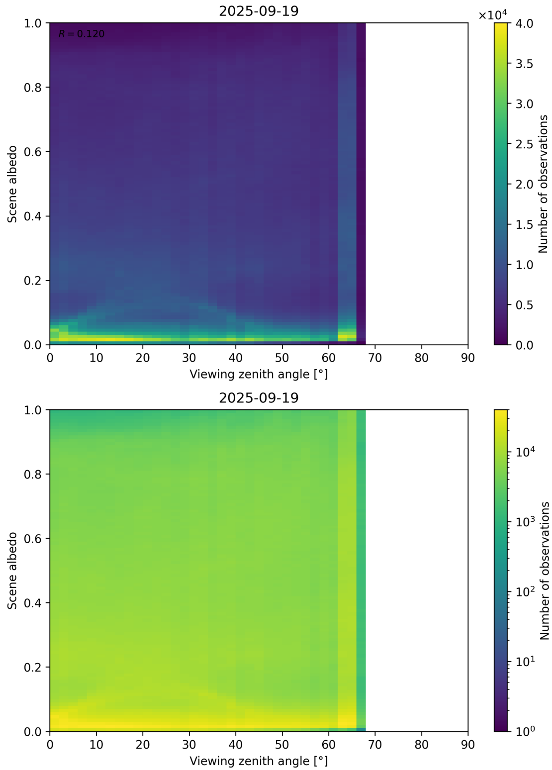
Figure 126: Scatter density plot of “Viewing zenith angle” against “Scene albedo” for 2025-09-18 to 2025-09-20.
