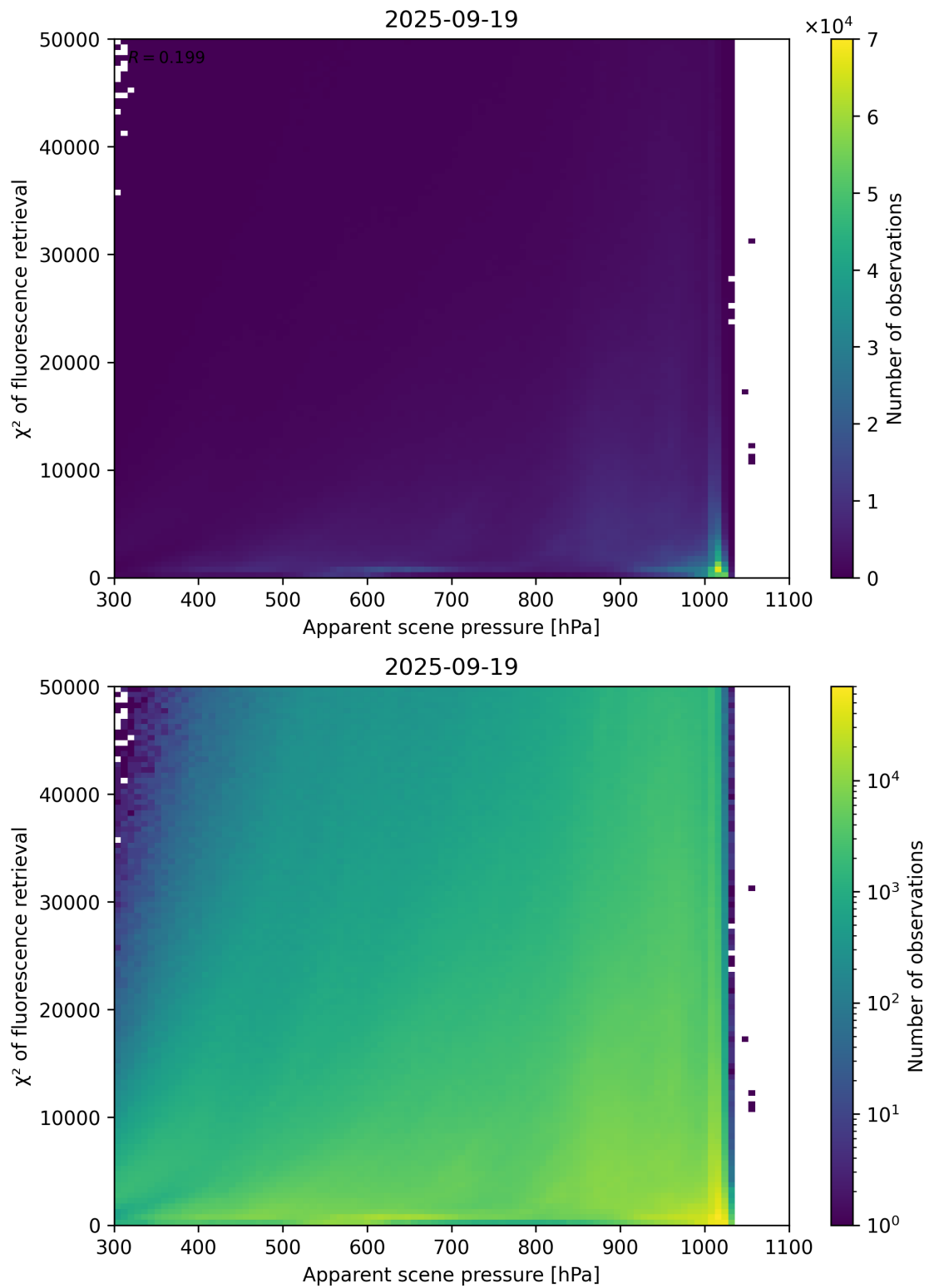
Figure 63: Scatter density plot of “Apparent scene pressure” against “ \chi^2 of fluorescence retrieval” for 2025-09-18 to 2025-09-20.
