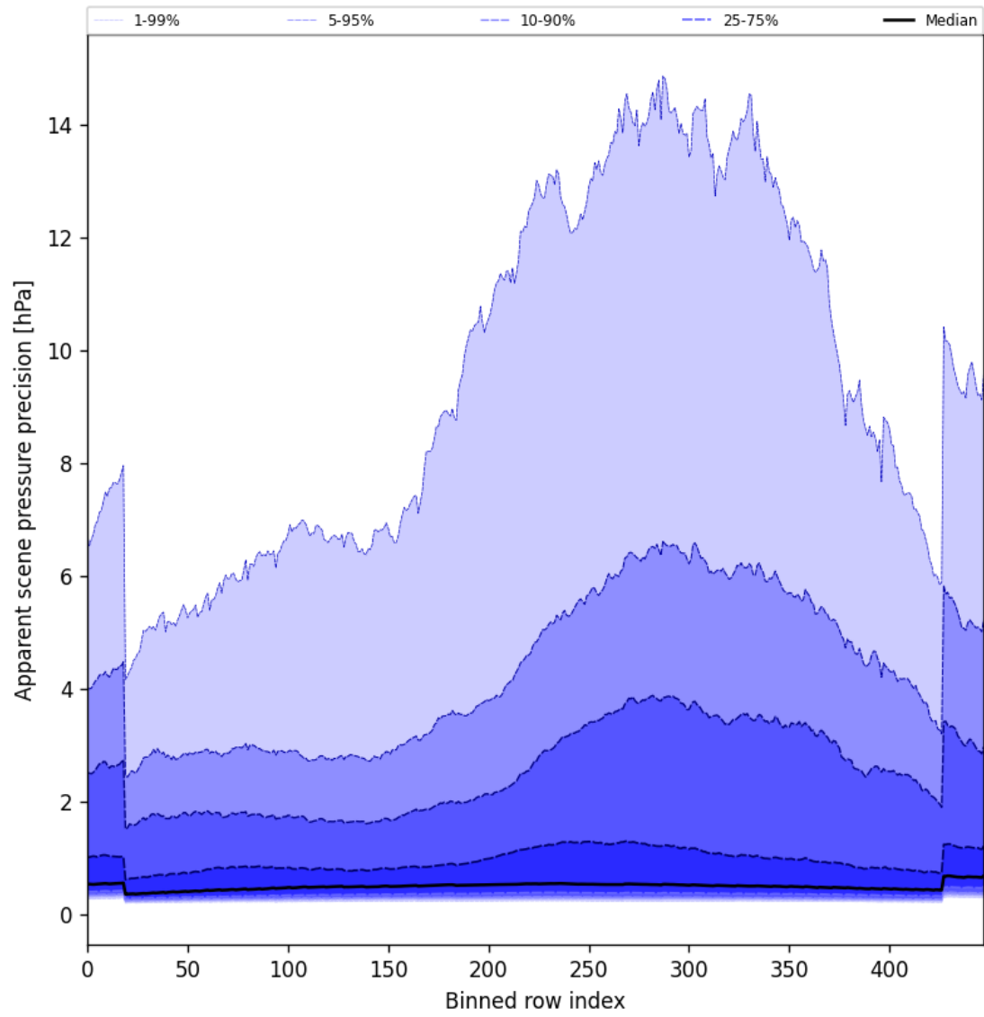
Figure 54: Along track statistics of “Apparent scene pressure precision” for 2025-09-18 to 2025-09-20
