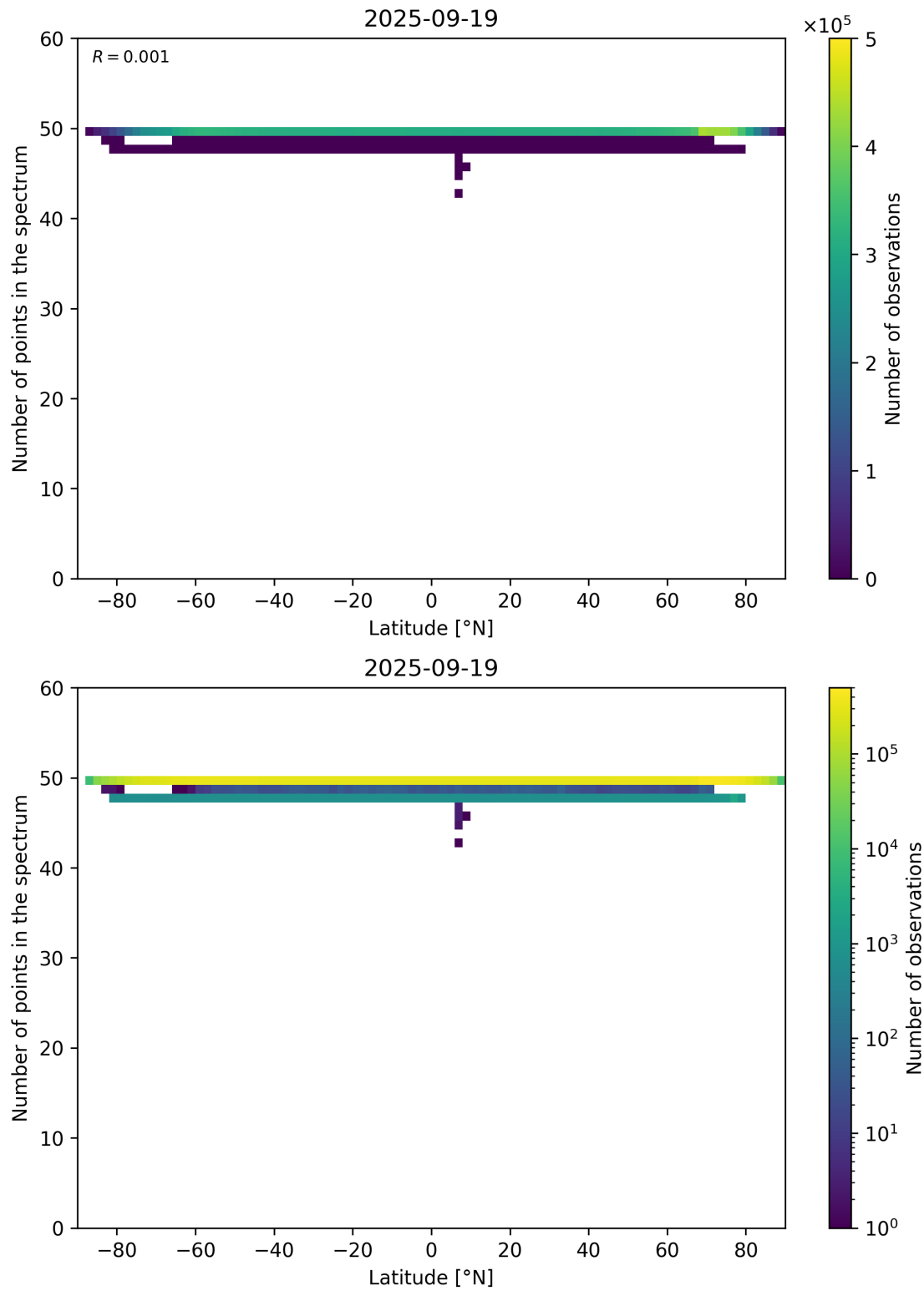
Figure 94: Scatter density plot of “Latitude” against “Number of points in the spectrum” for 2025-09-18 to 2025-09-20.
