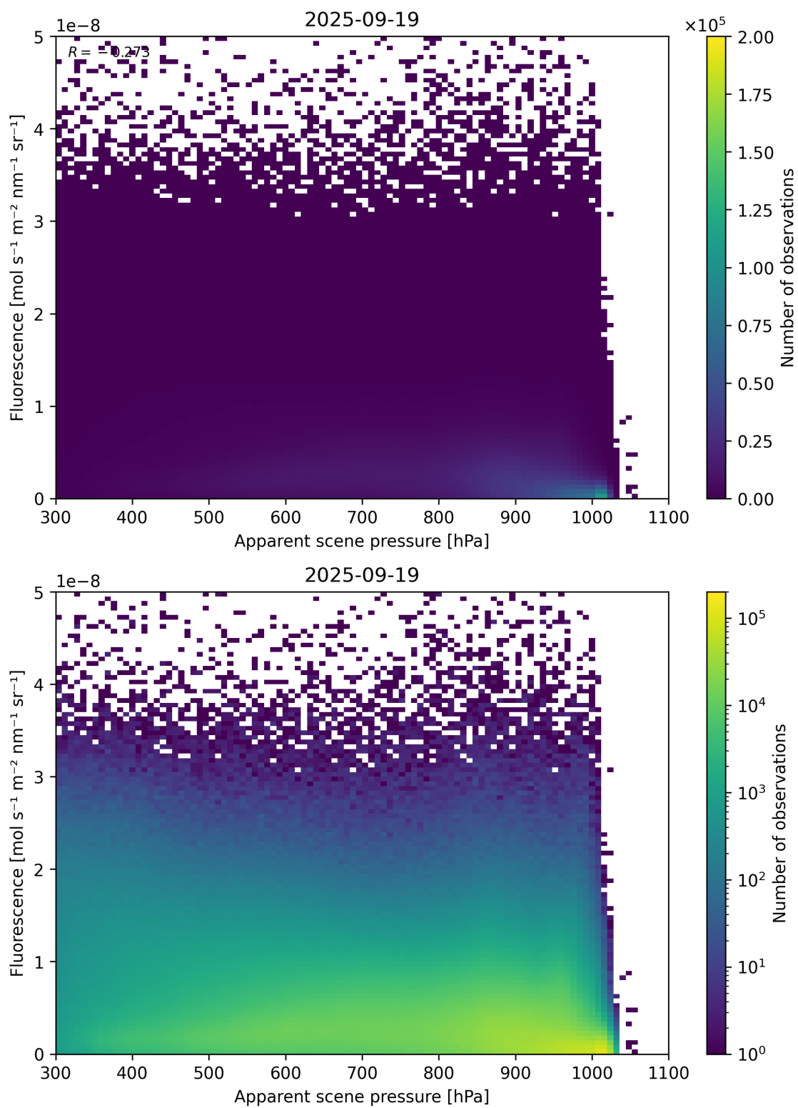
Figure 64: Scatter density plot of “Apparent scene pressure” against “Fluorescence” for 2025-09-18 to 2025-09-20.
