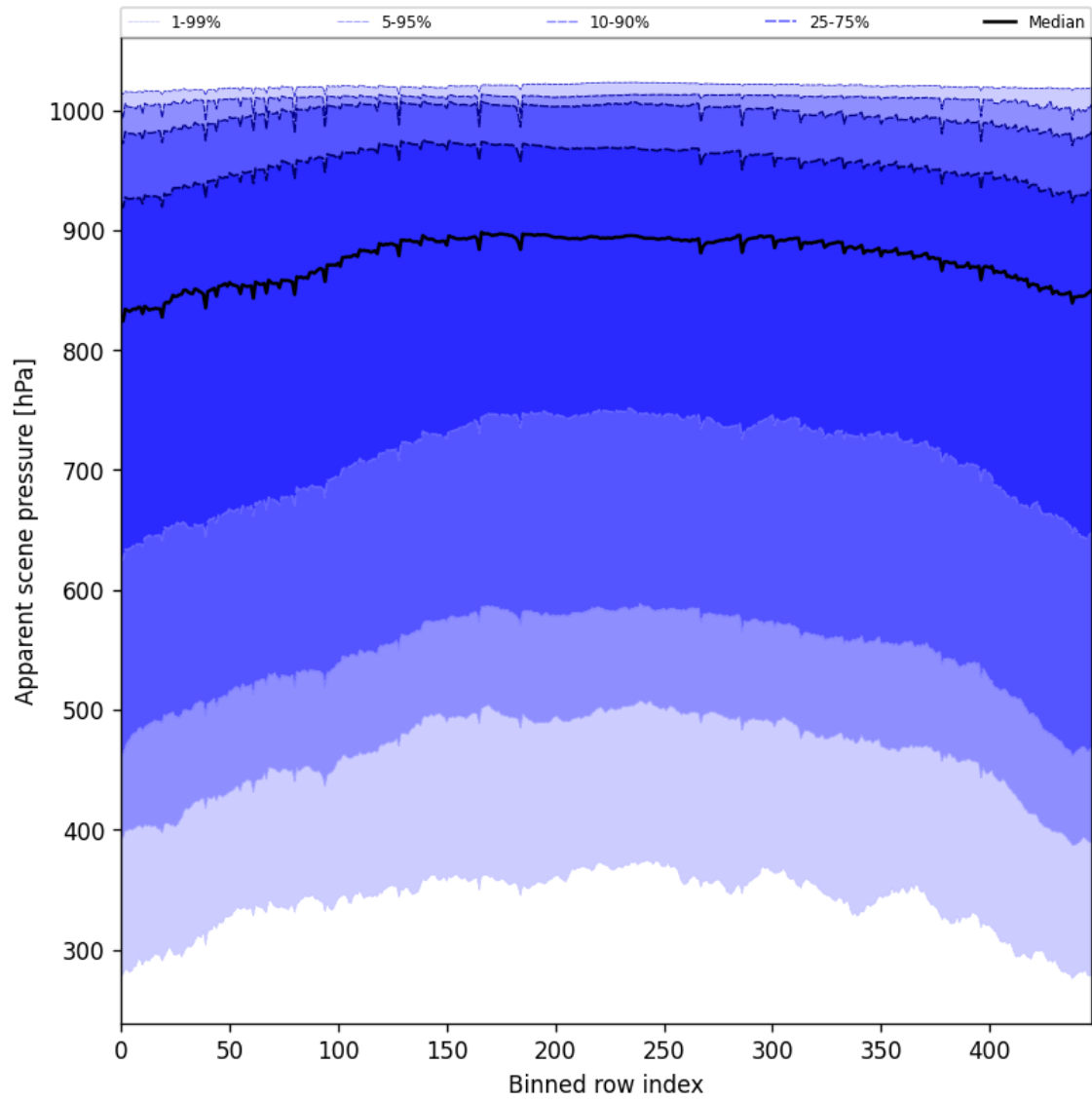
Figure 53: Along track statistics of “Apparent scene pressure” for 2025-09-18 to 2025-09-20
