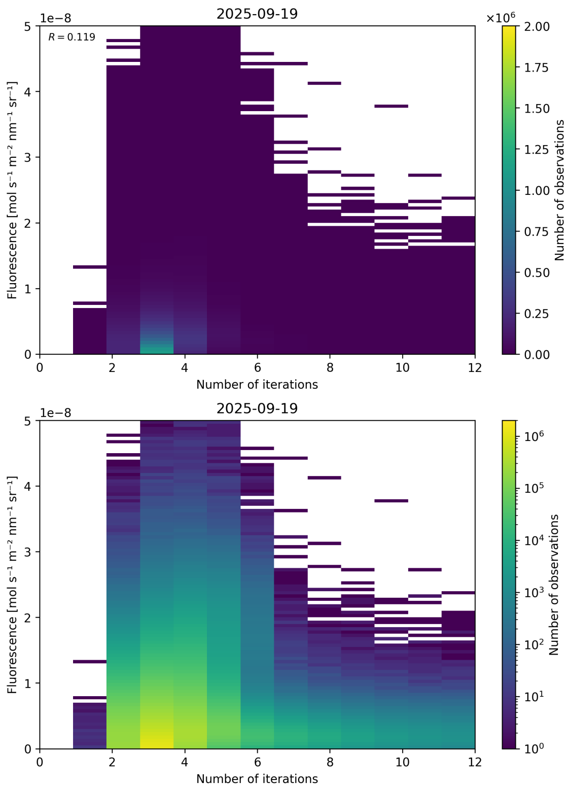
Figure 98: Scatter density plot of “Number of iterations” against “Fluorescence” for 2025-09-18 to 2025-09-20.
