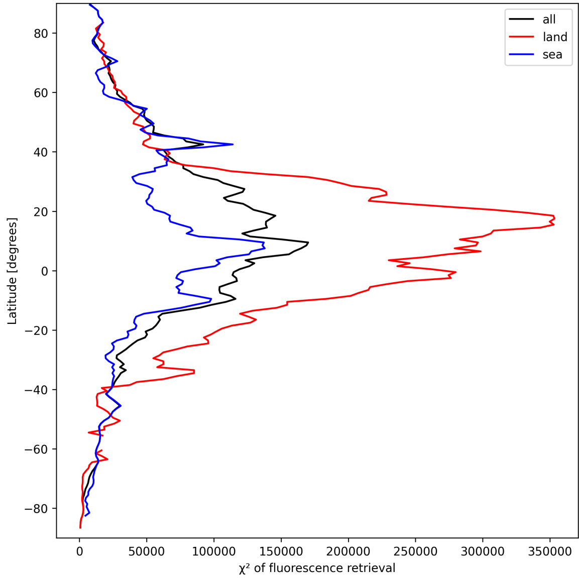
Figure 25: Zonal average of “ \chi^2 of fluorescence retrieval” for 2025-09-18 to 2025-09-20.
