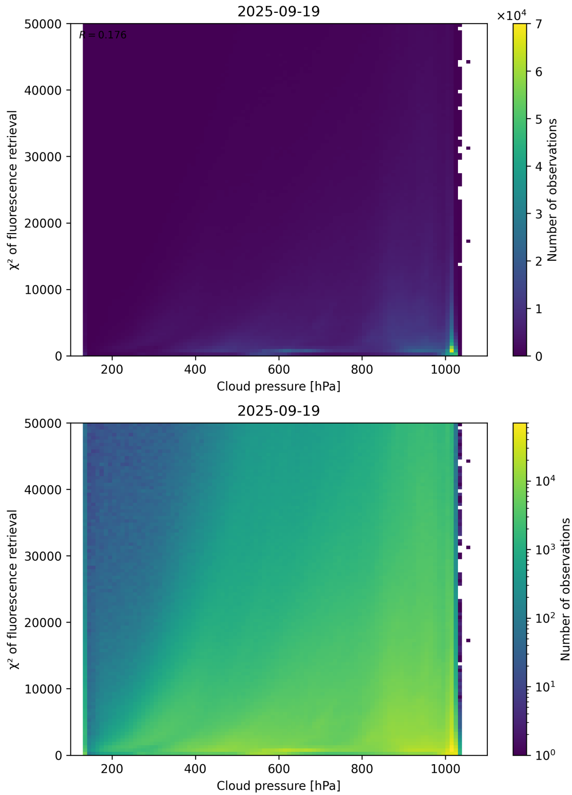
Figure 78: Scatter density plot of “Cloud pressure” against “ \chi^2 of fluorescence retrieval” for 2025-09-18 to 2025-09-20.
