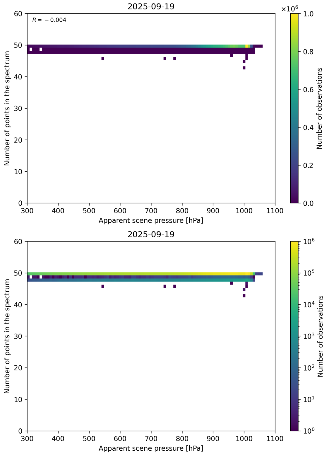
Figure 66: Scatter density plot of “Apparent scene pressure” against “Number of points in the spectrum” for 2025-09-18 to 2025-09-20.
