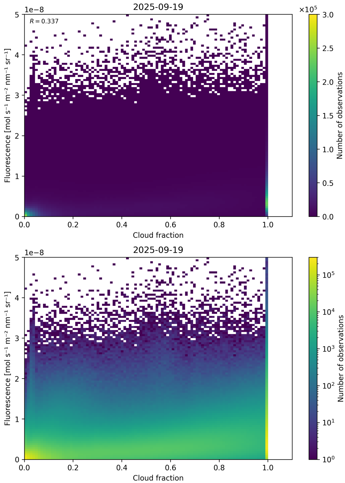
Figure 72: Scatter density plot of “Cloud fraction” against “Fluorescence” for 2025-09-18 to 2025-09-20.
