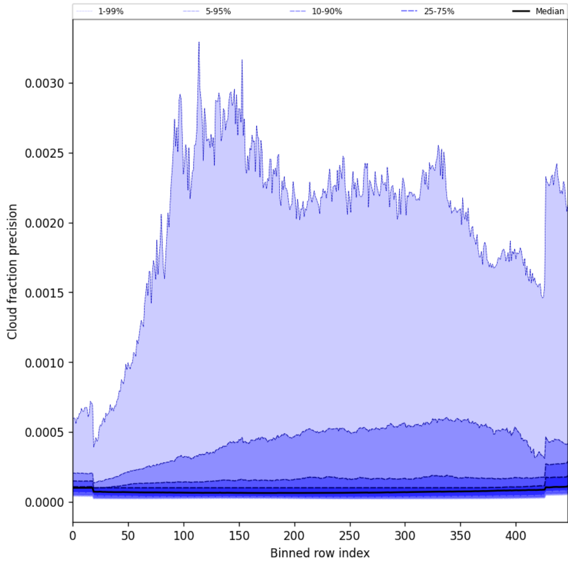
Figure 50: Along track statistics of “Cloud fraction precision” for 2025-09-18 to 2025-09-20
