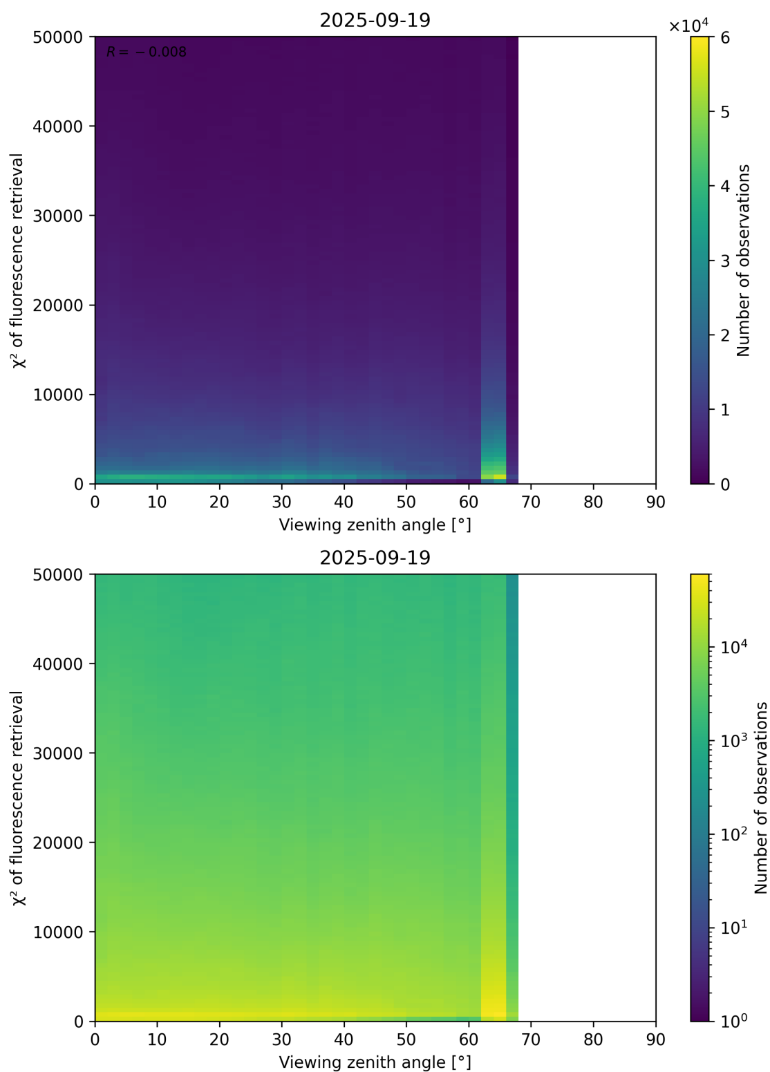
Figure 119: Scatter density plot of “Viewing zenith angle” against “ \chi^2 of fluorescence retrieval” for 2025-09-18 to 2025-09-20.
