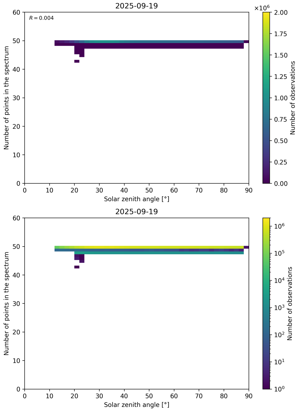
Figure 115: Scatter density plot of “Solar zenith angle” against “Number of points in the spectrum” for 2025-09-18 to 2025-09-20.
