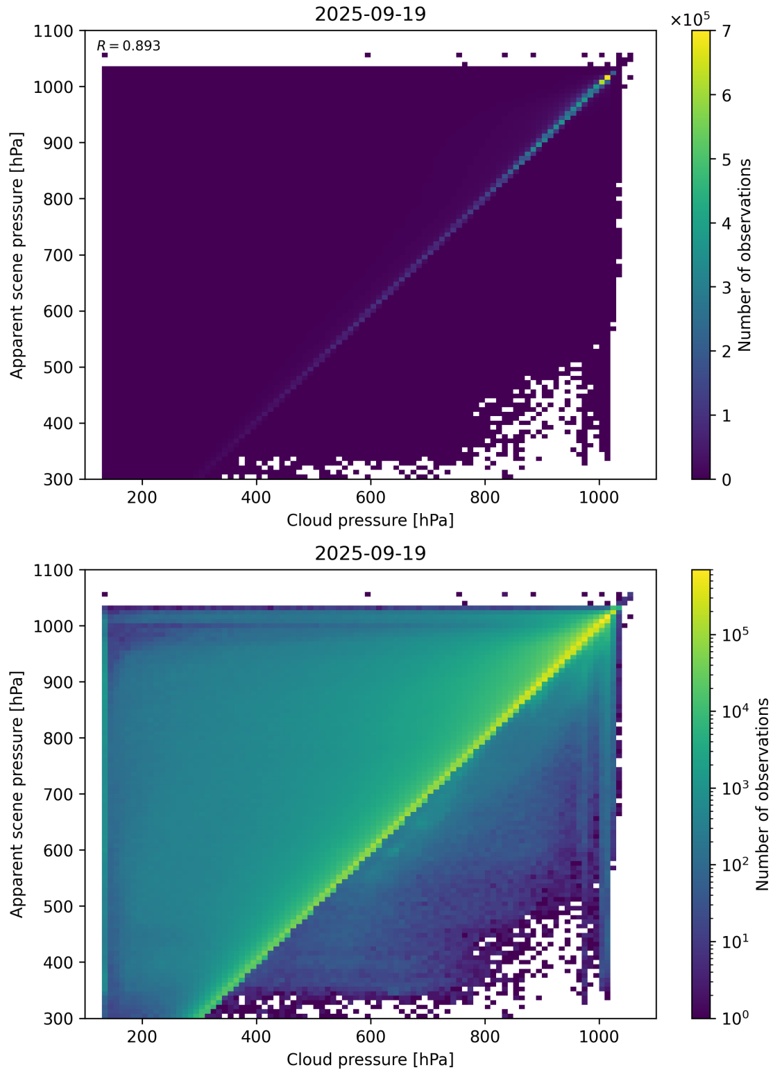
Figure 77: Scatter density plot of “Cloud pressure” against “Apparent scene pressure” for 2025-09-18 to 2025-09-20.
