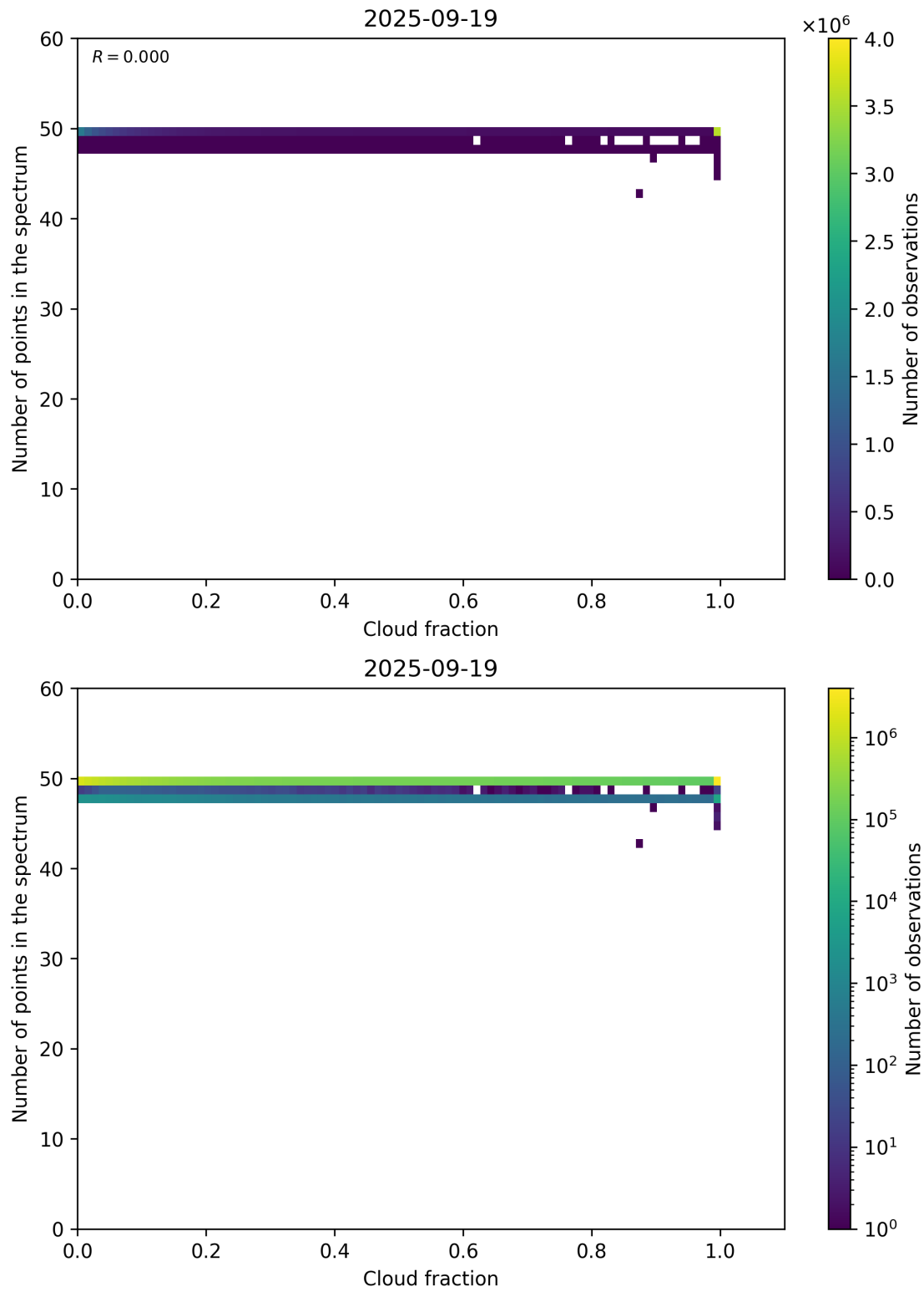
Figure 74: Scatter density plot of “Cloud fraction” against “Number of points in the spectrum” for 2025-09-18 to 2025-09-20.
