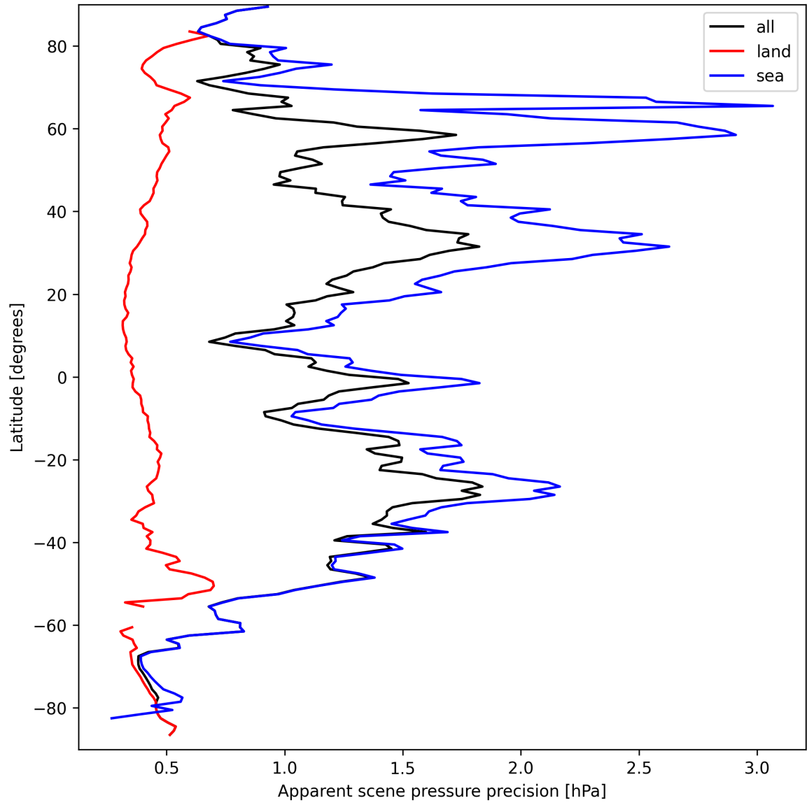
Figure 20: Zonal average of “Apparent scene pressure precision” for 2025-09-18 to 2025-09-20.
