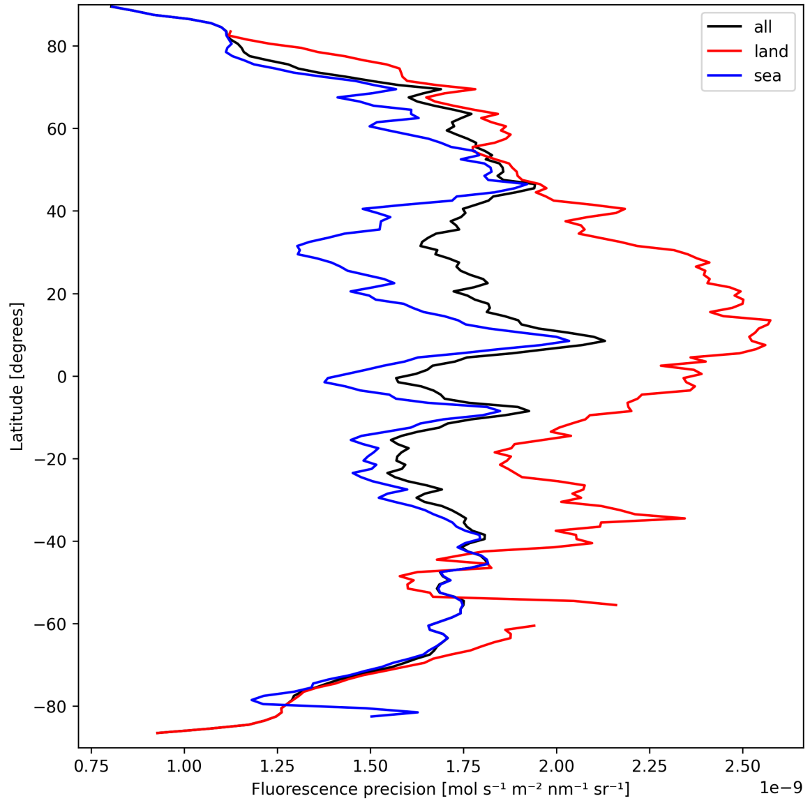
Figure 24: Zonal average of “Fluorescence precision” for 2025-09-18 to 2025-09-20.
