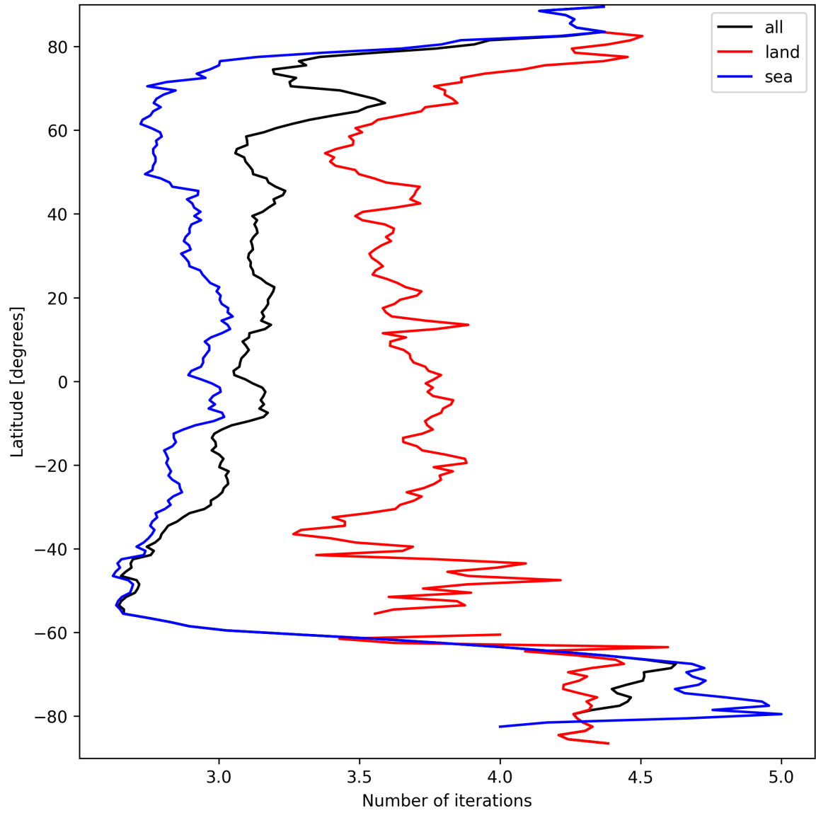
Figure 22: Zonal average of “Number of iterations” for 2025-09-18 to 2025-09-20.
