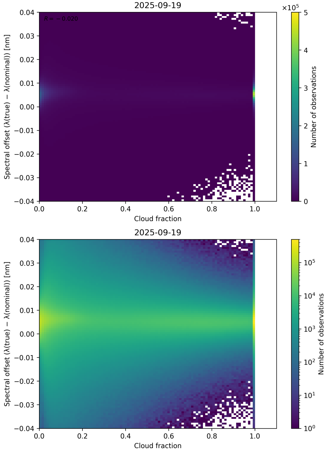
Figure 76: Scatter density plot of “Cloud fraction” against “Spectral offset ( \lambda_{\text{true}} - \lambda_{\text{nominal}} )” for 2025-09-18 to 2025-09-20.
