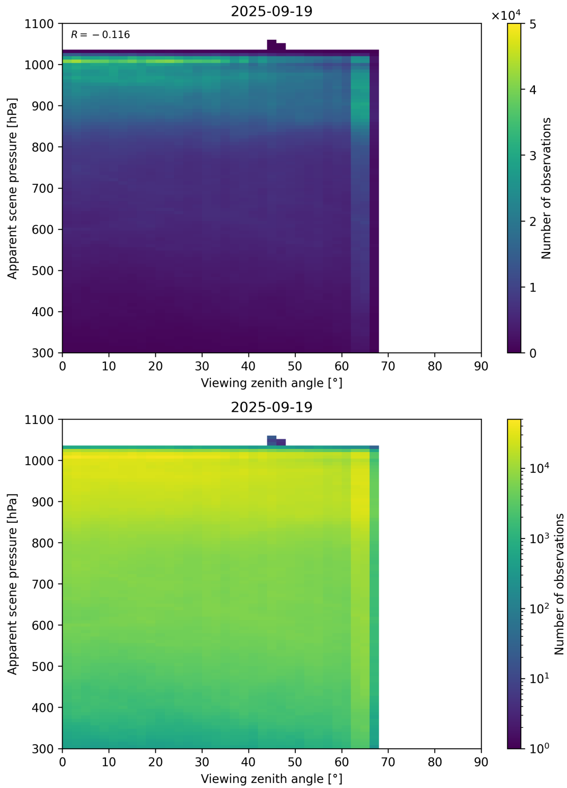
Figure 118: Scatter density plot of “Viewing zenith angle” against “Apparent scene pressure” for 2025-09-18 to 2025-09-20.
