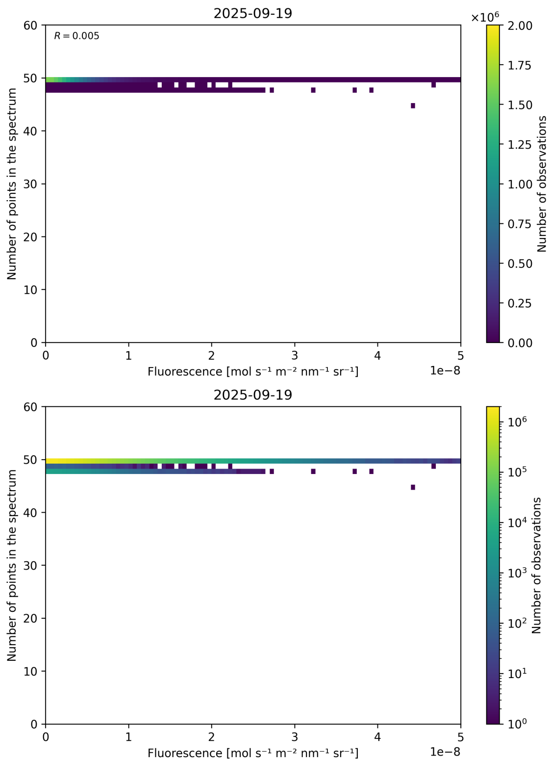
Figure 86: Scatter density plot of “Fluorescence” against “Number of points in the spectrum” for 2025-09-18 to 2025-09-20.
