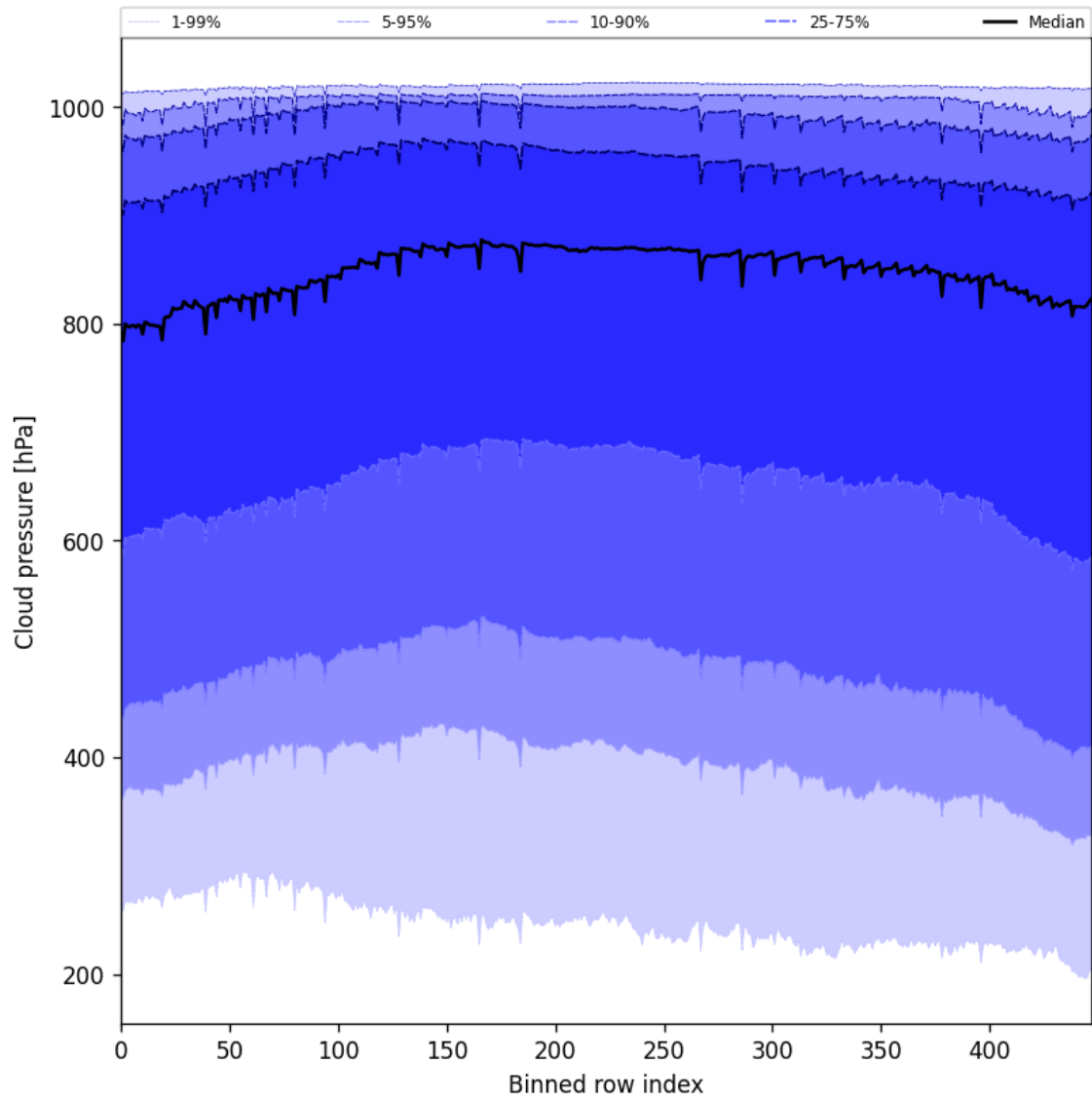
Figure 47: Along track statistics of “Cloud pressure” for 2025-09-18 to 2025-09-20
