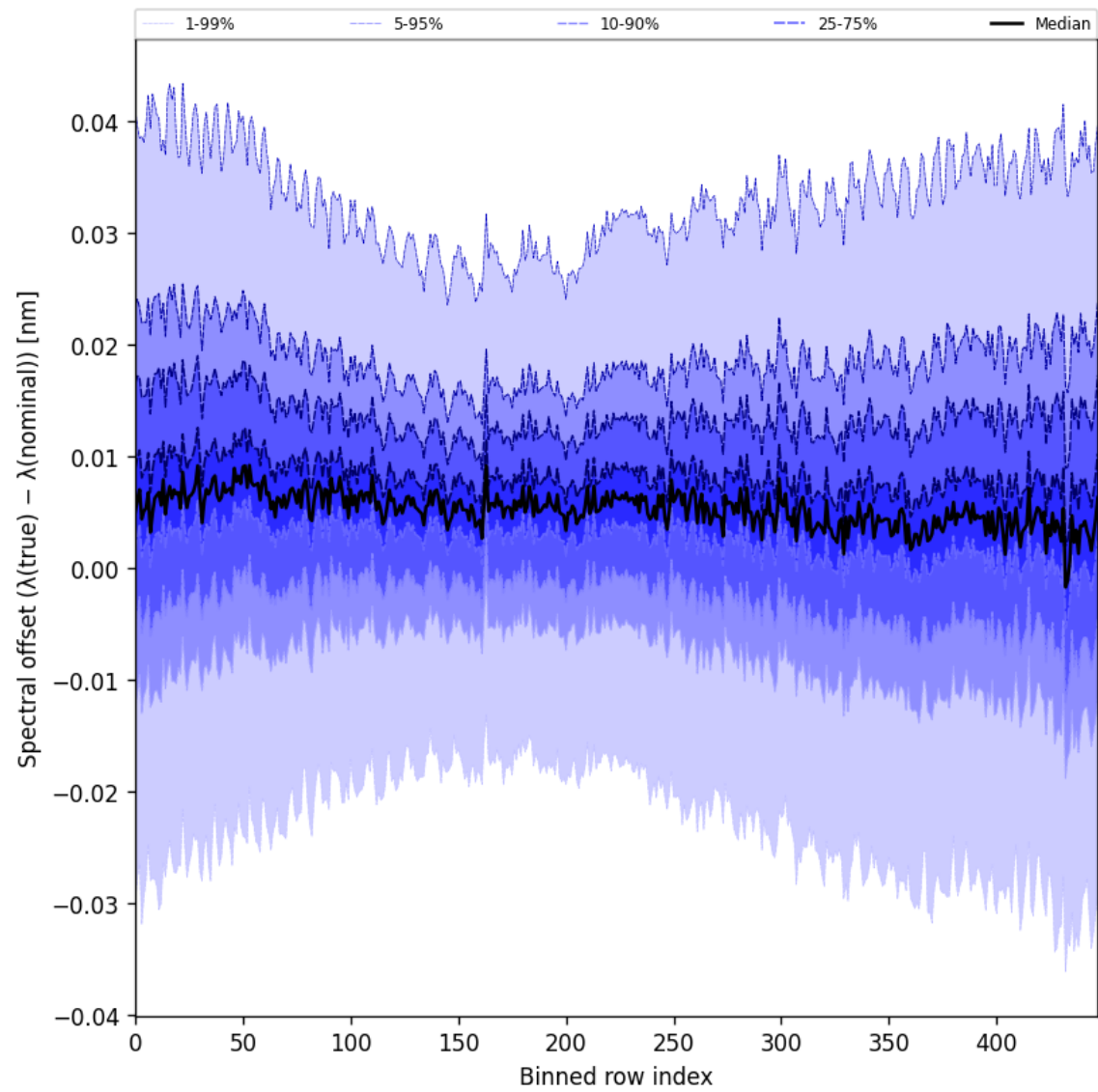
Figure 62: Along track statistics of “Spectral offset ( \lambda_{\text{true}} - \lambda_{\text{nominal}} )” for 2025-09-18 to 2025-09-20
