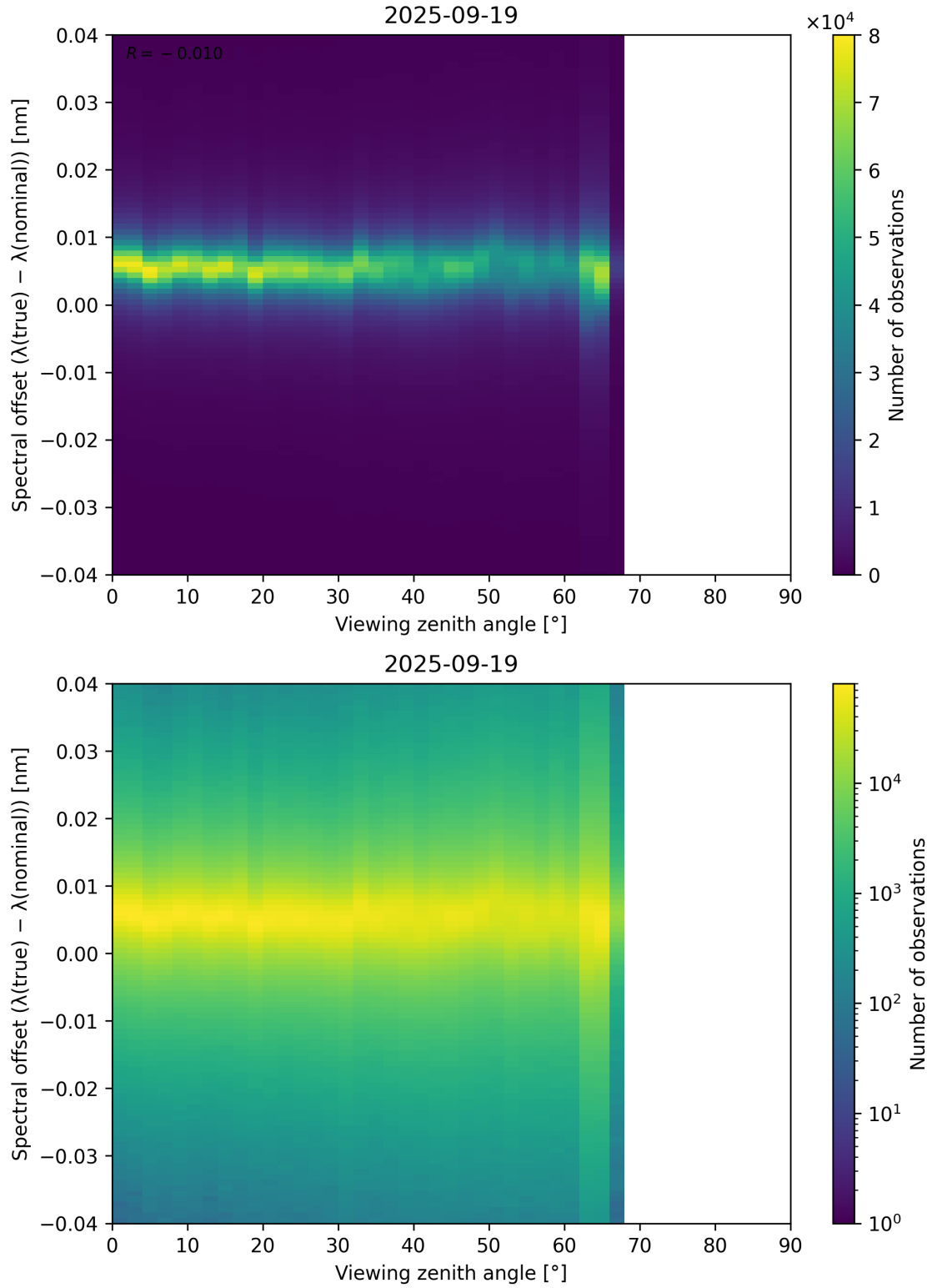
Figure 128: Scatter density plot of “Viewing zenith angle” against “Spectral offset ( \lambda_{\text{true}} - \lambda_{\text{nominal}} )” for 2025-09-18 to 2025-09-20.
