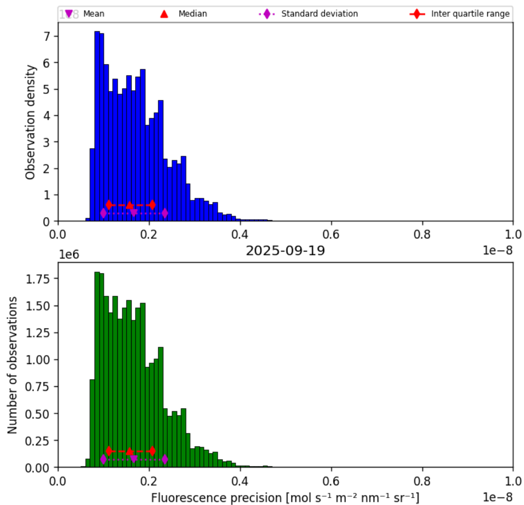
Figure 41: Histogram of “Fluorescence precision” for 2025-09-18 to 2025-09-20
