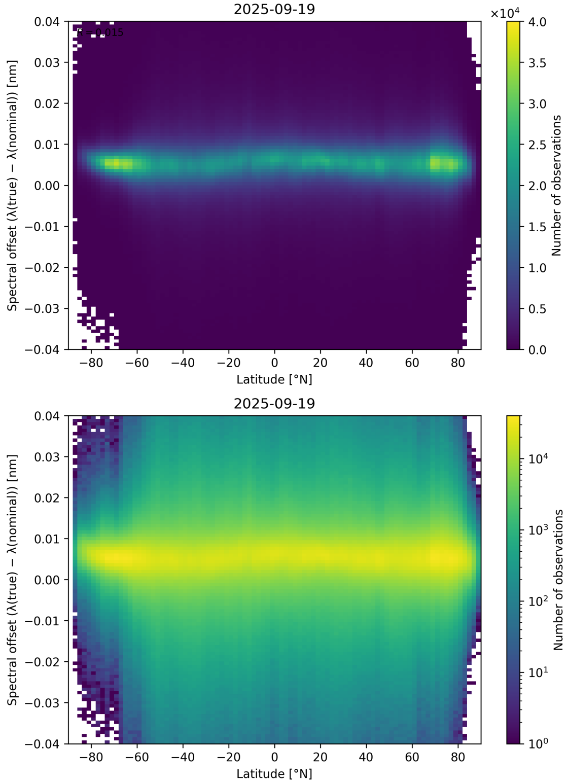
Figure 96: Scatter density plot of “Latitude” against “Spectral offset ( \lambda_{\text{true}} - \lambda_{\text{nominal}} )” for 2025-09-18 to 2025-09-20.
