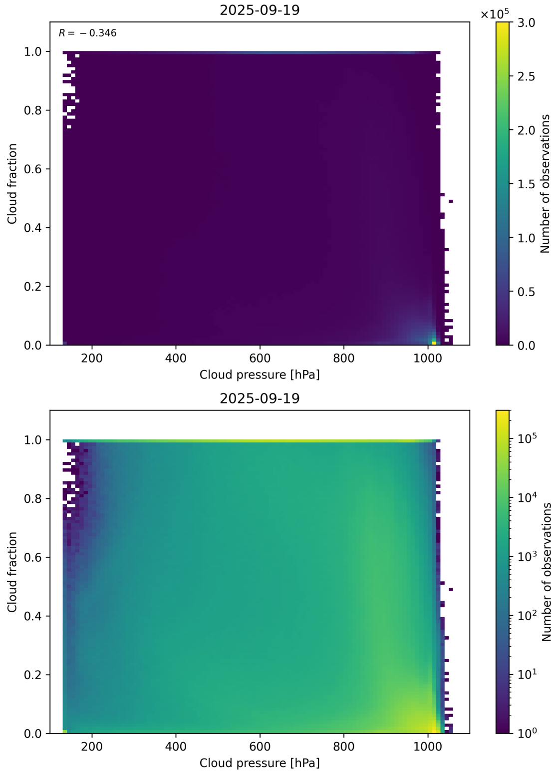
Figure 79: Scatter density plot of “Cloud pressure” against “Cloud fraction” for 2025-09-18 to 2025-09-20.
