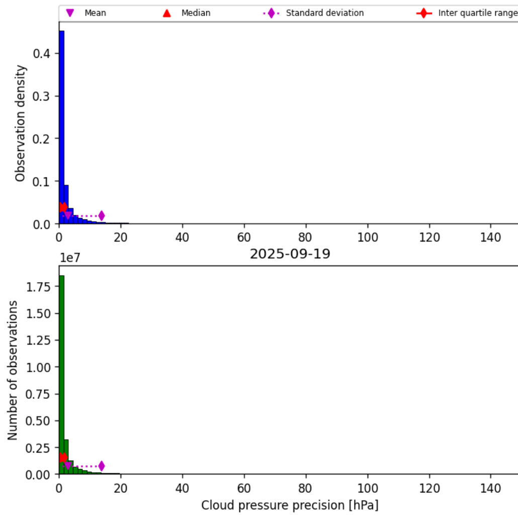
Figure 31: Histogram of “Cloud pressure precision” for 2025-09-18 to 2025-09-20
