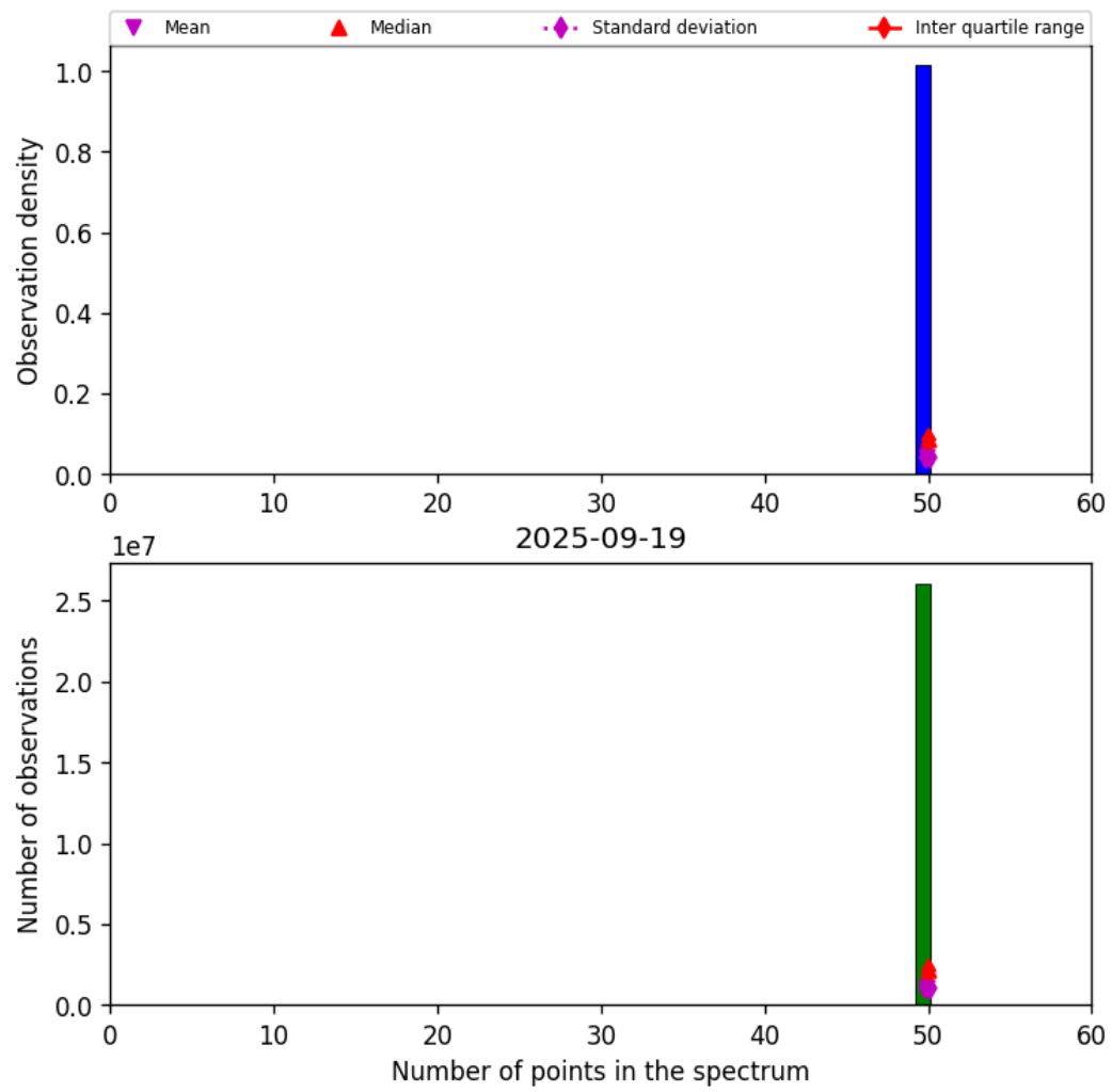
Figure 44: Histogram of “Number of points in the spectrum” for 2025-09-18 to 2025-09-20
