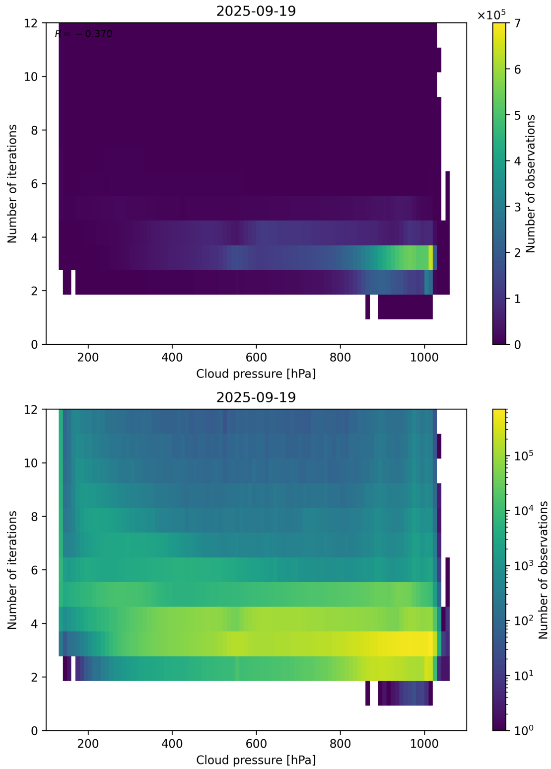
Figure 81: Scatter density plot of “Cloud pressure” against “Number of iterations” for 2025-09-18 to 2025-09-20.
