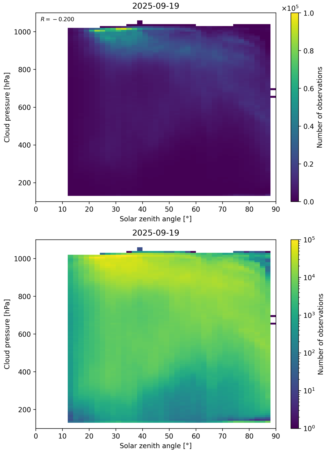
Figure 111: Scatter density plot of “Solar zenith angle” against “Cloud pressure” for 2025-09-18 to 2025-09-20.
