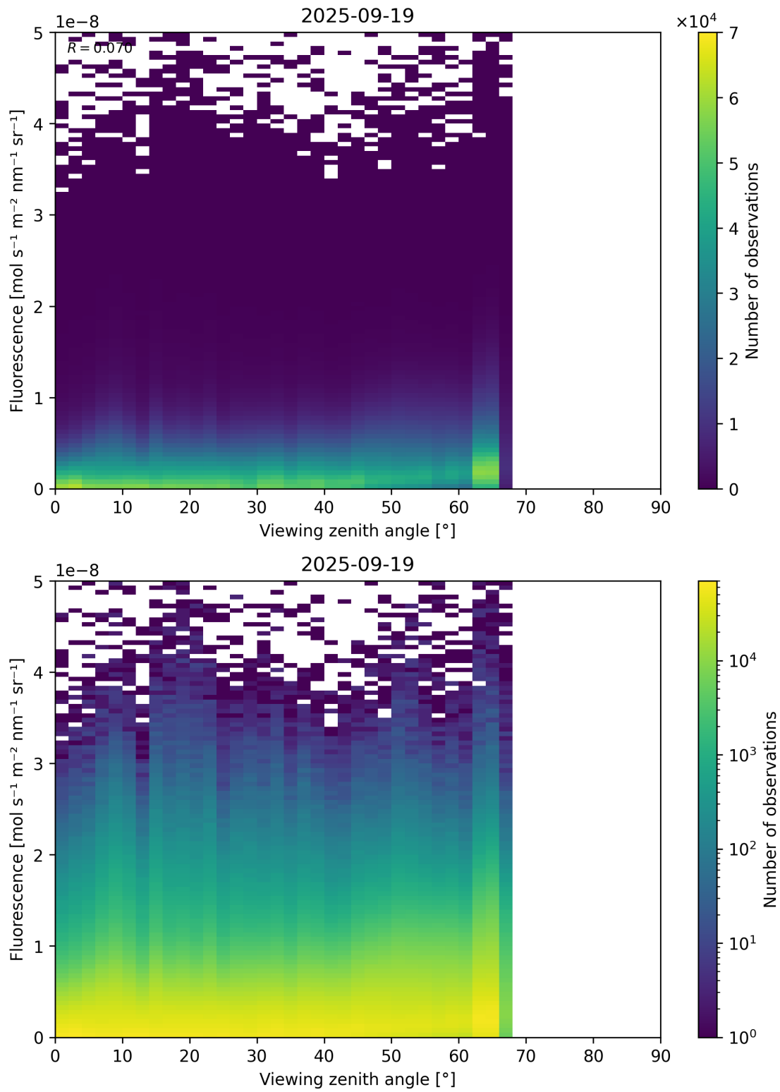
Figure 122: Scatter density plot of “Viewing zenith angle” against “Fluorescence” for 2025-09-18 to 2025-09-20.
