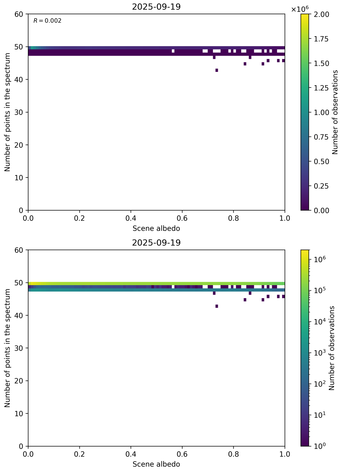
Figure 106: Scatter density plot of “Scene albedo” against “Number of points in the spectrum” for 2025-09-18 to 2025-09-20.
