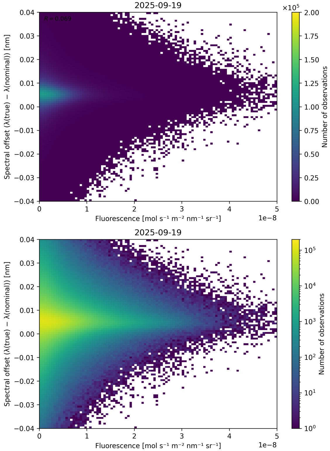
Figure 87: Scatter density plot of “Fluorescence” against “Spectral offset ( \lambda_{\text{true}} - \lambda_{\text{nominal}} )” for 2025-09-18 to 2025-09-20.
