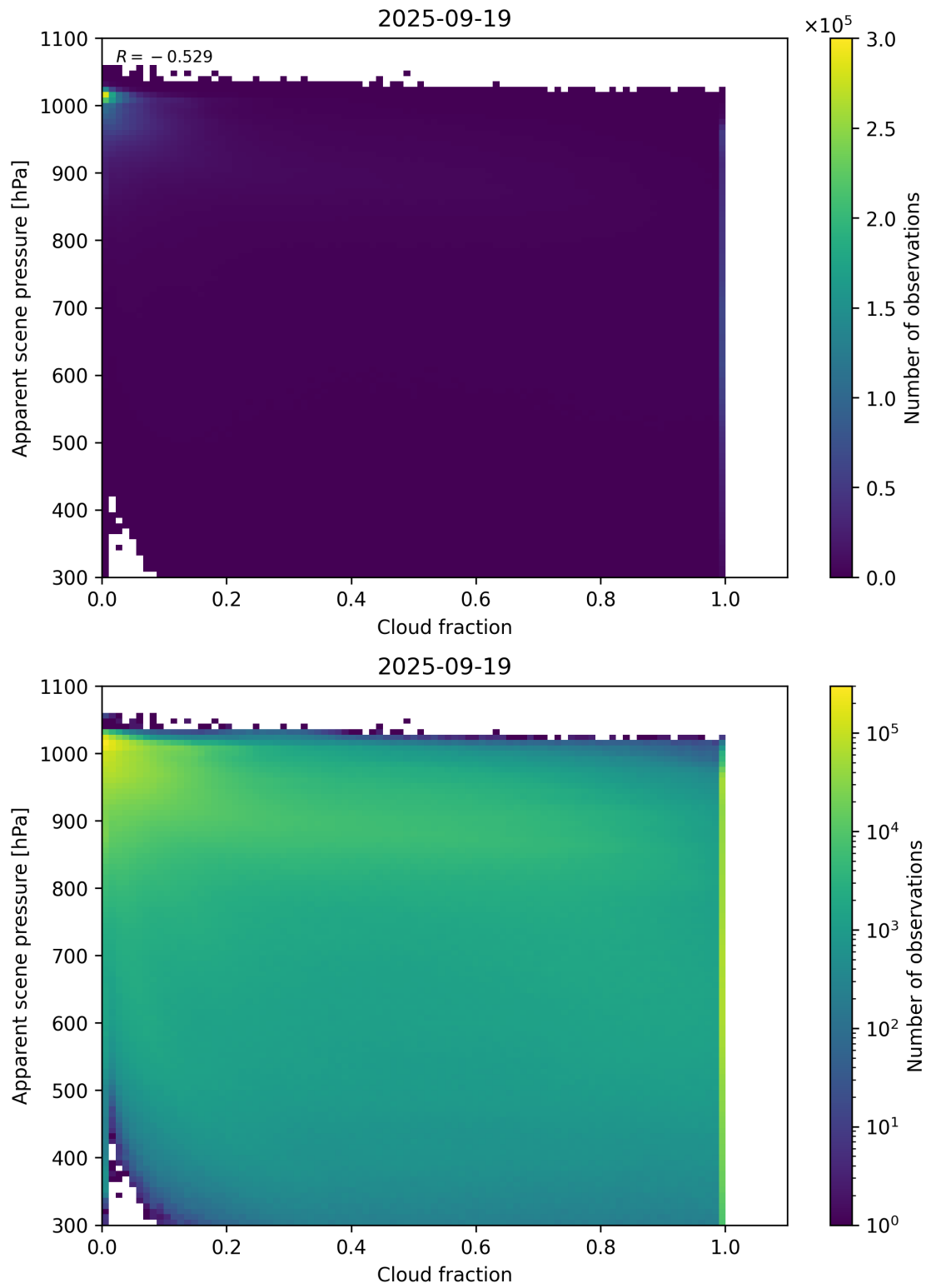
Figure 70: Scatter density plot of “Cloud fraction” against “Apparent scene pressure” for 2025-09-18 to 2025-09-20.
