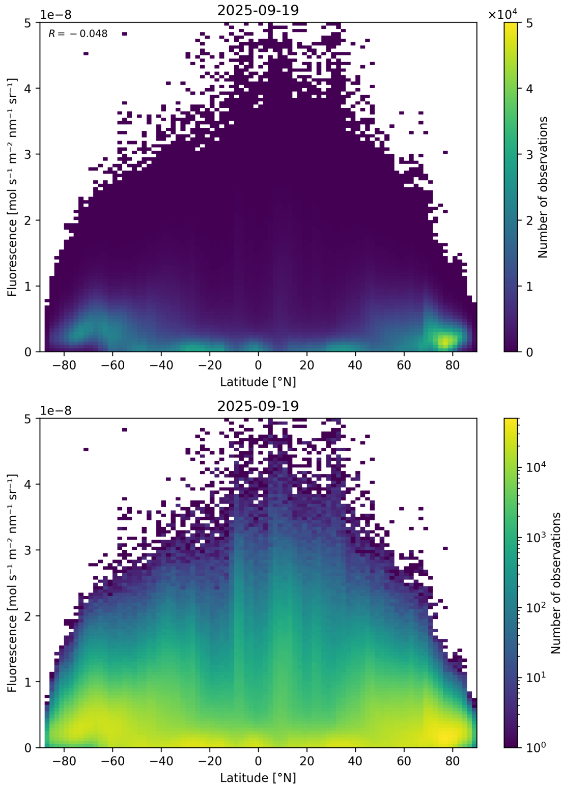
Figure 92: Scatter density plot of “Latitude” against “Fluorescence” for 2025-09-18 to 2025-09-20.
