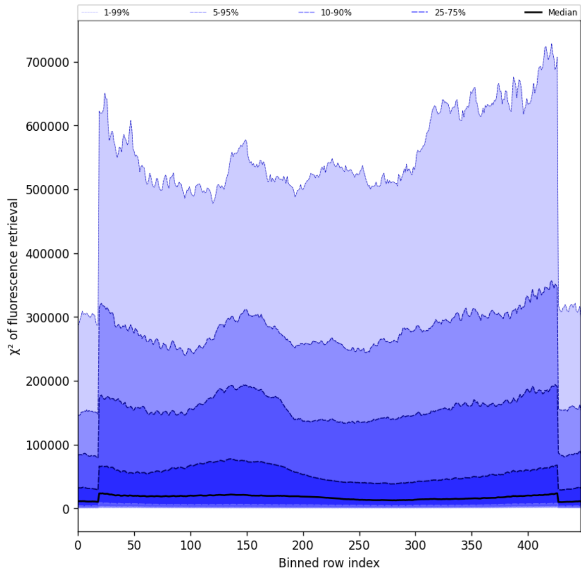
Figure 59: Along track statistics of “ \chi^2 of fluorescence retrieval” for 2025-09-18 to 2025-09-20
