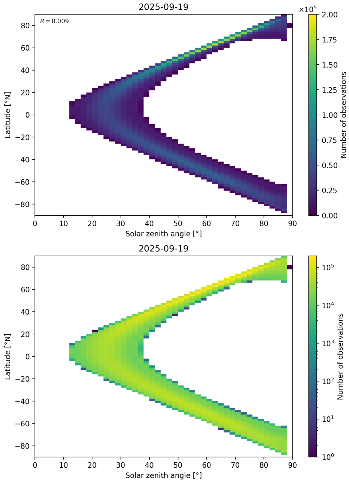
Figure 113: Scatter density plot of “Solar zenith angle” against “Latitude” for 2025-09-18 to 2025-09-20.
