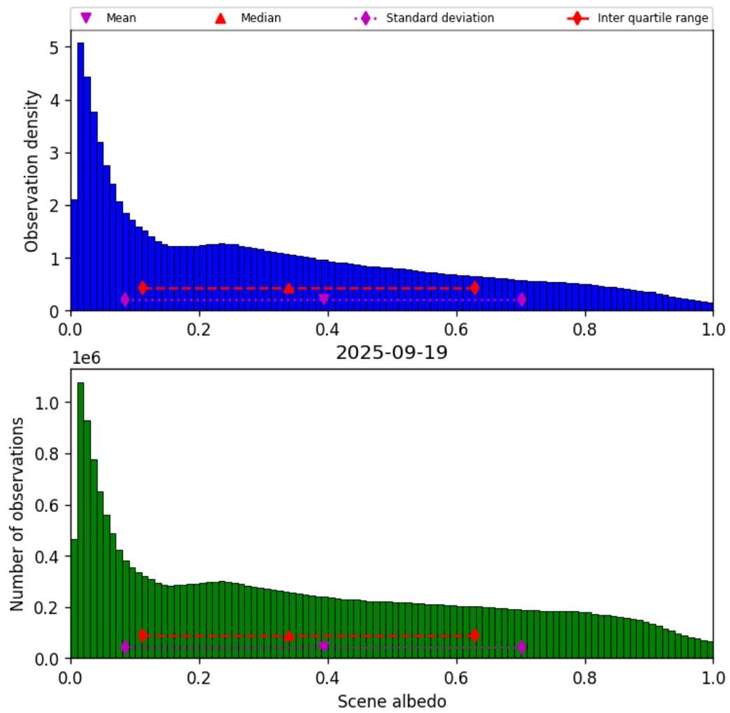
Figure 34: Histogram of “Scene albedo” for 2025-09-18 to 2025-09-20
