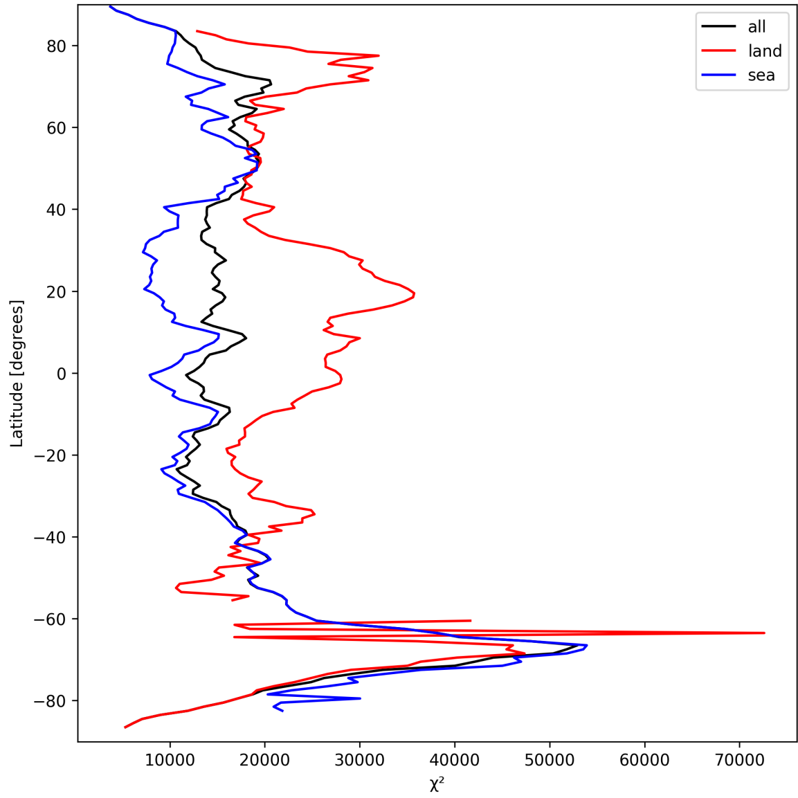
Figure 21: Zonal average of “ \chi^2 ” for 2025-09-18 to 2025-09-20.
