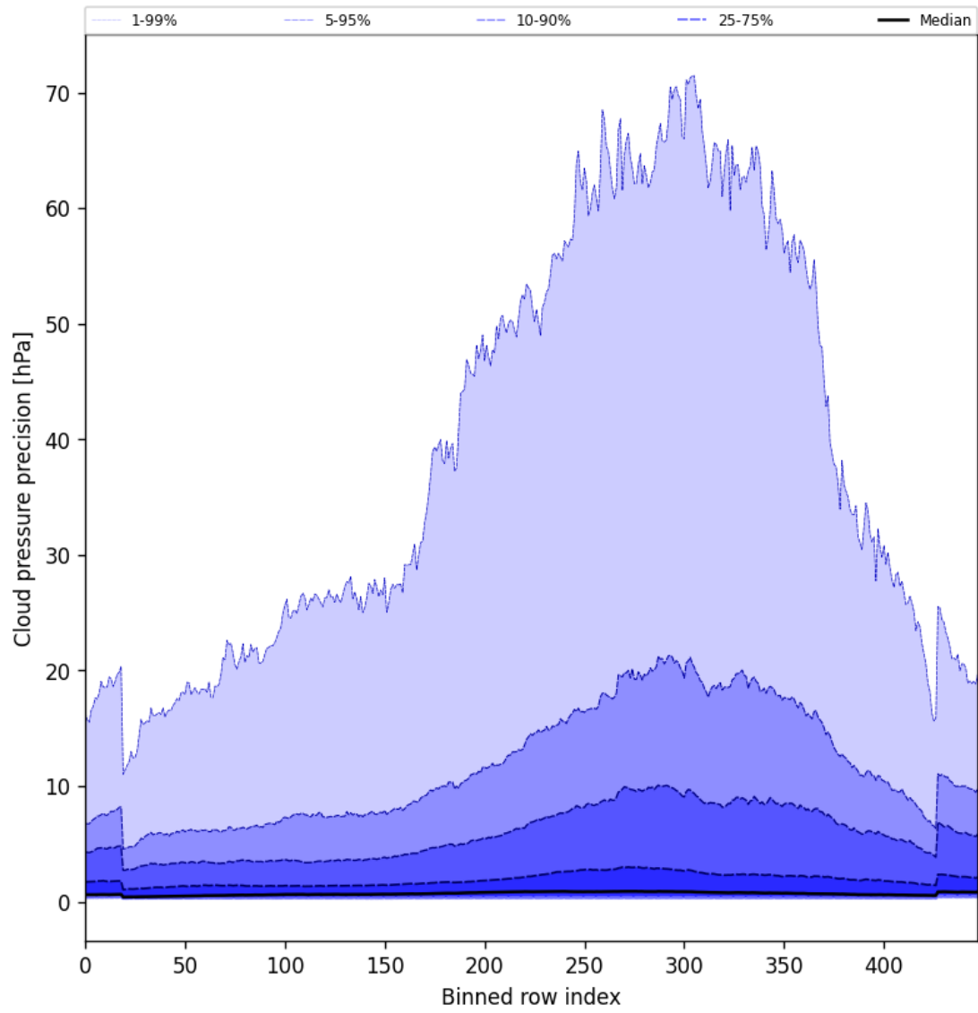
Figure 48: Along track statistics of “Cloud pressure precision” for 2025-09-18 to 2025-09-20
