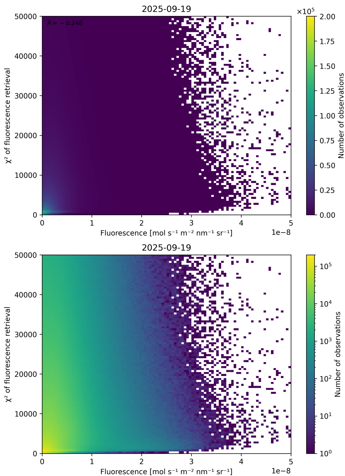
Figure 85: Scatter density plot of “Fluorescence” against “ \chi^2 of fluorescence retrieval” for 2025-09-18 to 2025-09-20.
