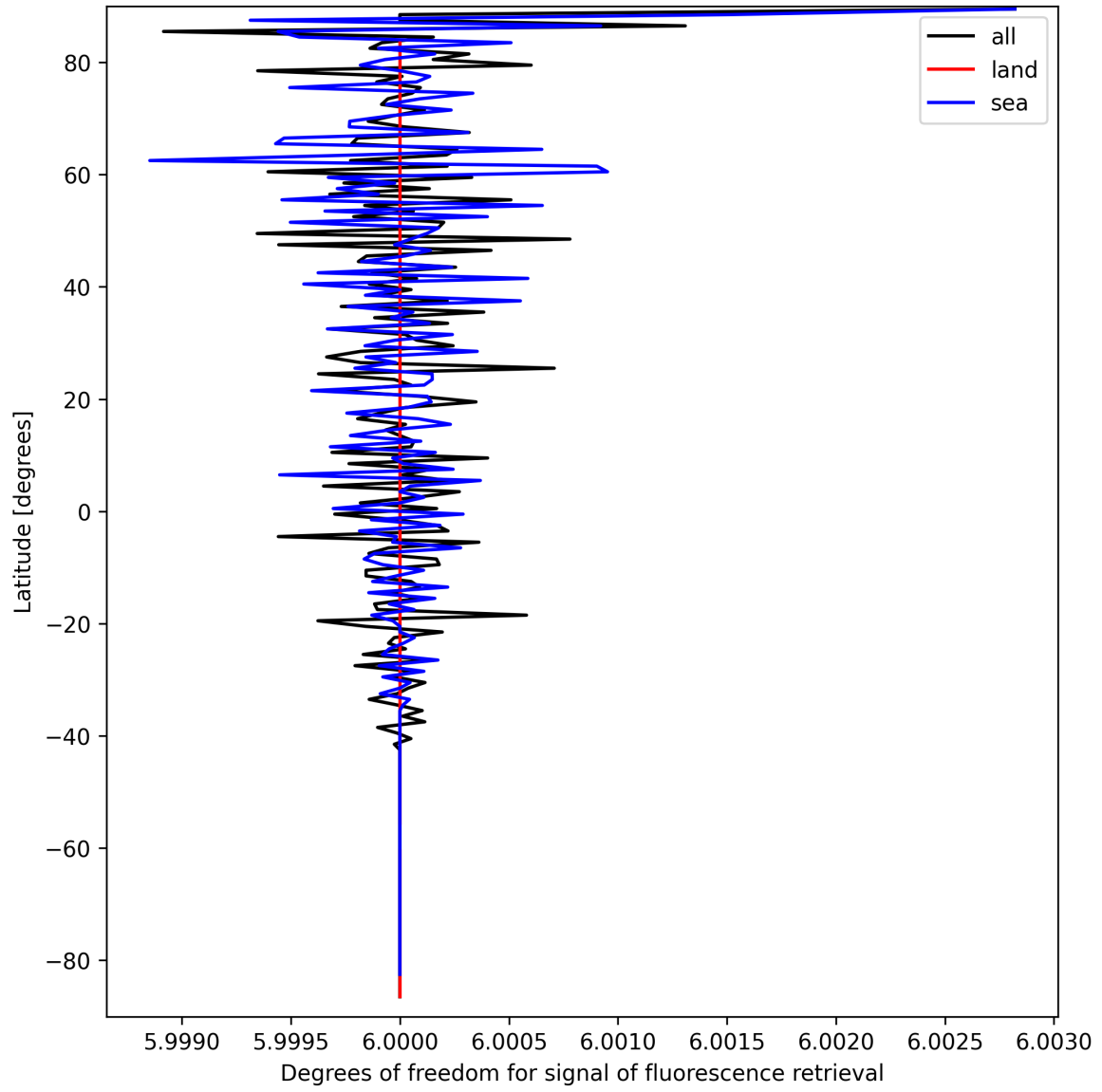
Figure 26: Zonal average of “Degrees of freedom for signal of fluorescence retrieval” for 2025-09-18 to 2025-09-20.
