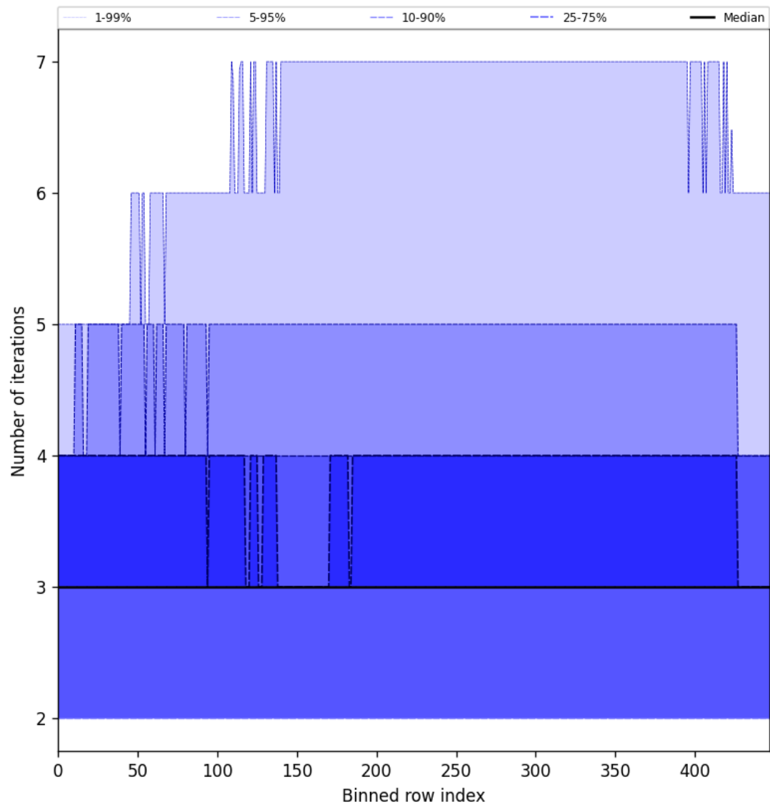
Figure 56: Along track statistics of “Number of iterations” for 2025-09-18 to 2025-09-20
