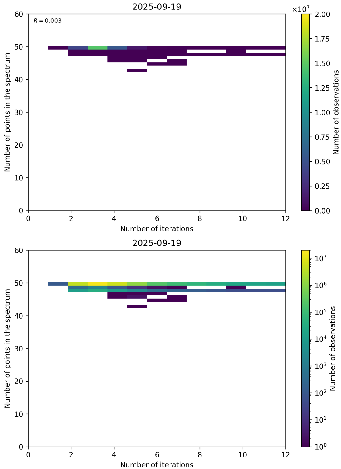
Figure 99: Scatter density plot of “Number of iterations” against “Number of points in the spectrum” for 2025-09-18 to 2025-09-20.
