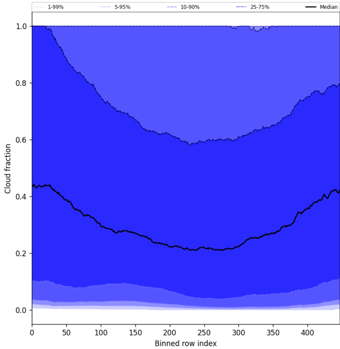
Figure 49: Along track statistics of “Cloud fraction” for 2025-09-18 to 2025-09-20
