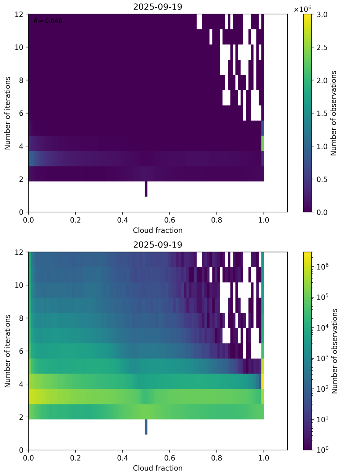
Figure 73: Scatter density plot of “Cloud fraction” against “Number of iterations” for 2025-09-18 to 2025-09-20.
