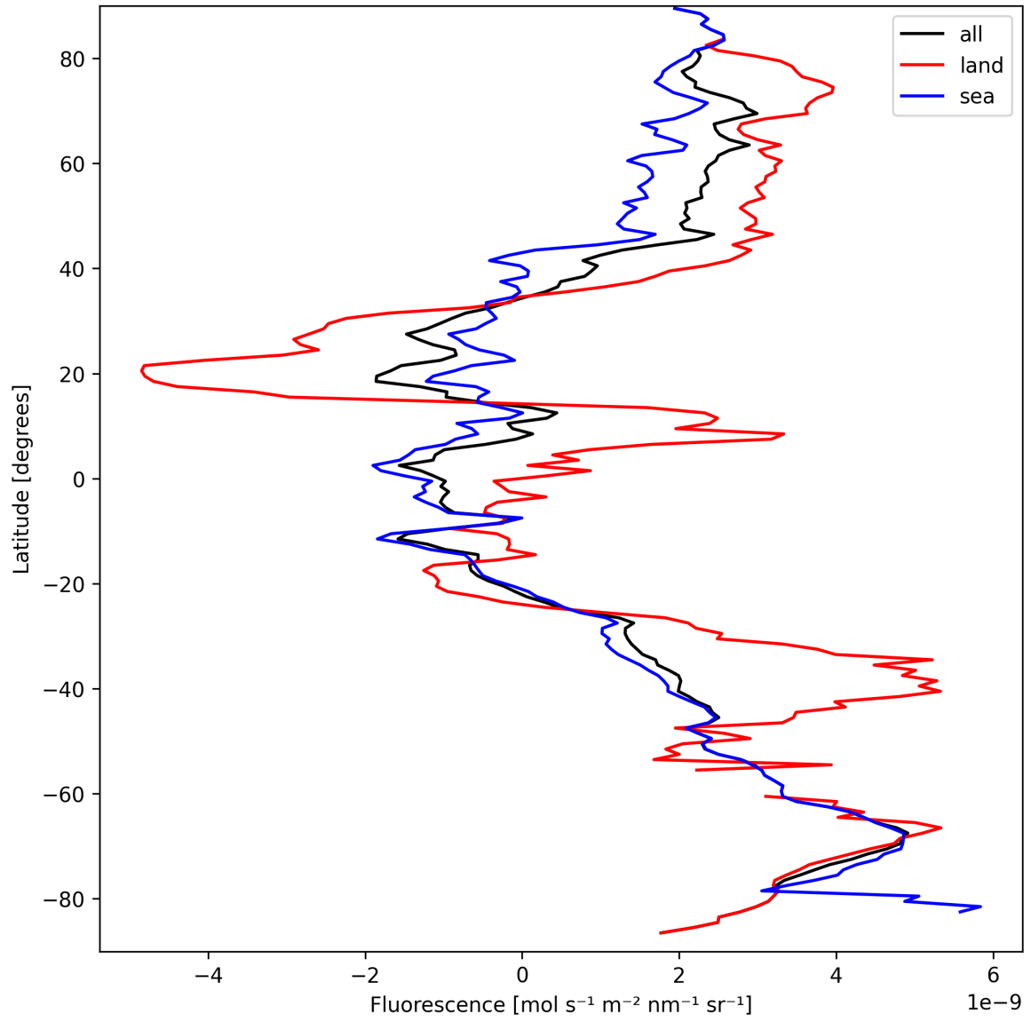
Figure 23: Zonal average of “Fluorescence” for 2025-09-18 to 2025-09-20.
