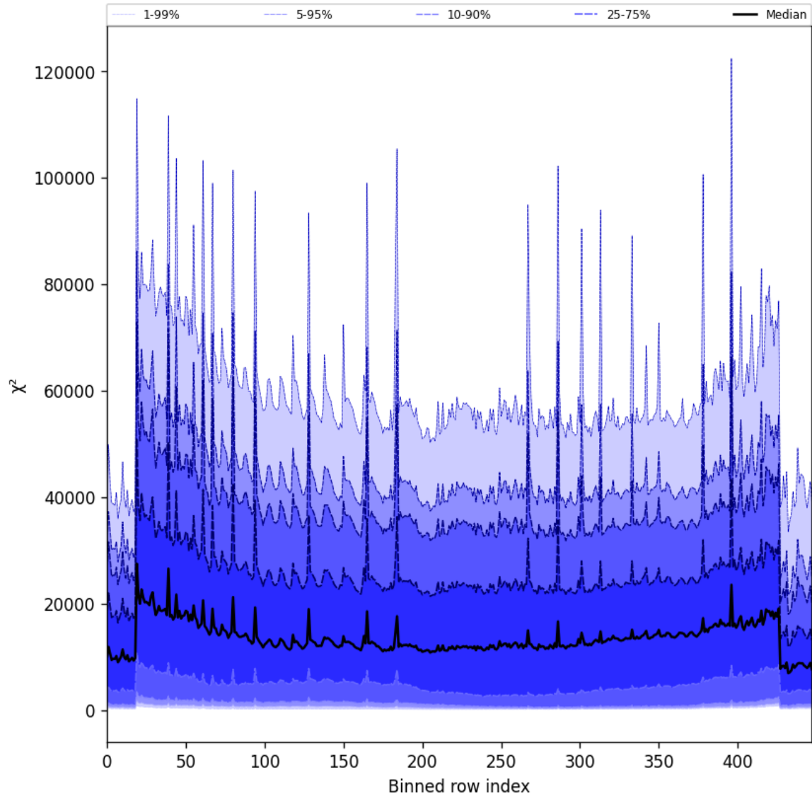
Figure 55: Along track statistics of “ \chi^2 ” for 2025-09-18 to 2025-09-20
