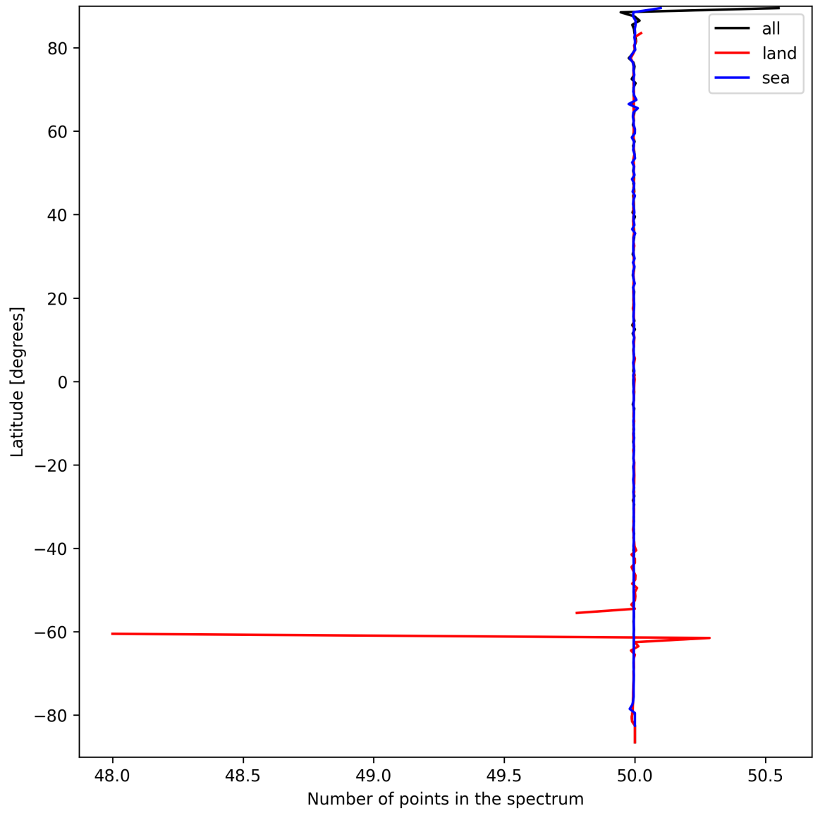
Figure 27: Zonal average of “Number of points in the spectrum” for 2025-09-18 to 2025-09-20.
