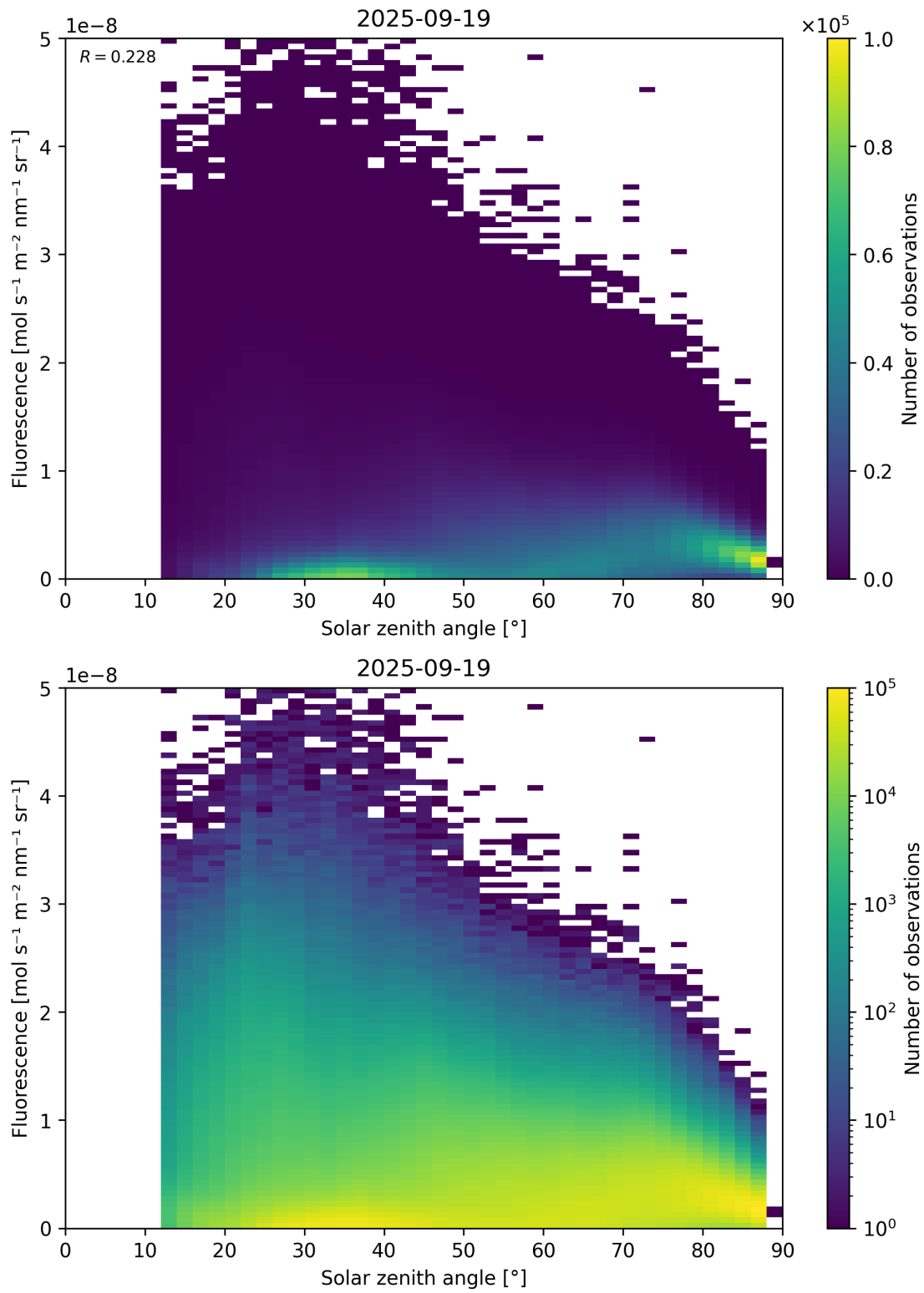
Figure 112: Scatter density plot of “Solar zenith angle” against “Fluorescence” for 2025-09-18 to 2025-09-20.
