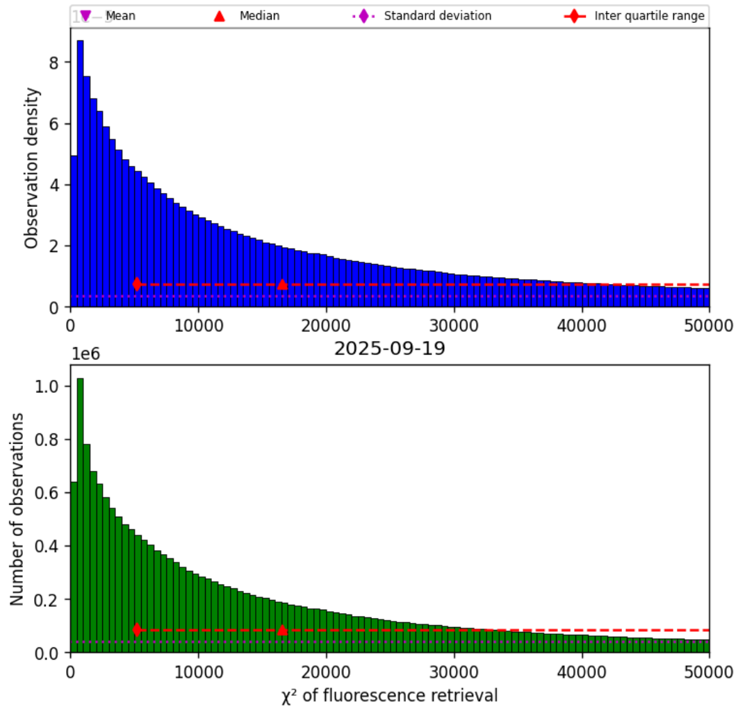
Figure 42: Histogram of “ \chi^2 of fluorescence retrieval” for 2025-09-18 to 2025-09-20
