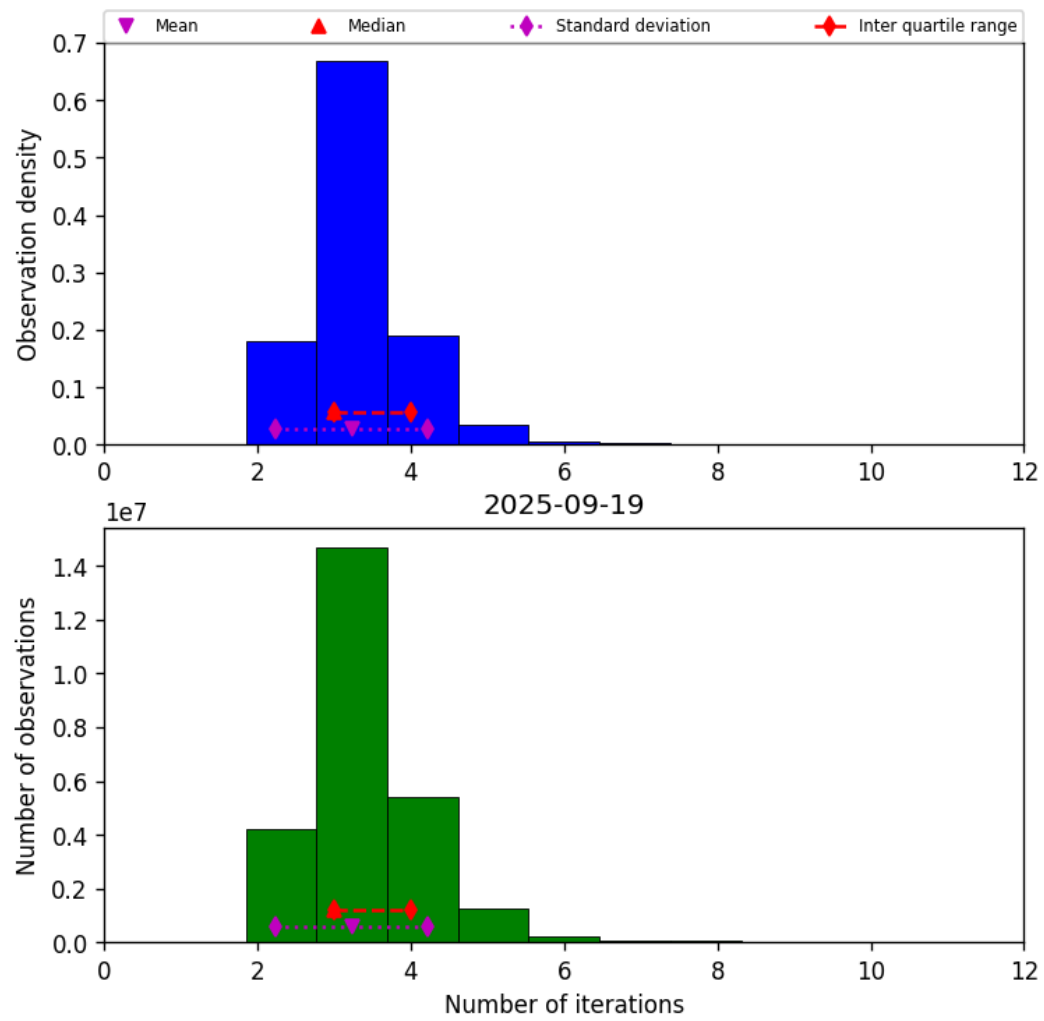
Figure 39: Histogram of “Number of iterations” for 2025-09-18 to 2025-09-20
