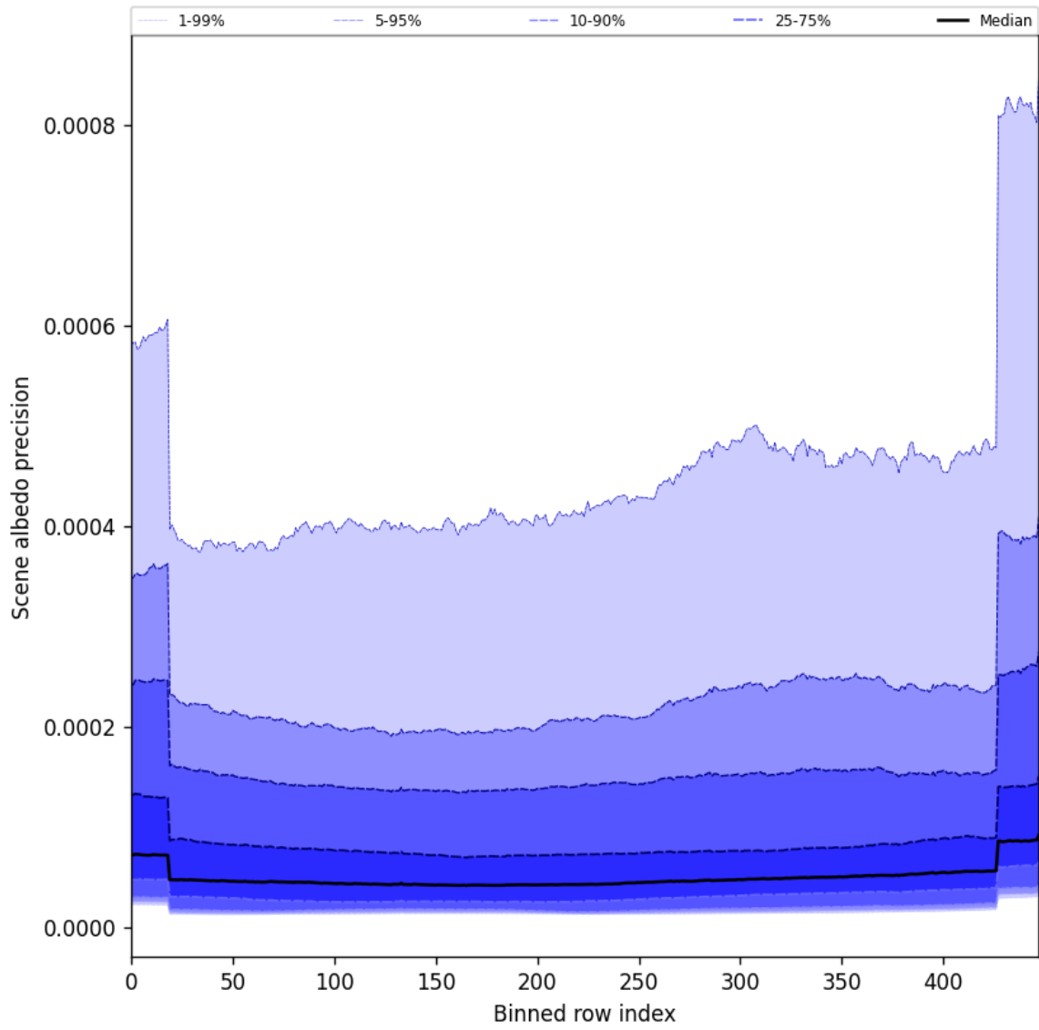
Figure 52: Along track statistics of “Scene albedo precision” for 2025-09-18 to 2025-09-20
