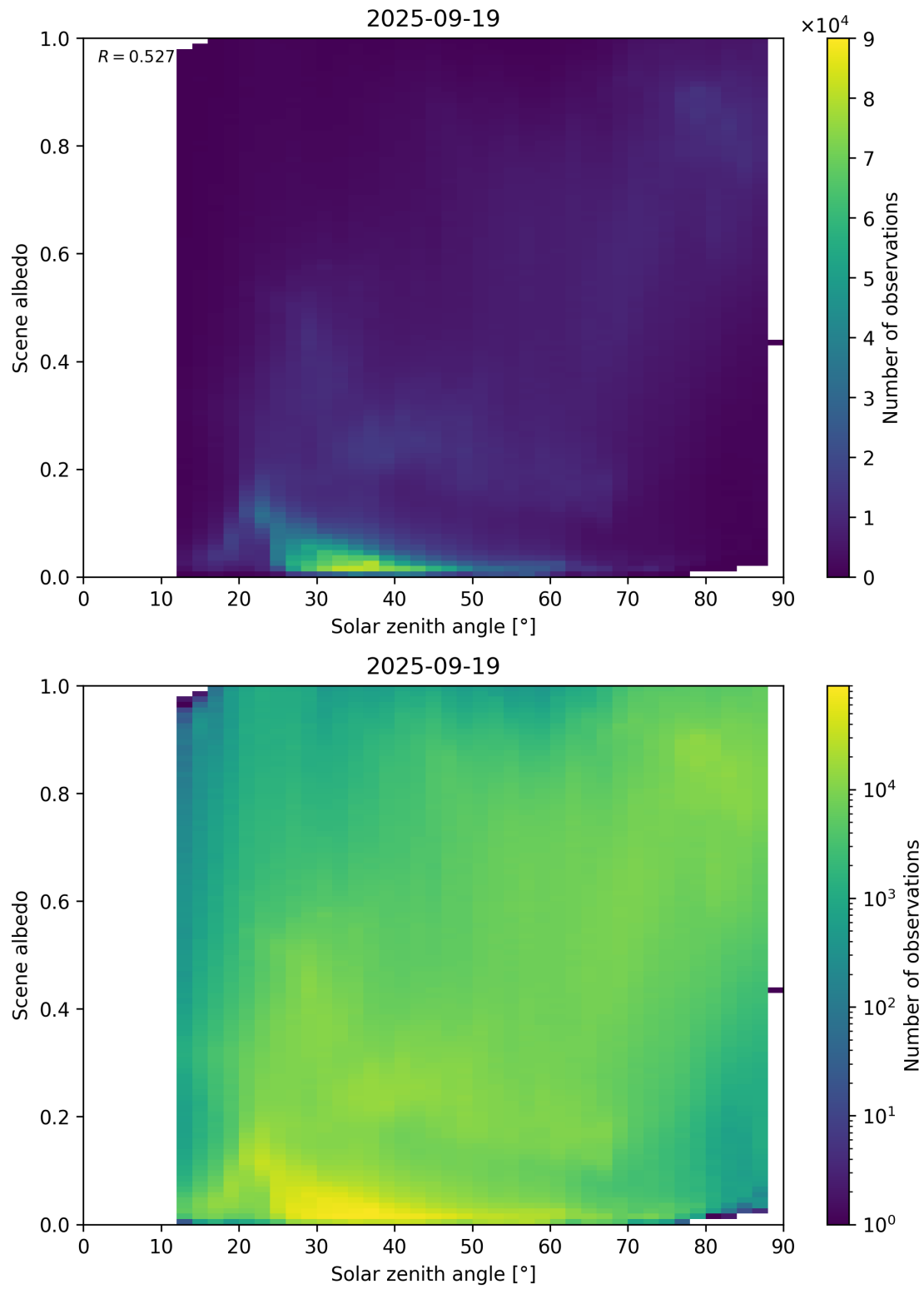
Figure 116: Scatter density plot of “Solar zenith angle” against “Scene albedo” for 2025-09-18 to 2025-09-20.
