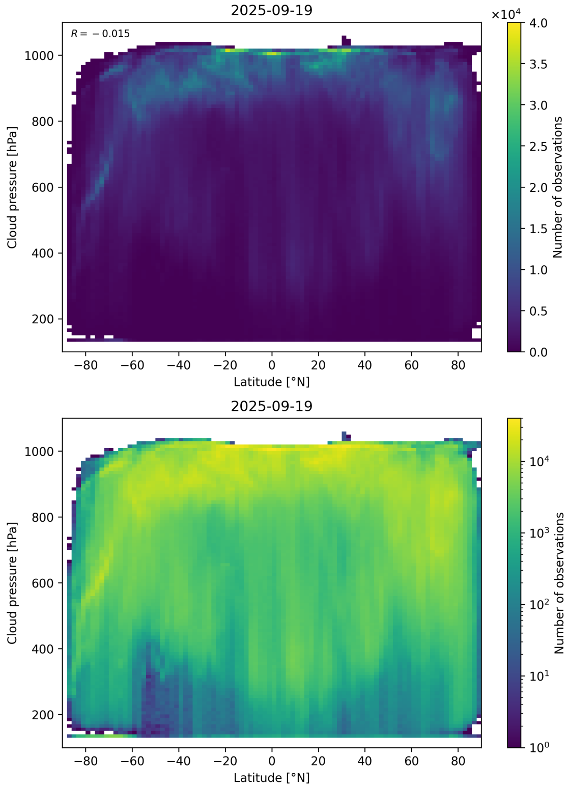
Figure 91: Scatter density plot of “Latitude” against “Cloud pressure” for 2025-09-18 to 2025-09-20.
