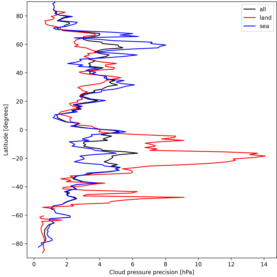
Figure 14: Zonal average of “Cloud pressure precision” for 2025-09-18 to 2025-09-20.
