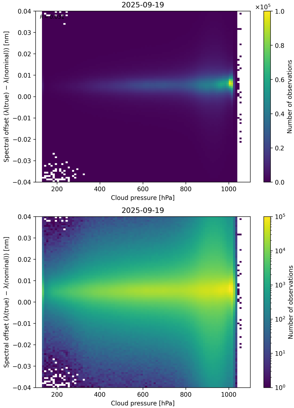
Figure 84: Scatter density plot of “Cloud pressure” against “Spectral offset ( \lambda_{\text{true}} - \lambda_{\text{nominal}} )” for 2025-09-18 to 2025-09-20.
