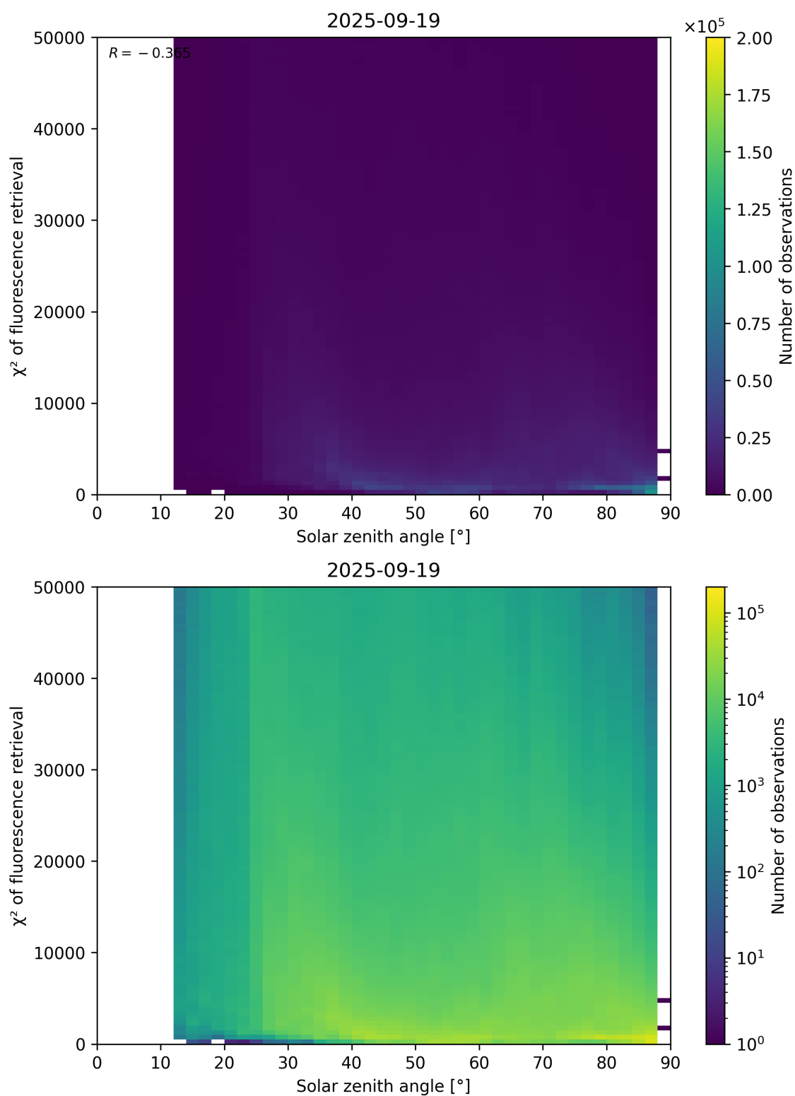
Figure 109: Scatter density plot of “Solar zenith angle” against “ \chi^2 of fluorescence retrieval” for 2025-09-18 to 2025-09-20.
