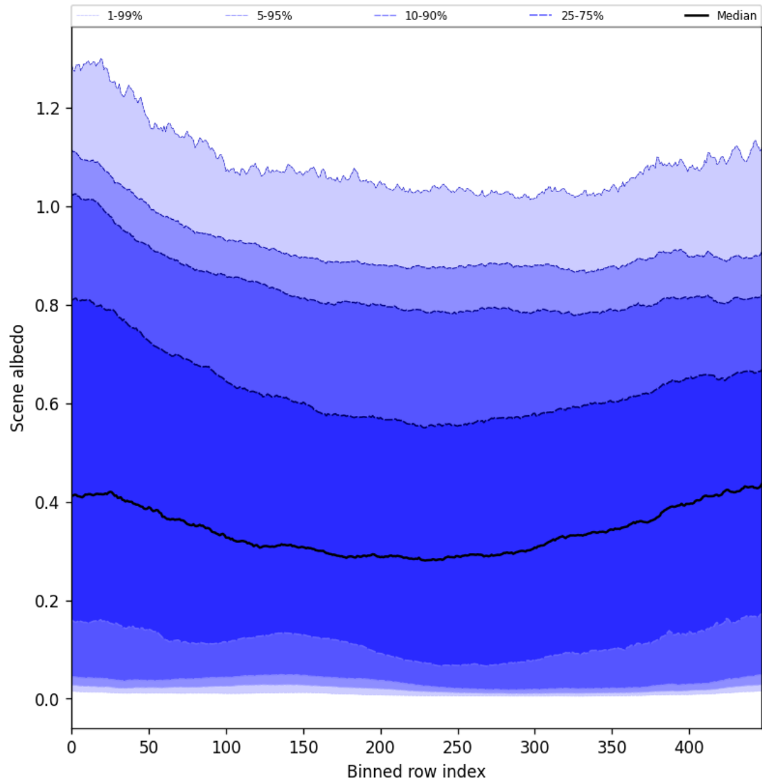
Figure 51: Along track statistics of “Scene albedo” for 2025-09-18 to 2025-09-20
