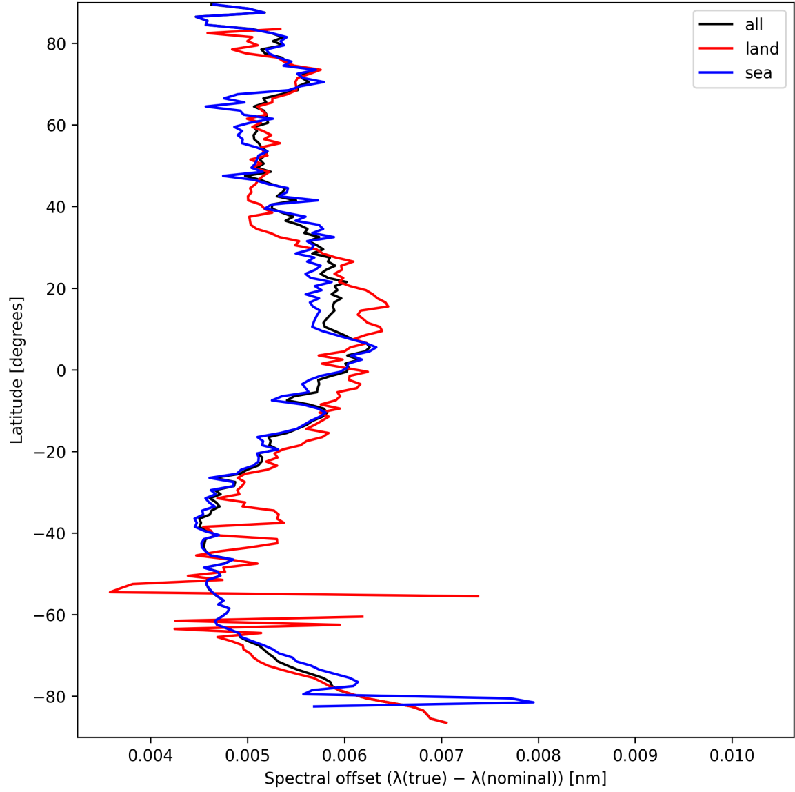
Figure 28: Zonal average of “Spectral offset ( \lambda_{\text{true}} - \lambda_{\text{nominal}} )” for 2025-09-18 to 2025-09-20.
