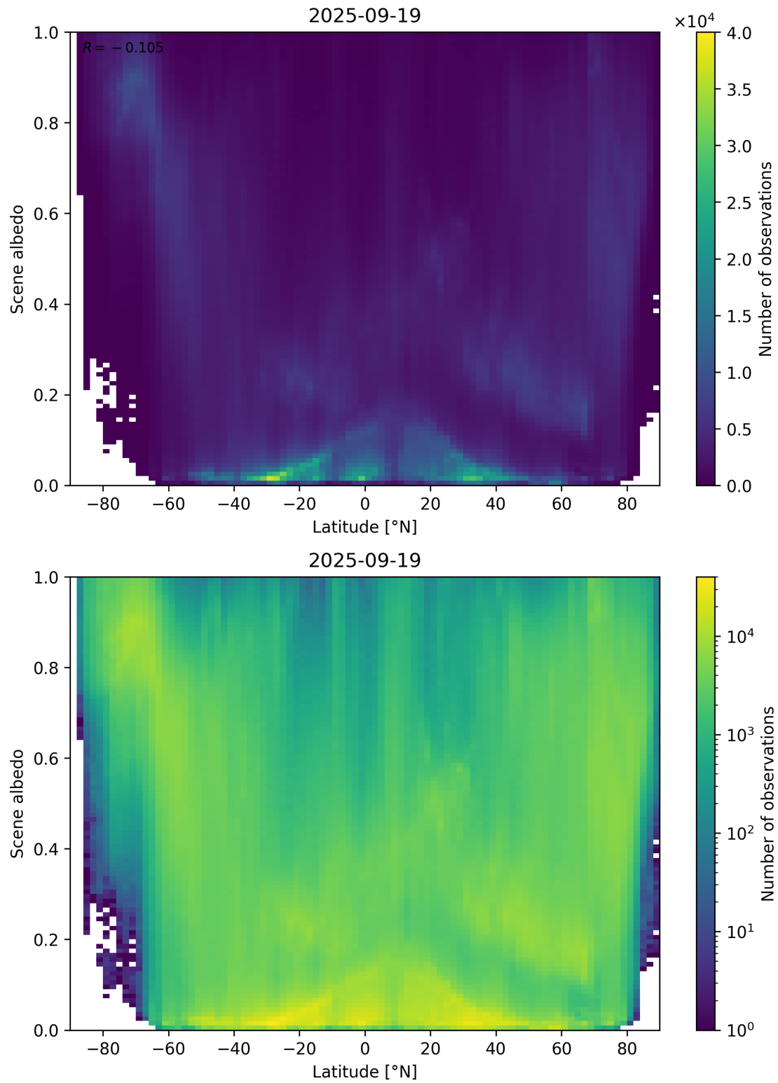
Figure 95: Scatter density plot of “Latitude” against “Scene albedo” for 2025-09-18 to 2025-09-20.
