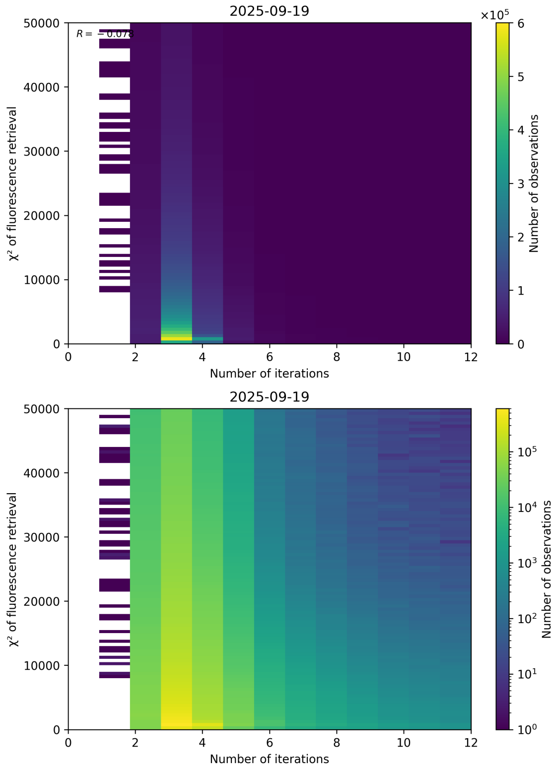
Figure 97: Scatter density plot of “Number of iterations” against “ \chi^2 of fluorescence retrieval” for 2025-09-18 to 2025-09-20.
