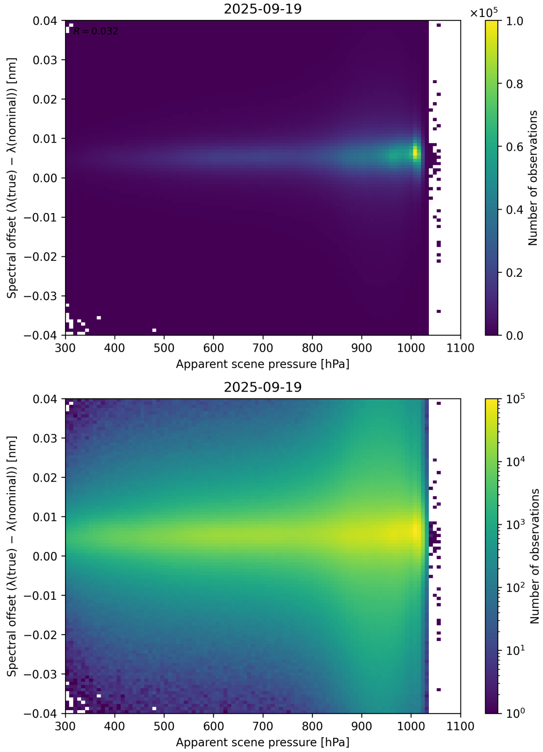
Figure 67: Scatter density plot of “Apparent scene pressure” against “Spectral offset ( \lambda_{\text{true}} - \lambda_{\text{nominal}} )” for 2025-09-18 to 2025-09-20.
