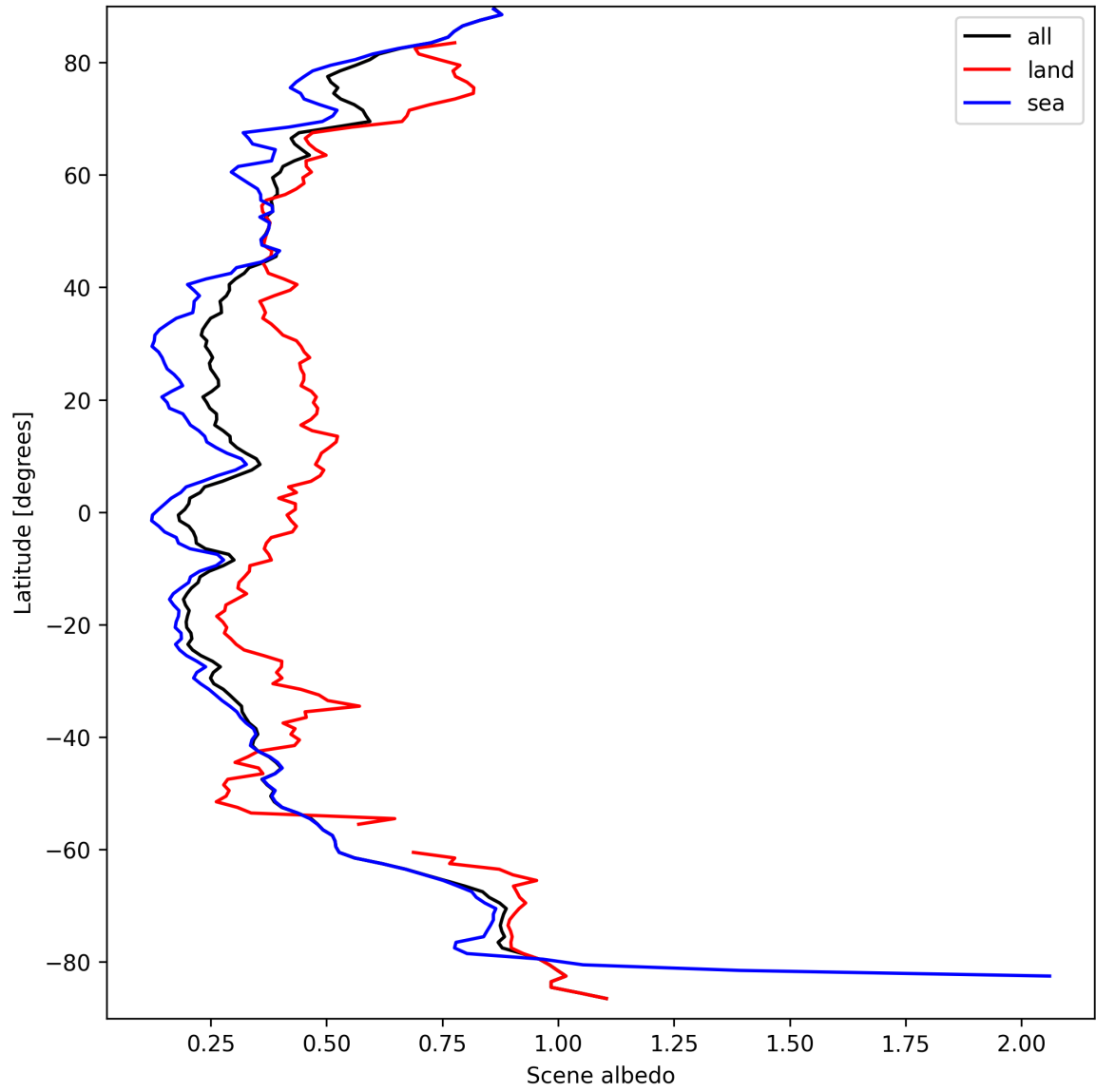
Figure 17: Zonal average of “Scene albedo” for 2025-09-18 to 2025-09-20.
