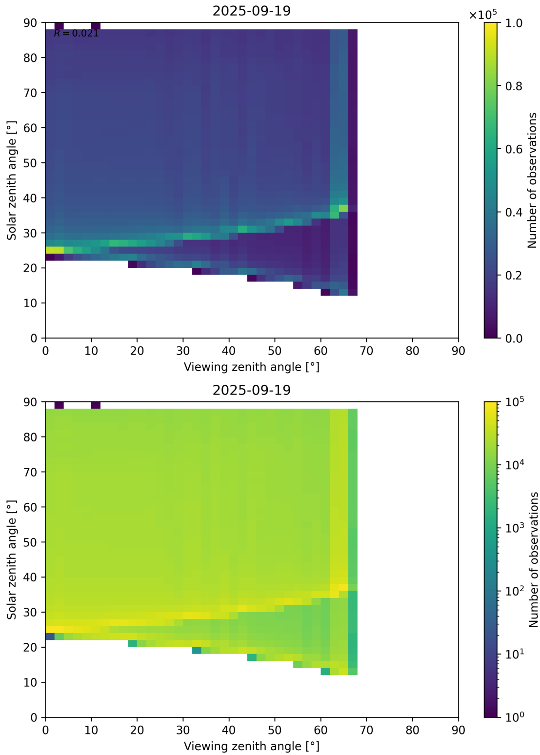
Figure 127: Scatter density plot of “Viewing zenith angle” against “Solar zenith angle” for 2025-09-18 to 2025-09-20.
