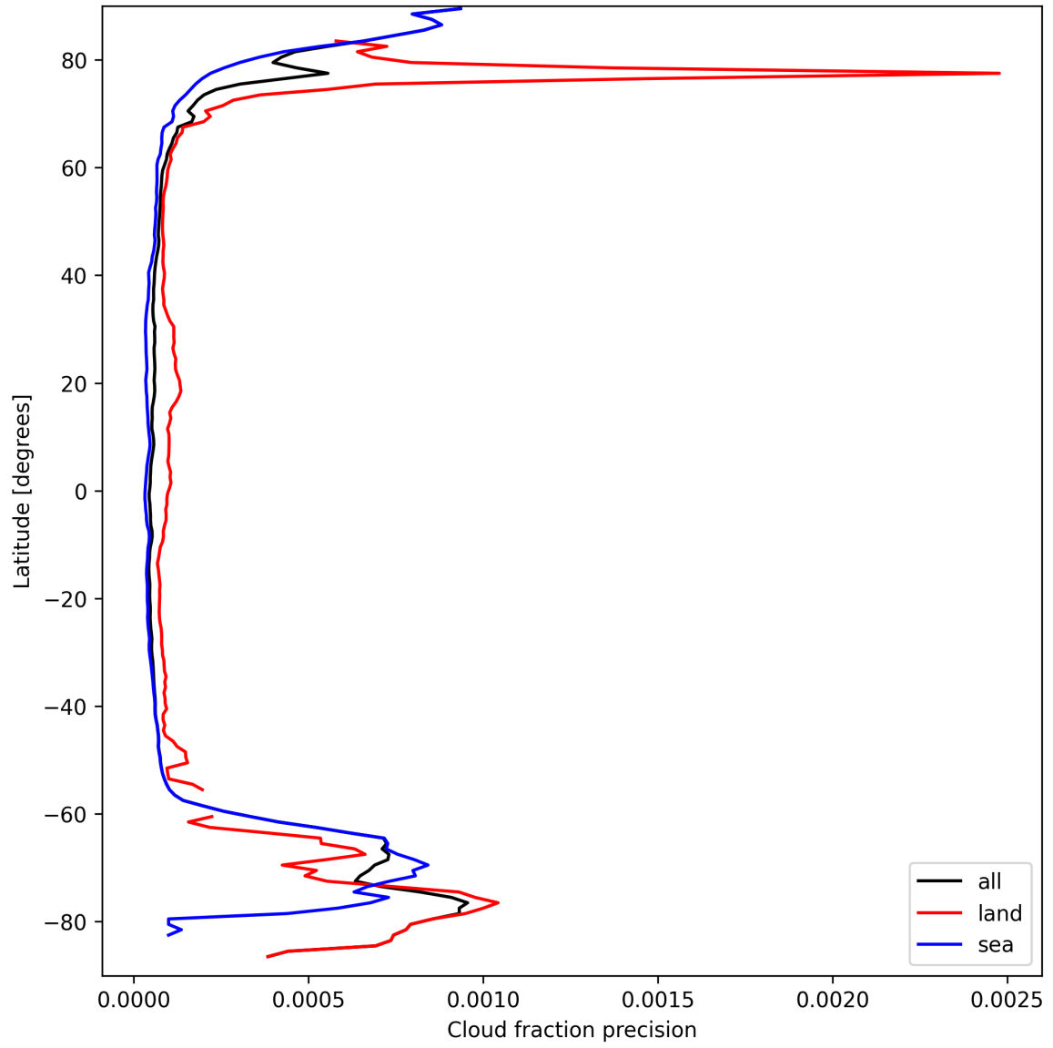
Figure 16: Zonal average of “Cloud fraction precision” for 2025-09-18 to 2025-09-20.
