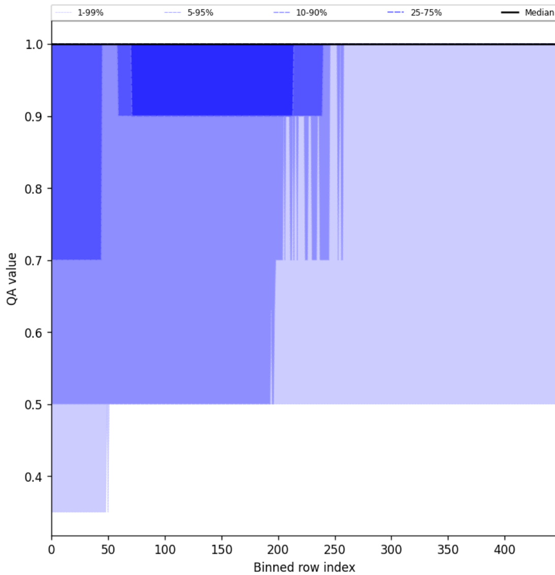
Figure 46: Along track statistics of “QA value” for 2025-09-18 to 2025-09-20
