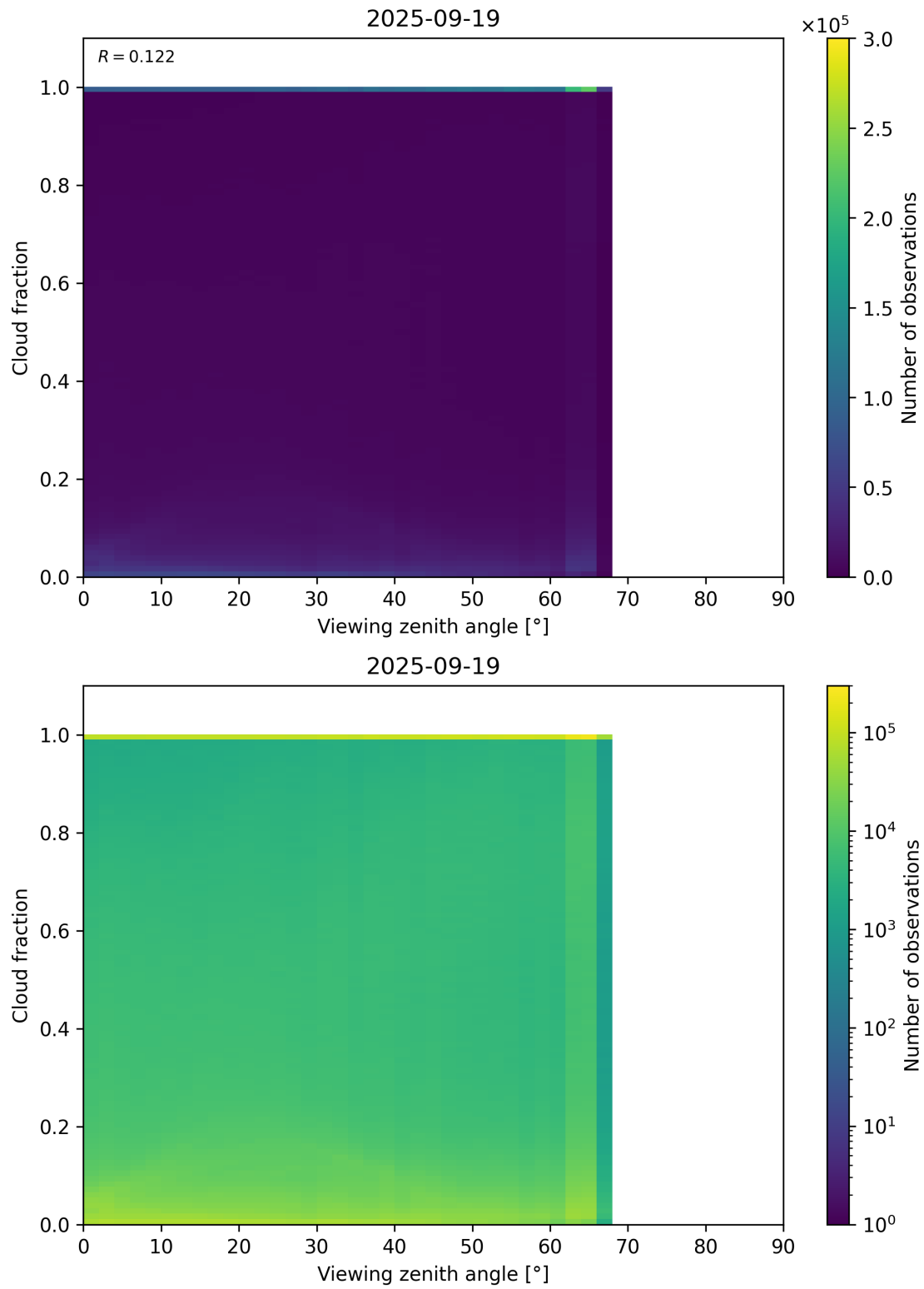
Figure 120: Scatter density plot of “Viewing zenith angle” against “Cloud fraction” for 2025-09-18 to 2025-09-20.
