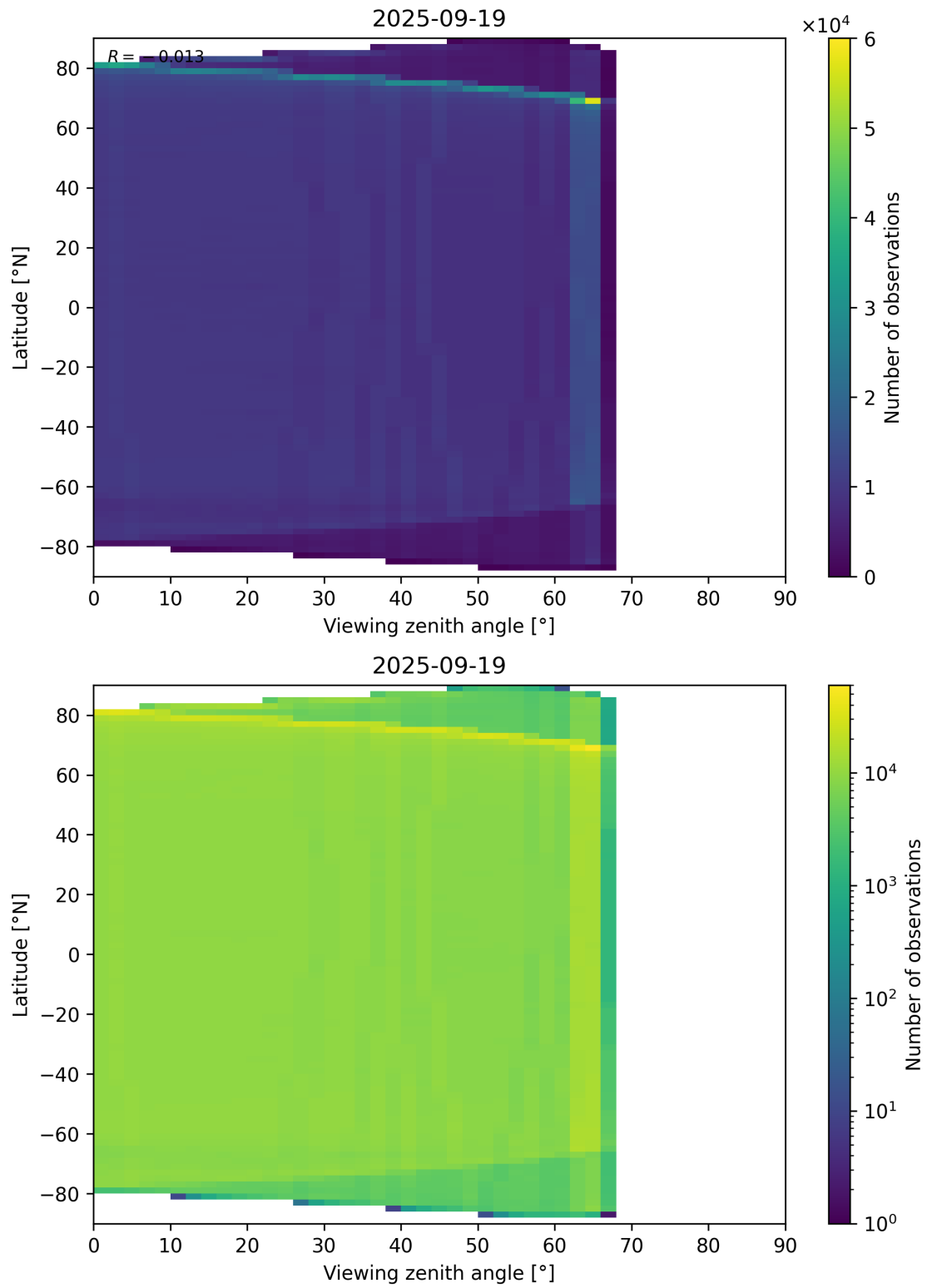
Figure 123: Scatter density plot of “Viewing zenith angle” against “Latitude” for 2025-09-18 to 2025-09-20.
