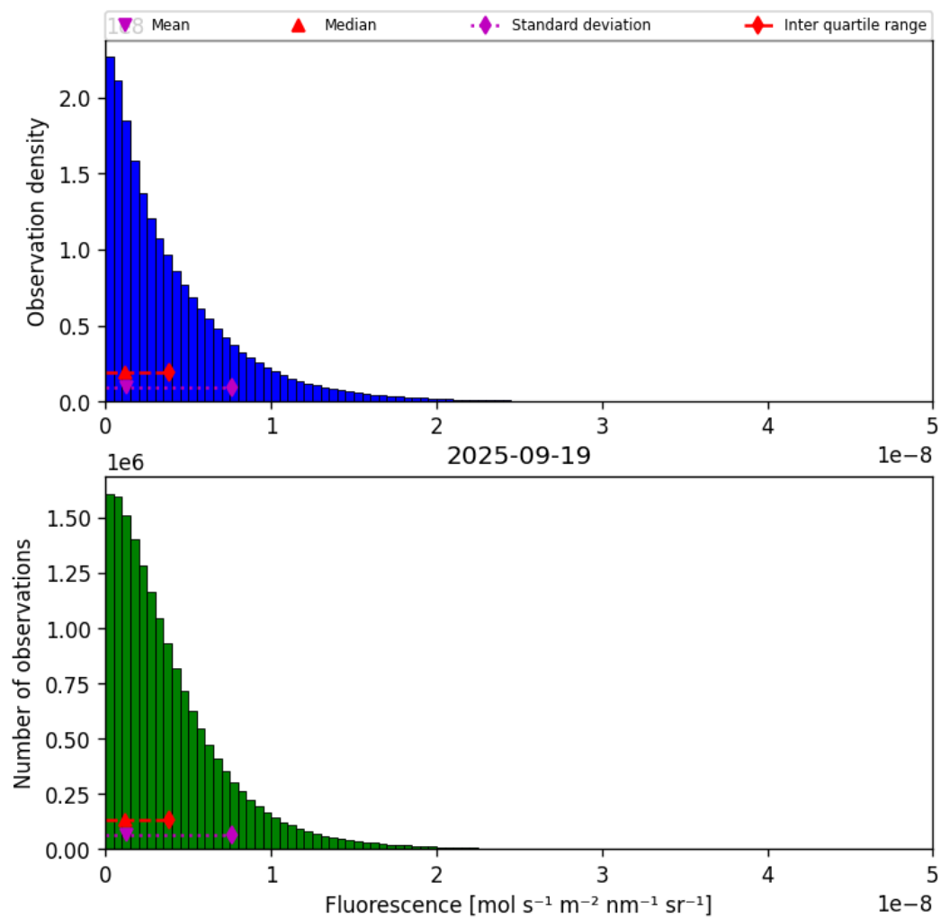
Figure 40: Histogram of “Fluorescence” for 2025-09-18 to 2025-09-20
