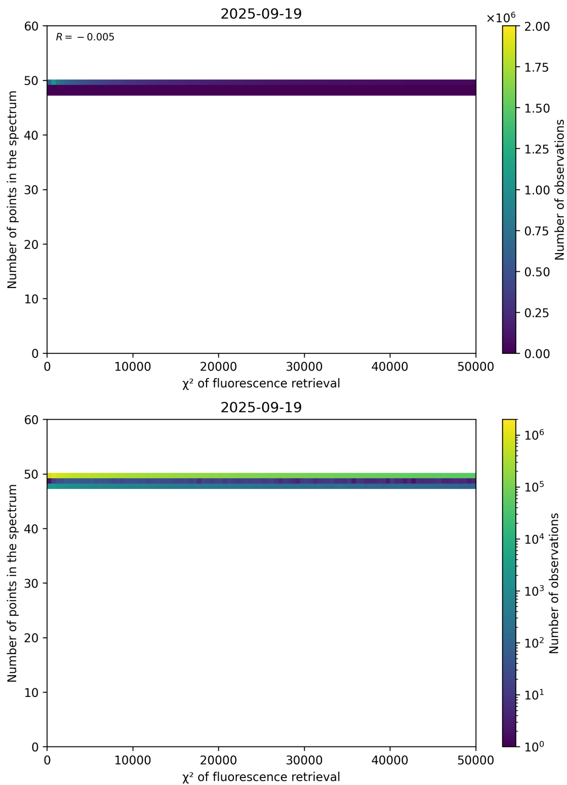
Figure 68: Scatter density plot of “ \chi^2 of fluorescence retrieval” against “Number of points in the spectrum” for 2025-09-18 to 2025-09-20.
