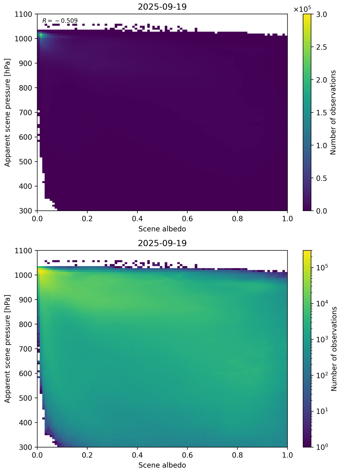
Figure 102: Scatter density plot of “Scene albedo” against “Apparent scene pressure” for 2025-09-18 to 2025-09-20.
