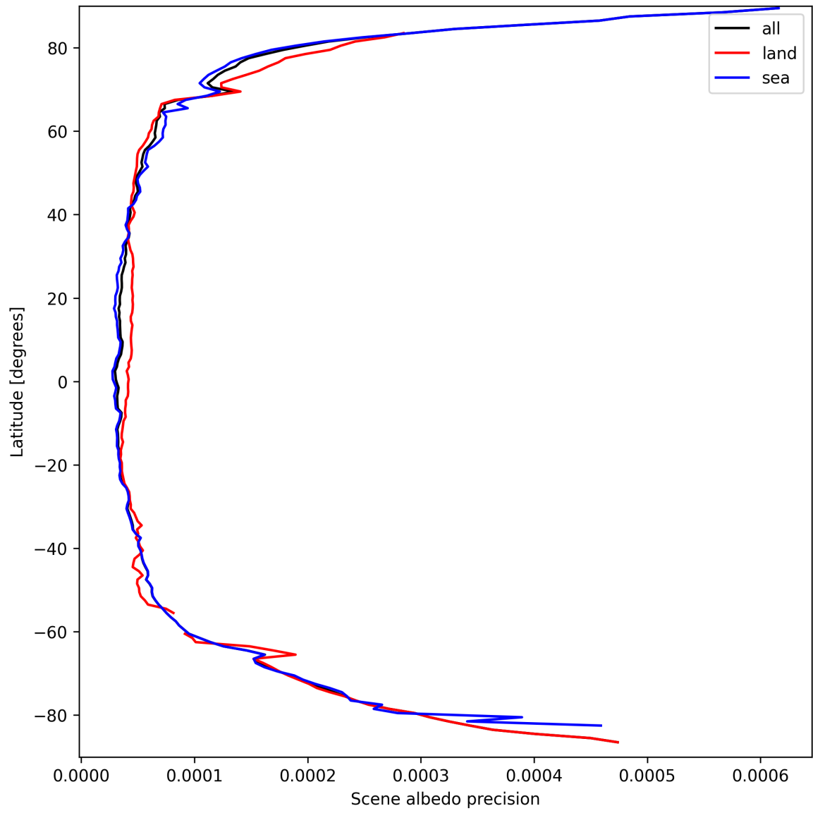
Figure 18: Zonal average of “Scene albedo precision” for 2025-09-18 to 2025-09-20.
