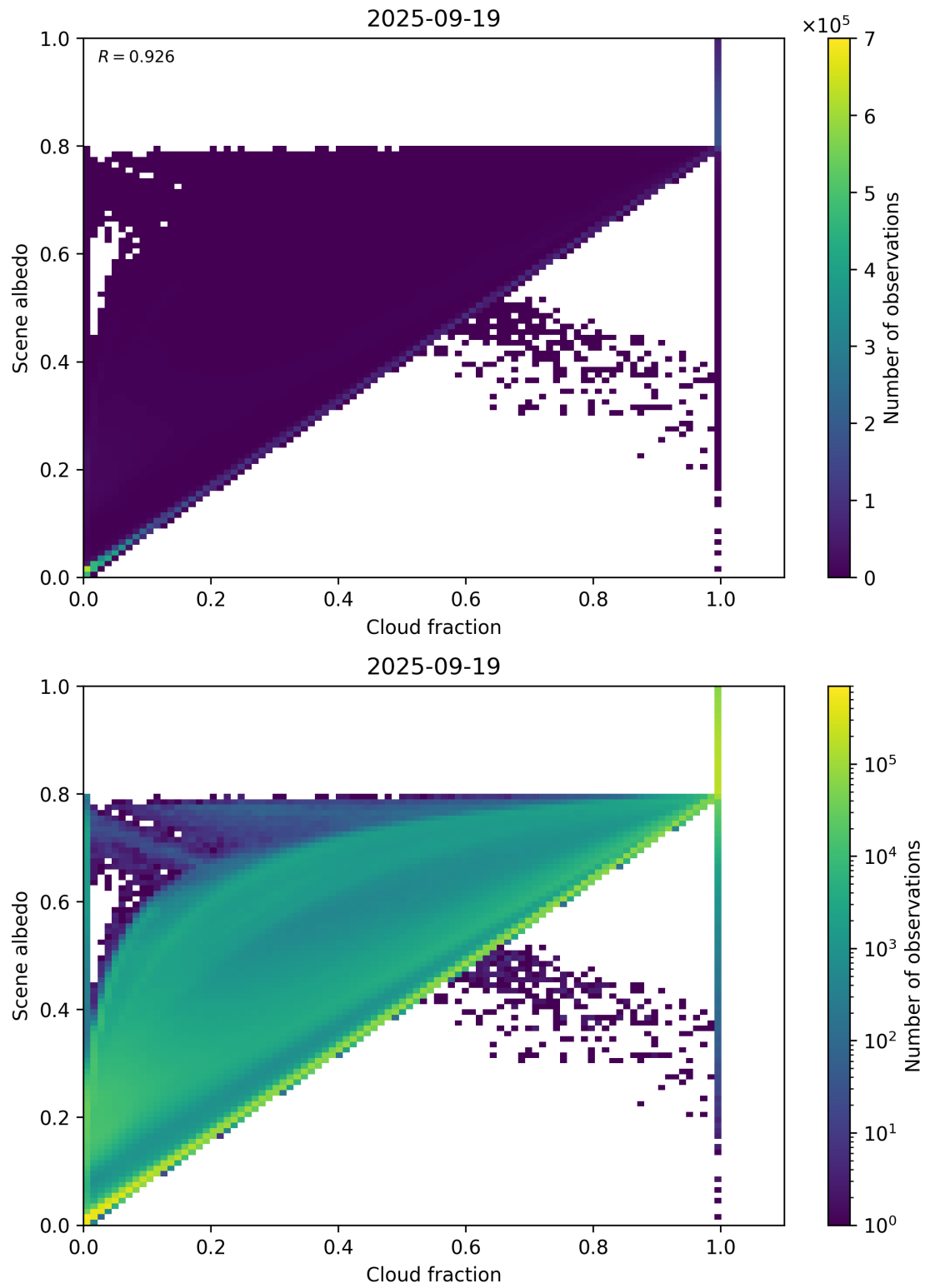
Figure 75: Scatter density plot of “Cloud fraction” against “Scene albedo” for 2025-09-18 to 2025-09-20.
