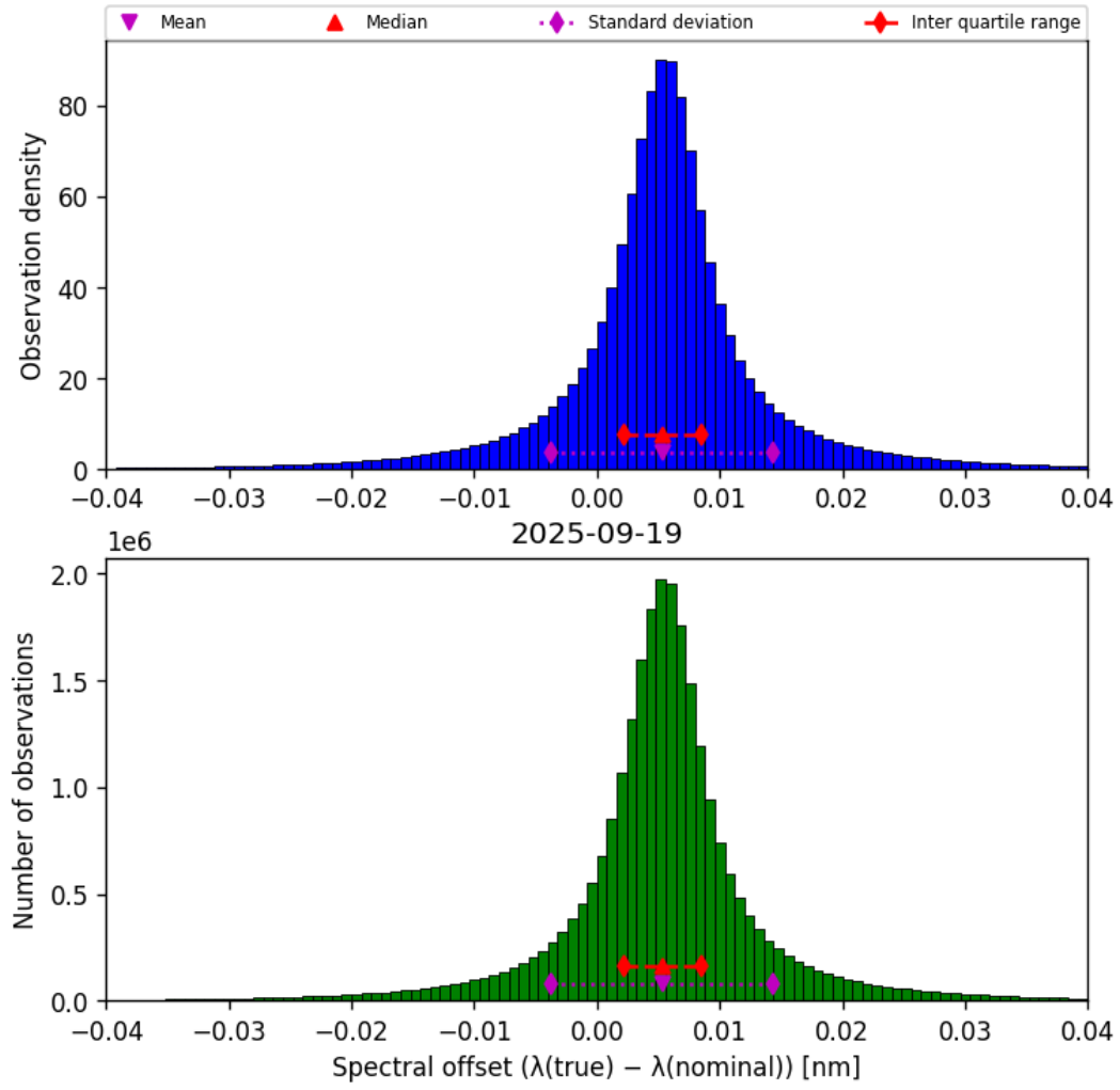
Figure 45: Histogram of “Spectral offset ( \lambda_{\text{true}} - \lambda_{\text{nominal}} )” for 2025-09-18 to 2025-09-20
