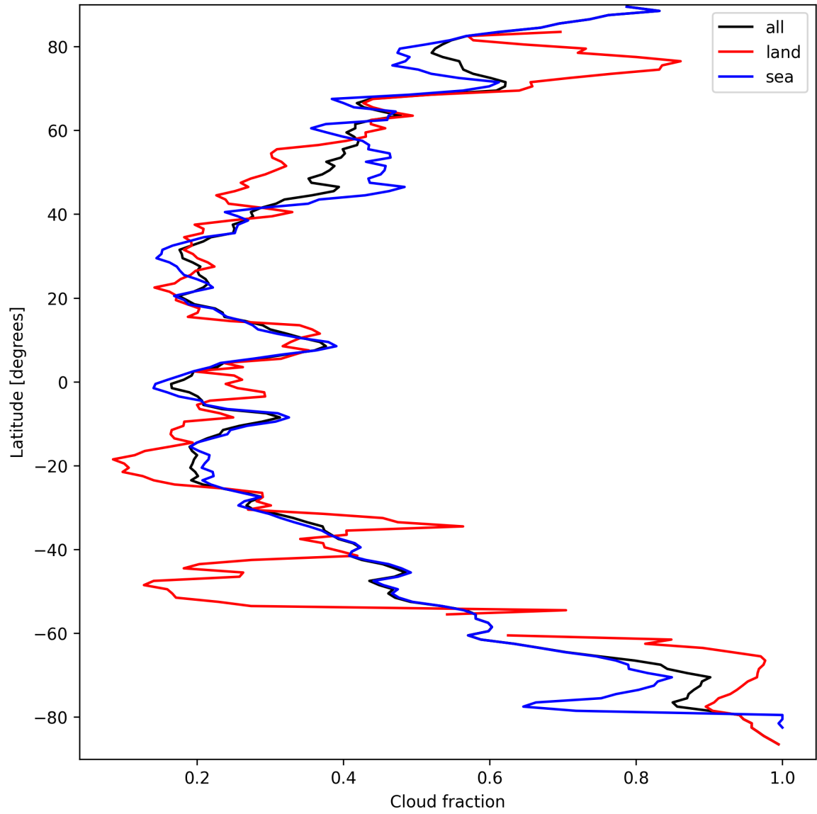
Figure 15: Zonal average of “Cloud fraction” for 2025-09-18 to 2025-09-20.
