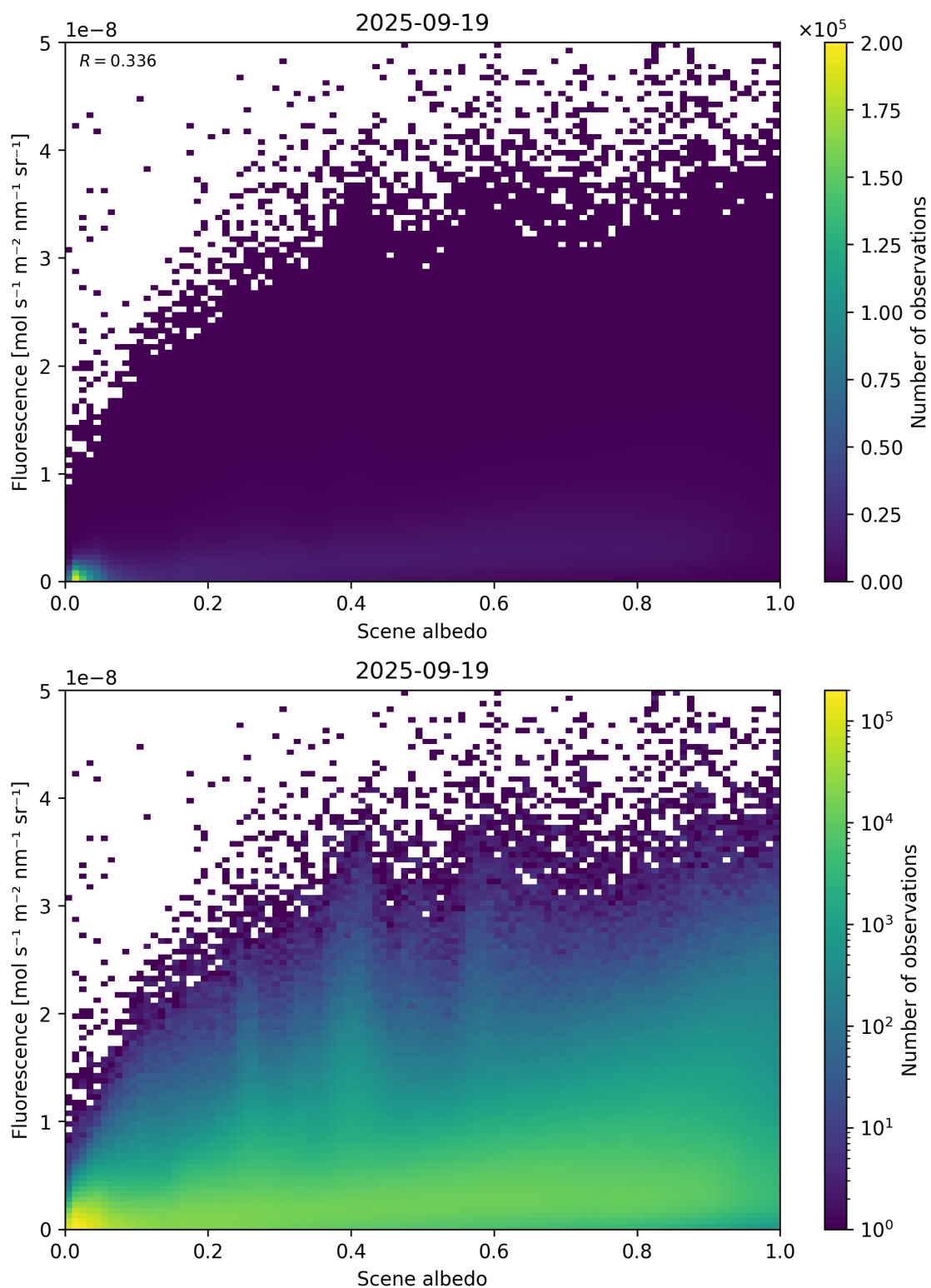
Figure 104: Scatter density plot of “Scene albedo” against “Fluorescence” for 2025-09-18 to 2025-09-20.
