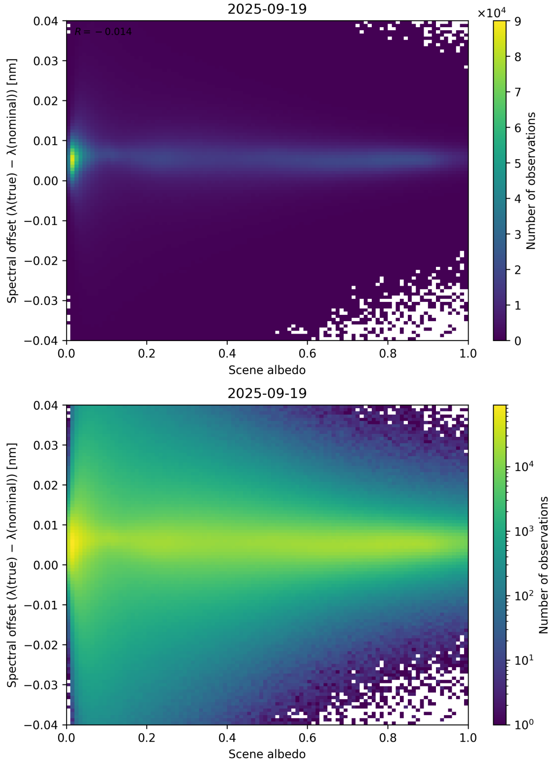
Figure 107: Scatter density plot of “Scene albedo” against “Spectral offset ( \lambda_{\text{true}} - \lambda_{\text{nominal}} )” for 2025-09-18 to 2025-09-20.
