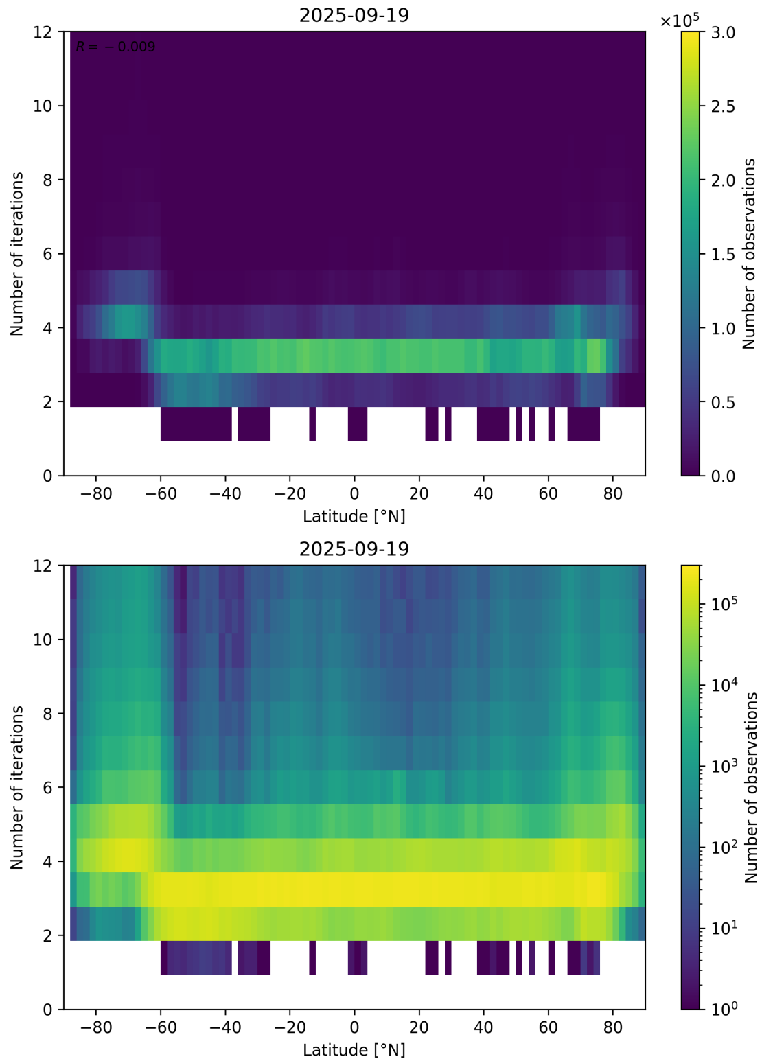
Figure 93: Scatter density plot of “Latitude” against “Number of iterations” for 2025-09-18 to 2025-09-20.
