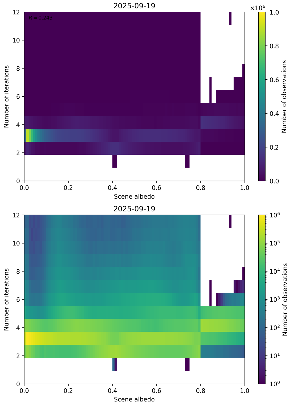
Figure 105: Scatter density plot of “Scene albedo” against “Number of iterations” for 2025-09-18 to 2025-09-20.
