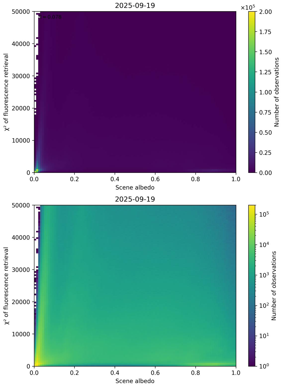
Figure 103: Scatter density plot of “Scene albedo” against “ \chi^2 of fluorescence retrieval” for 2025-09-18 to 2025-09-20.
