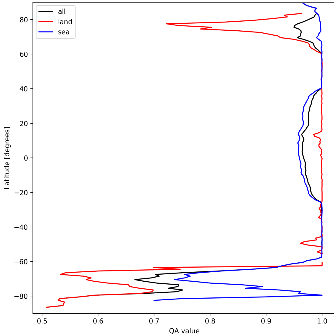
Figure 12: Zonal average of "QA value" for 2025-09-18 to 2025-09-20.
