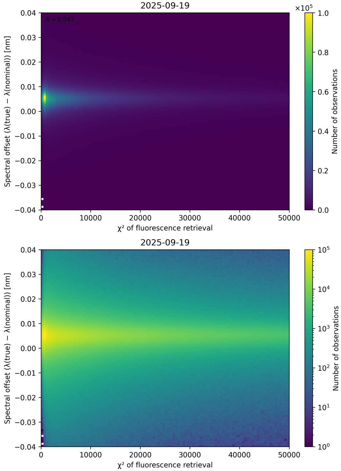
Figure 69: Scatter density plot of “ \chi^2 of fluorescence retrieval” against “Spectral offset ( \lambda_{\text{true}} - \lambda_{\text{nominal}} )” for 2025-09-18 to 2025-09-20.
