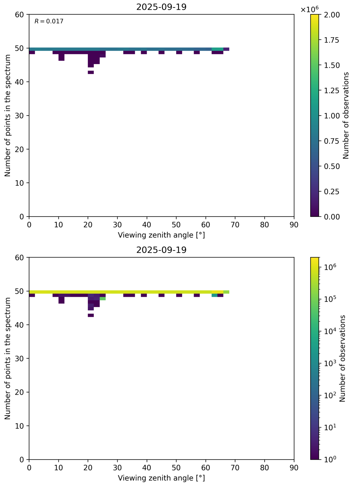
Figure 125: Scatter density plot of “Viewing zenith angle” against “Number of points in the spectrum” for 2025-09-18 to 2025-09-20.
