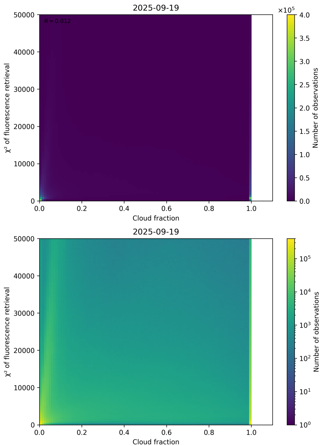
Figure 71: Scatter density plot of “Cloud fraction” against “ \chi^2 of fluorescence retrieval” for 2025-09-18 to 2025-09-20.
