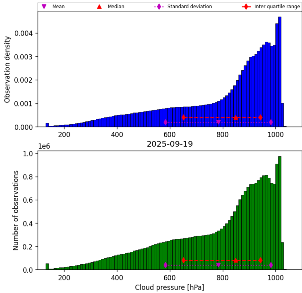
Figure 30: Histogram of “Cloud pressure” for 2025-09-18 to 2025-09-20
