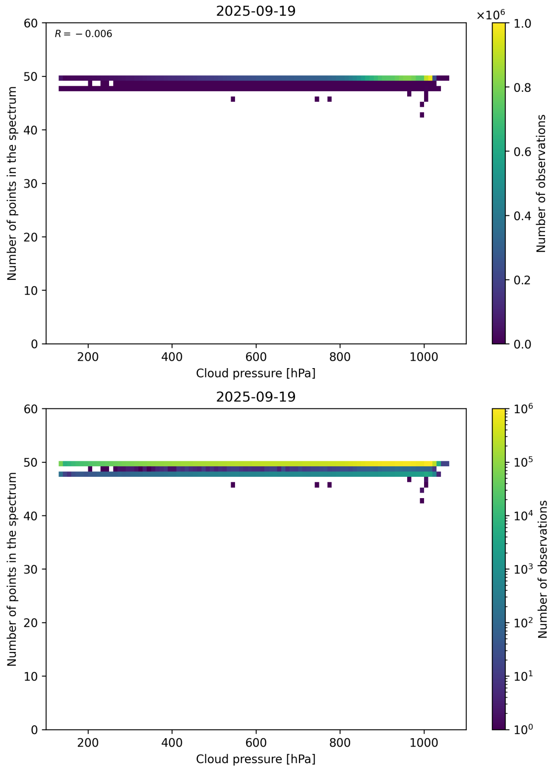
Figure 82: Scatter density plot of “Cloud pressure” against “Number of points in the spectrum” for 2025-09-18 to 2025-09-20.
