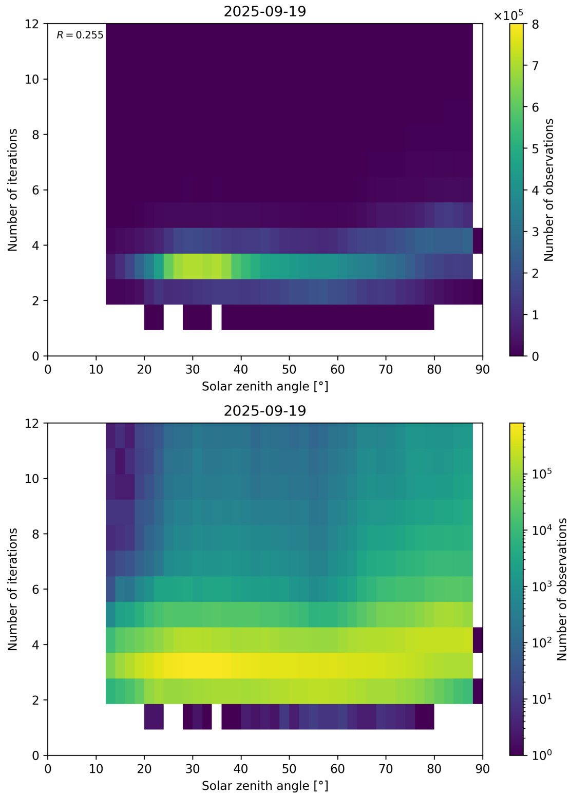
Figure 114: Scatter density plot of “Solar zenith angle” against “Number of iterations” for 2025-09-18 to 2025-09-20.
