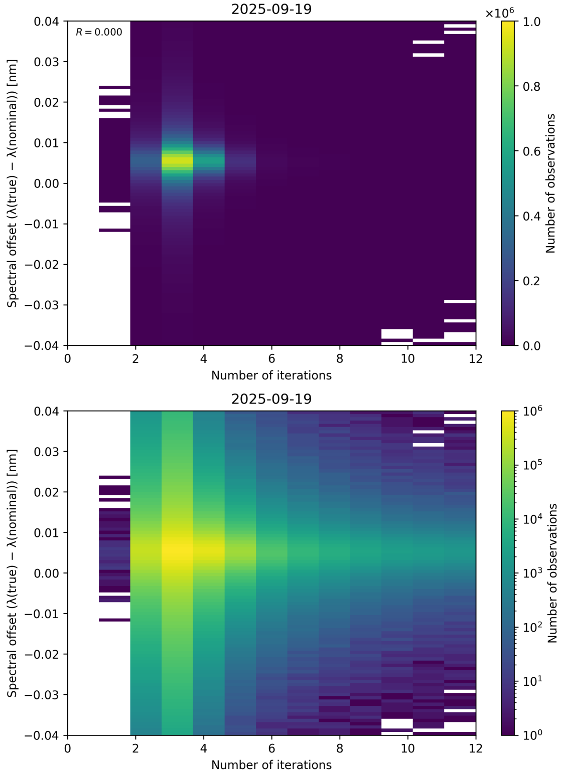
Figure 100: Scatter density plot of “Number of iterations” against “Spectral offset ( \lambda_{\text{true}} - \lambda_{\text{nominal}} )” for 2025-09-18 to 2025-09-20.
