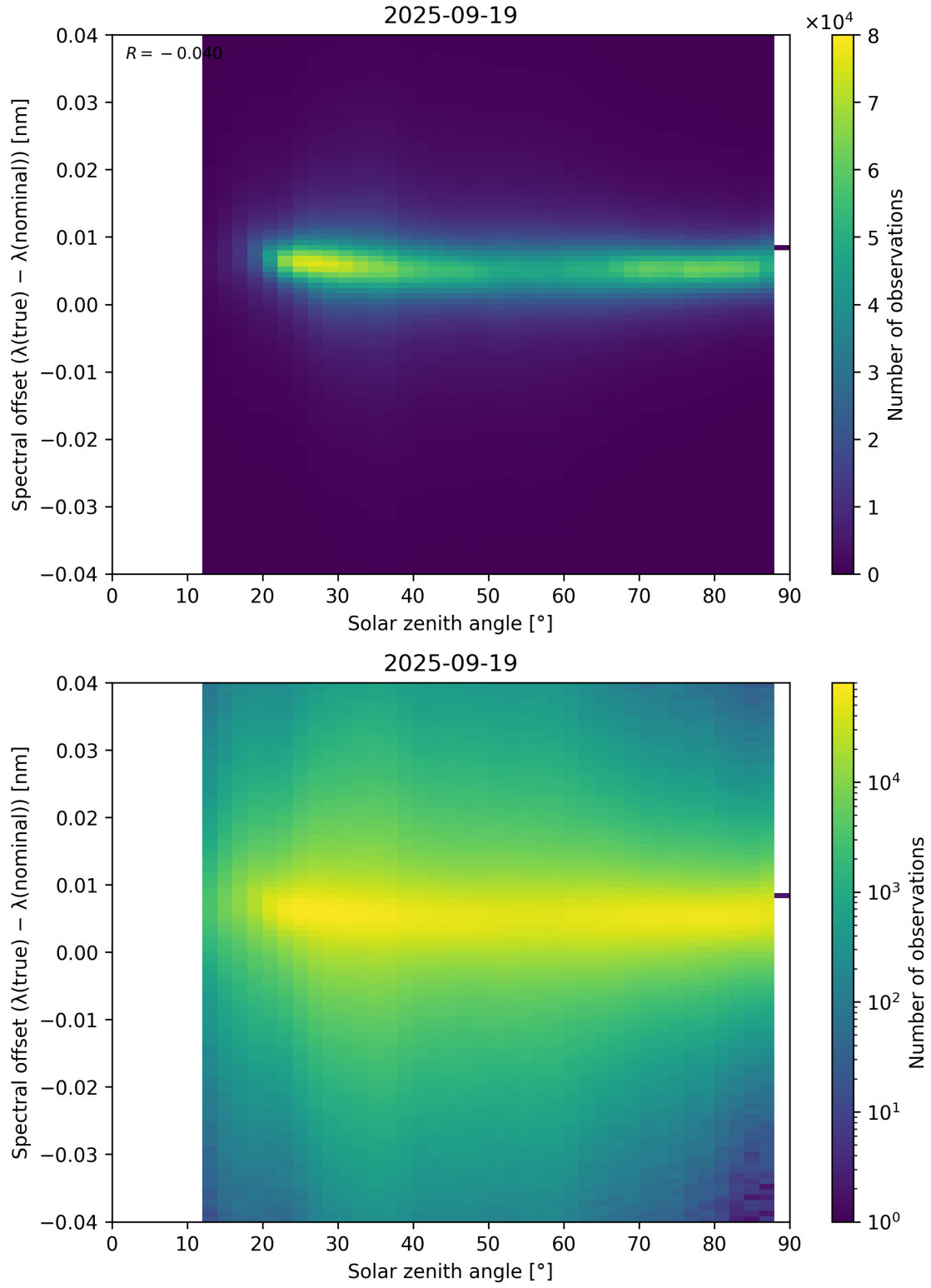
Figure 117: Scatter density plot of “Solar zenith angle” against “Spectral offset ( \lambda_{\text{true}} - \lambda_{\text{nominal}} )” for 2025-09-18 to 2025-09-20.
