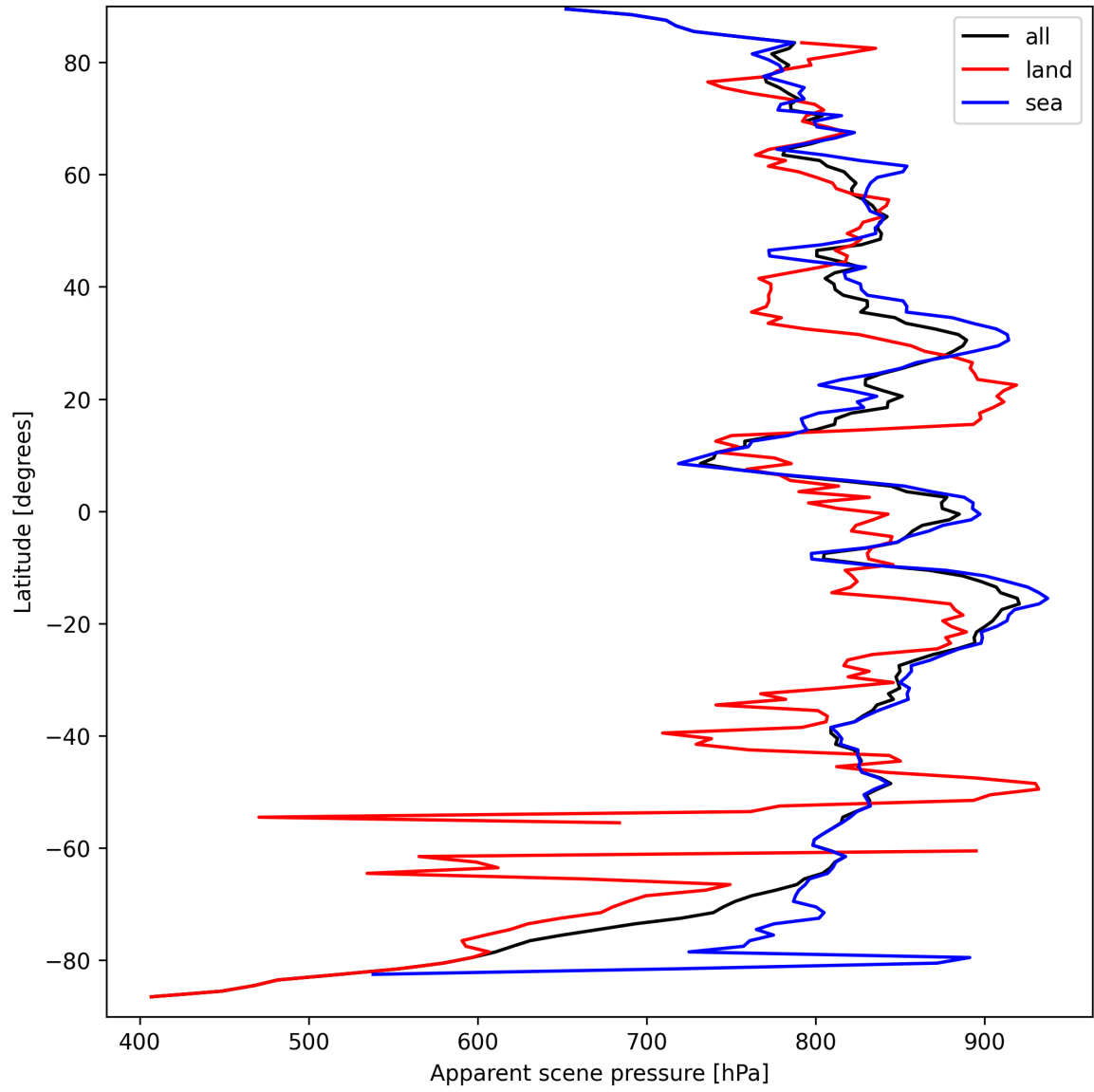
Figure 19: Zonal average of “Apparent scene pressure” for 2025-09-18 to 2025-09-20.
