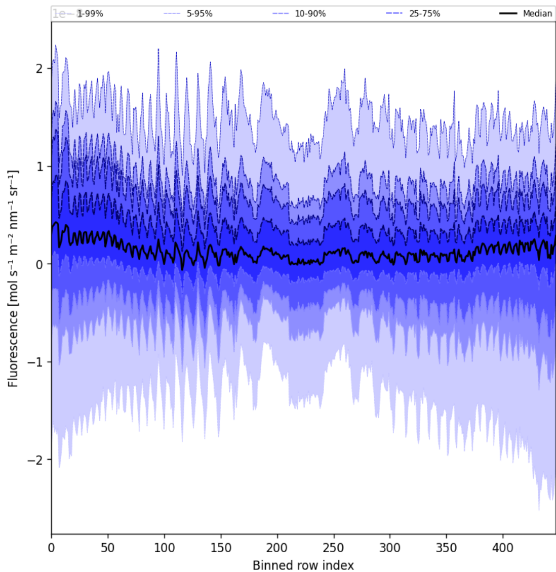
Figure 57: Along track statistics of "Fluorescence" for 2025-09-18 to 2025-09-20
