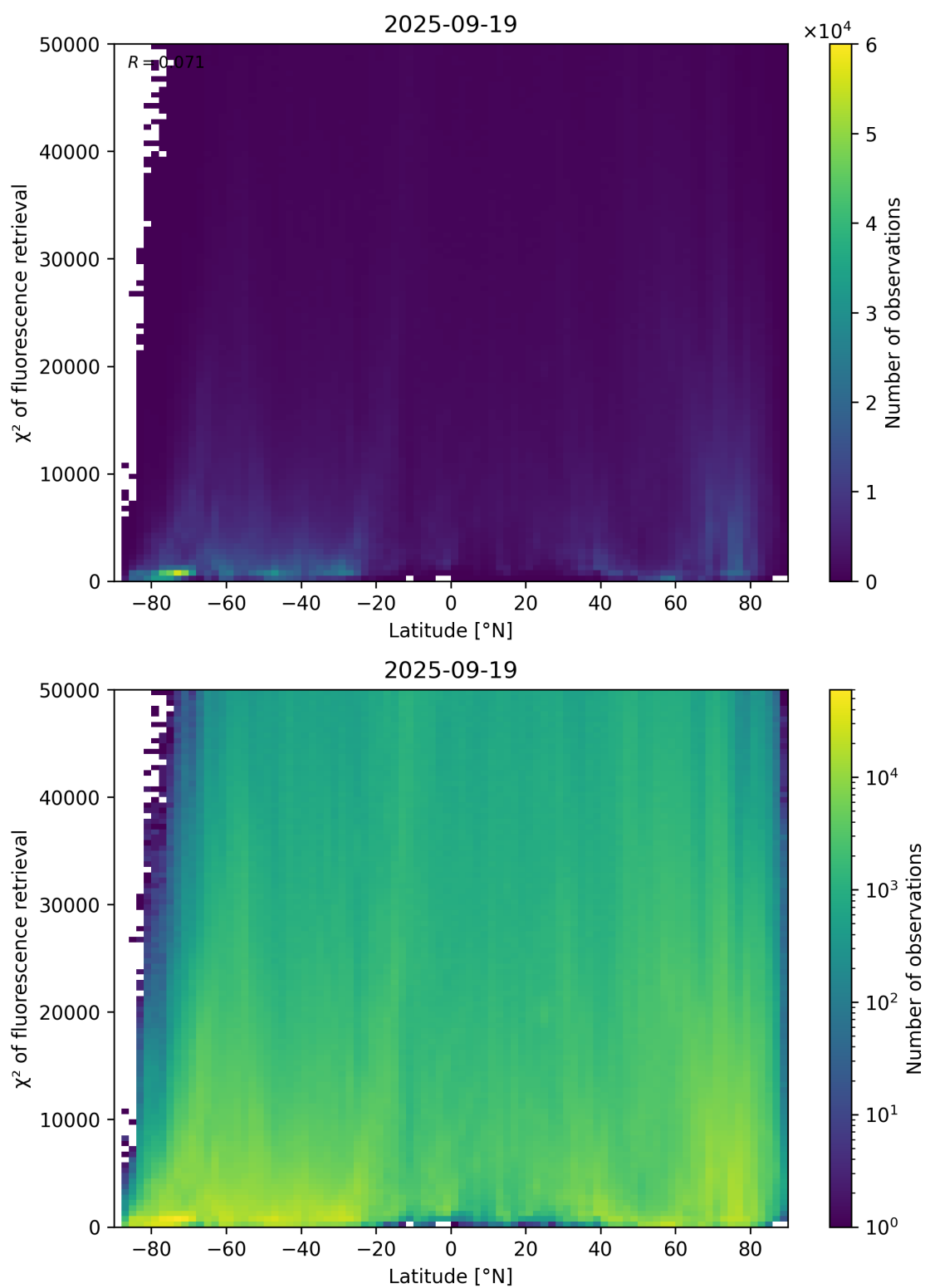
Figure 89: Scatter density plot of “Latitude” against “ \chi^2 of fluorescence retrieval” for 2025-09-18 to 2025-09-20.
