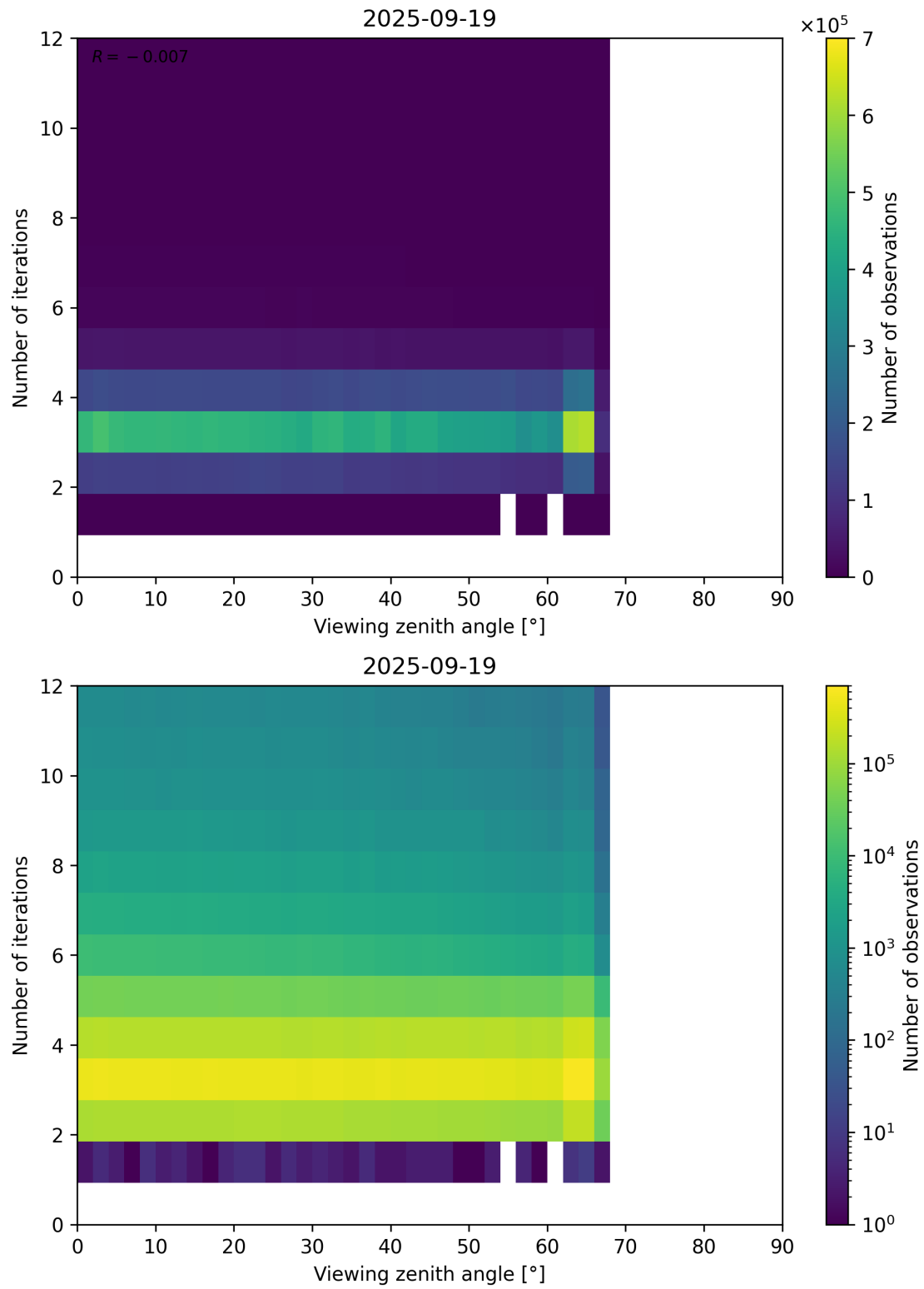
Figure 124: Scatter density plot of “Viewing zenith angle” against “Number of iterations” for 2025-09-18 to 2025-09-20.
