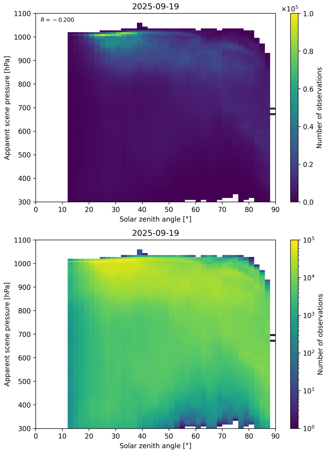
Figure 108: Scatter density plot of “Solar zenith angle” against “Apparent scene pressure” for 2025-09-18 to 2025-09-20.
