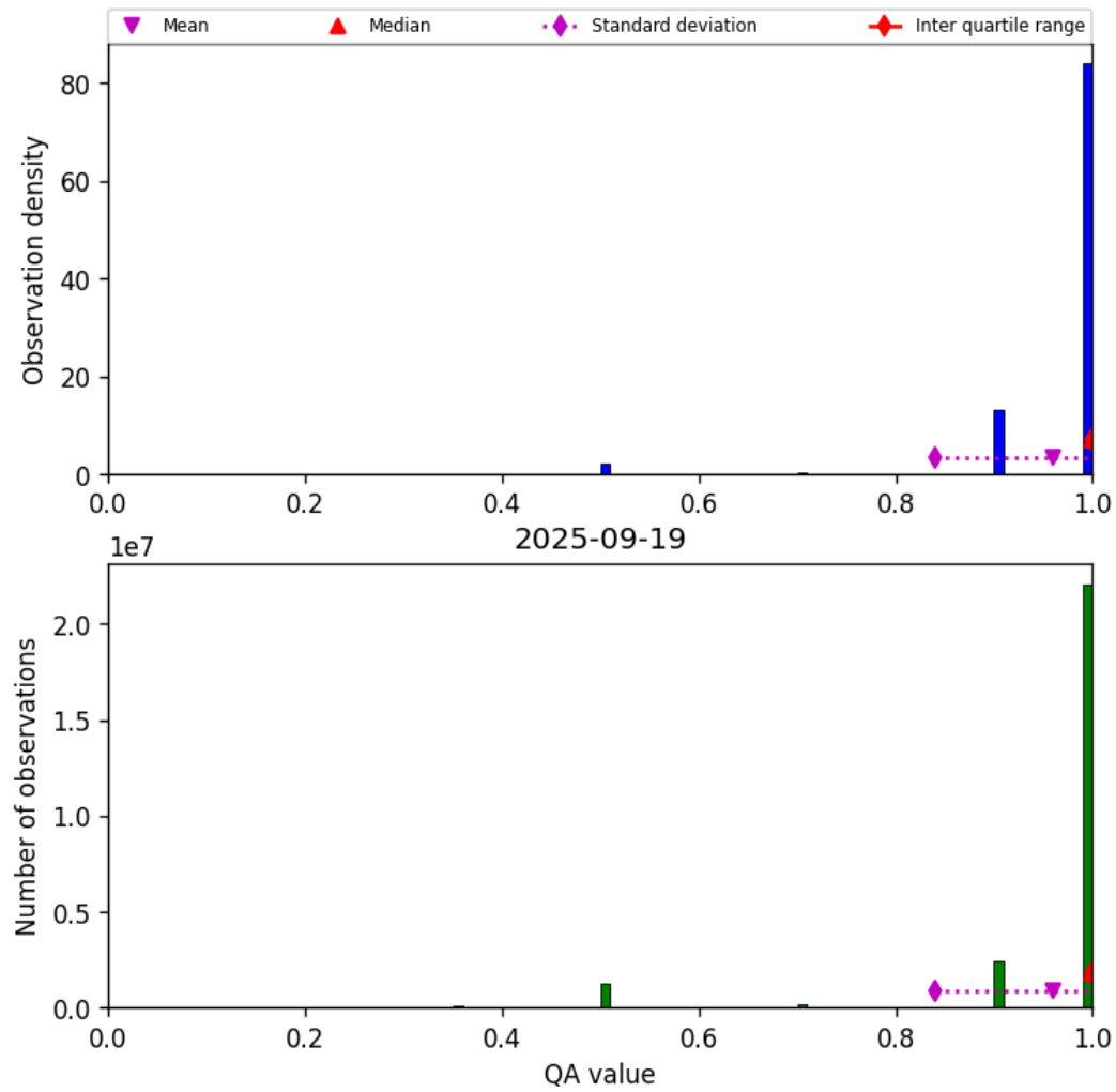
Figure 29: Histogram of “QA value” for 2025-09-18 to 2025-09-20
