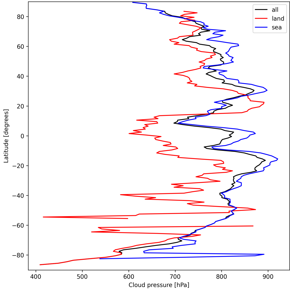
Figure 13: Zonal average of “Cloud pressure” for 2025-09-18 to 2025-09-20.
