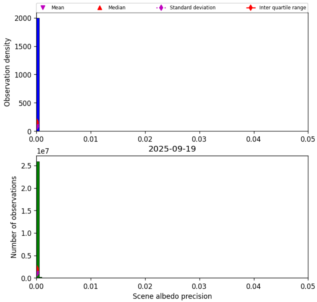
Figure 35: Histogram of “Scene albedo precision” for 2025-09-18 to 2025-09-20
