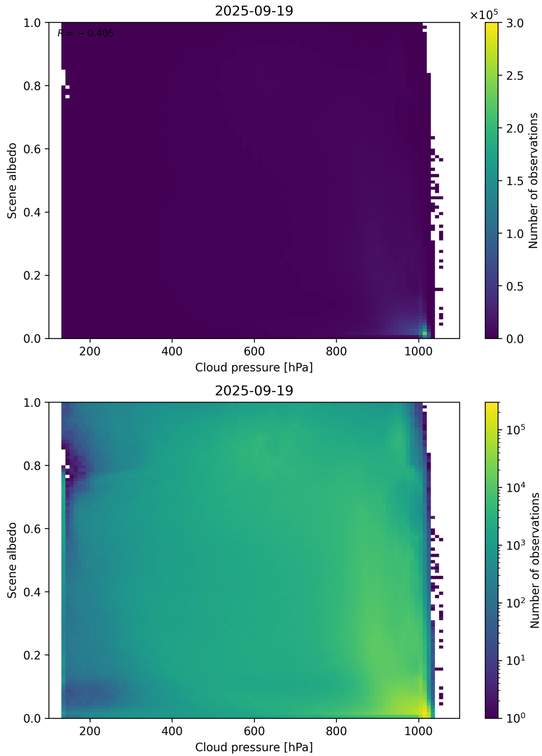
Figure 83: Scatter density plot of “Cloud pressure” against “Scene albedo” for 2025-09-18 to 2025-09-20.
