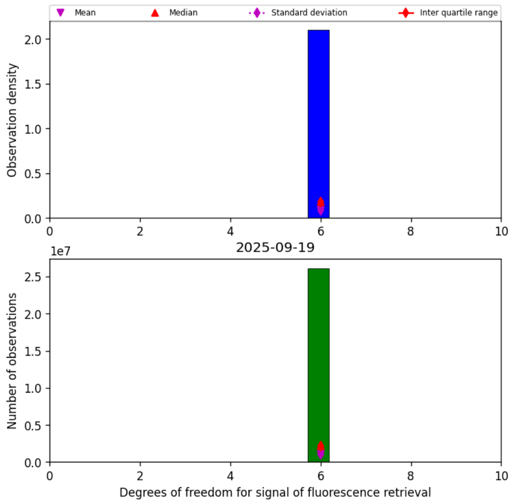
Figure 43: Histogram of "Degrees of freedom for signal of fluorescence retrieval" for 2025-09-18 to 2025-09-20
