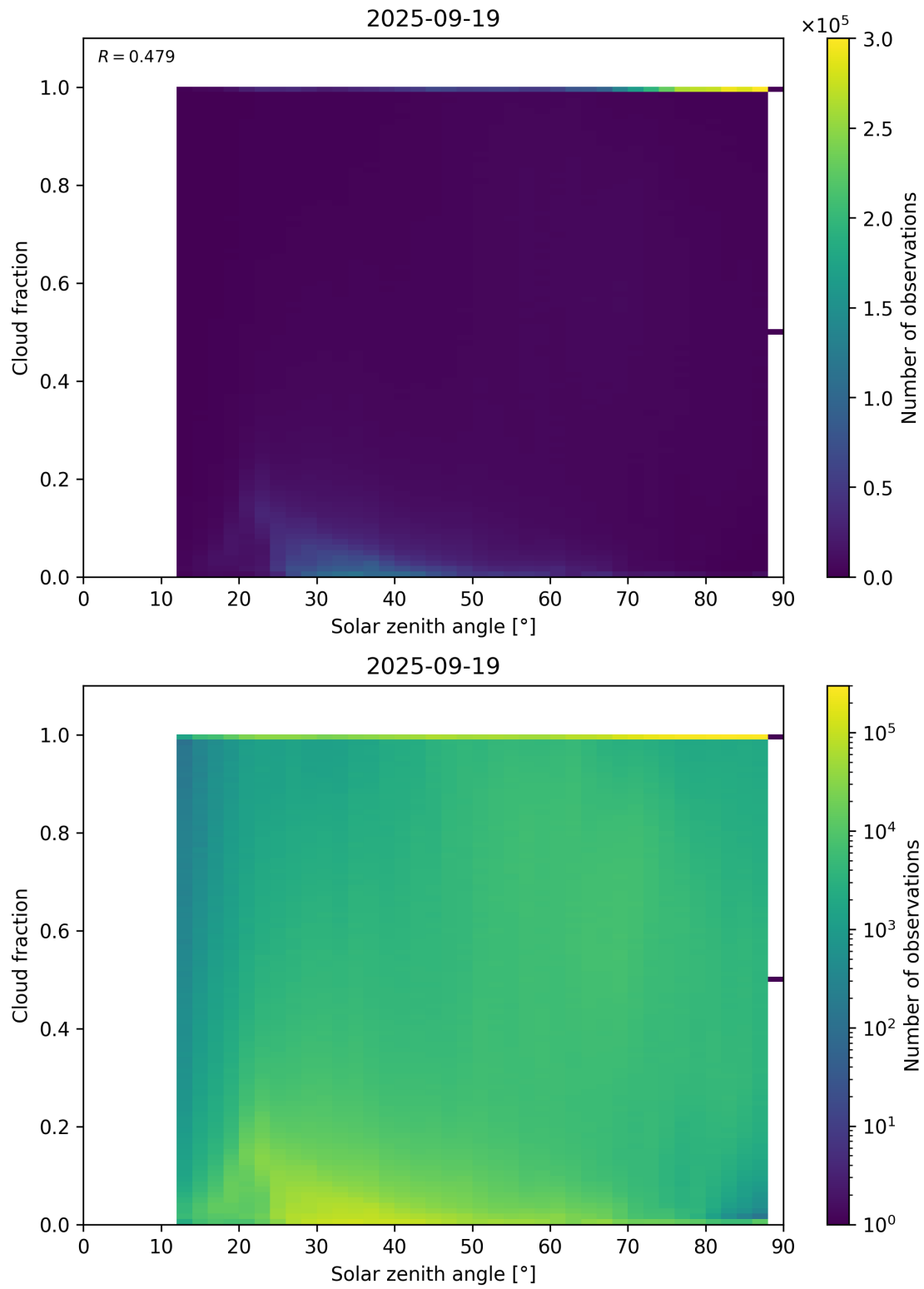
Figure 110: Scatter density plot of “Solar zenith angle” against “Cloud fraction” for 2025-09-18 to 2025-09-20.
