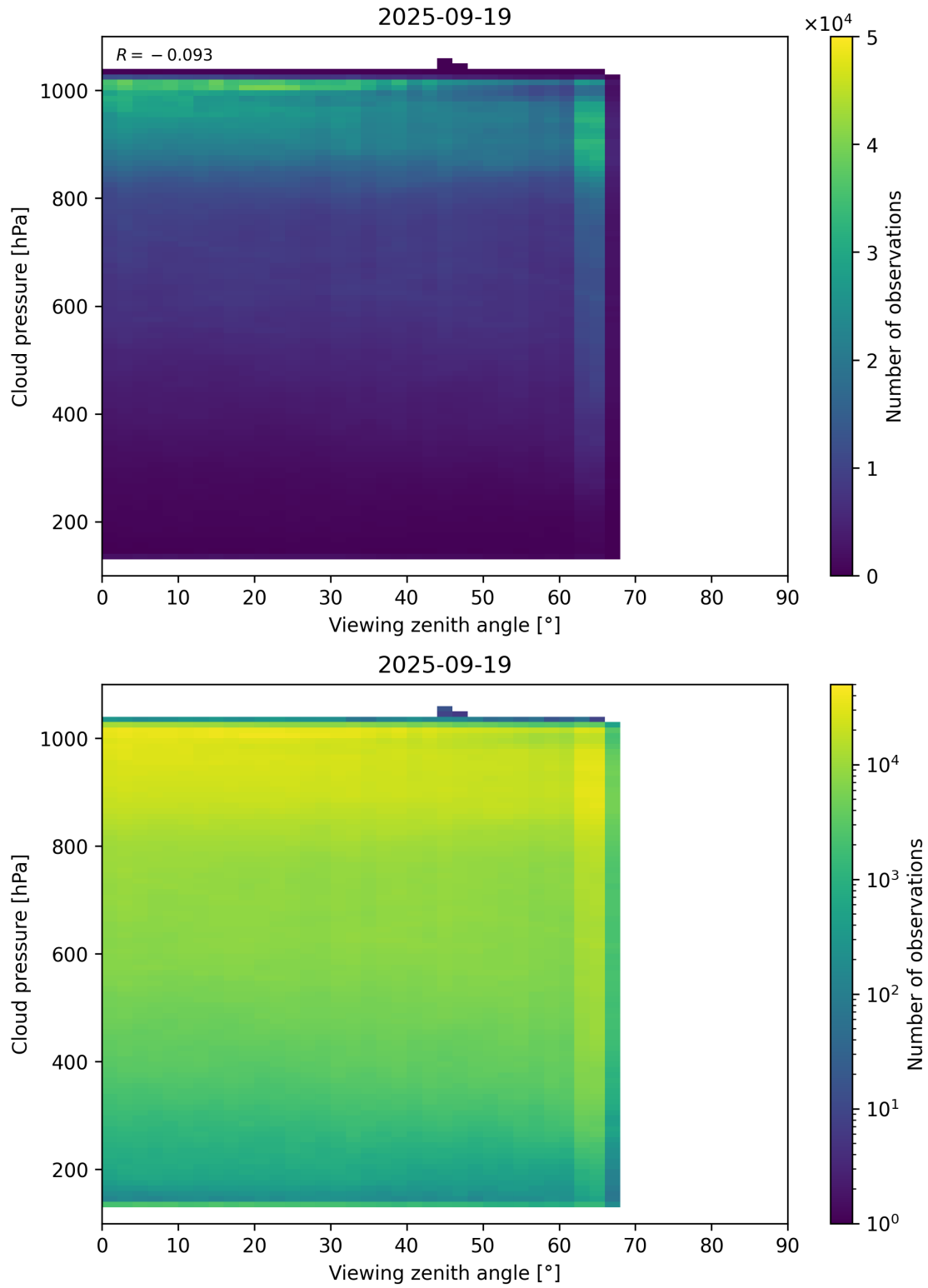
Figure 121: Scatter density plot of “Viewing zenith angle” against “Cloud pressure” for 2025-09-18 to 2025-09-20.
