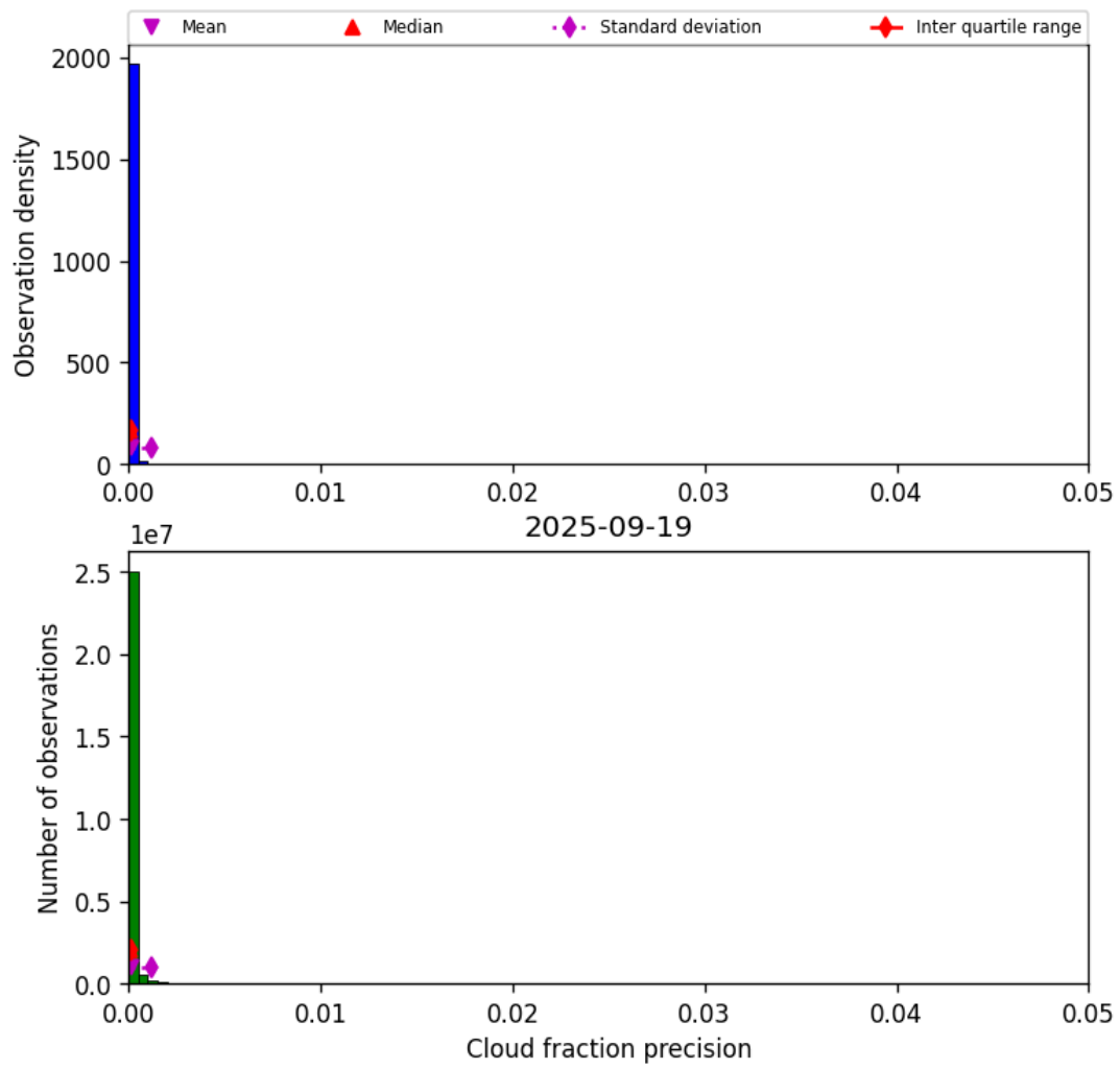
Figure 33: Histogram of “Cloud fraction precision” for 2025-09-18 to 2025-09-20
